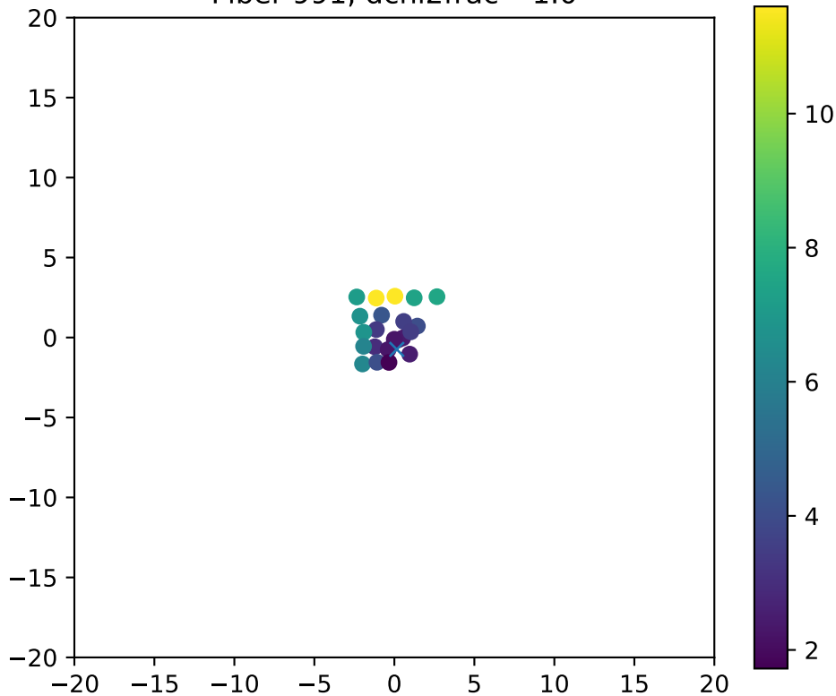
Fiber 991, dchi2frac= 1.0
