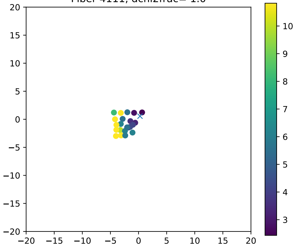
Fiber 4111, dchi2frac= 1.0
