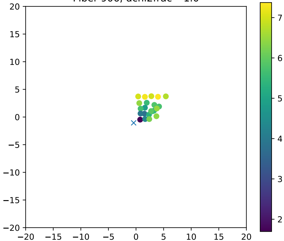
Fiber 906, dchi2frac= 1.0
