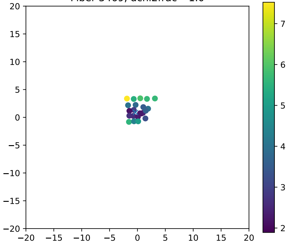
Fiber 3469, dchi2frac= 1.0
