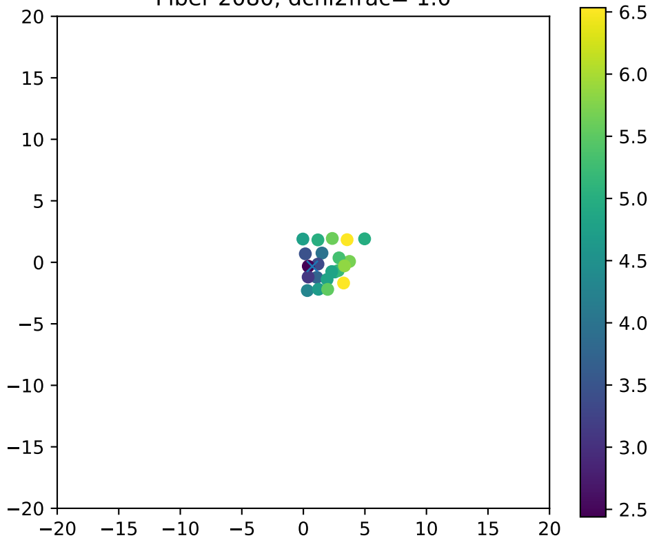
Fiber 2080, dchi2frac= 1.0
