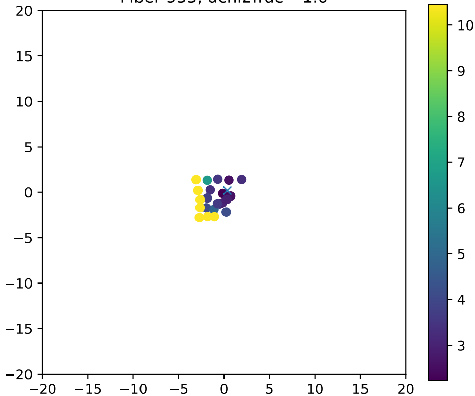
Fiber 933, dchi2frac= 1.0
