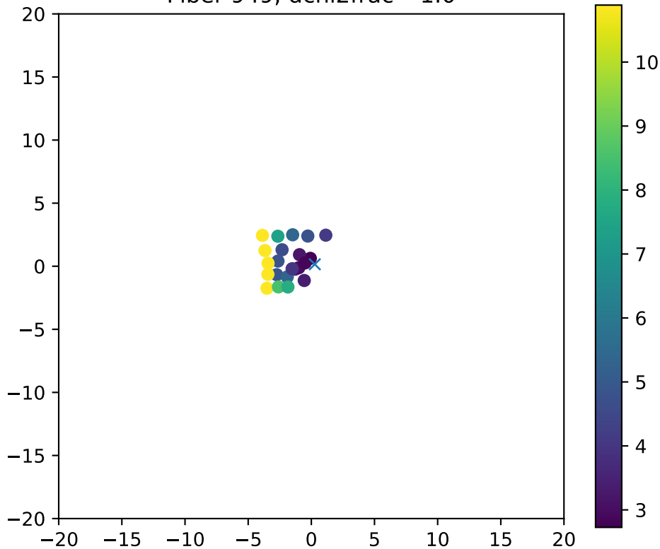
Fiber 949, dchi2frac= 1.0
