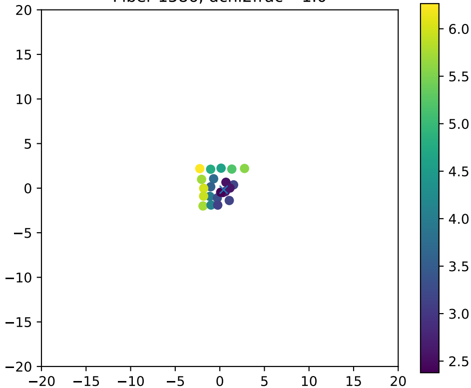
Fiber 1586, dchi2frac= 1.0
