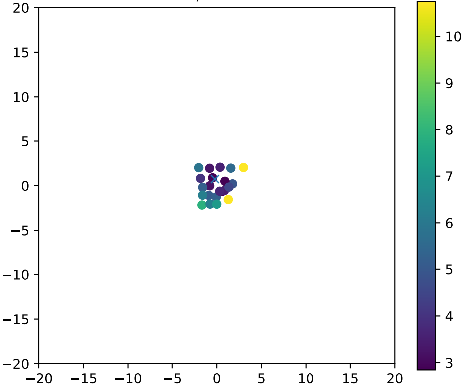
Fiber 3892, dchi2frac= 1.0
