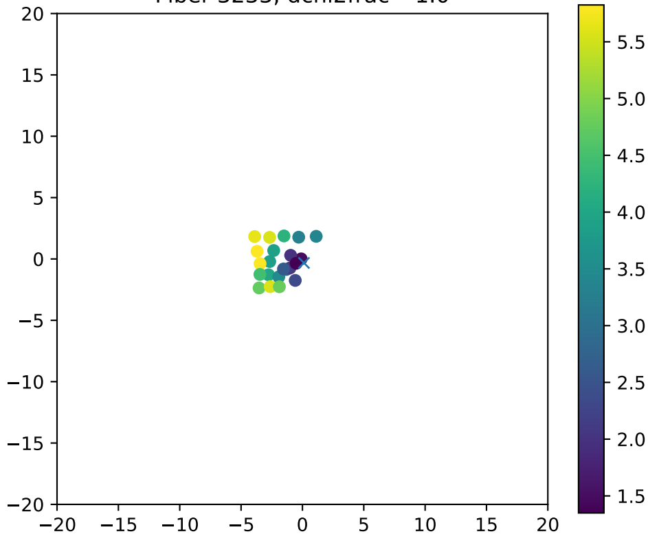
Fiber 3233, dchi2frac= 1.0
