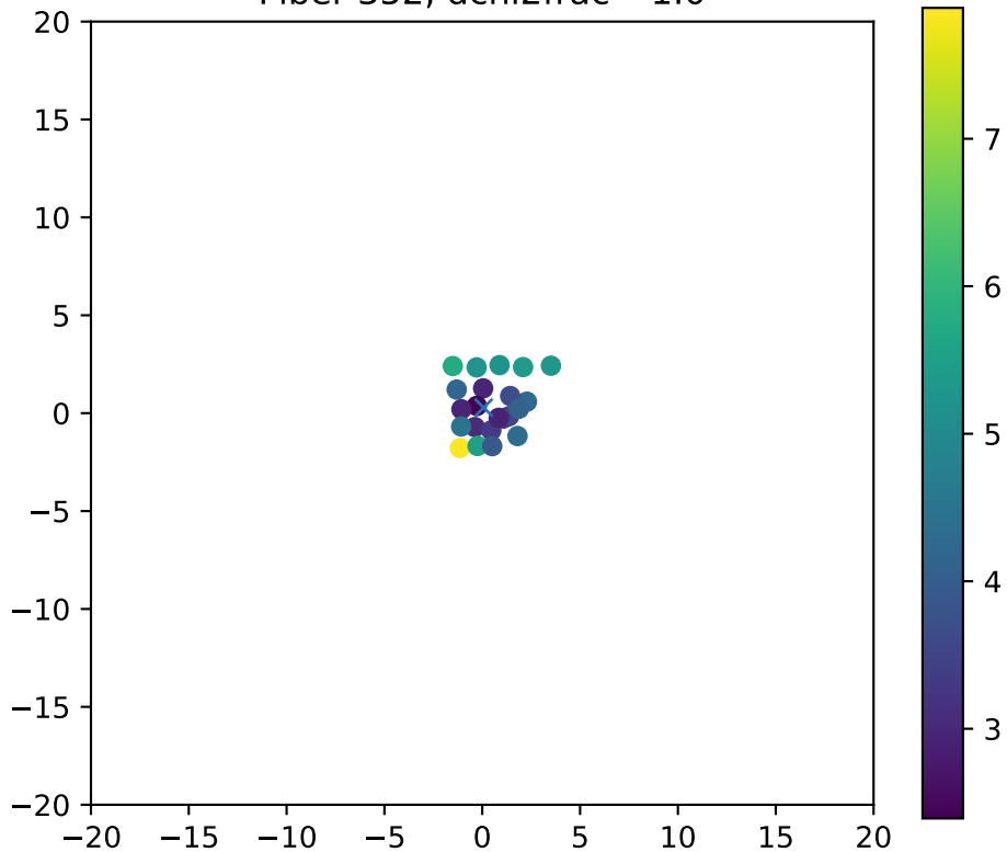
Fiber 352, dchi2frac= 1.0
