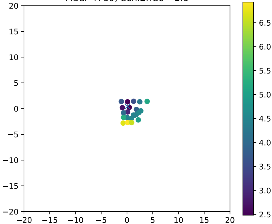
Fiber 4760, dchi2frac= 1.0
