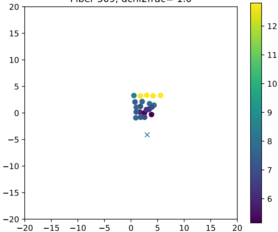
Fiber 509, dchi2frac= 1.0
