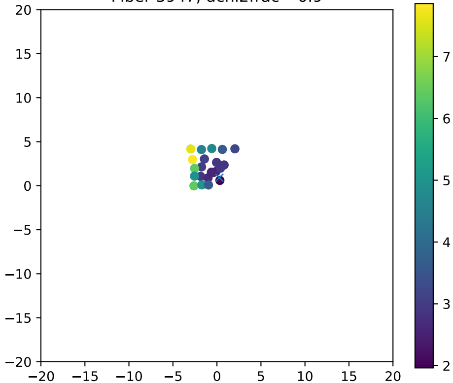
Fiber 3947, dchi2frac= 0.9
