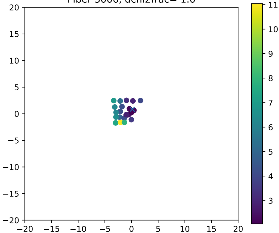
Fiber 3006, dchi2frac= 1.0
