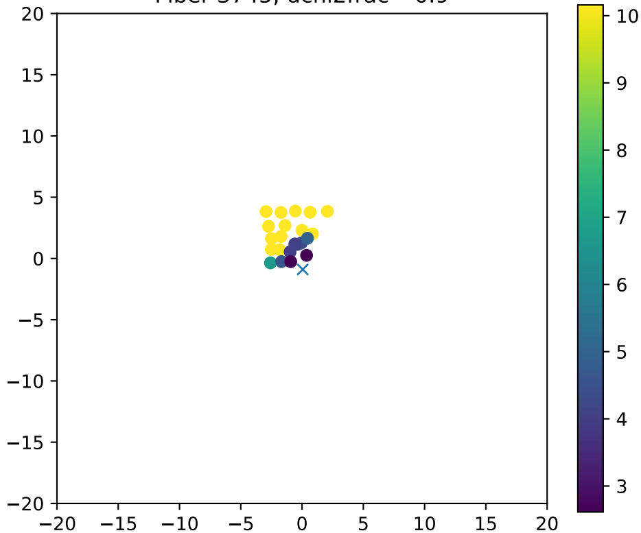
Fiber 3745, dchi2frac= 0.9
