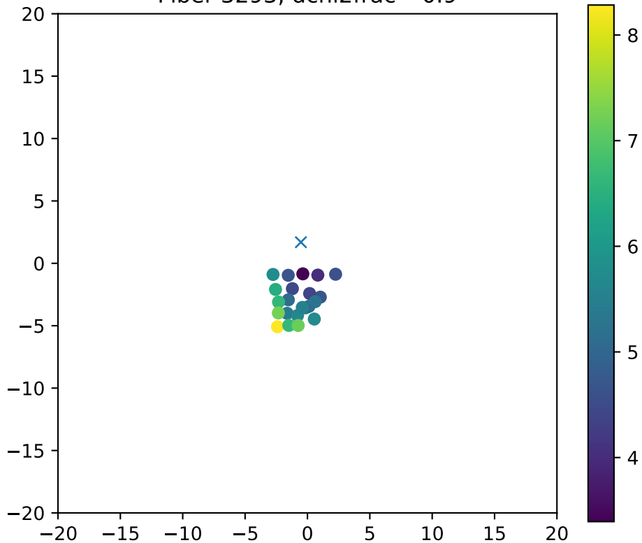
Fiber 3293, dchi2frac= 0.9
