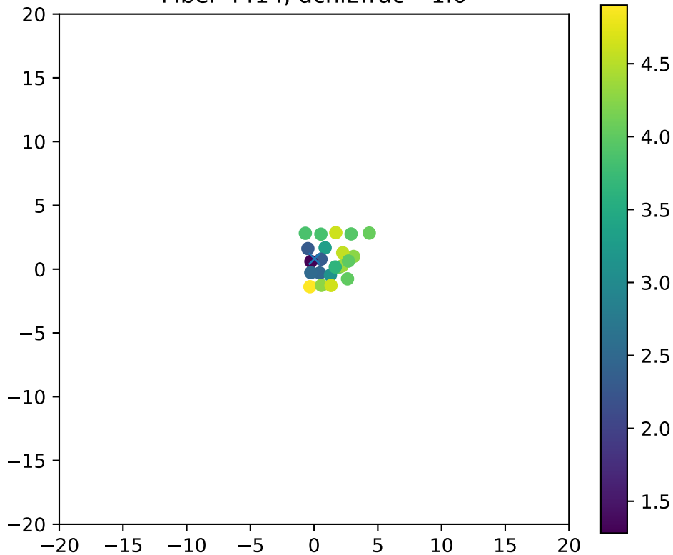
Fiber 4414, dchi2frac= 1.0
