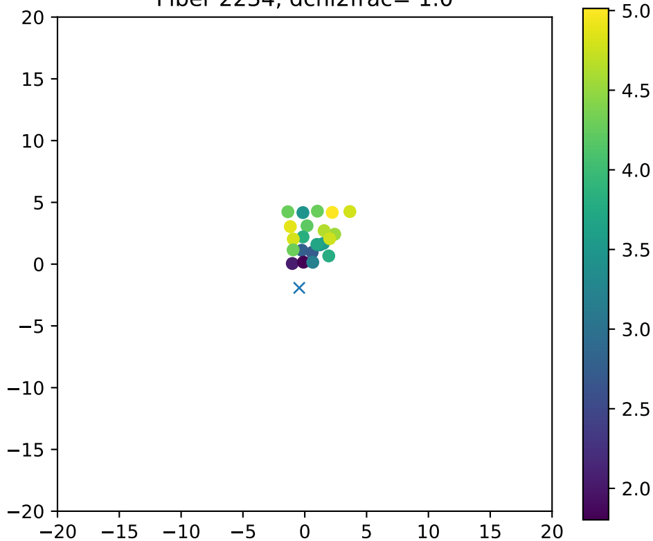
Fiber 2234, dchi2frac= 1.0
