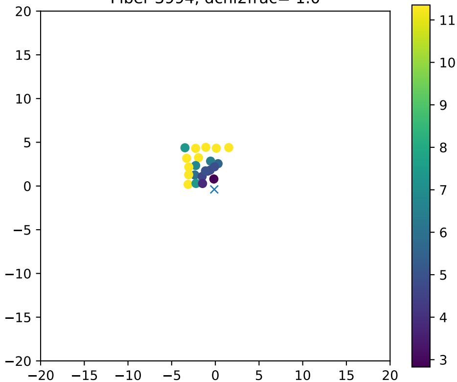
Fiber 3994, dchi2frac= 1.0
