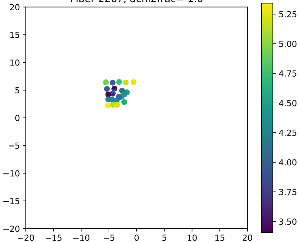
Fiber 2267, dchi2frac= 1.0
