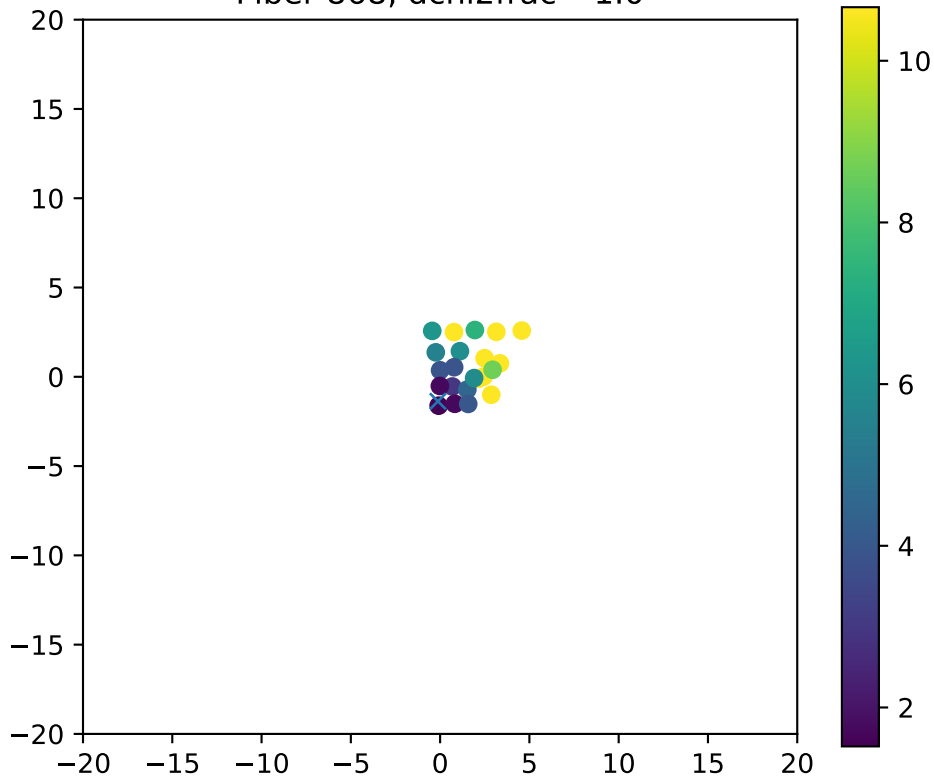
Fiber 868, dchi2frac= 1.0
