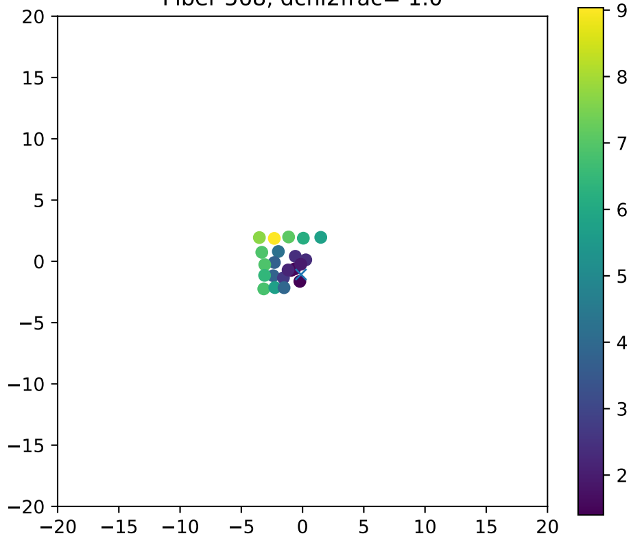
Fiber 568, dchi2frac= 1.0
