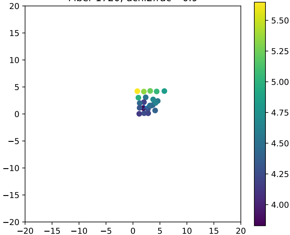
Fiber 1720, dchi2frac= 0.9
