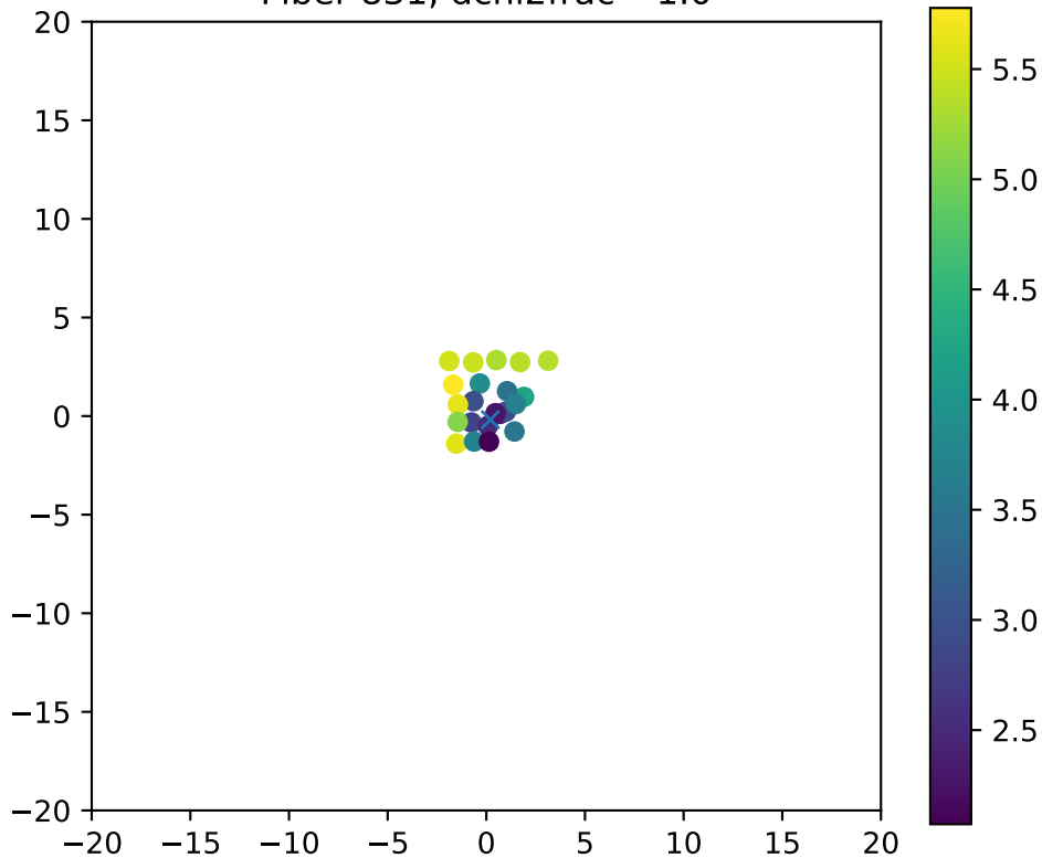
Fiber 831, dchi2frac= 1.0
