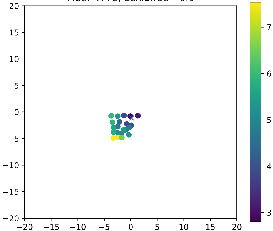
Fiber 4770, dchi2frac= 0.9
