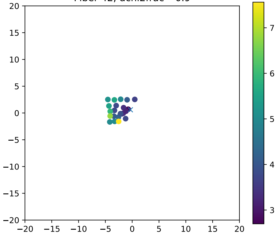
Fiber 42, dchi2frac= 0.9
