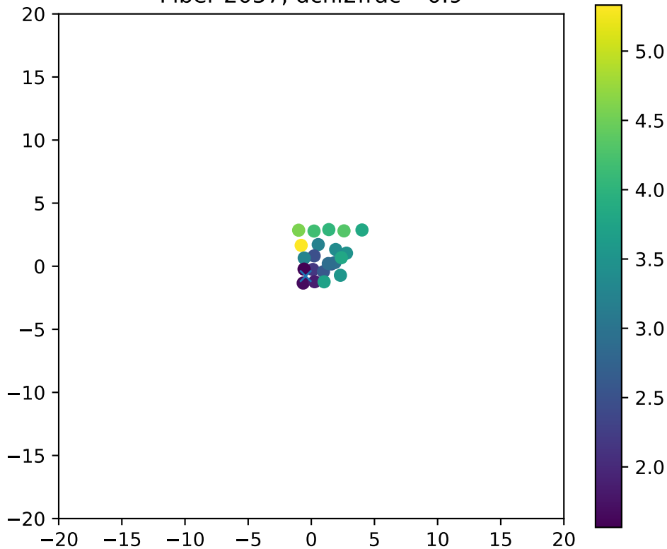
Fiber 2057, dchi2frac= 0.9
