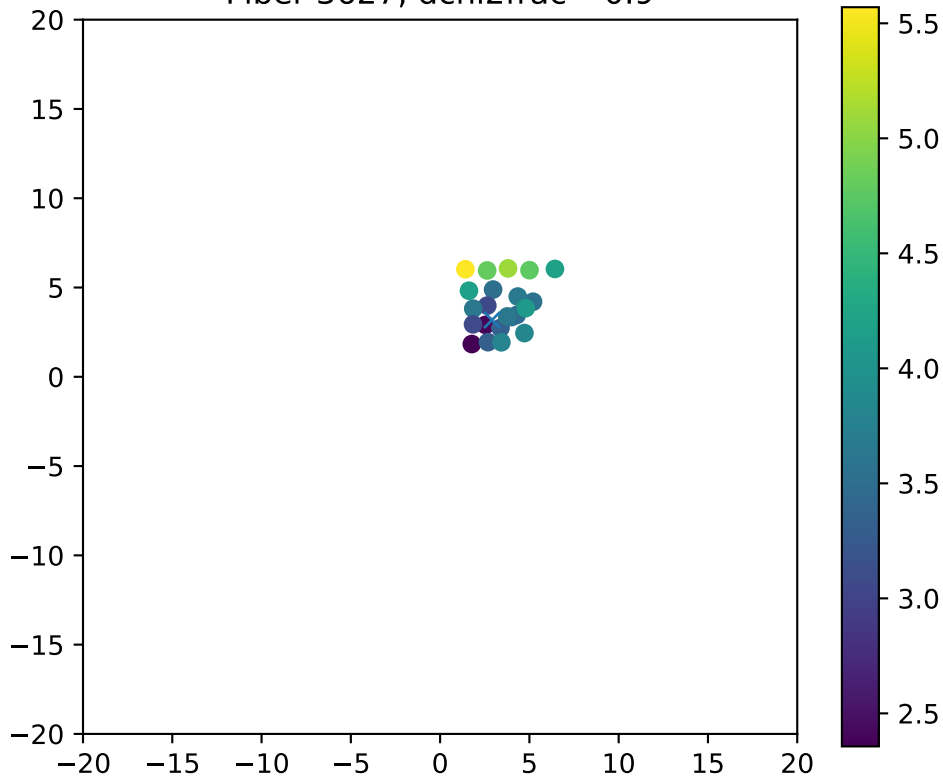
Fiber 3627, dchi2frac= 0.9
