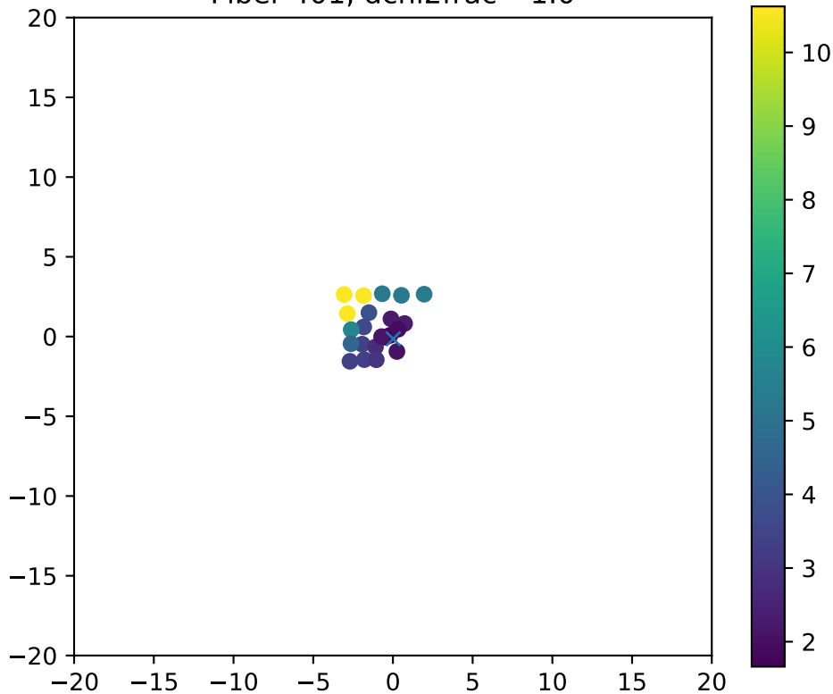
Fiber 401, dchi2frac= 1.0
