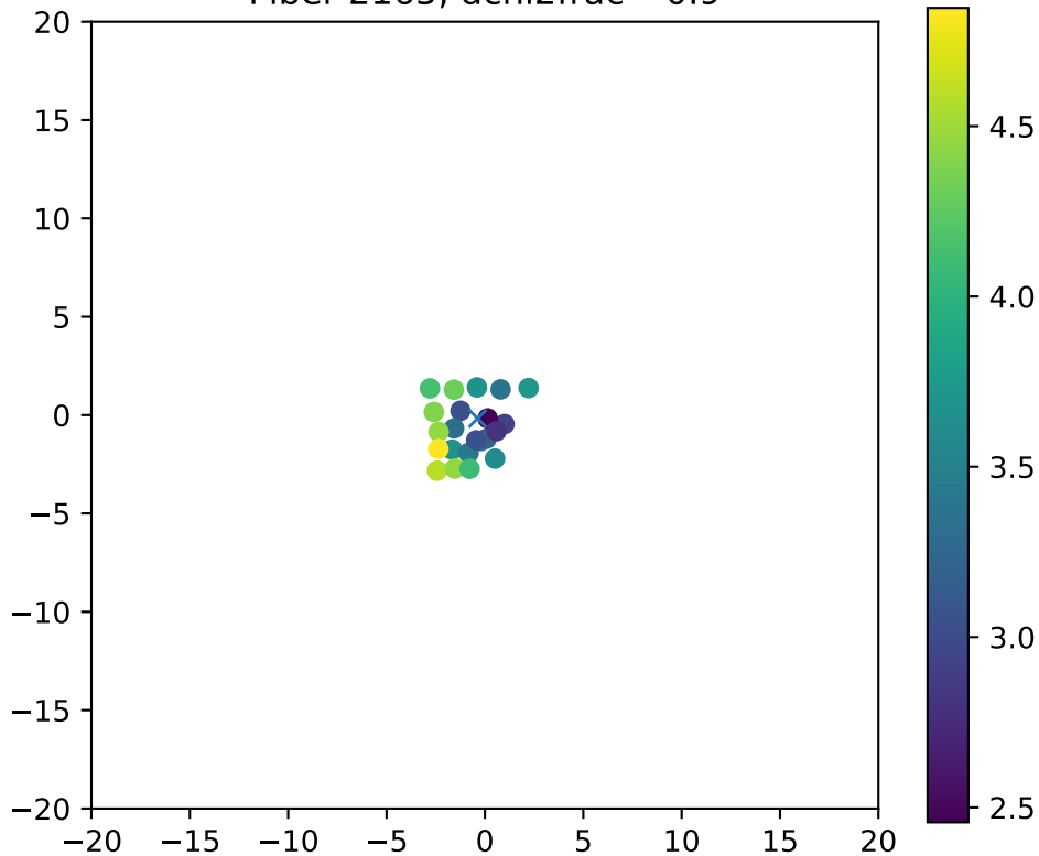
Fiber 2165, dchi2frac= 0.9
