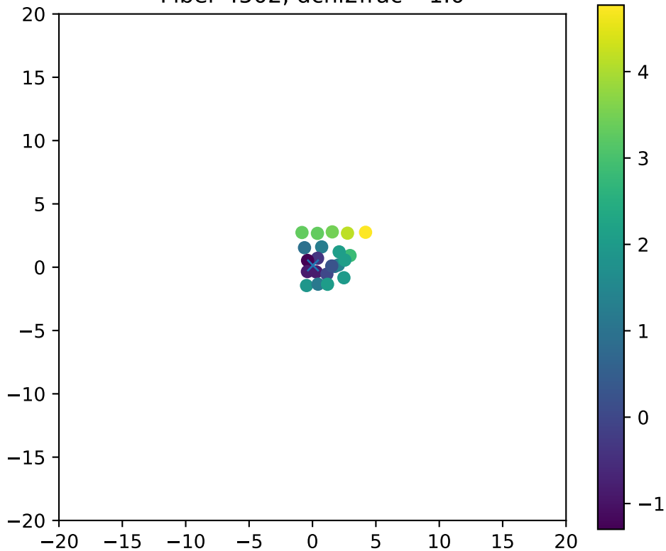
Fiber 4502, dchi2frac= 1.0
