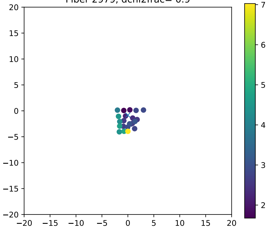
Fiber 2979, dchi2frac= 0.9
