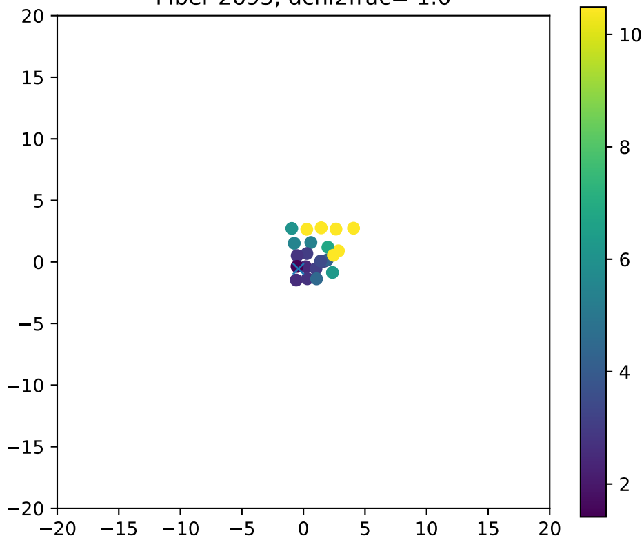
Fiber 2695, dchi2frac= 1.0
