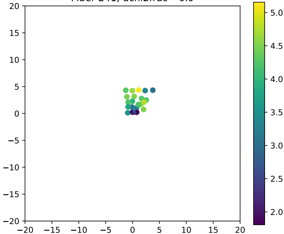
Fiber 241, dchi2frac= 0.9
