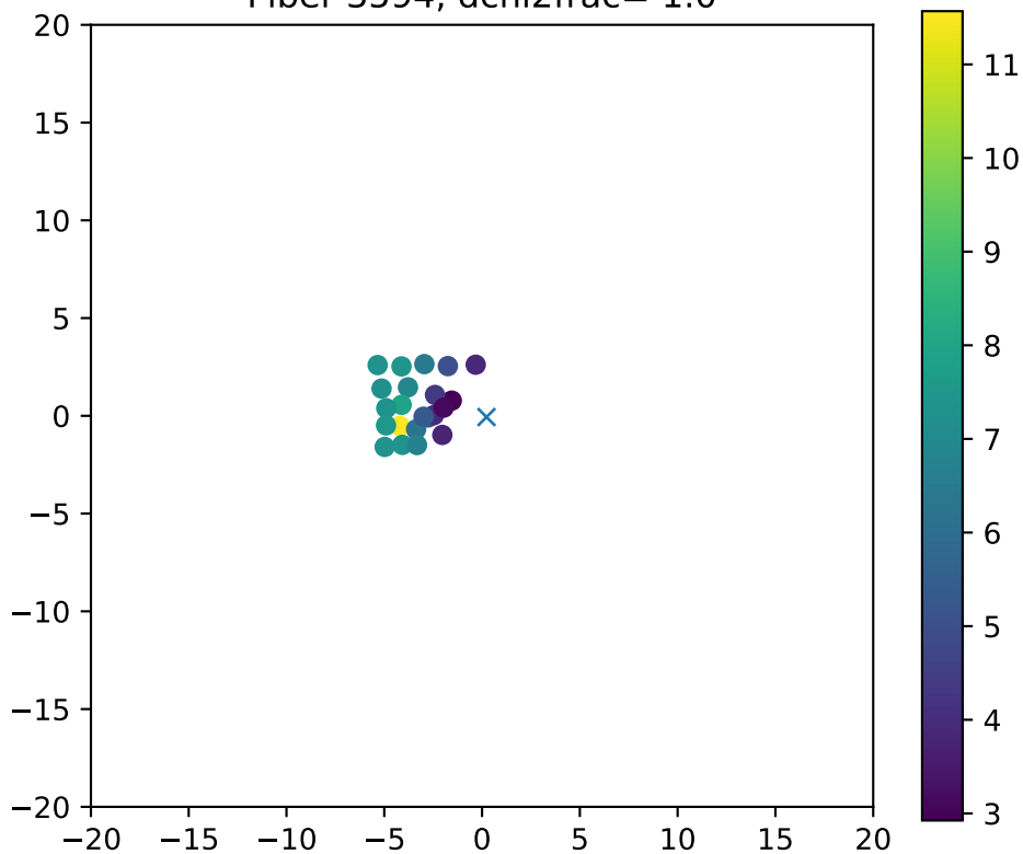
Fiber 3594, dchi2frac= 1.0
