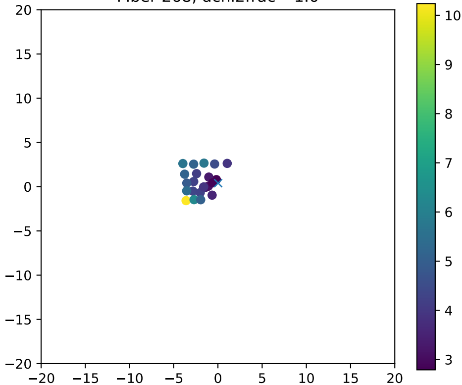
Fiber 268, dchi2frac= 1.0
