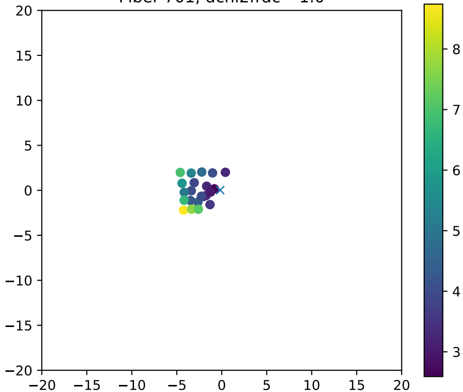
Fiber 701, dchi2frac= 1.0
