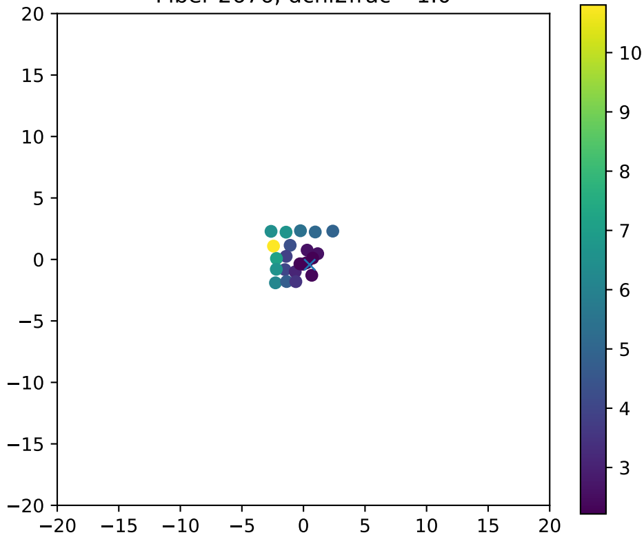
Fiber 2676, dchi2frac= 1.0
