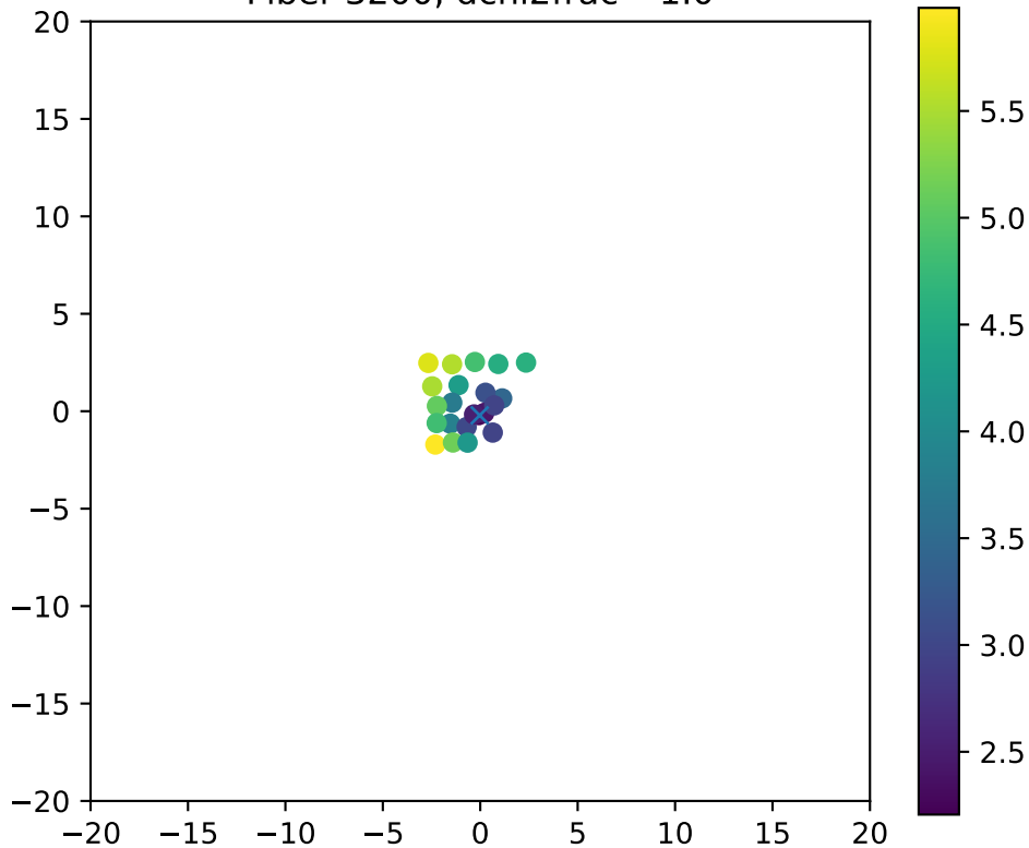
Fiber 3200, dchi2frac= 1.0
