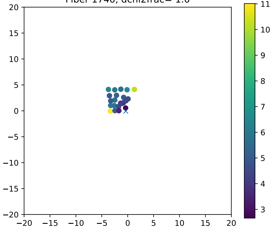
Fiber 1740, dchi2frac= 1.0
