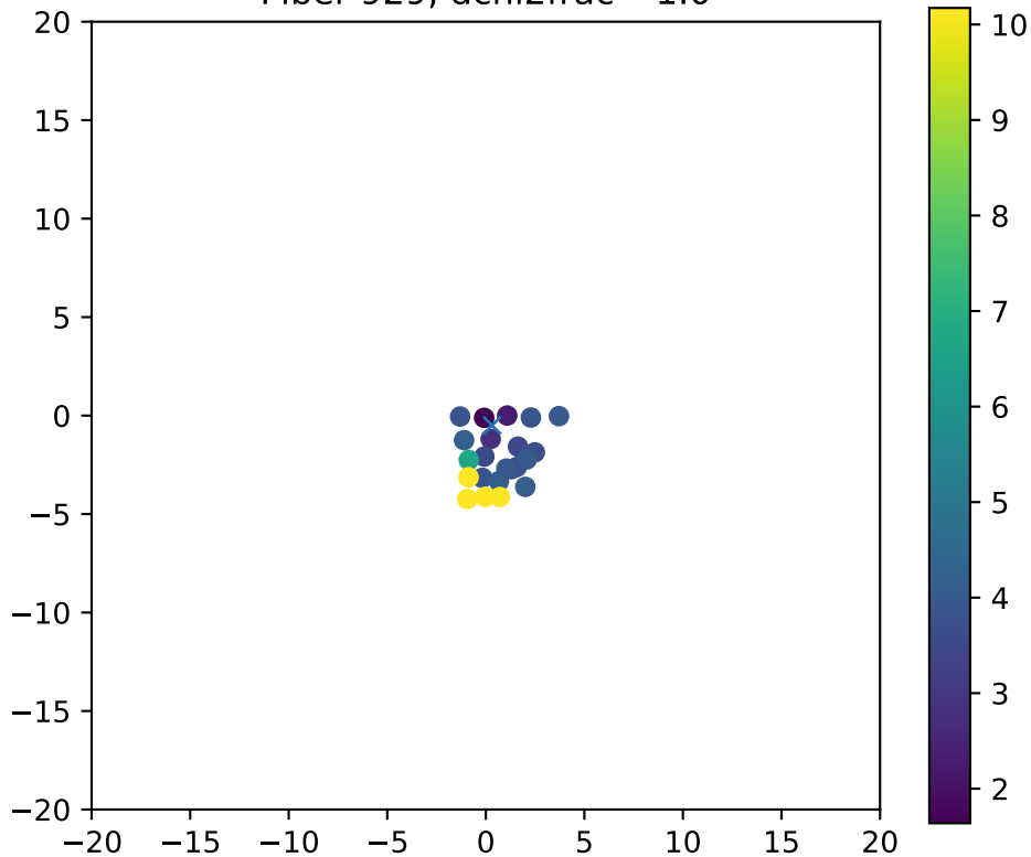
Fiber 929, dchi2frac= 1.0
