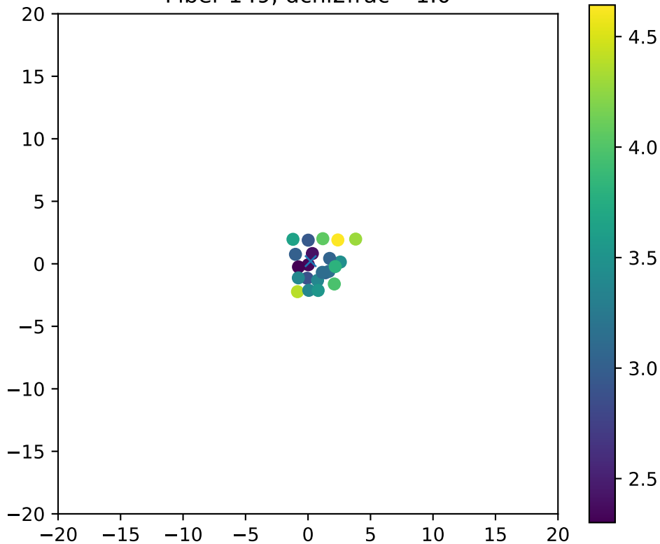
Fiber 149, dchi2frac= 1.0
