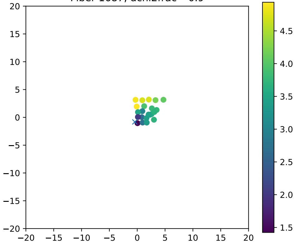
Fiber 1687, dchi2frac= 0.9
