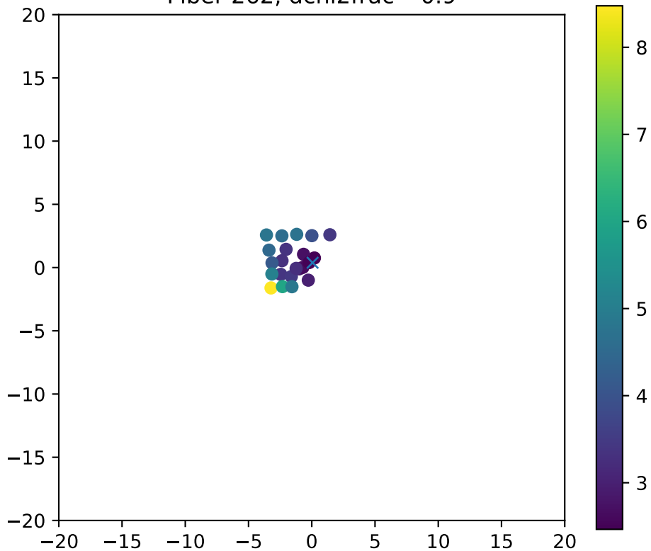
Fiber 262, dchi2frac= 0.9
