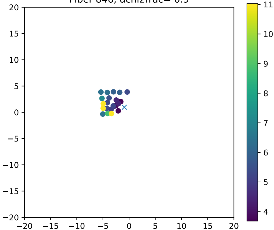
Fiber 846, dchi2frac= 0.9
