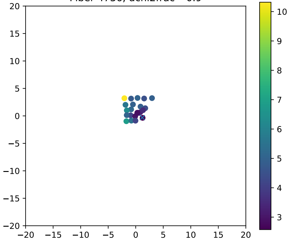
Fiber 4736, dchi2frac= 0.9
