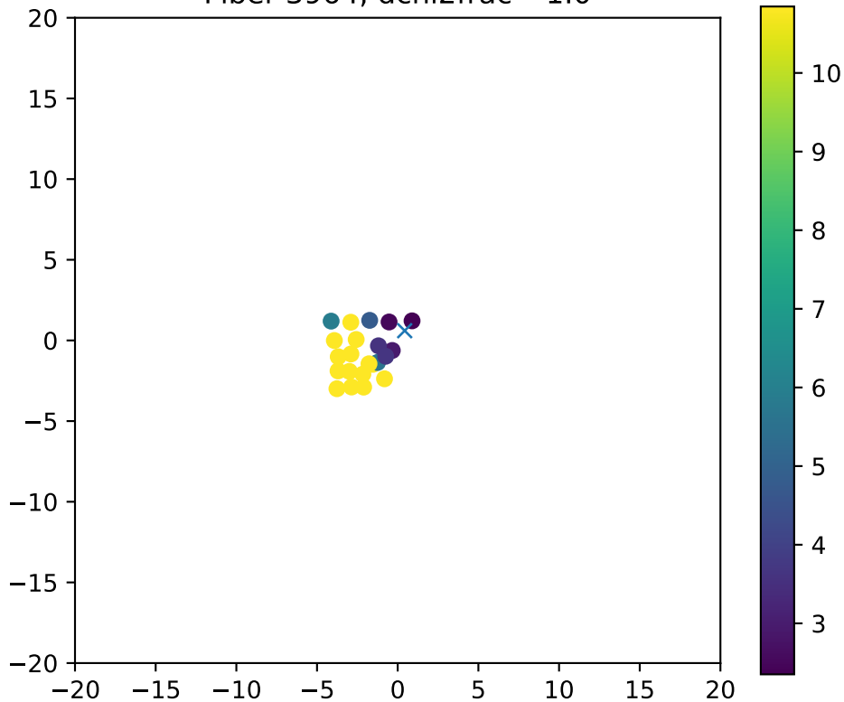
Fiber 3964, dchi2frac= 1.0
