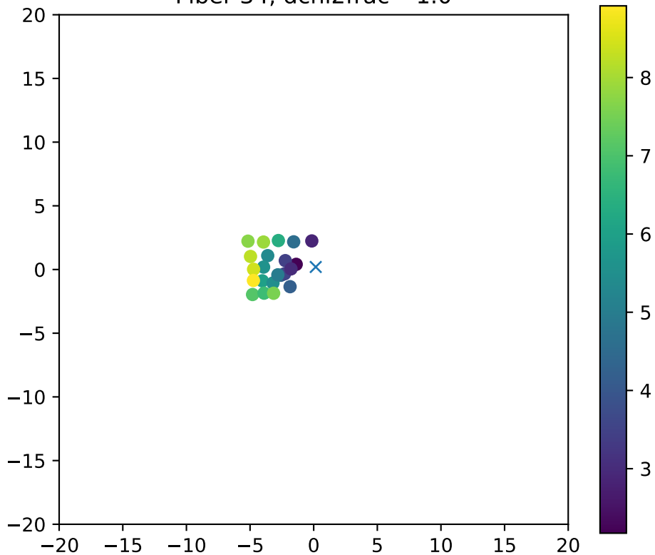
Fiber 34, dchi2frac= 1.0
