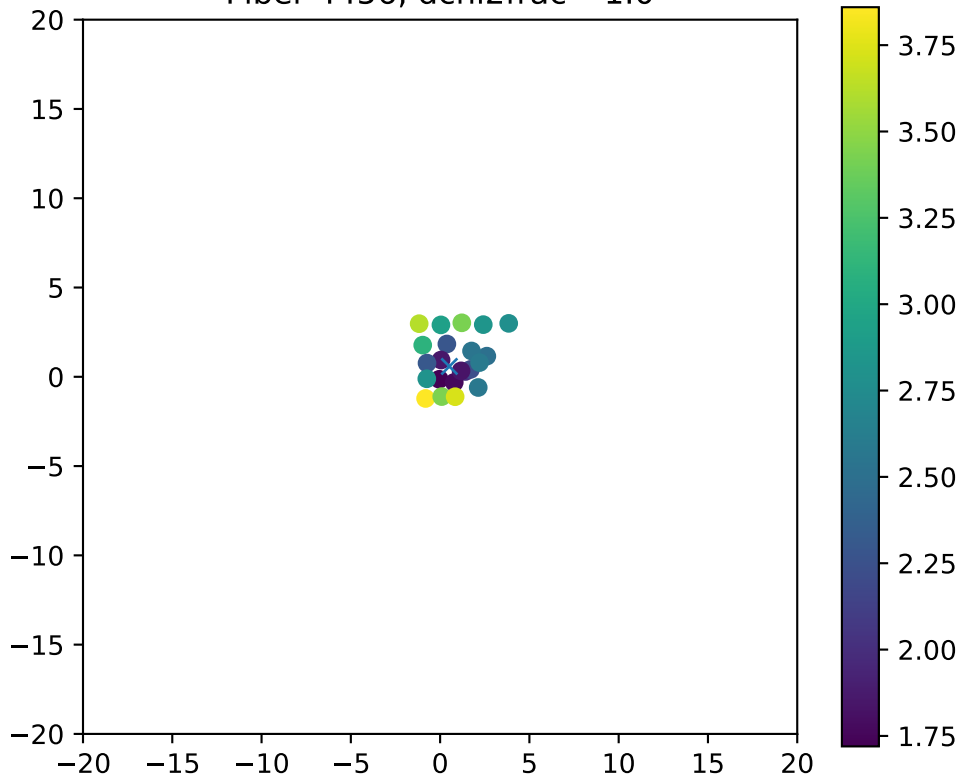
Fiber 4456, dchi2frac= 1.0
