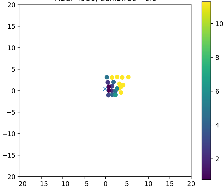
Fiber 4986, dchi2frac= 0.9
