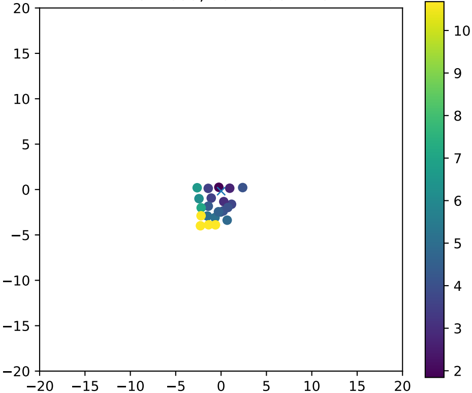
Fiber 2859, dchi2frac= 1.0
