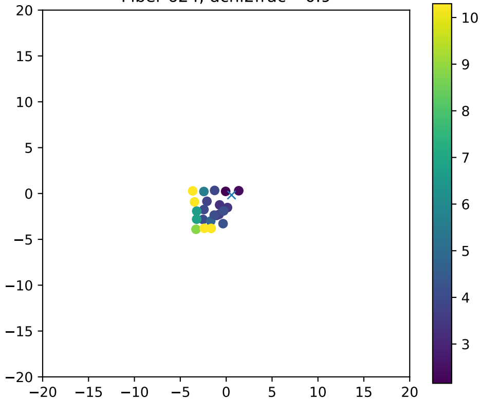
Fiber 624, dchi2frac= 0.9
