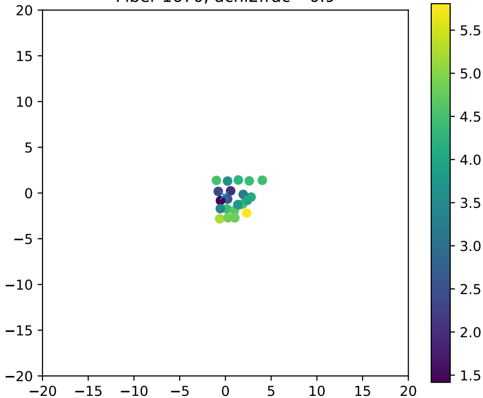
Fiber 1670, dchi2frac= 0.9
