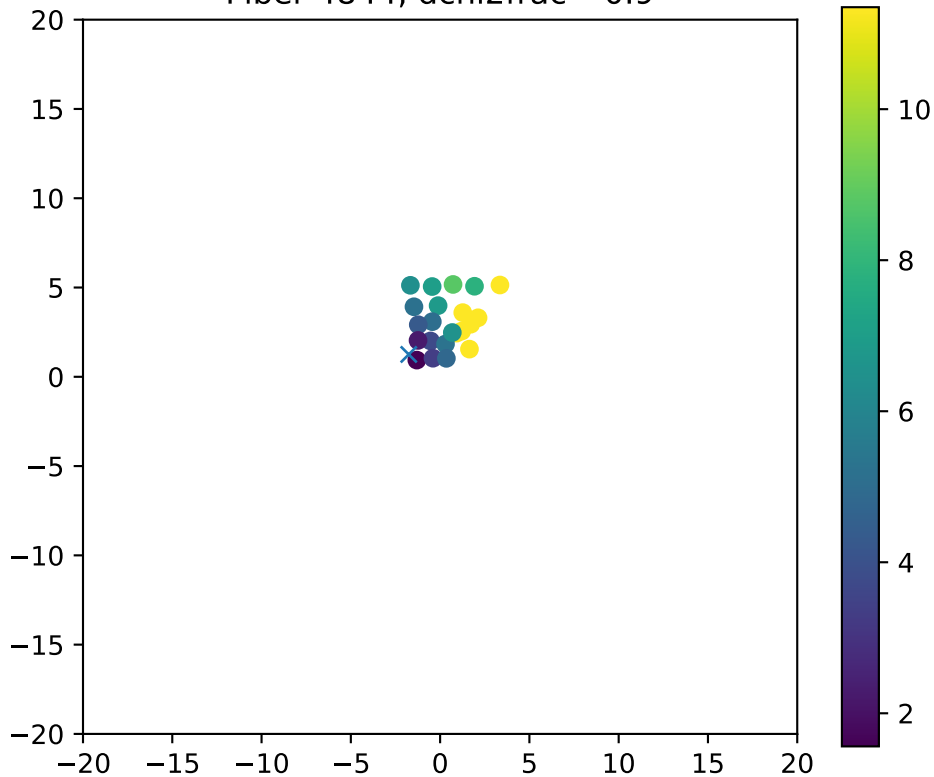
Fiber 4844, dchi2frac= 0.9
