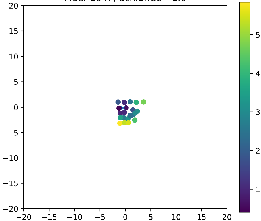
Fiber 2647, dchi2frac= 1.0
