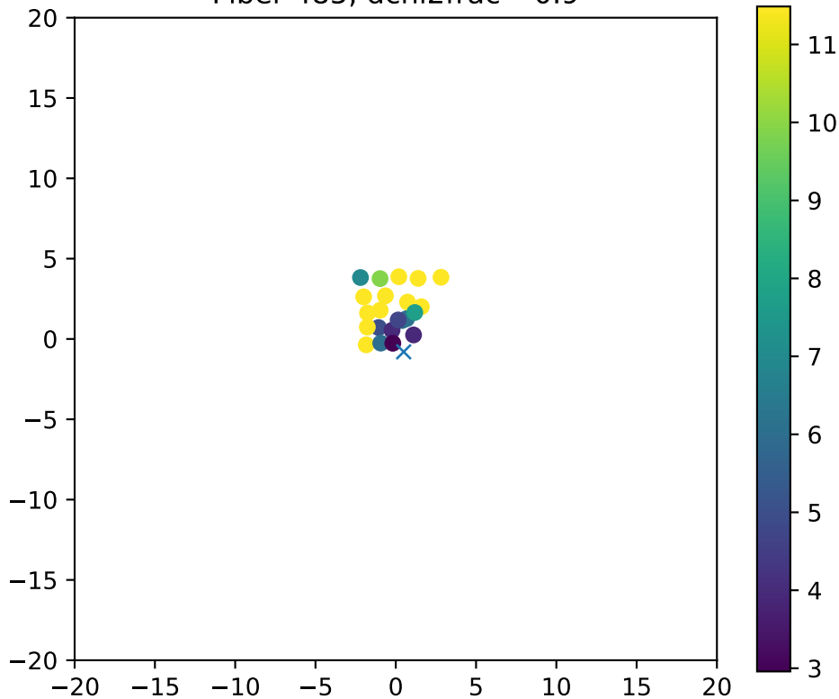
Fiber 485, dchi2frac= 0.9
