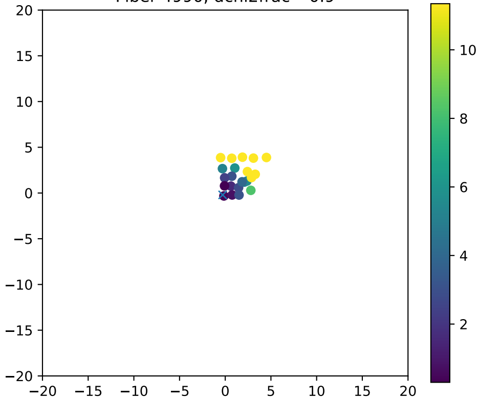
Fiber 4990, dchi2frac= 0.9
