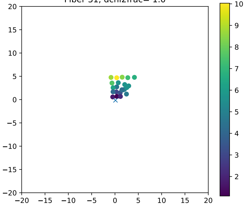
Fiber 31, dchi2frac= 1.0
