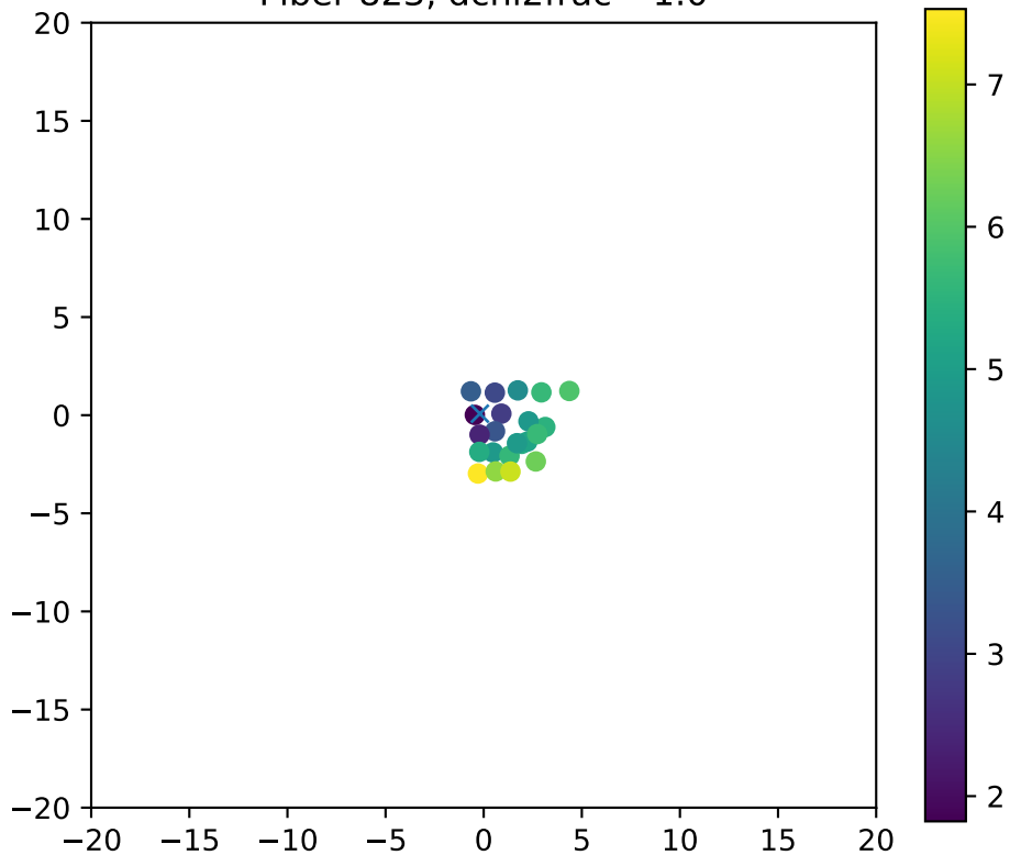
Fiber 823, dchi2frac= 1.0
