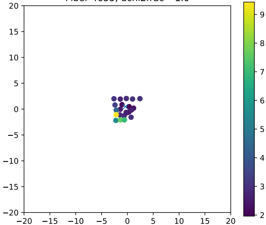
Fiber 4655, dchi2frac= 1.0
