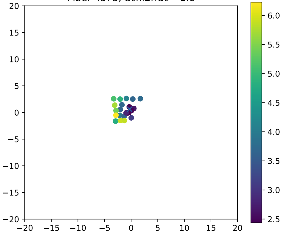
Fiber 4575, dchi2frac= 1.0
