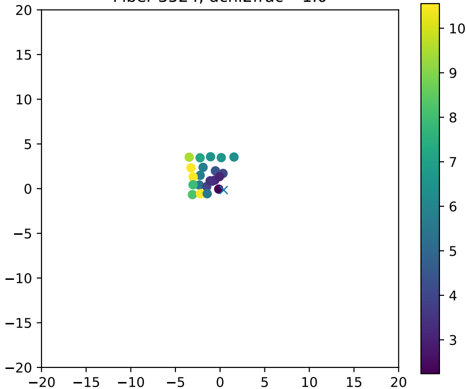
Fiber 3524, dchi2frac= 1.0
