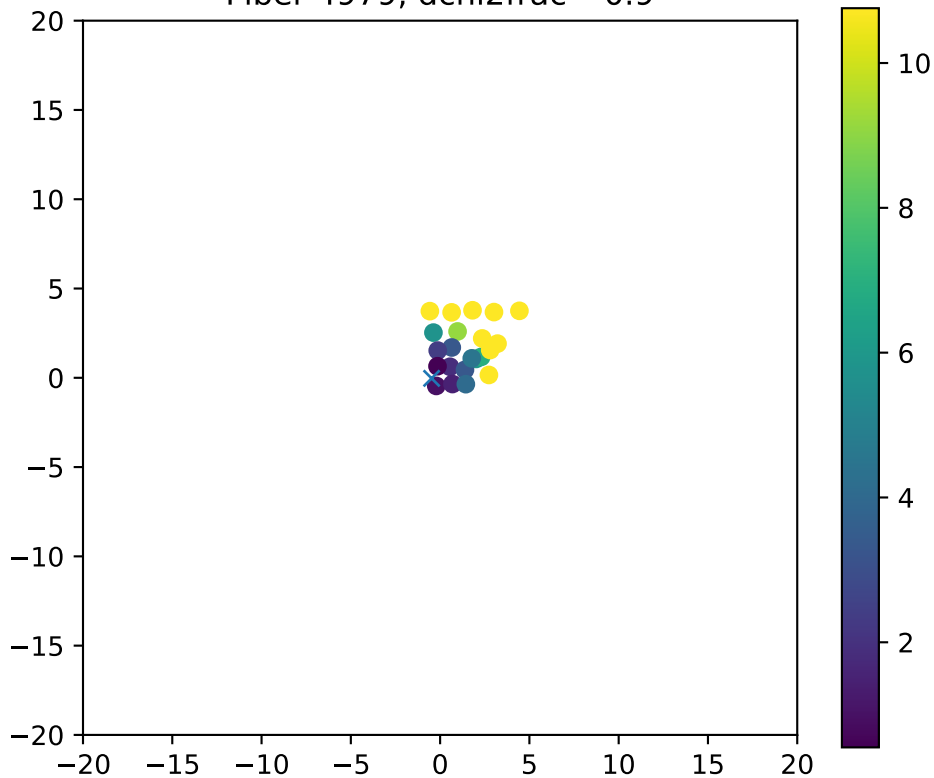
Fiber 4979, dchi2frac= 0.9
