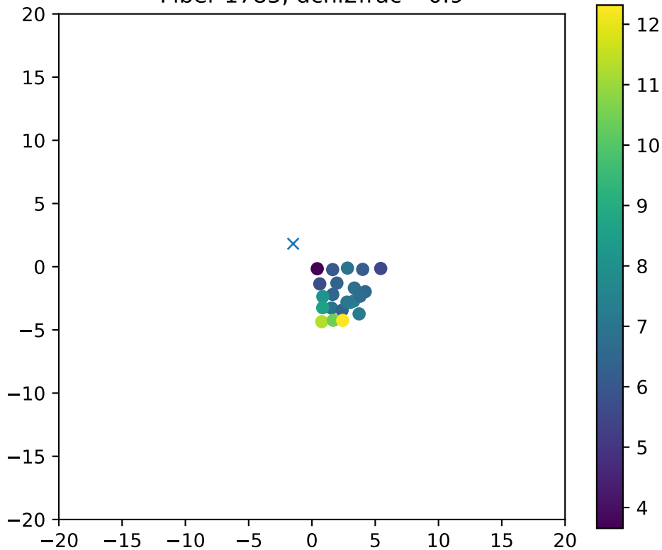
Fiber 1785, dchi2frac= 0.9
