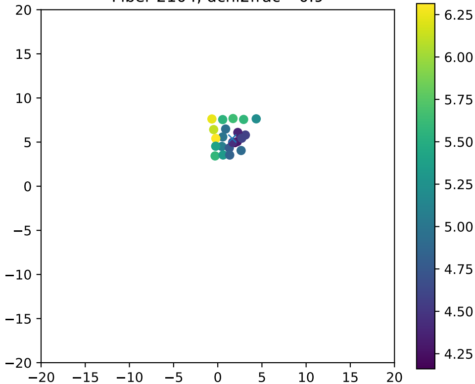
Fiber 2104, dchi2frac= 0.9
