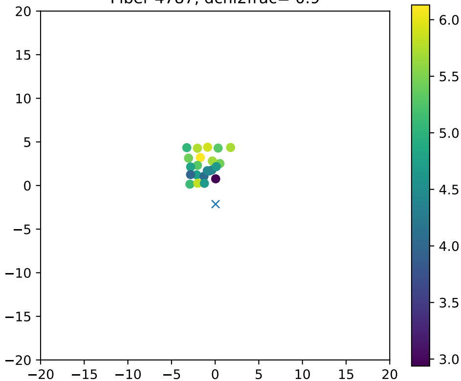
Fiber 4787, dchi2frac= 0.9
