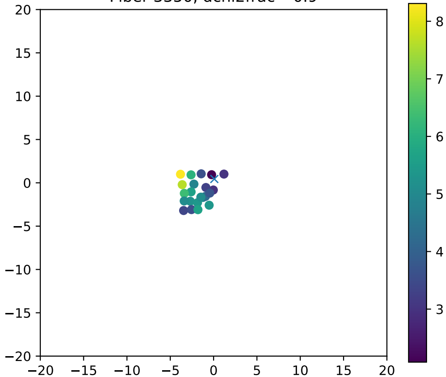
Fiber 3350, dchi2frac= 0.9
