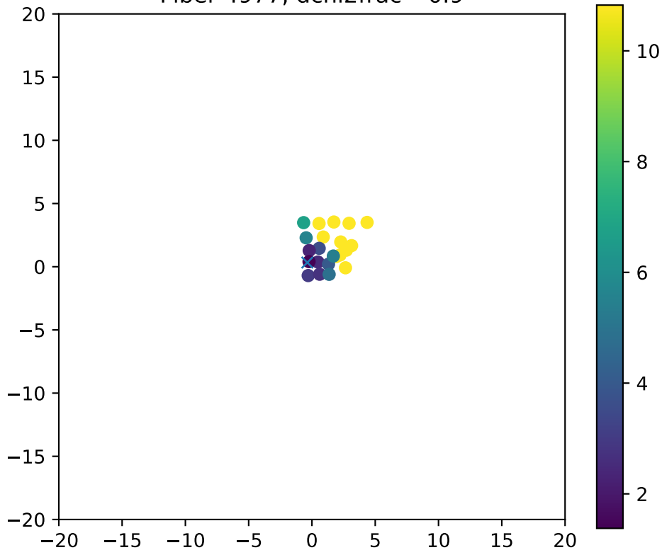
Fiber 4977, dchi2frac= 0.9
