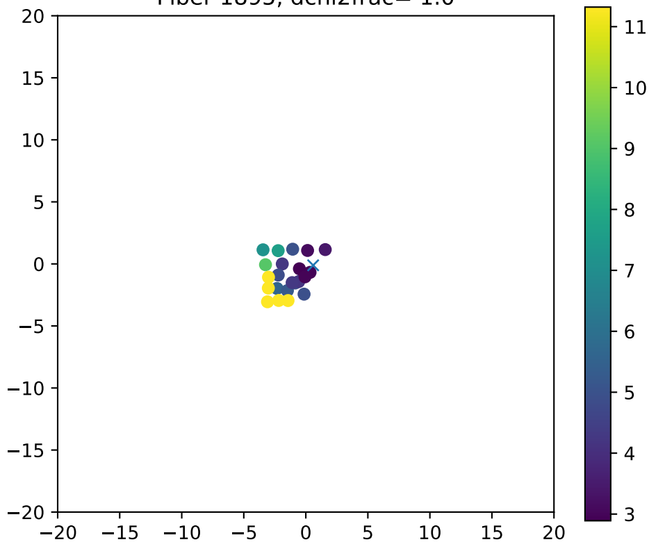
Fiber 1895, dchi2frac= 1.0
