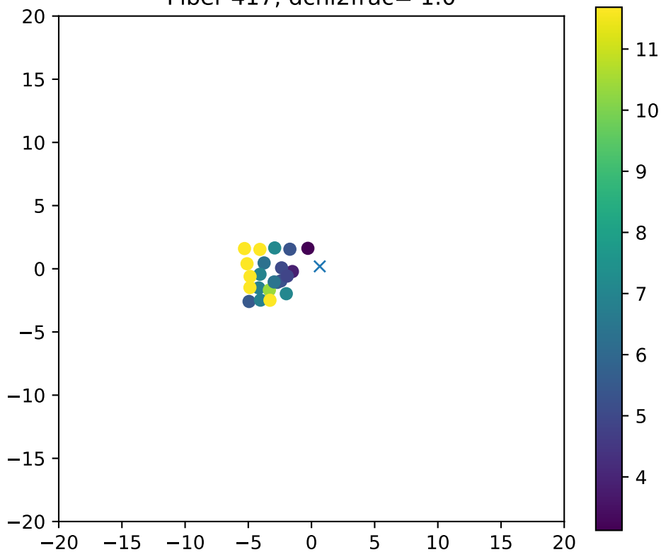
Fiber 417, dchi2frac= 1.0
