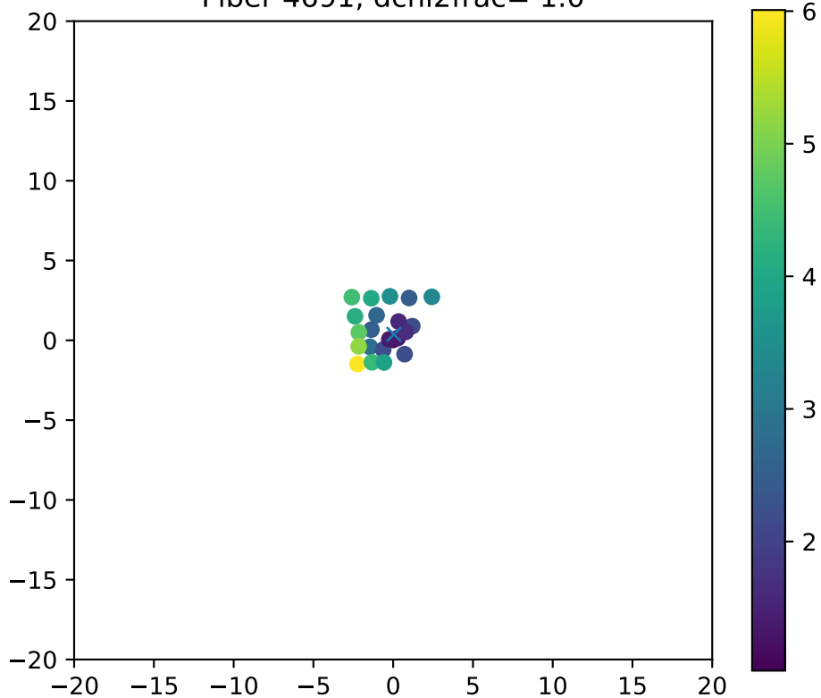
Fiber 4691, dchi2frac= 1.0
