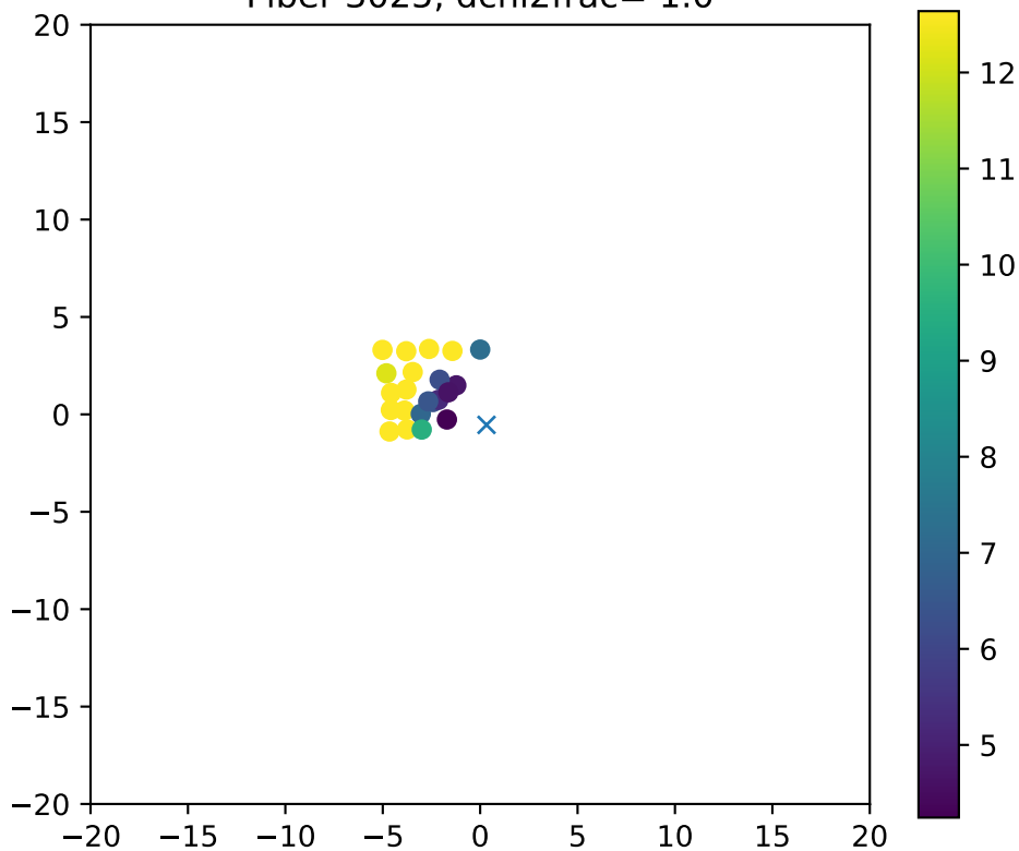
Fiber 3025, dchi2frac= 1.0
