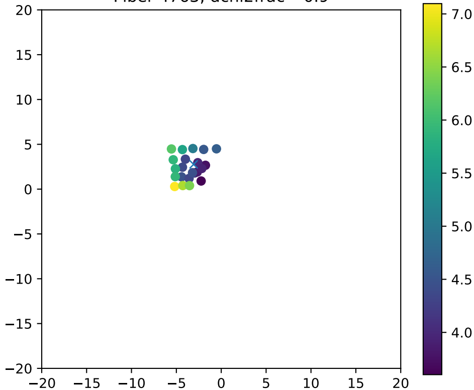
Fiber 4763, dchi2frac= 0.9
