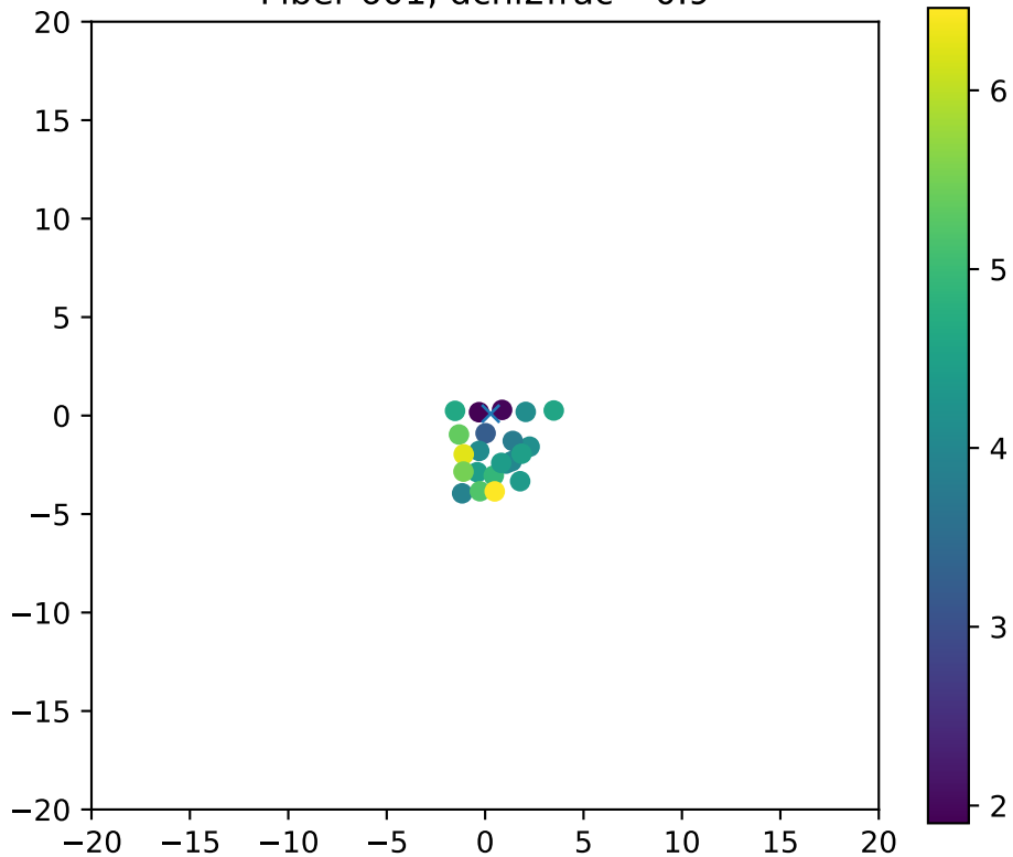
Fiber 601, dchi2frac= 0.9
