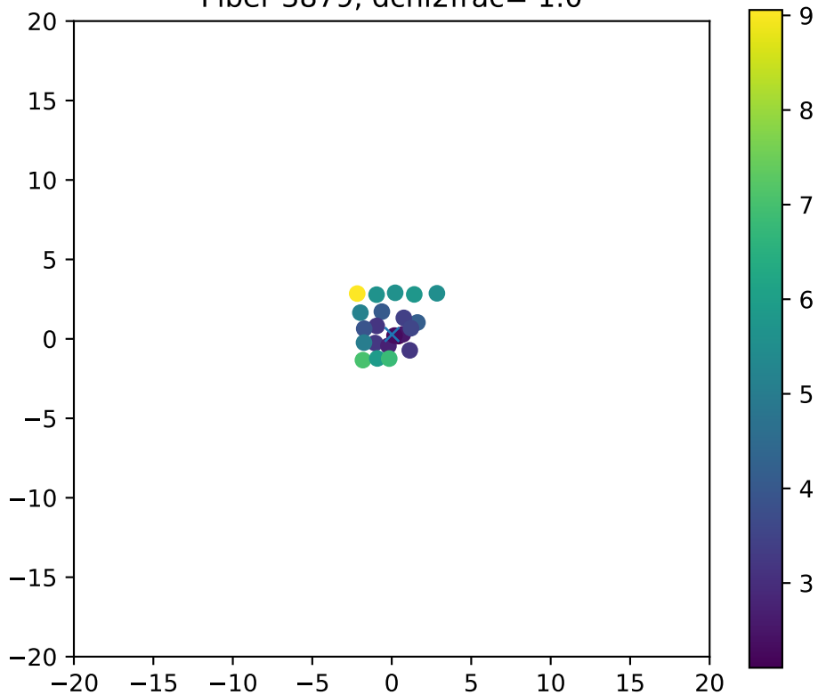
Fiber 3879, dchi2frac= 1.0
