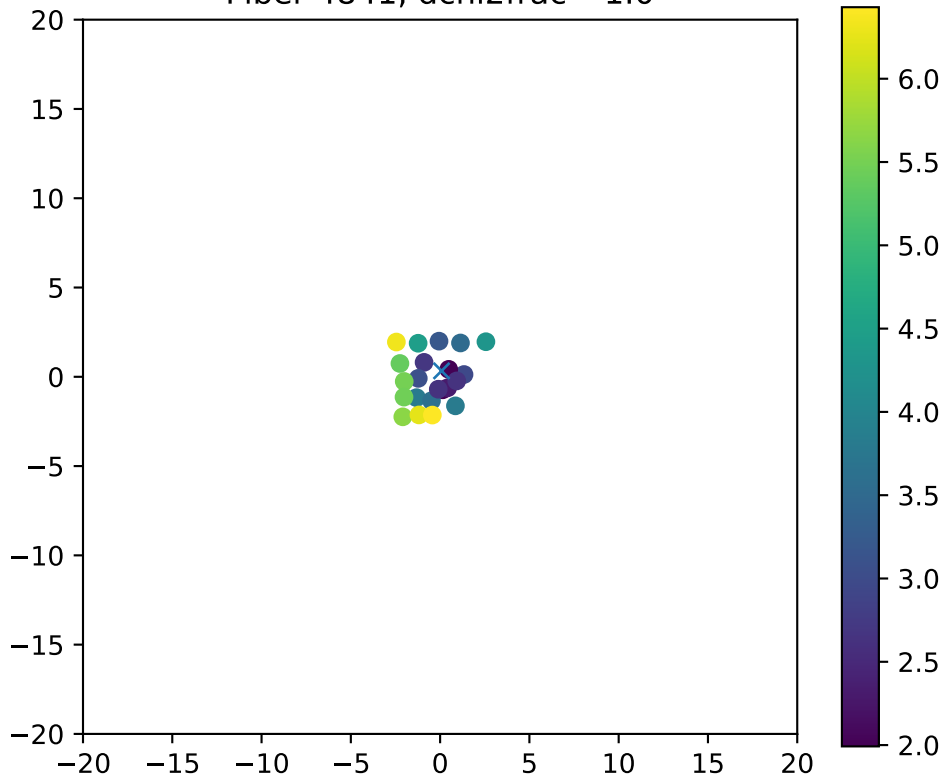
Fiber 4841, dchi2frac= 1.0
