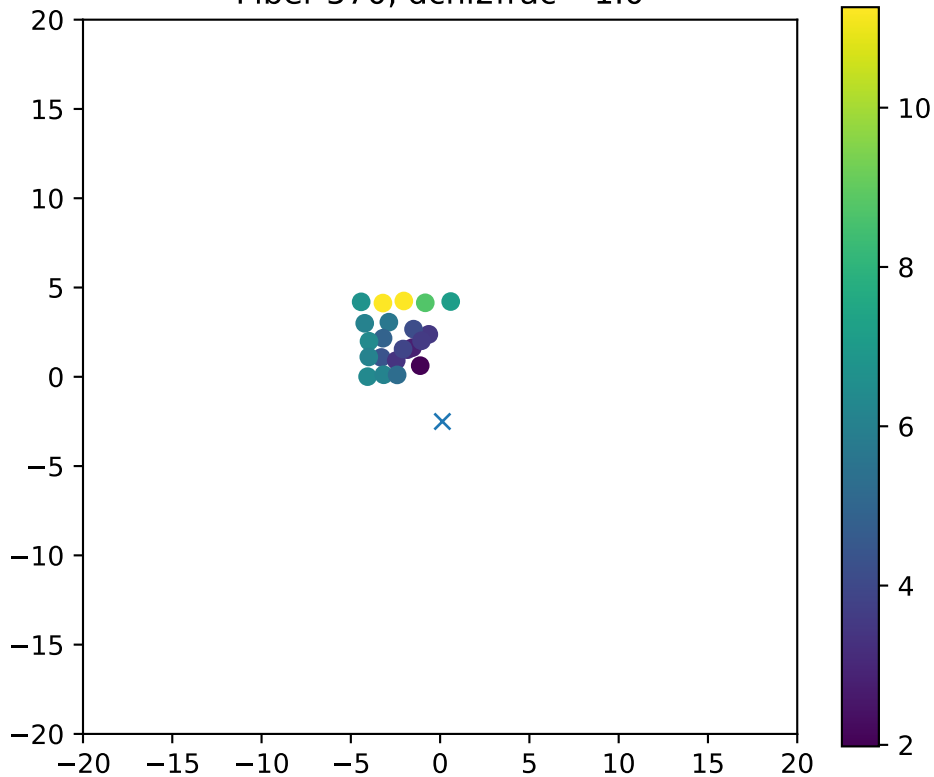
Fiber 570, dchi2frac= 1.0
