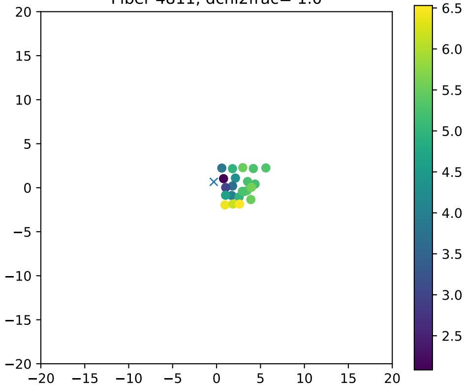
Fiber 4811, dchi2frac= 1.0
