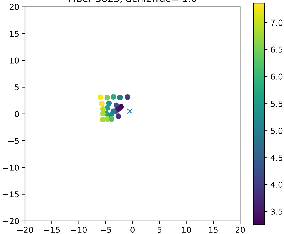
Fiber 3625, dchi2frac= 1.0
