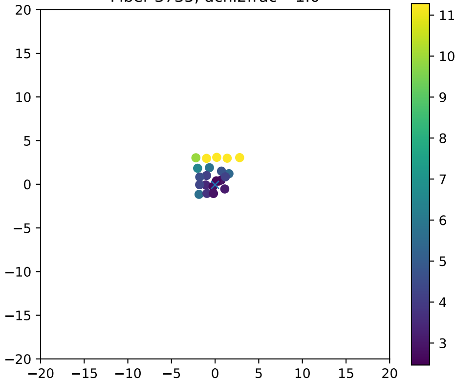
Fiber 3735, dchi2frac= 1.0
