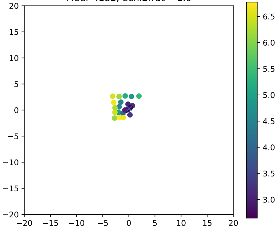
Fiber 4182, dchi2frac= 1.0
