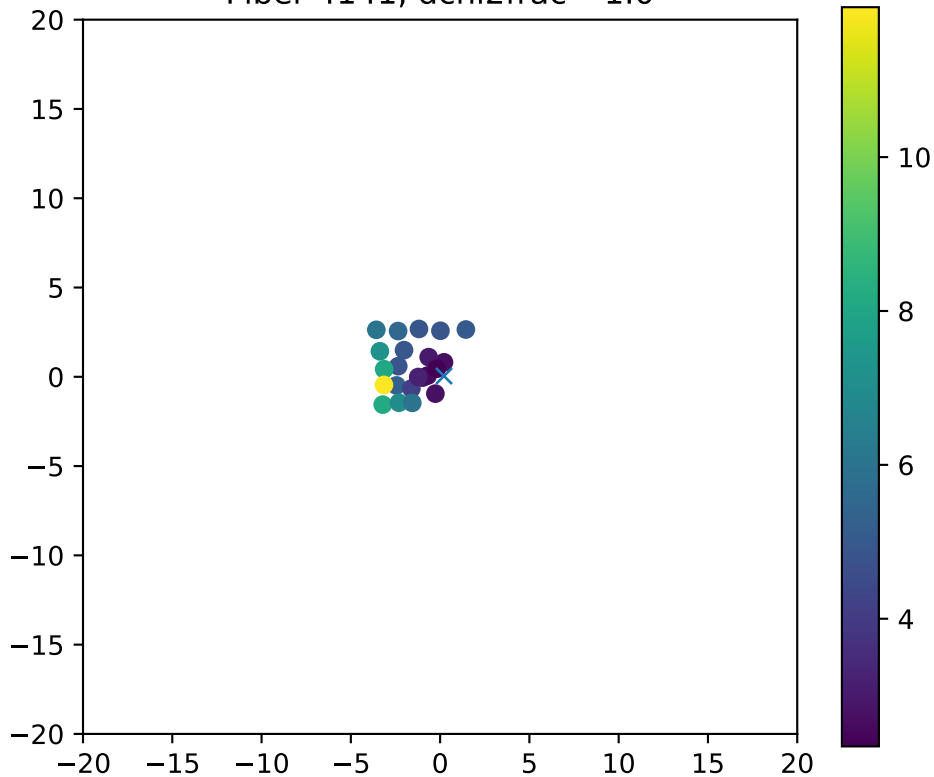
Fiber 4141, dchi2frac= 1.0
