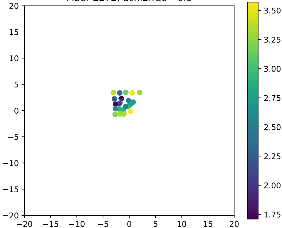
Fiber 2272, dchi2frac= 0.9
