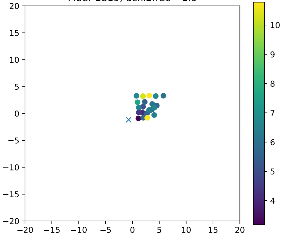
Fiber 1819, dchi2frac= 1.0
