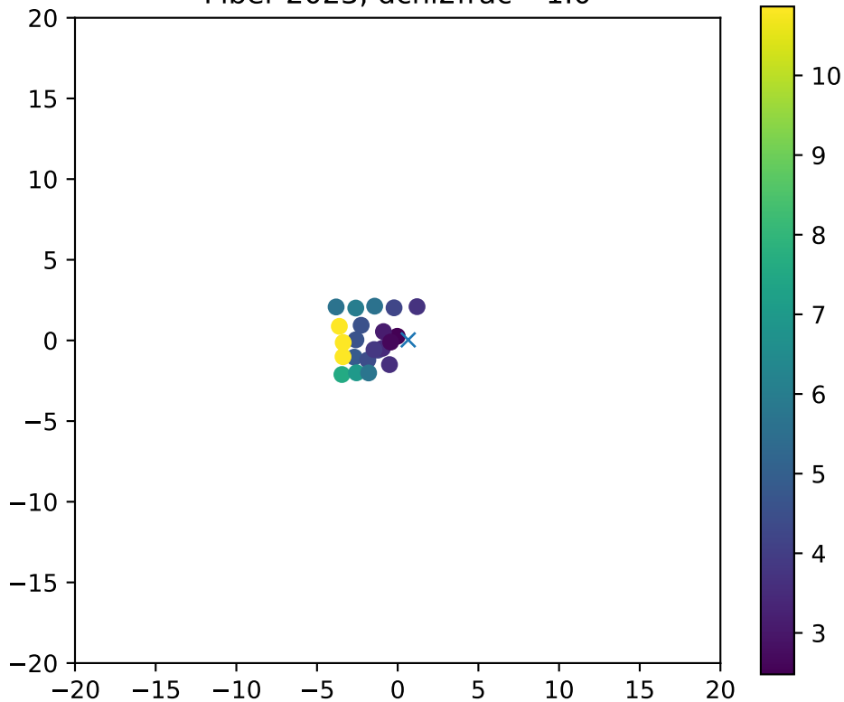
Fiber 2023, dchi2frac= 1.0
