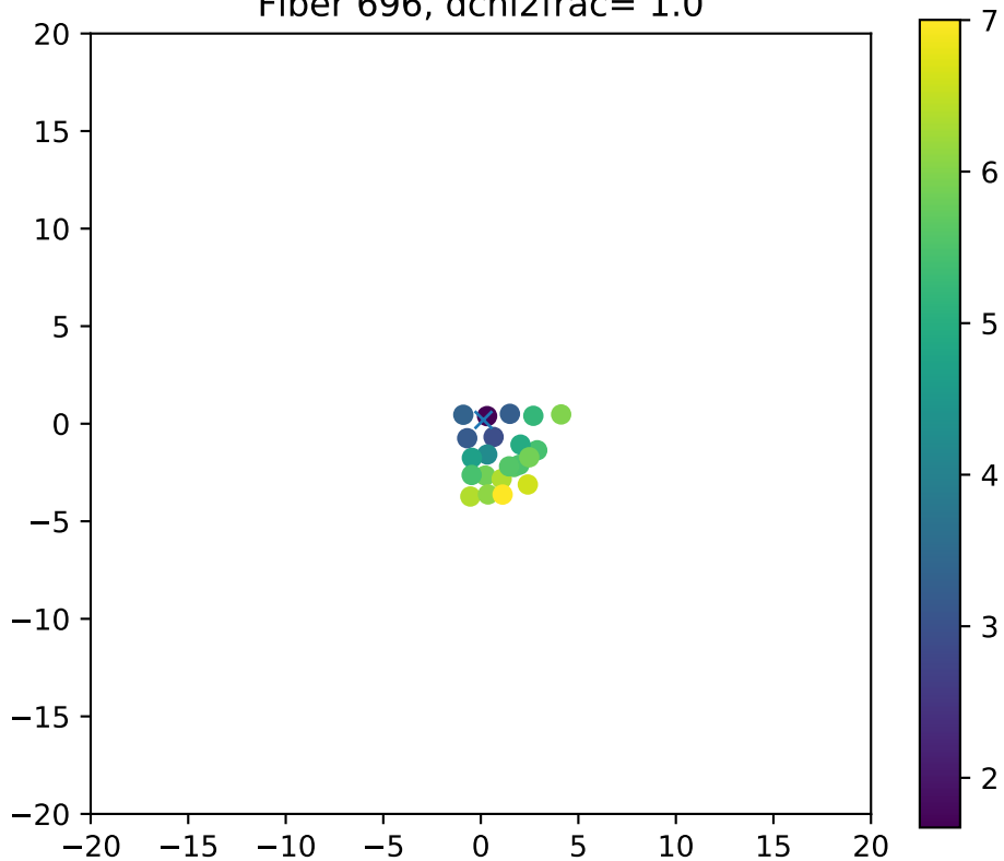
Fiber 696, dchi2frac= 1.0
