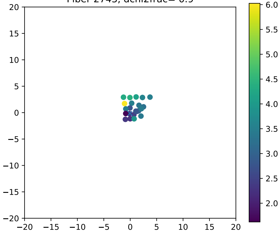
Fiber 2743, dchi2frac= 0.9
