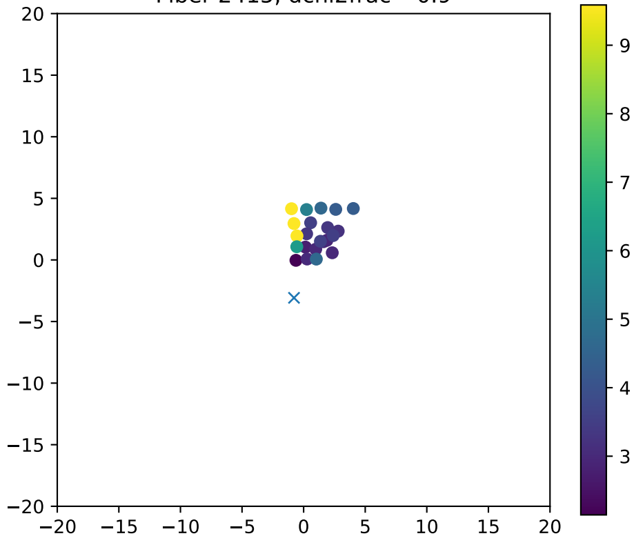
Fiber 2415, dchi2frac= 0.9
