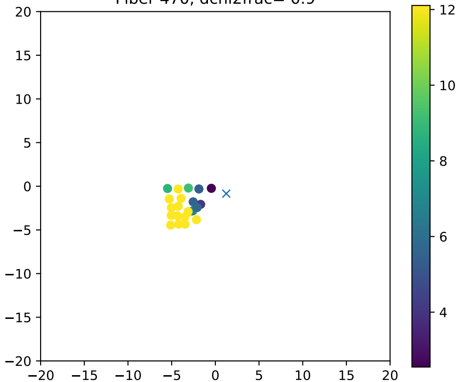
Fiber 470, dchi2frac= 0.9
