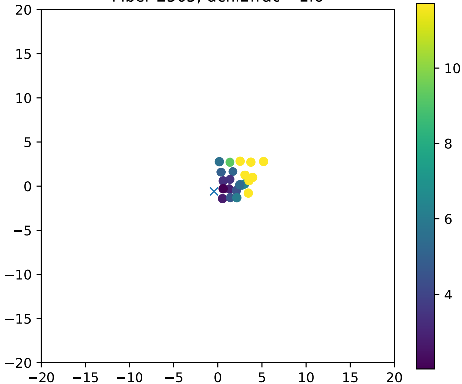
Fiber 2505, dchi2frac= 1.0
