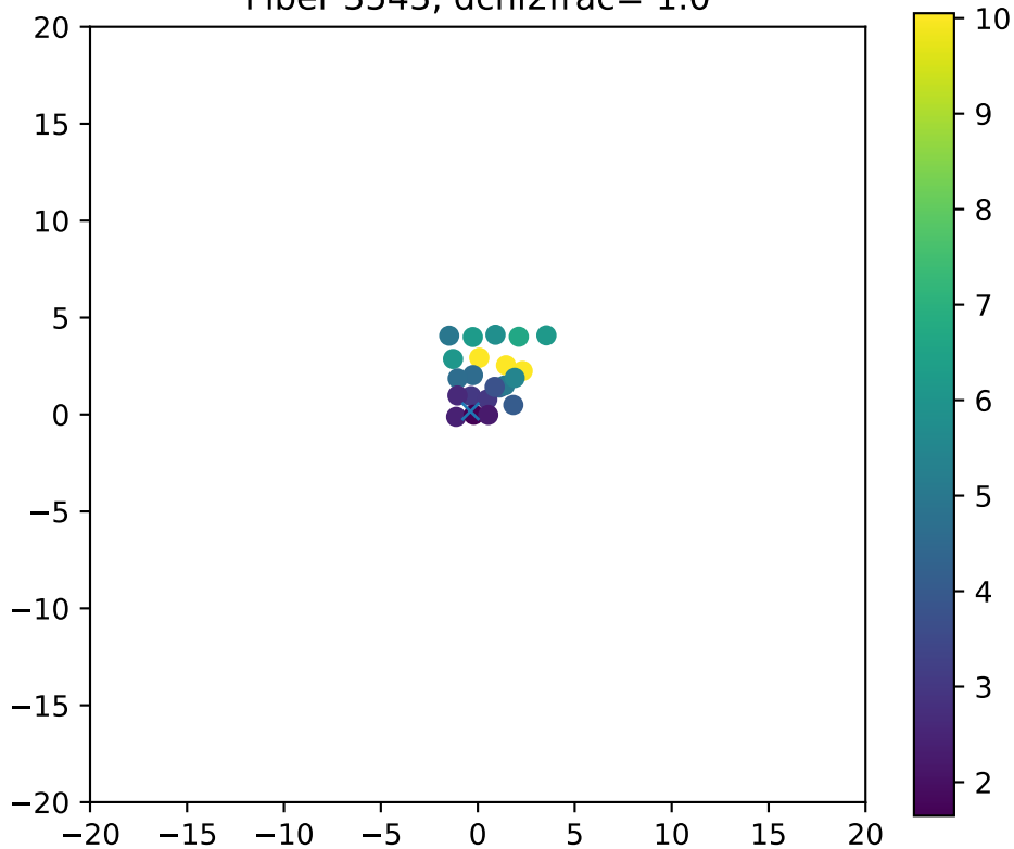
Fiber 3543, dchi2frac= 1.0
