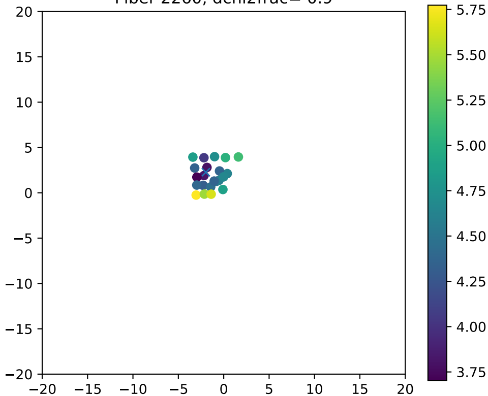
Fiber 2260, dchi2frac= 0.9
