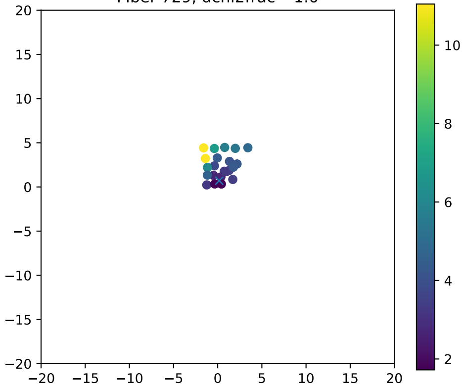
Fiber 729, dchi2frac= 1.0
