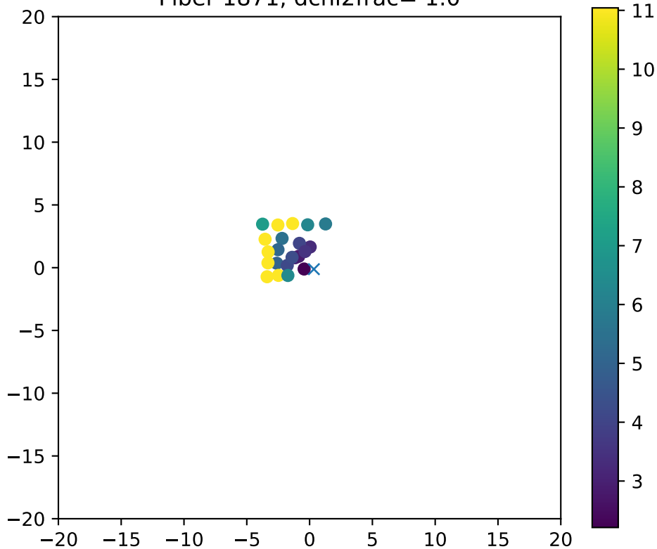
Fiber 1871, dchi2frac= 1.0
