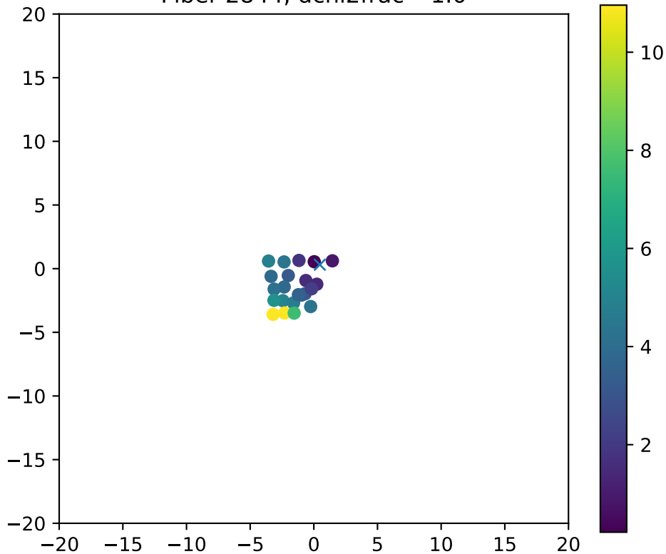
Fiber 2844, dchi2frac= 1.0
