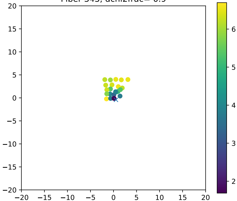
Fiber 343, dchi2frac= 0.9
