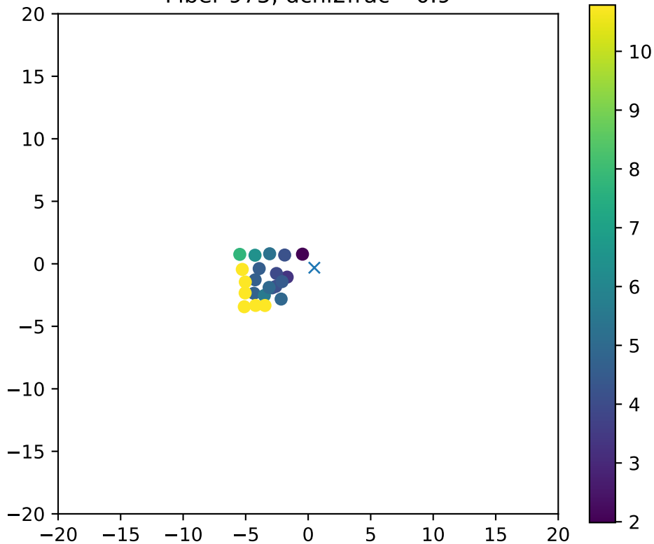
Fiber 975, dchi2frac= 0.9
