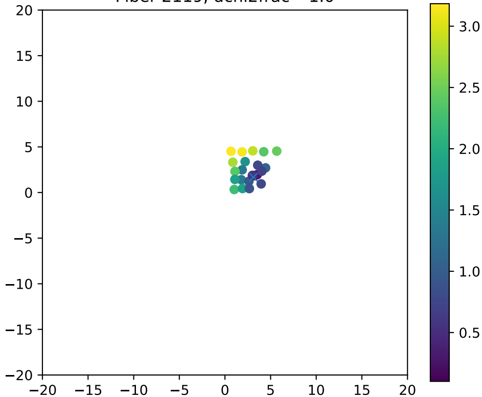
Fiber 2119, dchi2frac= 1.0
