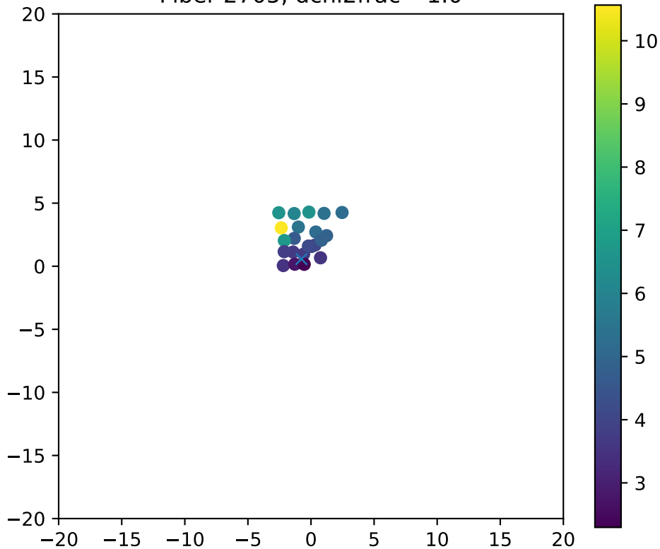
Fiber 2705, dchi2frac= 1.0
