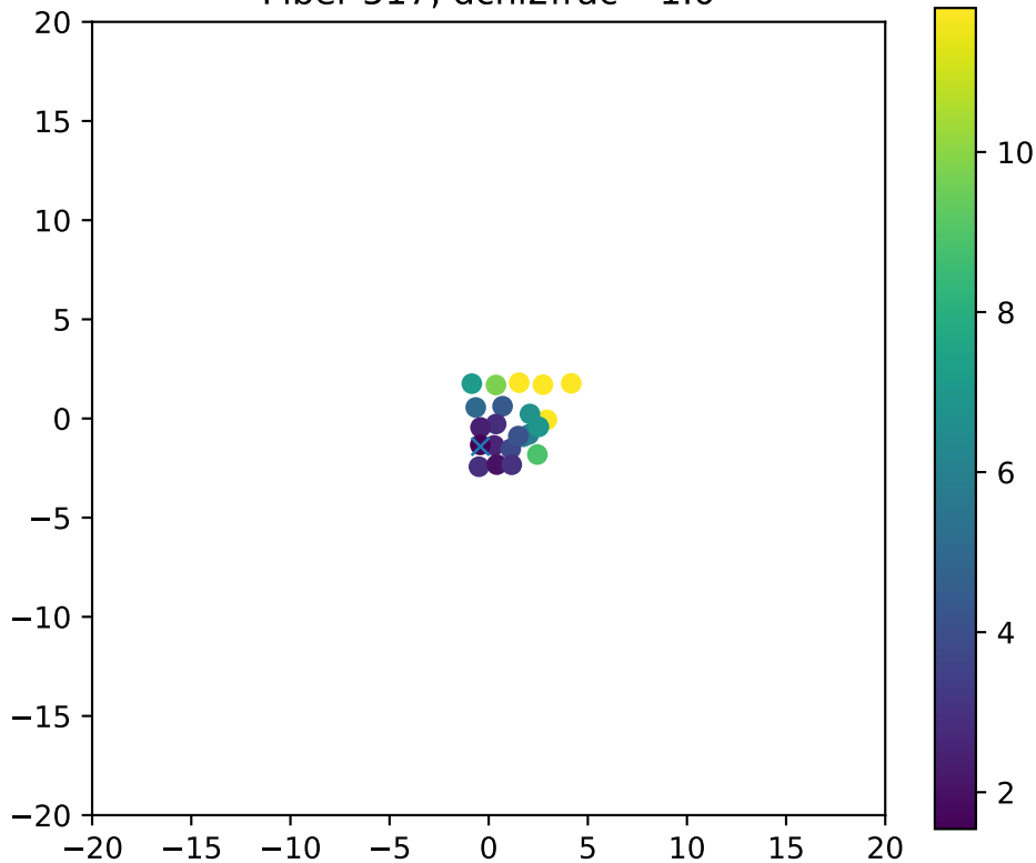
Fiber 517, dchi2frac= 1.0
