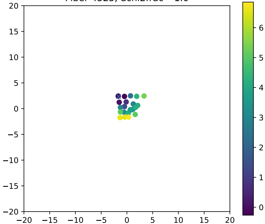
Fiber 4525, dchi2frac= 1.0
