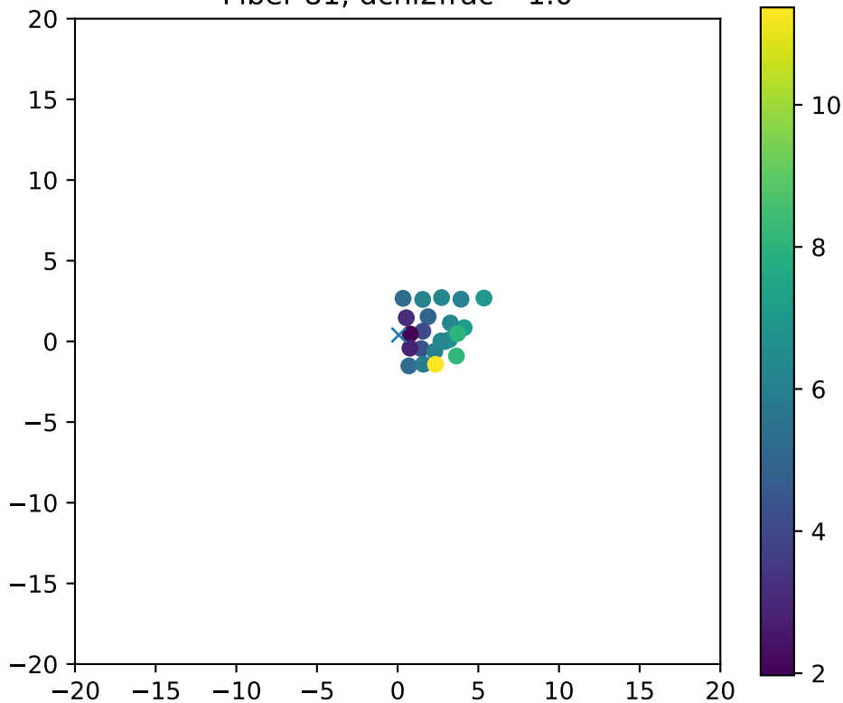
Fiber 81, dchi2frac= 1.0
