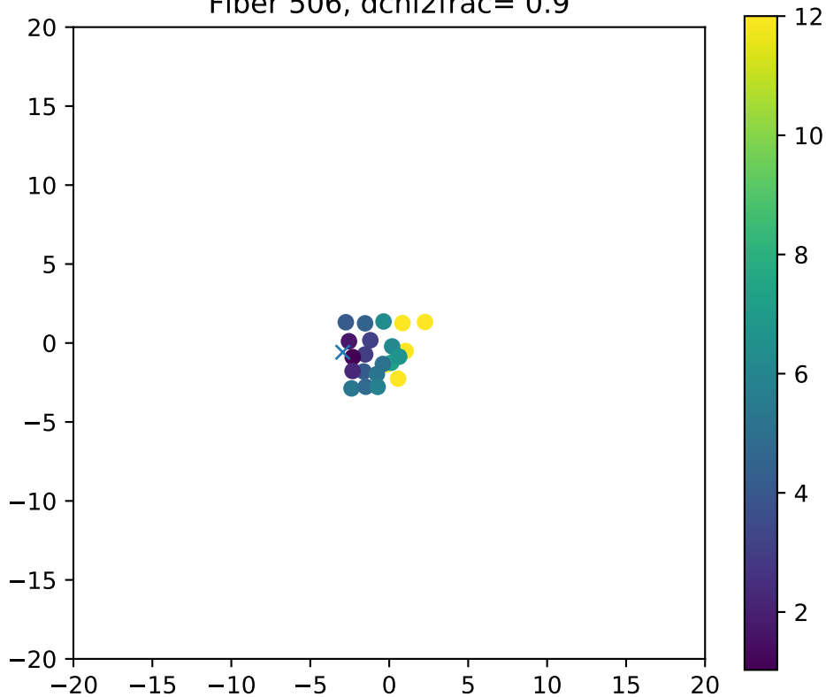
Fiber 506, dchi2frac= 0.9
