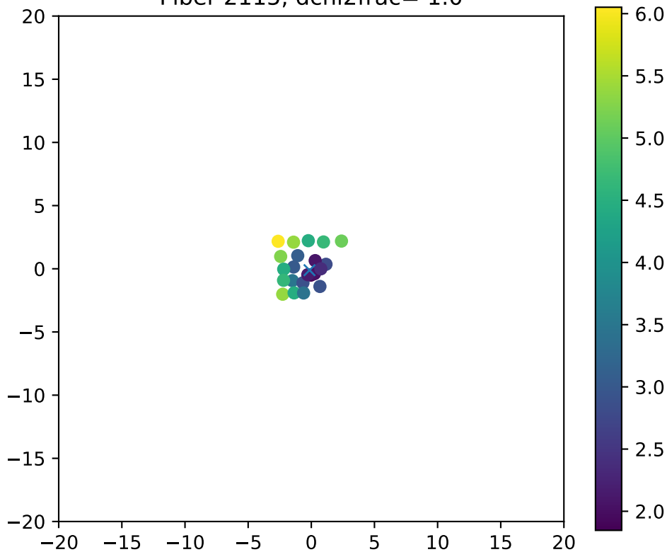
Fiber 2115, dchi2frac= 1.0
