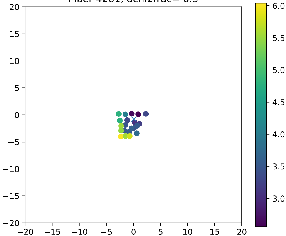
Fiber 4261, dchi2frac= 0.9
