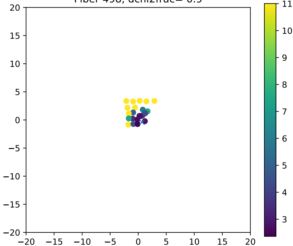
Fiber 498, dchi2frac= 0.9
