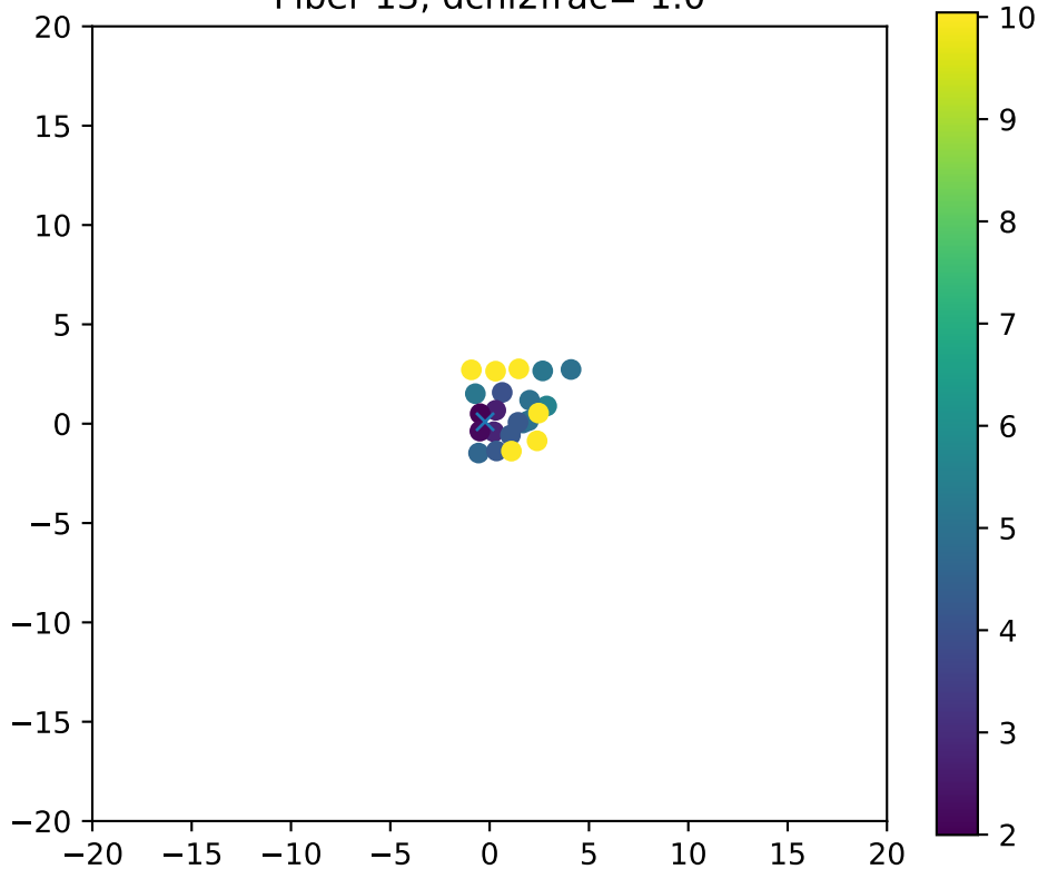
Fiber 13, dchi2frac= 1.0
