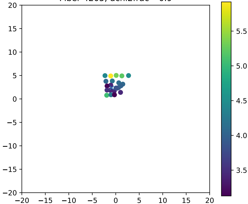
Fiber 4205, dchi2frac= 0.9
