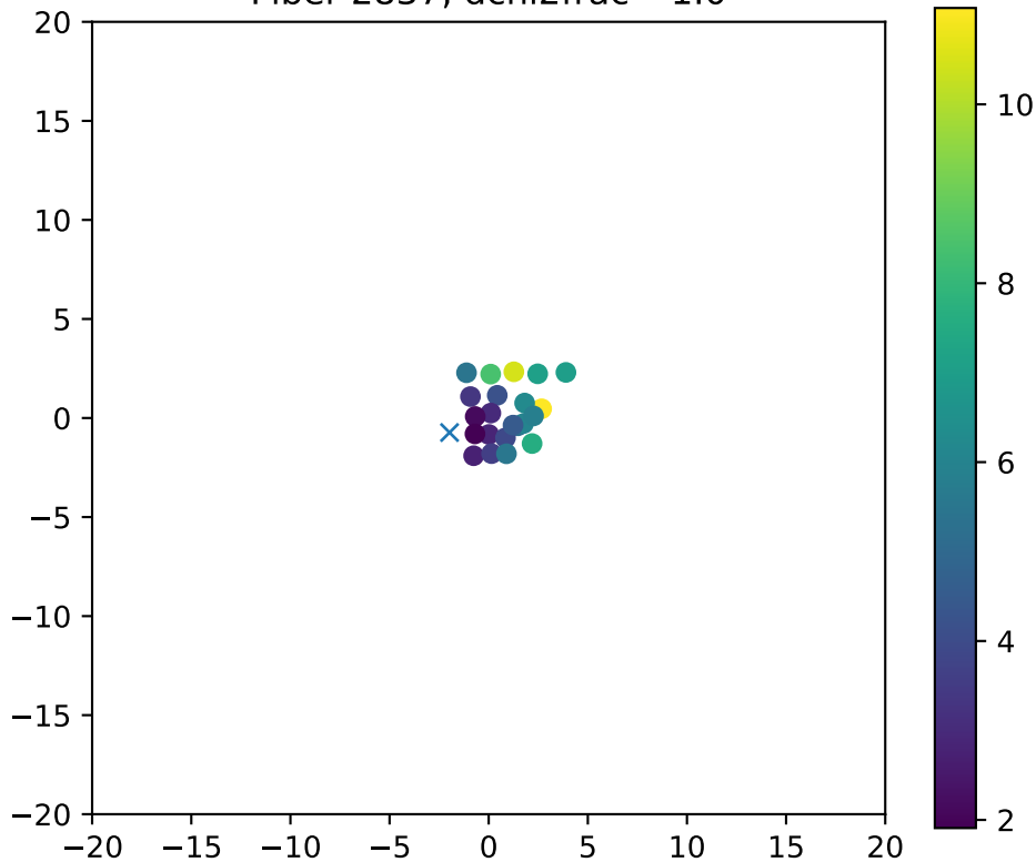
Fiber 2837, dchi2frac= 1.0
