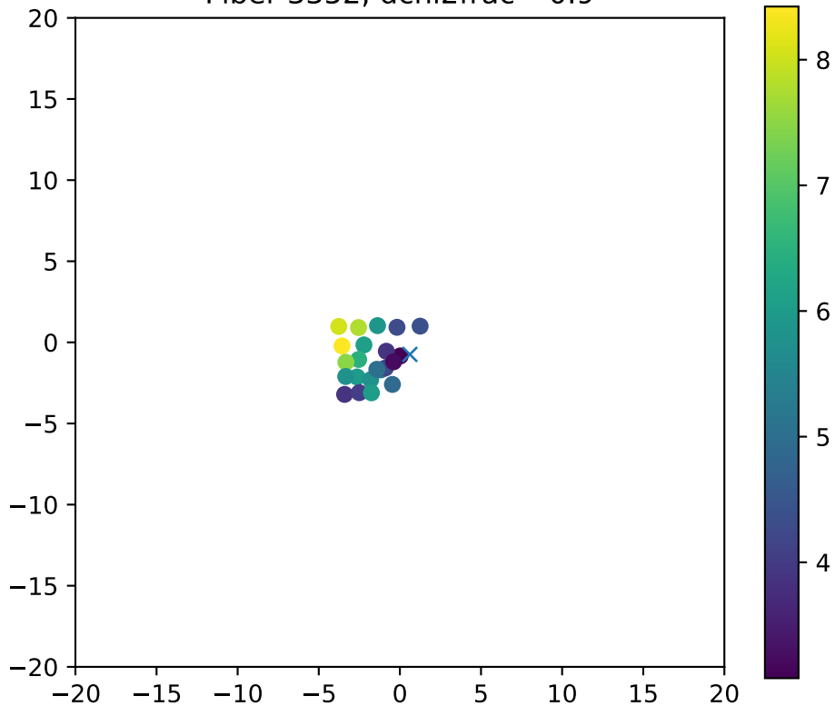
Fiber 3352, dchi2frac= 0.9
