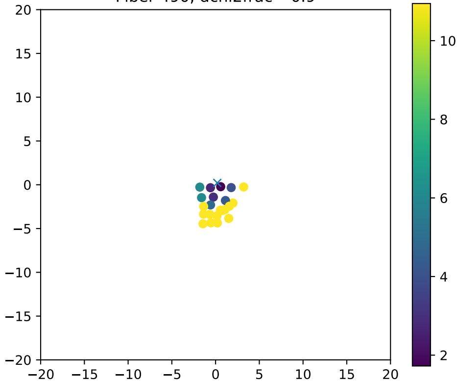
Fiber 490, dchi2frac= 0.9
