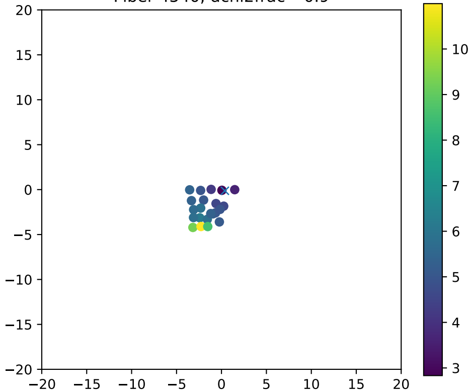
Fiber 4540, dchi2frac= 0.9
