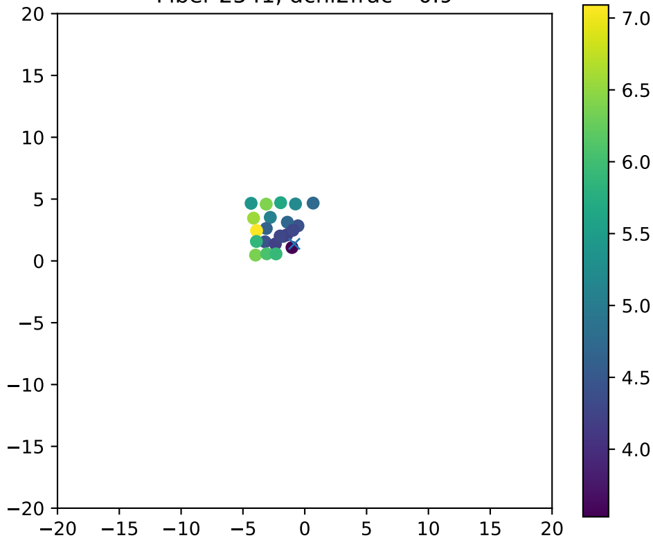
Fiber 2541, dchi2frac= 0.9
