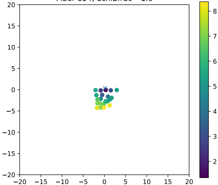
Fiber 854, dchi2frac= 1.0
