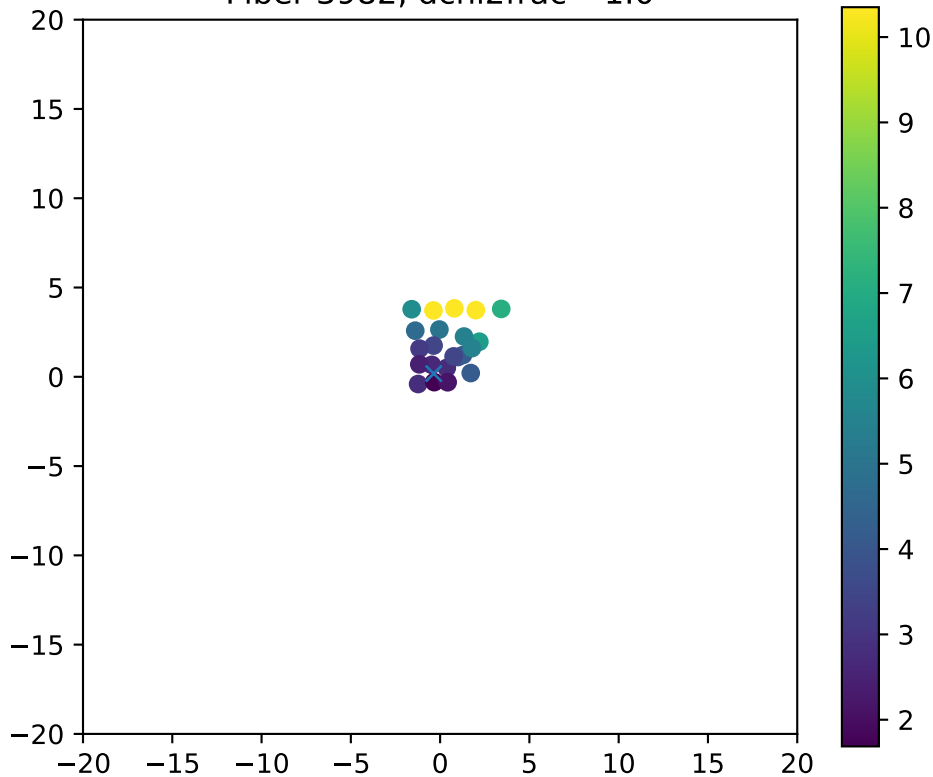
Fiber 3982, dchi2frac= 1.0
