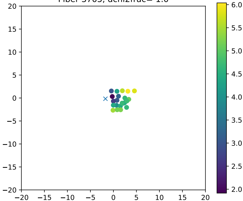
Fiber 3705, dchi2frac= 1.0
