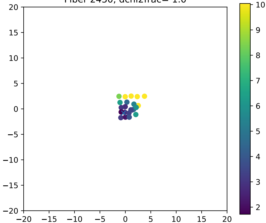
Fiber 2430, dchi2frac= 1.0
