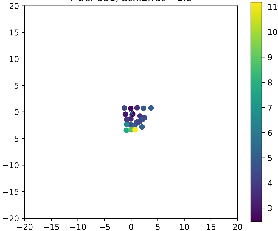
Fiber 931, dchi2frac= 1.0
