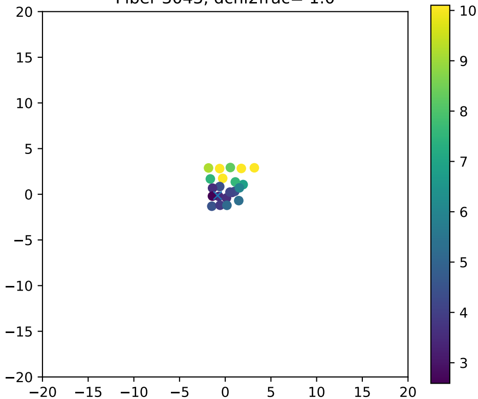
Fiber 3043, dchi2frac= 1.0
