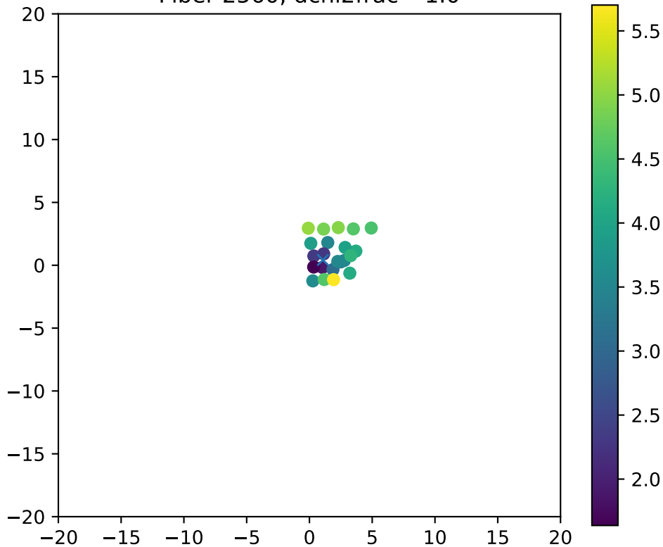
Fiber 2560, dchi2frac= 1.0
