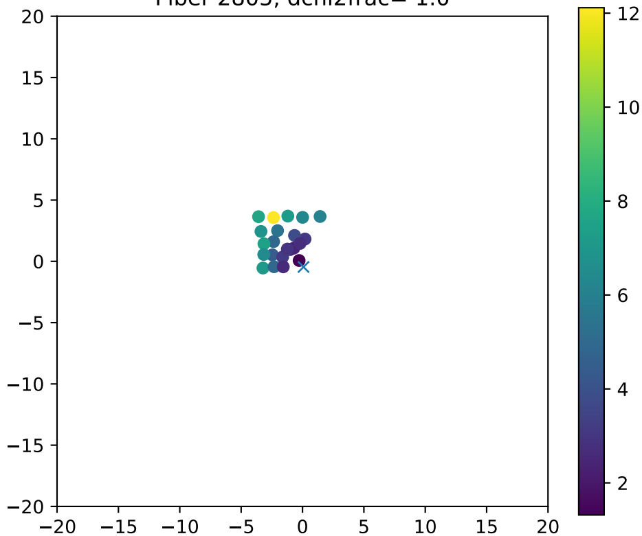
Fiber 2805, dchi2frac= 1.0
