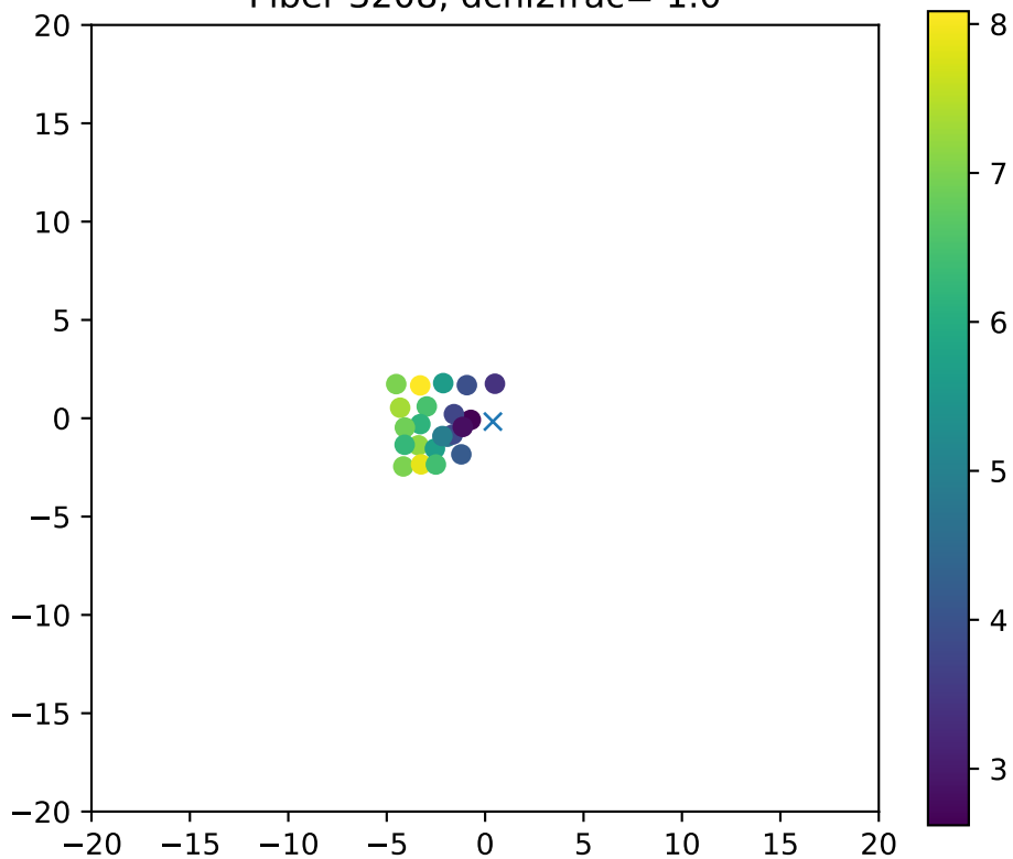
Fiber 3208, dchi2frac= 1.0
