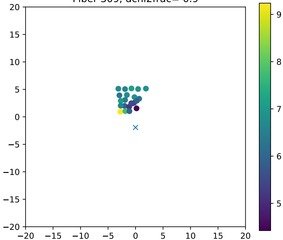
Fiber 309, dchi2frac= 0.9
