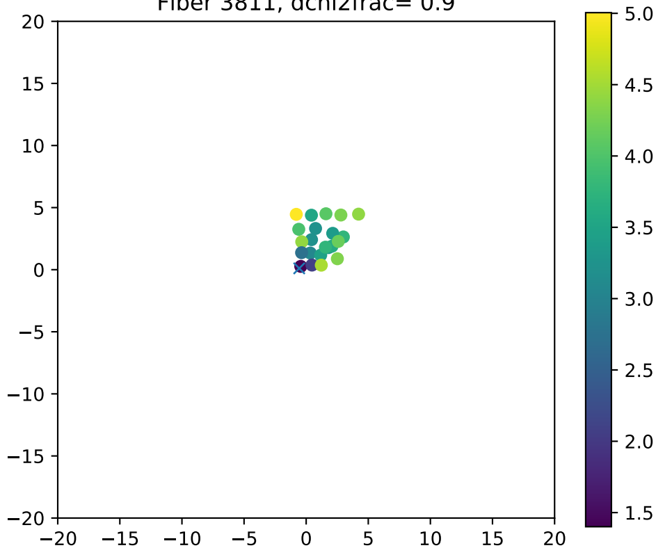
Fiber 3811, dchi2frac= 0.9
