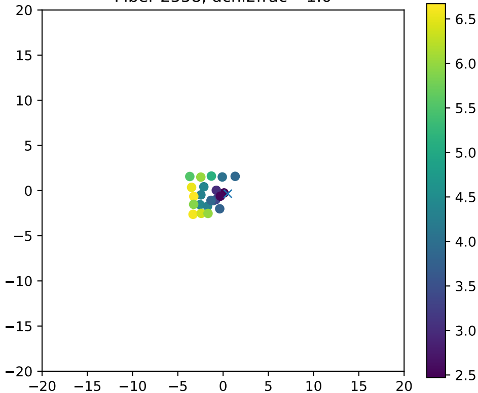
Fiber 2558, dchi2frac= 1.0
