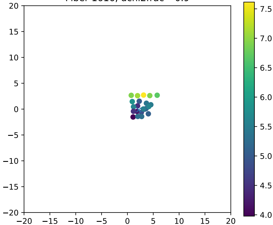
Fiber 1616, dchi2frac= 0.9
