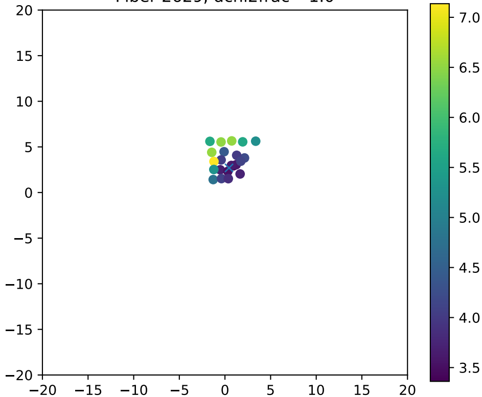
Fiber 2629, dchi2frac= 1.0
