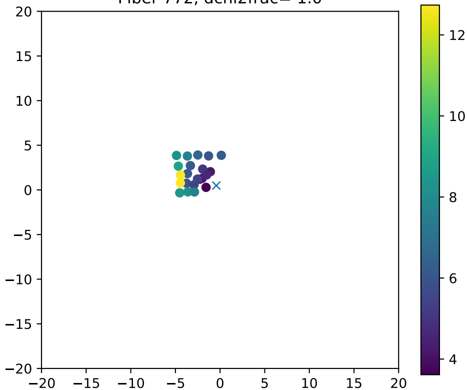
Fiber 772, dchi2frac= 1.0
