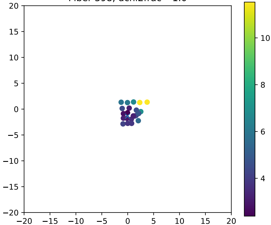
Fiber 398, dchi2frac= 1.0
