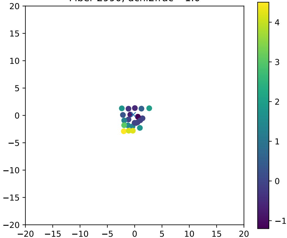
Fiber 2990, dchi2frac= 1.0
