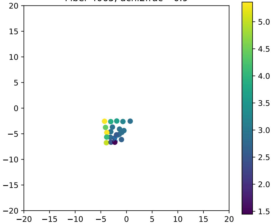
Fiber 4065, dchi2frac= 0.9
