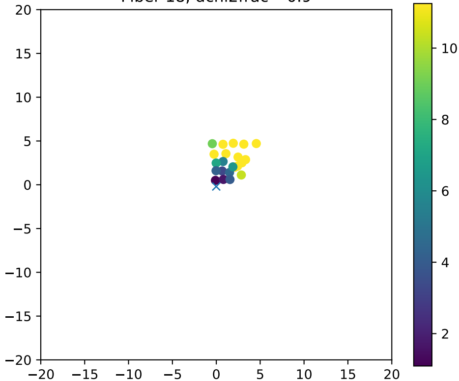
Fiber 18, dchi2frac= 0.9
