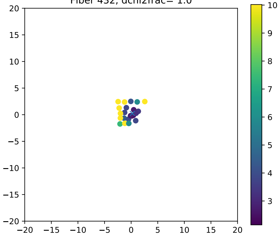
Fiber 432, dchi2frac= 1.0
