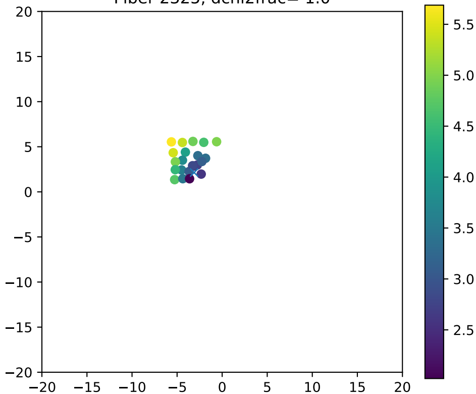
Fiber 2325, dchi2frac= 1.0
