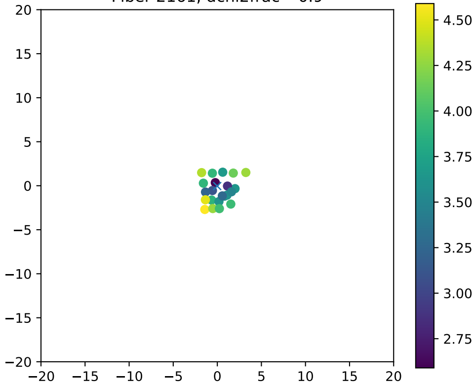
Fiber 2161, dchi2frac= 0.9
