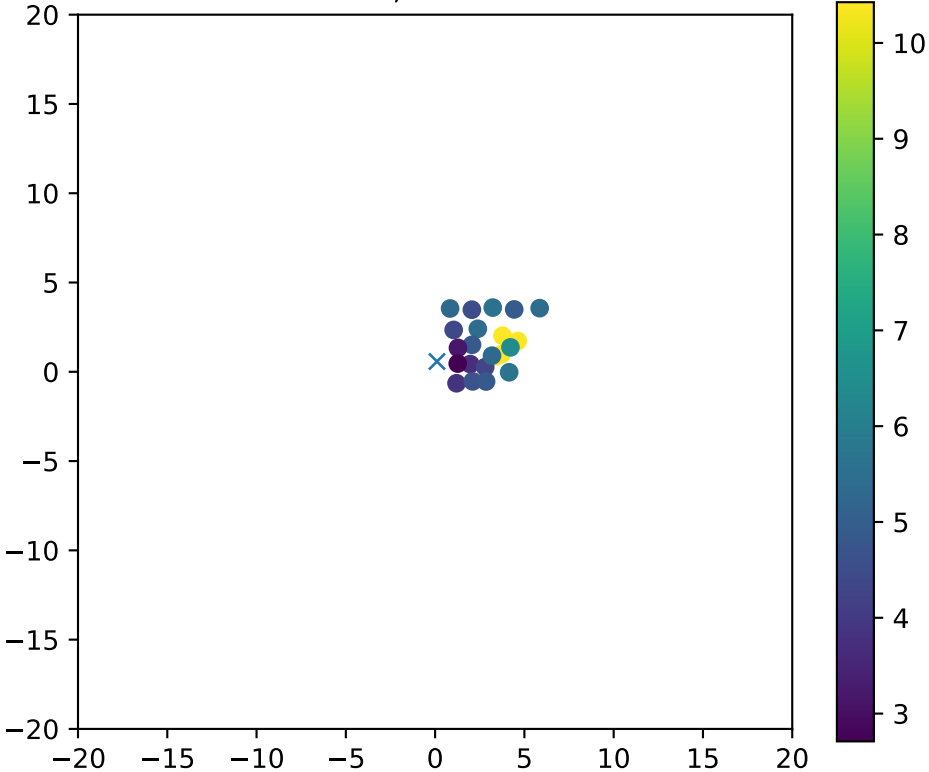
Fiber 4388, dchi2frac= 0.9
