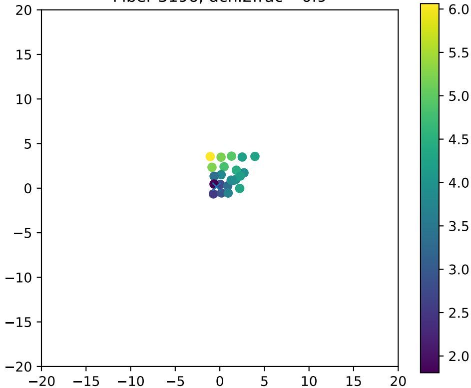
Fiber 3196, dchi2frac= 0.9
