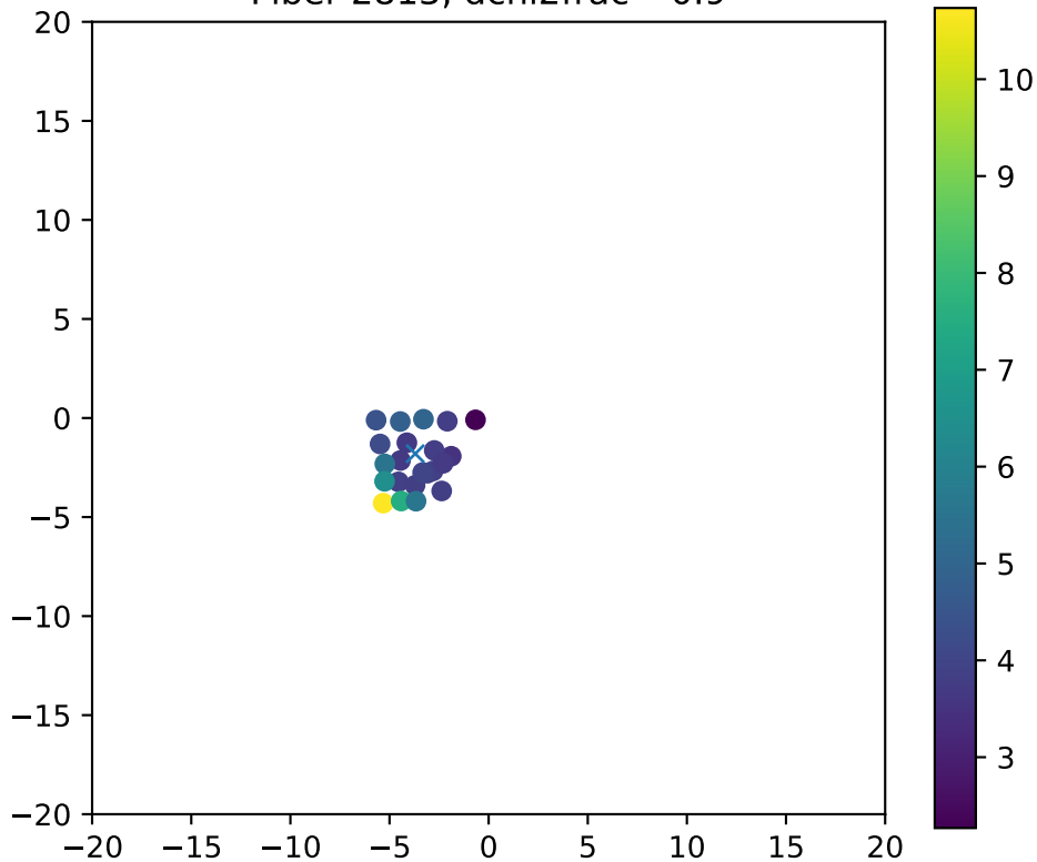
Fiber 2813, dchi2frac= 0.9
