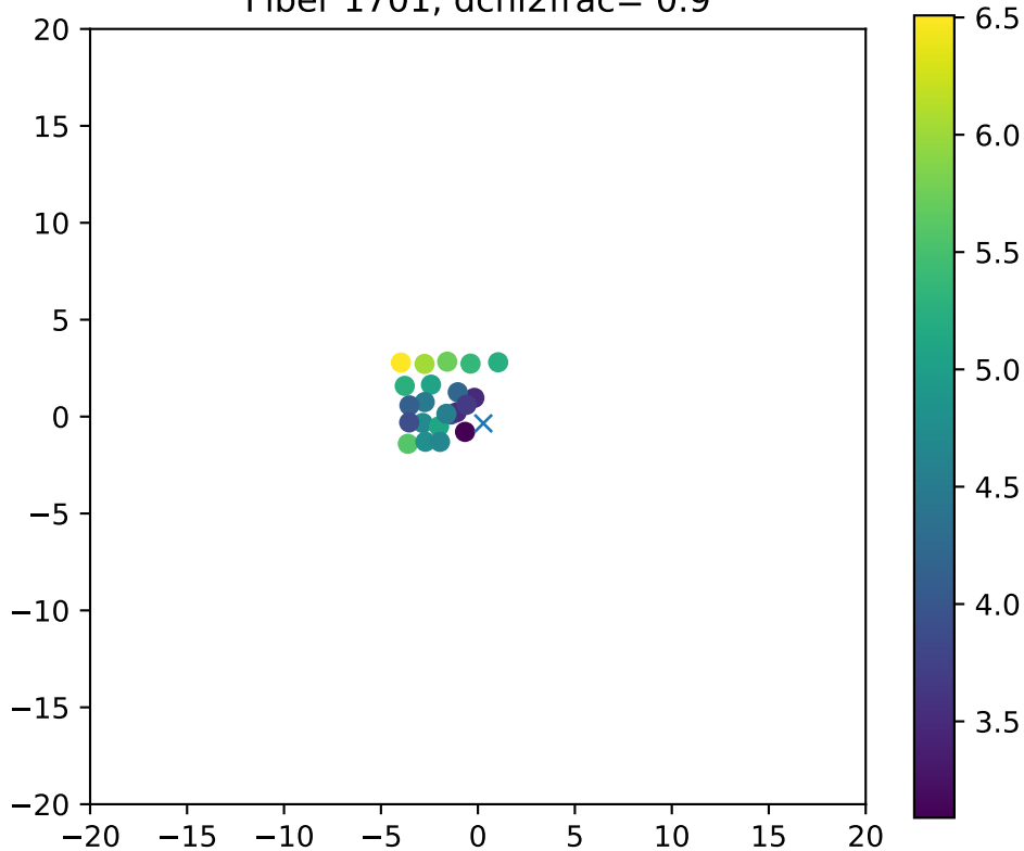
Fiber 1701, dchi2frac= 0.9
