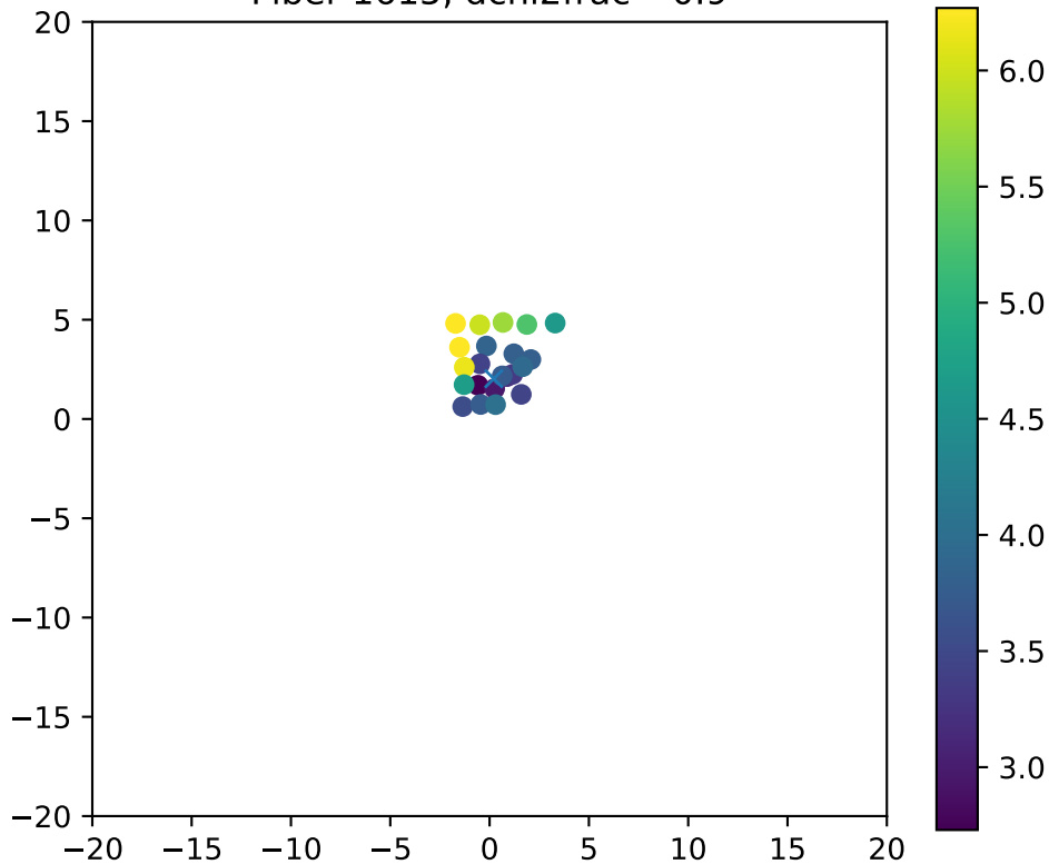
Fiber 1615, dchi2frac= 0.9
