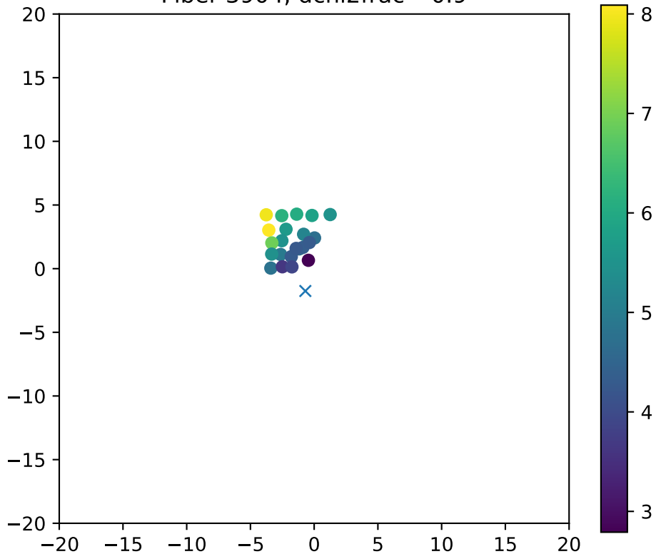
Fiber 3904, dchi2frac= 0.9
