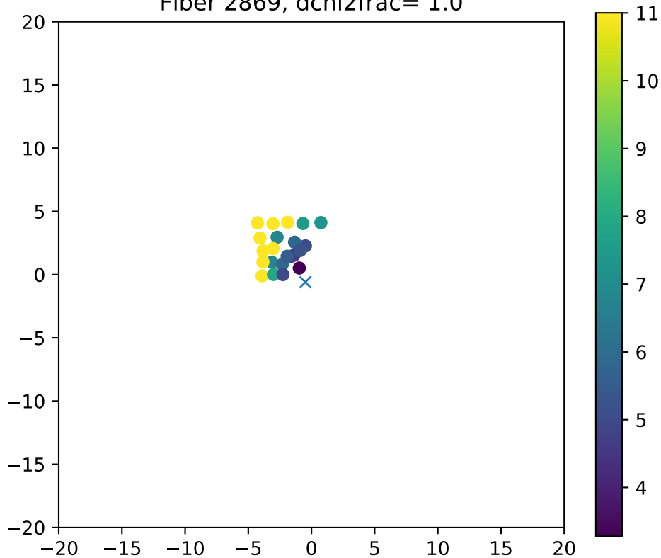
Fiber 2869, dchi2frac= 1.0
