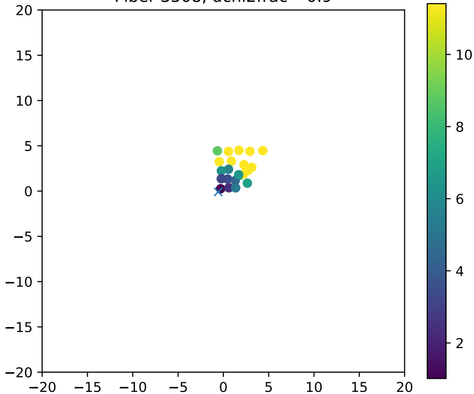
Fiber 3508, dchi2frac= 0.9
