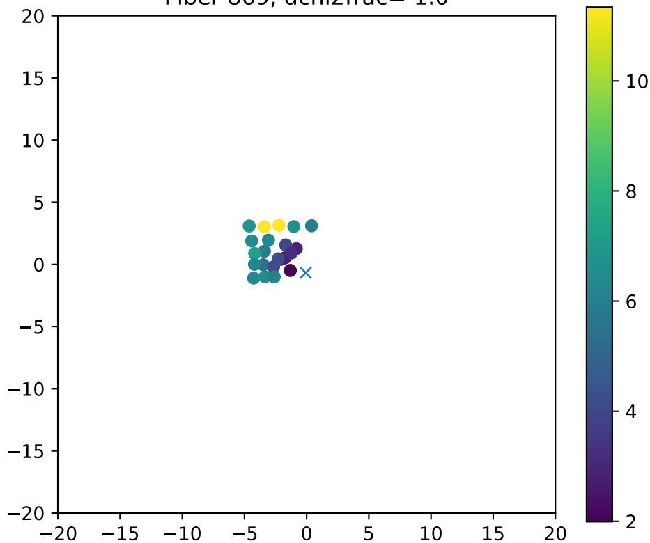
Fiber 869, dchi2frac= 1.0
