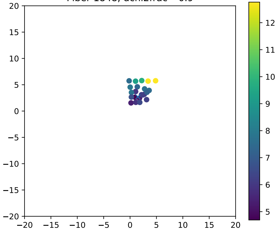
Fiber 1848, dchi2frac= 0.9
