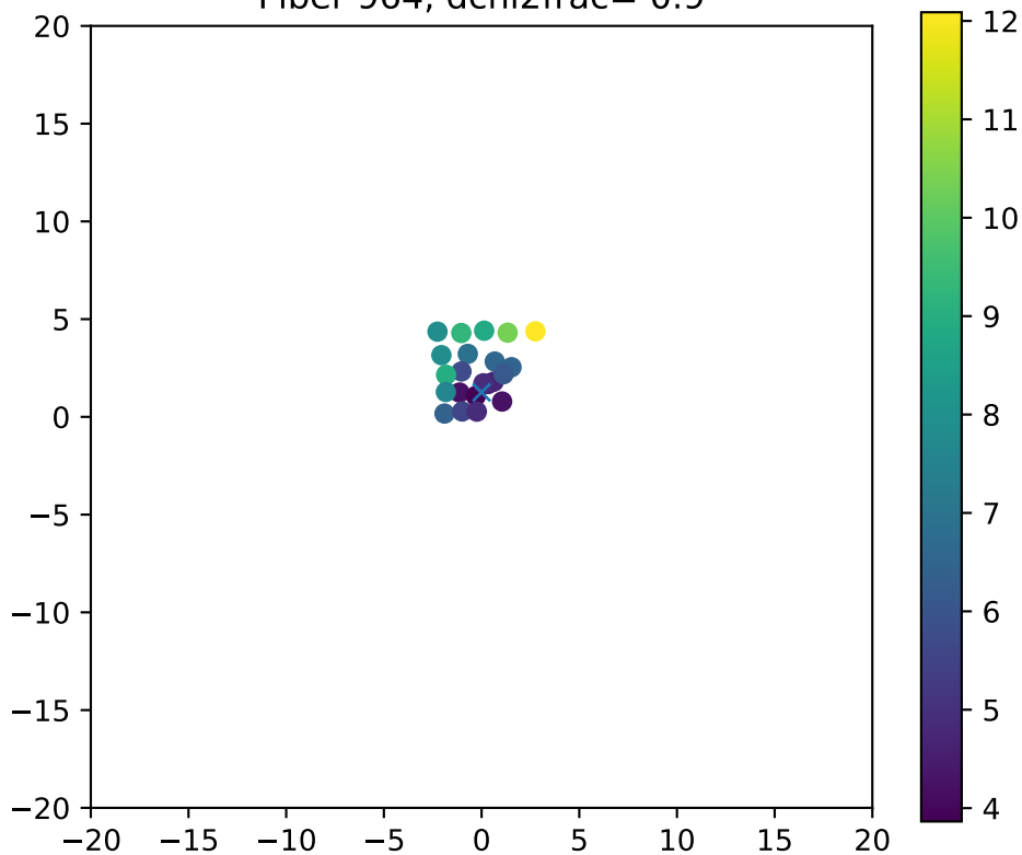
Fiber 964, dchi2frac= 0.9
