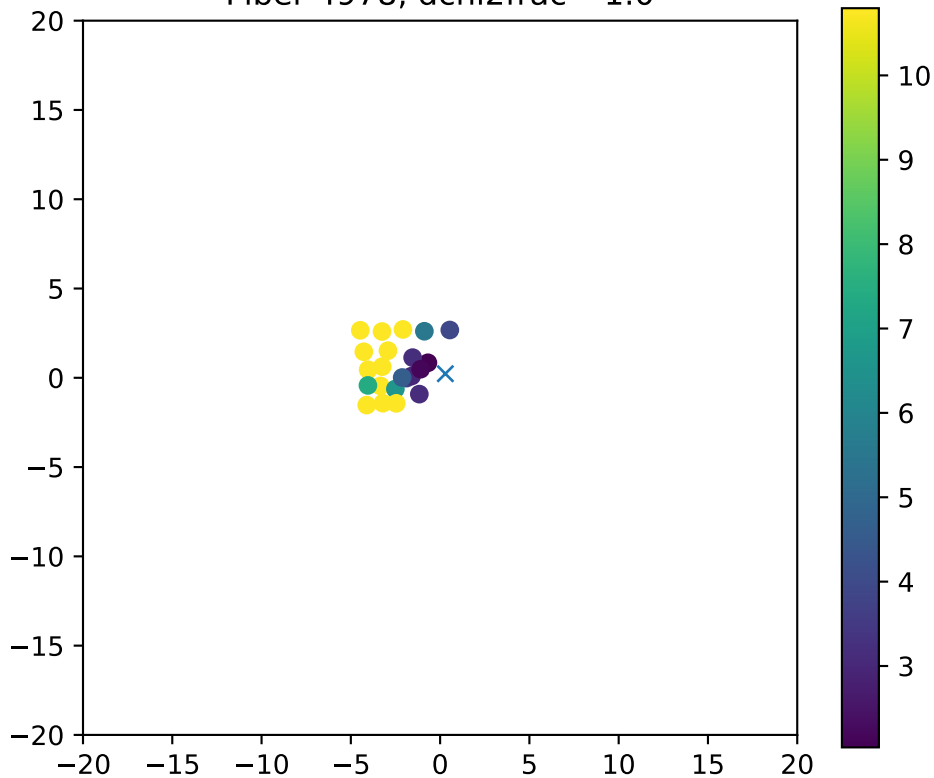
Fiber 4978, dchi2frac= 1.0
