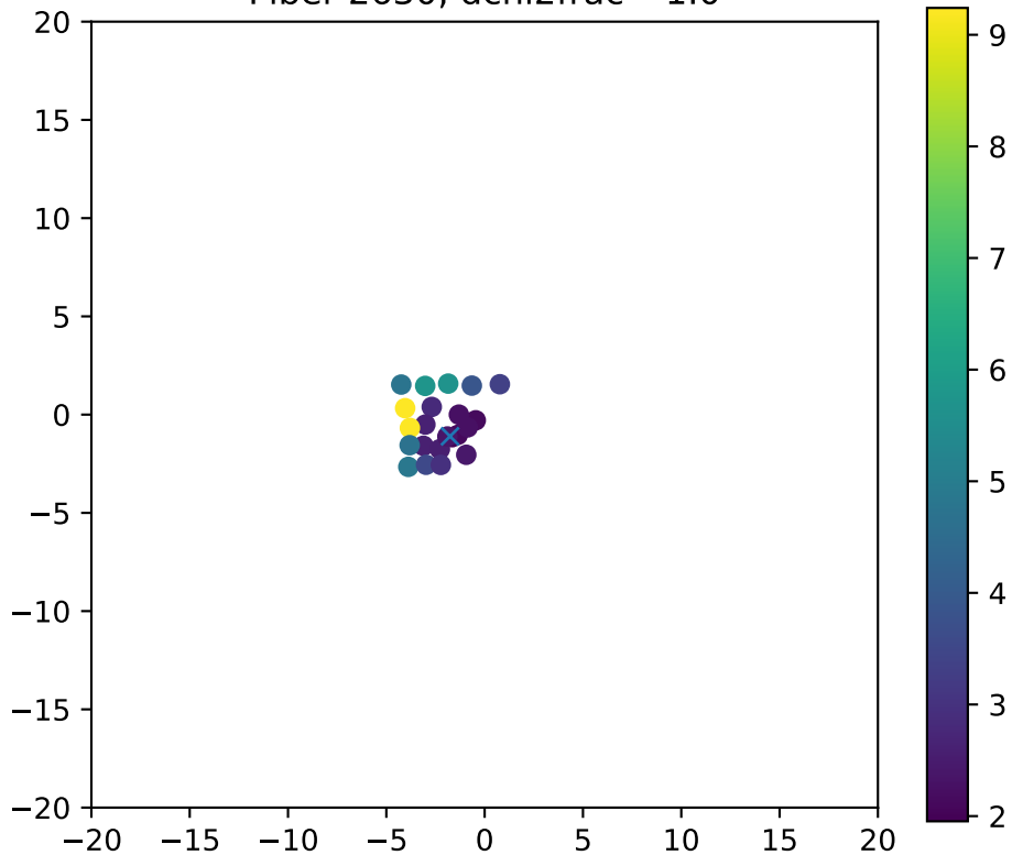
Fiber 2630, dchi2frac= 1.0
