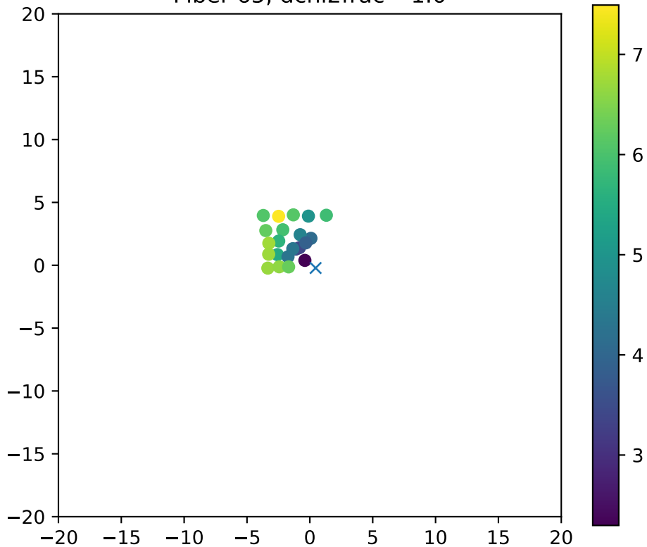
Fiber 65, dchi2frac= 1.0
