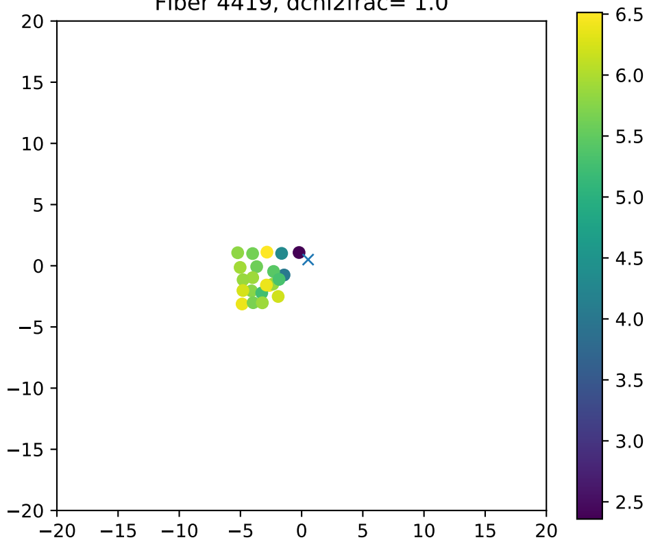
Fiber 4419, dchi2frac= 1.0
