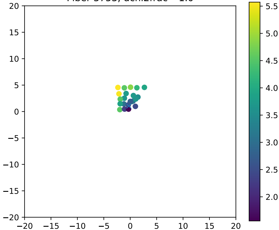
Fiber 3753, dchi2frac= 1.0
