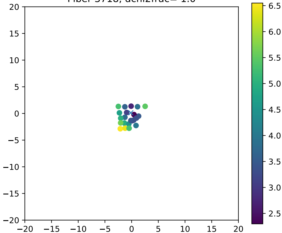
Fiber 3718, dchi2frac= 1.0
