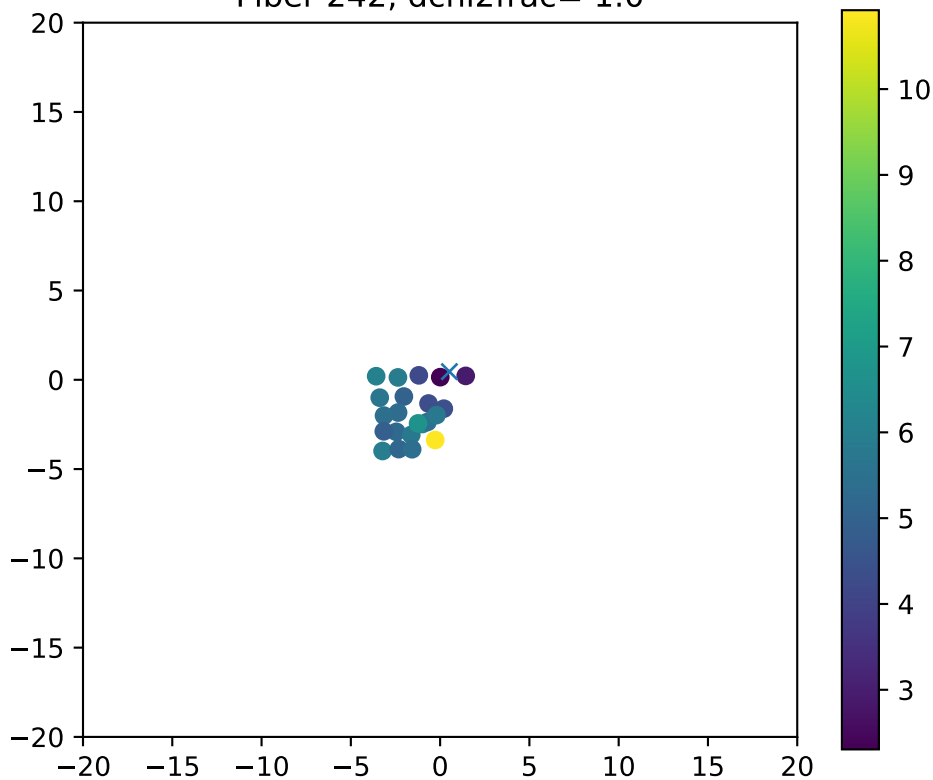
Fiber 242, dchi2frac= 1.0
