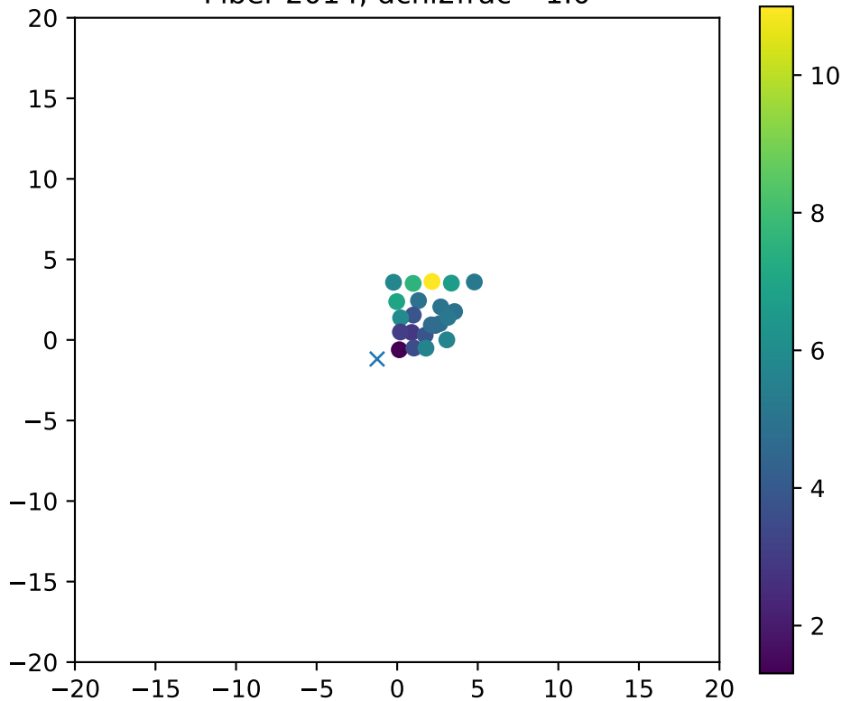
Fiber 2014, dchi2frac= 1.0
