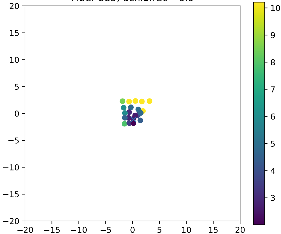
Fiber 885, dchi2frac= 0.9
