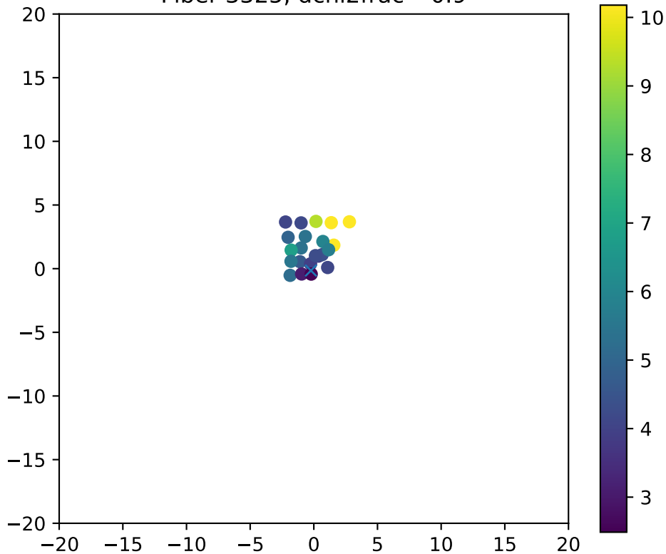
Fiber 3325, dchi2frac= 0.9
