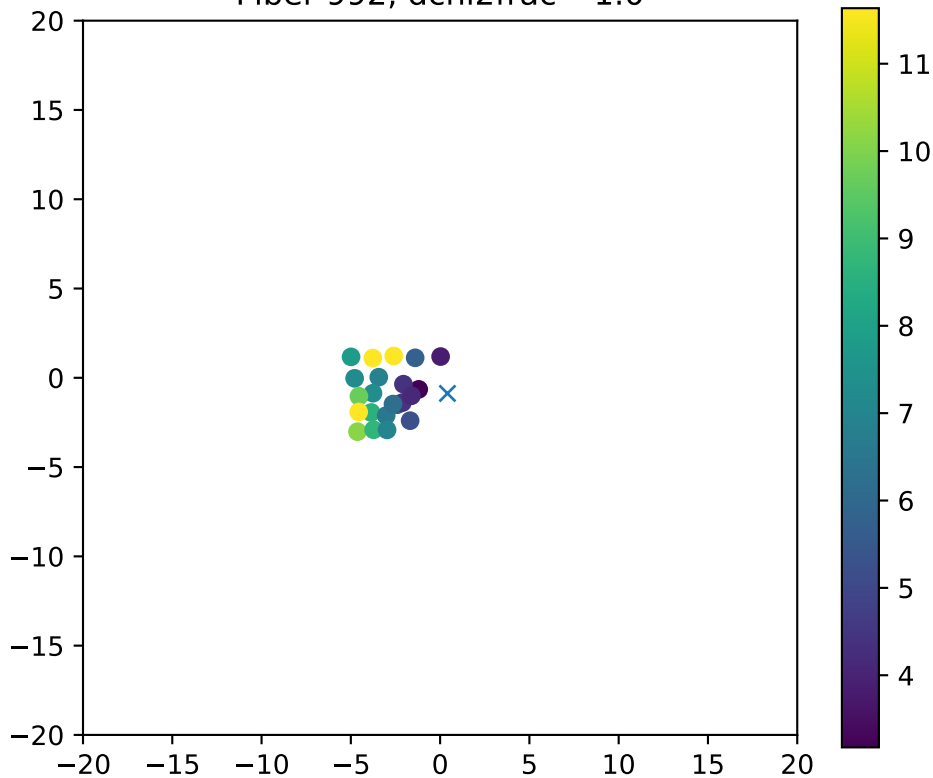
Fiber 992, dchi2frac= 1.0
