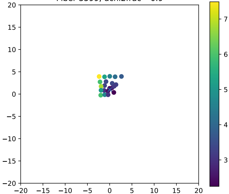
Fiber 3599, dchi2frac= 0.9
