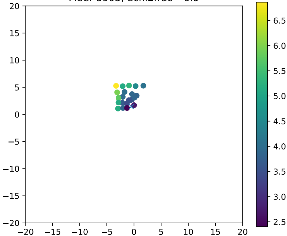
Fiber 3905, dchi2frac= 0.9
