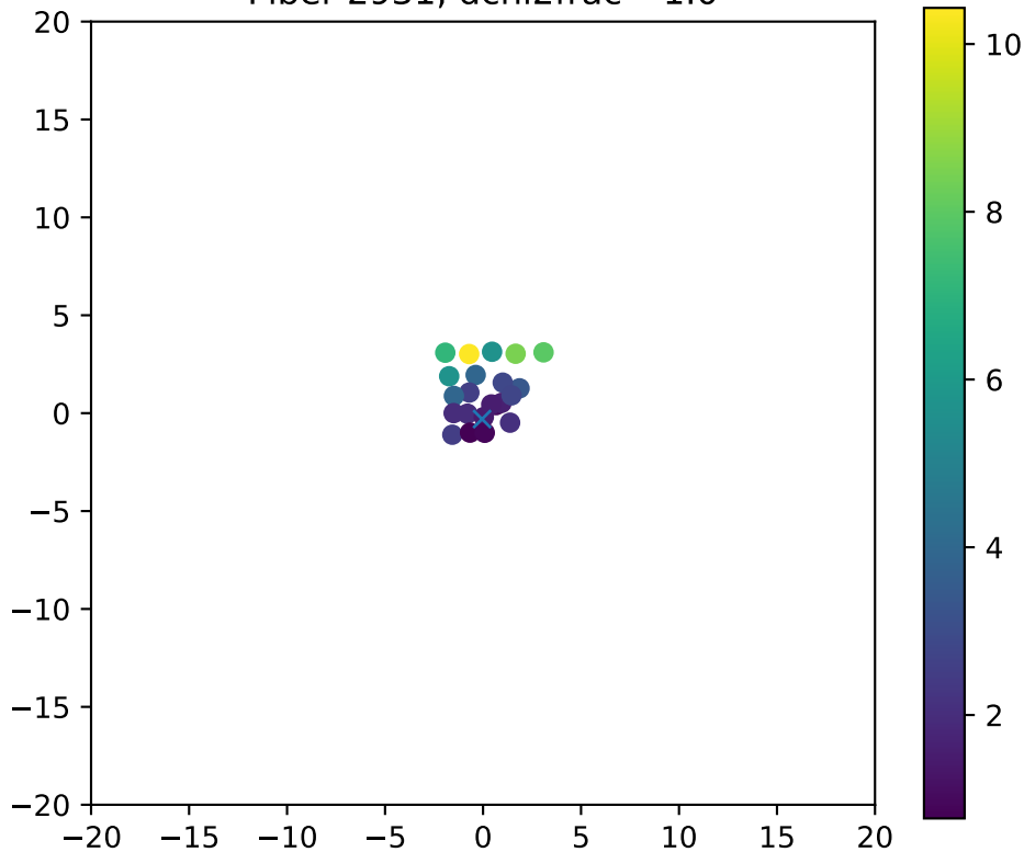
Fiber 2931, dchi2frac= 1.0
