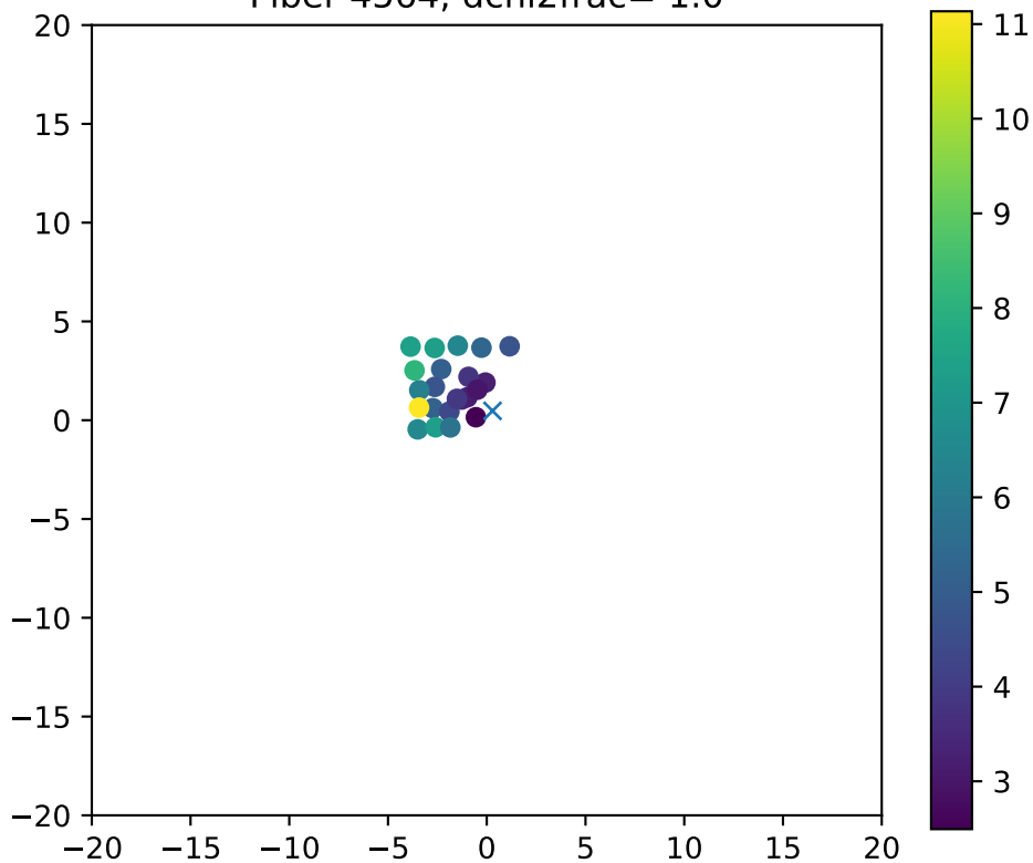
Fiber 4564, dchi2frac= 1.0
