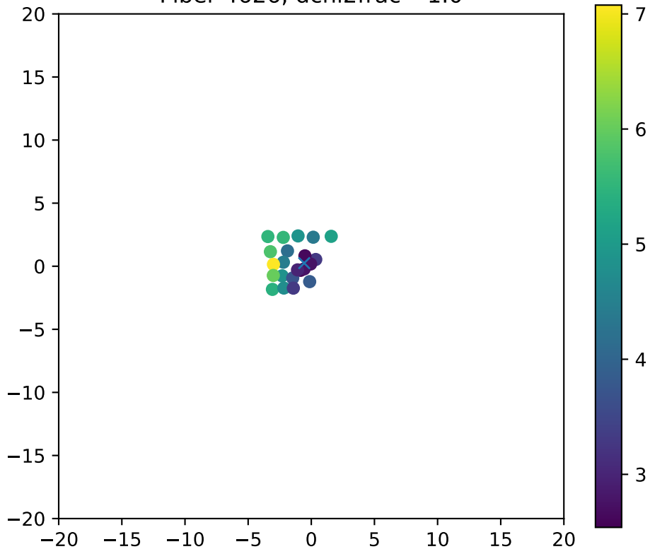
Fiber 4626, dchi2frac= 1.0
