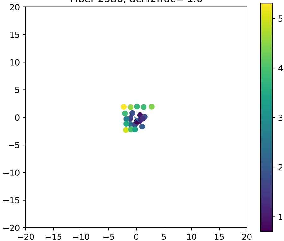
Fiber 2986, dchi2frac= 1.0
