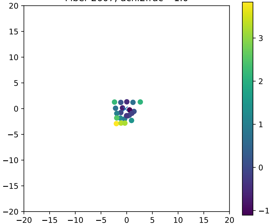
Fiber 2607, dchi2frac= 1.0
