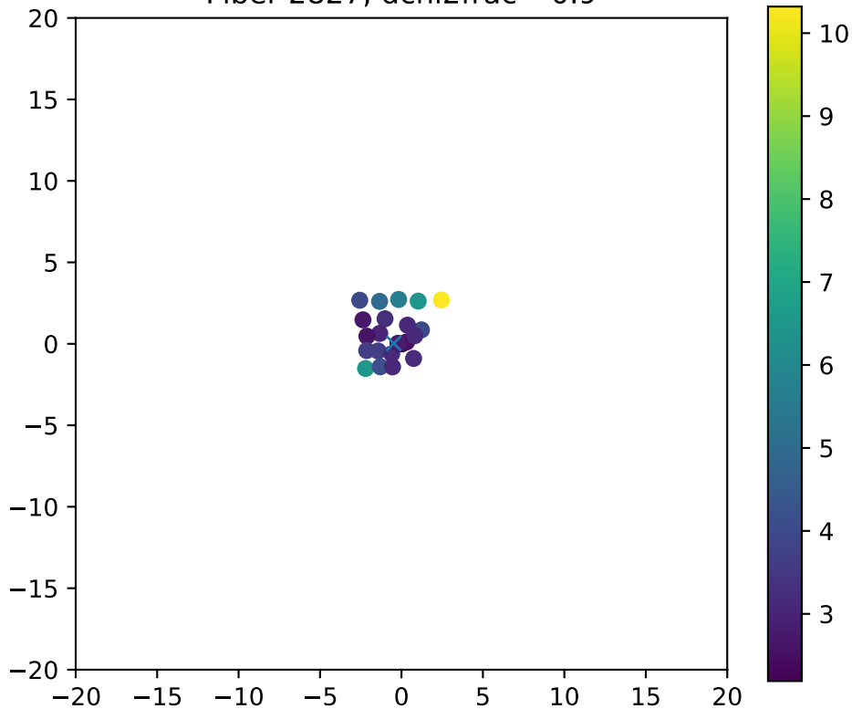
Fiber 2827, dchi2frac= 0.9
