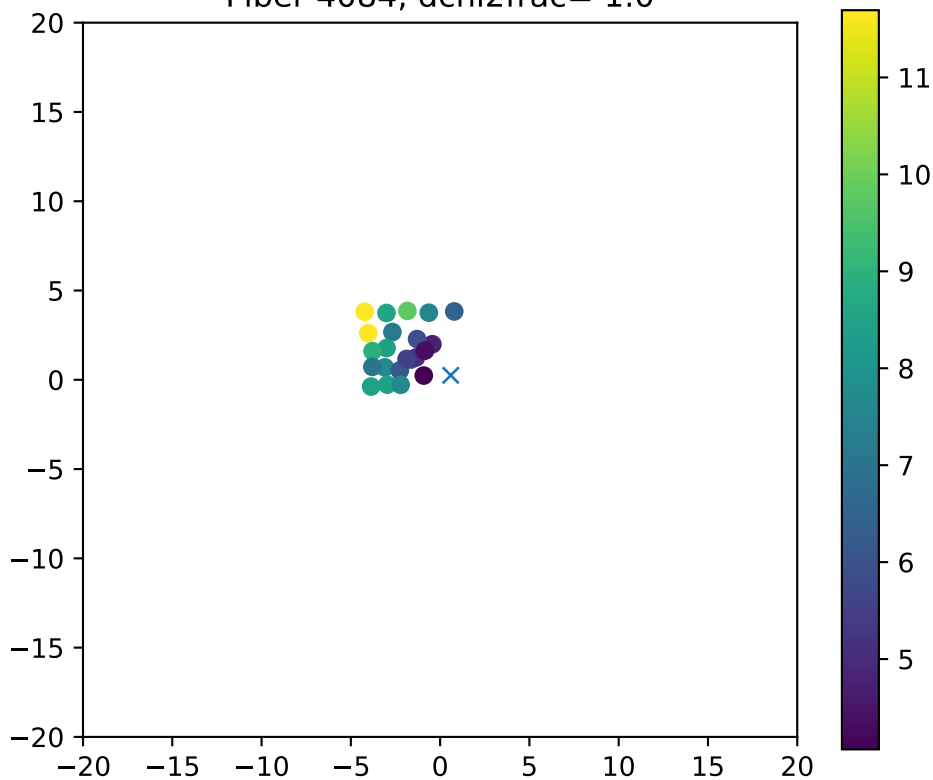
Fiber 4084, dchi2frac= 1.0
