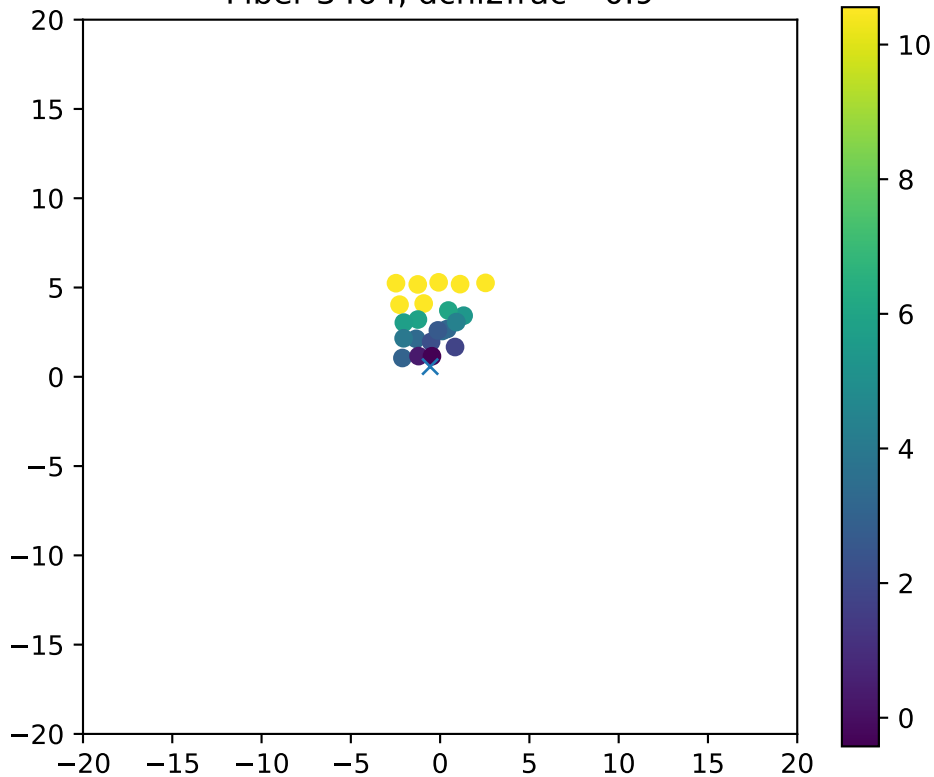
Fiber 3464, dchi2frac= 0.9
