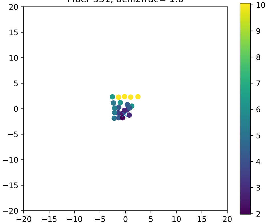
Fiber 551, dchi2frac= 1.0
