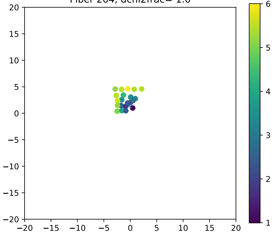
Fiber 204, dchi2frac= 1.0
