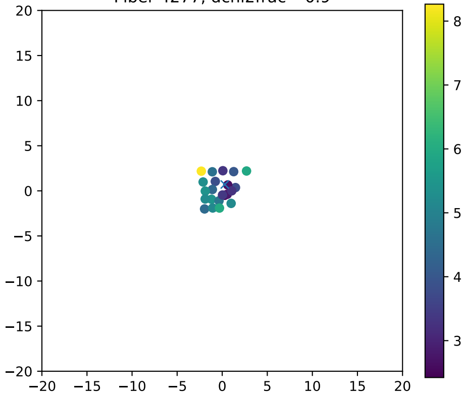
Fiber 4277, dchi2frac= 0.9
