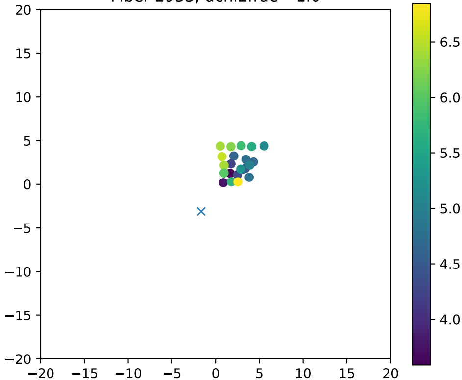
Fiber 2933, dchi2frac= 1.0
