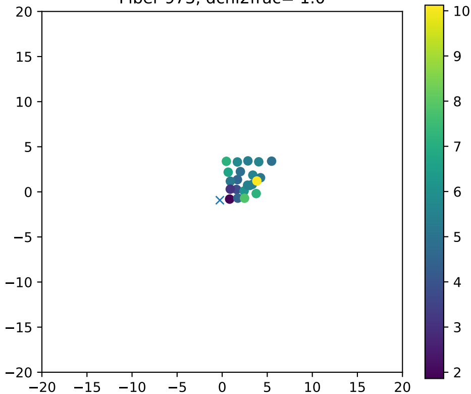
Fiber 973, dchi2frac= 1.0
