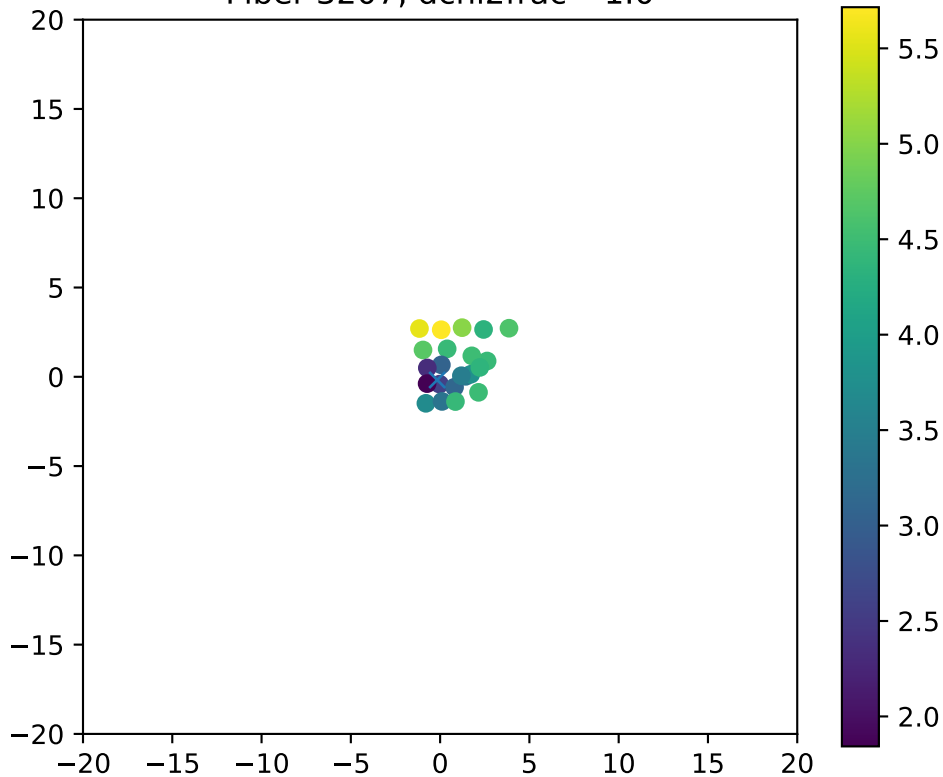
Fiber 3207, dchi2frac= 1.0
