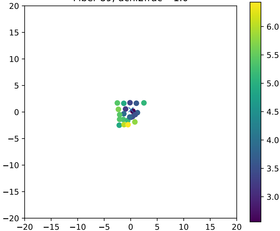
Fiber 89, dchi2frac= 1.0
