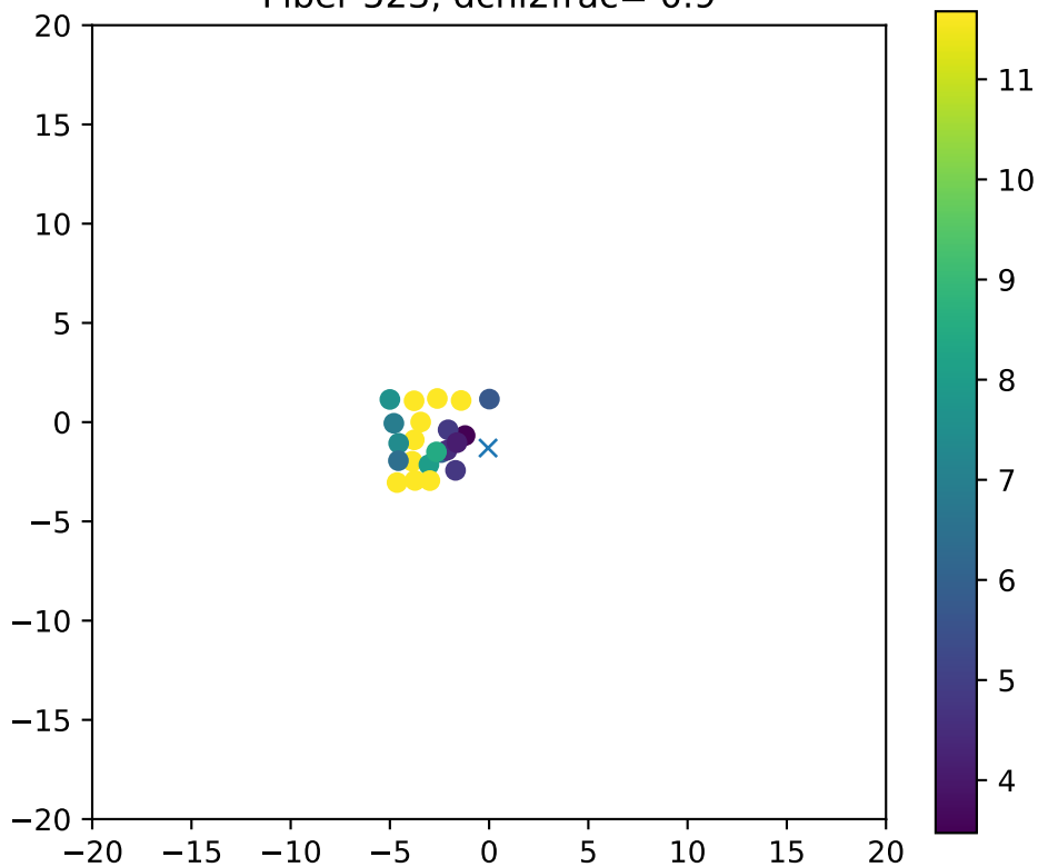
Fiber 523, dchi2frac= 0.9
