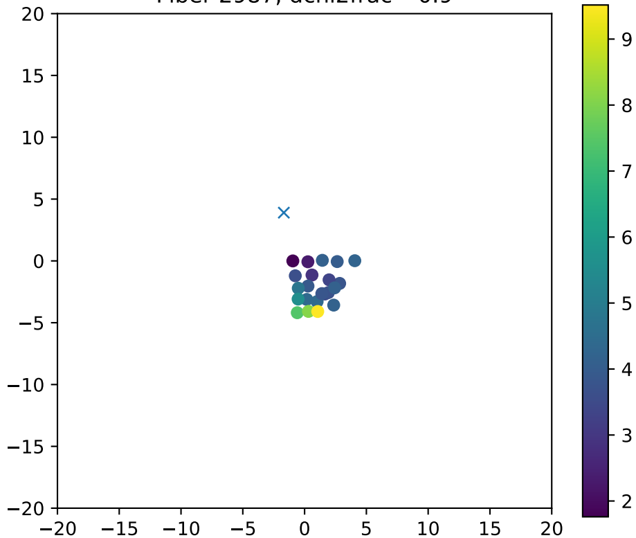
Fiber 2987, dchi2frac= 0.9
