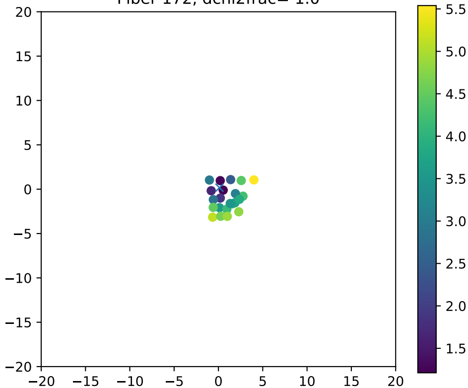
Fiber 172, dchi2frac= 1.0
