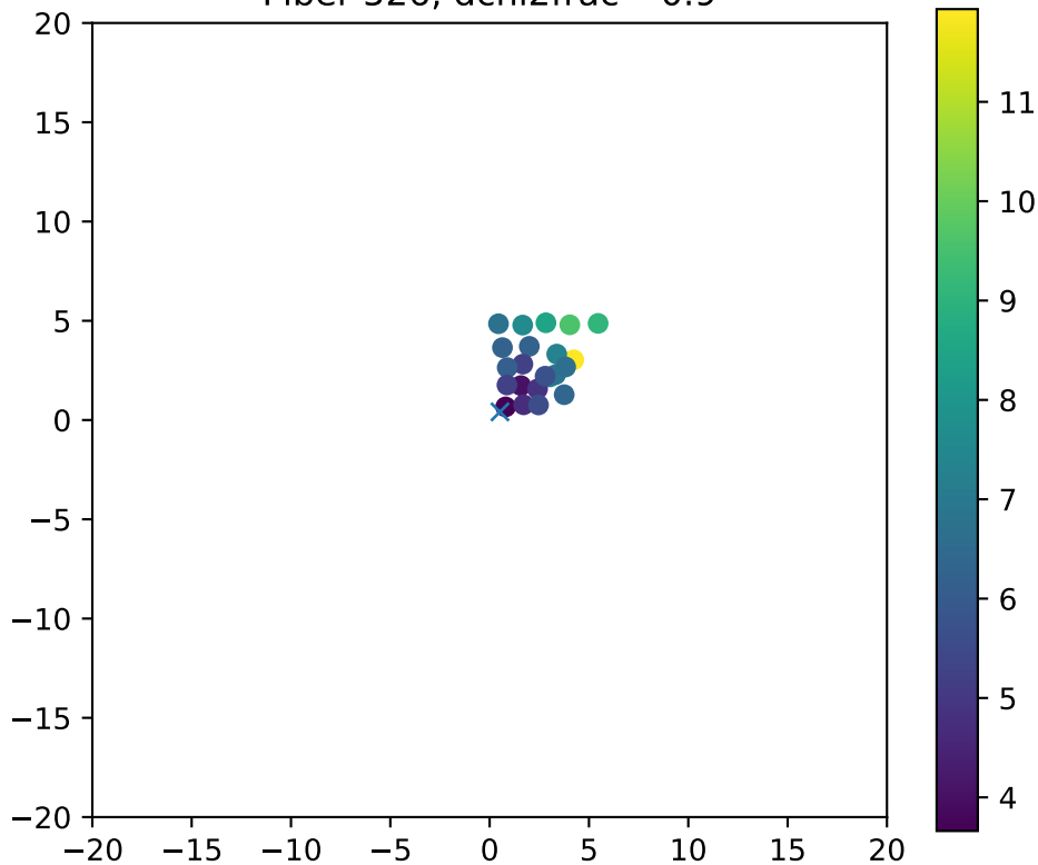
Fiber 526, dchi2frac= 0.9
