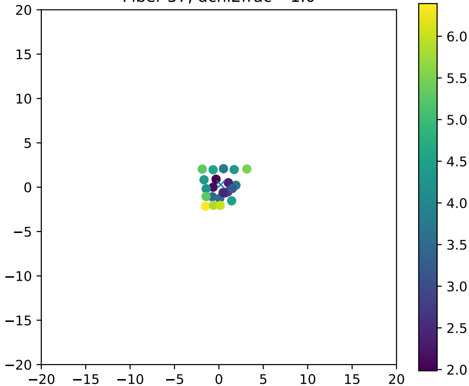
Fiber 57, dchi2frac= 1.0
