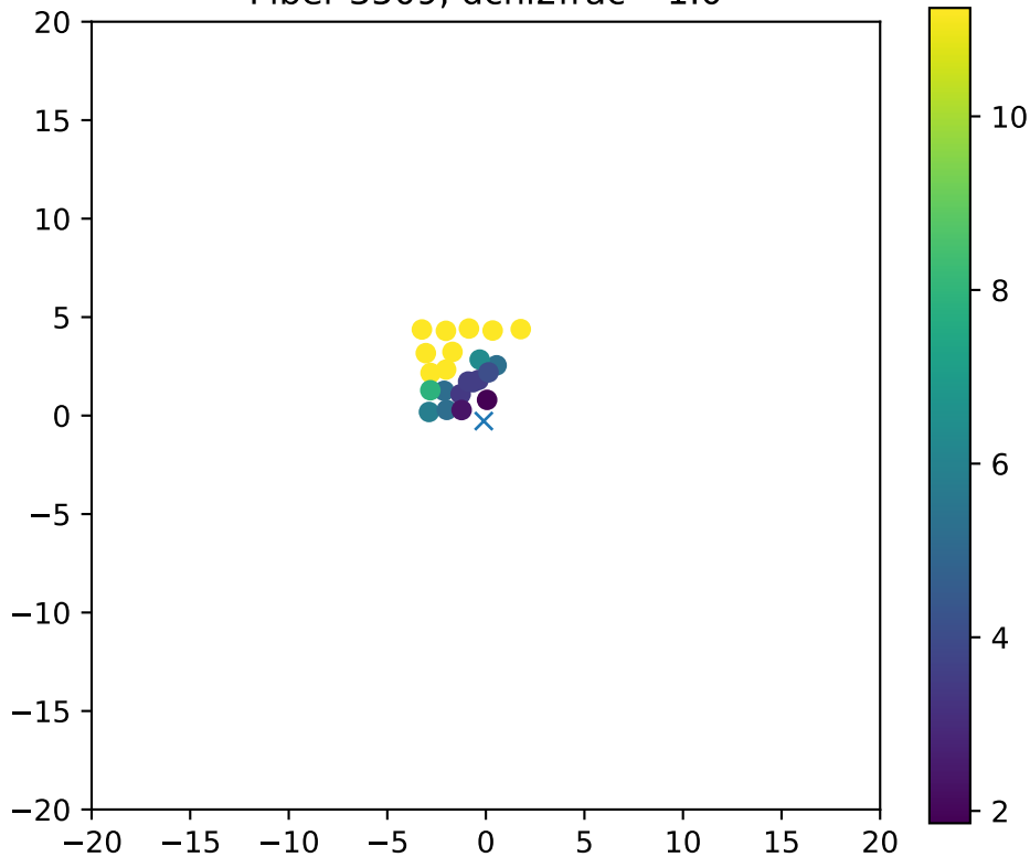
Fiber 3509, dchi2frac= 1.0
