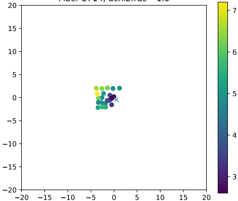
Fiber 2714, dchi2frac= 1.0
