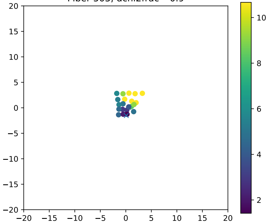
Fiber 503, dchi2frac= 0.9
