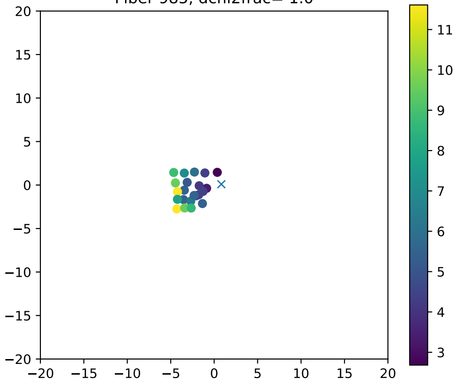
Fiber 985, dchi2frac= 1.0
