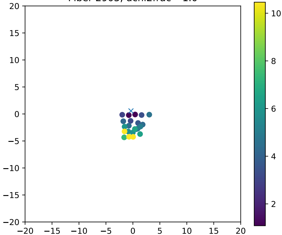
Fiber 2903, dchi2frac= 1.0
