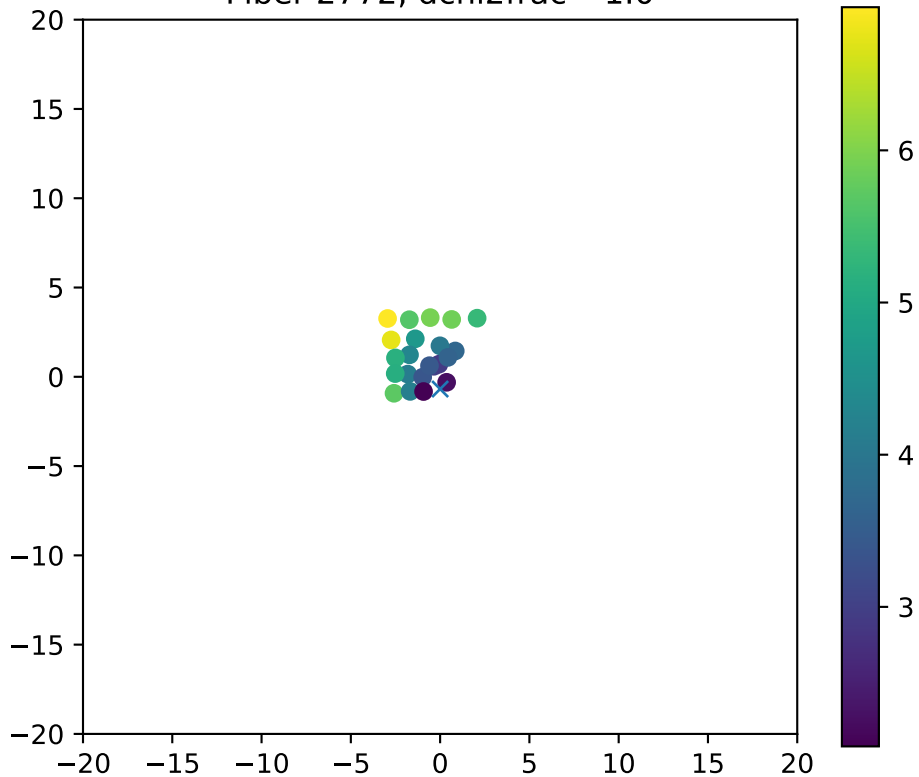
Fiber 2772, dchi2frac= 1.0
