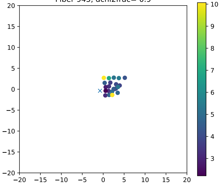
Fiber 945, dchi2frac= 0.9
