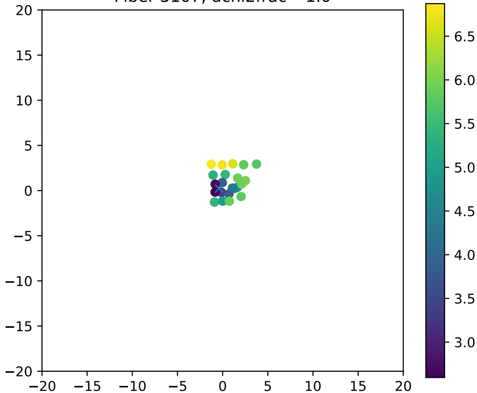
Fiber 3107, dchi2frac= 1.0
