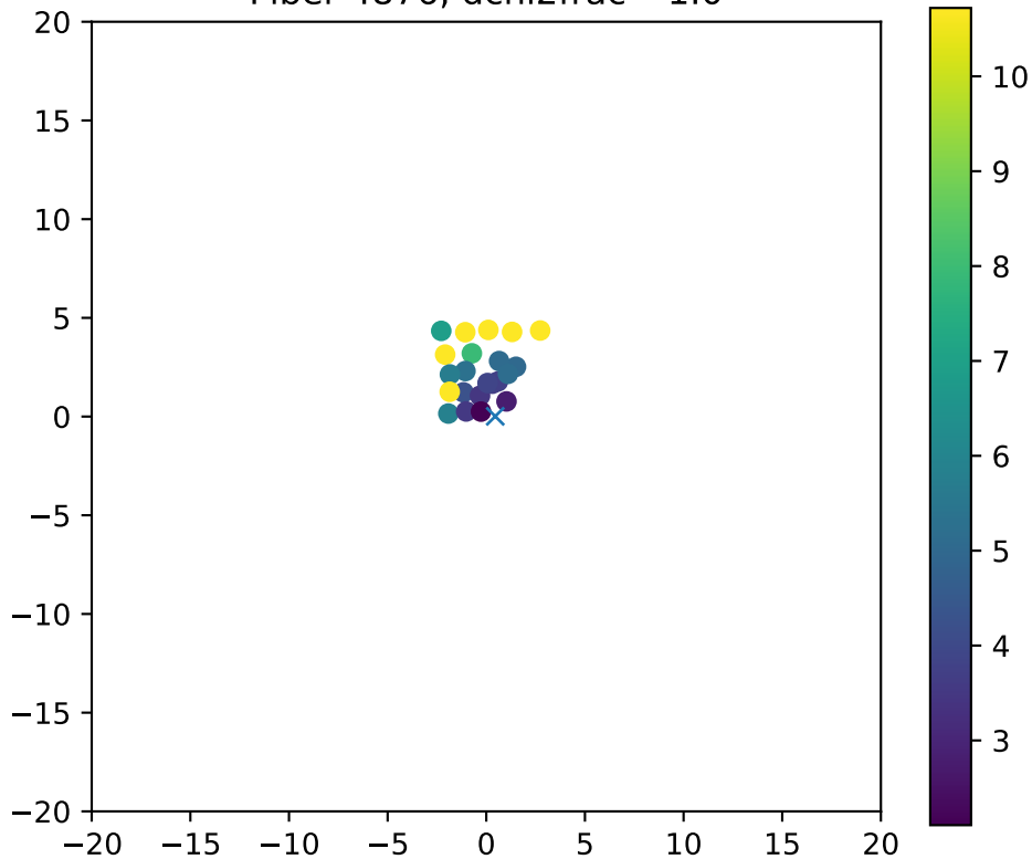
Fiber 4876, dchi2frac= 1.0
