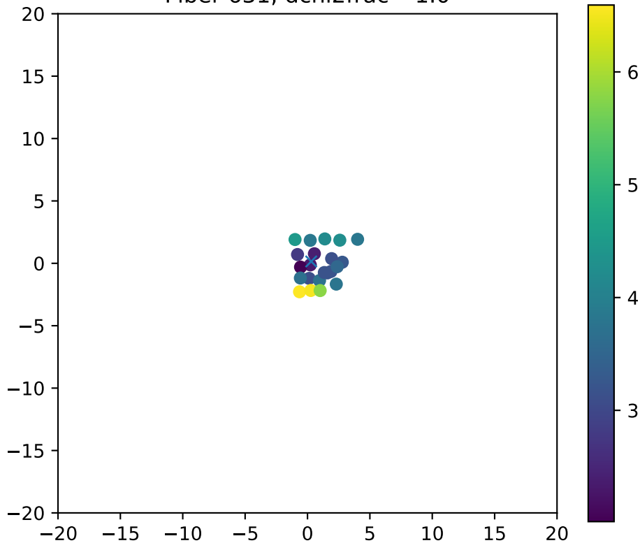
Fiber 631, dchi2frac= 1.0
