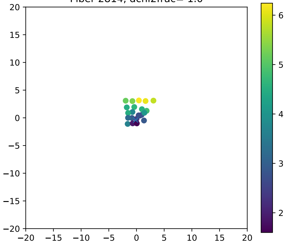
Fiber 2814, dchi2frac= 1.0
