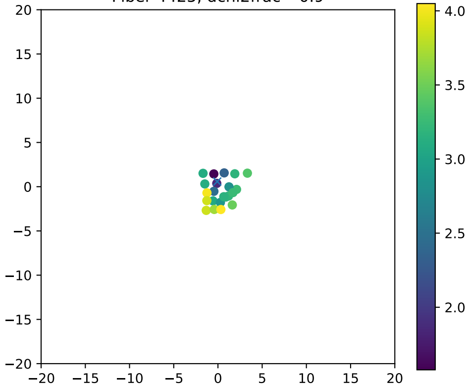
Fiber 4425, dchi2frac= 0.9
