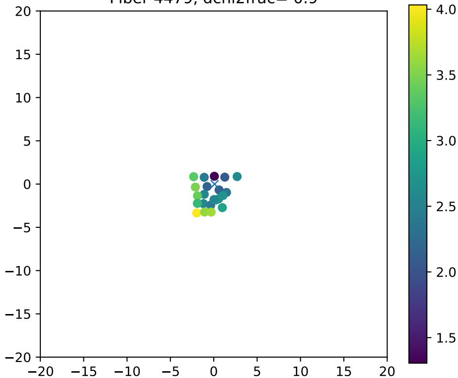
Fiber 4479, dchi2frac= 0.9
