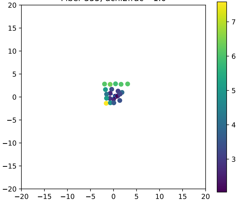
Fiber 355, dchi2frac= 1.0
