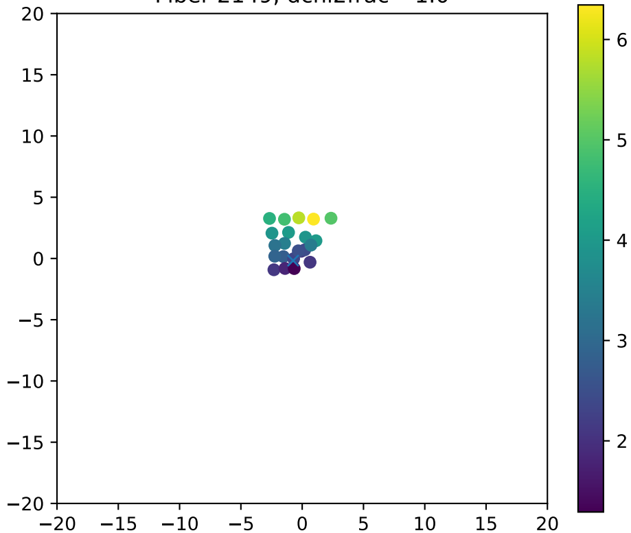
Fiber 2149, dchi2frac= 1.0
