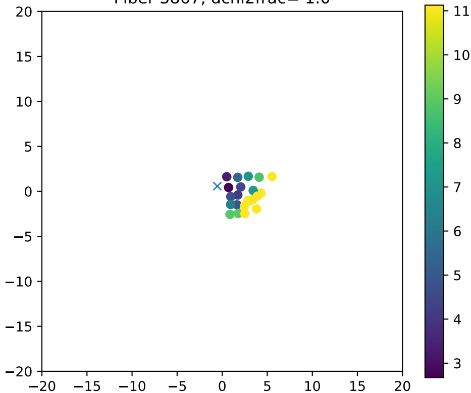
Fiber 3867, dchi2frac= 1.0
