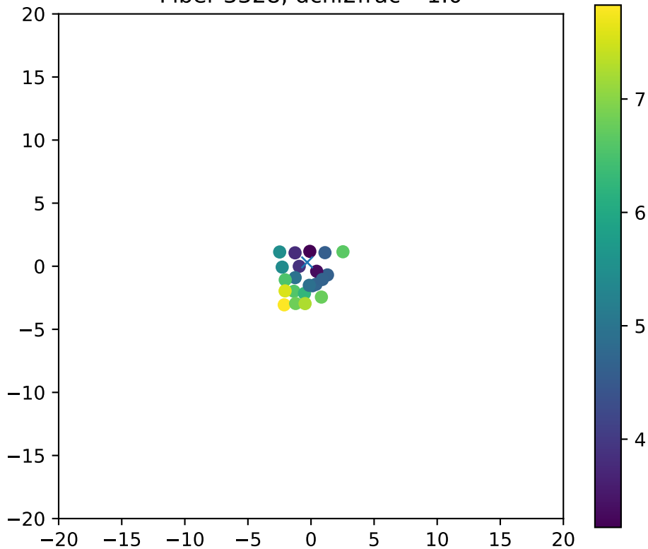
Fiber 3328, dchi2frac= 1.0
