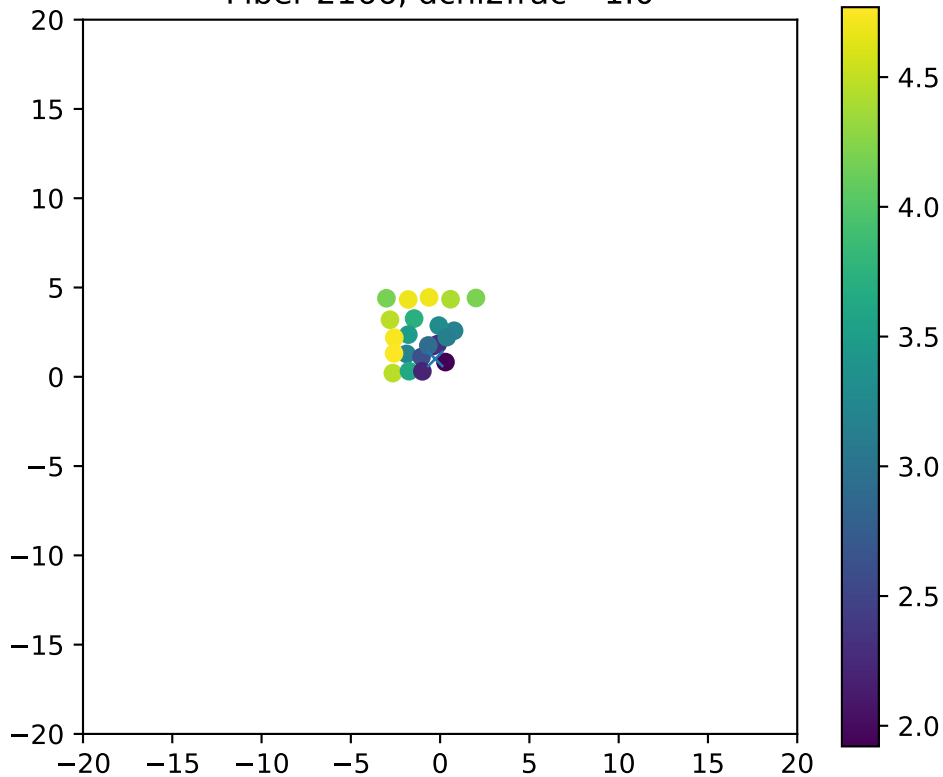
Fiber 2166, dchi2frac= 1.0
