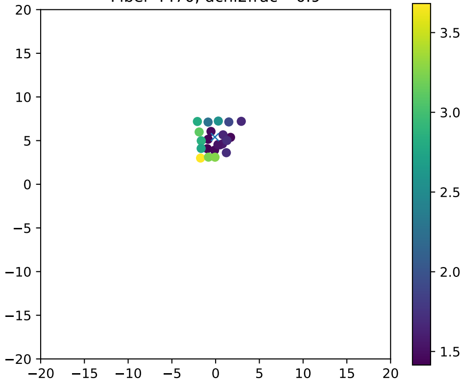
Fiber 4470, dchi2frac= 0.9
