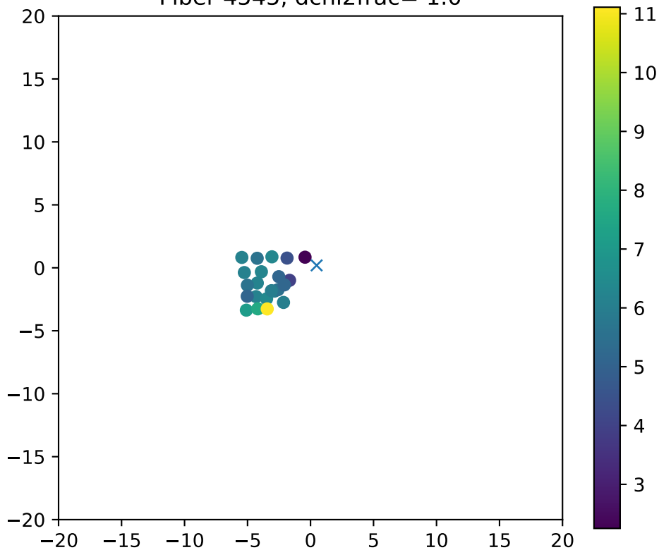
Fiber 4545, dchi2frac= 1.0
