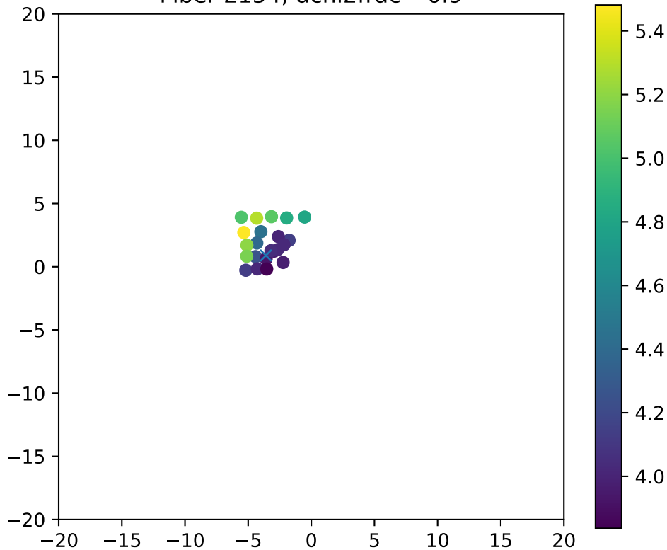
Fiber 2154, dchi2frac= 0.9
