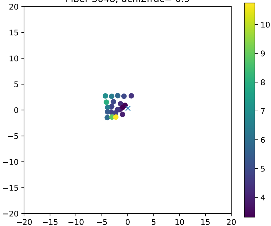
Fiber 3048, dchi2frac= 0.9
