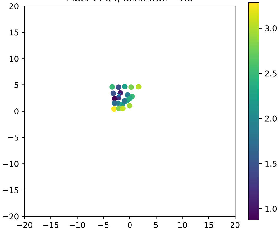
Fiber 2264, dchi2frac= 1.0
