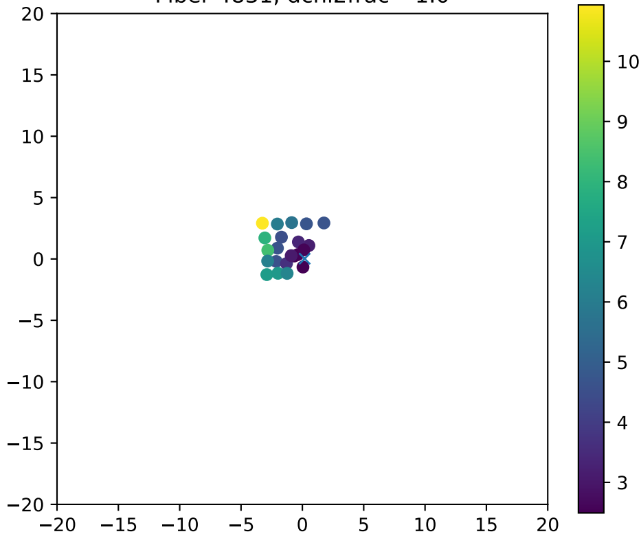
Fiber 4831, dchi2frac= 1.0
