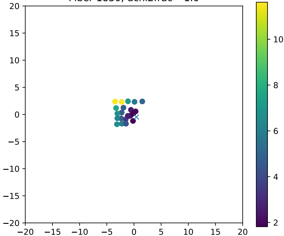
Fiber 1830, dchi2frac= 1.0
