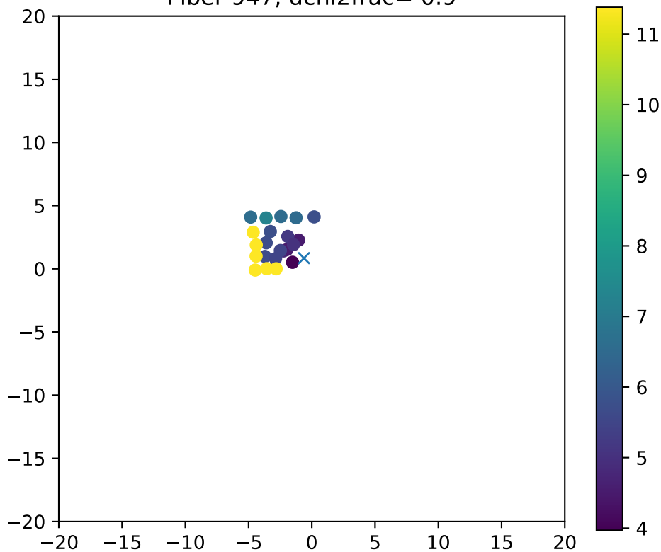
Fiber 947, dchi2frac= 0.9
