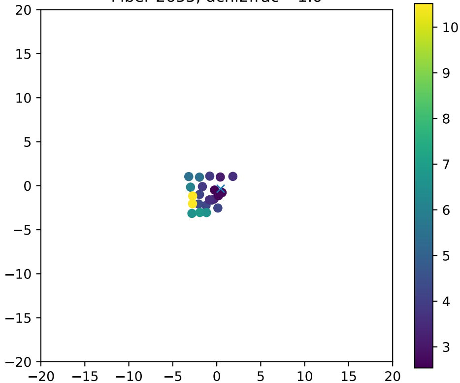
Fiber 2655, dchi2frac= 1.0
