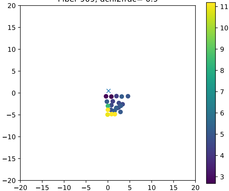
Fiber 909, dchi2frac= 0.9
