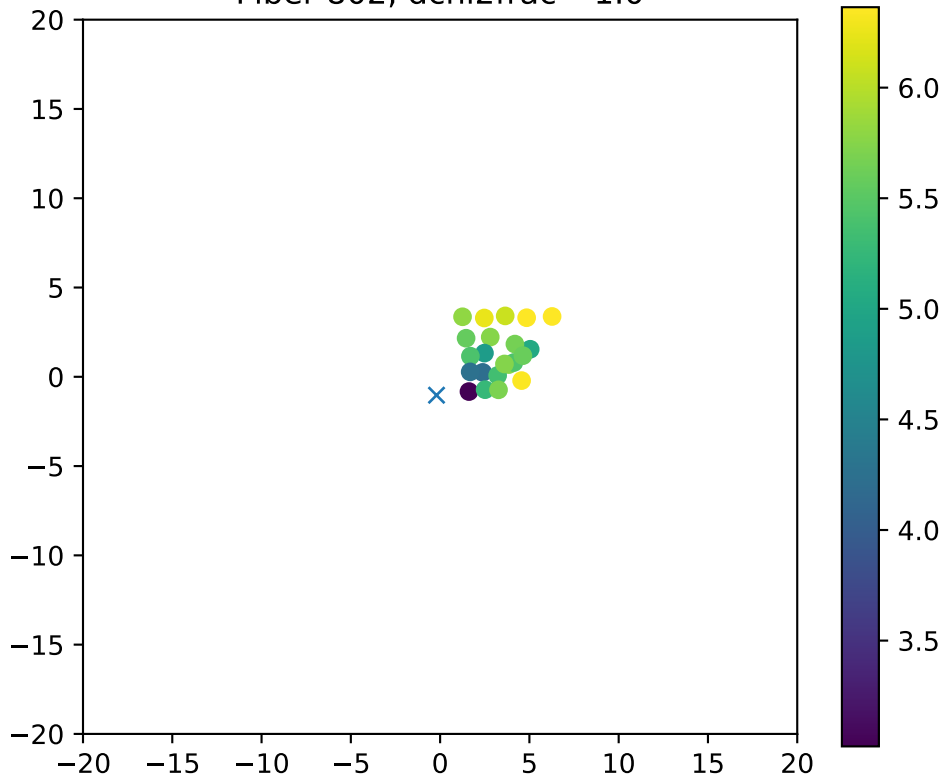
Fiber 802, dchi2frac= 1.0
