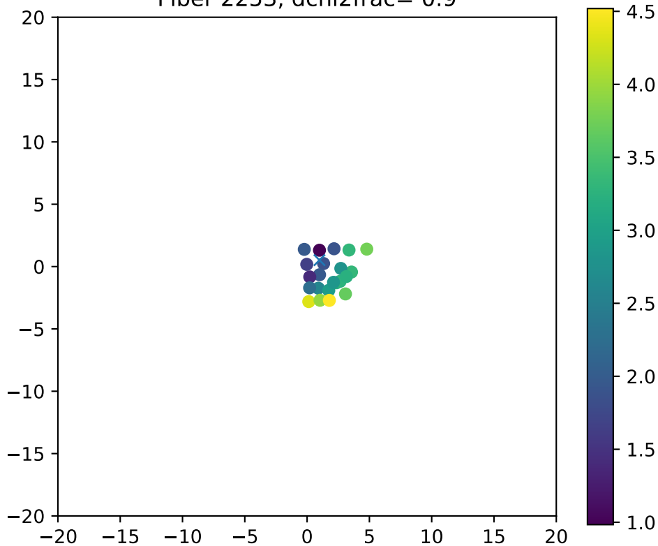
Fiber 2253, dchi2frac= 0.9
