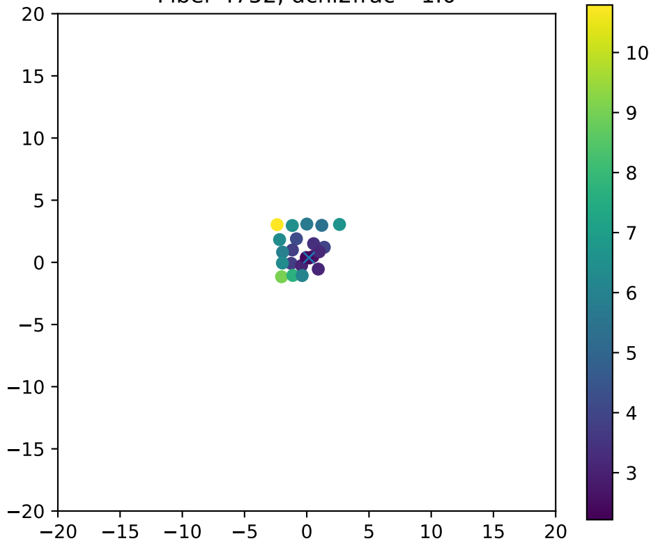
Fiber 4752, dchi2frac= 1.0
