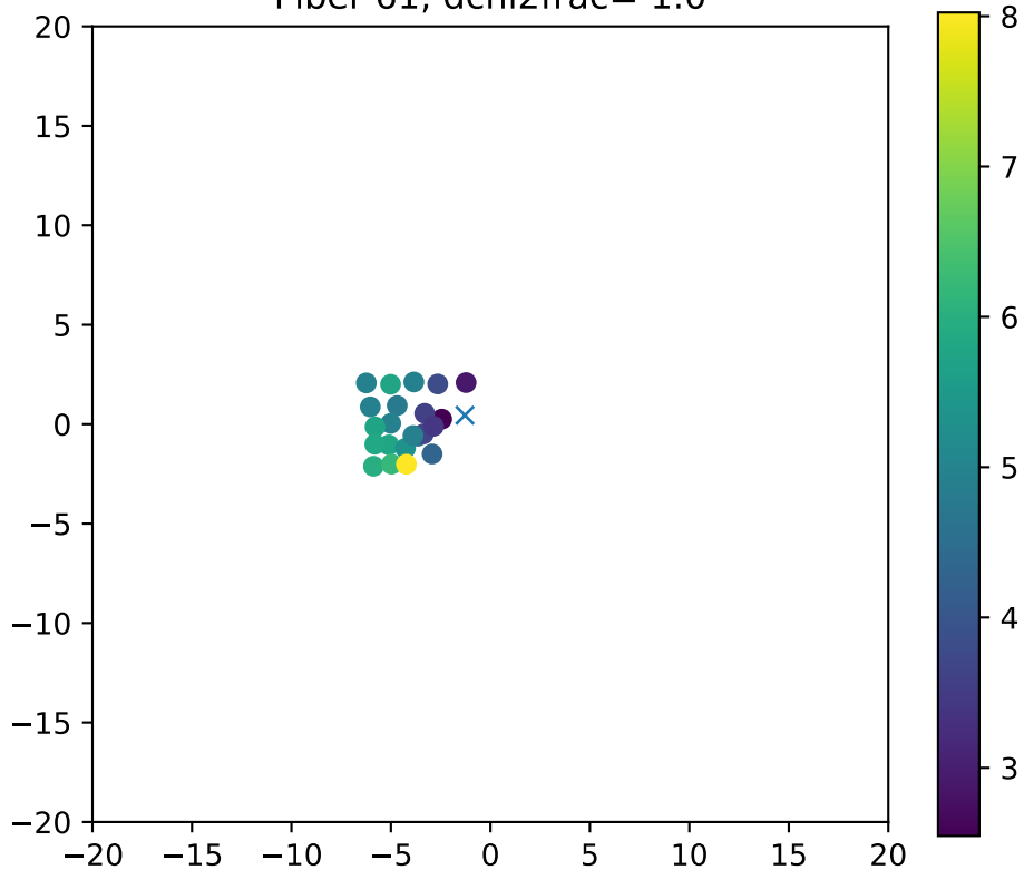
Fiber 61, dchi2frac= 1.0
