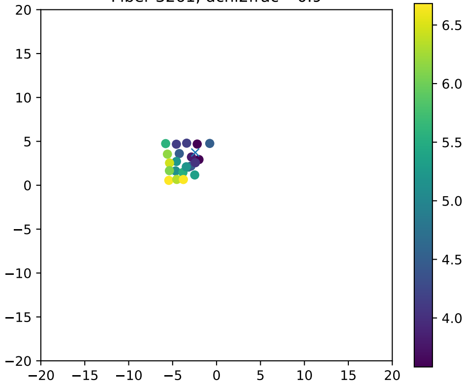
Fiber 3261, dchi2frac= 0.9
