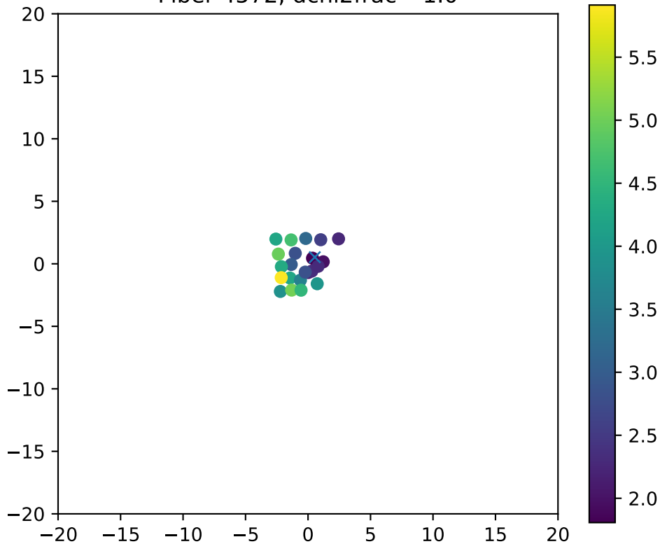
Fiber 4572, dchi2frac= 1.0
