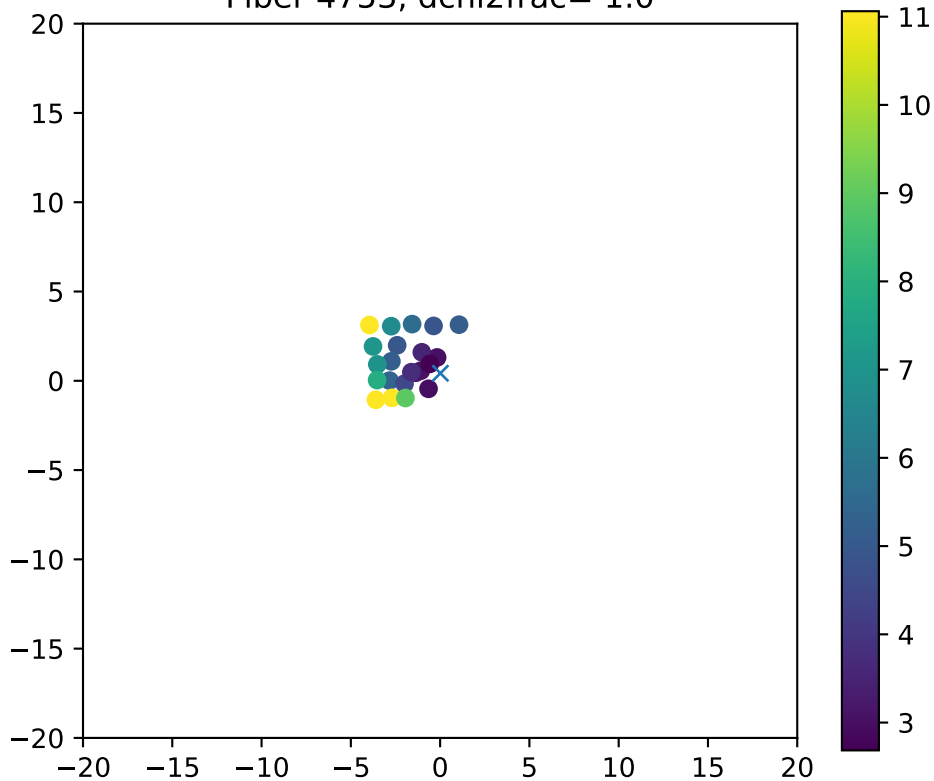
Fiber 4753, dchi2frac= 1.0
