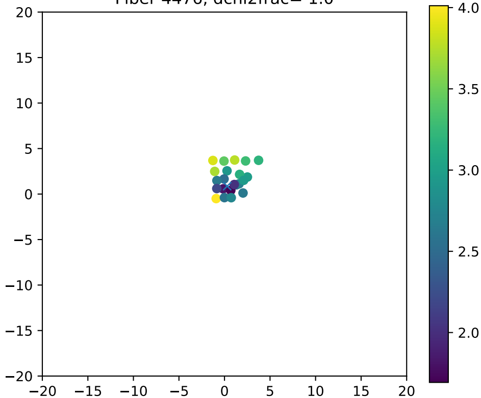
Fiber 4476, dchi2frac= 1.0
