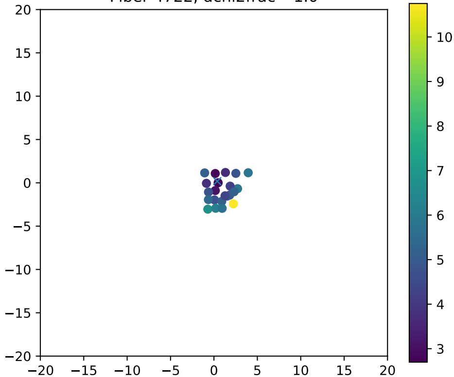
Fiber 4722, dchi2frac= 1.0
