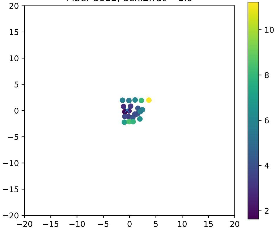
Fiber 3022, dchi2frac= 1.0
