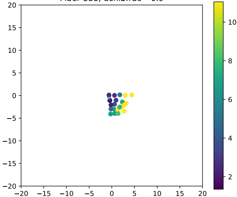
Fiber 888, dchi2frac= 0.9
