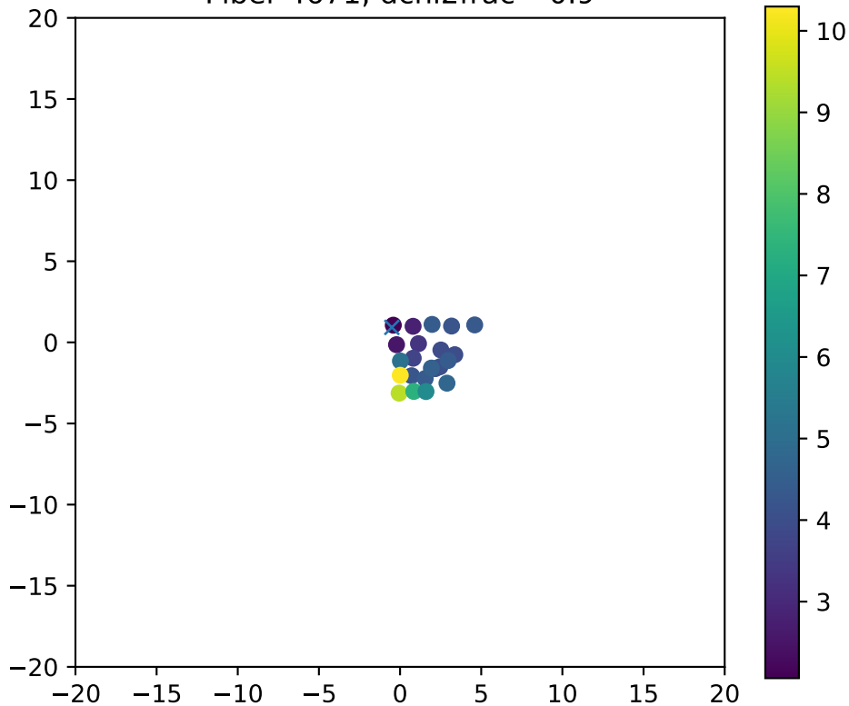
Fiber 4671, dchi2frac= 0.9
