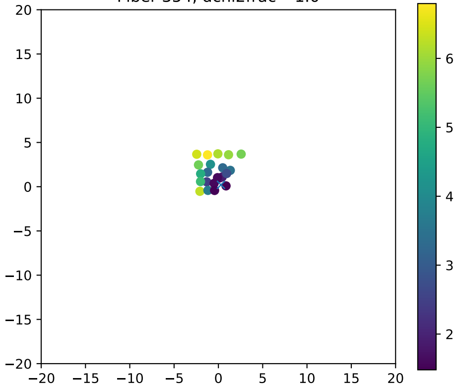
Fiber 354, dchi2frac= 1.0
