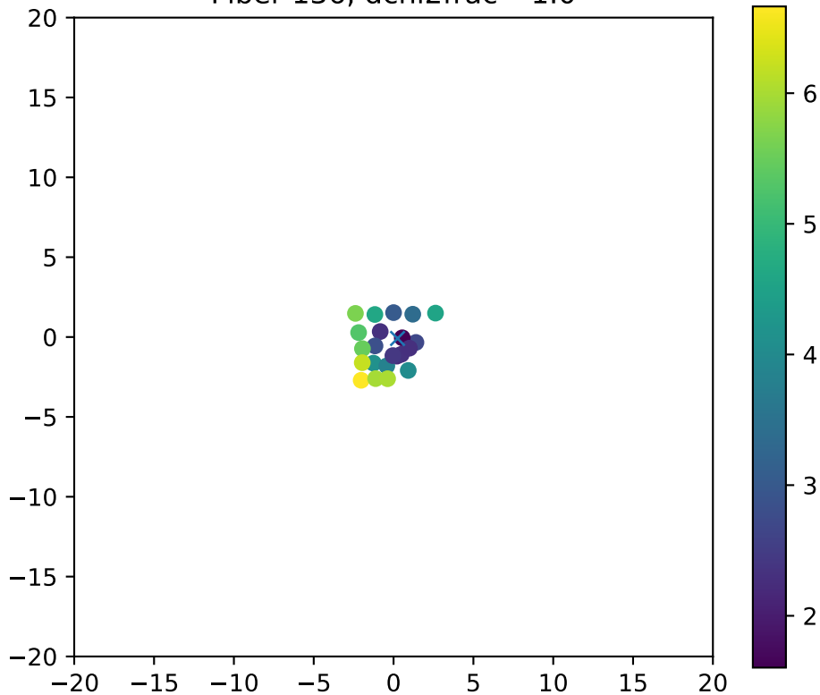
Fiber 136, dchi2frac= 1.0
