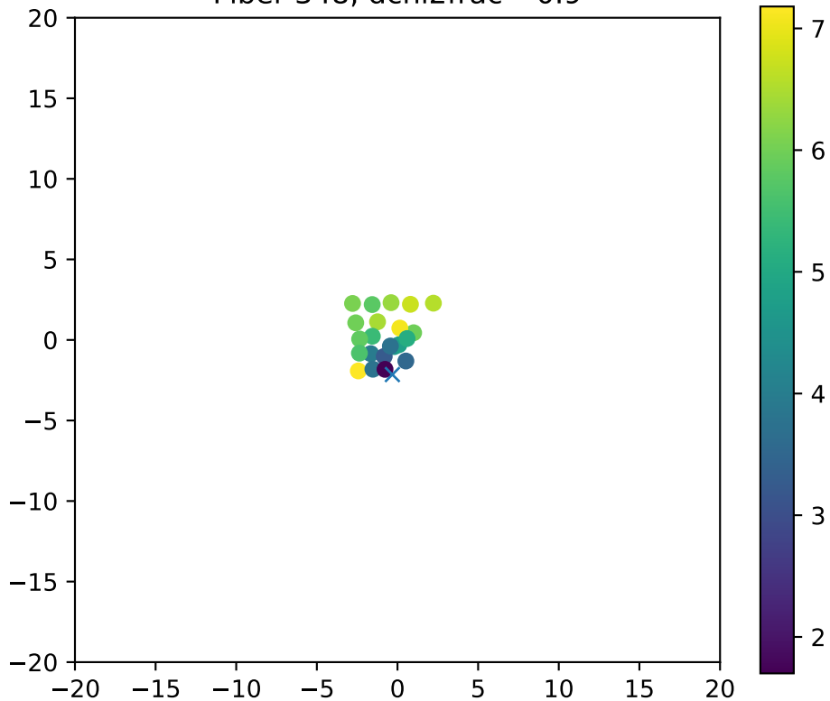
Fiber 348, dchi2frac= 0.9
