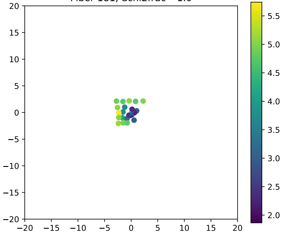
Fiber 181, dchi2frac= 1.0
