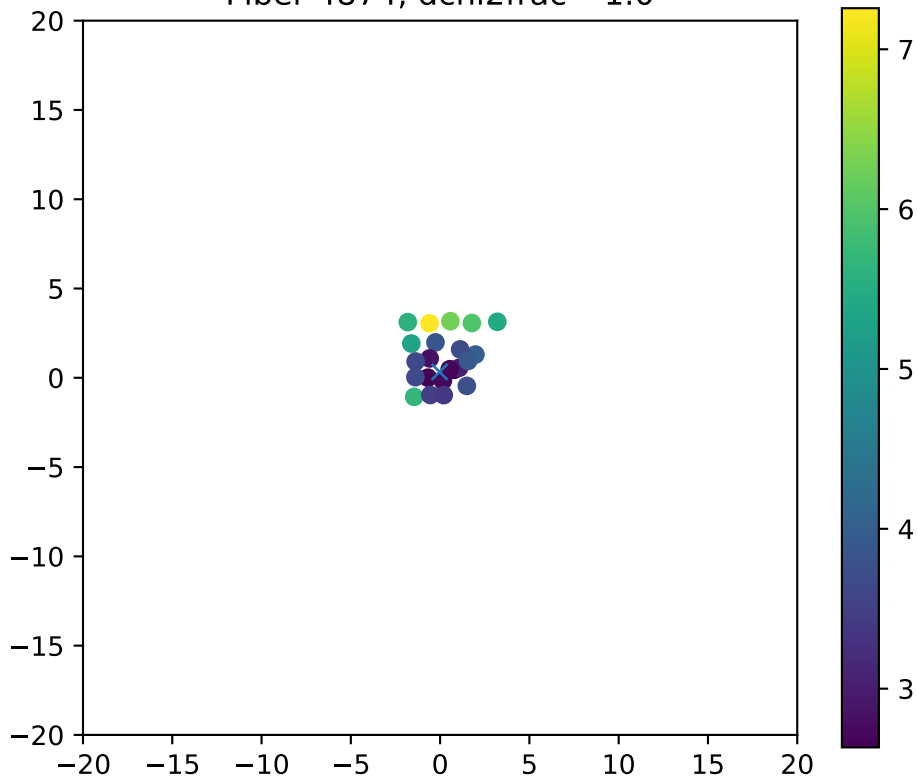
Fiber 4874, dchi2frac= 1.0
