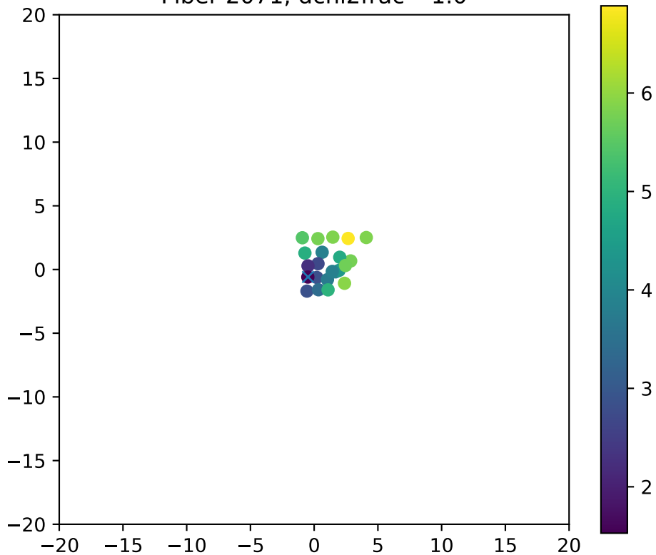
Fiber 2071, dchi2frac= 1.0
