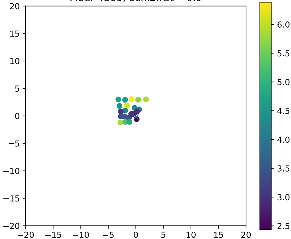
Fiber 4509, dchi2frac= 0.9
