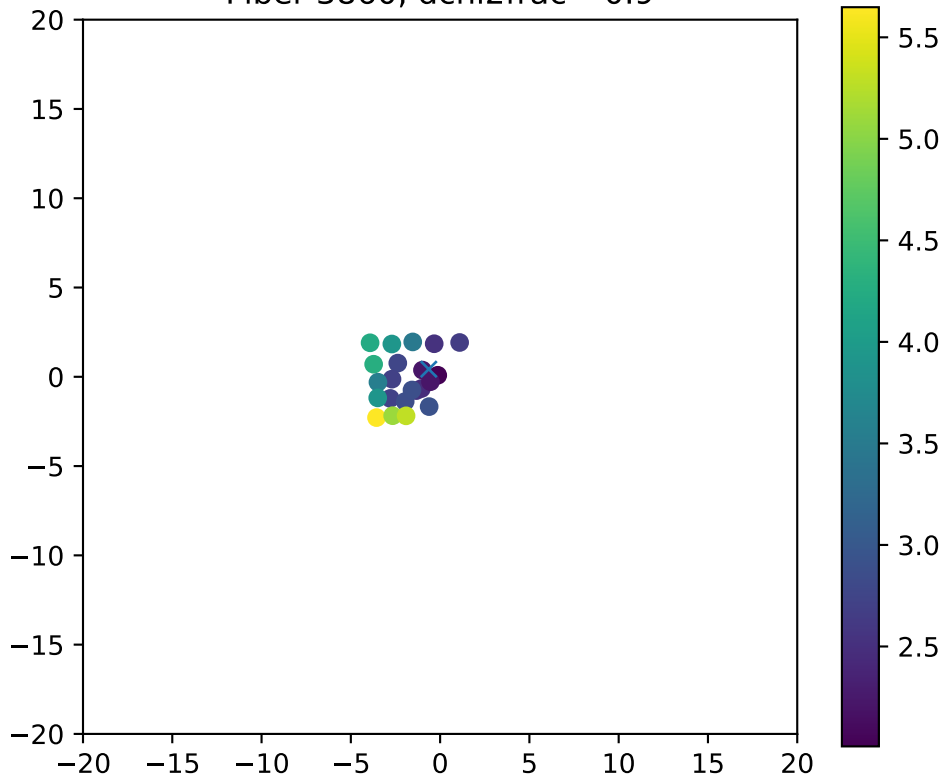
Fiber 3860, dchi2frac= 0.9
