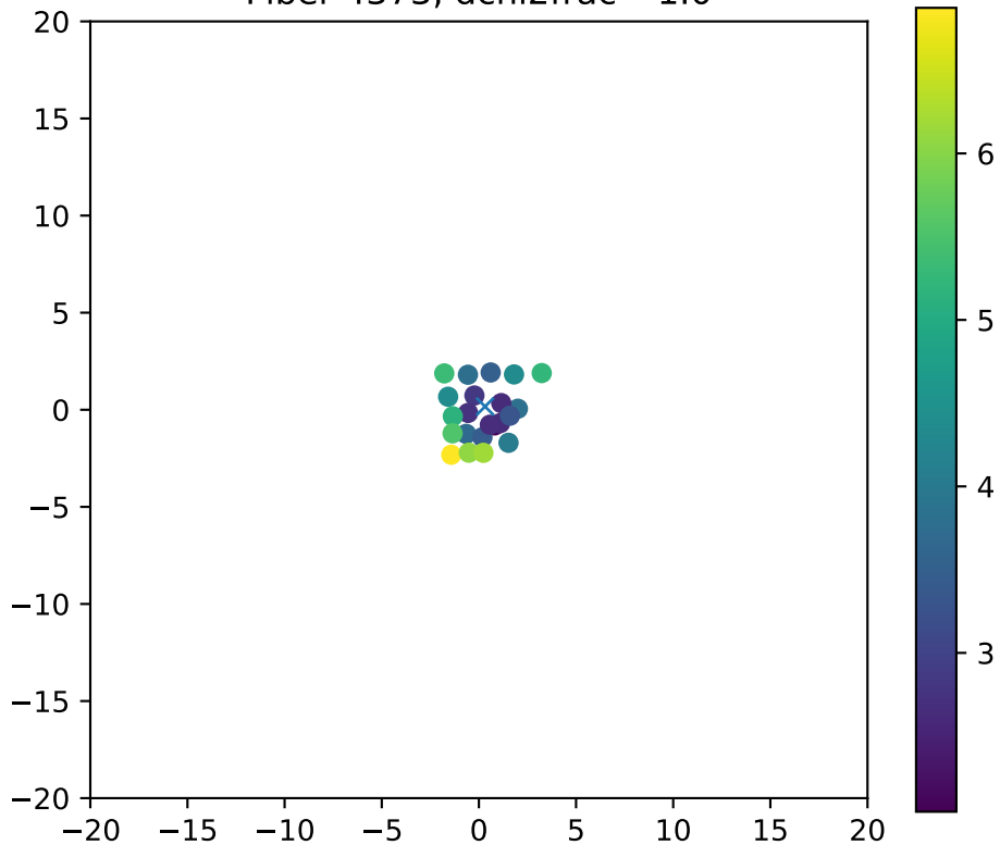
Fiber 4373, dchi2frac= 1.0
