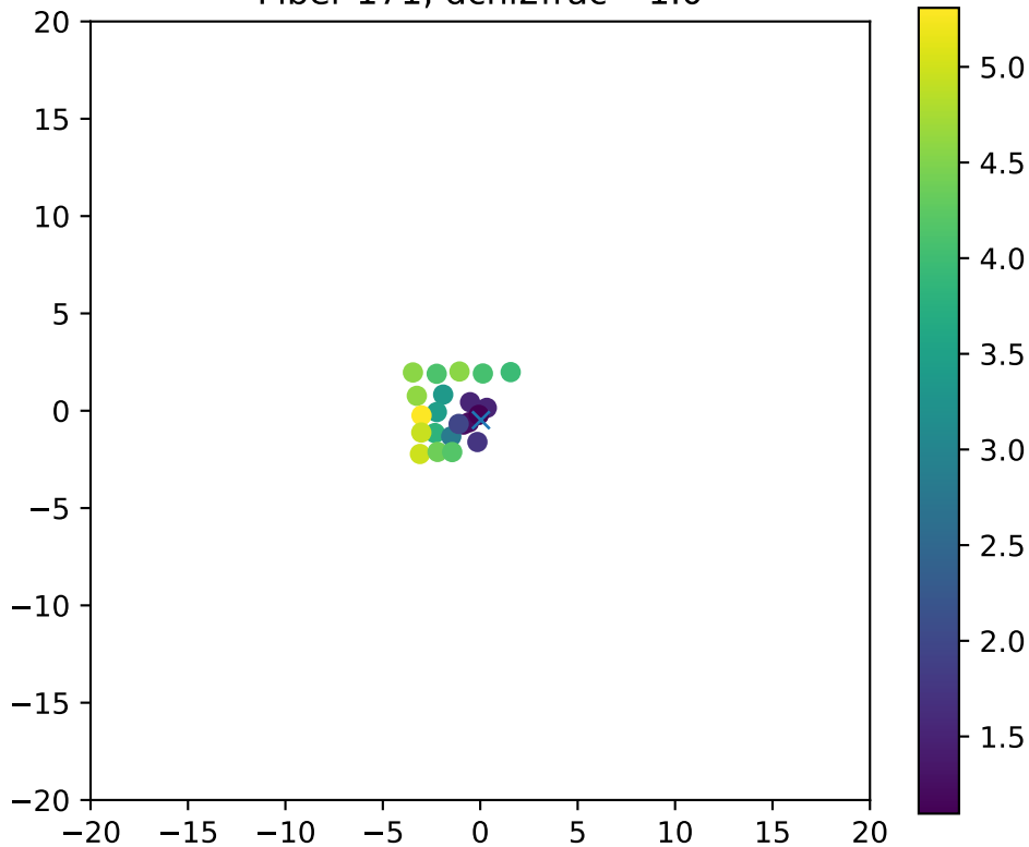
Fiber 171, dchi2frac= 1.0
