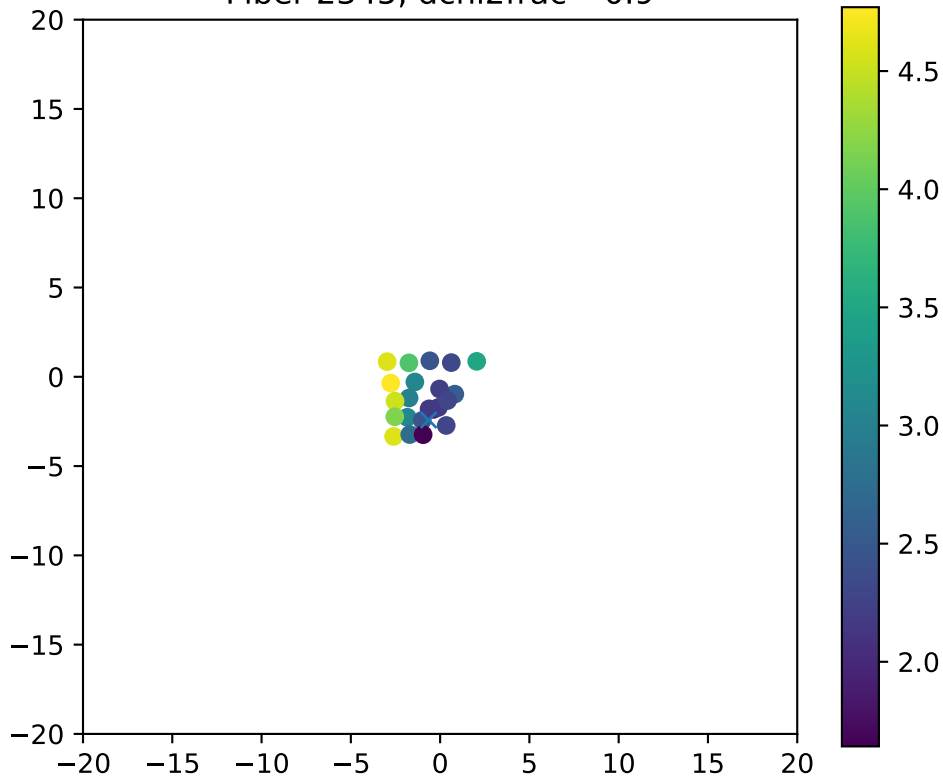
Fiber 2345, dchi2frac= 0.9
