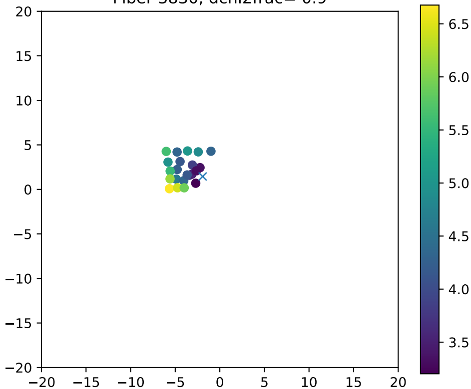
Fiber 3830, dchi2frac= 0.9
