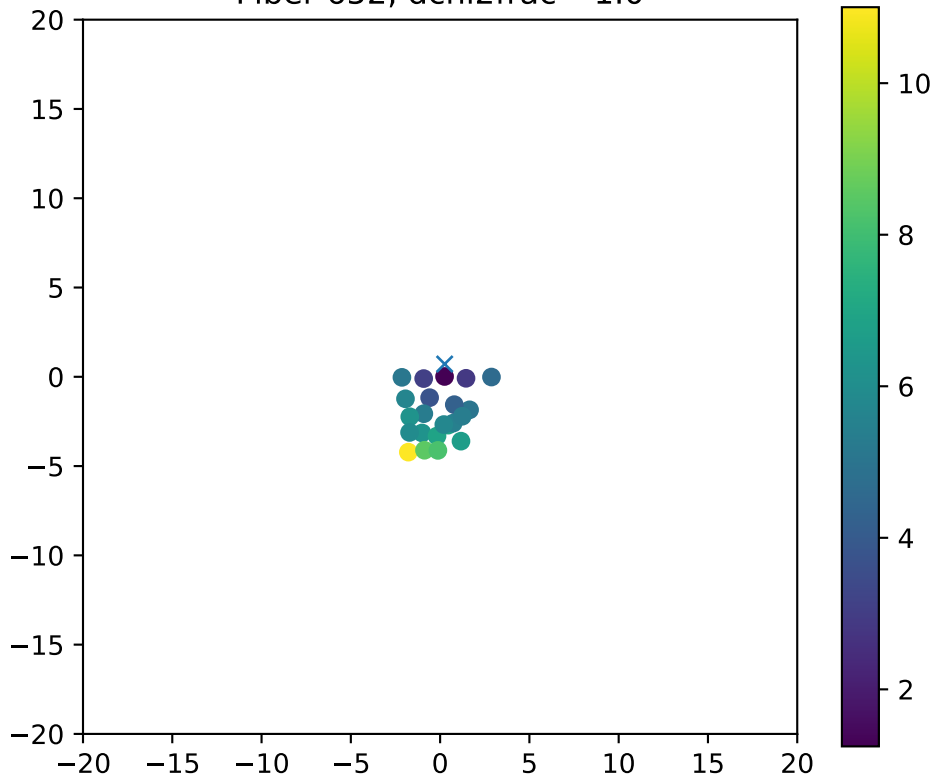
Fiber 652, dchi2frac= 1.0
