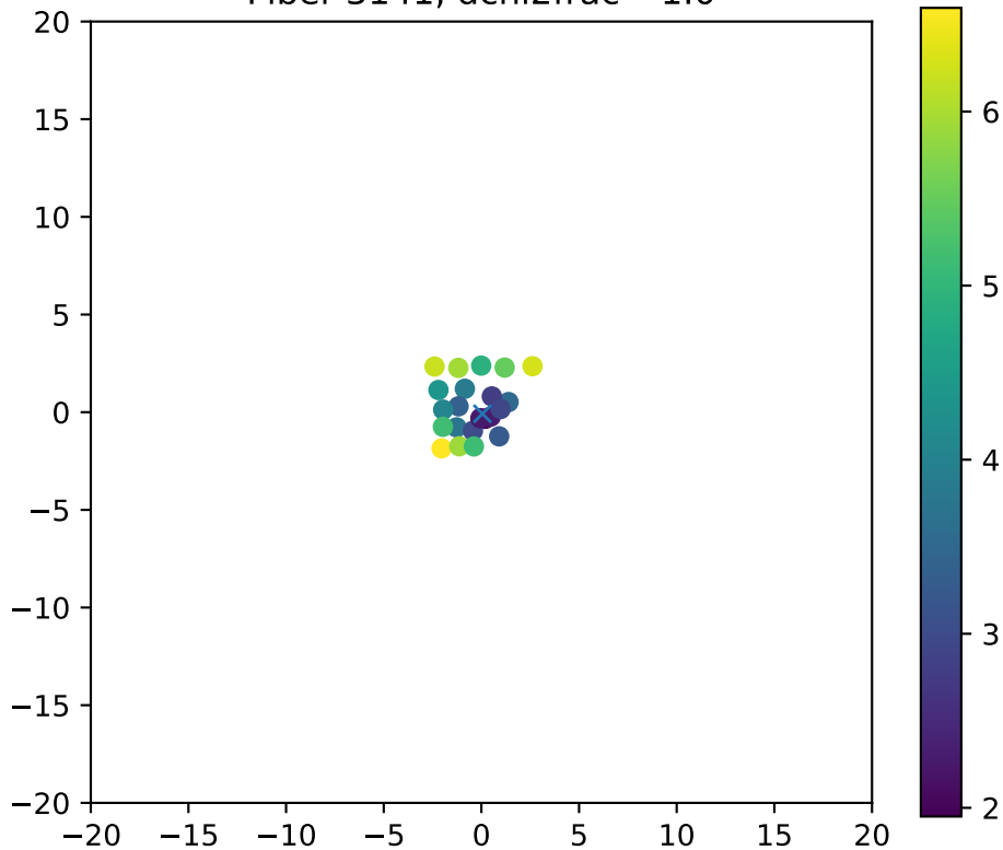
Fiber 3141, dchi2frac= 1.0
