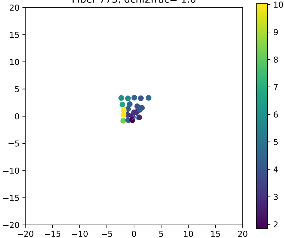
Fiber 775, dchi2frac= 1.0
