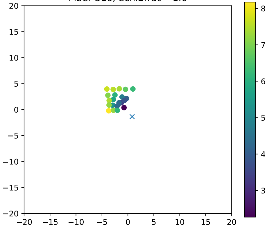
Fiber 316, dchi2frac= 1.0
