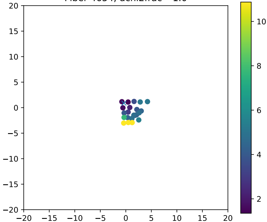
Fiber 4654, dchi2frac= 1.0
