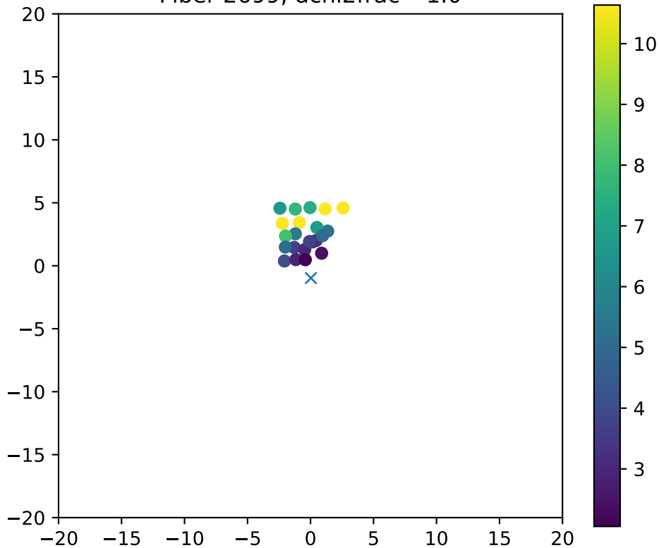
Fiber 2699, dchi2frac= 1.0
