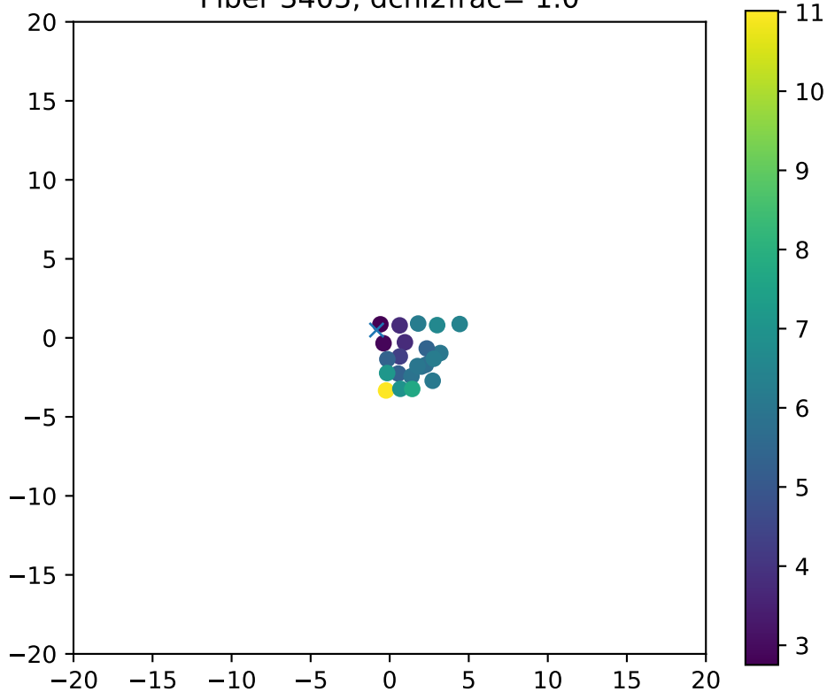
Fiber 3405, dchi2frac= 1.0
