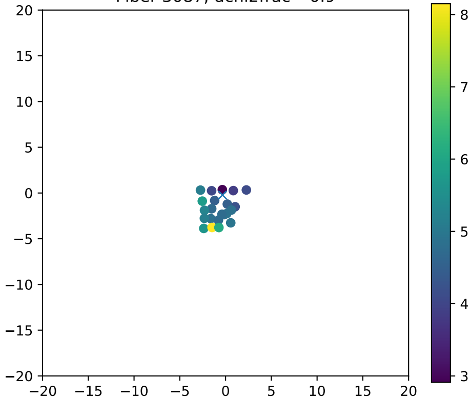
Fiber 3087, dchi2frac= 0.9
