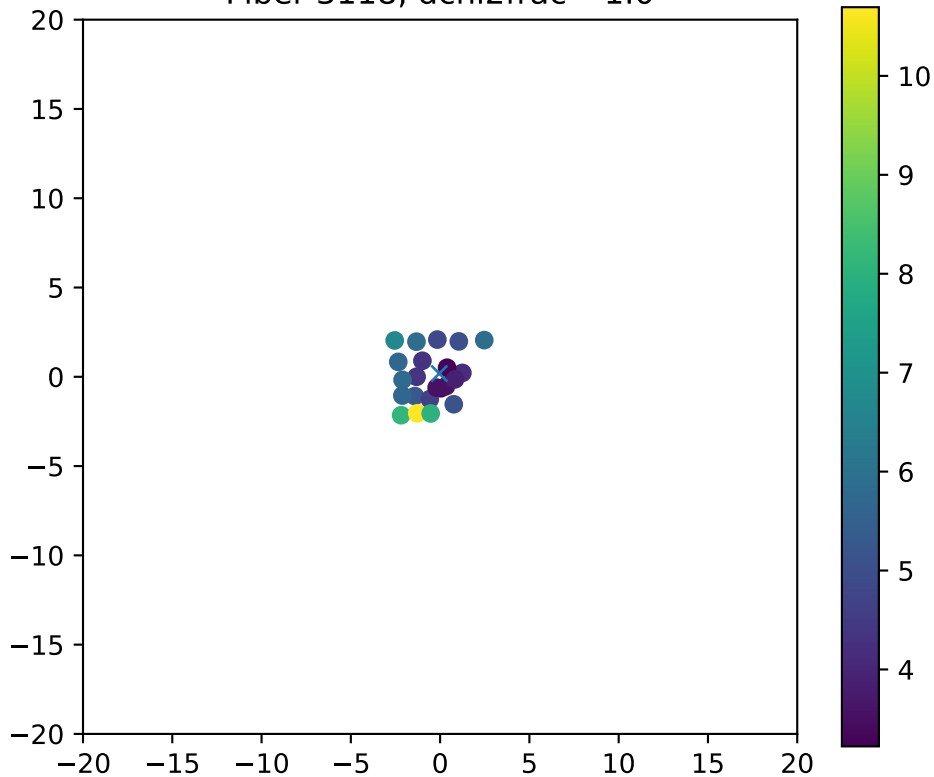
Fiber 3118, dchi2frac= 1.0
