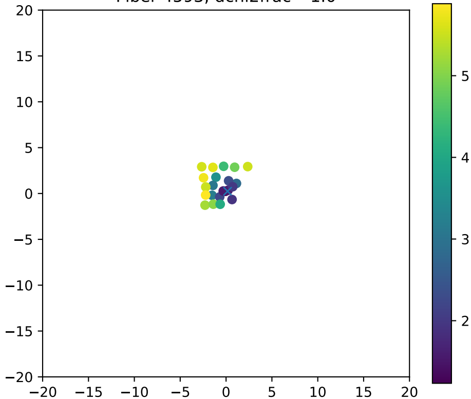
Fiber 4593, dchi2frac= 1.0
