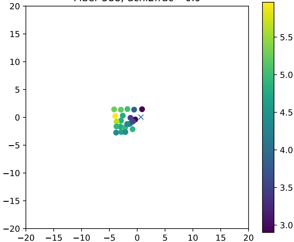
Fiber 588, dchi2frac= 0.9
