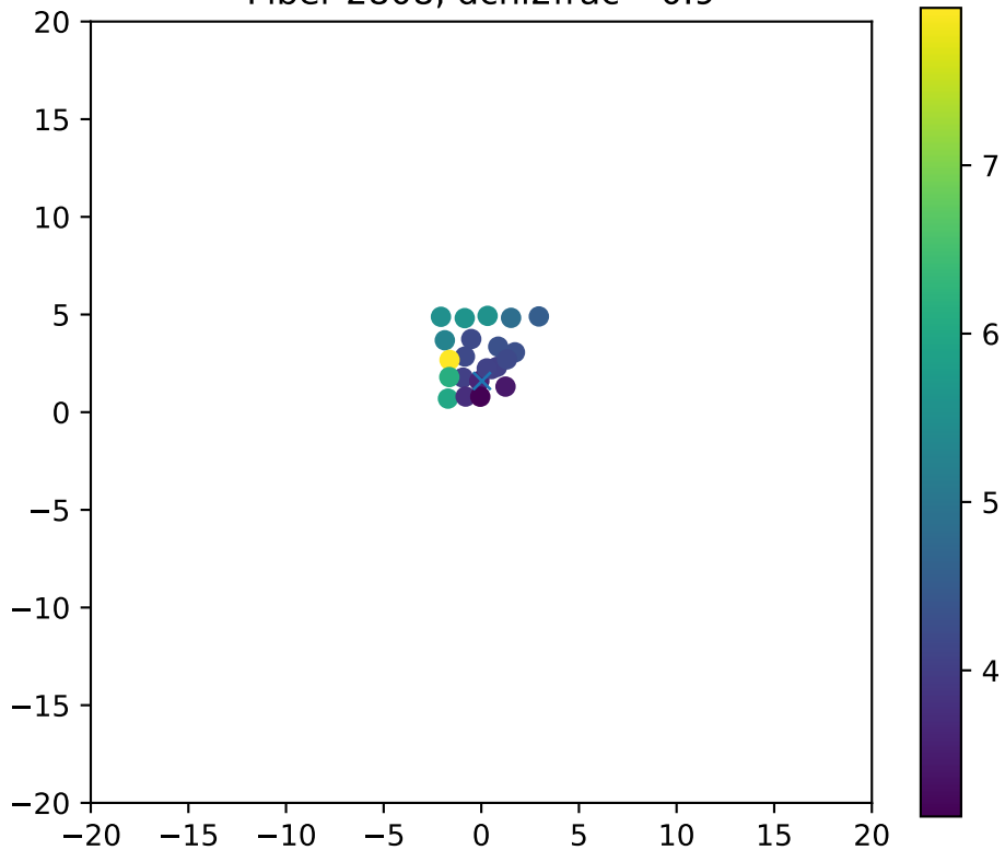
Fiber 2808, dchi2frac= 0.9
