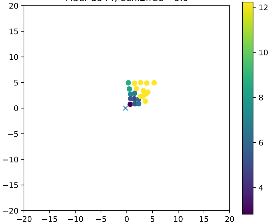
Fiber 3544, dchi2frac= 0.9
