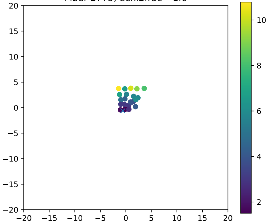
Fiber 2775, dchi2frac= 1.0
