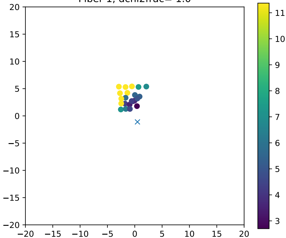
Fiber 1, dchi2frac= 1.0
