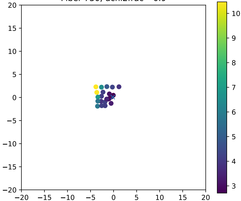
Fiber 730, dchi2frac= 0.9
