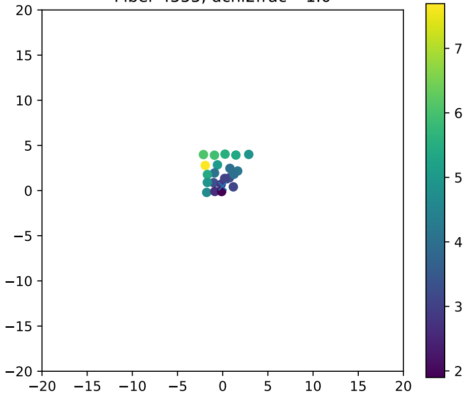
Fiber 4555, dchi2frac= 1.0
