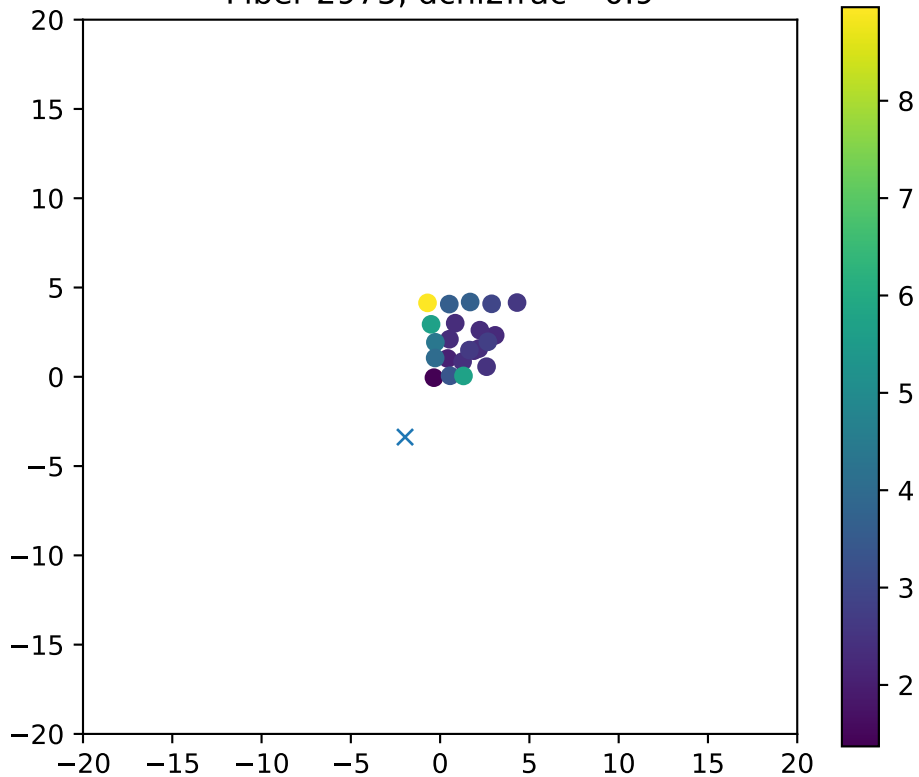
Fiber 2975, dchi2frac= 0.9
