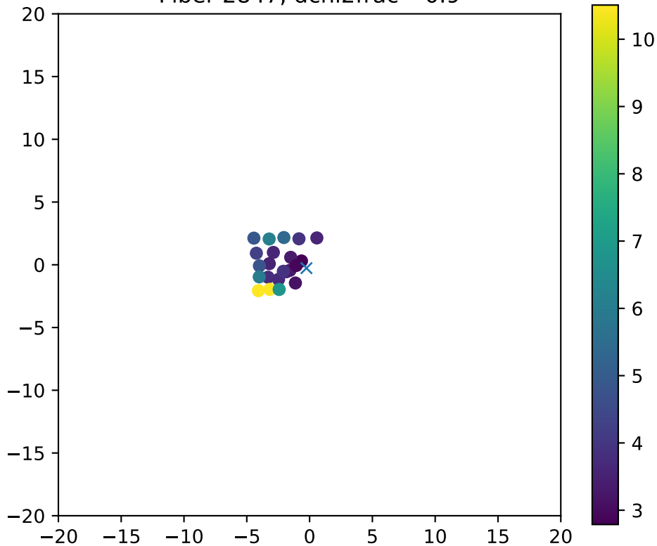
Fiber 2847, dchi2frac= 0.9
