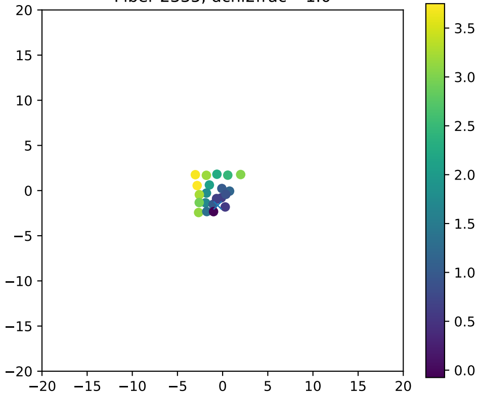
Fiber 2335, dchi2frac= 1.0
