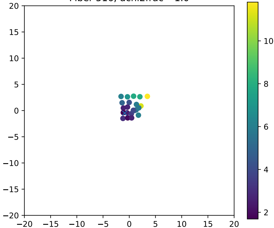
Fiber 516, dchi2frac= 1.0
