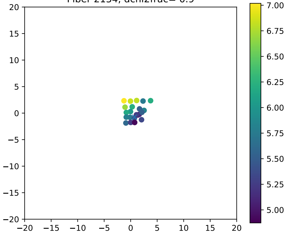
Fiber 2134, dchi2frac= 0.9
