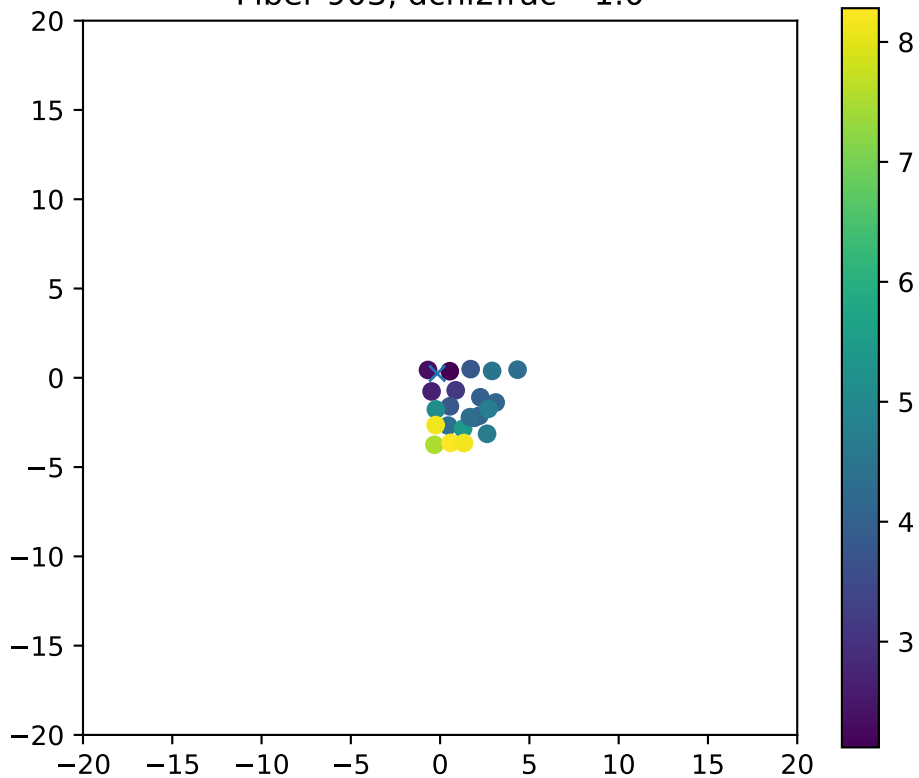
Fiber 903, dchi2frac= 1.0
