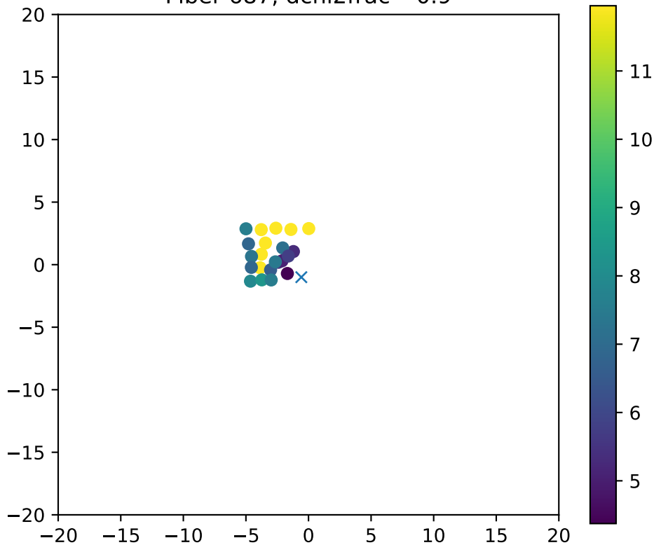
Fiber 687, dchi2frac= 0.9
