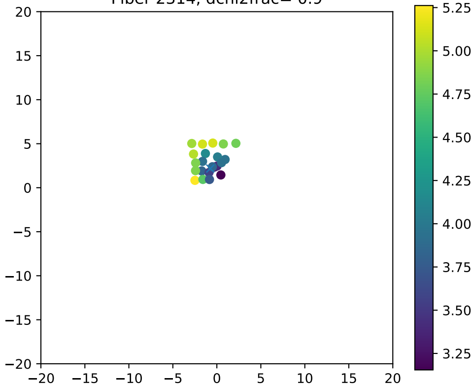
Fiber 2314, dchi2frac= 0.9
