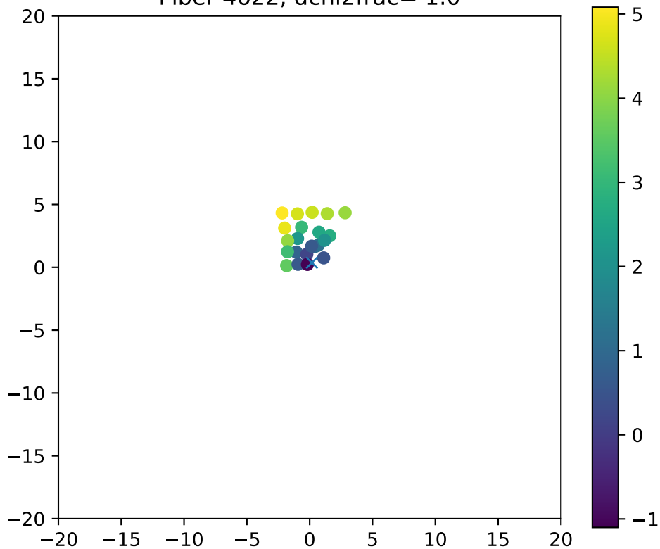
Fiber 4622, dchi2frac= 1.0
