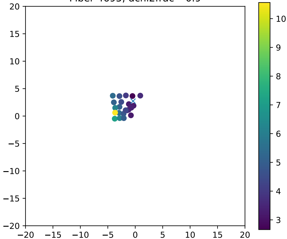
Fiber 4695, dchi2frac= 0.9
