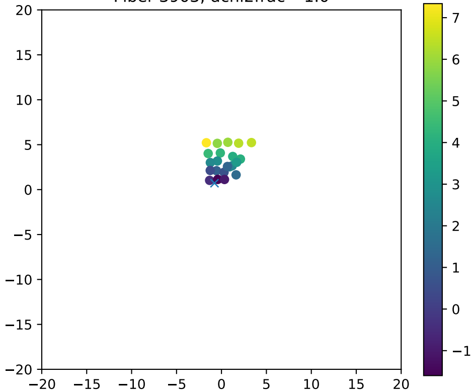
Fiber 3903, dchi2frac= 1.0
