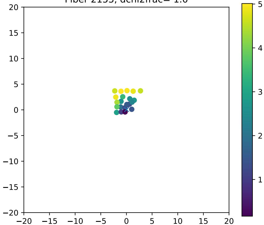
Fiber 2153, dchi2frac= 1.0
