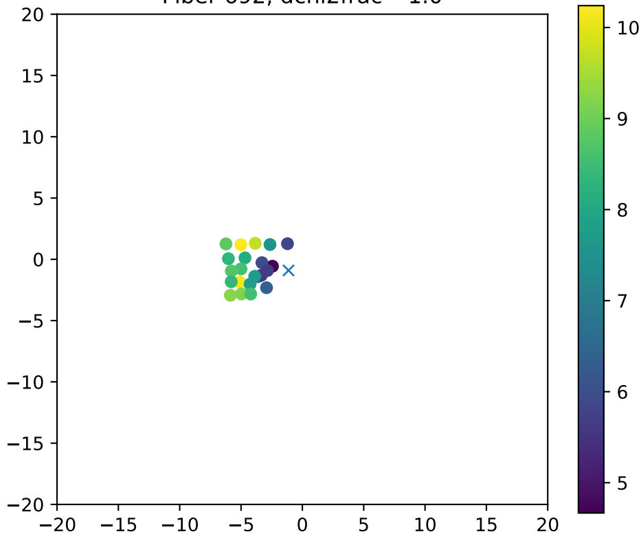
Fiber 692, dchi2frac= 1.0
