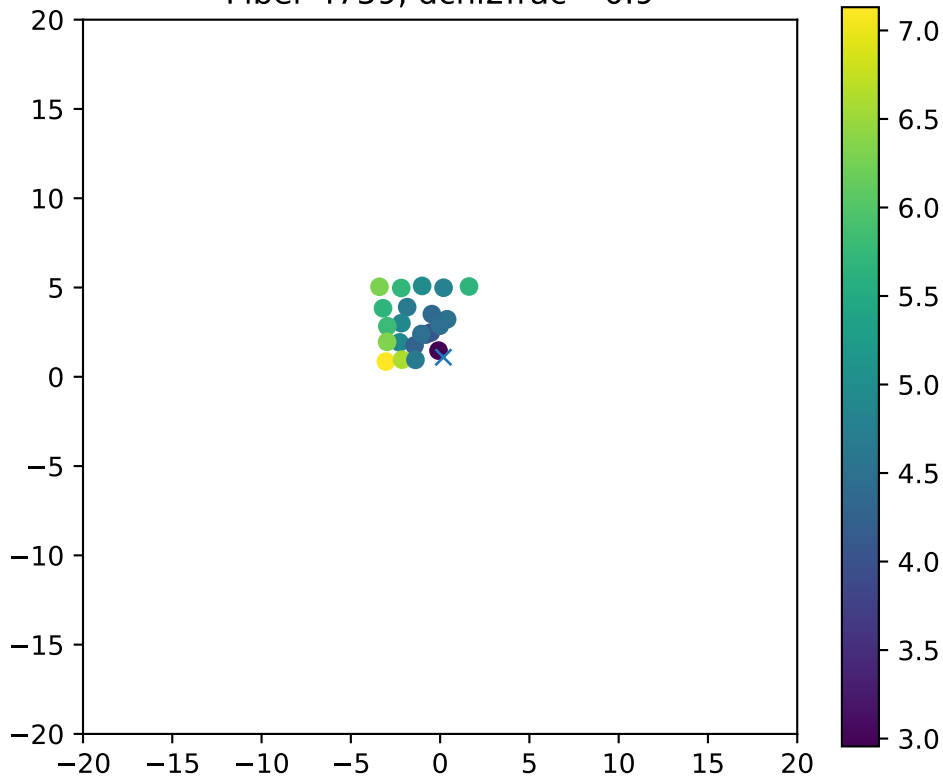
Fiber 4759, dchi2frac= 0.9
