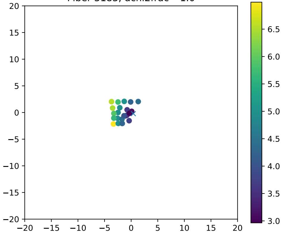
Fiber 3183, dchi2frac= 1.0
