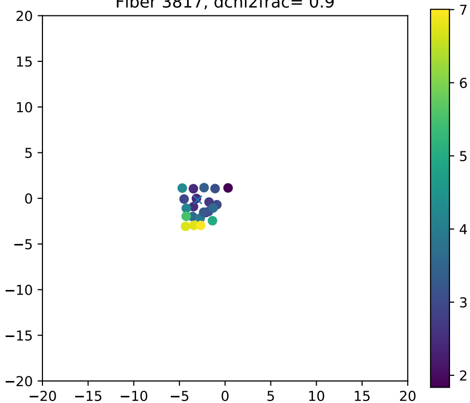
Fiber 3817, dchi2frac= 0.9
