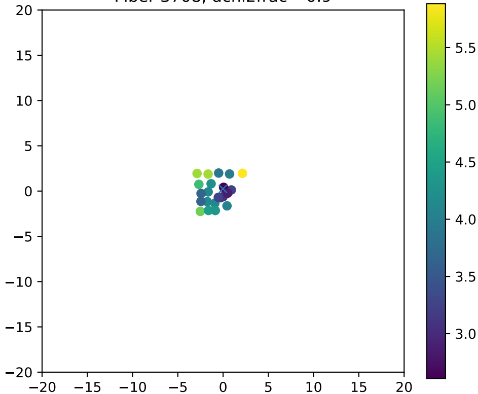
Fiber 3708, dchi2frac= 0.9
