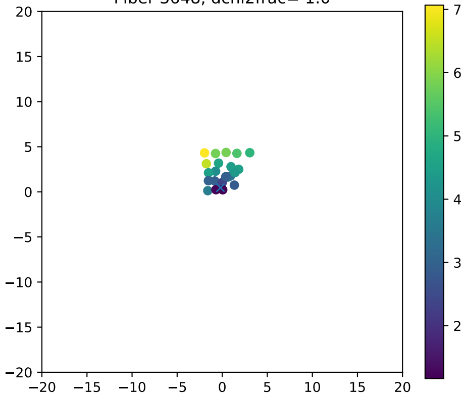
Fiber 3648, dchi2frac= 1.0
