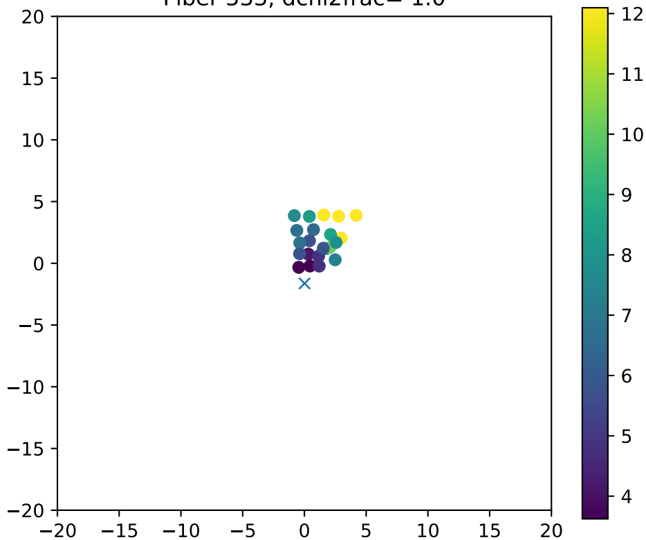
Fiber 533, dchi2frac= 1.0
