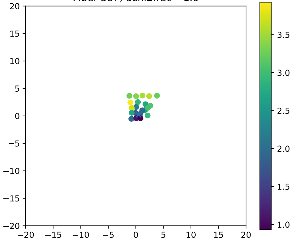
Fiber 587, dchi2frac= 1.0
