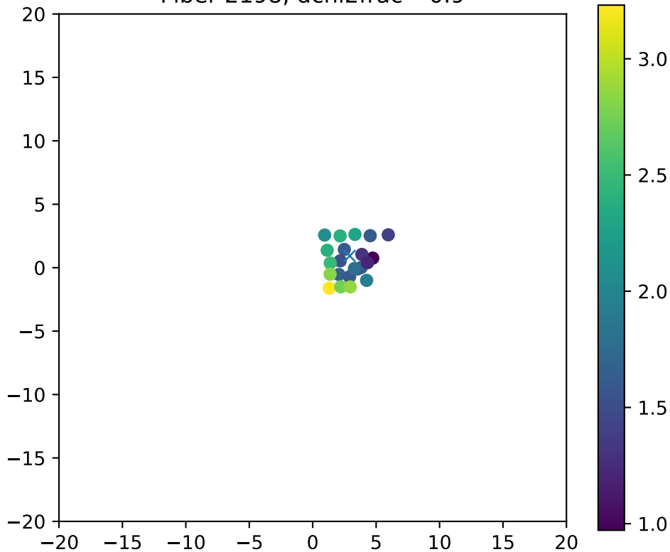
Fiber 2198, dchi2frac= 0.9
