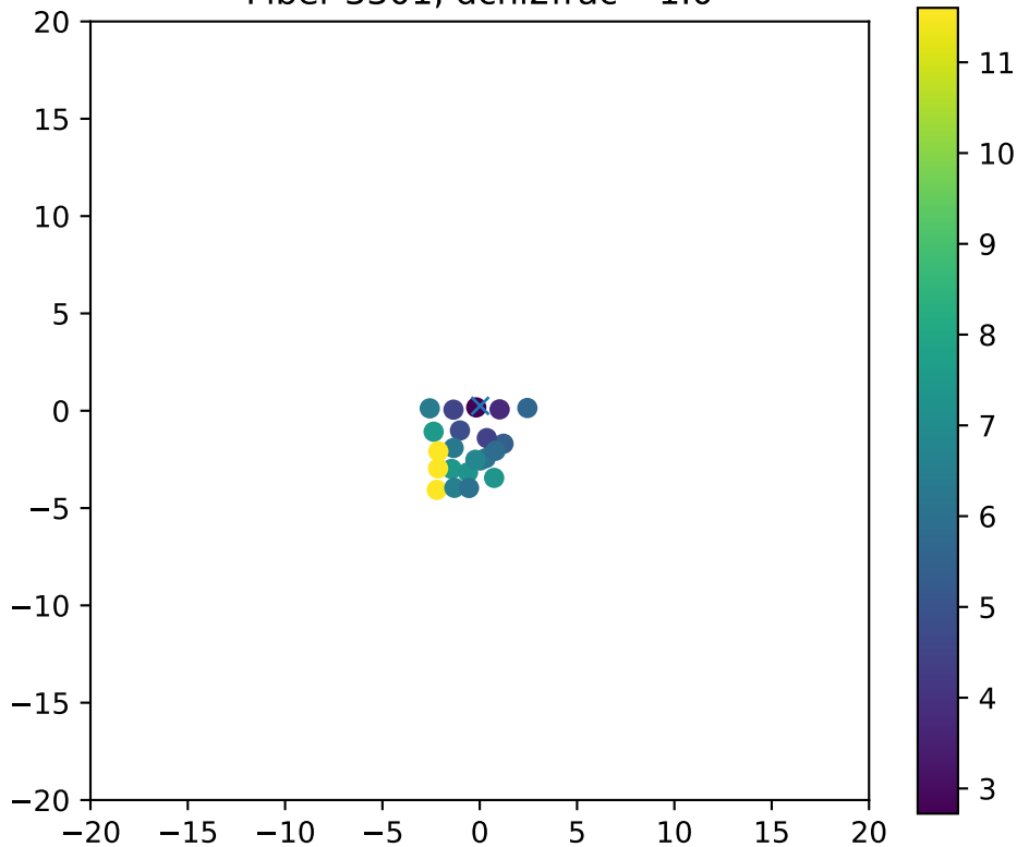
Fiber 3301, dchi2frac= 1.0
