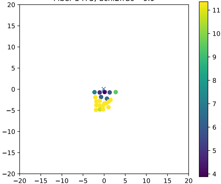
Fiber 3473, dchi2frac= 0.9
