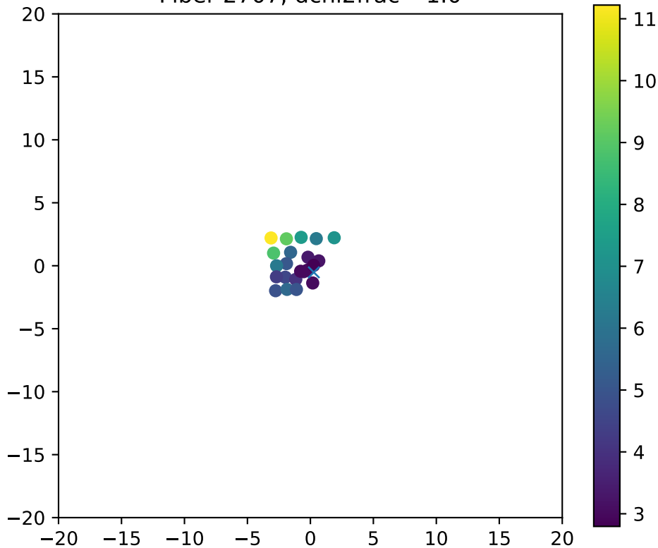
Fiber 2707, dchi2frac= 1.0
