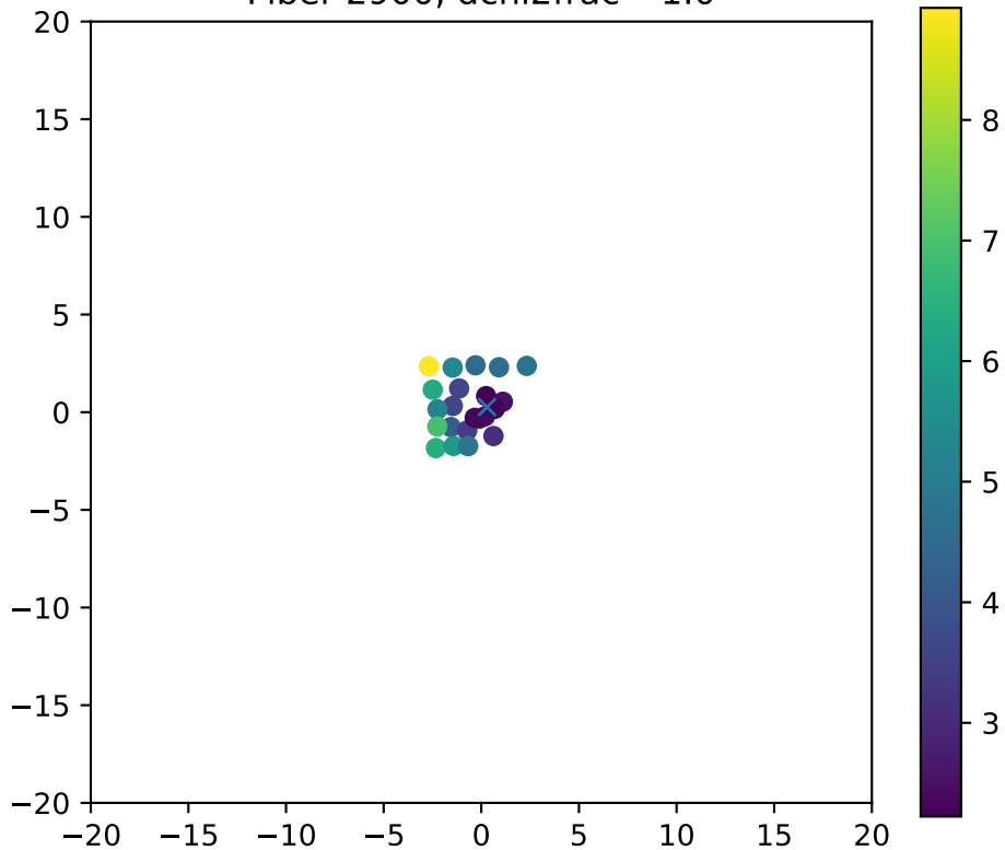
Fiber 2900, dchi2frac= 1.0
