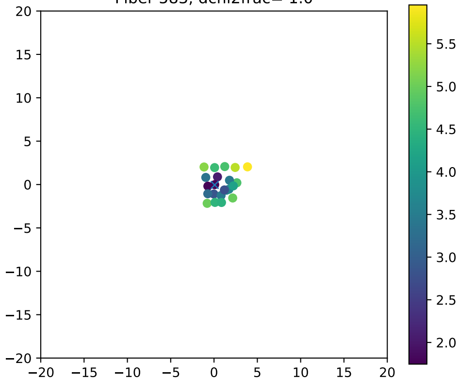
Fiber 583, dchi2frac= 1.0
