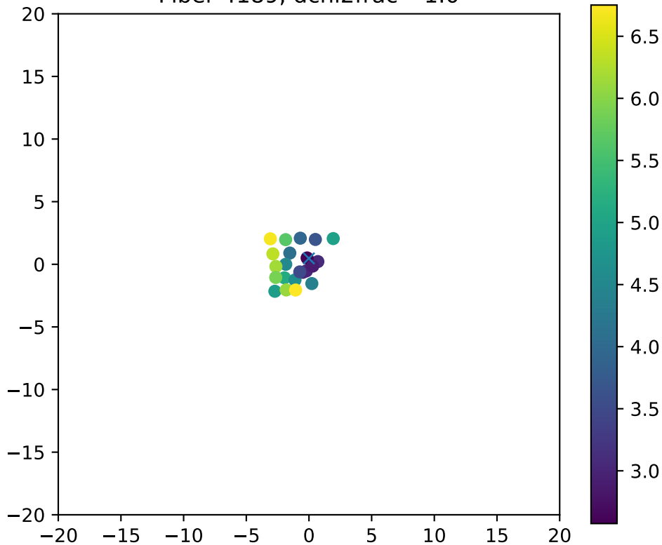
Fiber 4189, dchi2frac= 1.0
