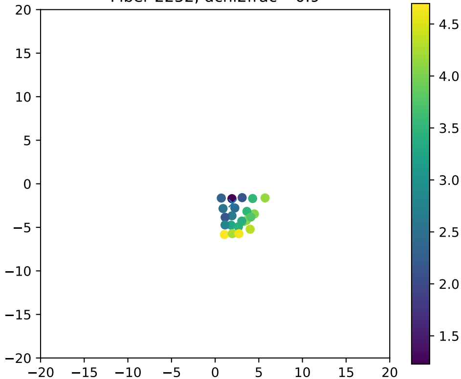
Fiber 2252, dchi2frac= 0.9
