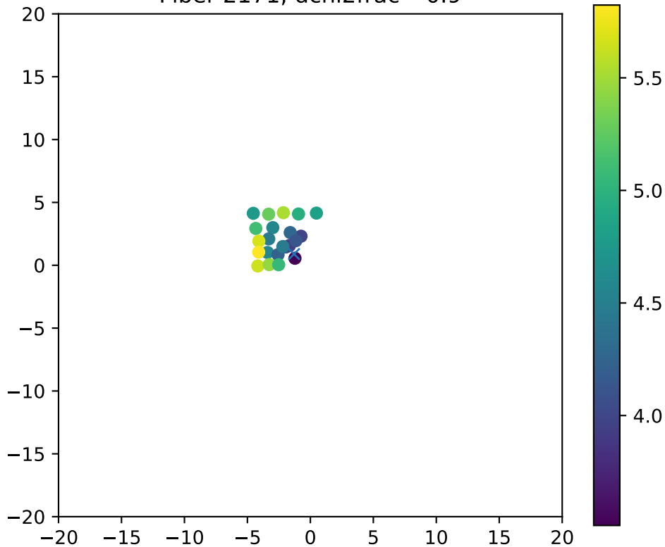
Fiber 2171, dchi2frac= 0.9
