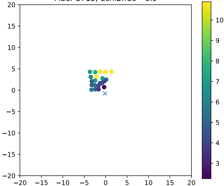
Fiber 3715, dchi2frac= 0.9
