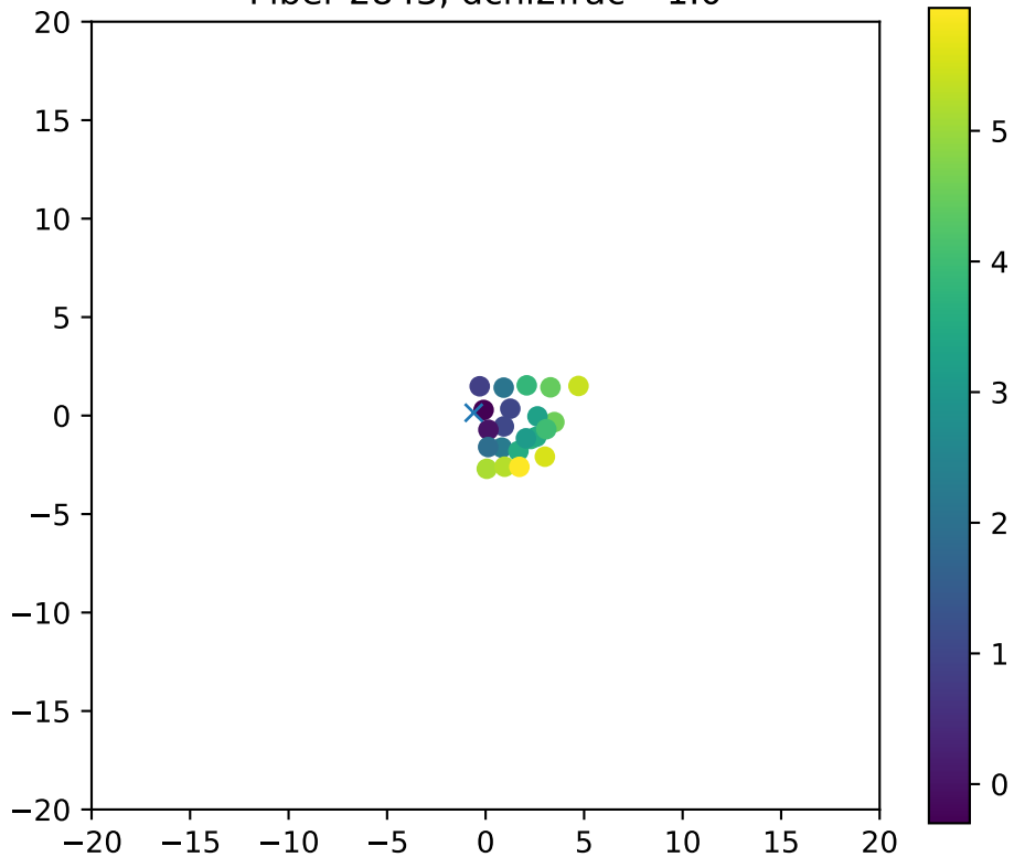
Fiber 2843, dchi2frac= 1.0
