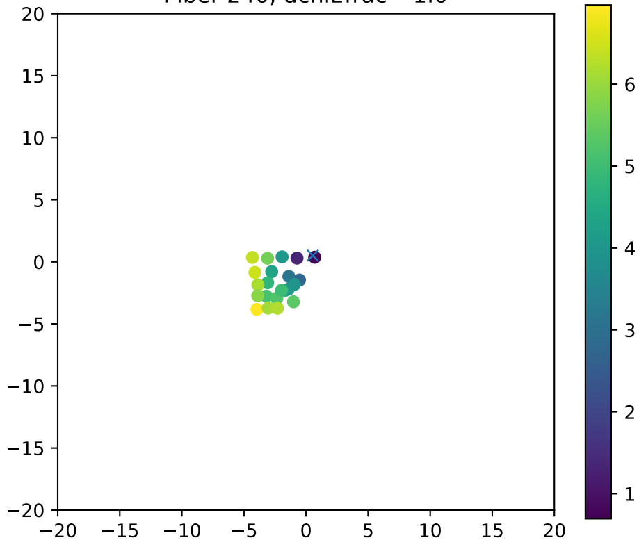
Fiber 240, dchi2frac= 1.0
