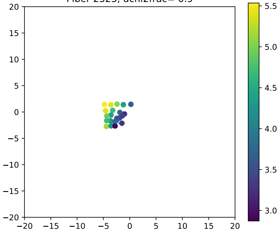
Fiber 2323, dchi2frac= 0.9
