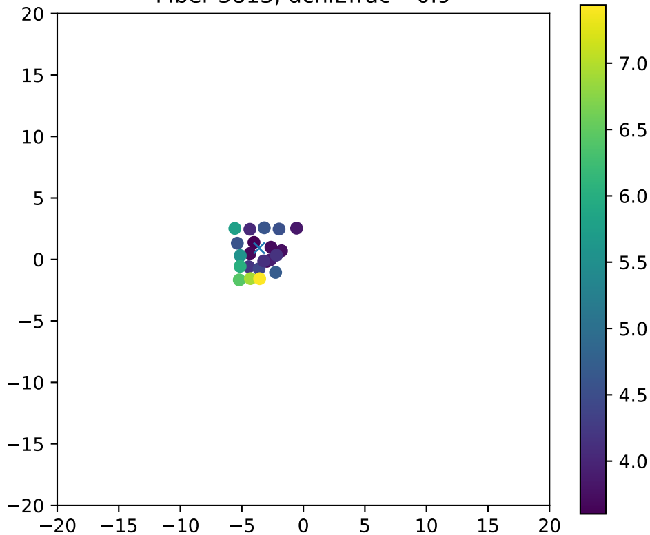
Fiber 3813, dchi2frac= 0.9
