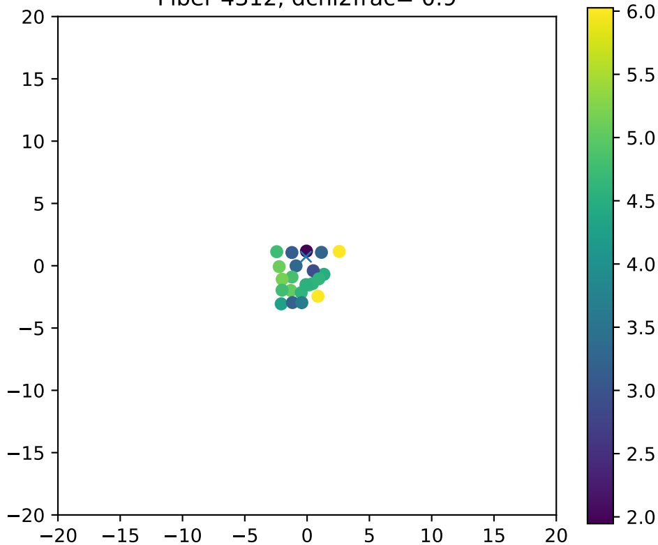
Fiber 4312, dchi2frac= 0.9
