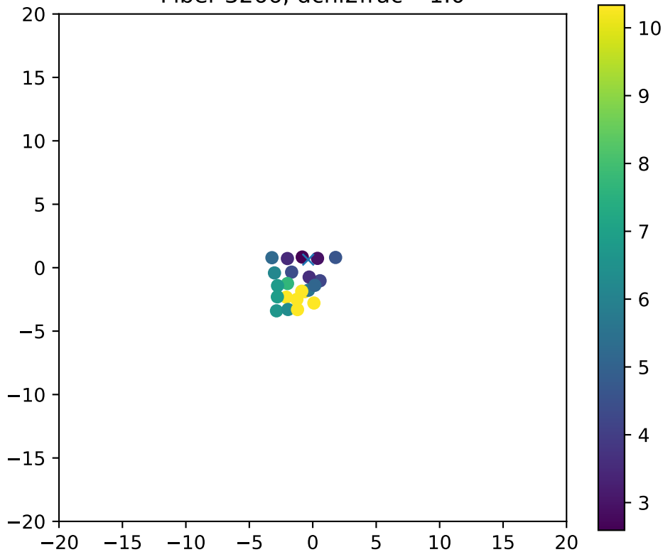
Fiber 3266, dchi2frac= 1.0
