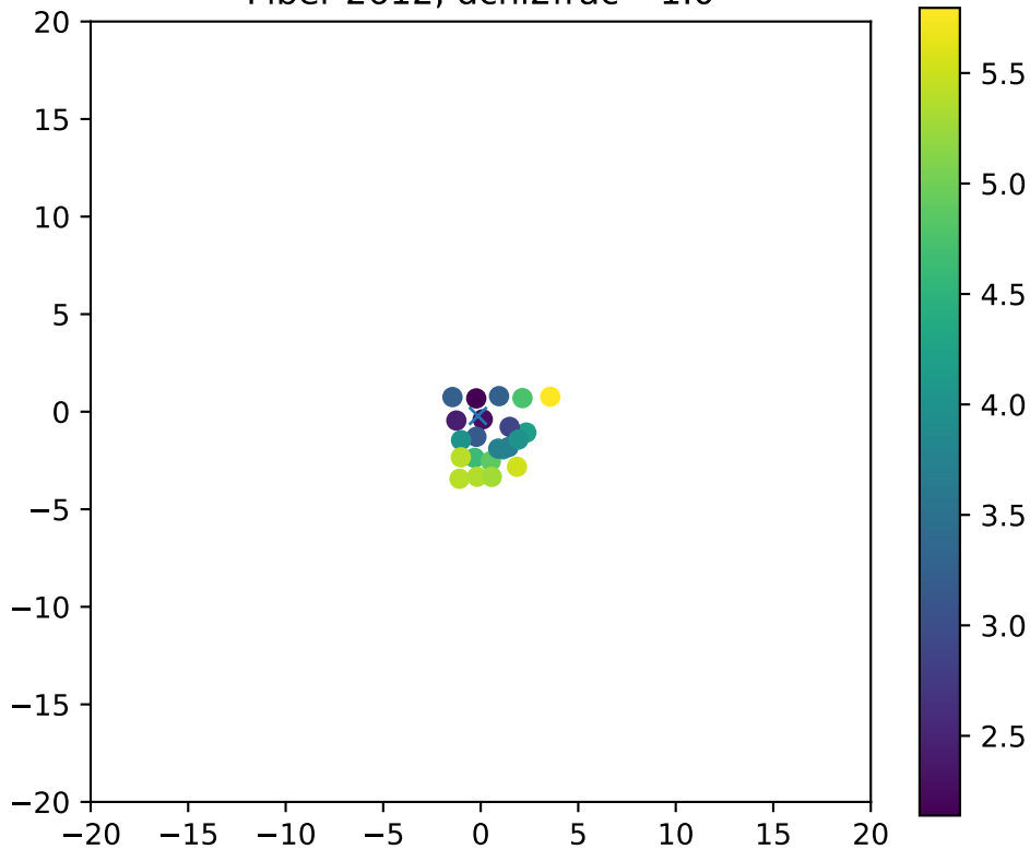
Fiber 2612, dchi2frac= 1.0
