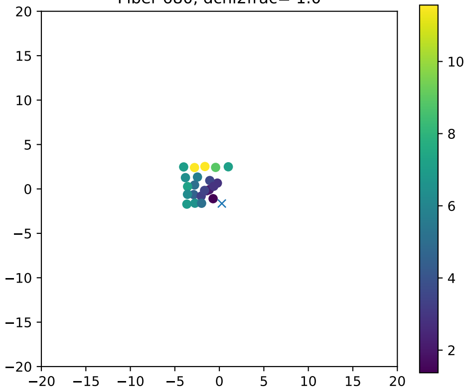
Fiber 680, dchi2frac= 1.0
