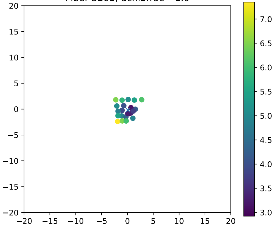
Fiber 3201, dchi2frac= 1.0
