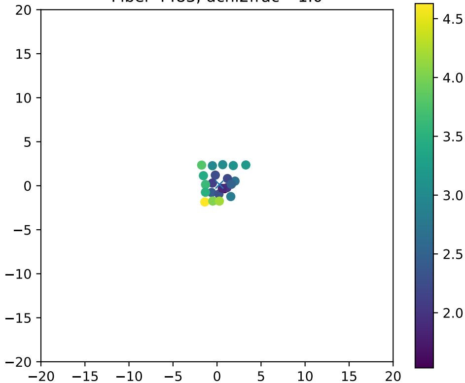
Fiber 4483, dchi2frac= 1.0
