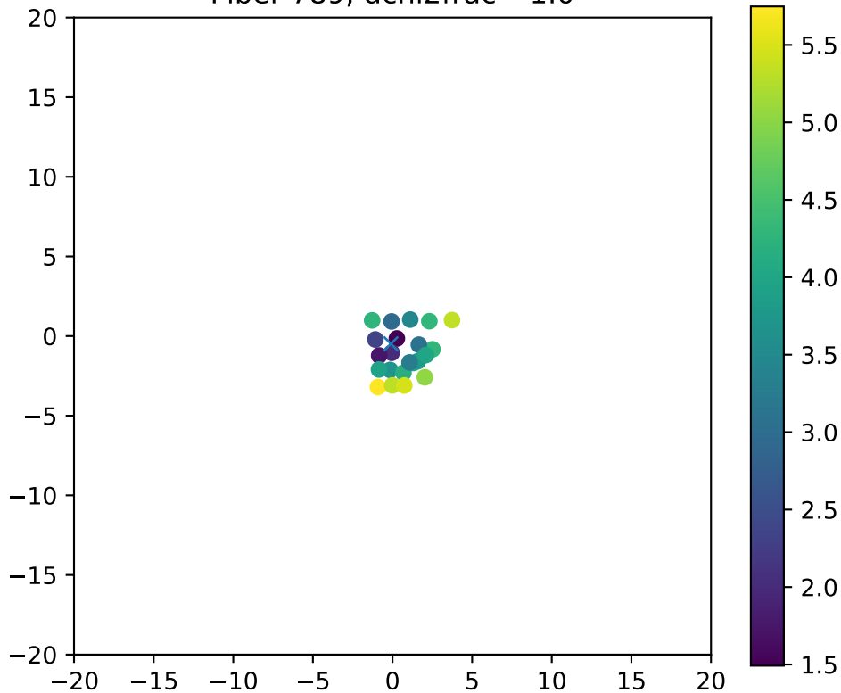
Fiber 789, dchi2frac= 1.0
