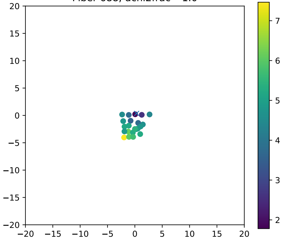
Fiber 688, dchi2frac= 1.0
