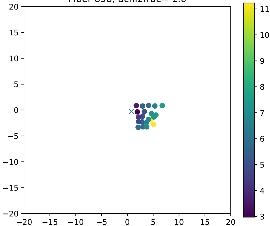
Fiber 858, dchi2frac= 1.0
