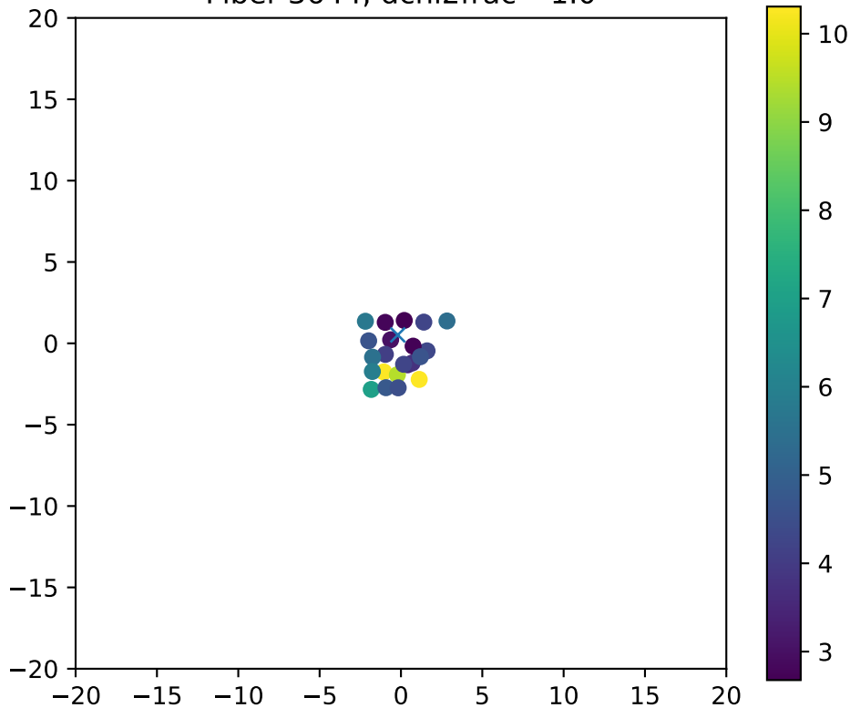
Fiber 3644, dchi2frac= 1.0
