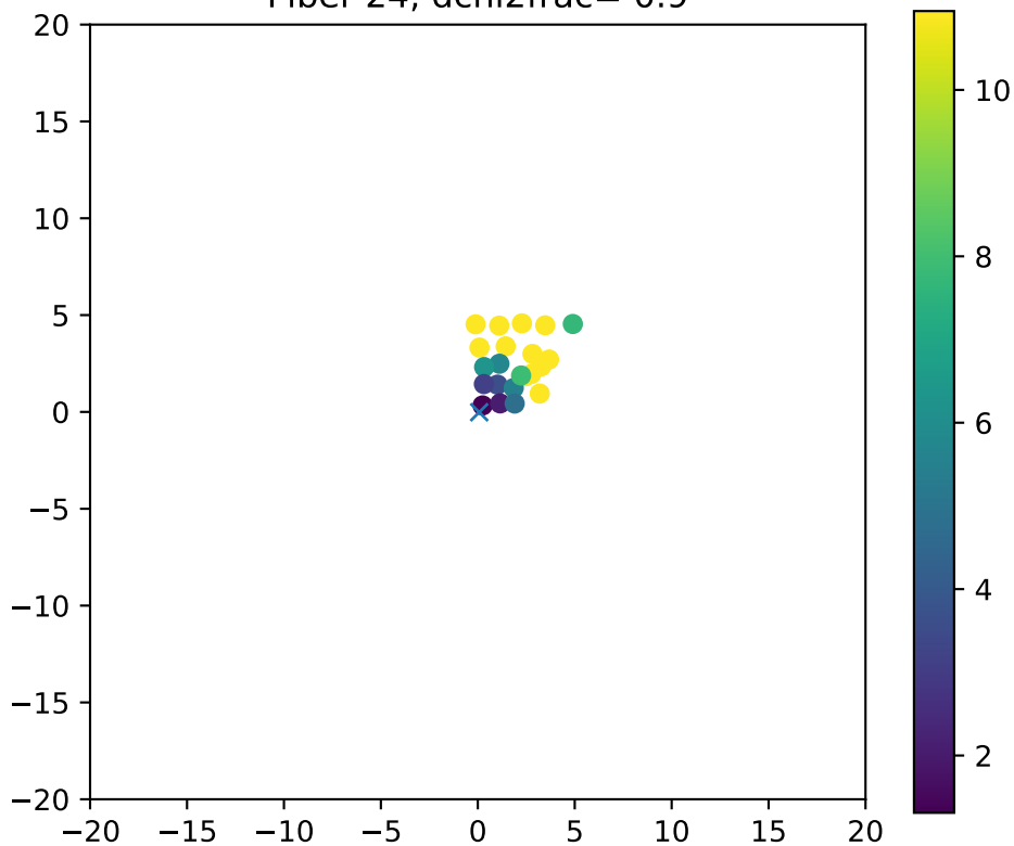
Fiber 24, dchi2frac= 0.9
