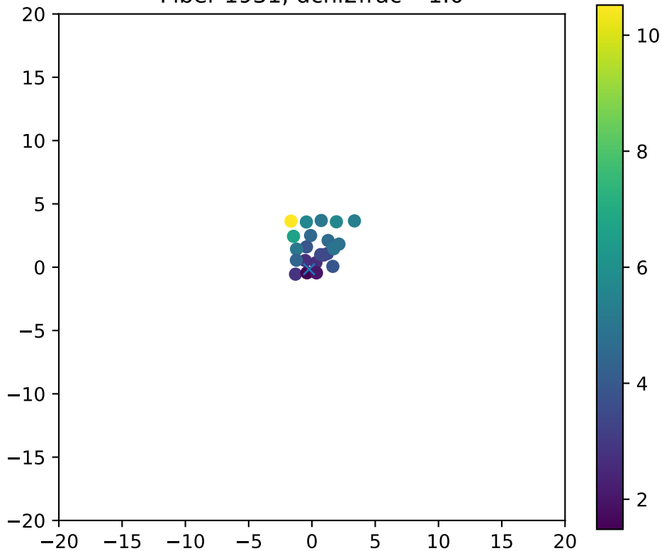
Fiber 1931, dchi2frac= 1.0
