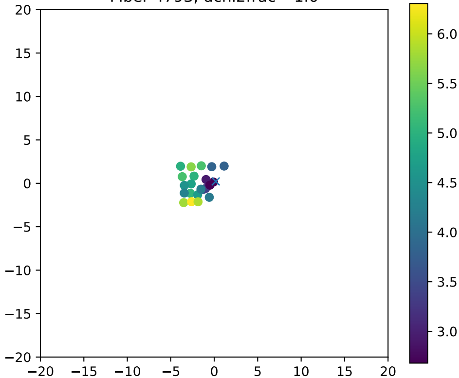
Fiber 4793, dchi2frac= 1.0
