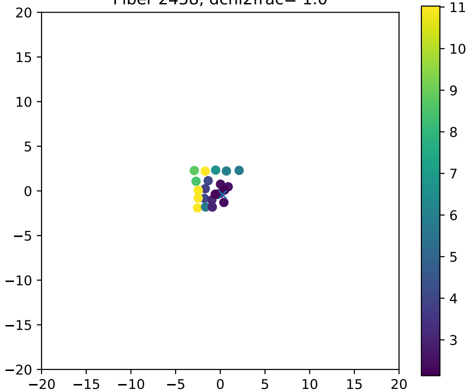
Fiber 2438, dchi2frac= 1.0
