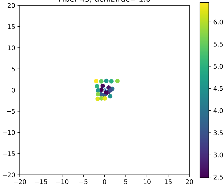
Fiber 43, dchi2frac= 1.0
