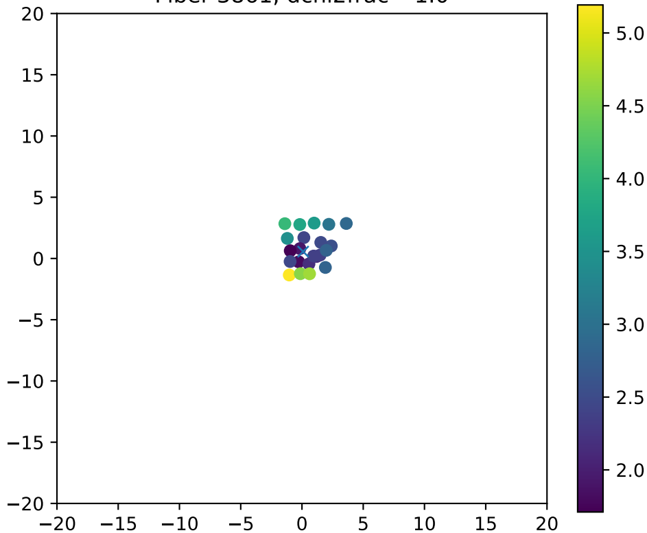
Fiber 3861, dchi2frac= 1.0
