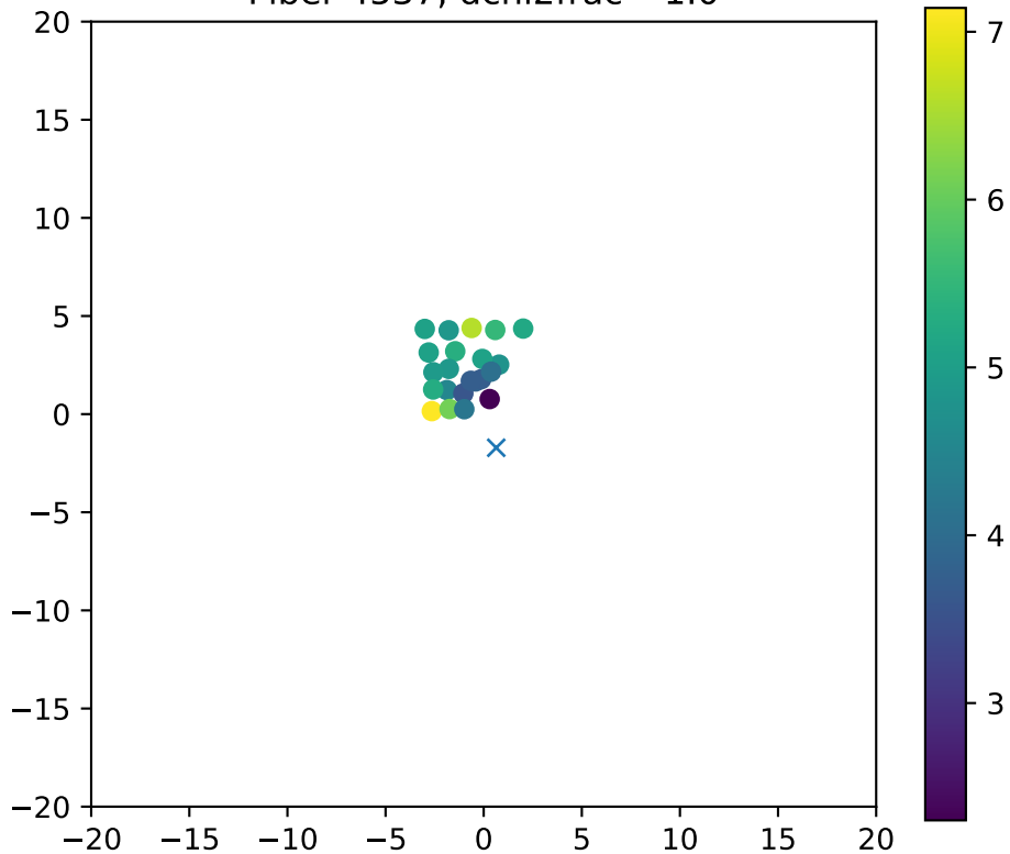
Fiber 4537, dchi2frac= 1.0
