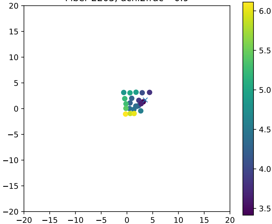
Fiber 2203, dchi2frac= 0.9
