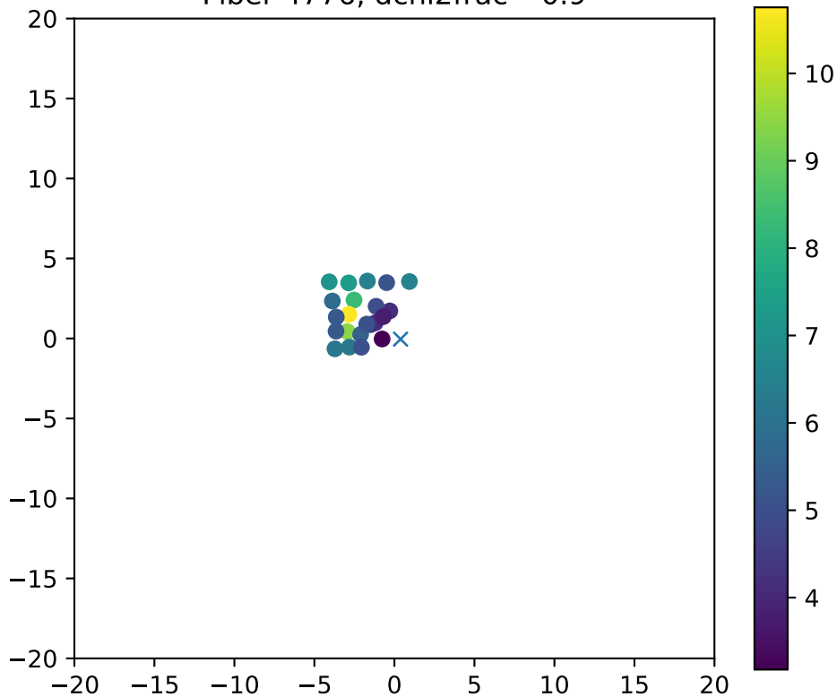
Fiber 4776, dchi2frac= 0.9
