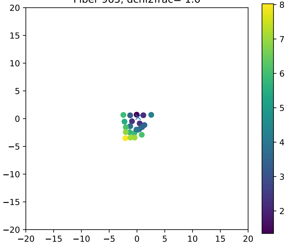
Fiber 965, dchi2frac= 1.0
