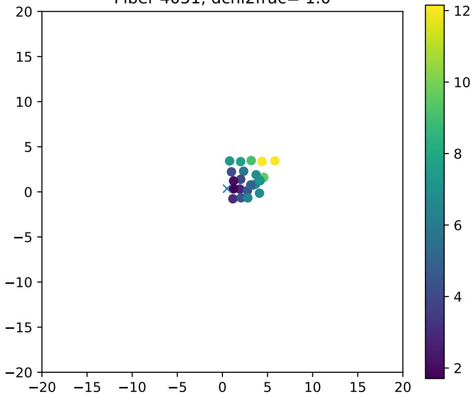
Fiber 4051, dchi2frac= 1.0
