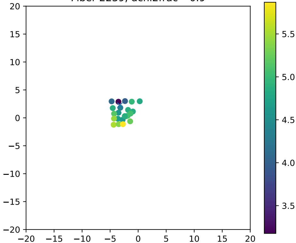
Fiber 2239, dchi2frac= 0.9
