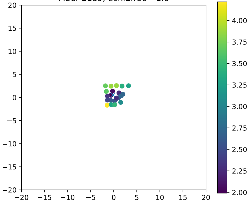
Fiber 2189, dchi2frac= 1.0
