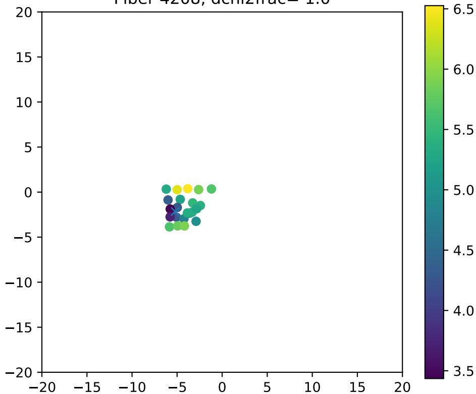
Fiber 4208, dchi2frac= 1.0
