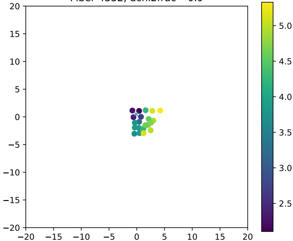
Fiber 4332, dchi2frac= 0.9
