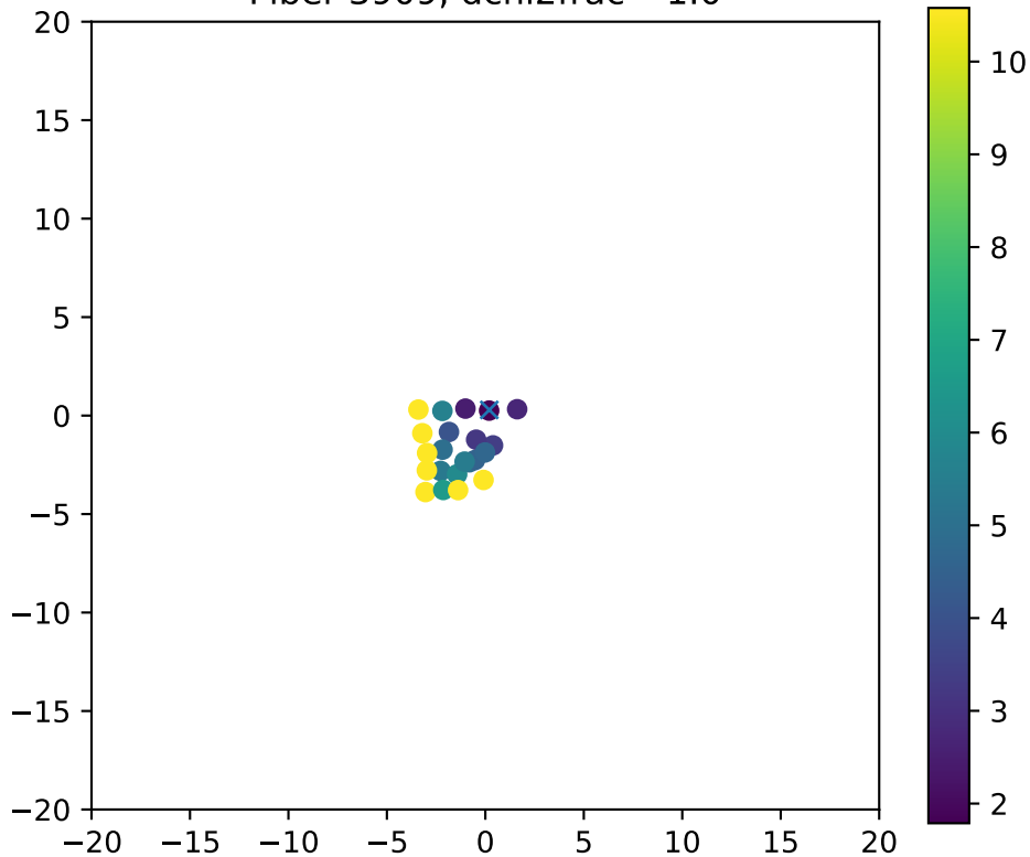
Fiber 3909, dchi2frac= 1.0
