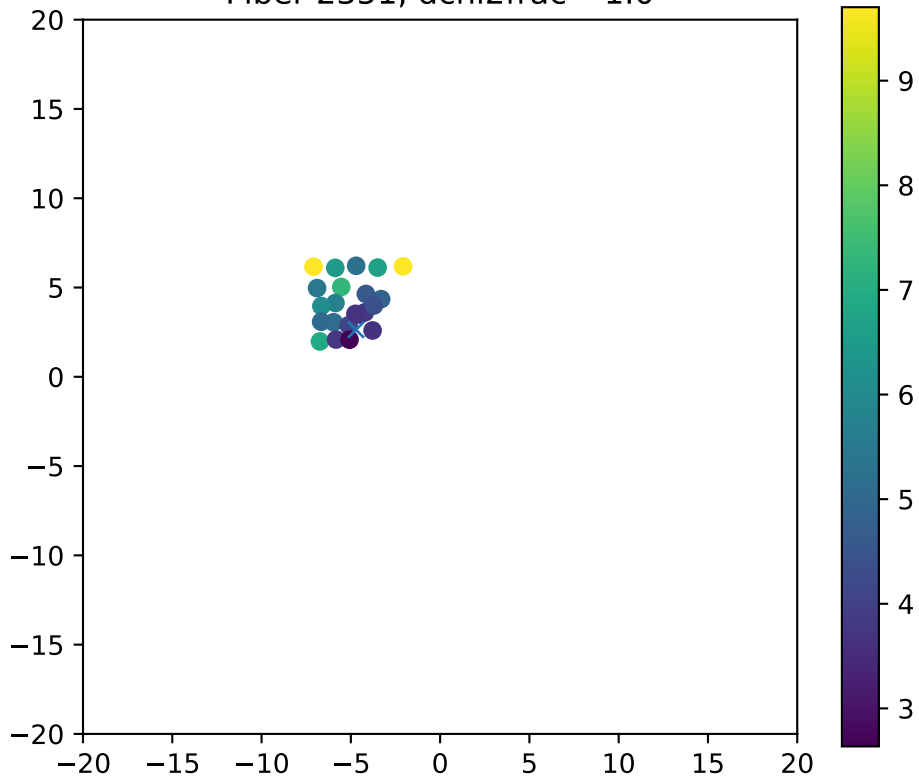
Fiber 2351, dchi2frac= 1.0
