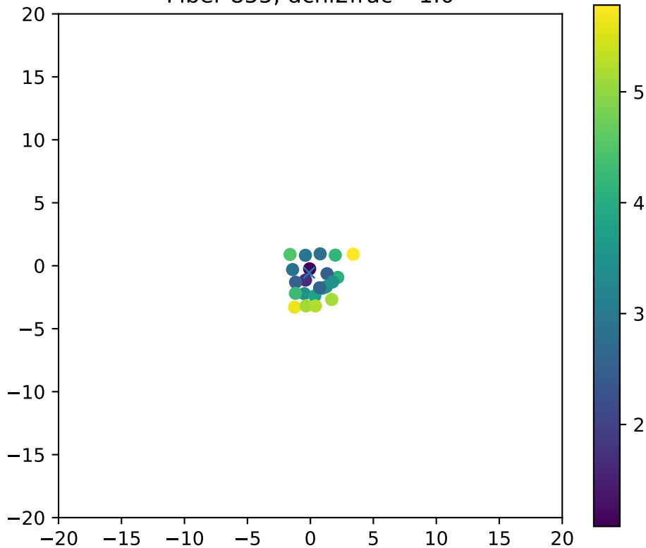
Fiber 855, dchi2frac= 1.0
