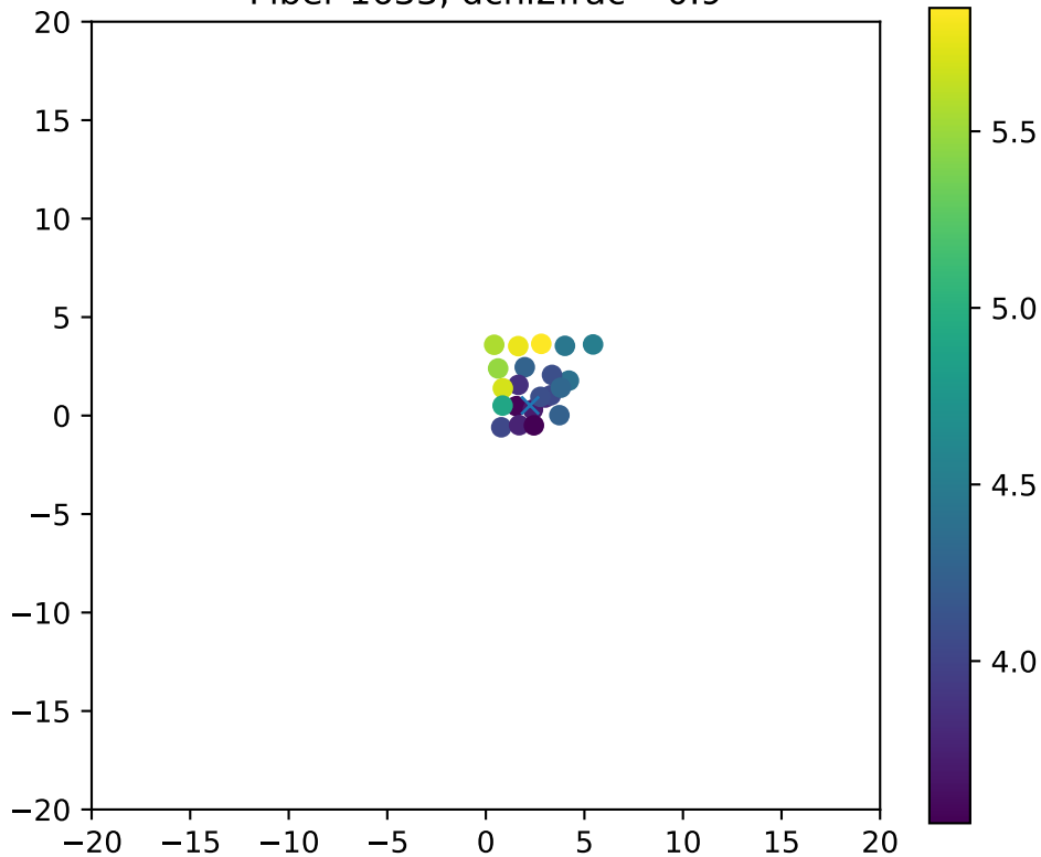
Fiber 1633, dchi2frac= 0.9
