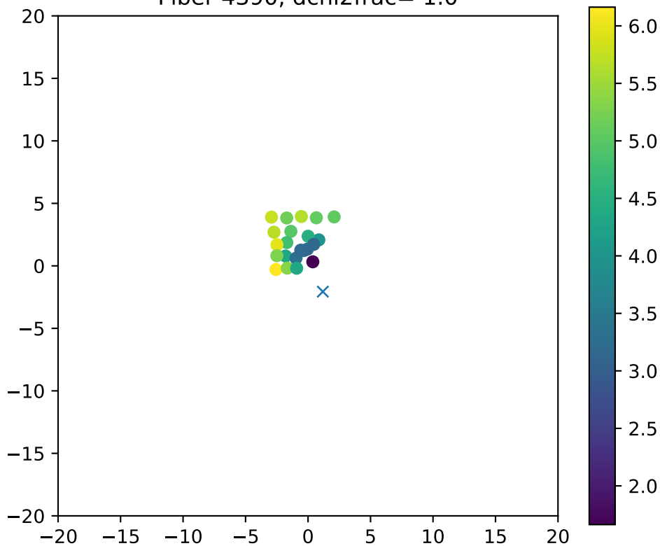
Fiber 4390, dchi2frac= 1.0
