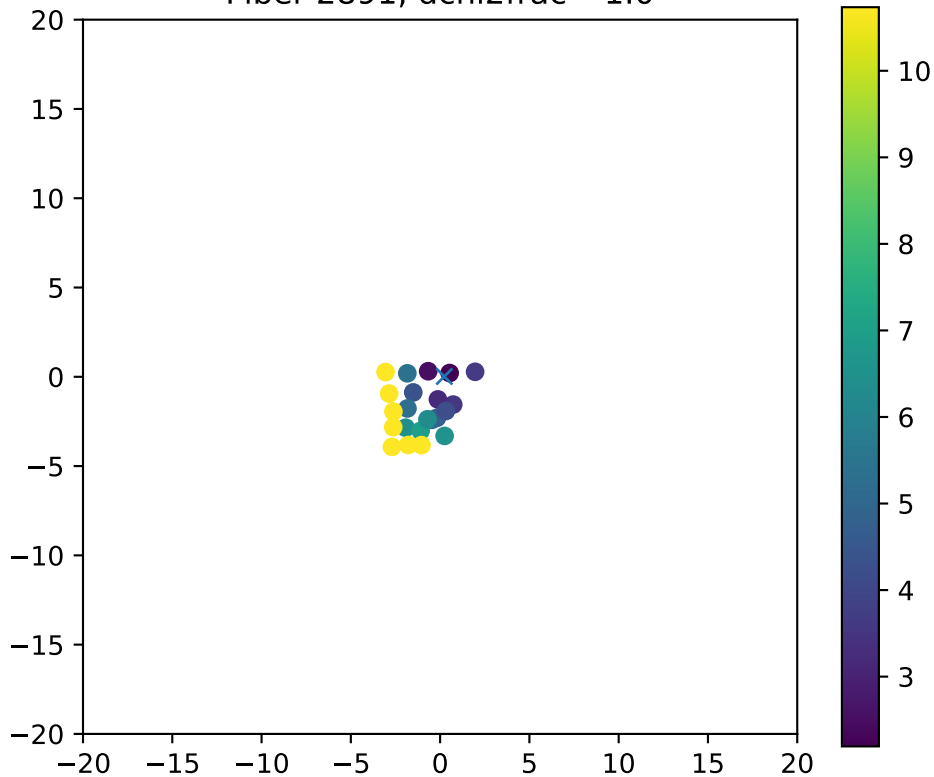
Fiber 2891, dchi2frac= 1.0
