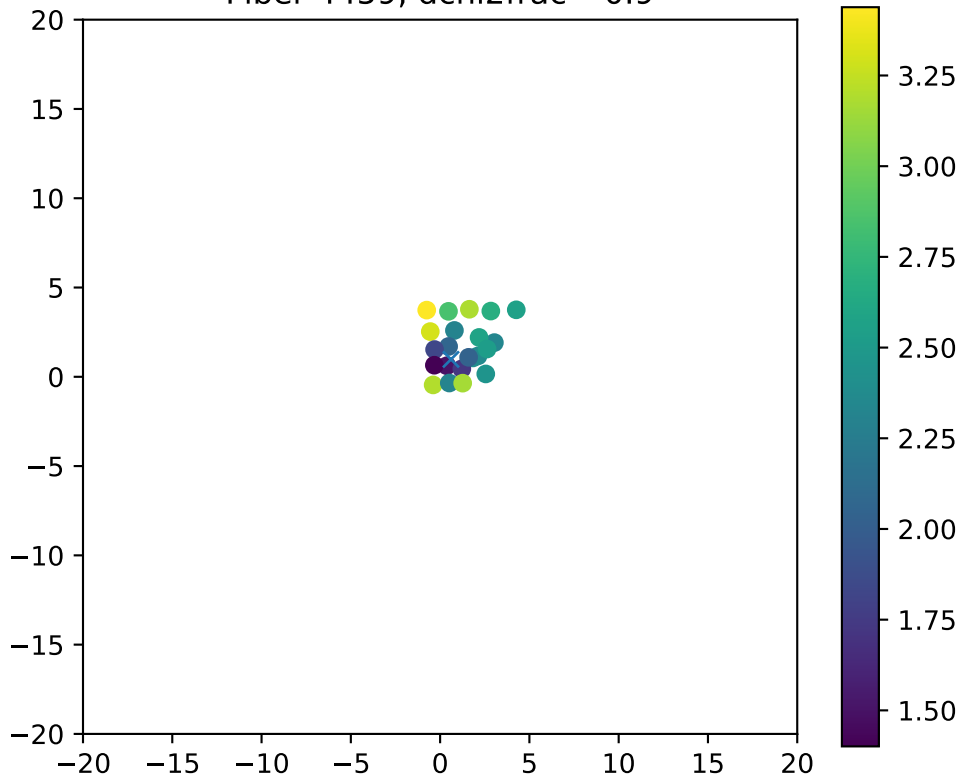
Fiber 4459, dchi2frac= 0.9
