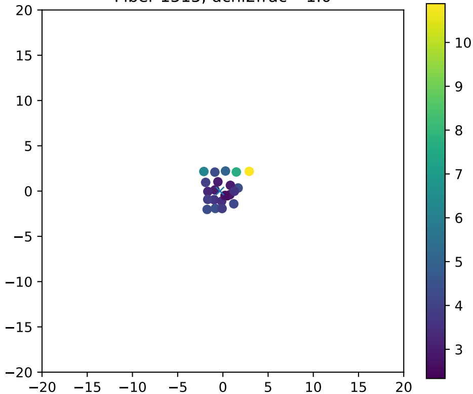
Fiber 1515, dchi2frac= 1.0
