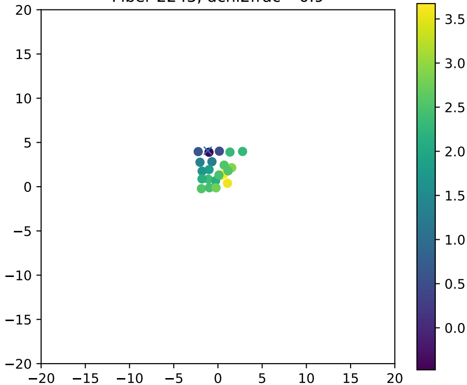
Fiber 2243, dchi2frac= 0.9
