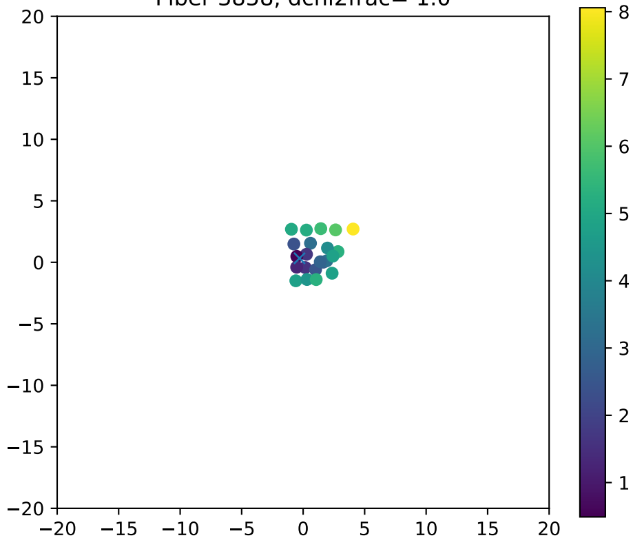
Fiber 3858, dchi2frac= 1.0
