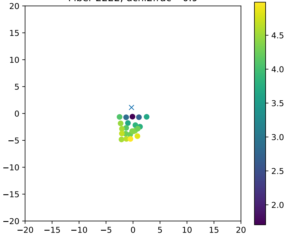
Fiber 2222, dchi2frac= 0.9
