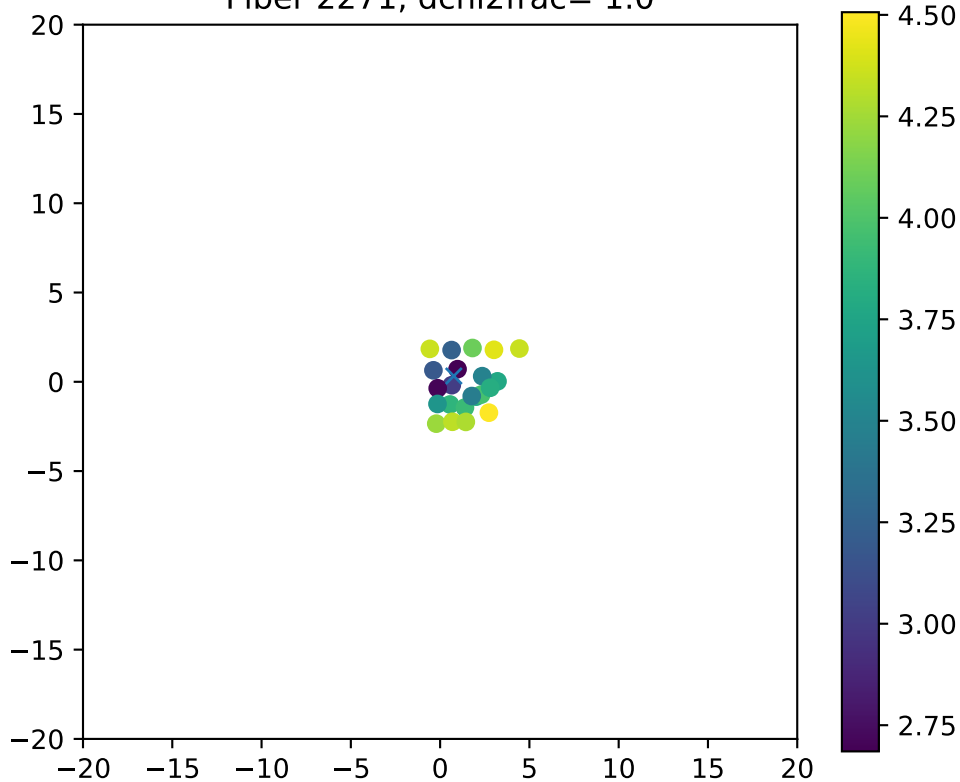
Fiber 2271, dchi2frac= 1.0
