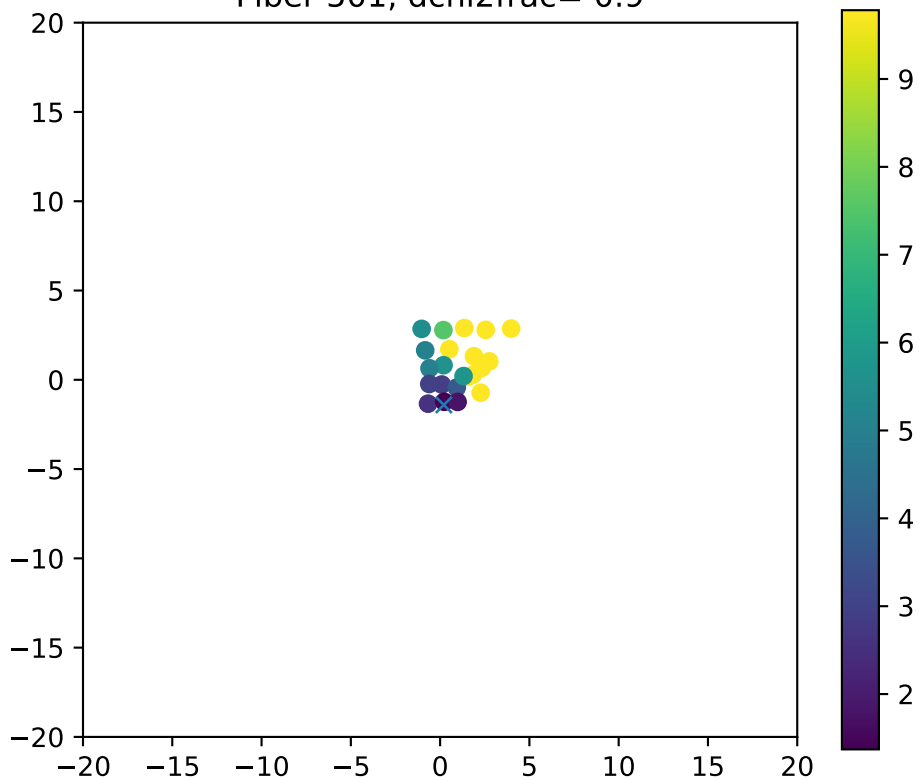
Fiber 501, dchi2frac= 0.9
