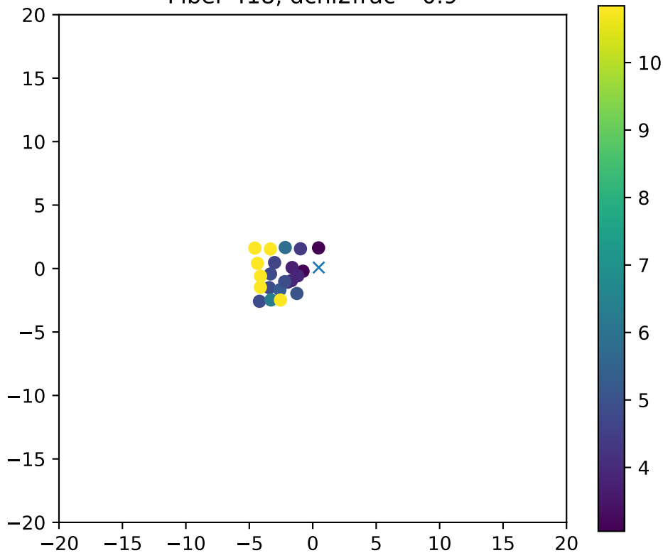
Fiber 418, dchi2frac= 0.9
