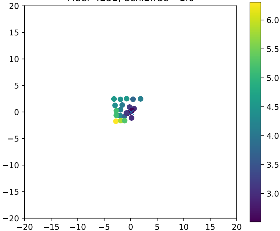
Fiber 4251, dchi2frac= 1.0
