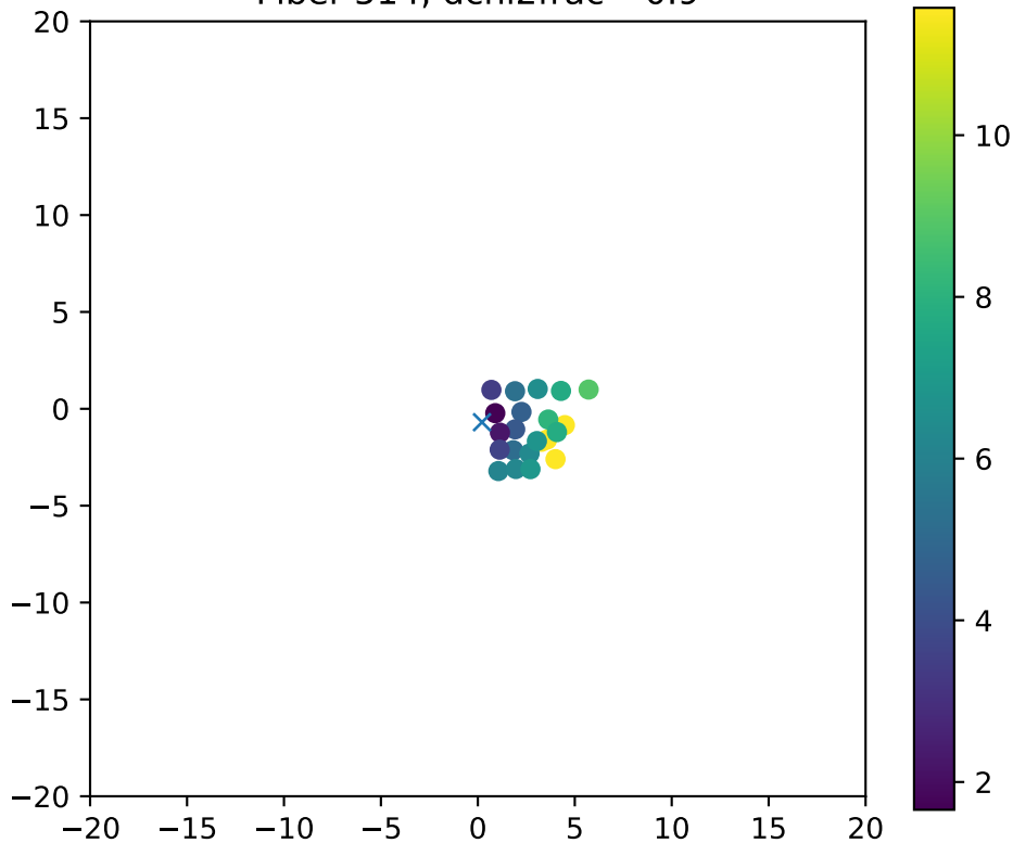
Fiber 514, dchi2frac= 0.9
