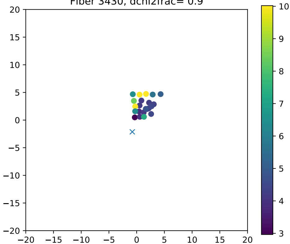
Fiber 3430, dchi2frac= 0.9
