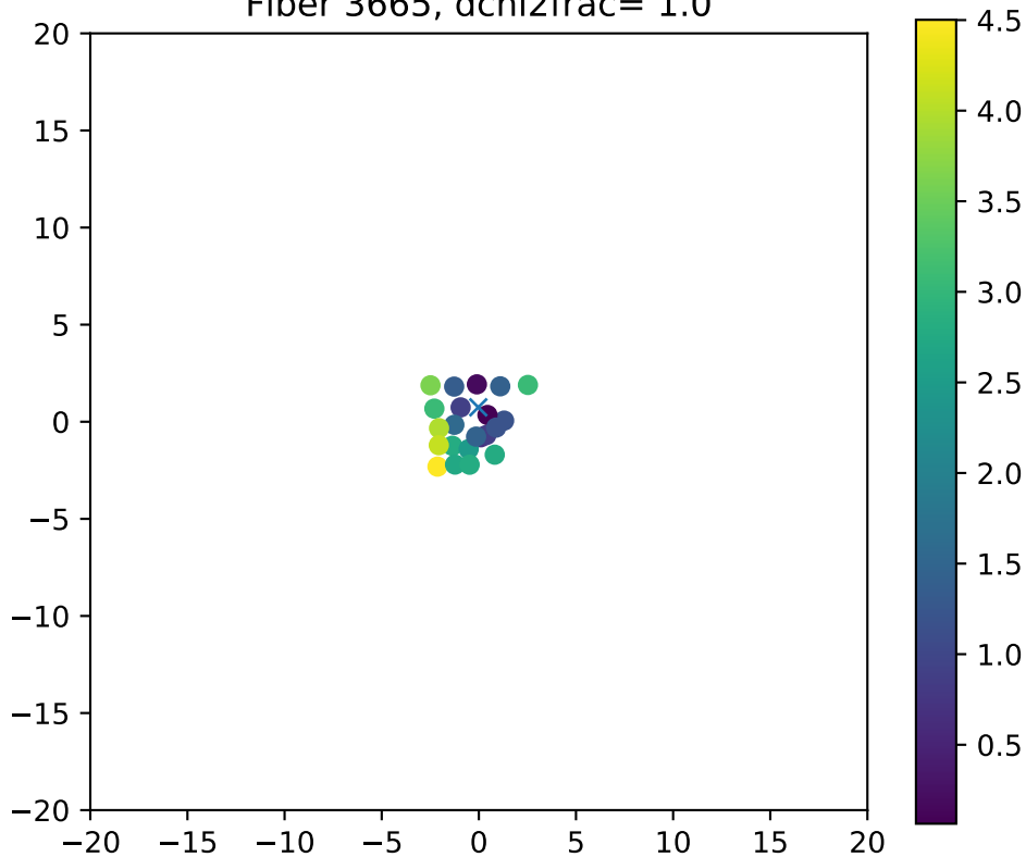
Fiber 3665, dchi2frac= 1.0
