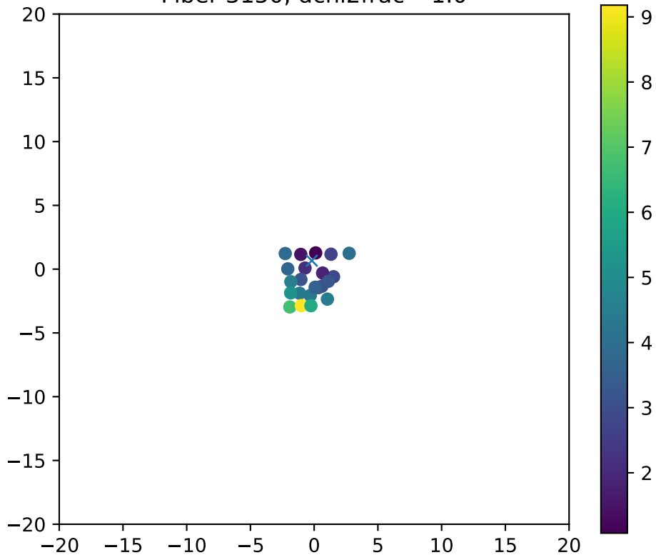
Fiber 3150, dchi2frac= 1.0
