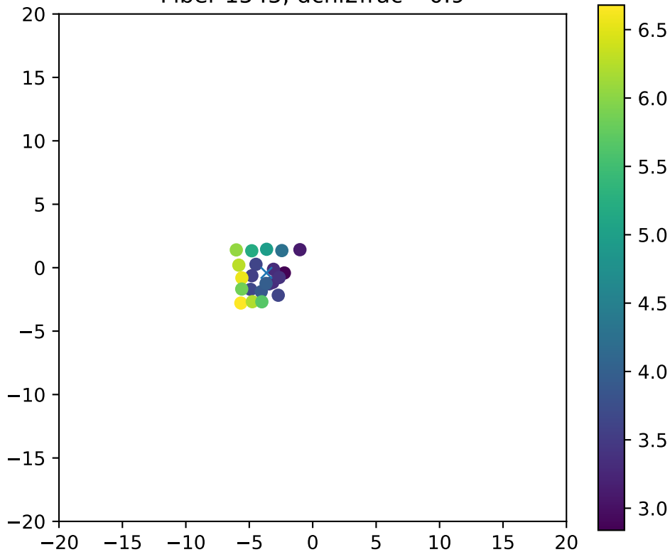
Fiber 1545, dchi2frac= 0.9
