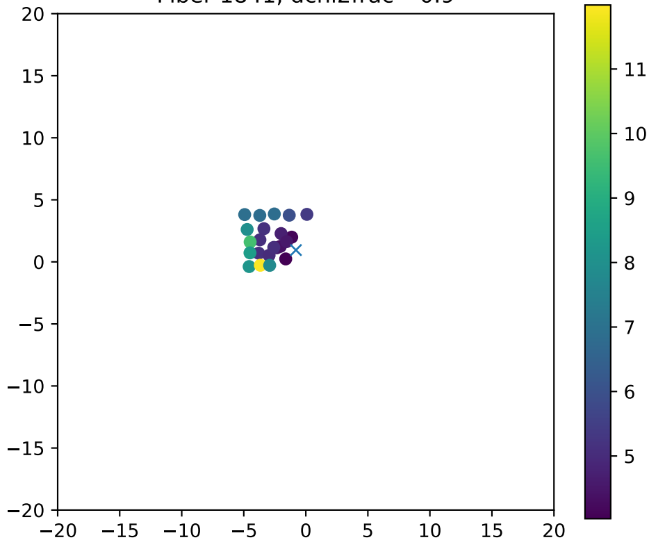
Fiber 1841, dchi2frac= 0.9
