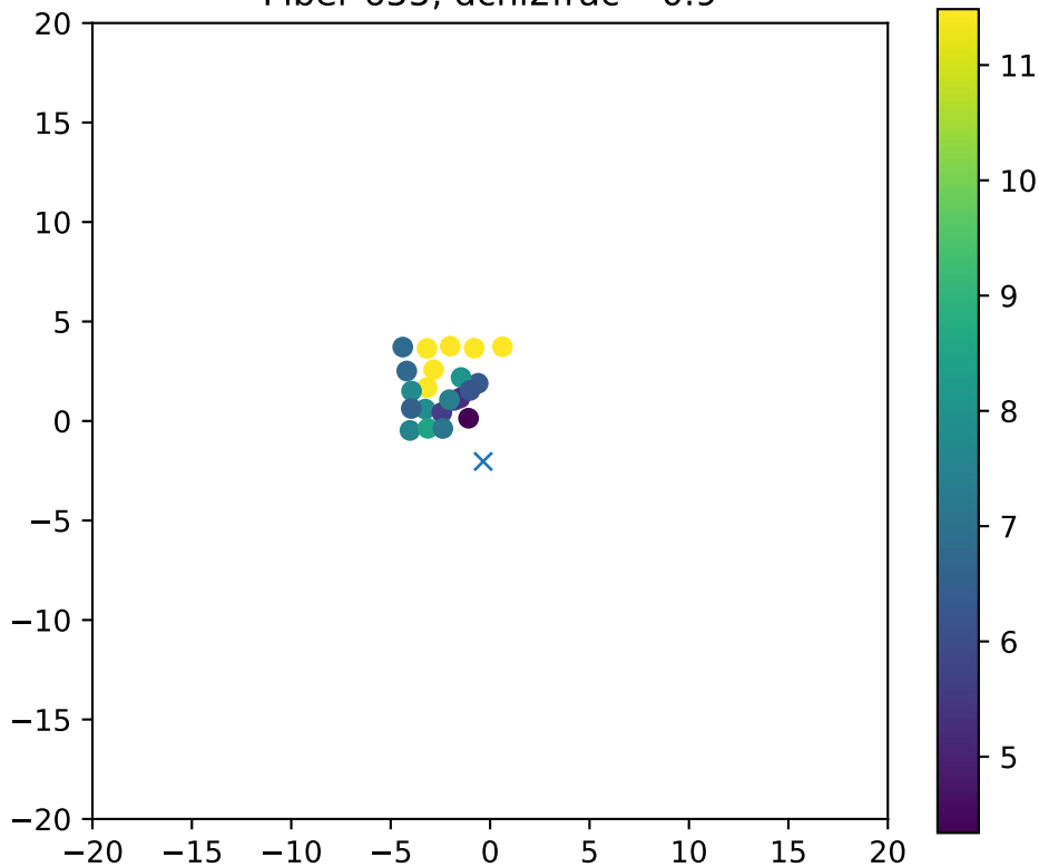
Fiber 655, dchi2frac= 0.9
