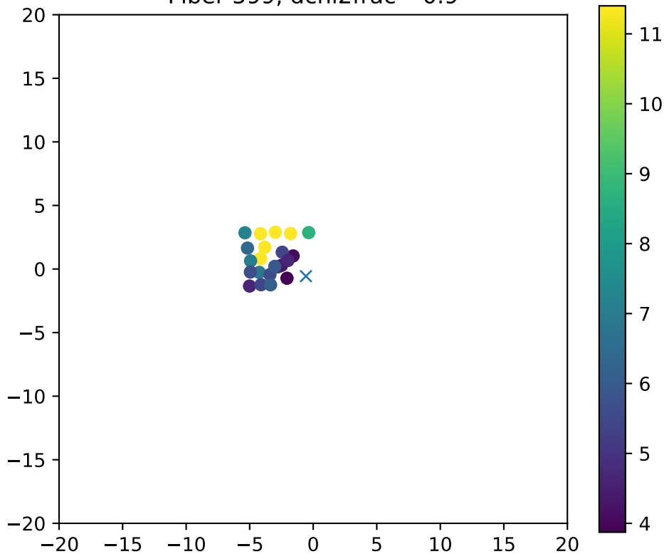
Fiber 599, dchi2frac= 0.9
