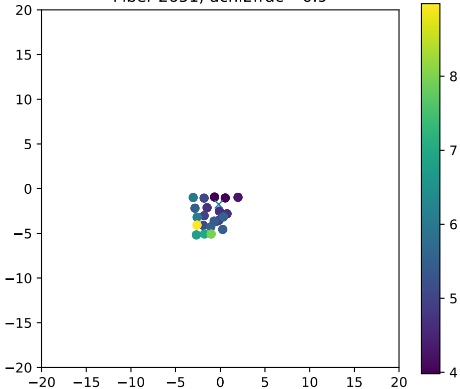
Fiber 2651, dchi2frac= 0.9
