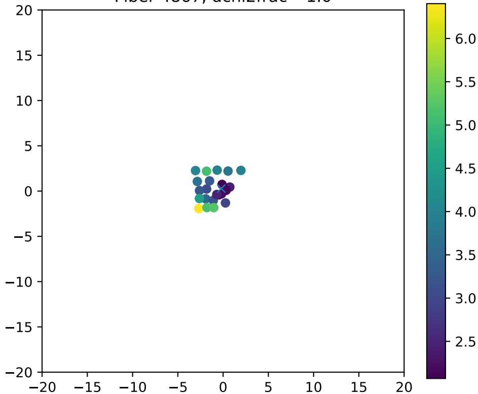
Fiber 4867, dchi2frac= 1.0
