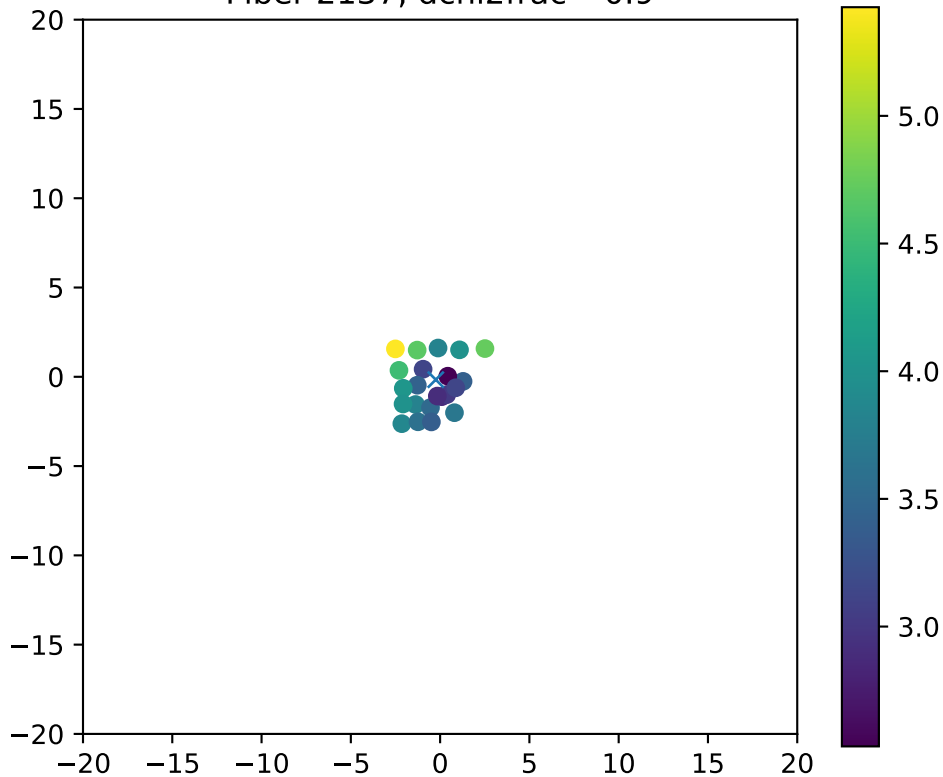
Fiber 2137, dchi2frac= 0.9
