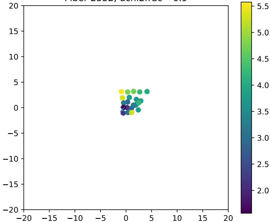
Fiber 2552, dchi2frac= 0.9
