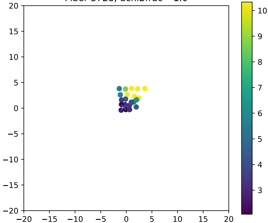
Fiber 3728, dchi2frac= 1.0
