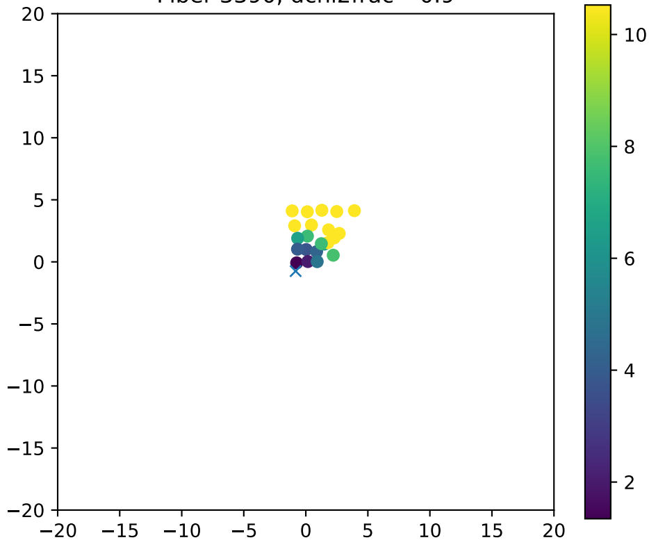
Fiber 3390, dchi2frac= 0.9
