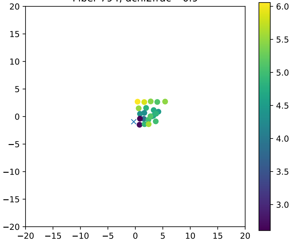
Fiber 794, dchi2frac= 0.9
