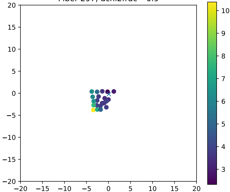
Fiber 297, dchi2frac= 0.9
