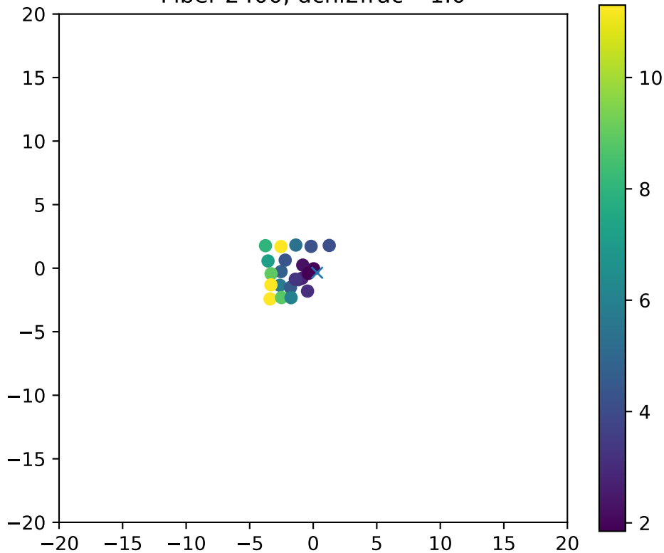
Fiber 2400, dchi2frac= 1.0
