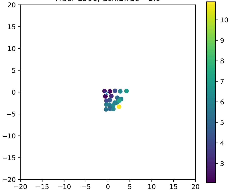
Fiber 1906, dchi2frac= 1.0
