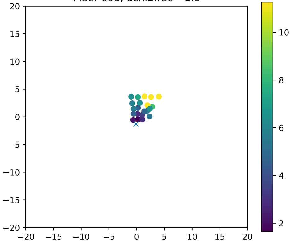
Fiber 695, dchi2frac= 1.0
