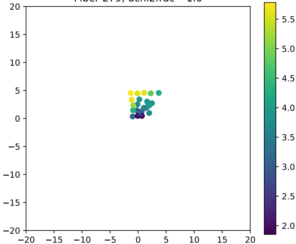
Fiber 279, dchi2frac= 1.0
