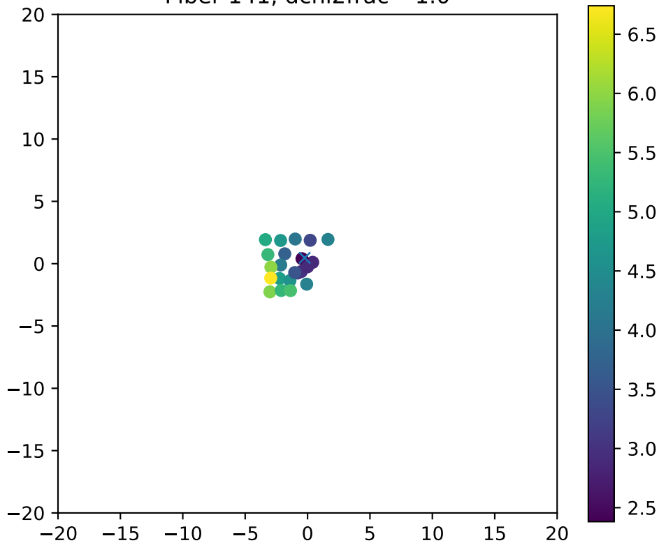
Fiber 141, dchi2frac= 1.0
