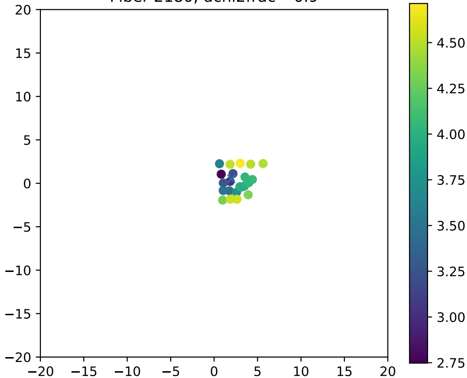
Fiber 2180, dchi2frac= 0.9
