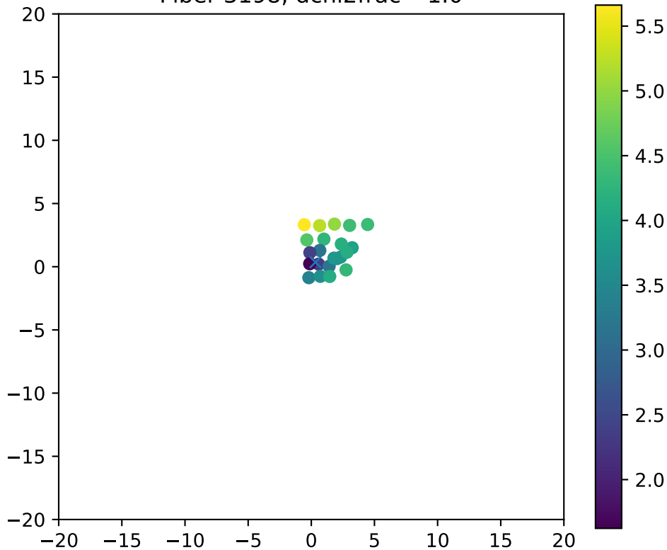
Fiber 3198, dchi2frac= 1.0
