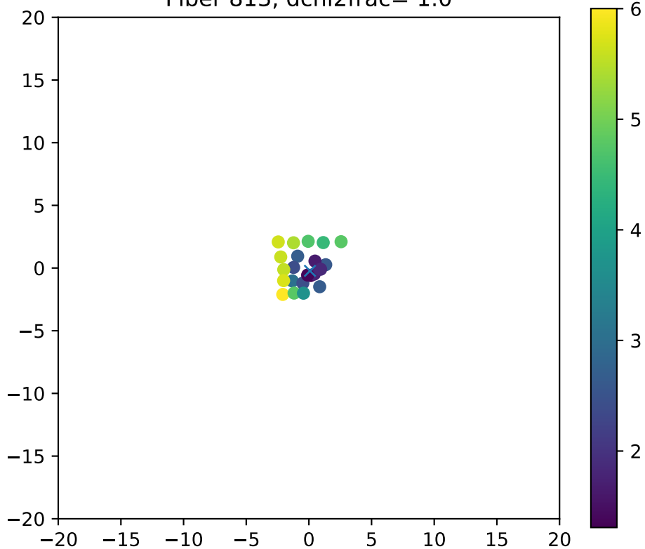
Fiber 813, dchi2frac= 1.0
