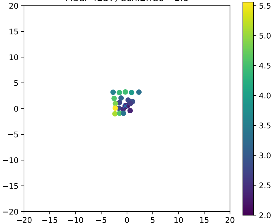
Fiber 4237, dchi2frac= 1.0
