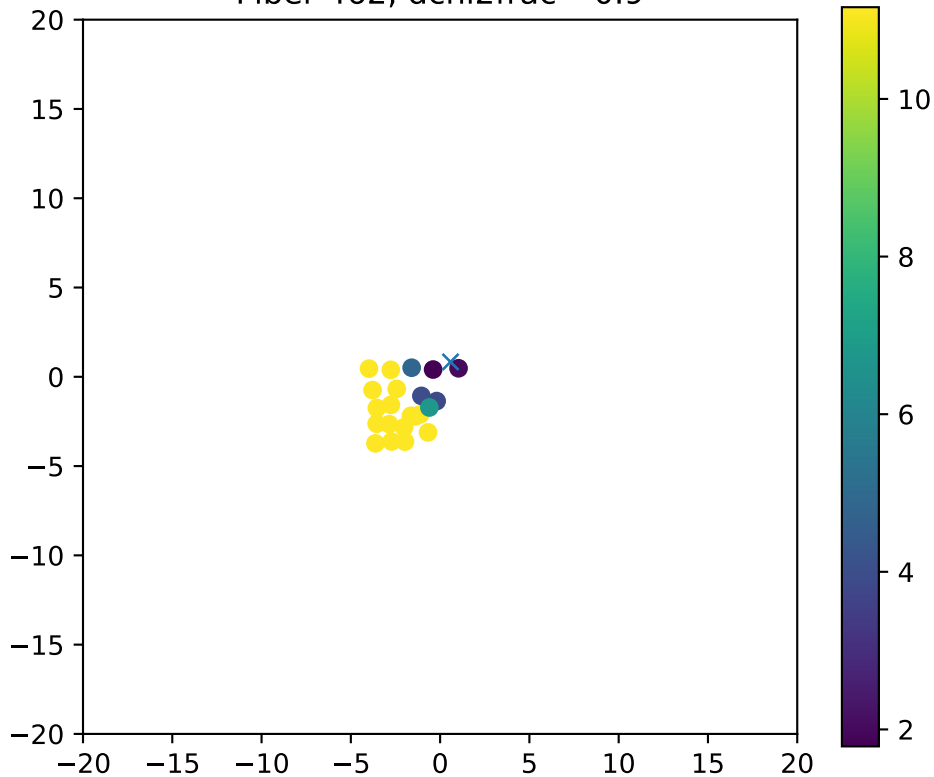
Fiber 462, dchi2frac= 0.9
