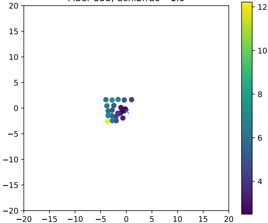
Fiber 353, dchi2frac= 1.0
