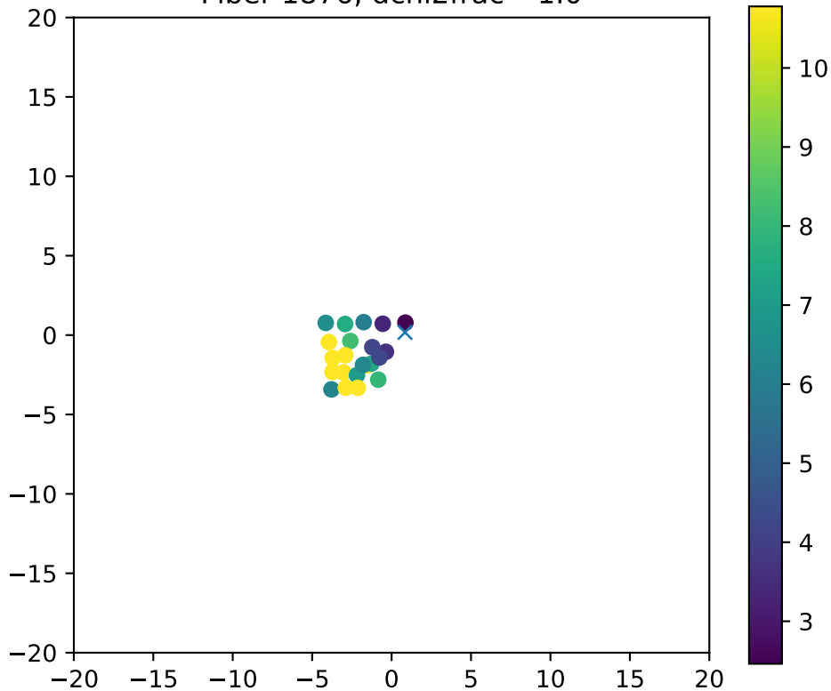
Fiber 1876, dchi2frac= 1.0
