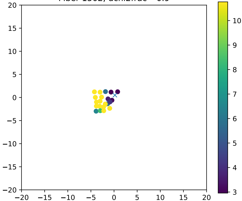
Fiber 1502, dchi2frac= 0.9
