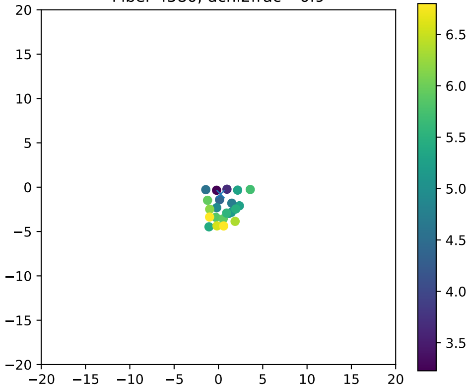
Fiber 4580, dchi2frac= 0.9
