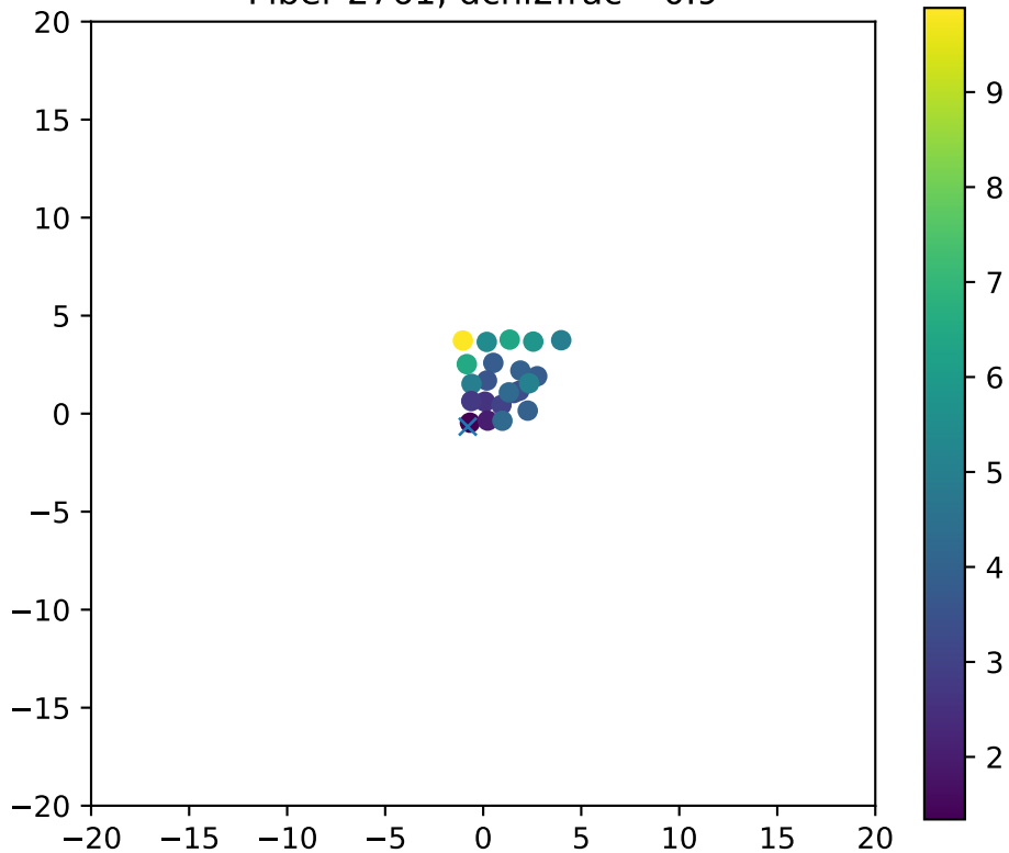
Fiber 2761, dchi2frac= 0.9
