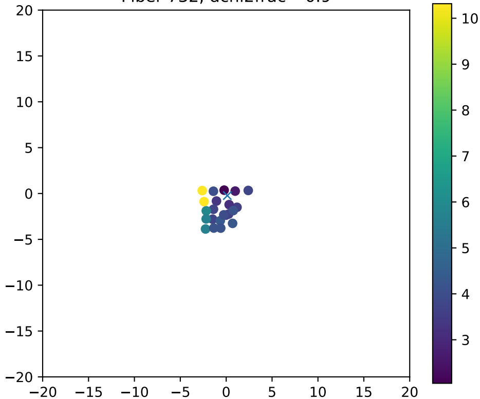
Fiber 732, dchi2frac= 0.9
