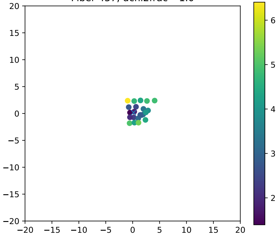
Fiber 437, dchi2frac= 1.0
