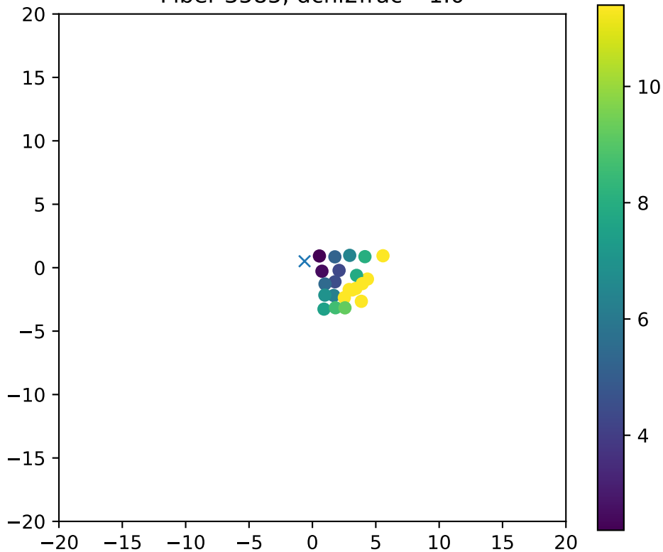
Fiber 3585, dchi2frac= 1.0
