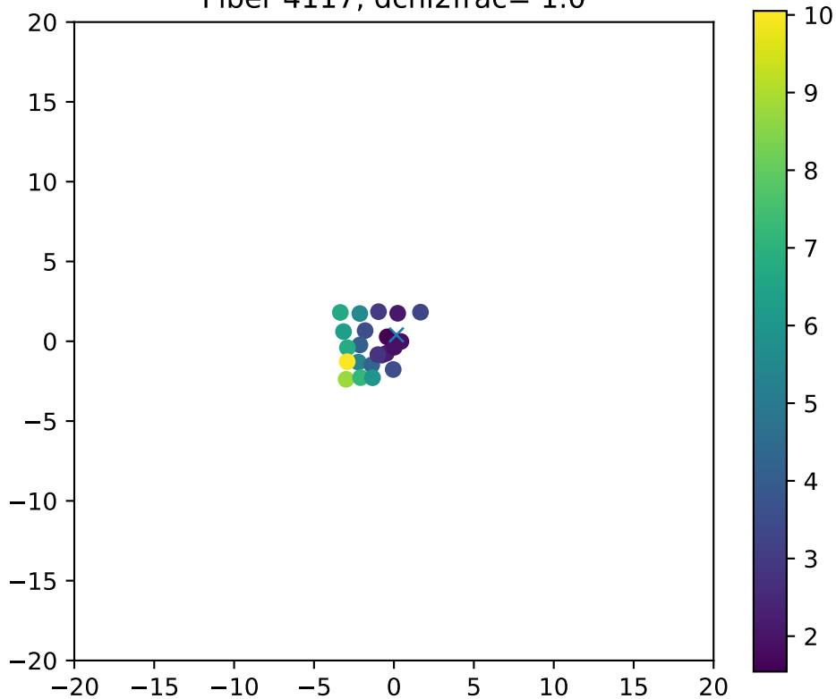
Fiber 4117, dchi2frac= 1.0
