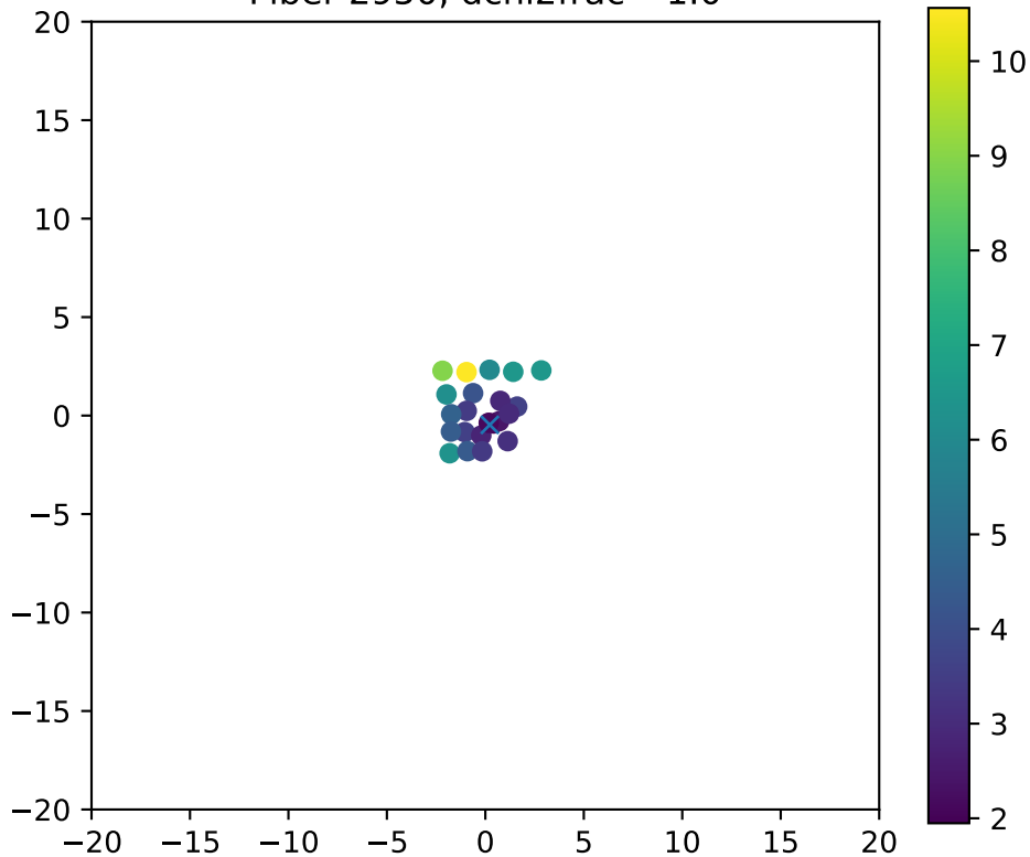
Fiber 2950, dchi2frac= 1.0
