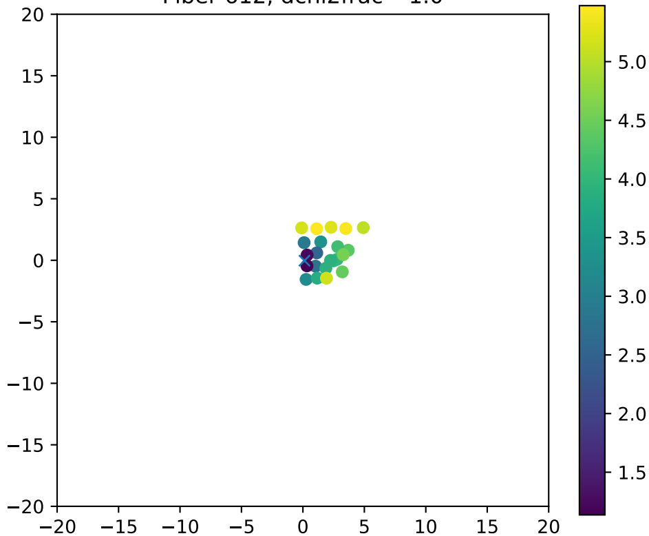
Fiber 612, dchi2frac= 1.0
