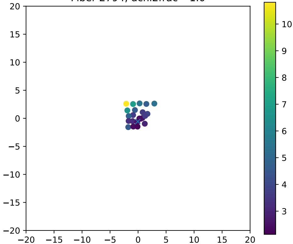
Fiber 2794, dchi2frac= 1.0
