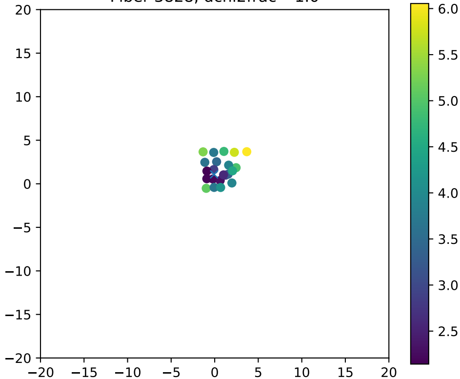
Fiber 3828, dchi2frac= 1.0
