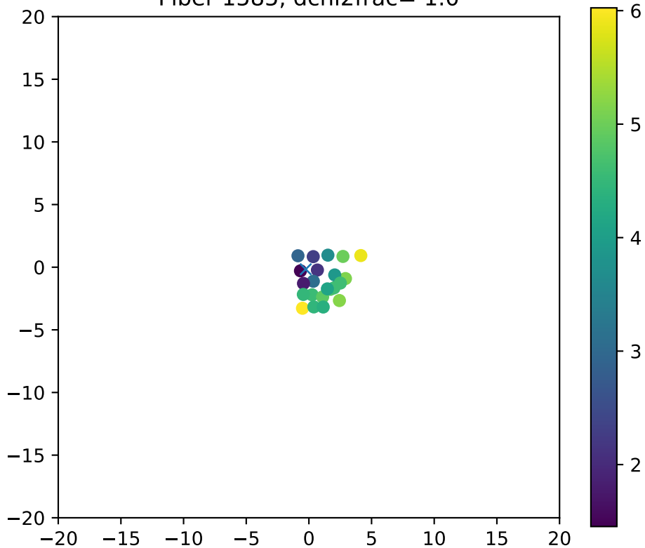
Fiber 1585, dchi2frac= 1.0
