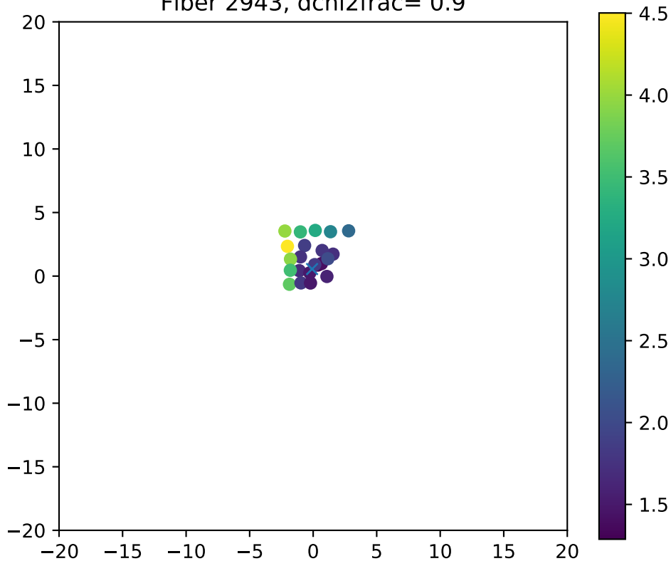
Fiber 2943, dchi2frac= 0.9
