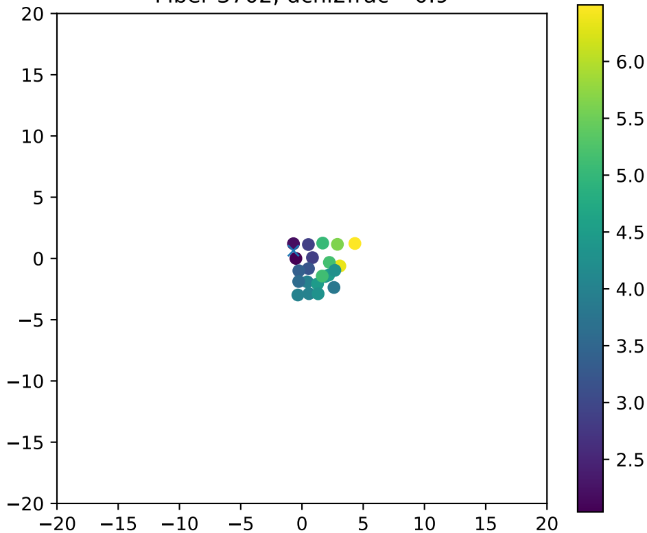
Fiber 3702, dchi2frac= 0.9
