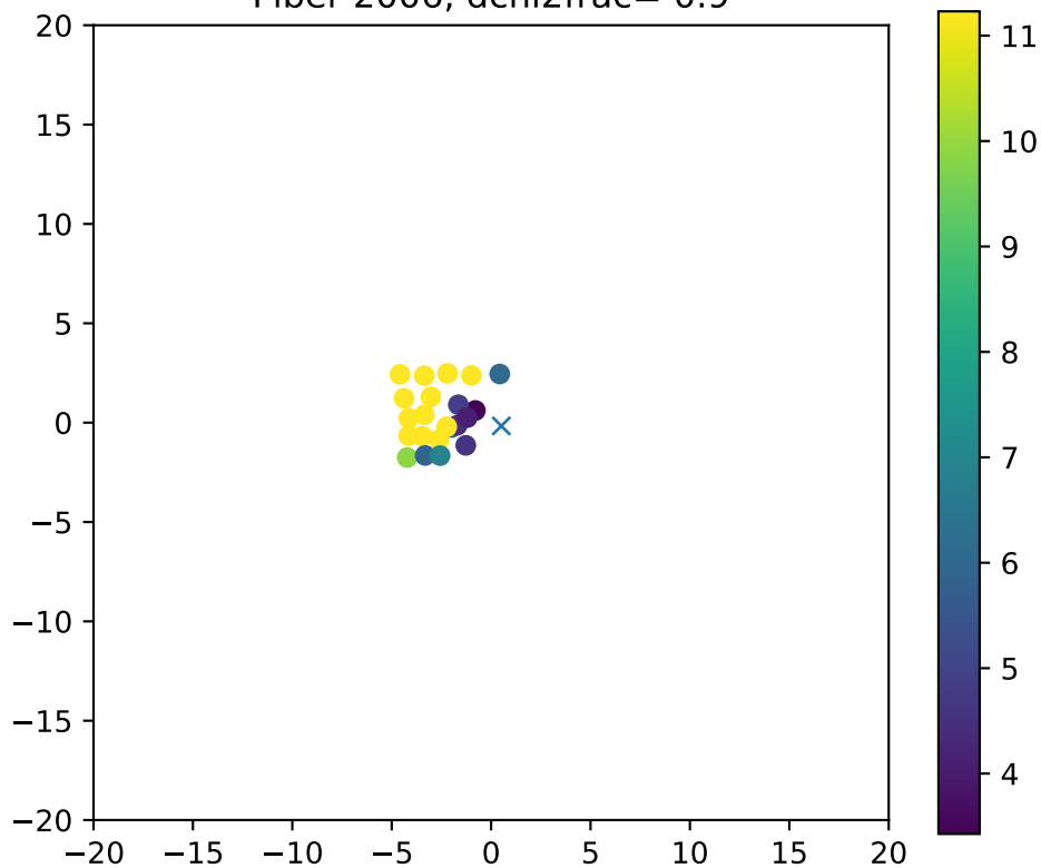
Fiber 2006, dchi2frac= 0.9
