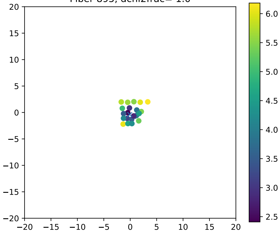
Fiber 895, dchi2frac= 1.0
