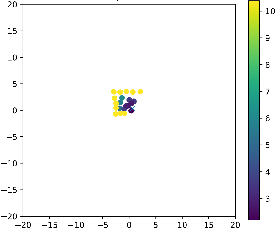
Fiber 4976, dchi2frac= 1.0
