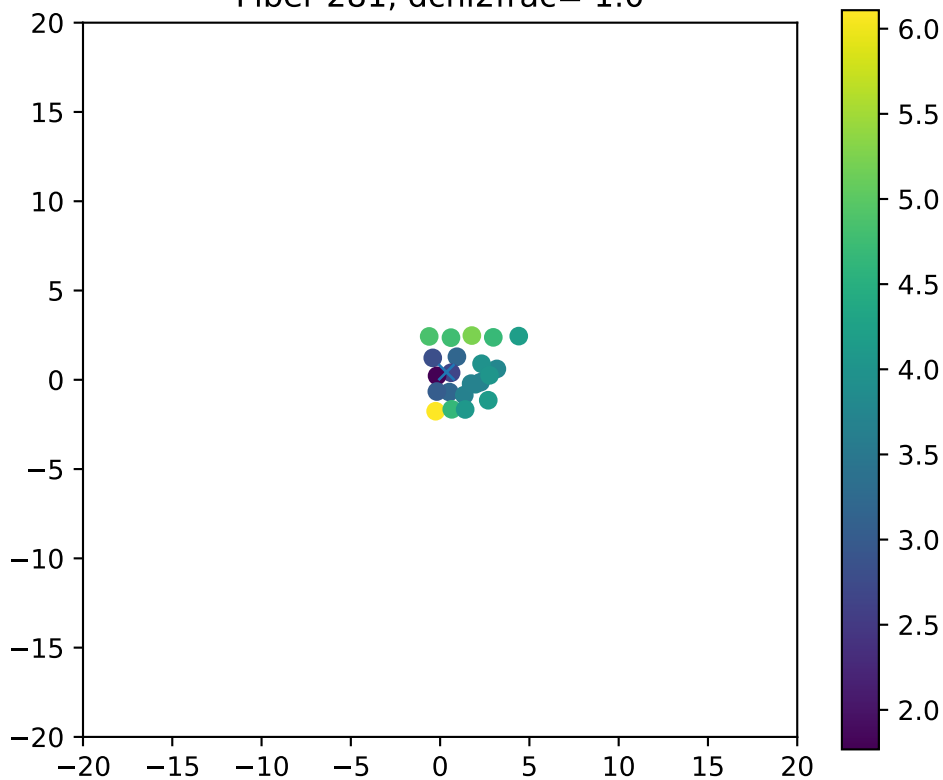
Fiber 281, dchi2frac= 1.0
