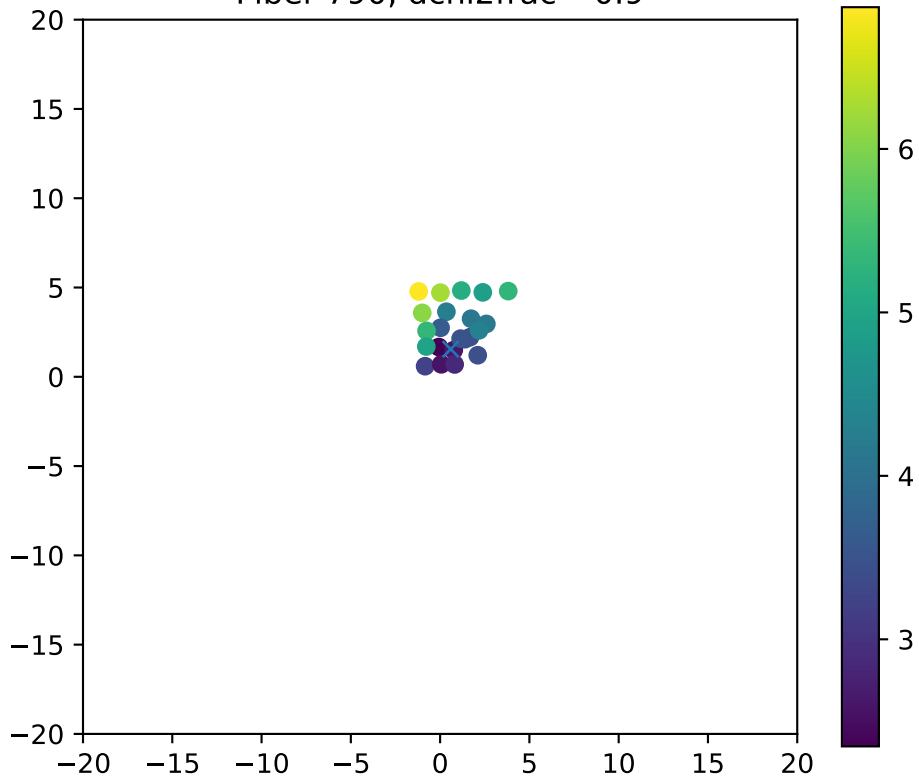
Fiber 790, dchi2frac= 0.9
