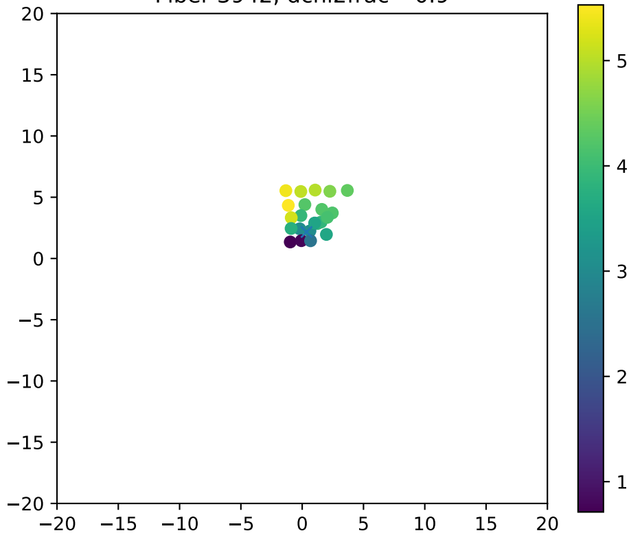
Fiber 3942, dchi2frac= 0.9
