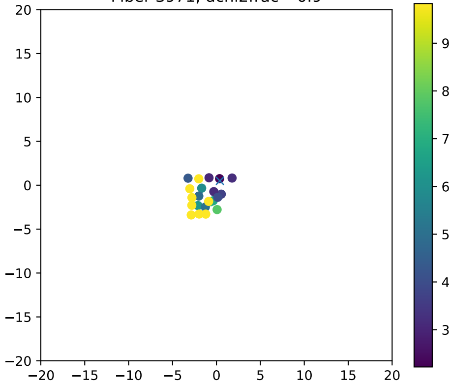
Fiber 3971, dchi2frac= 0.9
