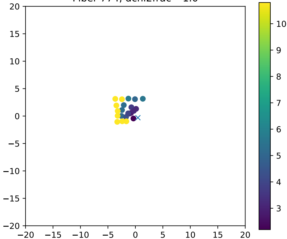
Fiber 774, dchi2frac= 1.0
