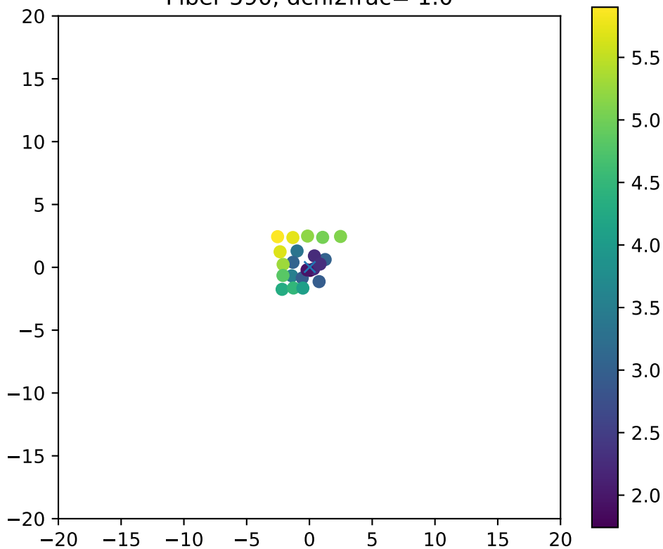
Fiber 590, dchi2frac= 1.0
