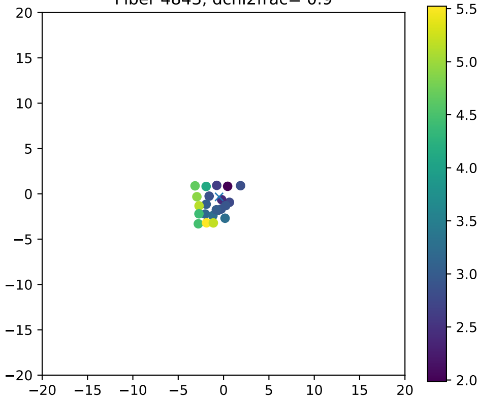
Fiber 4843, dchi2frac= 0.9
