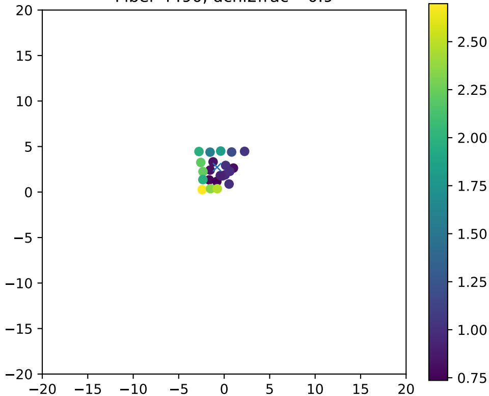
Fiber 4490, dchi2frac= 0.9
