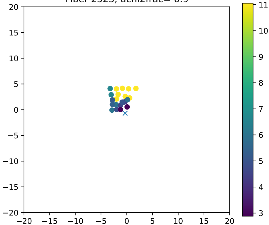
Fiber 2523, dchi2frac= 0.9
