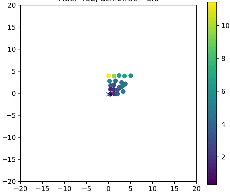
Fiber 402, dchi2frac= 1.0
