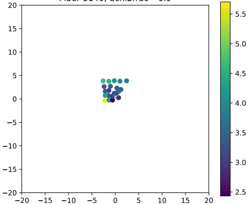
Fiber 3140, dchi2frac= 0.9
