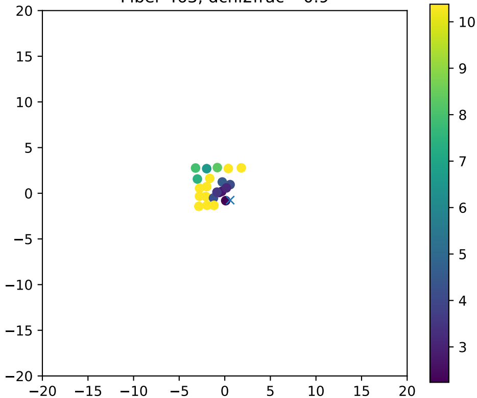
Fiber 463, dchi2frac= 0.9
