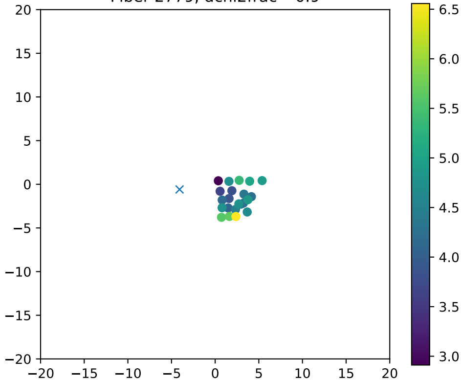
Fiber 2779, dchi2frac= 0.9
