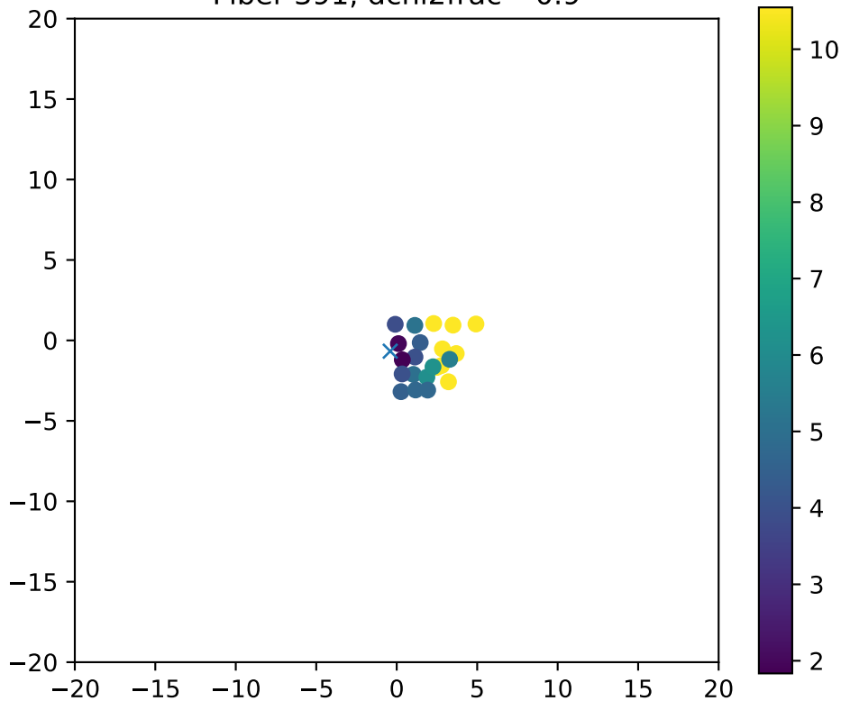
Fiber 391, dchi2frac= 0.9
