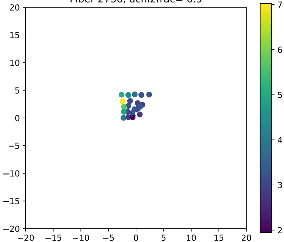
Fiber 2736, dchi2frac= 0.9
