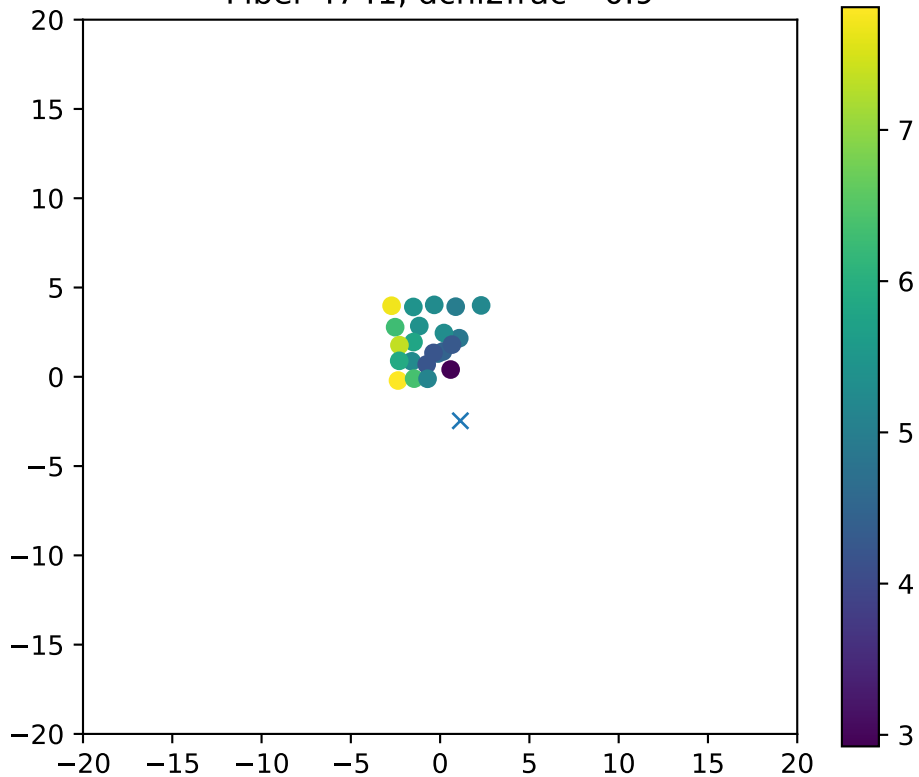
Fiber 4741, dchi2frac= 0.9
