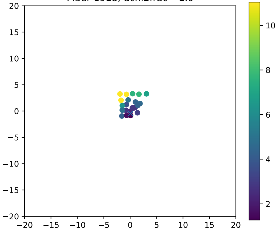
Fiber 1918, dchi2frac= 1.0
