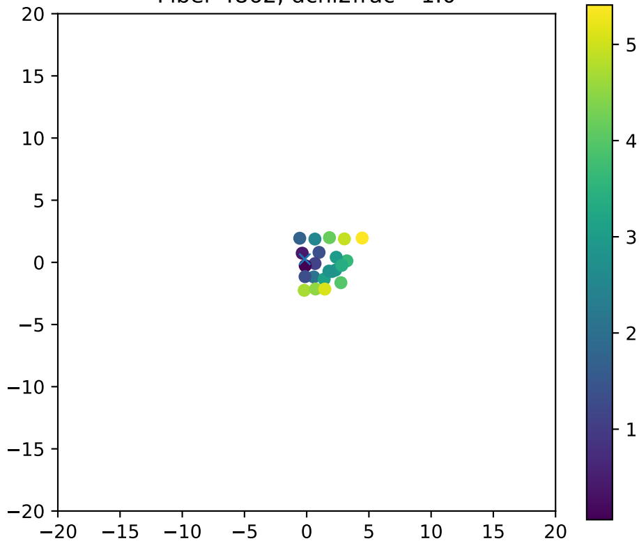
Fiber 4862, dchi2frac= 1.0
