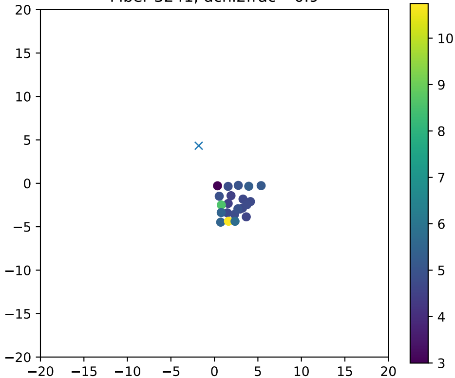
Fiber 3241, dchi2frac= 0.9
