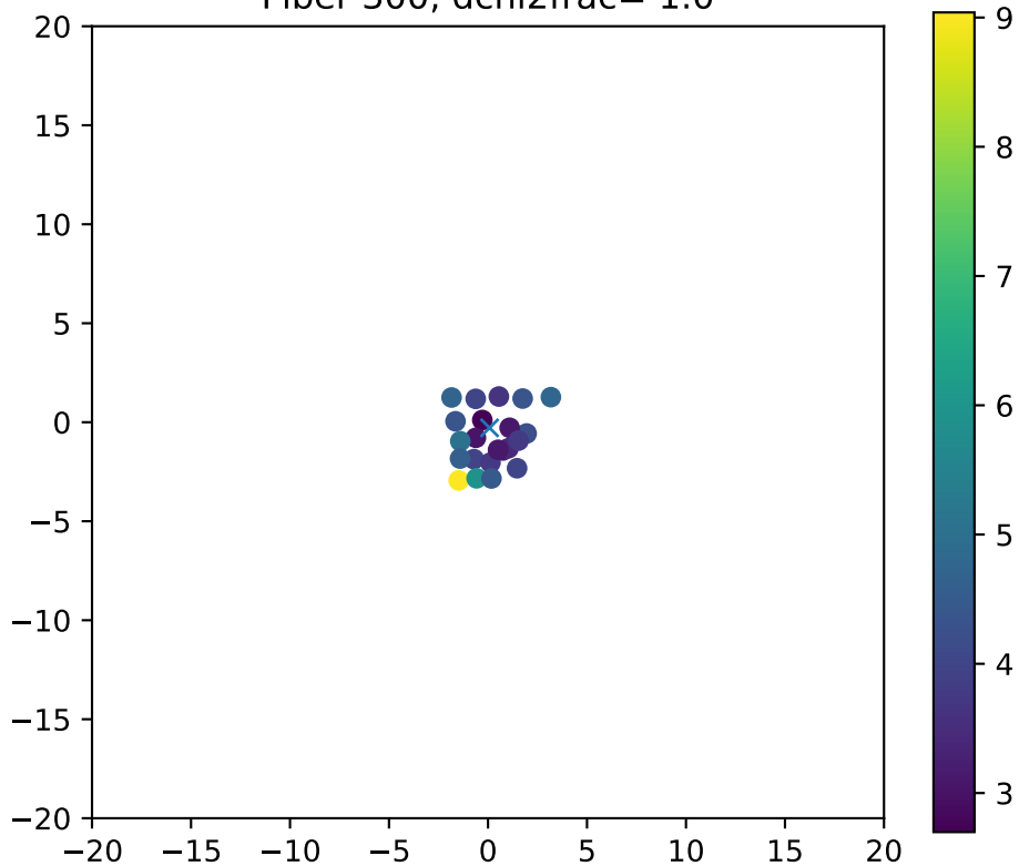
Fiber 300, dchi2frac= 1.0
