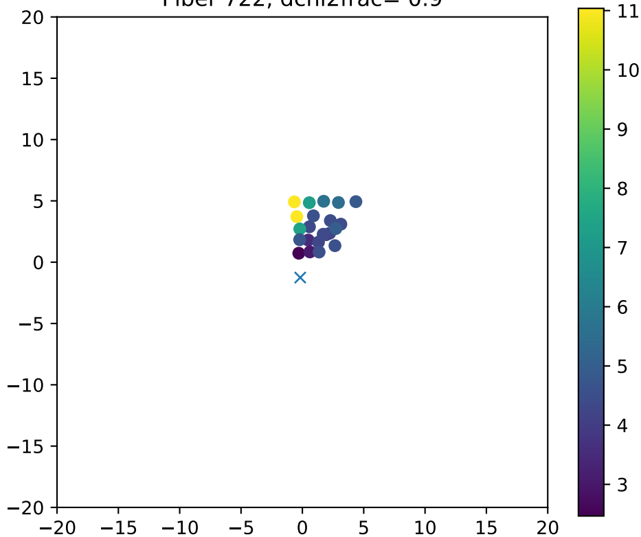
Fiber 722, dchi2frac= 0.9
