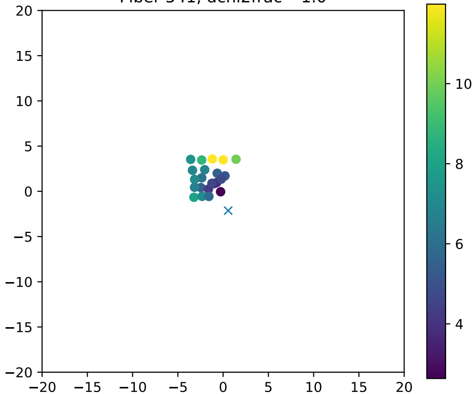
Fiber 541, dchi2frac= 1.0
