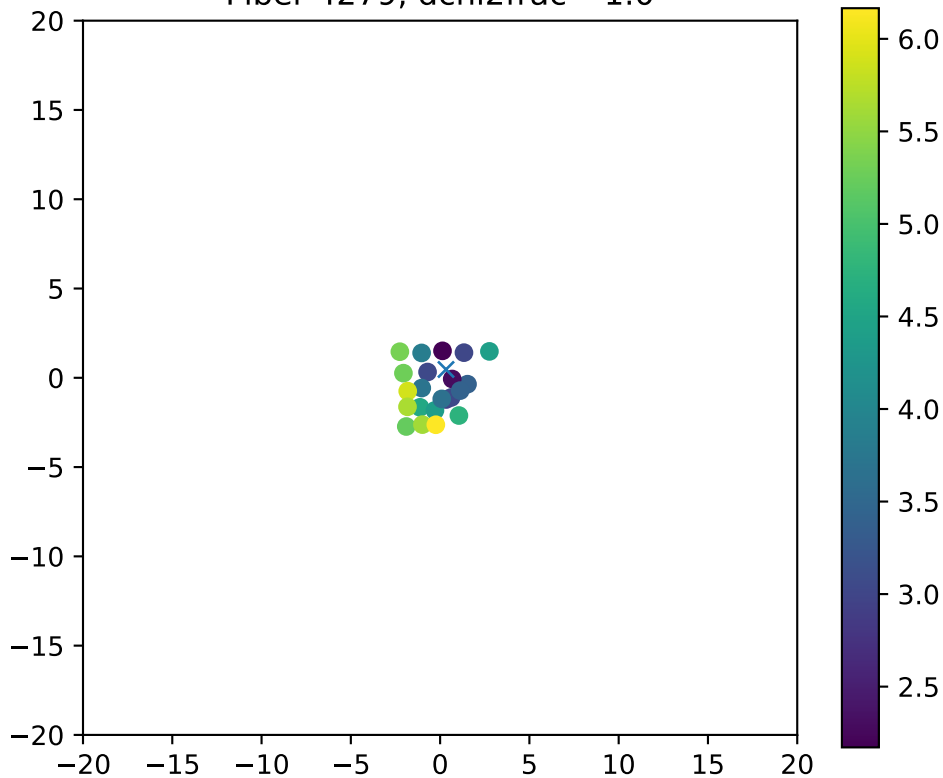
Fiber 4279, dchi2frac= 1.0
