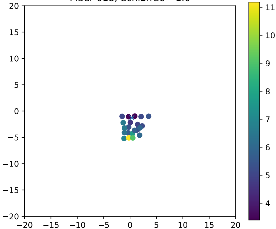
Fiber 618, dchi2frac= 1.0
