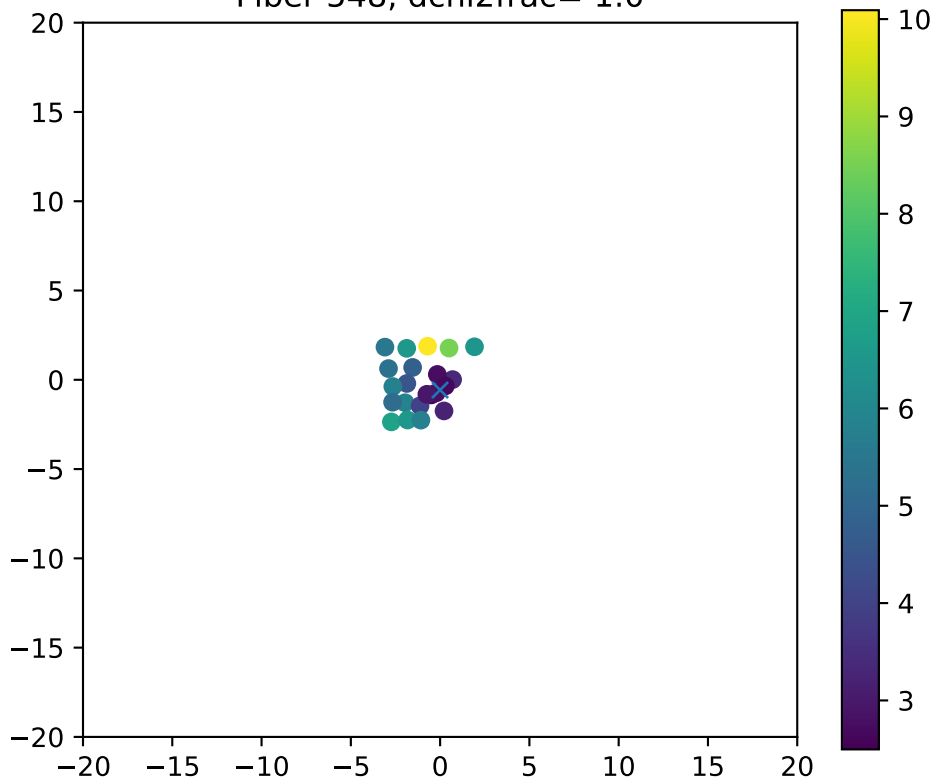
Fiber 548, dchi2frac= 1.0
