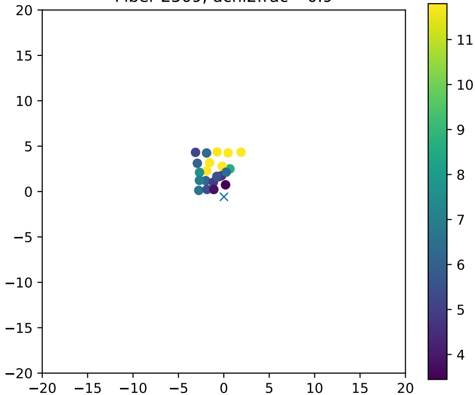
Fiber 2509, dchi2frac= 0.9
