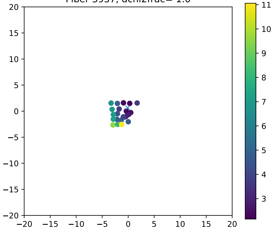
Fiber 3937, dchi2frac= 1.0
