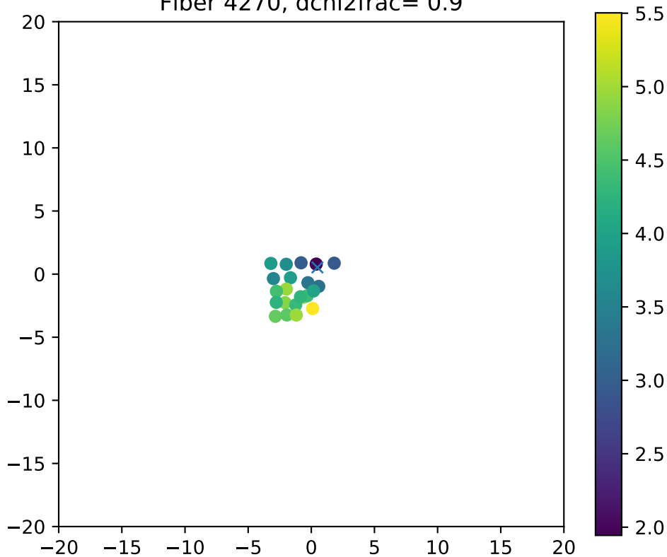
Fiber 4270, dchi2frac= 0.9
