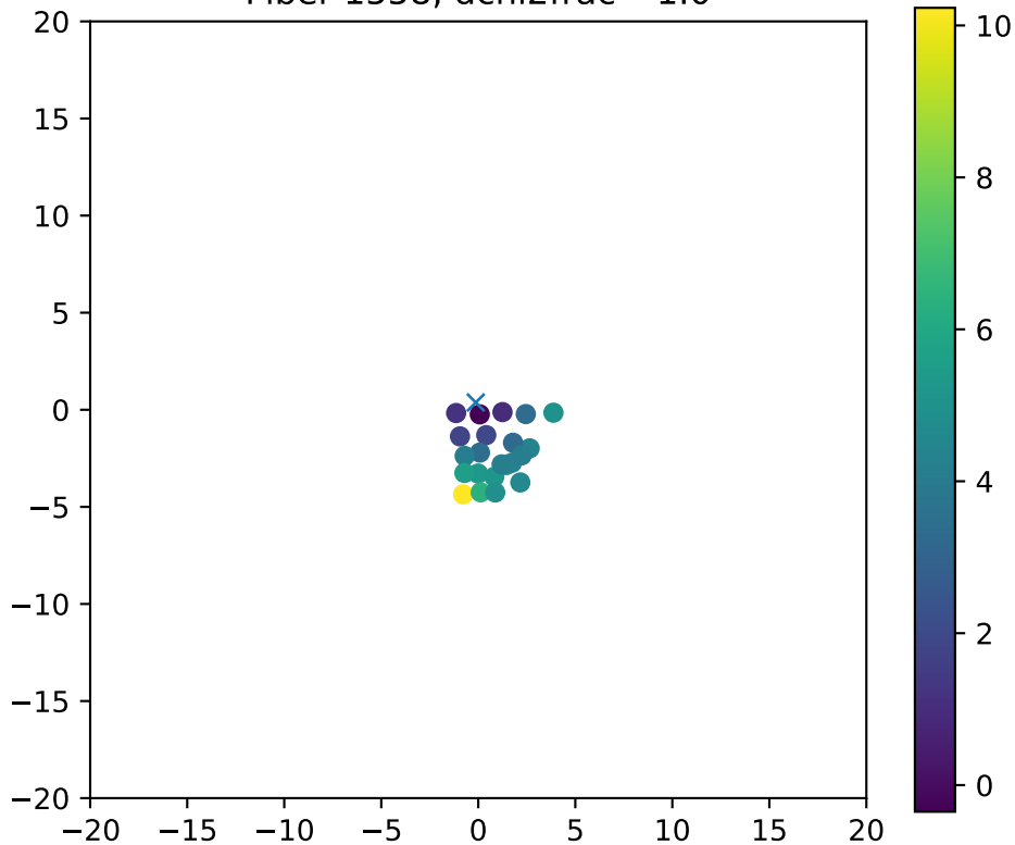
Fiber 1558, dchi2frac= 1.0
