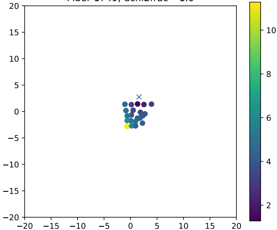
Fiber 1749, dchi2frac= 1.0
