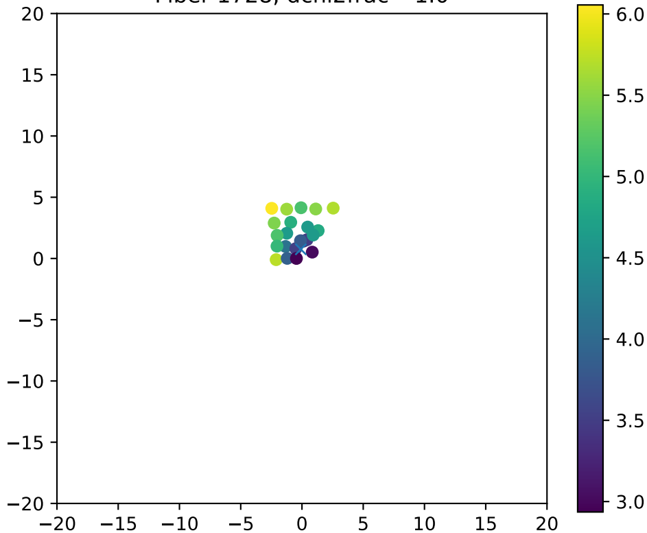
Fiber 1728, dchi2frac= 1.0
