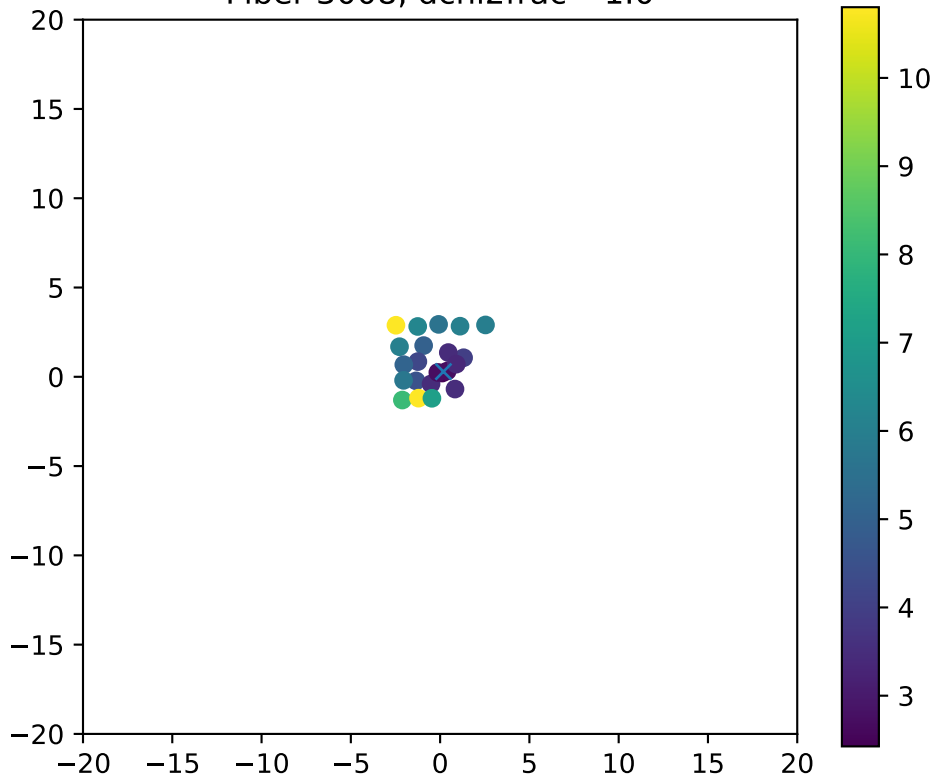
Fiber 3008, dchi2frac= 1.0
