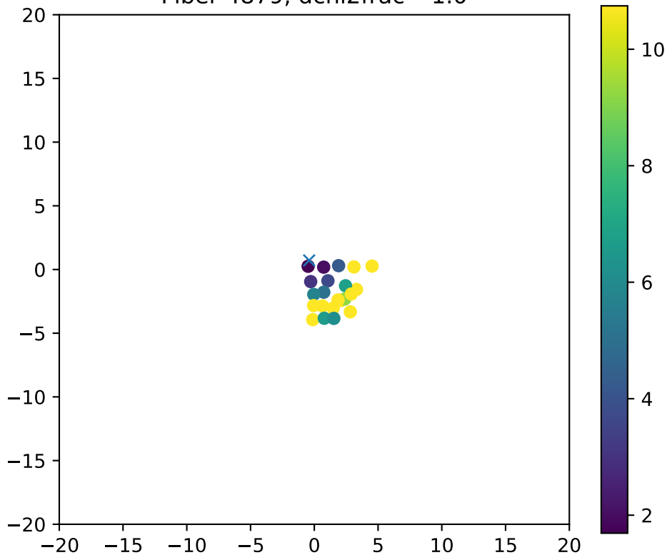
Fiber 4879, dchi2frac= 1.0
