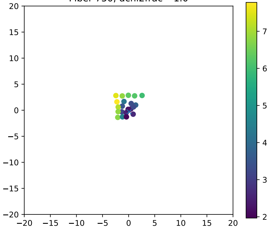
Fiber 750, dchi2frac= 1.0
