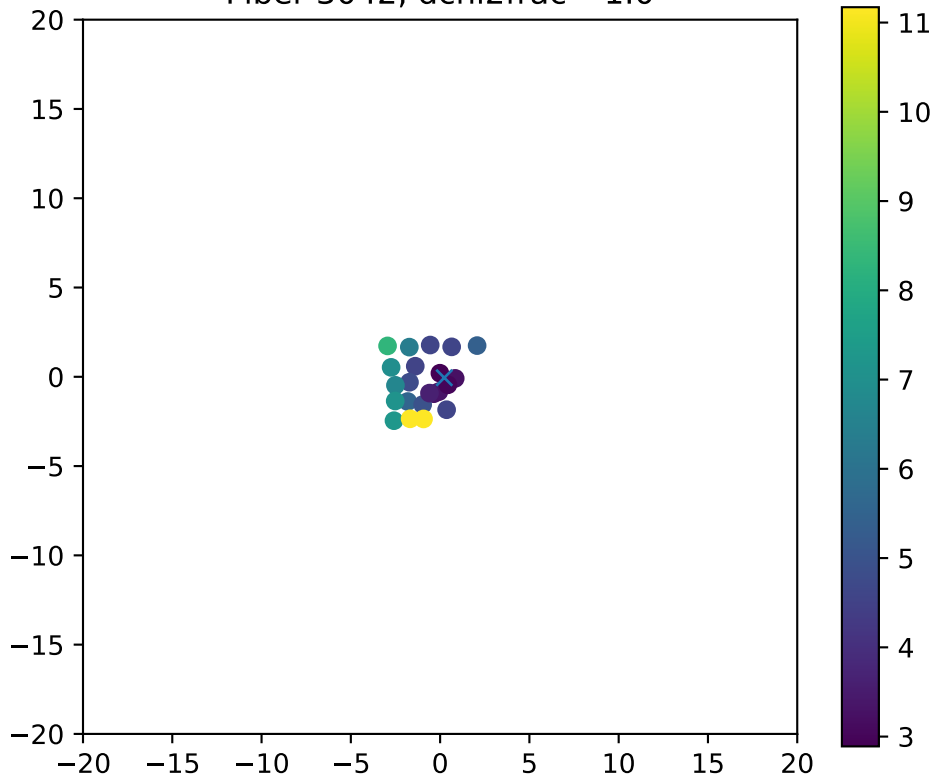
Fiber 3042, dchi2frac= 1.0
