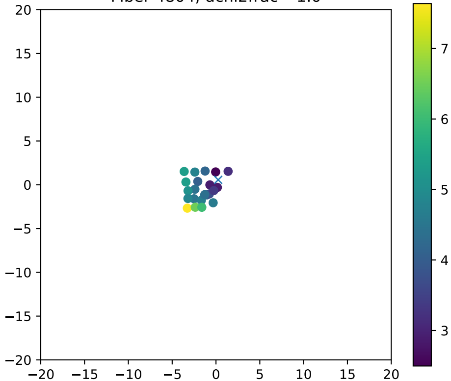
Fiber 4804, dchi2frac= 1.0
