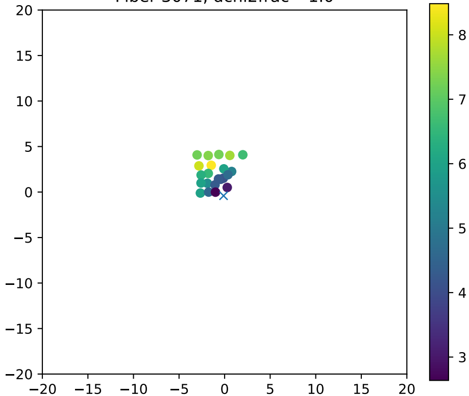
Fiber 3071, dchi2frac= 1.0
