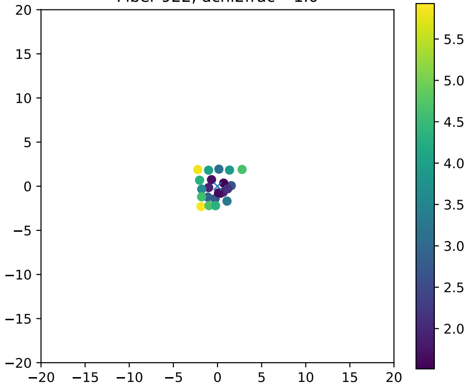
Fiber 922, dchi2frac= 1.0
