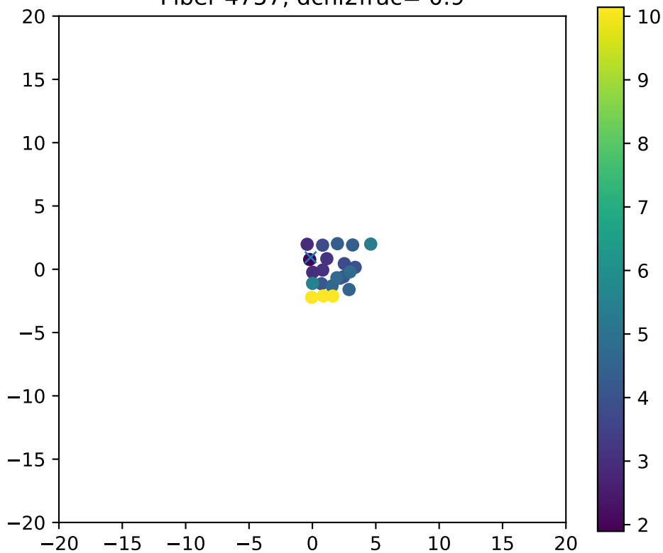
Fiber 4757, dchi2frac= 0.9
