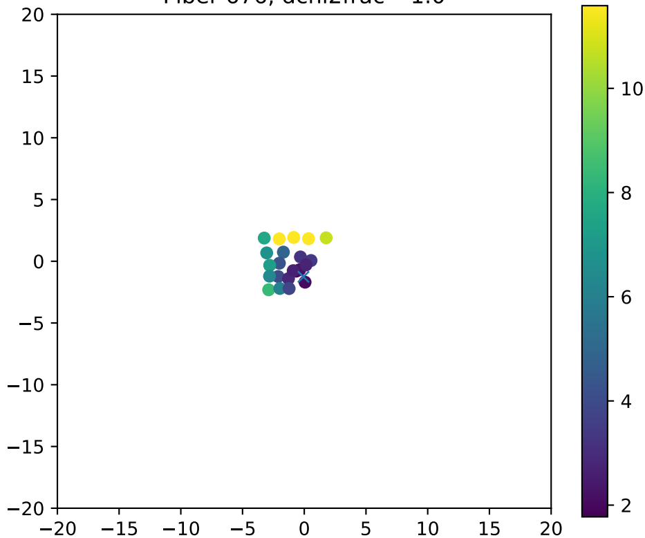
Fiber 676, dchi2frac= 1.0
