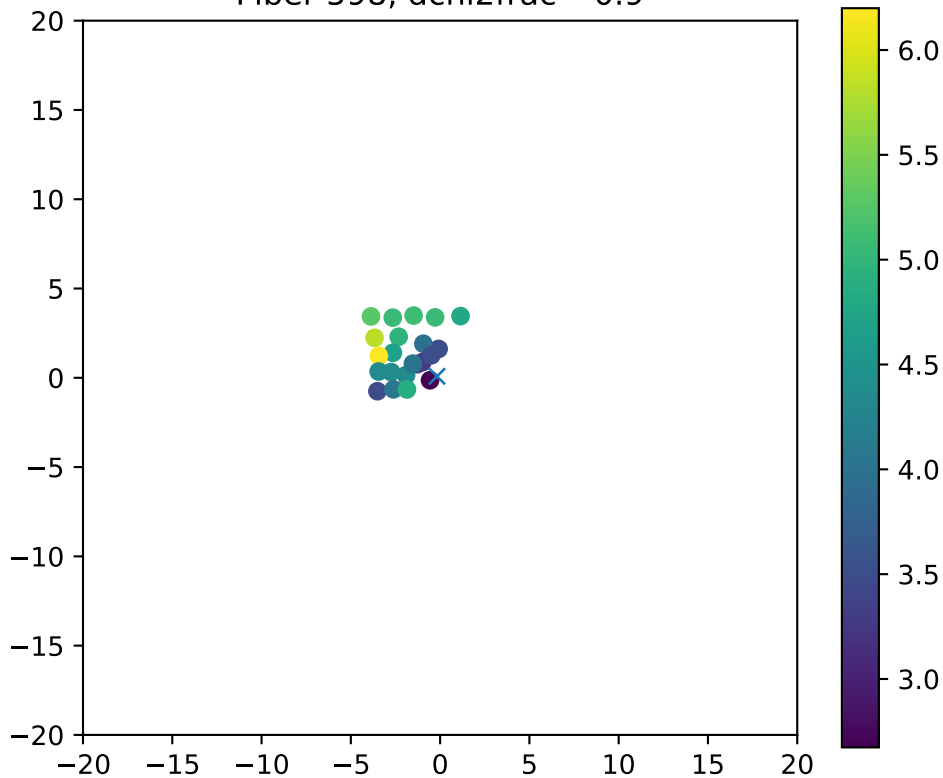
Fiber 598, dchi2frac= 0.9
