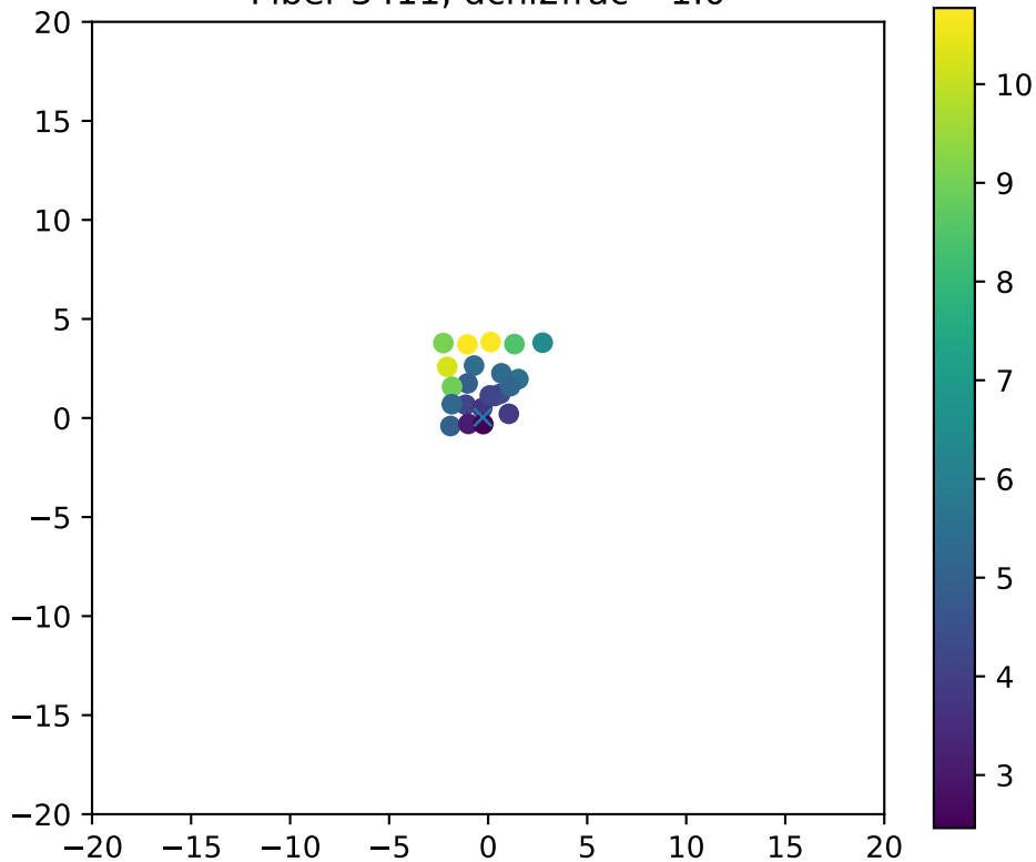
Fiber 3411, dchi2frac= 1.0
