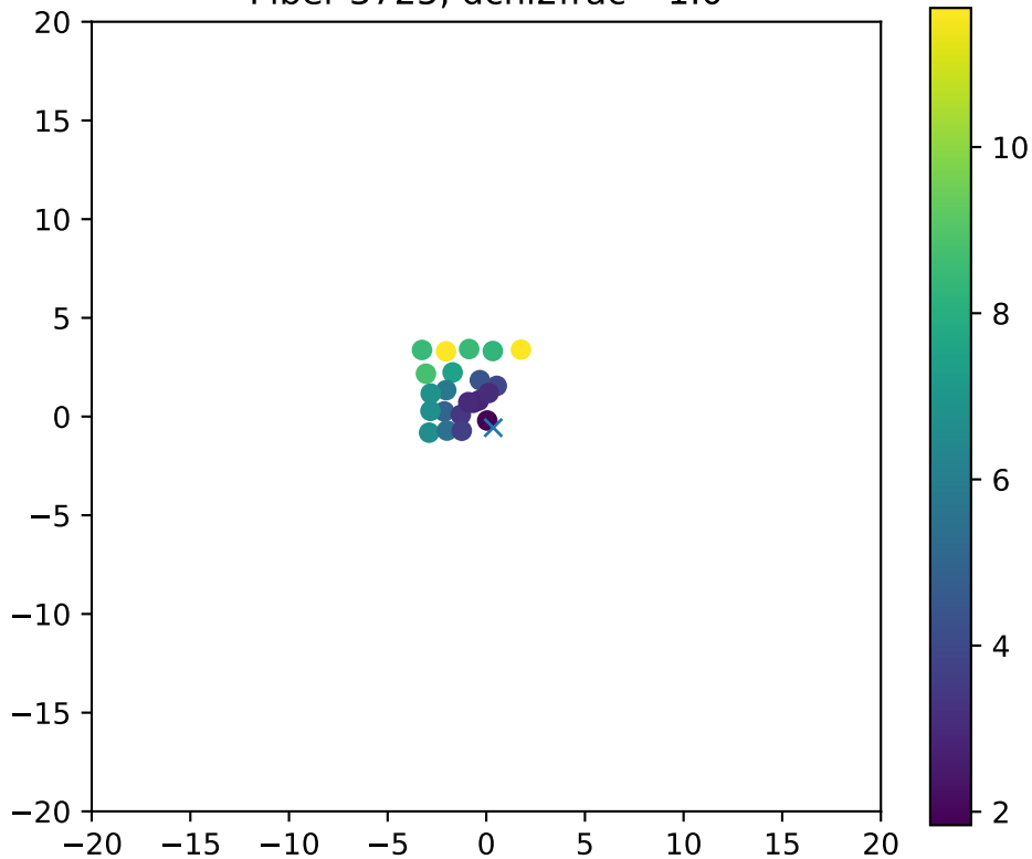
Fiber 3725, dchi2frac= 1.0
