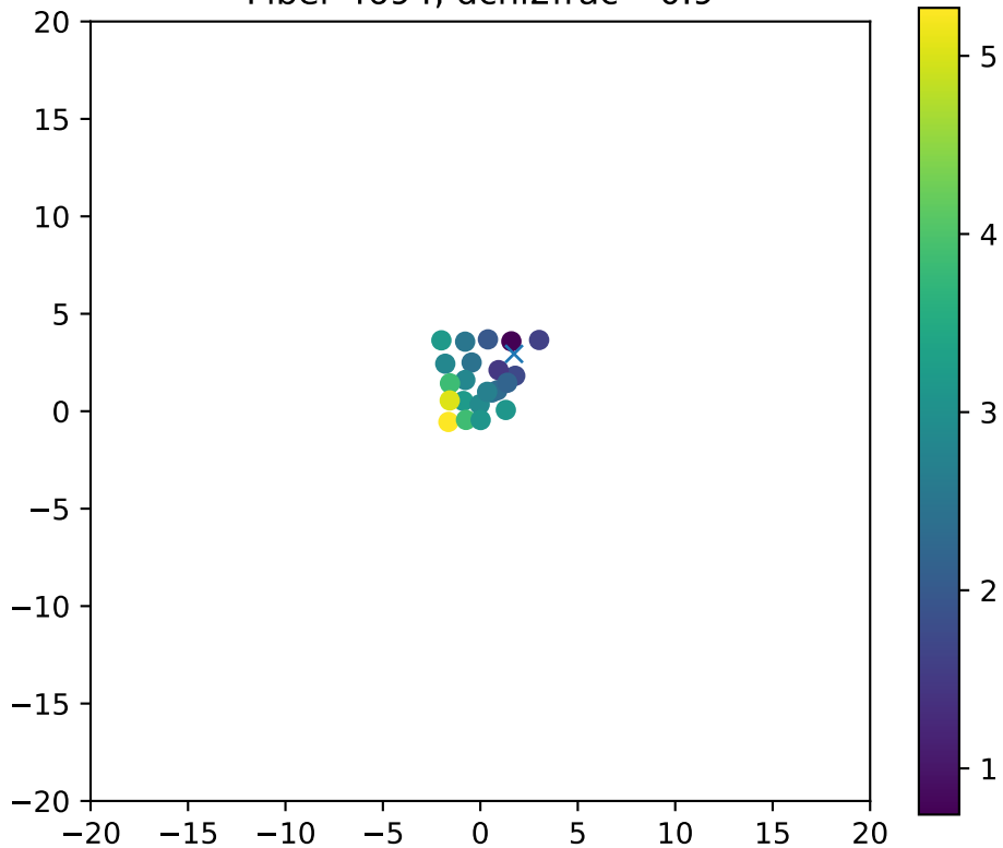
Fiber 4694, dchi2frac= 0.9
