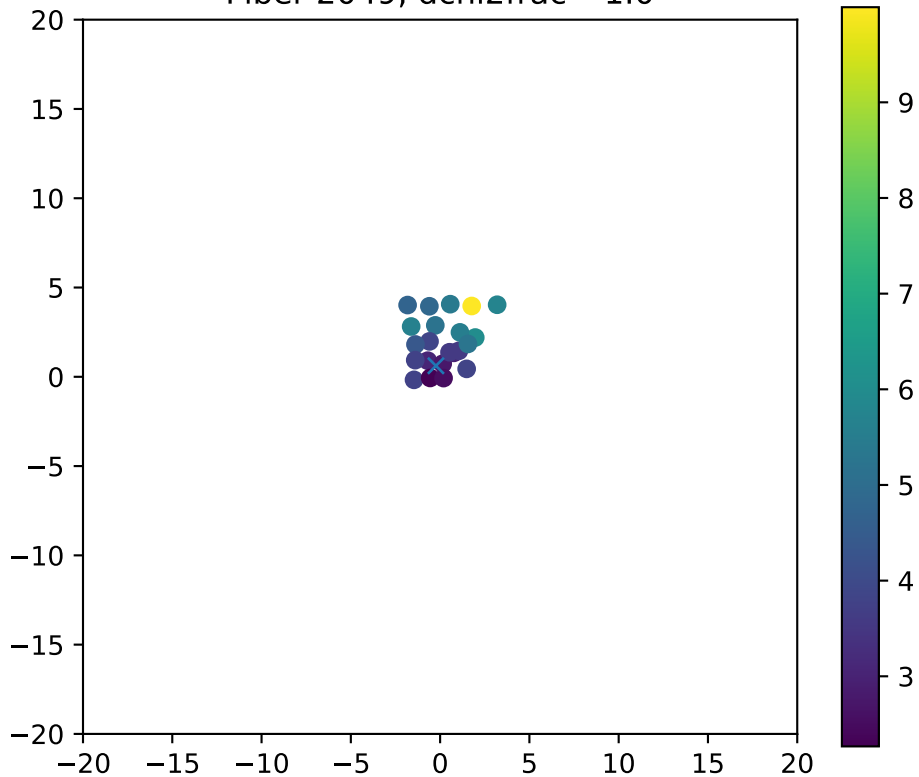
Fiber 2049, dchi2frac= 1.0
