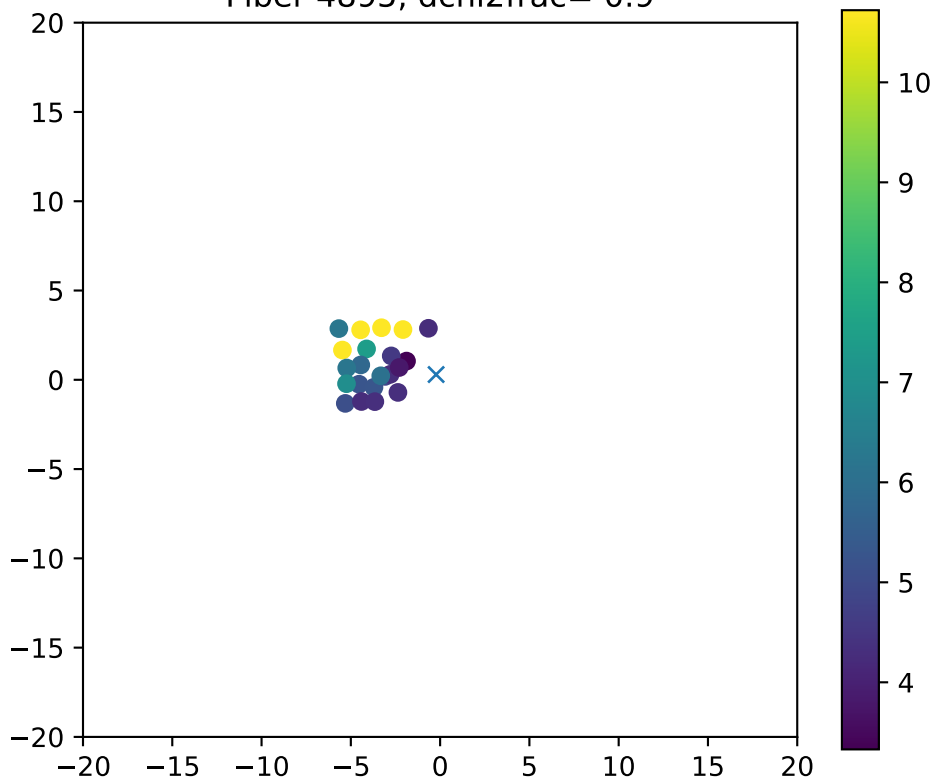
Fiber 4895, dchi2frac= 0.9
