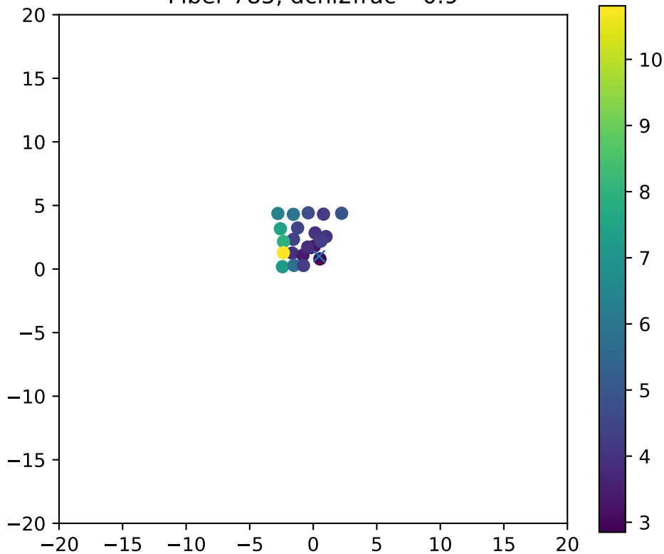
Fiber 785, dchi2frac= 0.9
