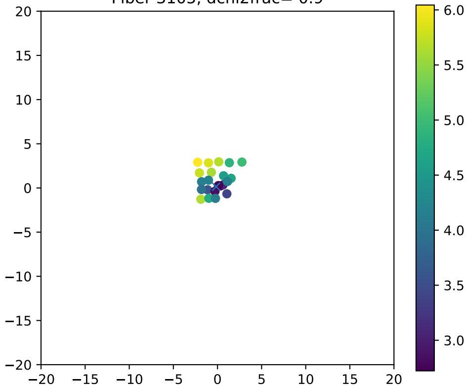
Fiber 3105, dchi2frac= 0.9
