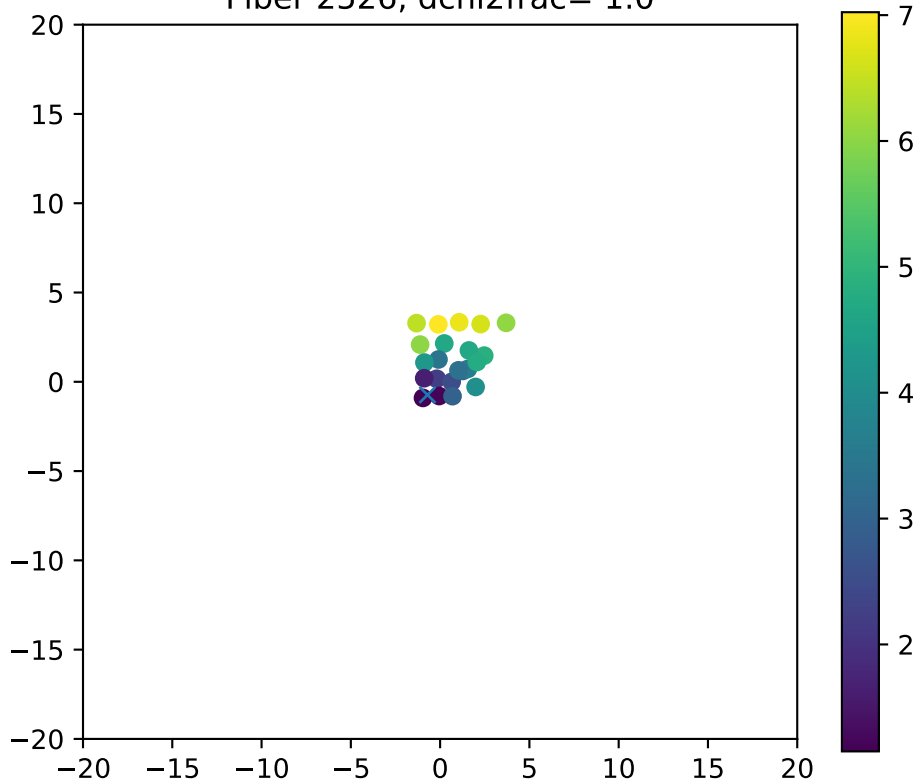
Fiber 2526, dchi2frac= 1.0
