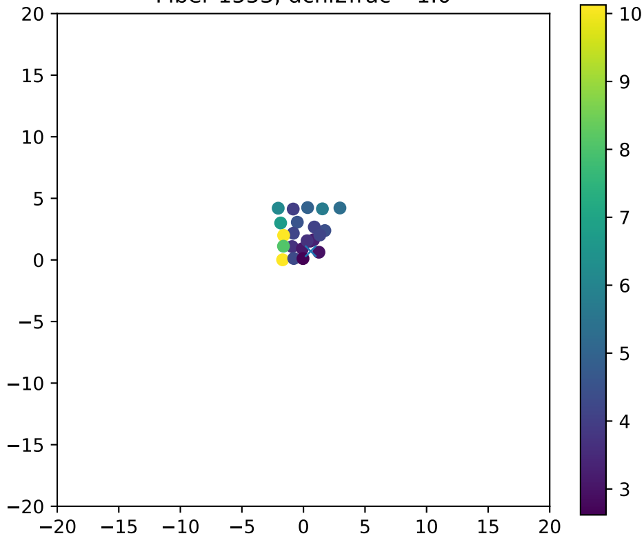
Fiber 1553, dchi2frac= 1.0
