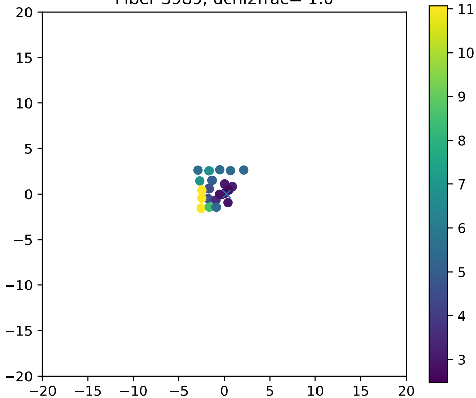
Fiber 3989, dchi2frac= 1.0
