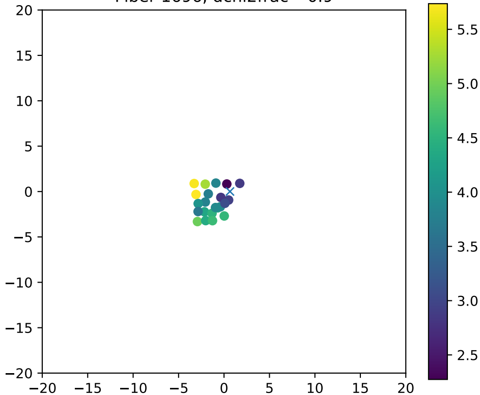
Fiber 1696, dchi2frac= 0.9
