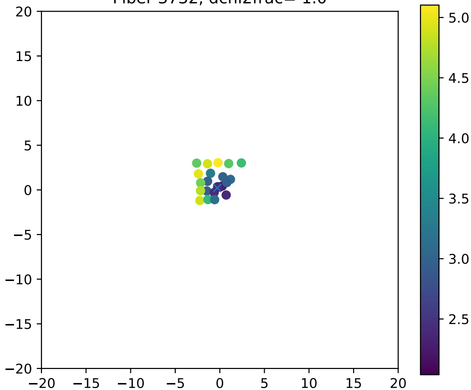
Fiber 3732, dchi2frac= 1.0
