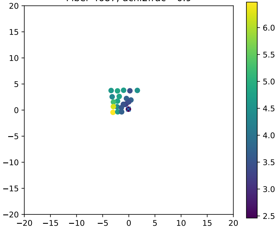
Fiber 4687, dchi2frac= 0.9
