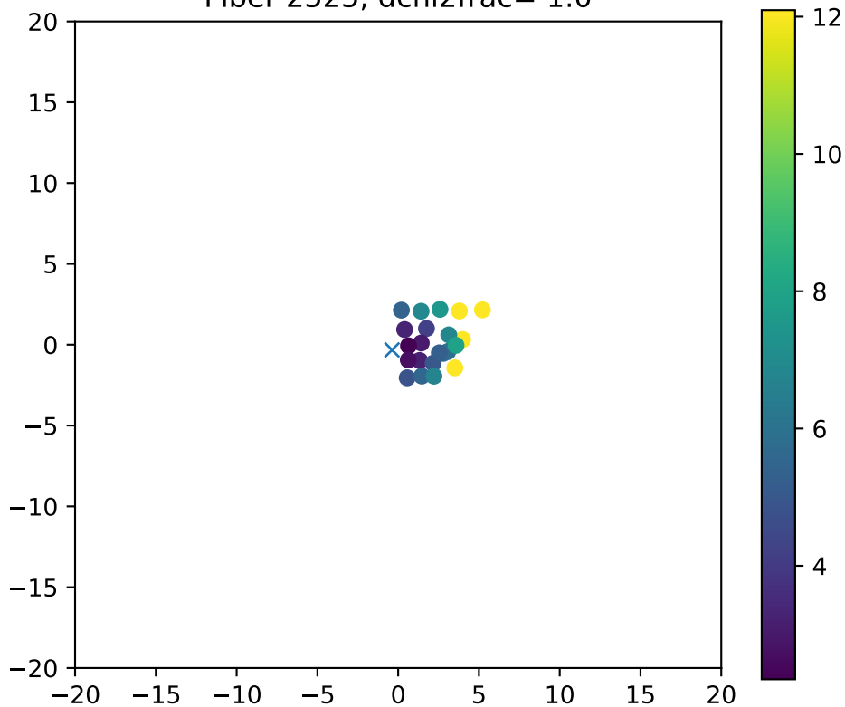
Fiber 2525, dchi2frac= 1.0
