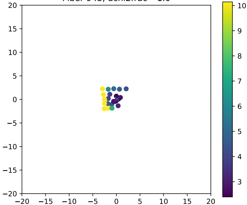
Fiber 943, dchi2frac= 1.0
