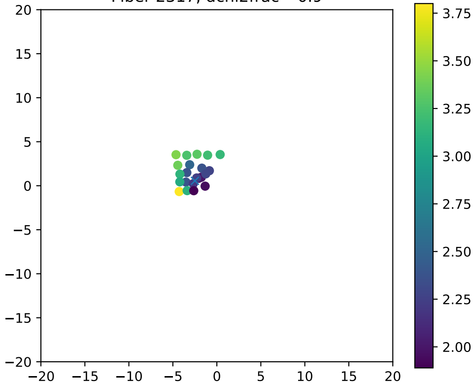
Fiber 2317, dchi2frac= 0.9
