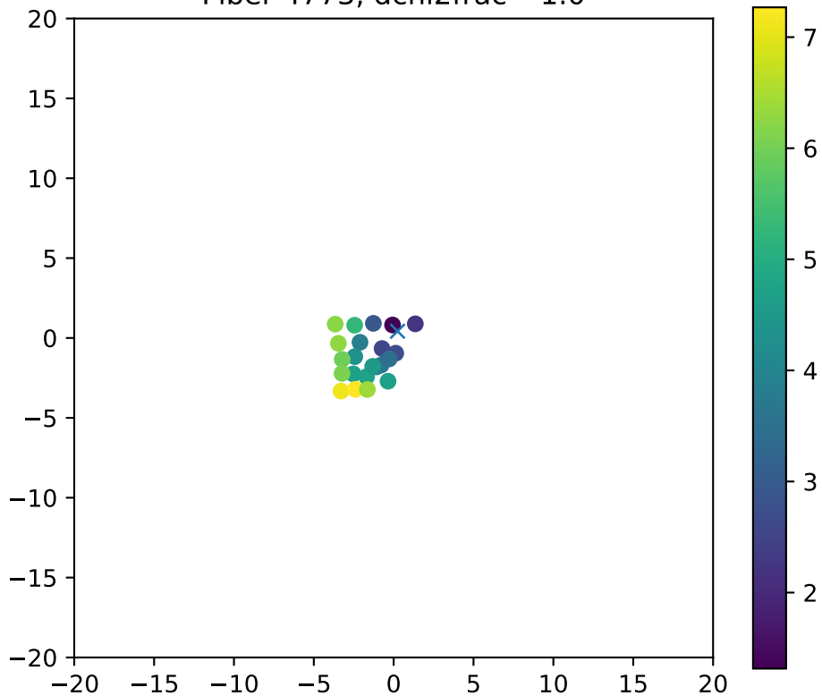
Fiber 4773, dchi2frac= 1.0
