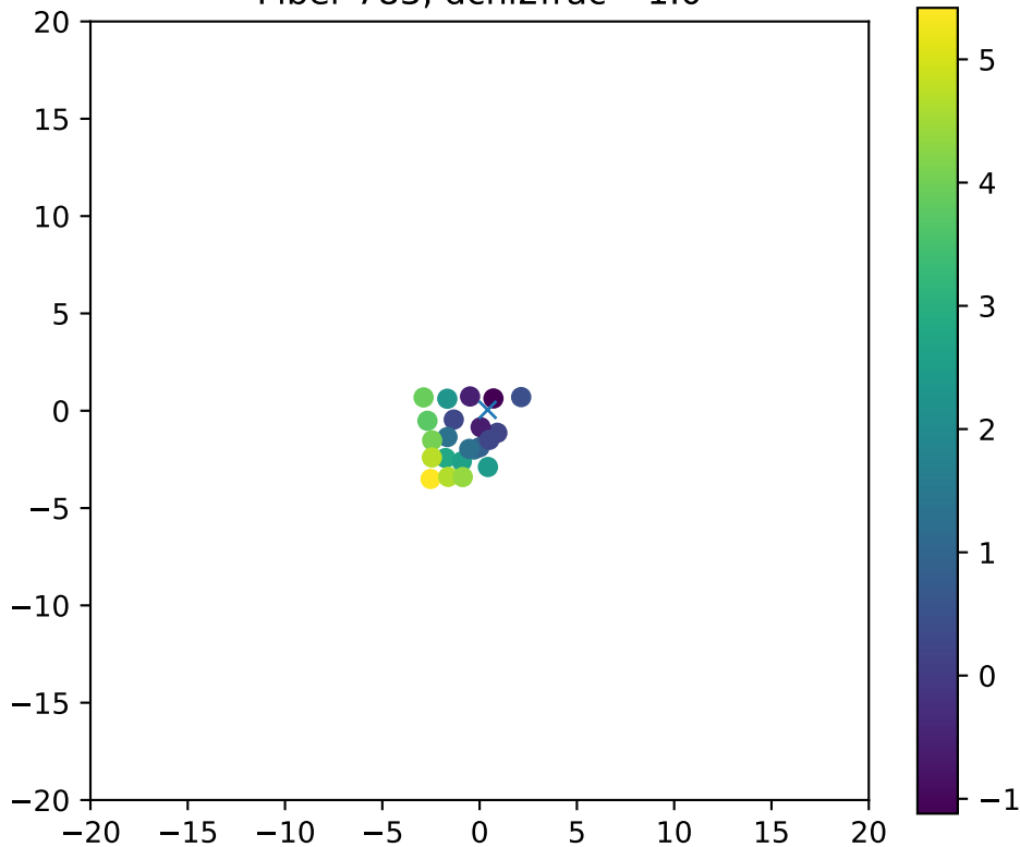
Fiber 783, dchi2frac= 1.0
