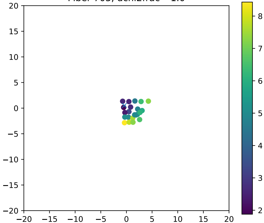
Fiber 703, dchi2frac= 1.0
