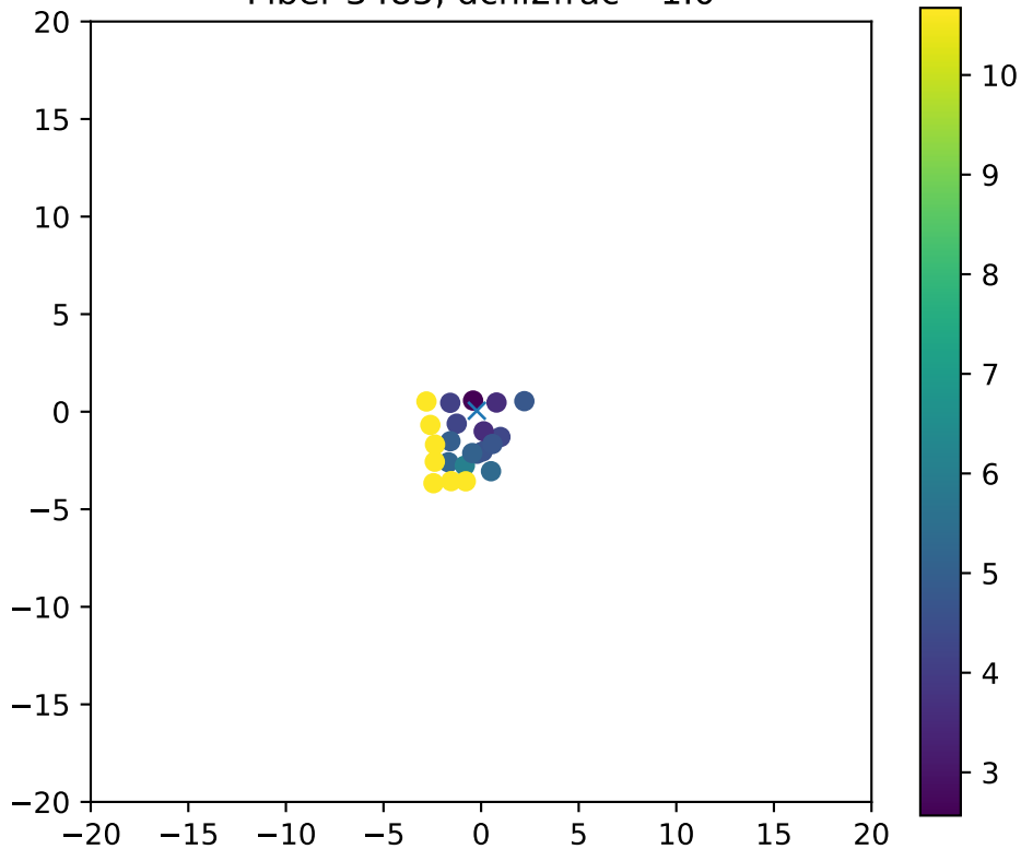
Fiber 3485, dchi2frac= 1.0
