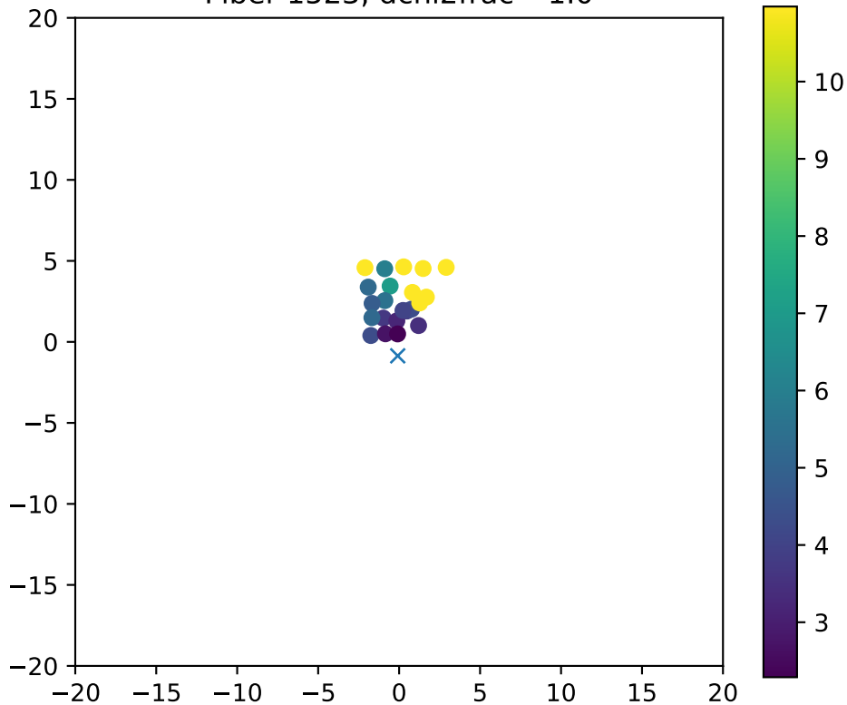
Fiber 1523, dchi2frac= 1.0
