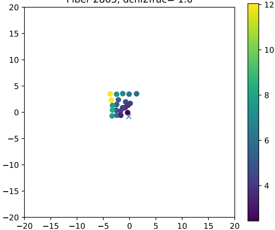
Fiber 2863, dchi2frac= 1.0
