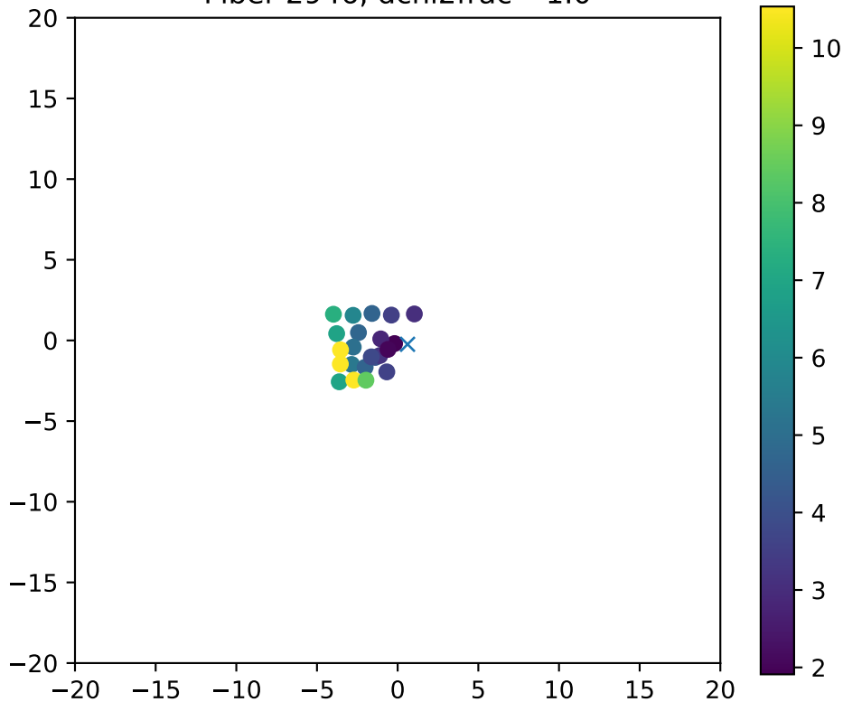
Fiber 2946, dchi2frac= 1.0
