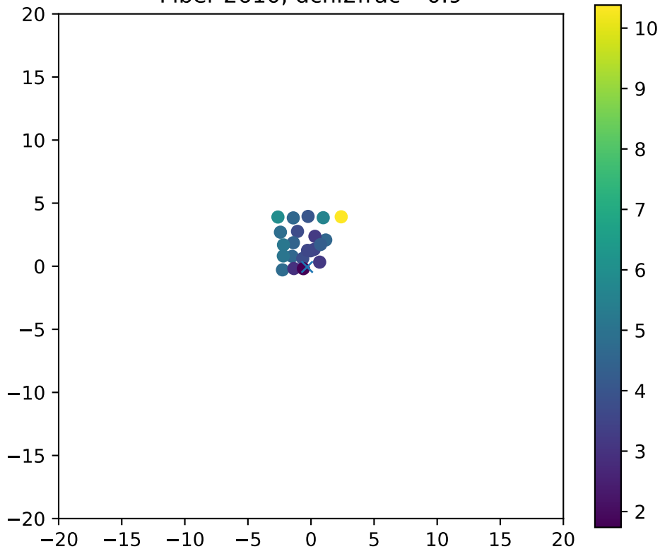
Fiber 2610, dchi2frac= 0.9
