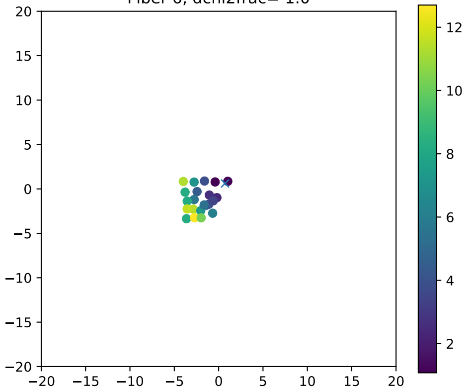
Fiber 6, dchi2frac= 1.0
