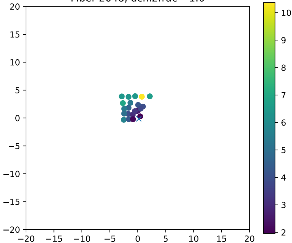
Fiber 2048, dchi2frac= 1.0
