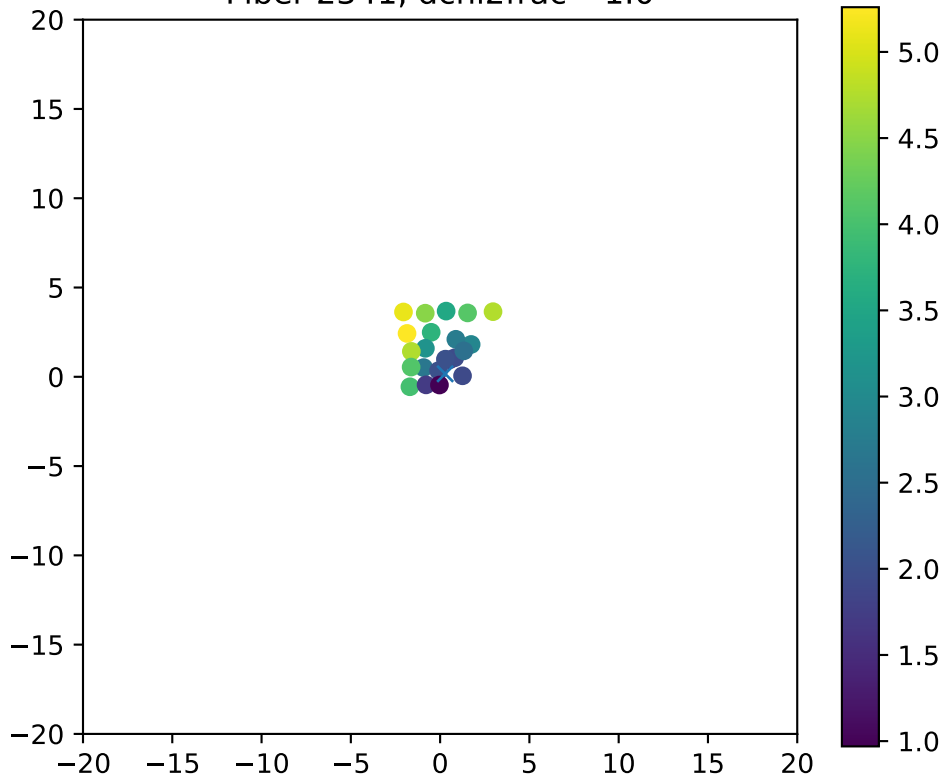
Fiber 2341, dchi2frac= 1.0
