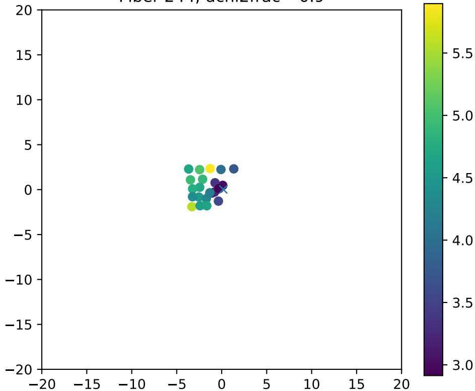
Fiber 244, dchi2frac= 0.9
