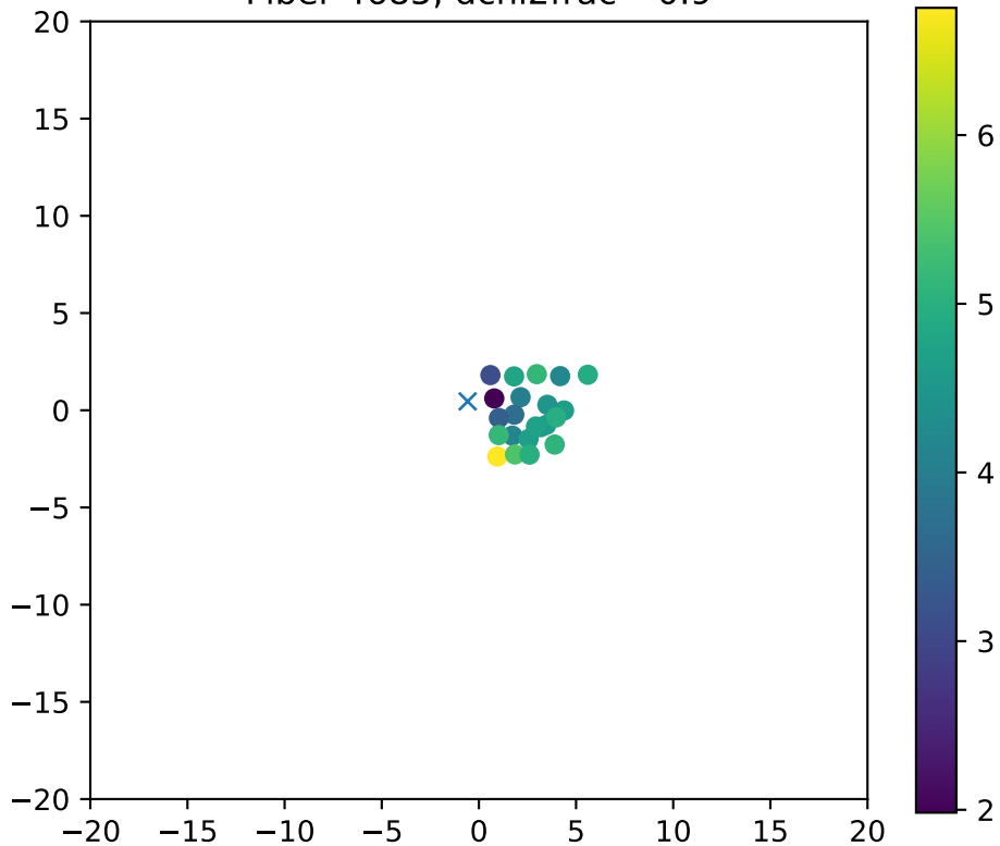
Fiber 4685, dchi2frac= 0.9
