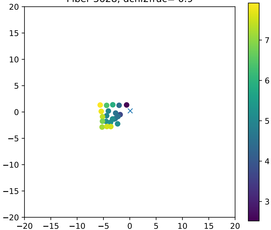
Fiber 3628, dchi2frac= 0.9
