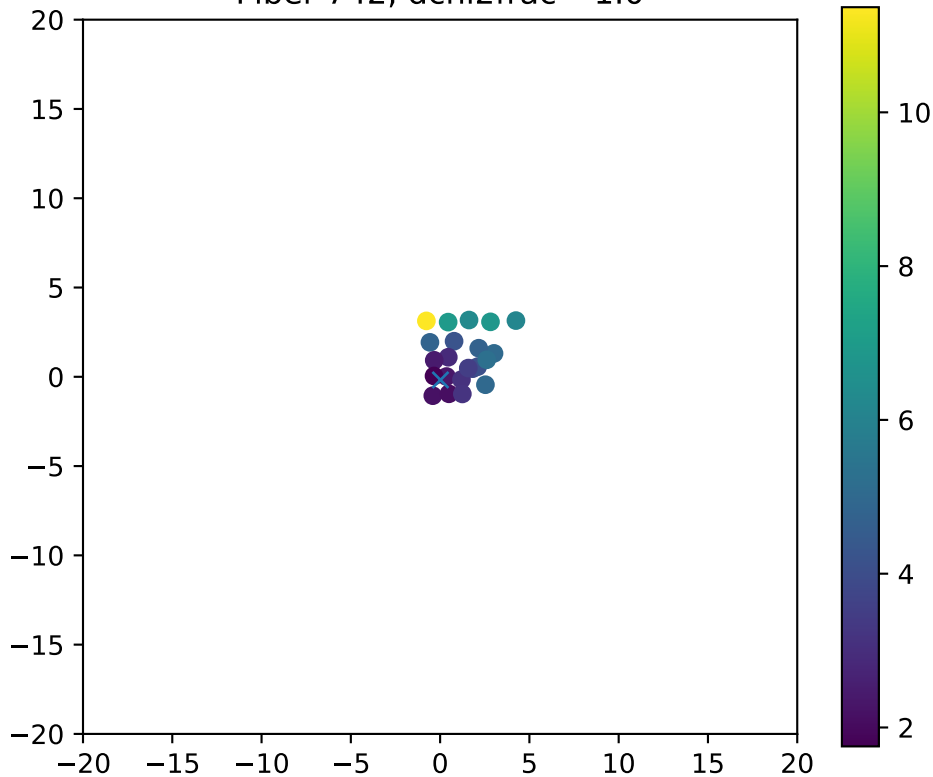
Fiber 742, dchi2frac= 1.0
