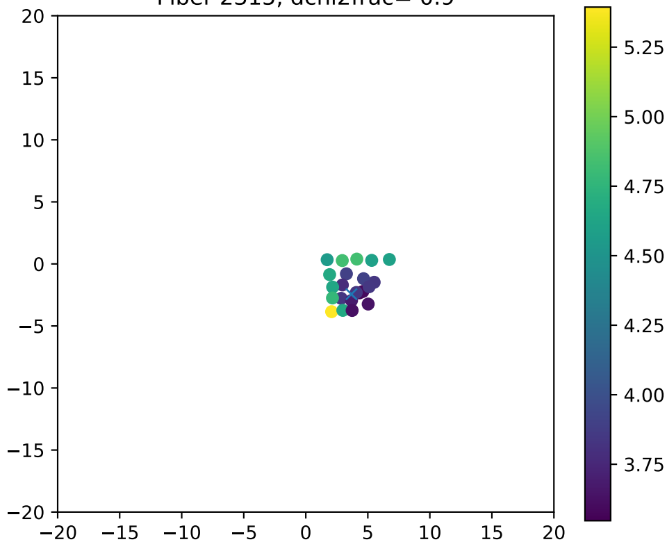
Fiber 2315, dchi2frac= 0.9
