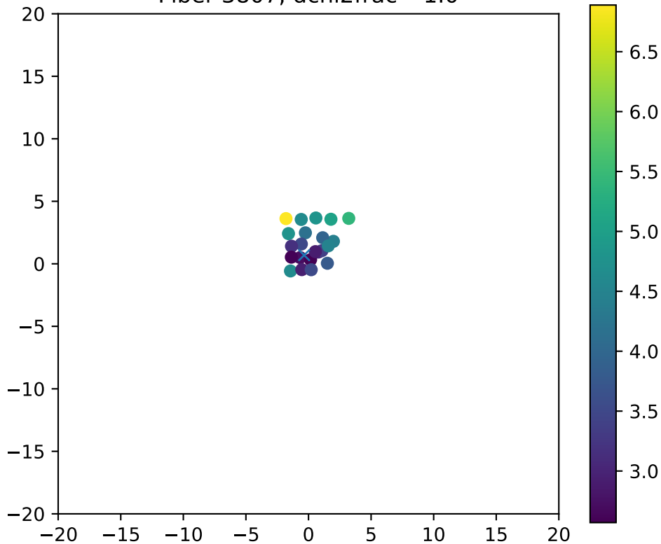
Fiber 3807, dchi2frac= 1.0
