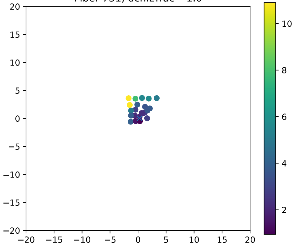
Fiber 731, dchi2frac= 1.0
