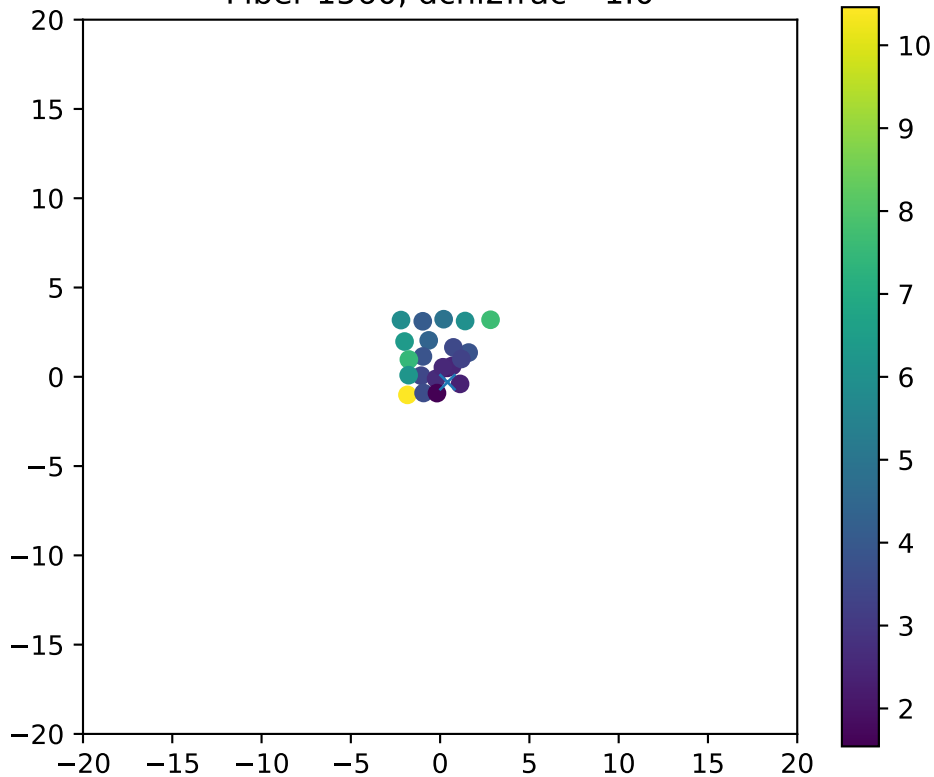
Fiber 1560, dchi2frac= 1.0
