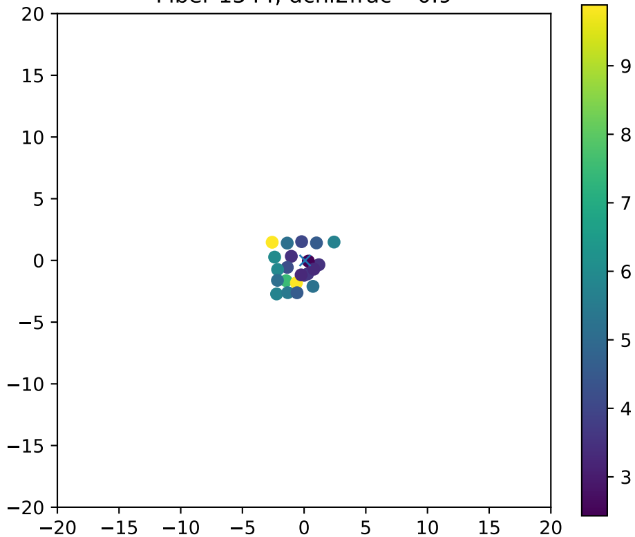
Fiber 1544, dchi2frac= 0.9
