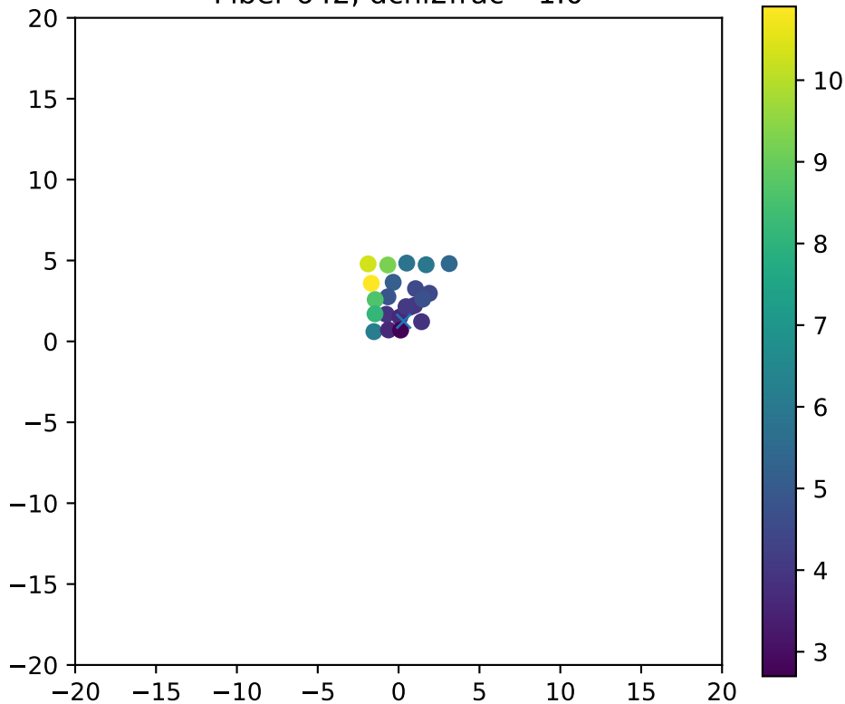
Fiber 642, dchi2frac= 1.0
