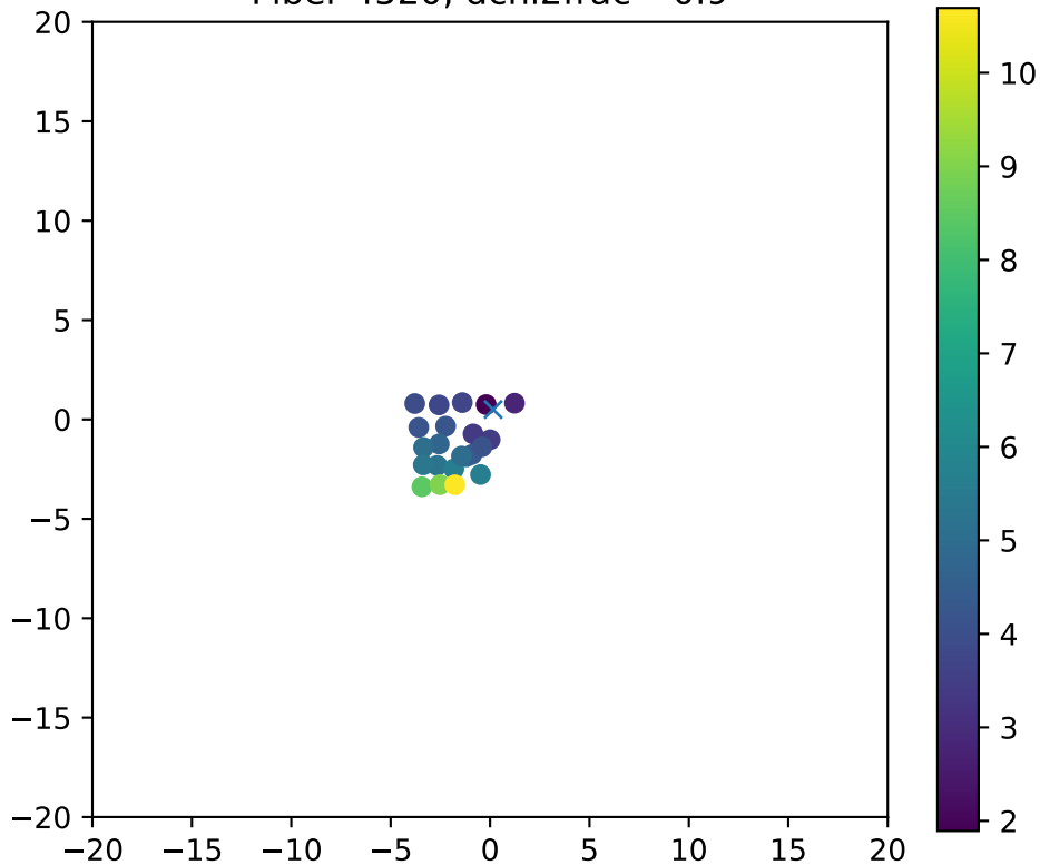
Fiber 4520, dchi2frac= 0.9
