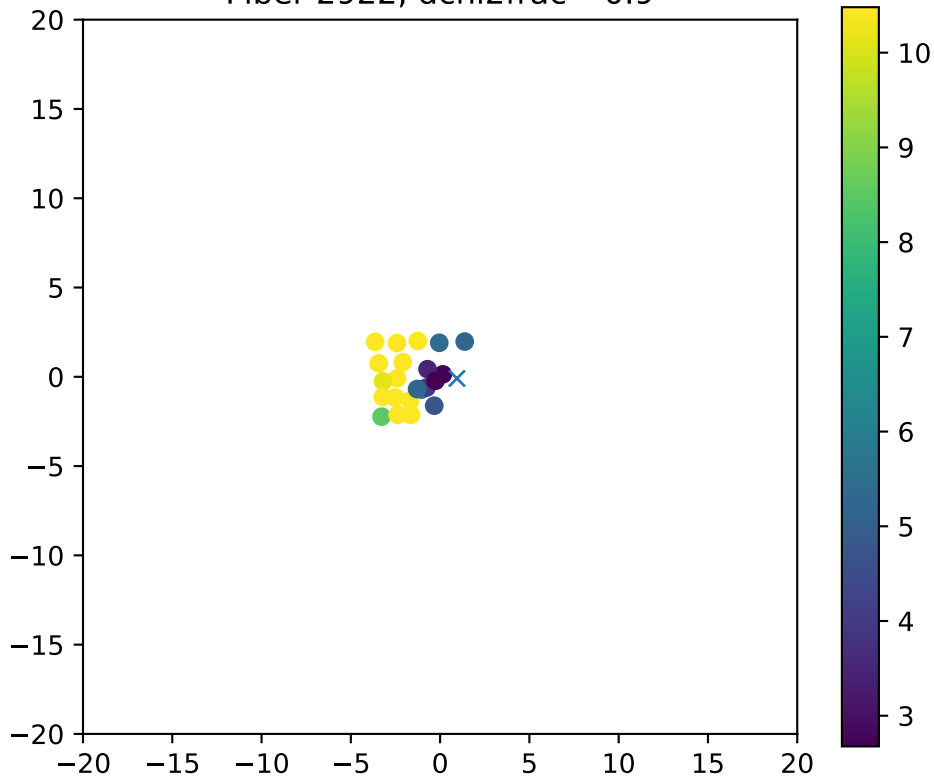
Fiber 2922, dchi2frac= 0.9
