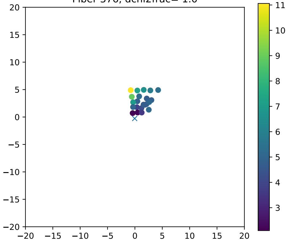
Fiber 376, dchi2frac= 1.0
