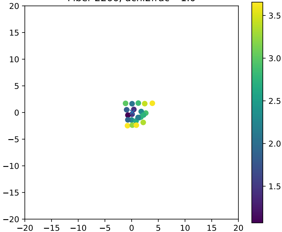
Fiber 2266, dchi2frac= 1.0
