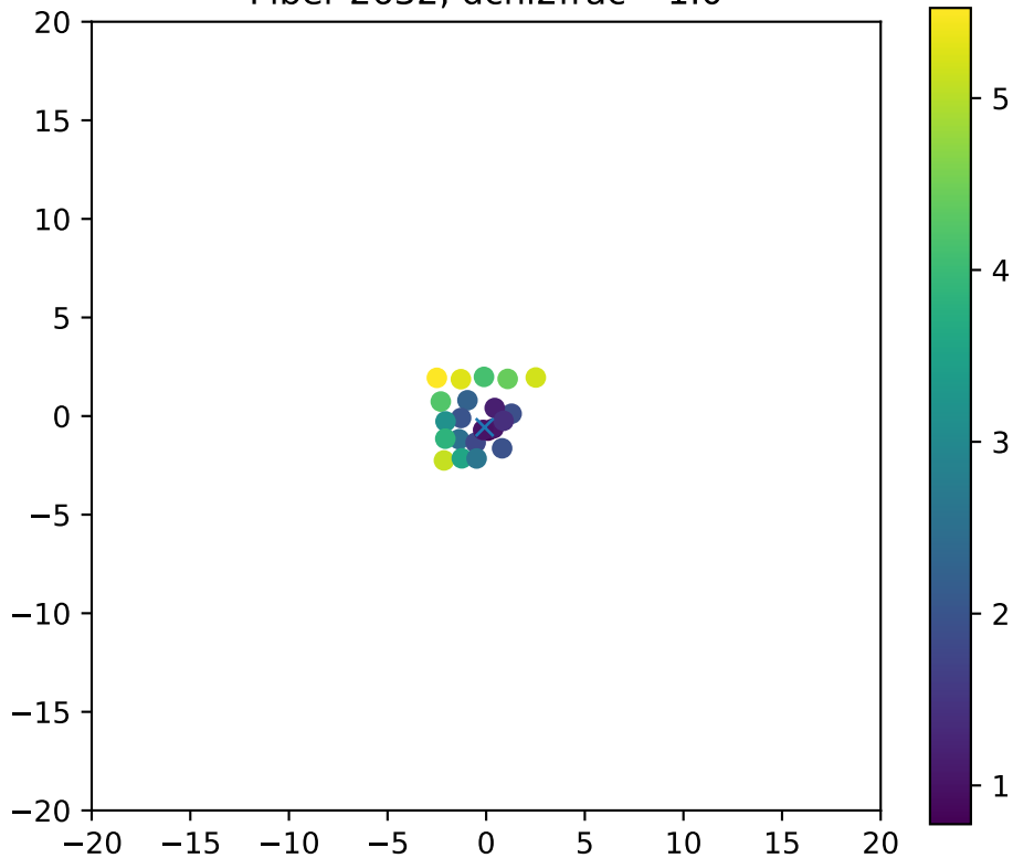
Fiber 2632, dchi2frac= 1.0
