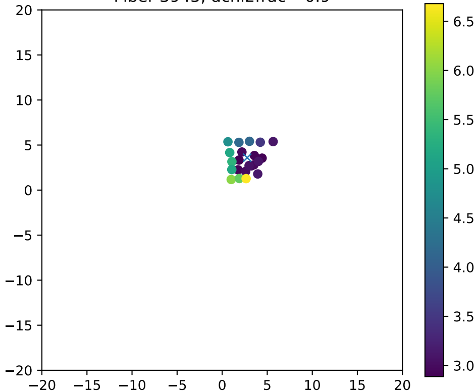
Fiber 3945, dchi2frac= 0.9
