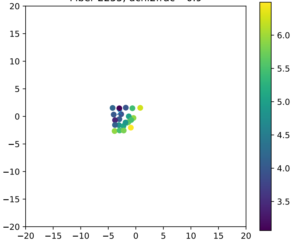
Fiber 2255, dchi2frac= 0.9
