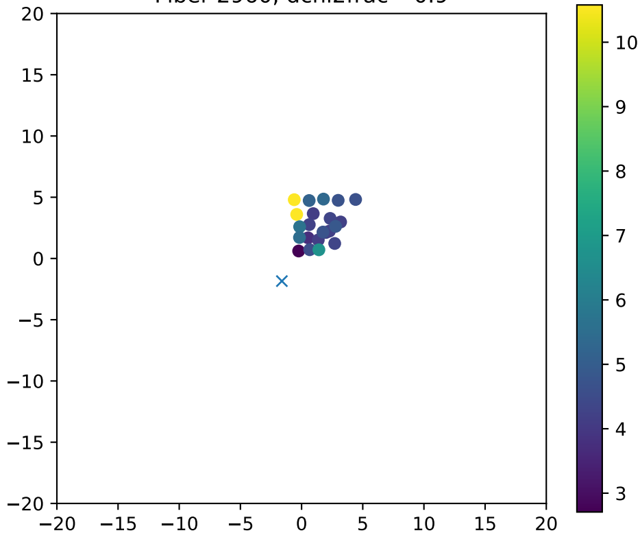
Fiber 2960, dchi2frac= 0.9
