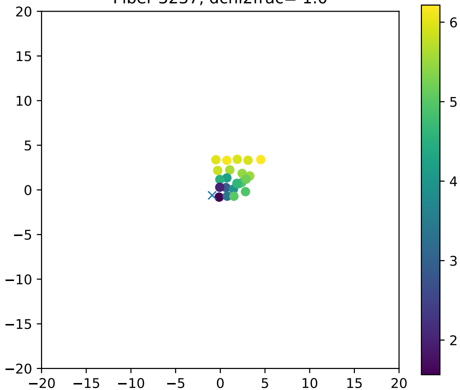
Fiber 3237, dchi2frac= 1.0
