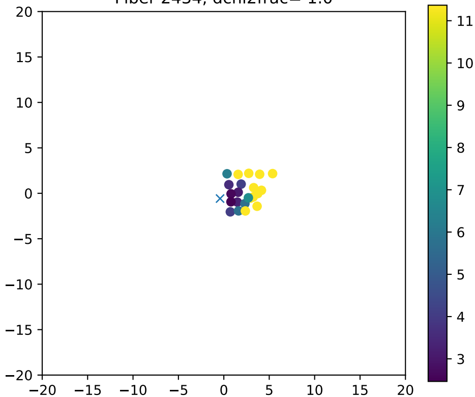
Fiber 2434, dchi2frac= 1.0
