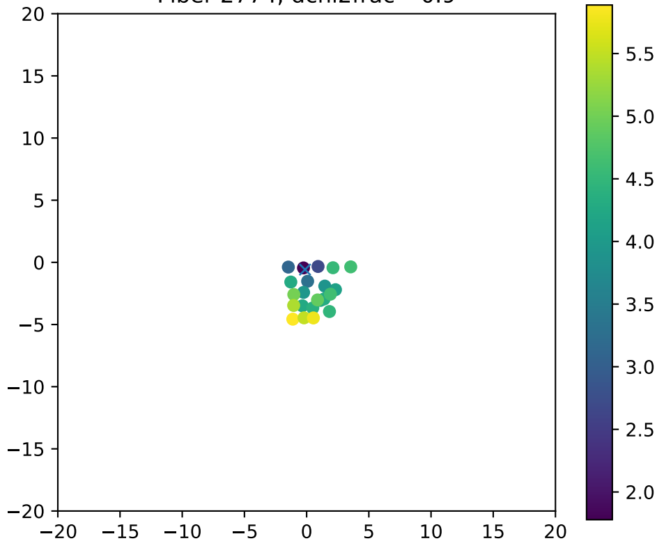
Fiber 2774, dchi2frac= 0.9
