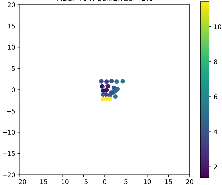
Fiber 464, dchi2frac= 1.0
