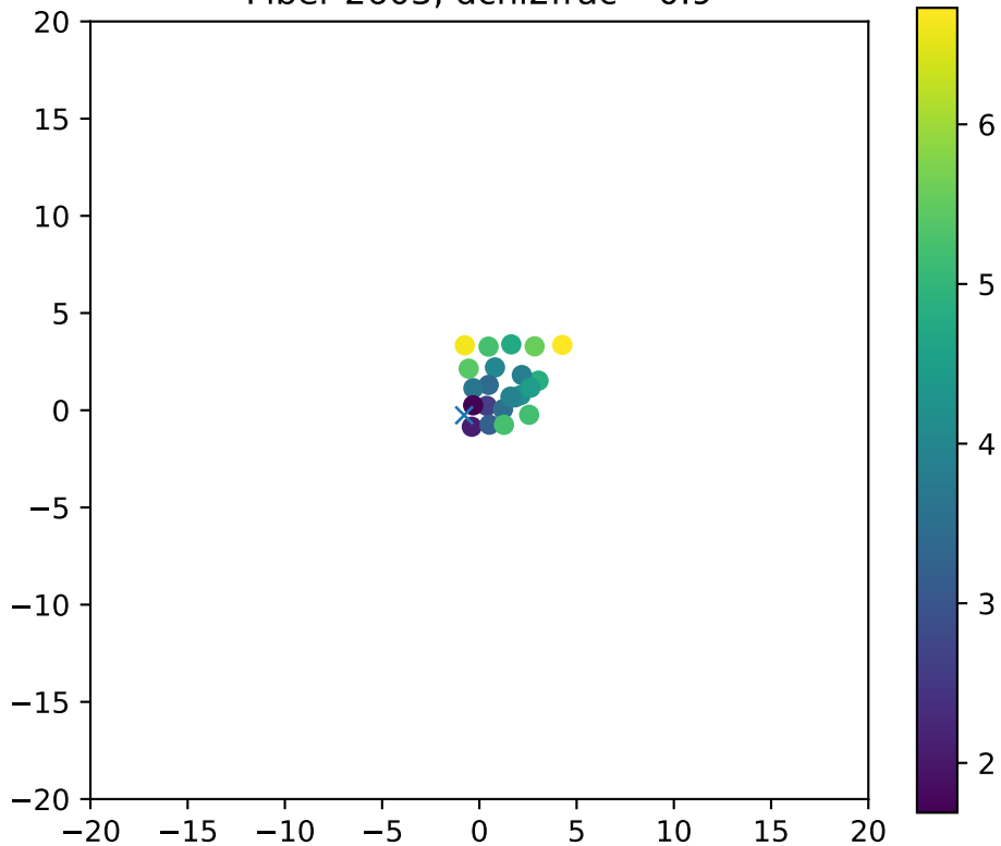
Fiber 2603, dchi2frac= 0.9
