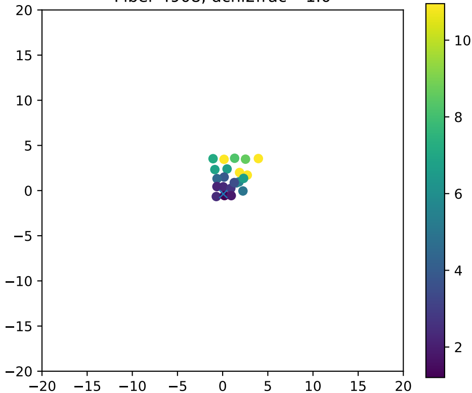
Fiber 4908, dchi2frac= 1.0
