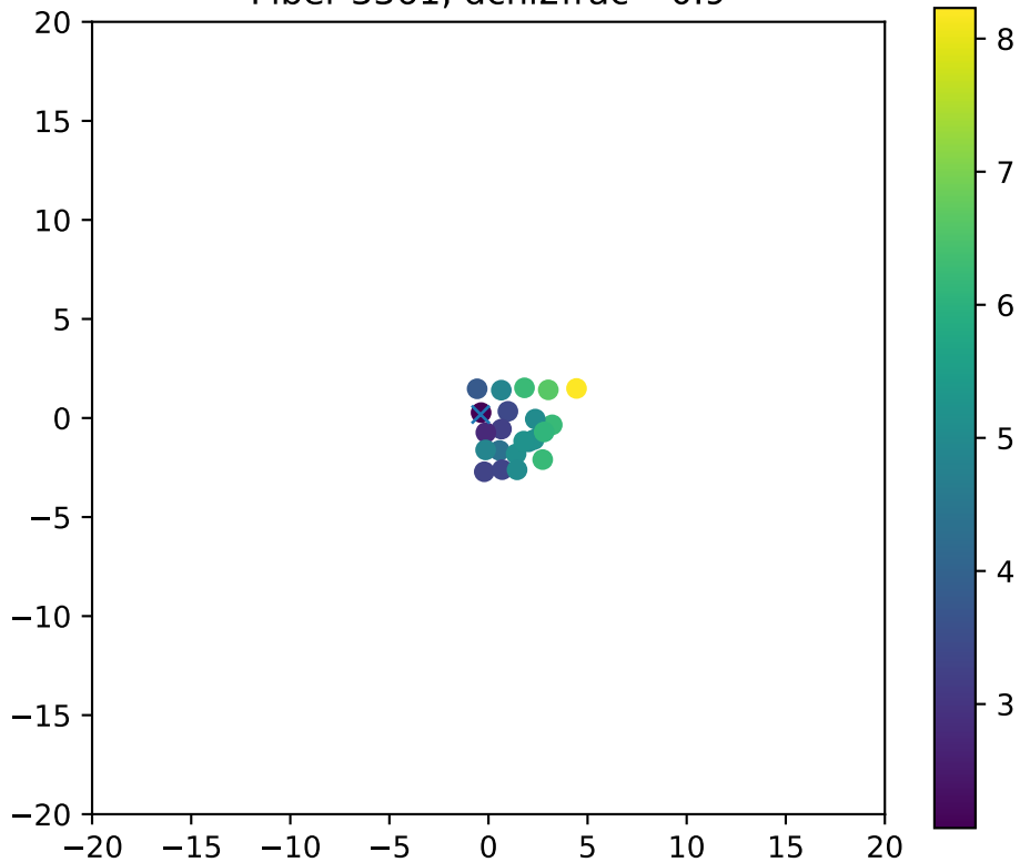
Fiber 3361, dchi2frac= 0.9
