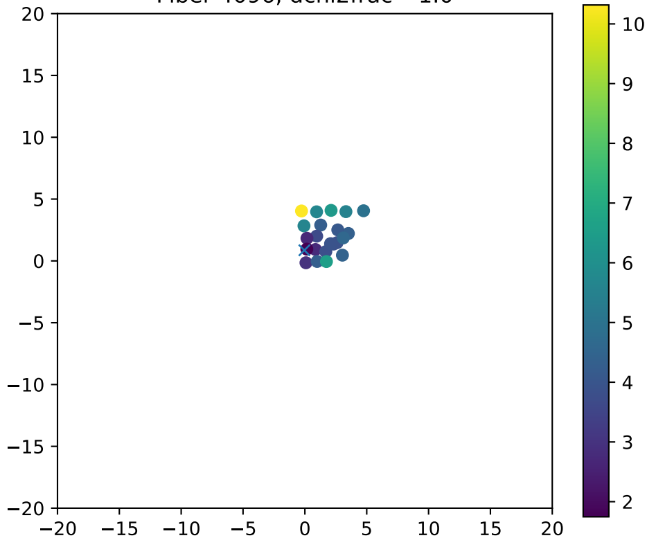
Fiber 4096, dchi2frac= 1.0
