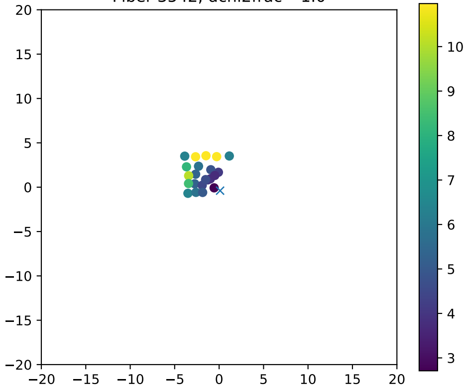
Fiber 3542, dchi2frac= 1.0
