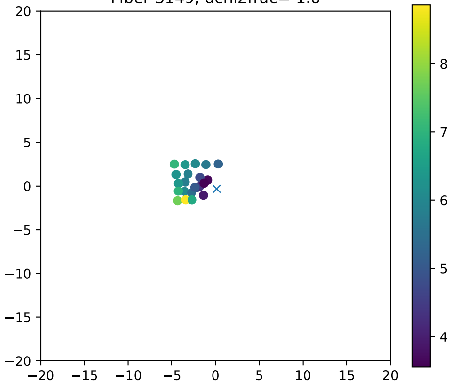
Fiber 3149, dchi2frac= 1.0
