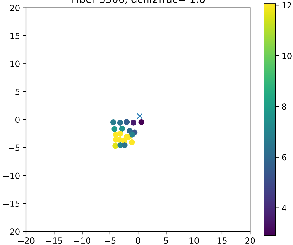
Fiber 3306, dchi2frac= 1.0
