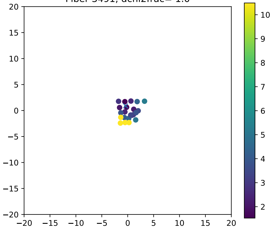
Fiber 3491, dchi2frac= 1.0
