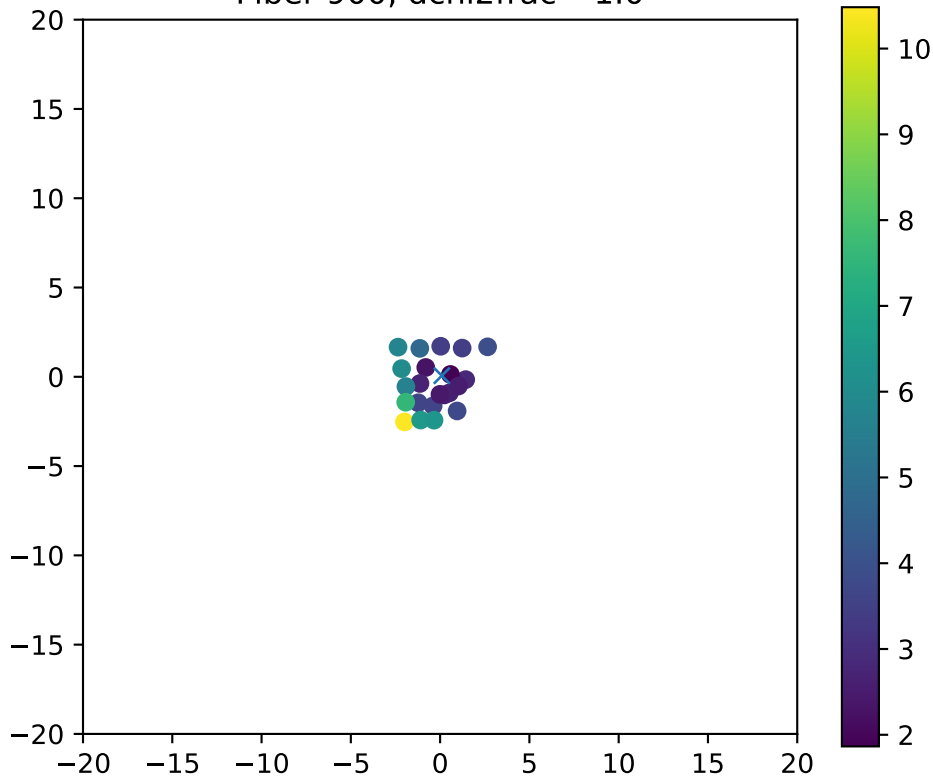
Fiber 900, dchi2frac= 1.0
