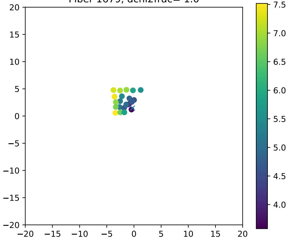
Fiber 1679, dchi2frac= 1.0
