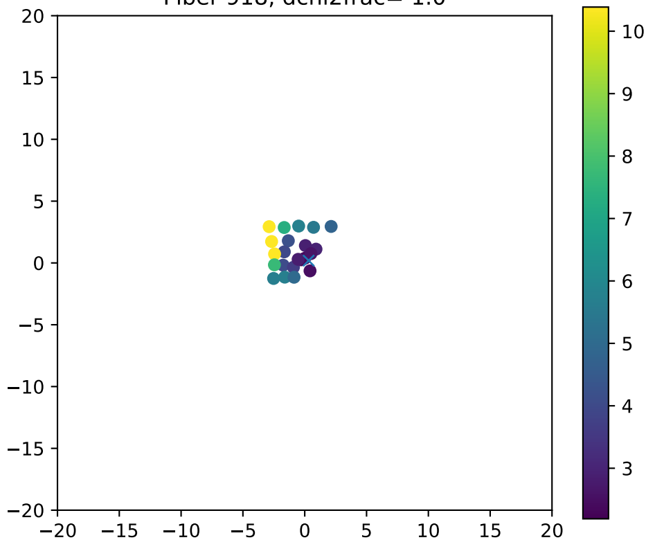
Fiber 918, dchi2frac= 1.0
