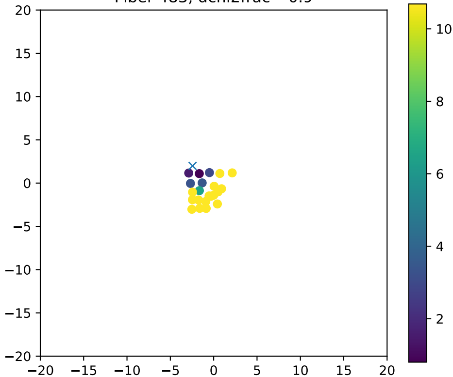
Fiber 483, dchi2frac= 0.9
