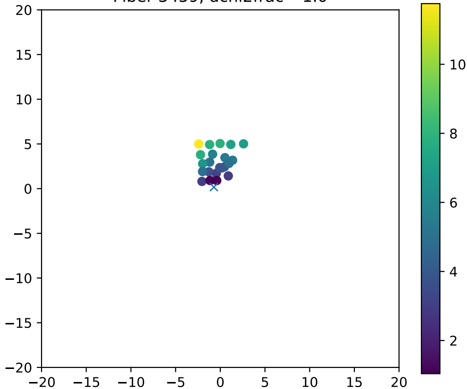
Fiber 3459, dchi2frac= 1.0
