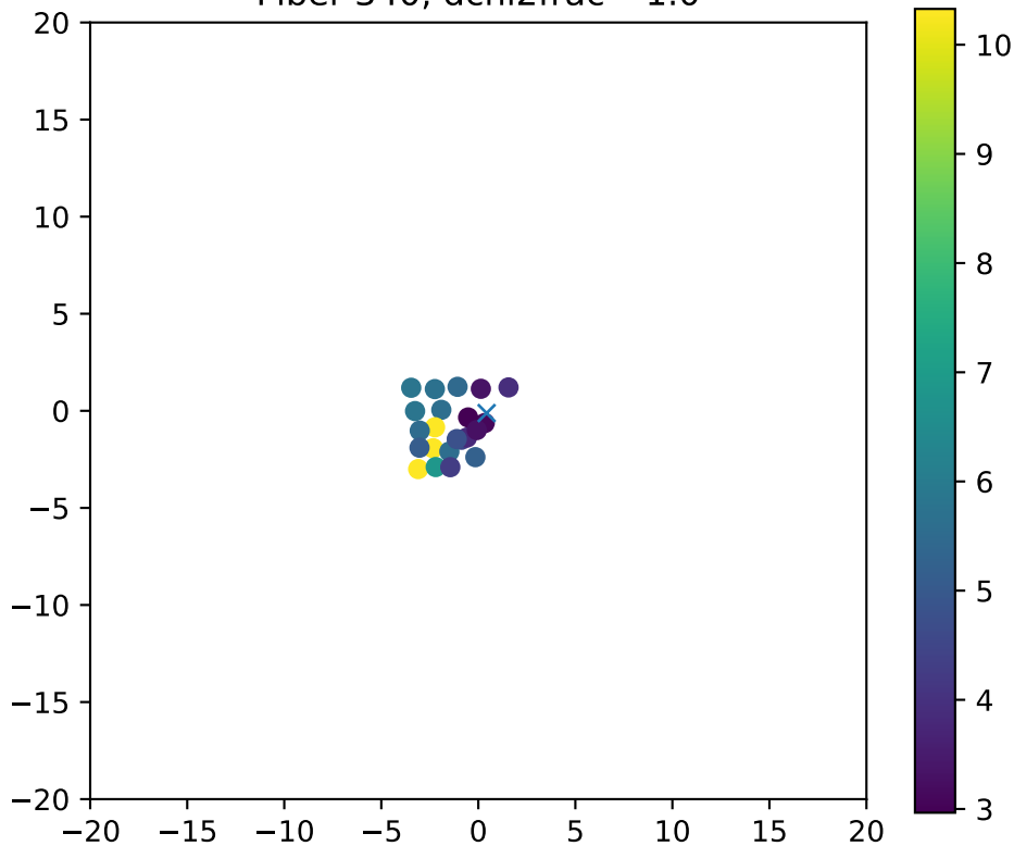
Fiber 340, dchi2frac= 1.0
