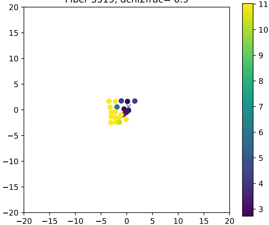
Fiber 3519, dchi2frac= 0.9
