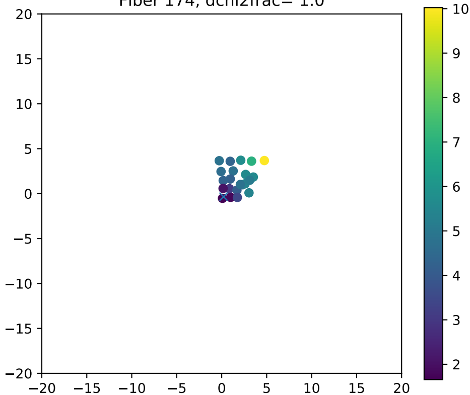
Fiber 174, dchi2frac= 1.0
