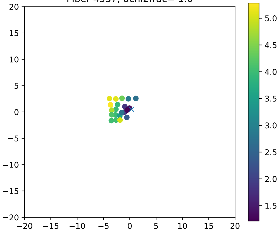
Fiber 4337, dchi2frac= 1.0
