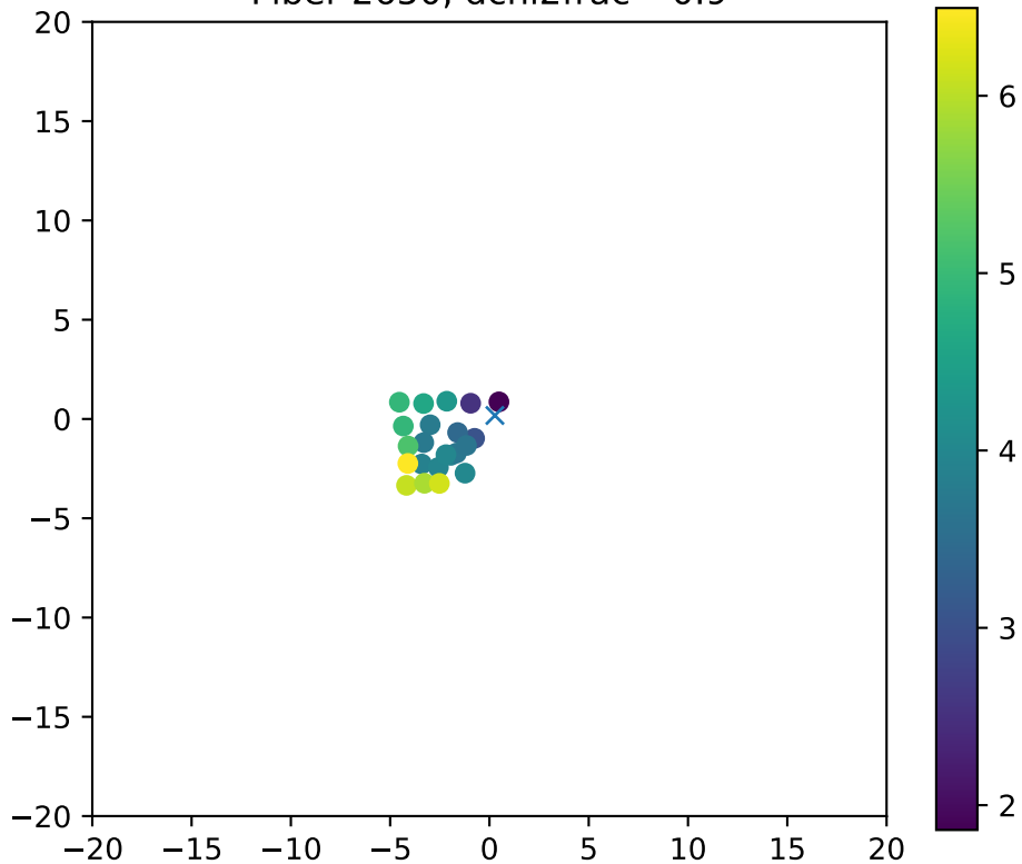
Fiber 2650, dchi2frac= 0.9
