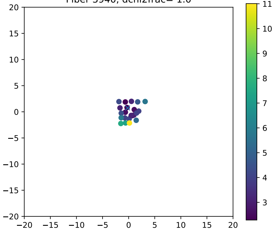
Fiber 3940, dchi2frac= 1.0
