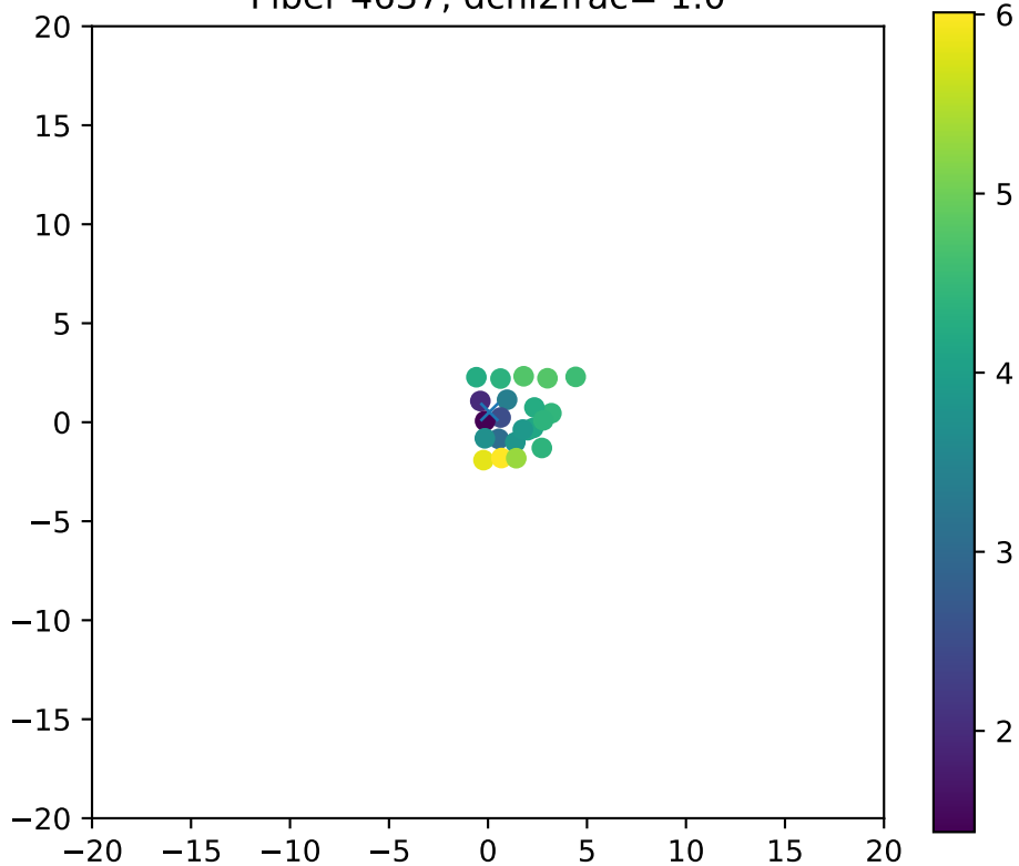
Fiber 4637, dchi2frac= 1.0
