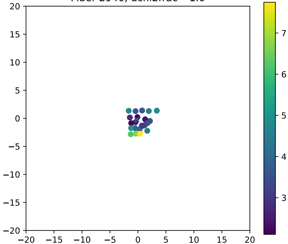
Fiber 2940, dchi2frac= 1.0
