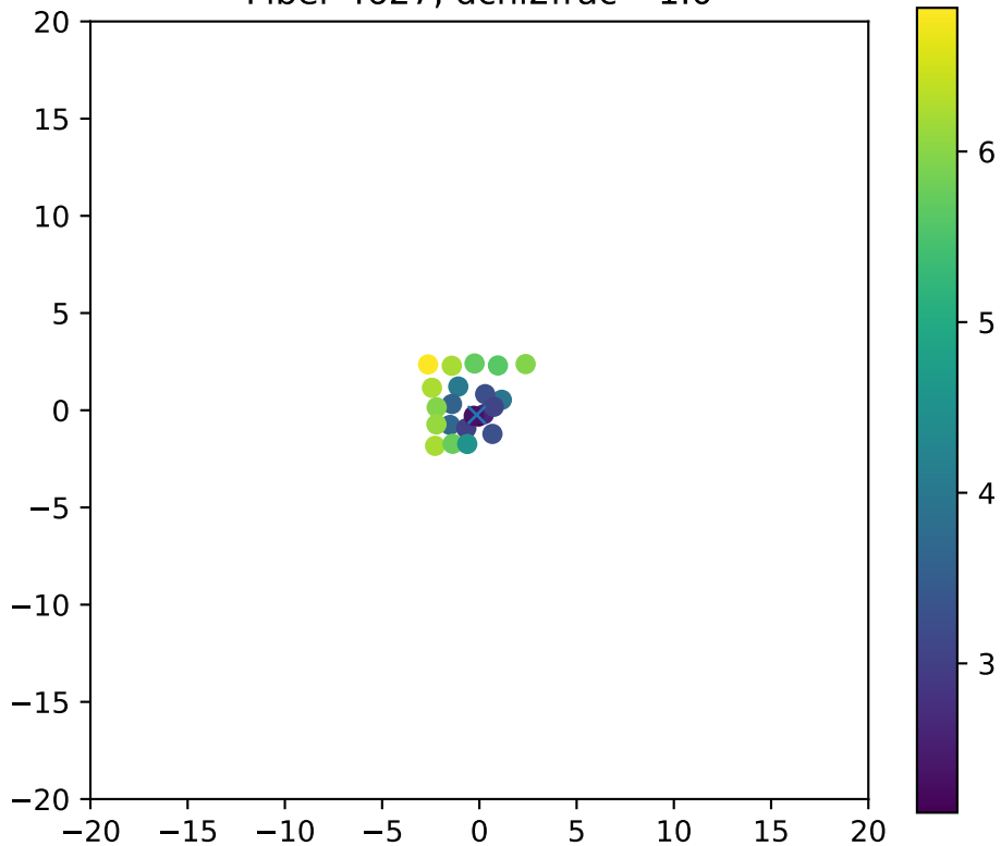
Fiber 4627, dchi2frac= 1.0
