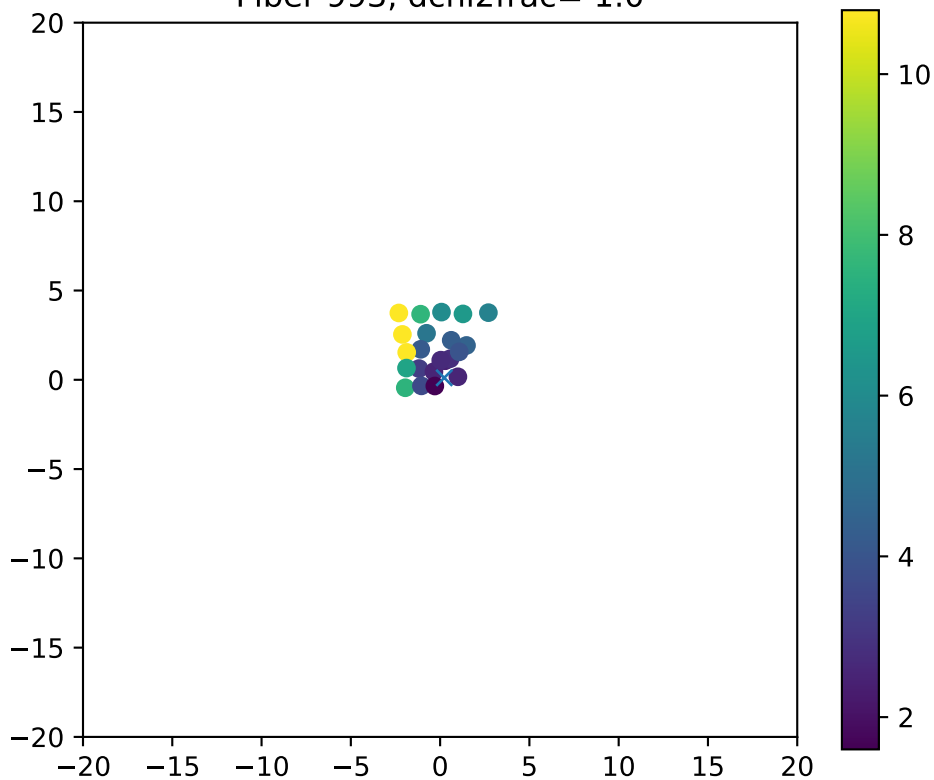
Fiber 993, dchi2frac= 1.0
