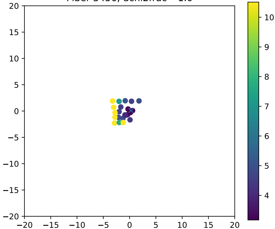
Fiber 3456, dchi2frac= 1.0
