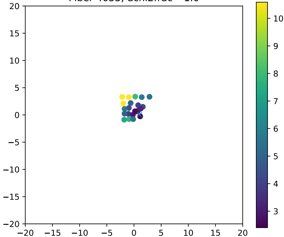
Fiber 4053, dchi2frac= 1.0
