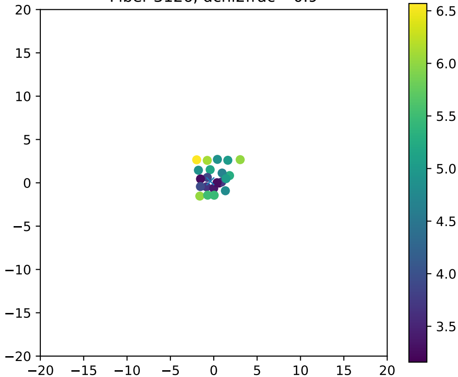
Fiber 3126, dchi2frac= 0.9
