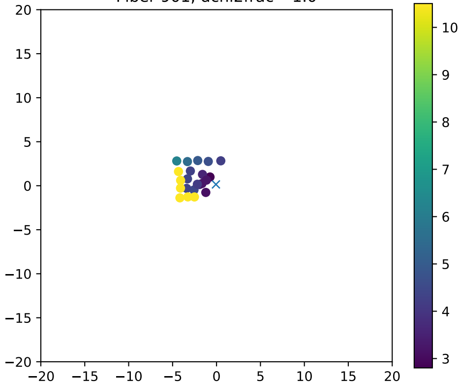
Fiber 901, dchi2frac= 1.0
