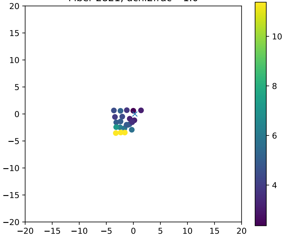
Fiber 2821, dchi2frac= 1.0
