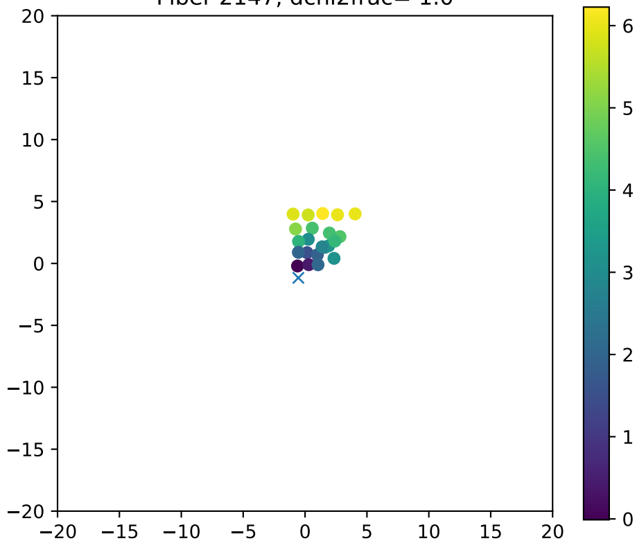
Fiber 2147, dchi2frac= 1.0
