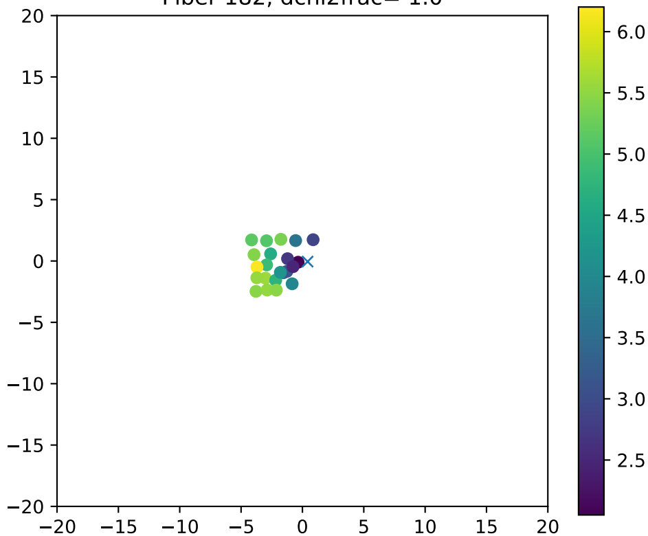
Fiber 182, dchi2frac= 1.0
