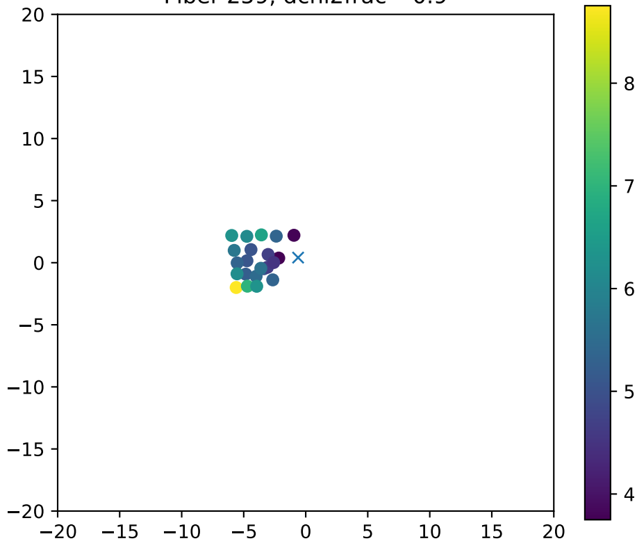
Fiber 259, dchi2frac= 0.9
