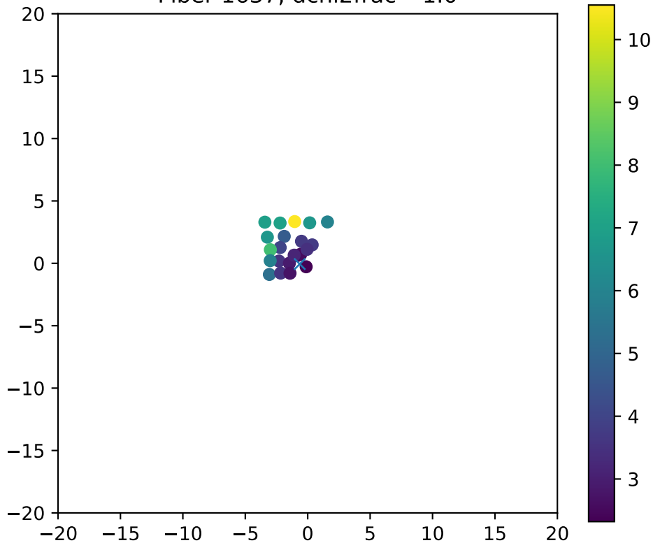
Fiber 1637, dchi2frac= 1.0
