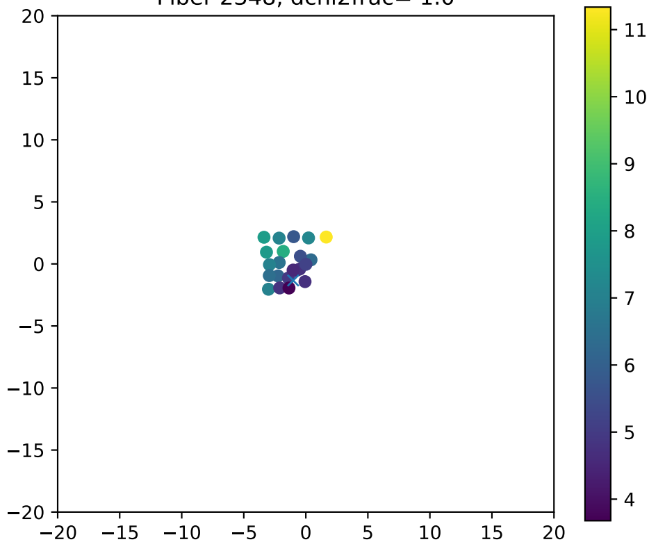
Fiber 2348, dchi2frac= 1.0
