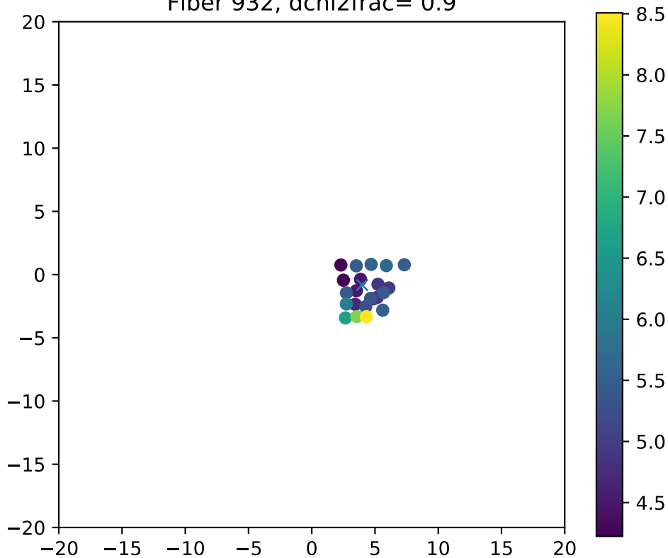
Fiber 932, dchi2frac= 0.9
