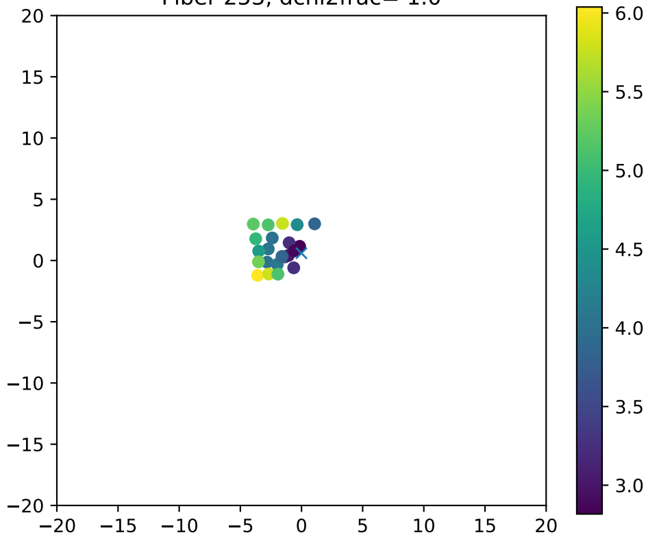
Fiber 253, dchi2frac= 1.0
