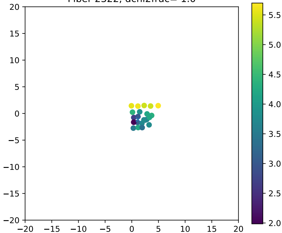
Fiber 2322, dchi2frac= 1.0
