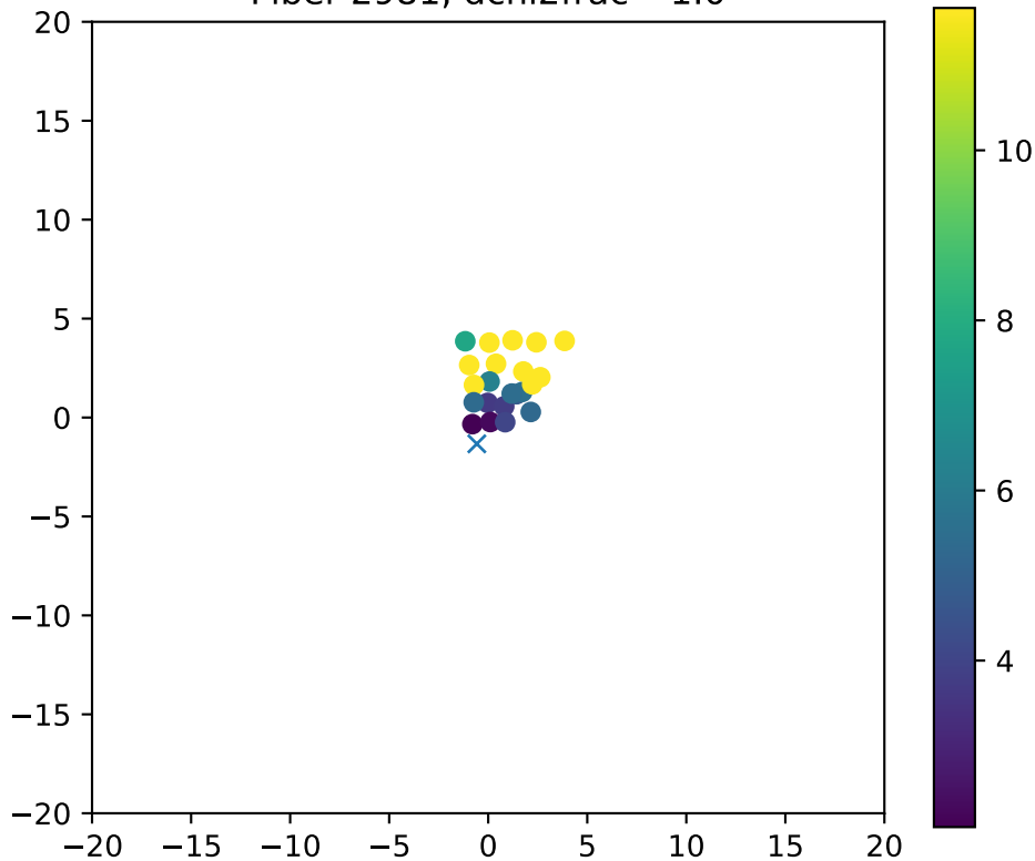
Fiber 2981, dchi2frac= 1.0
