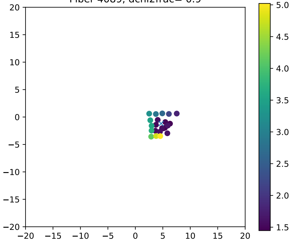
Fiber 4089, dchi2frac= 0.9
