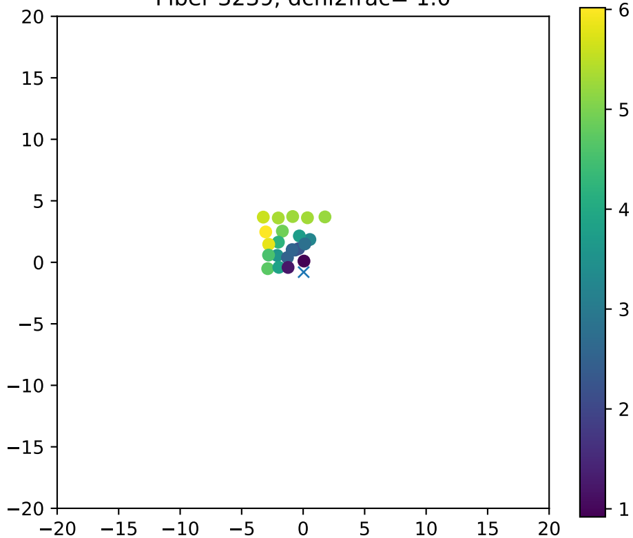
Fiber 3239, dchi2frac= 1.0
