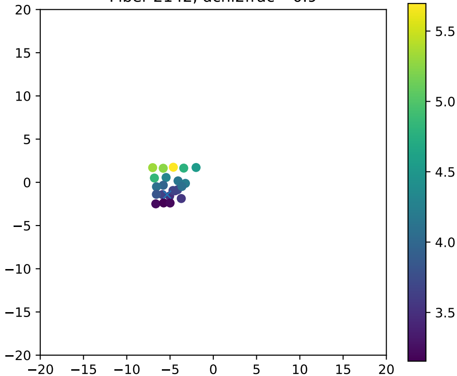
Fiber 2142, dchi2frac= 0.9
