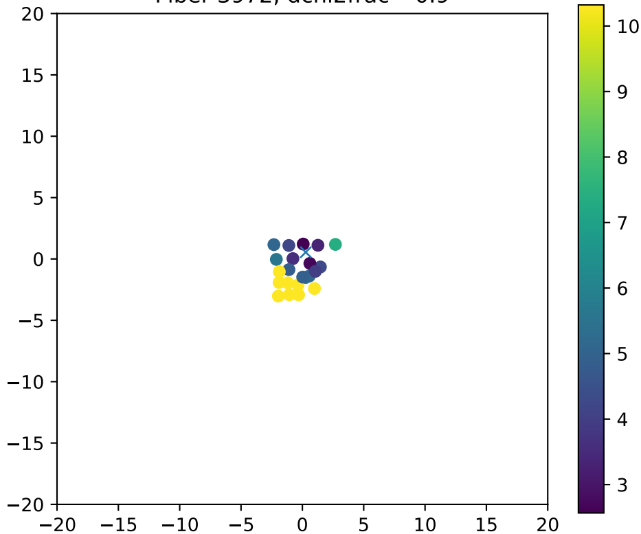
Fiber 3972, dchi2frac= 0.9
