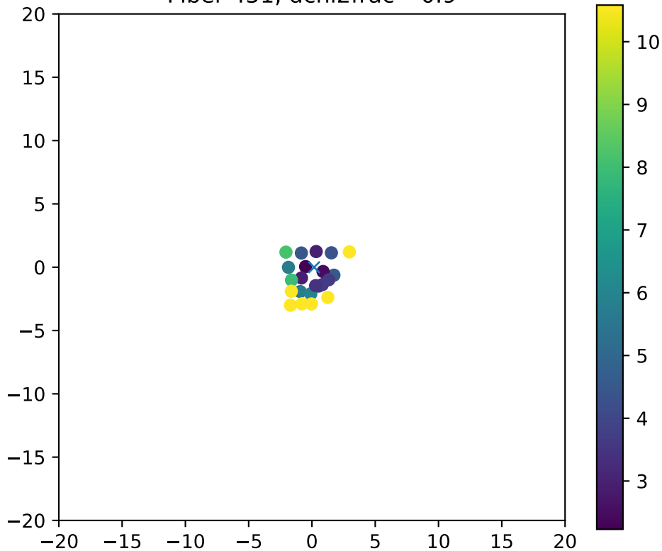
Fiber 451, dchi2frac= 0.9
