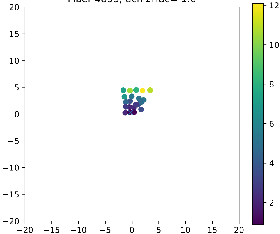
Fiber 4893, dchi2frac= 1.0
