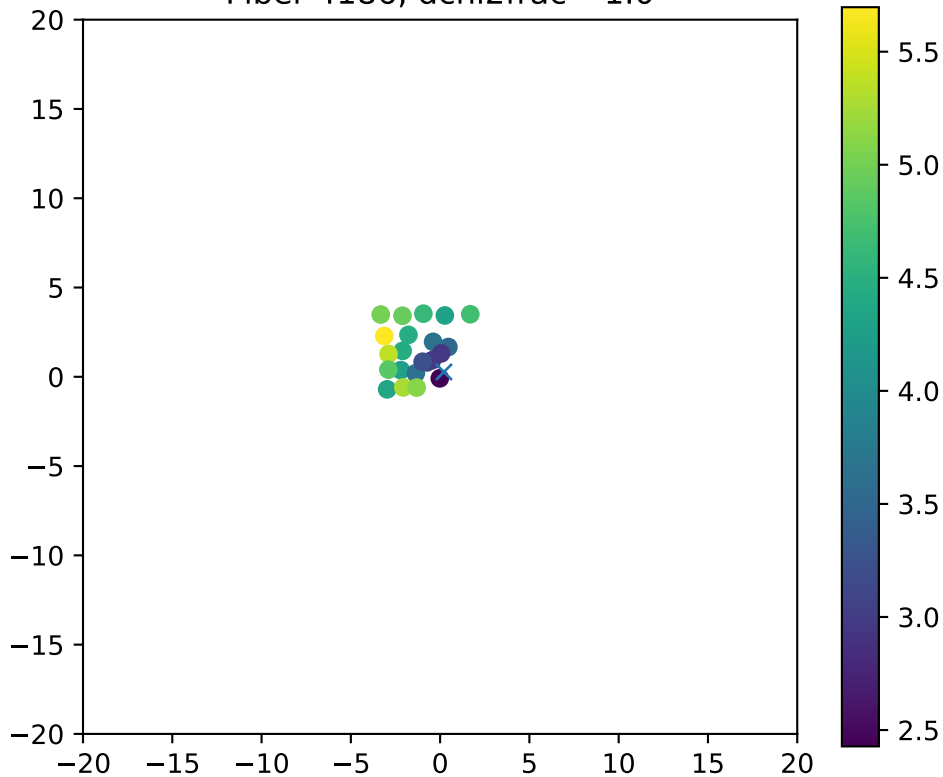
Fiber 4186, dchi2frac= 1.0
