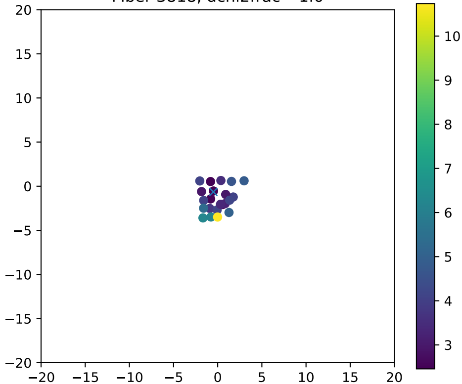
Fiber 3818, dchi2frac= 1.0
