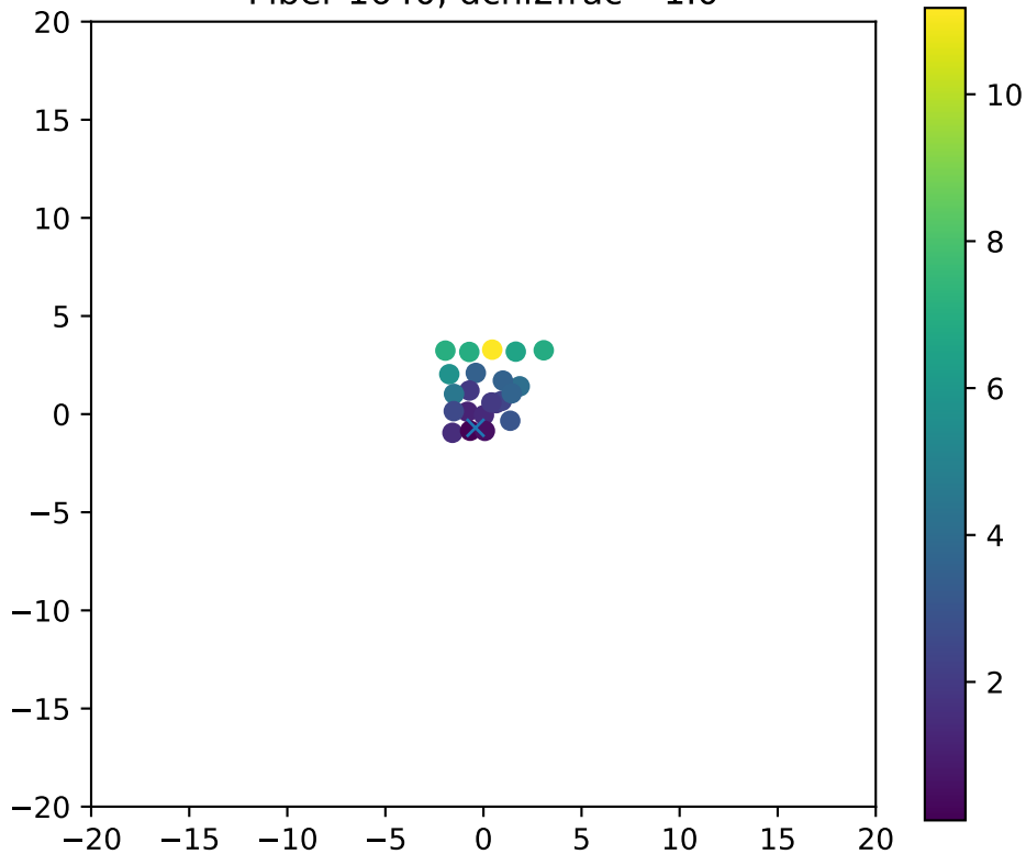
Fiber 1640, dchi2frac= 1.0
