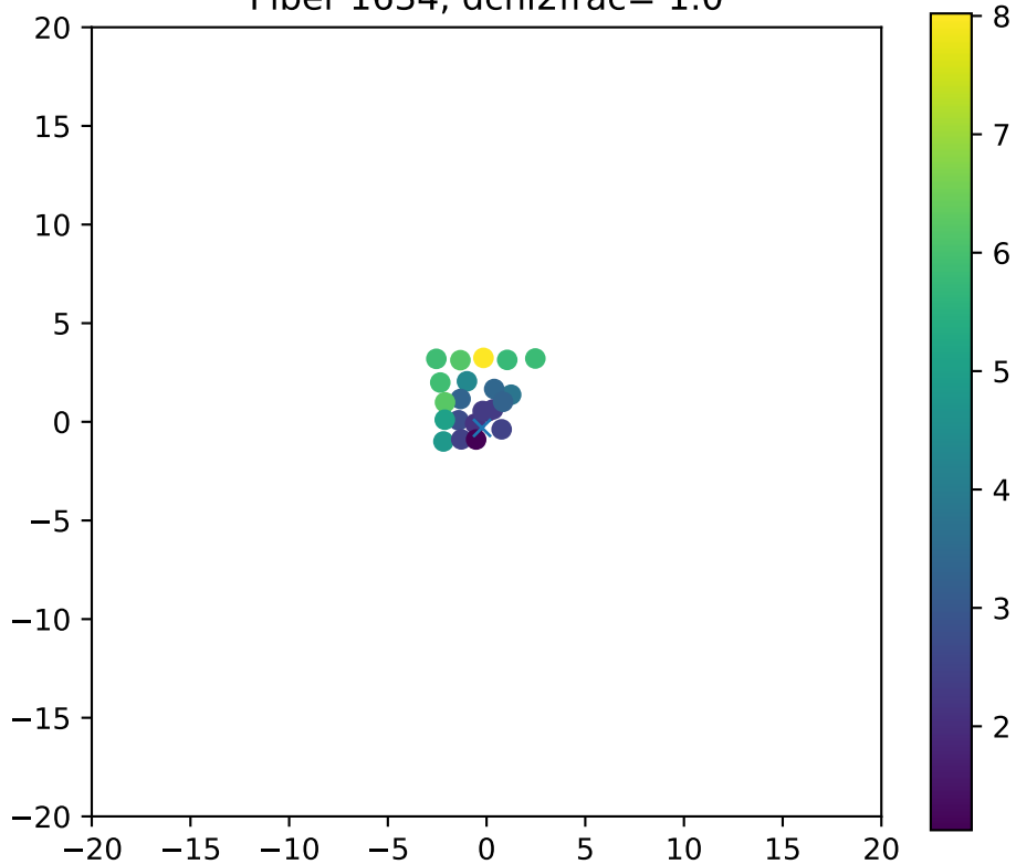
Fiber 1634, dchi2frac= 1.0
