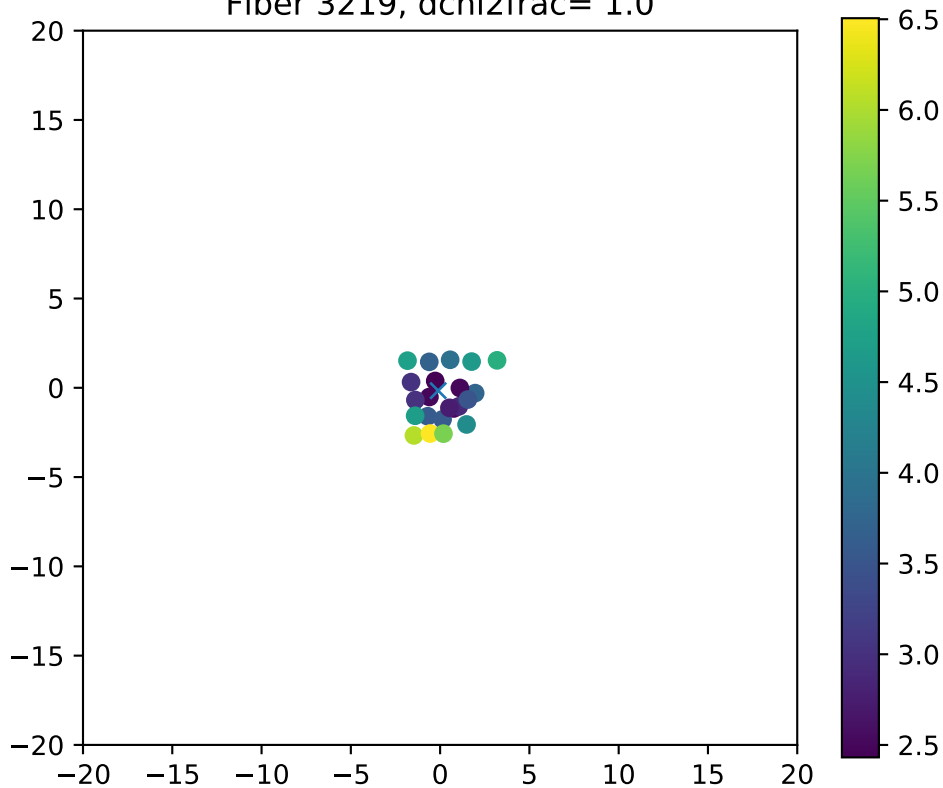
Fiber 3219, dchi2frac= 1.0
