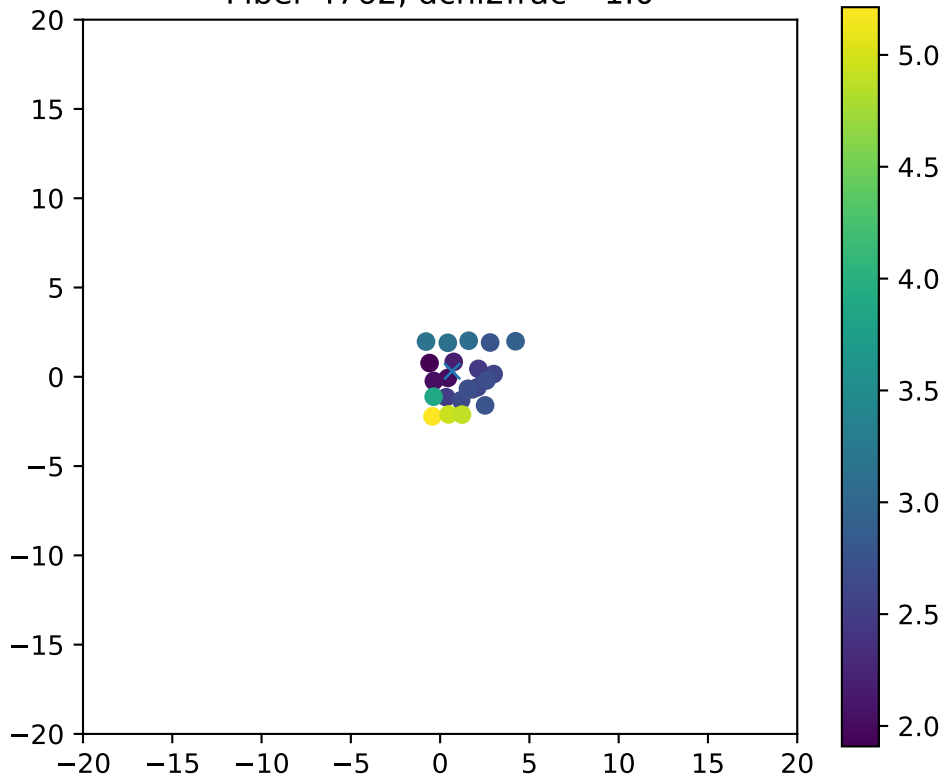
Fiber 4762, dchi2frac= 1.0
