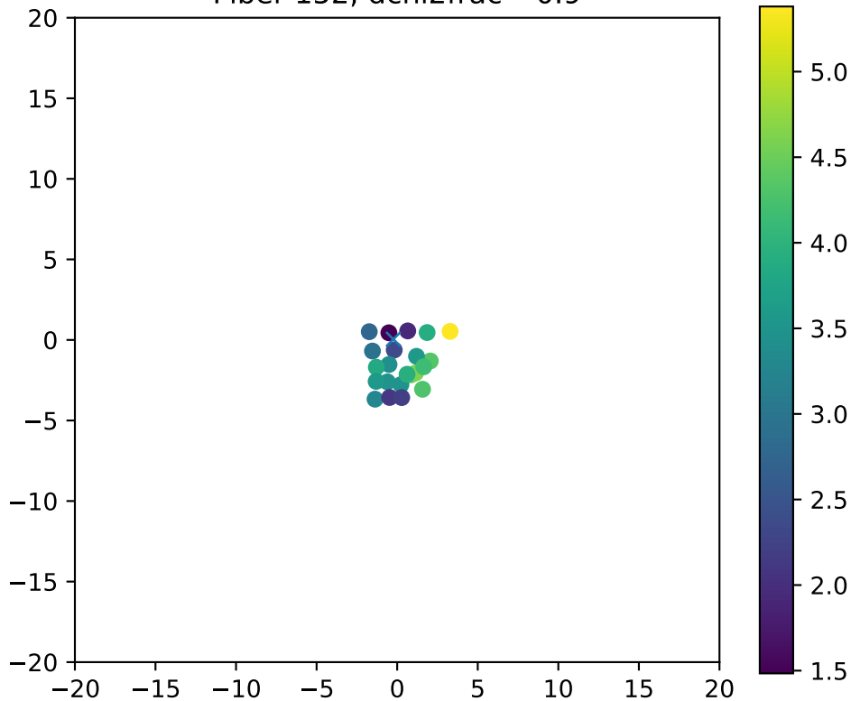
Fiber 152, dchi2frac= 0.9
