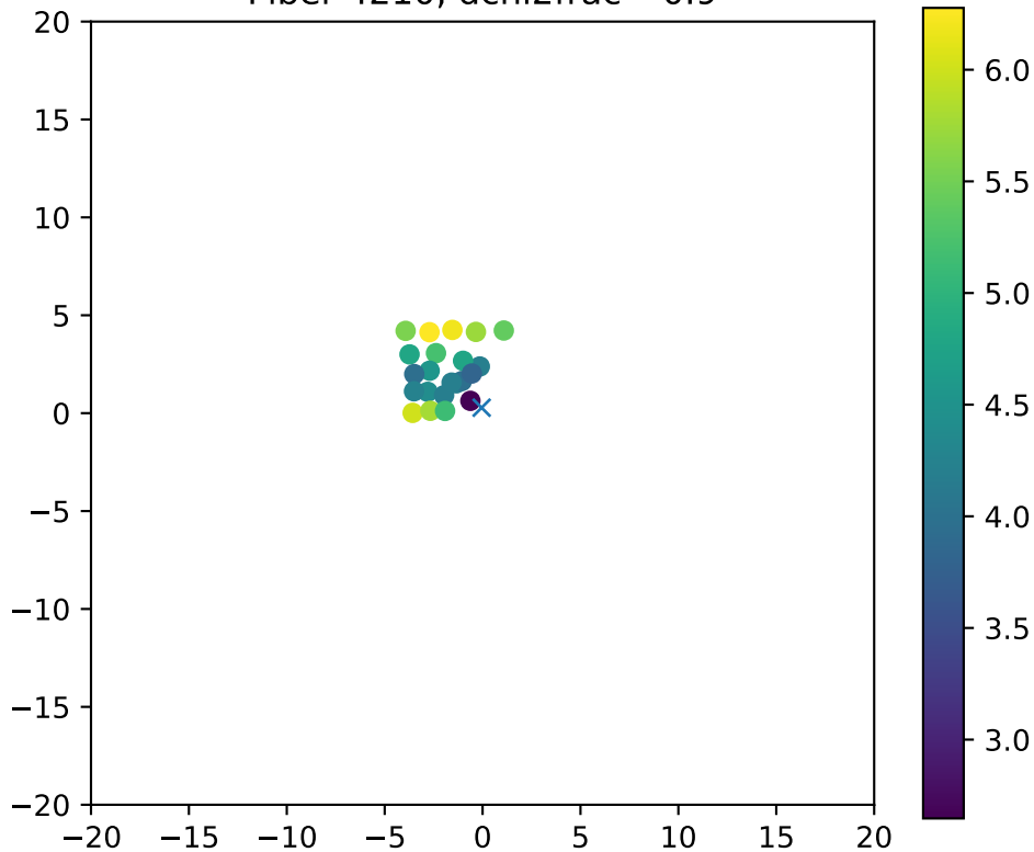
Fiber 4210, dchi2frac= 0.9
