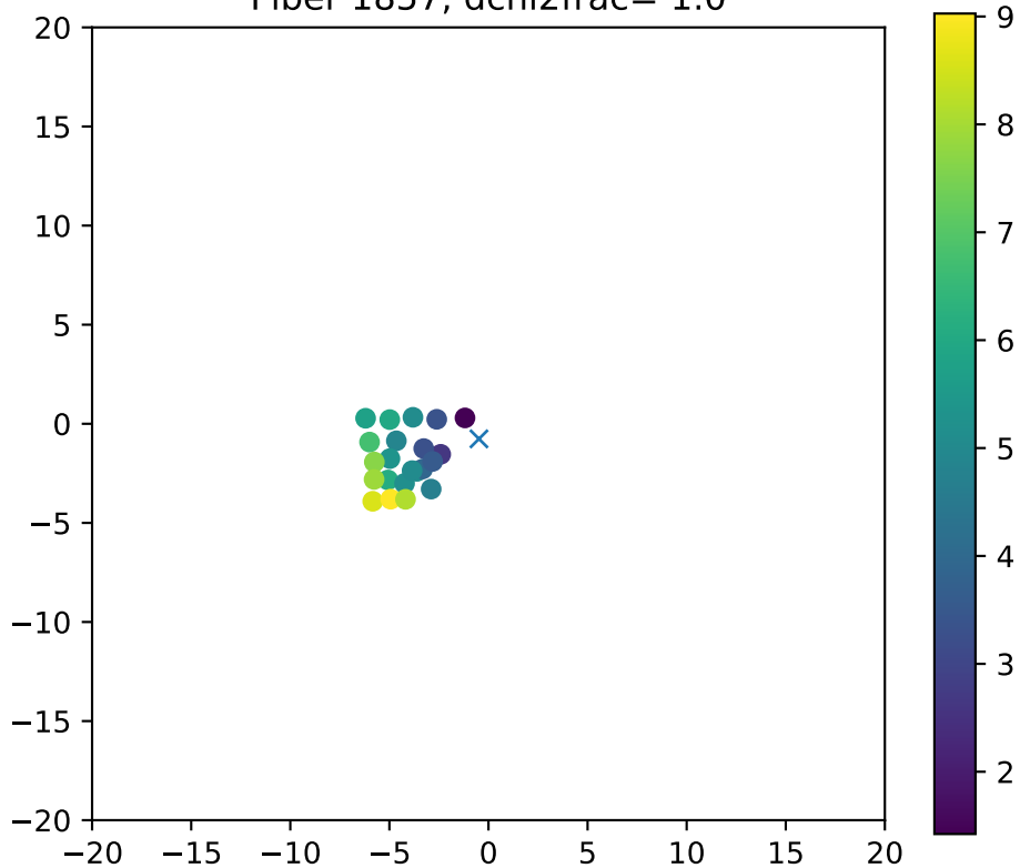
Fiber 1857, dchi2frac= 1.0
