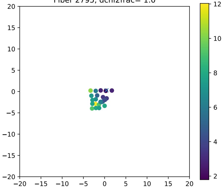
Fiber 2795, dchi2frac= 1.0
