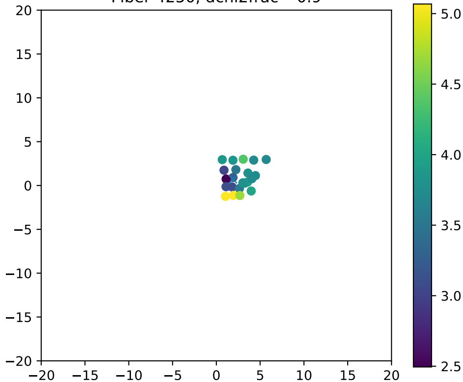
Fiber 4250, dchi2frac= 0.9
