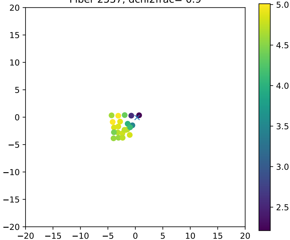
Fiber 2537, dchi2frac= 0.9
