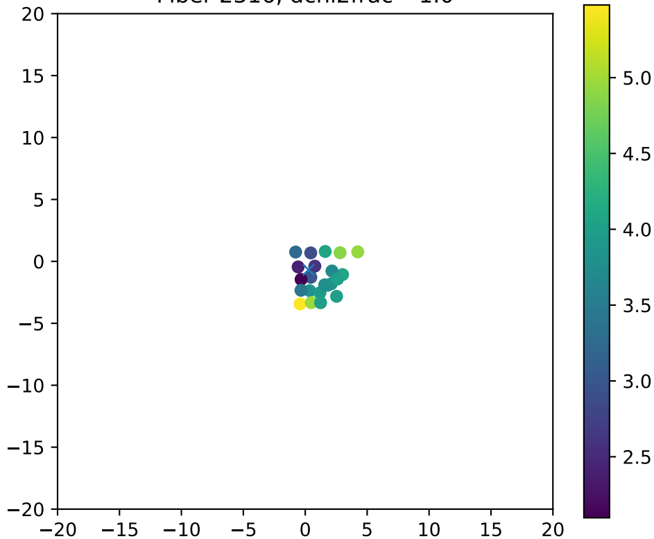
Fiber 2316, dchi2frac= 1.0
