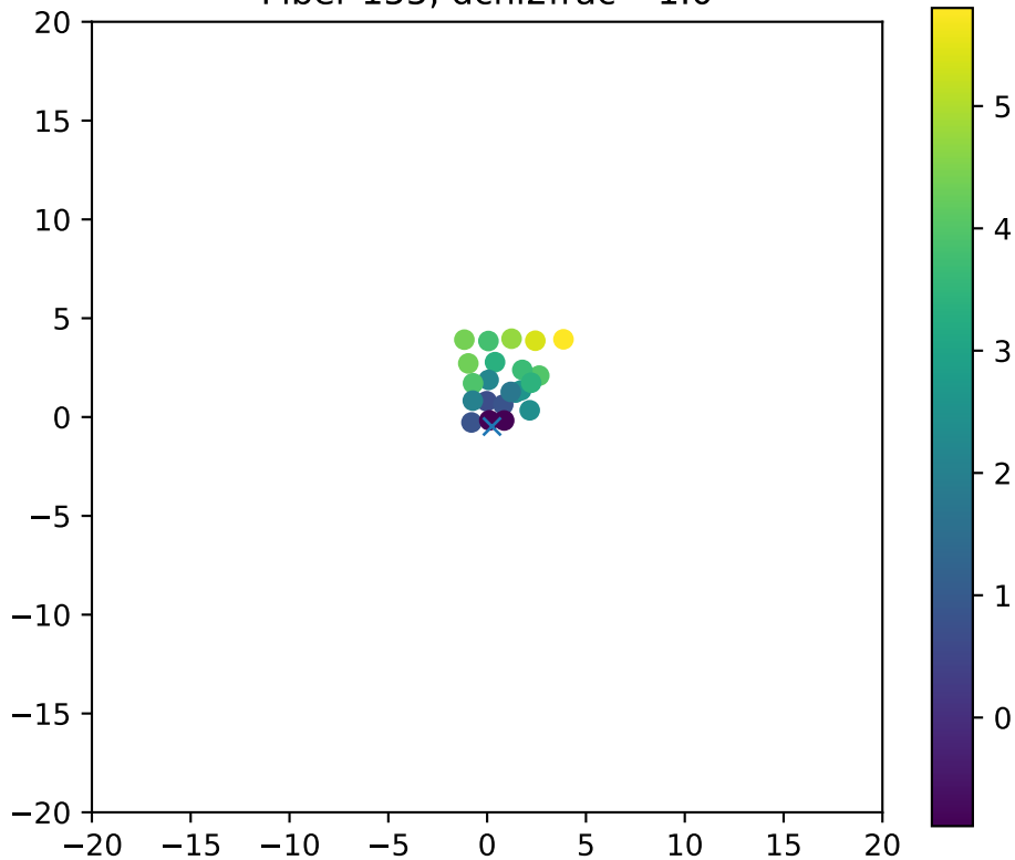
Fiber 155, dchi2frac= 1.0
