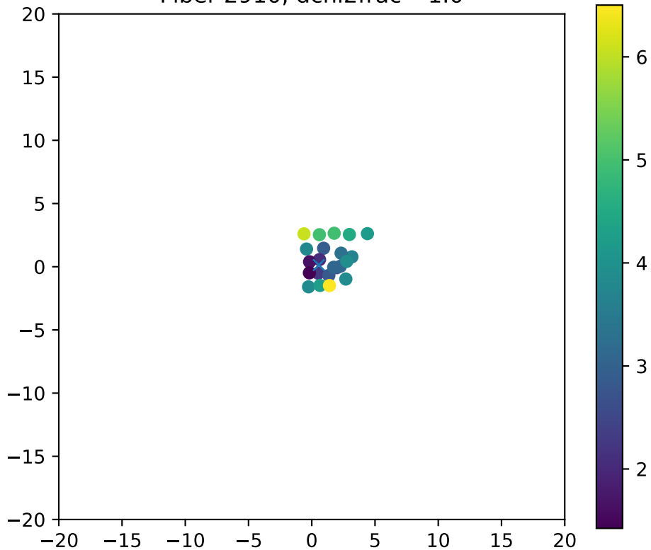
Fiber 2910, dchi2frac= 1.0
