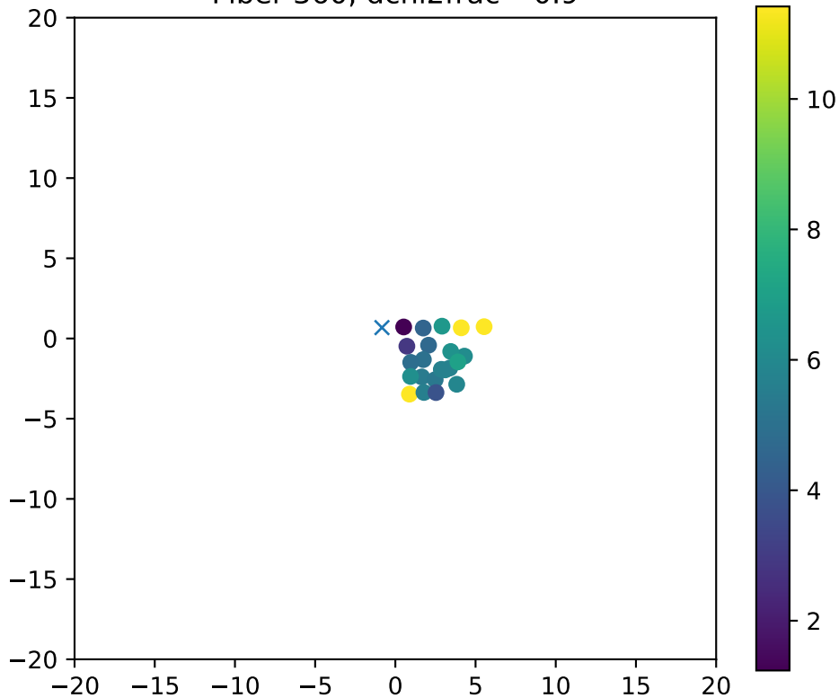
Fiber 360, dchi2frac= 0.9
