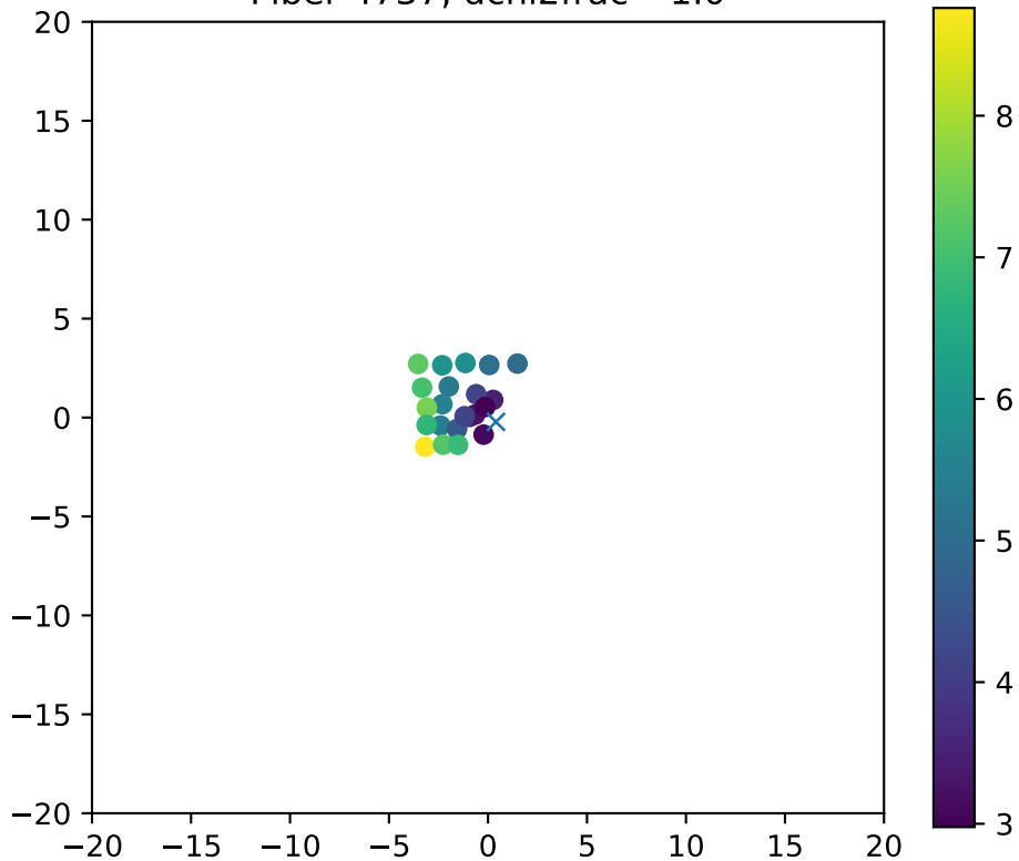
Fiber 4737, dchi2frac= 1.0
