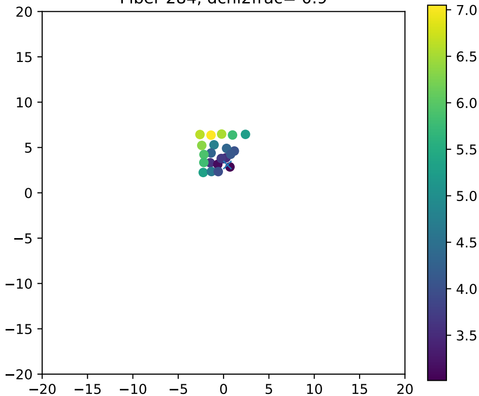
Fiber 284, dchi2frac= 0.9
