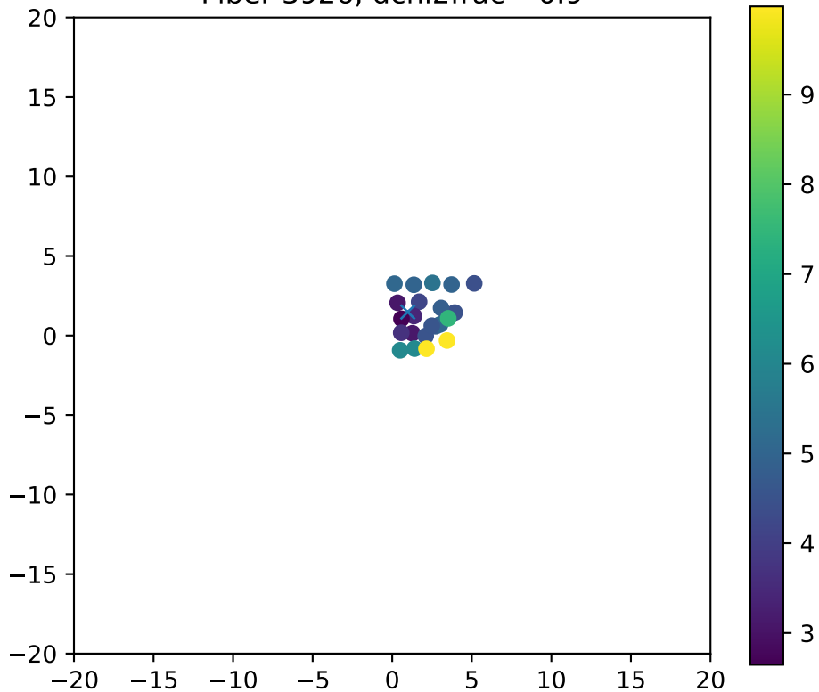
Fiber 3926, dchi2frac= 0.9
