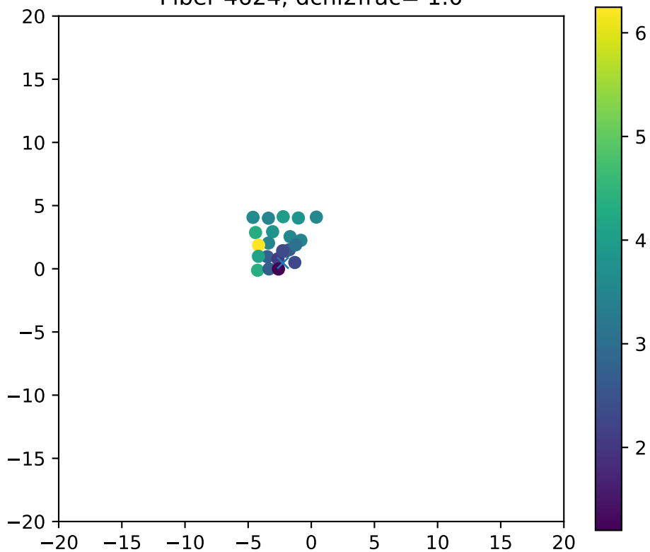
Fiber 4624, dchi2frac= 1.0
