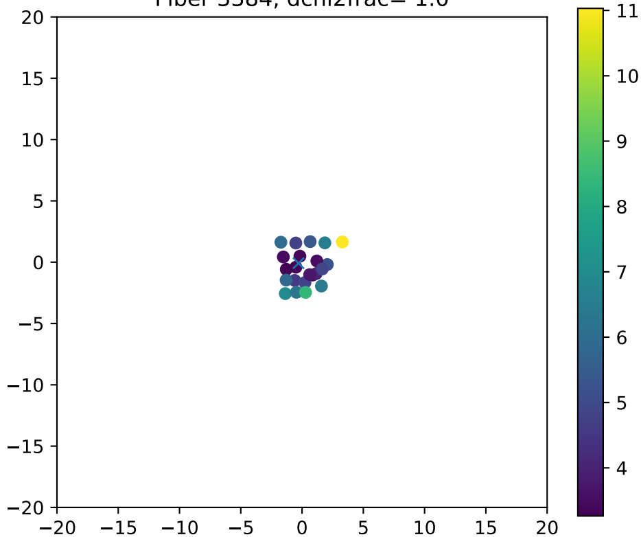
Fiber 3384, dchi2frac= 1.0
