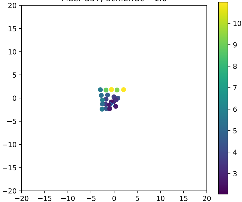
Fiber 557, dchi2frac= 1.0
