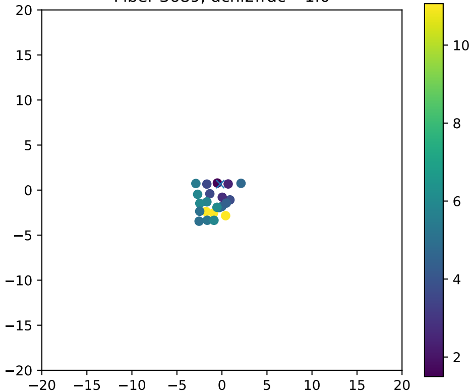
Fiber 3689, dchi2frac= 1.0
