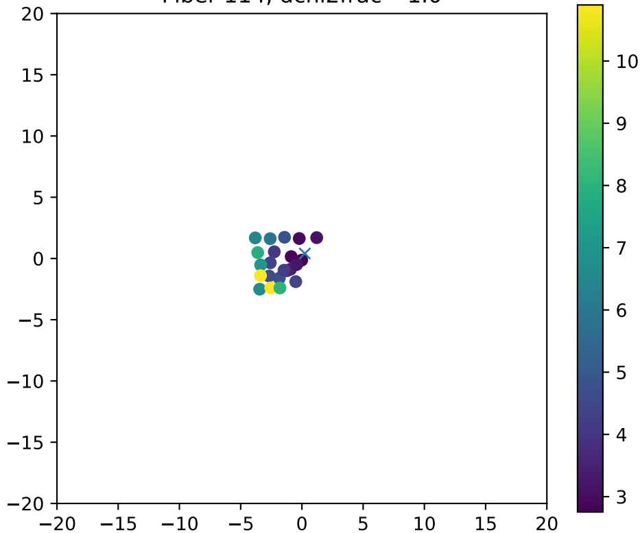
Fiber 114, dchi2frac= 1.0
