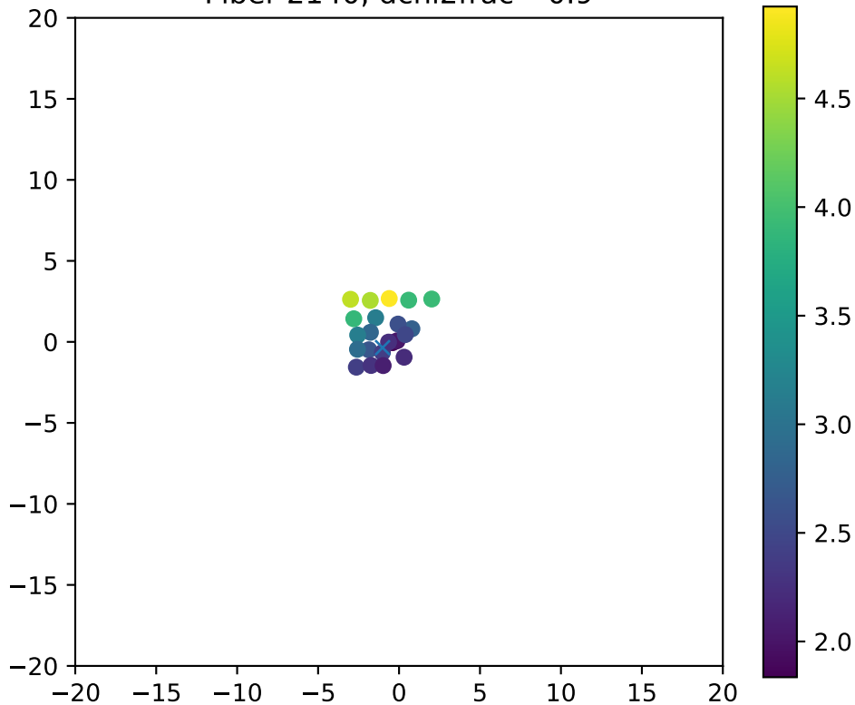
Fiber 2140, dchi2frac= 0.9
