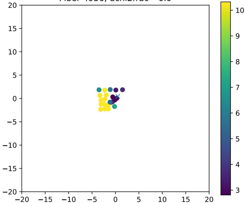
Fiber 4956, dchi2frac= 0.9
