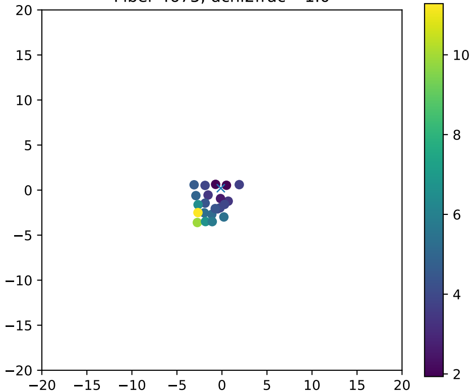
Fiber 4675, dchi2frac= 1.0
