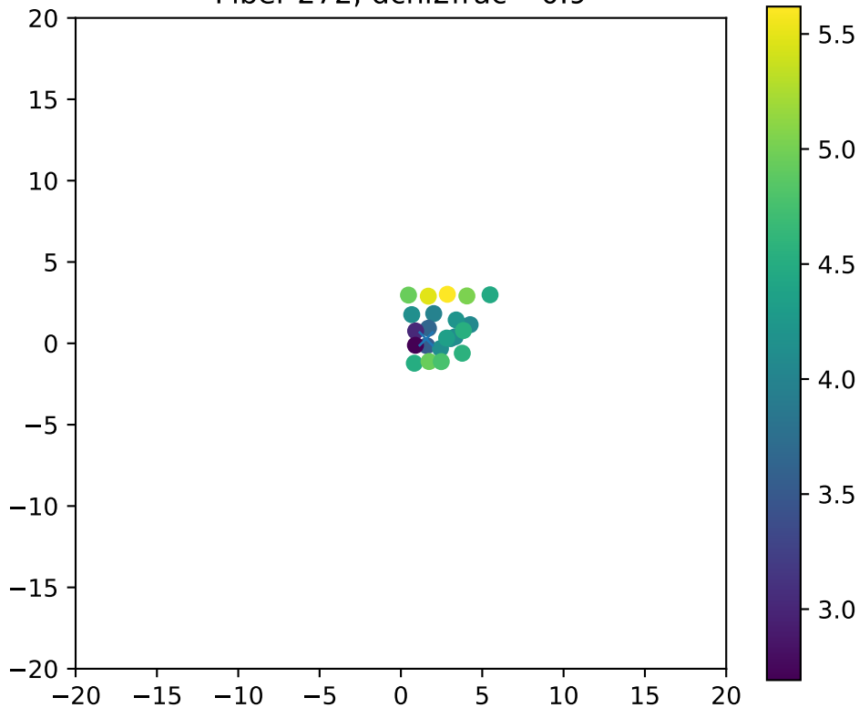
Fiber 272, dchi2frac= 0.9
