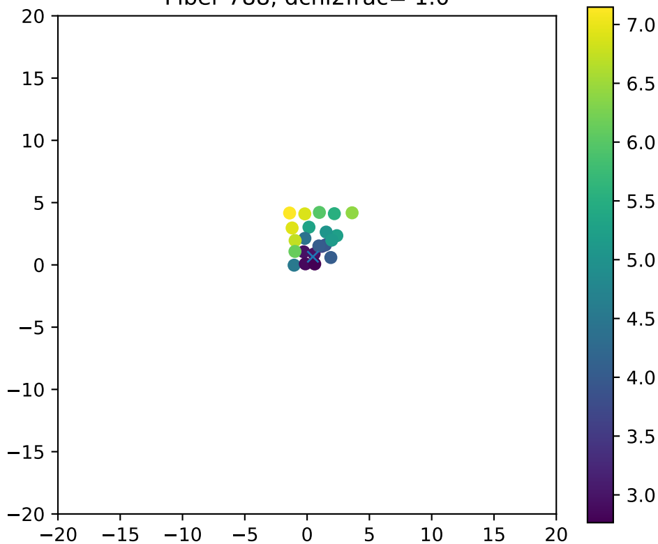
Fiber 788, dchi2frac= 1.0
