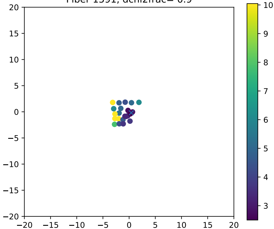
Fiber 1591, dchi2frac= 0.9
