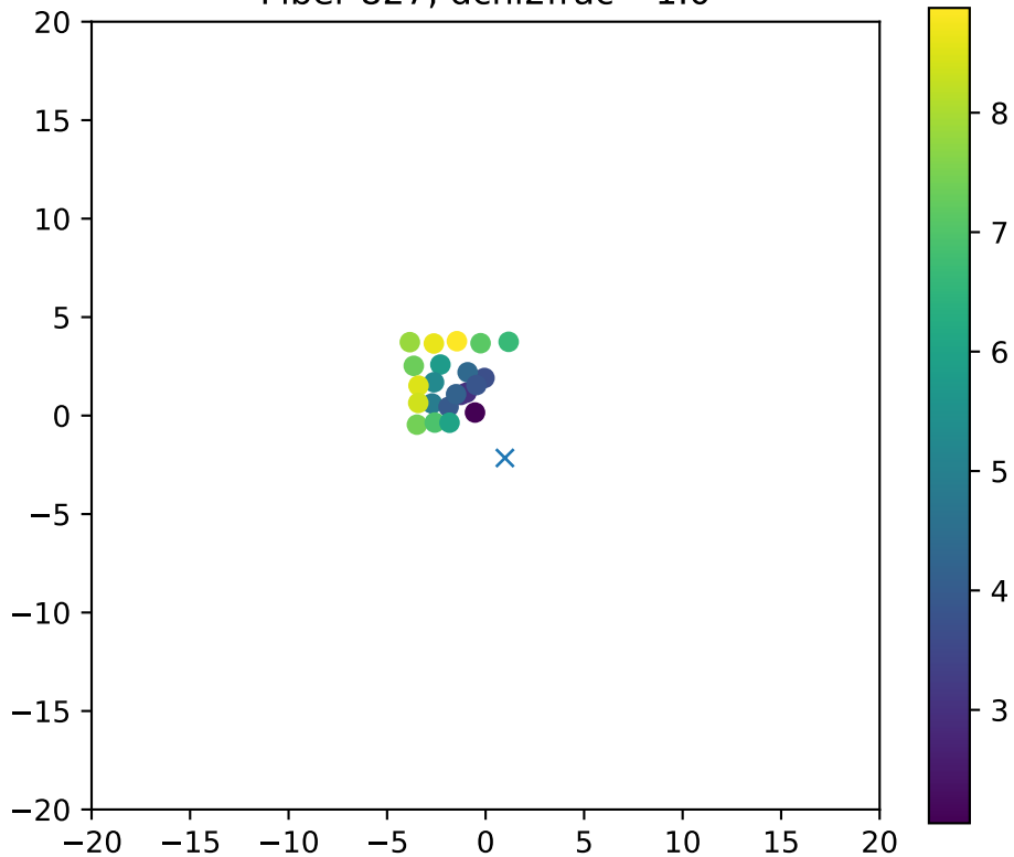
Fiber 827, dchi2frac= 1.0
