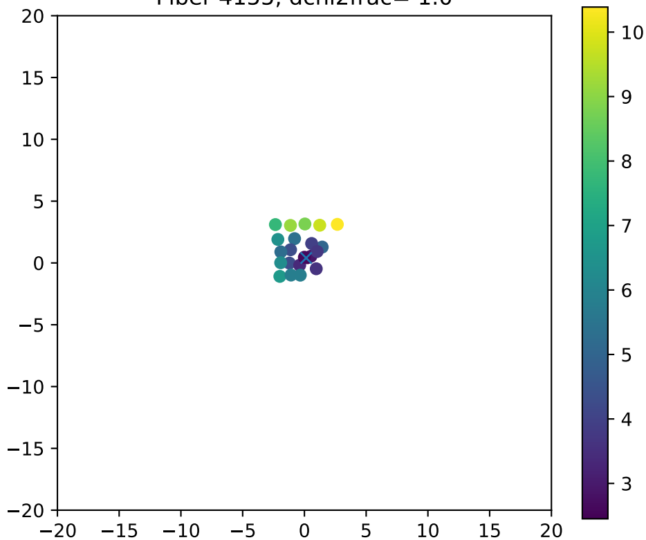
Fiber 4155, dchi2frac= 1.0
