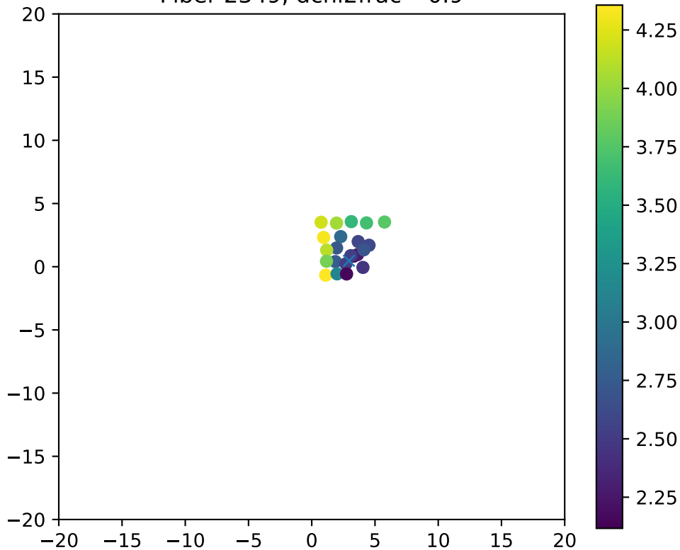
Fiber 2349, dchi2frac= 0.9
