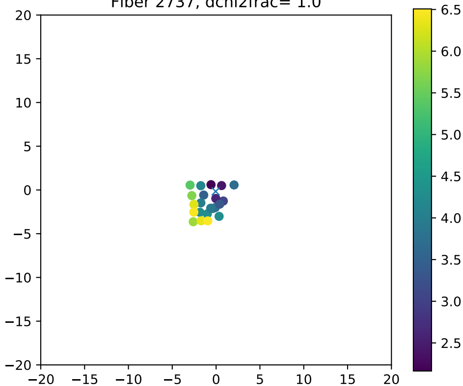
Fiber 2737, dchi2frac= 1.0
