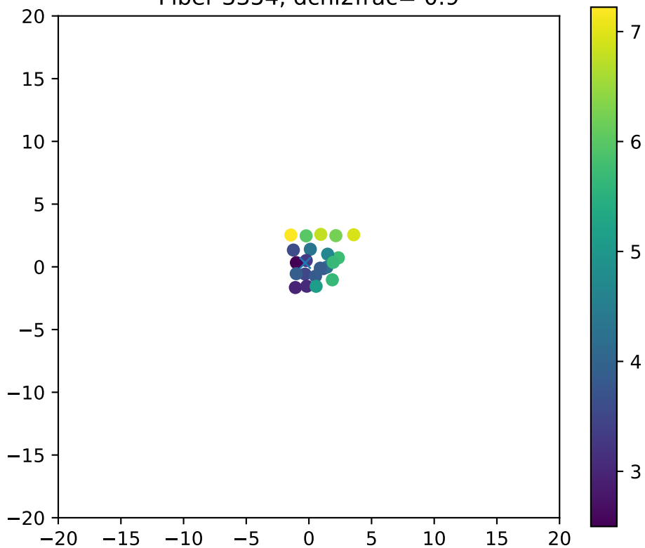
Fiber 3354, dchi2frac= 0.9
