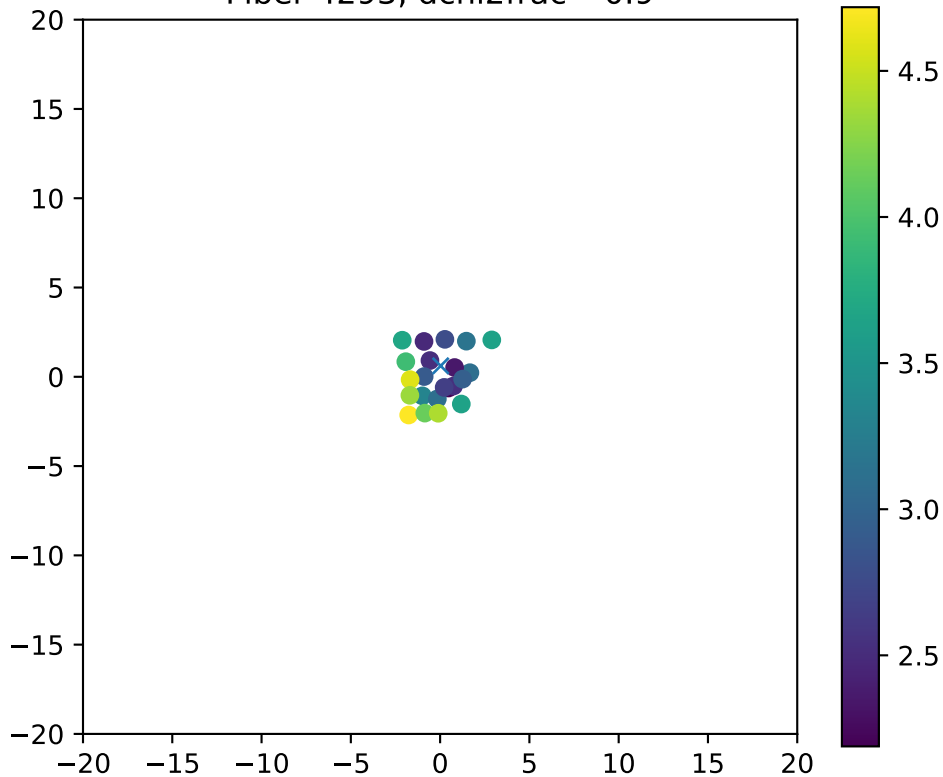
Fiber 4293, dchi2frac= 0.9
