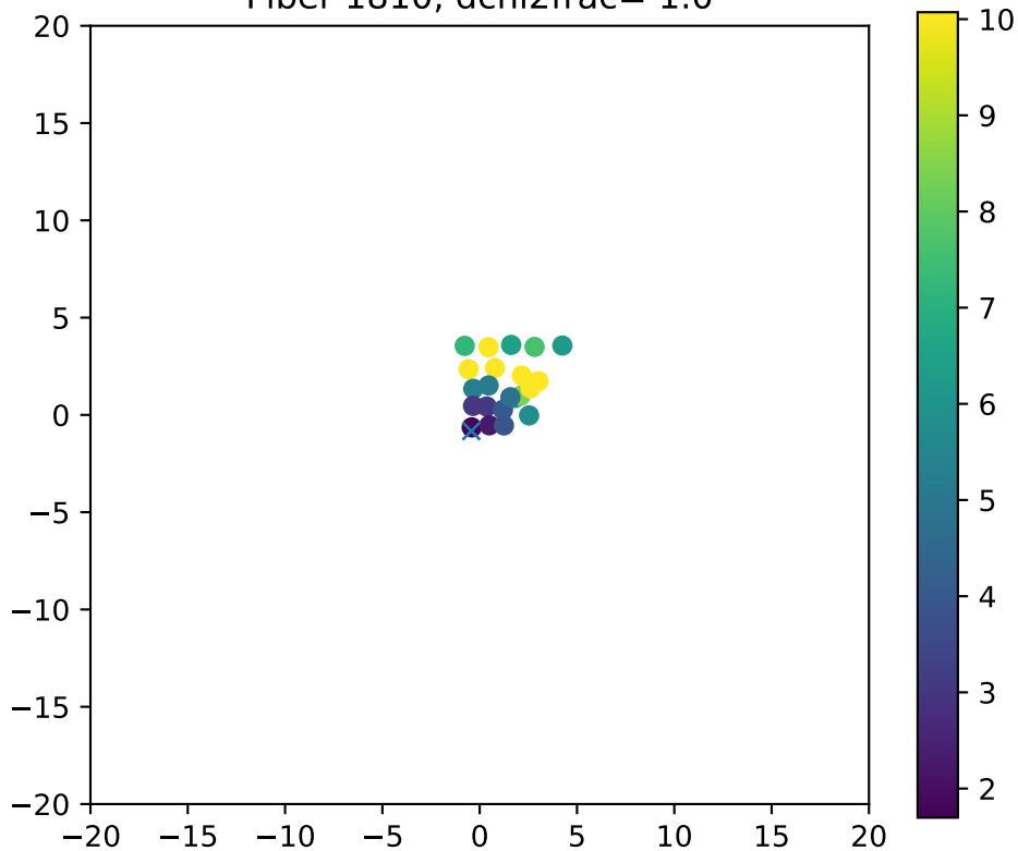
Fiber 1810, dchi2frac= 1.0
