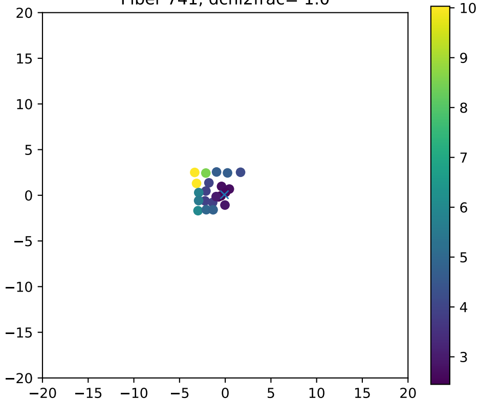
Fiber 741, dchi2frac= 1.0
