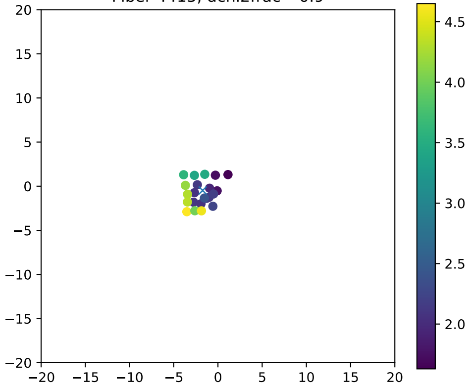
Fiber 4415, dchi2frac= 0.9
