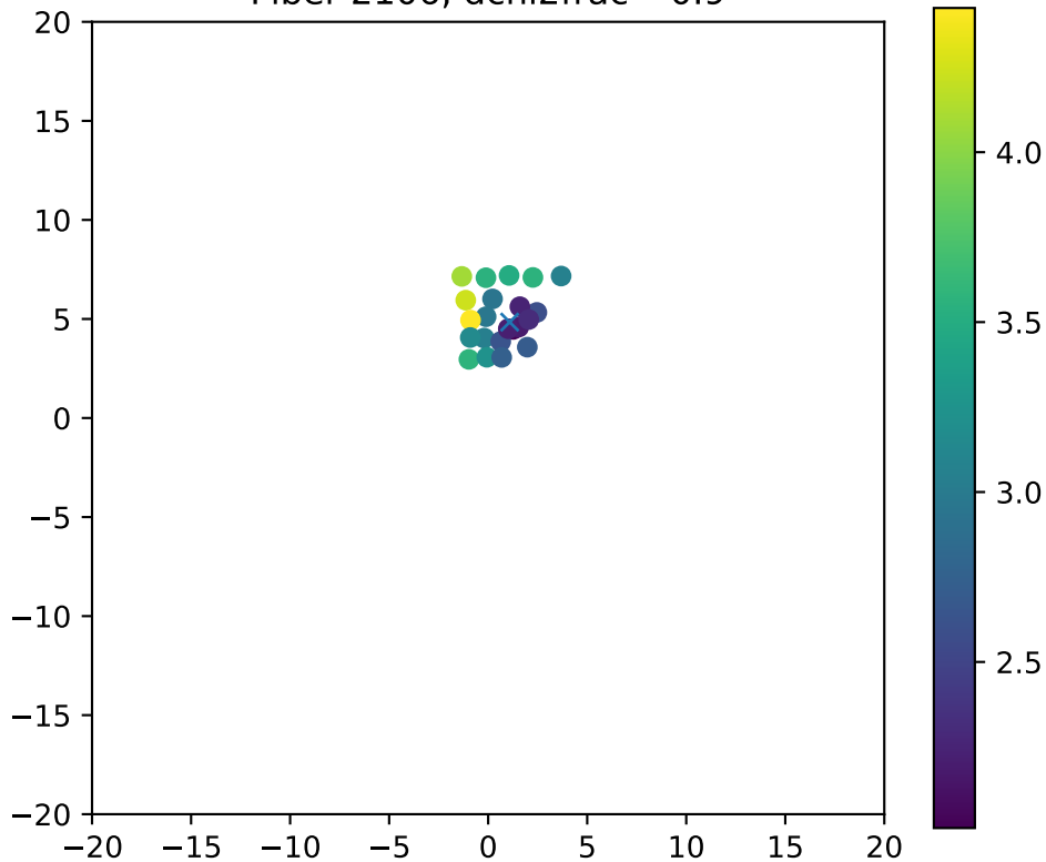
Fiber 2106, dchi2frac= 0.9
