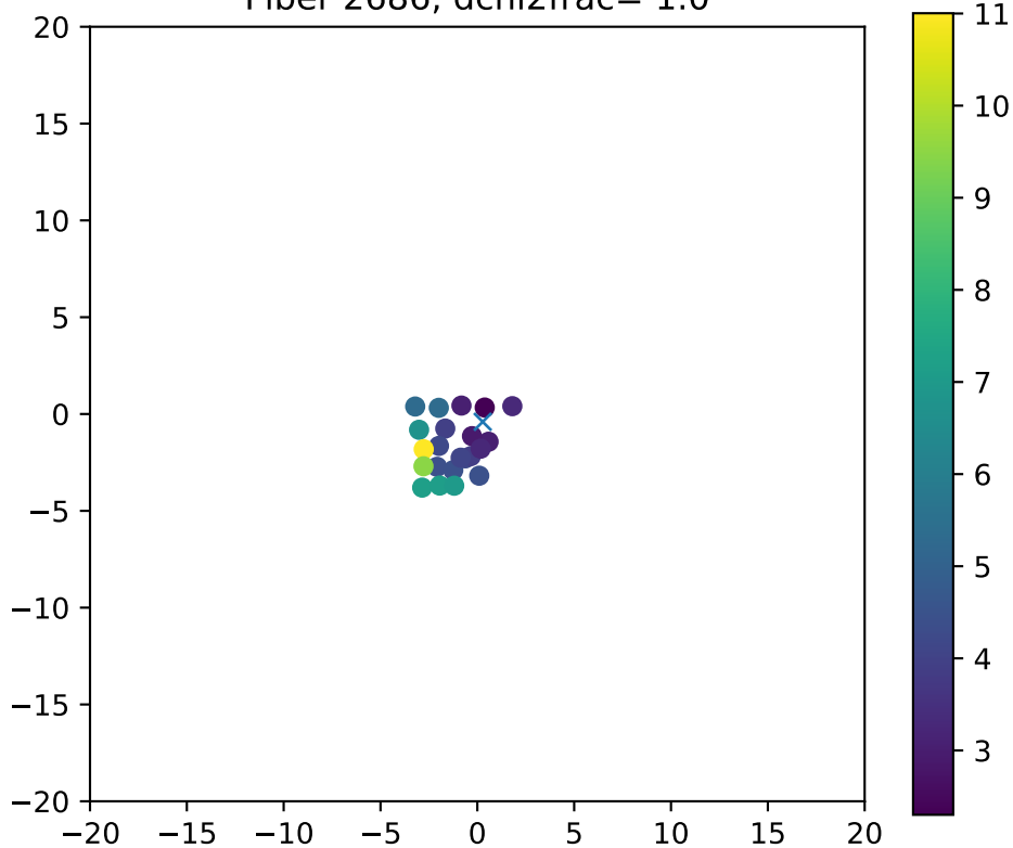
Fiber 2686, dchi2frac= 1.0
