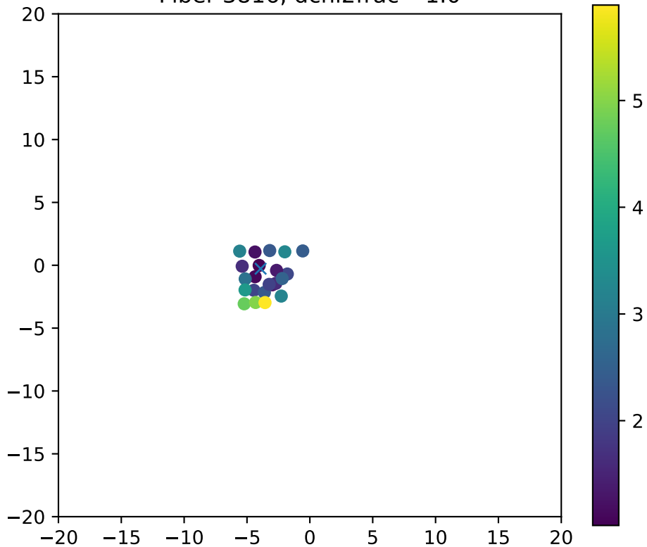
Fiber 3816, dchi2frac= 1.0
