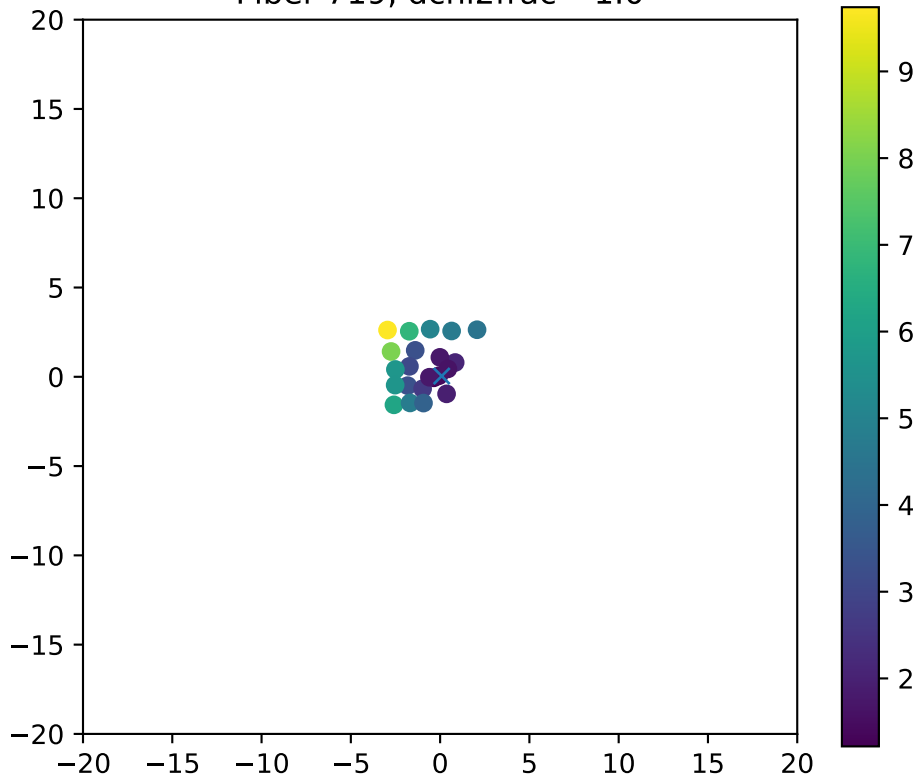
Fiber 719, dchi2frac= 1.0
