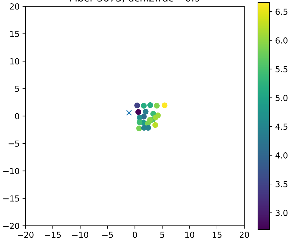
Fiber 3673, dchi2frac= 0.9
