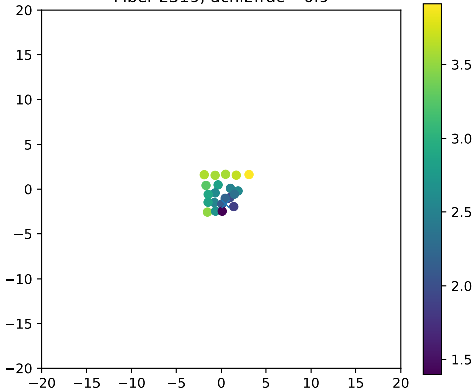
Fiber 2319, dchi2frac= 0.9
