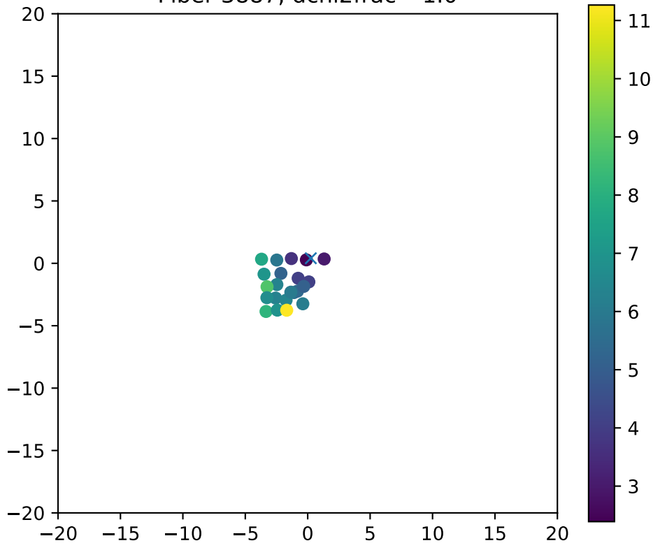
Fiber 3887, dchi2frac= 1.0
