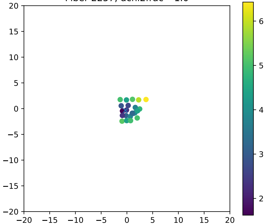
Fiber 2257, dchi2frac= 1.0
