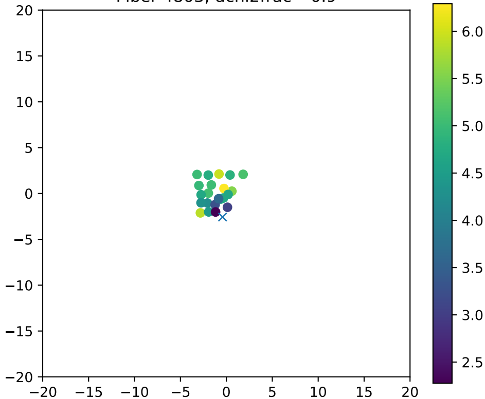
Fiber 4803, dchi2frac= 0.9
