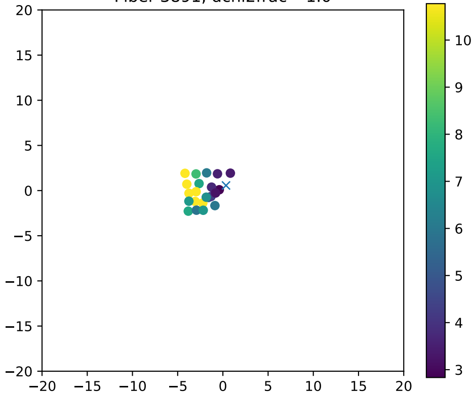
Fiber 3891, dchi2frac= 1.0
