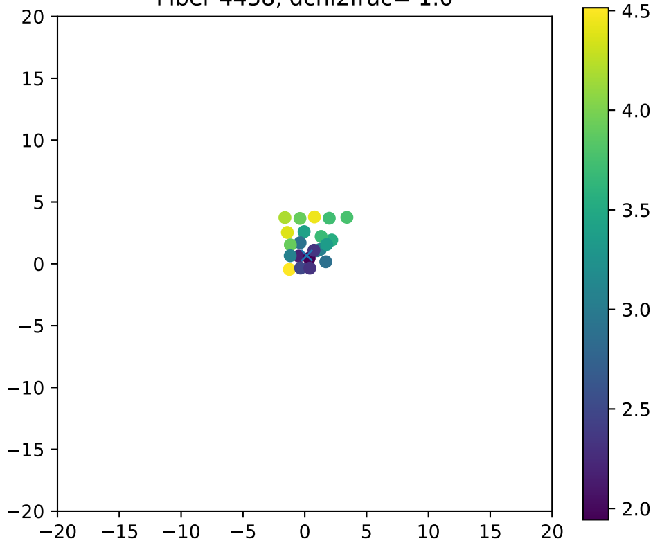
Fiber 4438, dchi2frac= 1.0
