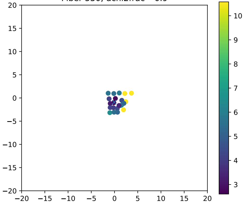
Fiber 530, dchi2frac= 0.9
