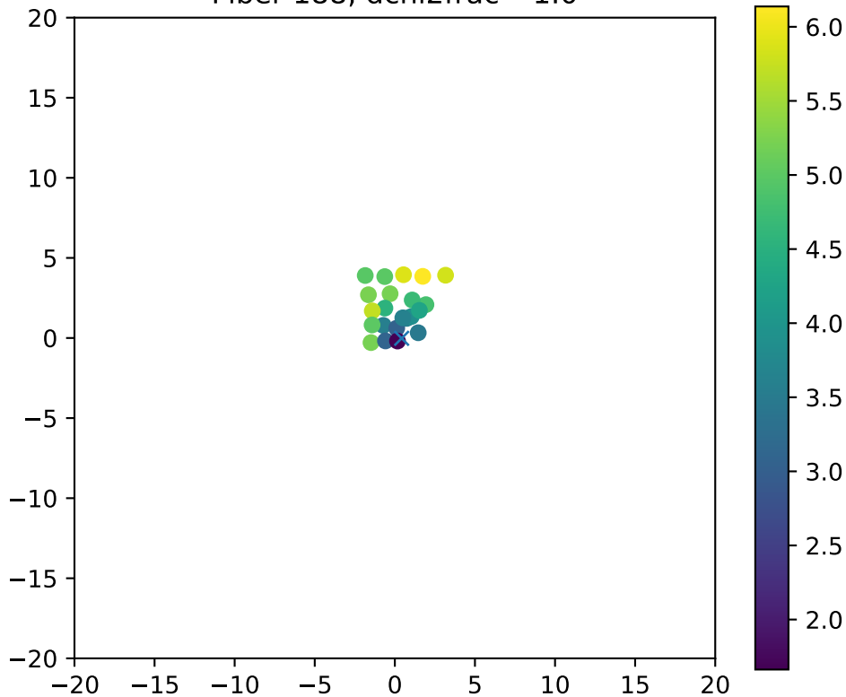
Fiber 188, dchi2frac= 1.0
