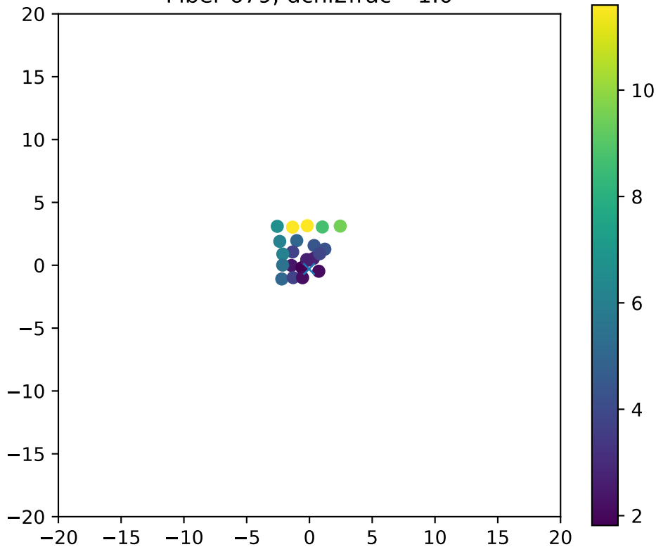
Fiber 679, dchi2frac= 1.0
