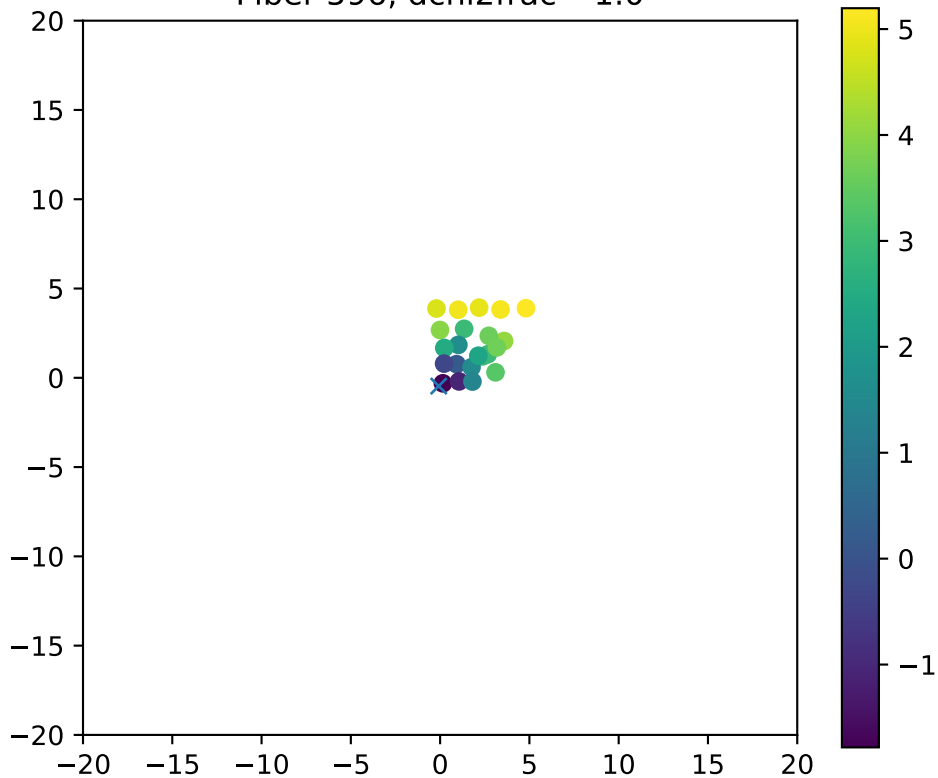
Fiber 596, dchi2frac= 1.0
