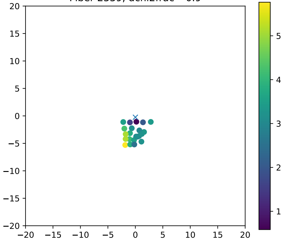
Fiber 2339, dchi2frac= 0.9
