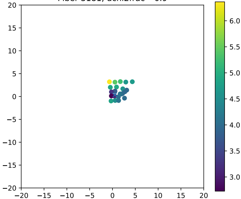
Fiber 3181, dchi2frac= 0.9
