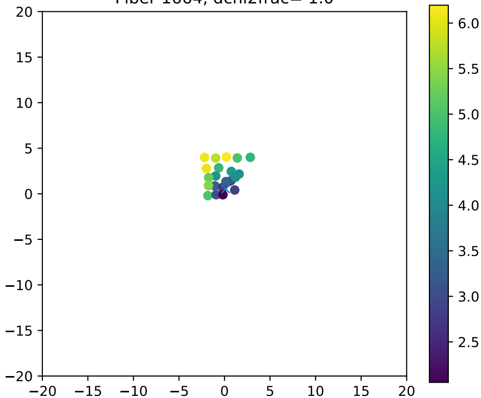
Fiber 1664, dchi2frac= 1.0
