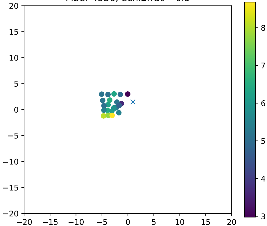
Fiber 4536, dchi2frac= 0.9
