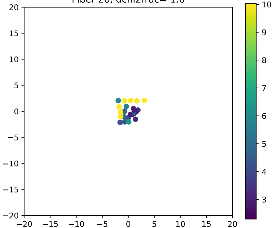
Fiber 26, dchi2frac= 1.0
