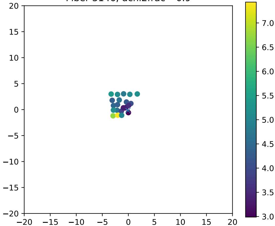
Fiber 3146, dchi2frac= 0.9
