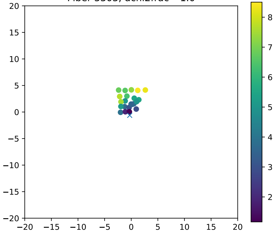
Fiber 3303, dchi2frac= 1.0
