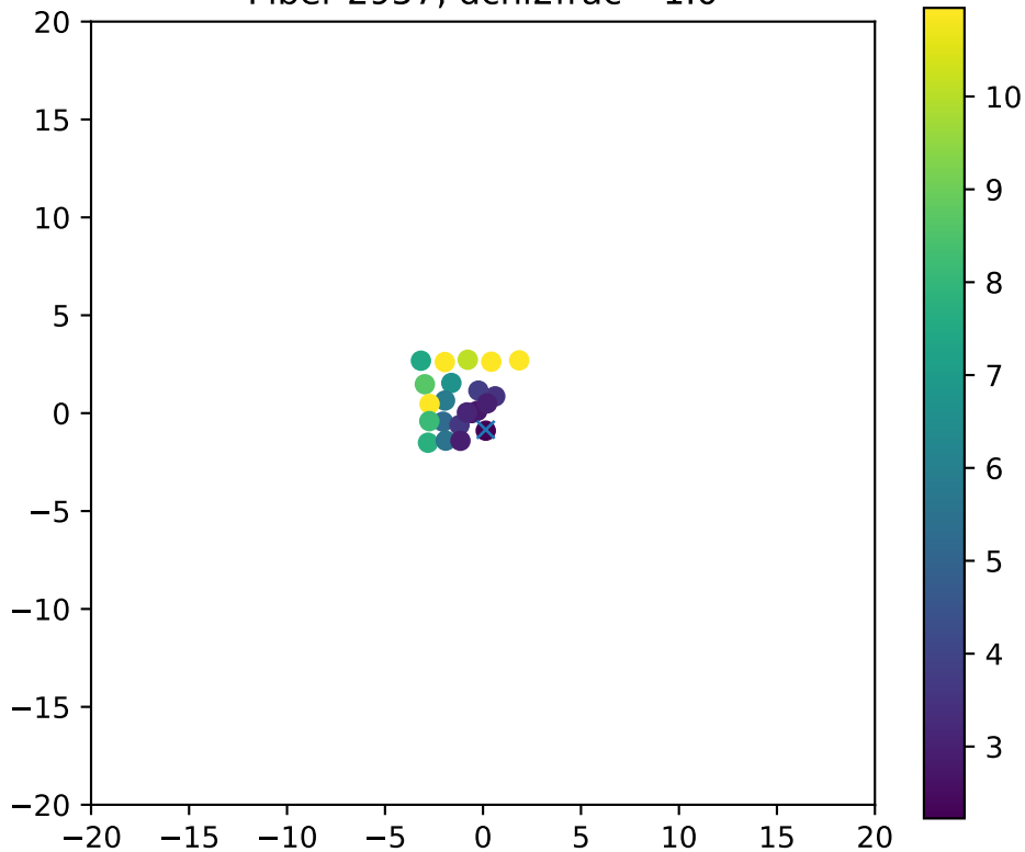
Fiber 2957, dchi2frac= 1.0
