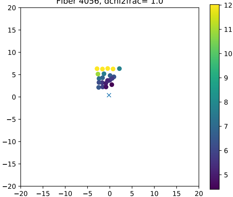
Fiber 4056, dchi2frac= 1.0
