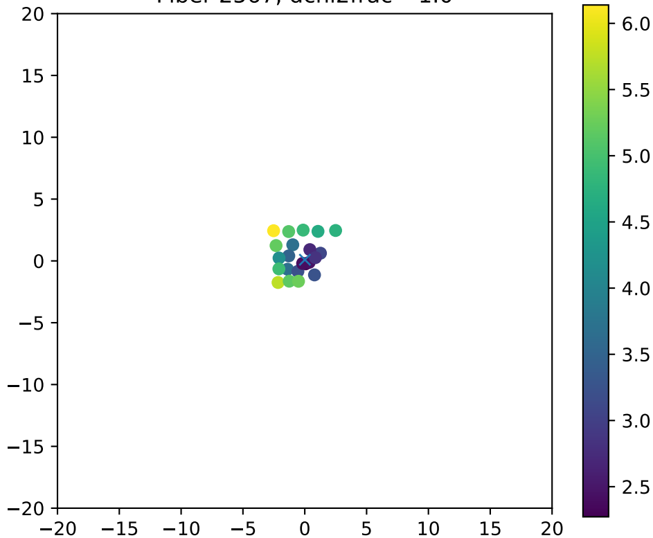
Fiber 2567, dchi2frac= 1.0
