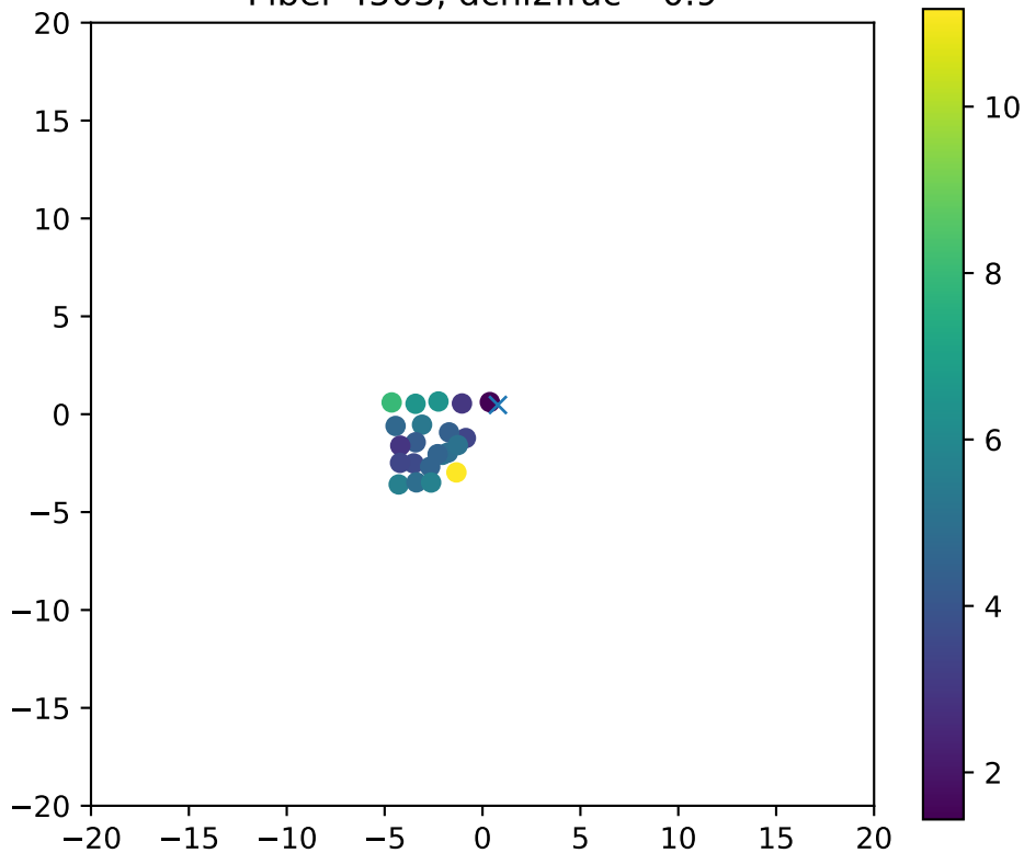
Fiber 4503, dchi2frac= 0.9
