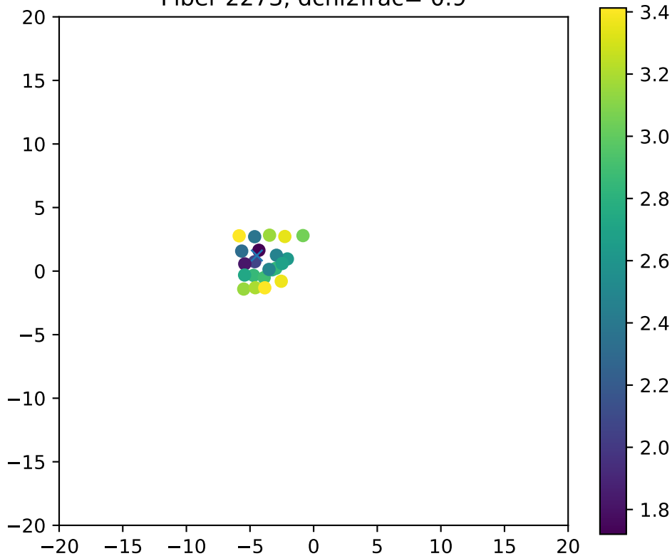
Fiber 2273, dchi2frac= 0.9
