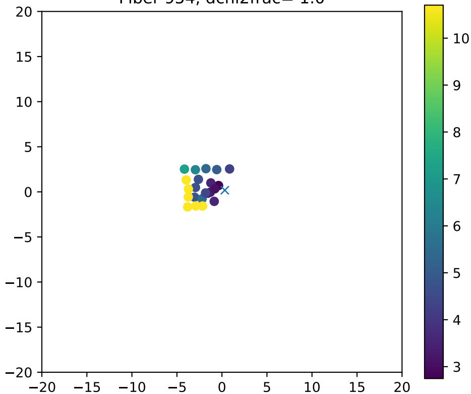
Fiber 954, dchi2frac= 1.0
