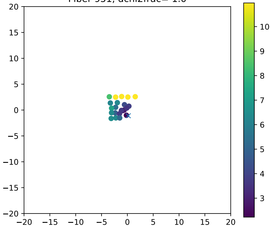
Fiber 951, dchi2frac= 1.0
