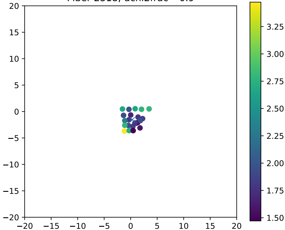
Fiber 2318, dchi2frac= 0.9
