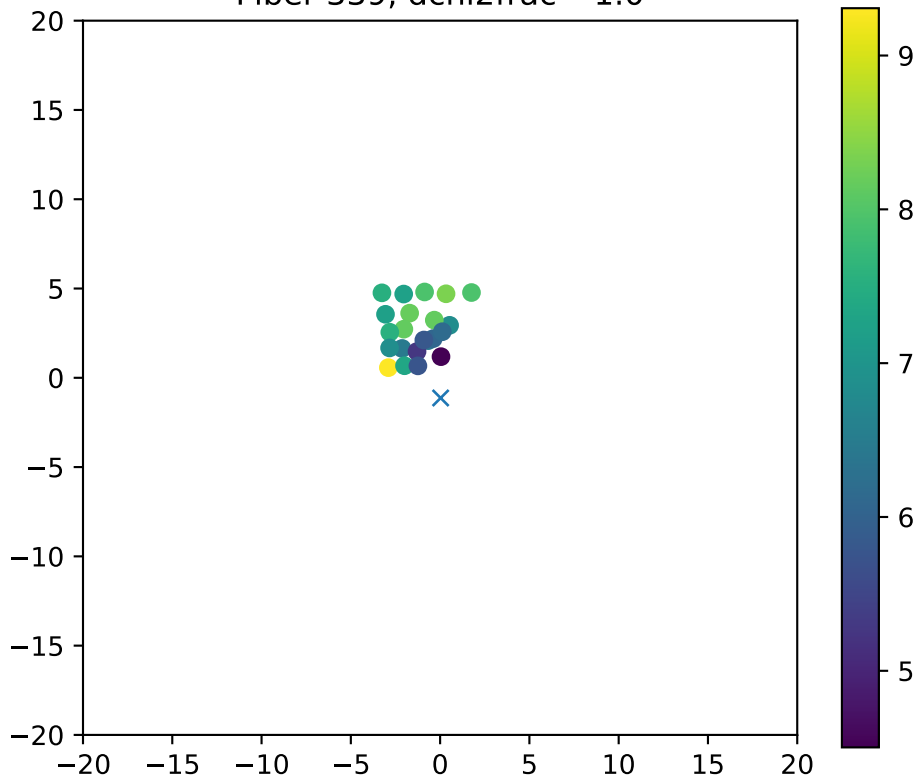
Fiber 339, dchi2frac= 1.0
