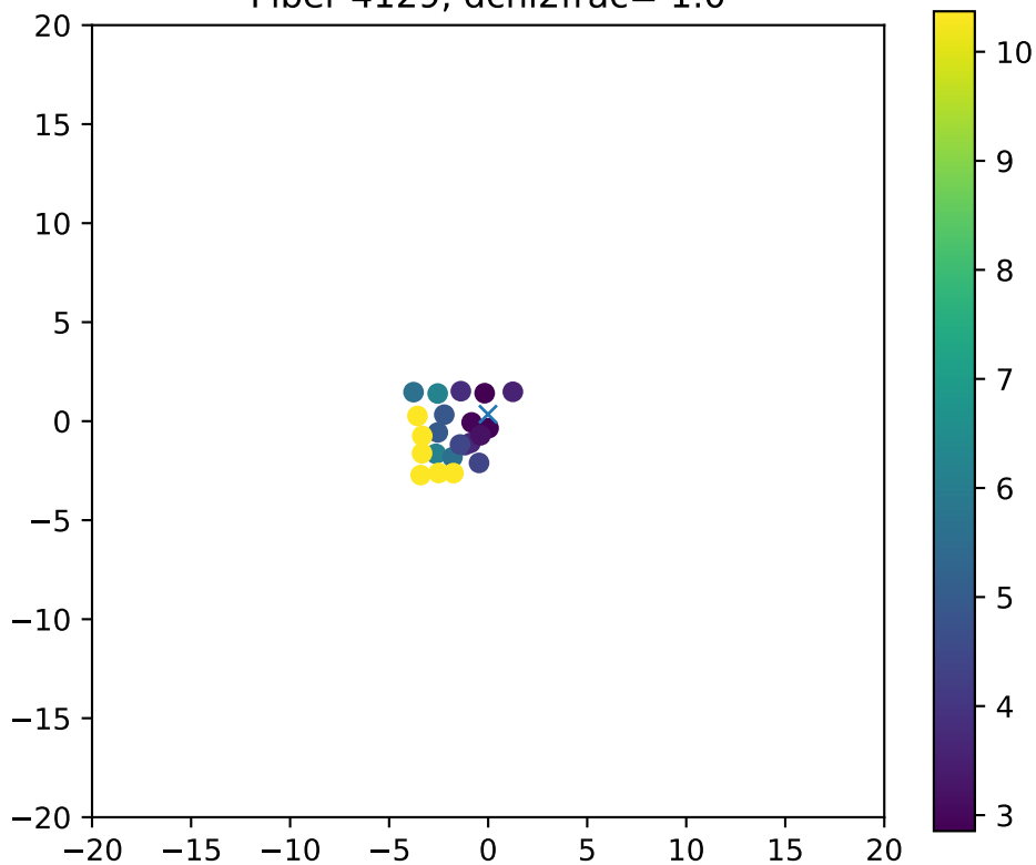
Fiber 4129, dchi2frac= 1.0
