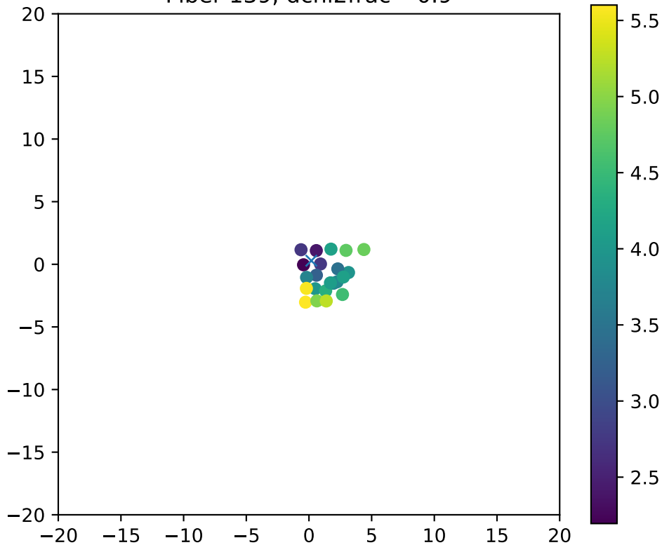
Fiber 139, dchi2frac= 0.9
