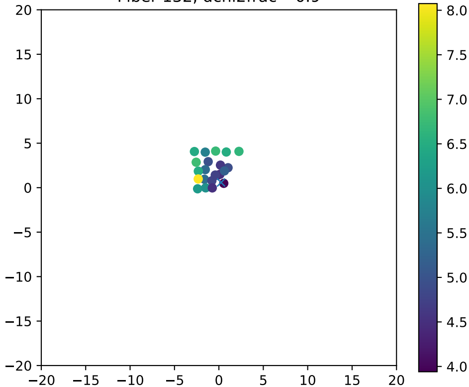
Fiber 132, dchi2frac= 0.9
