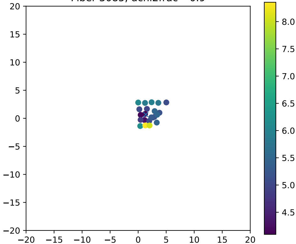
Fiber 3085, dchi2frac= 0.9
