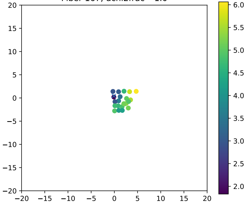
Fiber 167, dchi2frac= 1.0
