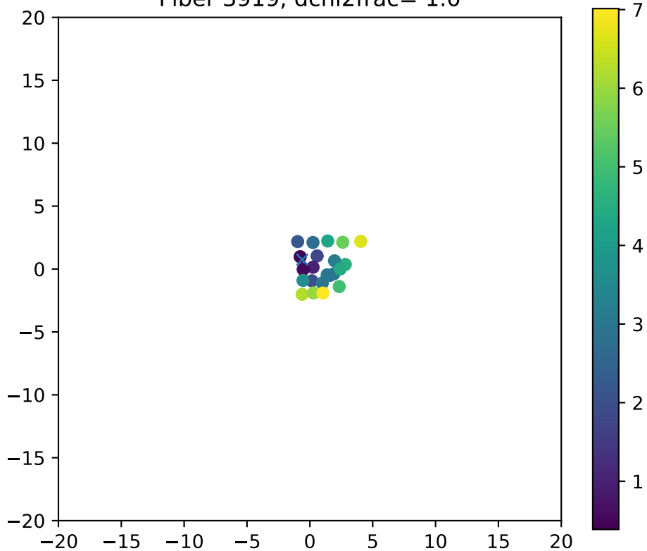
Fiber 3919, dchi2frac= 1.0
