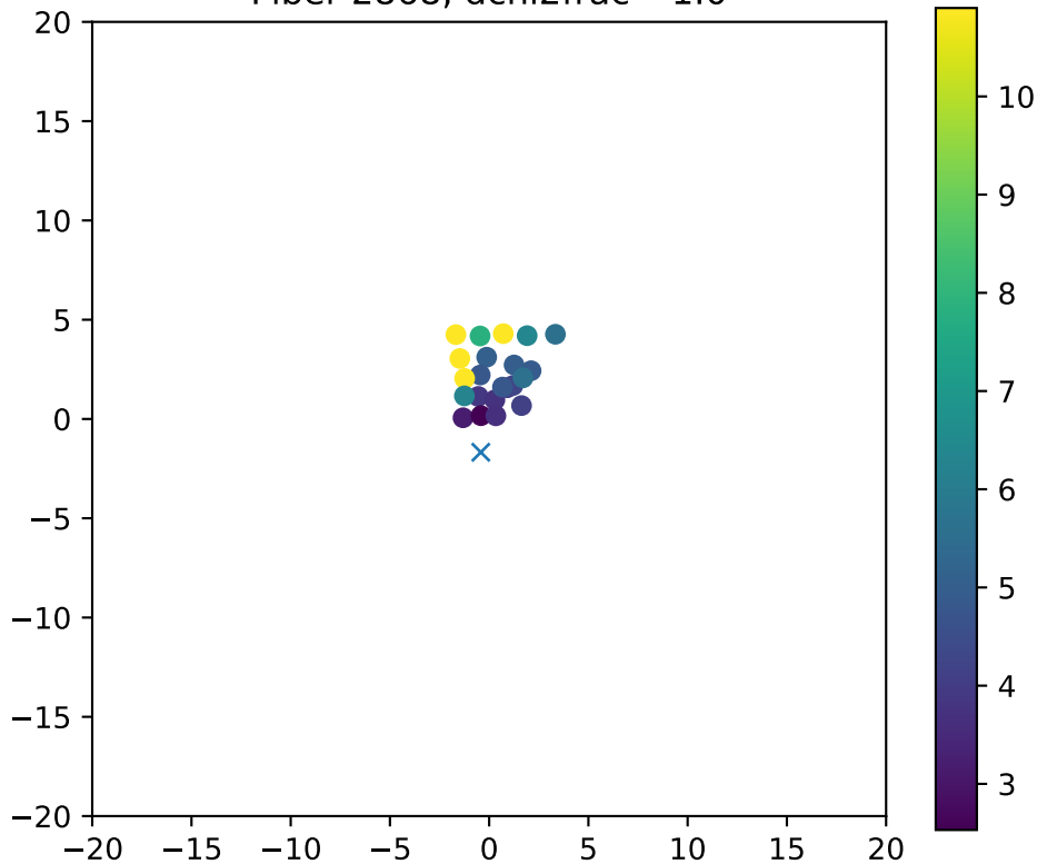
Fiber 2868, dchi2frac= 1.0
