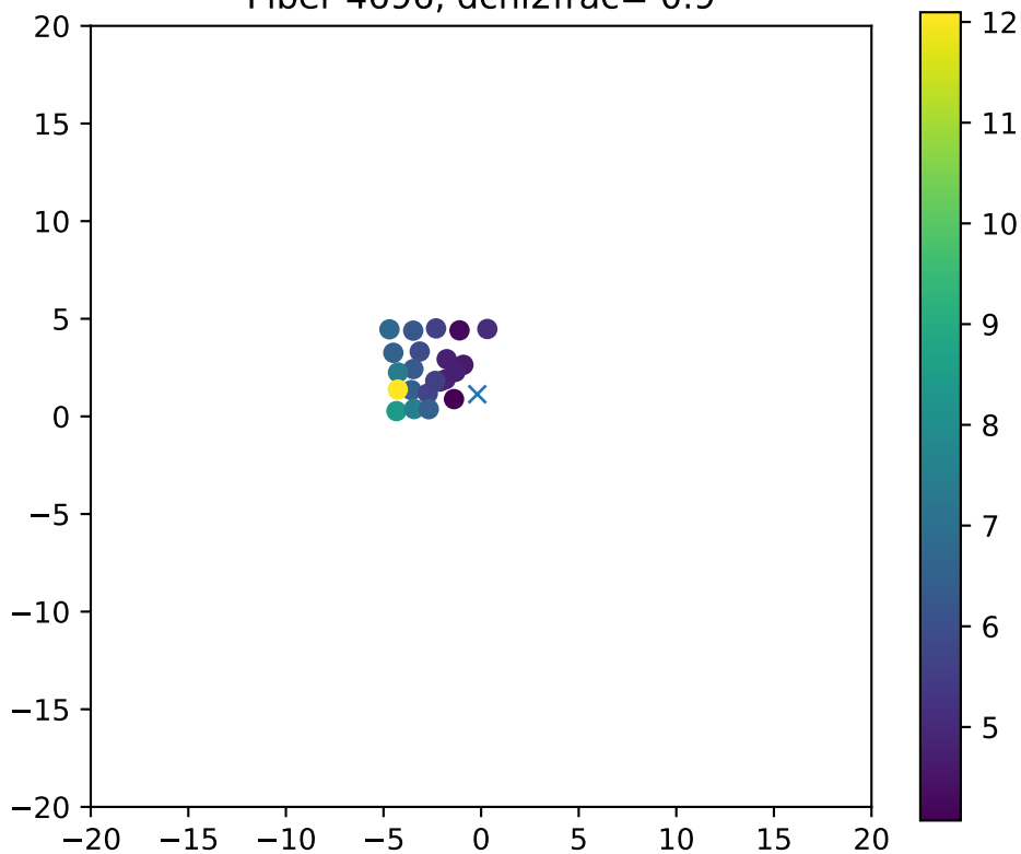
Fiber 4696, dchi2frac= 0.9
