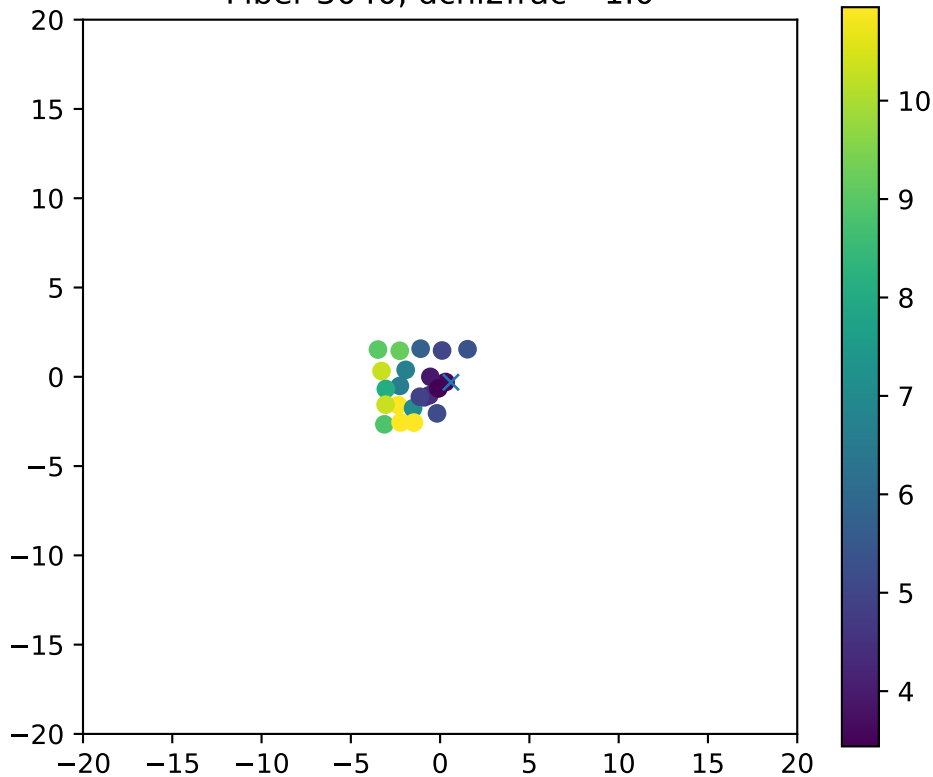
Fiber 3040, dchi2frac= 1.0
