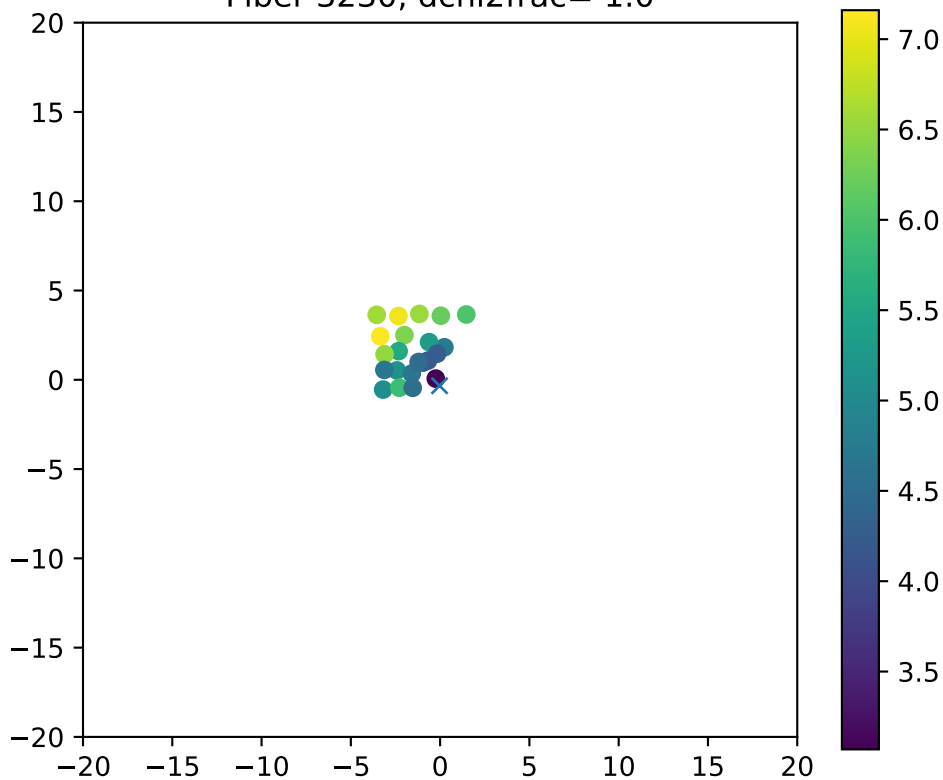
Fiber 3230, dchi2frac= 1.0
