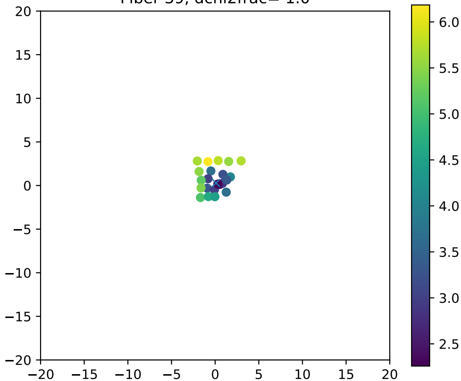
Fiber 39, dchi2frac= 1.0
