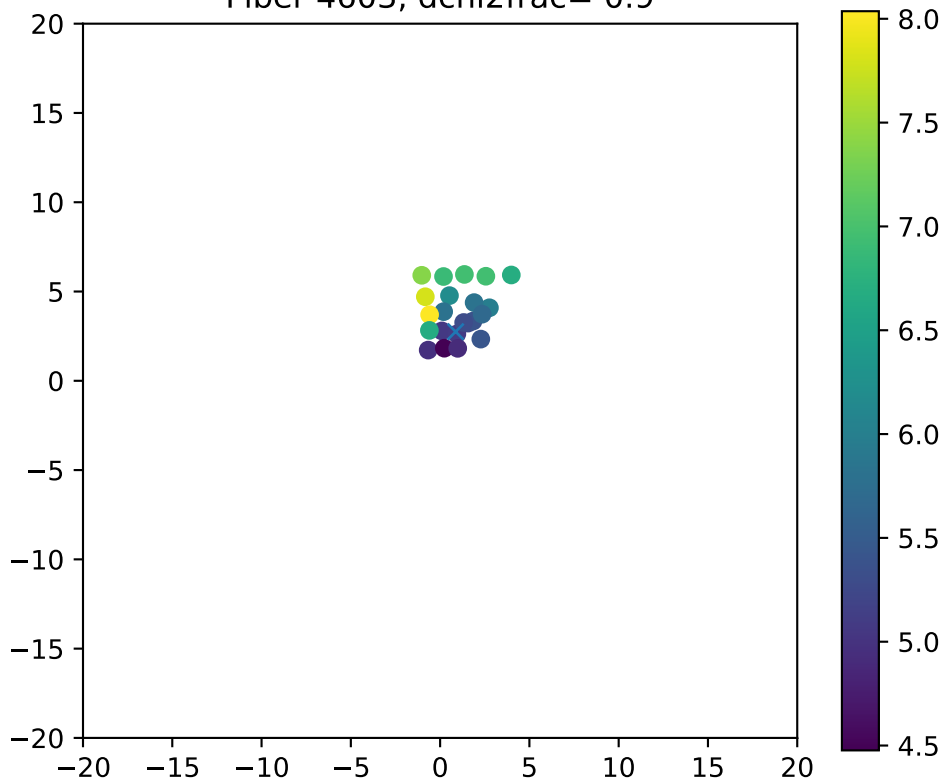
Fiber 4603, dchi2frac= 0.9
