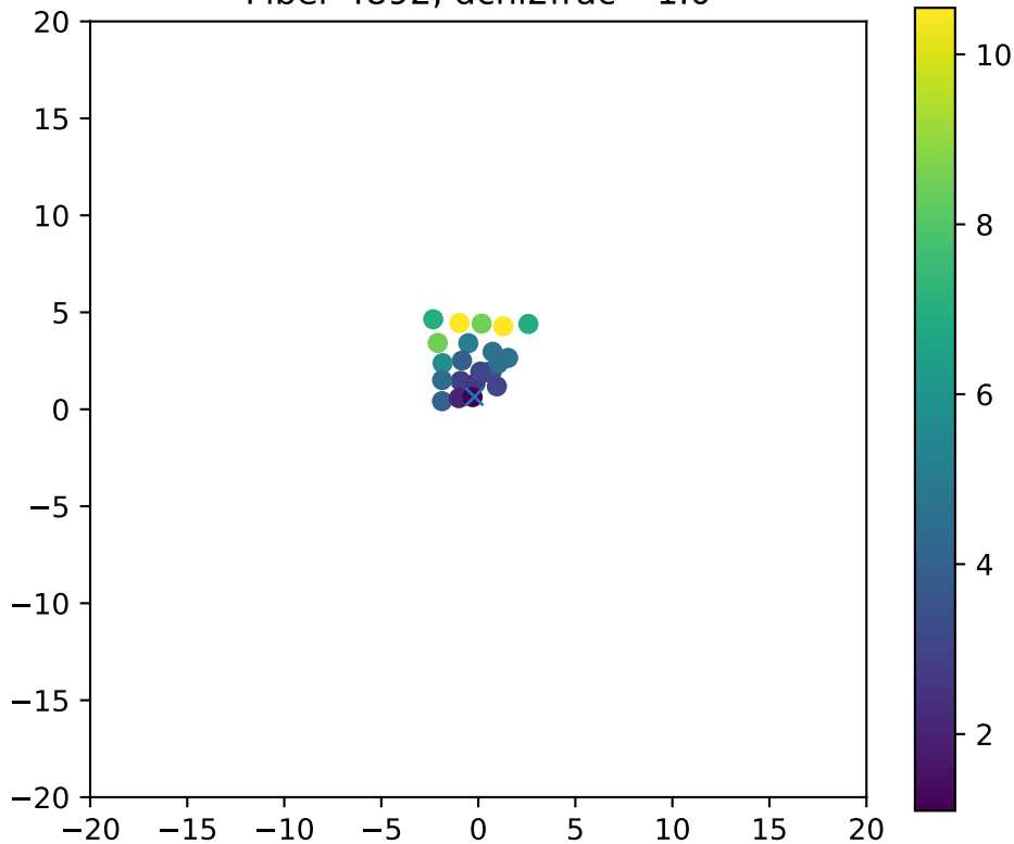
Fiber 4892, dchi2frac= 1.0
