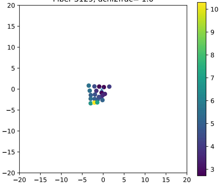
Fiber 3129, dchi2frac= 1.0
