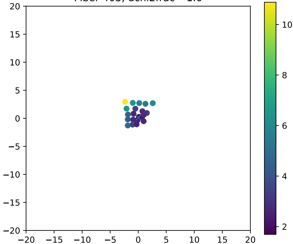
Fiber 403, dchi2frac= 1.0
