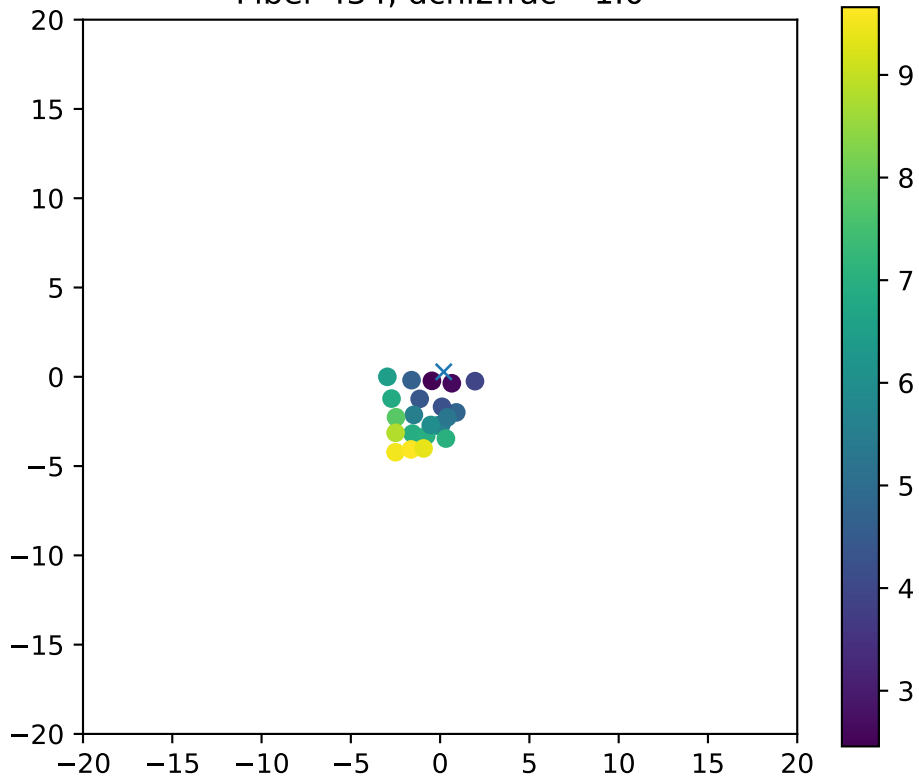
Fiber 434, dchi2frac= 1.0
