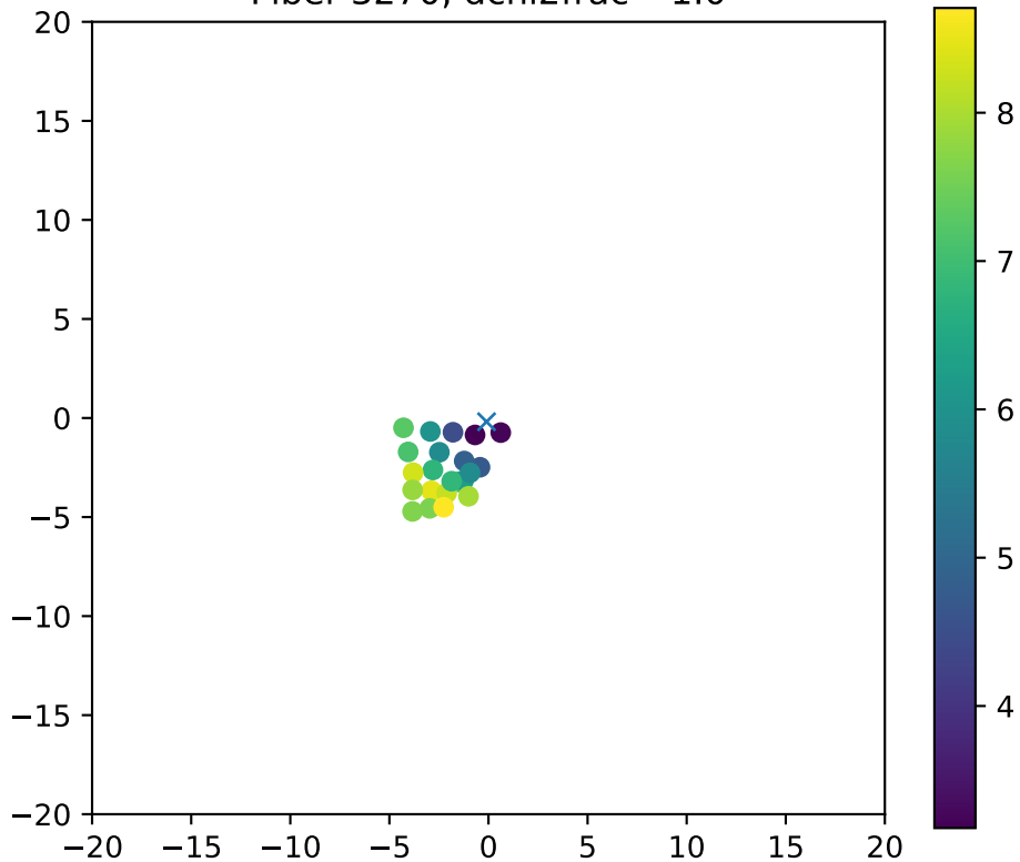
Fiber 3270, dchi2frac= 1.0
