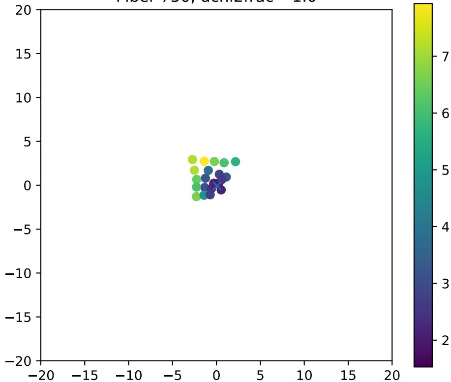
Fiber 750, dchi2frac= 1.0
