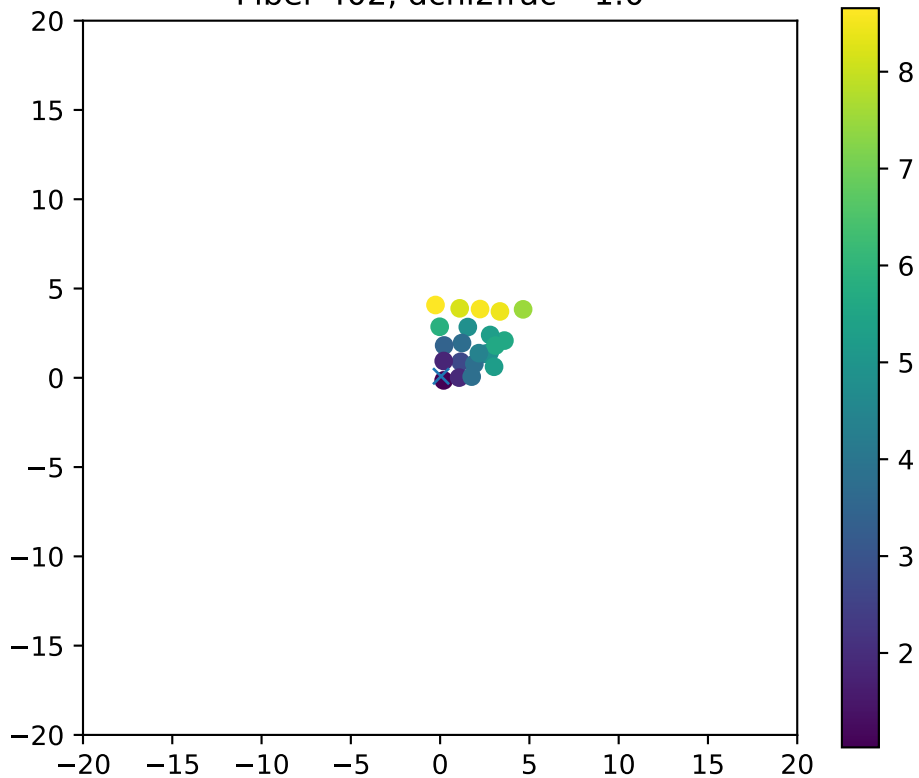
Fiber 402, dchi2frac= 1.0
