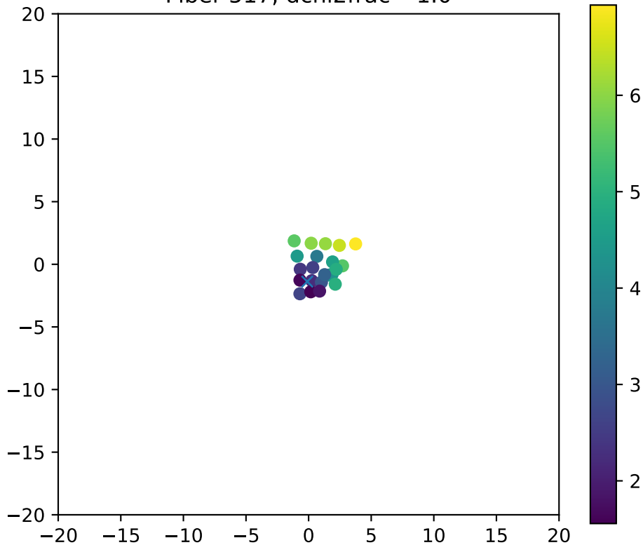
Fiber 517, dchi2frac= 1.0
