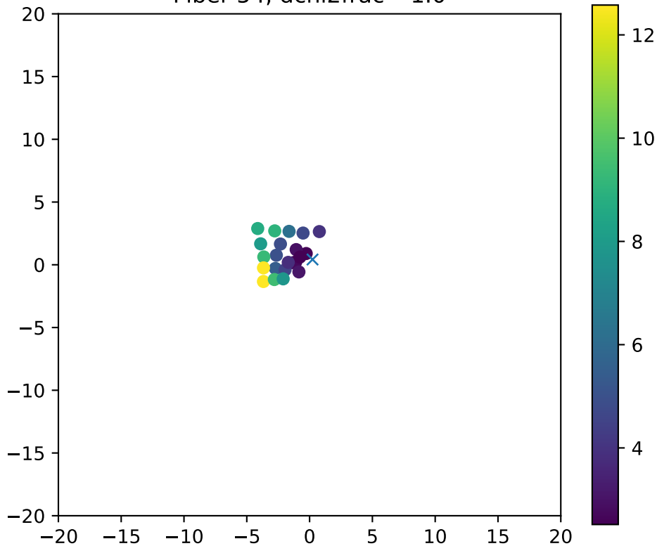
Fiber 54, dchi2frac= 1.0
