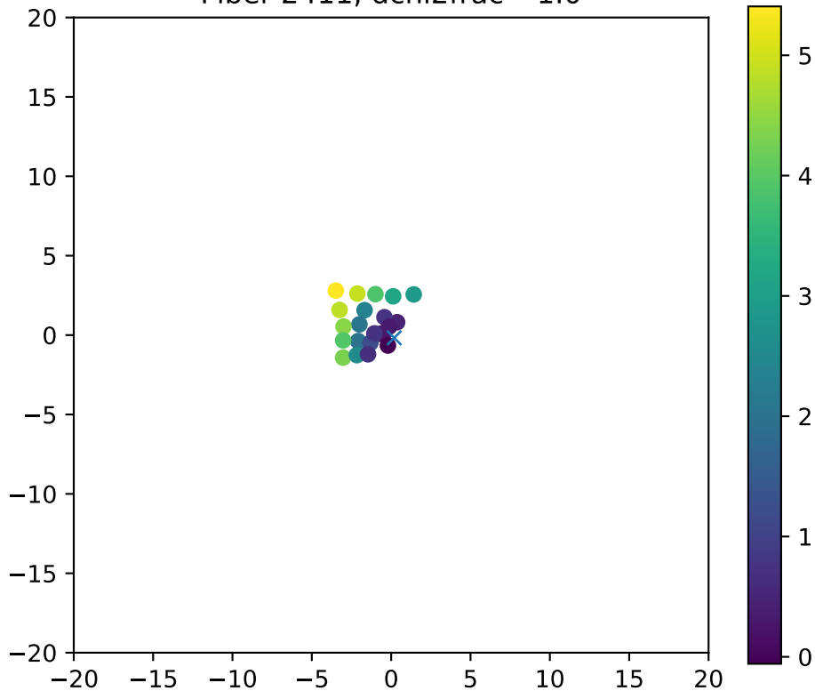
Fiber 2411, dchi2frac= 1.0
