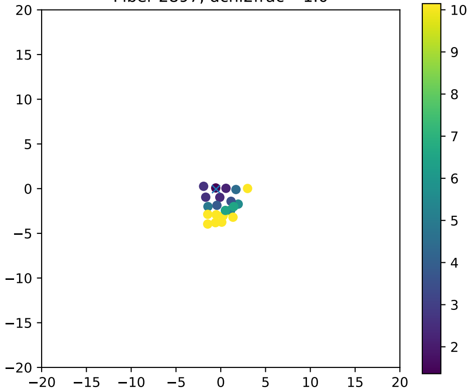
Fiber 2897, dchi2frac= 1.0
