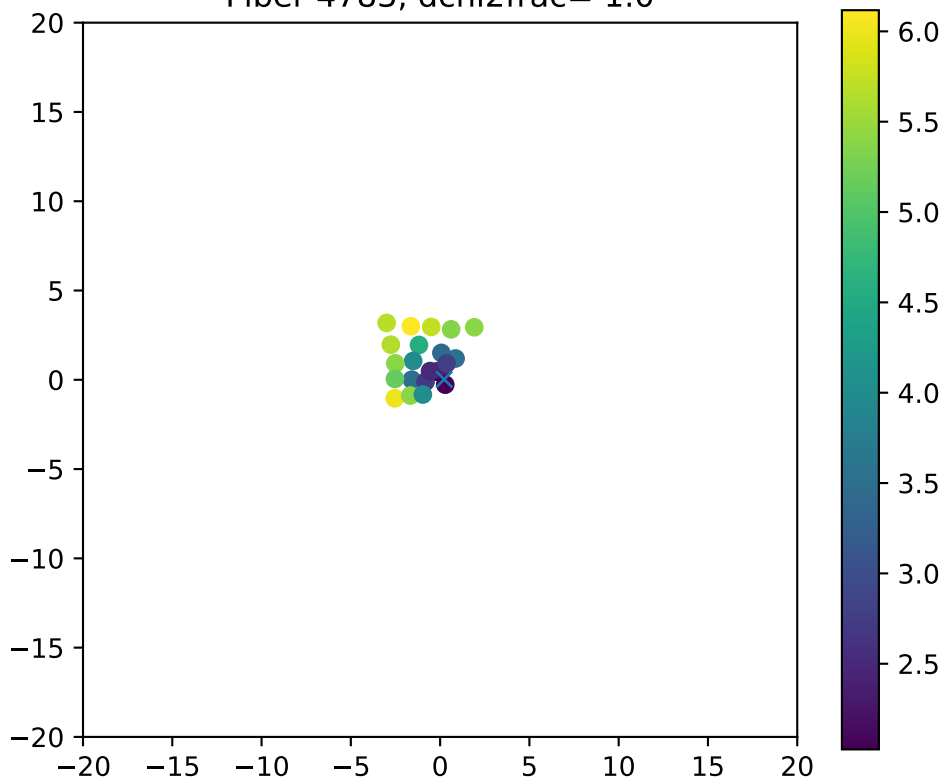
Fiber 4783, dchi2frac= 1.0
