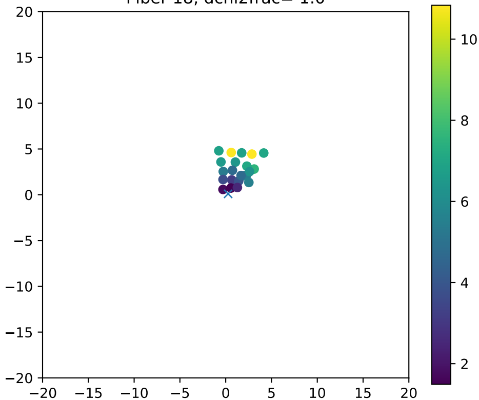
Fiber 18, dchi2frac= 1.0
