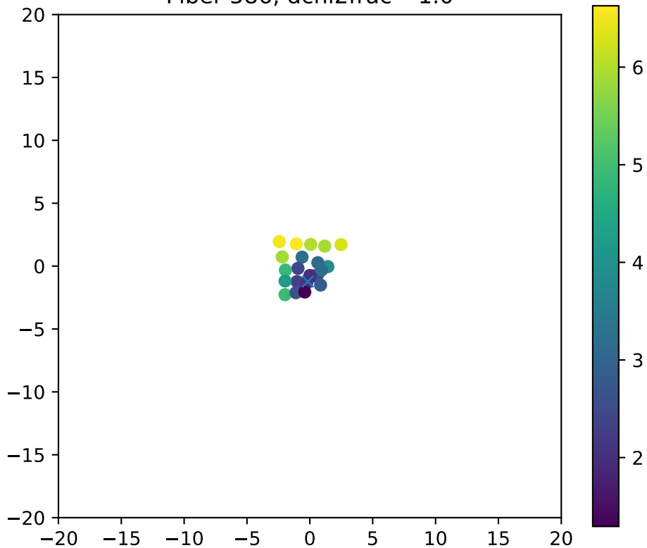
Fiber 586, dchi2frac= 1.0
