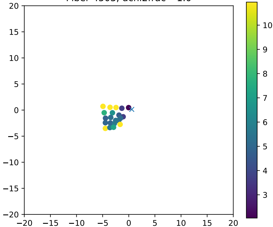
Fiber 4503, dchi2frac= 1.0
