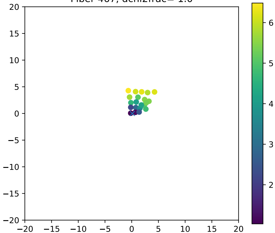
Fiber 467, dchi2frac= 1.0
