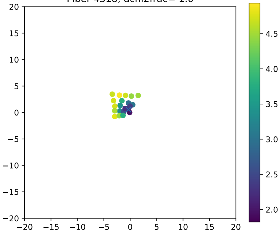
Fiber 4318, dchi2frac= 1.0
