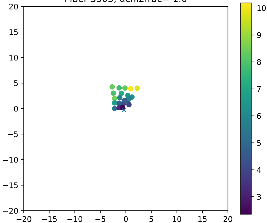
Fiber 3303, dchi2frac= 1.0
