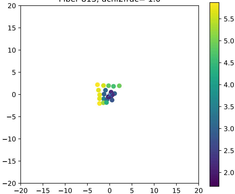
Fiber 813, dchi2frac= 1.0
