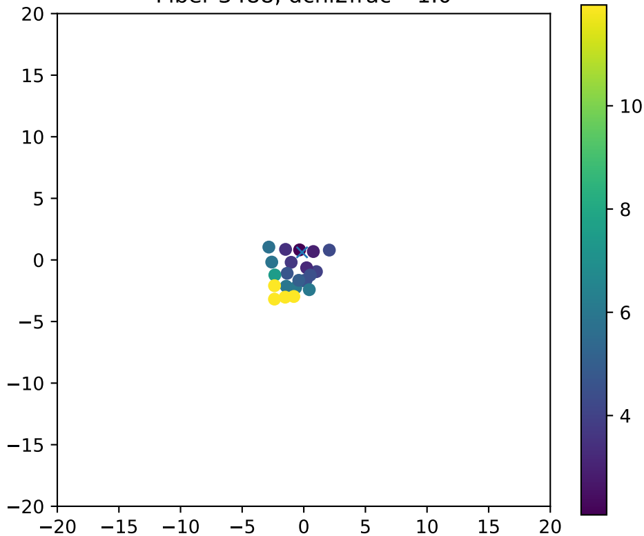
Fiber 3488, dchi2frac= 1.0
