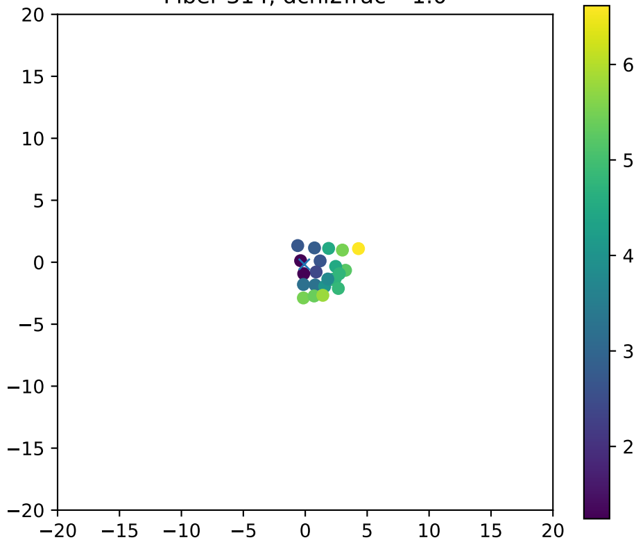
Fiber 314, dchi2frac= 1.0
