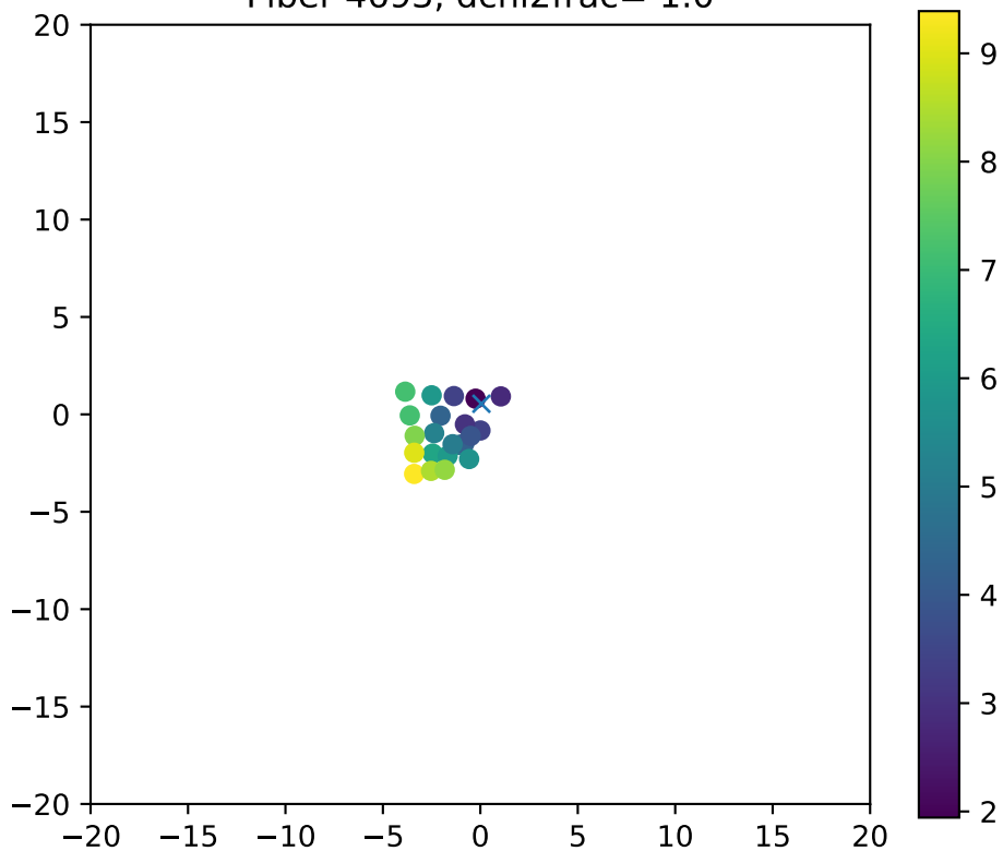
Fiber 4693, dchi2frac= 1.0
