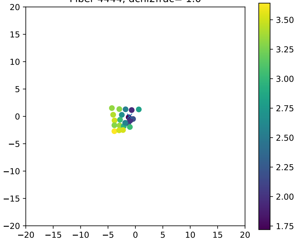
Fiber 4444, dchi2frac= 1.0
