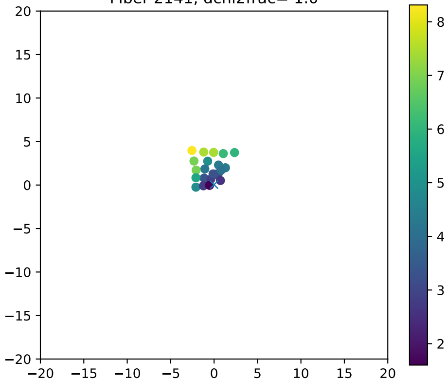
Fiber 2141, dchi2frac= 1.0
