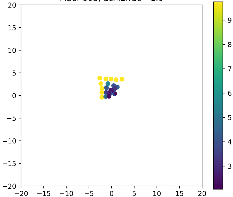
Fiber 993, dchi2frac= 1.0
