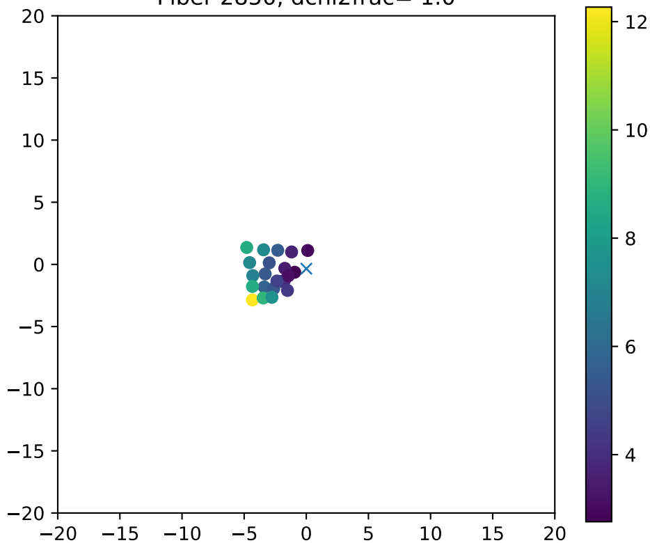
Fiber 2850, dchi2frac= 1.0
