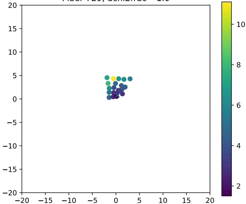
Fiber 729, dchi2frac= 1.0
