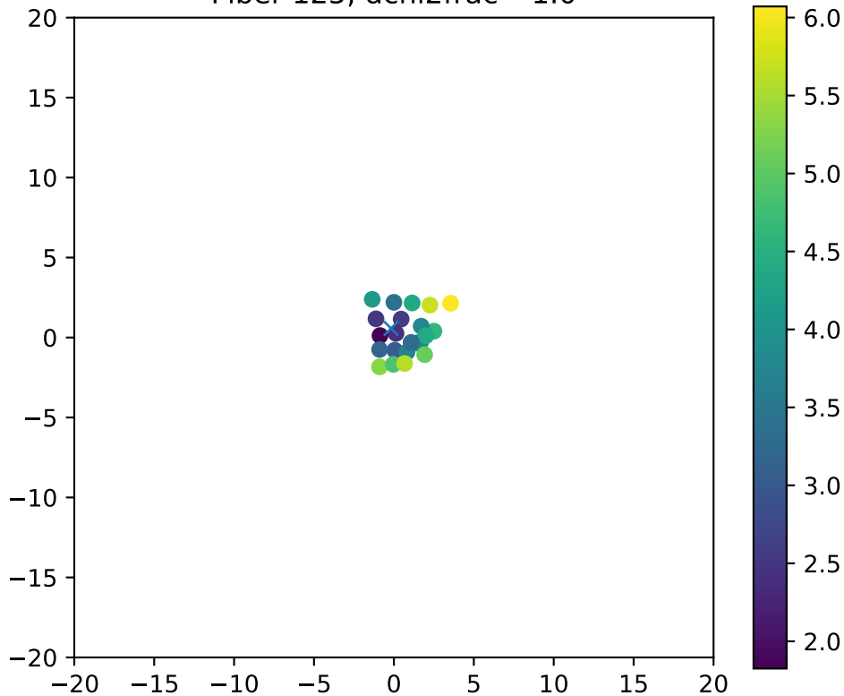
Fiber 125, dchi2frac= 1.0
