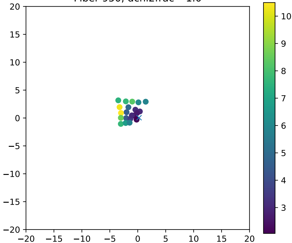
Fiber 950, dchi2frac= 1.0
