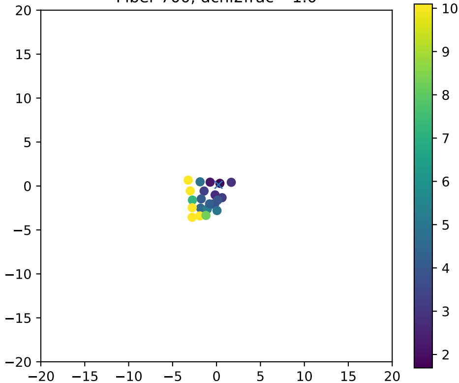
Fiber 700, dchi2frac= 1.0
