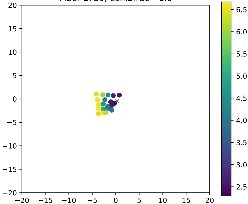
Fiber 2730, dchi2frac= 1.0
