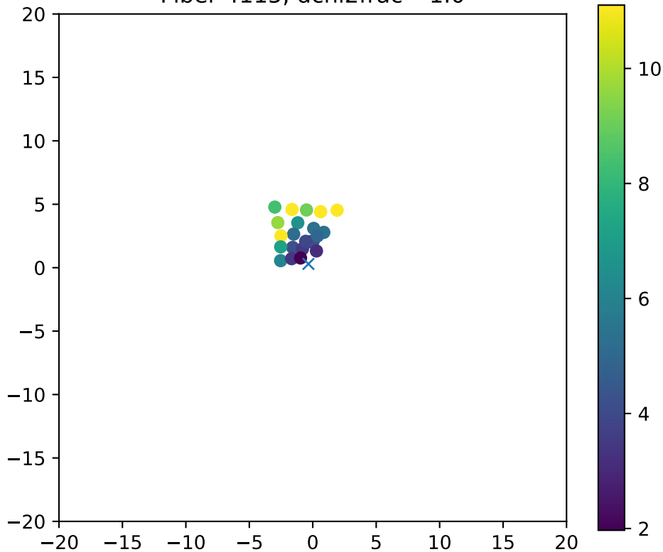
Fiber 4115, dchi2frac= 1.0
