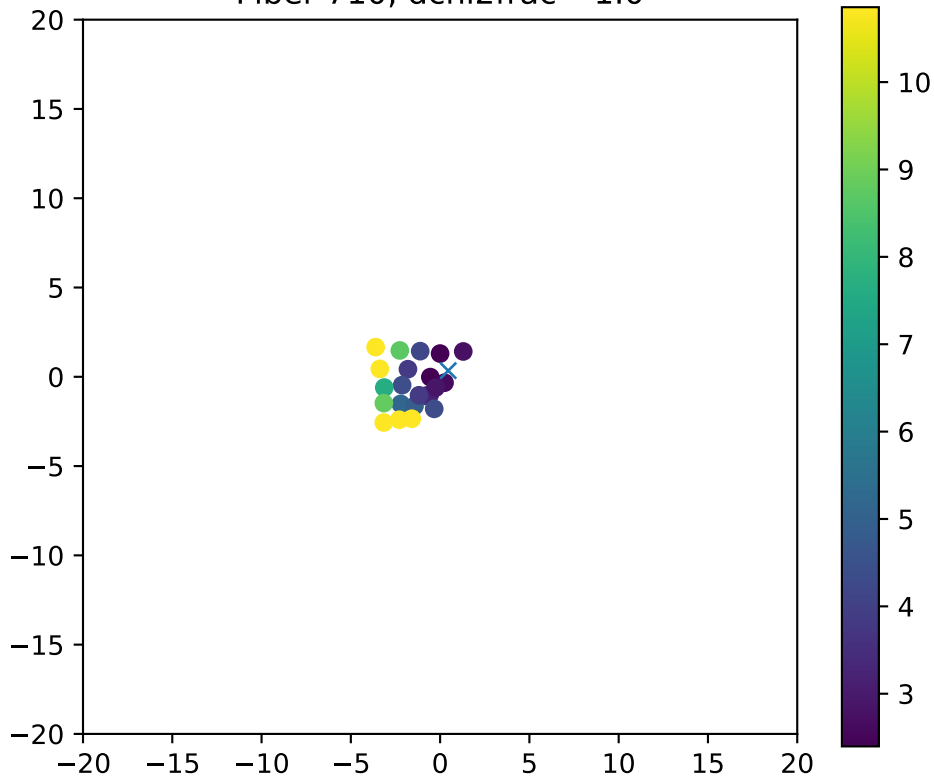
Fiber 710, dchi2frac= 1.0
