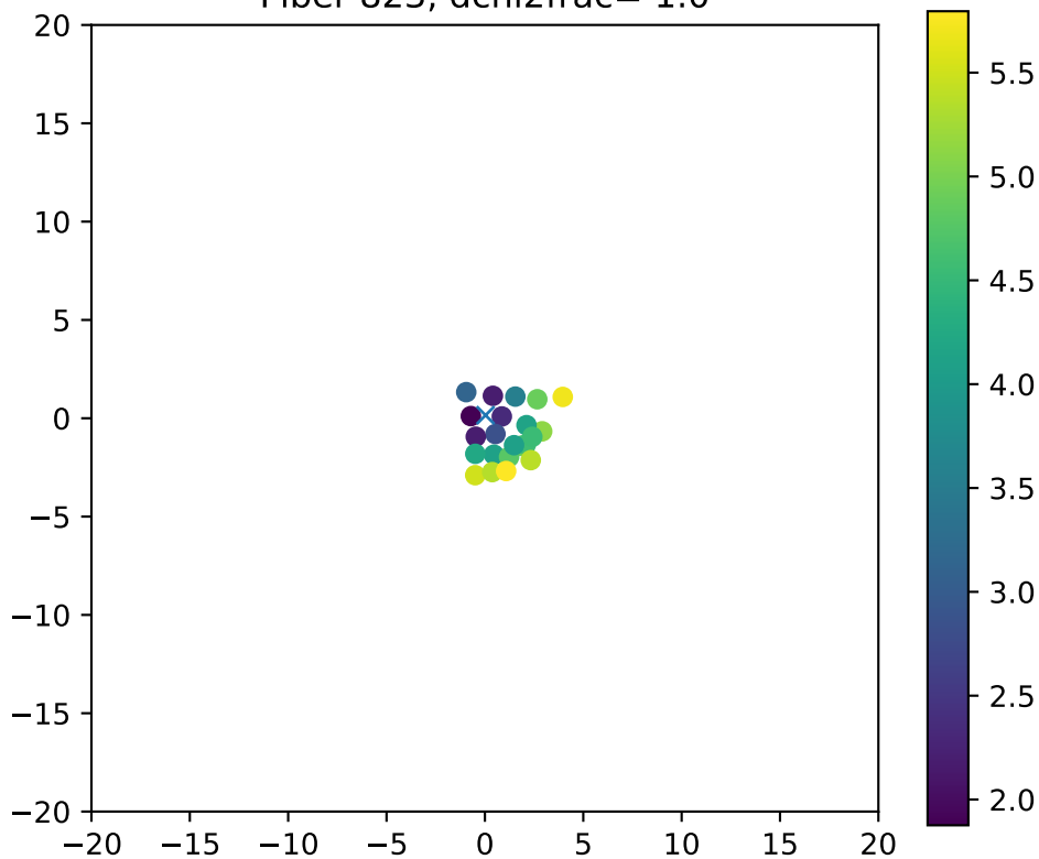
Fiber 823, dchi2frac= 1.0
