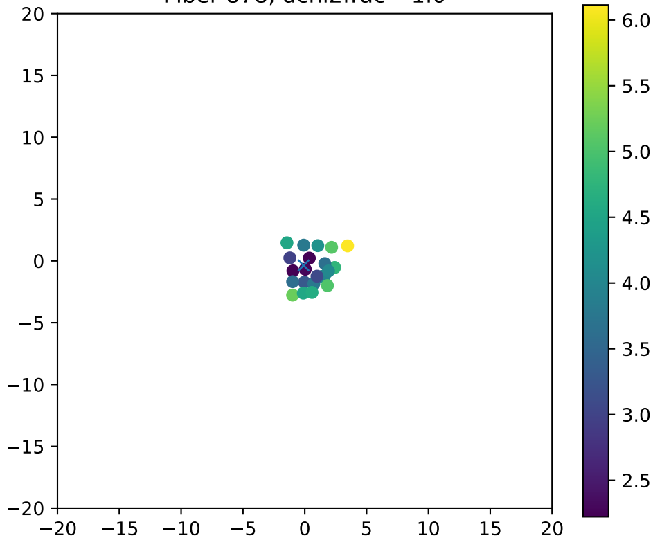
Fiber 878, dchi2frac= 1.0
