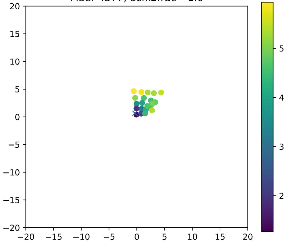
Fiber 4577, dchi2frac= 1.0
