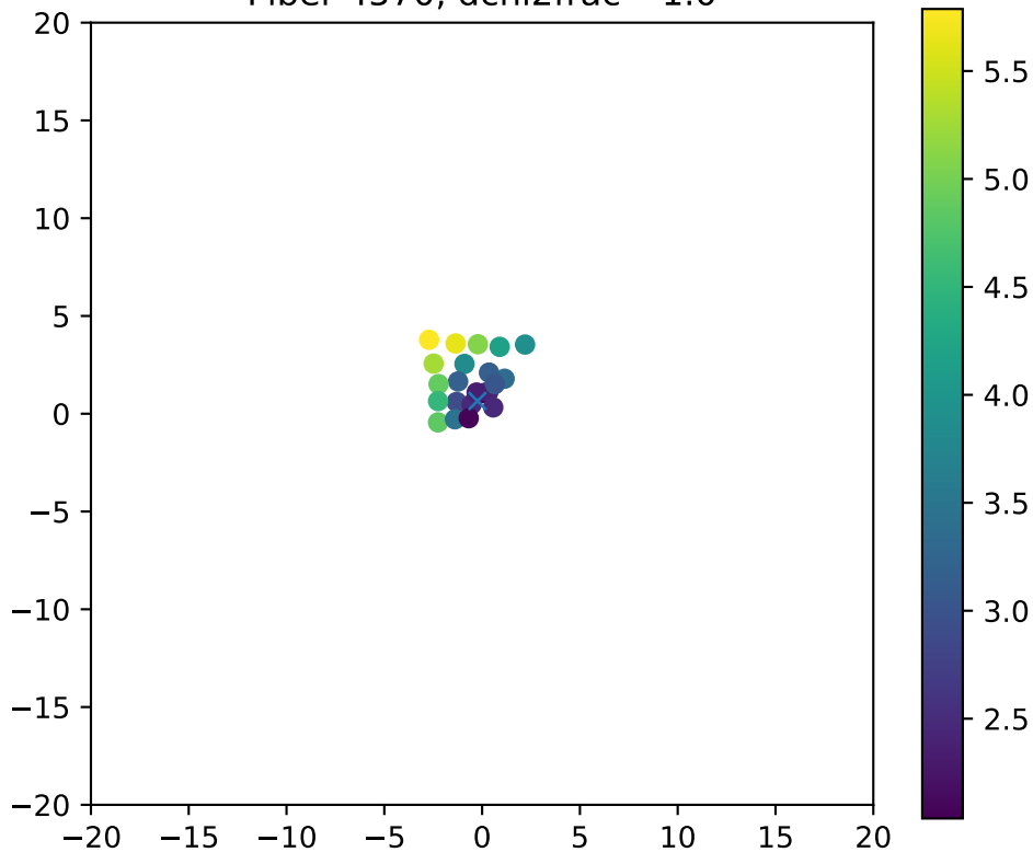
Fiber 4570, dchi2frac= 1.0
