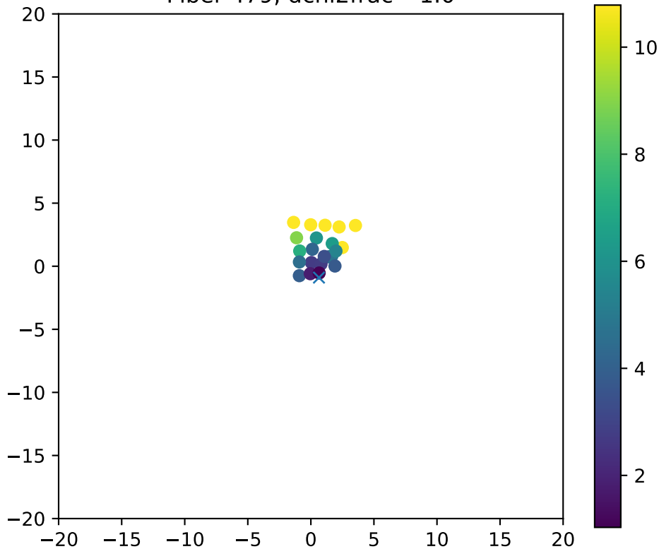
Fiber 479, dchi2frac= 1.0
