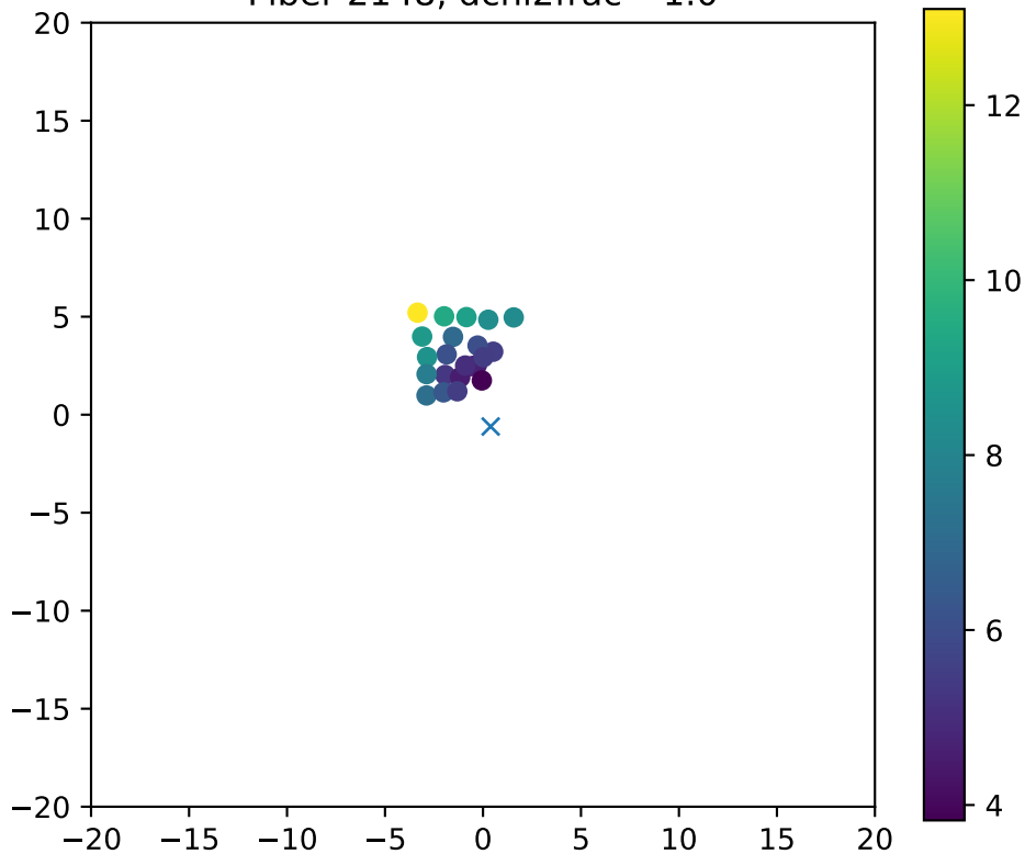
Fiber 2148, dchi2frac= 1.0
