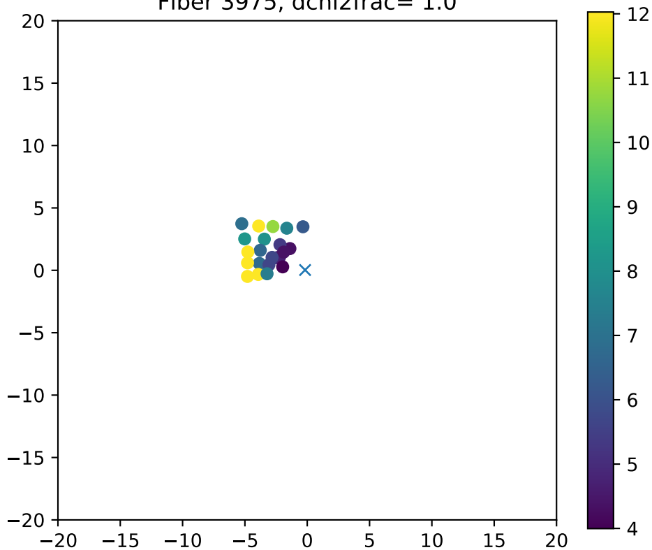
Fiber 3975, dchi2frac= 1.0
