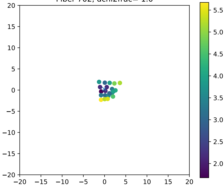
Fiber 702, dchi2frac= 1.0
