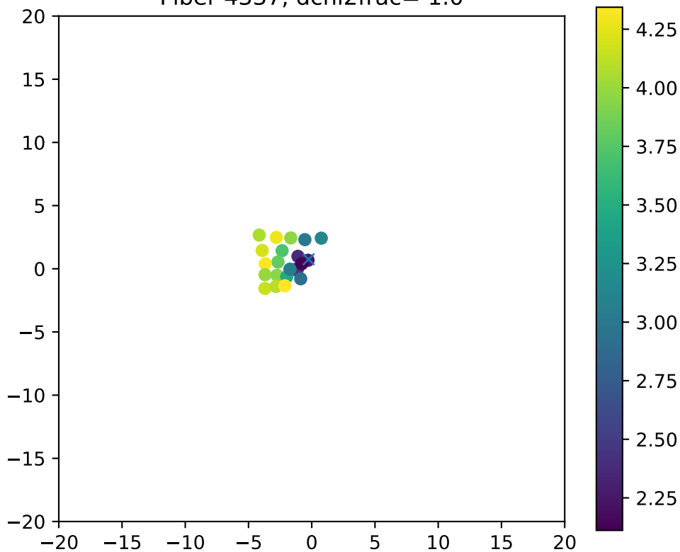
Fiber 4337, dchi2frac= 1.0
