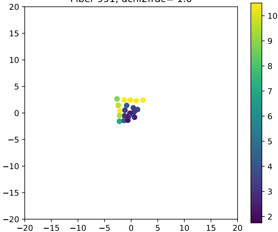
Fiber 991, dchi2frac= 1.0
