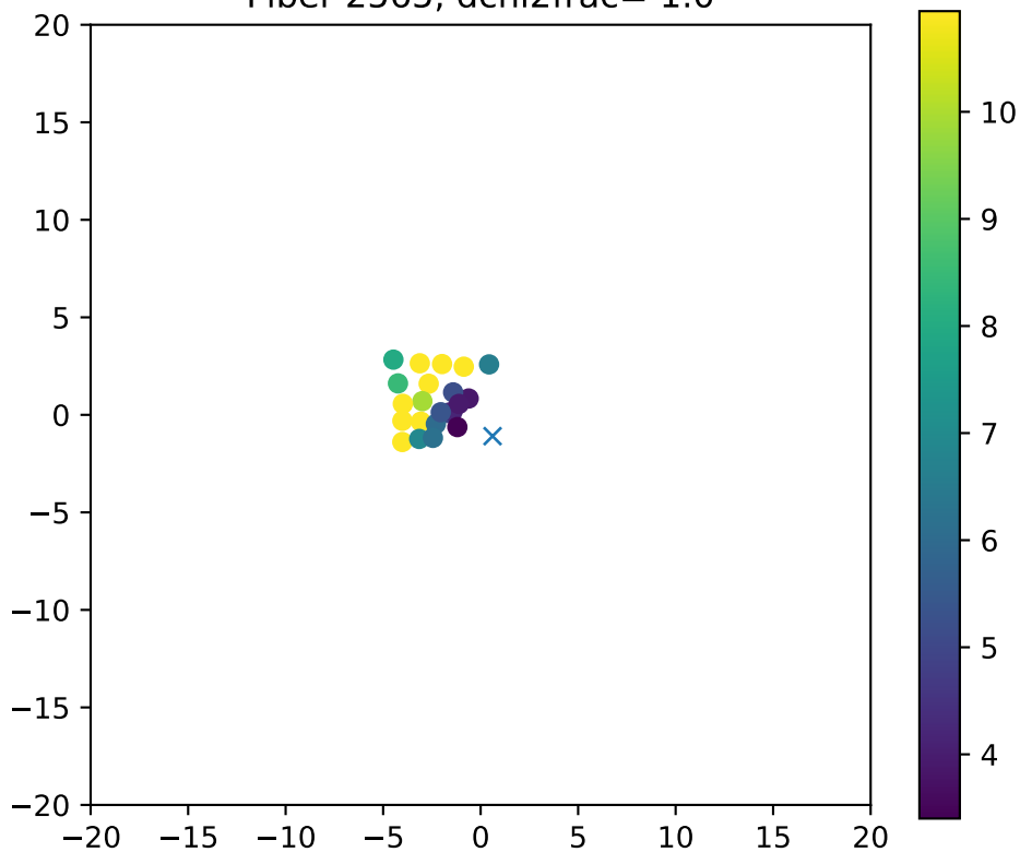
Fiber 2565, dchi2frac= 1.0
