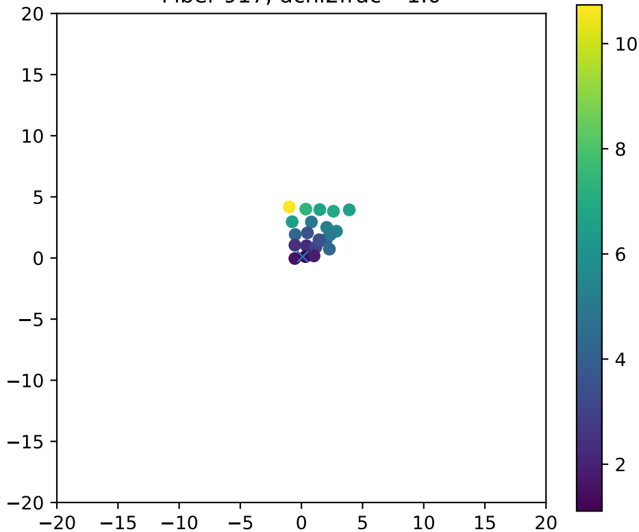
Fiber 917, dchi2frac= 1.0
