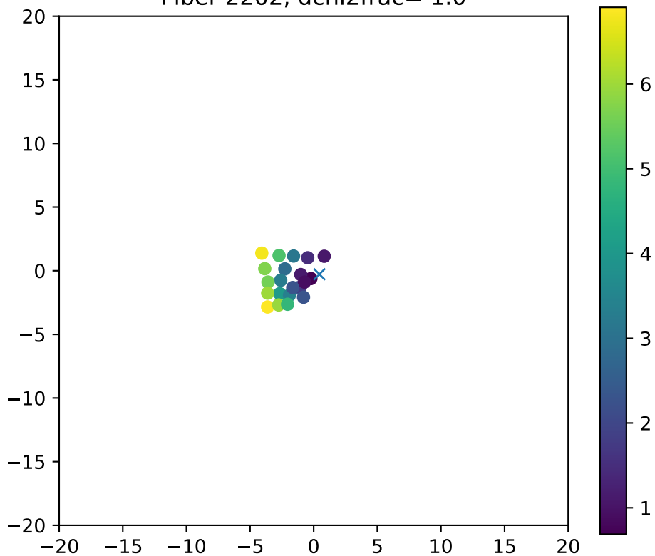
Fiber 2202, dchi2frac= 1.0
