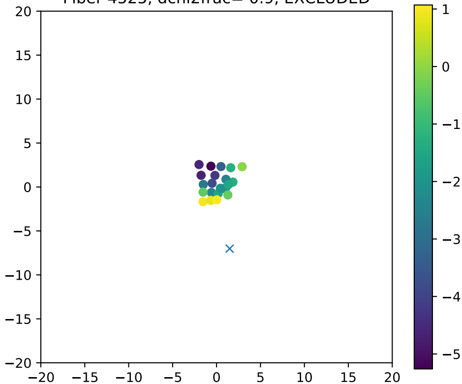
Fiber 4525, dchi2frac= 0.9, EXCLUDED
