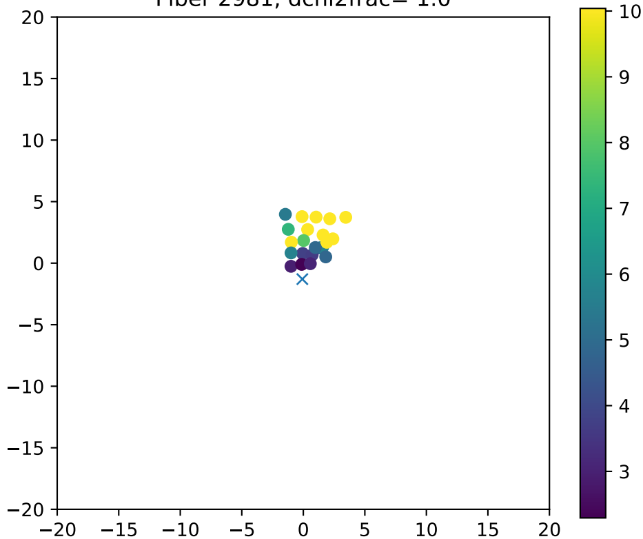
Fiber 2981, dchi2frac= 1.0
