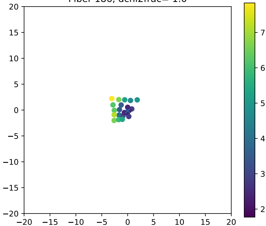
Fiber 186, dchi2frac= 1.0
