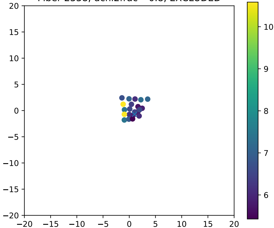
Fiber 2338, dchi2frac= 0.8, EXCLUDED
