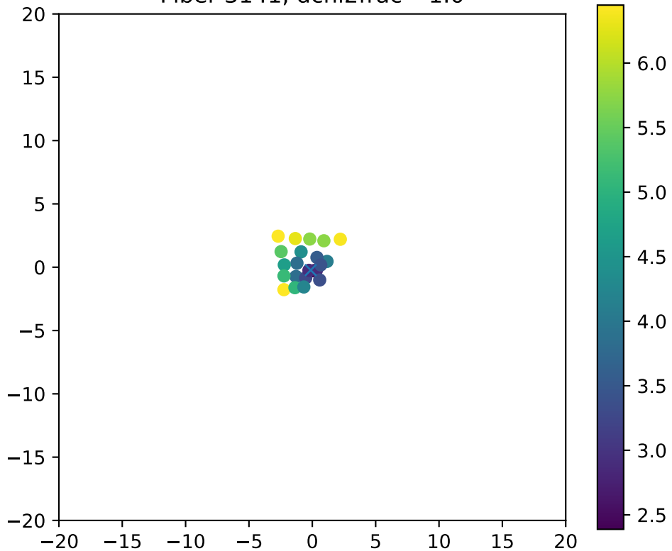
Fiber 3141, dchi2frac= 1.0
