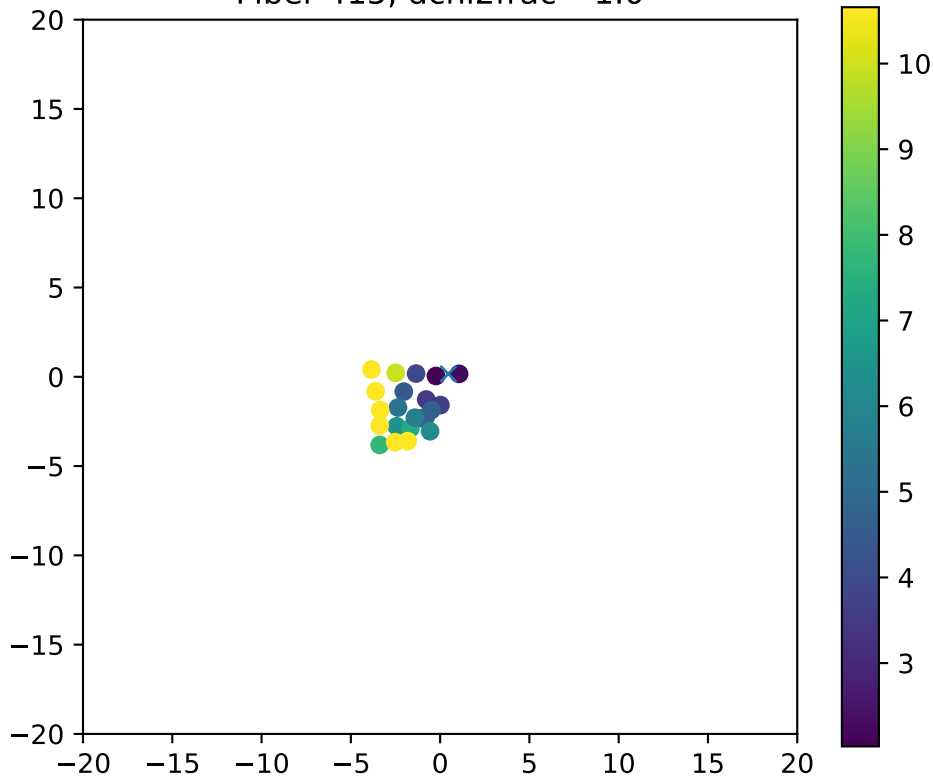
Fiber 415, dchi2frac= 1.0
