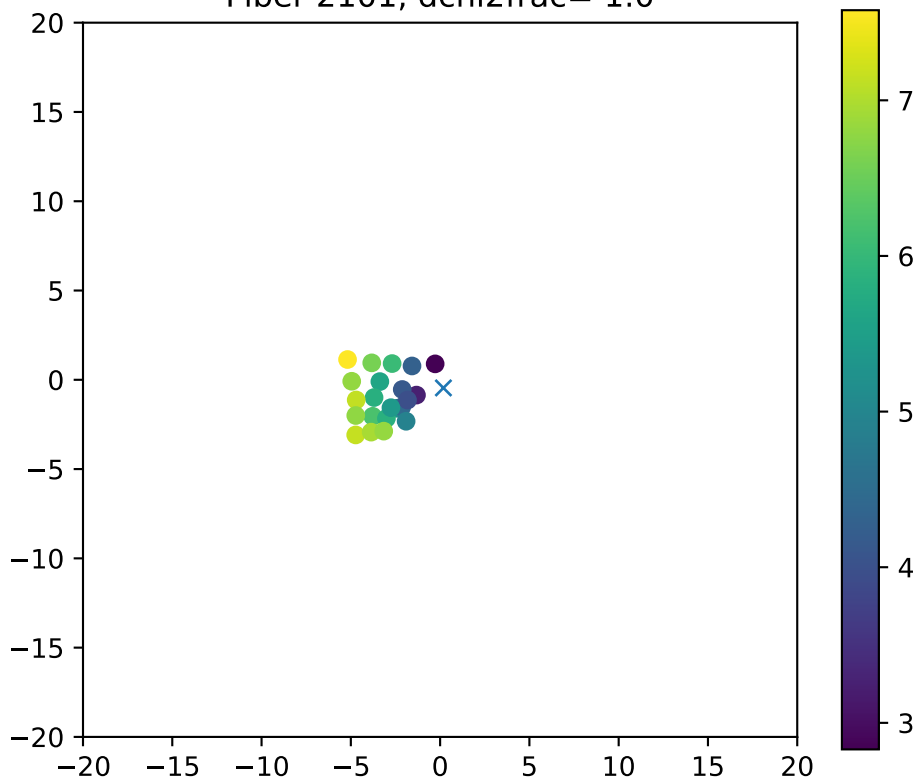
Fiber 2101, dchi2frac= 1.0
