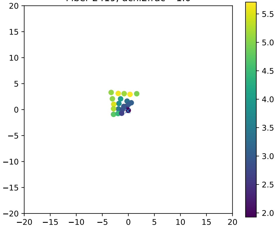
Fiber 2419, dchi2frac= 1.0
