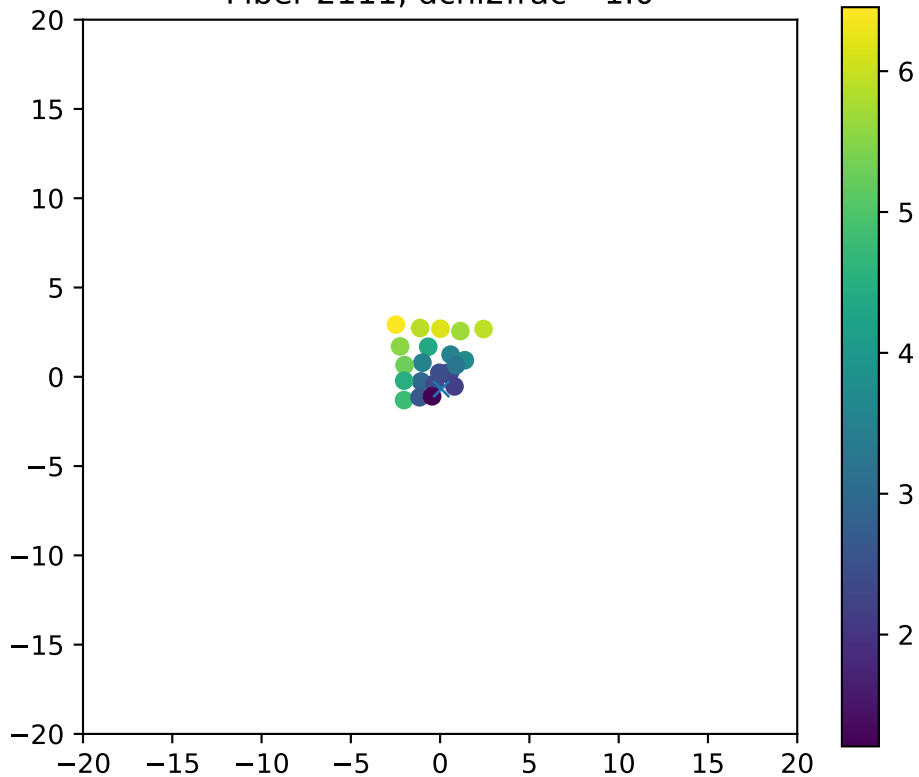
Fiber 2111, dchi2frac= 1.0
