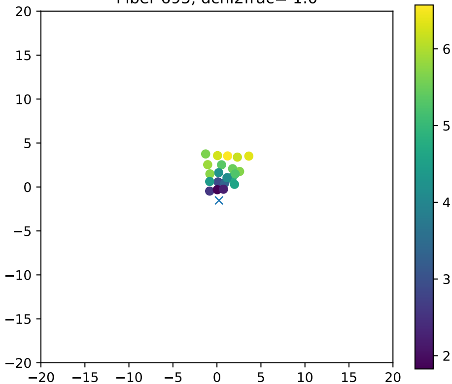
Fiber 695, dchi2frac= 1.0
