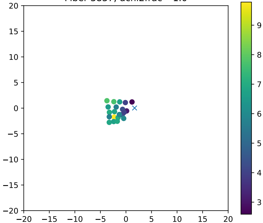
Fiber 3837, dchi2frac= 1.0
