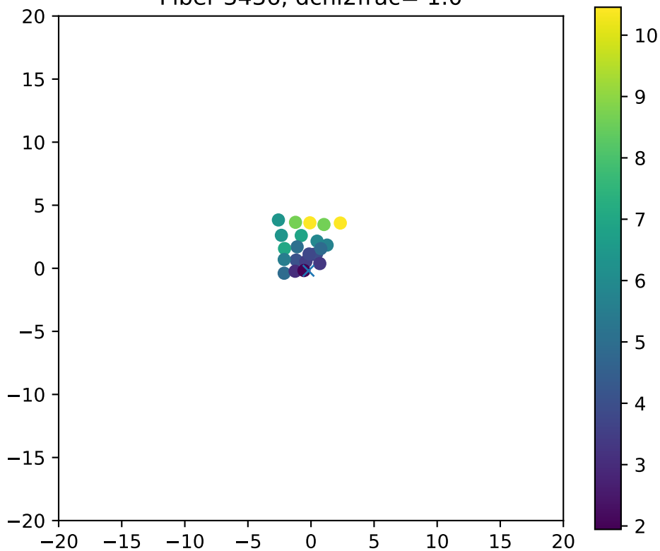
Fiber 3436, dchi2frac= 1.0
