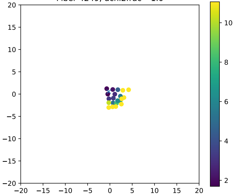
Fiber 4249, dchi2frac= 1.0
