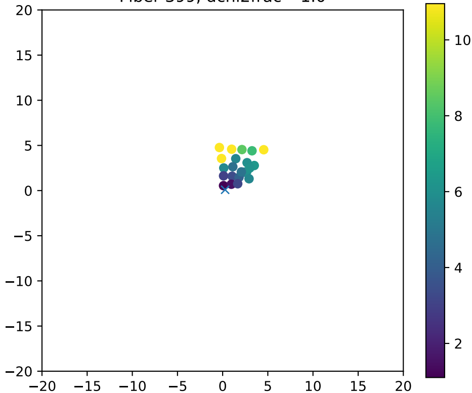
Fiber 399, dchi2frac= 1.0
