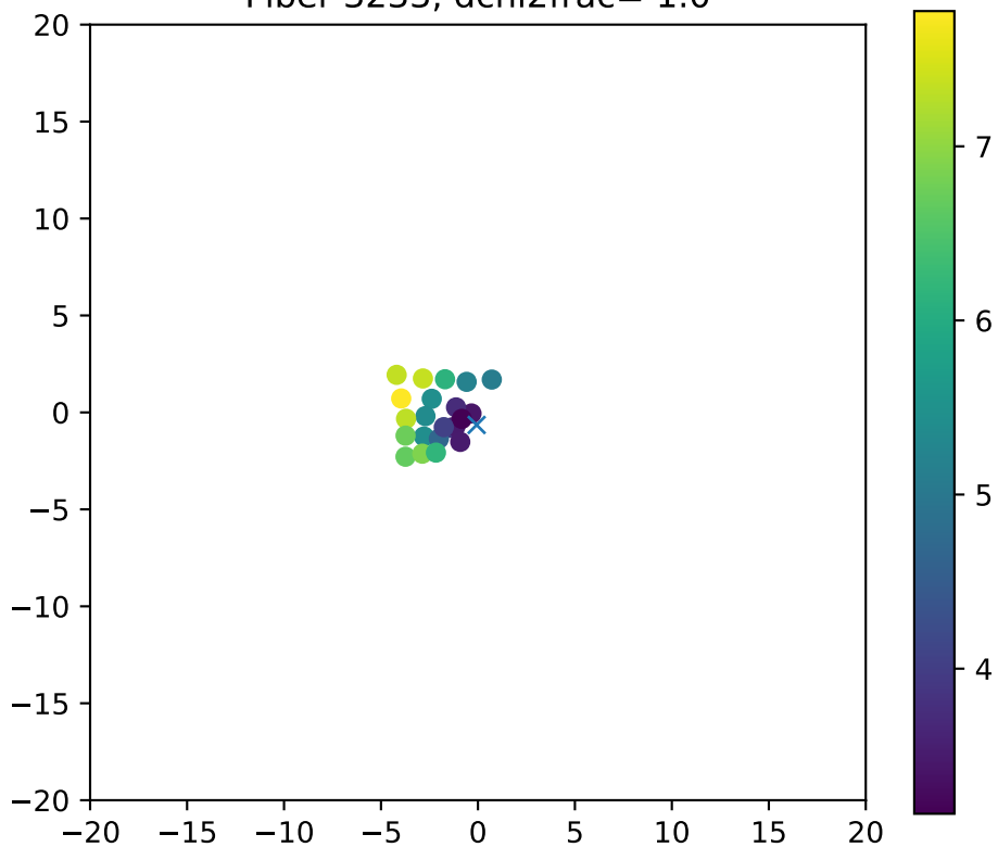
Fiber 3233, dchi2frac= 1.0
