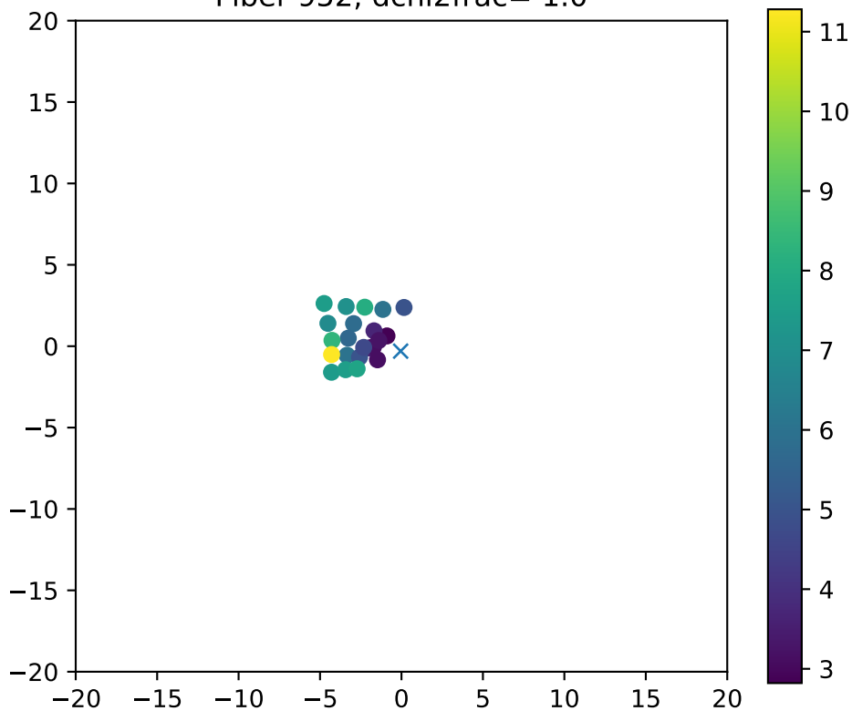
Fiber 952, dchi2frac= 1.0
