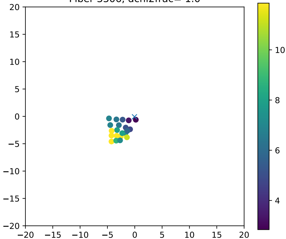
Fiber 3306, dchi2frac= 1.0
