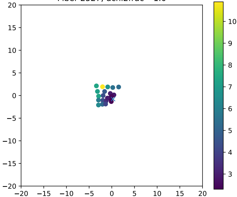
Fiber 2527, dchi2frac= 1.0
