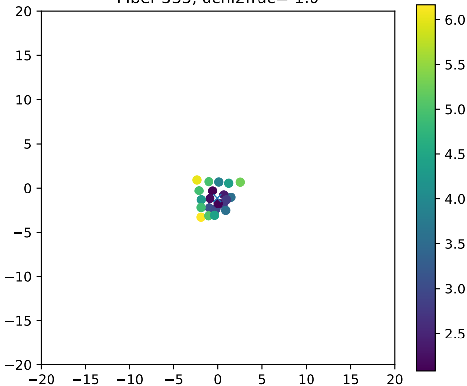
Fiber 535, dchi2frac= 1.0
