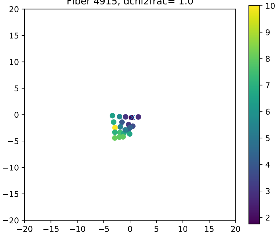
Fiber 4915, dchi2frac= 1.0
