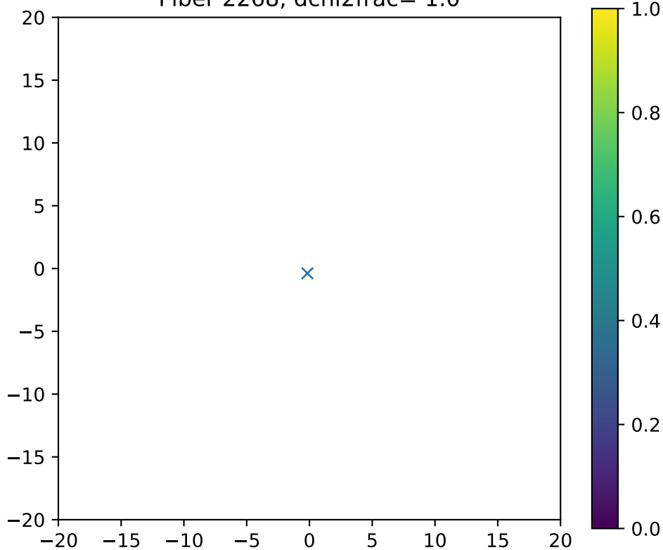
Fiber 2268, dchi2frac= 1.0
