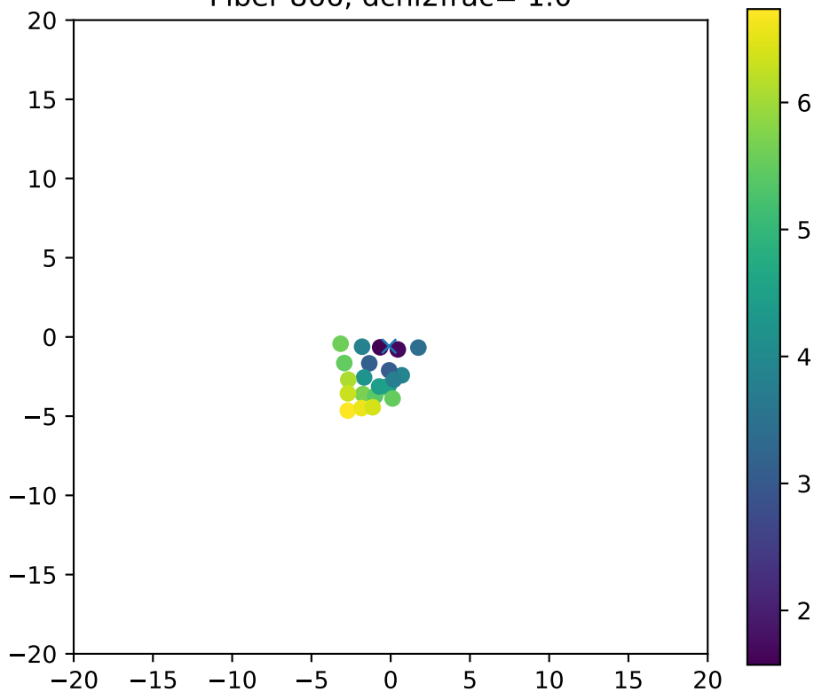
Fiber 866, dchi2frac= 1.0
