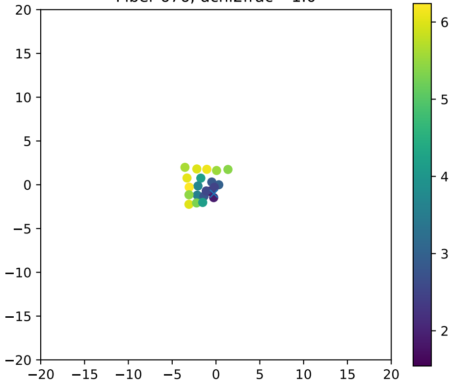
Fiber 676, dchi2frac= 1.0
