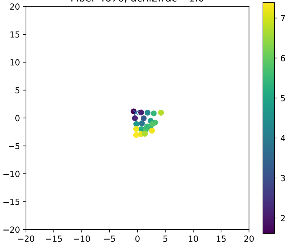
Fiber 4676, dchi2frac= 1.0
