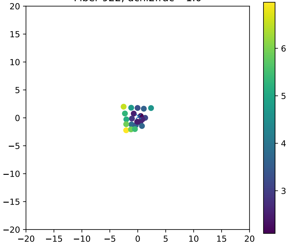
Fiber 922, dchi2frac= 1.0
