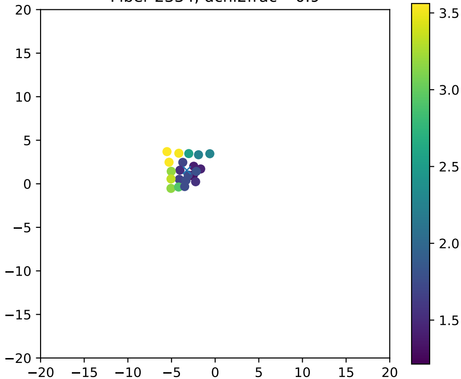
Fiber 2334, dchi2frac= 0.9
