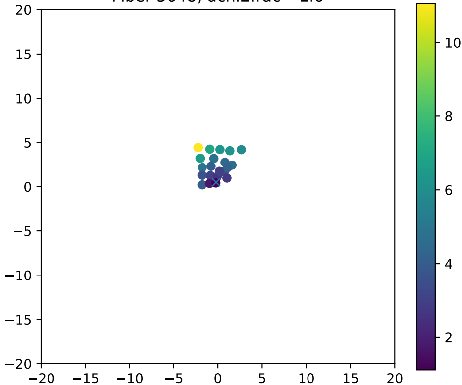
Fiber 3648, dchi2frac= 1.0
