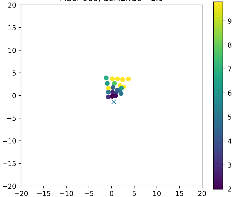
Fiber 980, dchi2frac= 1.0
