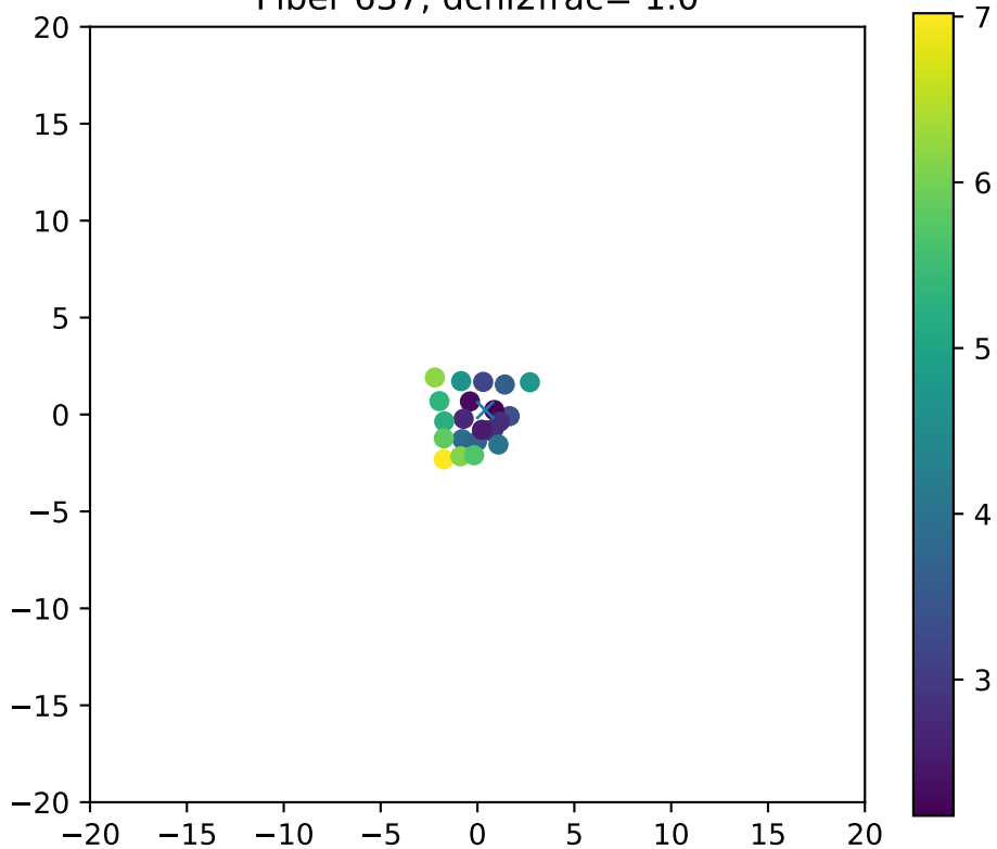
Fiber 637, dchi2frac= 1.0
