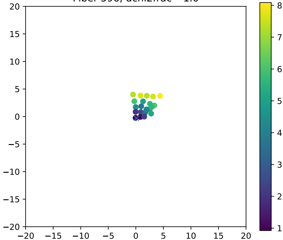
Fiber 596, dchi2frac= 1.0
