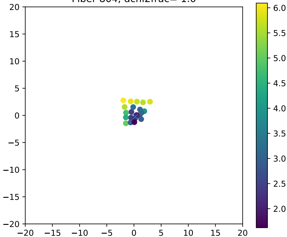
Fiber 804, dchi2frac= 1.0
