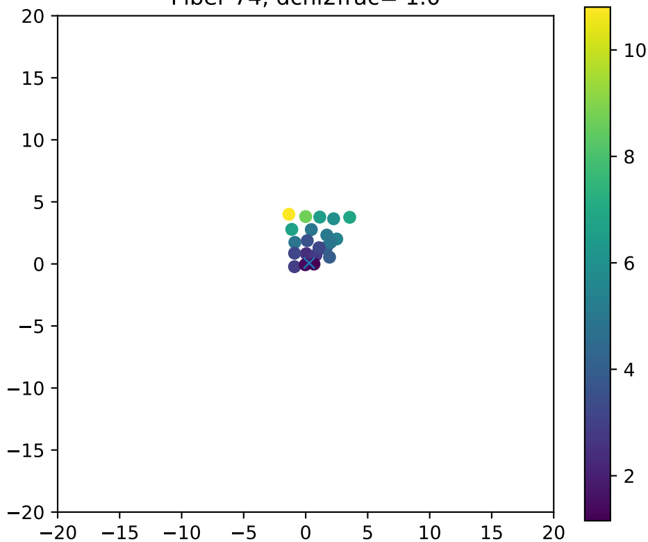
Fiber 74, dchi2frac= 1.0
