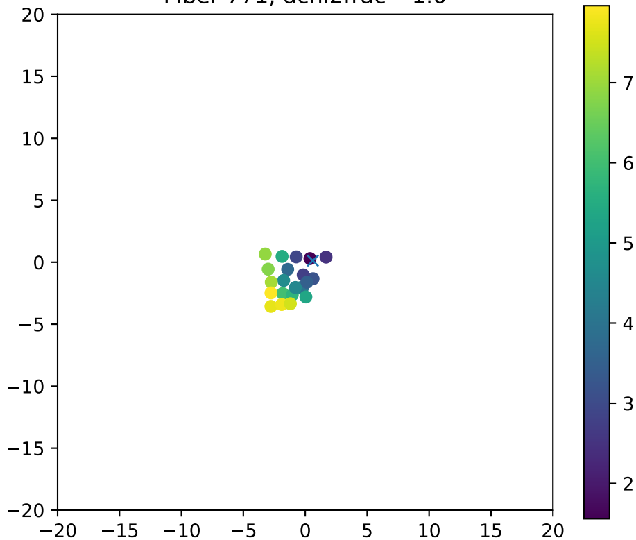
Fiber 771, dchi2frac= 1.0
