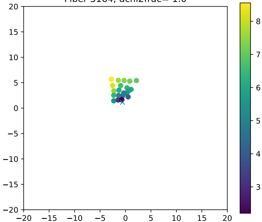
Fiber 3164, dchi2frac= 1.0
