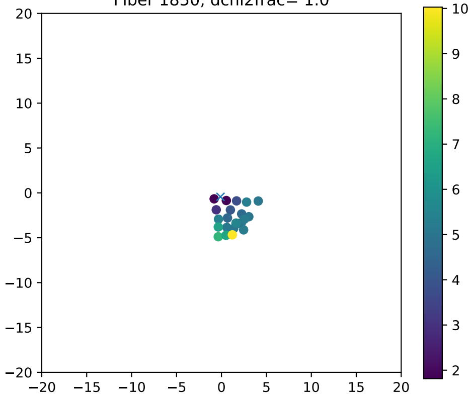
Fiber 1850, dchi2frac= 1.0
