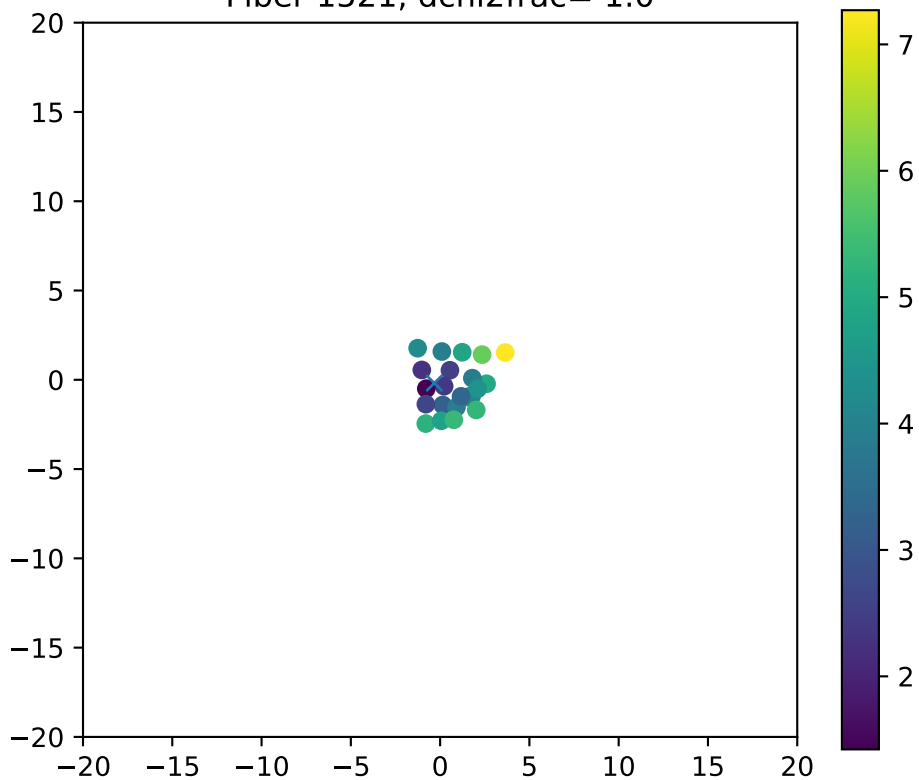
Fiber 1521, dchi2frac= 1.0
