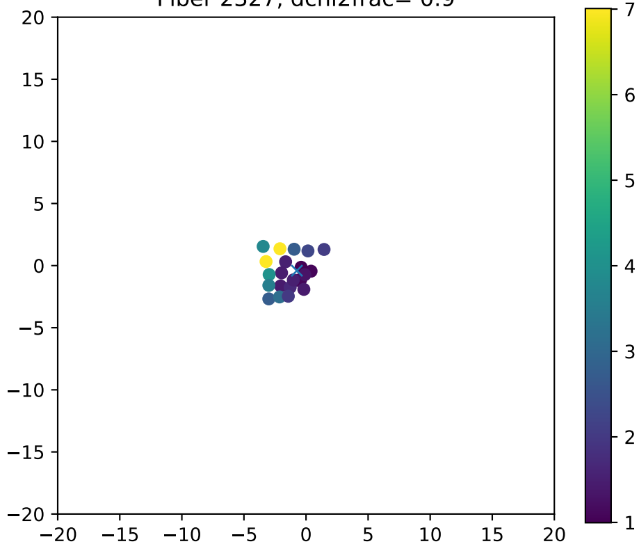
Fiber 2327, dchi2frac= 0.9
