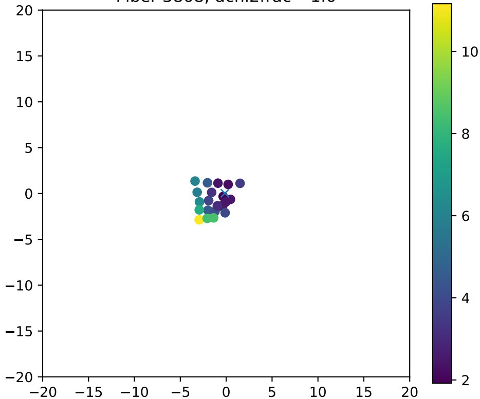
Fiber 3808, dchi2frac= 1.0
