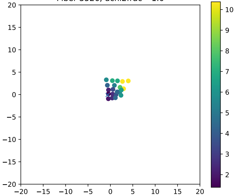
Fiber 3526, dchi2frac= 1.0
