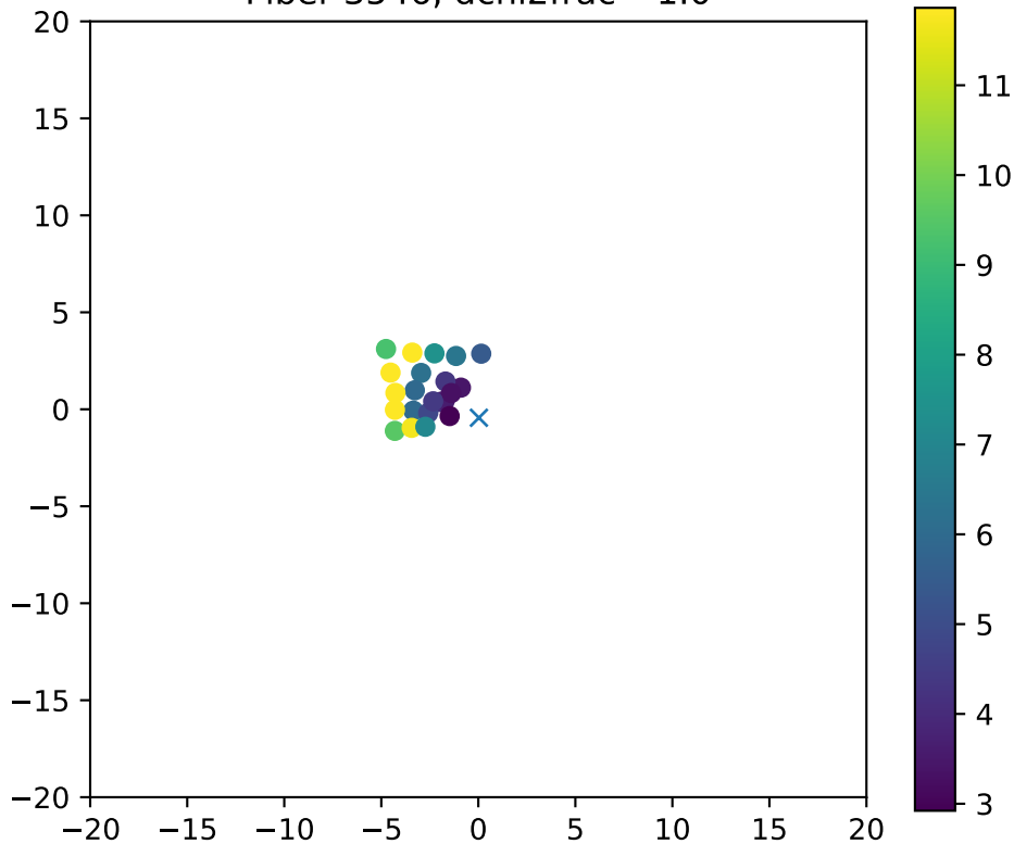
Fiber 3546, dchi2frac= 1.0
