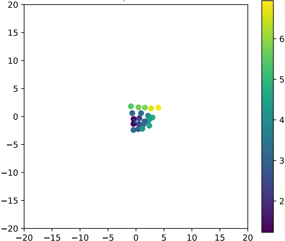
Fiber 2522, dchi2frac= 1.0
