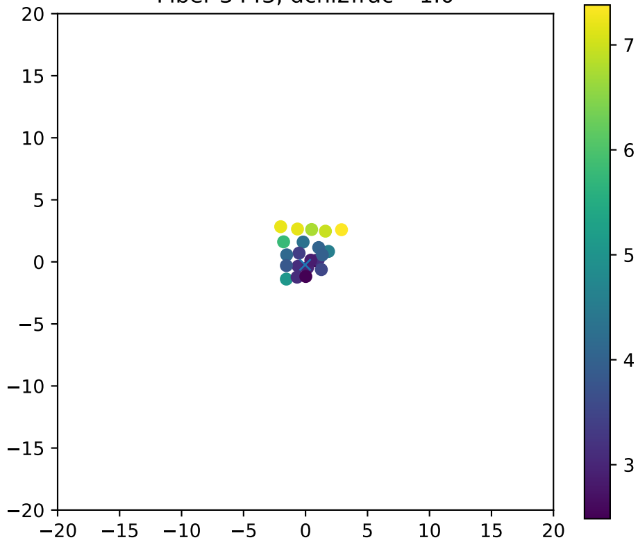
Fiber 3443, dchi2frac= 1.0
