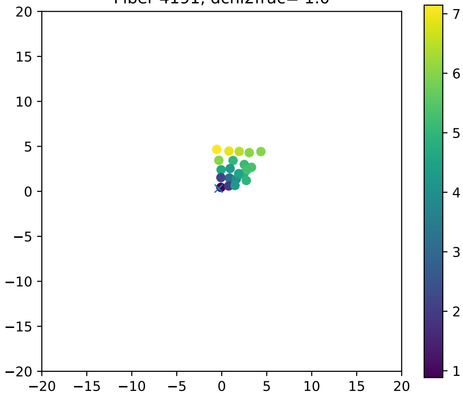
Fiber 4191, dchi2frac= 1.0
