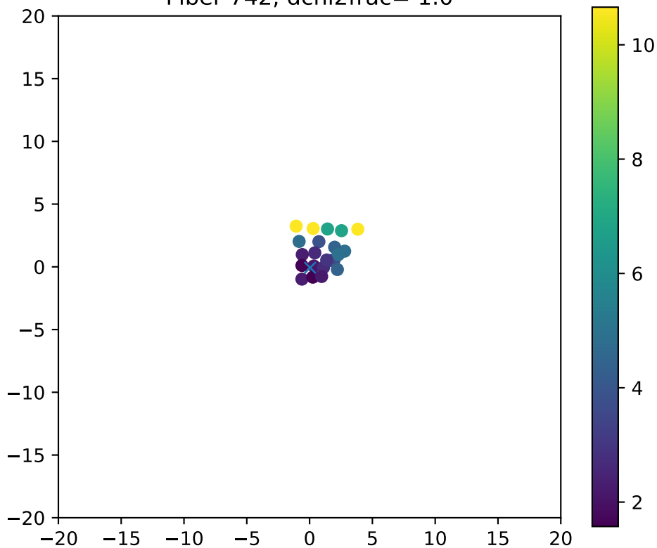
Fiber 742, dchi2frac= 1.0
