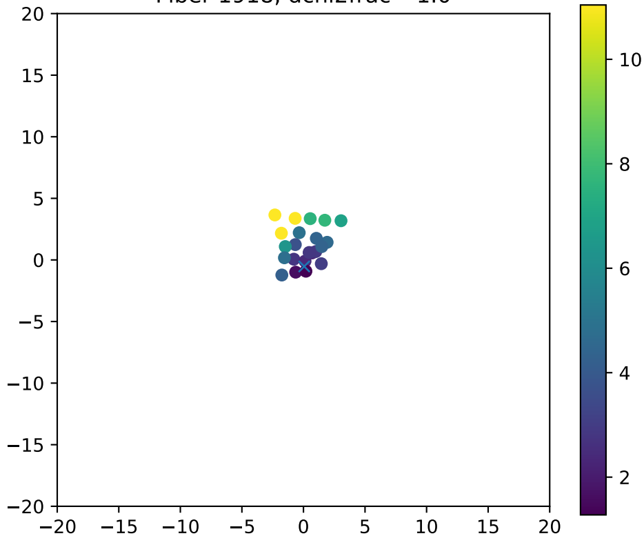
Fiber 1918, dchi2frac= 1.0
