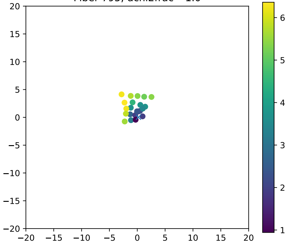
Fiber 795, dchi2frac= 1.0
