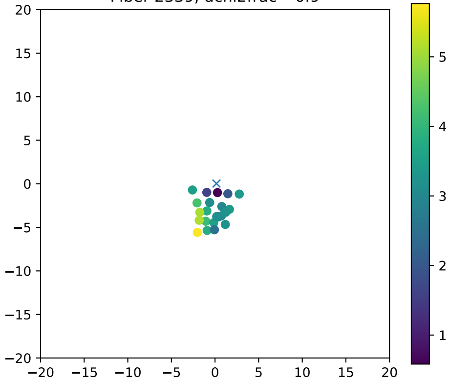
Fiber 2339, dchi2frac= 0.9
