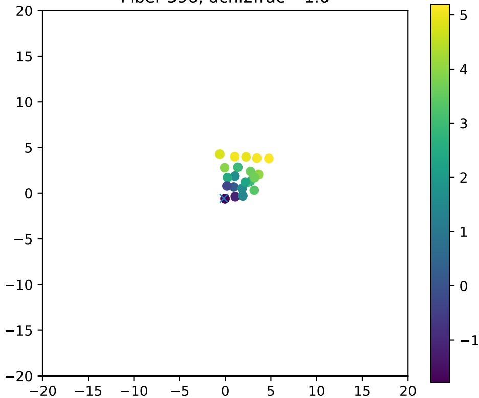
Fiber 596, dchi2frac= 1.0
