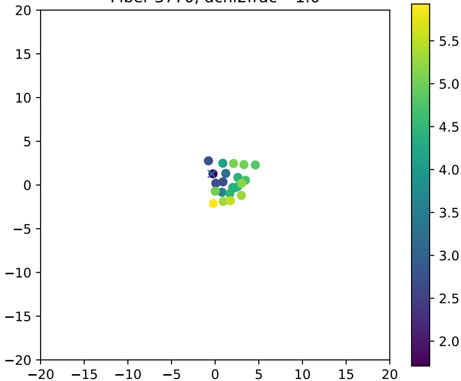
Fiber 3770, dchi2frac= 1.0
