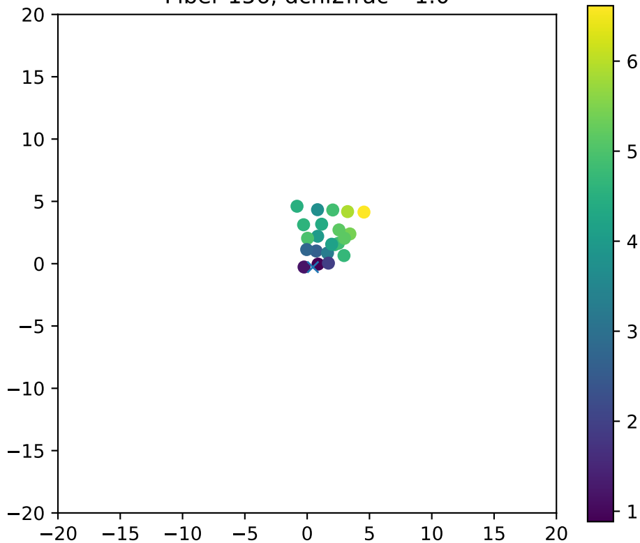
Fiber 156, dchi2frac= 1.0
