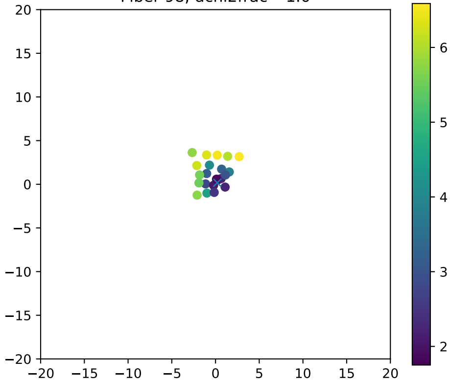
Fiber 98, dchi2frac= 1.0
