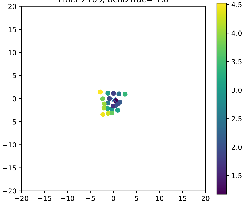
Fiber 2109, dchi2frac= 1.0
