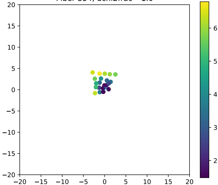
Fiber 354, dchi2frac= 1.0
