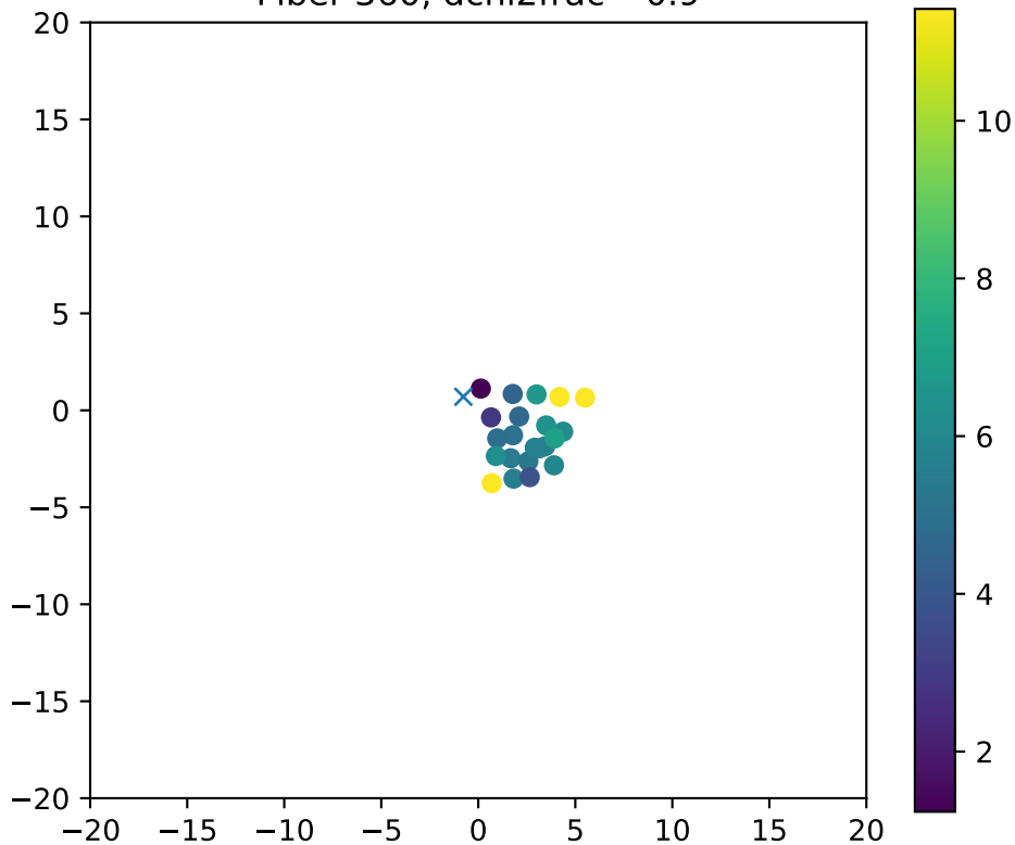
Fiber 360, dchi2frac= 0.9
