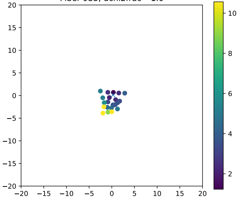
Fiber 935, dchi2frac= 1.0
