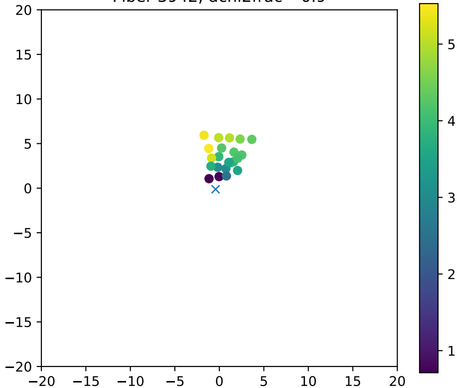
Fiber 3942, dchi2frac= 0.9
