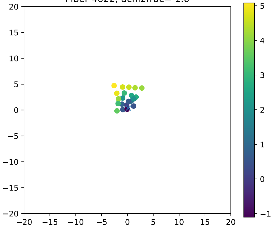
Fiber 4622, dchi2frac= 1.0
