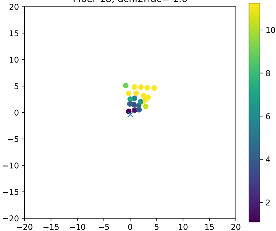
Fiber 18, dchi2frac= 1.0
