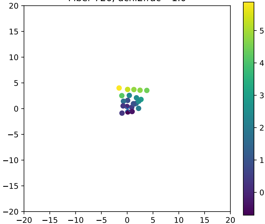
Fiber 726, dchi2frac= 1.0
