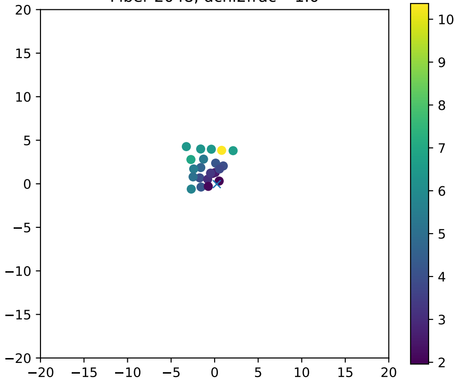
Fiber 2048, dchi2frac= 1.0
