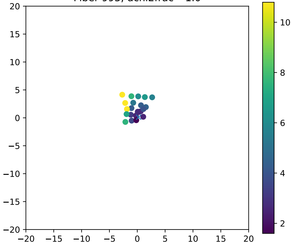
Fiber 993, dchi2frac= 1.0
