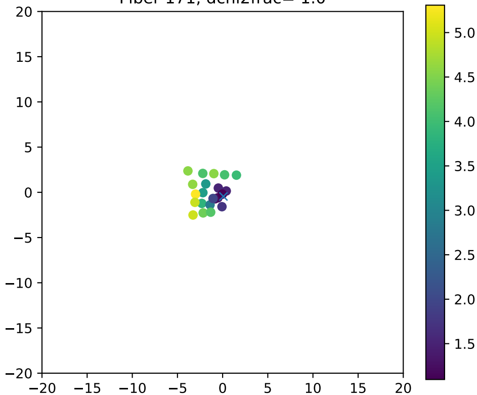
Fiber 171, dchi2frac= 1.0
