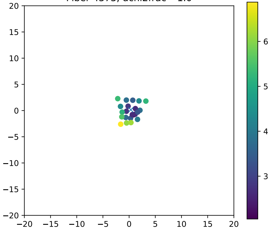
Fiber 4373, dchi2frac= 1.0
