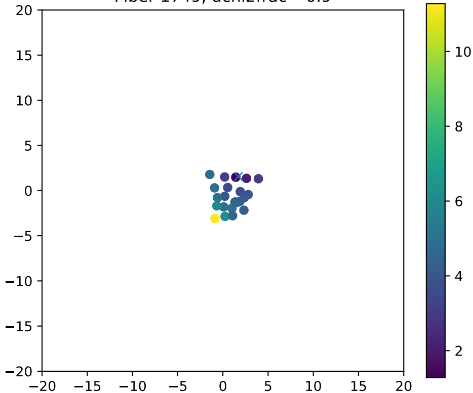
Fiber 1749, dchi2frac= 0.9
