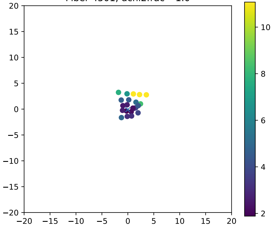
Fiber 4501, dchi2frac= 1.0
