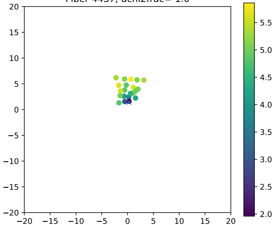
Fiber 4437, dchi2frac= 1.0
