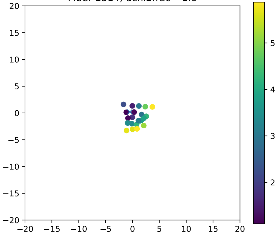
Fiber 1514, dchi2frac= 1.0
