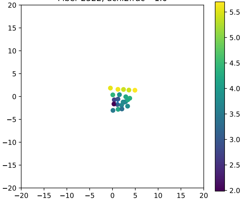
Fiber 2322, dchi2frac= 1.0
