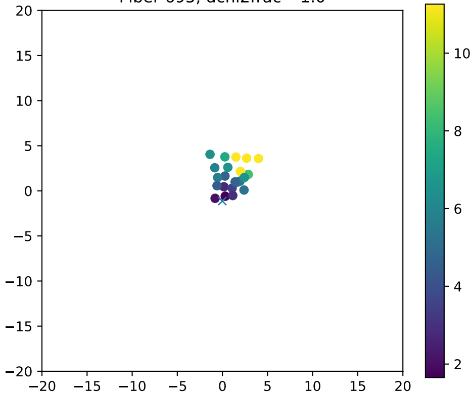
Fiber 695, dchi2frac= 1.0
