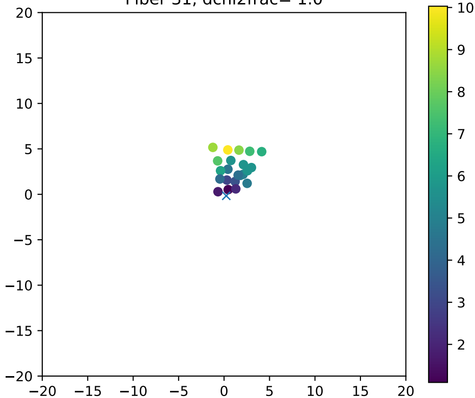
Fiber 31, dchi2frac= 1.0
