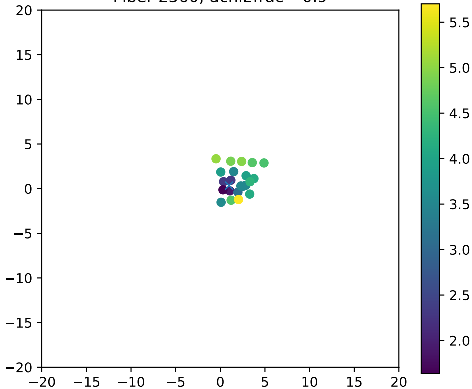
Fiber 2560, dchi2frac= 0.9
