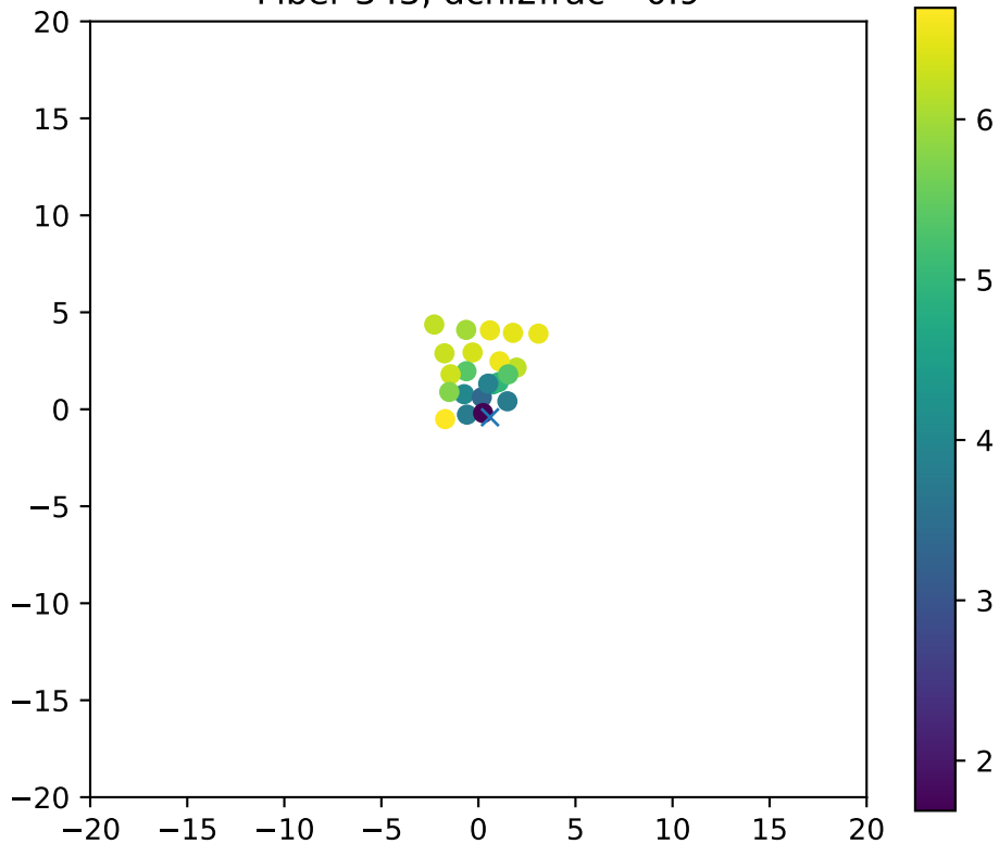
Fiber 343, dchi2frac= 0.9
