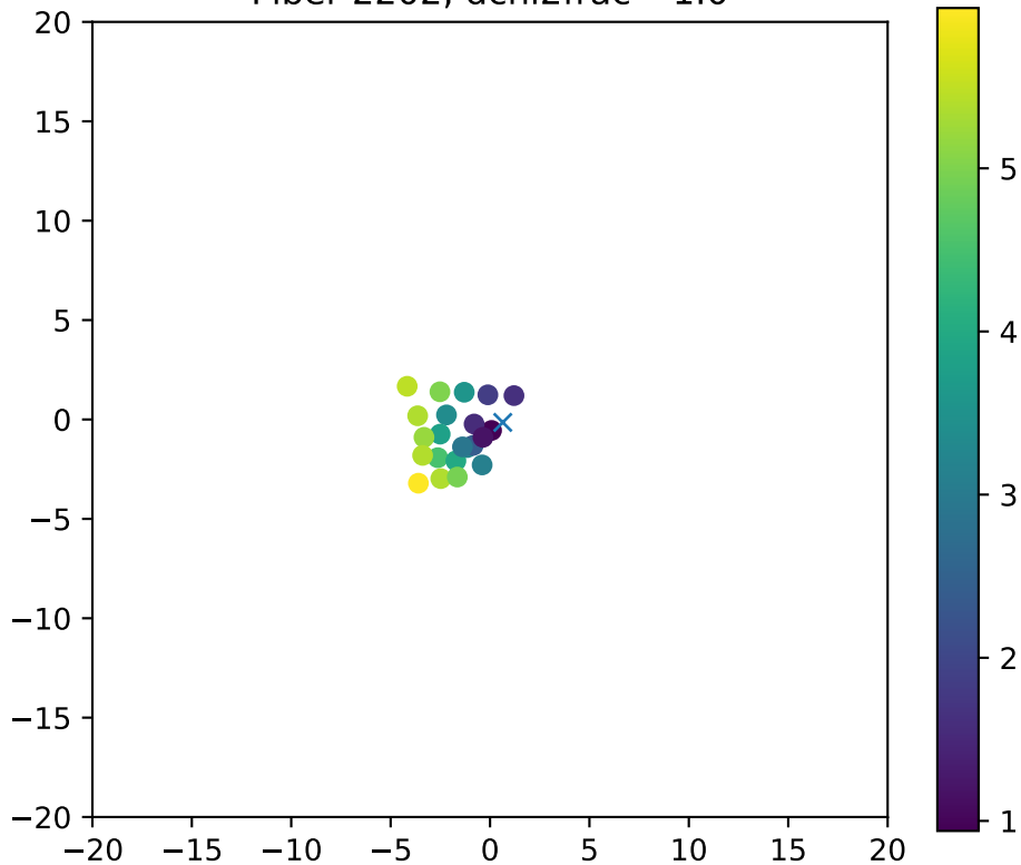
Fiber 2202, dchi2frac= 1.0
