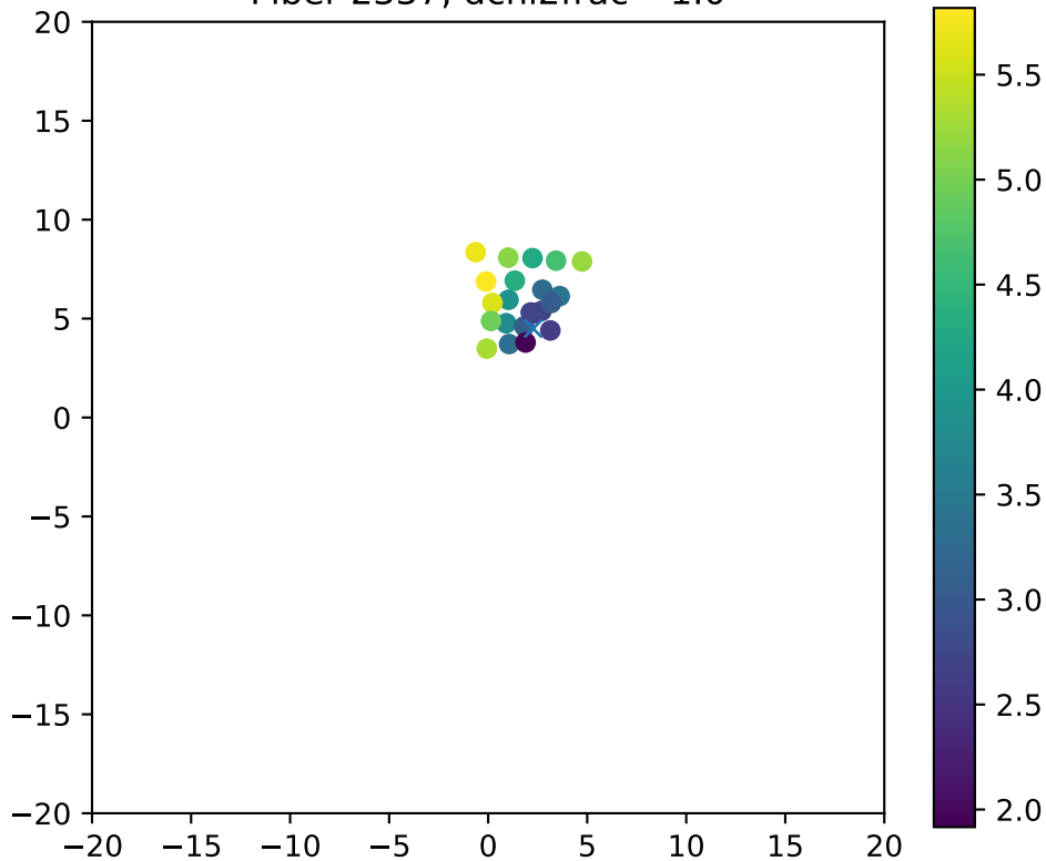
Fiber 2337, dchi2frac= 1.0
