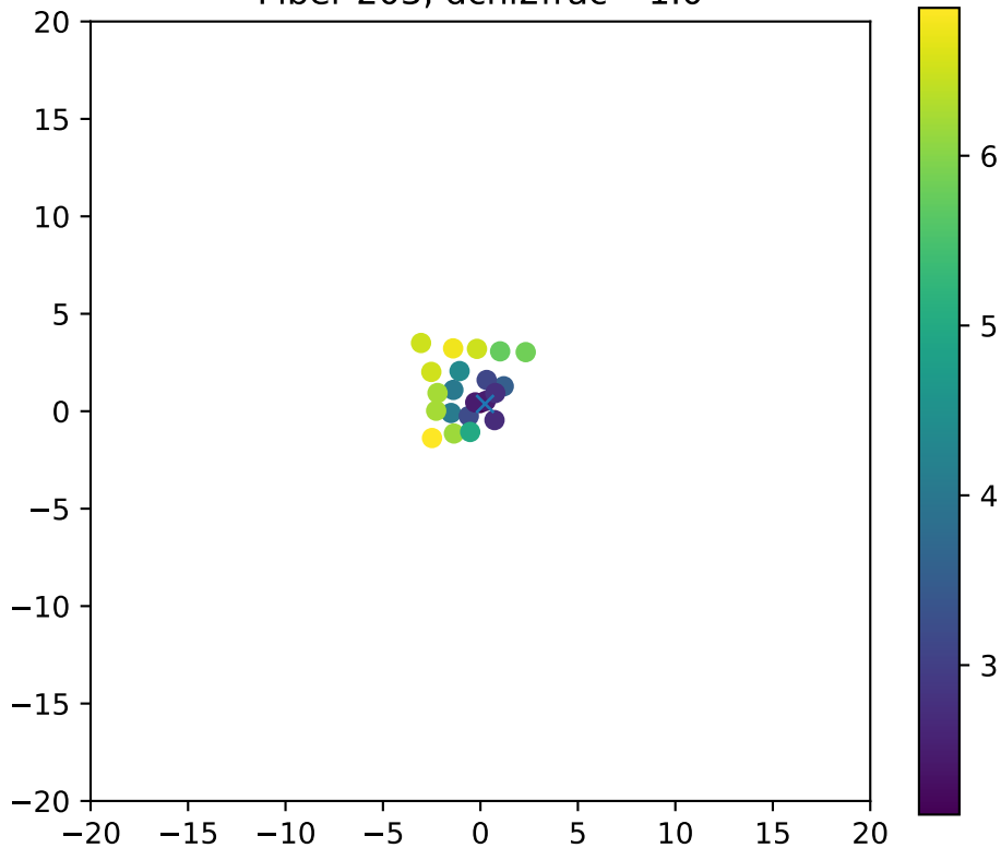
Fiber 203, dchi2frac= 1.0
