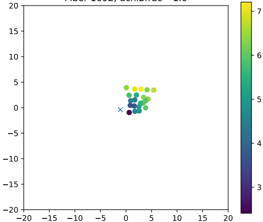
Fiber 1692, dchi2frac= 1.0
