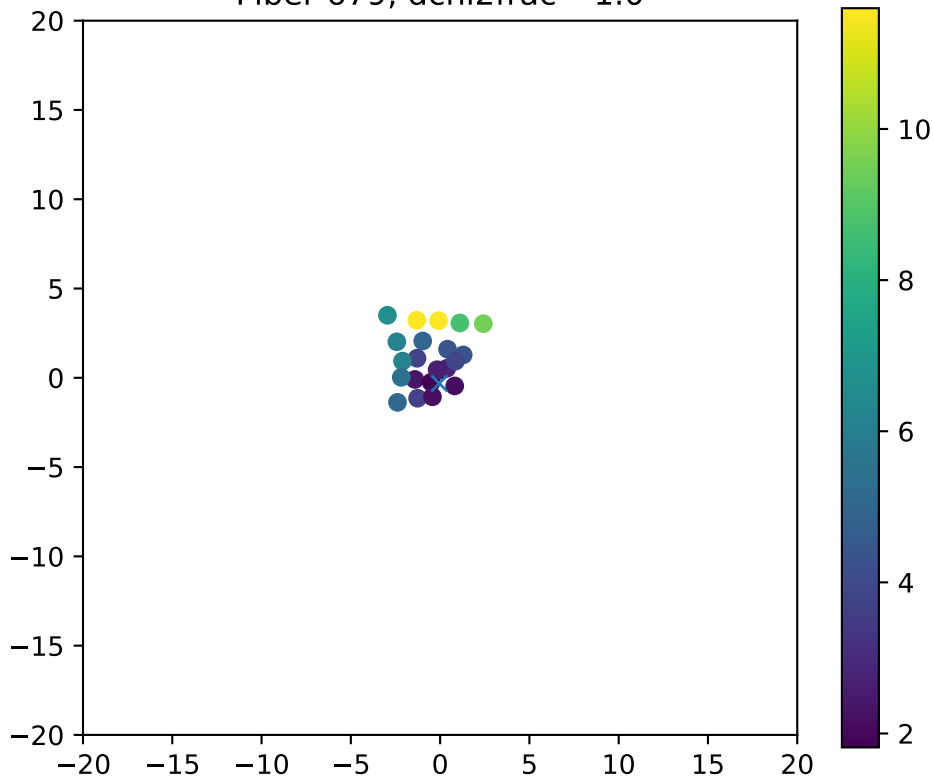
Fiber 679, dchi2frac= 1.0
