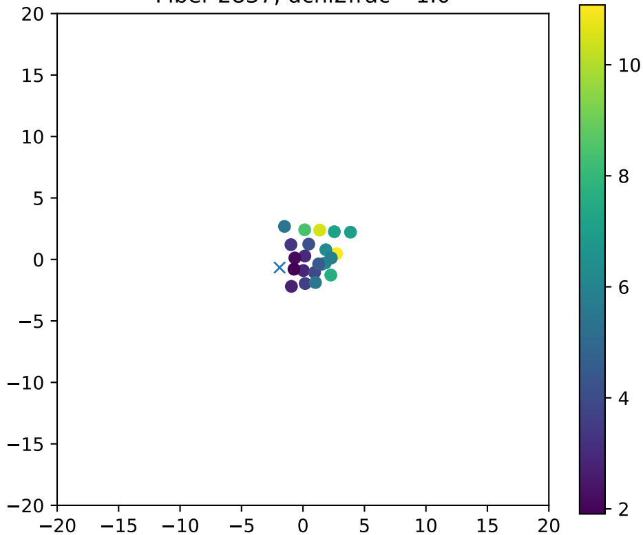
Fiber 2837, dchi2frac= 1.0
