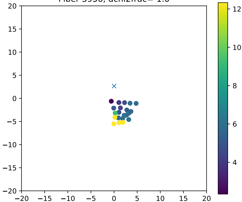
Fiber 3956, dchi2frac= 1.0
