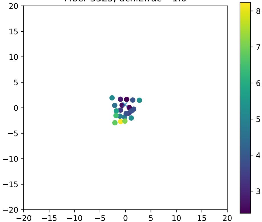
Fiber 3525, dchi2frac= 1.0
