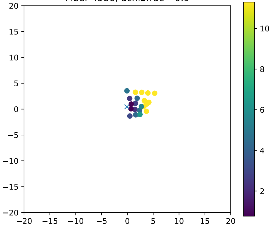
Fiber 4986, dchi2frac= 0.9
