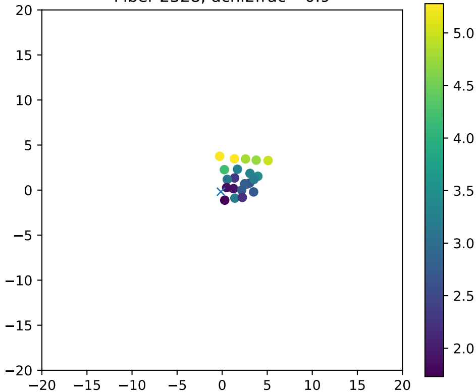
Fiber 2328, dchi2frac= 0.9
