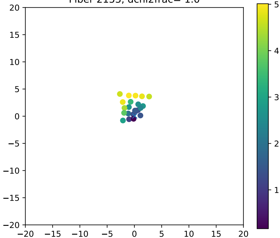
Fiber 2153, dchi2frac= 1.0
