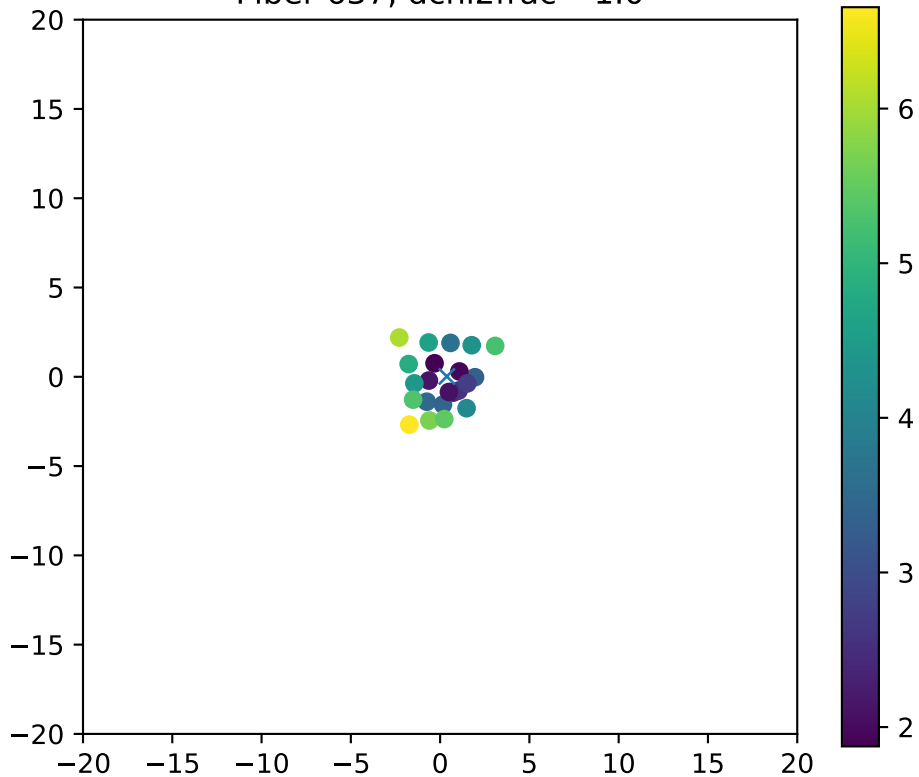
Fiber 637, dchi2frac= 1.0
