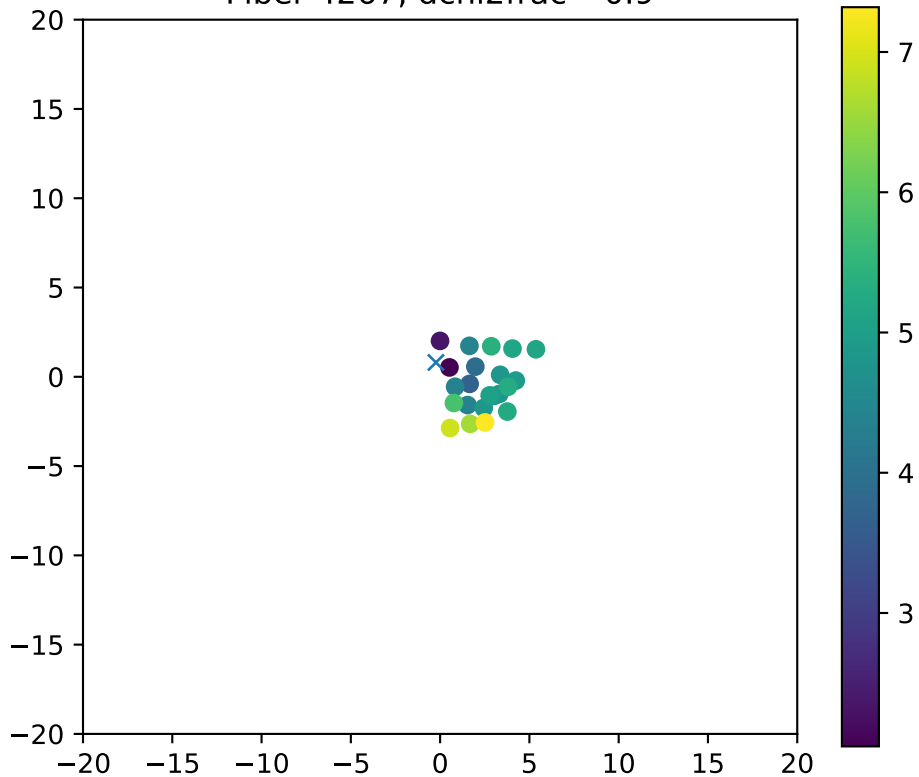
Fiber 4267, dchi2frac= 0.9
