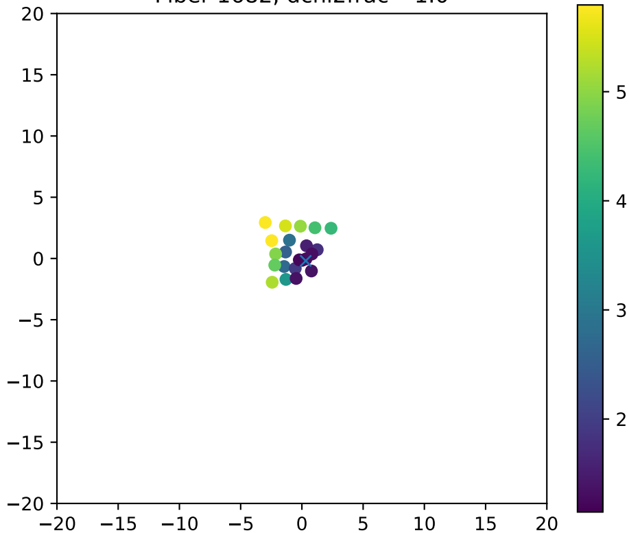
Fiber 1682, dchi2frac= 1.0
