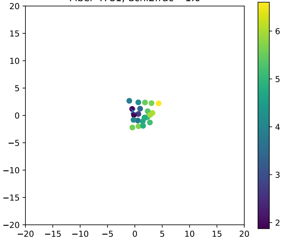
Fiber 4781, dchi2frac= 1.0
