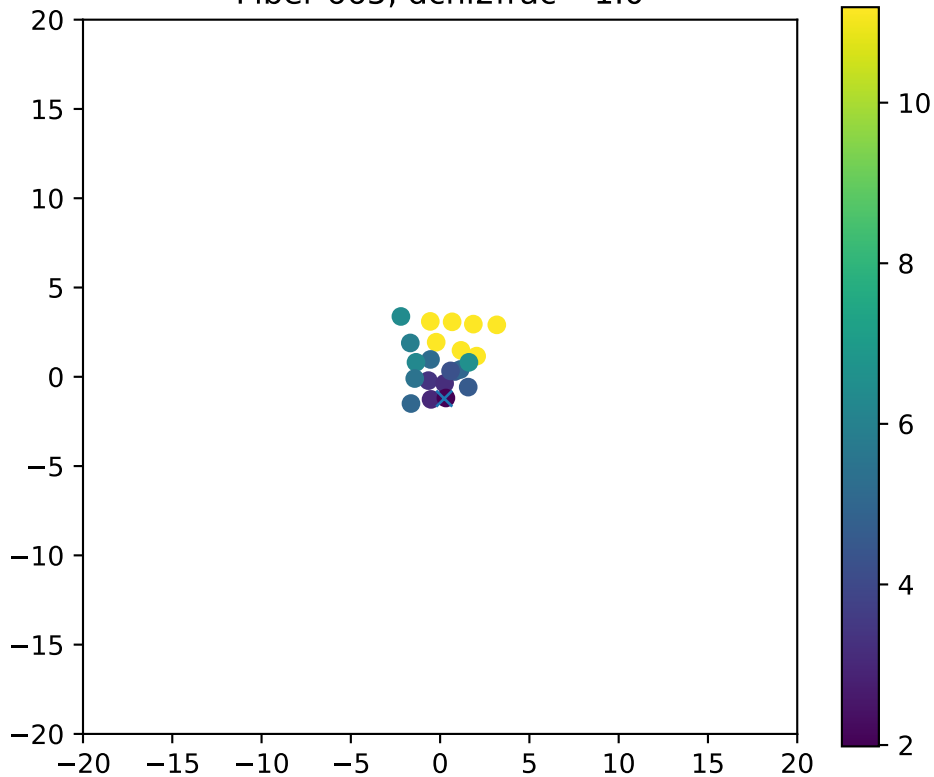
Fiber 665, dchi2frac= 1.0
