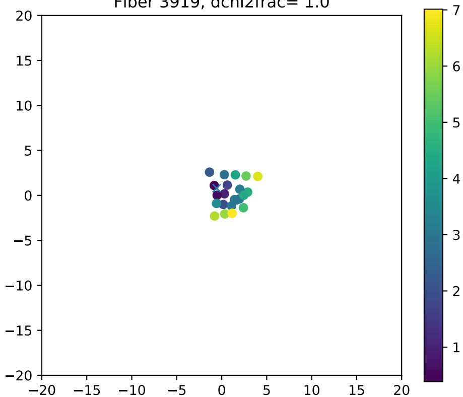
Fiber 3919, dchi2frac= 1.0
