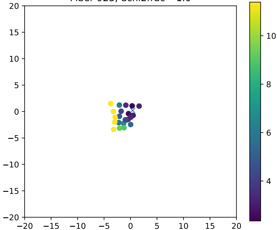
Fiber 923, dchi2frac= 1.0
