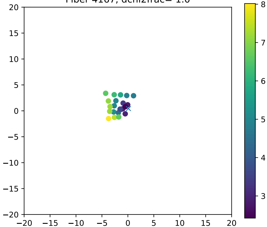
Fiber 4167, dchi2frac= 1.0
