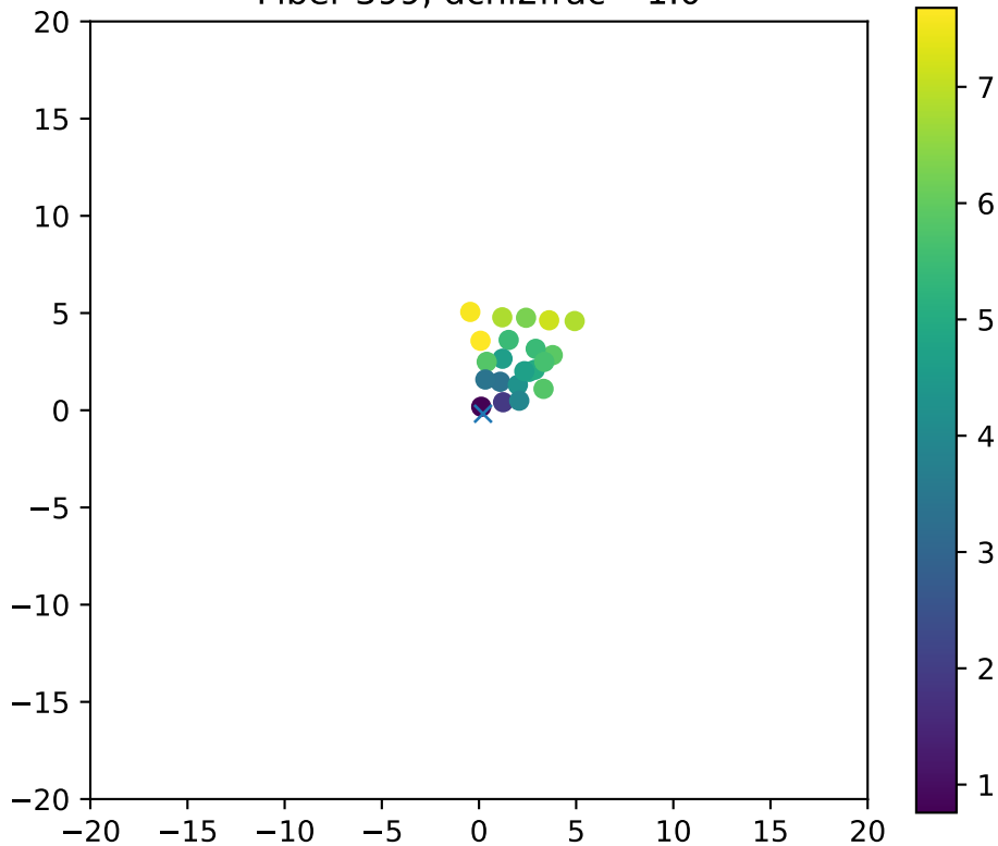
Fiber 399, dchi2frac= 1.0
