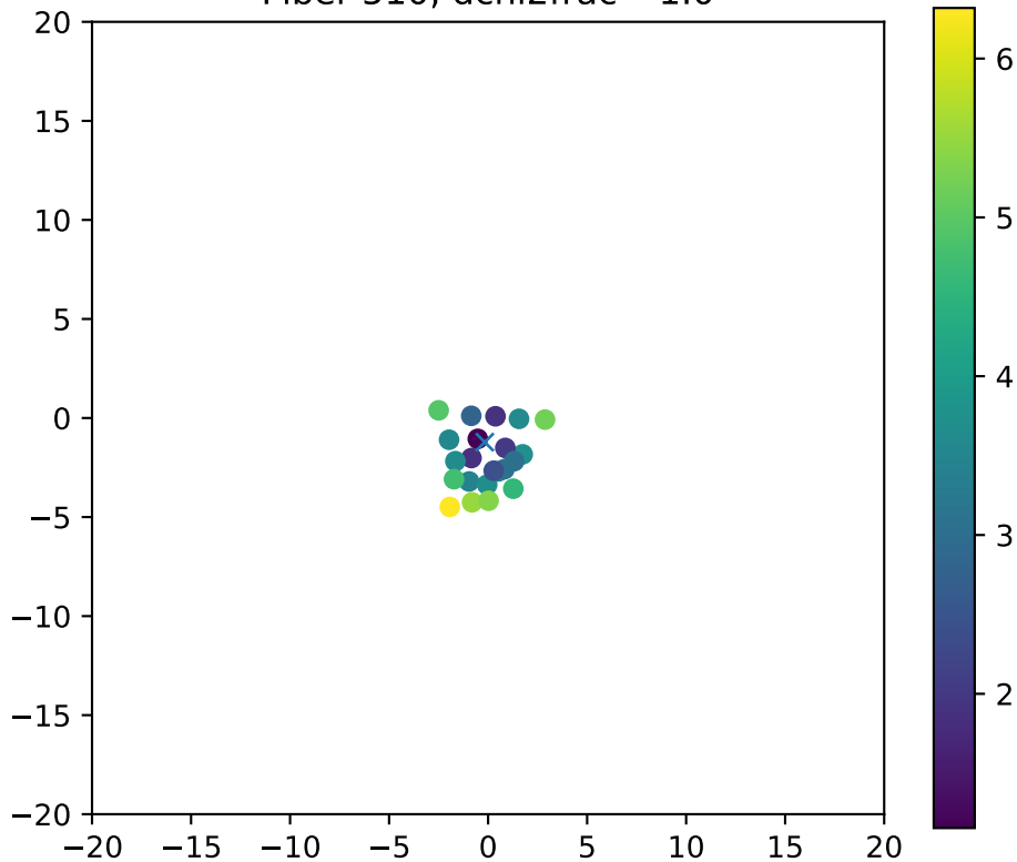
Fiber 510, dchi2frac= 1.0
