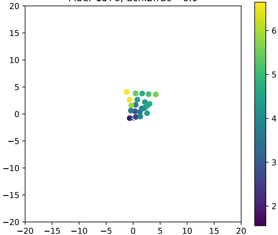
Fiber 1576, dchi2frac= 0.9
