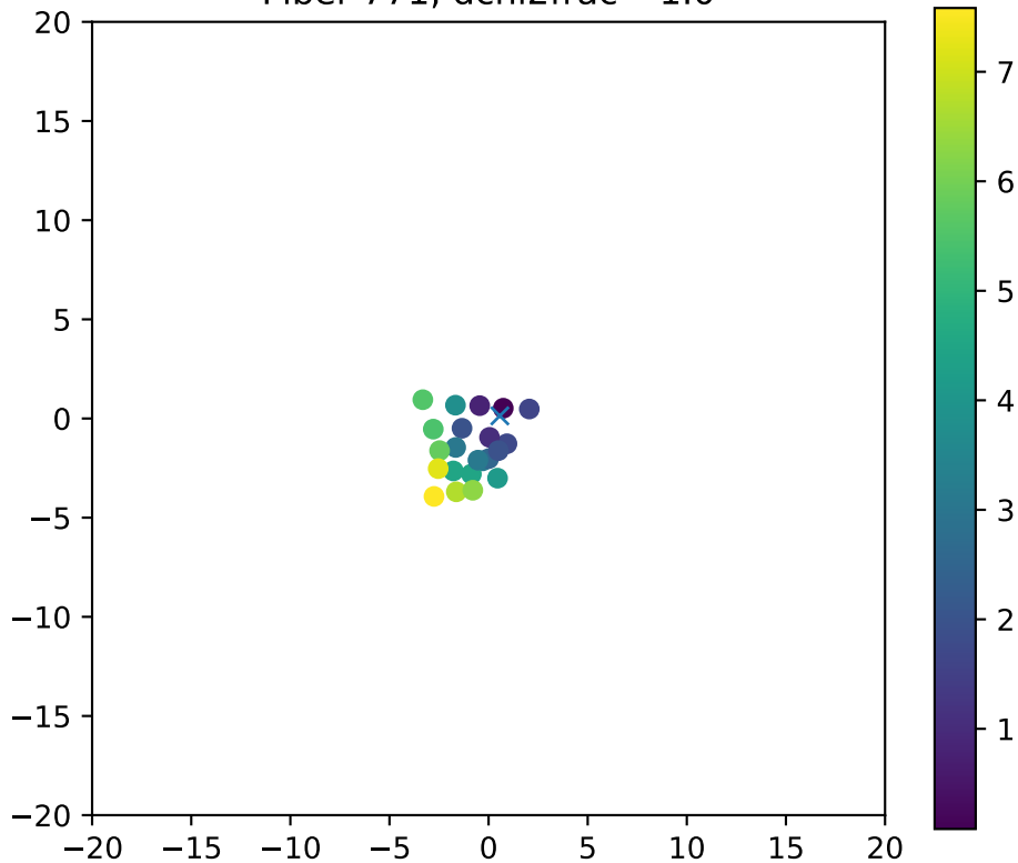
Fiber 771, dchi2frac= 1.0
