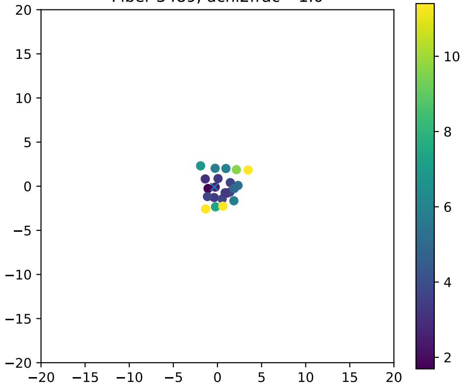
Fiber 3489, dchi2frac= 1.0
