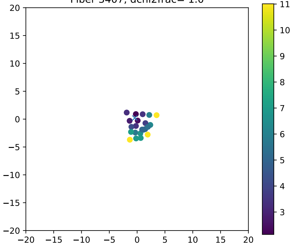
Fiber 3407, dchi2frac= 1.0
