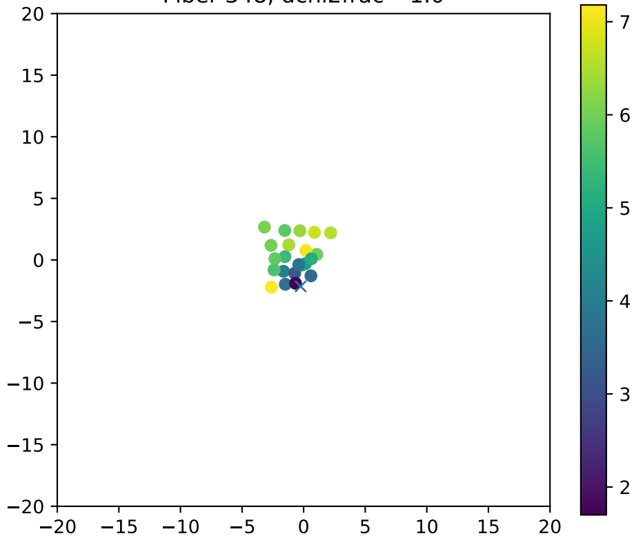
Fiber 348, dchi2frac= 1.0
