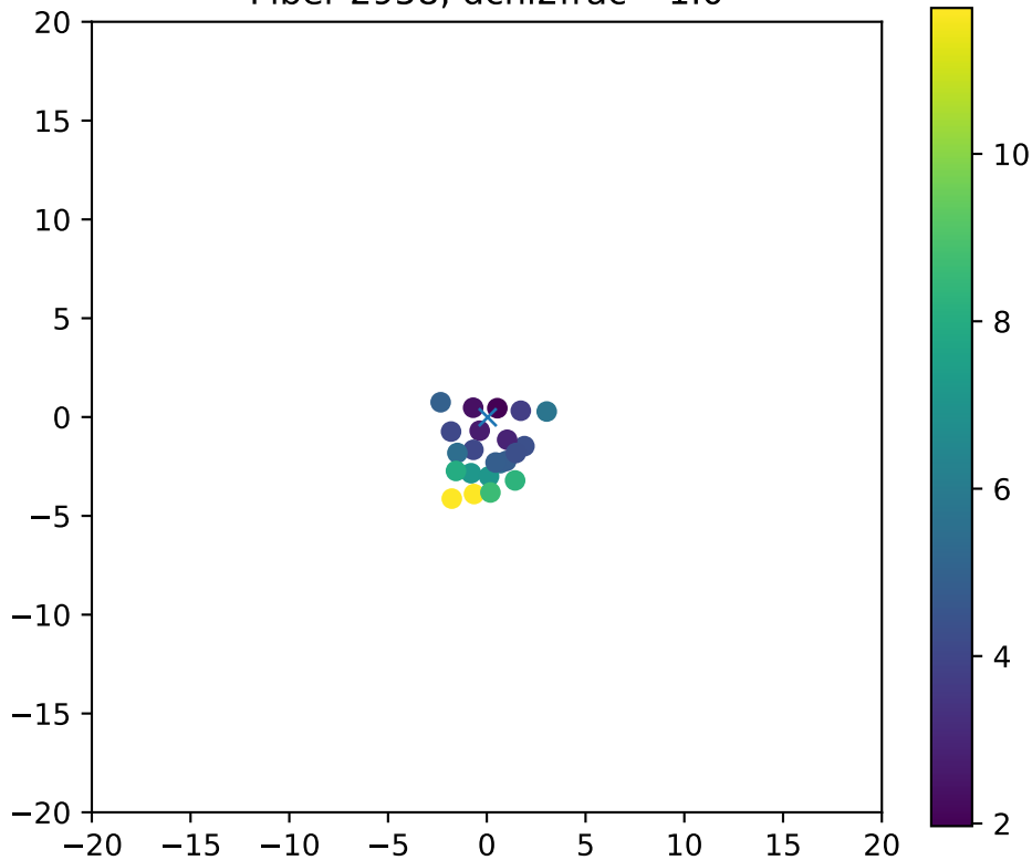
Fiber 2958, dchi2frac= 1.0
