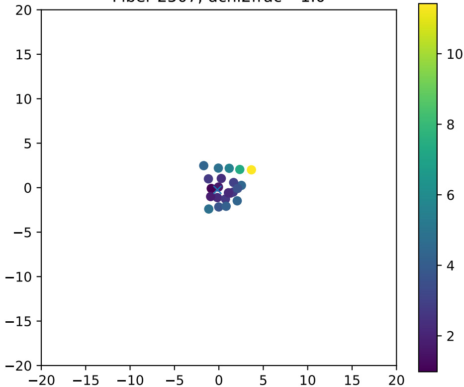
Fiber 2507, dchi2frac= 1.0
