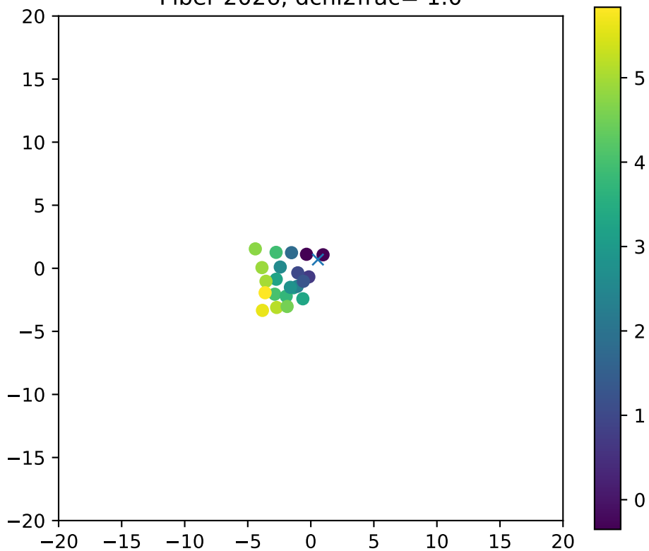
Fiber 2026, dchi2frac= 1.0
