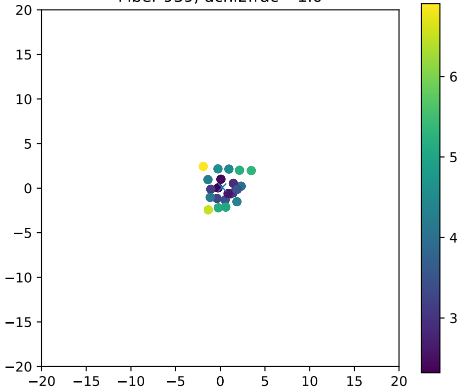
Fiber 939, dchi2frac= 1.0
