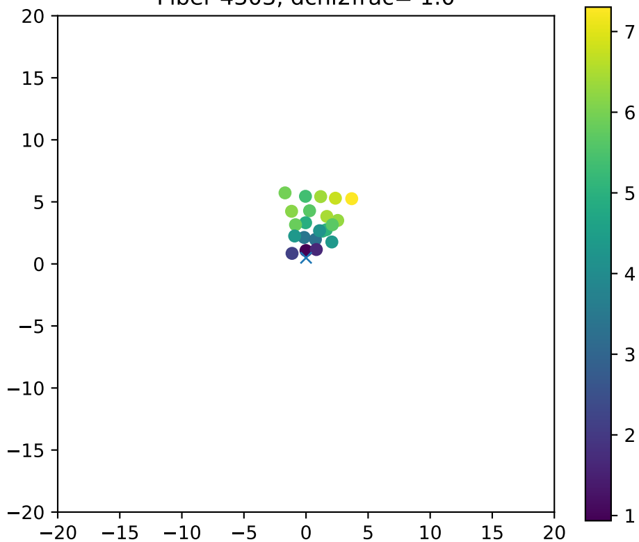
Fiber 4303, dchi2frac= 1.0
