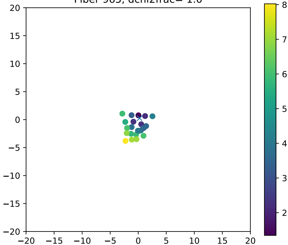
Fiber 965, dchi2frac= 1.0
