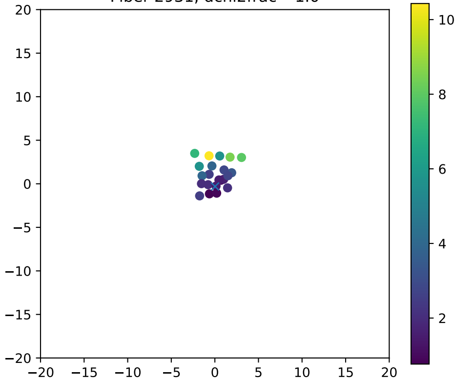
Fiber 2931, dchi2frac= 1.0
