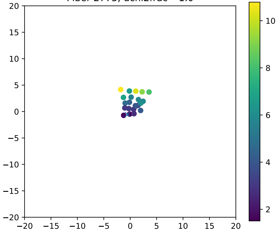
Fiber 2775, dchi2frac= 1.0
