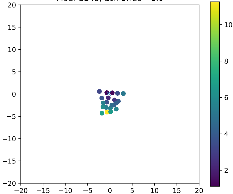
Fiber 3248, dchi2frac= 1.0
