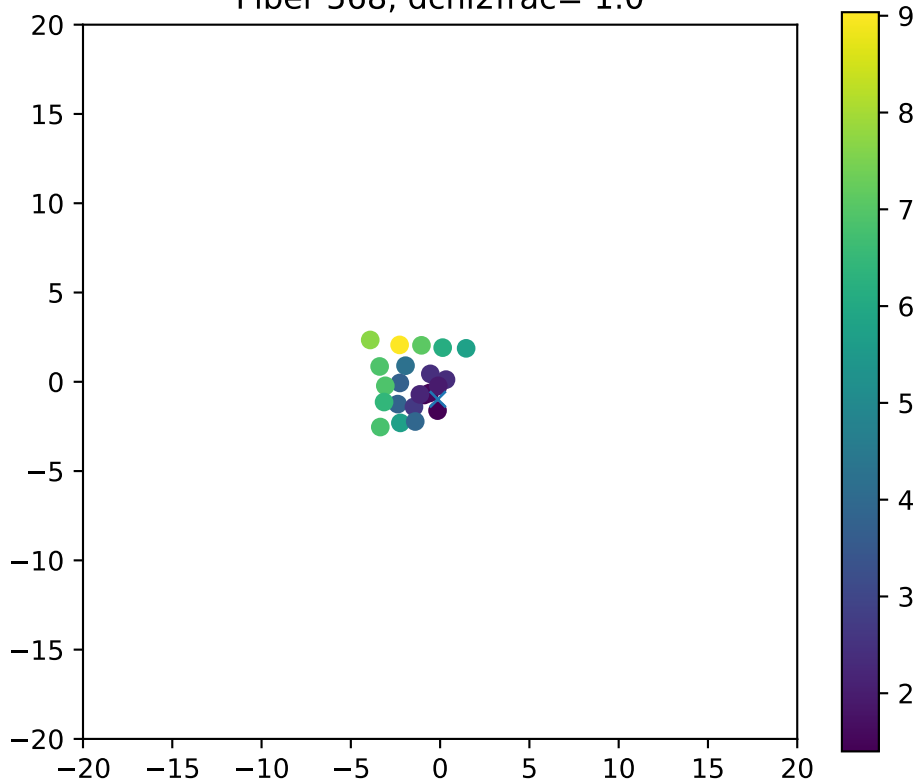
Fiber 568, dchi2frac= 1.0
