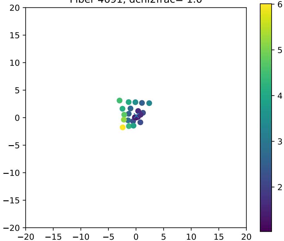
Fiber 4691, dchi2frac= 1.0
