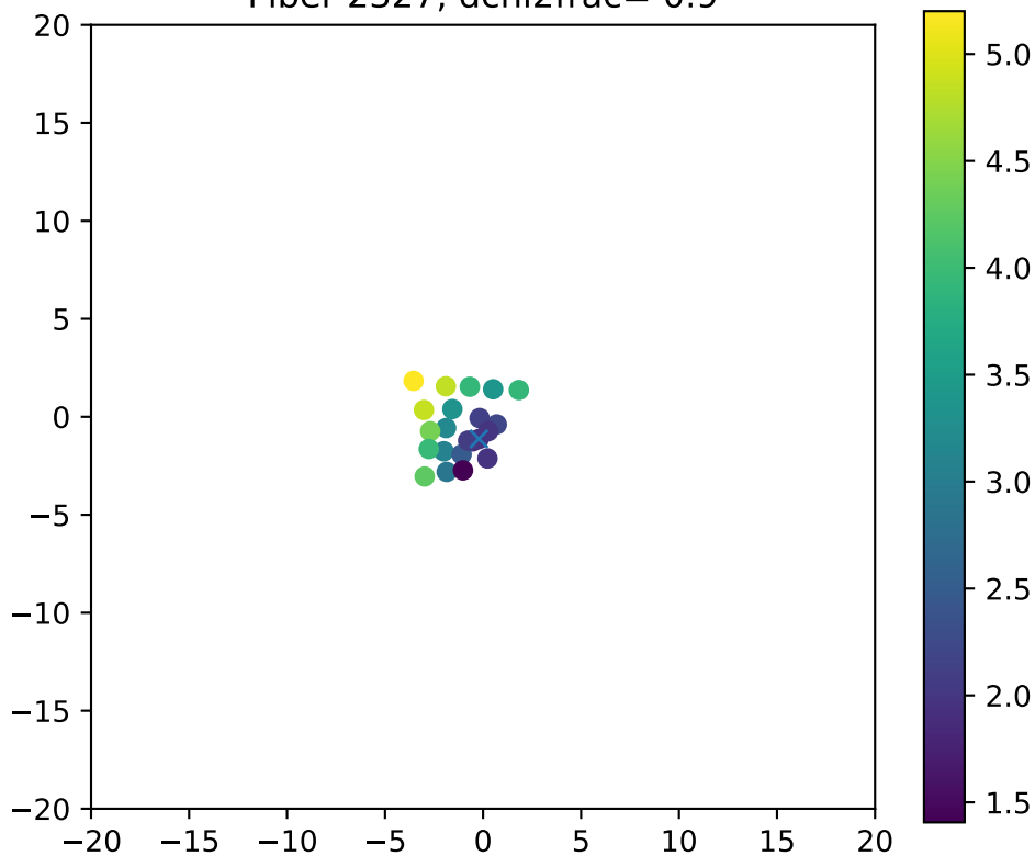
Fiber 2327, dchi2frac= 0.9
