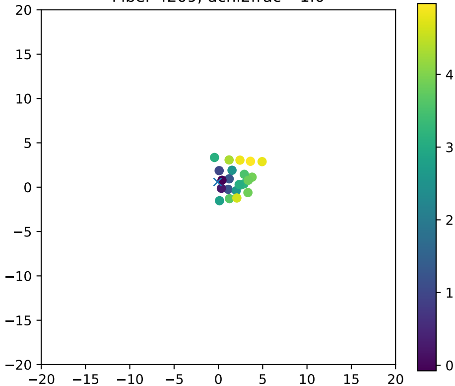
Fiber 4209, dchi2frac= 1.0
