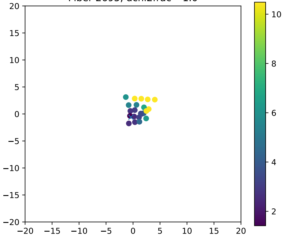
Fiber 2695, dchi2frac= 1.0
