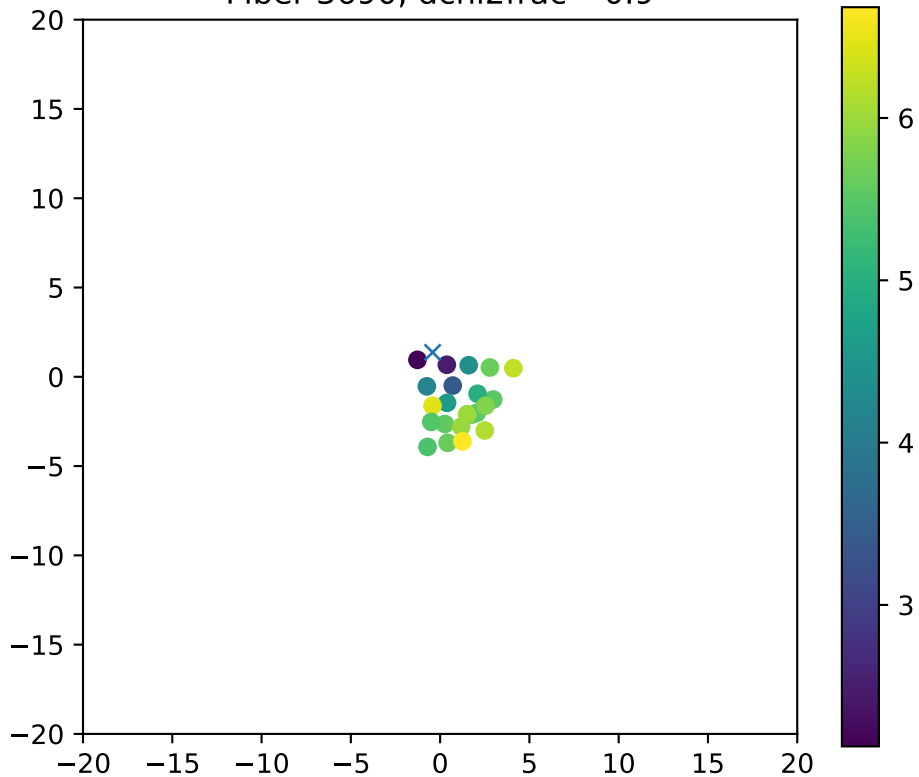
Fiber 3690, dchi2frac= 0.9
