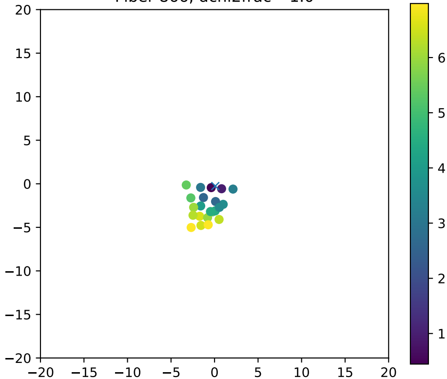
Fiber 866, dchi2frac= 1.0
