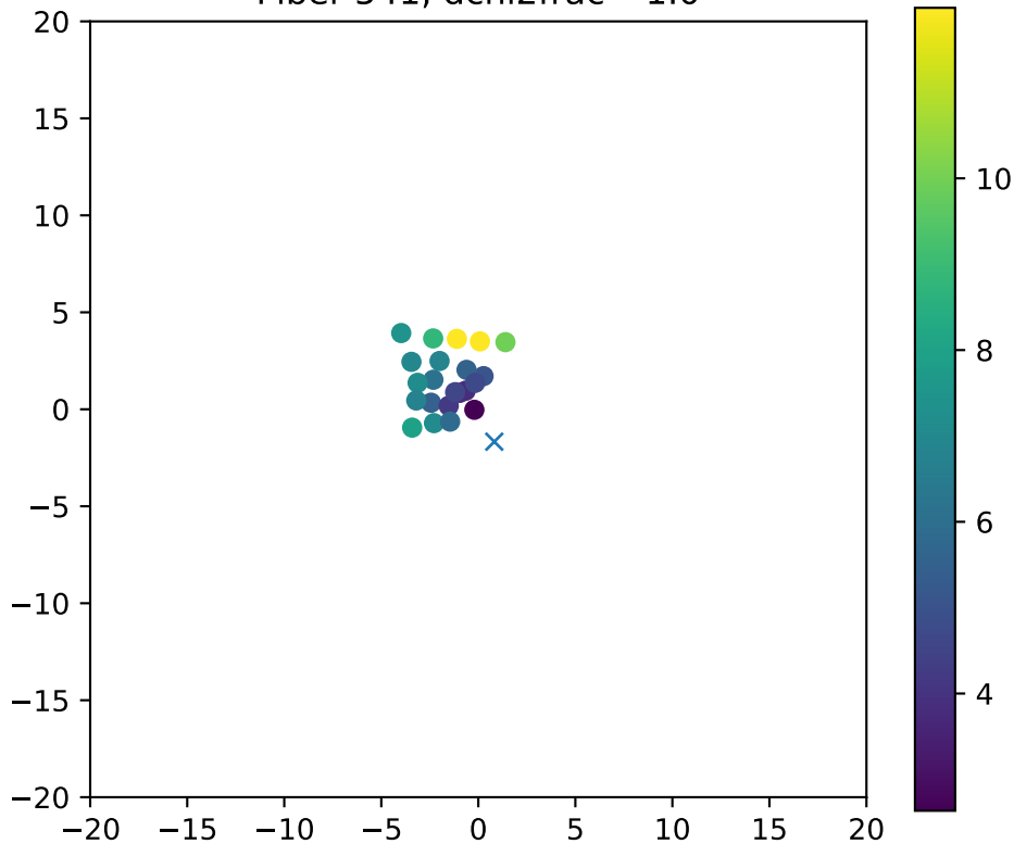
Fiber 541, dchi2frac= 1.0
