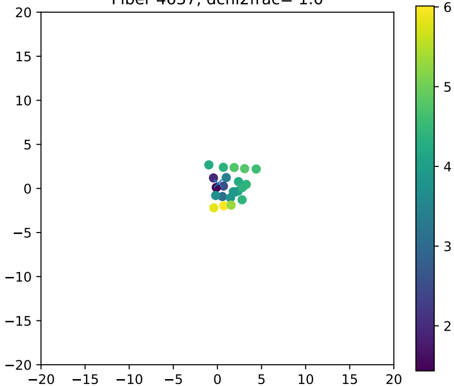
Fiber 4637, dchi2frac= 1.0
