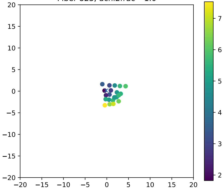
Fiber 823, dchi2frac= 1.0
