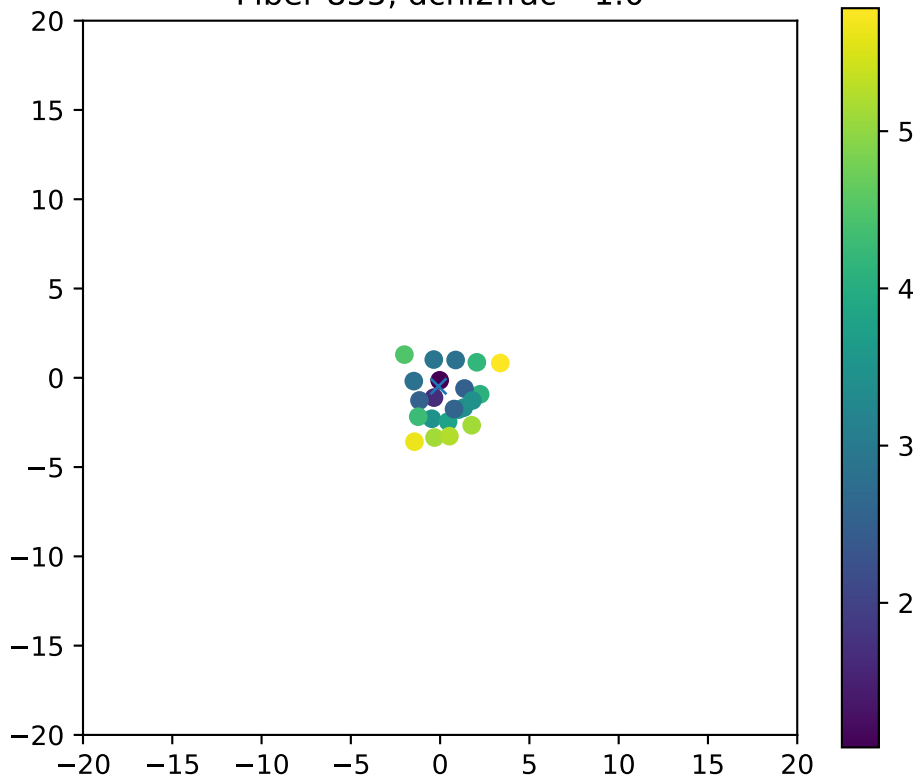
Fiber 855, dchi2frac= 1.0
