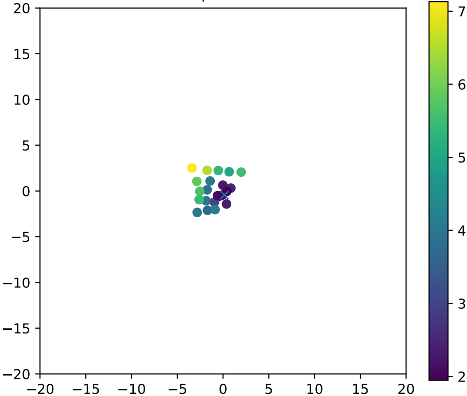
Fiber 3367, dchi2frac= 1.0
