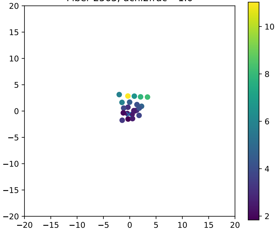
Fiber 2563, dchi2frac= 1.0
