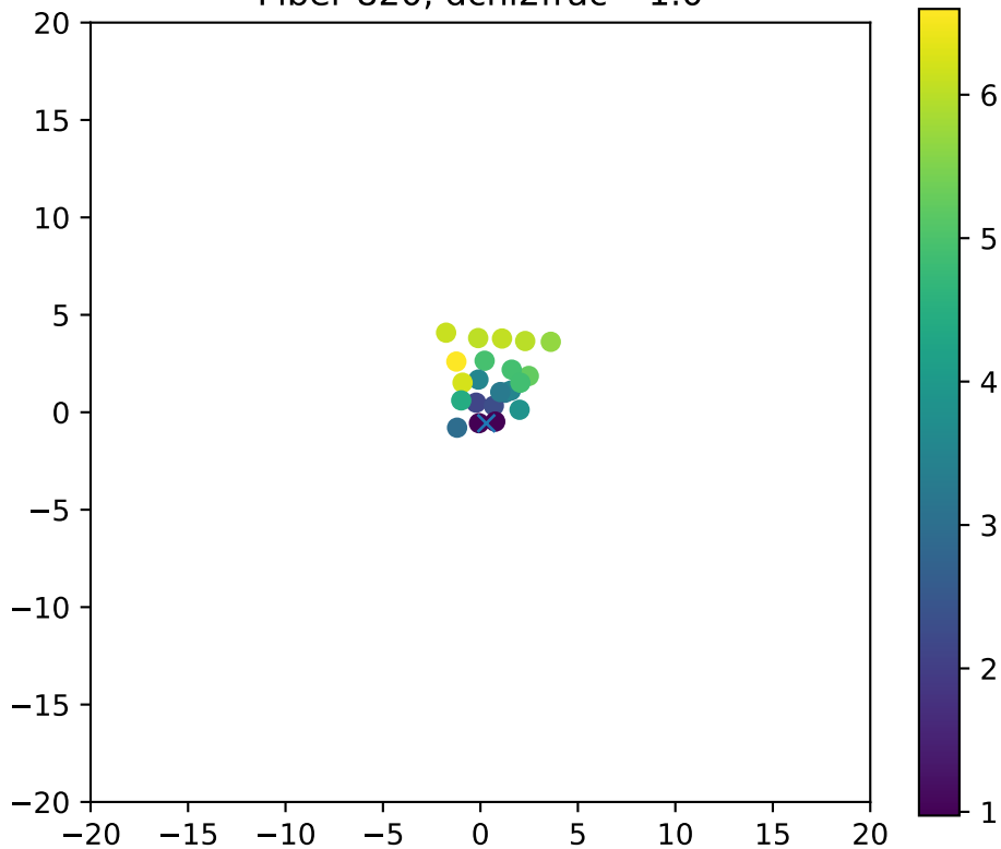
Fiber 820, dchi2frac= 1.0
