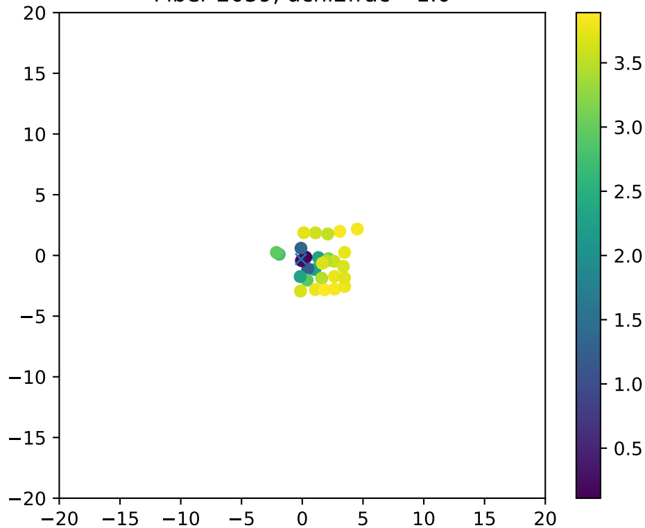
Fiber 2059, dchi2frac= 1.0
