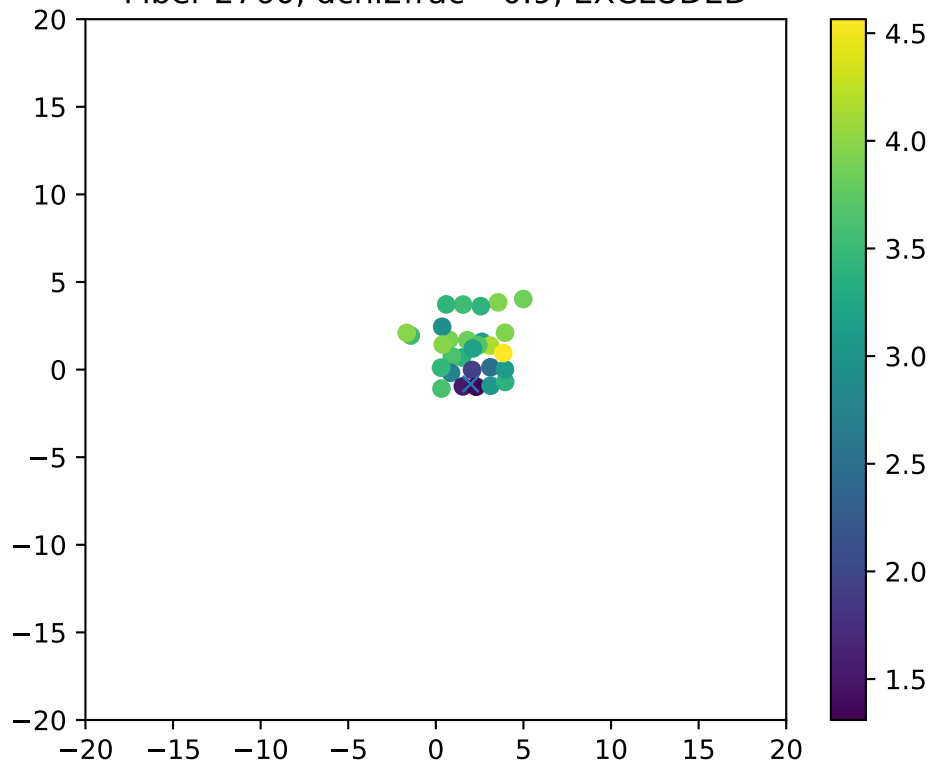
Fiber 2760, dchi2frac= 0.9, EXCLUDED
