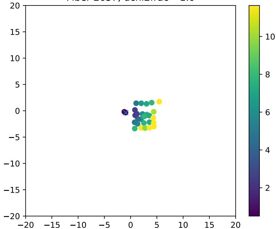
Fiber 2637, dchi2frac= 1.0
