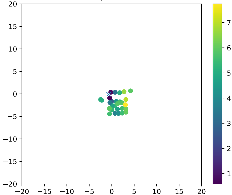
Fiber 2768, dchi2frac= 1.0
