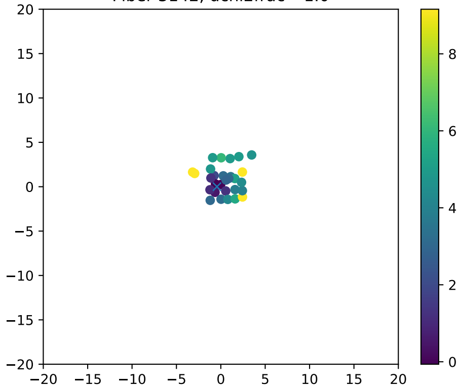
Fiber 3142, dchi2frac= 1.0
