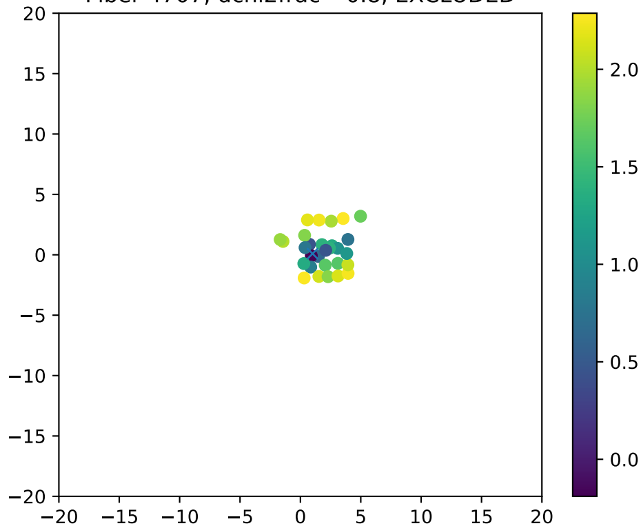
Fiber 4707, dchi2frac= 0.8, EXCLUDED
