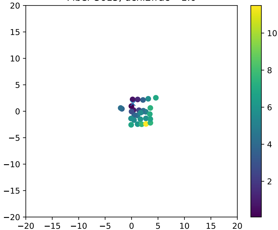
Fiber 3615, dchi2frac= 1.0
