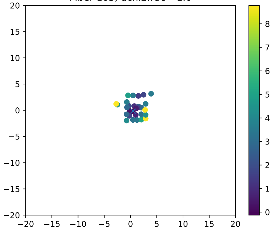
Fiber 103, dchi2frac= 1.0
