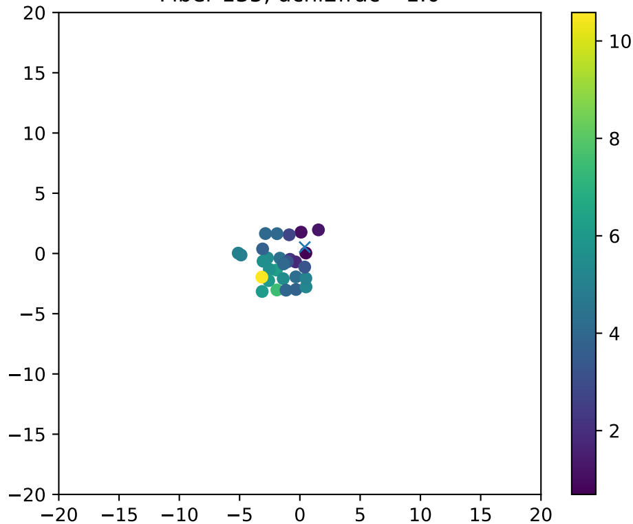
Fiber 135, dchi2frac= 1.0
