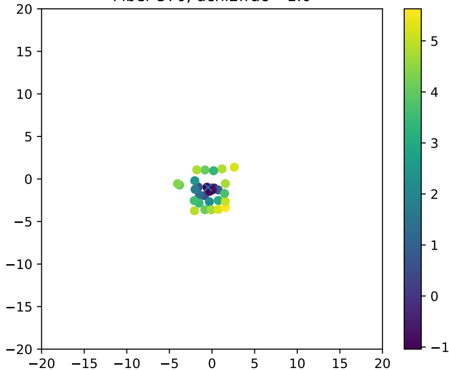
Fiber 570, dchi2frac= 1.0
