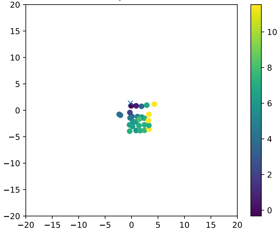
Fiber 3534, dchi2frac= 1.0
