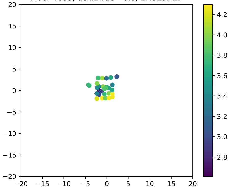
Fiber 4683, dchi2frac= 0.8, EXCLUDED
