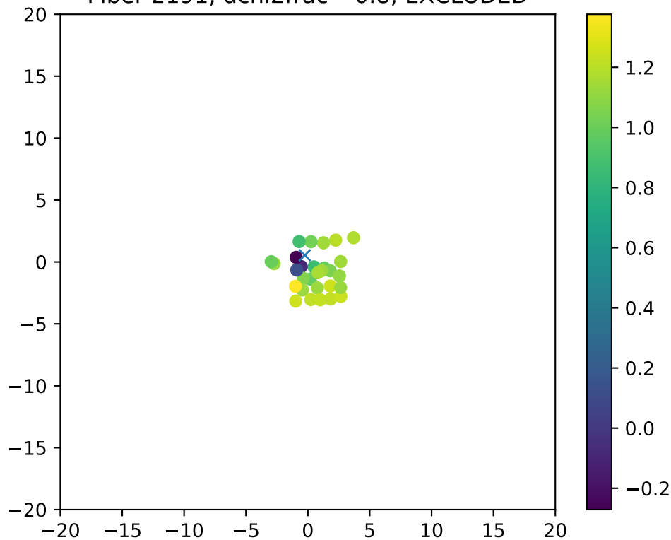
Fiber 2191, dchi2frac= 0.8, EXCLUDED
