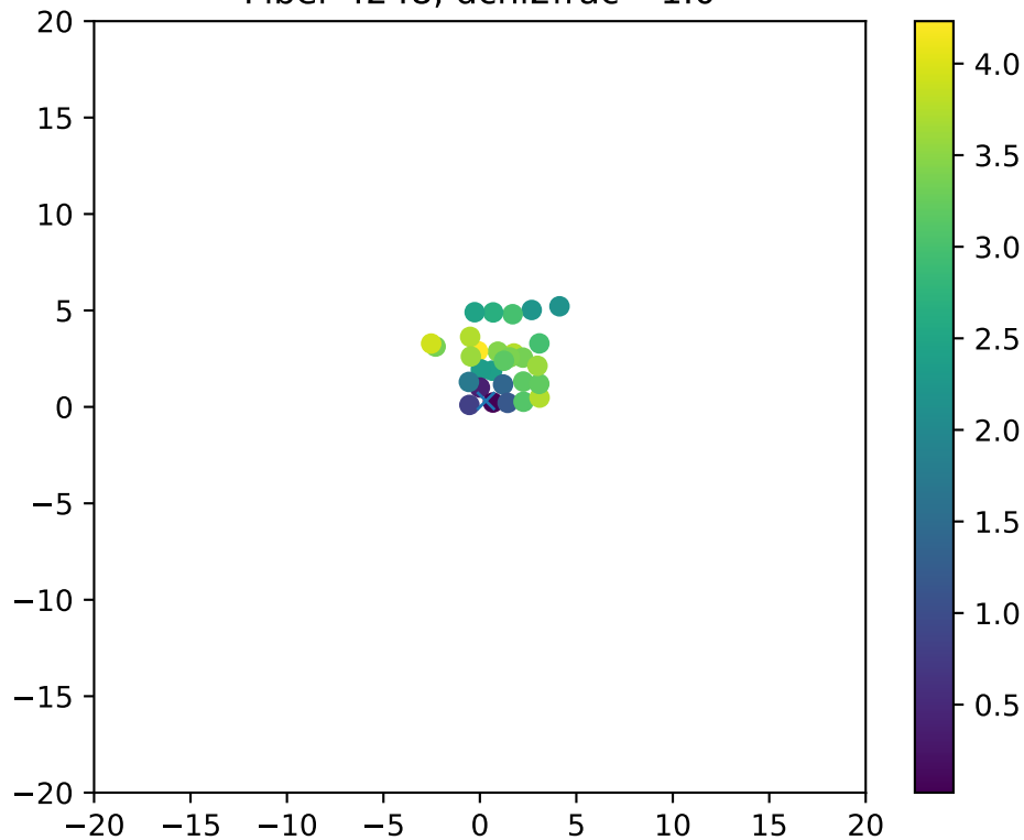
Fiber 4248, dchi2frac= 1.0
