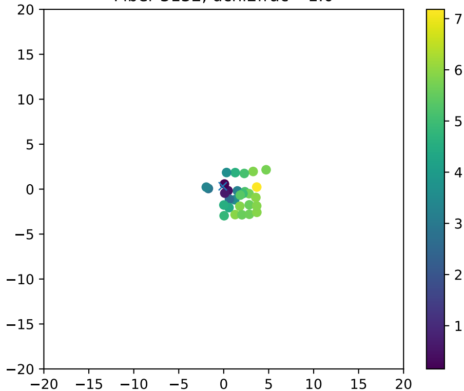
Fiber 3132, dchi2frac= 1.0
