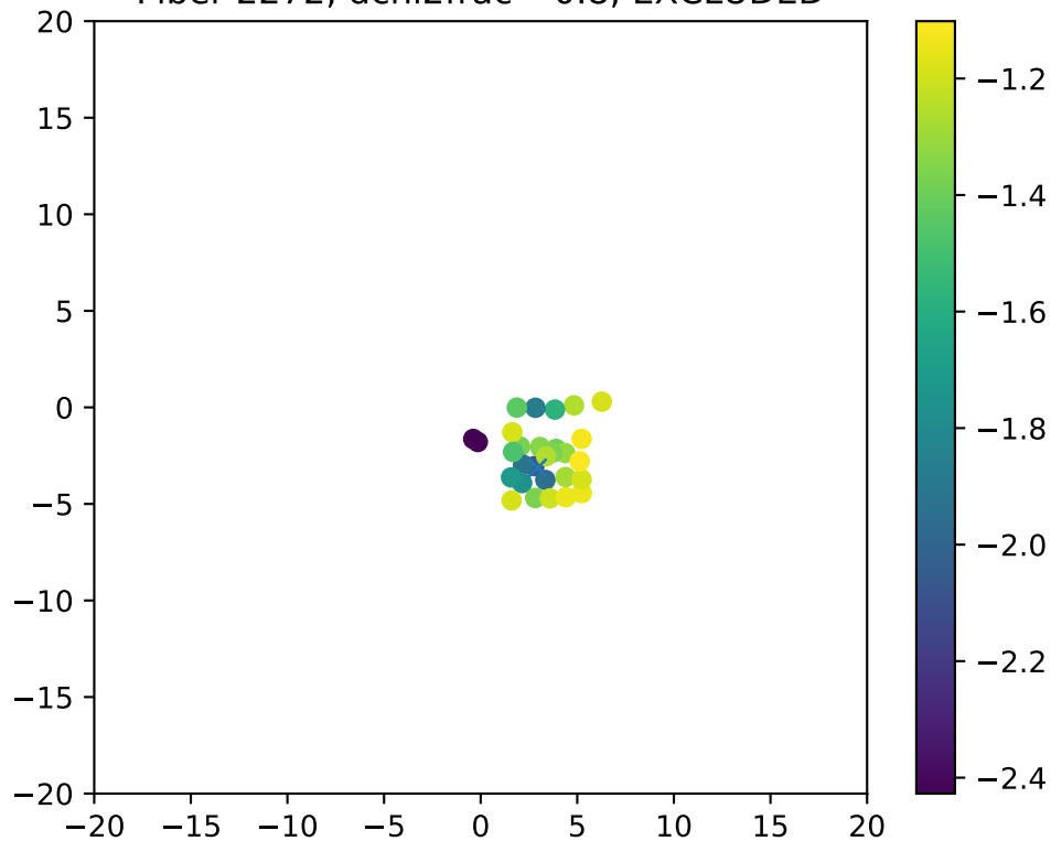
Fiber 2272, dchi2frac= 0.8, EXCLUDED
