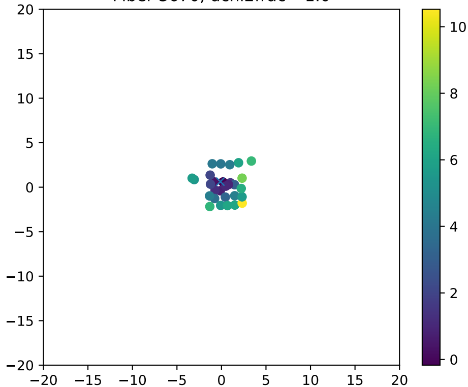
Fiber 3670, dchi2frac= 1.0
