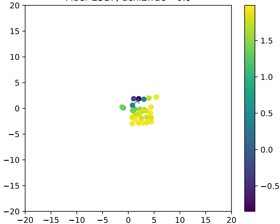
Fiber 2317, dchi2frac= 0.9
