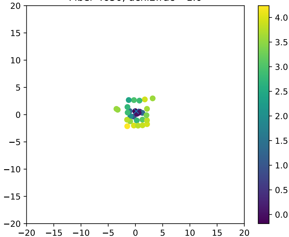
Fiber 4650, dchi2frac= 1.0
