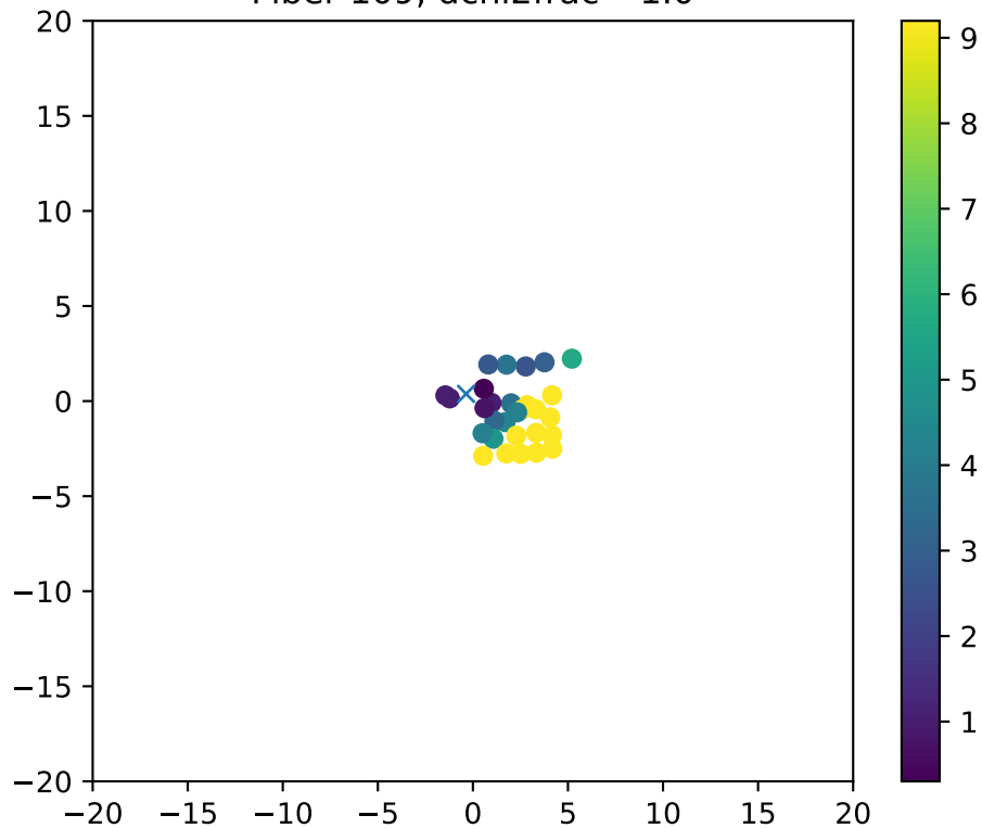
Fiber 109, dchi2frac= 1.0
