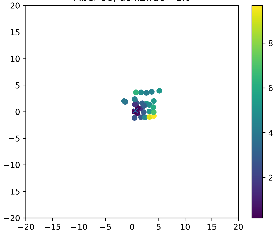
Fiber 88, dchi2frac= 1.0
