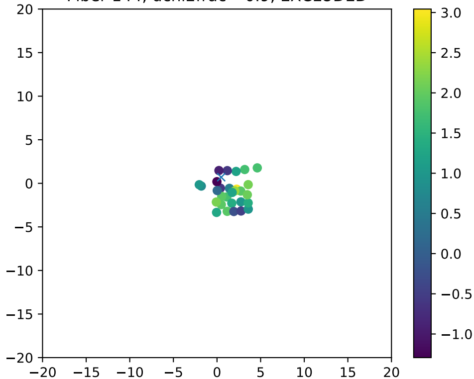
Fiber 144, dchi2frac= 0.9, EXCLUDED
