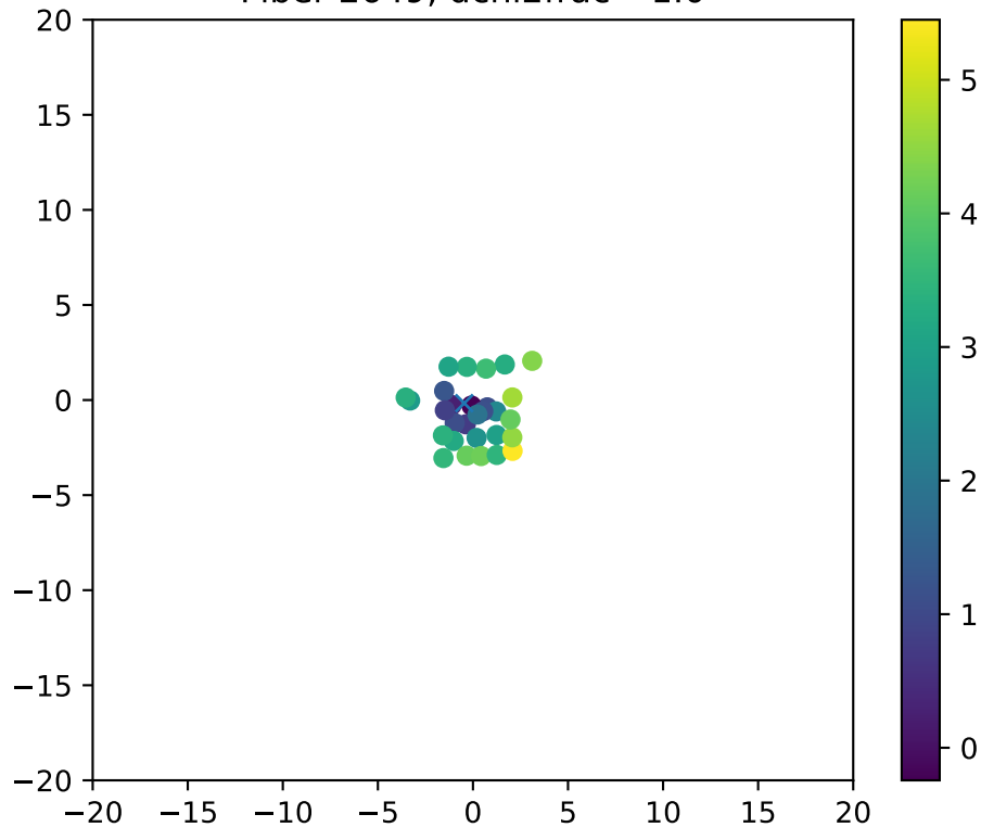
Fiber 2649, dchi2frac= 1.0
