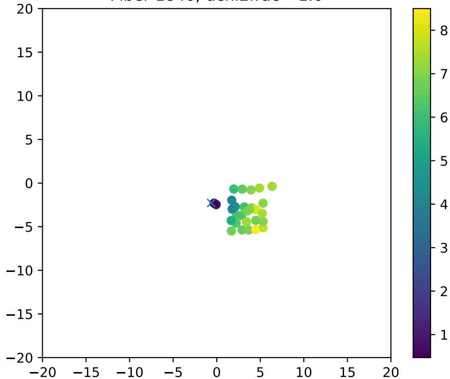
Fiber 1840, dchi2frac= 1.0
