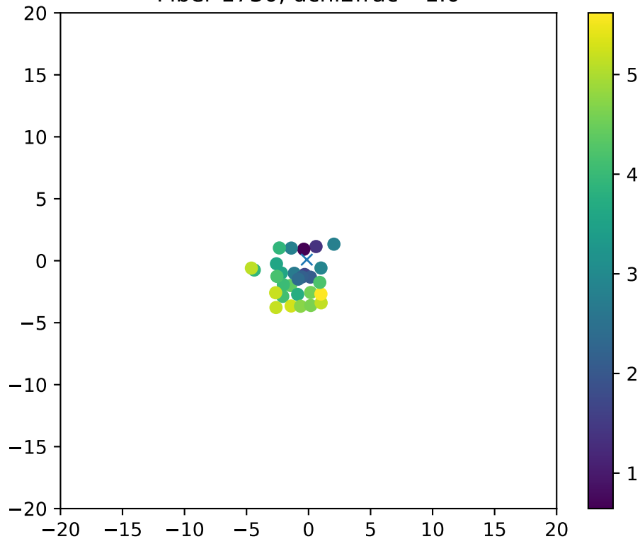
Fiber 1730, dchi2frac= 1.0
