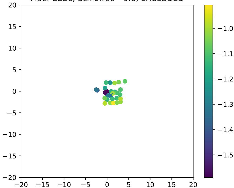
Fiber 2226, dchi2frac= 0.8, EXCLUDED
