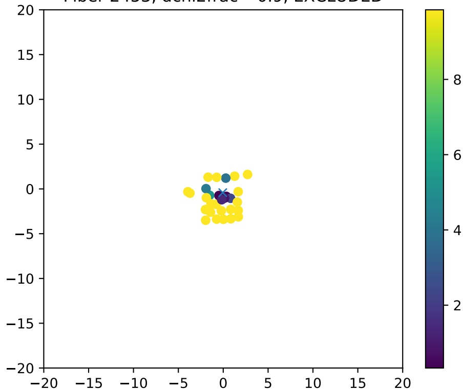
Fiber 2453, dchi2frac= 0.9, EXCLUDED
