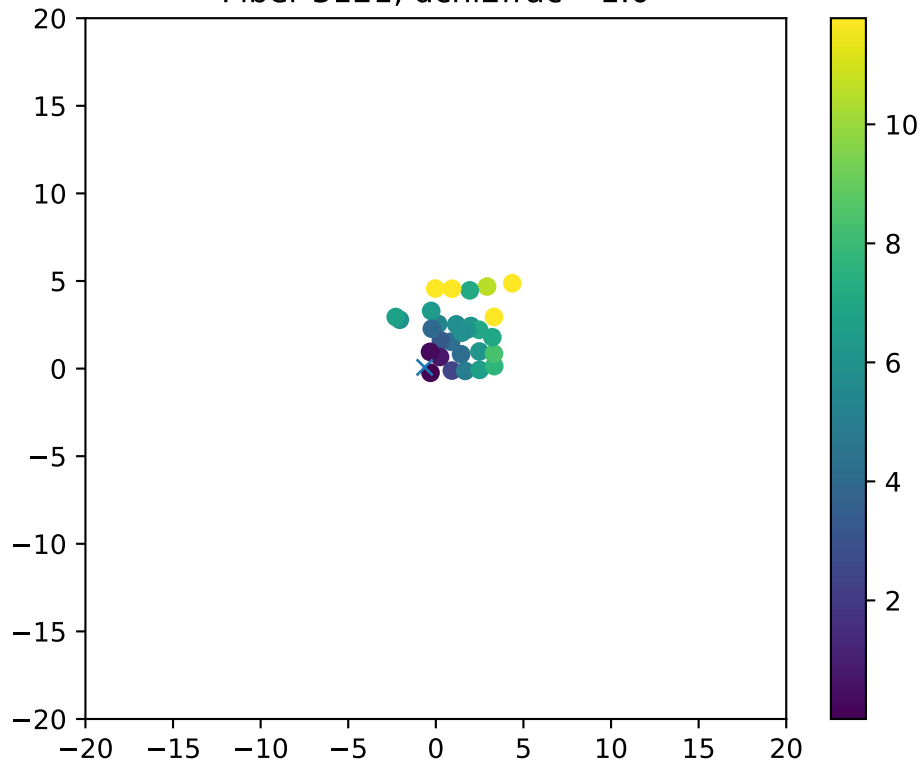
Fiber 3121, dchi2frac= 1.0
