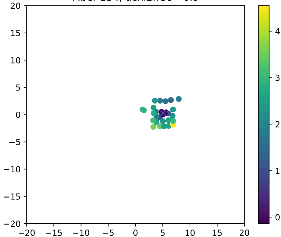
Fiber 234, dchi2frac= 0.9
