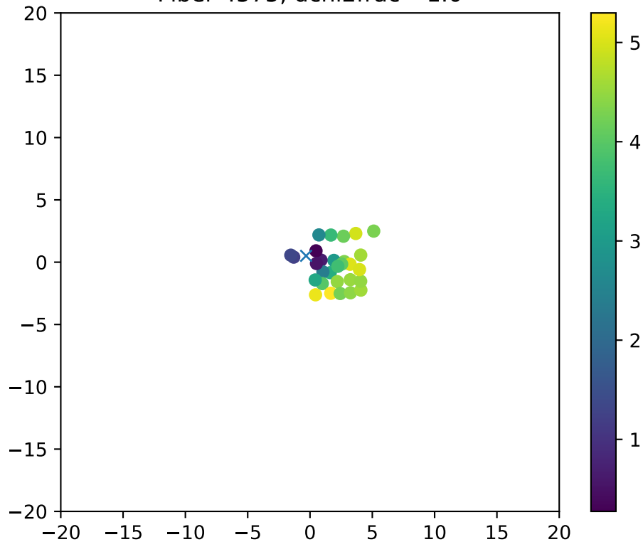
Fiber 4575, dchi2frac= 1.0
