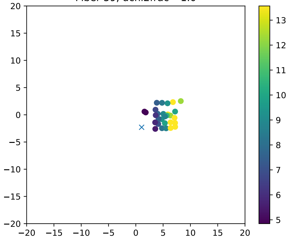
Fiber 59, dchi2frac= 1.0
