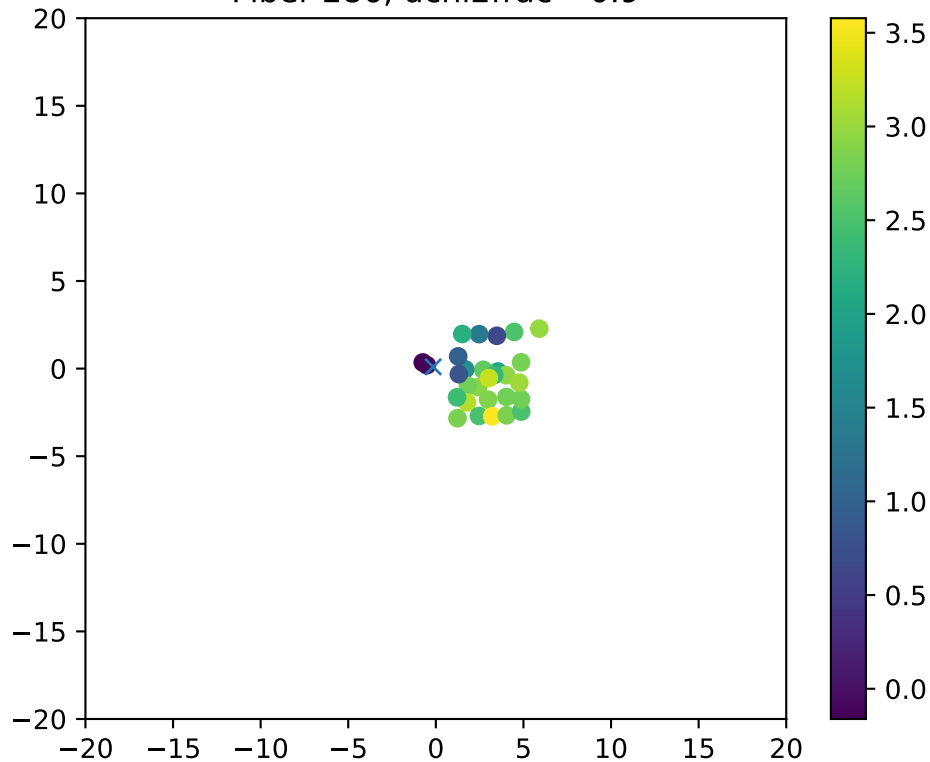
Fiber 286, dchi2frac= 0.9
