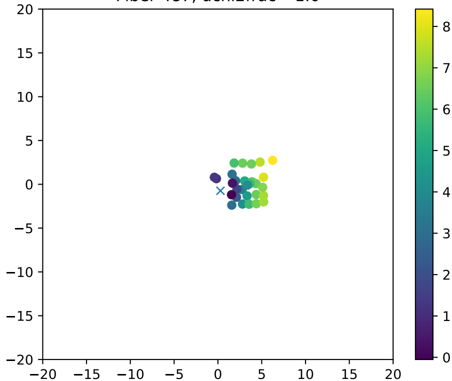
Fiber 487, dchi2frac= 1.0
