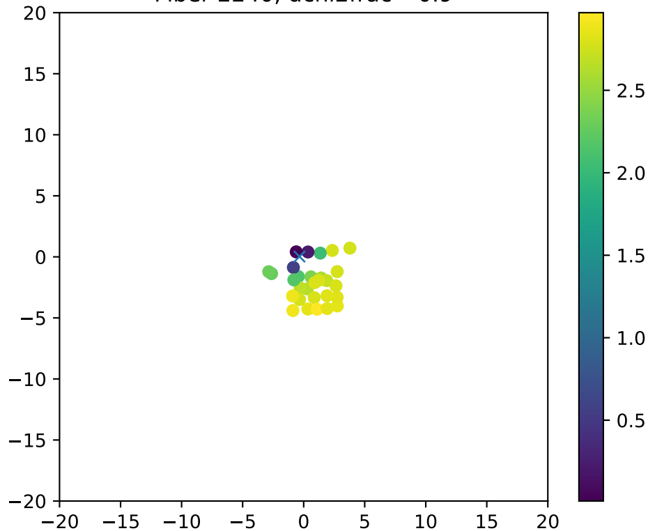
Fiber 2240, dchi2frac= 0.9
