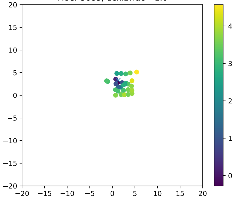
Fiber 3683, dchi2frac= 1.0
