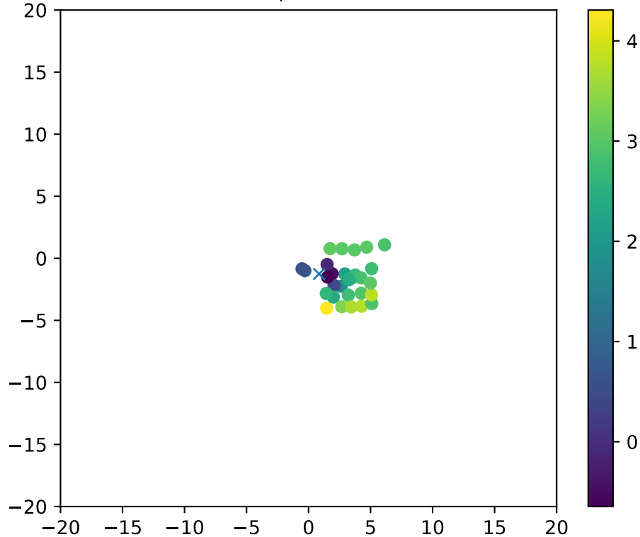
Fiber 3806, dchi2frac= 1.0
