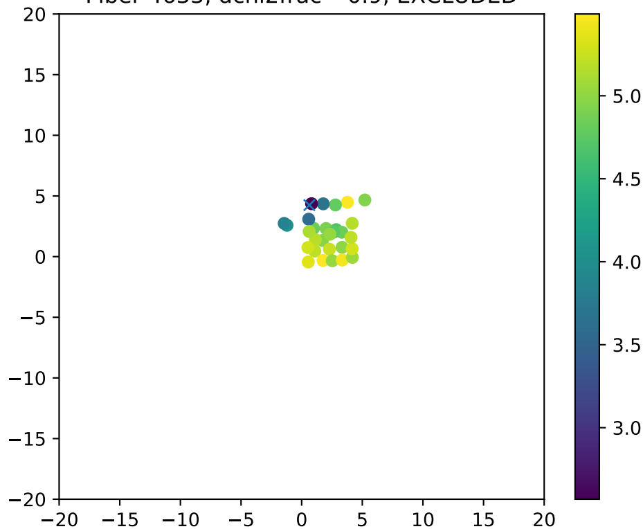
Fiber 4633, dchi2frac= 0.9, EXCLUDED
