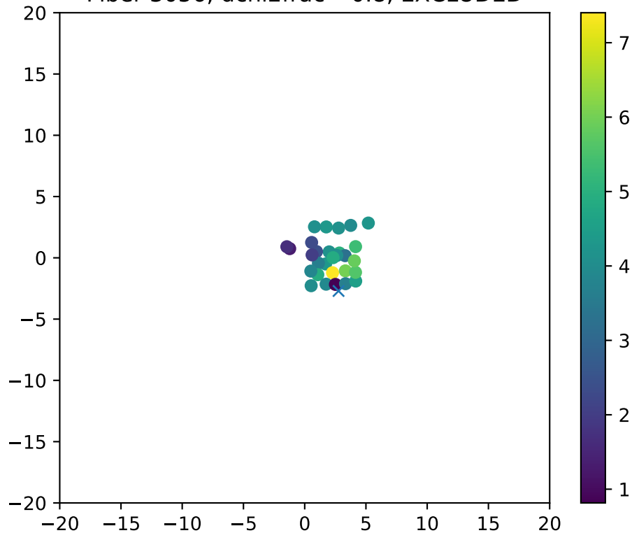
Fiber 3056, dchi2frac= 0.8, EXCLUDED
