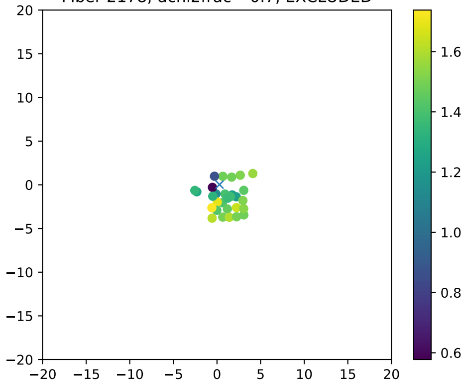
Fiber 2178, dchi2frac= 0.7, EXCLUDED
