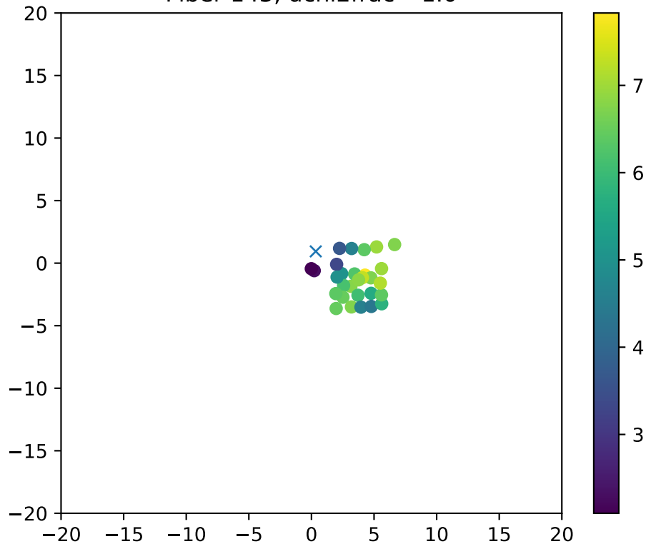
Fiber 143, dchi2frac= 1.0
