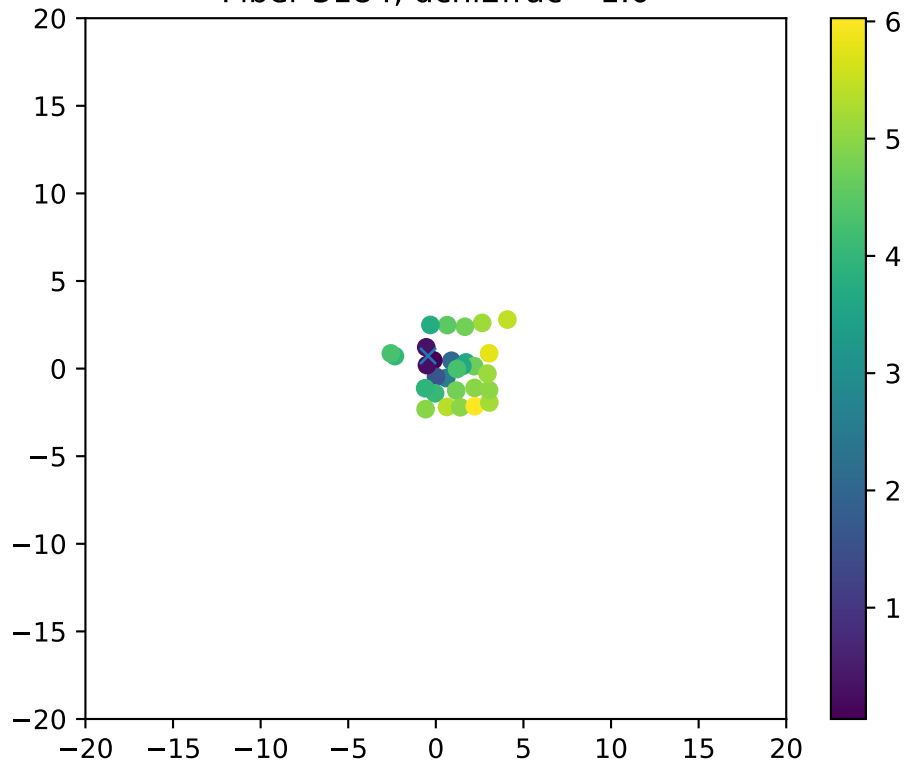
Fiber 3184, dchi2frac= 1.0
