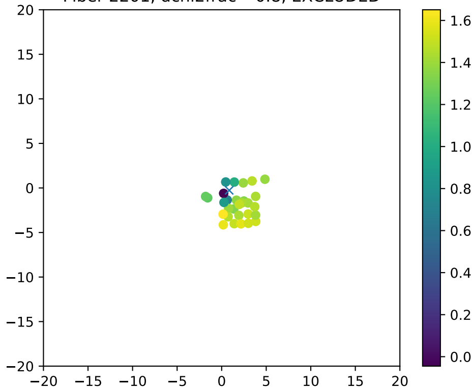
Fiber 2201, dchi2frac= 0.8, EXCLUDED
