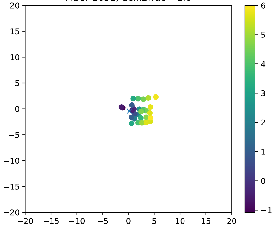
Fiber 2652, dchi2frac= 1.0
