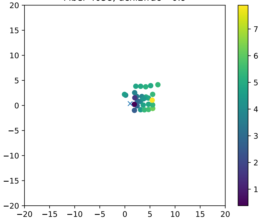
Fiber 4058, dchi2frac= 0.9
