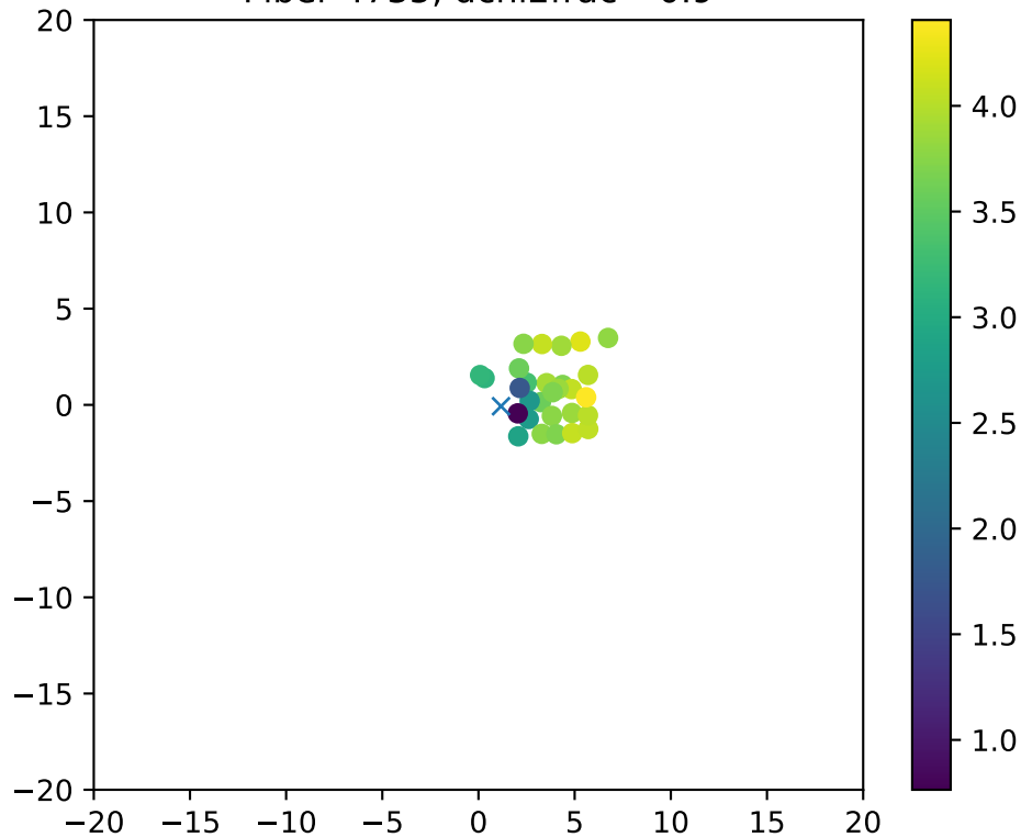
Fiber 4735, dchi2frac= 0.9
