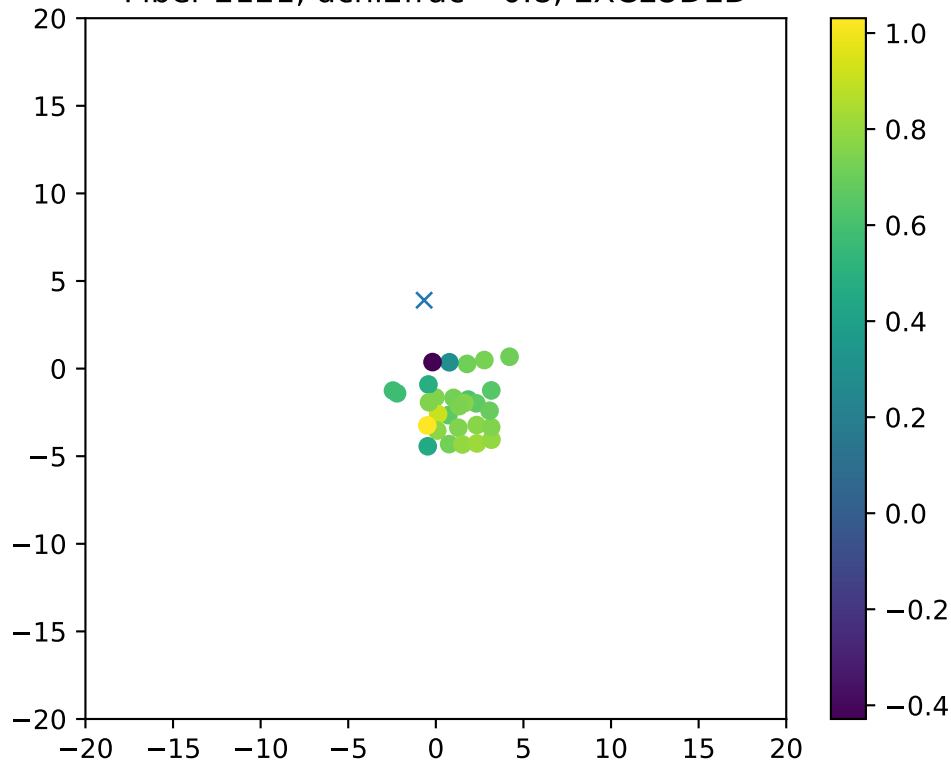
Fiber 2121, dchi2frac= 0.8, EXCLUDED
