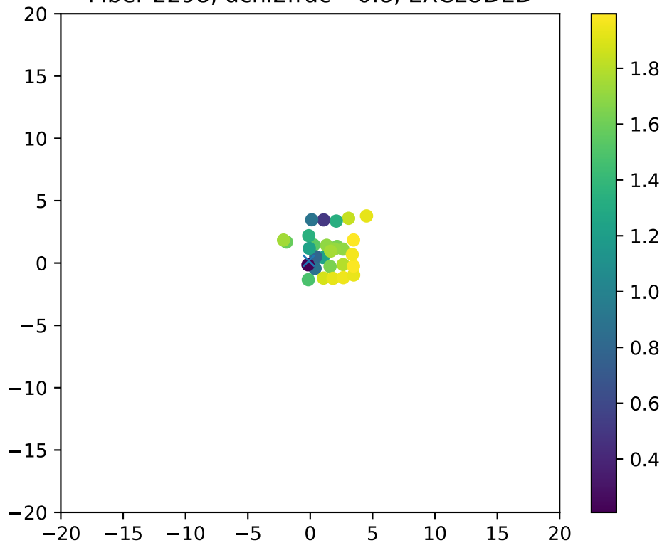
Fiber 2298, dchi2frac= 0.8, EXCLUDED
