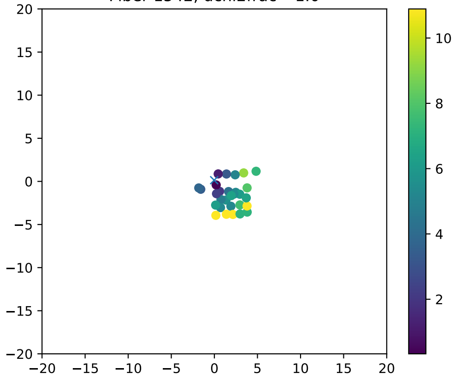
Fiber 1542, dchi2frac= 1.0
