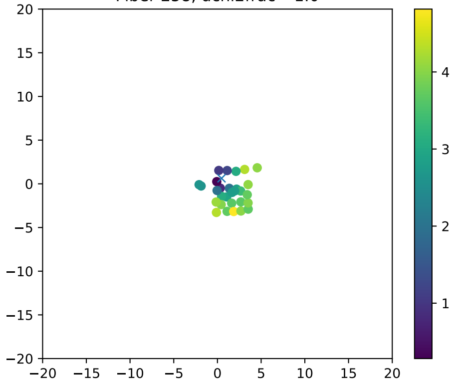
Fiber 258, dchi2frac= 1.0
