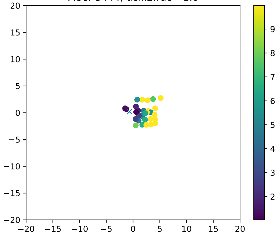
Fiber 3444, dchi2frac= 1.0
