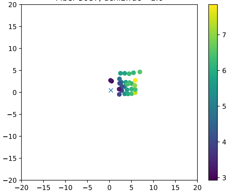
Fiber 3087, dchi2frac= 1.0
