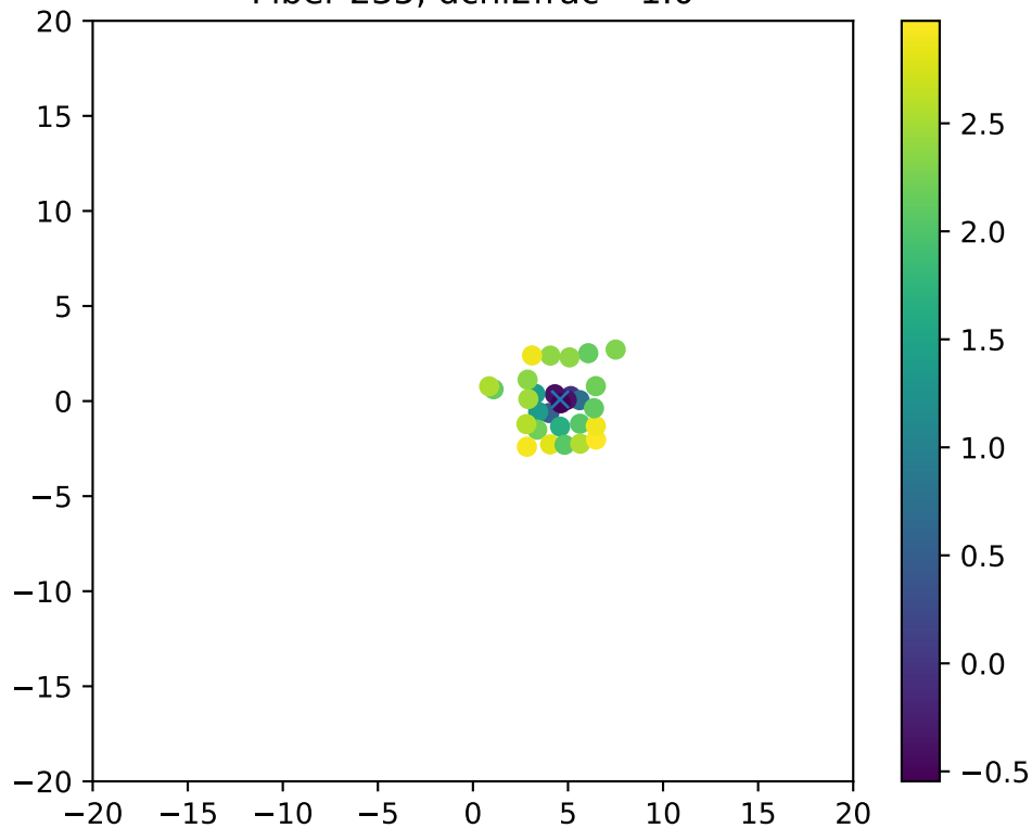
Fiber 235, dchi2frac= 1.0
