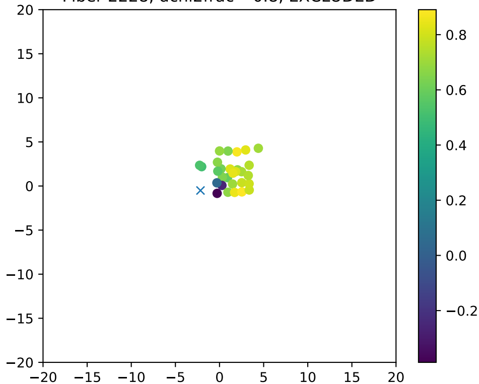
Fiber 2228, dchi2frac= 0.8, EXCLUDED
