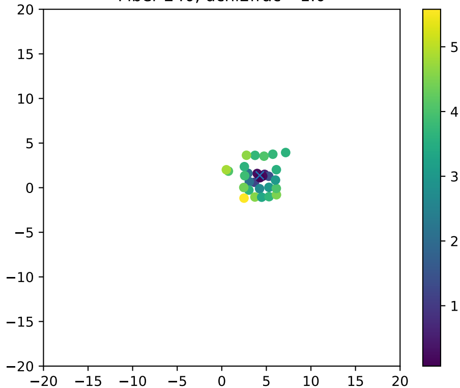
Fiber 240, dchi2frac= 1.0
