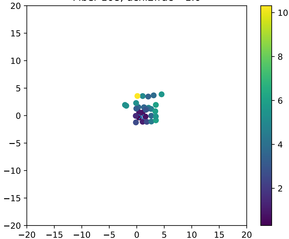
Fiber 108, dchi2frac= 1.0
