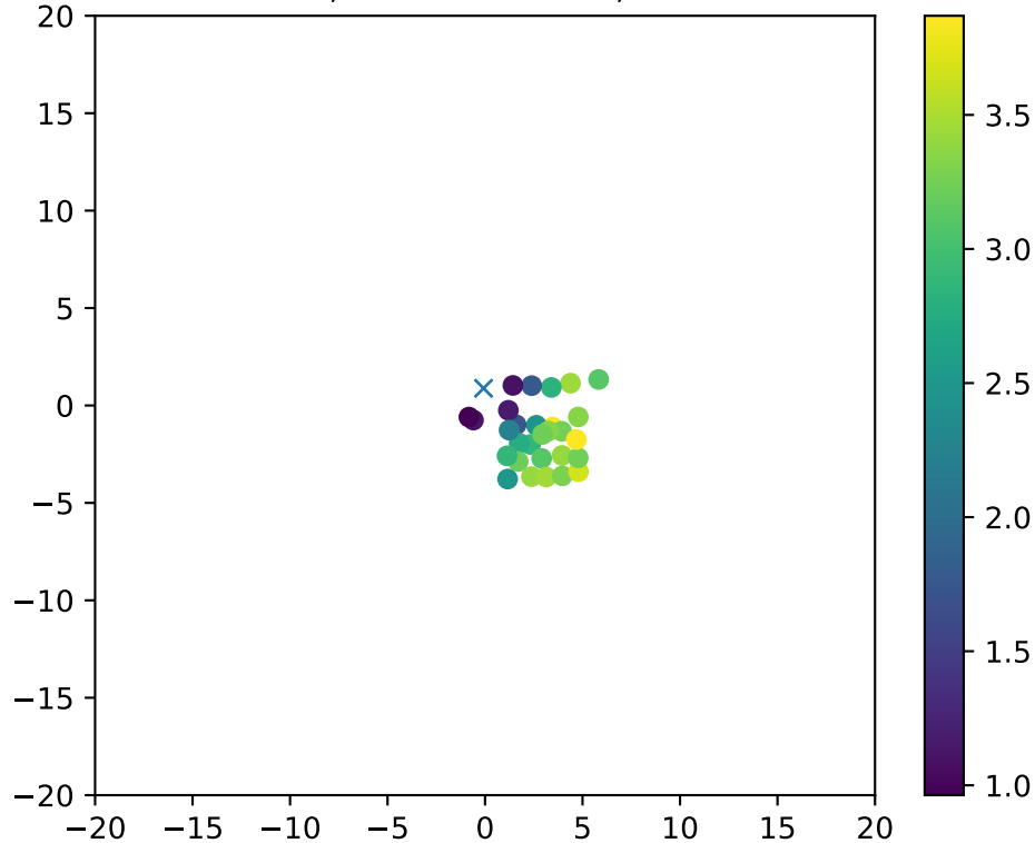
Fiber 4200, dchi2frac= 0.9, EXCLUDED
