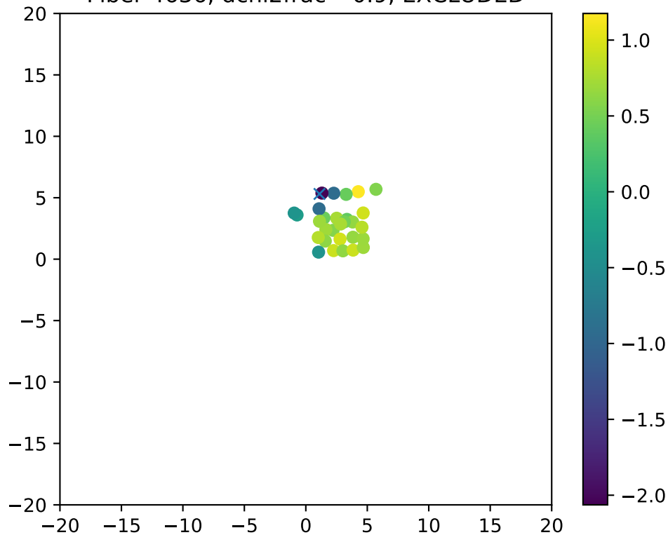
Fiber 4636, dchi2frac= 0.9, EXCLUDED
