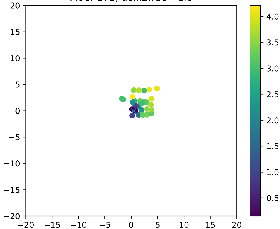
Fiber 272, dchi2frac= 1.0
