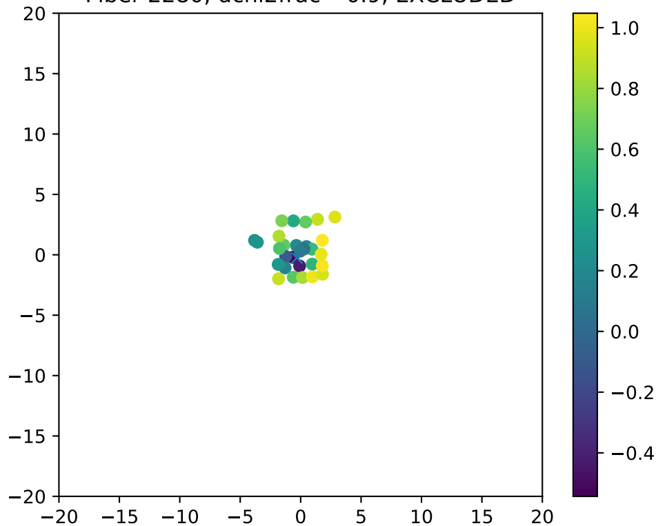
Fiber 2280, dchi2frac= 0.9, EXCLUDED
