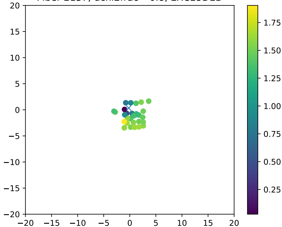
Fiber 2137, dchi2frac= 0.8, EXCLUDED
