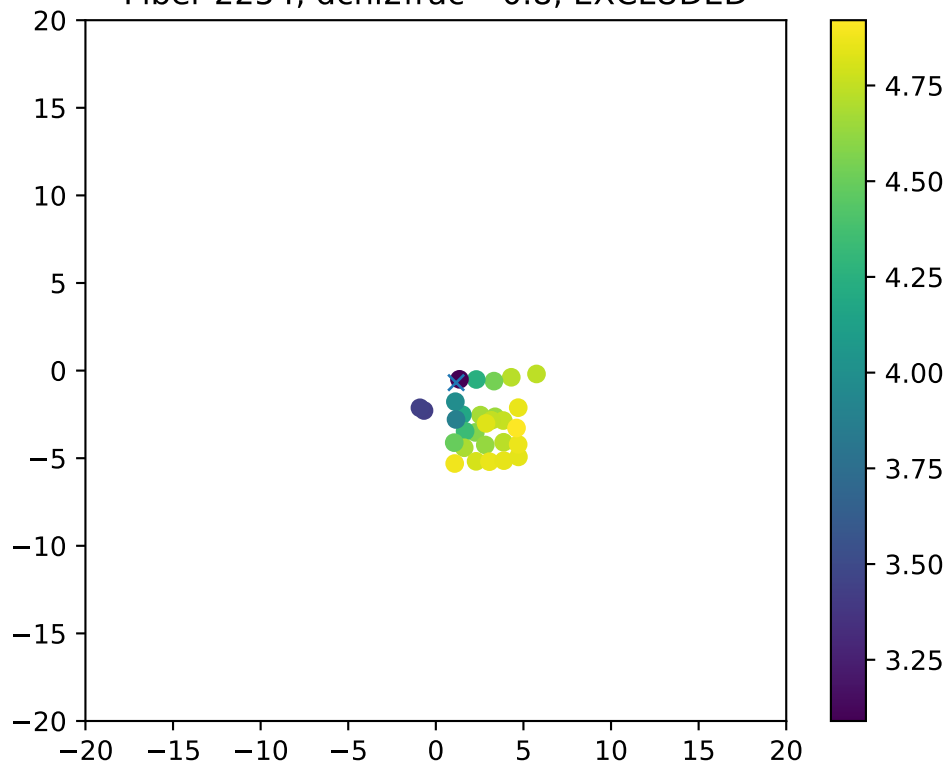
Fiber 2254, dchi2frac= 0.8, EXCLUDED
