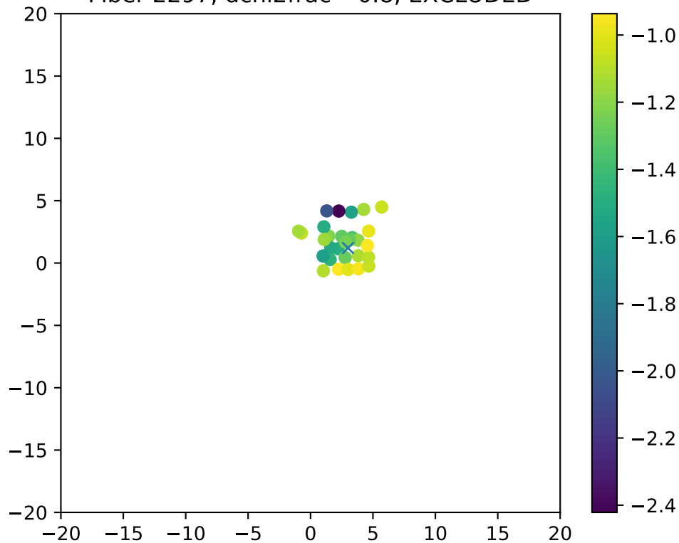
Fiber 2297, dchi2frac= 0.8, EXCLUDED
