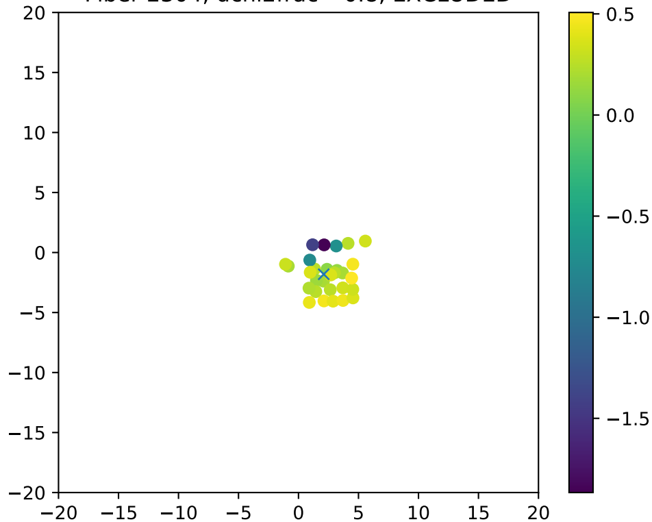
Fiber 2304, dchi2frac= 0.8, EXCLUDED
