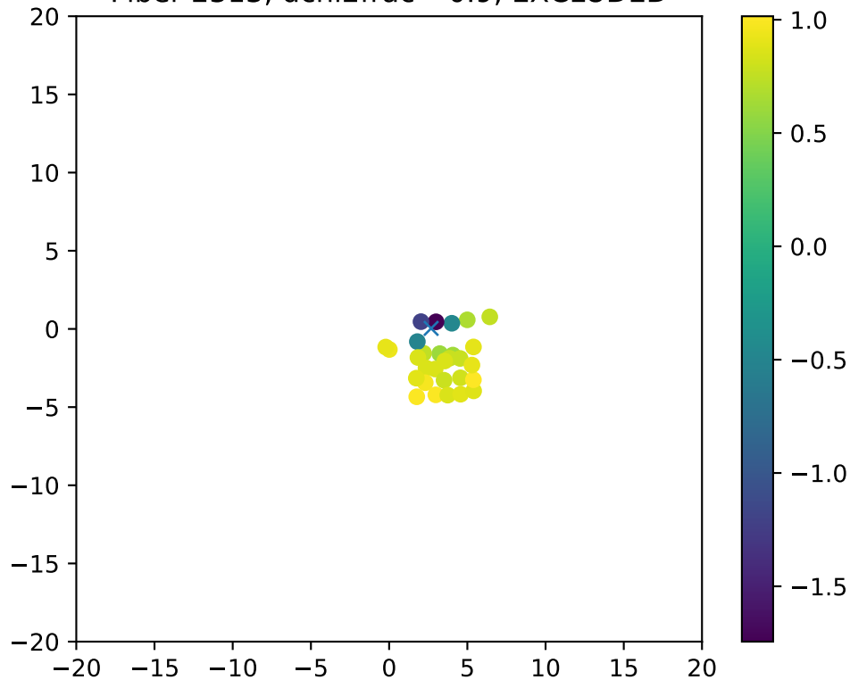
Fiber 2313, dchi2frac= 0.9, EXCLUDED
