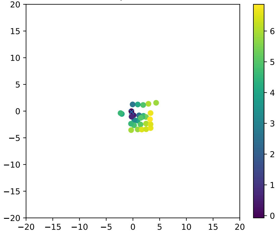
Fiber 1726, dchi2frac= 1.0
