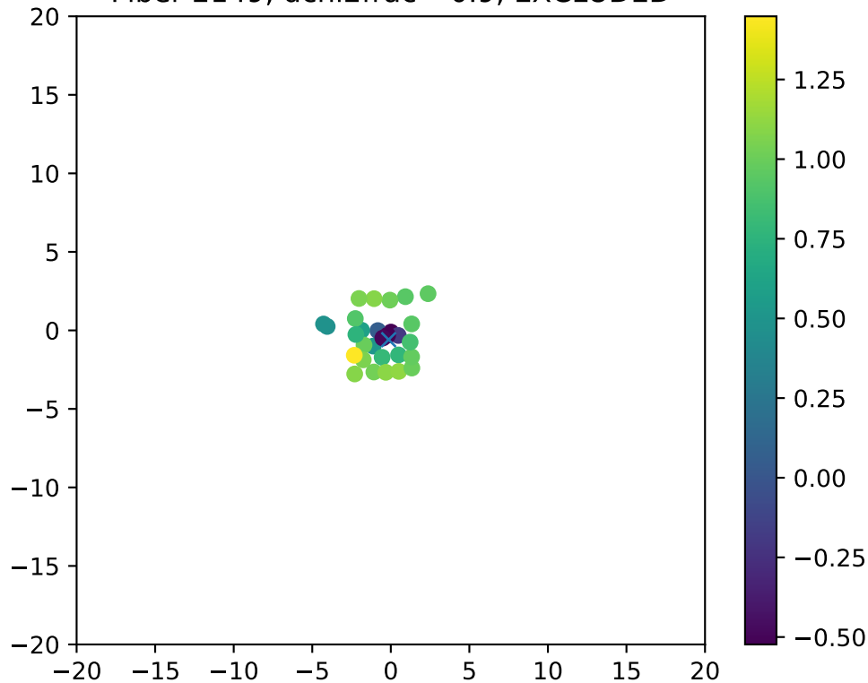
Fiber 2149, dchi2frac= 0.9, EXCLUDED
