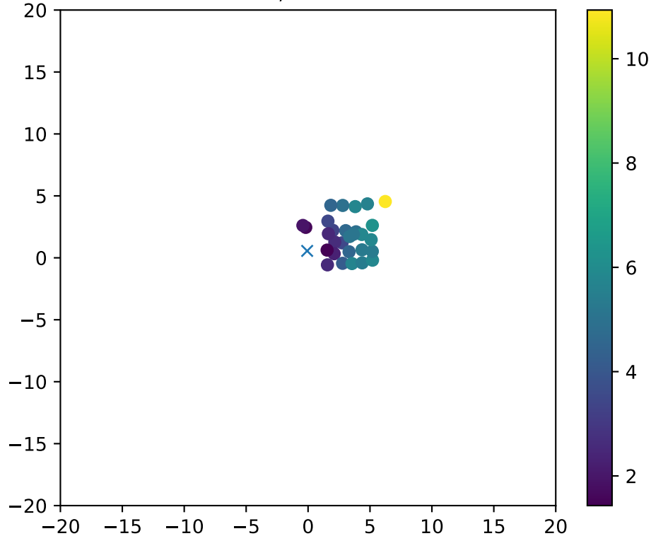
Fiber 3092, dchi2frac= 1.0
