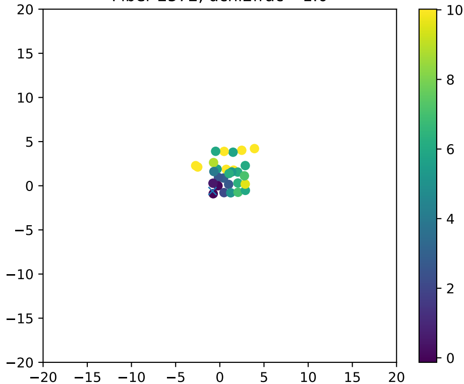
Fiber 2572, dchi2frac= 1.0
