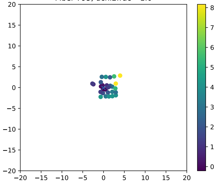
Fiber 795, dchi2frac= 1.0
