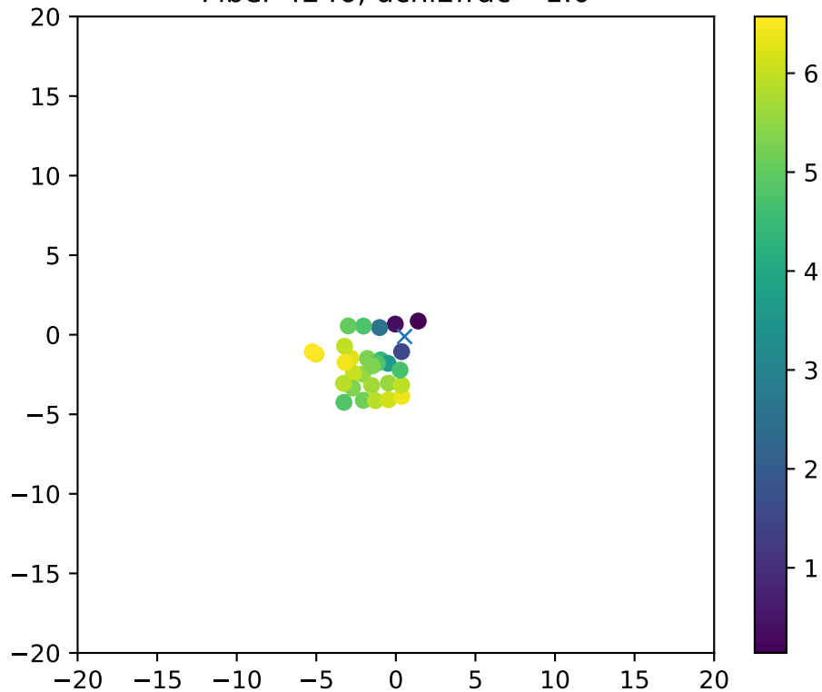
Fiber 4246, dchi2frac= 1.0
