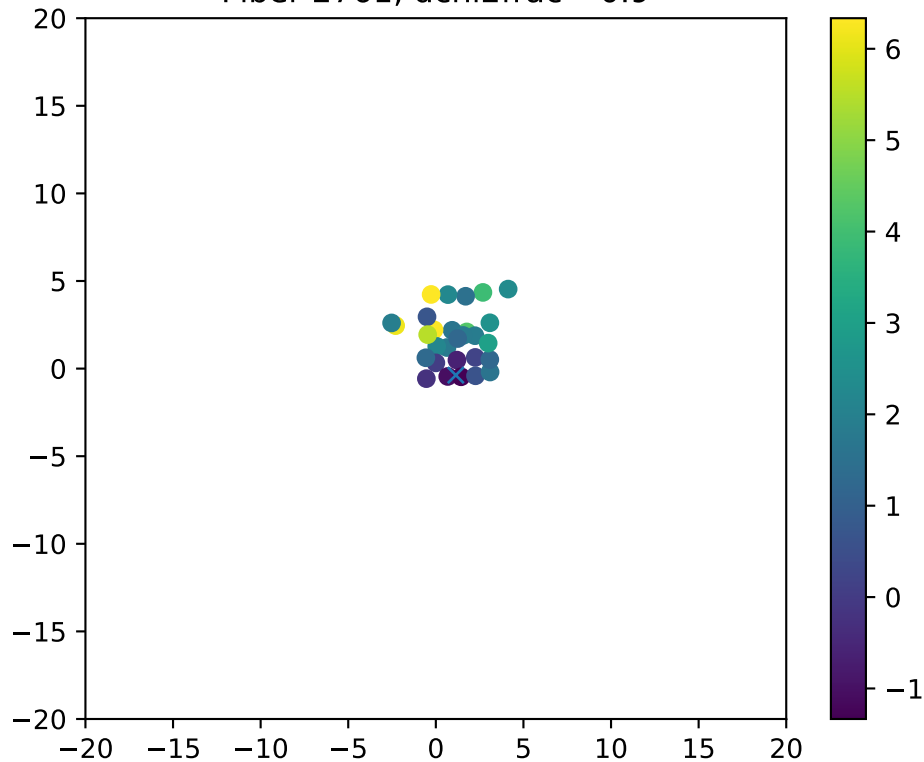
Fiber 2761, dchi2frac= 0.9
