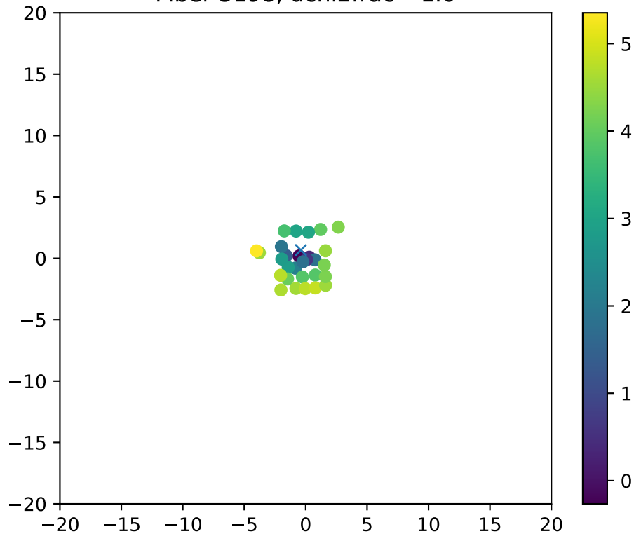
Fiber 3198, dchi2frac= 1.0
