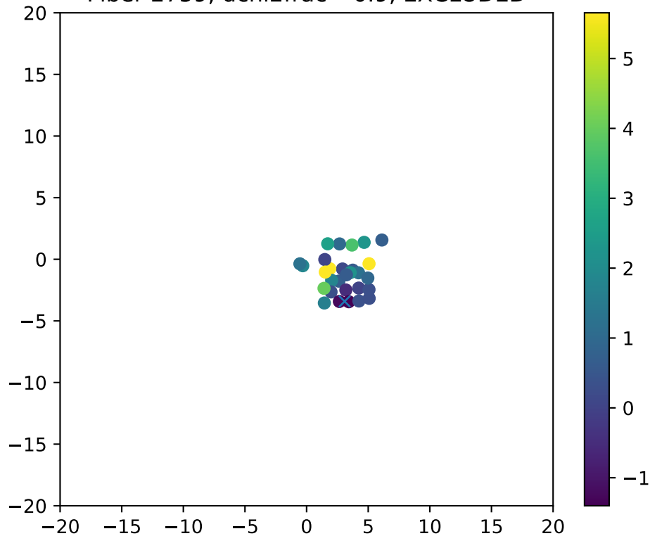
Fiber 2759, dchi2frac= 0.9, EXCLUDED
