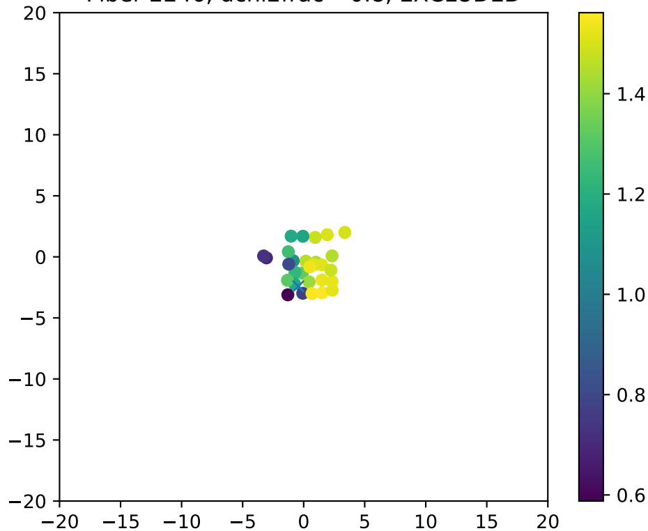
Fiber 2246, dchi2frac= 0.8, EXCLUDED
