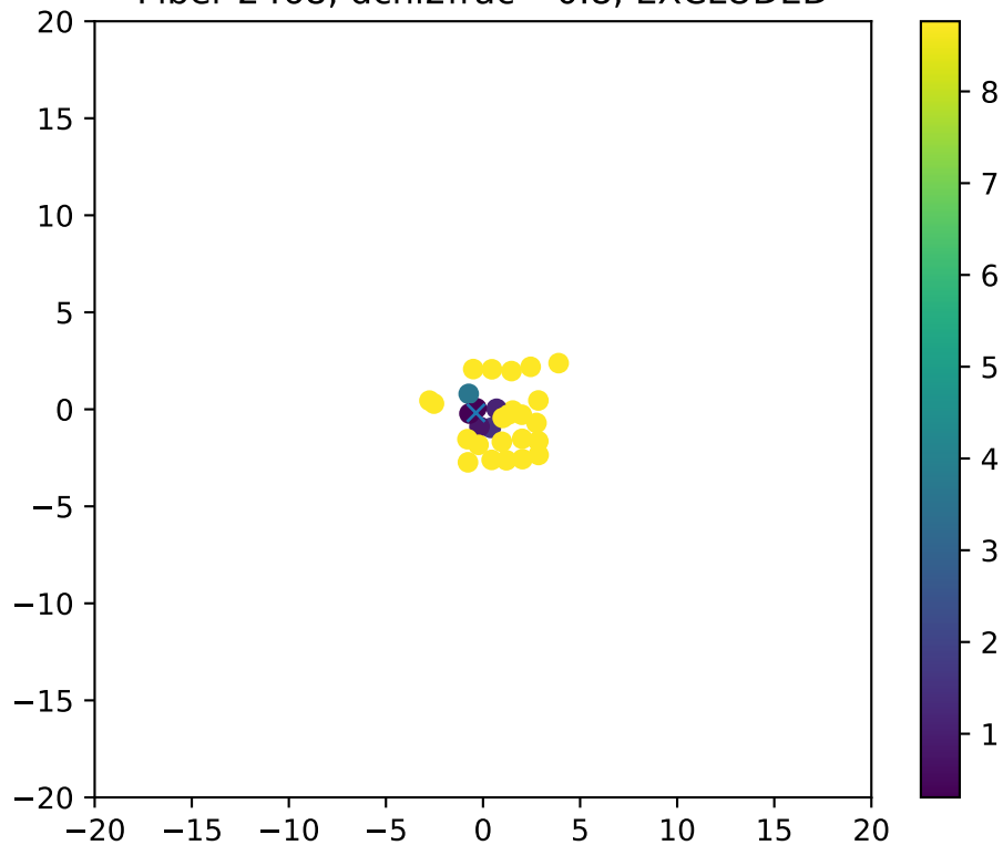
Fiber 2468, dchi2frac= 0.8, EXCLUDED
