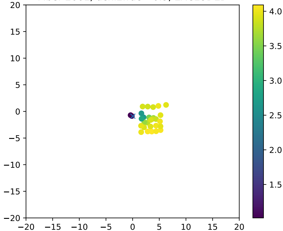
Fiber 2061, dchi2frac= 0.9, EXCLUDED
