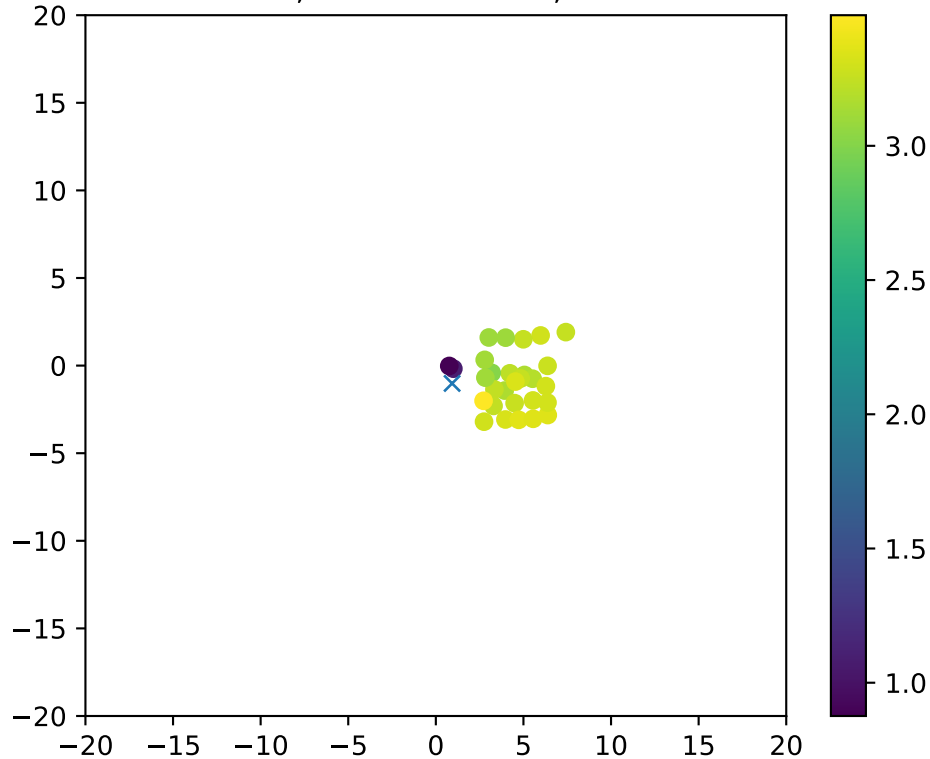
Fiber 2216, dchi2frac= 0.8, EXCLUDED
