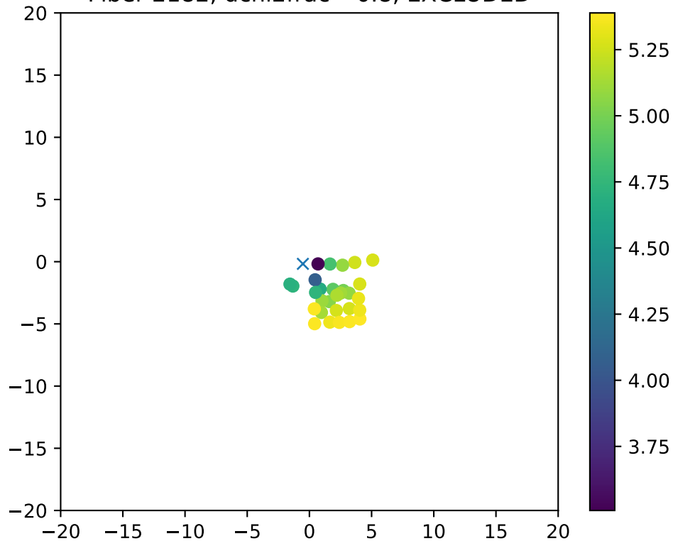
Fiber 2182, dchi2frac= 0.8, EXCLUDED
