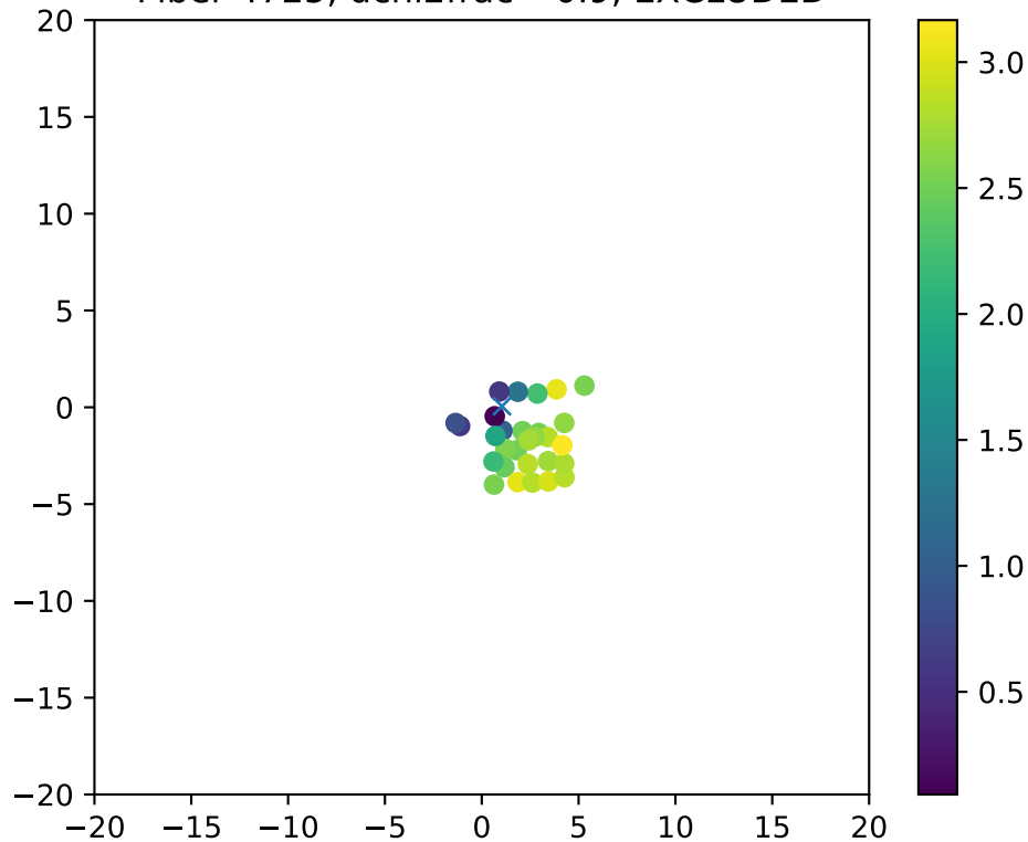
Fiber 4725, dchi2frac= 0.9, EXCLUDED
