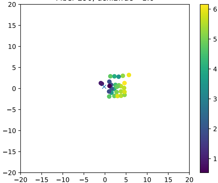
Fiber 290, dchi2frac= 1.0
