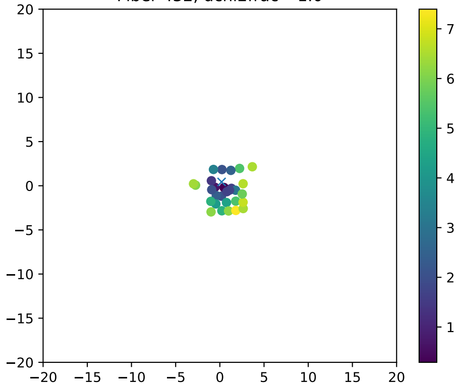
Fiber 432, dchi2frac= 1.0
