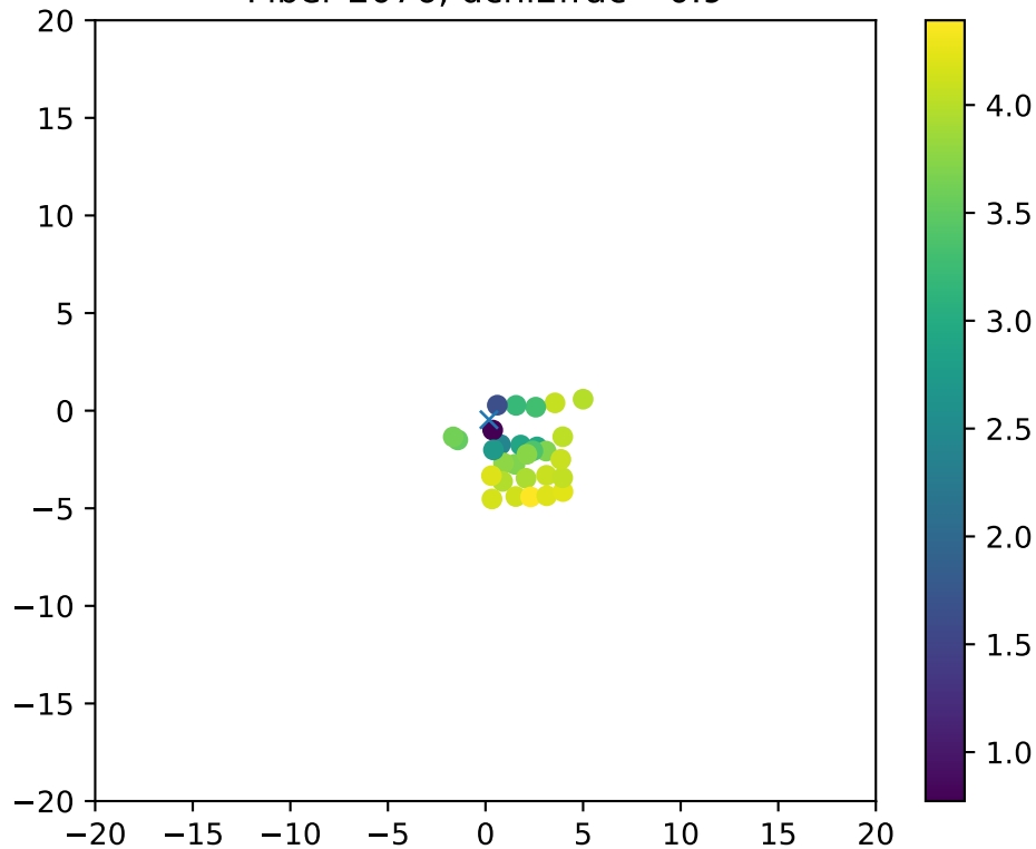
Fiber 2076, dchi2frac= 0.9
