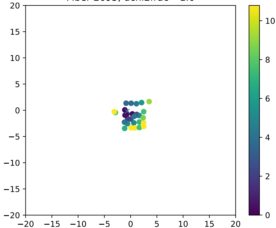
Fiber 2695, dchi2frac= 1.0
