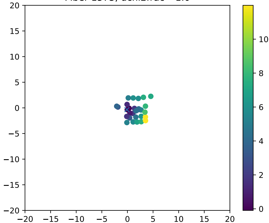
Fiber 1573, dchi2frac= 1.0
