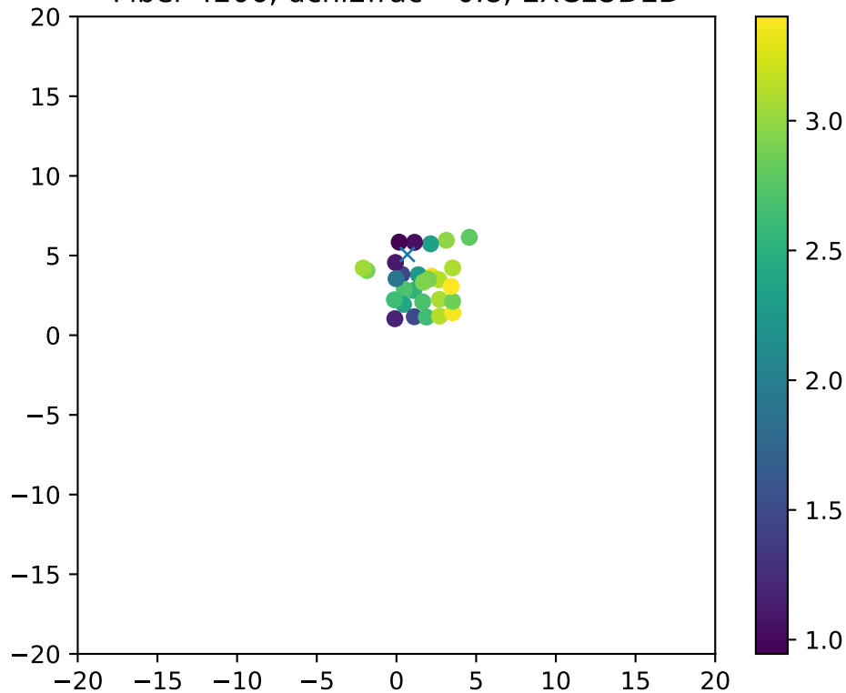
Fiber 4206, dchi2frac= 0.8, EXCLUDED
