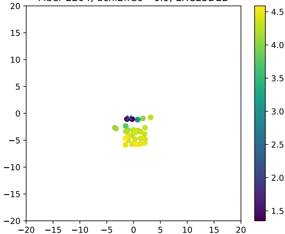
Fiber 2204, dchi2frac= 0.9, EXCLUDED
