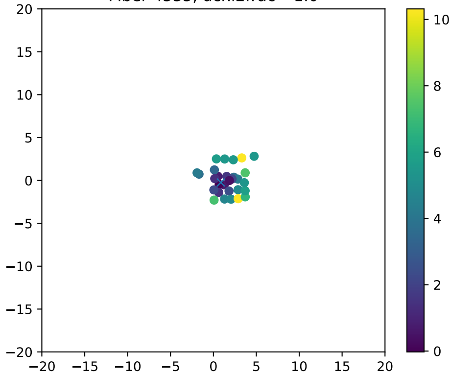
Fiber 4535, dchi2frac= 1.0
