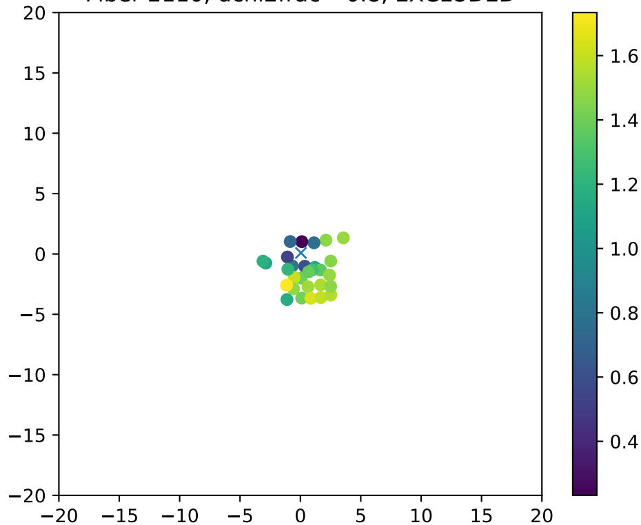
Fiber 2110, dchi2frac= 0.8, EXCLUDED
