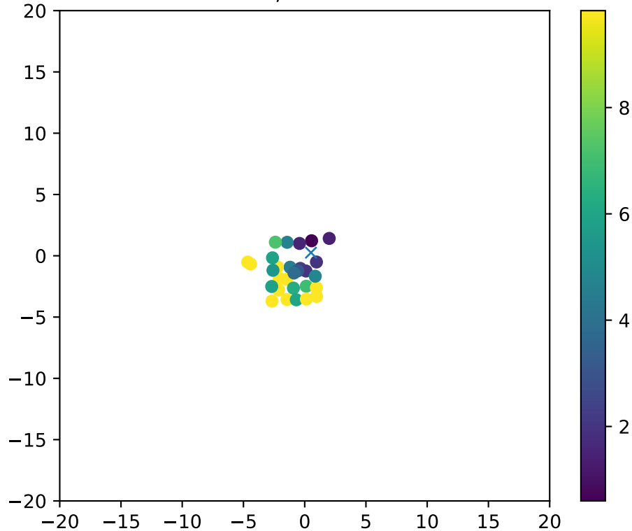
Fiber 3406, dchi2frac= 1.0
