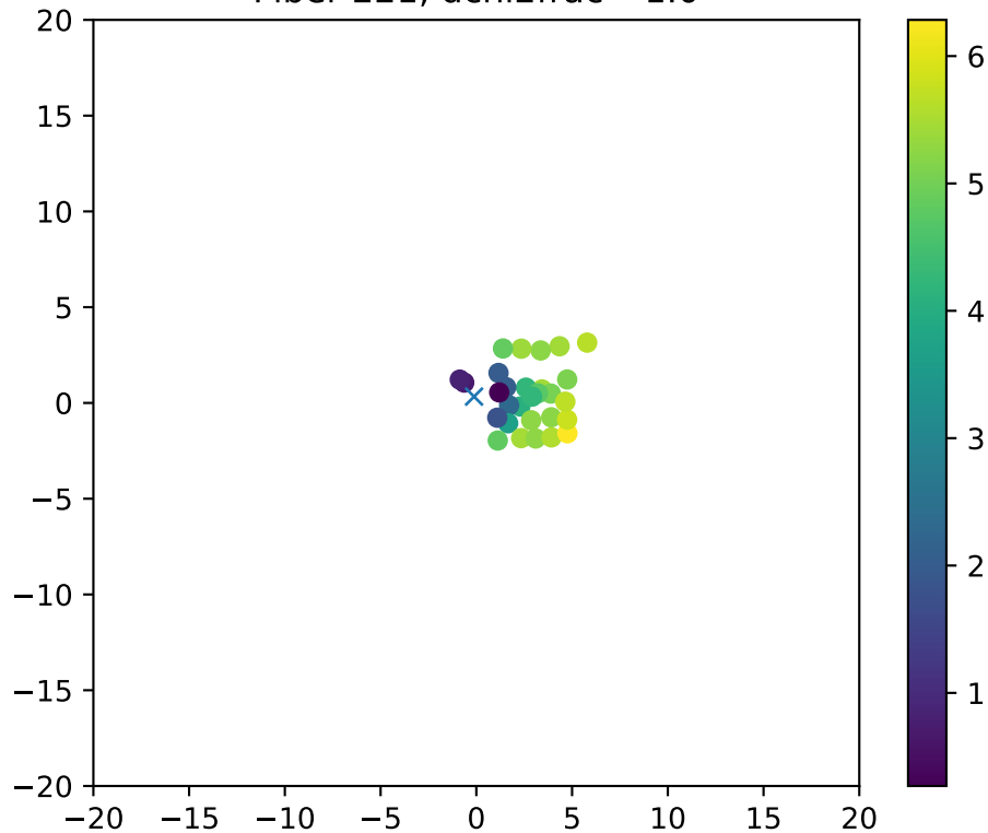
Fiber 221, dchi2frac= 1.0
