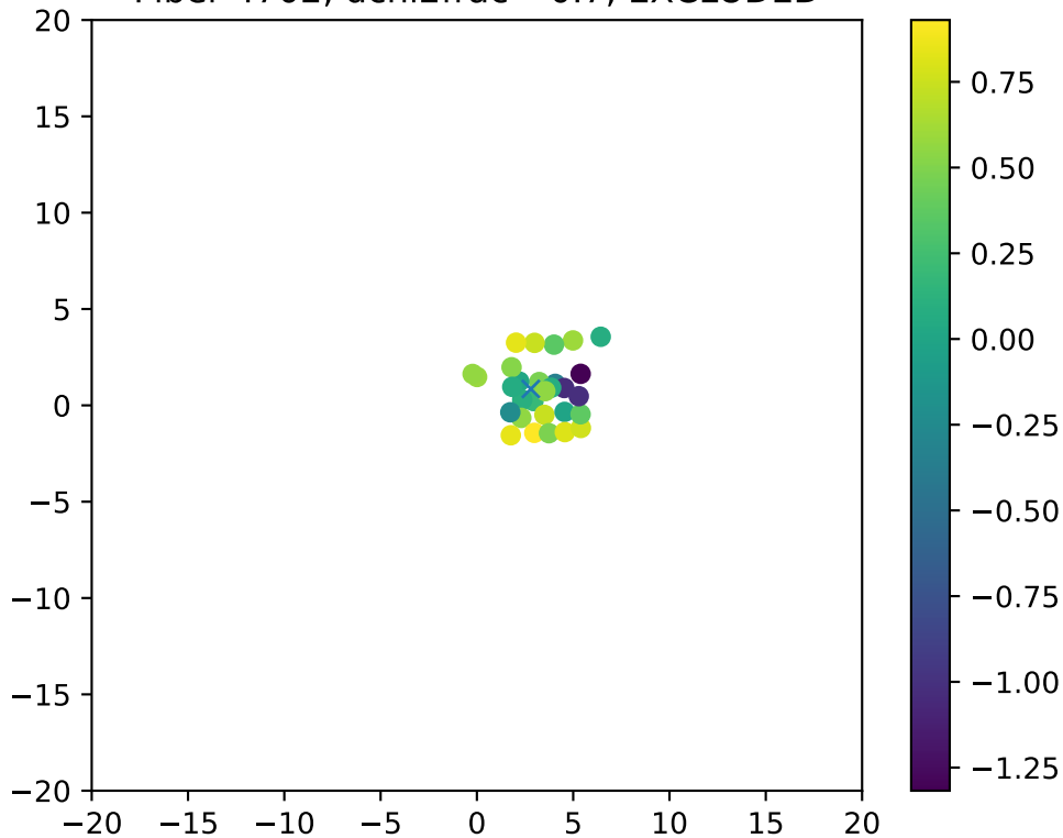
Fiber 4702, dchi2frac= 0.7, EXCLUDED
