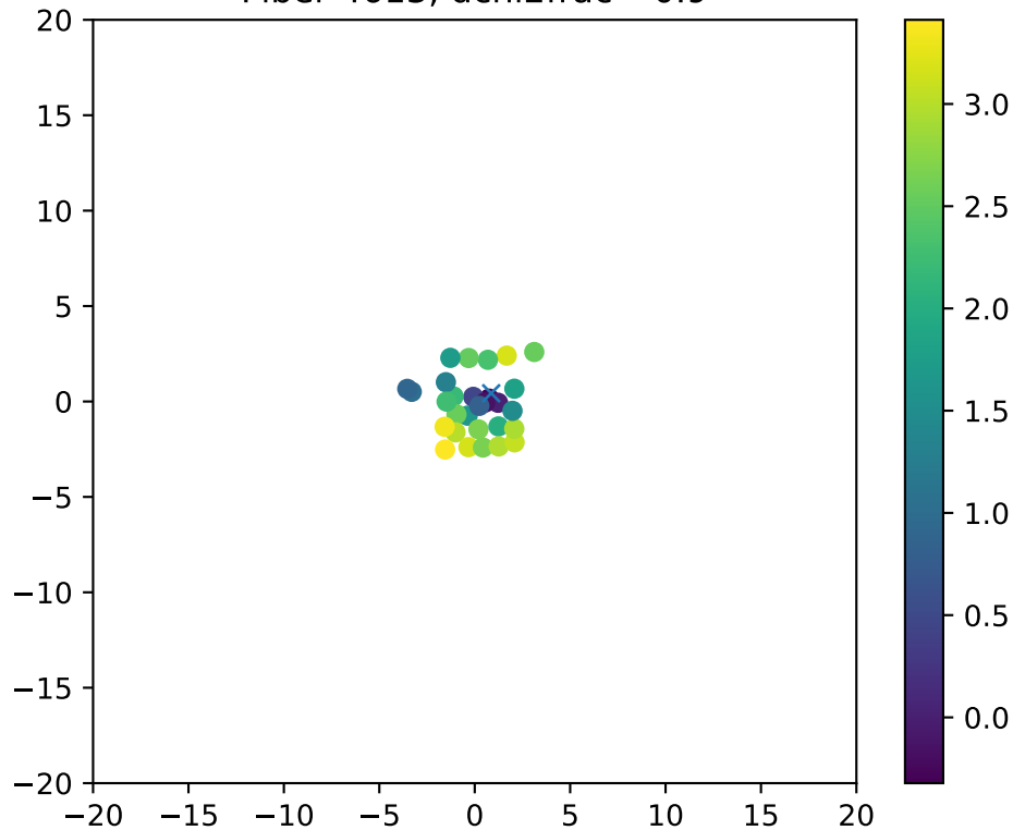
Fiber 4613, dchi2frac= 0.9
