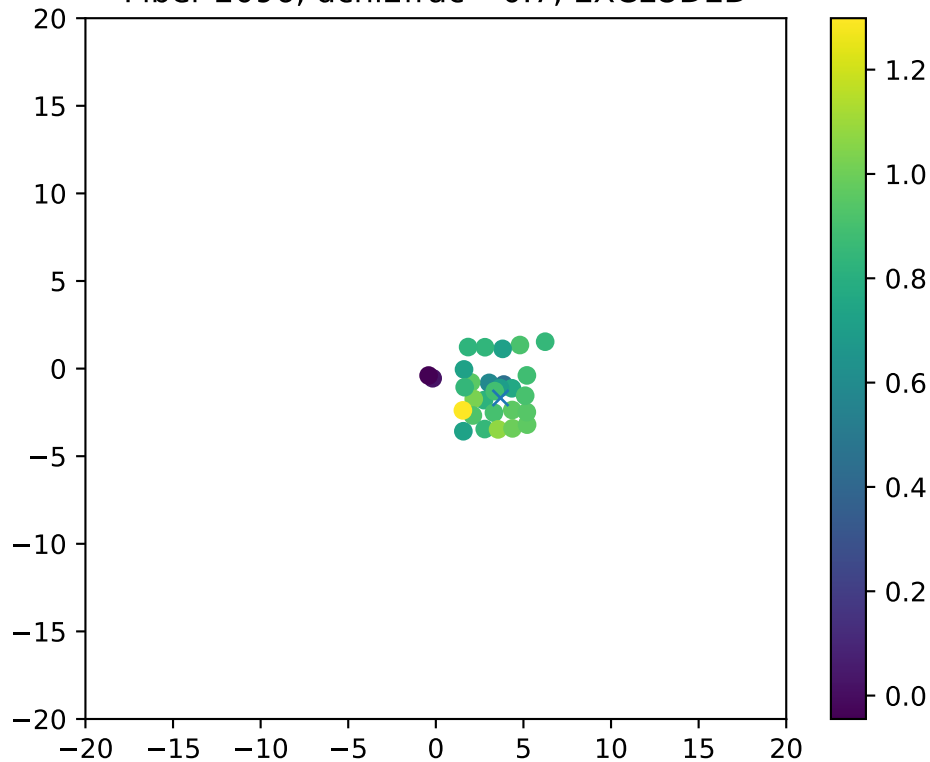
Fiber 2096, dchi2frac= 0.7, EXCLUDED
