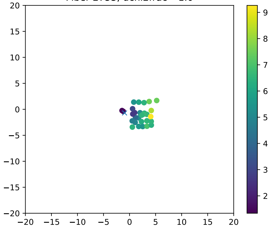
Fiber 2753, dchi2frac= 1.0
