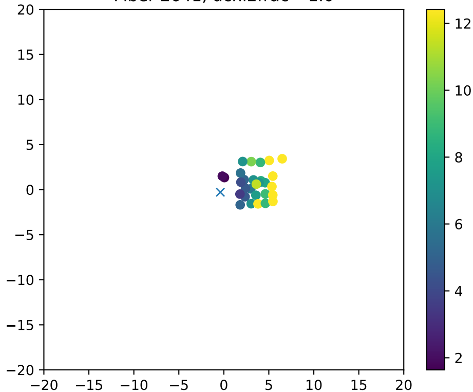
Fiber 2641, dchi2frac= 1.0
