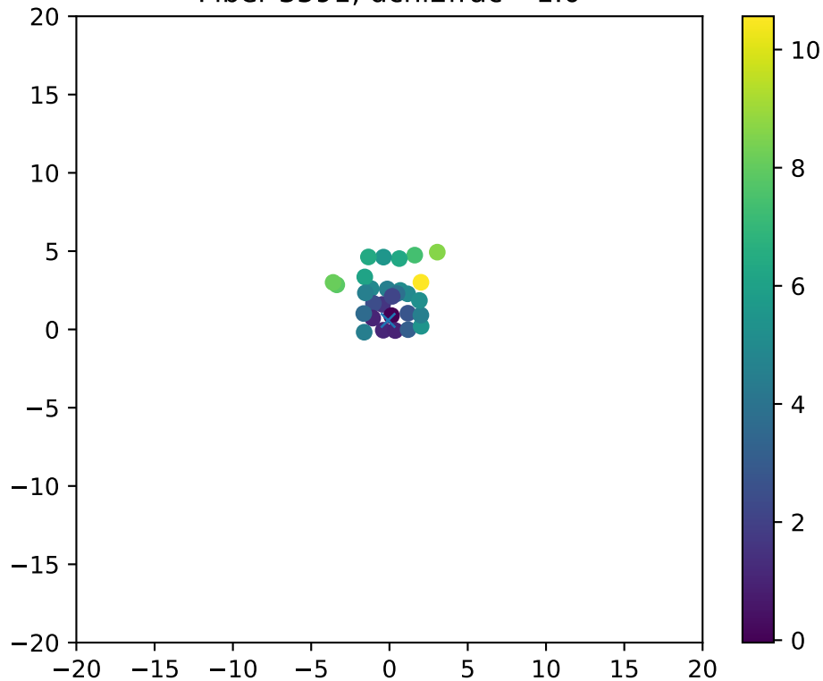
Fiber 3591, dchi2frac= 1.0
