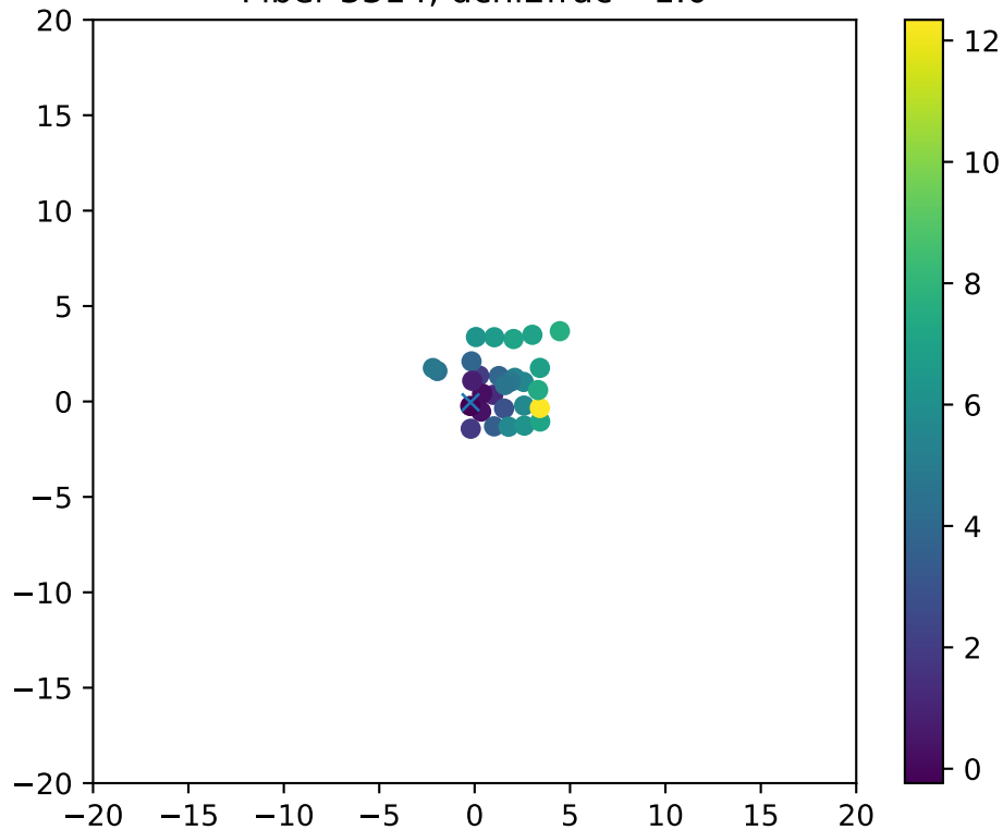
Fiber 3314, dchi2frac= 1.0
