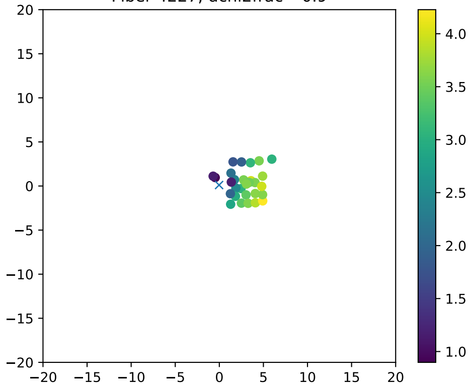
Fiber 4227, dchi2frac= 0.9
