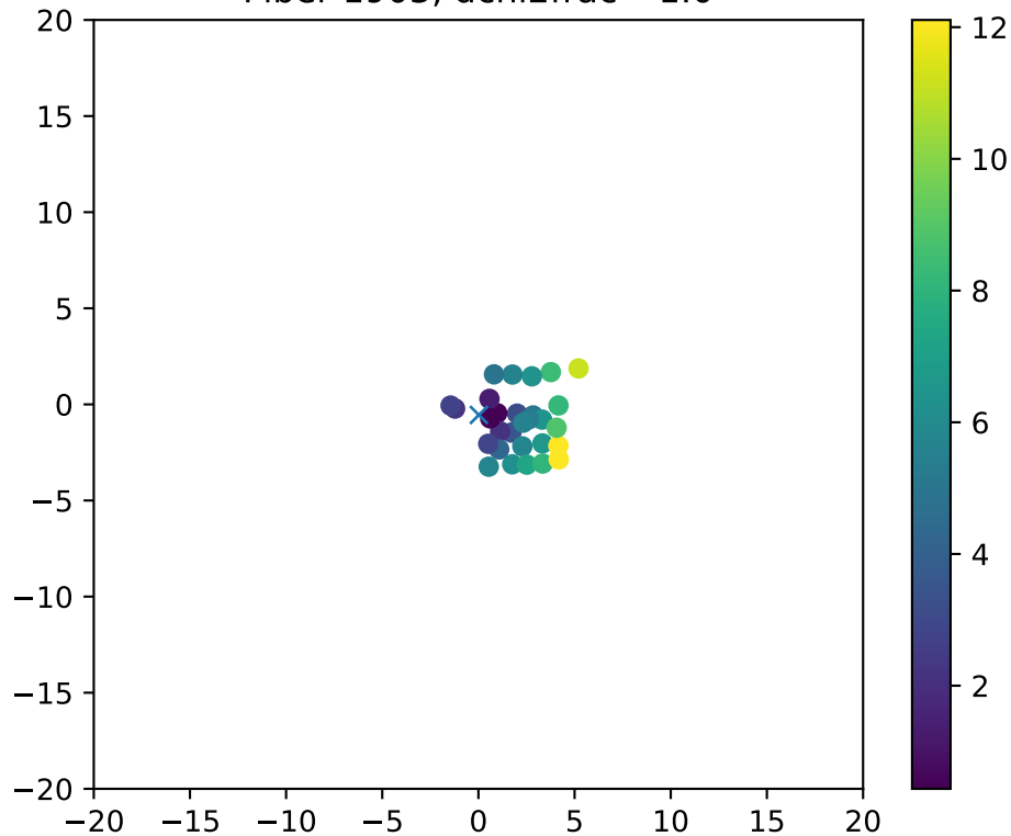
Fiber 1903, dchi2frac= 1.0
