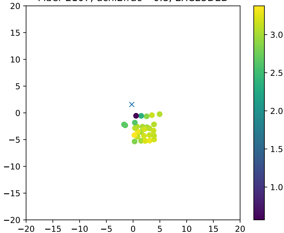
Fiber 2107, dchi2frac= 0.8, EXCLUDED
