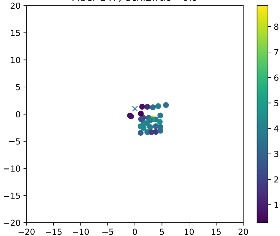
Fiber 147, dchi2frac= 0.9
