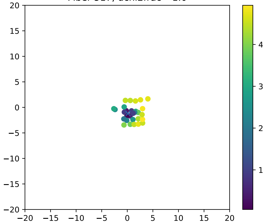
Fiber 517, dchi2frac= 1.0
