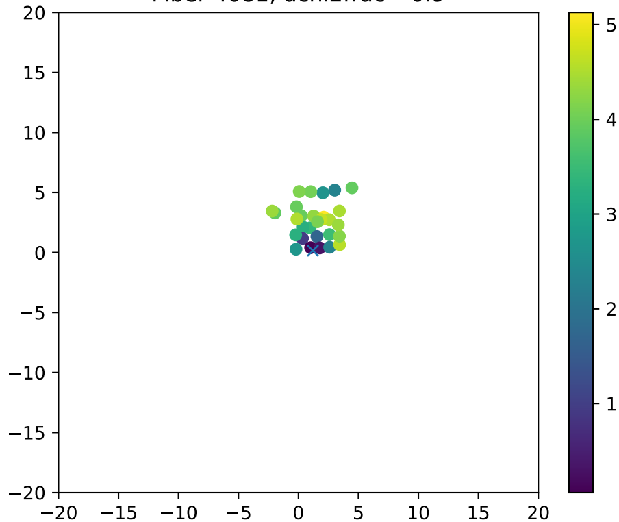
Fiber 4081, dchi2frac= 0.9
