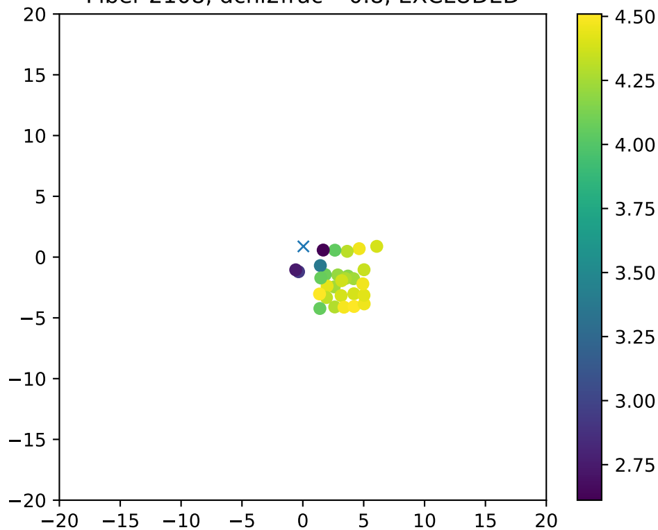
Fiber 2108, dchi2frac= 0.8, EXCLUDED
