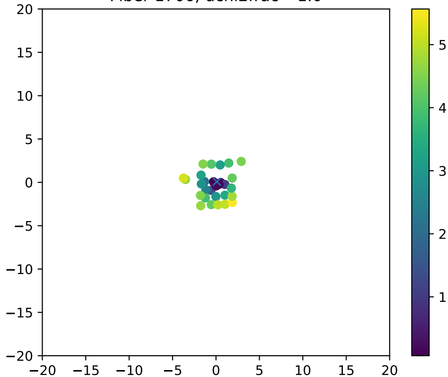
Fiber 1706, dchi2frac= 1.0
