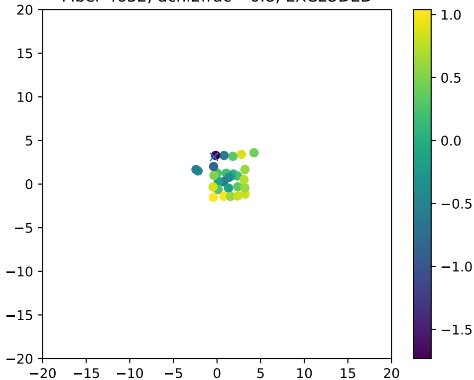
Fiber 4632, dchi2frac= 0.8, EXCLUDED
