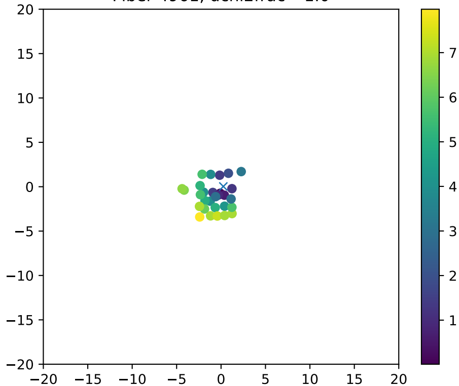
Fiber 4961, dchi2frac= 1.0
