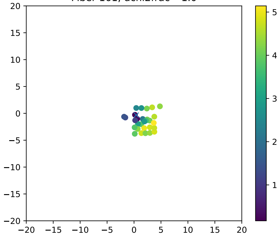
Fiber 161, dchi2frac= 1.0
