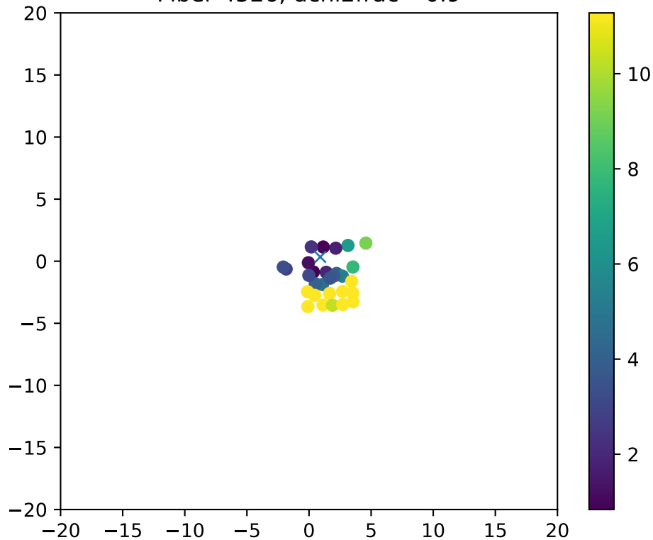
Fiber 4526, dchi2frac= 0.9
