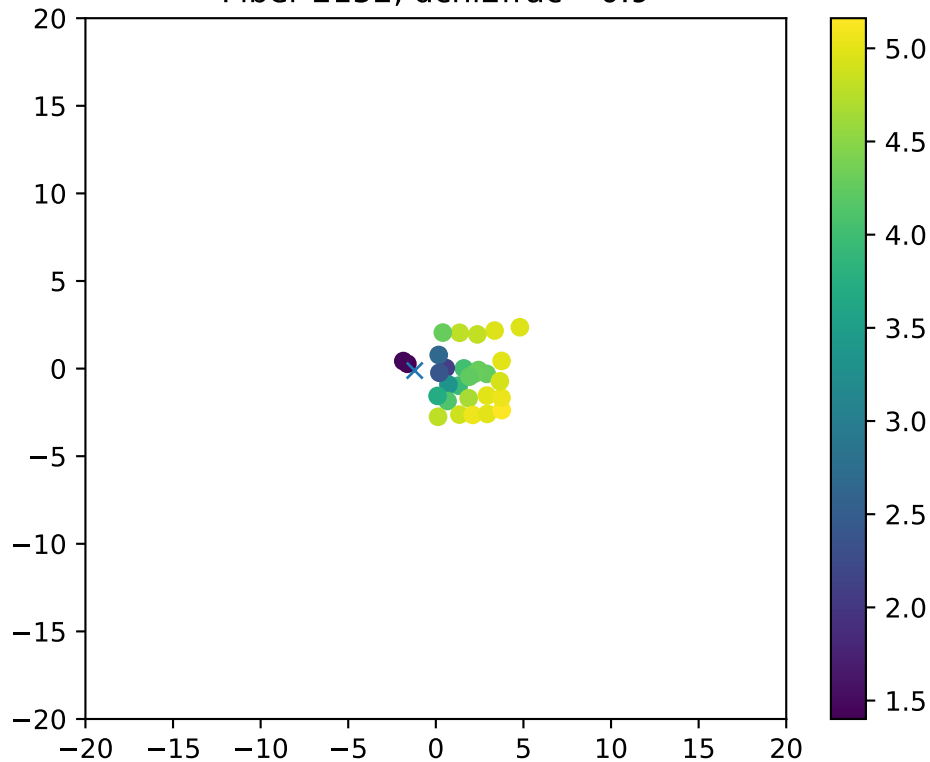
Fiber 2152, dchi2frac= 0.9
