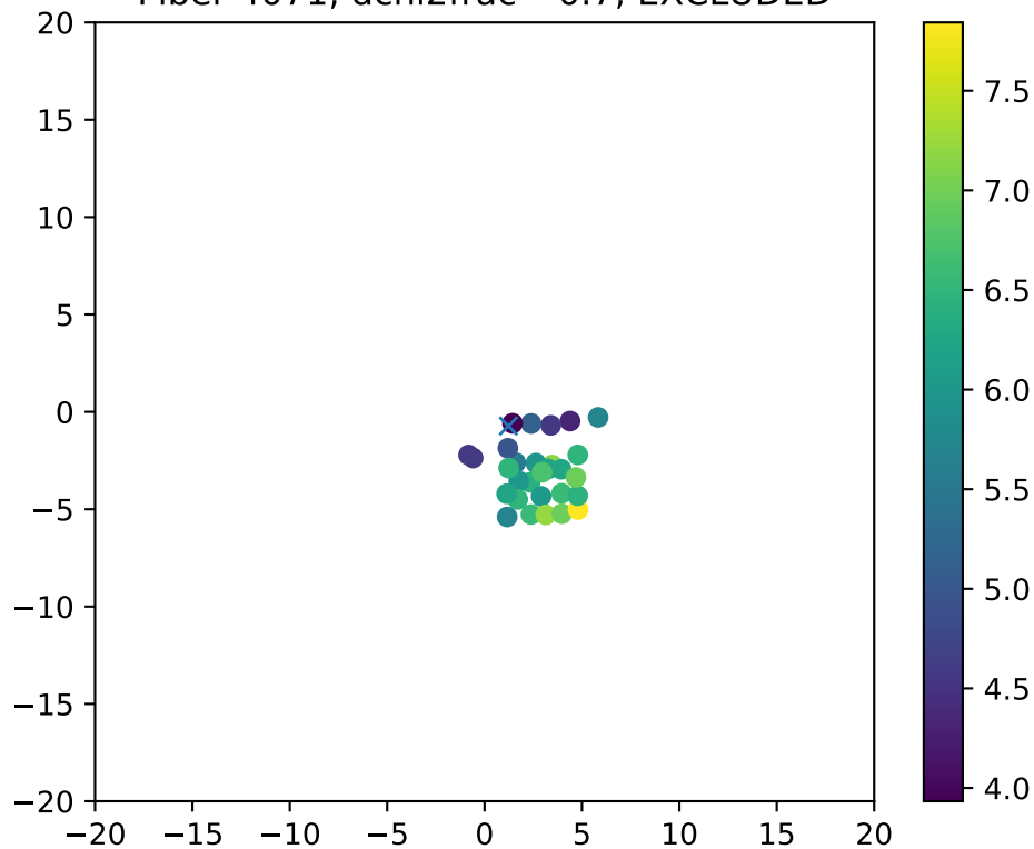
Fiber 4071, dchi2frac= 0.7, EXCLUDED
