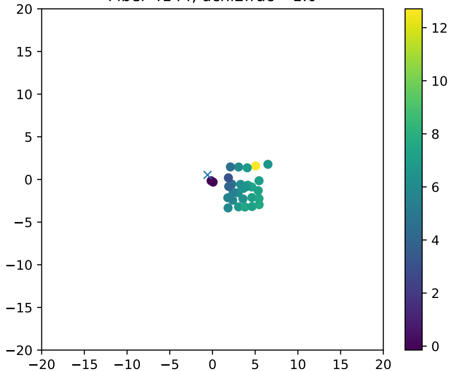
Fiber 4144, dchi2frac= 1.0
