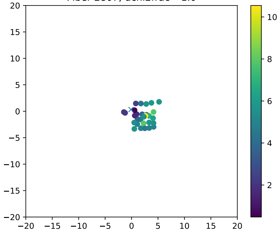
Fiber 2807, dchi2frac= 1.0
