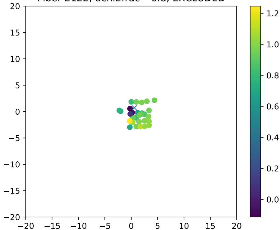
Fiber 2122, dchi2frac= 0.8, EXCLUDED
