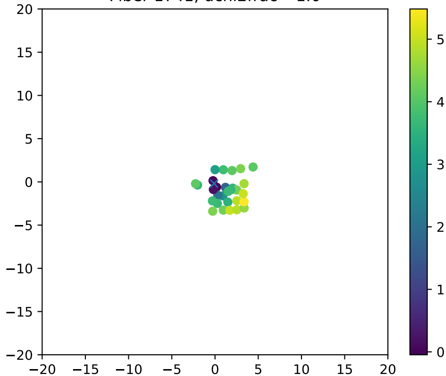
Fiber 1741, dchi2frac= 1.0
