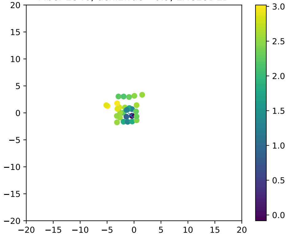
Fiber 2346, dchi2frac= 0.9, EXCLUDED
