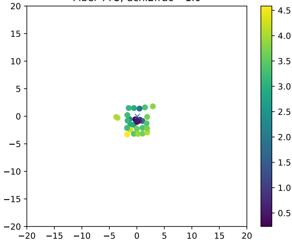
Fiber 773, dchi2frac= 1.0
