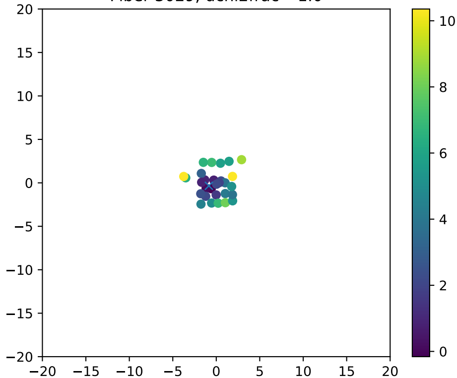
Fiber 3029, dchi2frac= 1.0
