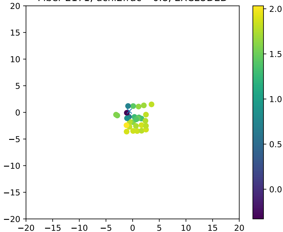
Fiber 2171, dchi2frac= 0.8, EXCLUDED
