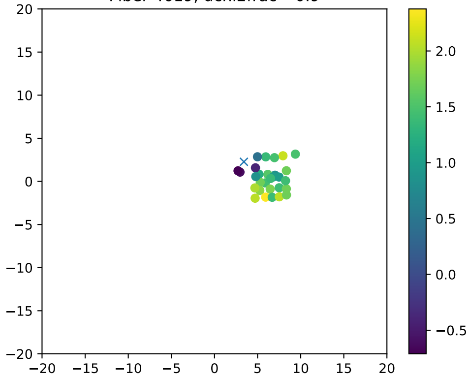
Fiber 4619, dchi2frac= 0.9
