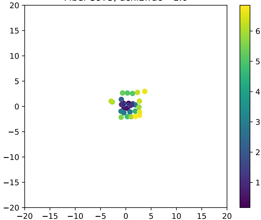
Fiber 3975, dchi2frac= 1.0
