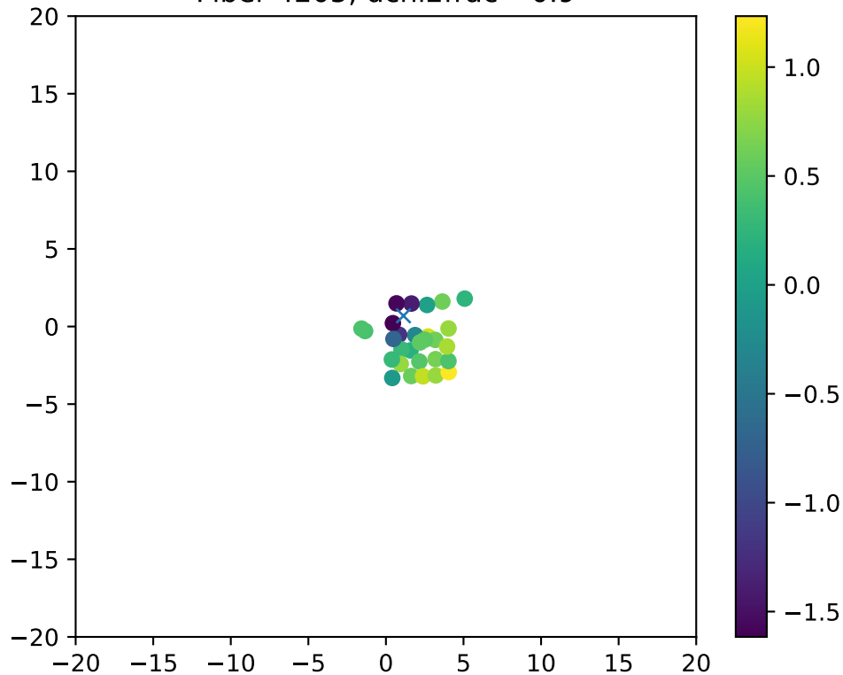
Fiber 4205, dchi2frac= 0.9
