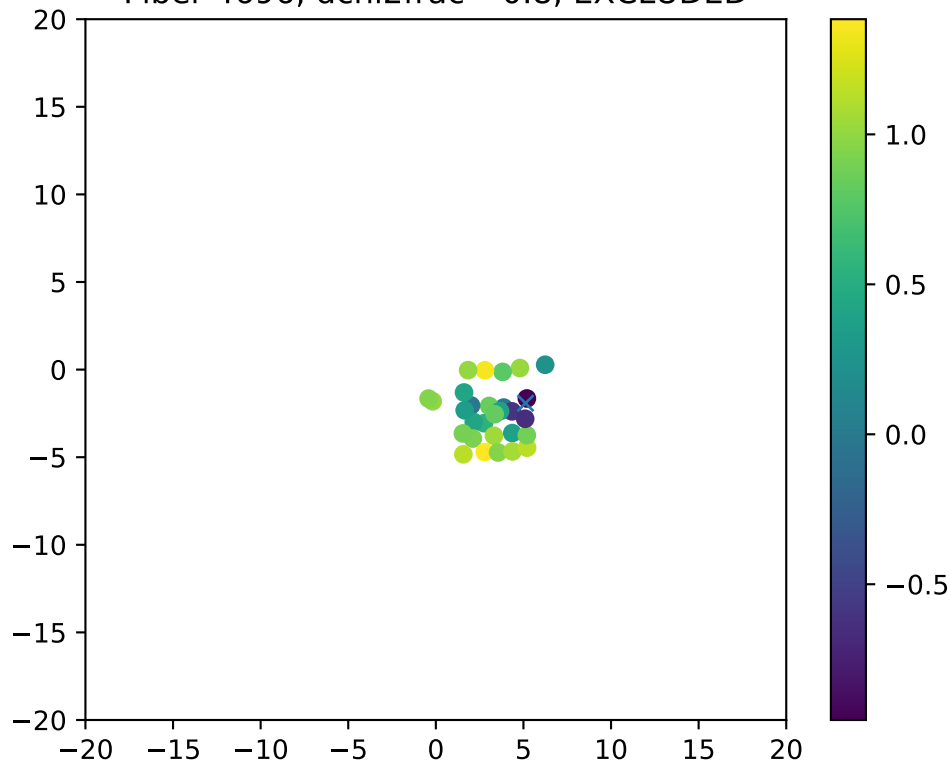
Fiber 4696, dchi2frac= 0.8, EXCLUDED
