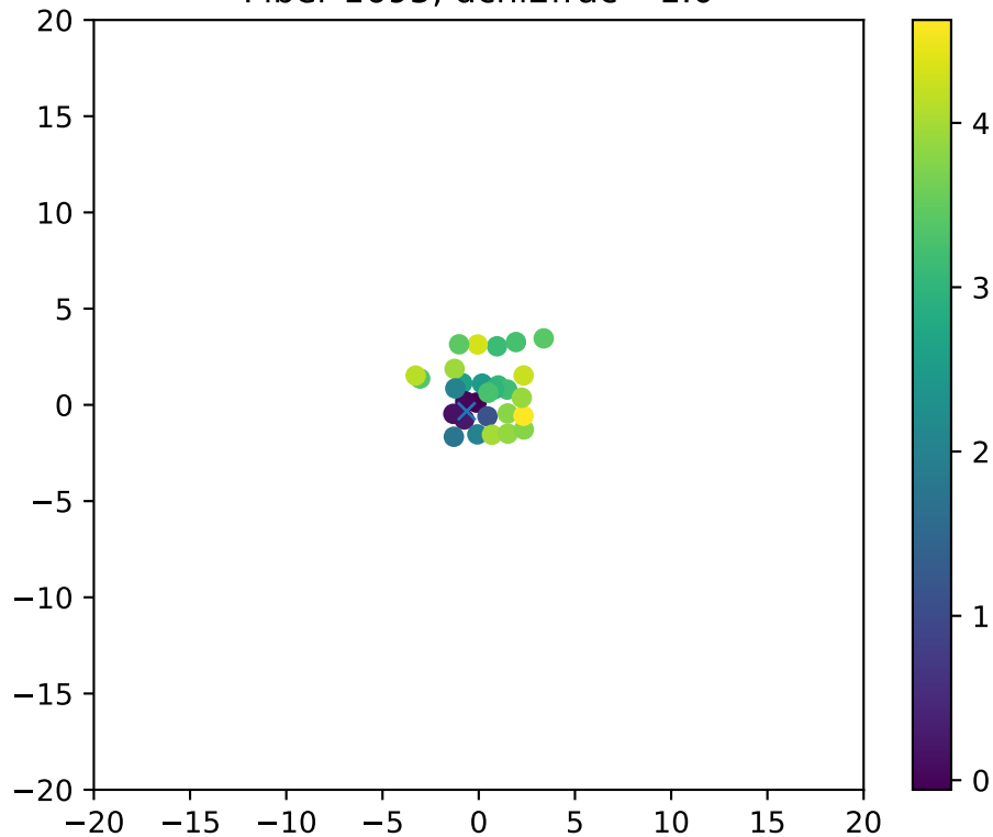
Fiber 1695, dchi2frac= 1.0
