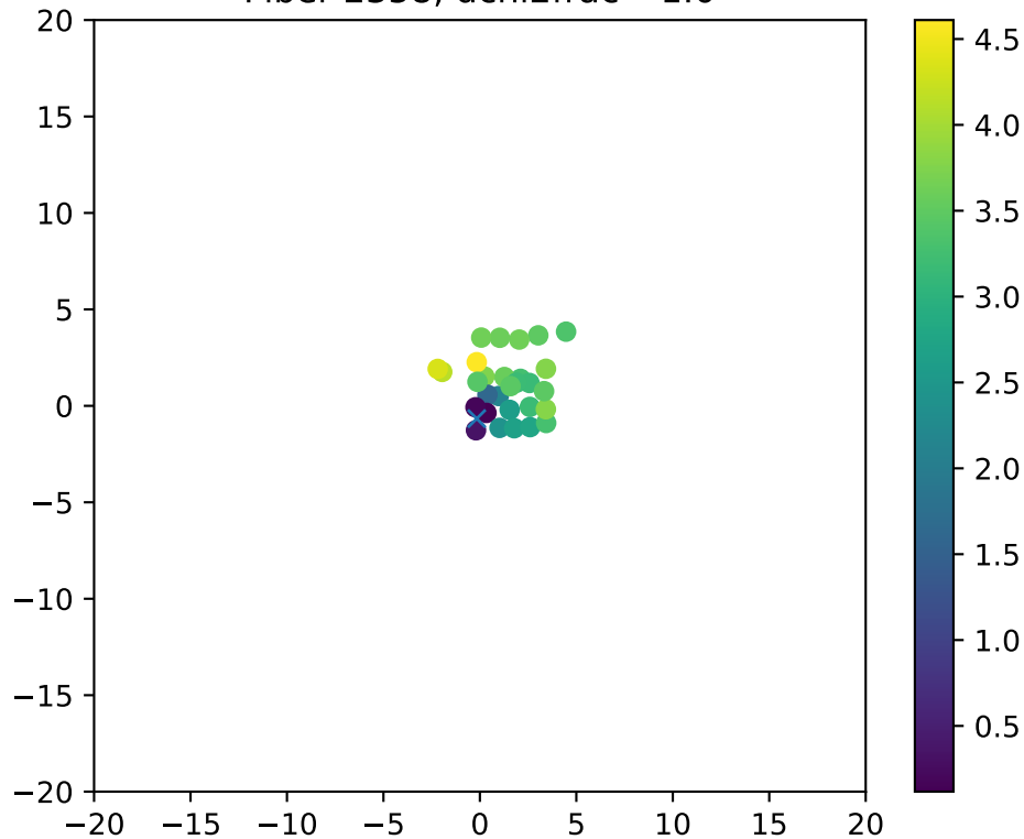
Fiber 2358, dchi2frac= 1.0
