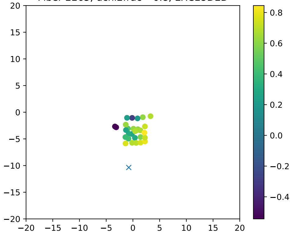
Fiber 2265, dchi2frac= 0.8, EXCLUDED
