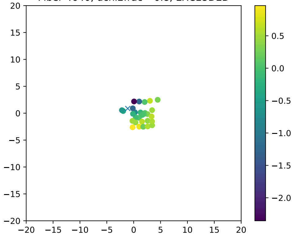
Fiber 4640, dchi2frac= 0.8, EXCLUDED
