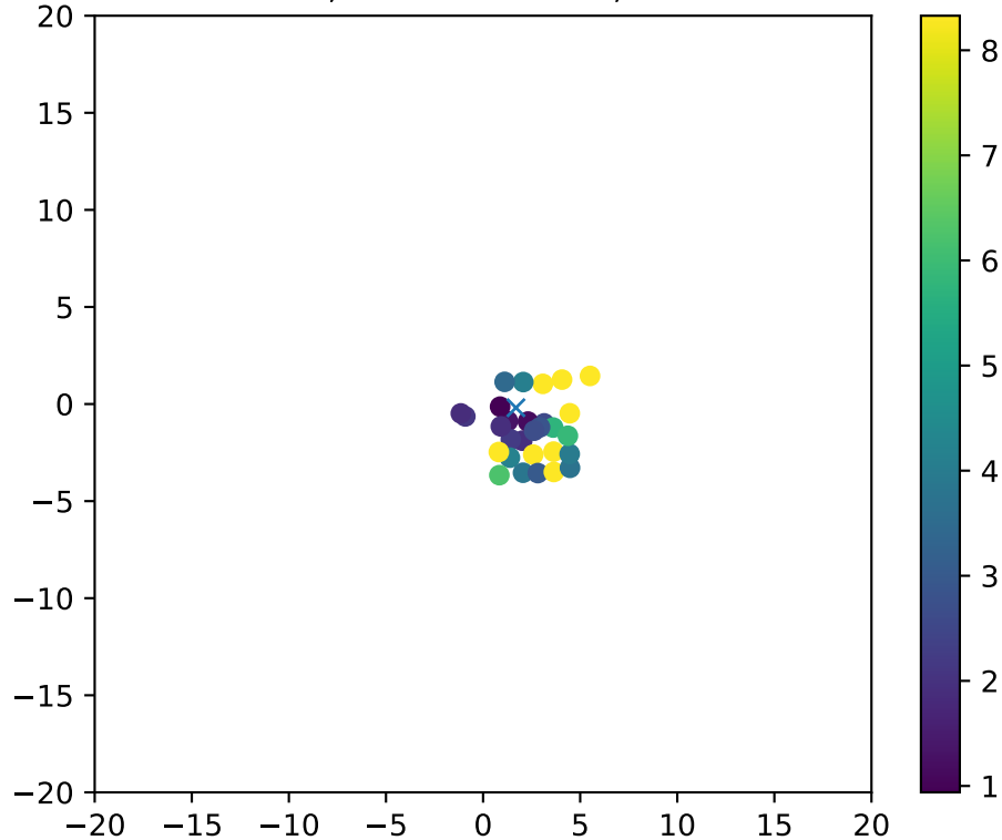
Fiber 2801, dchi2frac= 0.9, EXCLUDED
