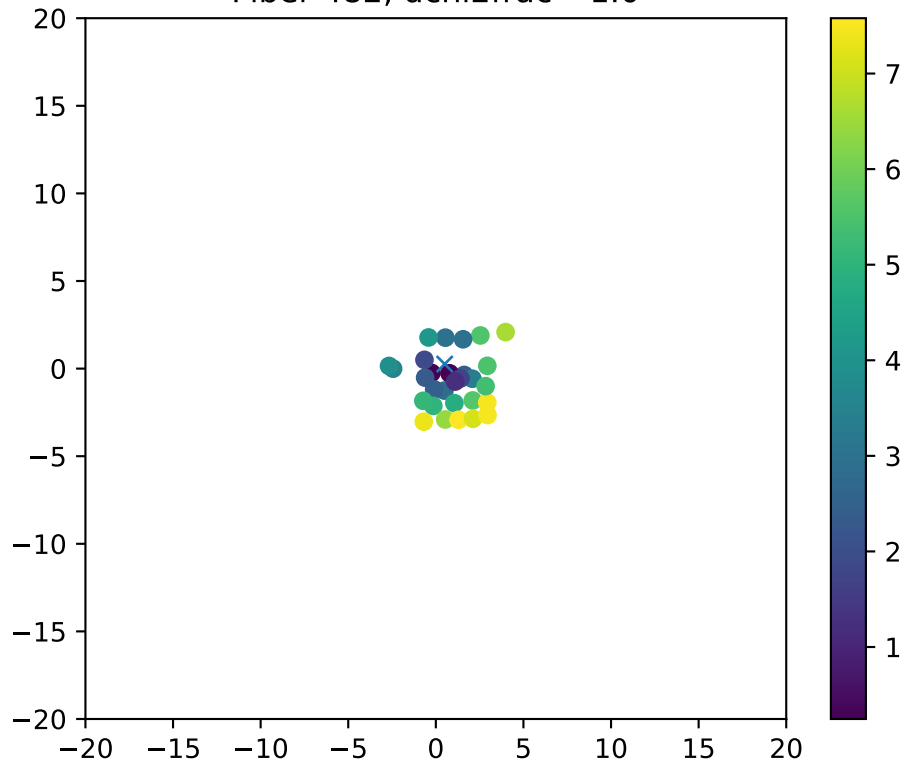
Fiber 482, dchi2frac= 1.0
