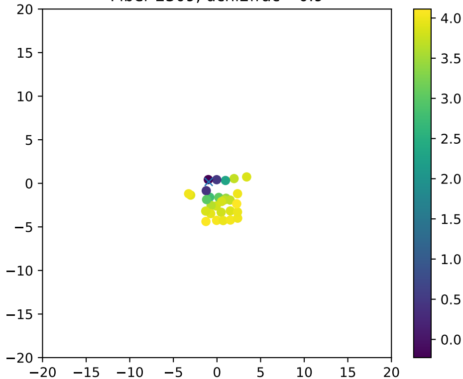
Fiber 2309, dchi2frac= 0.9
