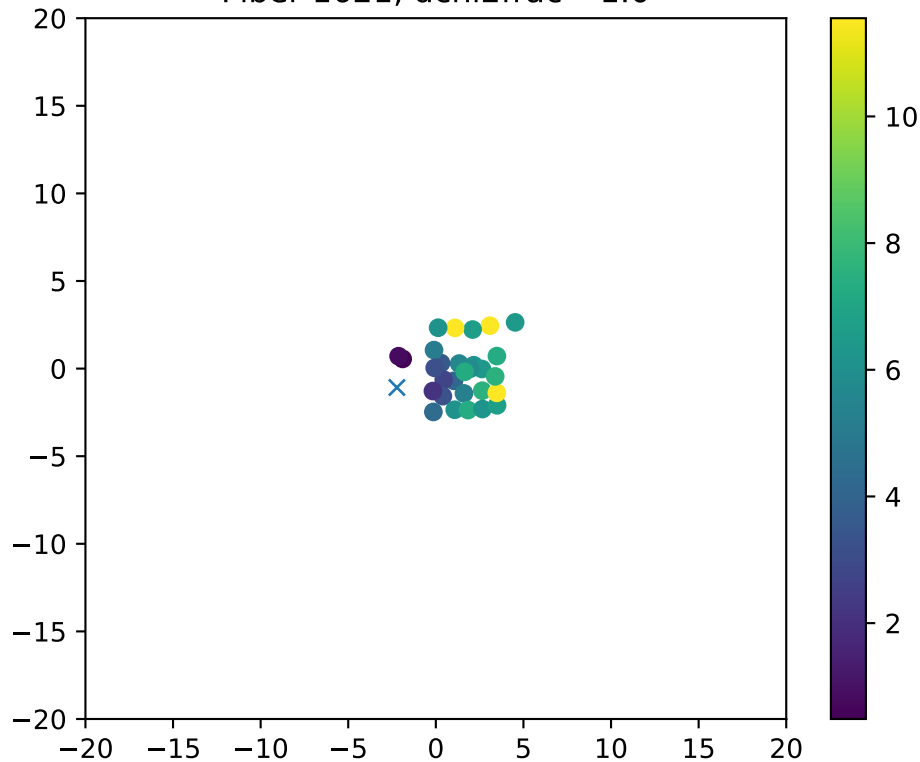
Fiber 1621, dchi2frac= 1.0
