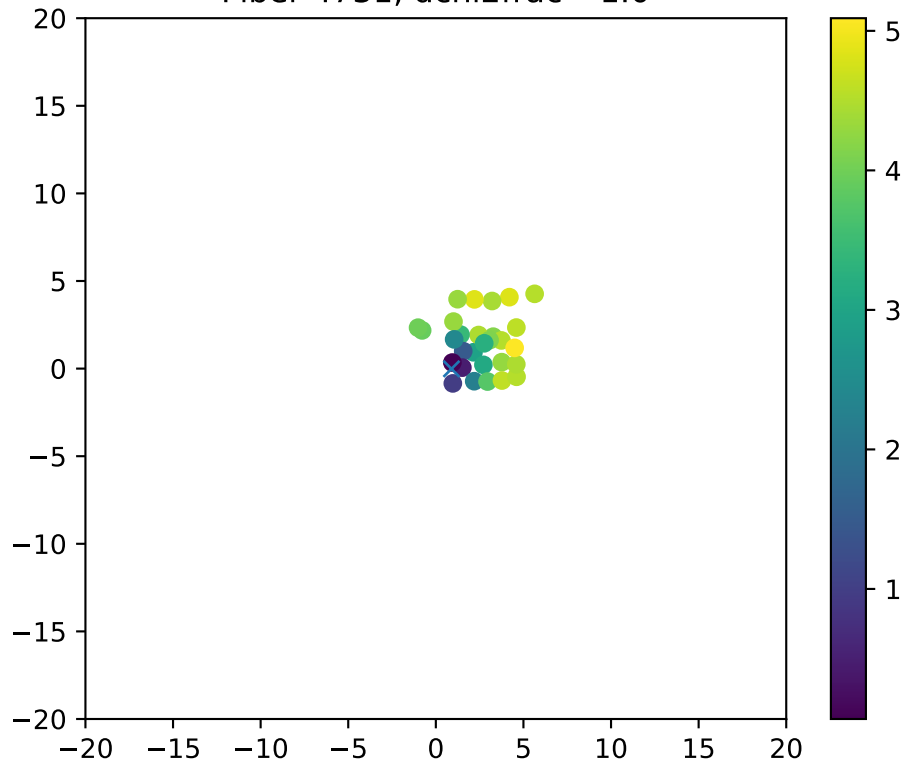
Fiber 4731, dchi2frac= 1.0
