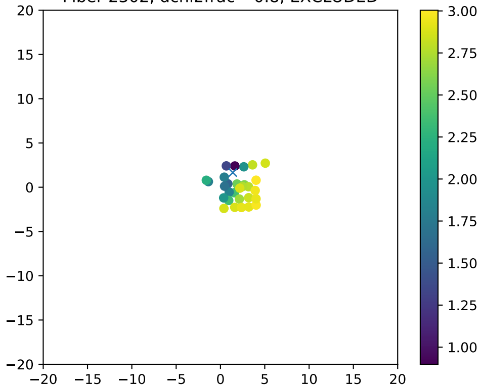
Fiber 2302, dchi2frac= 0.8, EXCLUDED
