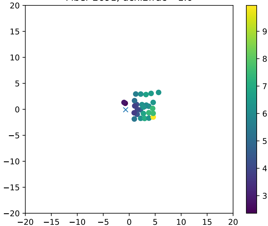
Fiber 2691, dchi2frac= 1.0
