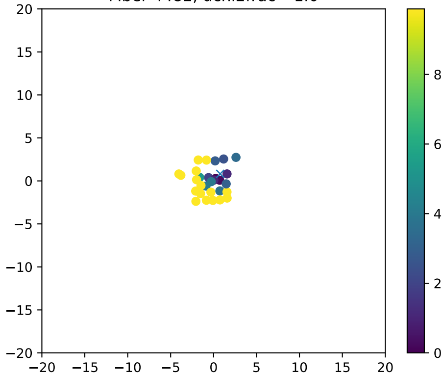
Fiber 4482, dchi2frac= 1.0
