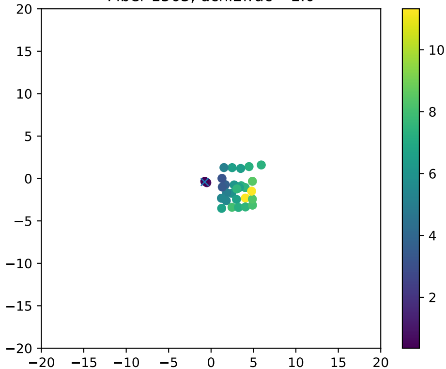
Fiber 1563, dchi2frac= 1.0
