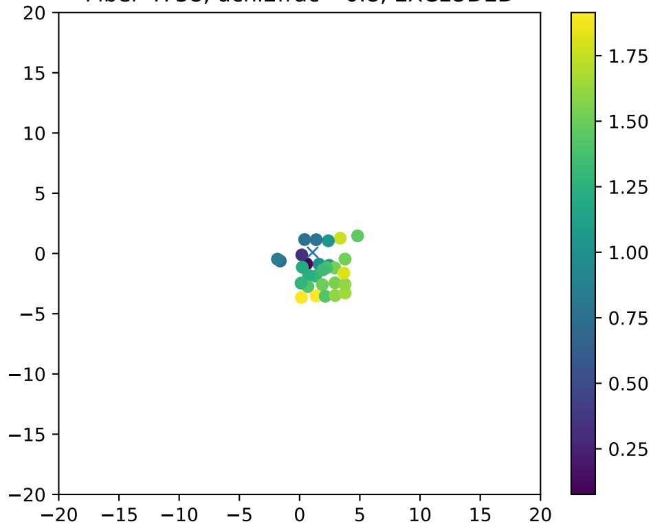
Fiber 4738, dchi2frac= 0.8, EXCLUDED
