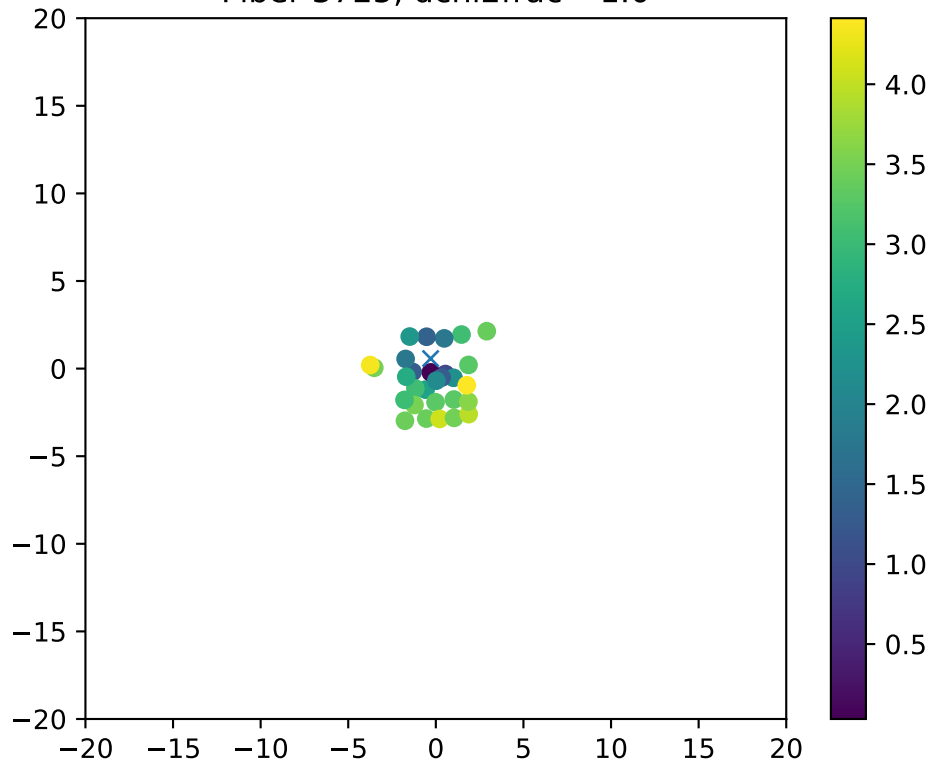
Fiber 3725, dchi2frac= 1.0
