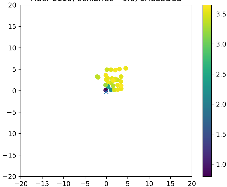
Fiber 2118, dchi2frac= 0.8, EXCLUDED
