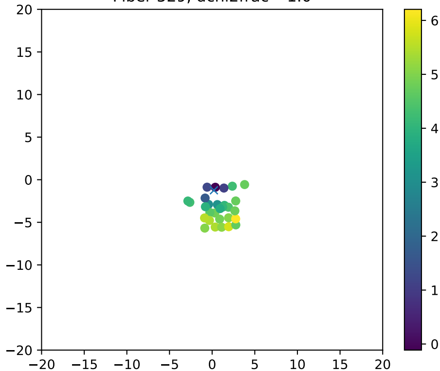
Fiber 529, dchi2frac= 1.0
