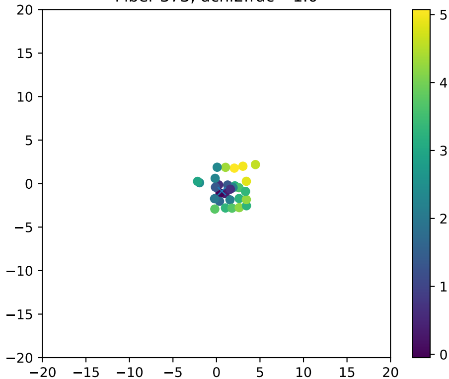
Fiber 373, dchi2frac= 1.0
