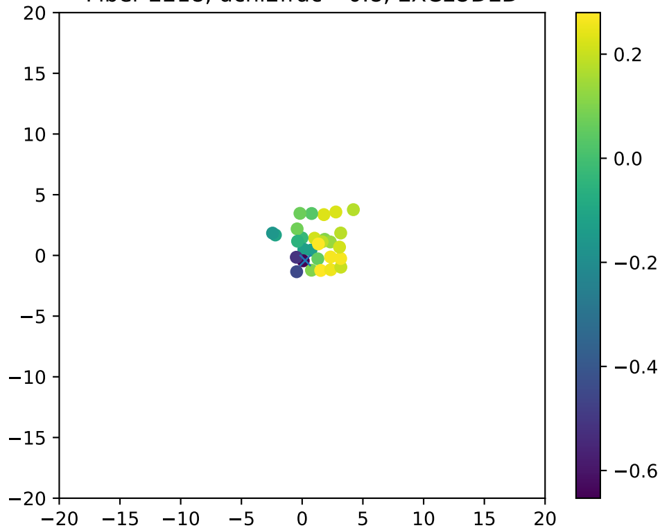
Fiber 2218, dchi2frac= 0.8, EXCLUDED
