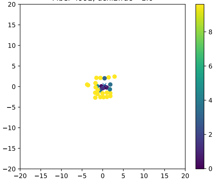
Fiber 4992, dchi2frac= 1.0
