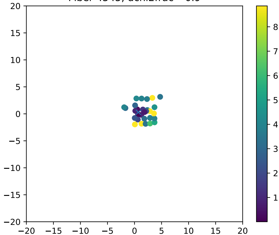
Fiber 4545, dchi2frac= 0.9
