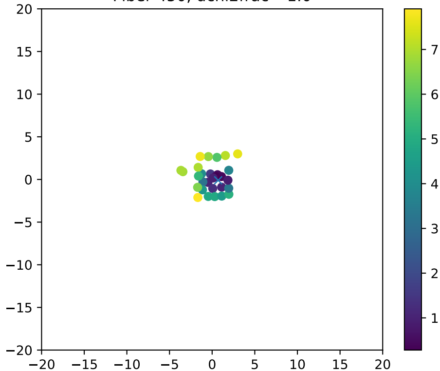
Fiber 450, dchi2frac= 1.0
