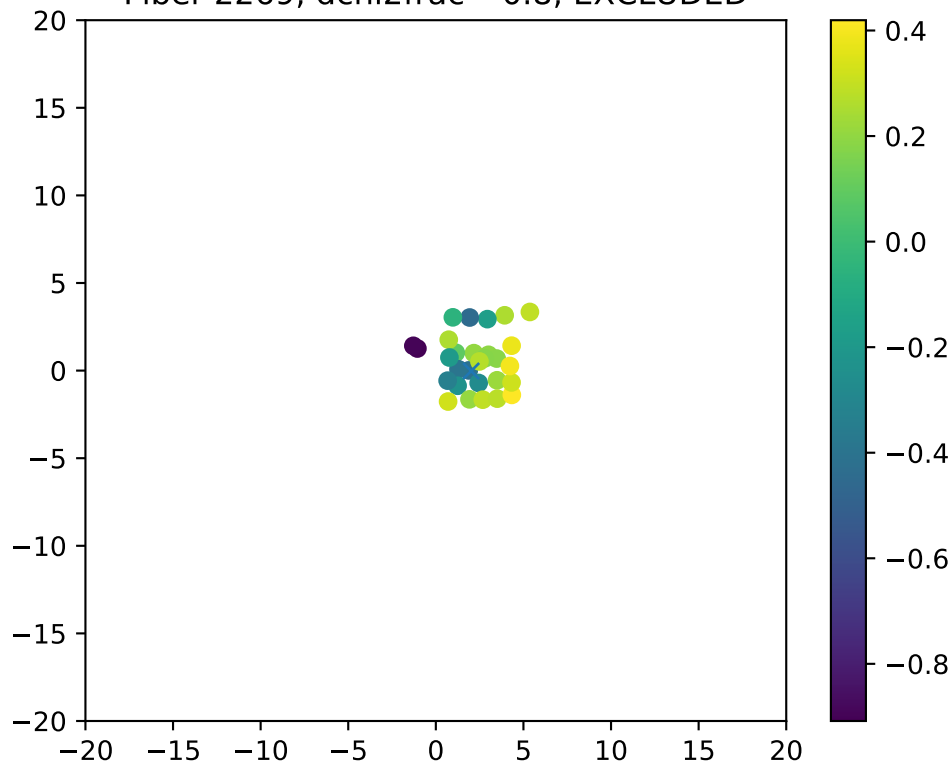
Fiber 2269, dchi2frac= 0.8, EXCLUDED
