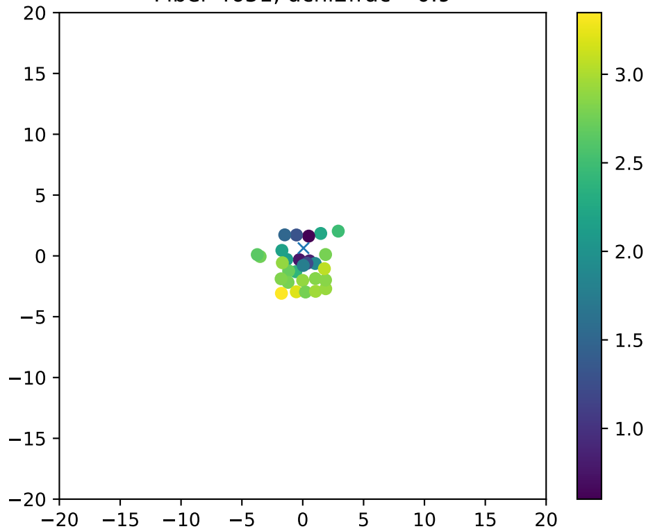
Fiber 4651, dchi2frac= 0.9
