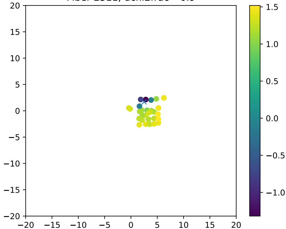
Fiber 2311, dchi2frac= 0.9
