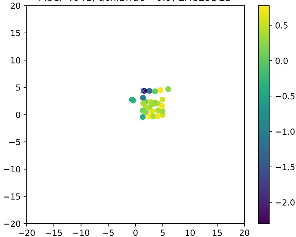
Fiber 4641, dchi2frac= 0.9, EXCLUDED
