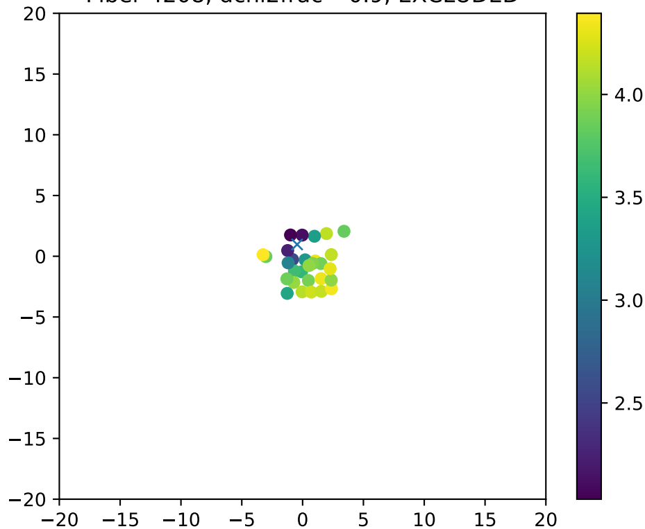
Fiber 4208, dchi2frac= 0.9, EXCLUDED
