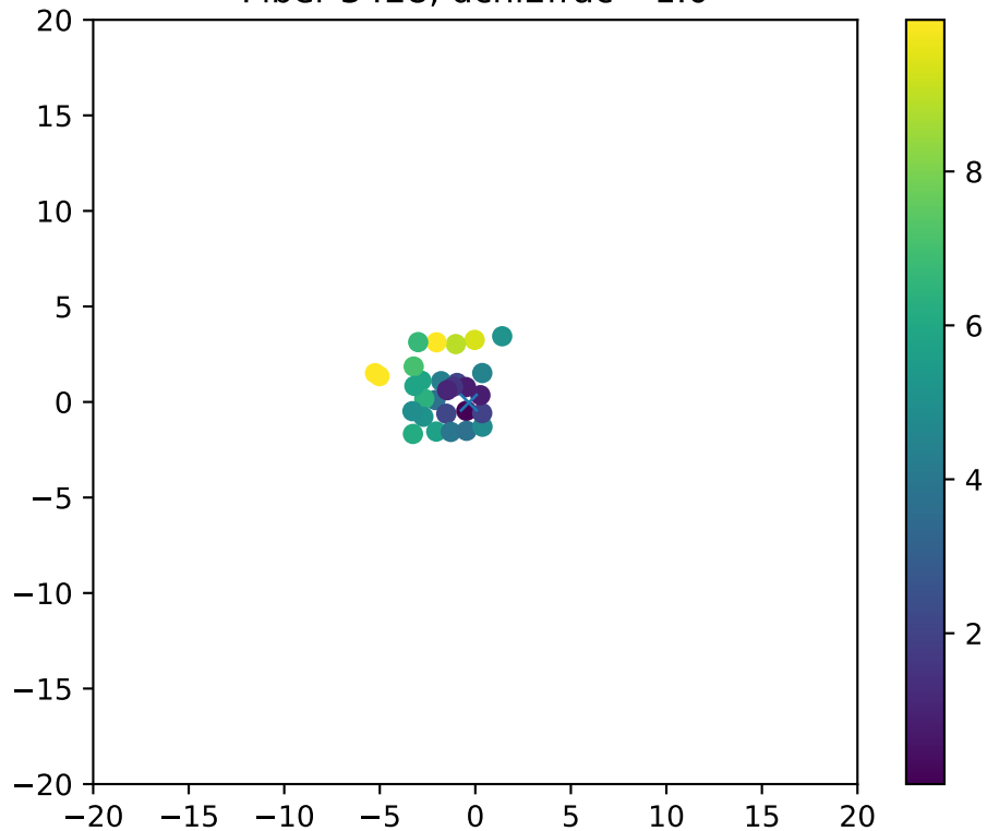
Fiber 3428, dchi2frac= 1.0
