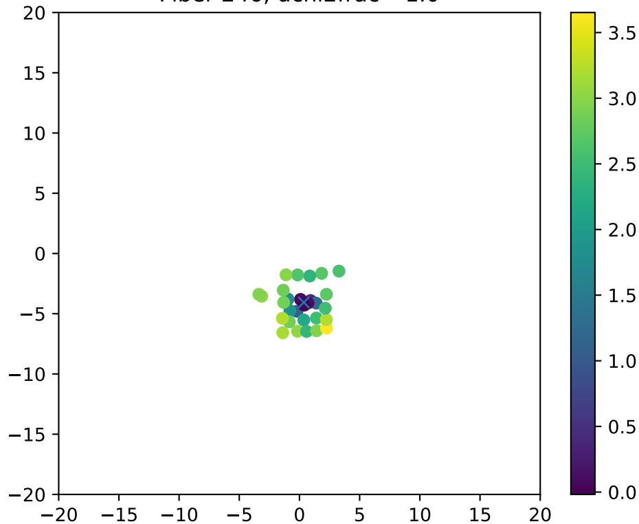
Fiber 246, dchi2frac= 1.0
