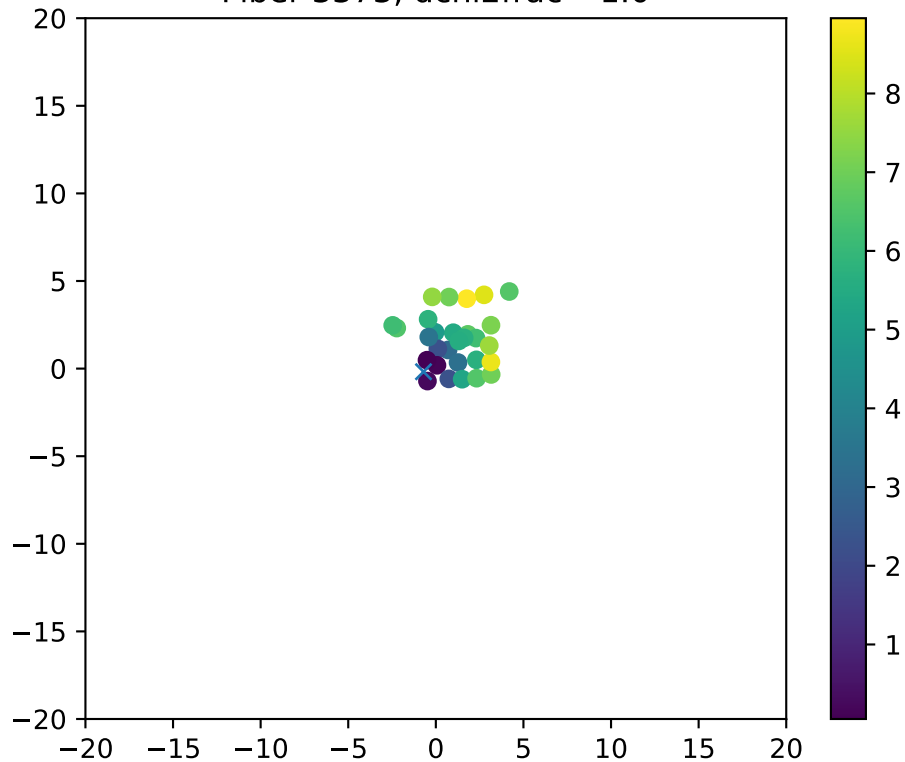
Fiber 3373, dchi2frac= 1.0
