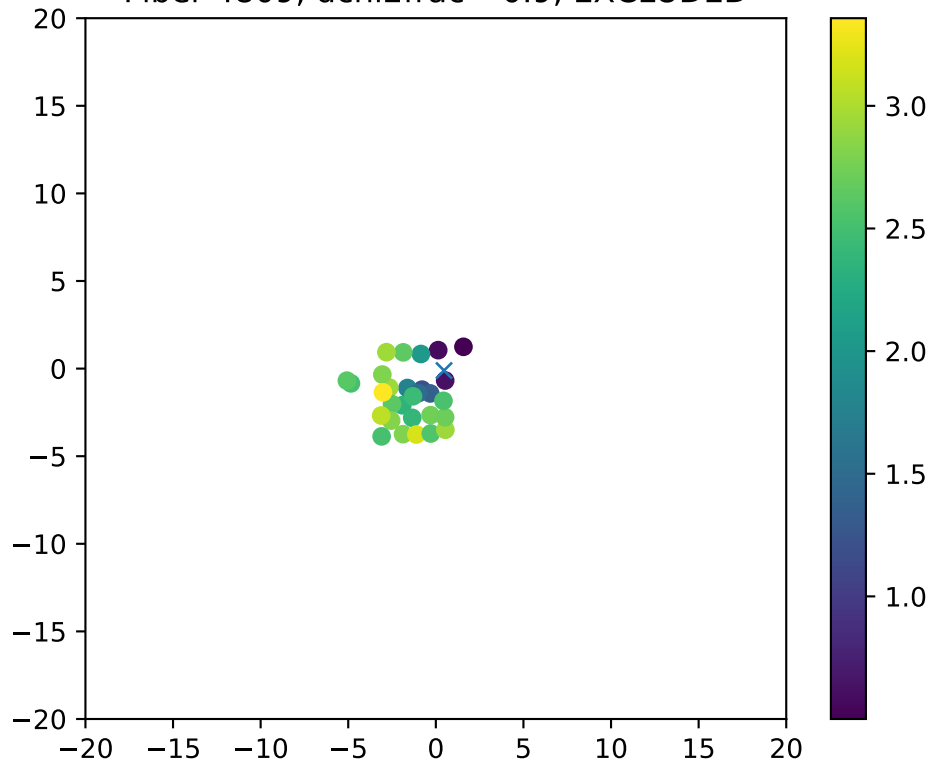
Fiber 4809, dchi2frac= 0.9, EXCLUDED
