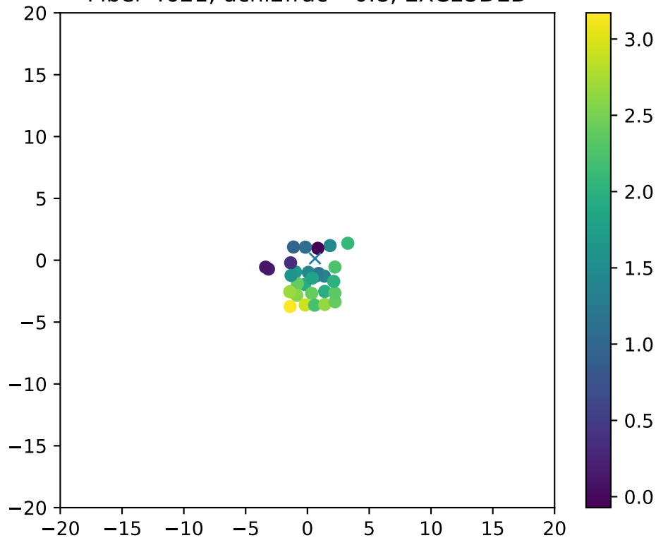
Fiber 4621, dchi2frac= 0.8, EXCLUDED
