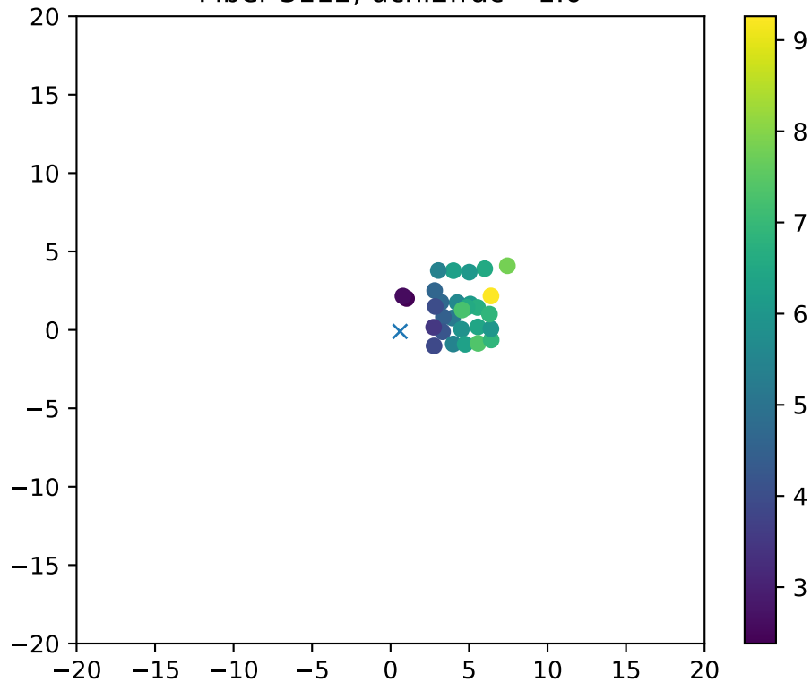
Fiber 3112, dchi2frac= 1.0
