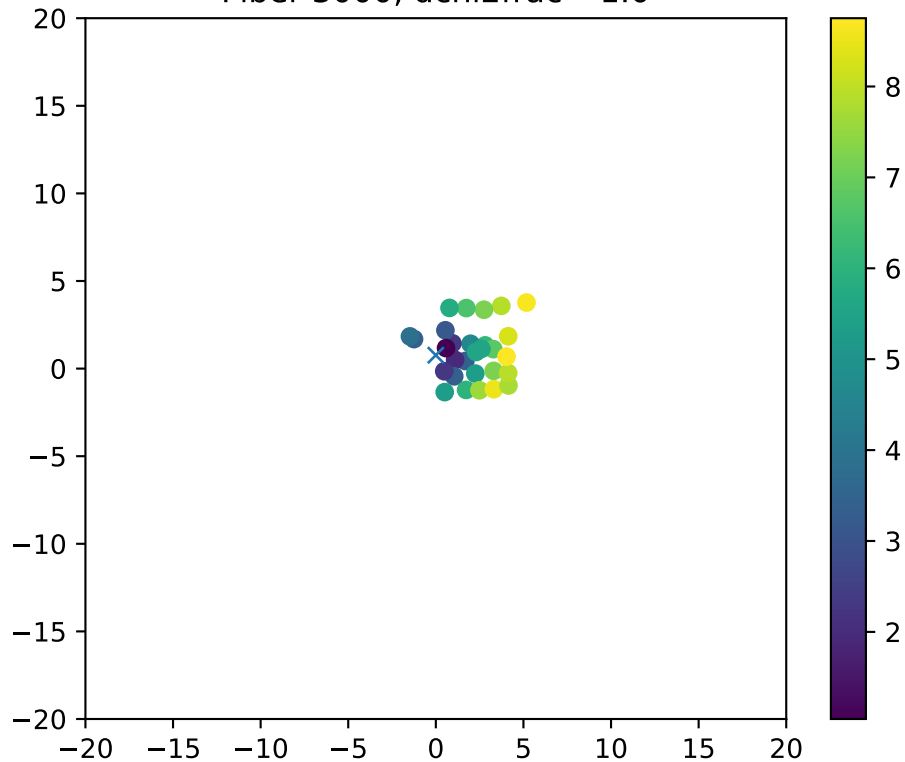
Fiber 3000, dchi2frac= 1.0
