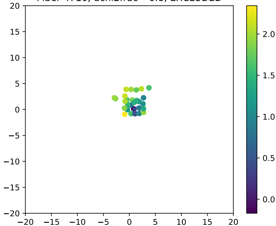
Fiber 4710, dchi2frac= 0.8, EXCLUDED
