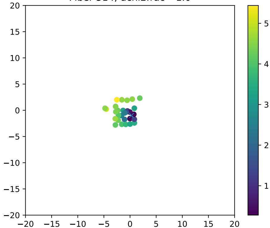
Fiber 514, dchi2frac= 1.0
