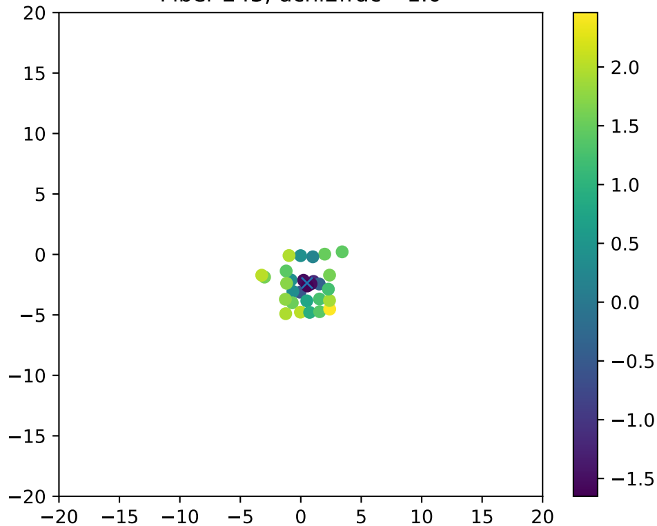
Fiber 243, dchi2frac= 1.0
