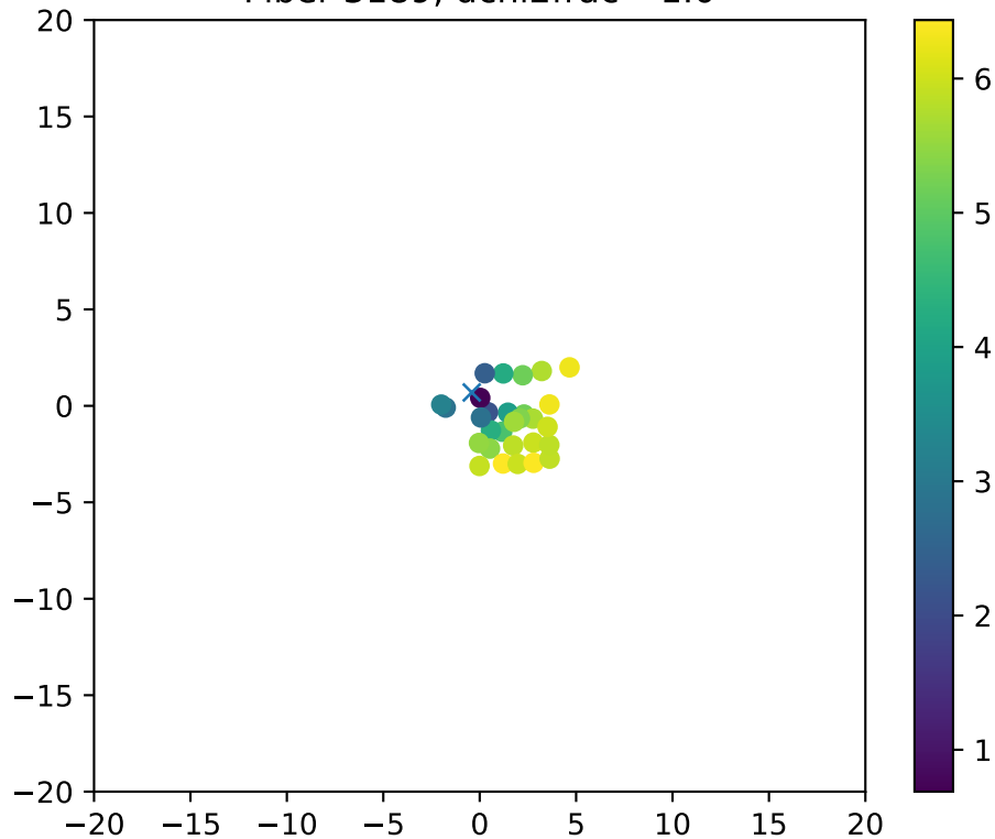
Fiber 3189, dchi2frac= 1.0
