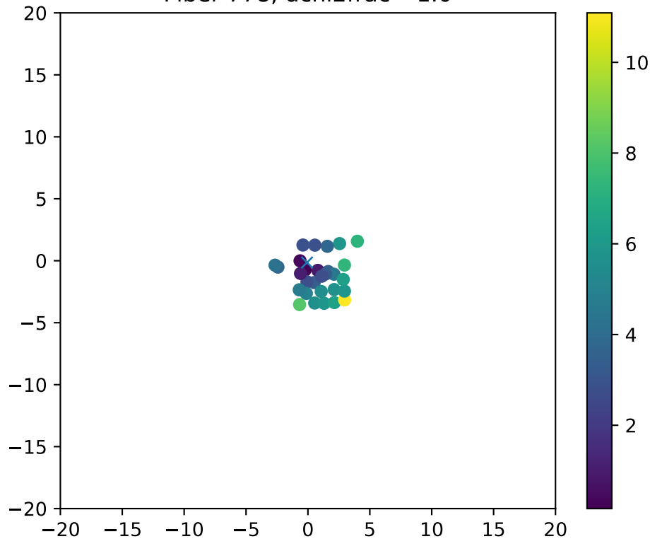
Fiber 778, dchi2frac= 1.0
