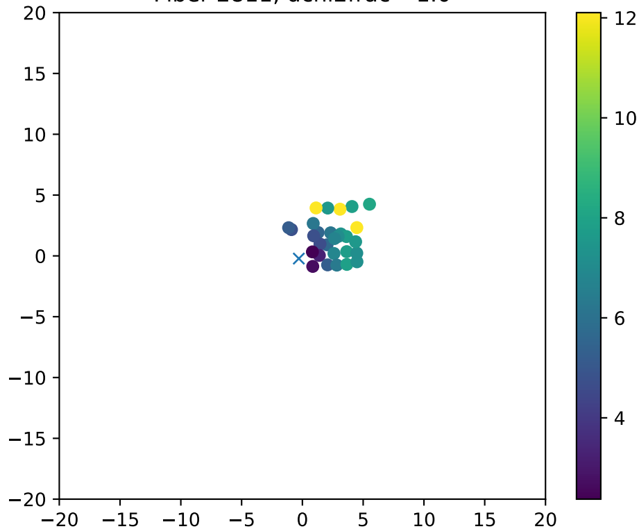
Fiber 2811, dchi2frac= 1.0
