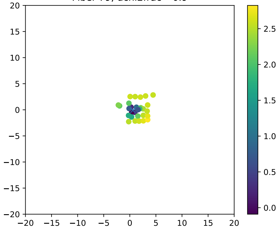
Fiber 79, dchi2frac= 0.9
