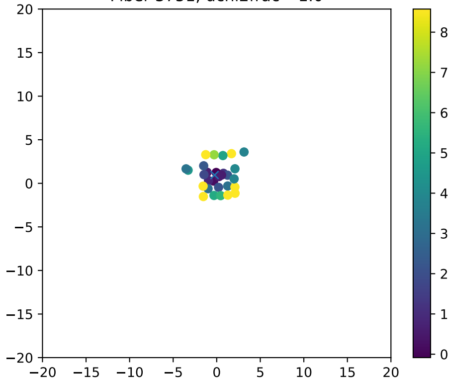
Fiber 3751, dchi2frac= 1.0
