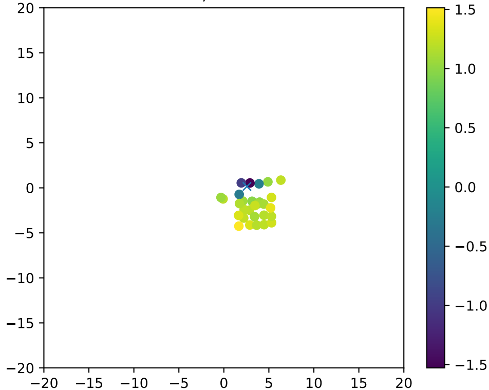
Fiber 2314, dchi2frac= 0.9
