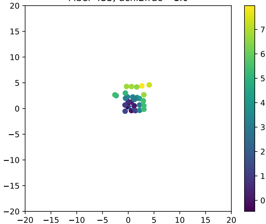
Fiber 433, dchi2frac= 1.0
