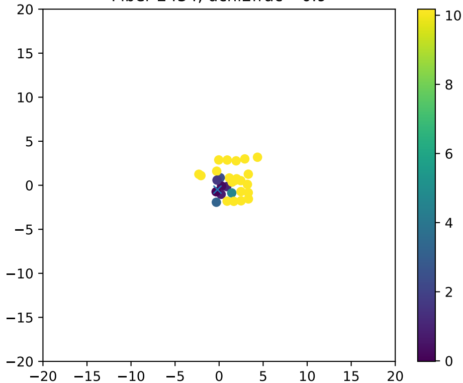
Fiber 2434, dchi2frac= 0.9
