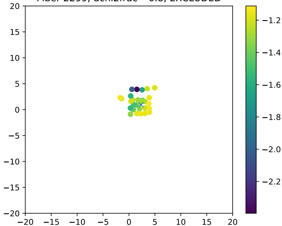
Fiber 2299, dchi2frac= 0.8, EXCLUDED
