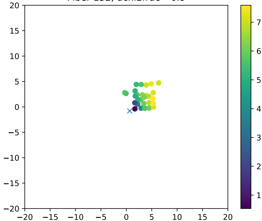
Fiber 152, dchi2frac= 0.9
