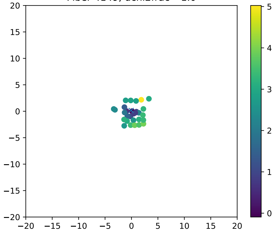
Fiber 4149, dchi2frac= 1.0
