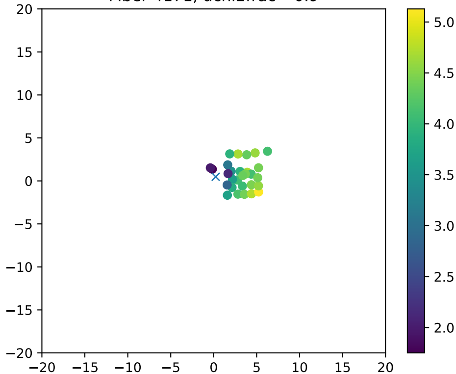
Fiber 4171, dchi2frac= 0.9
