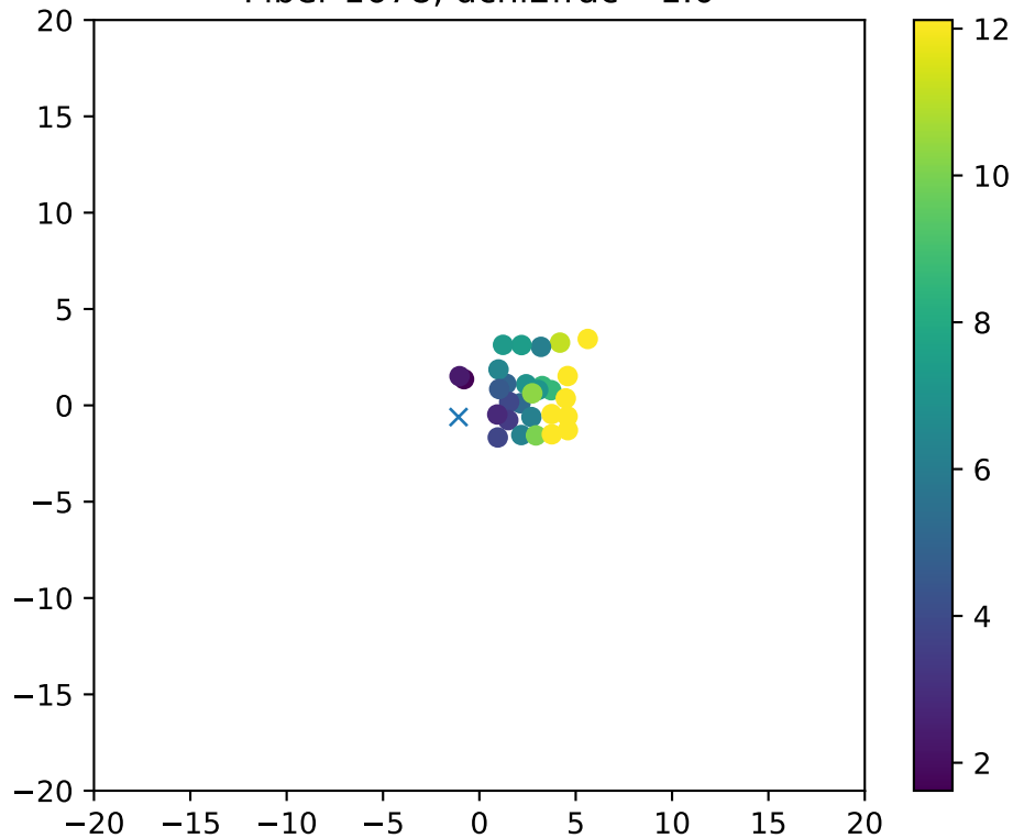
Fiber 1678, dchi2frac= 1.0
