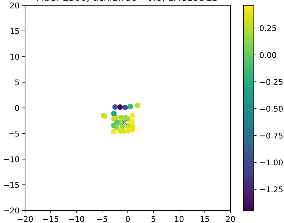
Fiber 2300, dchi2frac= 0.8, EXCLUDED
