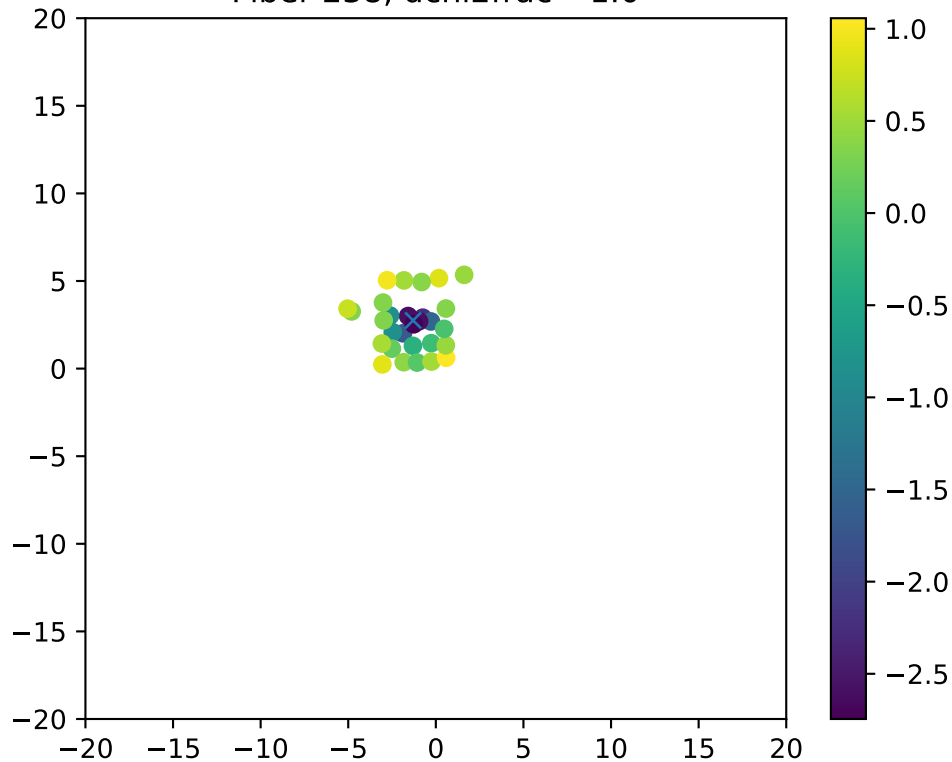
Fiber 238, dchi2frac= 1.0
