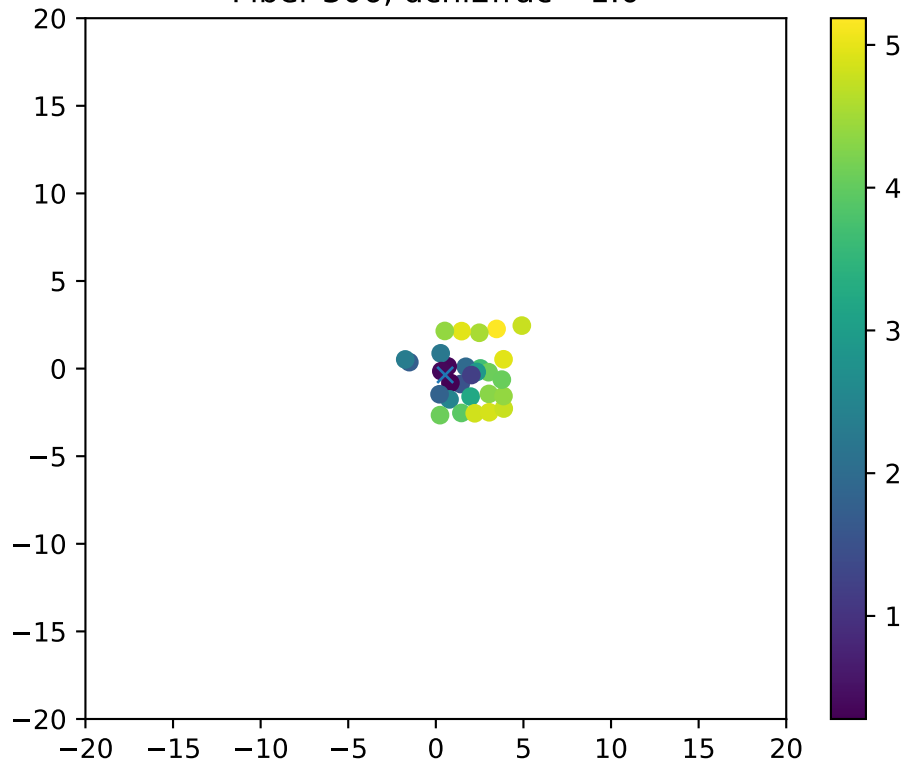
Fiber 306, dchi2frac= 1.0
