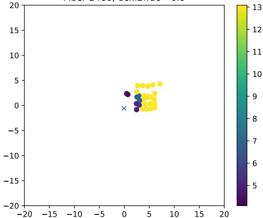
Fiber 2466, dchi2frac= 0.9
