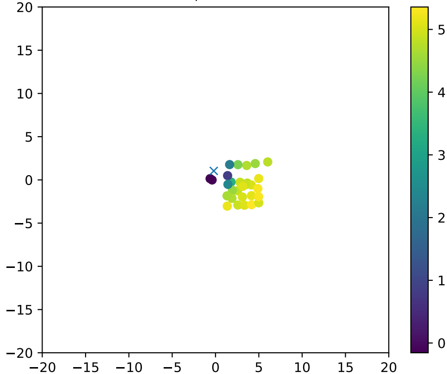
Fiber 4270, dchi2frac= 1.0
