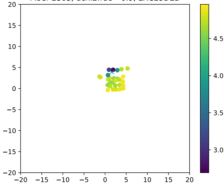
Fiber 2303, dchi2frac= 0.9, EXCLUDED
