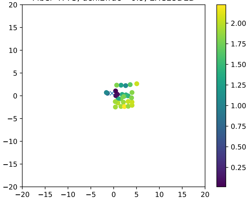
Fiber 4773, dchi2frac= 0.9, EXCLUDED
