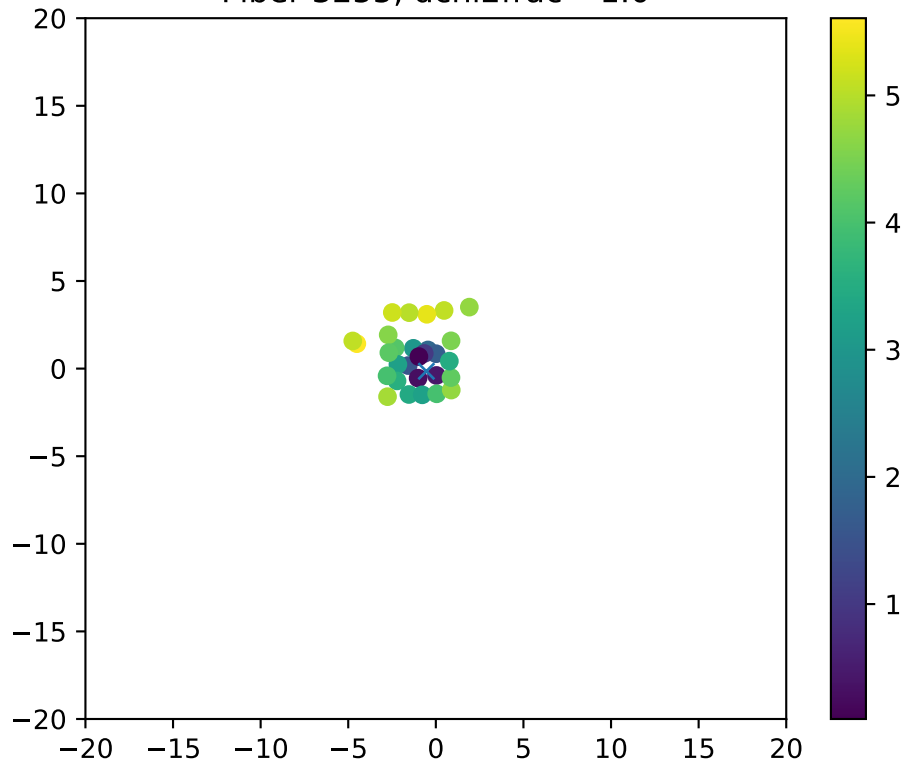
Fiber 3255, dchi2frac= 1.0
