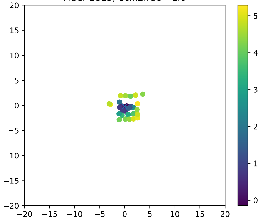
Fiber 1813, dchi2frac= 1.0
