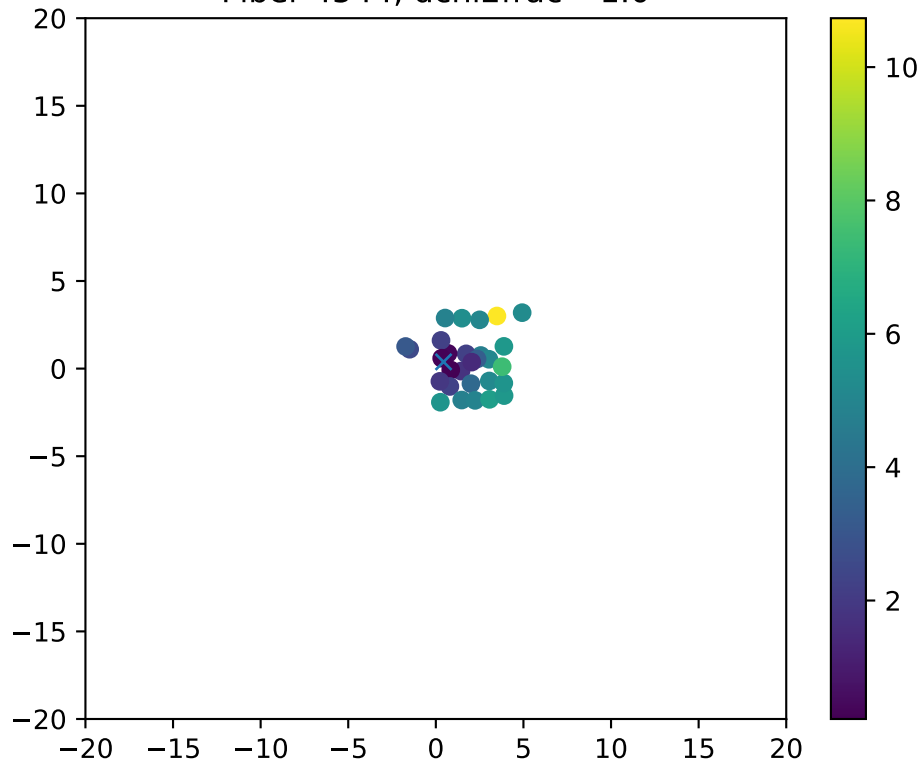
Fiber 4544, dchi2frac= 1.0
