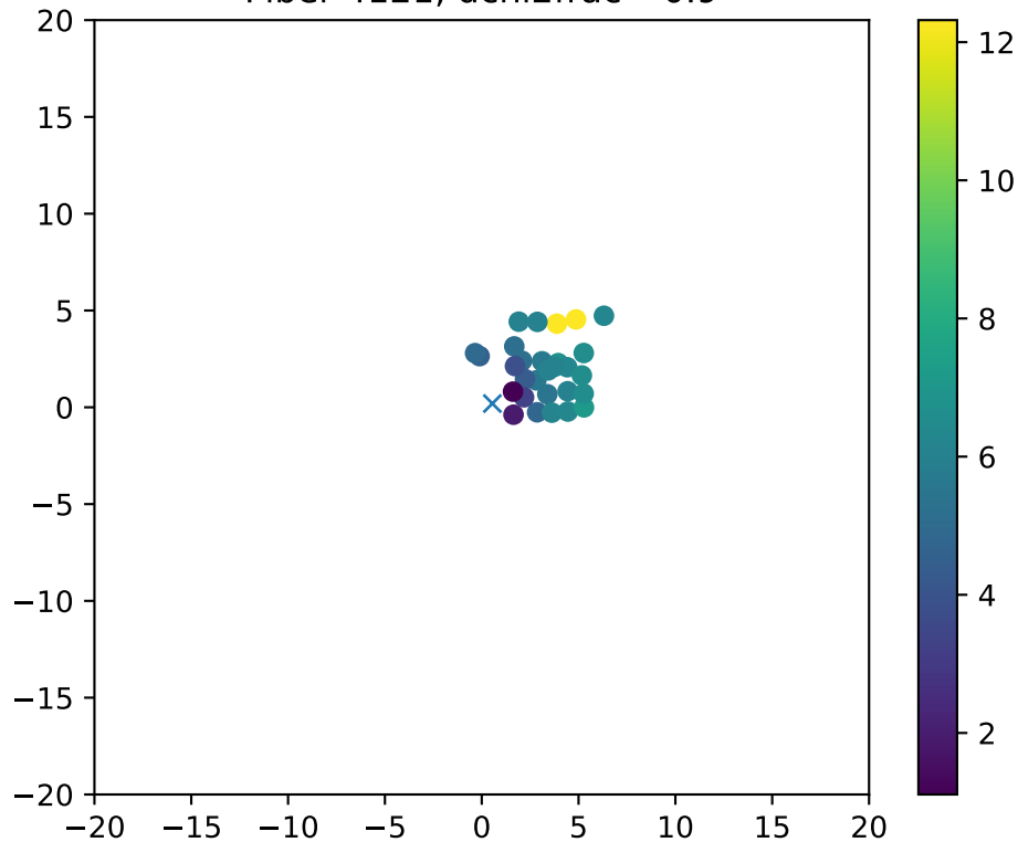
Fiber 4121, dchi2frac= 0.9
