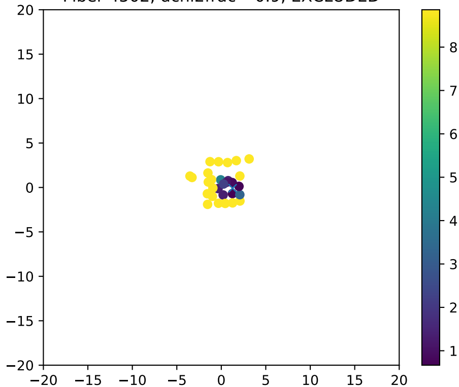
Fiber 4502, dchi2frac= 0.9, EXCLUDED
