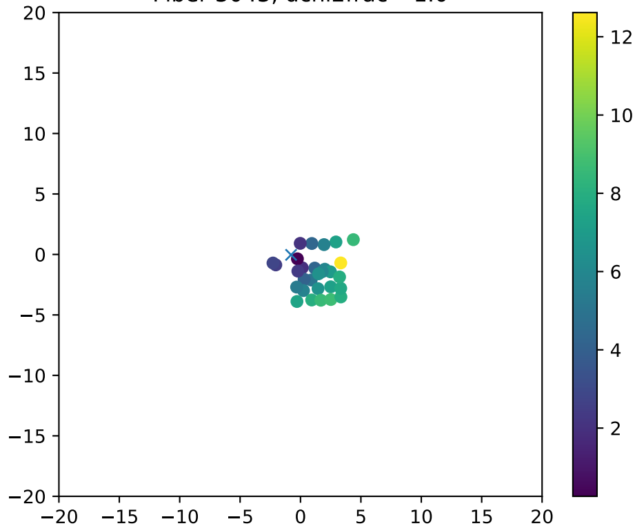
Fiber 3043, dchi2frac= 1.0
