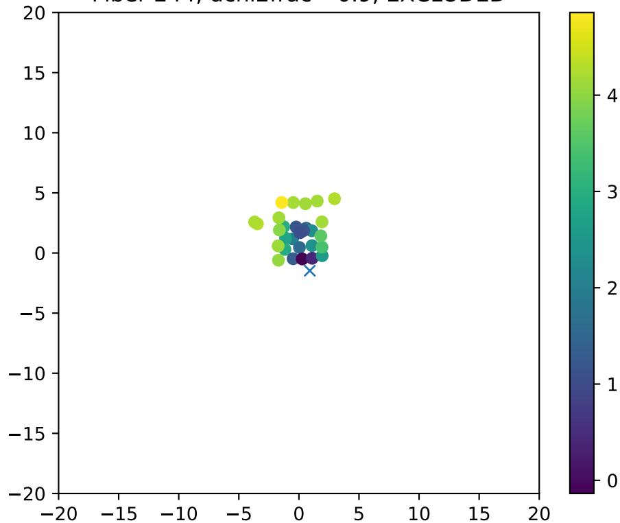
Fiber 244, dchi2frac= 0.9, EXCLUDED
