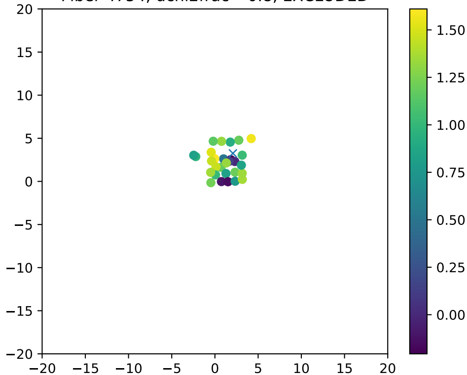
Fiber 4754, dchi2frac= 0.8, EXCLUDED
