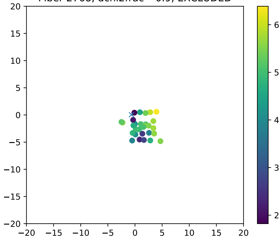
Fiber 2768, dchi2frac= 0.9, EXCLUDED
