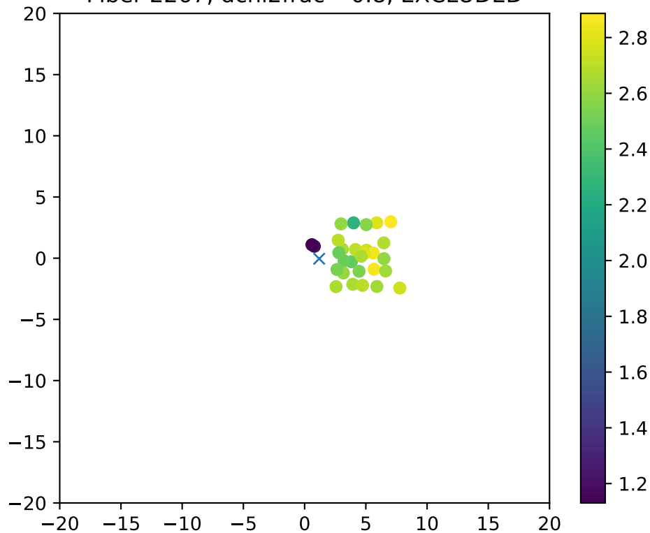
Fiber 2267, dchi2frac= 0.8, EXCLUDED
