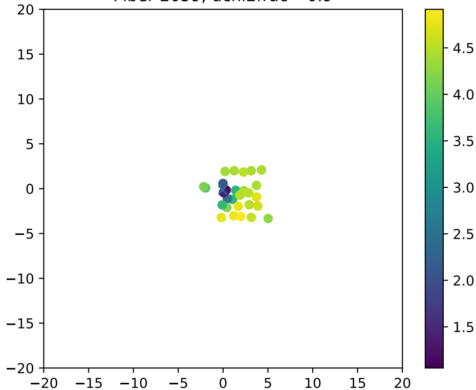
Fiber 2059, dchi2frac= 0.9
