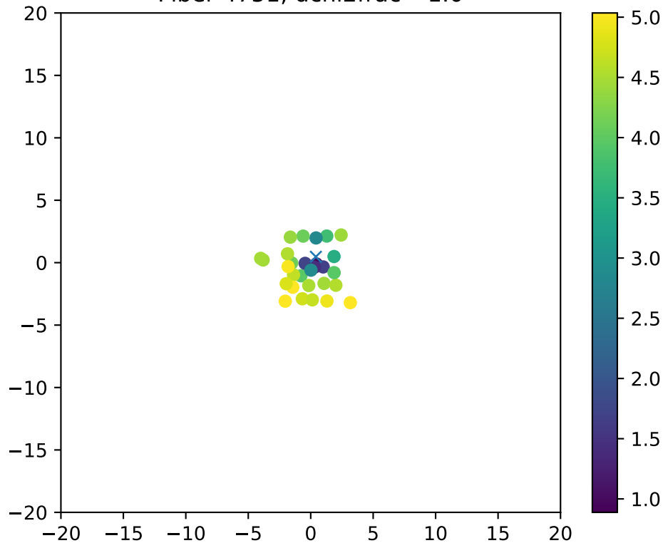
Fiber 4751, dchi2frac= 1.0
