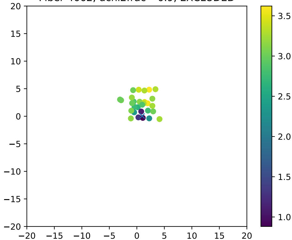
Fiber 4662, dchi2frac= 0.9, EXCLUDED
