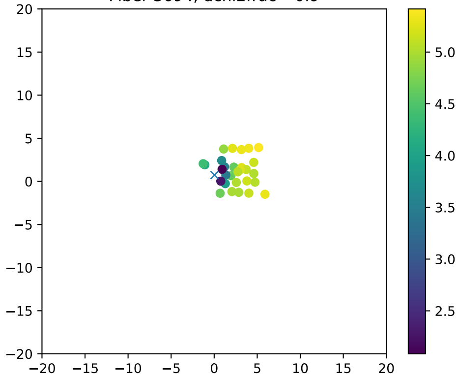
Fiber 3694, dchi2frac= 0.9
