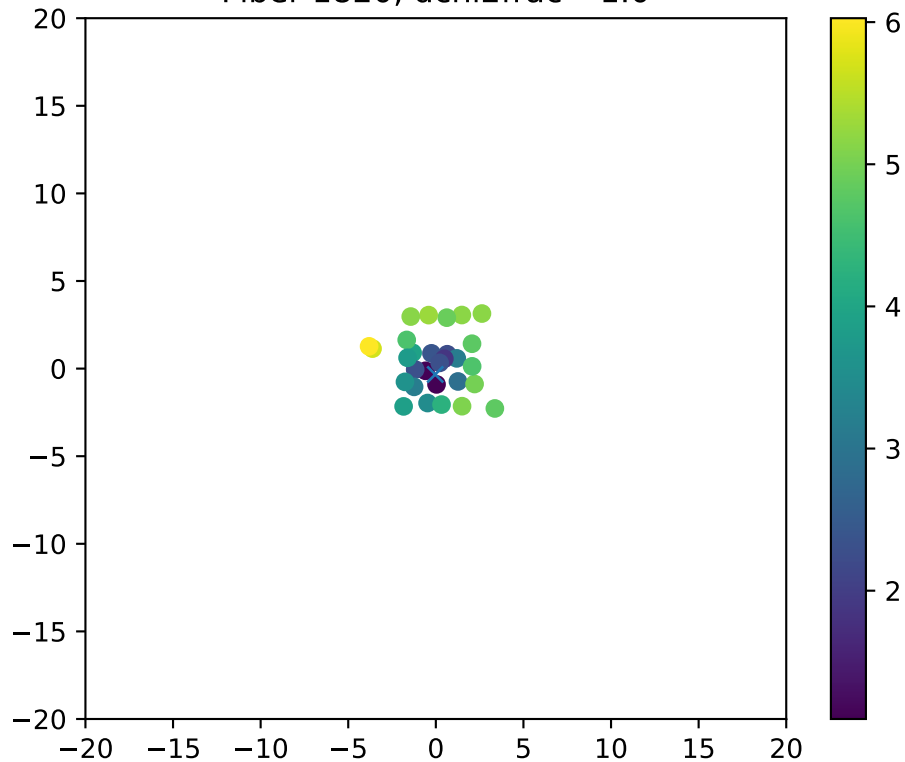
Fiber 1820, dchi2frac= 1.0
