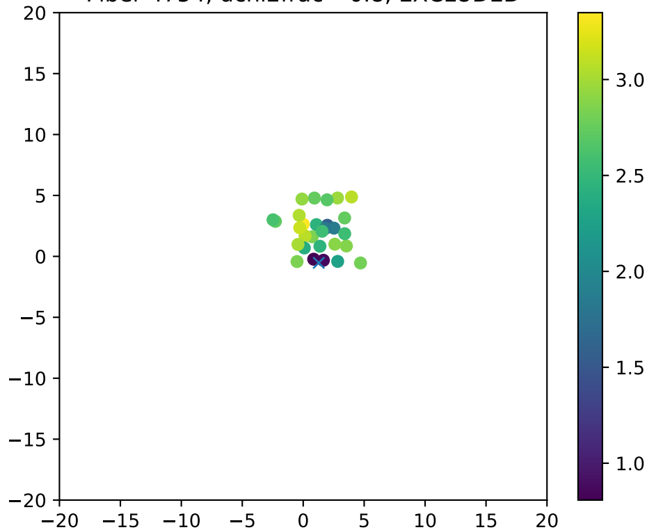
Fiber 4754, dchi2frac= 0.8, EXCLUDED
