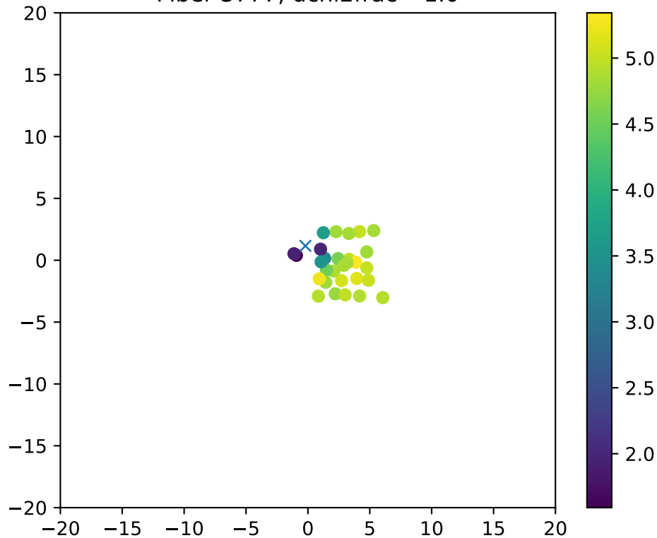
Fiber 3777, dchi2frac= 1.0
