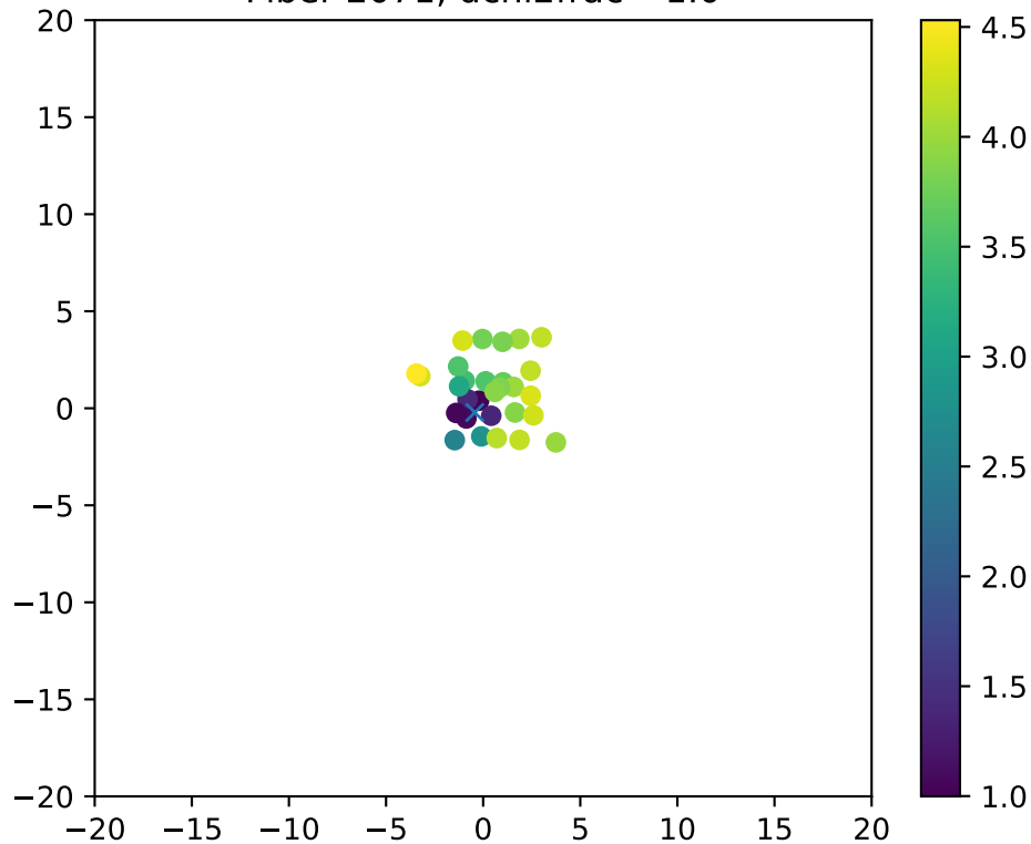
Fiber 2071, dchi2frac= 1.0
