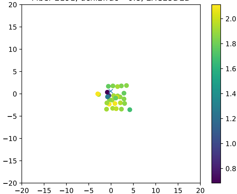
Fiber 2191, dchi2frac= 0.8, EXCLUDED
