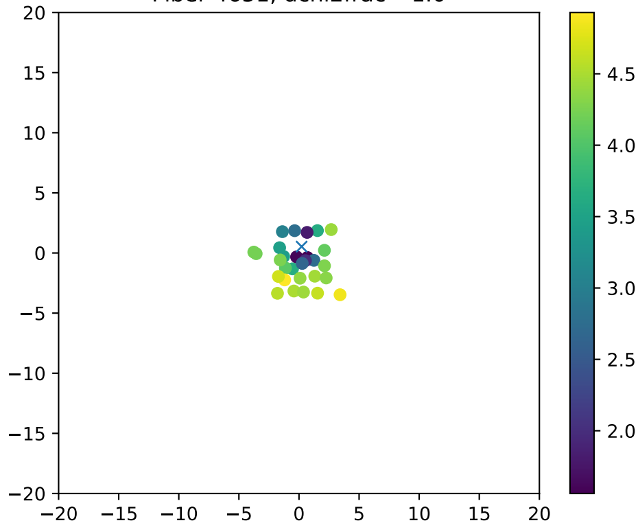
Fiber 4651, dchi2frac= 1.0
