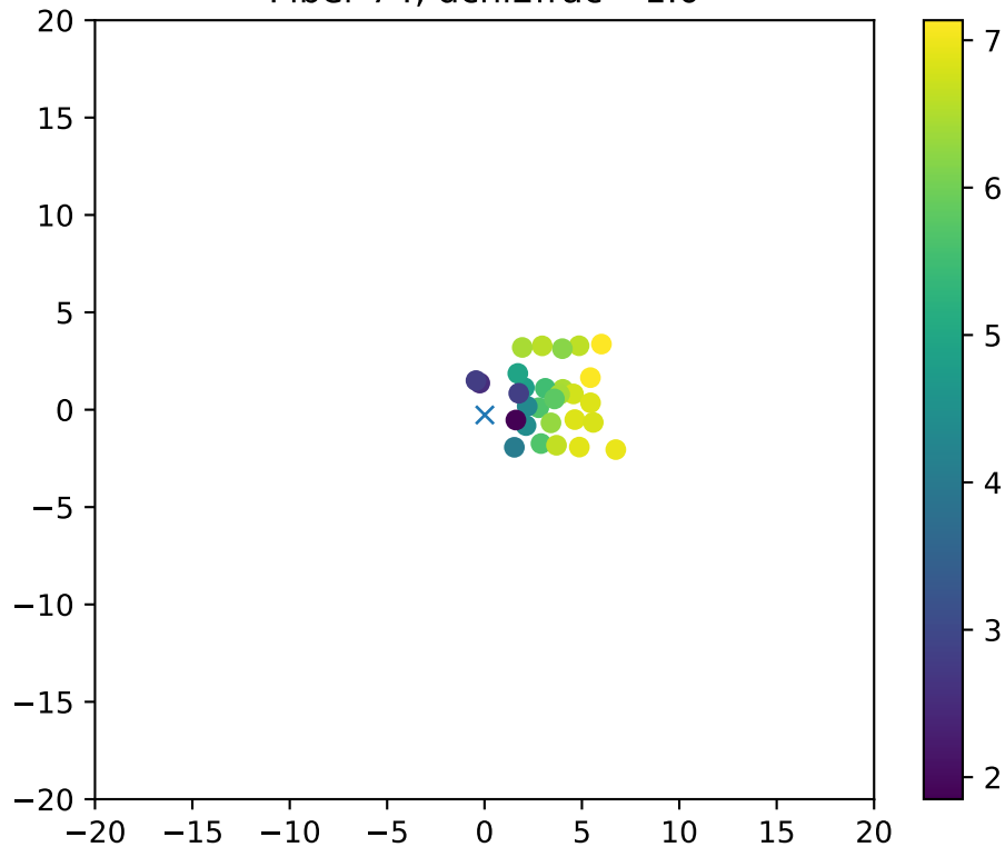
Fiber 74, dchi2frac= 1.0
