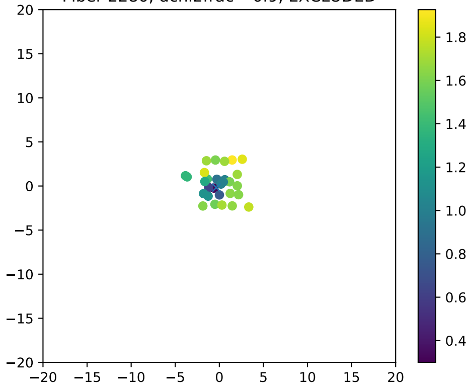
Fiber 2280, dchi2frac= 0.9, EXCLUDED
