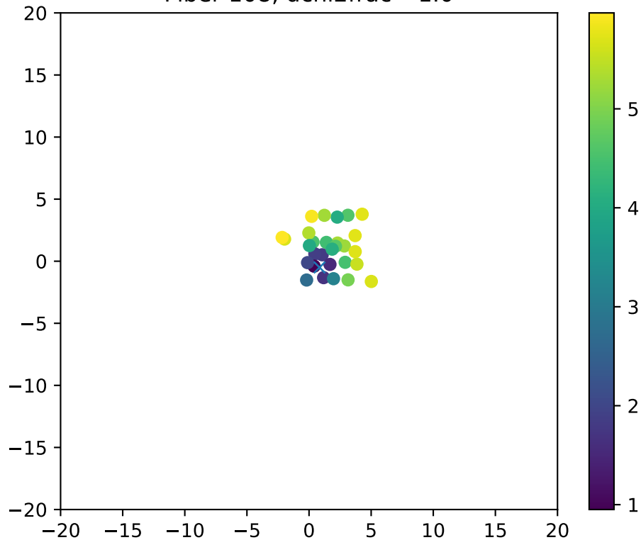
Fiber 108, dchi2frac= 1.0
