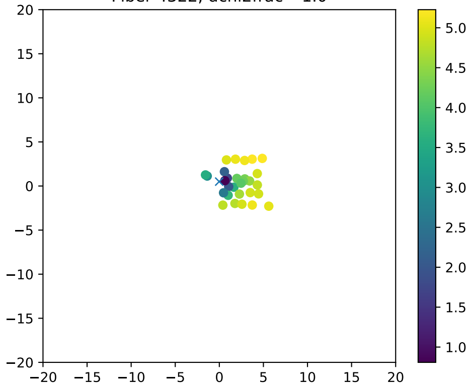
Fiber 4322, dchi2frac= 1.0
