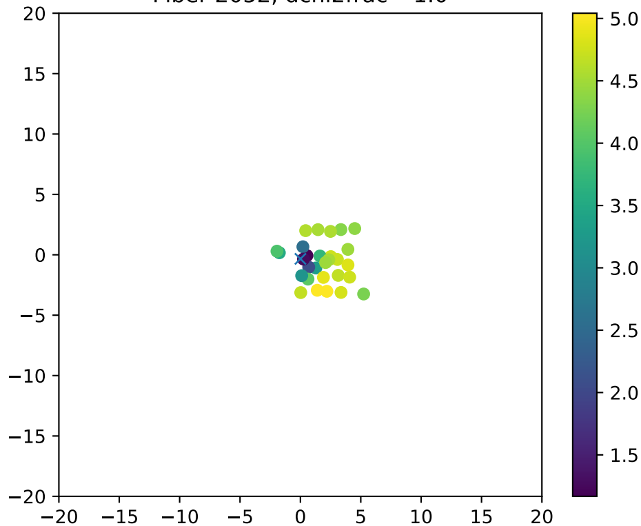
Fiber 2052, dchi2frac= 1.0
