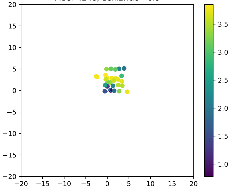
Fiber 4248, dchi2frac= 0.9
