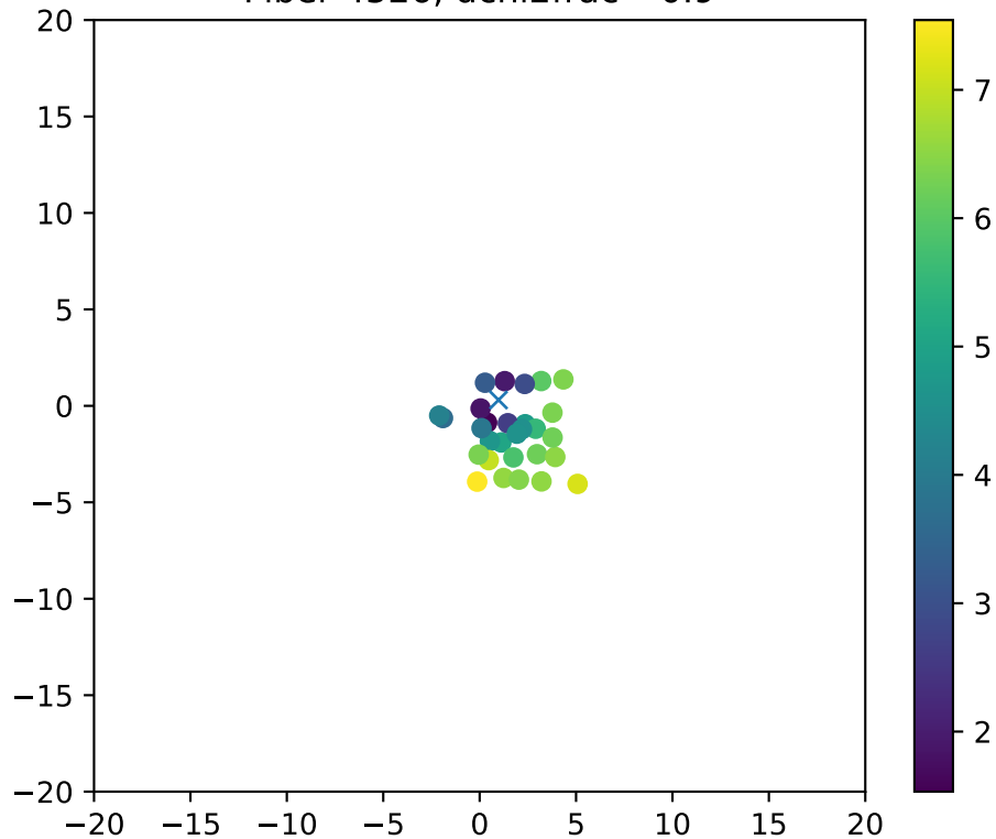
Fiber 4526, dchi2frac= 0.9
