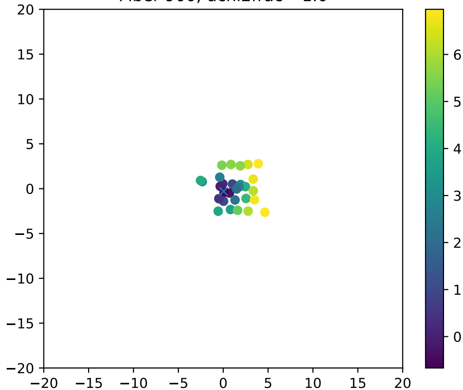
Fiber 900, dchi2frac= 1.0
