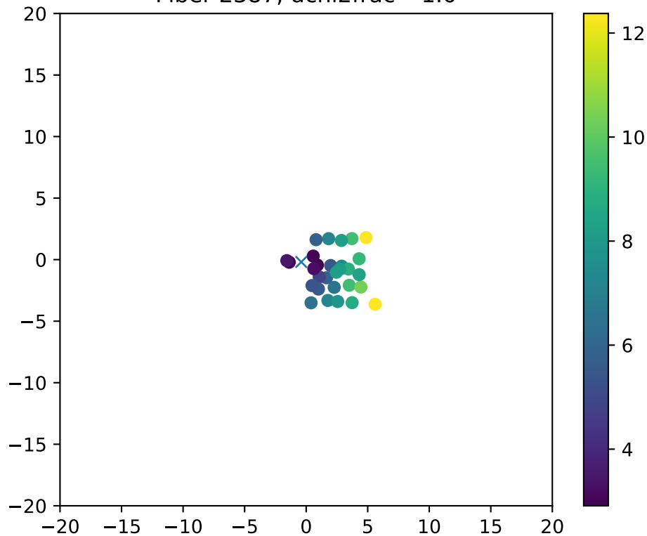
Fiber 2387, dchi2frac= 1.0
