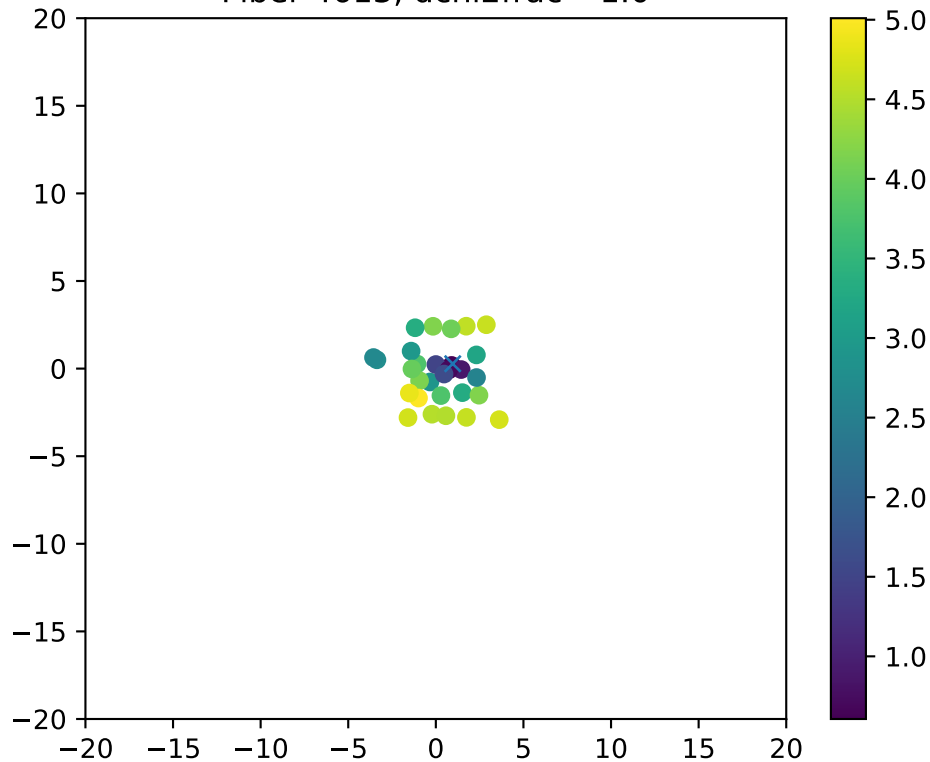
Fiber 4613, dchi2frac= 1.0
