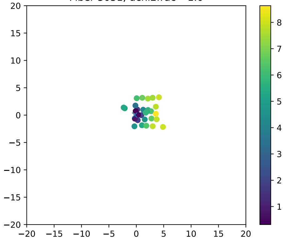
Fiber 3031, dchi2frac= 1.0
