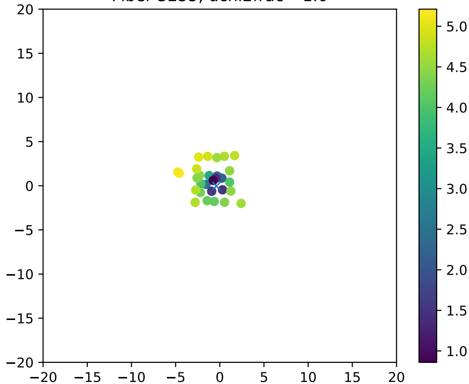
Fiber 3255, dchi2frac= 1.0
