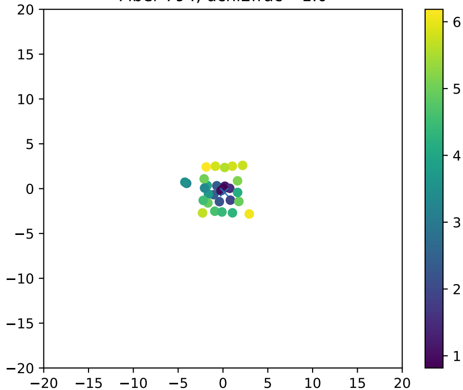
Fiber 794, dchi2frac= 1.0
