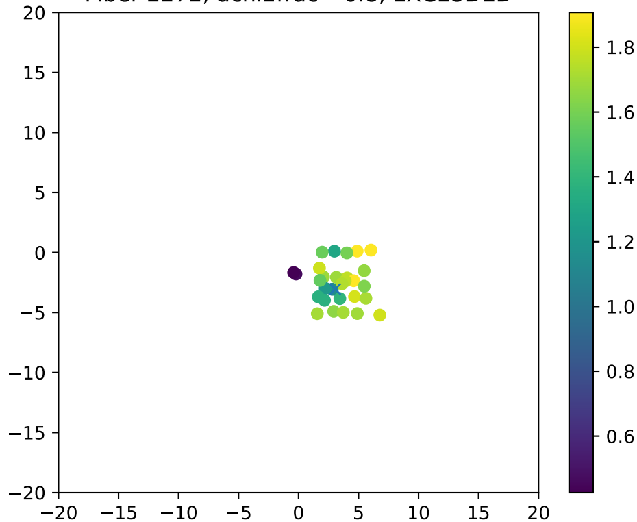
Fiber 2272, dchi2frac= 0.8, EXCLUDED
