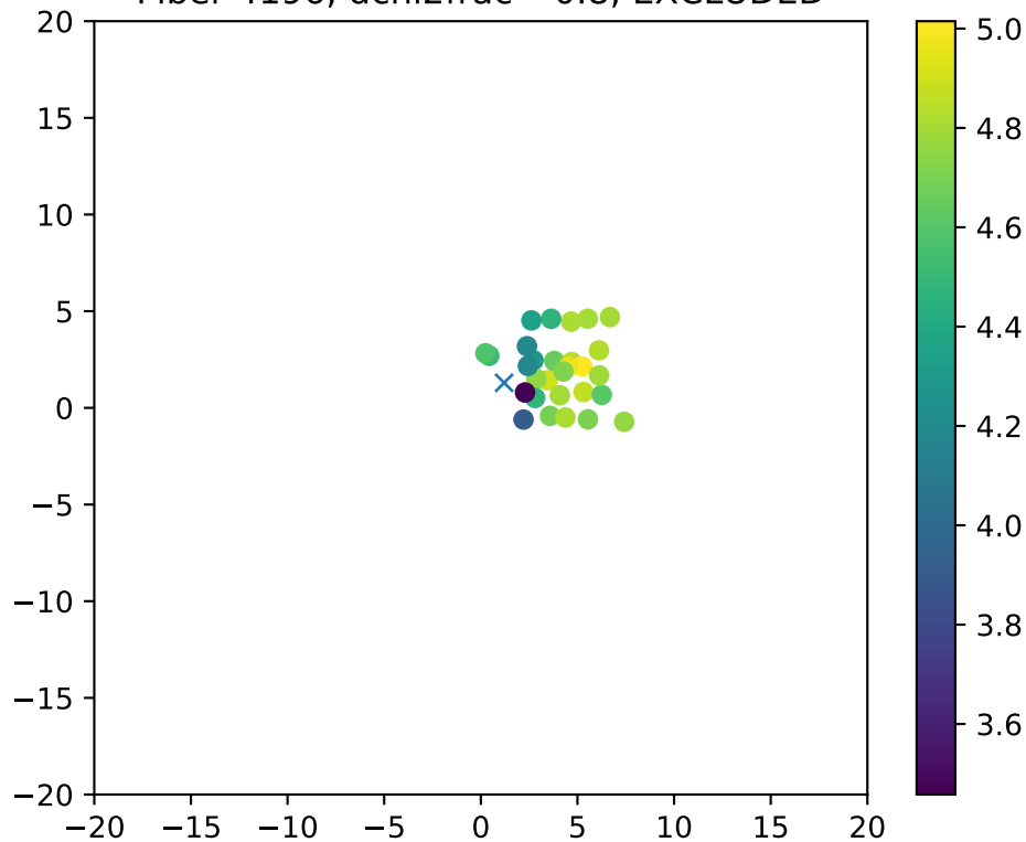
Fiber 4196, dchi2frac= 0.8, EXCLUDED
