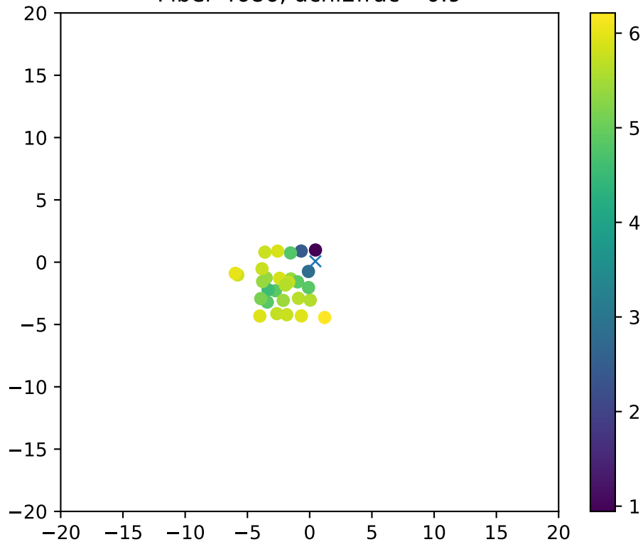
Fiber 4686, dchi2frac= 0.9
