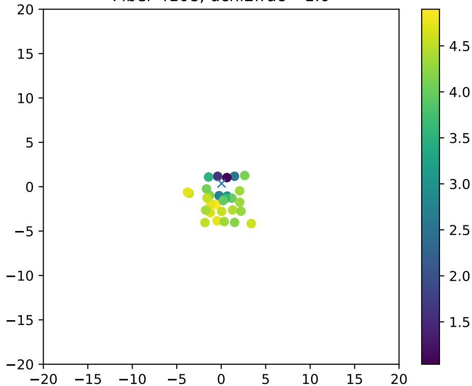
Fiber 4108, dchi2frac= 1.0
