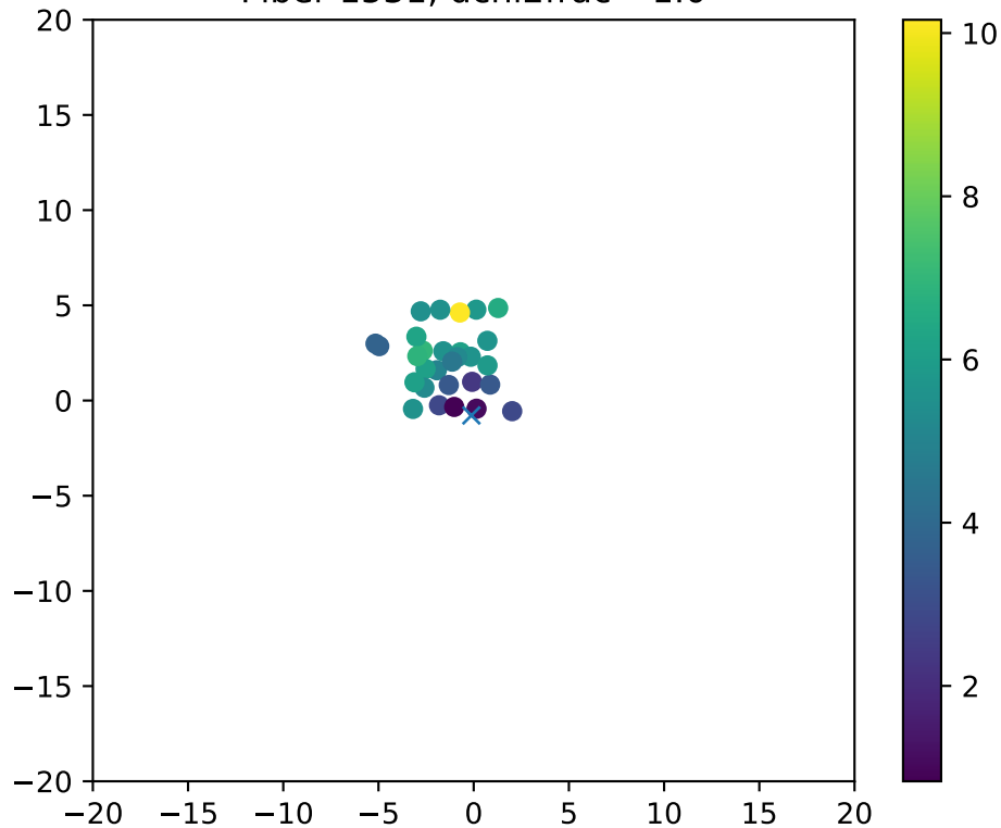
Fiber 1531, dchi2frac= 1.0
