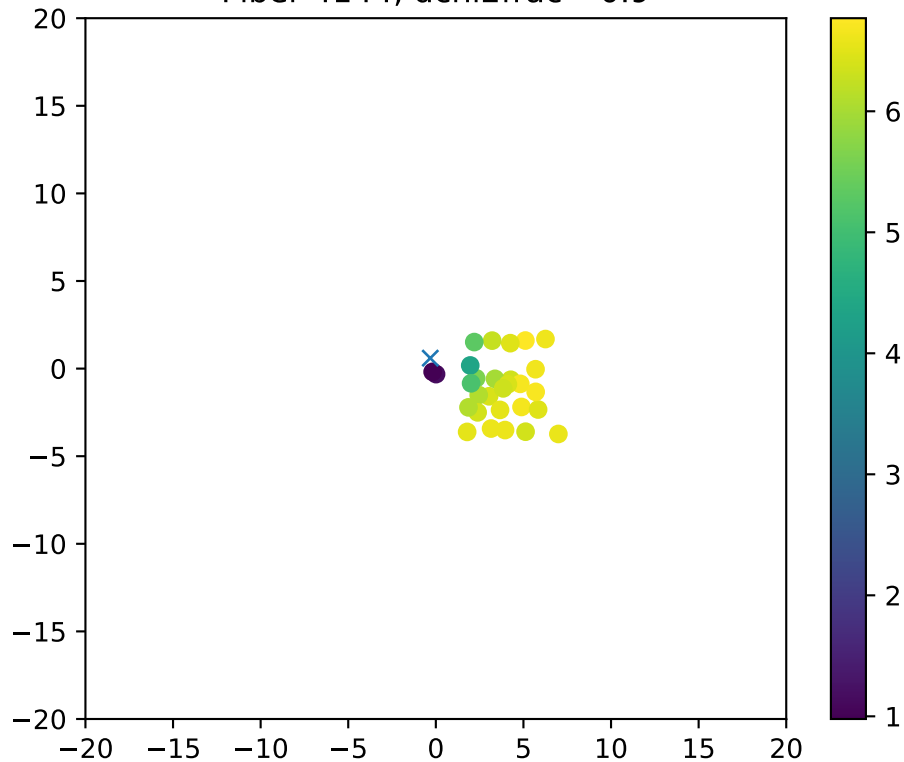
Fiber 4144, dchi2frac= 0.9
