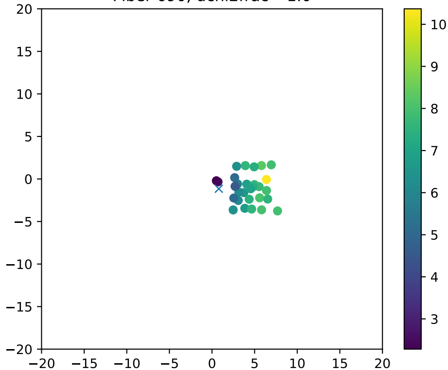
Fiber 690, dchi2frac= 1.0
