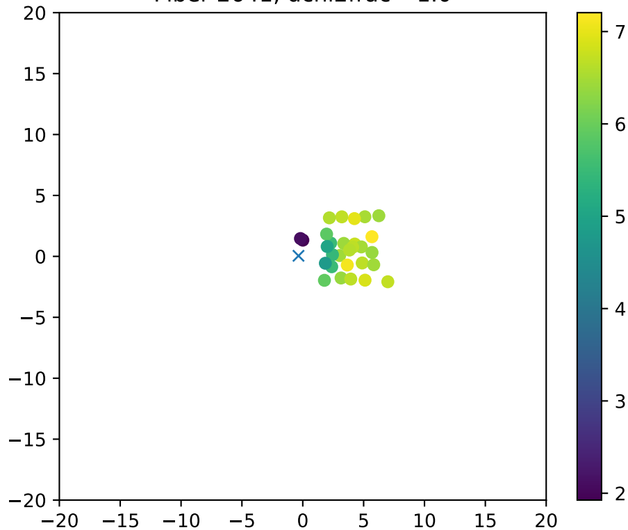
Fiber 2641, dchi2frac= 1.0
