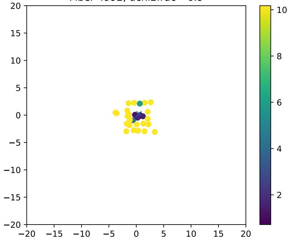
Fiber 4992, dchi2frac= 0.9
