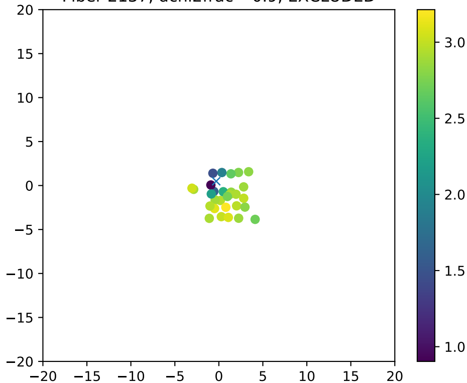
Fiber 2137, dchi2frac= 0.9, EXCLUDED
