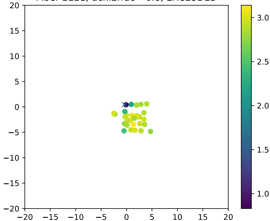
Fiber 2121, dchi2frac= 0.8, EXCLUDED
