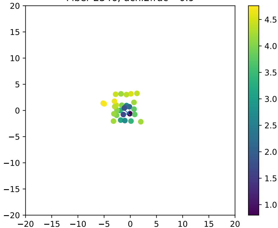
Fiber 2346, dchi2frac= 0.9
