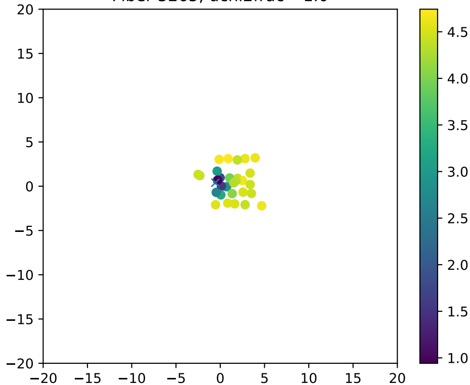
Fiber 3265, dchi2frac= 1.0
