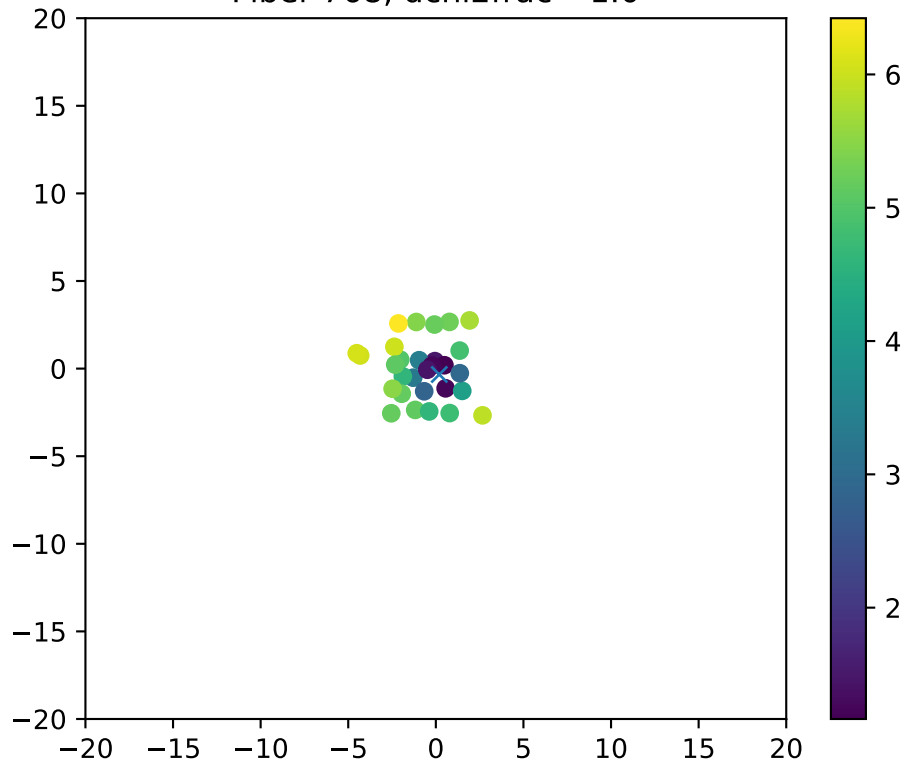
Fiber 768, dchi2frac= 1.0
