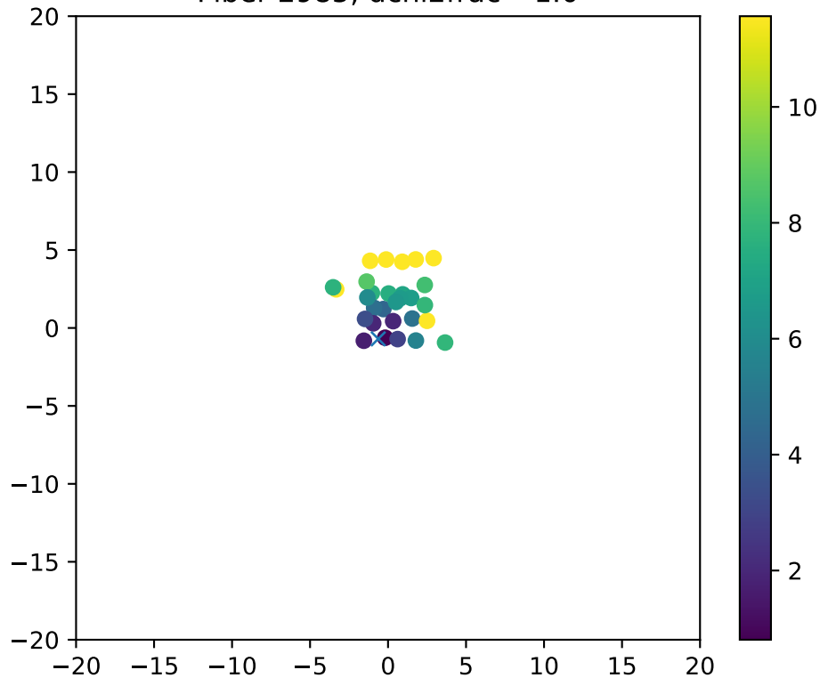
Fiber 2985, dchi2frac= 1.0
