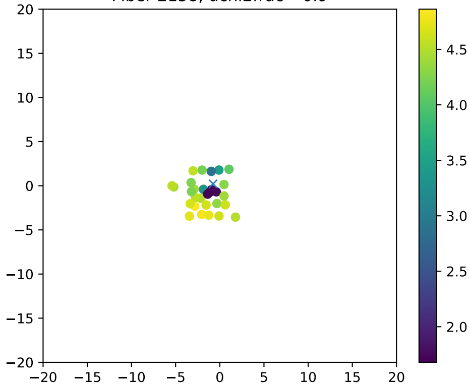
Fiber 2158, dchi2frac= 0.9
