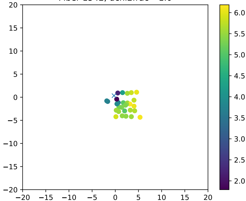
Fiber 1542, dchi2frac= 1.0
