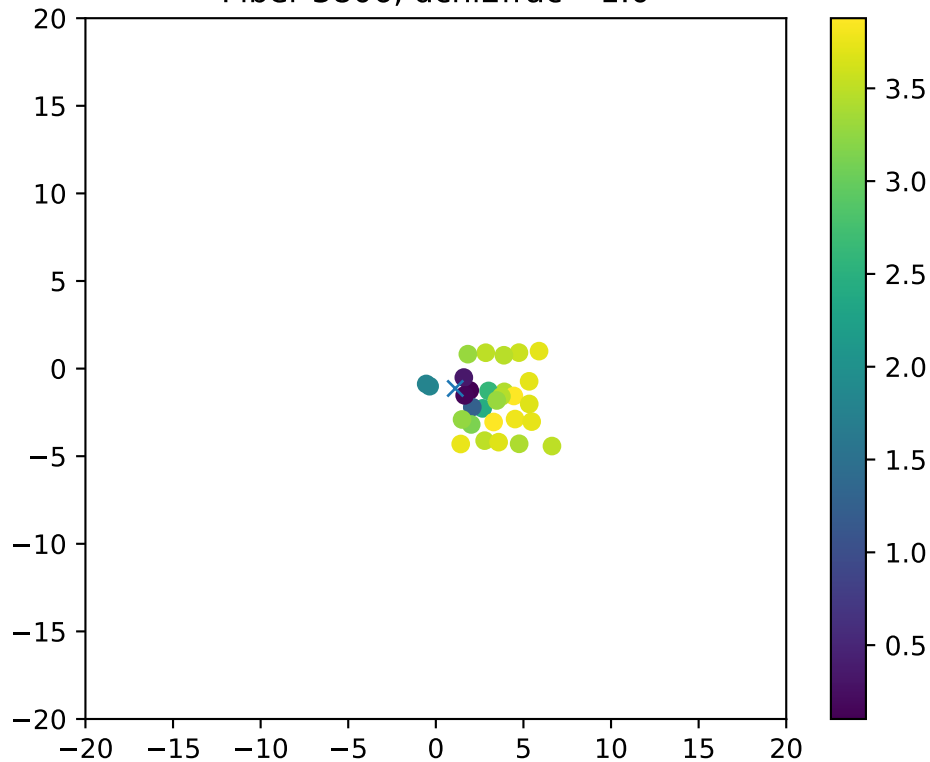
Fiber 3806, dchi2frac= 1.0
