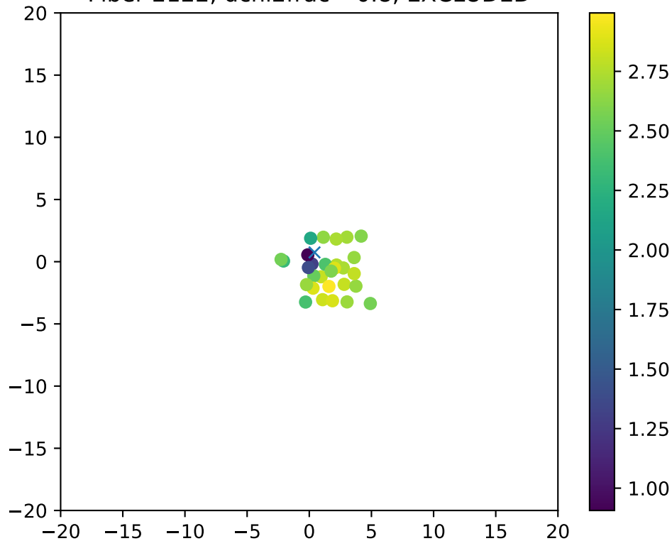
Fiber 2122, dchi2frac= 0.8, EXCLUDED
