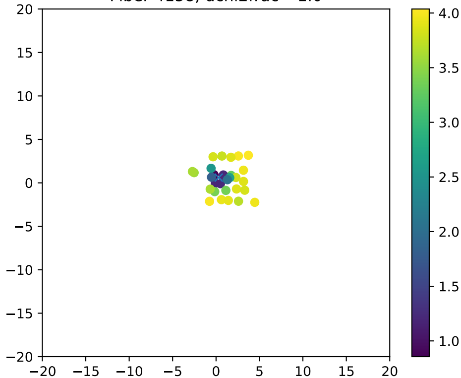
Fiber 4158, dchi2frac= 1.0
