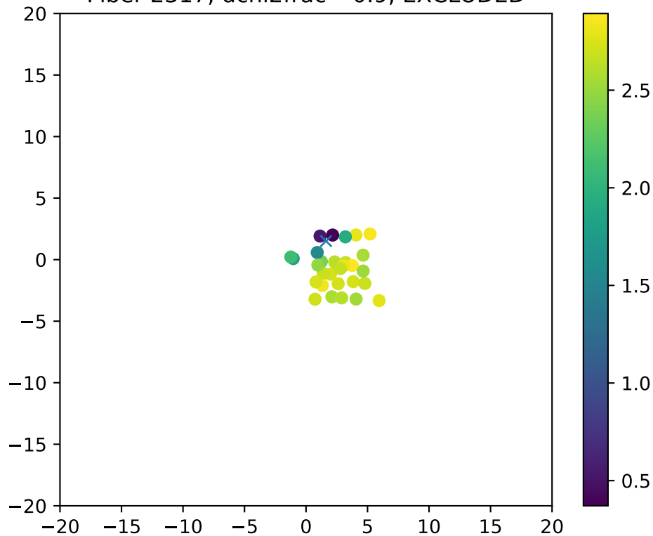
Fiber 2317, dchi2frac= 0.9, EXCLUDED
