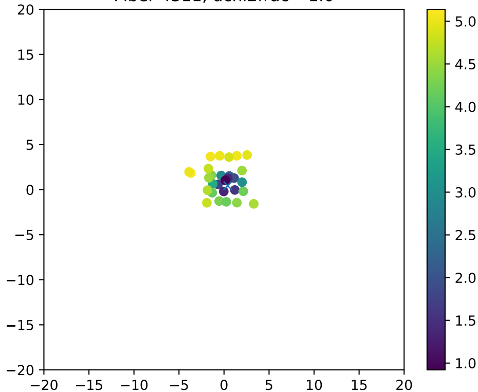
Fiber 4311, dchi2frac= 1.0
