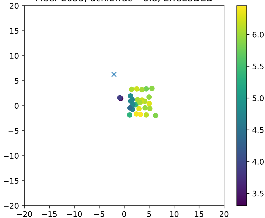
Fiber 2055, dchi2frac= 0.8, EXCLUDED
