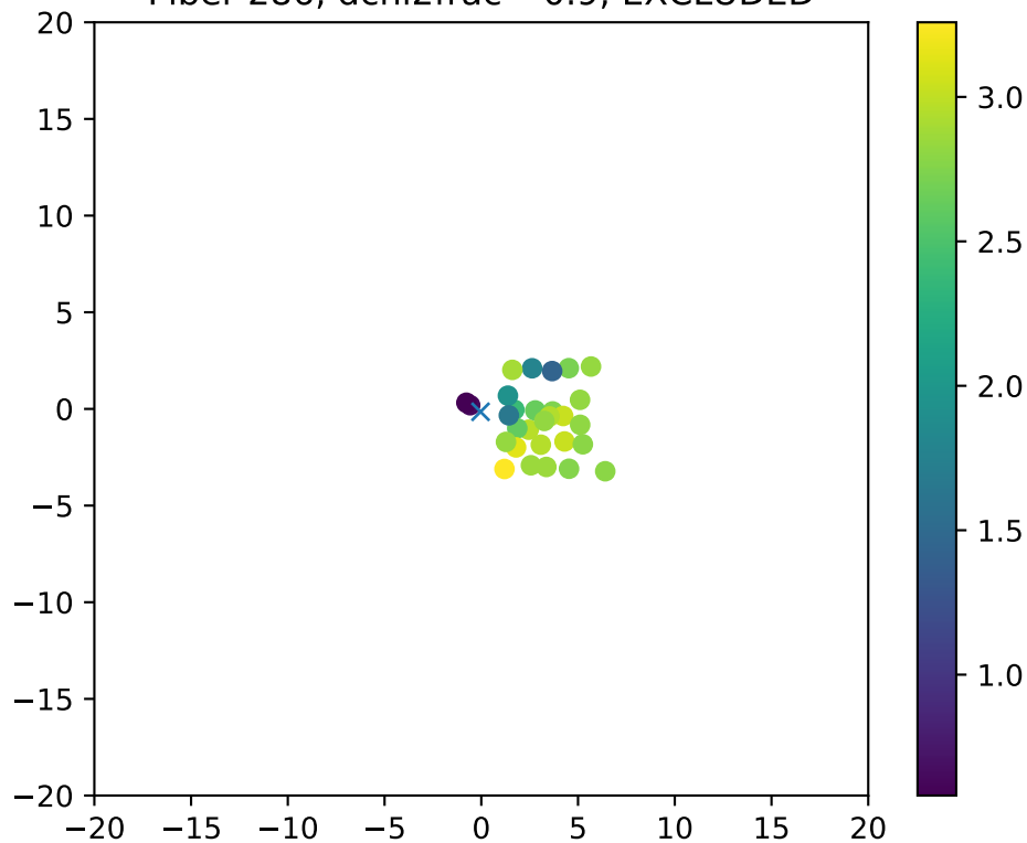
Fiber 286, dchi2frac= 0.9, EXCLUDED
