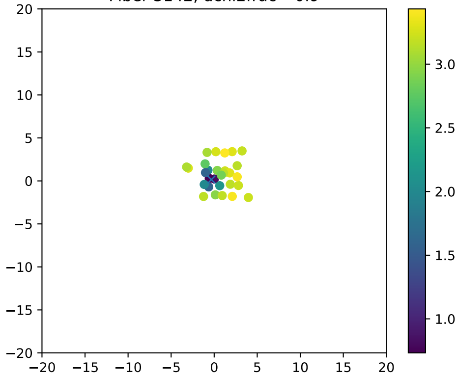
Fiber 3142, dchi2frac= 0.9
