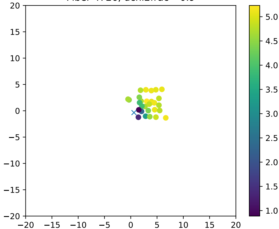
Fiber 4726, dchi2frac= 0.9
