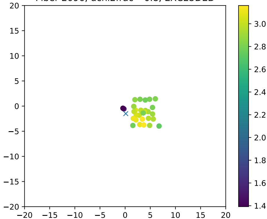
Fiber 2096, dchi2frac= 0.8, EXCLUDED
