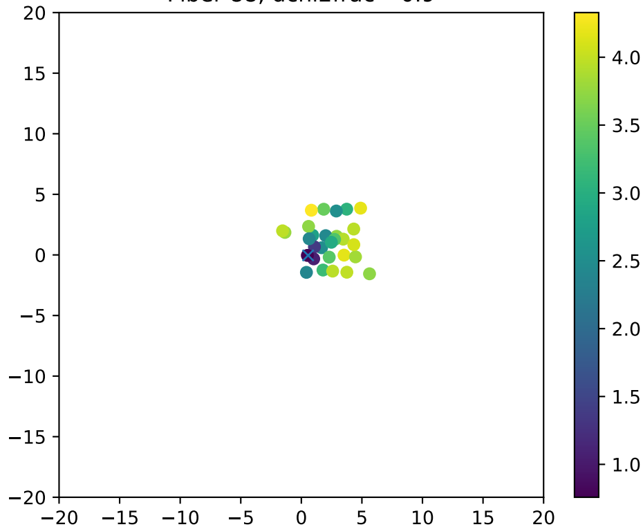
Fiber 88, dchi2frac= 0.9
