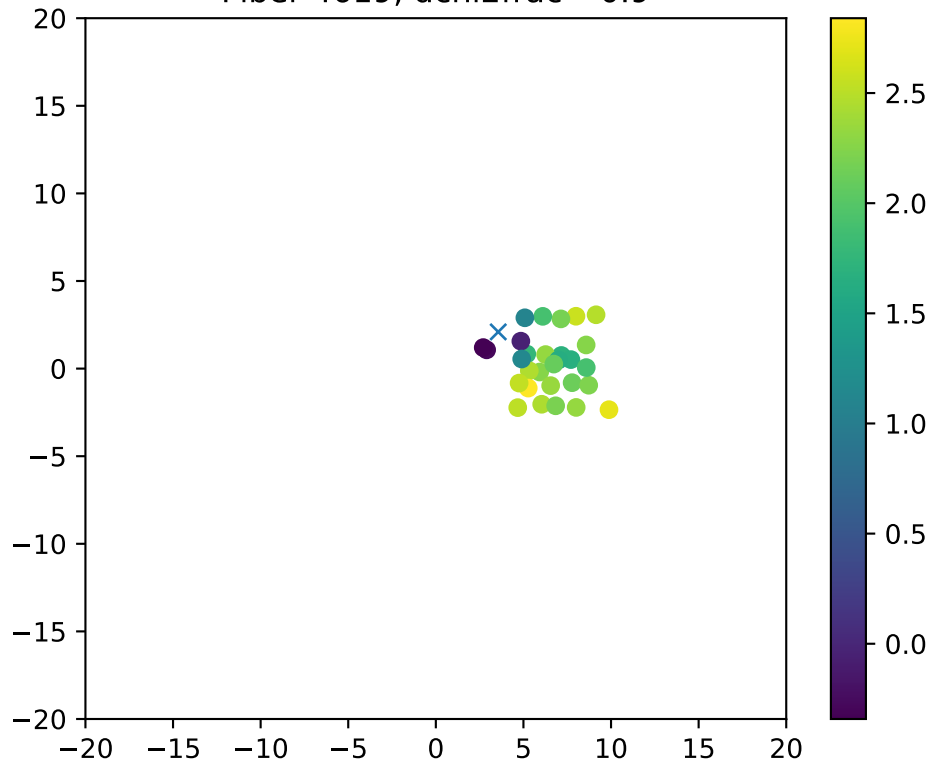
Fiber 4619, dchi2frac= 0.9
