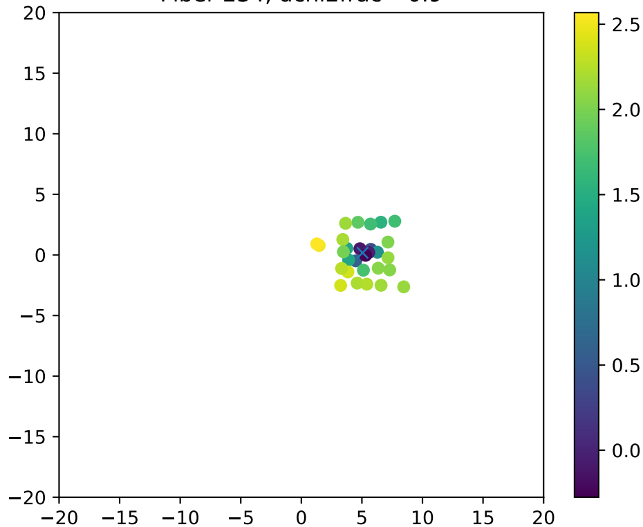
Fiber 234, dchi2frac= 0.9
