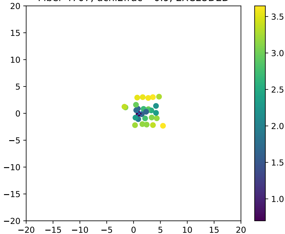
Fiber 4707, dchi2frac= 0.9, EXCLUDED
