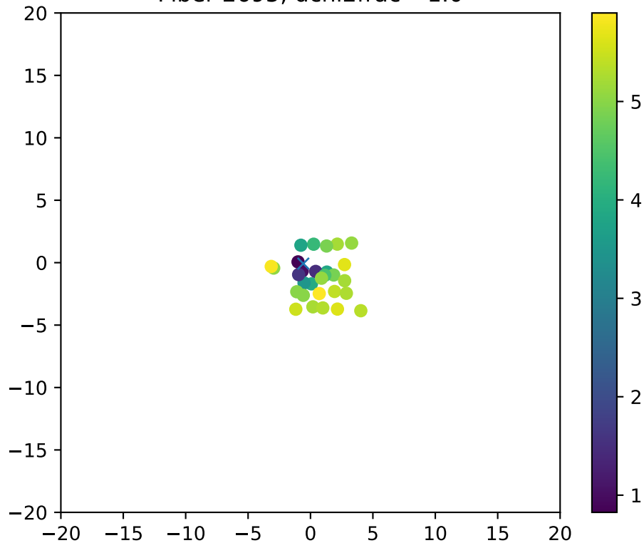
Fiber 2695, dchi2frac= 1.0
