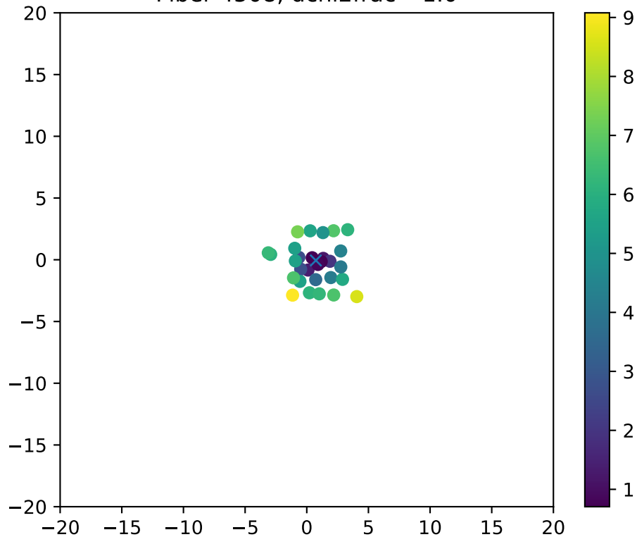
Fiber 4508, dchi2frac= 1.0
