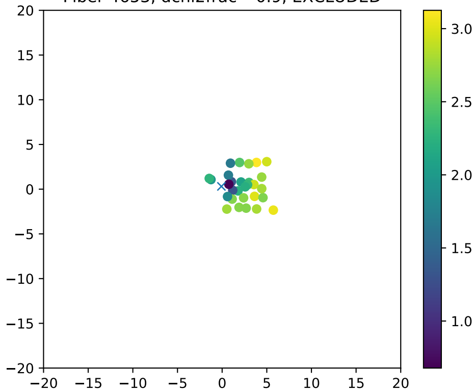
Fiber 4653, dchi2frac= 0.9, EXCLUDED
