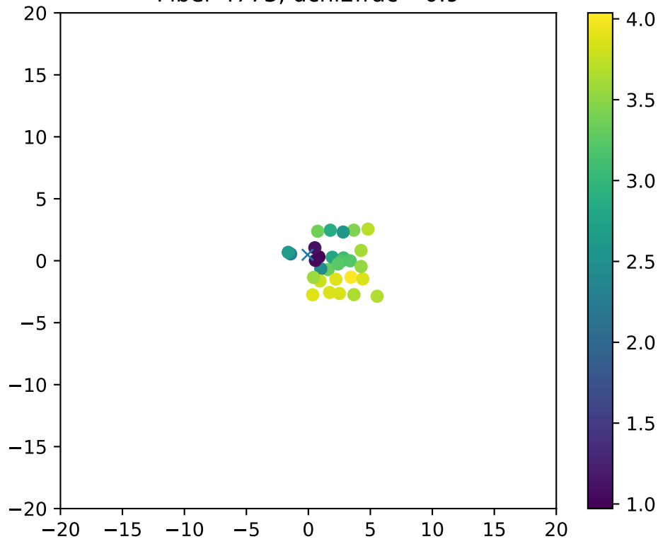
Fiber 4773, dchi2frac= 0.9
