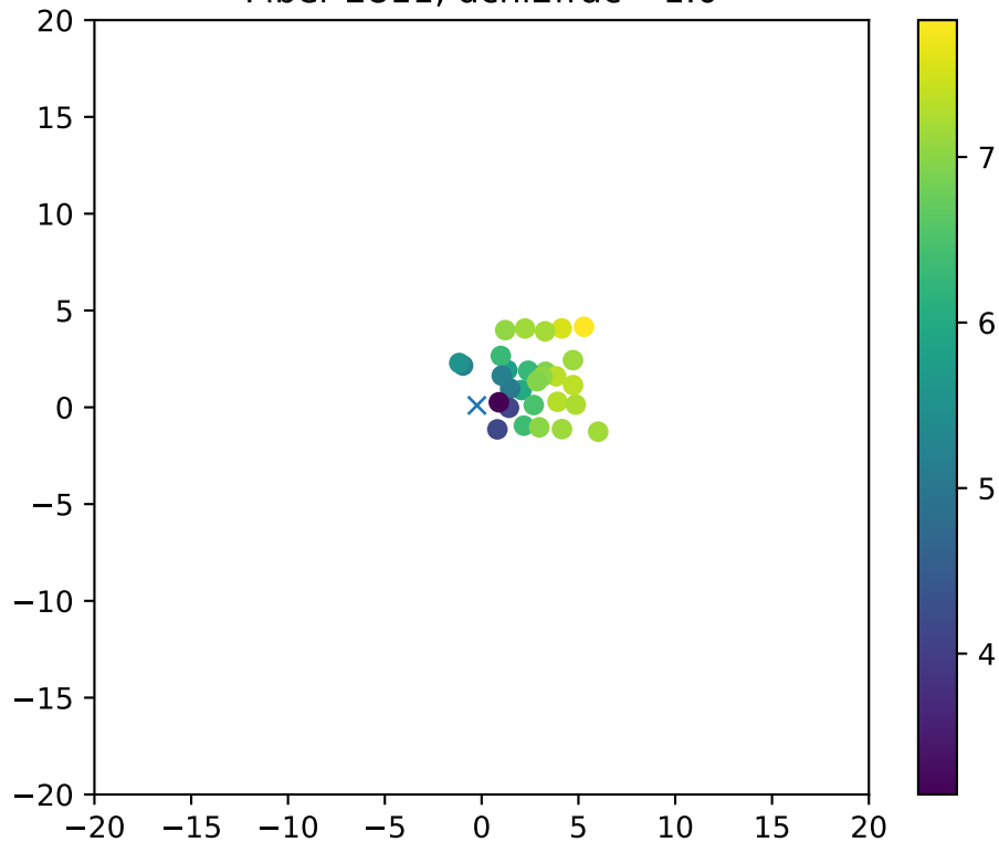
Fiber 2811, dchi2frac= 1.0
