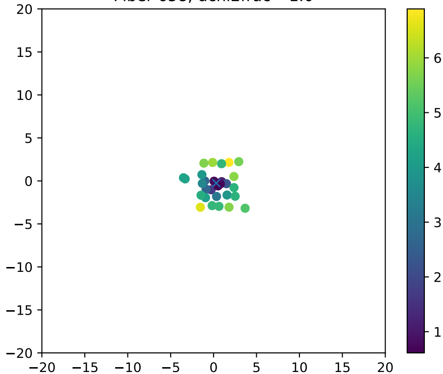
Fiber 658, dchi2frac= 1.0
