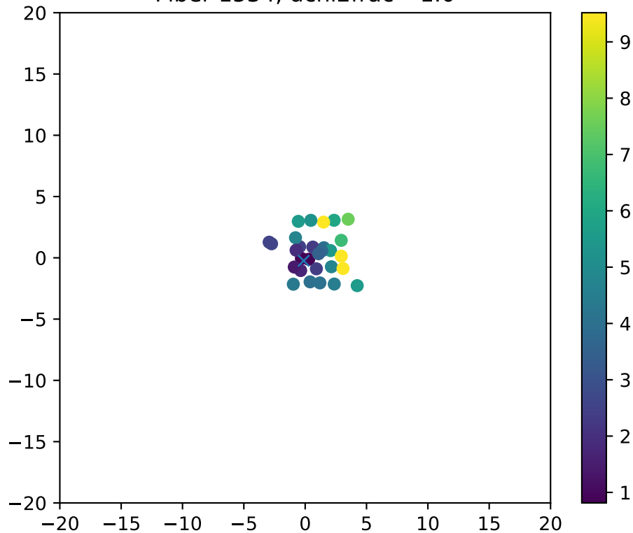
Fiber 1534, dchi2frac= 1.0
