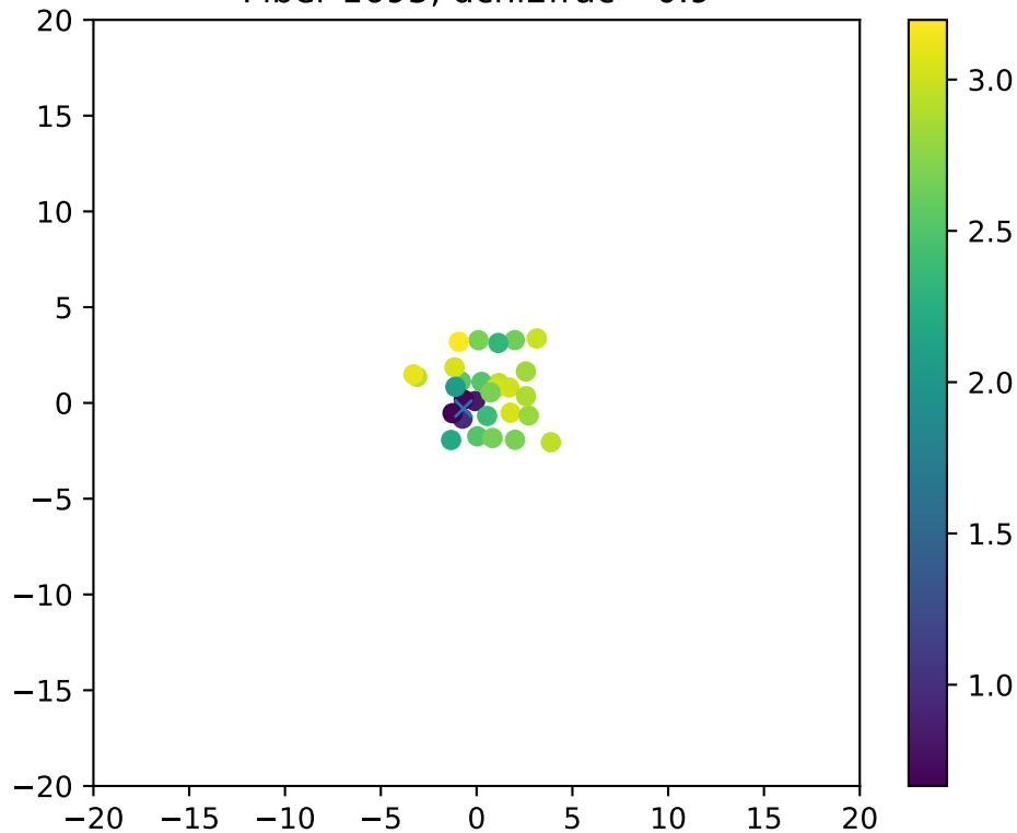
Fiber 1695, dchi2frac= 0.9
