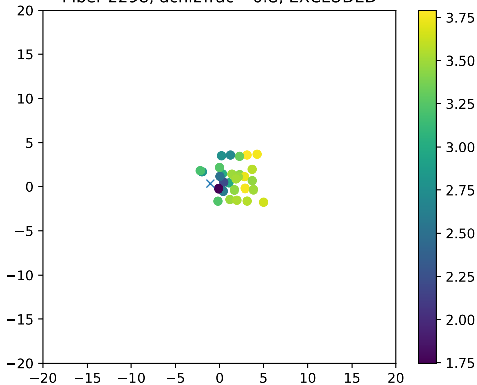
Fiber 2298, dchi2frac= 0.8, EXCLUDED
