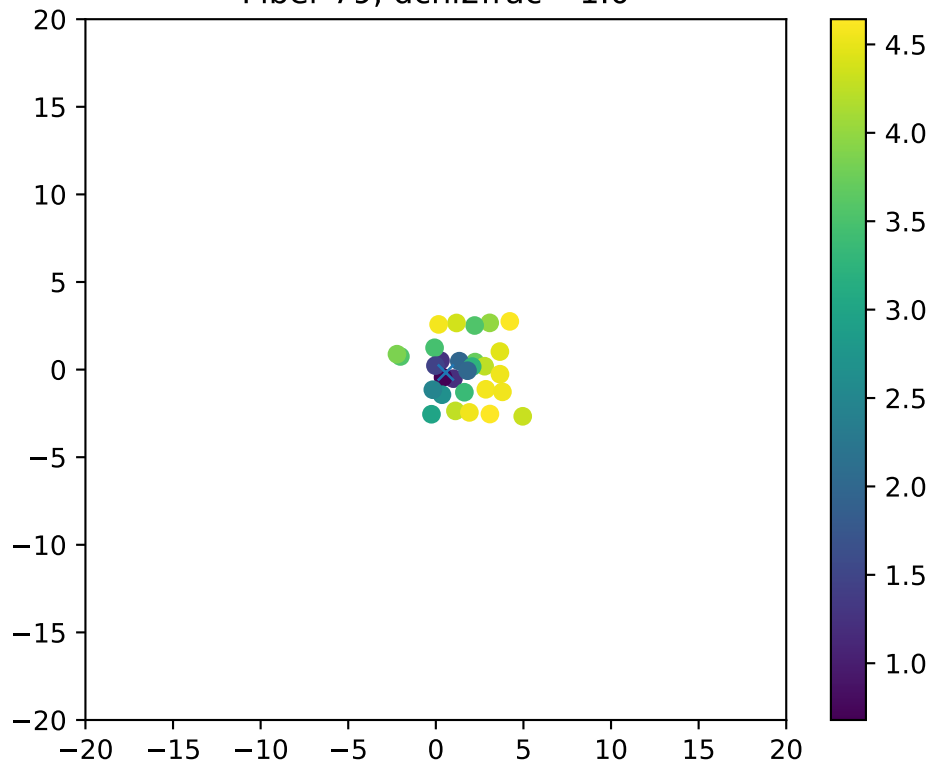
Fiber 79, dchi2frac= 1.0
