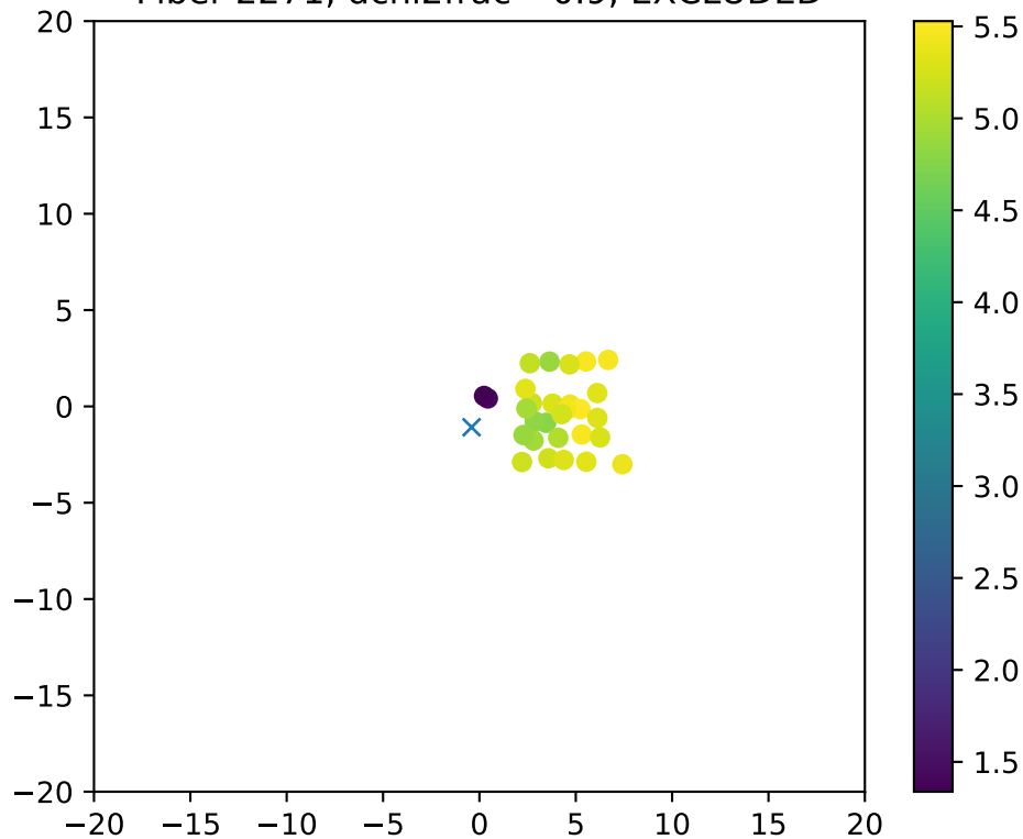
Fiber 2271, dchi2frac= 0.9, EXCLUDED
