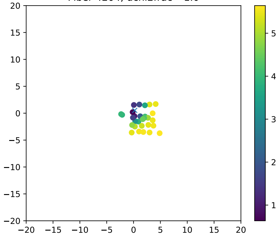
Fiber 4204, dchi2frac= 1.0
