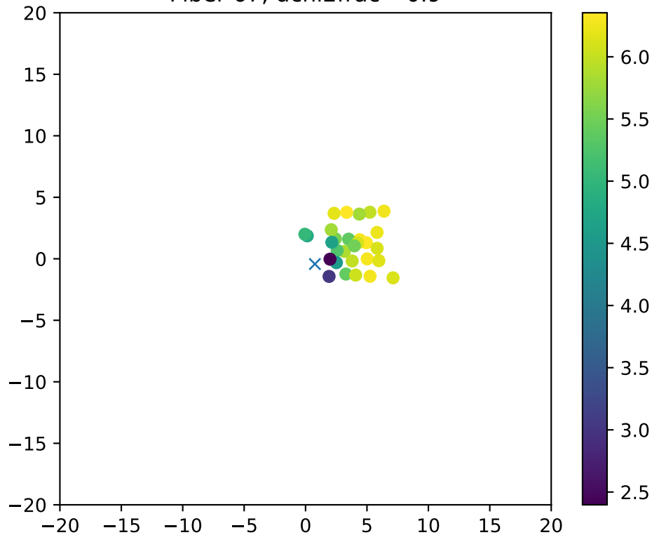
Fiber 67, dchi2frac= 0.9
