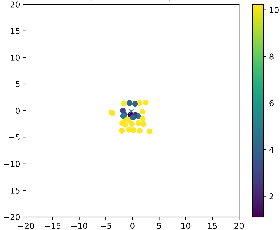
Fiber 2453, dchi2frac= 0.9, EXCLUDED
