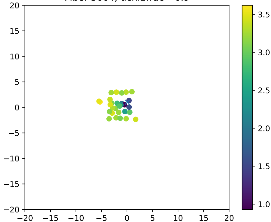
Fiber 3664, dchi2frac= 0.9
