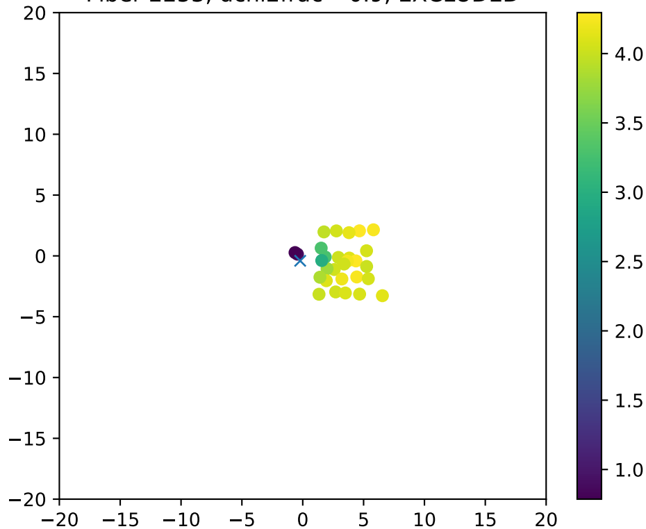
Fiber 2253, dchi2frac= 0.9, EXCLUDED
