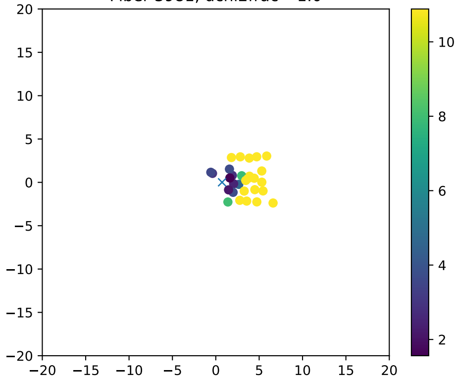
Fiber 3981, dchi2frac= 1.0
