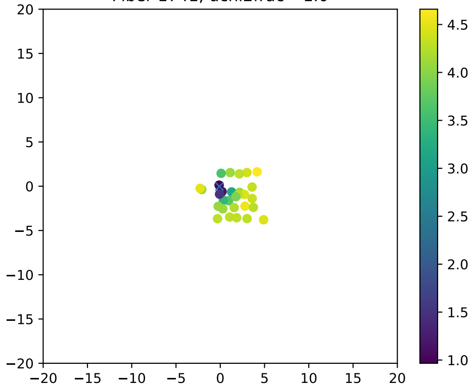
Fiber 1741, dchi2frac= 1.0
