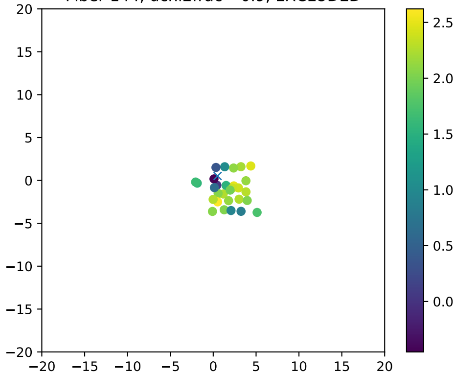
Fiber 144, dchi2frac= 0.9, EXCLUDED
