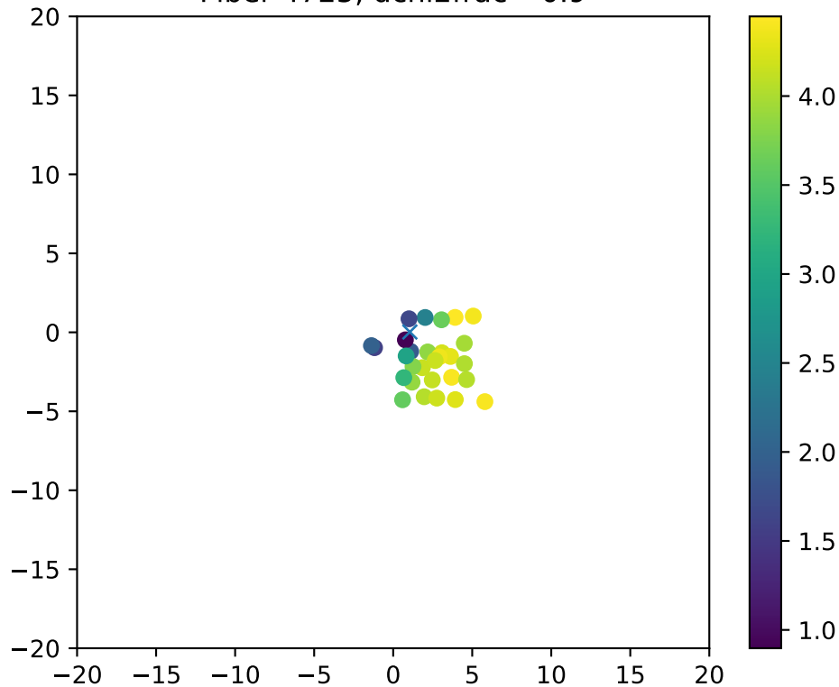
Fiber 4725, dchi2frac= 0.9
