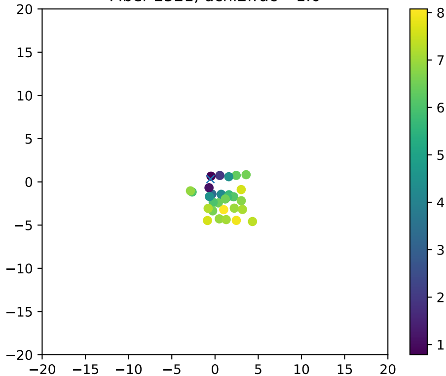
Fiber 2521, dchi2frac= 1.0
