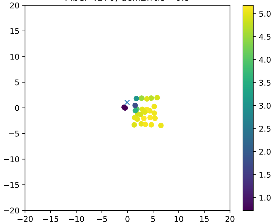
Fiber 4270, dchi2frac= 0.9
