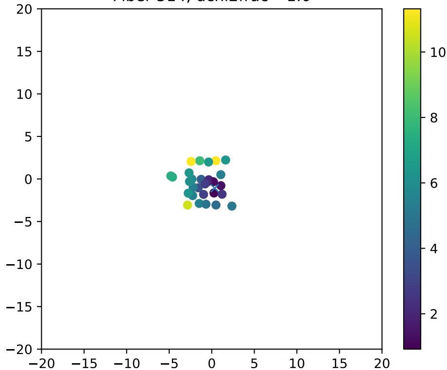
Fiber 514, dchi2frac= 1.0
