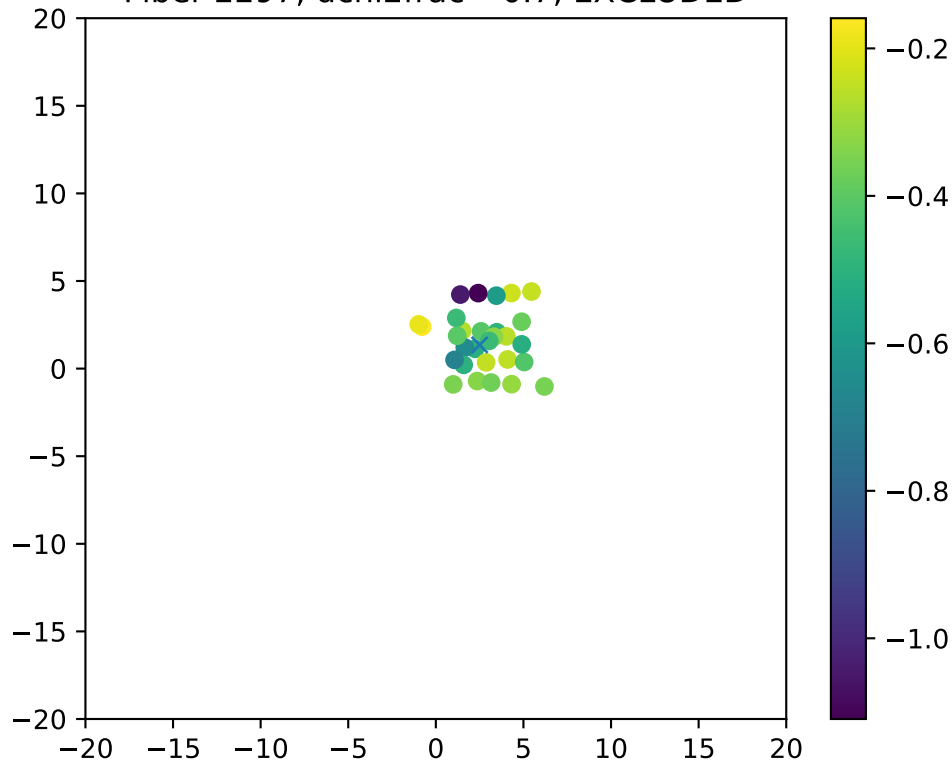
Fiber 2297, dchi2frac= 0.7, EXCLUDED
