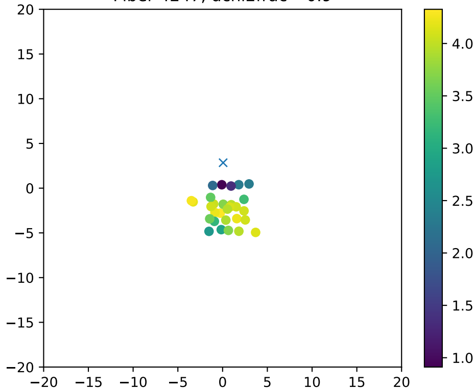
Fiber 4247, dchi2frac= 0.9
