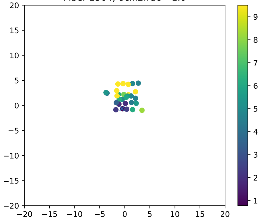
Fiber 2504, dchi2frac= 1.0
