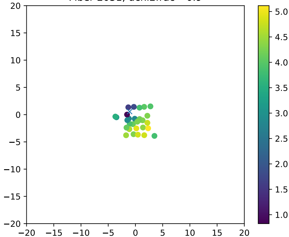
Fiber 2031, dchi2frac= 0.9
