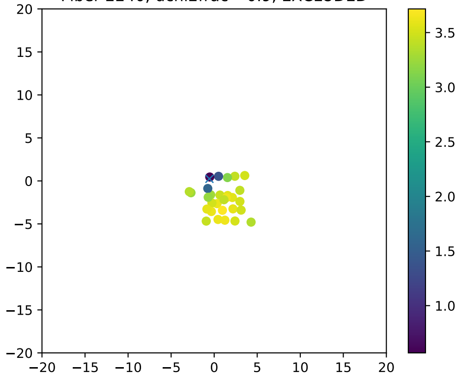
Fiber 2240, dchi2frac= 0.9, EXCLUDED
