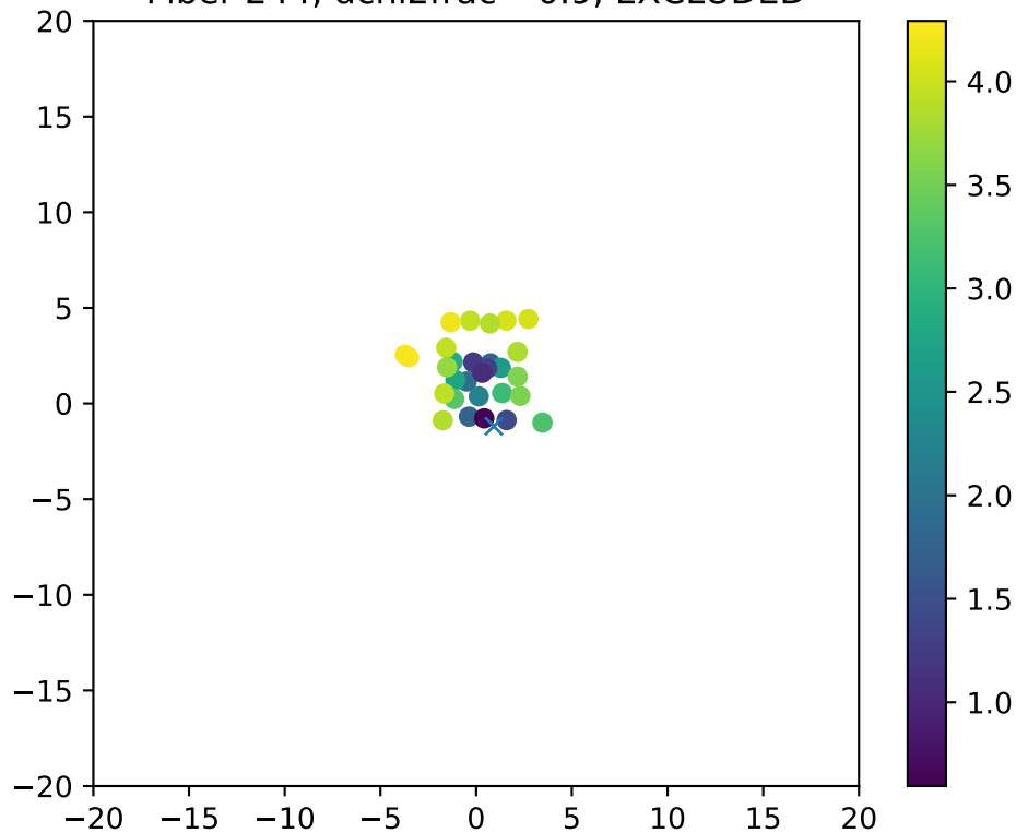
Fiber 244, dchi2frac= 0.9, EXCLUDED
