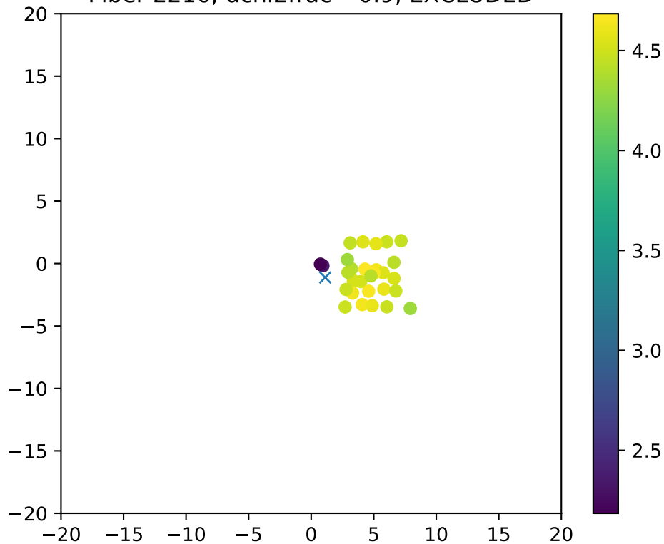
Fiber 2216, dchi2frac= 0.9, EXCLUDED
