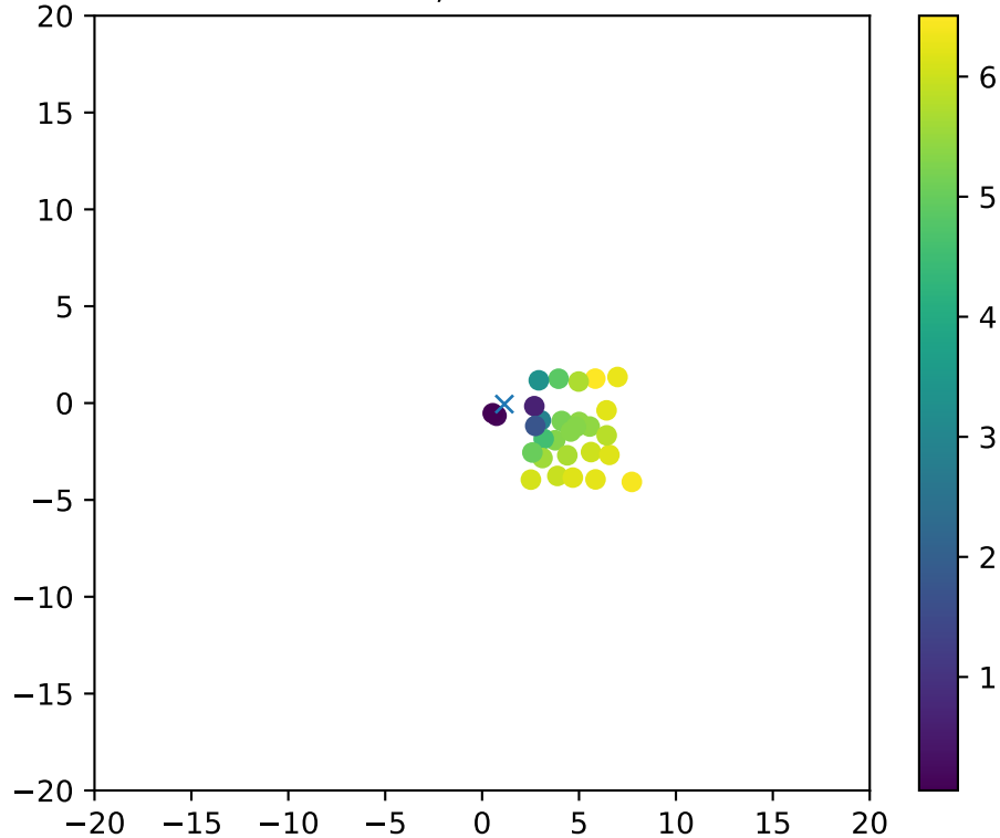
Fiber 4618, dchi2frac= 1.0
