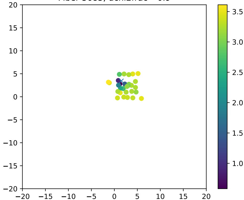
Fiber 3683, dchi2frac= 0.9
