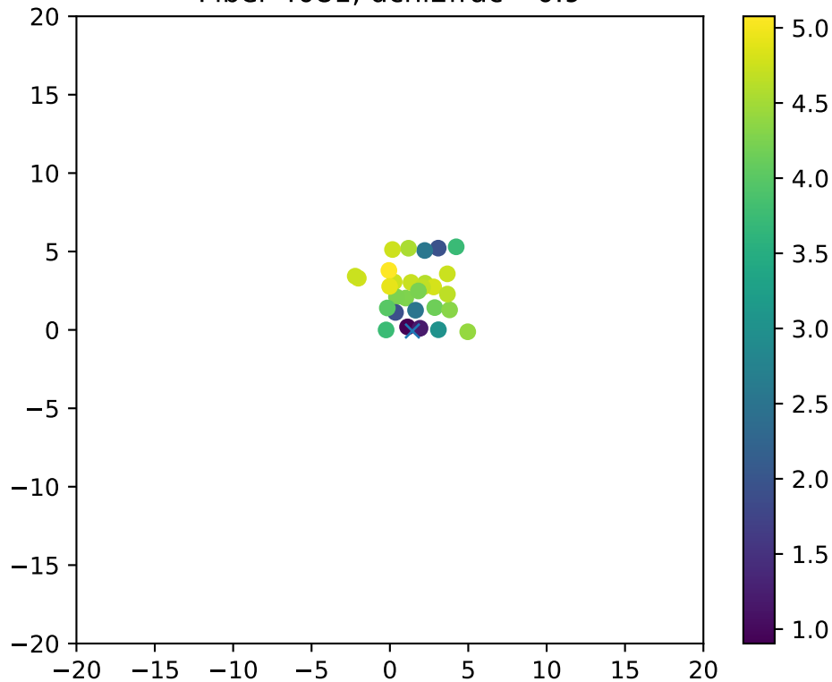
Fiber 4081, dchi2frac= 0.9
