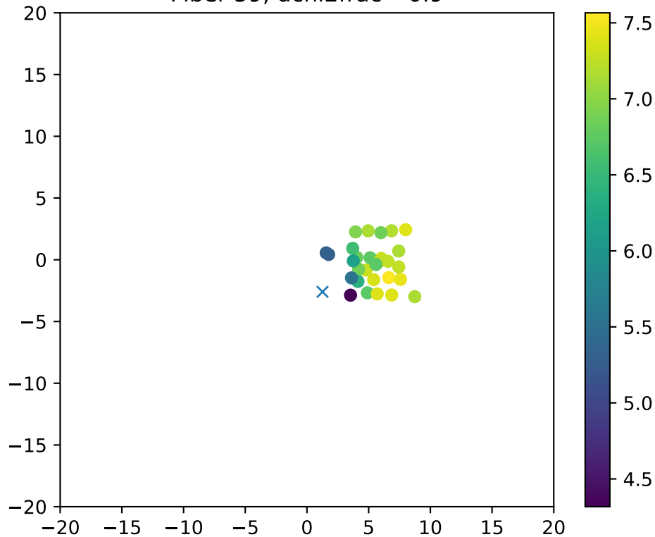
Fiber 59, dchi2frac= 0.9
