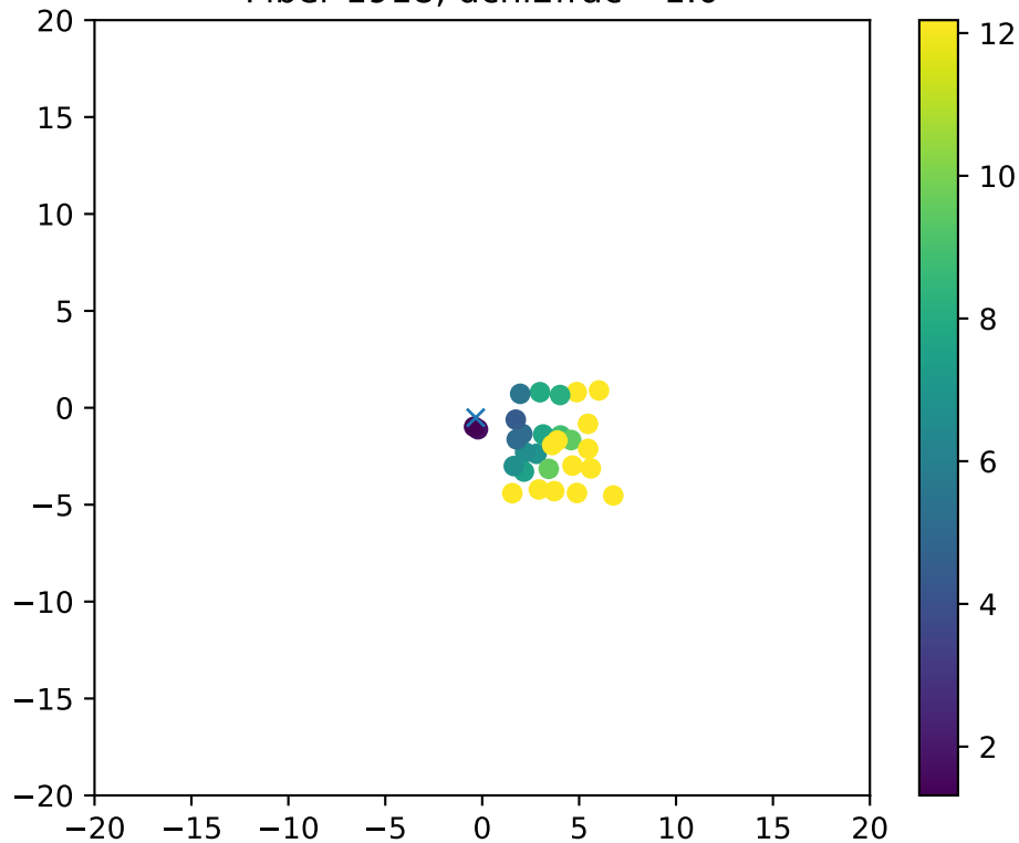
Fiber 1918, dchi2frac= 1.0
