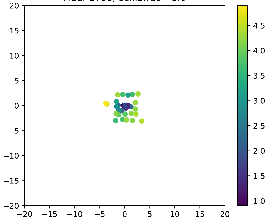
Fiber 1706, dchi2frac= 1.0
