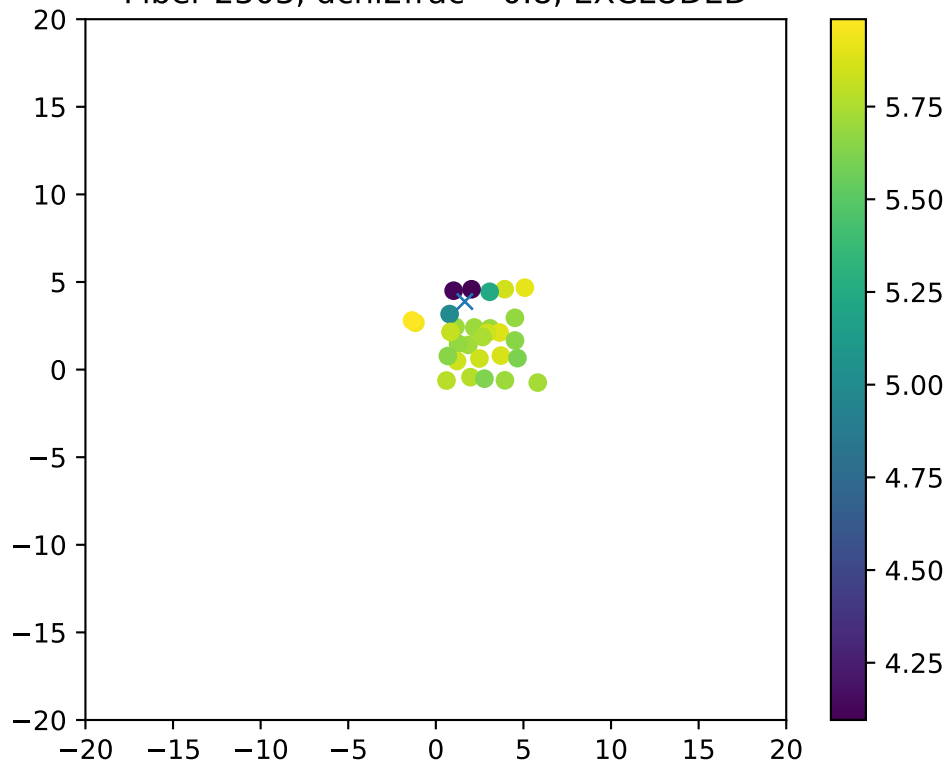
Fiber 2303, dchi2frac= 0.8, EXCLUDED
