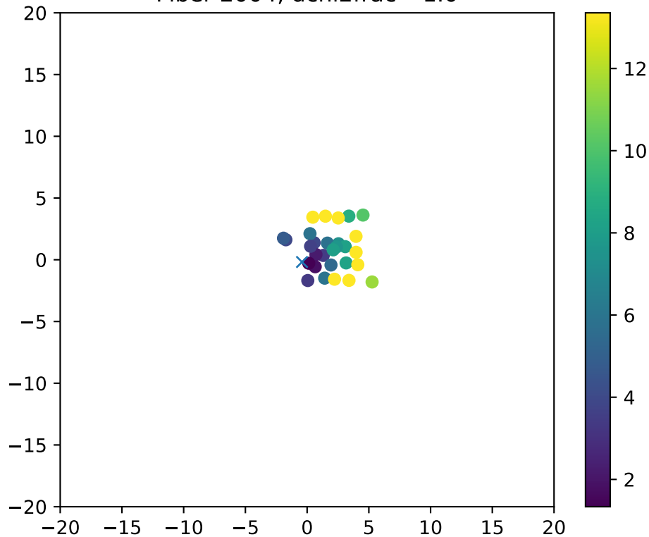
Fiber 2004, dchi2frac= 1.0
