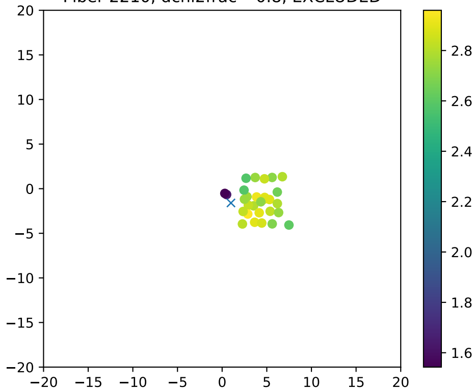
Fiber 2210, dchi2frac= 0.8, EXCLUDED
