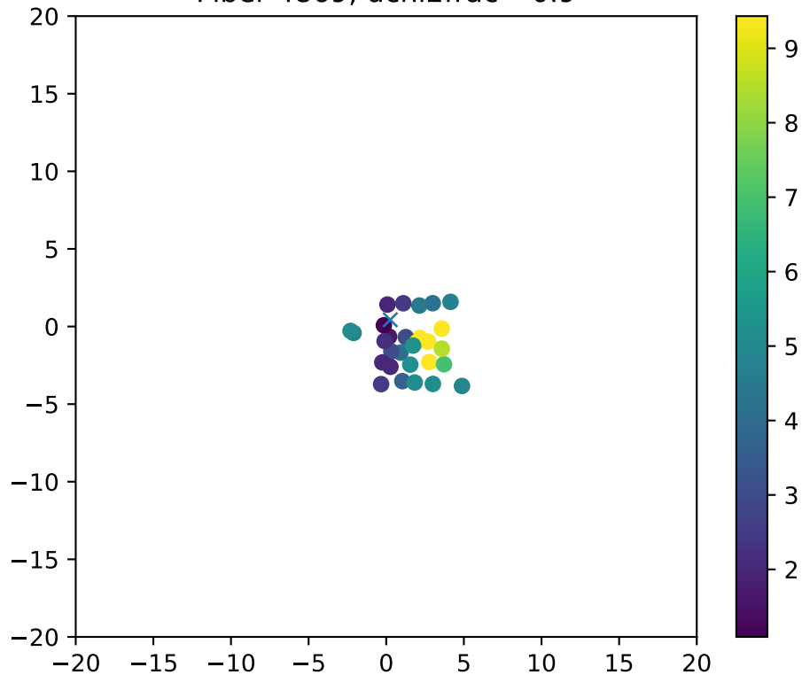
Fiber 4869, dchi2frac= 0.9
