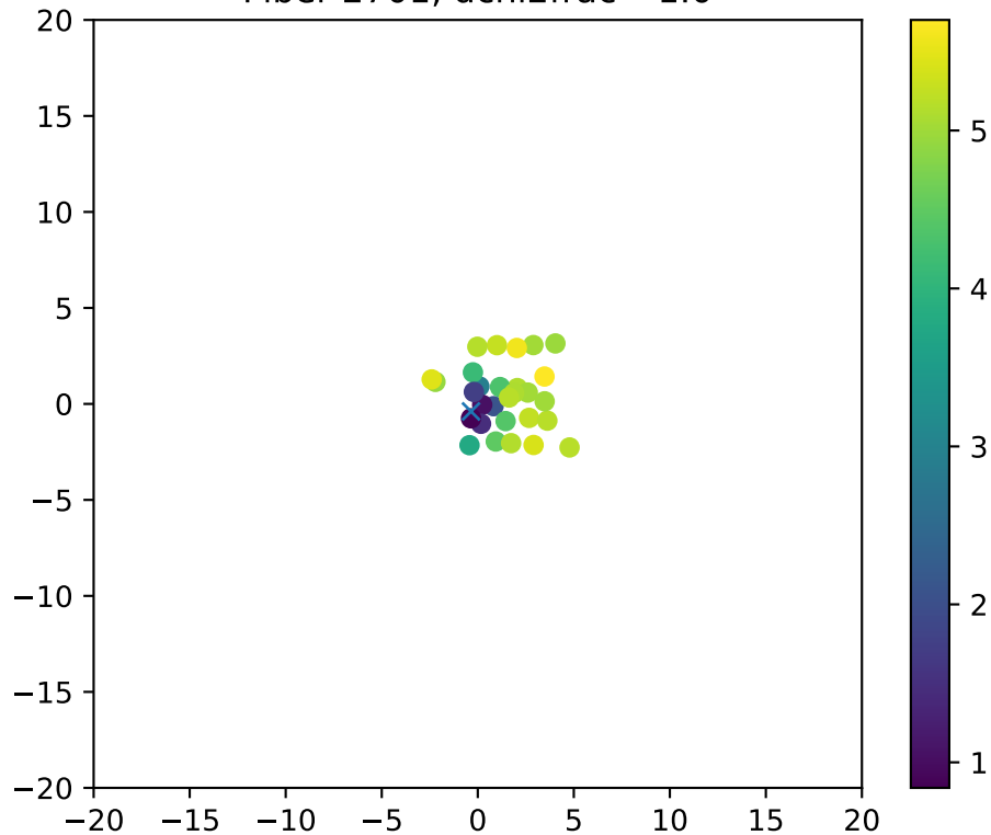
Fiber 2701, dchi2frac= 1.0
