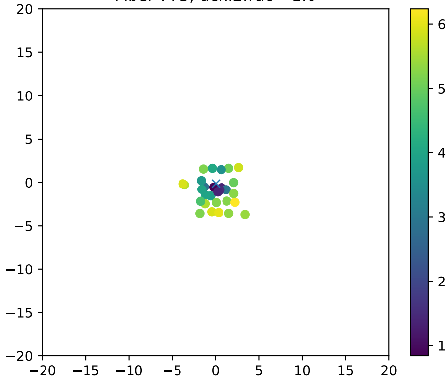
Fiber 773, dchi2frac= 1.0
