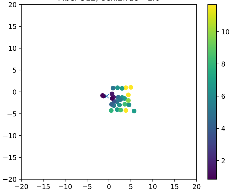
Fiber 512, dchi2frac= 1.0
