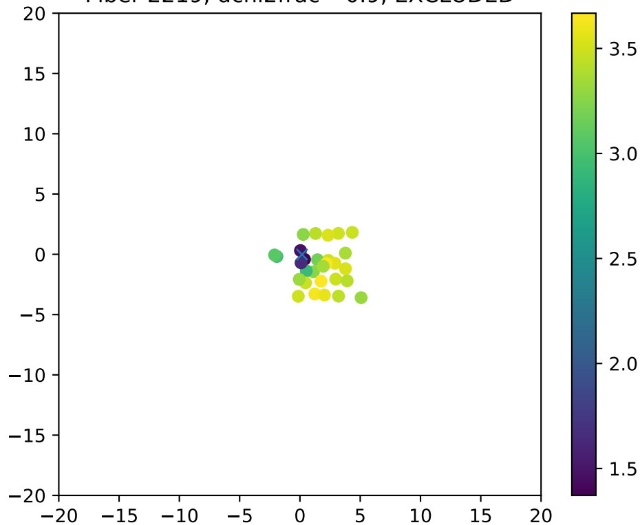
Fiber 2219, dchi2frac= 0.9, EXCLUDED
