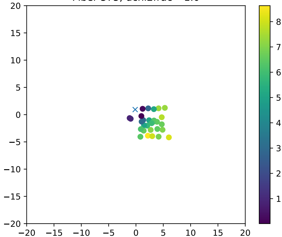
Fiber 375, dchi2frac= 1.0
