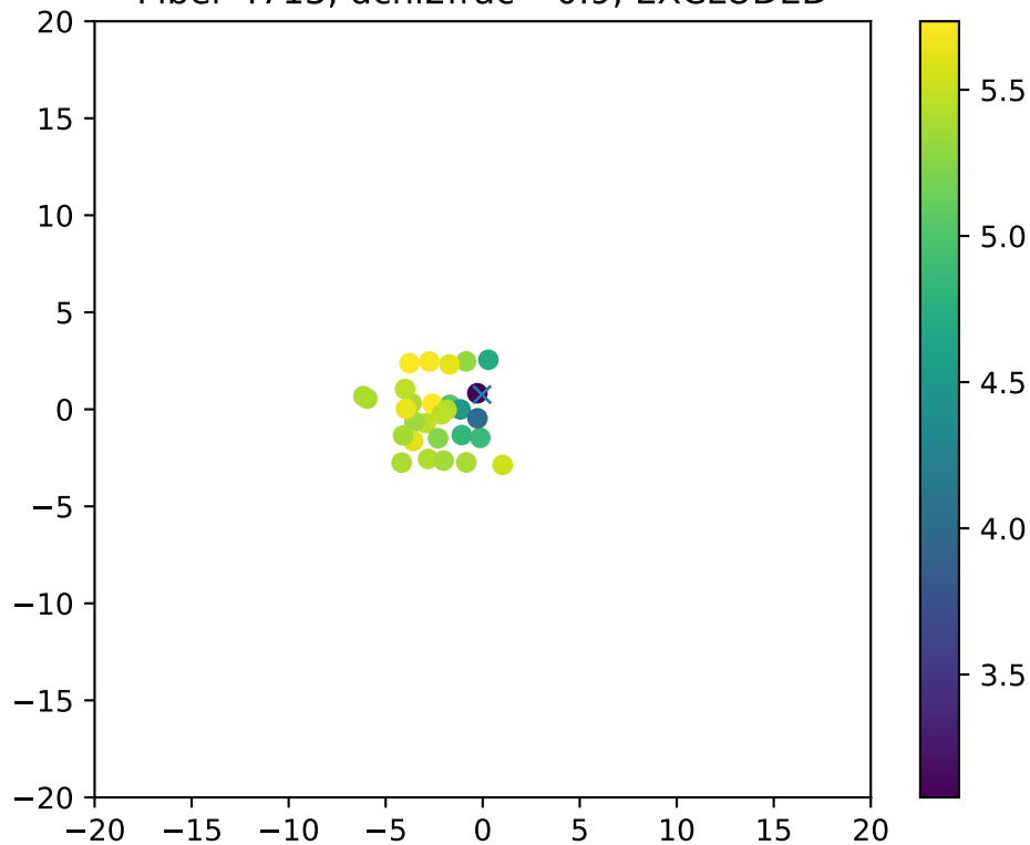
Fiber 4713, dchi2frac= 0.9, EXCLUDED
