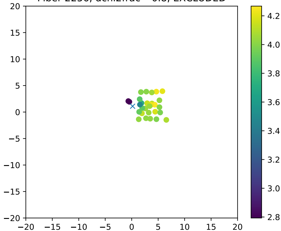
Fiber 2256, dchi2frac= 0.8, EXCLUDED
