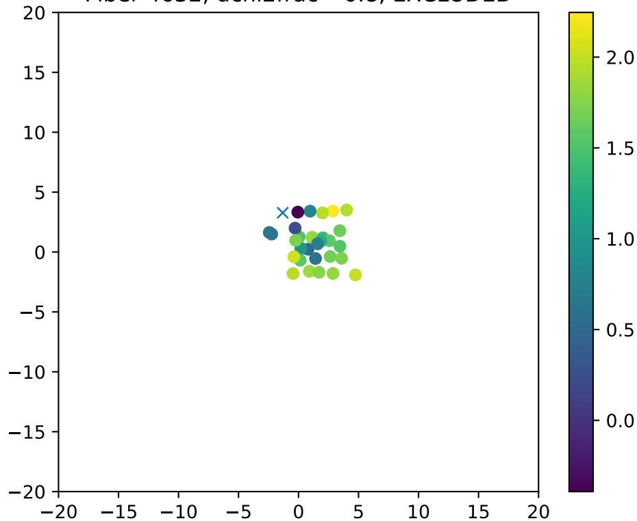
Fiber 4632, dchi2frac= 0.8, EXCLUDED
