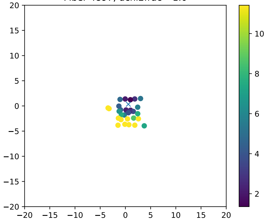
Fiber 4897, dchi2frac= 1.0
