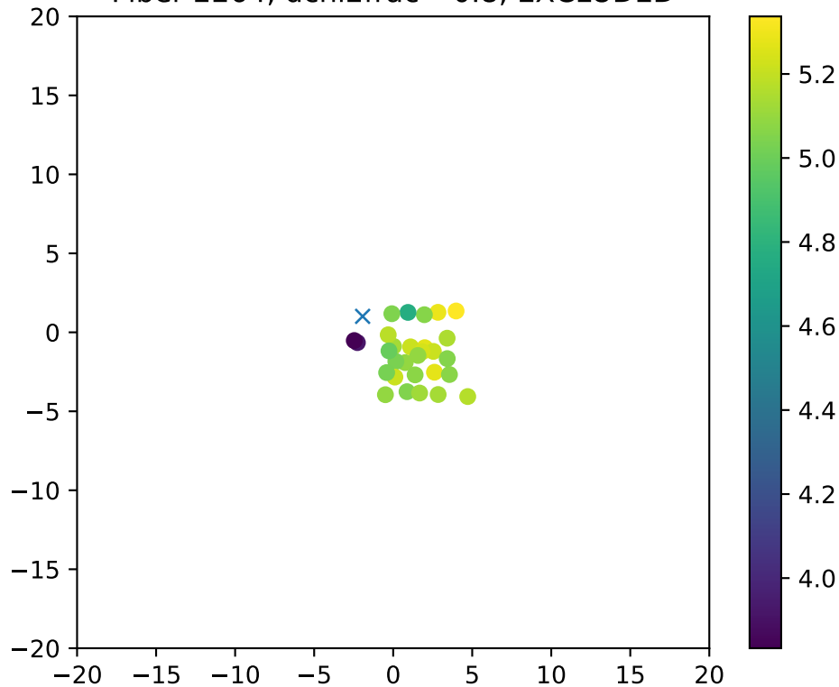
Fiber 2264, dchi2frac= 0.8, EXCLUDED
