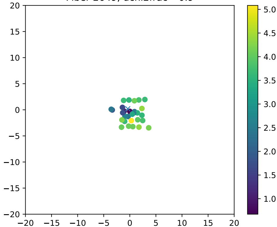
Fiber 2649, dchi2frac= 0.9
