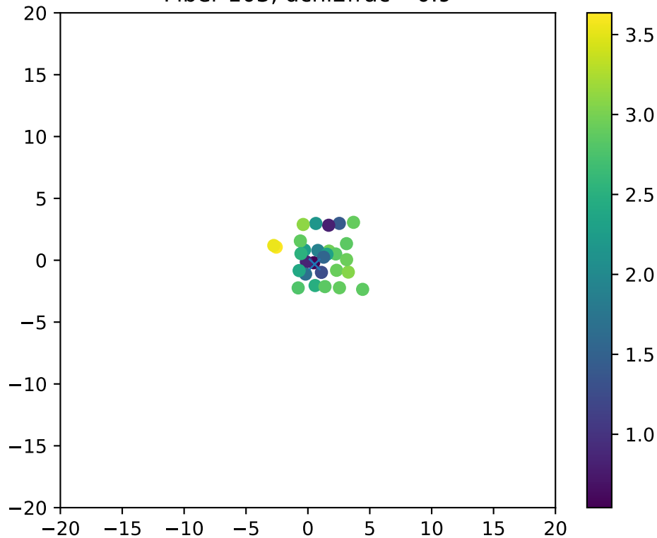
Fiber 103, dchi2frac= 0.9
