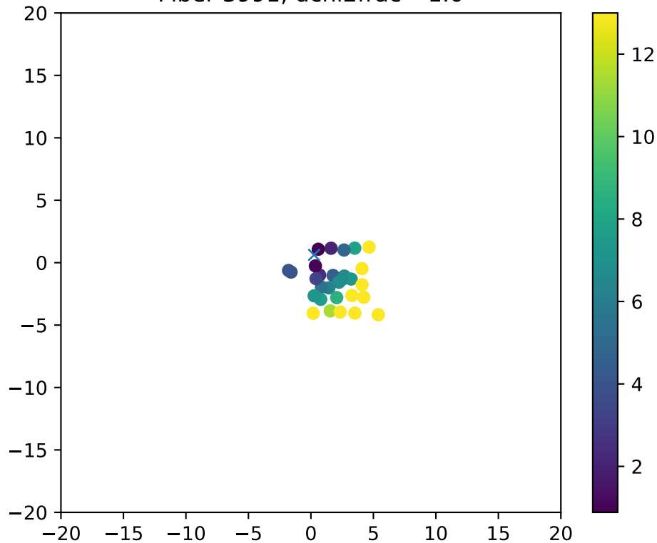
Fiber 3991, dchi2frac= 1.0
