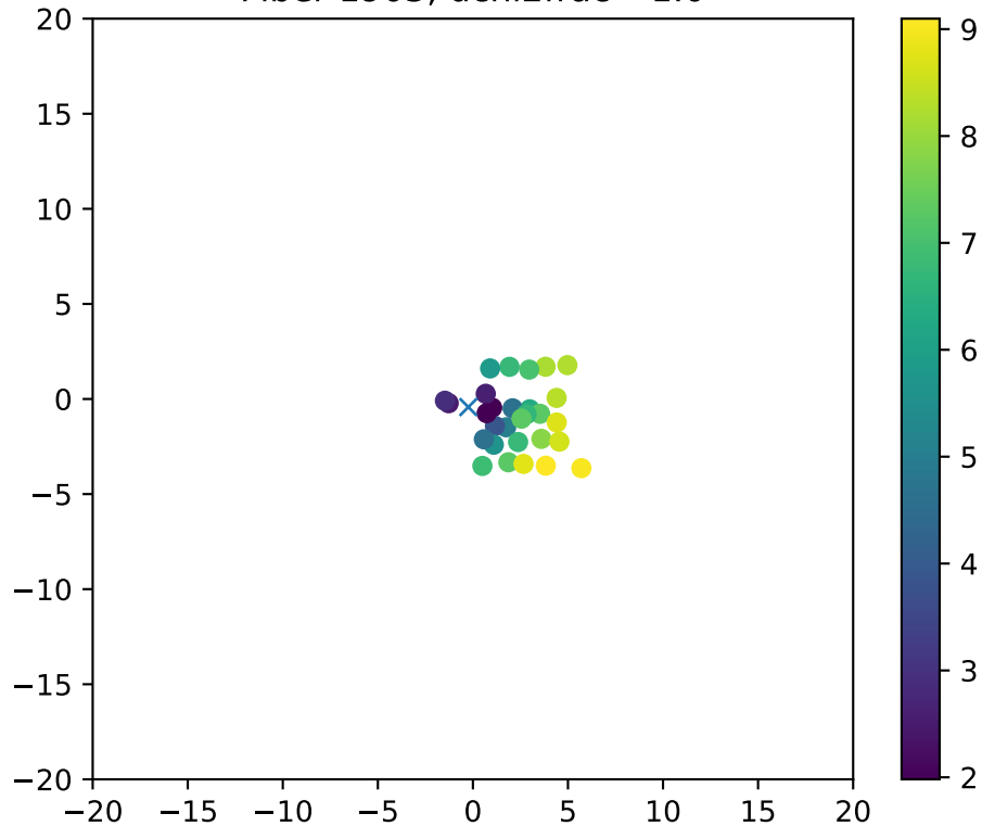
Fiber 1903, dchi2frac= 1.0
