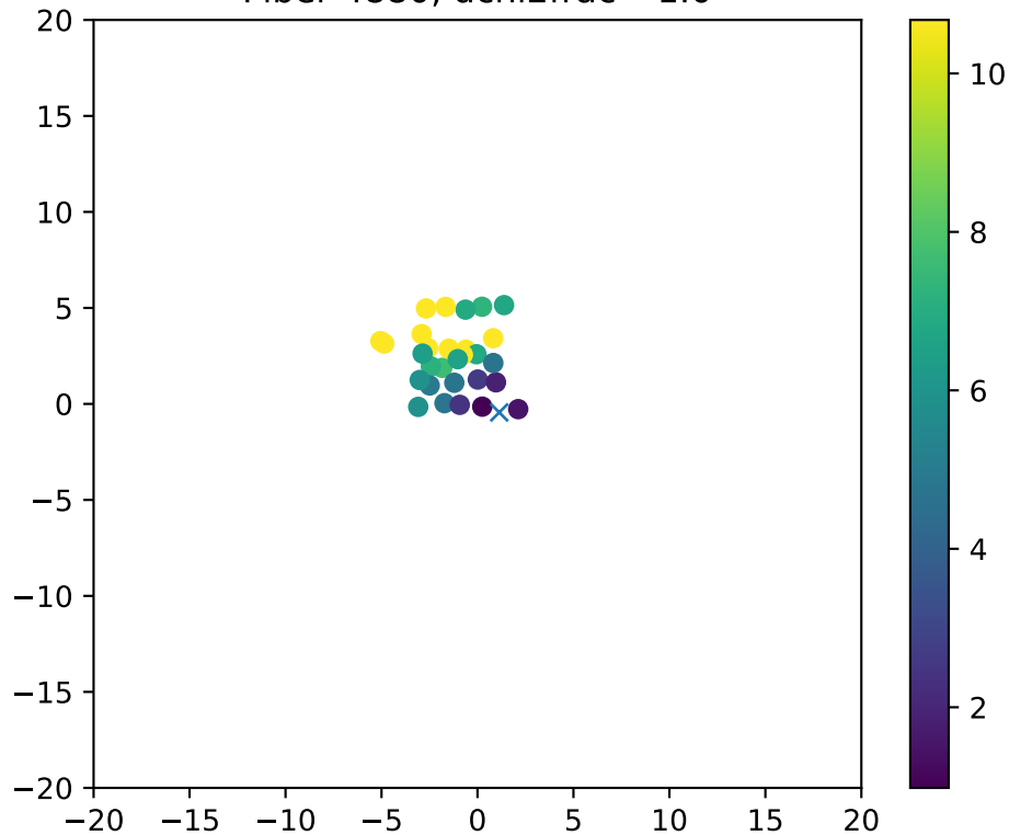
Fiber 4880, dchi2frac= 1.0
