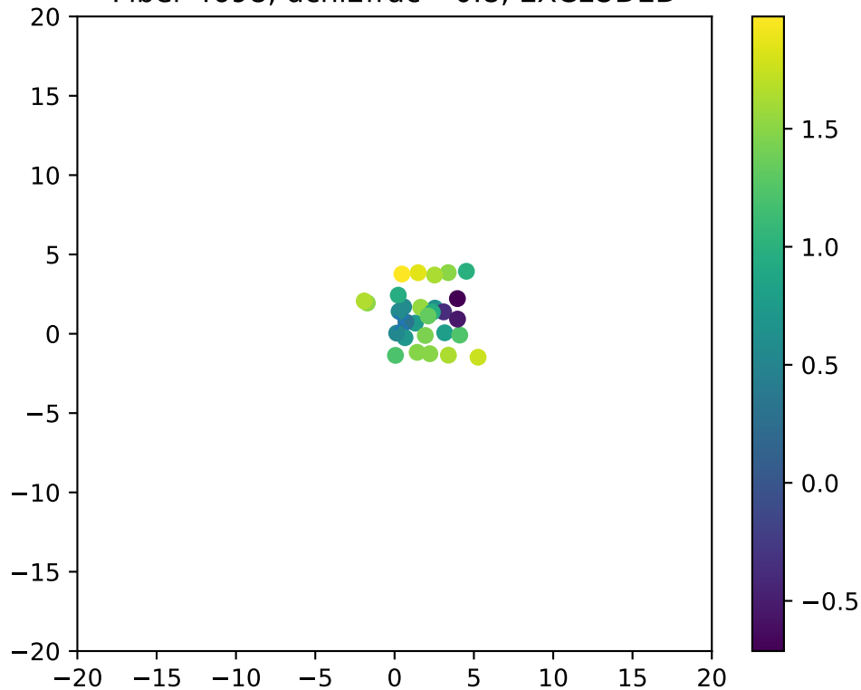
Fiber 4698, dchi2frac= 0.8, EXCLUDED
