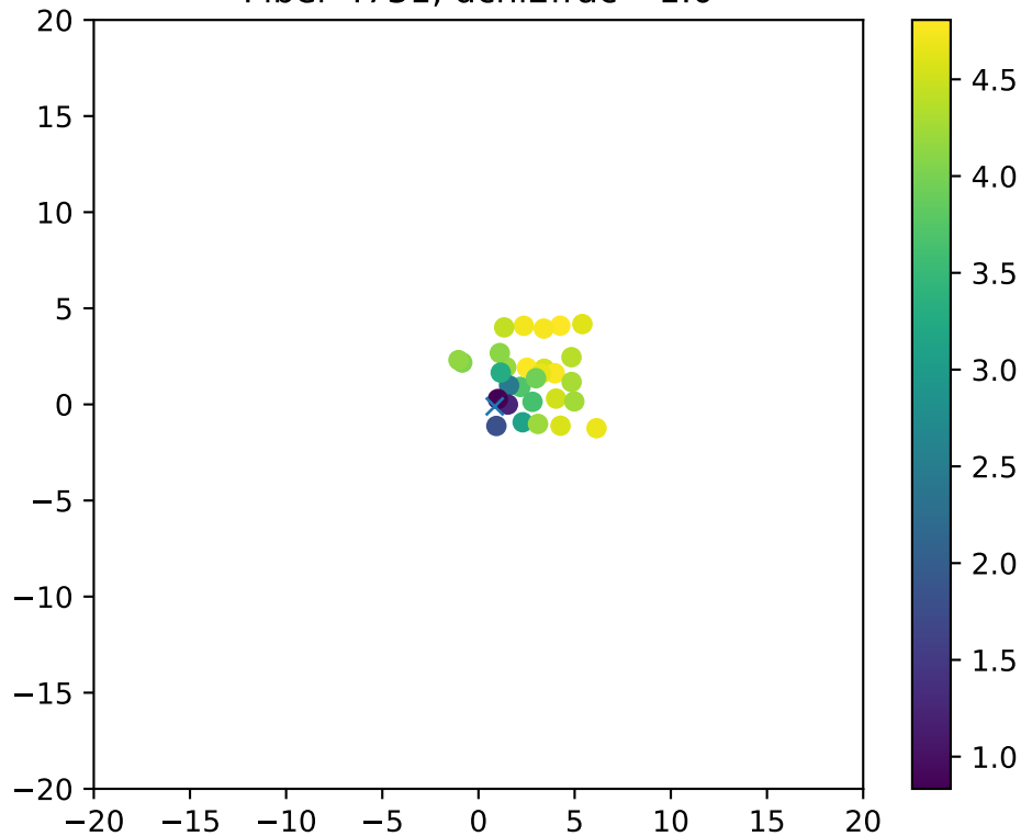
Fiber 4731, dchi2frac= 1.0
