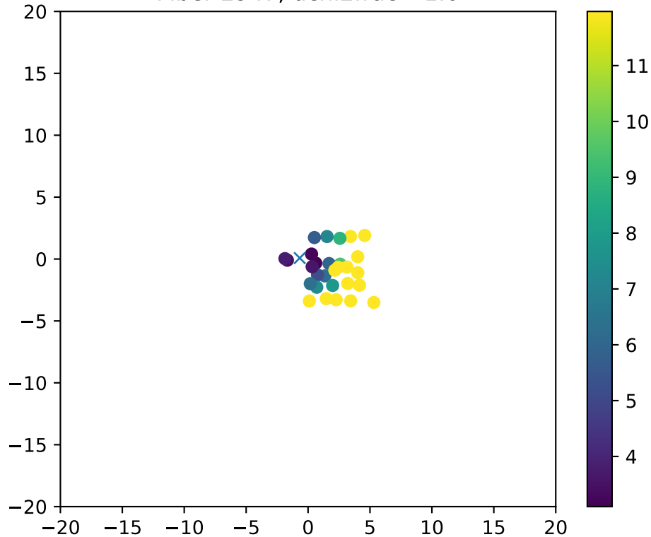
Fiber 2947, dchi2frac= 1.0
