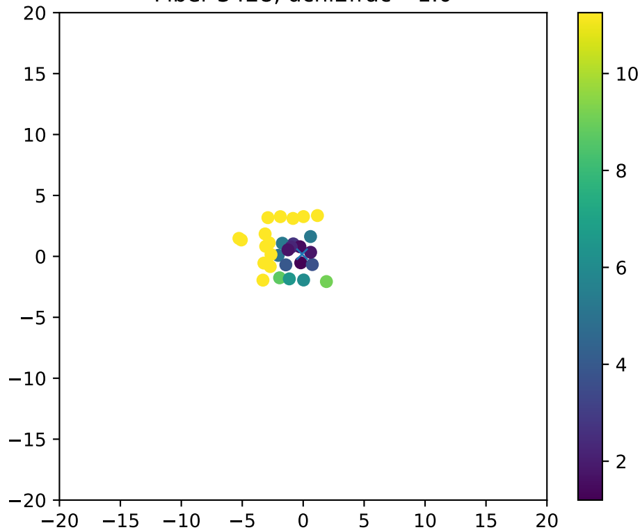
Fiber 3428, dchi2frac= 1.0
