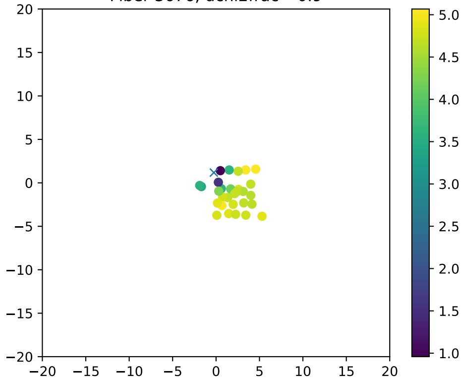
Fiber 3676, dchi2frac= 0.9
