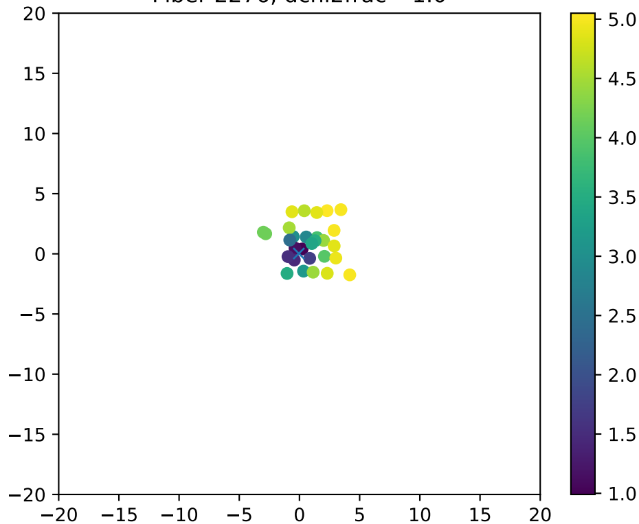
Fiber 2276, dchi2frac= 1.0
