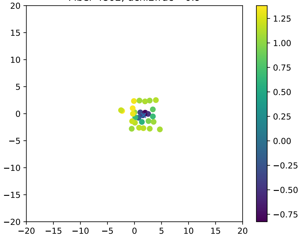
Fiber 4802, dchi2frac= 0.9
