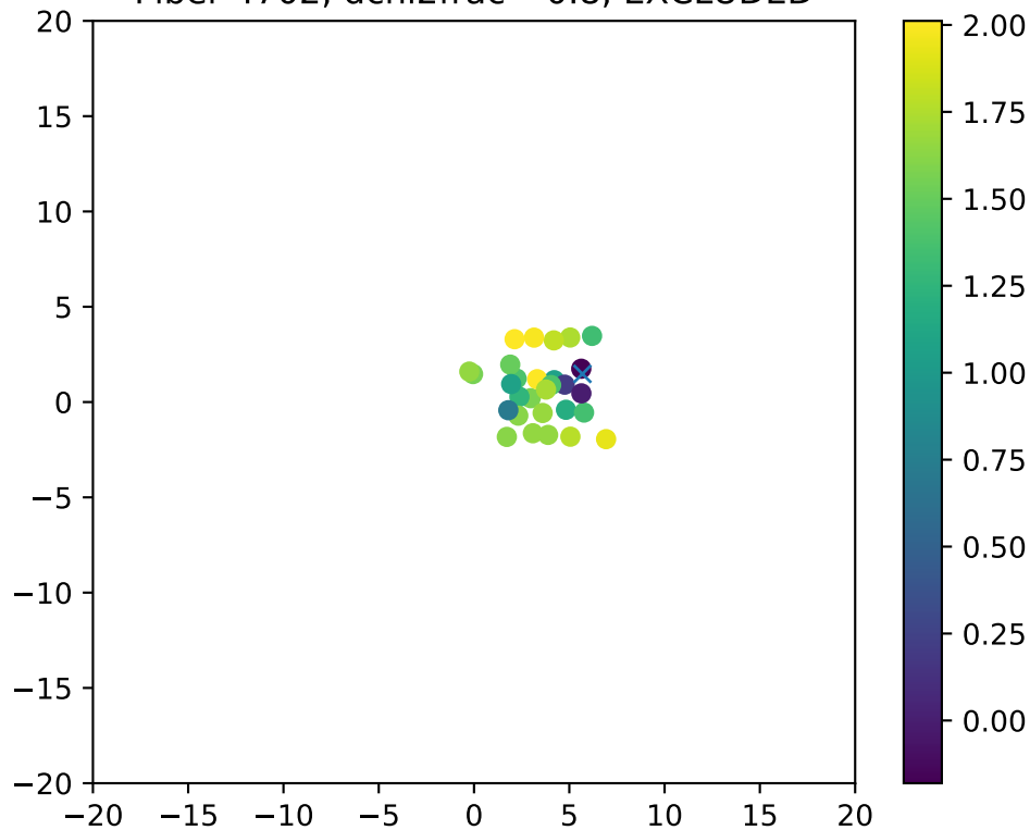
Fiber 4702, dchi2frac= 0.8, EXCLUDED
