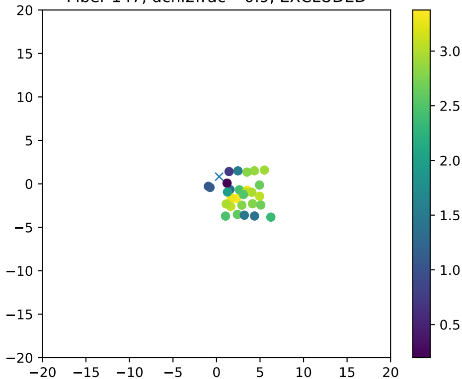
Fiber 147, dchi2frac= 0.9, EXCLUDED
