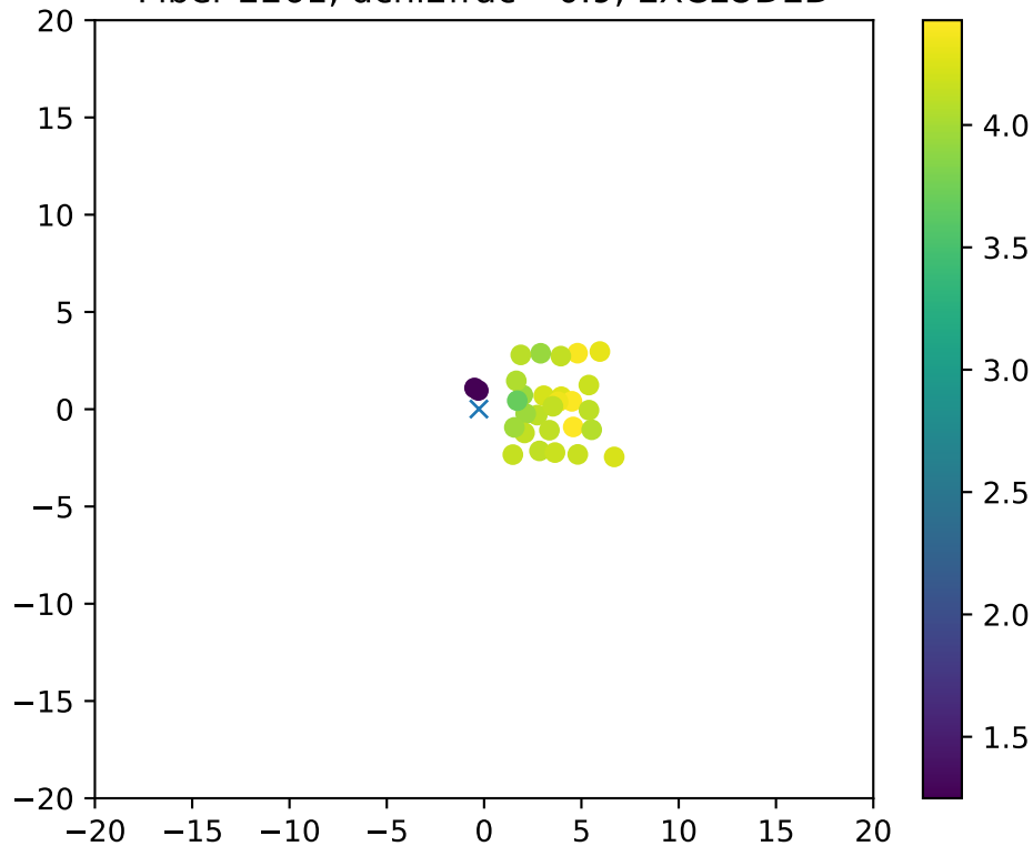
Fiber 2261, dchi2frac= 0.9, EXCLUDED
