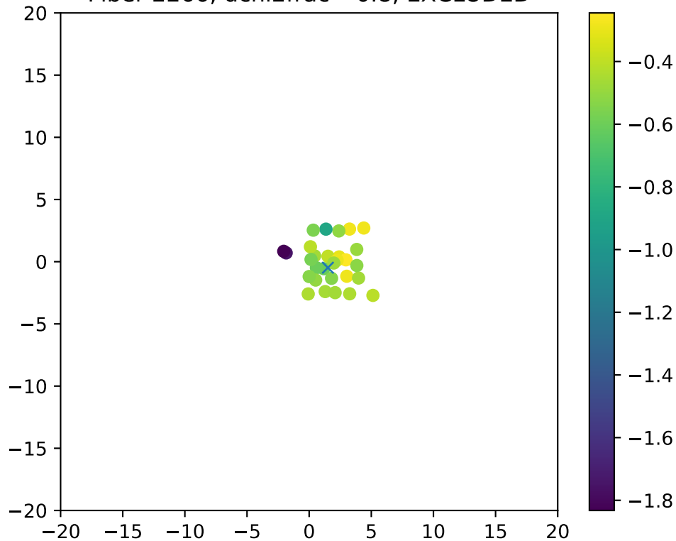
Fiber 2266, dchi2frac= 0.8, EXCLUDED
