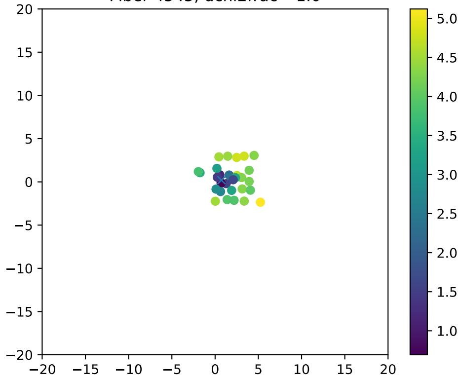
Fiber 4545, dchi2frac= 1.0
