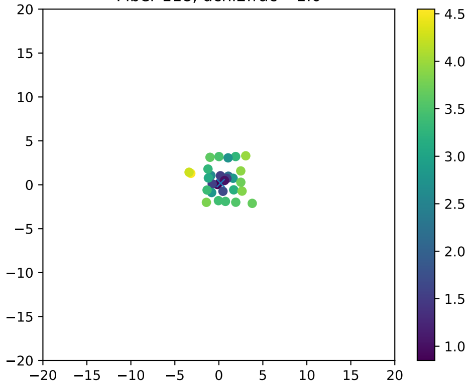
Fiber 118, dchi2frac= 1.0
