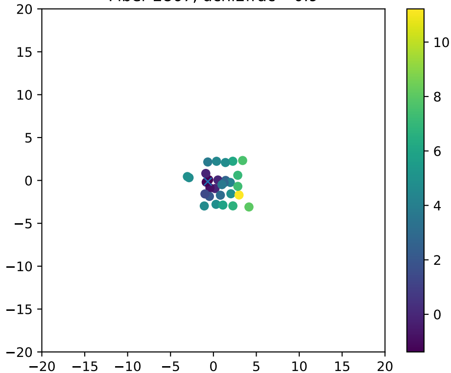
Fiber 2867, dchi2frac= 0.9
