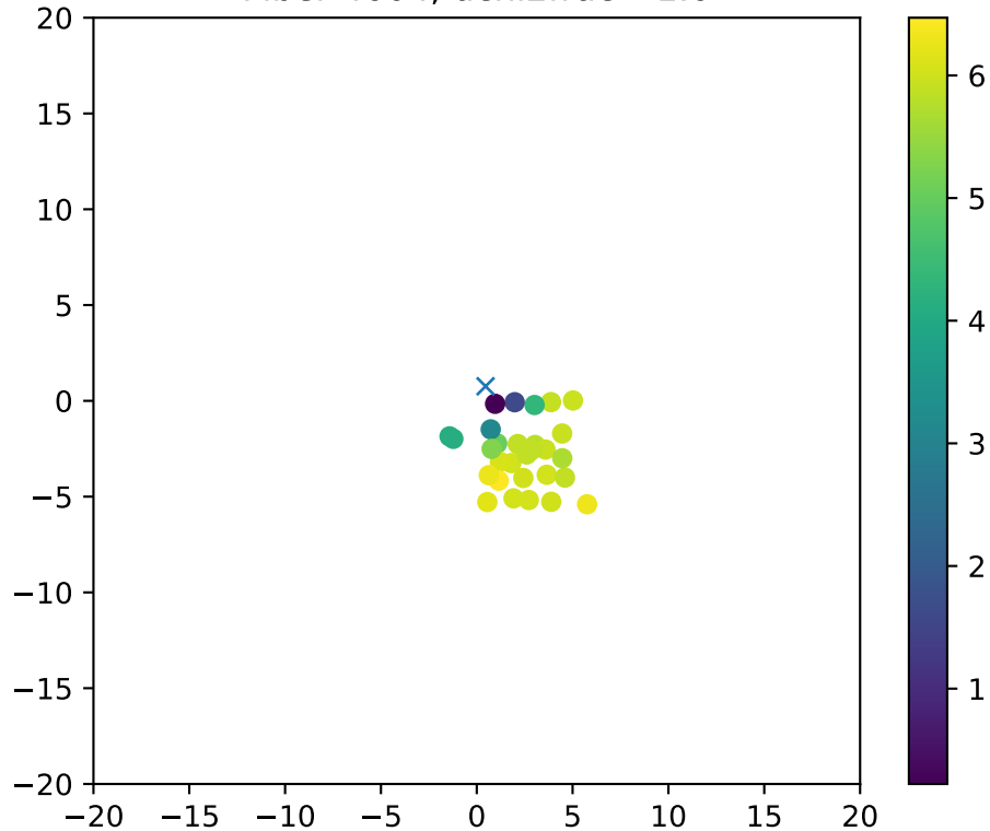
Fiber 4604, dchi2frac= 1.0
