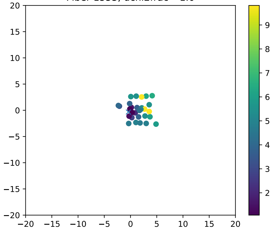
Fiber 1553, dchi2frac= 1.0
