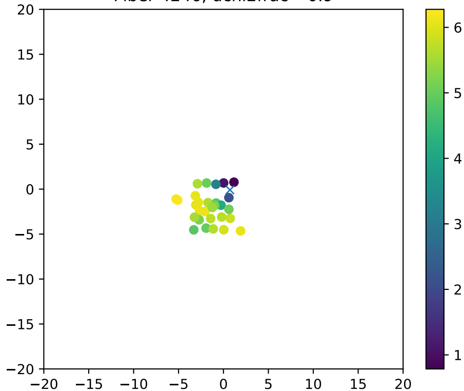
Fiber 4246, dchi2frac= 0.9
