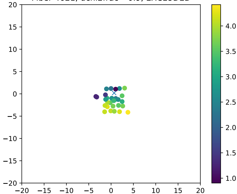
Fiber 4621, dchi2frac= 0.9, EXCLUDED
