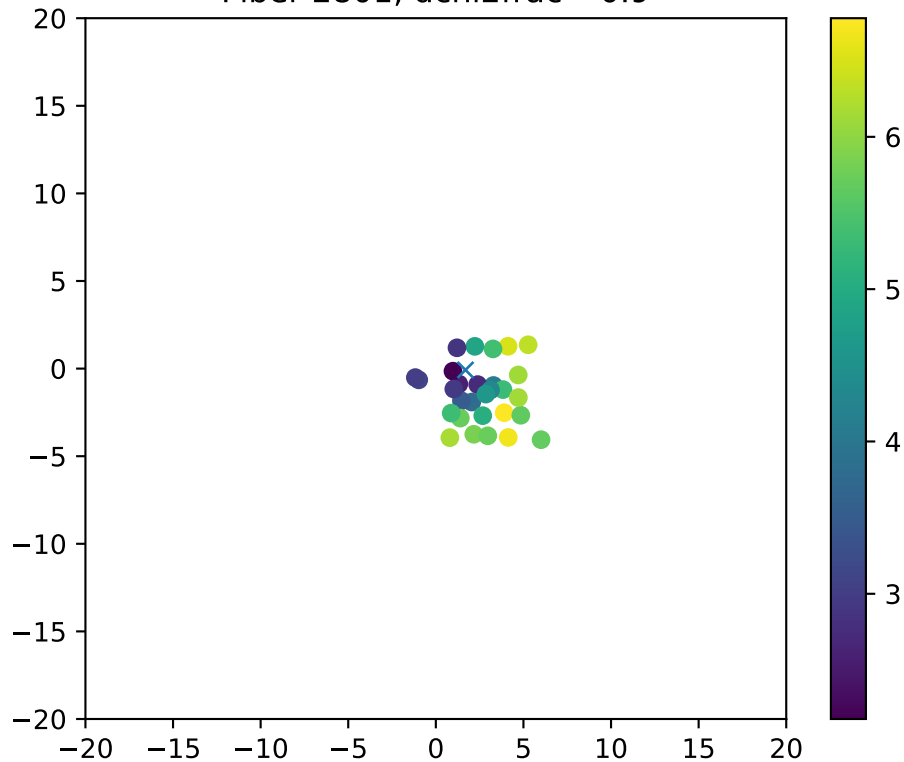
Fiber 2801, dchi2frac= 0.9
