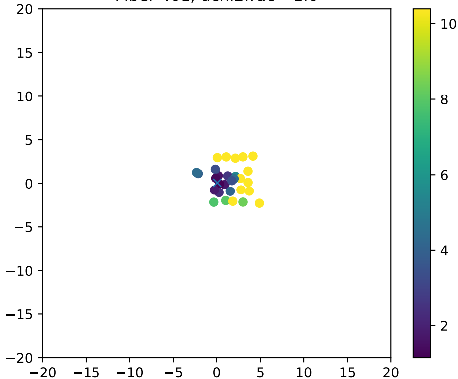
Fiber 401, dchi2frac= 1.0
