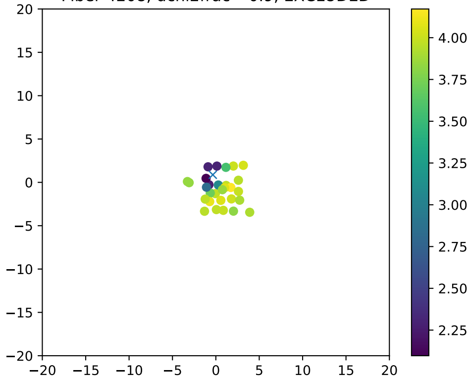
Fiber 4208, dchi2frac= 0.9, EXCLUDED
