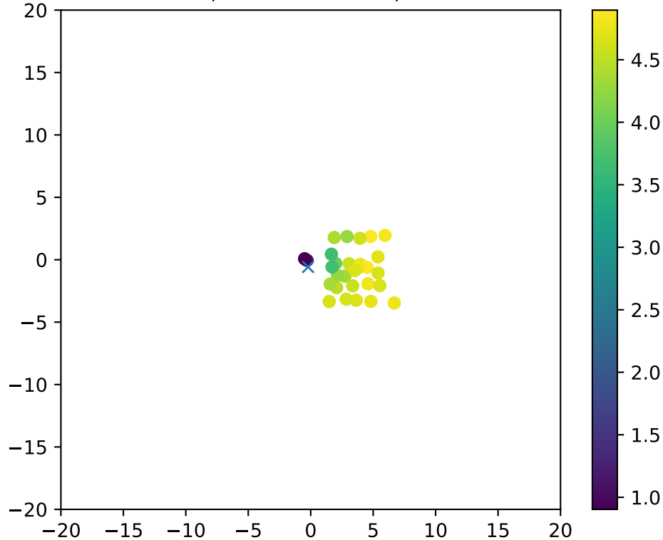
Fiber 2268, dchi2frac= 0.9, EXCLUDED
