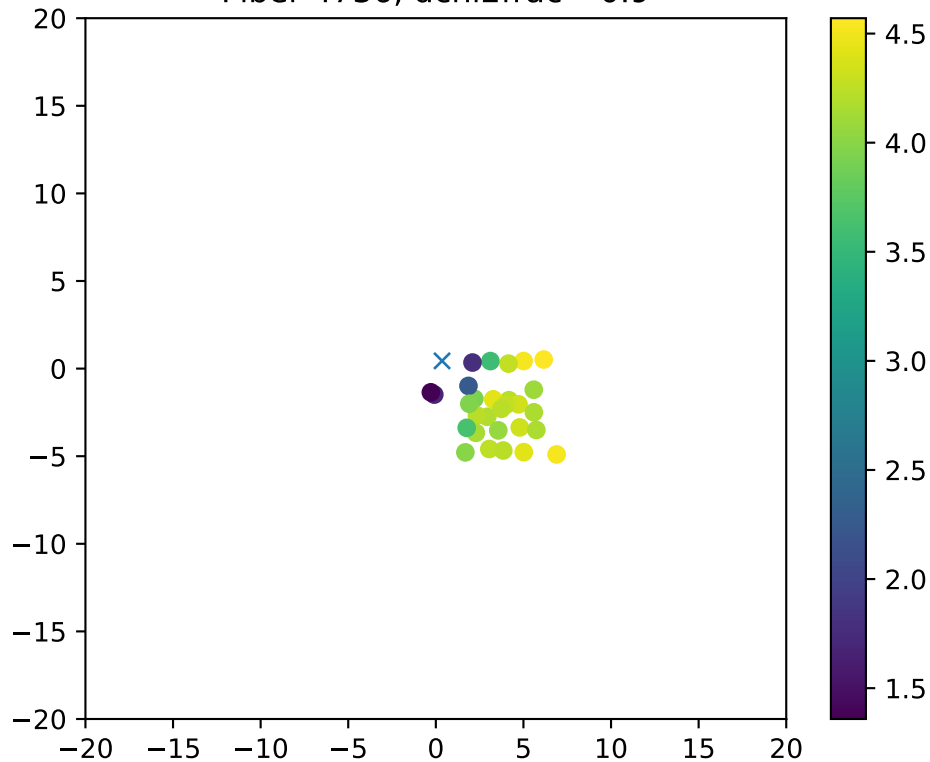
Fiber 4736, dchi2frac= 0.9
