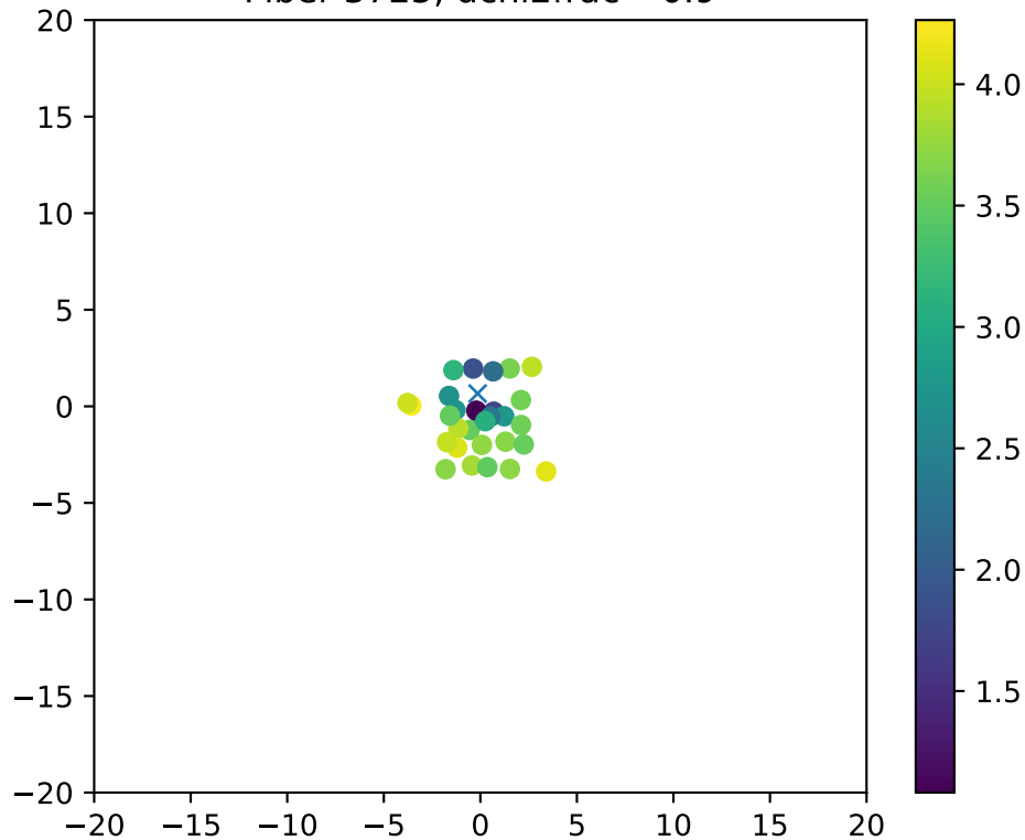
Fiber 3725, dchi2frac= 0.9
