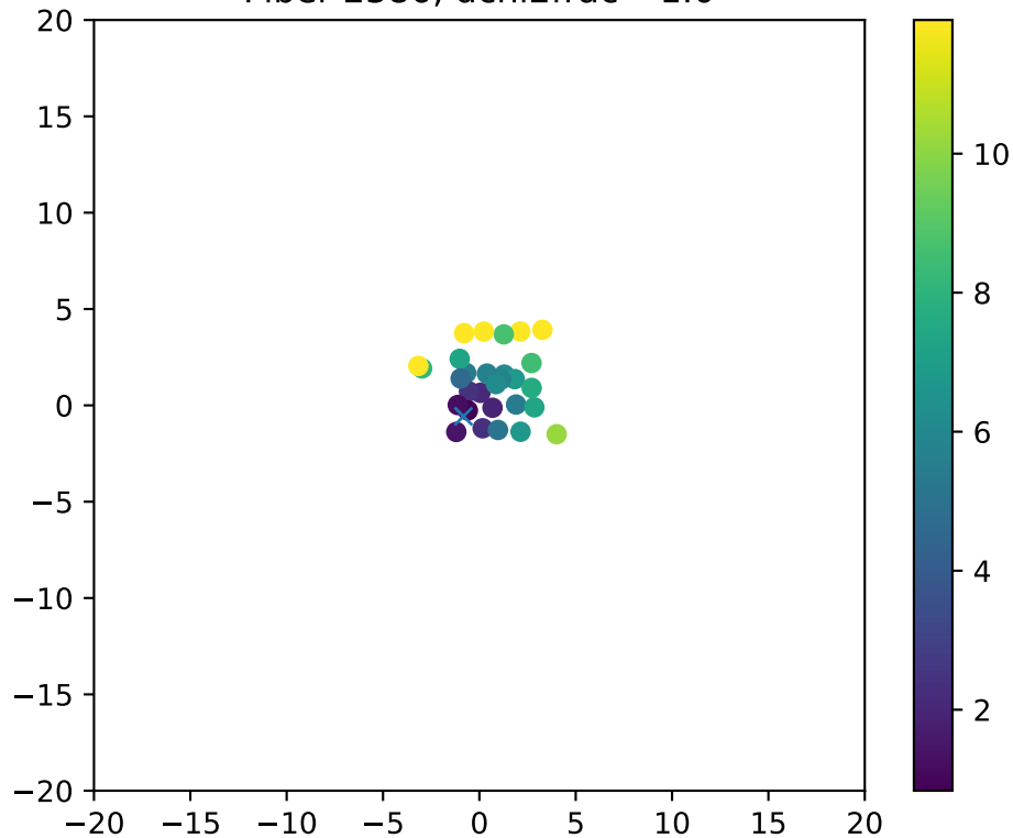
Fiber 2386, dchi2frac= 1.0
