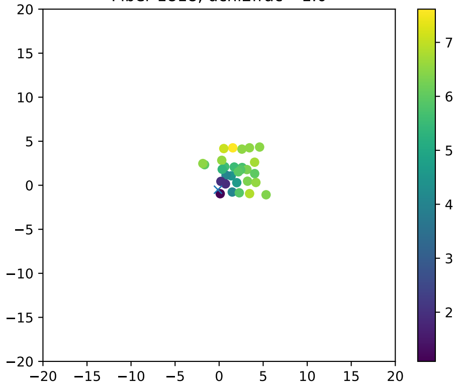
Fiber 1818, dchi2frac= 1.0
