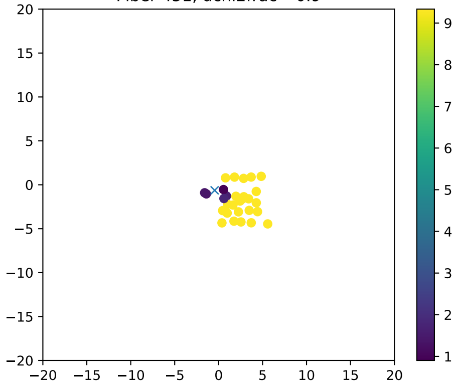
Fiber 451, dchi2frac= 0.9
