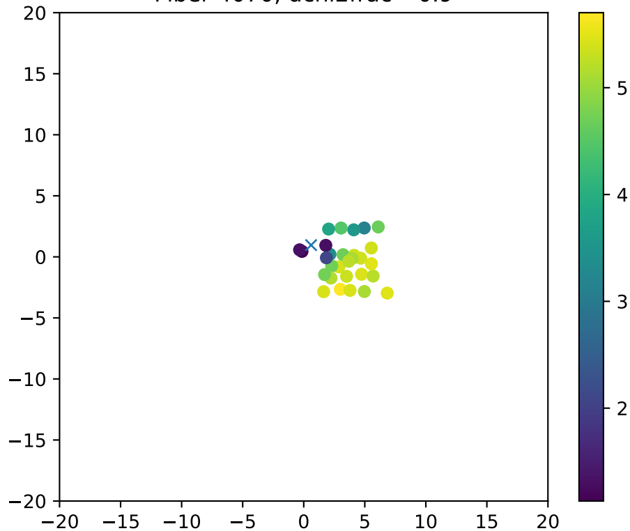
Fiber 4070, dchi2frac= 0.9
