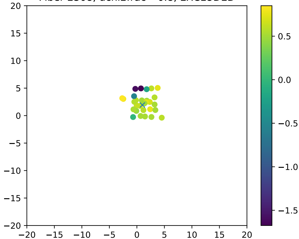
Fiber 2308, dchi2frac= 0.8, EXCLUDED
