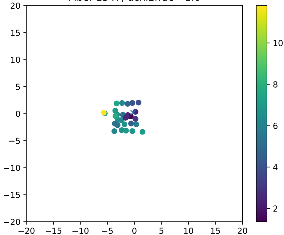
Fiber 2547, dchi2frac= 1.0
