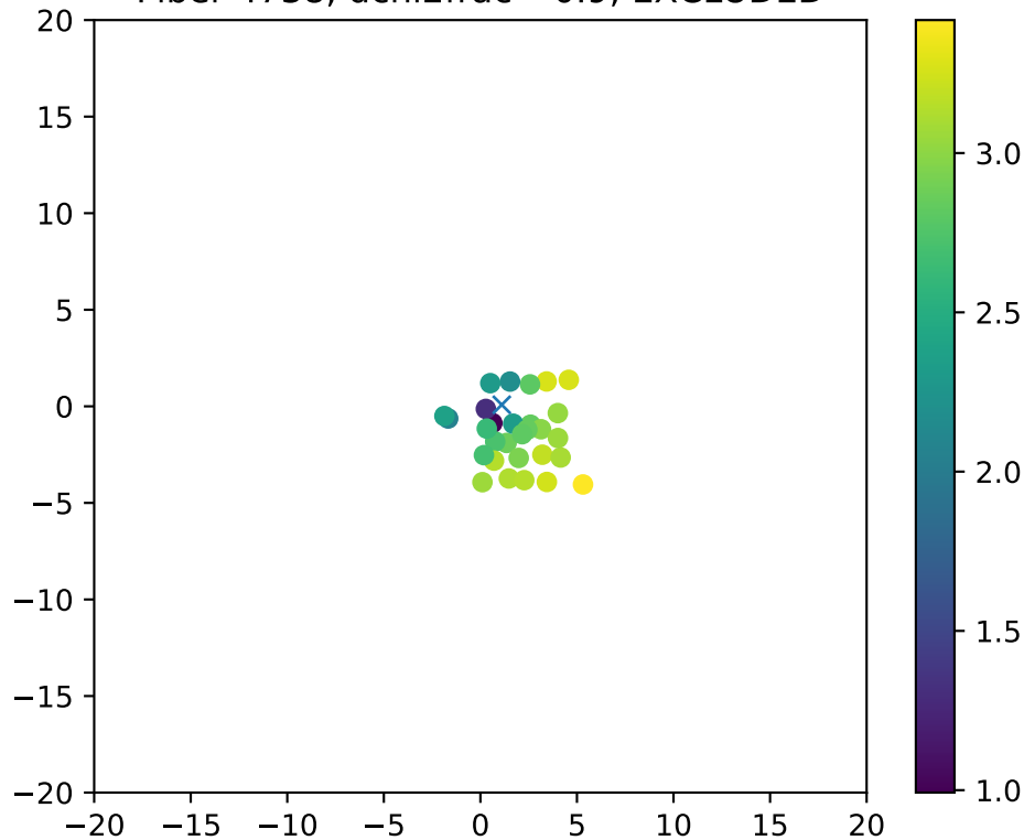
Fiber 4738, dchi2frac= 0.9, EXCLUDED
