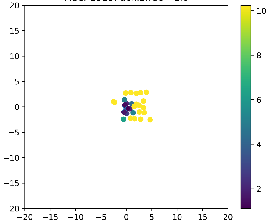
Fiber 2915, dchi2frac= 1.0
