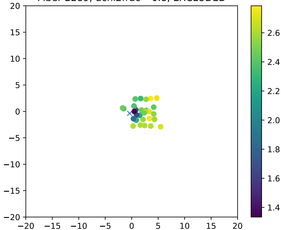
Fiber 2289, dchi2frac= 0.8, EXCLUDED
