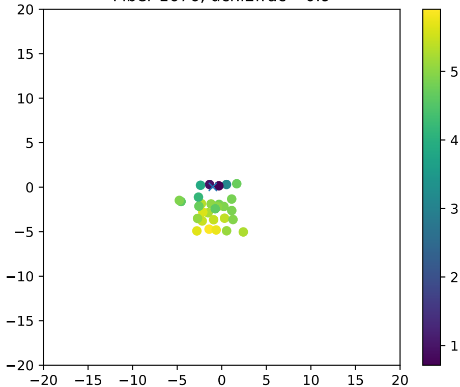
Fiber 1676, dchi2frac= 0.9
