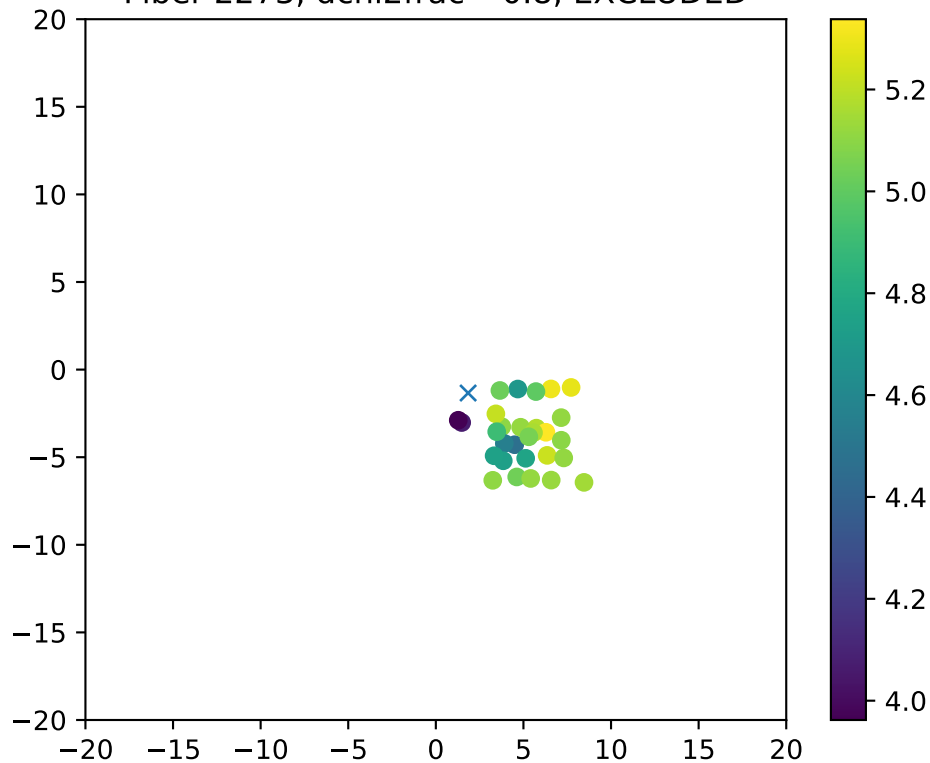
Fiber 2273, dchi2frac= 0.8, EXCLUDED
