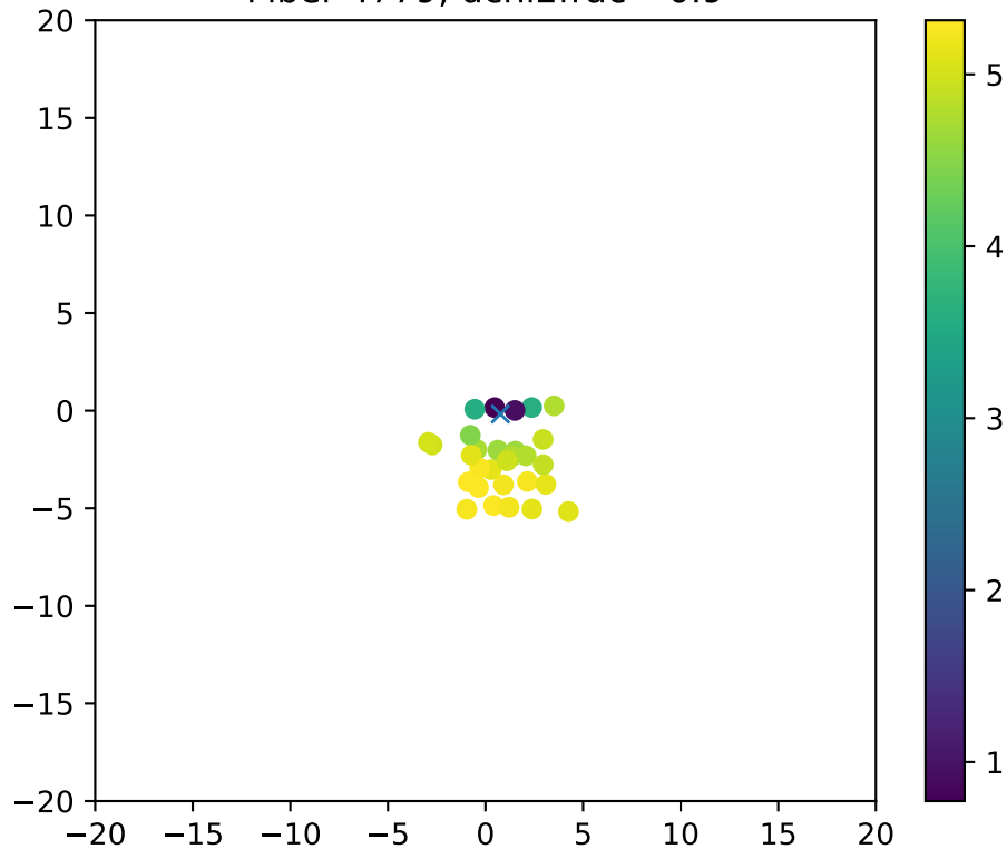
Fiber 4779, dchi2frac= 0.9
