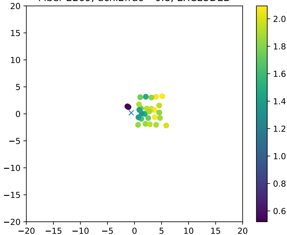
Fiber 2269, dchi2frac= 0.8, EXCLUDED
