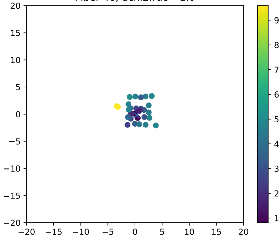
Fiber 46, dchi2frac= 1.0
