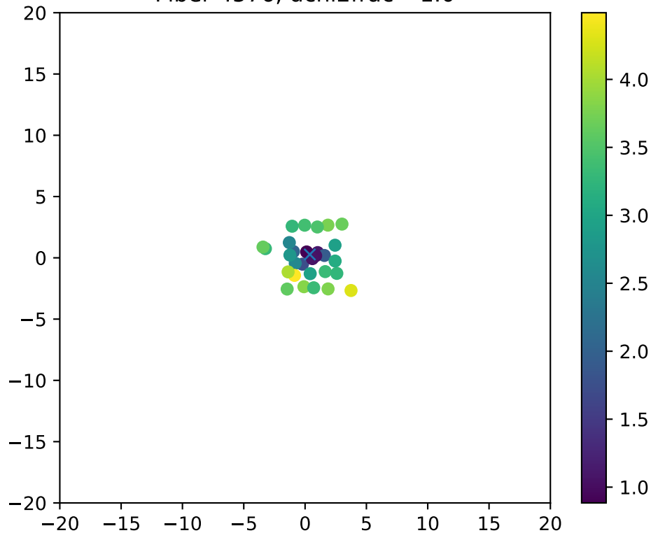
Fiber 4576, dchi2frac= 1.0
