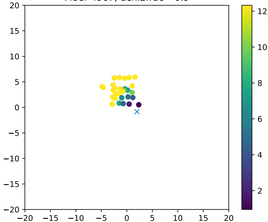
Fiber 4967, dchi2frac= 0.9
