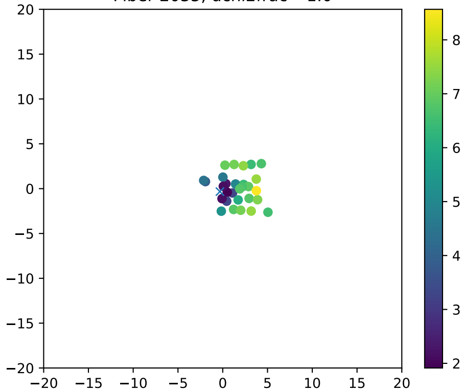
Fiber 2035, dchi2frac= 1.0
