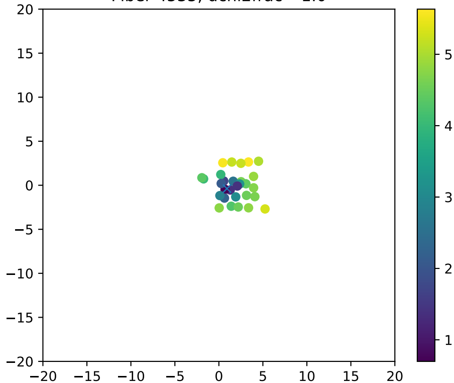
Fiber 4535, dchi2frac= 1.0
