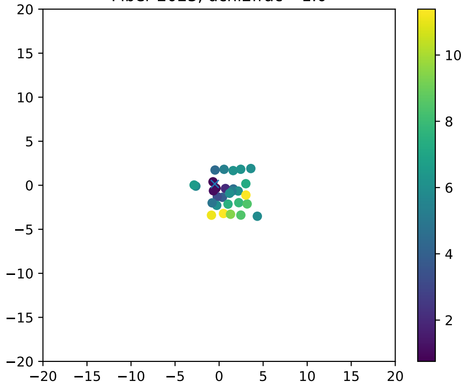
Fiber 2023, dchi2frac= 1.0
