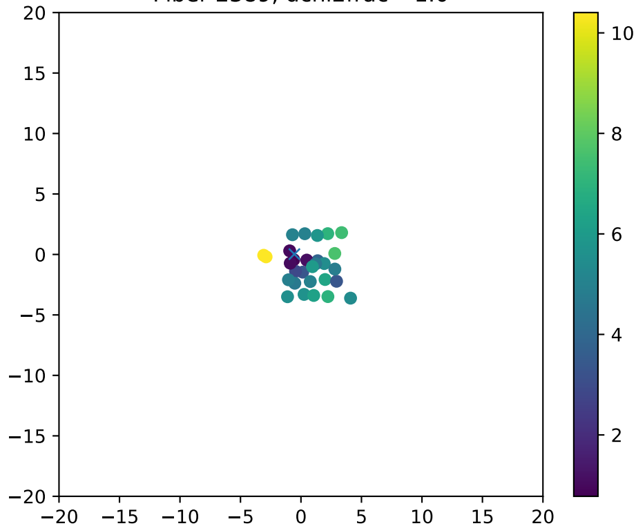
Fiber 2389, dchi2frac= 1.0
