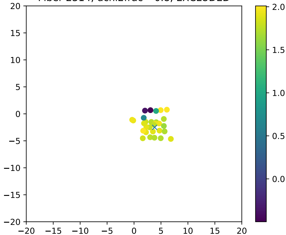
Fiber 2314, dchi2frac= 0.8, EXCLUDED
