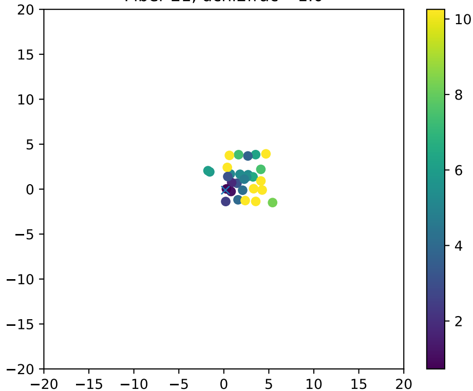
Fiber 21, dchi2frac= 1.0
