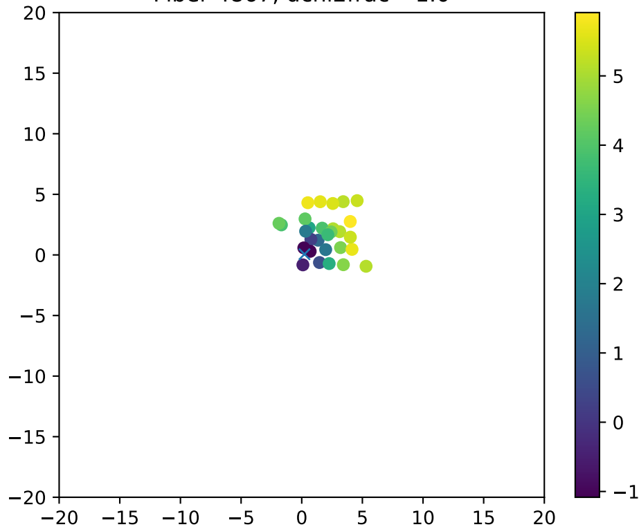
Fiber 4867, dchi2frac= 1.0
