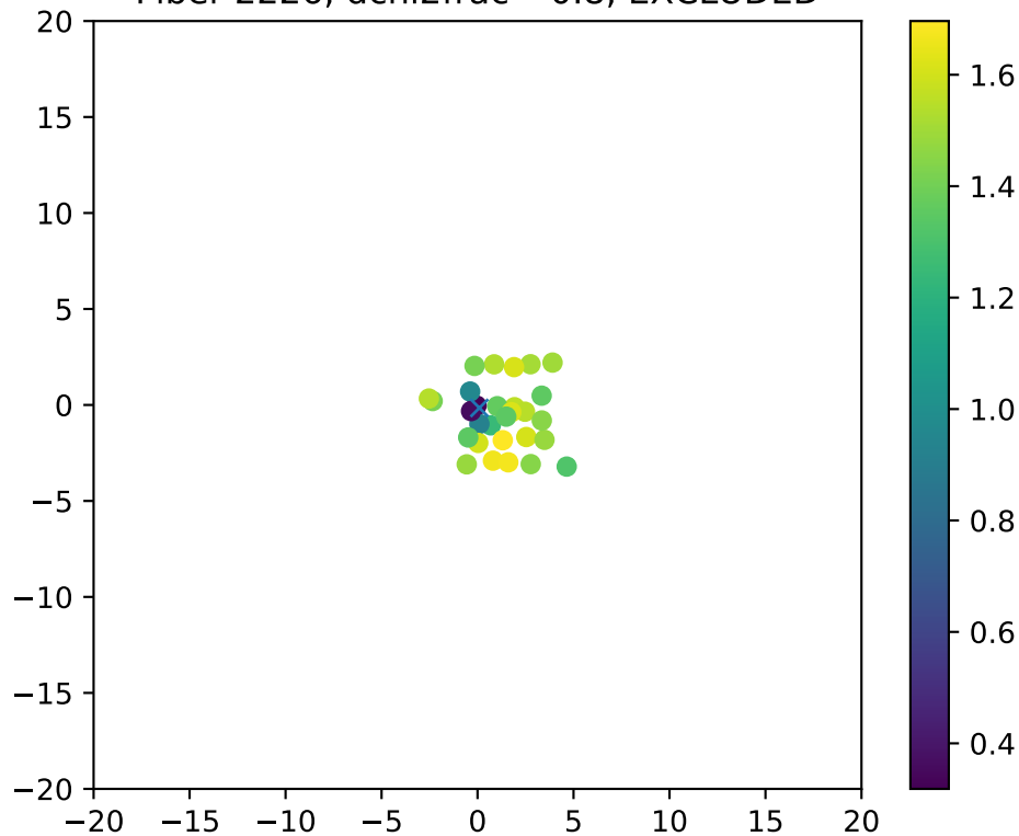
Fiber 2226, dchi2frac= 0.8, EXCLUDED
