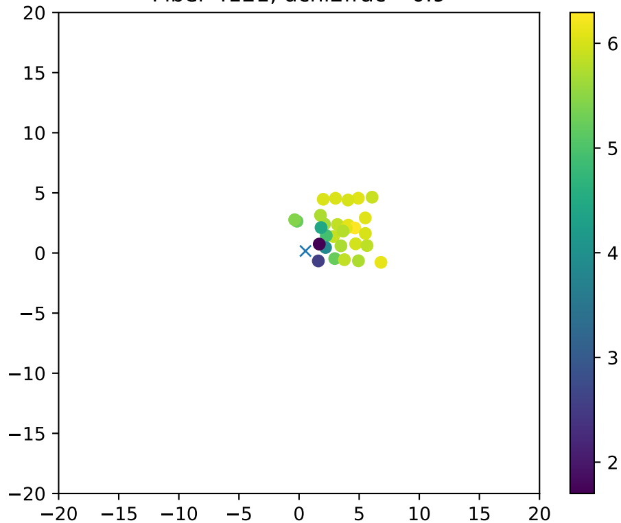
Fiber 4121, dchi2frac= 0.9
