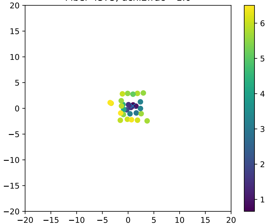
Fiber 4375, dchi2frac= 1.0
