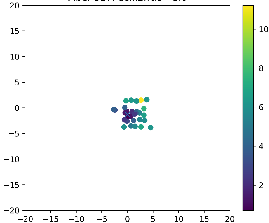
Fiber 517, dchi2frac= 1.0
