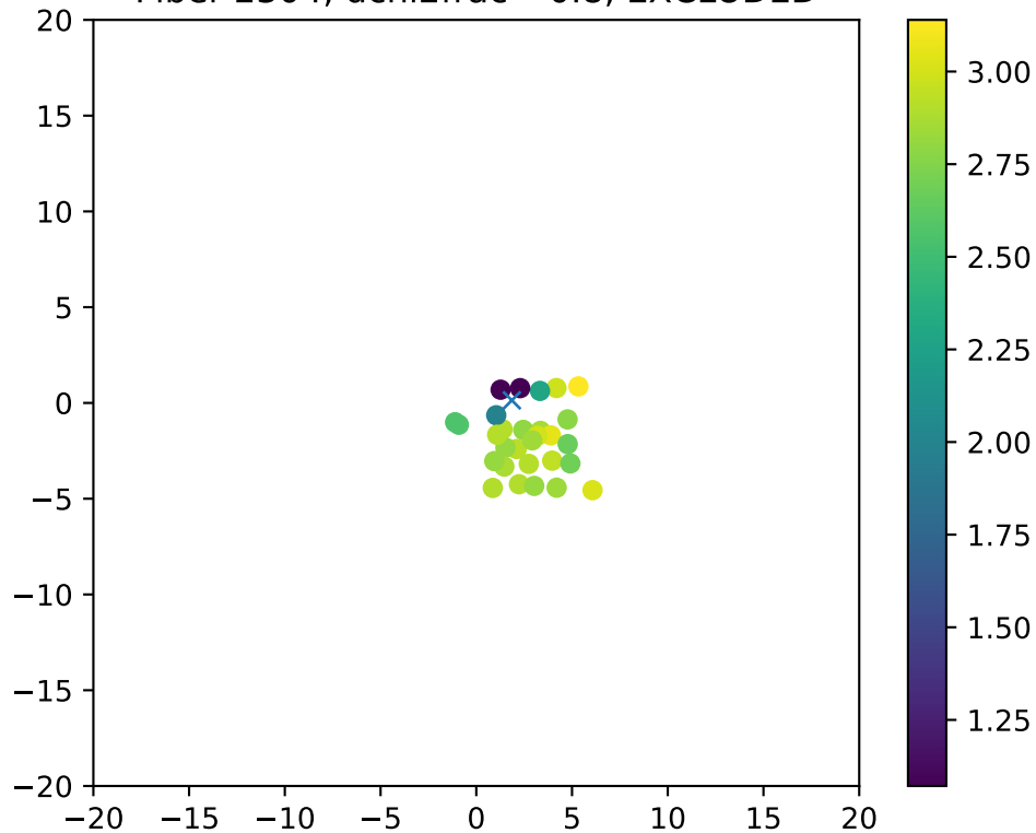
Fiber 2304, dchi2frac= 0.8, EXCLUDED
