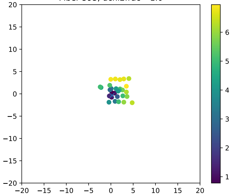
Fiber 593, dchi2frac= 1.0
