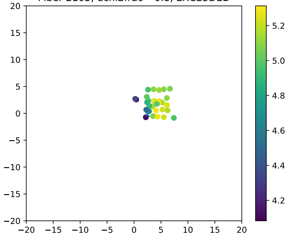
Fiber 2105, dchi2frac= 0.8, EXCLUDED
