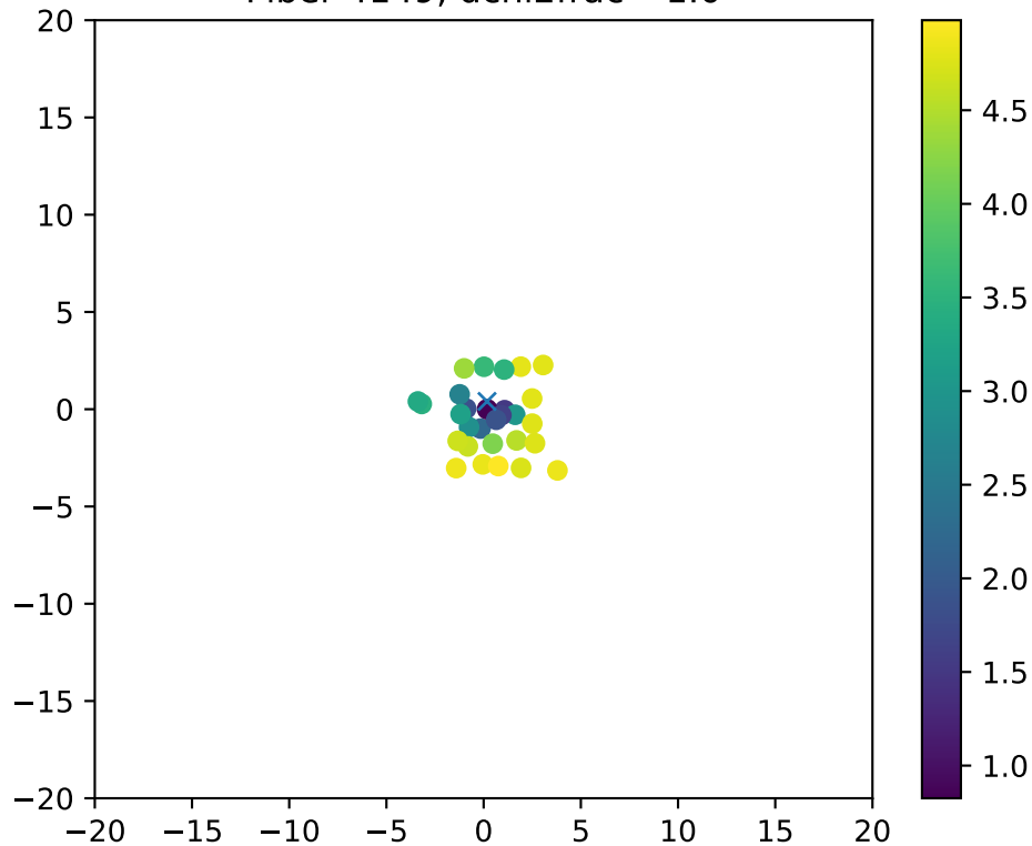
Fiber 4149, dchi2frac= 1.0
