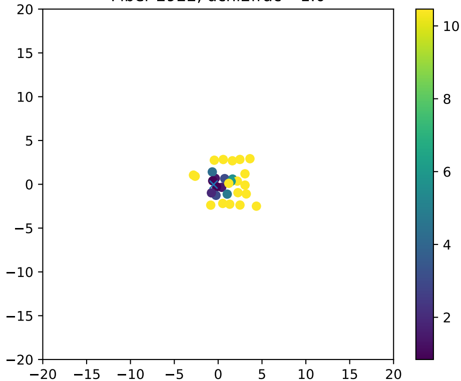
Fiber 2922, dchi2frac= 1.0
