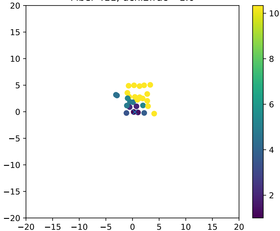
Fiber 411, dchi2frac= 1.0
