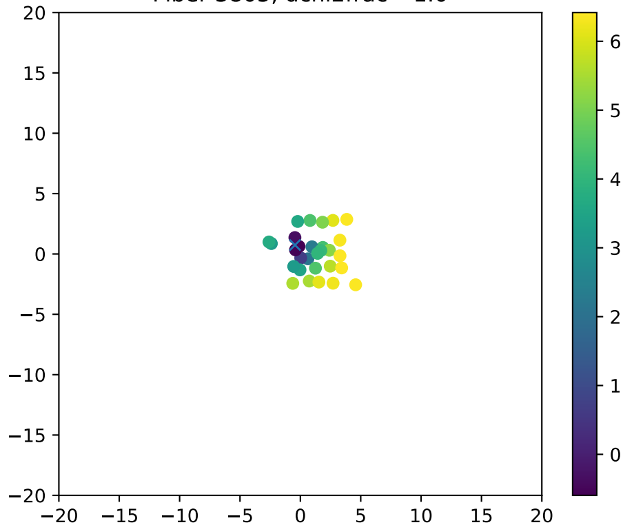
Fiber 3805, dchi2frac= 1.0
