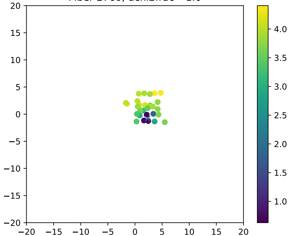
Fiber 2760, dchi2frac= 1.0
