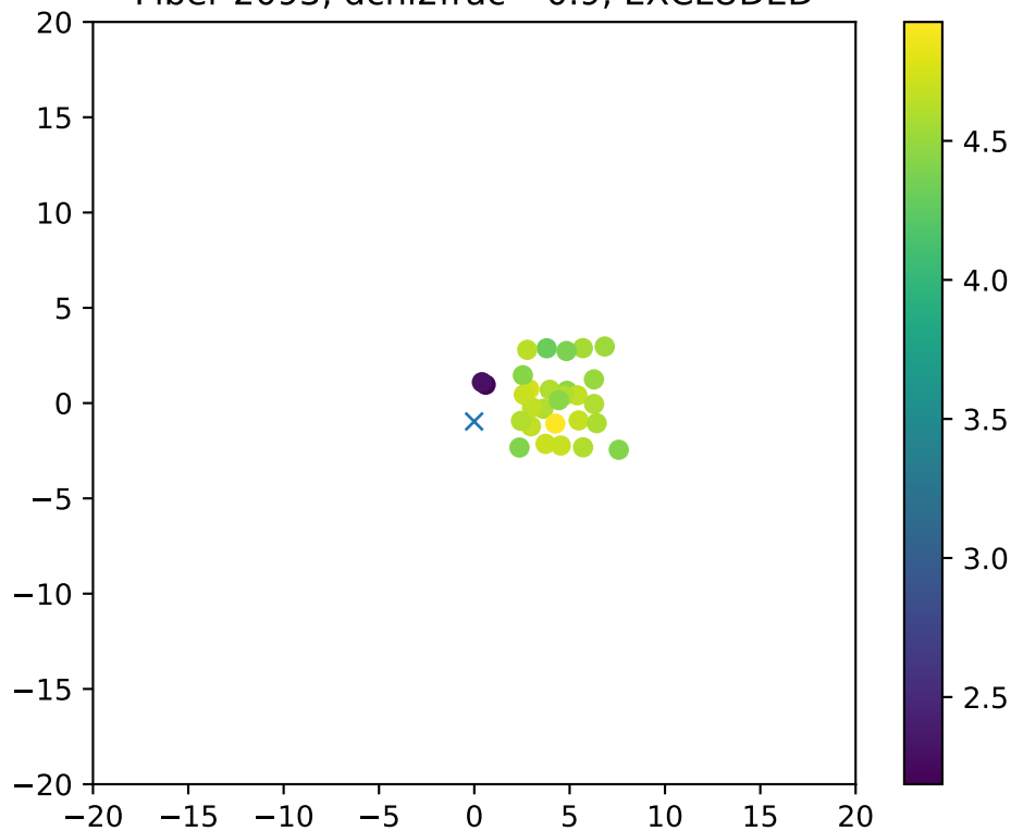
Fiber 2093, dchi2frac= 0.9, EXCLUDED
