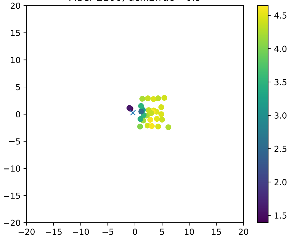
Fiber 2106, dchi2frac= 0.9
