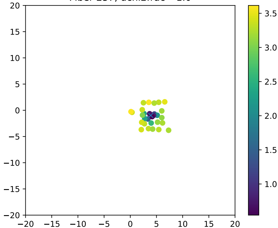
Fiber 237, dchi2frac= 1.0
