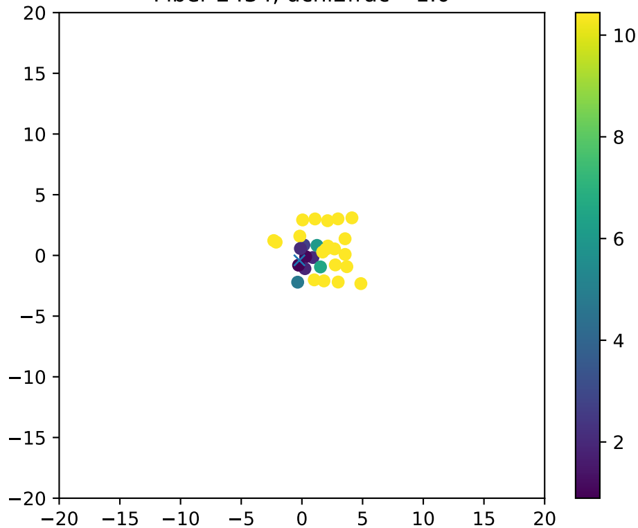
Fiber 2434, dchi2frac= 1.0
