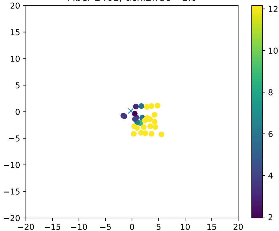
Fiber 2461, dchi2frac= 1.0
