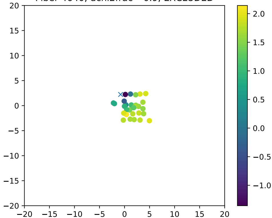
Fiber 4640, dchi2frac= 0.9, EXCLUDED
