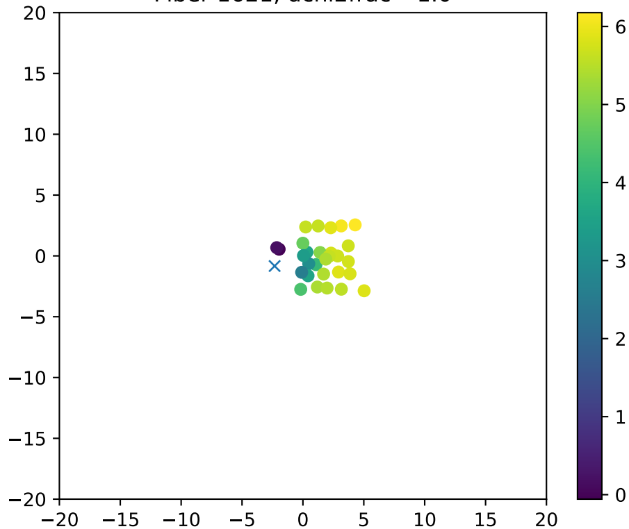
Fiber 1621, dchi2frac= 1.0
