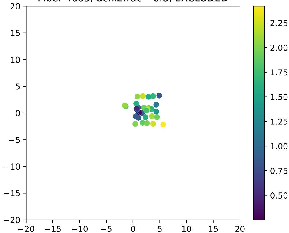
Fiber 4685, dchi2frac= 0.8, EXCLUDED
