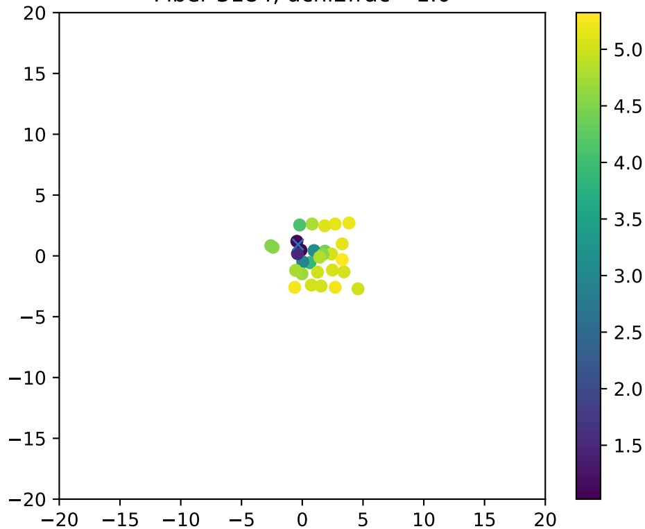
Fiber 3184, dchi2frac= 1.0
