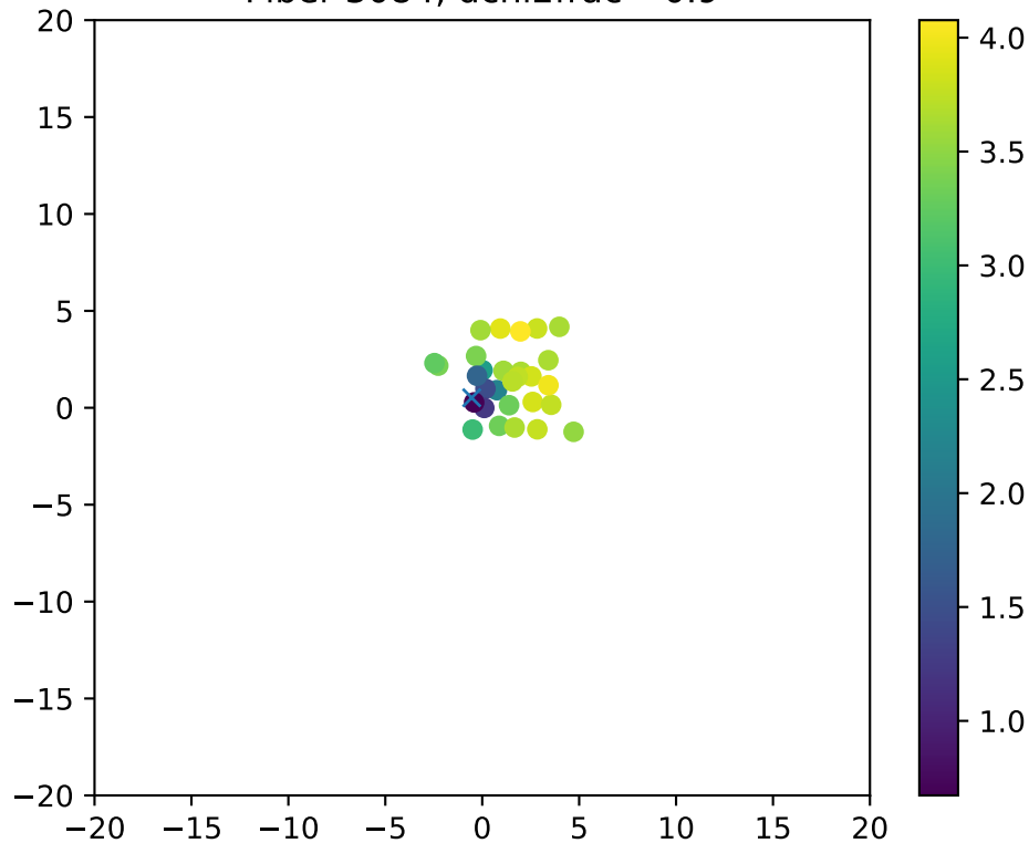
Fiber 3084, dchi2frac= 0.9
