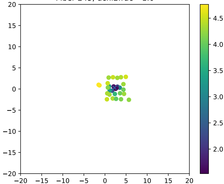
Fiber 245, dchi2frac= 1.0
