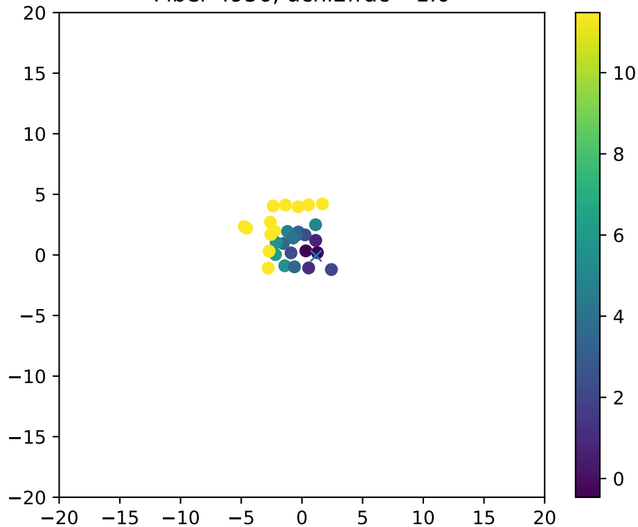
Fiber 4956, dchi2frac= 1.0
