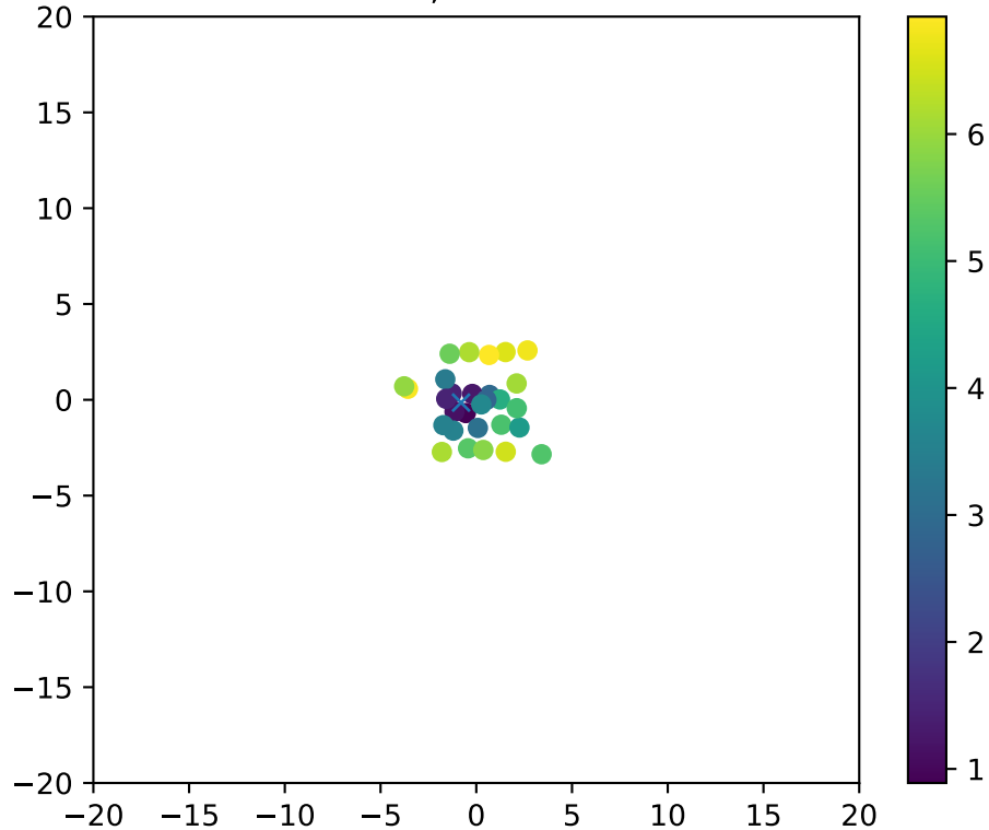
Fiber 3029, dchi2frac= 1.0
