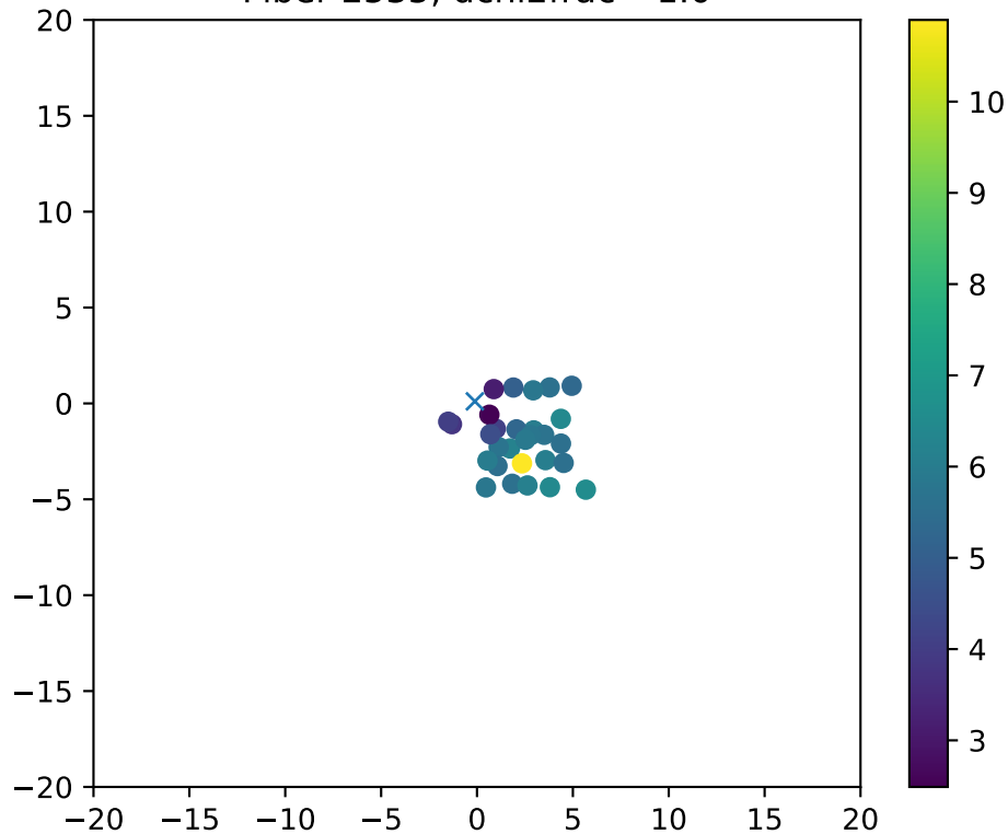
Fiber 2535, dchi2frac= 1.0
