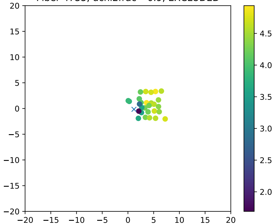
Fiber 4735, dchi2frac= 0.9, EXCLUDED
