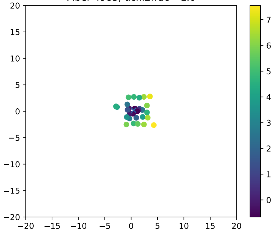
Fiber 4983, dchi2frac= 1.0
