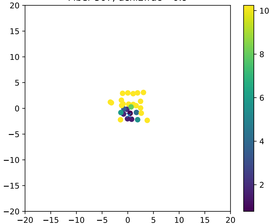
Fiber 507, dchi2frac= 0.9
