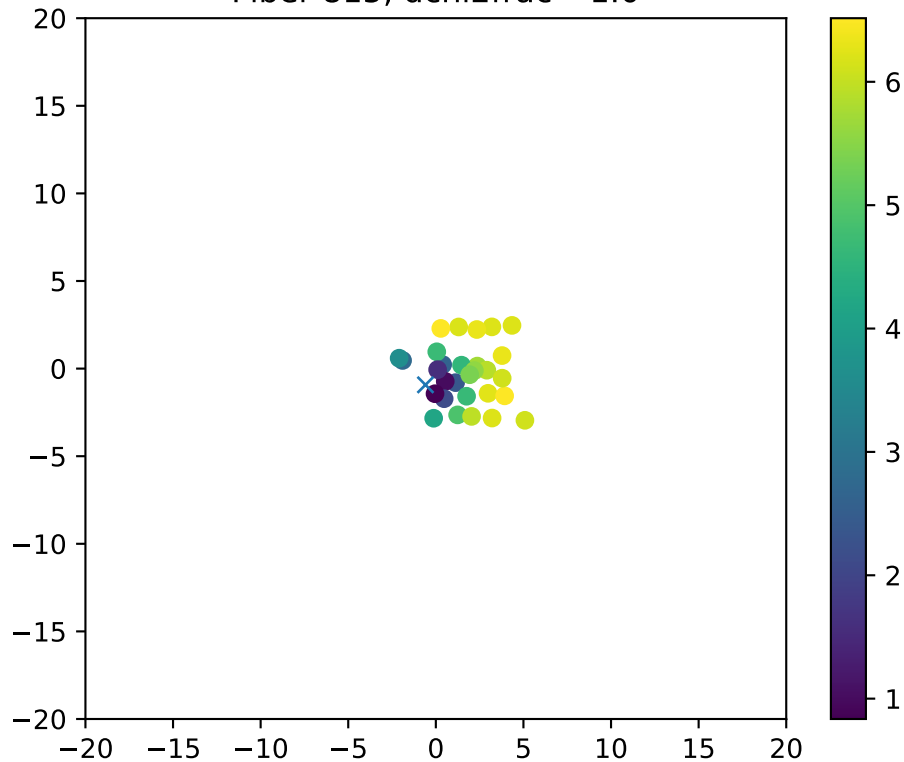
Fiber 815, dchi2frac= 1.0
