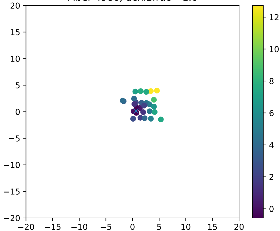
Fiber 4986, dchi2frac= 1.0
