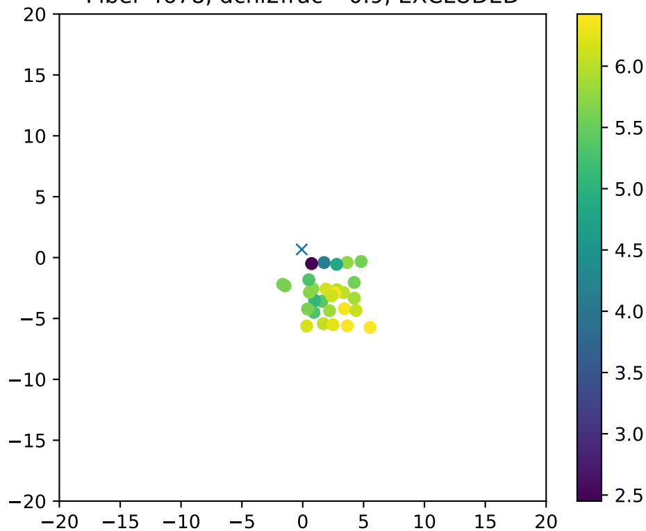
Fiber 4678, dchi2frac= 0.9, EXCLUDED
