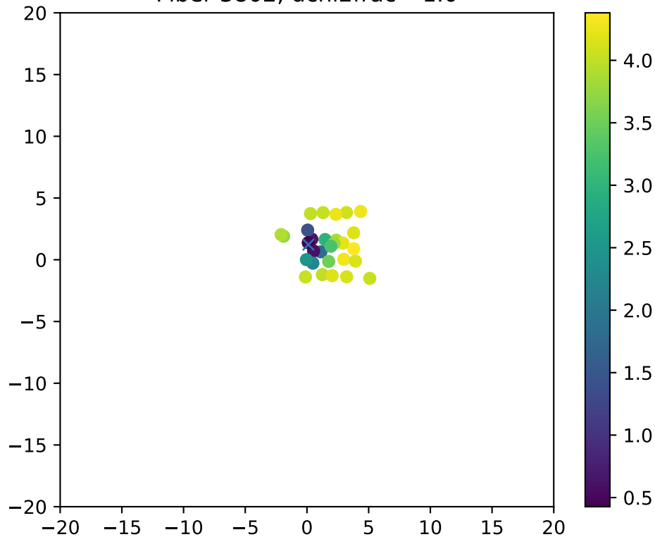
Fiber 3802, dchi2frac= 1.0
