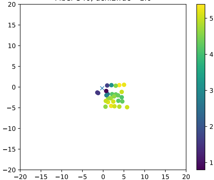
Fiber 340, dchi2frac= 1.0
