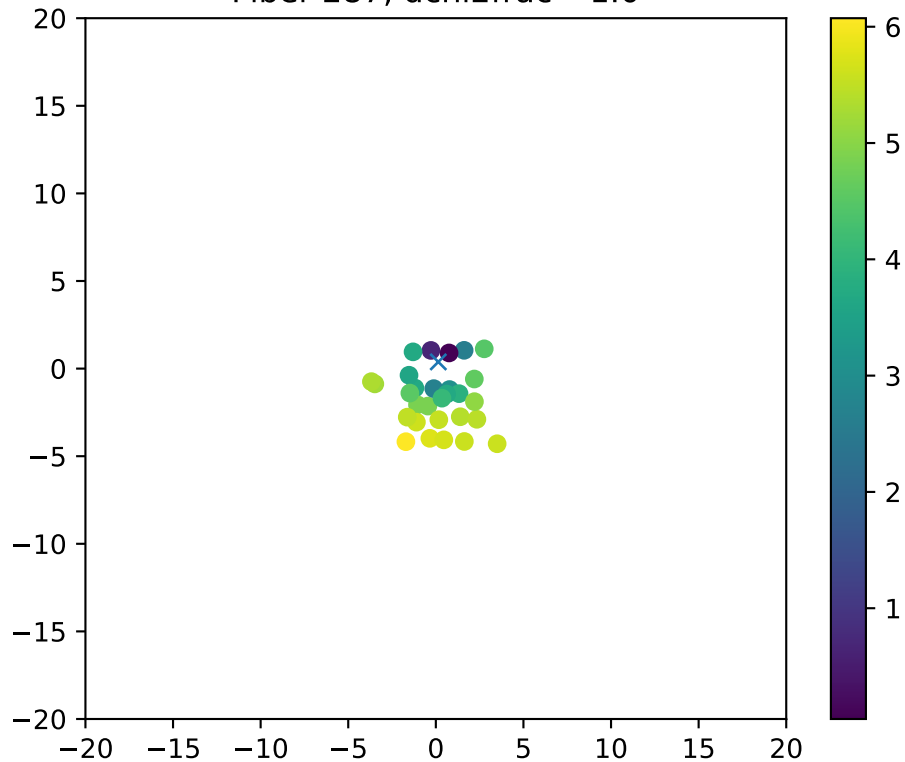
Fiber 287, dchi2frac= 1.0
