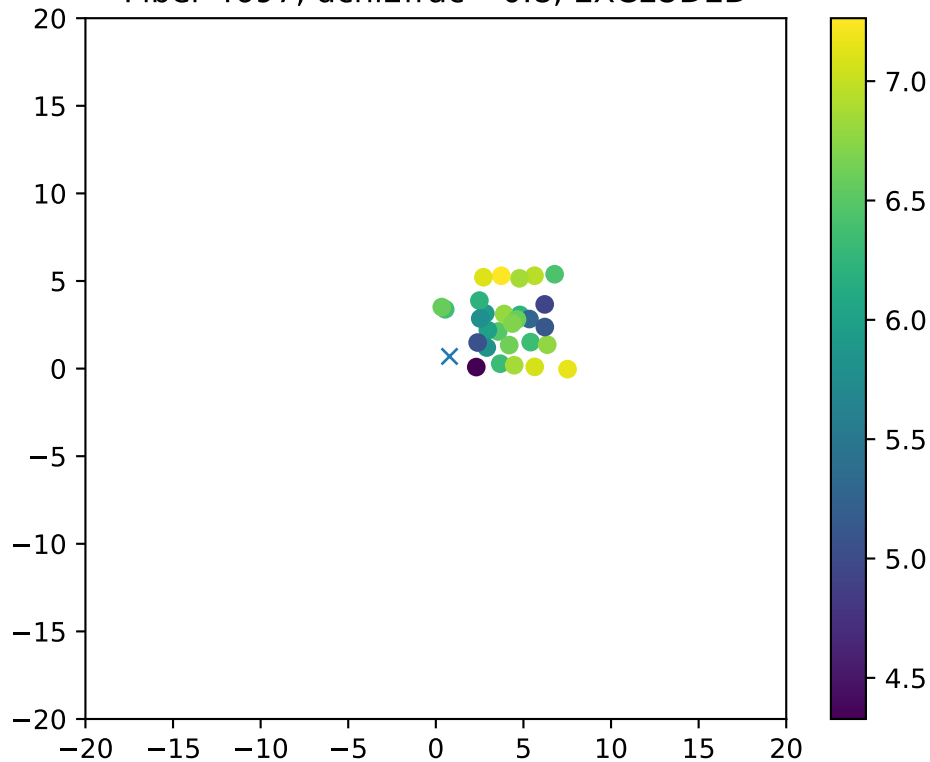
Fiber 4697, dchi2frac= 0.8, EXCLUDED
