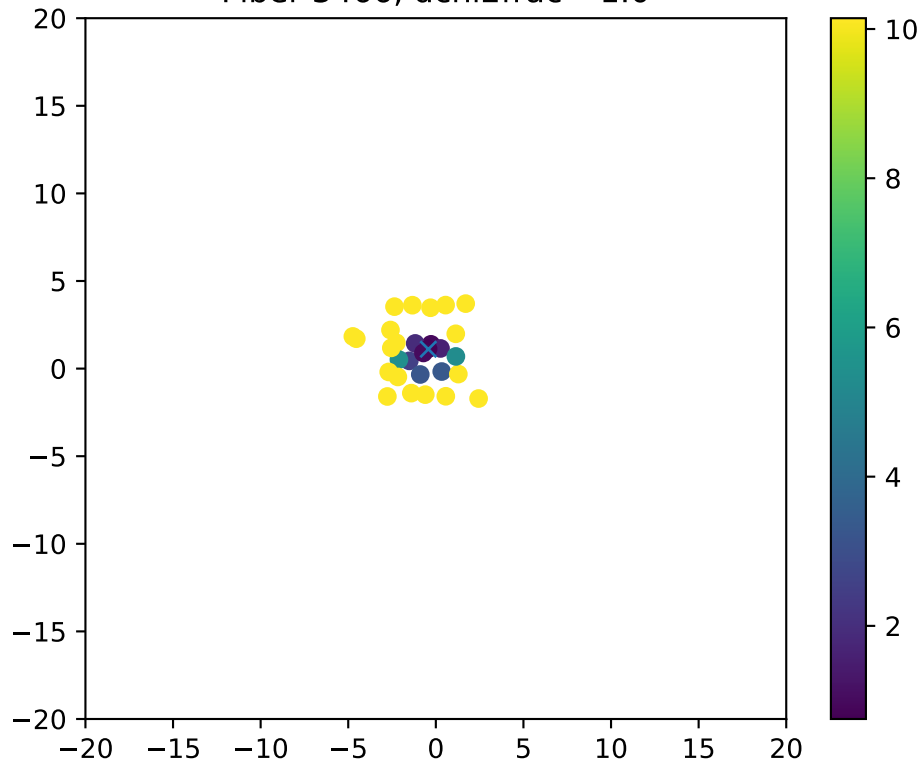
Fiber 3466, dchi2frac= 1.0
