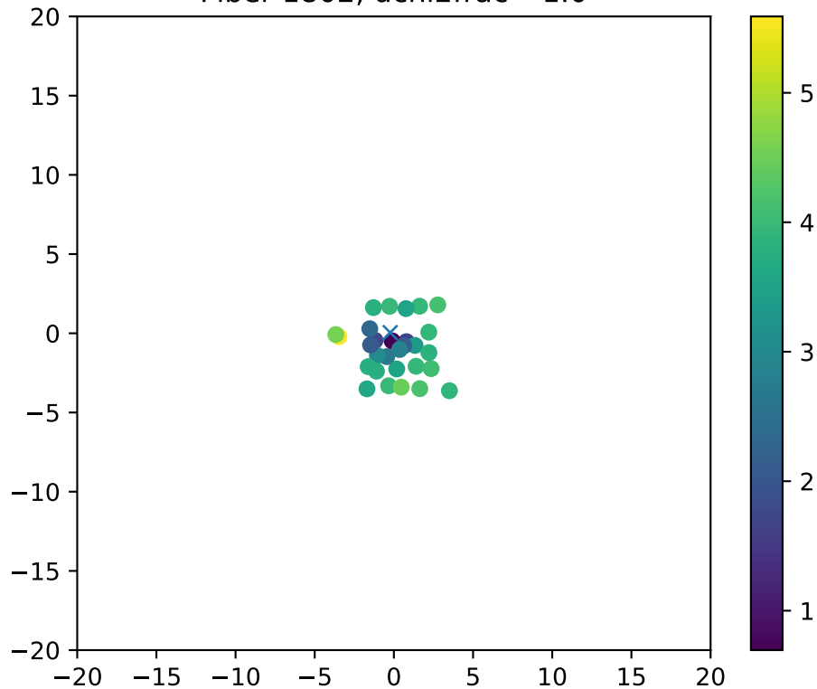
Fiber 1802, dchi2frac= 1.0
