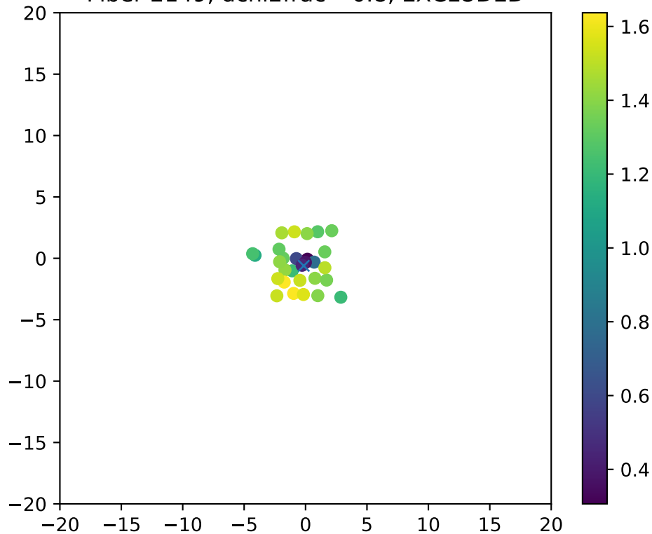
Fiber 2149, dchi2frac= 0.8, EXCLUDED
