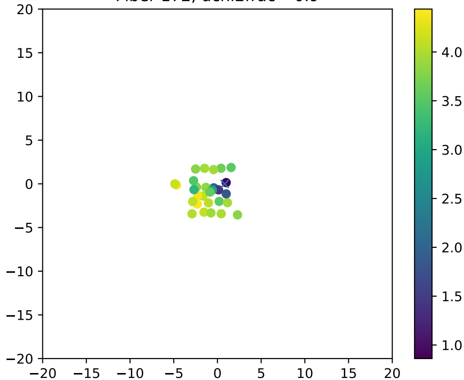
Fiber 172, dchi2frac= 0.9
