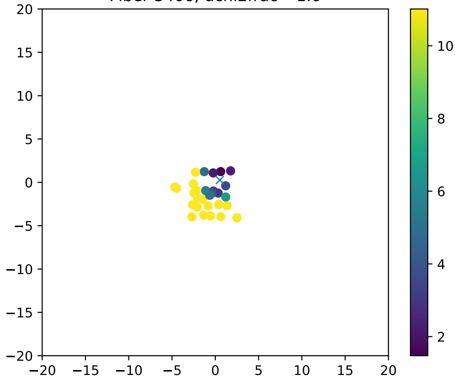
Fiber 3406, dchi2frac= 1.0
