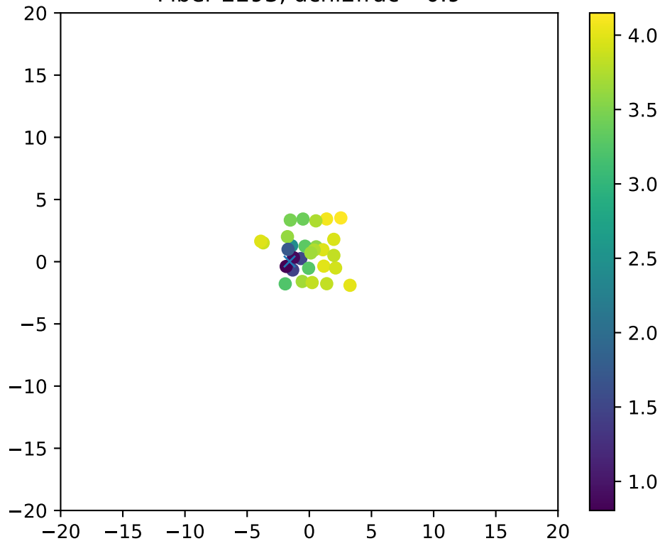
Fiber 2293, dchi2frac= 0.9
