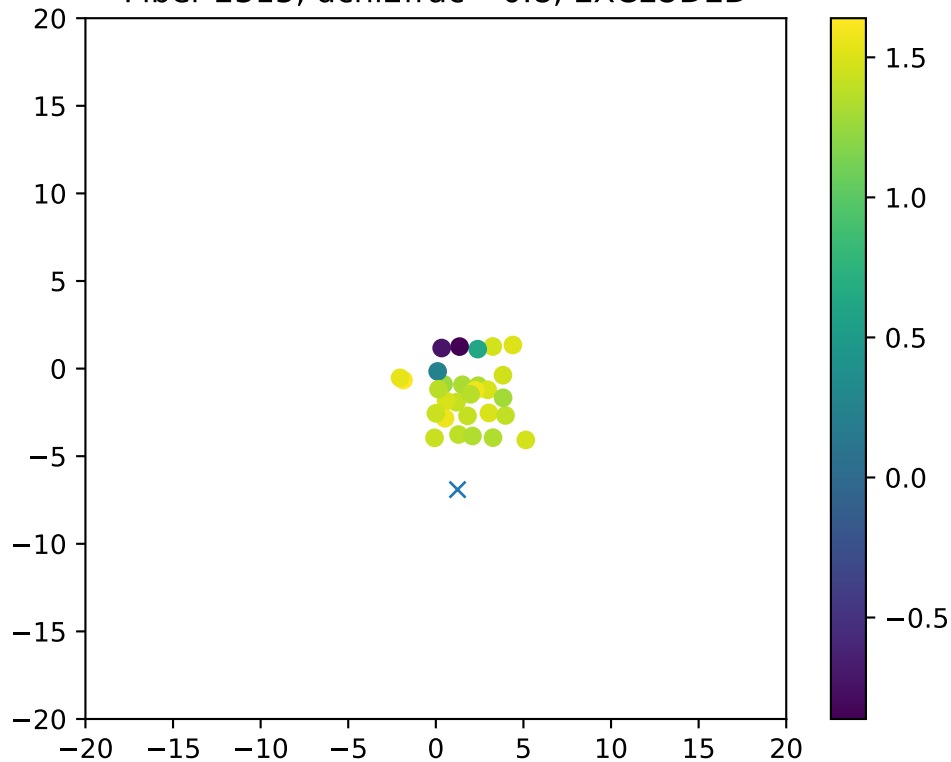
Fiber 2315, dchi2frac= 0.8, EXCLUDED
