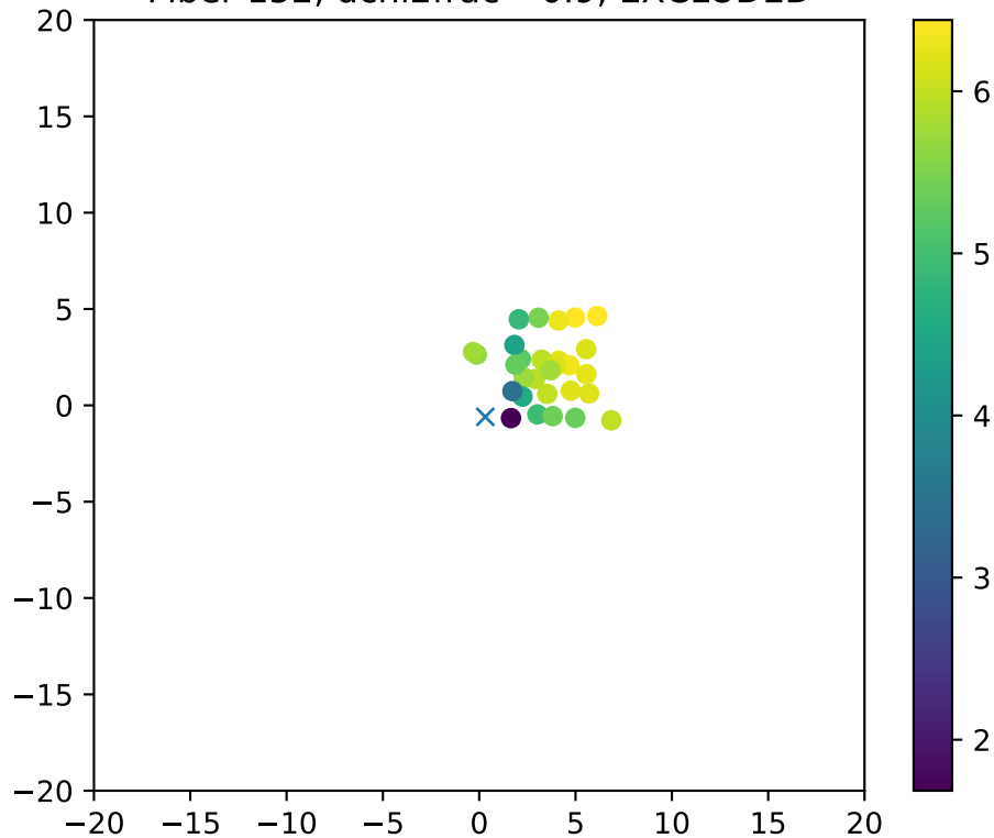
Fiber 152, dchi2frac= 0.9, EXCLUDED
