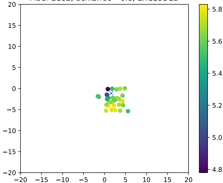
Fiber 2182, dchi2frac= 0.8, EXCLUDED
