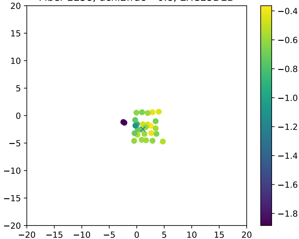
Fiber 2258, dchi2frac= 0.8, EXCLUDED
