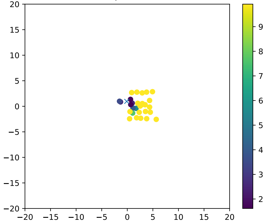
Fiber 3928, dchi2frac= 1.0
