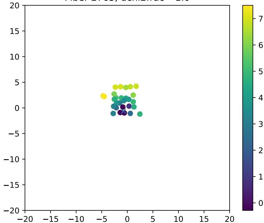
Fiber 2763, dchi2frac= 1.0
