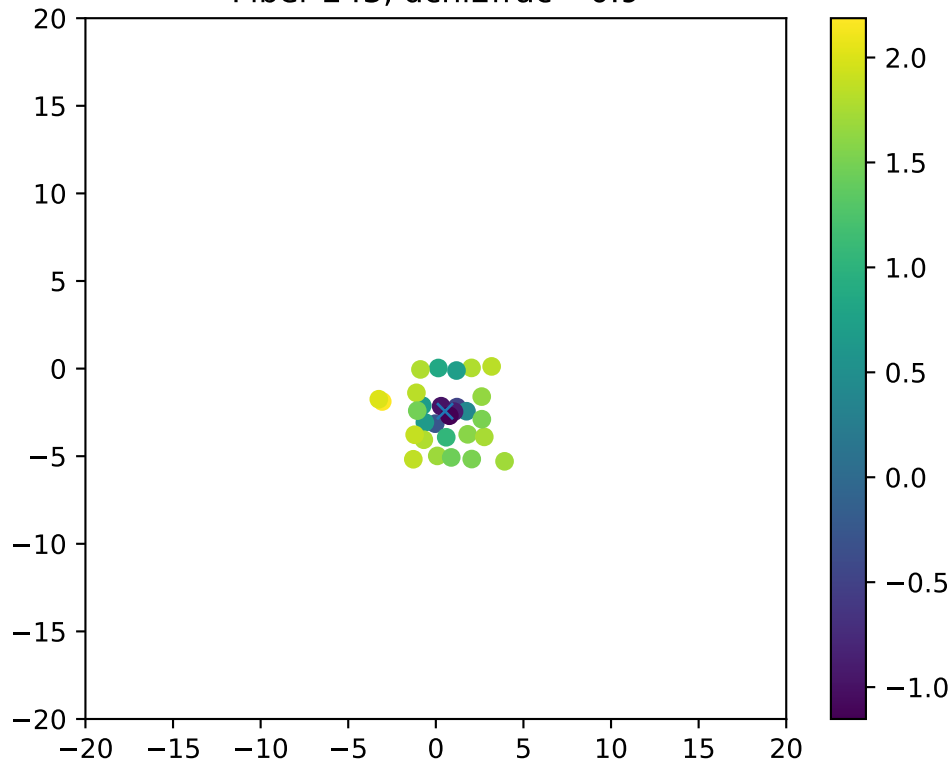
Fiber 243, dchi2frac= 0.9
