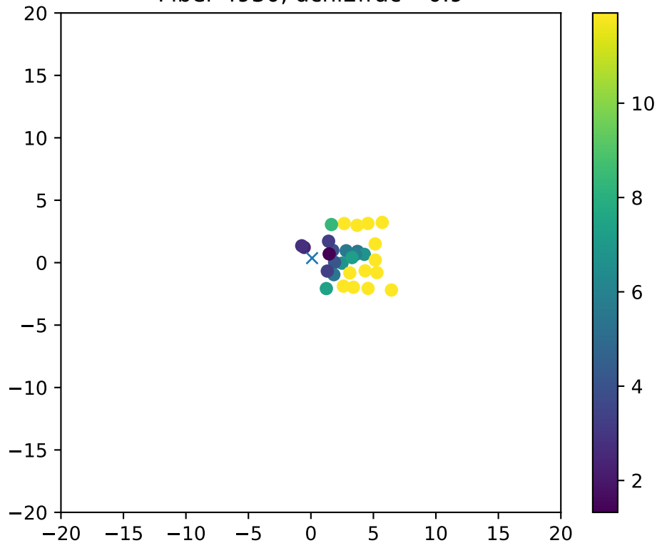
Fiber 4930, dchi2frac= 0.9
