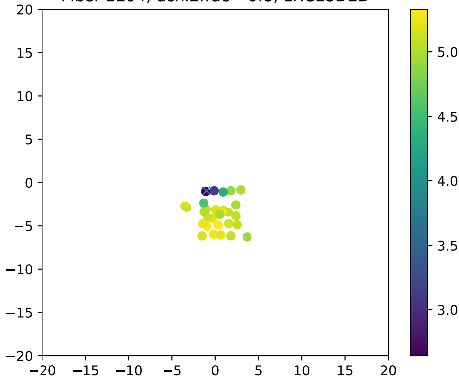
Fiber 2204, dchi2frac= 0.8, EXCLUDED
