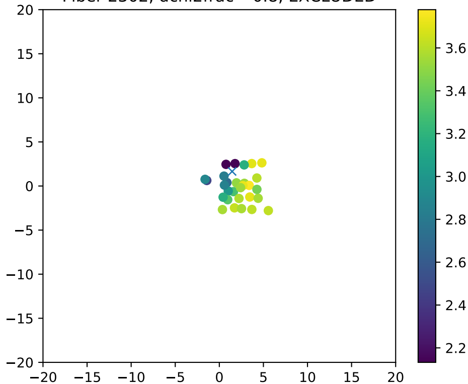
Fiber 2302, dchi2frac= 0.8, EXCLUDED
