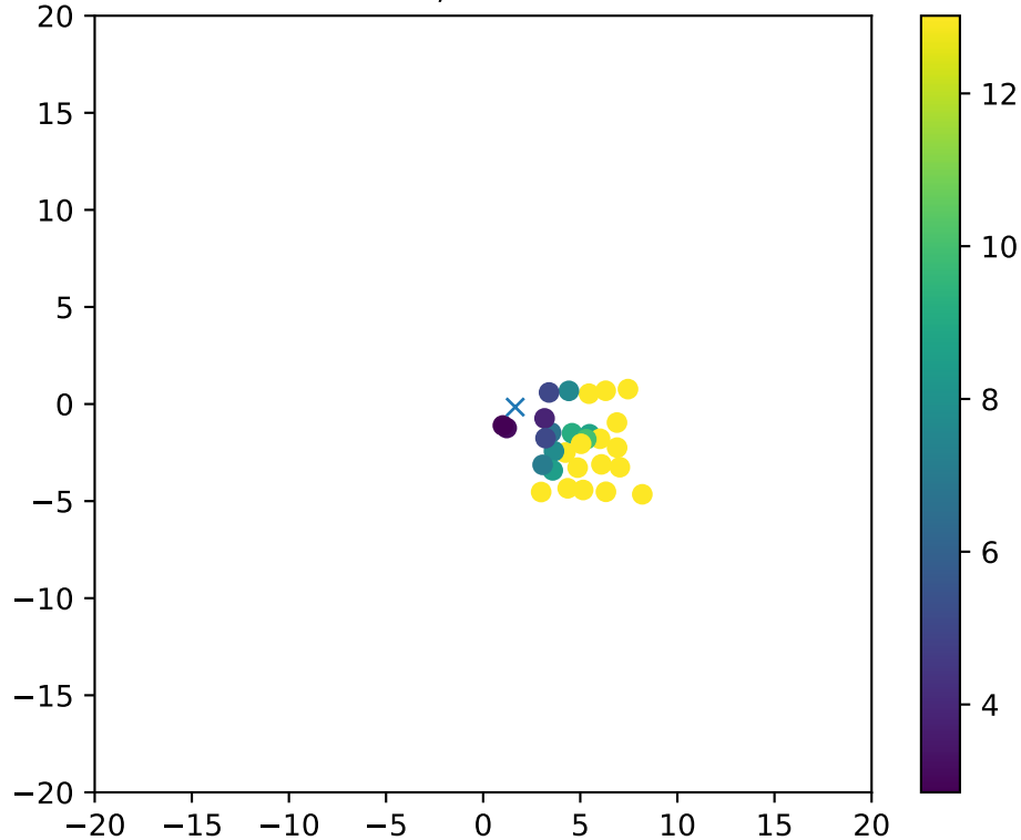
Fiber 4938, dchi2frac= 1.0
