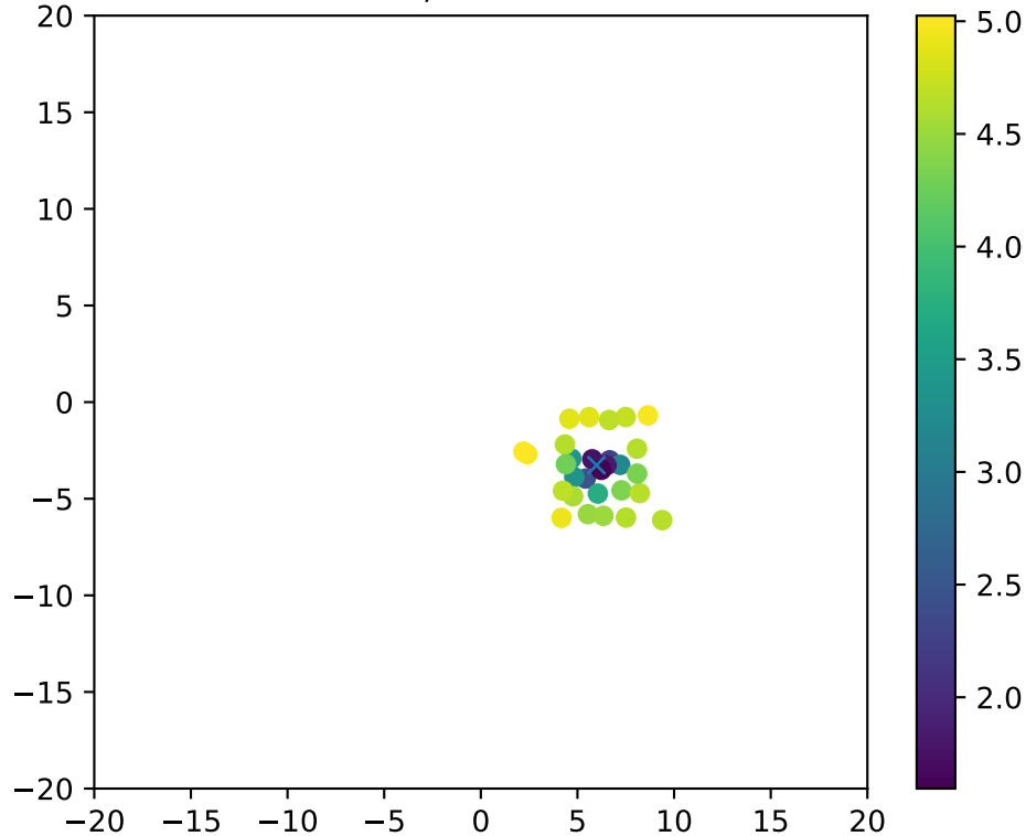
Fiber 242, dchi2frac= 1.0
