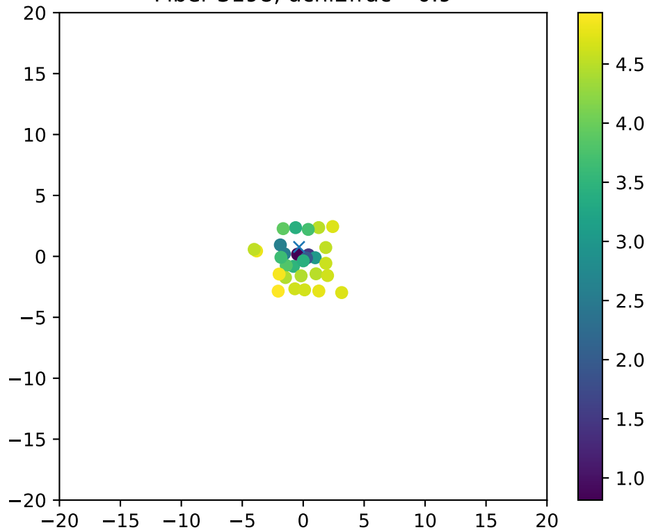
Fiber 3198, dchi2frac= 0.9
