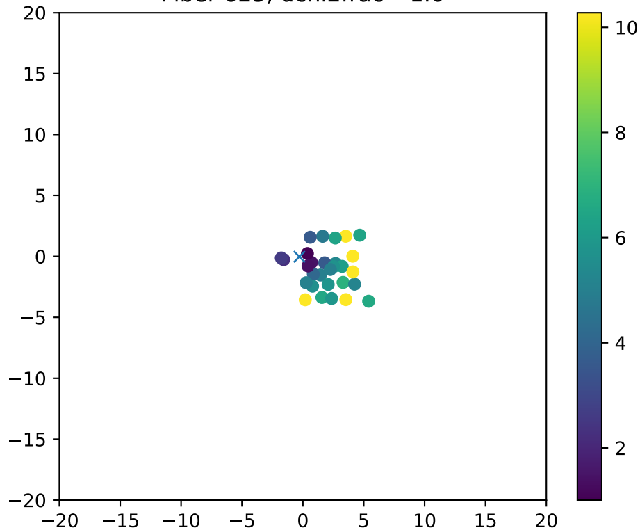
Fiber 625, dchi2frac= 1.0
