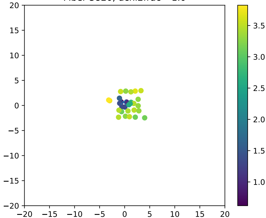
Fiber 3820, dchi2frac= 1.0
