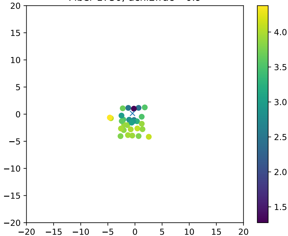
Fiber 1730, dchi2frac= 0.9
