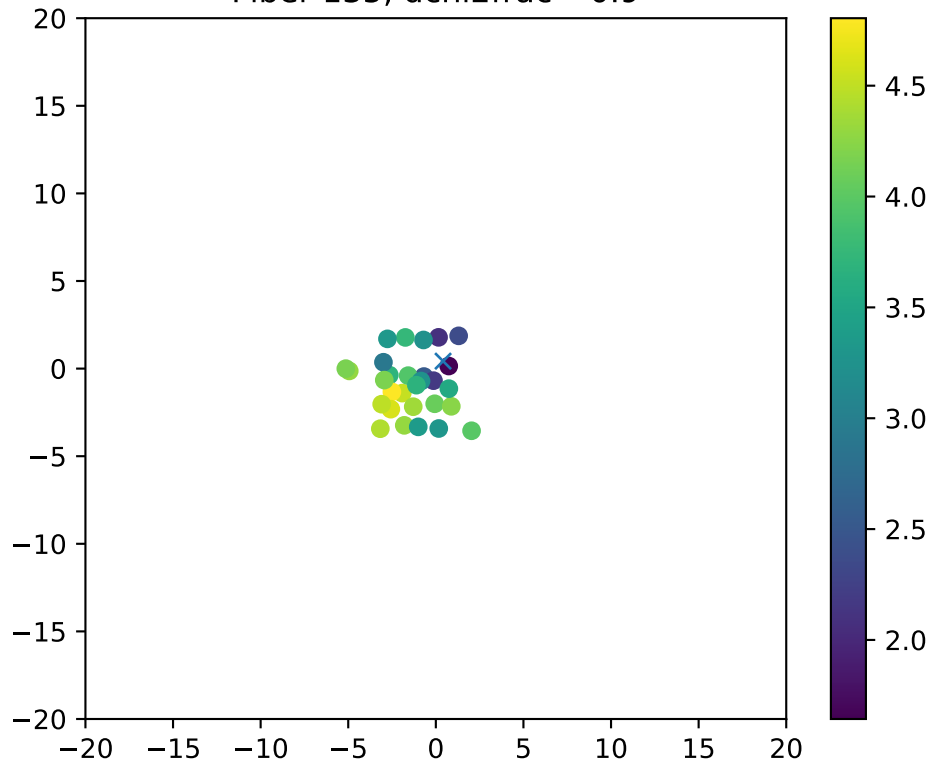
Fiber 135, dchi2frac= 0.9
