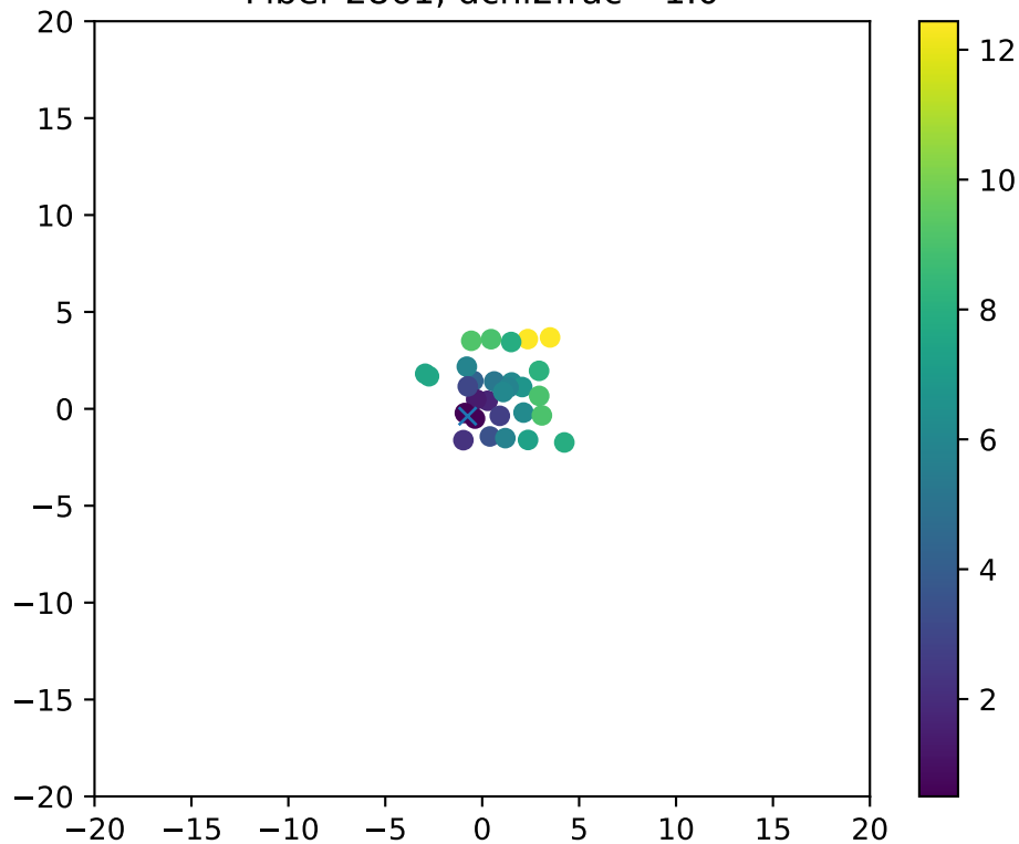
Fiber 2861, dchi2frac= 1.0
