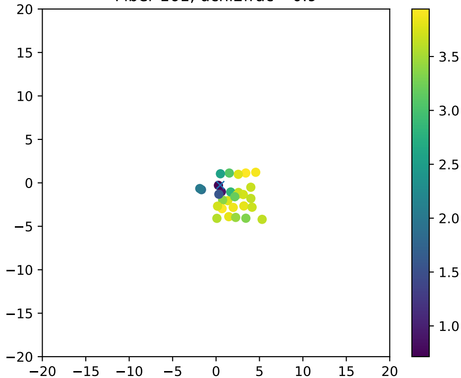
Fiber 161, dchi2frac= 0.9
