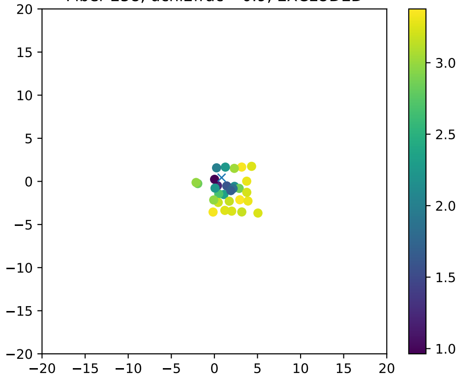
Fiber 258, dchi2frac= 0.9, EXCLUDED
