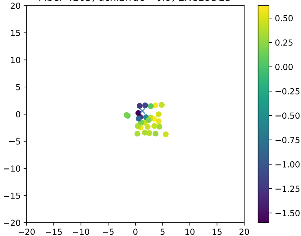
Fiber 4205, dchi2frac= 0.9, EXCLUDED
