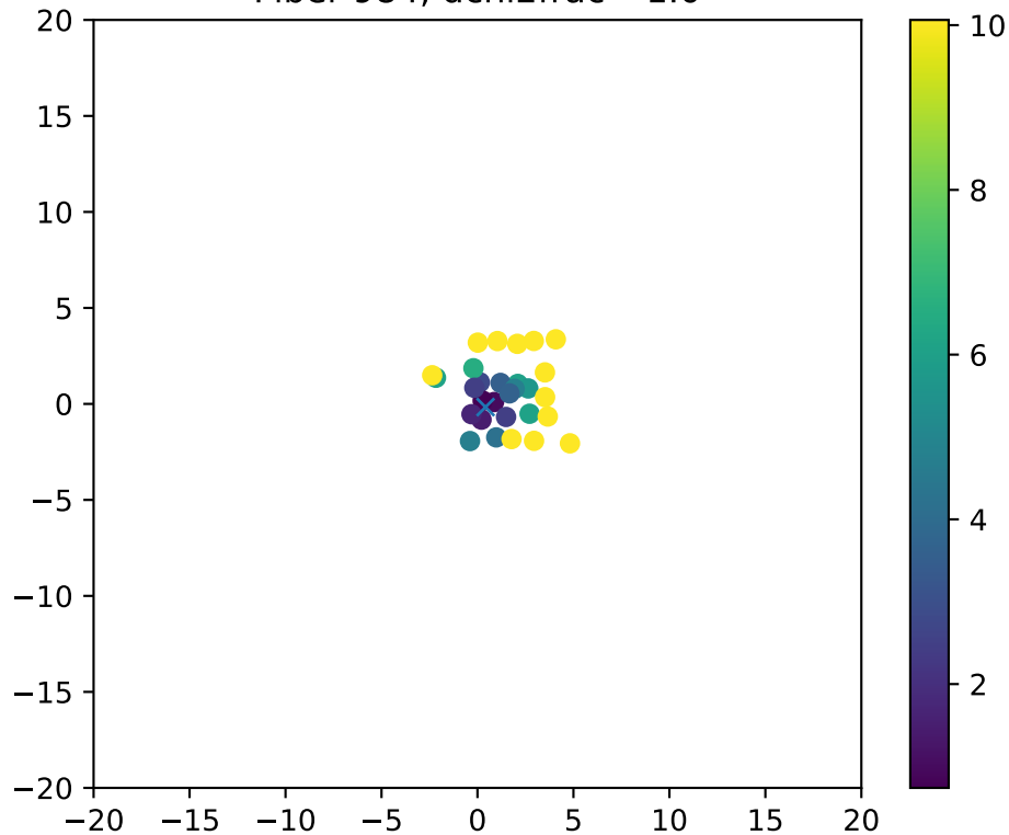
Fiber 984, dchi2frac= 1.0
