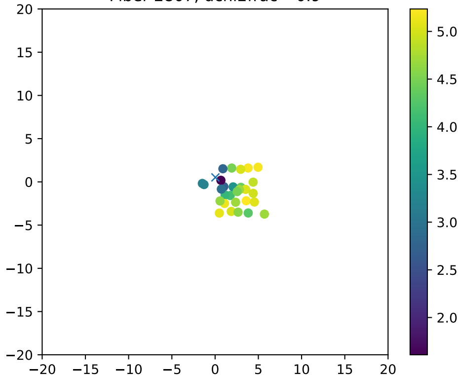
Fiber 2807, dchi2frac= 0.9
