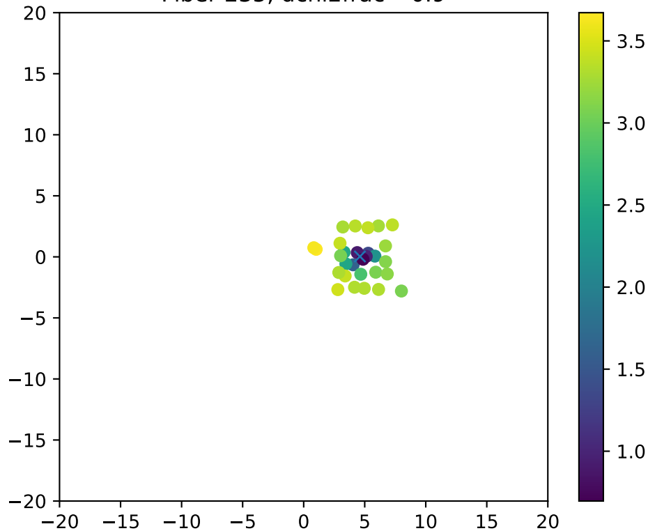
Fiber 235, dchi2frac= 0.9
