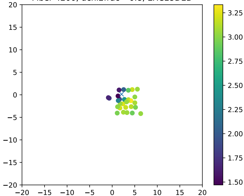
Fiber 4200, dchi2frac= 0.8, EXCLUDED
