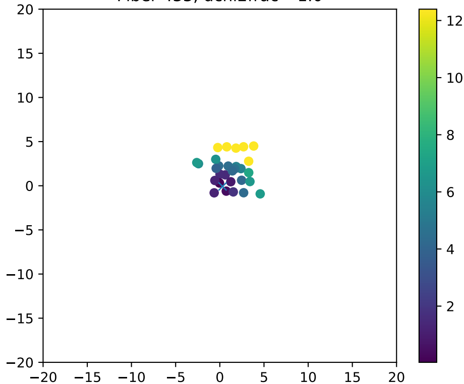
Fiber 433, dchi2frac= 1.0
