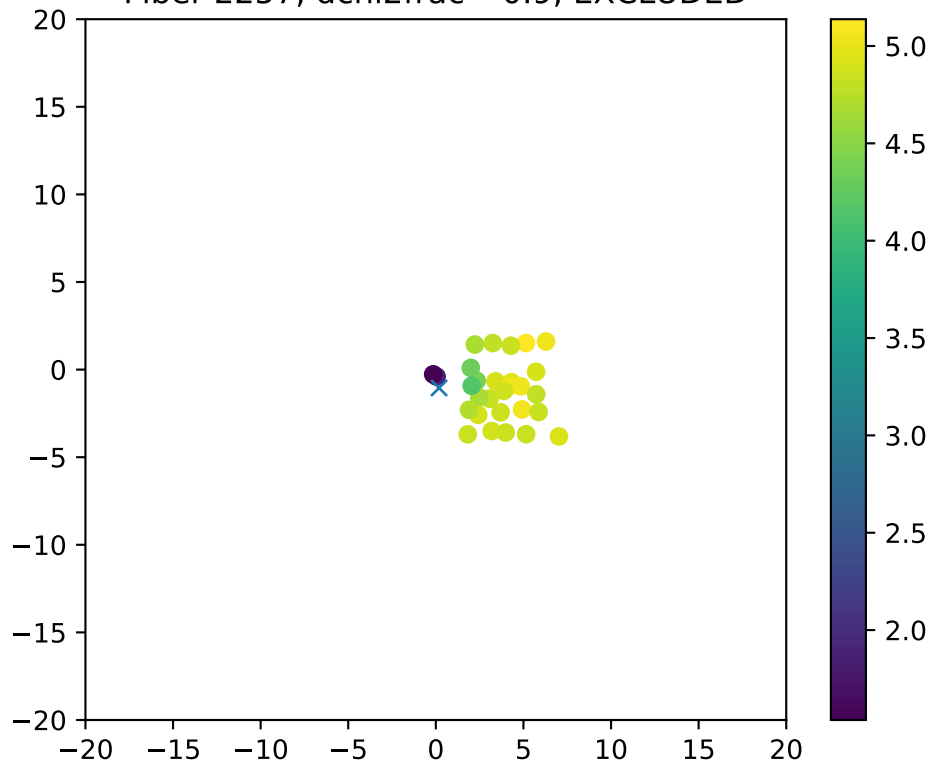
Fiber 2257, dchi2frac= 0.9, EXCLUDED
