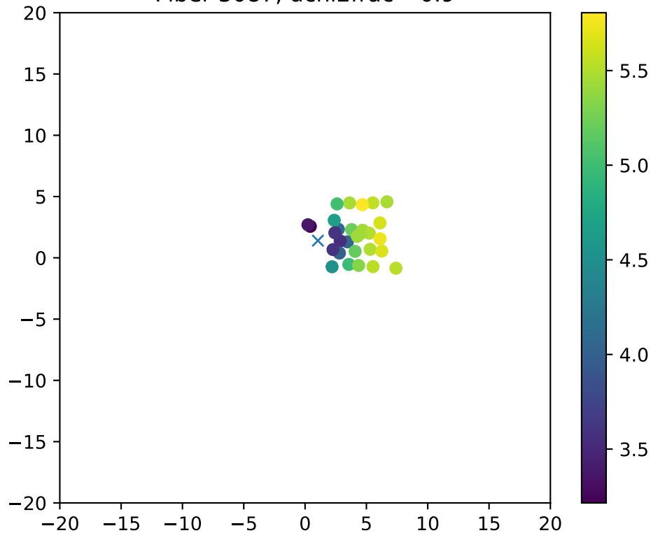
Fiber 3087, dchi2frac= 0.9
