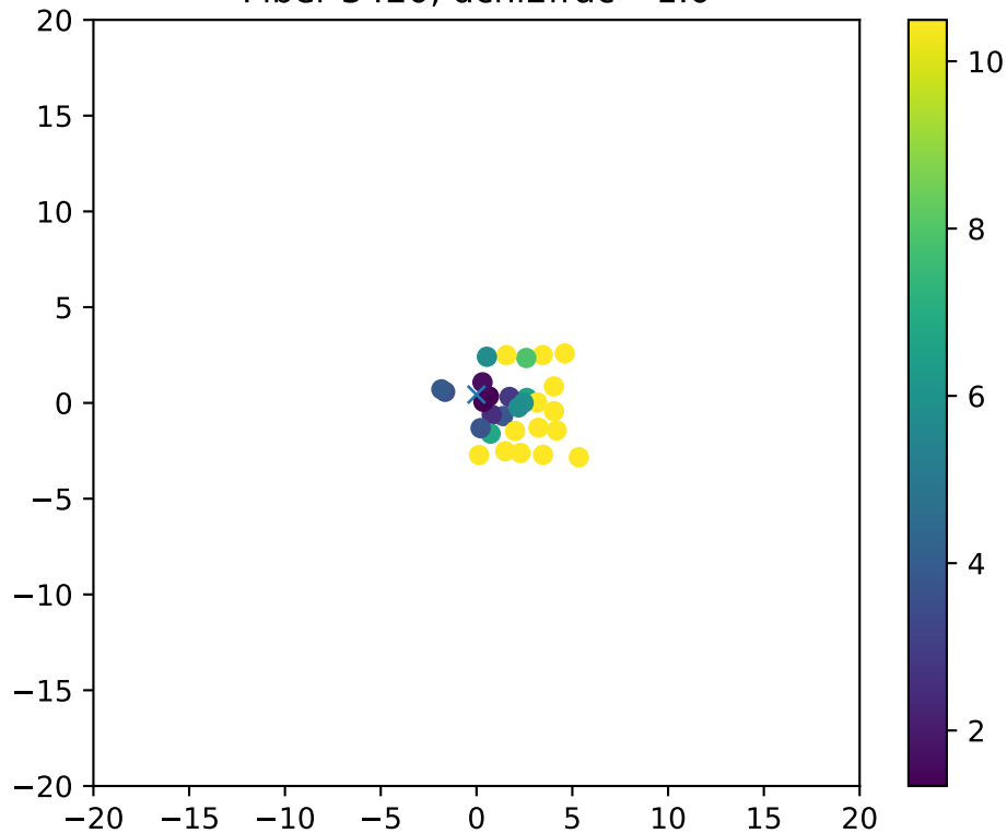
Fiber 3420, dchi2frac= 1.0
