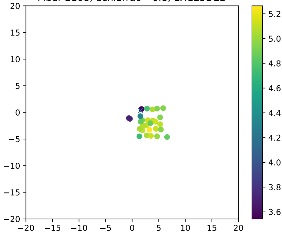
Fiber 2108, dchi2frac= 0.8, EXCLUDED
