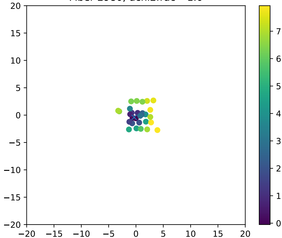
Fiber 2980, dchi2frac= 1.0
