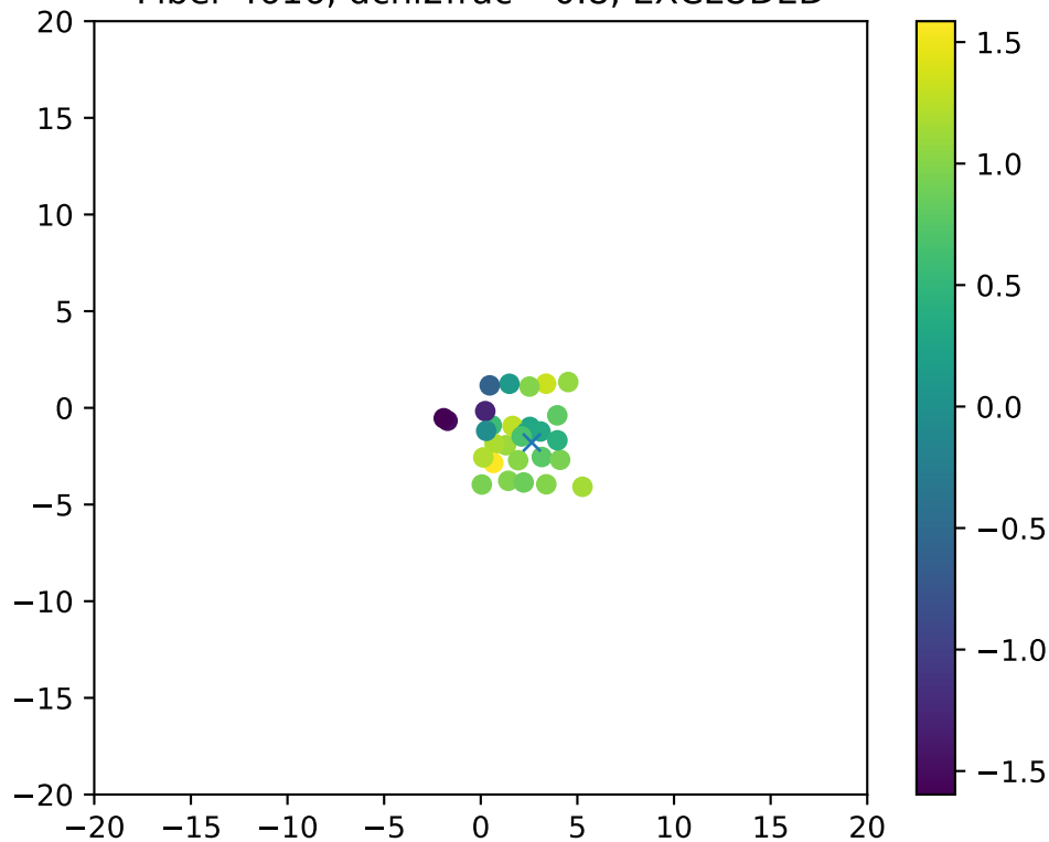
Fiber 4616, dchi2frac= 0.8, EXCLUDED
