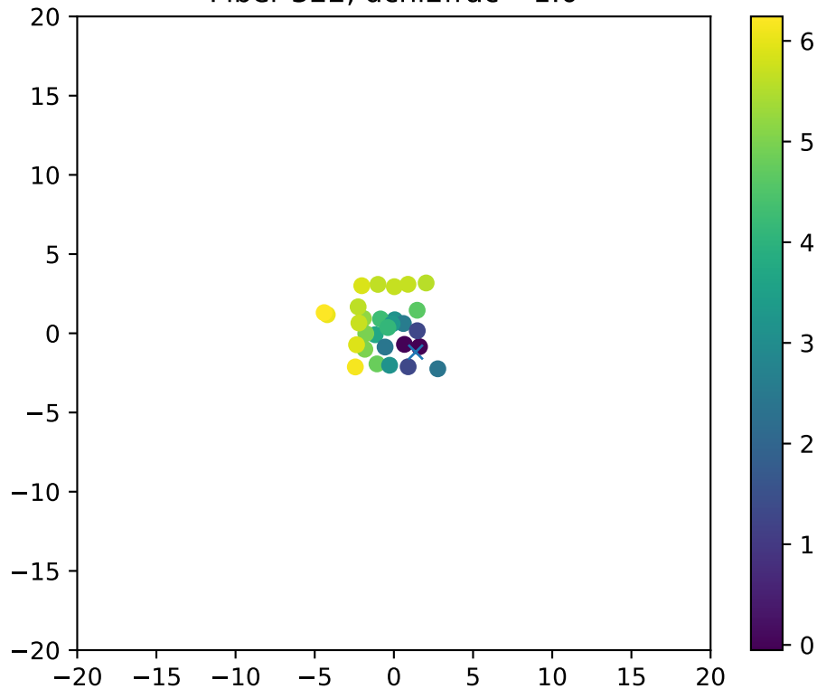
Fiber 322, dchi2frac= 1.0
