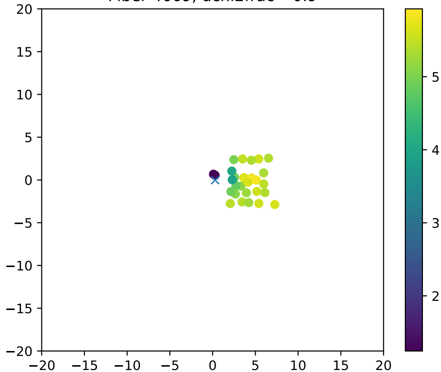
Fiber 4669, dchi2frac= 0.9
