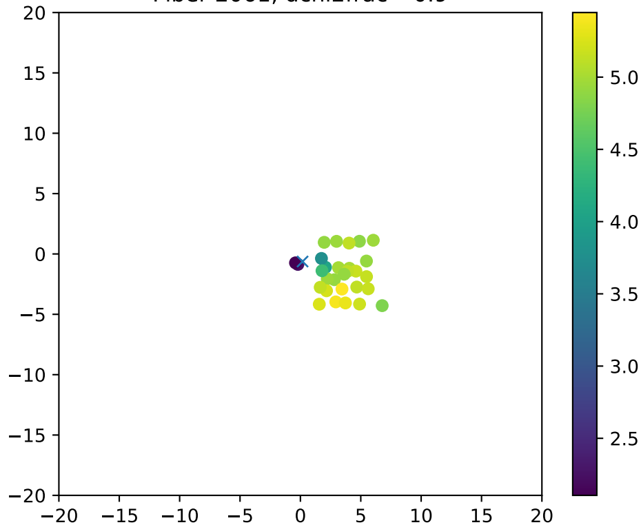
Fiber 2061, dchi2frac= 0.9
