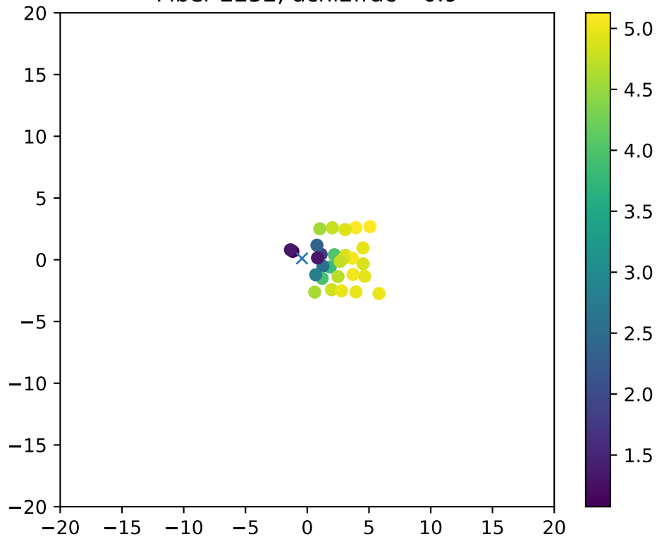
Fiber 2252, dchi2frac= 0.9
