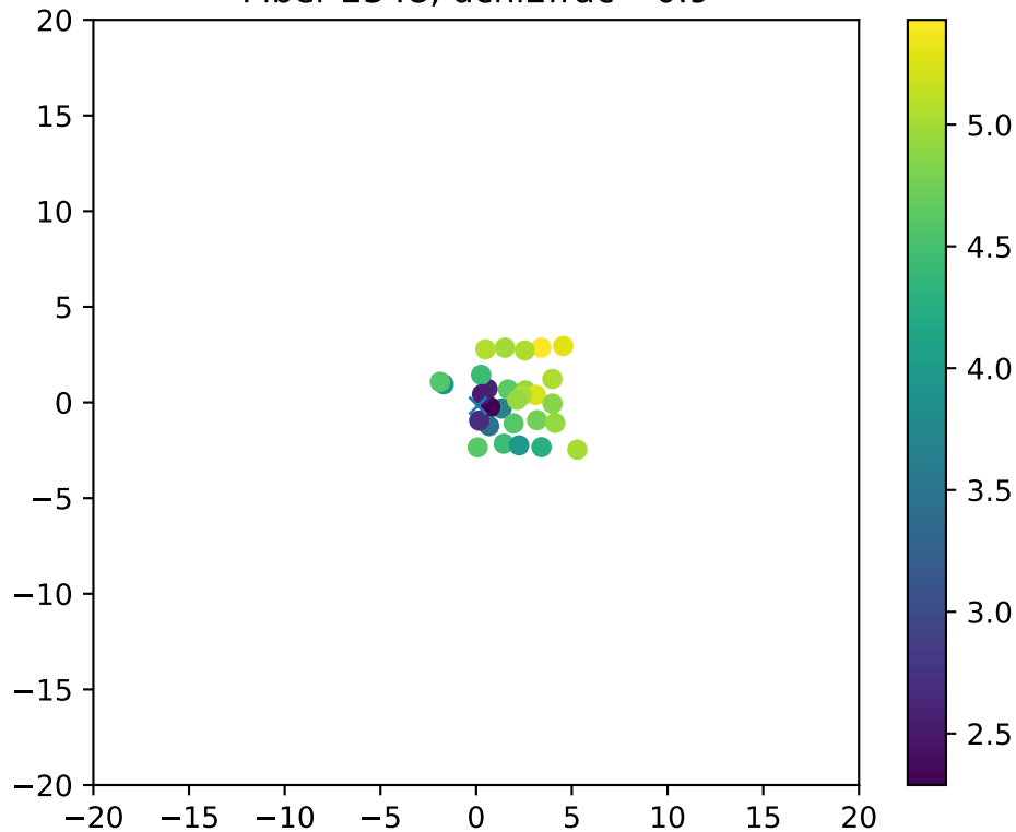
Fiber 2348, dchi2frac= 0.9
