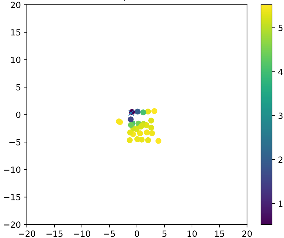
Fiber 2309, dchi2frac= 0.9
