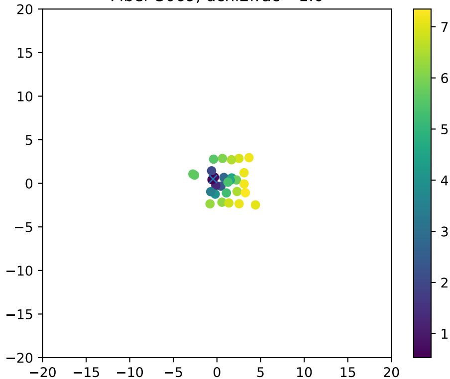
Fiber 3069, dchi2frac= 1.0
