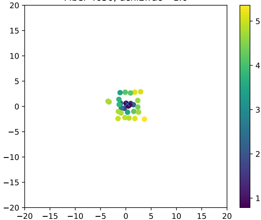
Fiber 4650, dchi2frac= 1.0
