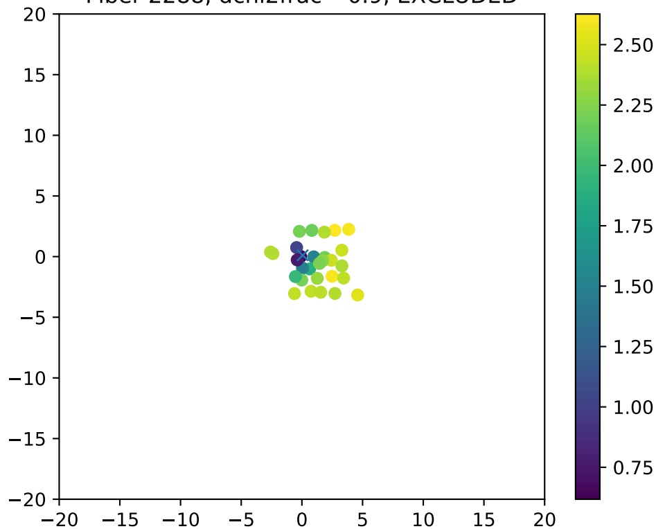
Fiber 2288, dchi2frac= 0.9, EXCLUDED
