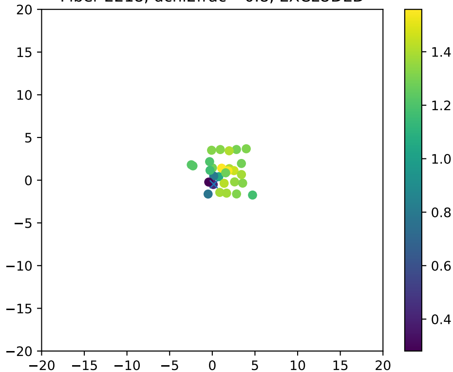
Fiber 2218, dchi2frac= 0.8, EXCLUDED
