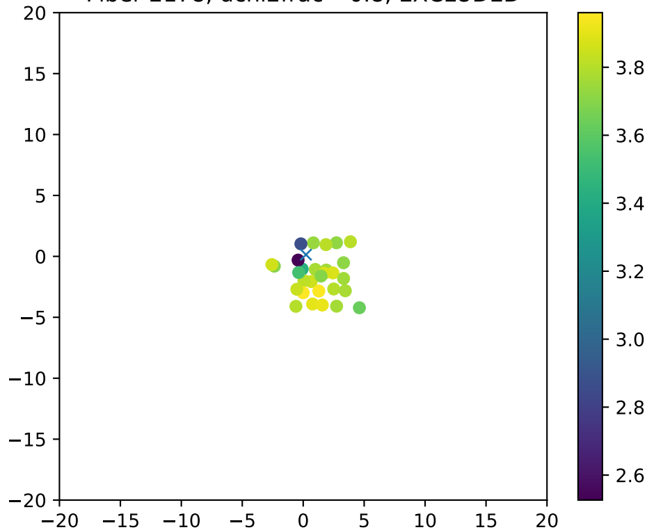
Fiber 2178, dchi2frac= 0.8, EXCLUDED
