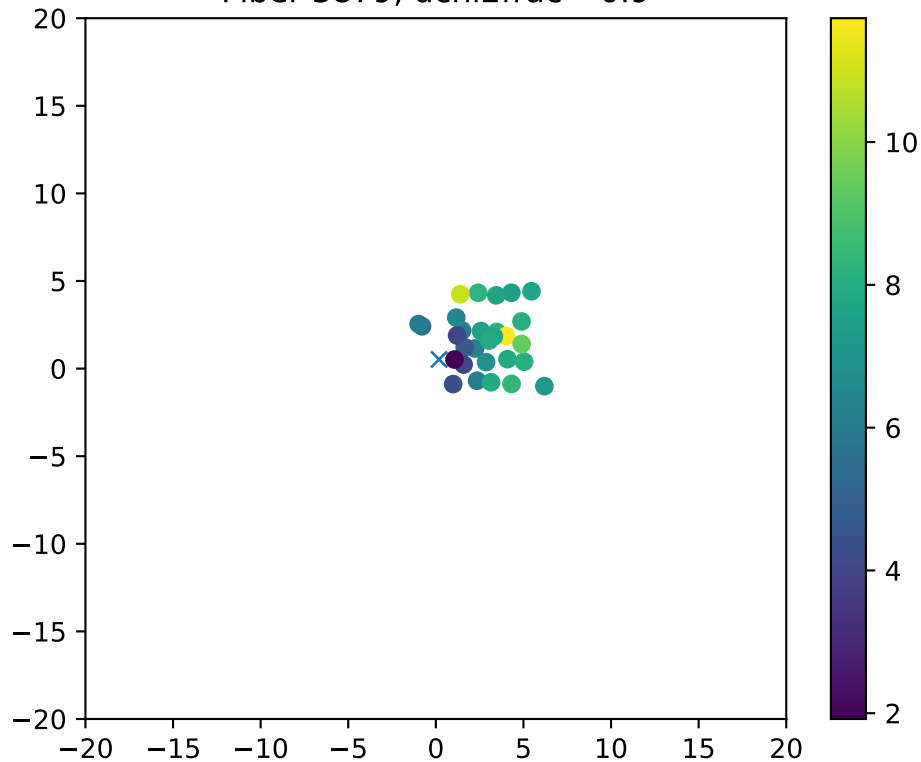
Fiber 3879, dchi2frac= 0.9
