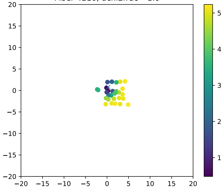
Fiber 4210, dchi2frac= 1.0
