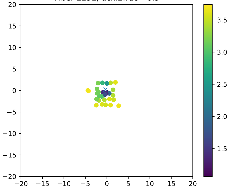
Fiber 2291, dchi2frac= 0.9
