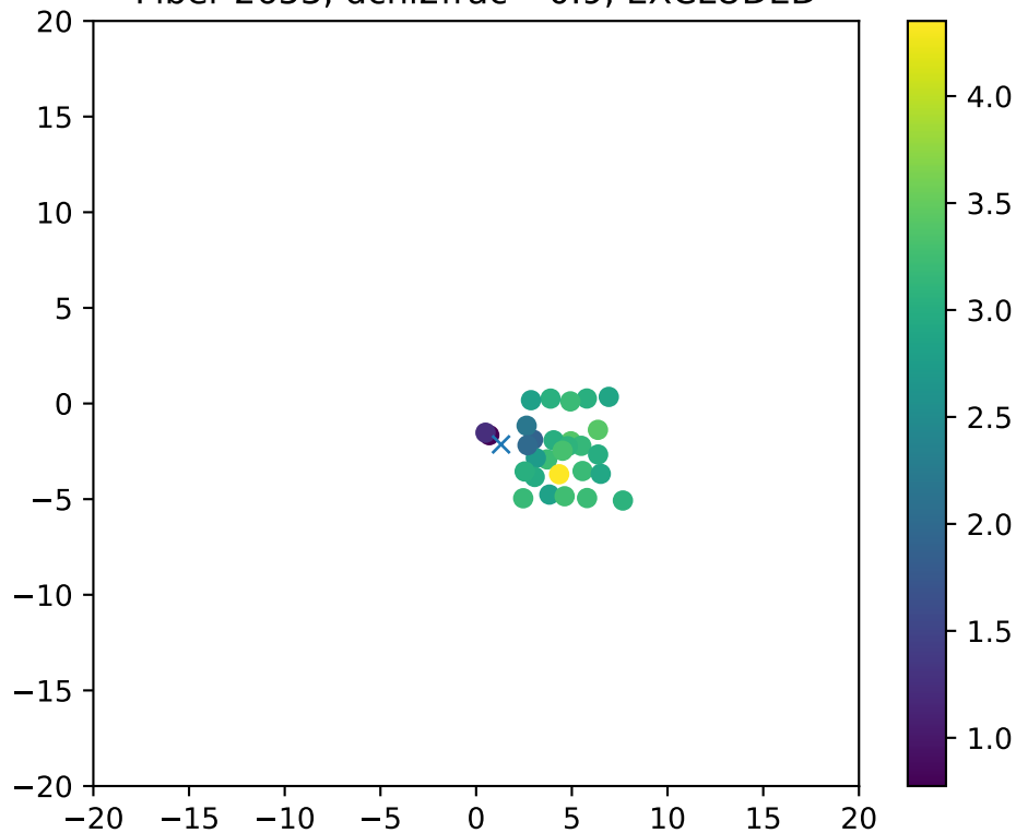
Fiber 2653, dchi2frac= 0.9, EXCLUDED
