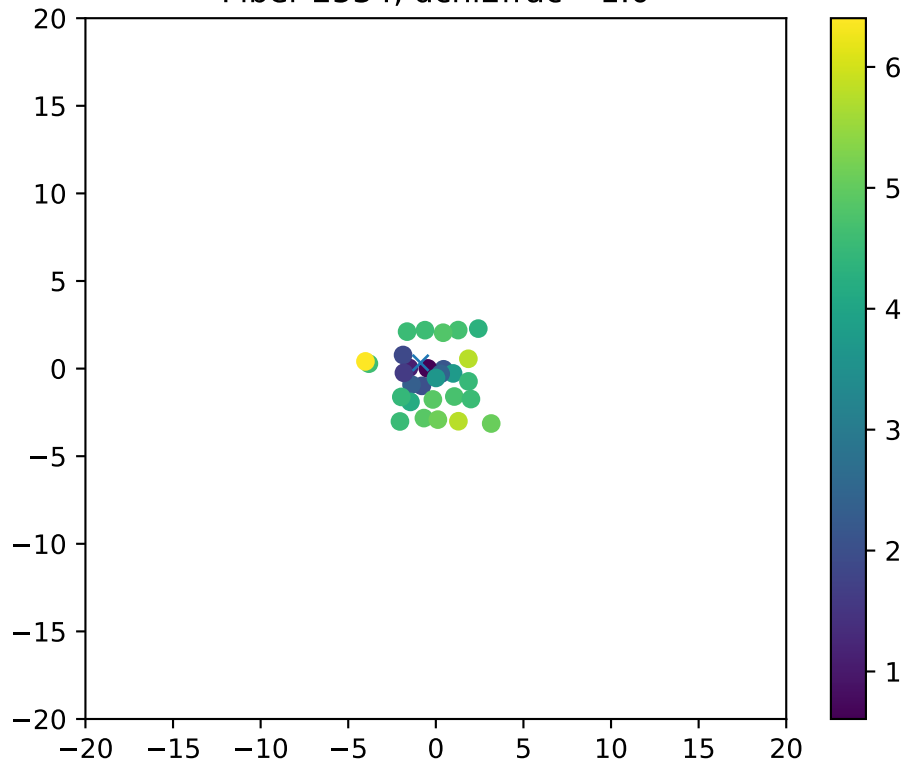
Fiber 2534, dchi2frac= 1.0
