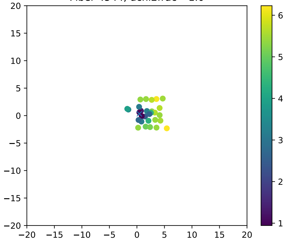
Fiber 4544, dchi2frac= 1.0
