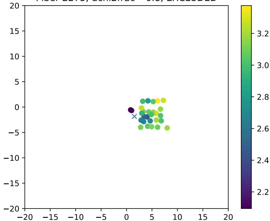
Fiber 2275, dchi2frac= 0.8, EXCLUDED
