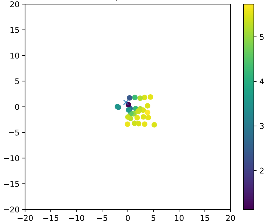
Fiber 3189, dchi2frac= 1.0
