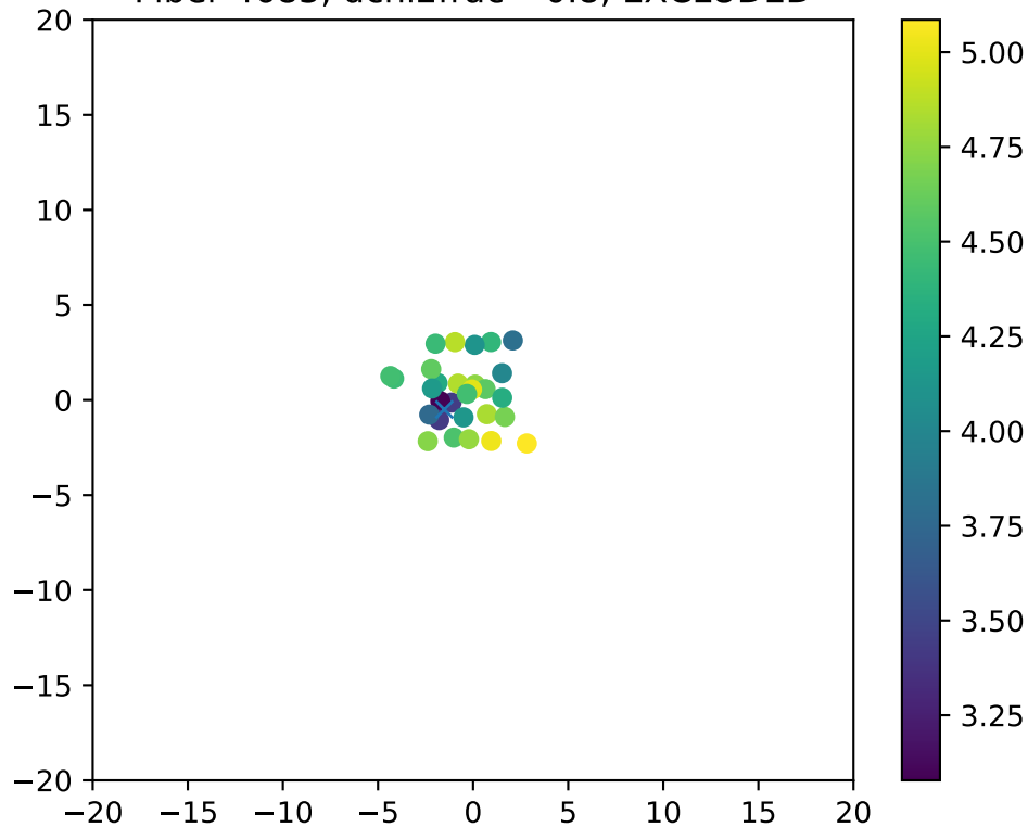
Fiber 4683, dchi2frac= 0.8, EXCLUDED
