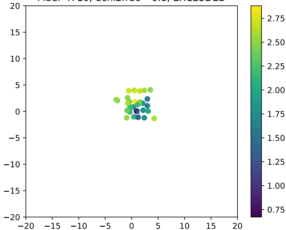
Fiber 4710, dchi2frac= 0.8, EXCLUDED
