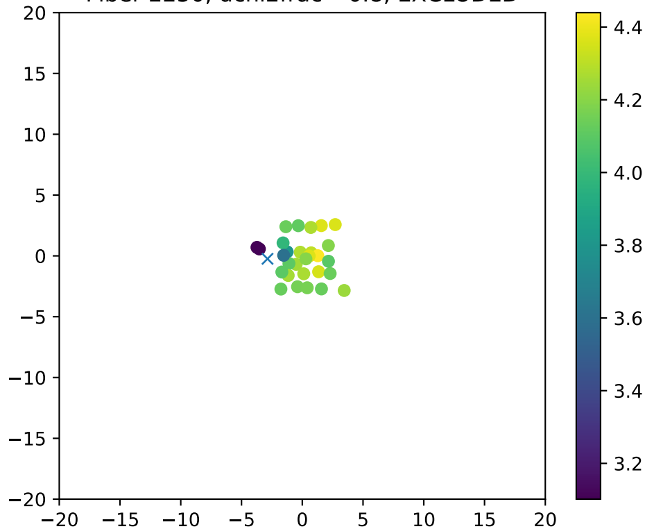
Fiber 2250, dchi2frac= 0.8, EXCLUDED
