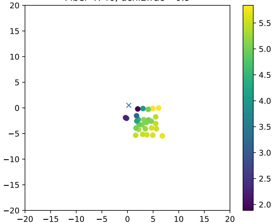
Fiber 4746, dchi2frac= 0.9
