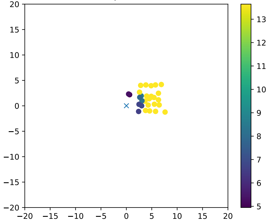
Fiber 2466, dchi2frac= 0.9
