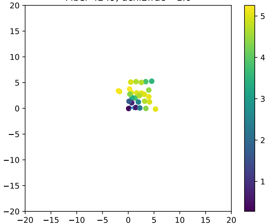
Fiber 4249, dchi2frac= 1.0
