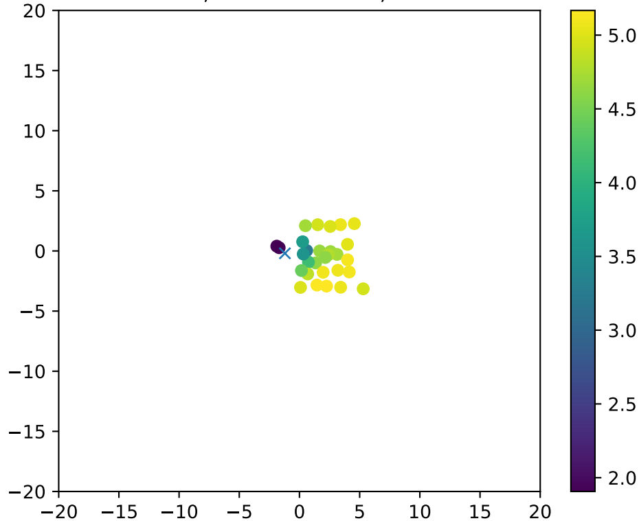
Fiber 2152, dchi2frac= 0.9, EXCLUDED
