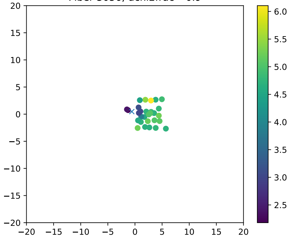
Fiber 3056, dchi2frac= 0.9
