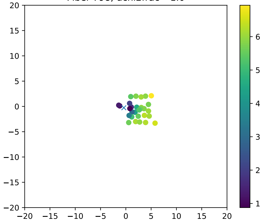
Fiber 798, dchi2frac= 1.0
