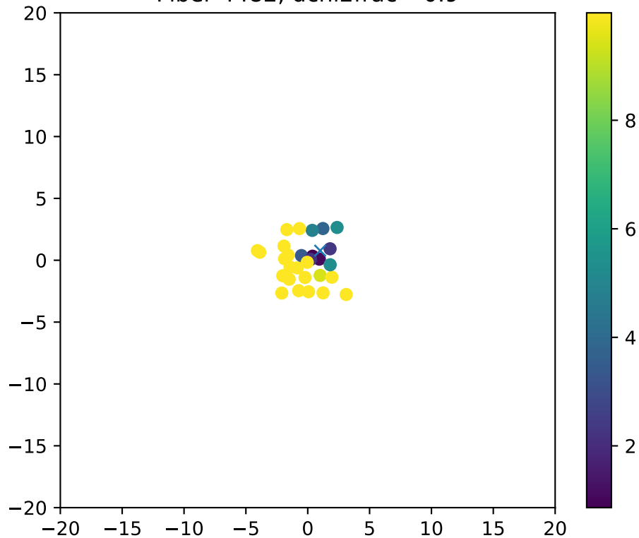
Fiber 4482, dchi2frac= 0.9
