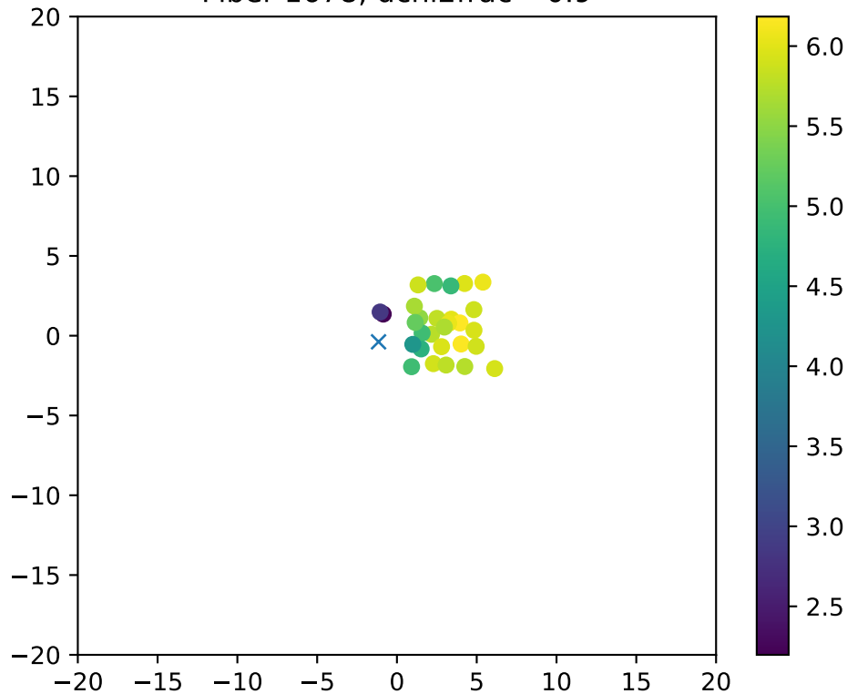
Fiber 1678, dchi2frac= 0.9
