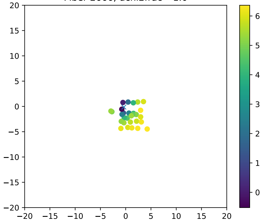
Fiber 2666, dchi2frac= 1.0
