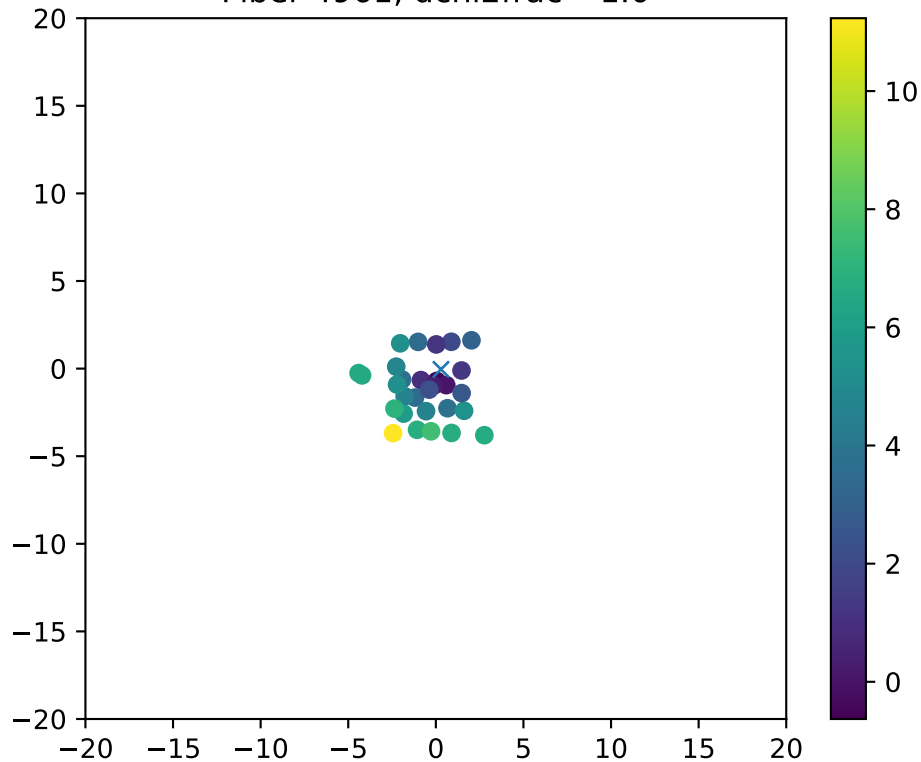
Fiber 4961, dchi2frac= 1.0
