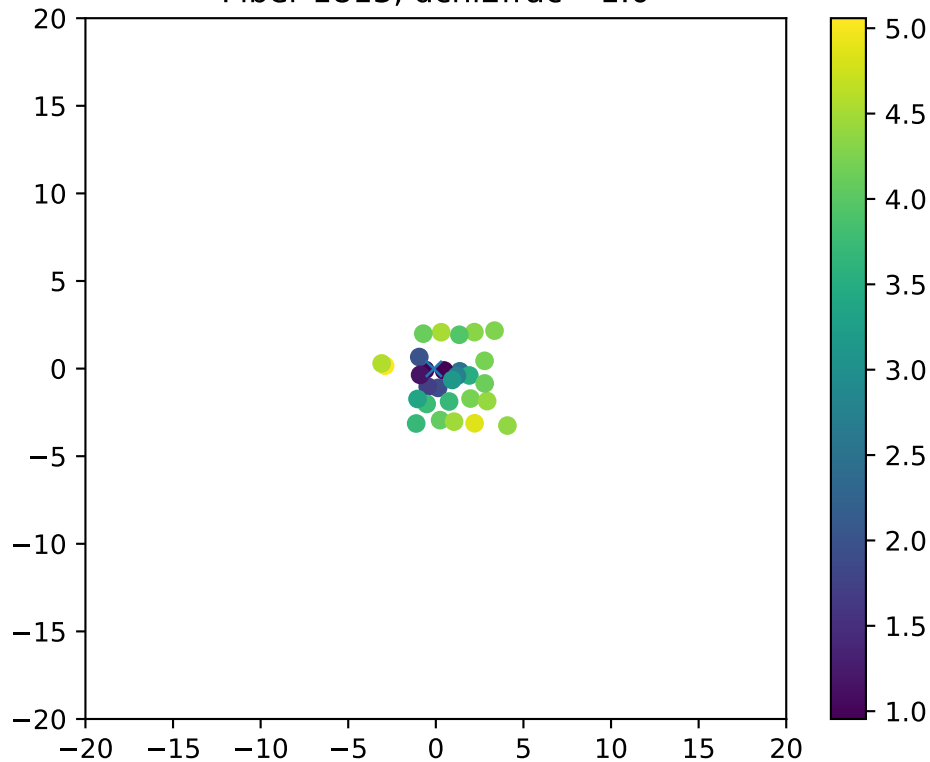
Fiber 1813, dchi2frac= 1.0
