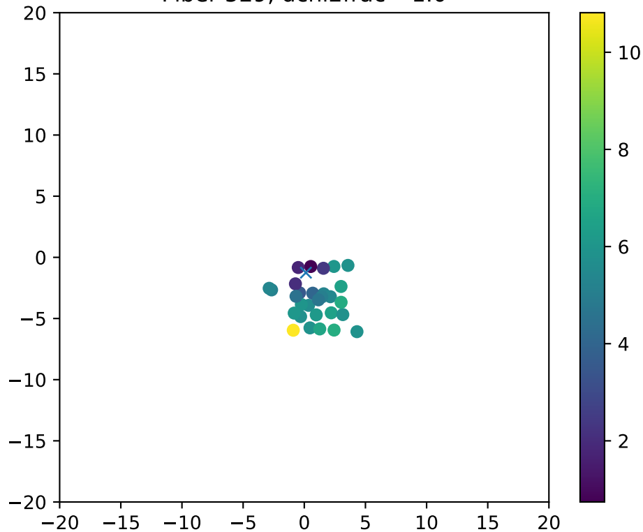
Fiber 529, dchi2frac= 1.0
