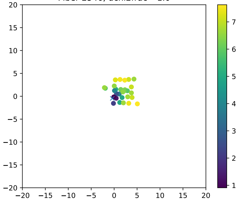
Fiber 2546, dchi2frac= 1.0
