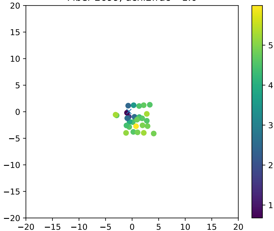
Fiber 2699, dchi2frac= 1.0
