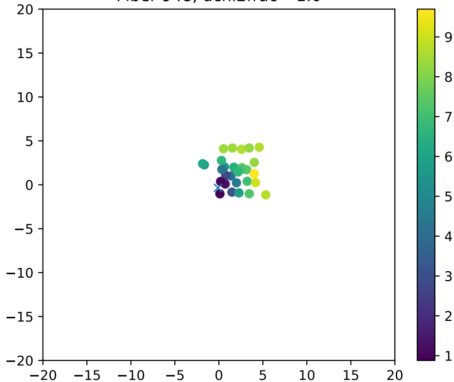
Fiber 948, dchi2frac= 1.0
