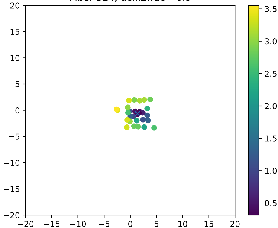
Fiber 324, dchi2frac= 0.9
