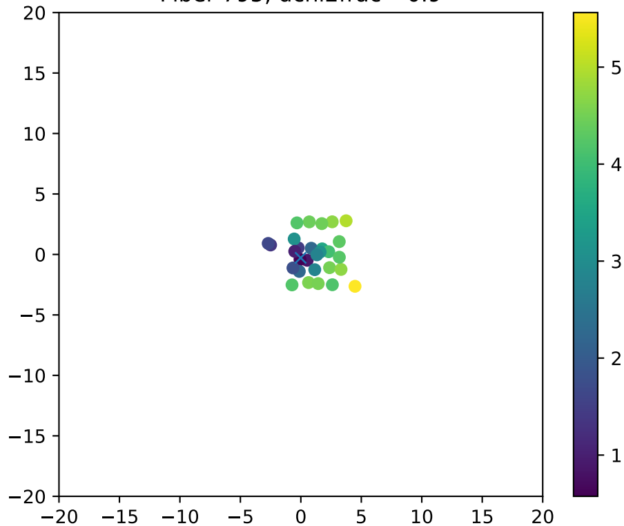
Fiber 795, dchi2frac= 0.9
