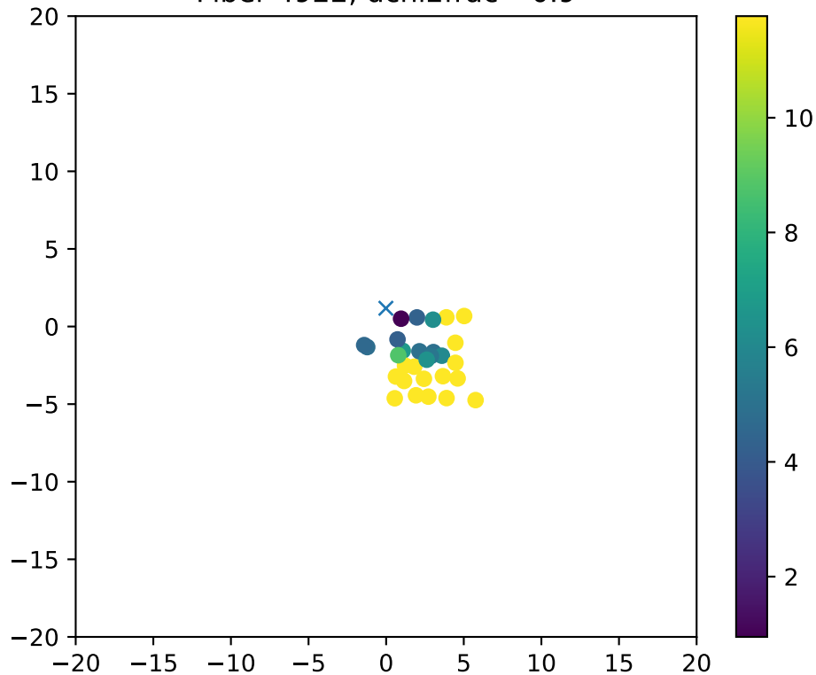
Fiber 4922, dchi2frac= 0.9
