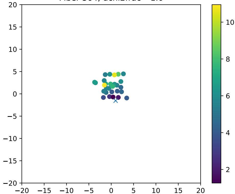
Fiber 364, dchi2frac= 1.0
