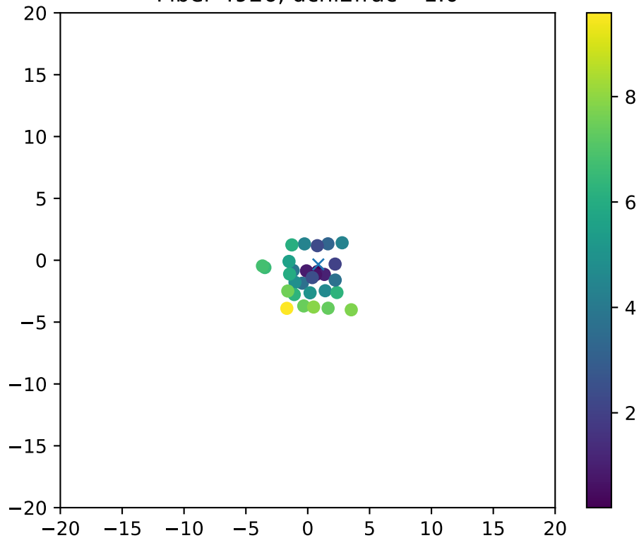
Fiber 4926, dchi2frac= 1.0
