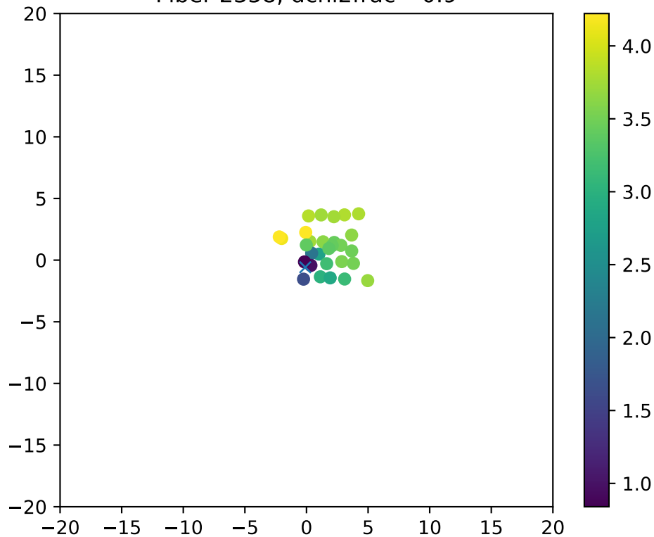
Fiber 2358, dchi2frac= 0.9
