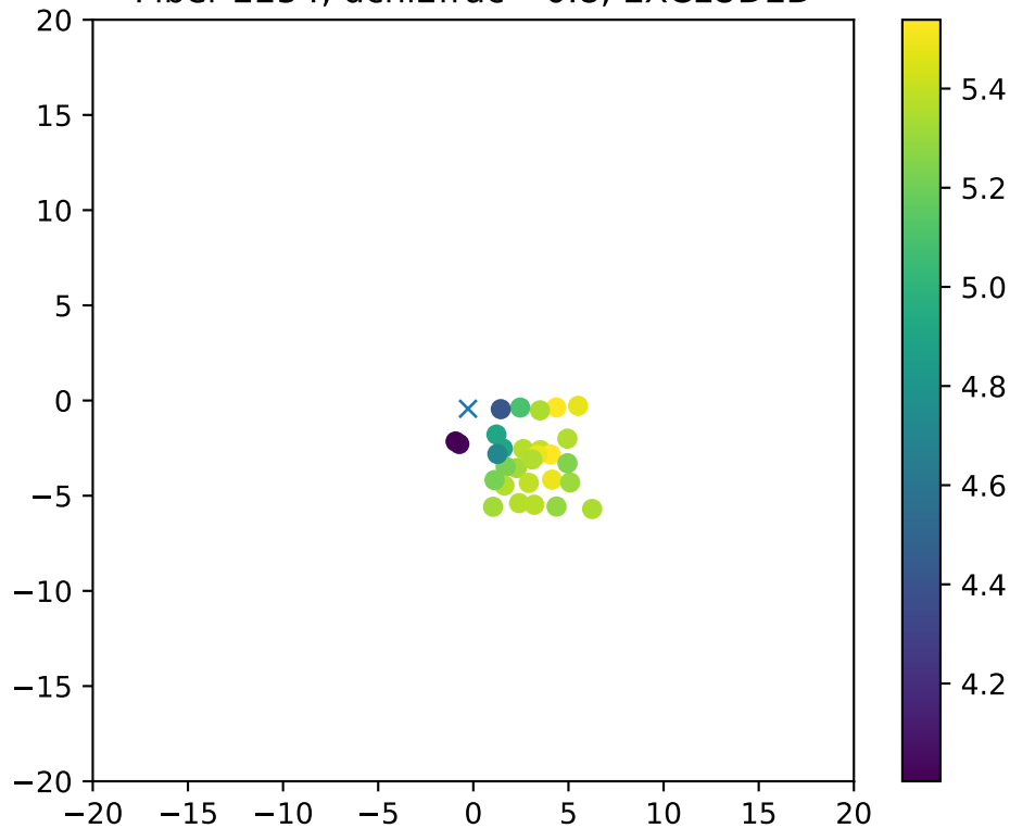
Fiber 2254, dchi2frac= 0.8, EXCLUDED
