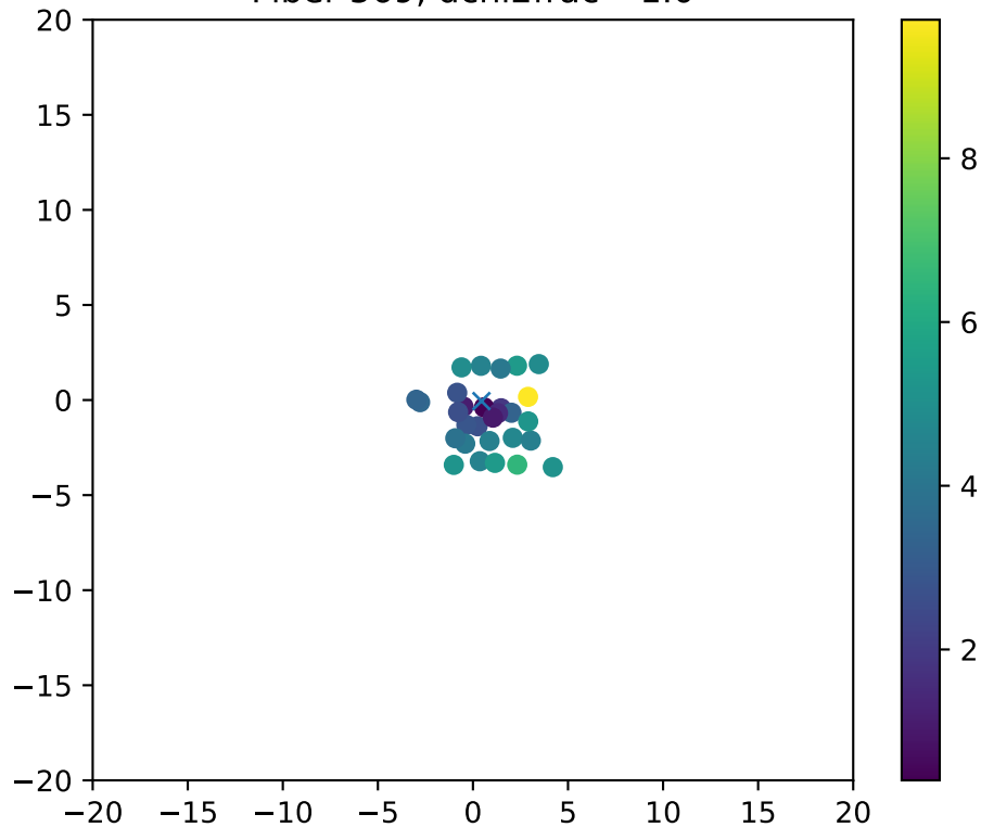
Fiber 569, dchi2frac= 1.0
