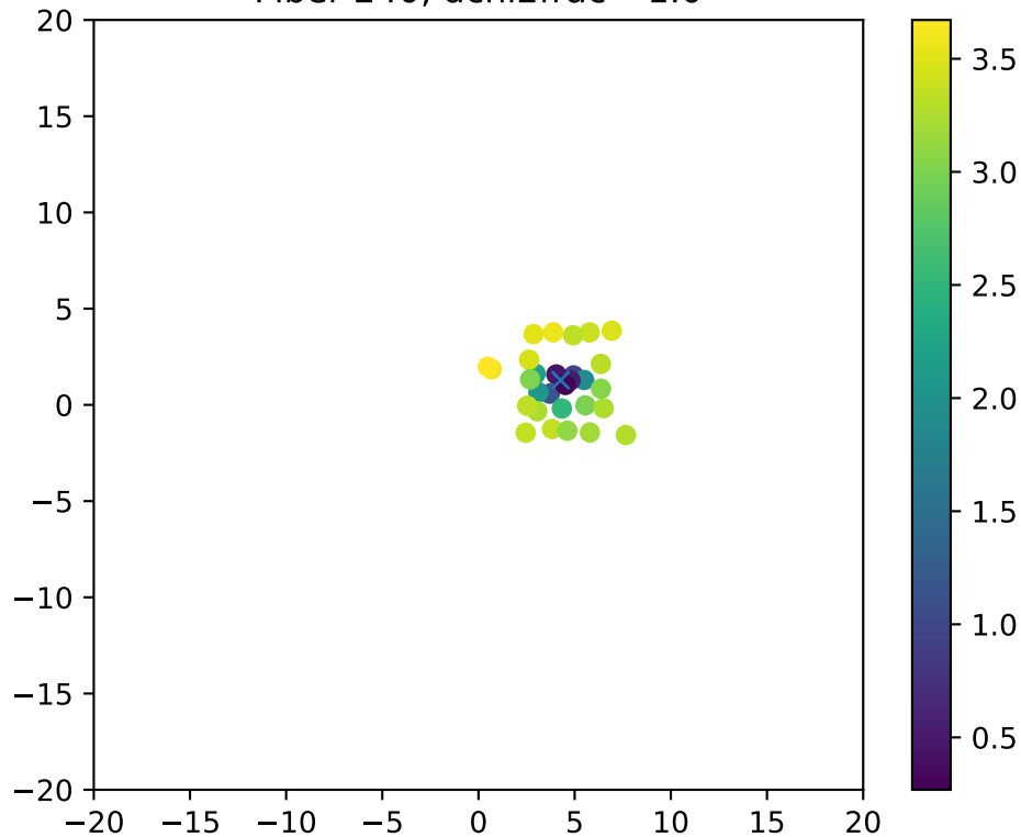
Fiber 240, dchi2frac= 1.0
