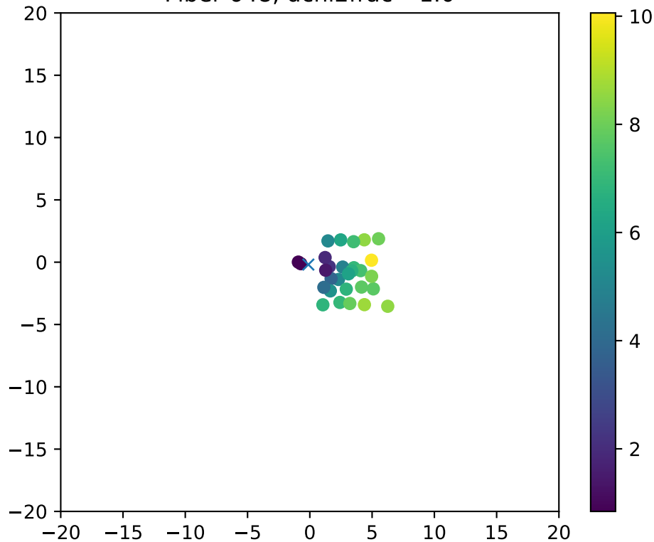
Fiber 648, dchi2frac= 1.0
