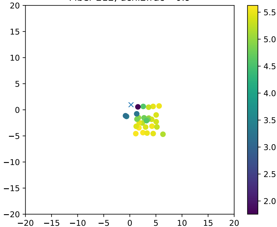
Fiber 212, dchi2frac= 0.9
