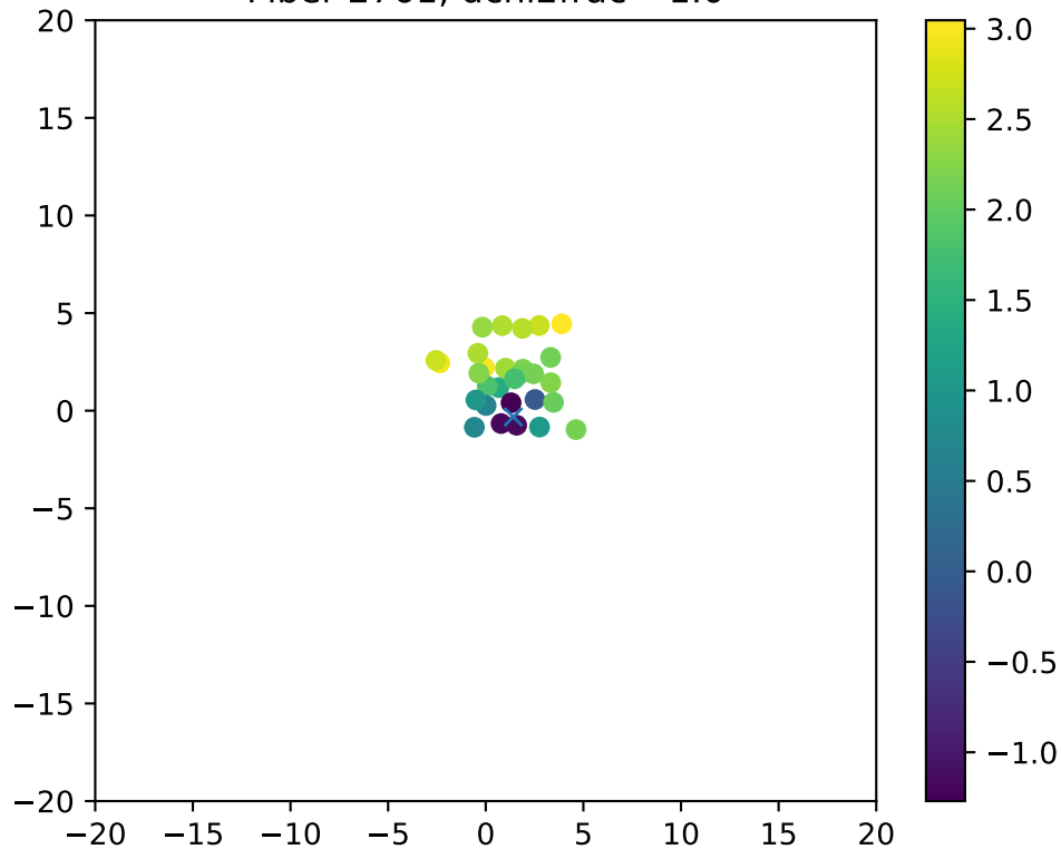
Fiber 2761, dchi2frac= 1.0
