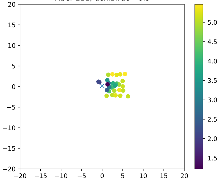
Fiber 221, dchi2frac= 0.9
