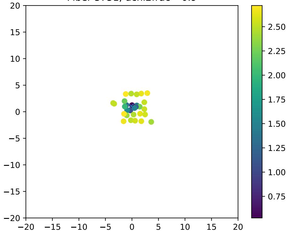
Fiber 3751, dchi2frac= 0.9
