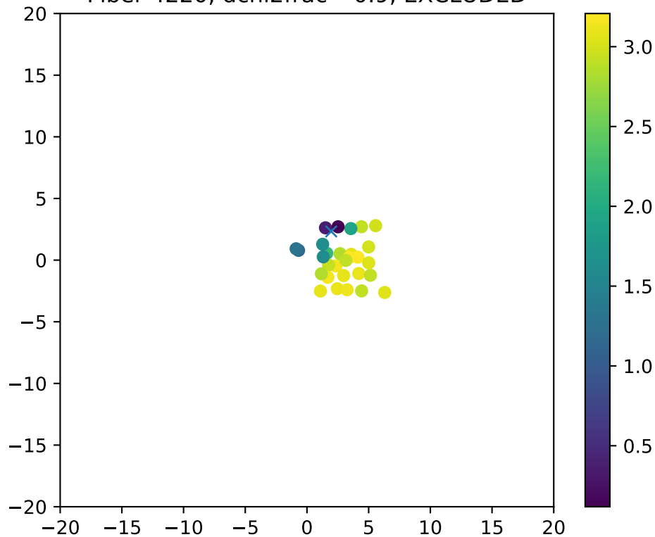
Fiber 4220, dchi2frac= 0.9, EXCLUDED
