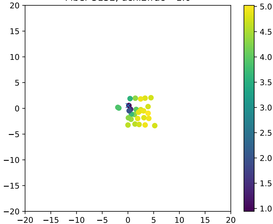
Fiber 3132, dchi2frac= 1.0
