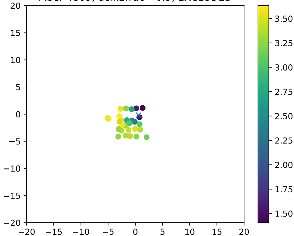
Fiber 4809, dchi2frac= 0.9, EXCLUDED
