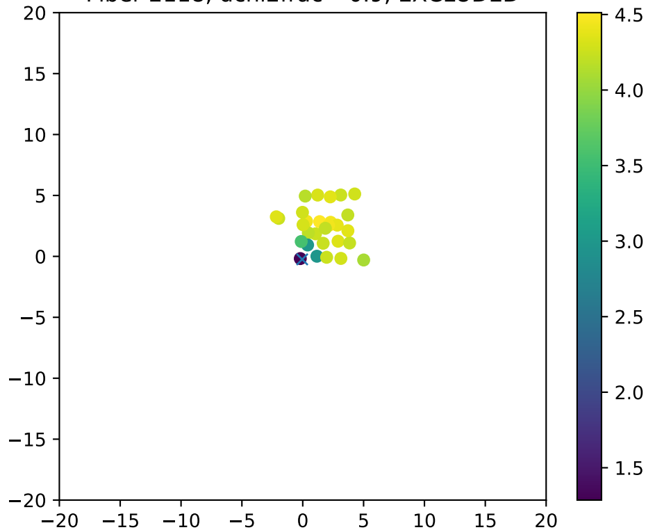
Fiber 2118, dchi2frac= 0.9, EXCLUDED
