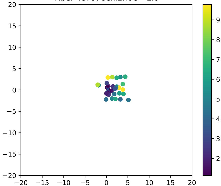
Fiber 4879, dchi2frac= 1.0
