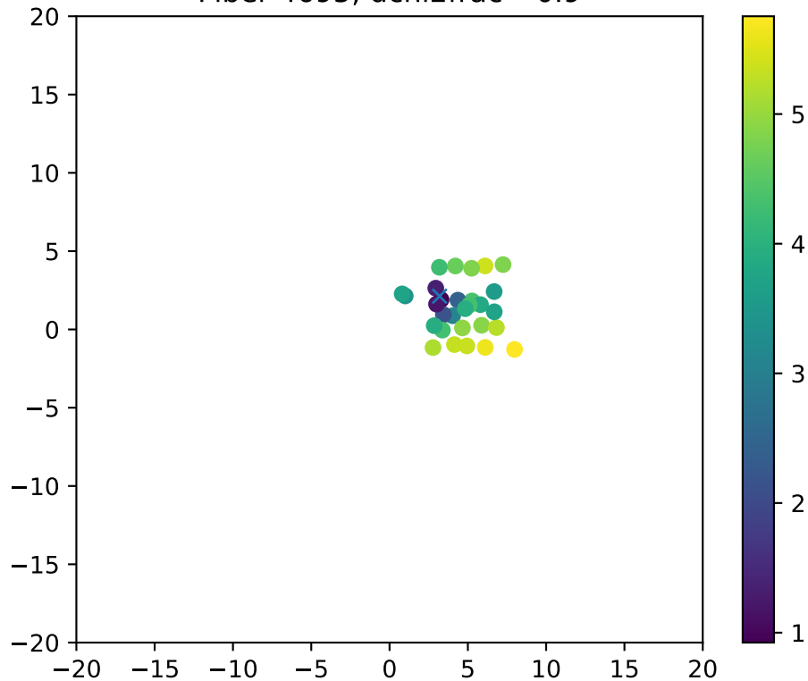
Fiber 4695, dchi2frac= 0.9
