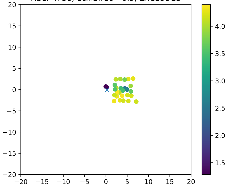
Fiber 4758, dchi2frac= 0.9, EXCLUDED
