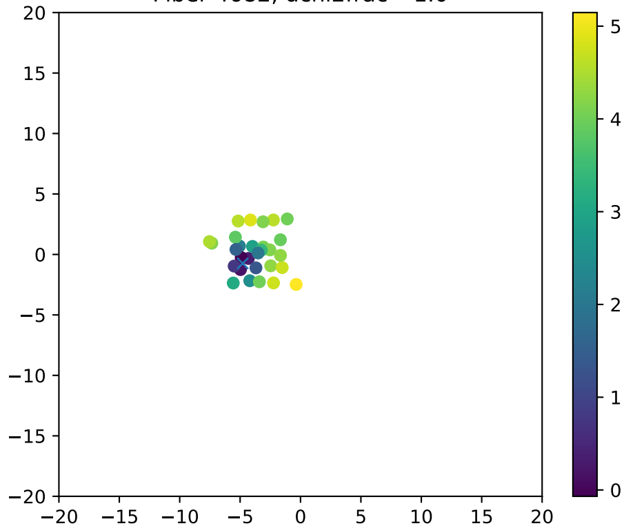
Fiber 4682, dchi2frac= 1.0
