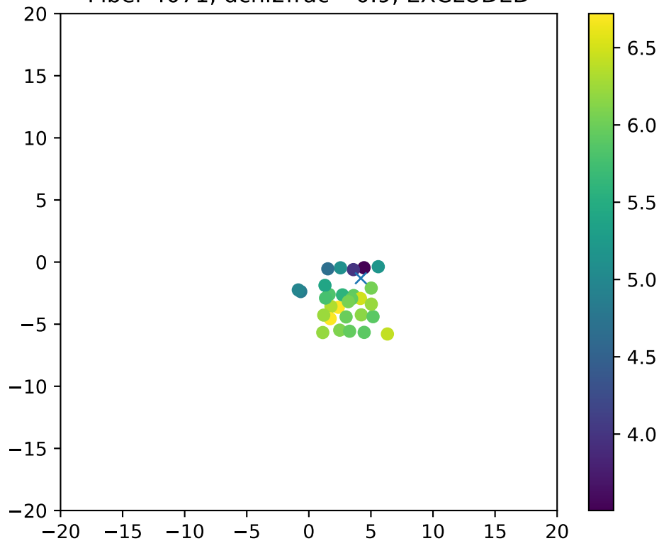
Fiber 4071, dchi2frac= 0.9, EXCLUDED
