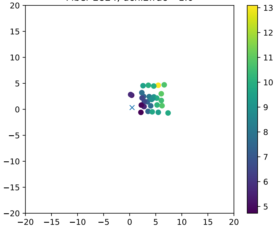
Fiber 2824, dchi2frac= 1.0
