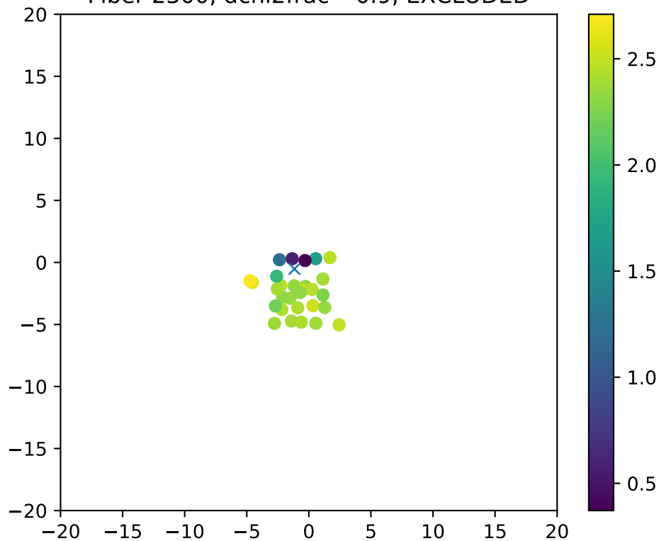
Fiber 2300, dchi2frac= 0.9, EXCLUDED
