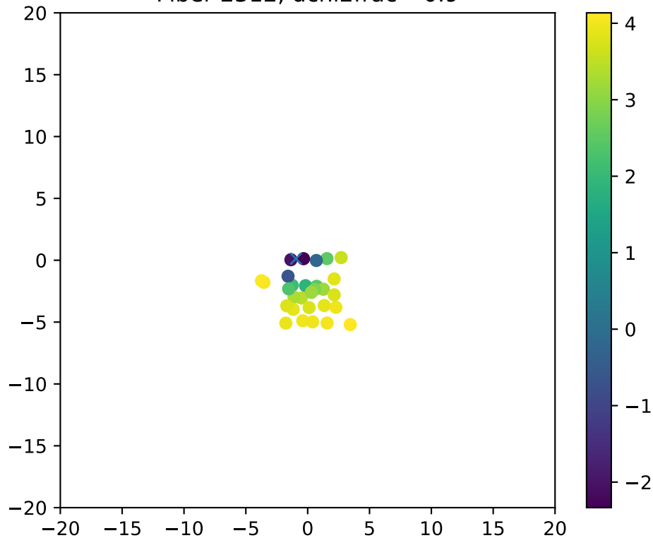
Fiber 2312, dchi2frac= 0.9
