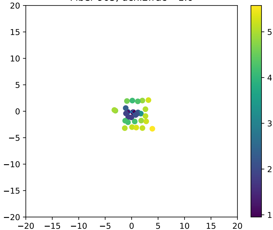
Fiber 905, dchi2frac= 1.0
