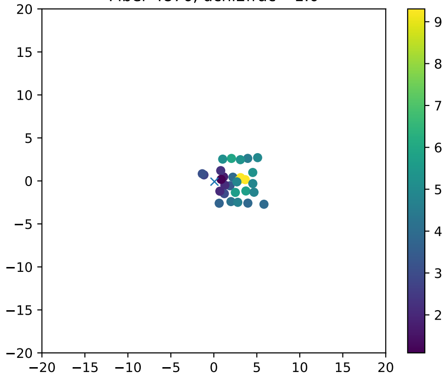
Fiber 4876, dchi2frac= 1.0
