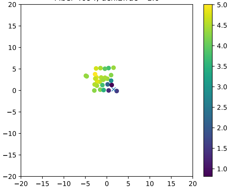
Fiber 4094, dchi2frac= 1.0
