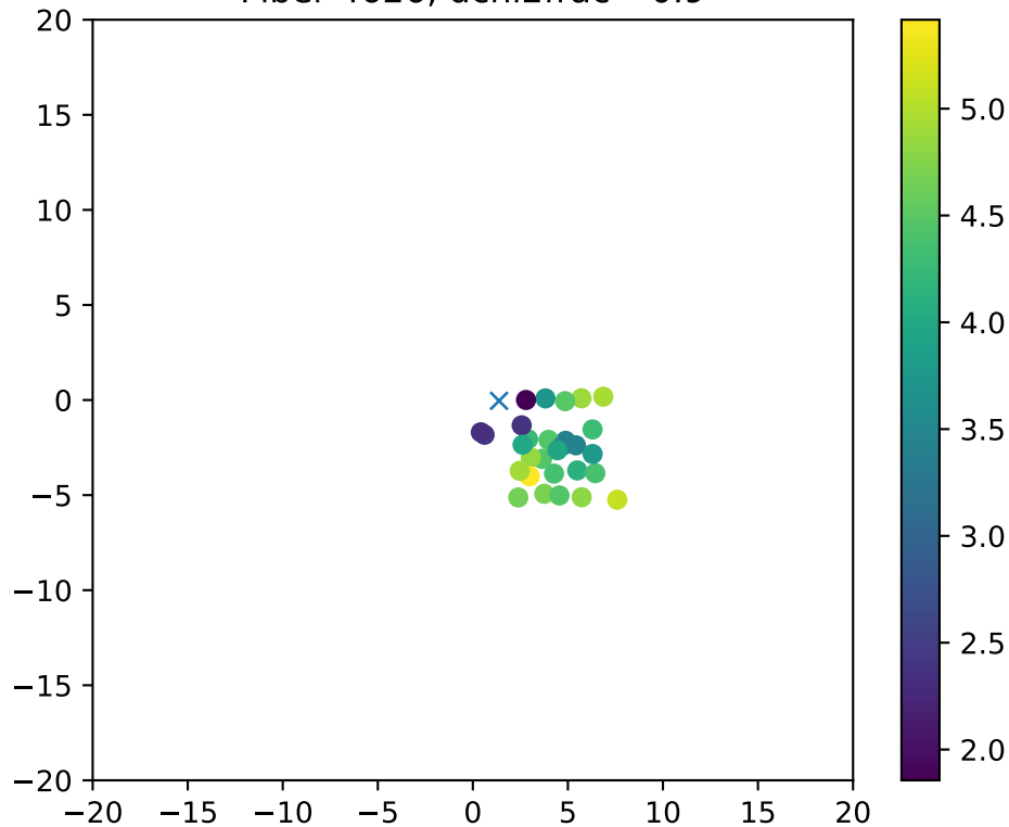
Fiber 4626, dchi2frac= 0.9
