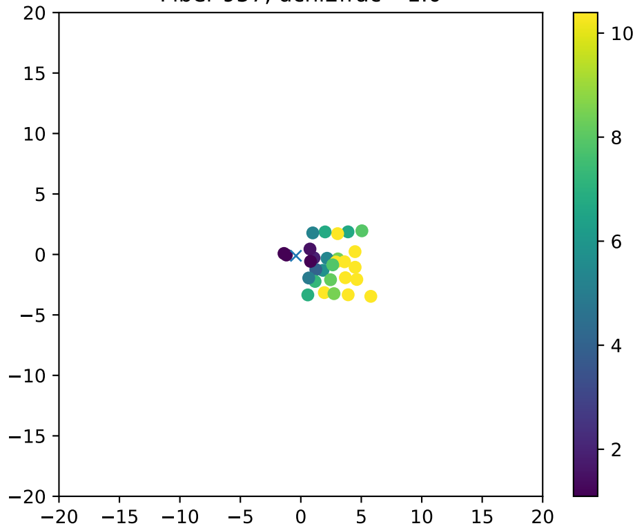
Fiber 957, dchi2frac= 1.0
