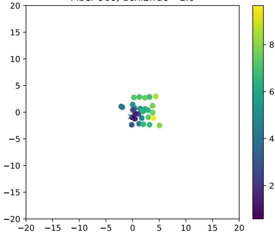
Fiber 960, dchi2frac= 1.0
