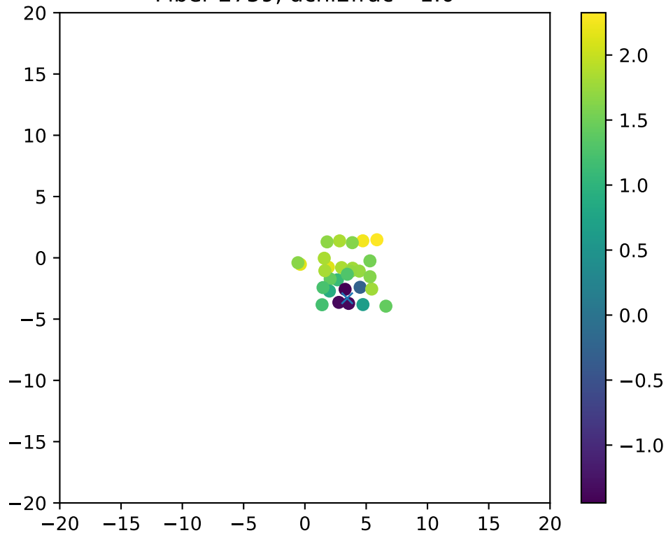
Fiber 2759, dchi2frac= 1.0
