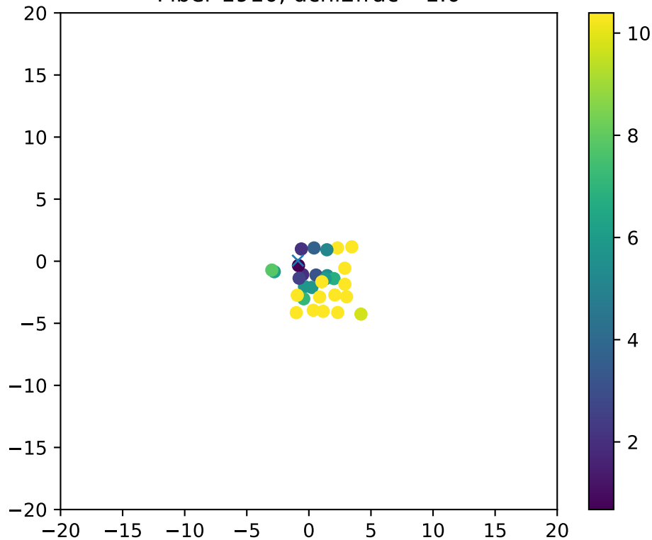
Fiber 1910, dchi2frac= 1.0
