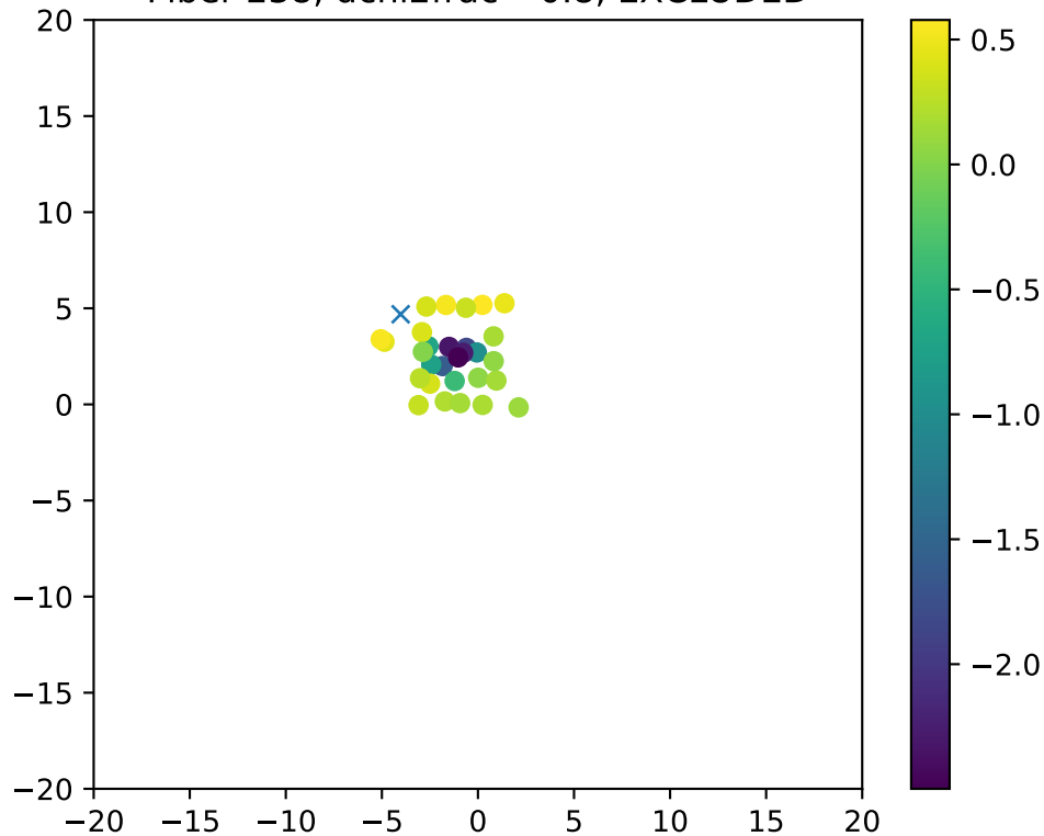
Fiber 238, dchi2frac= 0.8, EXCLUDED
