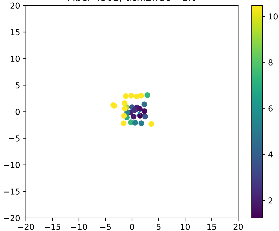
Fiber 4502, dchi2frac= 1.0
