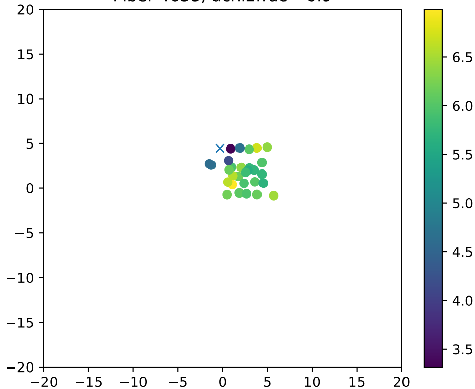
Fiber 4633, dchi2frac= 0.9
