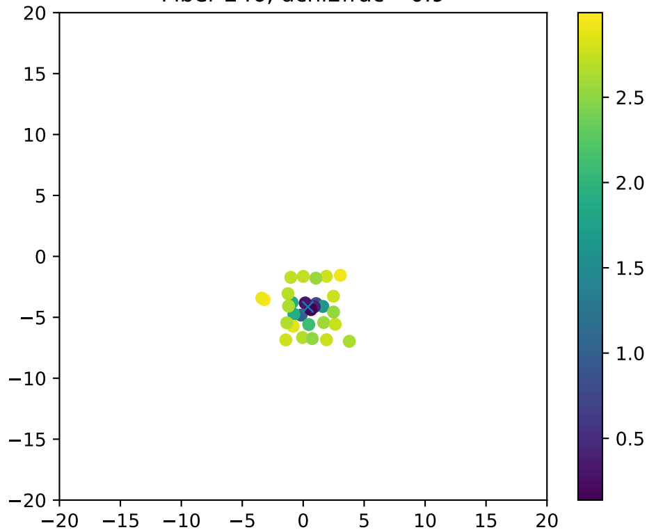
Fiber 246, dchi2frac= 0.9
