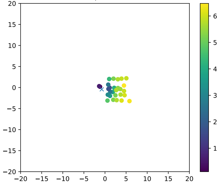
Fiber 2652, dchi2frac= 1.0
