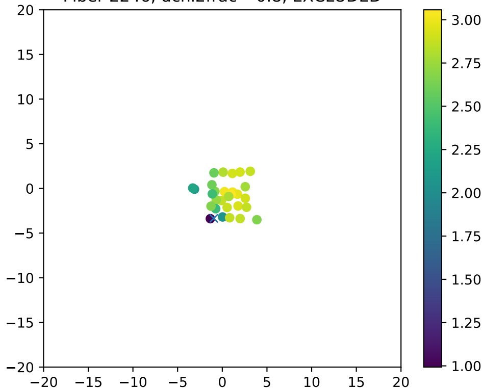
Fiber 2246, dchi2frac= 0.8, EXCLUDED
