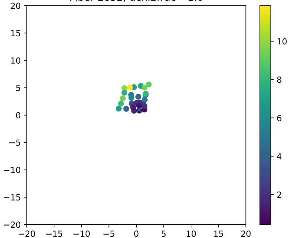
Fiber 2832, dchi2frac= 1.0
