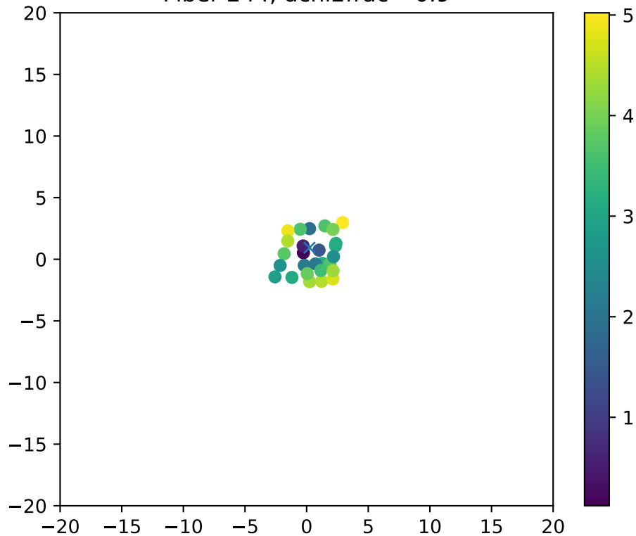
Fiber 244, dchi2frac= 0.9
