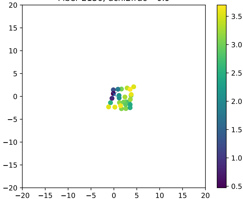
Fiber 2136, dchi2frac= 0.9
