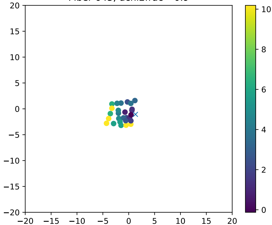
Fiber 643, dchi2frac= 0.9
