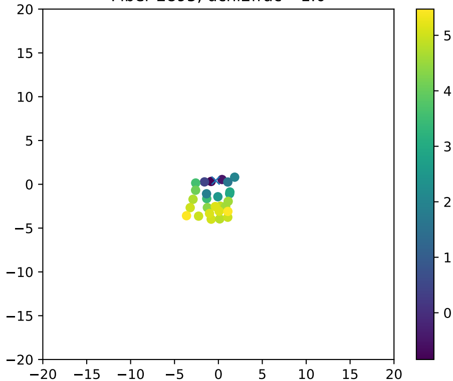
Fiber 2895, dchi2frac= 1.0
