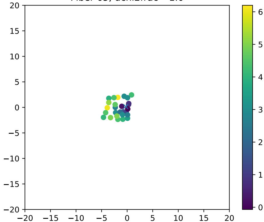
Fiber 65, dchi2frac= 1.0
