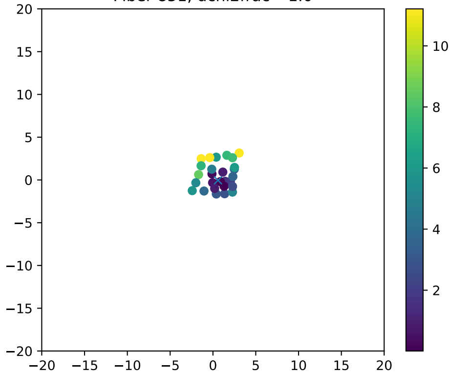
Fiber 851, dchi2frac= 1.0
