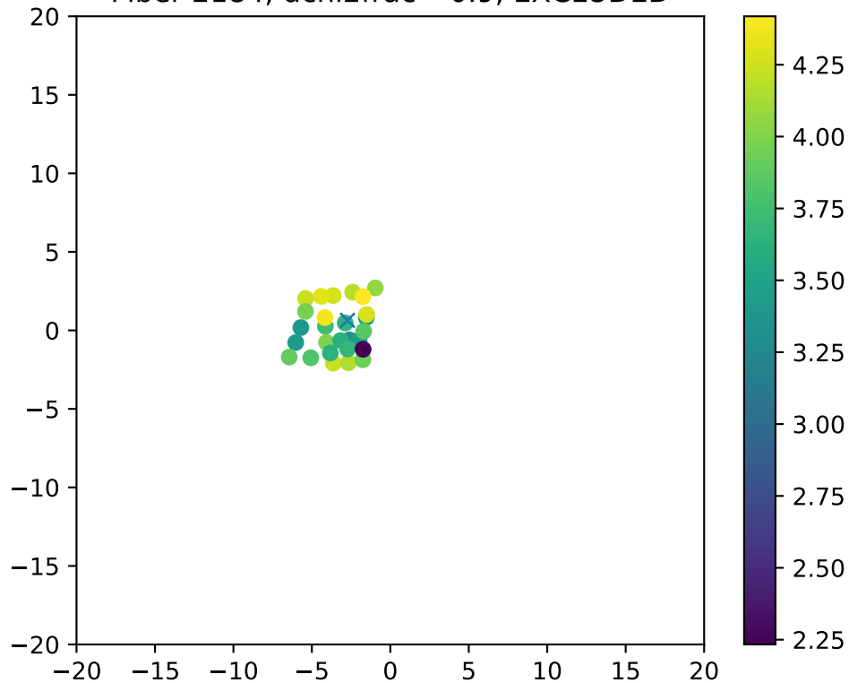
Fiber 2184, dchi2frac= 0.9, EXCLUDED
