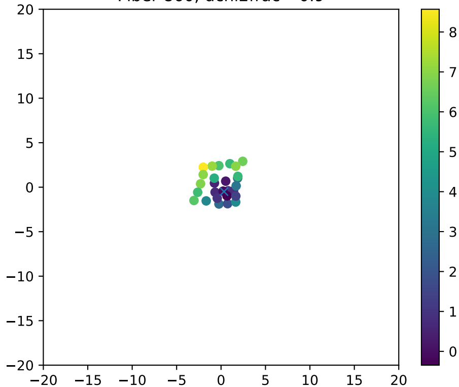
Fiber 860, dchi2frac= 0.9
