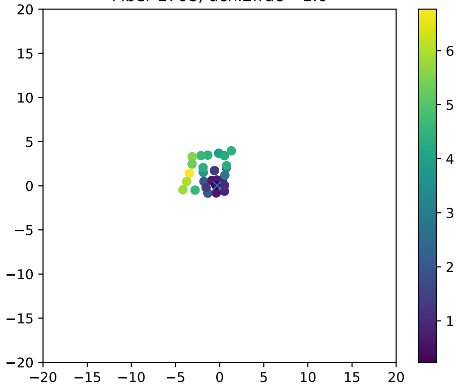
Fiber 1708, dchi2frac= 1.0
