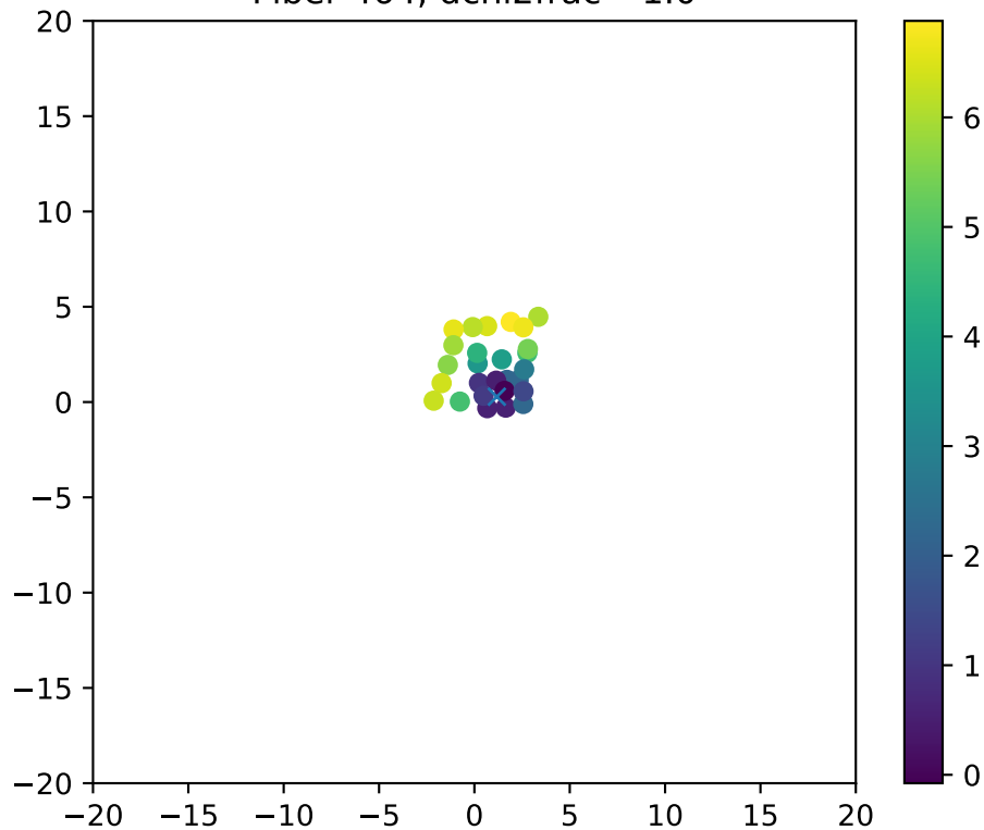
Fiber 464, dchi2frac= 1.0
