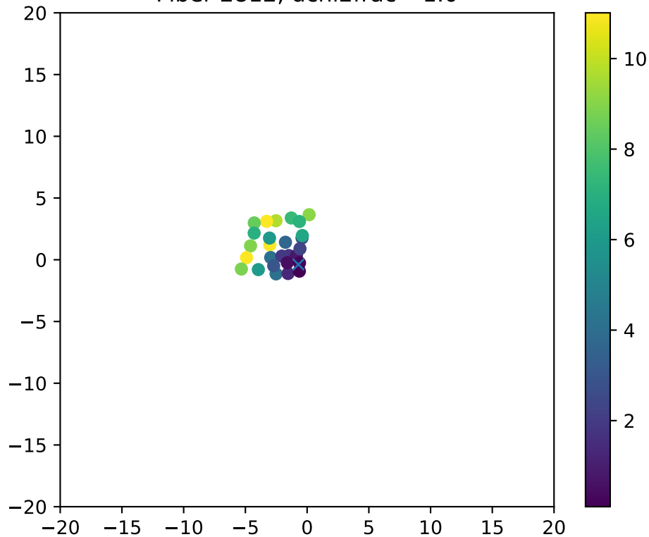
Fiber 2812, dchi2frac= 1.0
