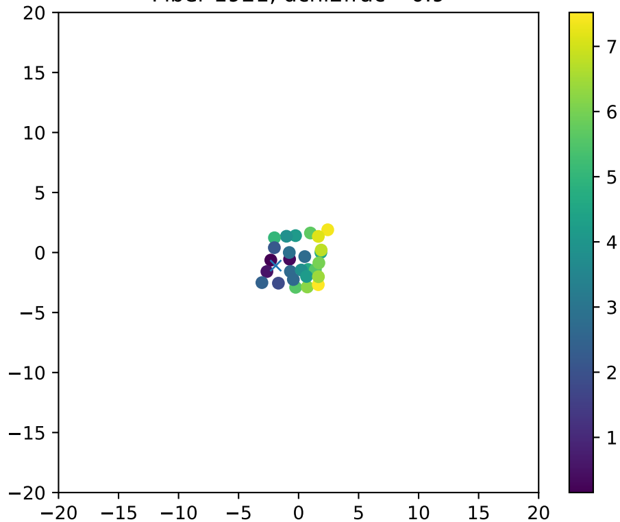
Fiber 1921, dchi2frac= 0.9
