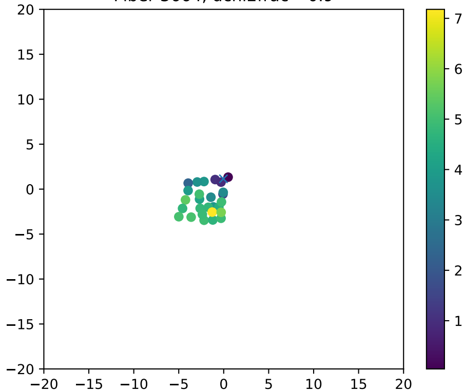
Fiber 3664, dchi2frac= 0.9
