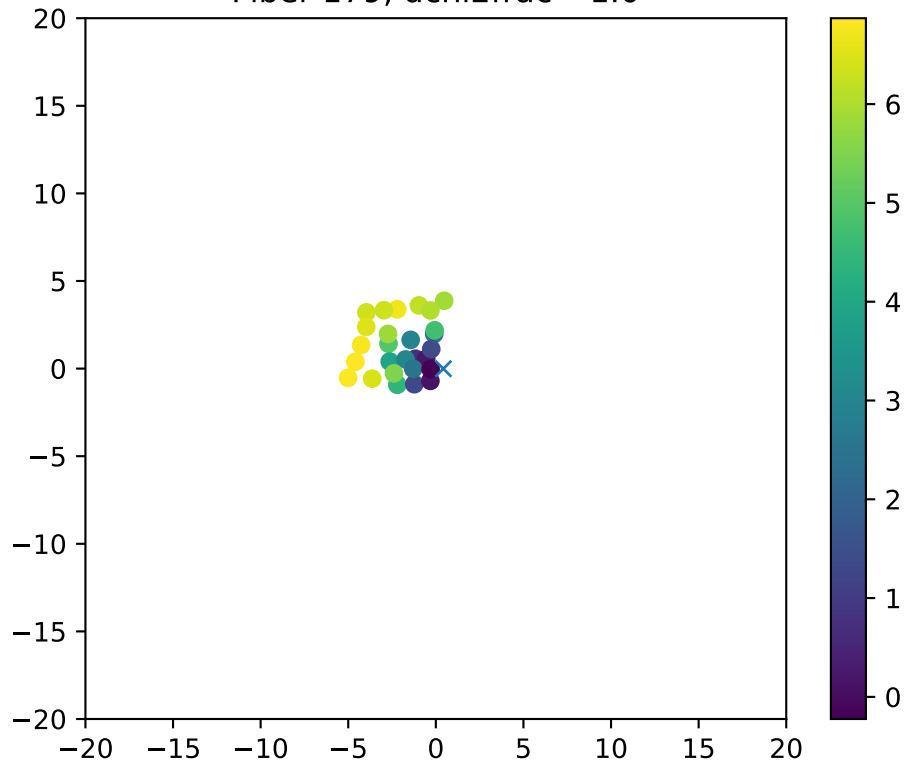
Fiber 179, dchi2frac= 1.0
