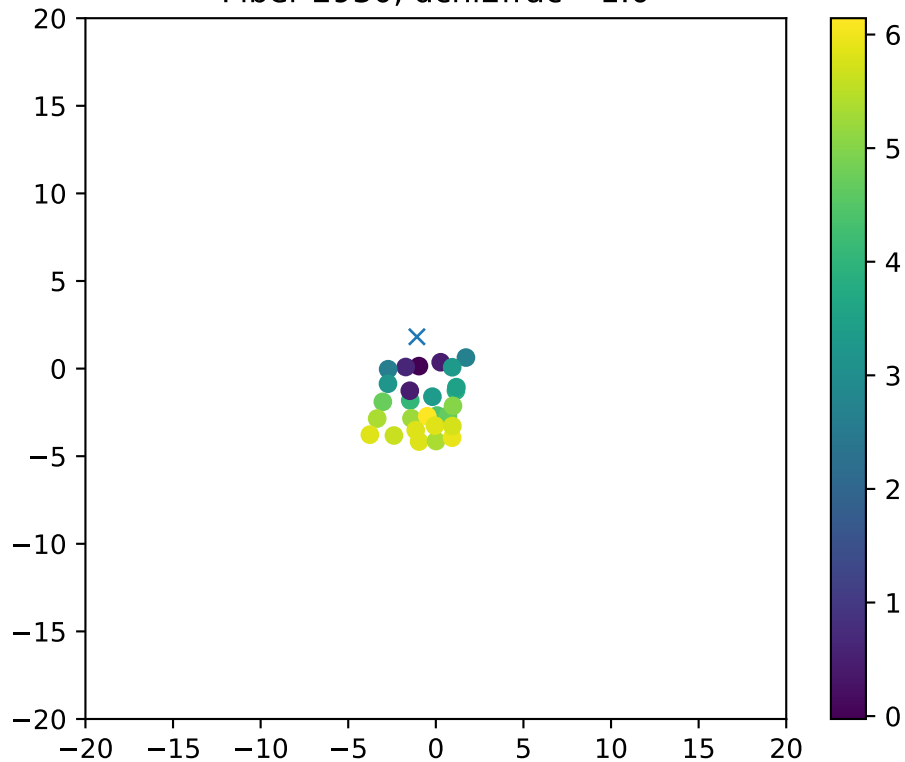
Fiber 2930, dchi2frac= 1.0
