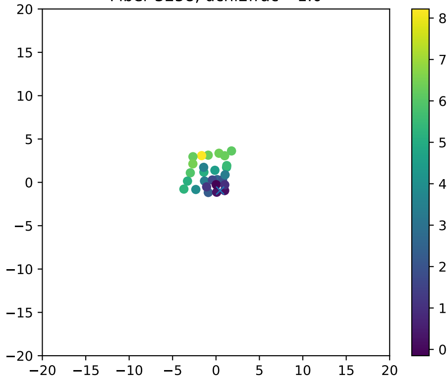
Fiber 3258, dchi2frac= 1.0
