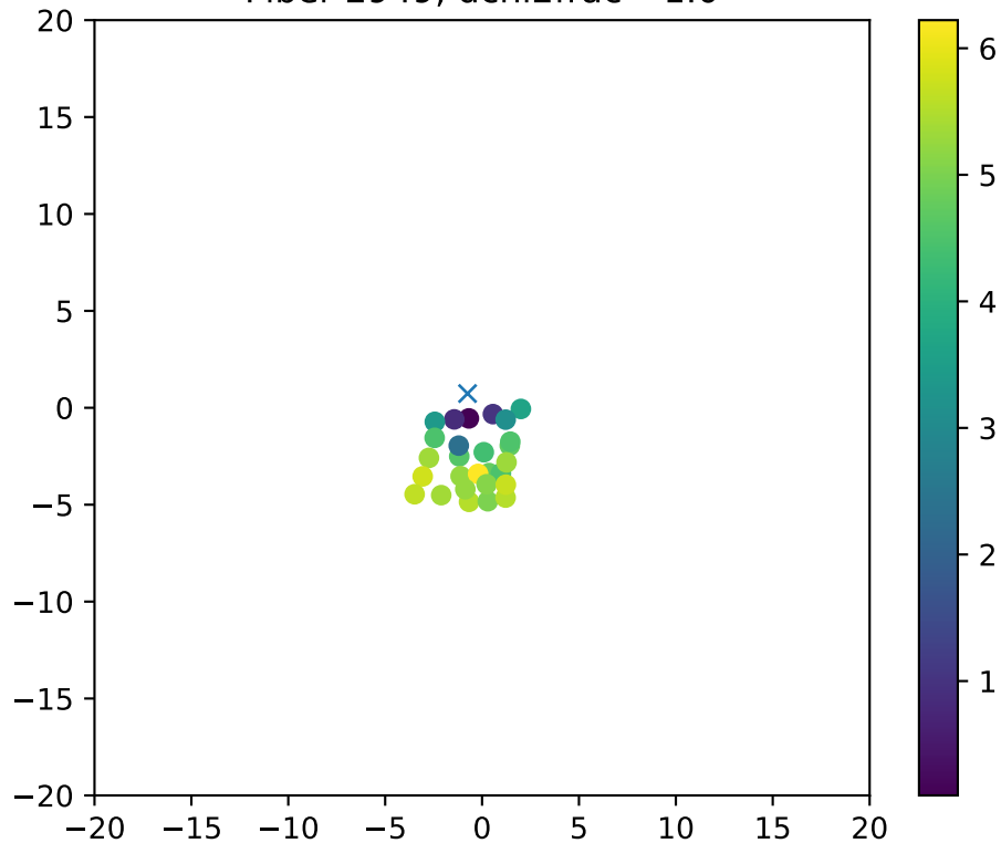
Fiber 2949, dchi2frac= 1.0
