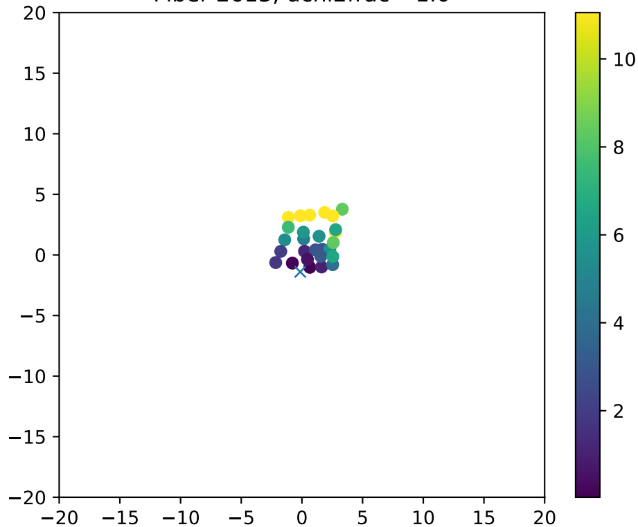
Fiber 2613, dchi2frac= 1.0
