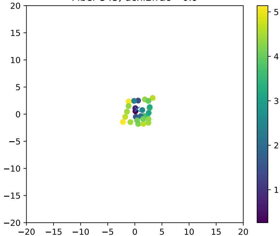
Fiber 345, dchi2frac= 0.9
