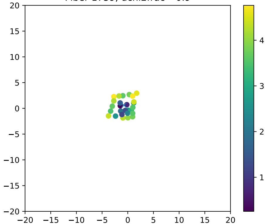
Fiber 1739, dchi2frac= 0.9
