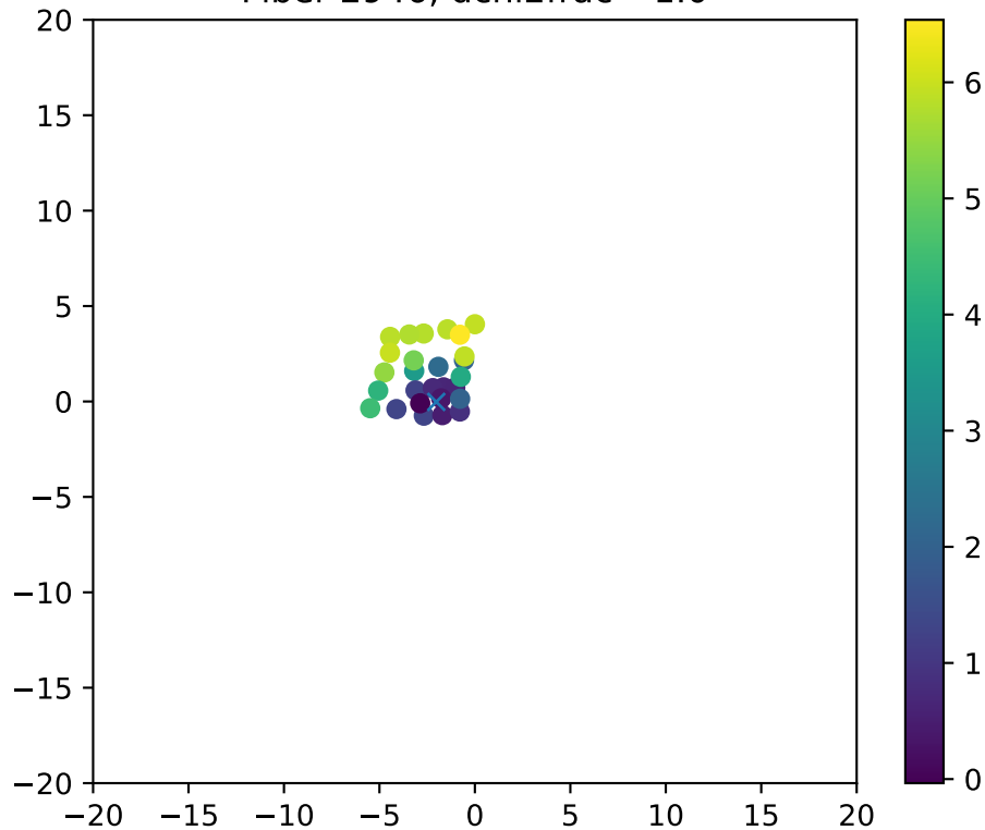
Fiber 2946, dchi2frac= 1.0
