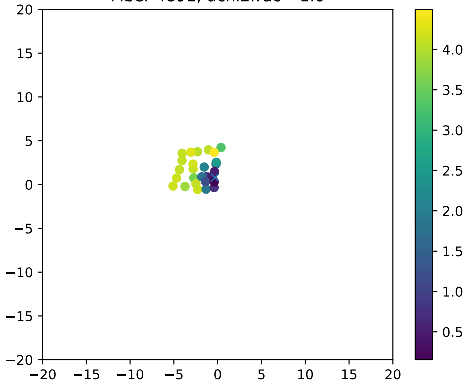
Fiber 4891, dchi2frac= 1.0
