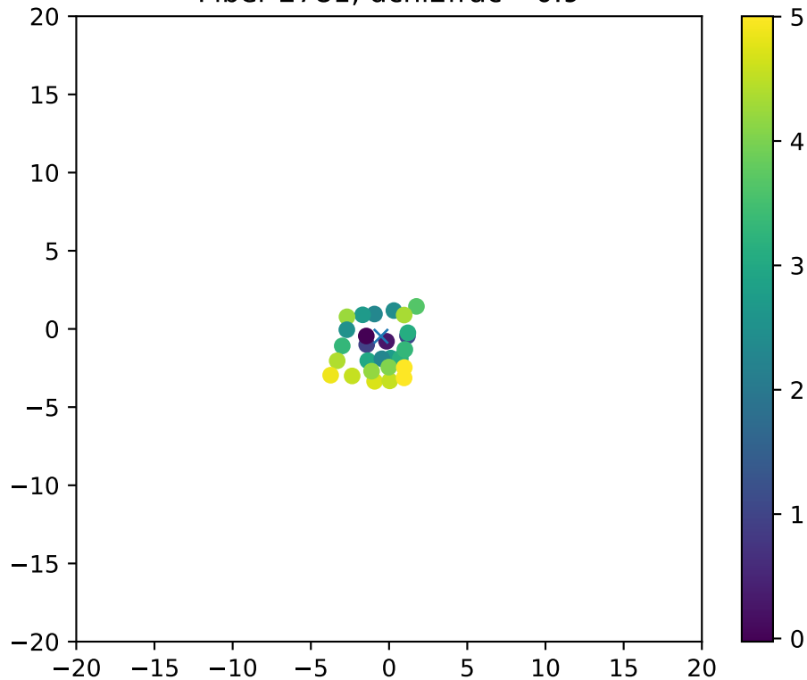
Fiber 2781, dchi2frac= 0.9
