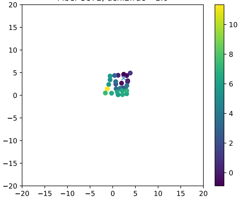
Fiber 3872, dchi2frac= 1.0
