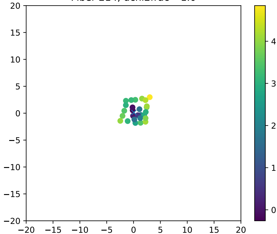
Fiber 214, dchi2frac= 1.0
