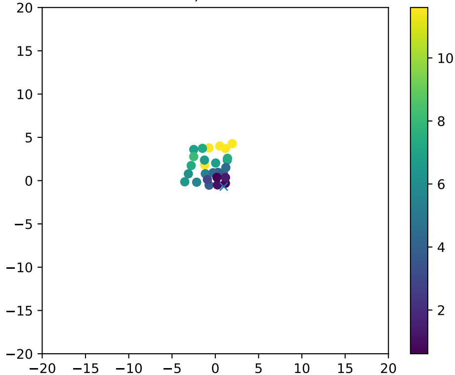
Fiber 3589, dchi2frac= 0.9
