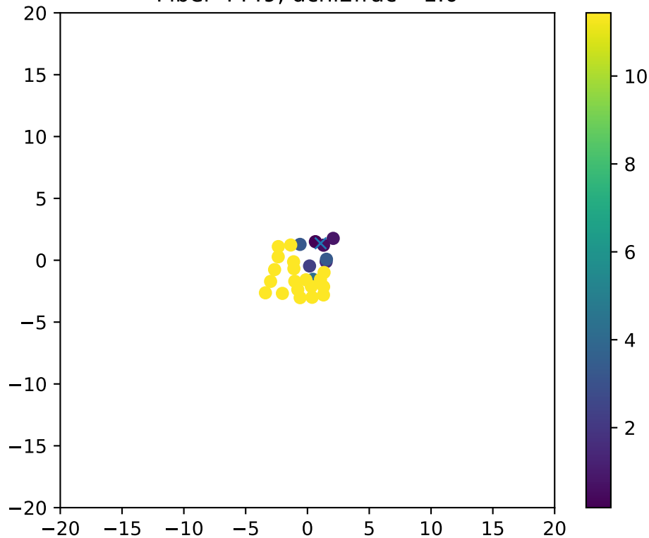
Fiber 4449, dchi2frac= 1.0
