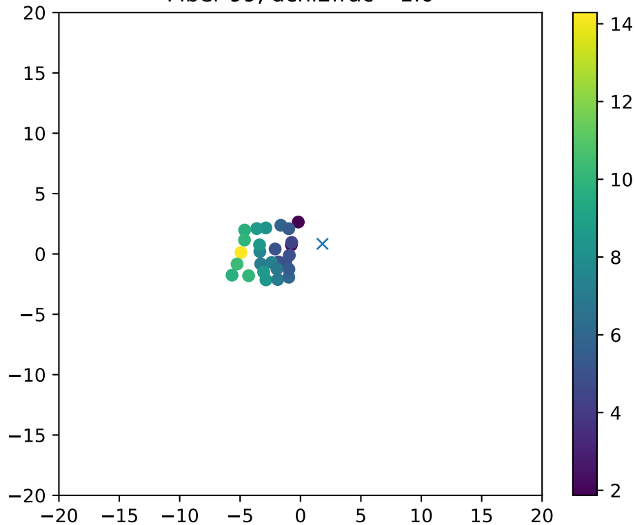
Fiber 99, dchi2frac= 1.0
