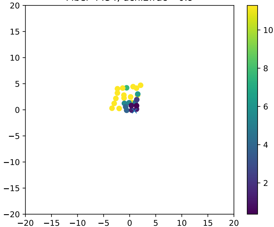
Fiber 4454, dchi2frac= 0.9
