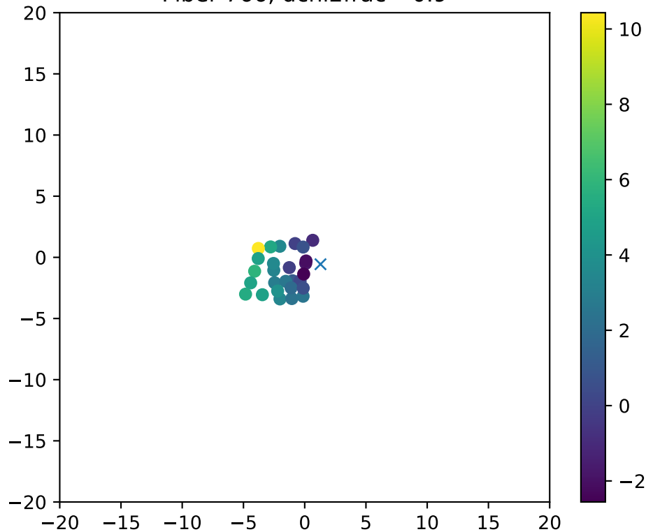
Fiber 766, dchi2frac= 0.9
