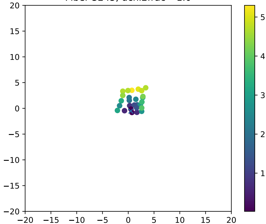
Fiber 3245, dchi2frac= 1.0
