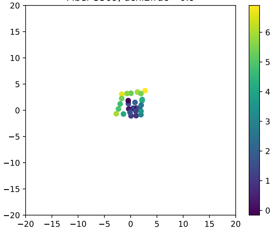
Fiber 3509, dchi2frac= 0.9
