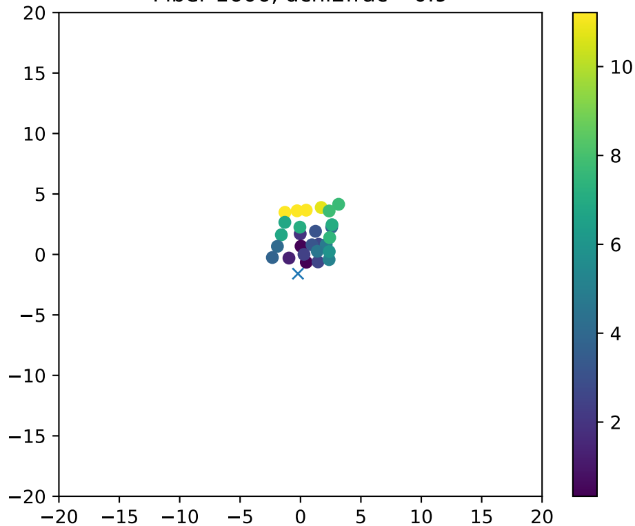
Fiber 1606, dchi2frac= 0.9
