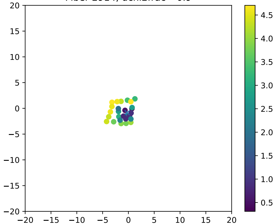
Fiber 2914, dchi2frac= 0.9
