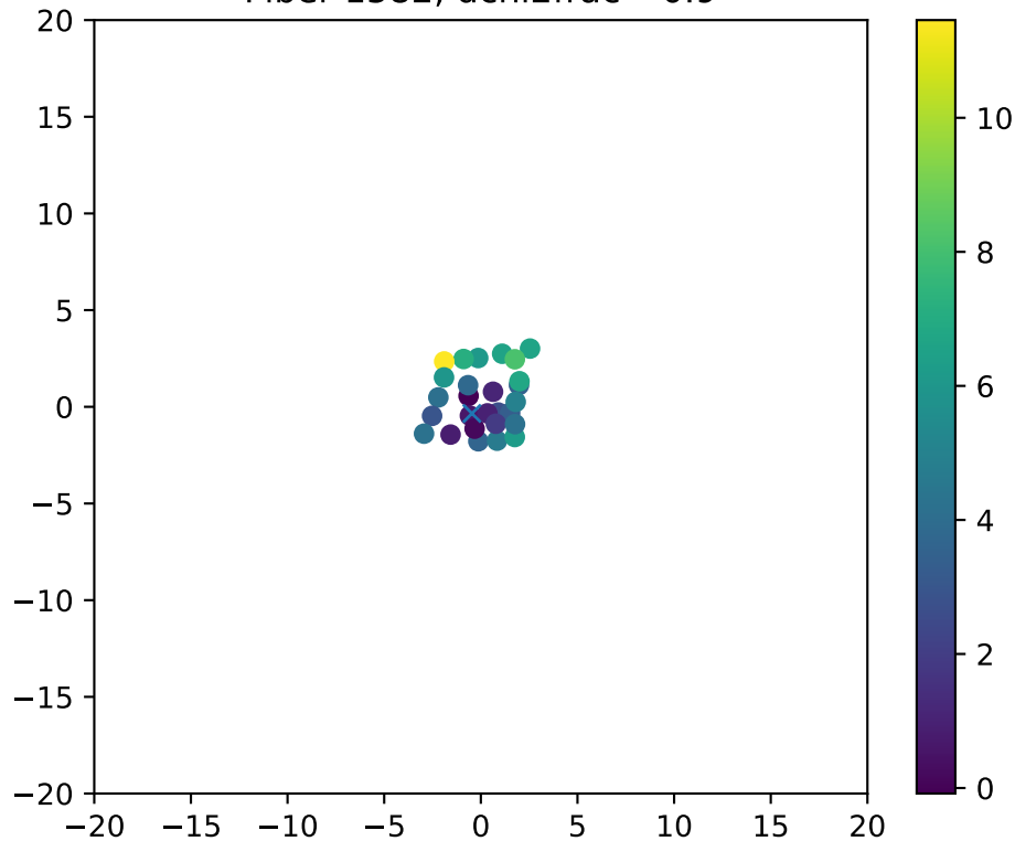
Fiber 1582, dchi2frac= 0.9
