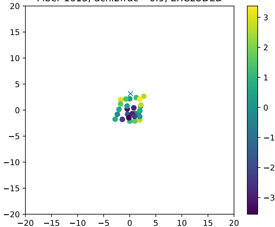
Fiber 1615, dchi2frac= 0.9, EXCLUDED
