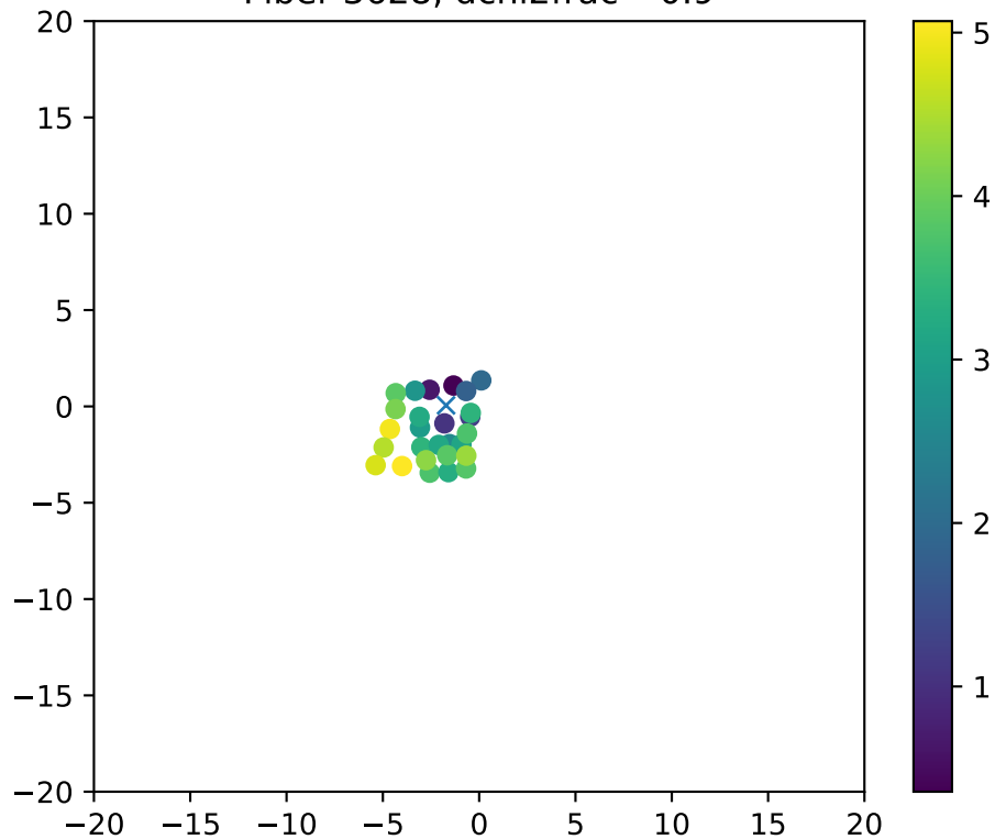
Fiber 3628, dchi2frac= 0.9
