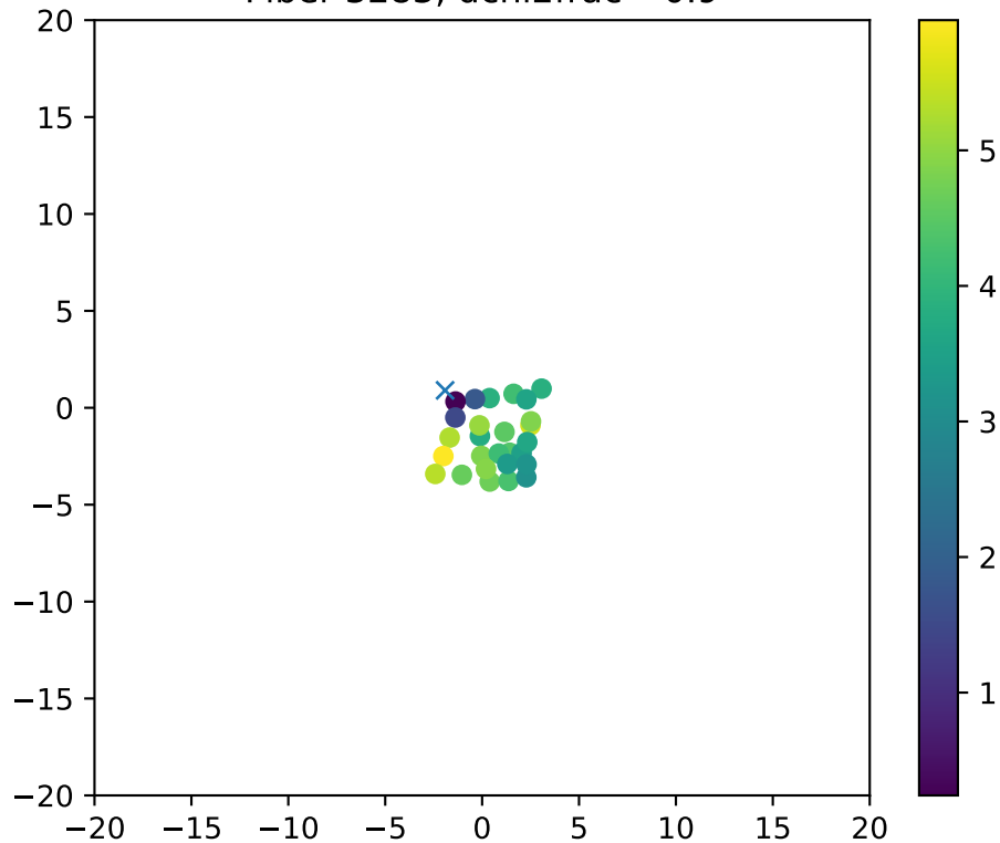
Fiber 3283, dchi2frac= 0.9
