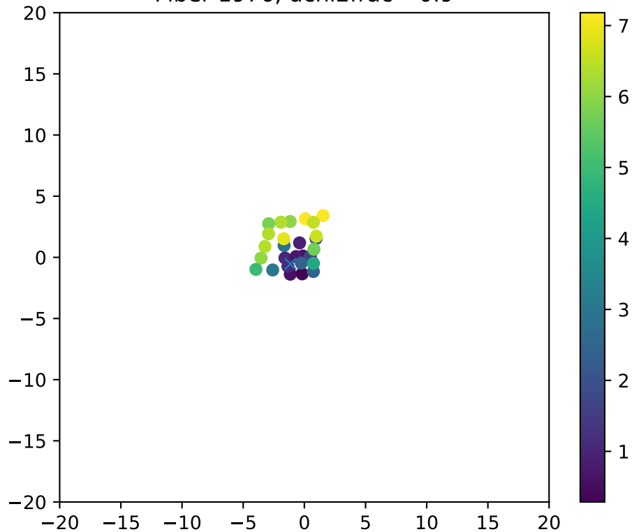
Fiber 1976, dchi2frac= 0.9
