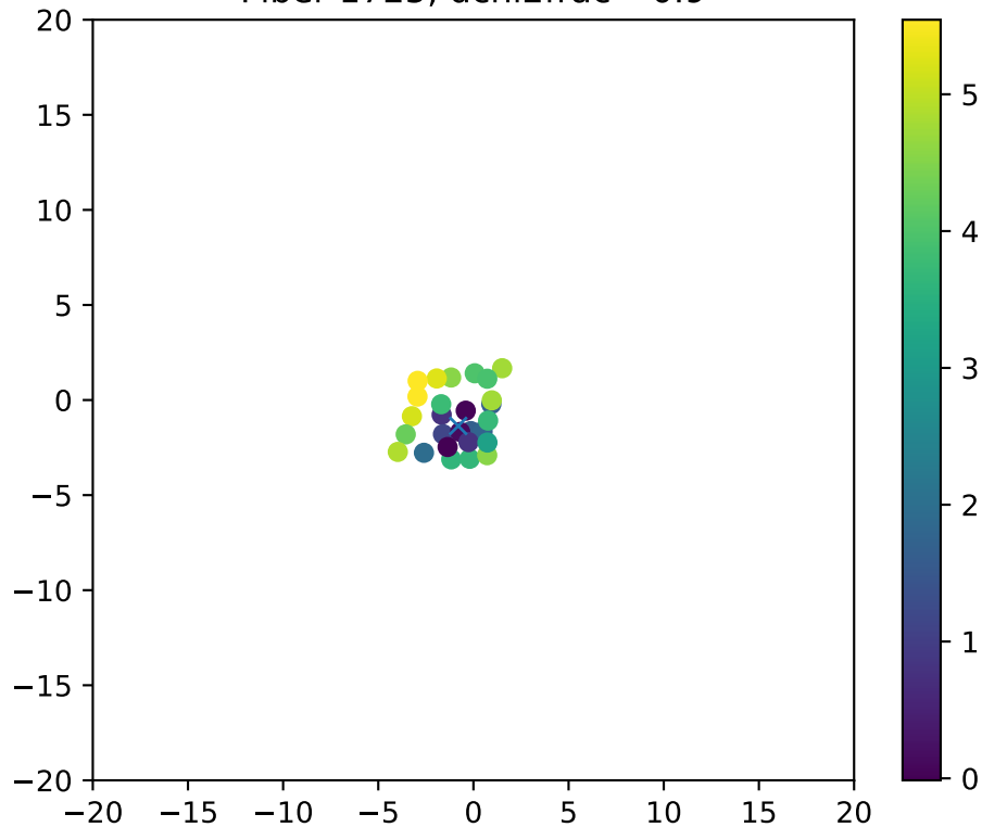
Fiber 1725, dchi2frac= 0.9
