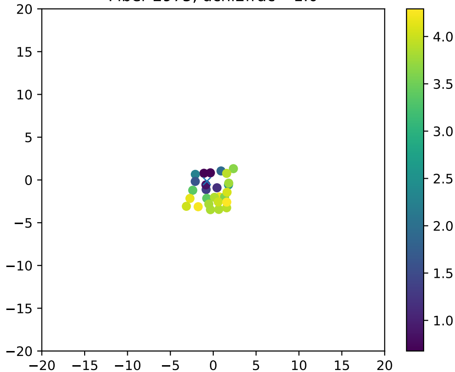
Fiber 2975, dchi2frac= 1.0
