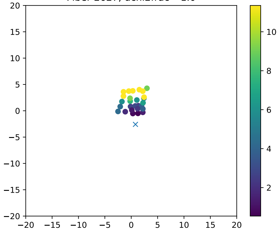
Fiber 2627, dchi2frac= 1.0
