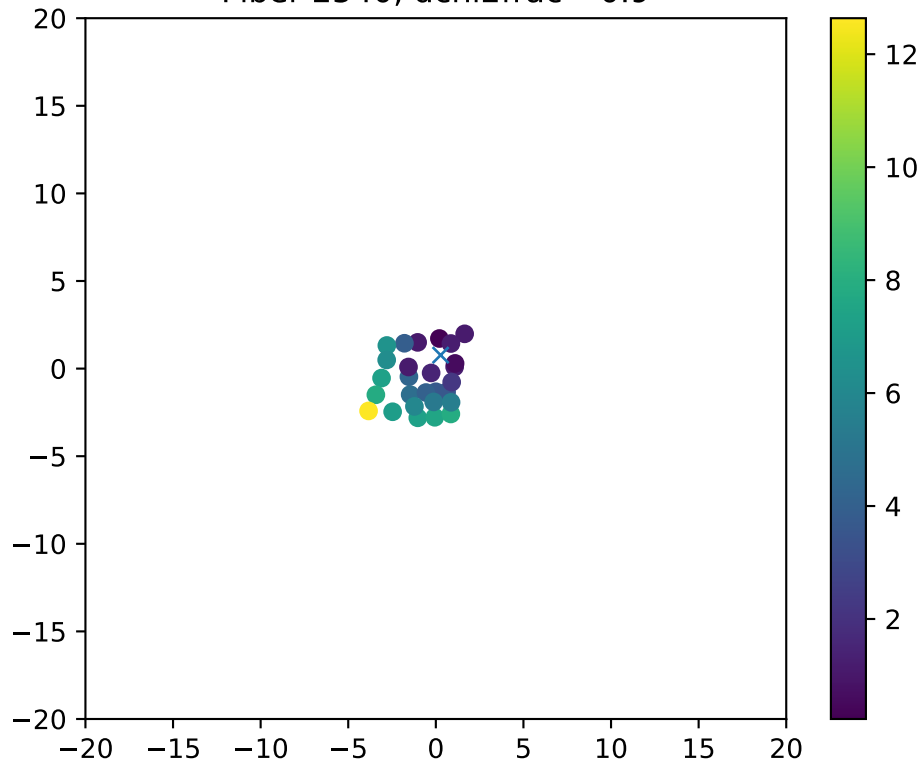
Fiber 2540, dchi2frac= 0.9
