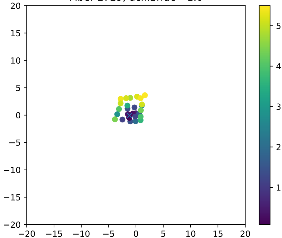
Fiber 2729, dchi2frac= 1.0
