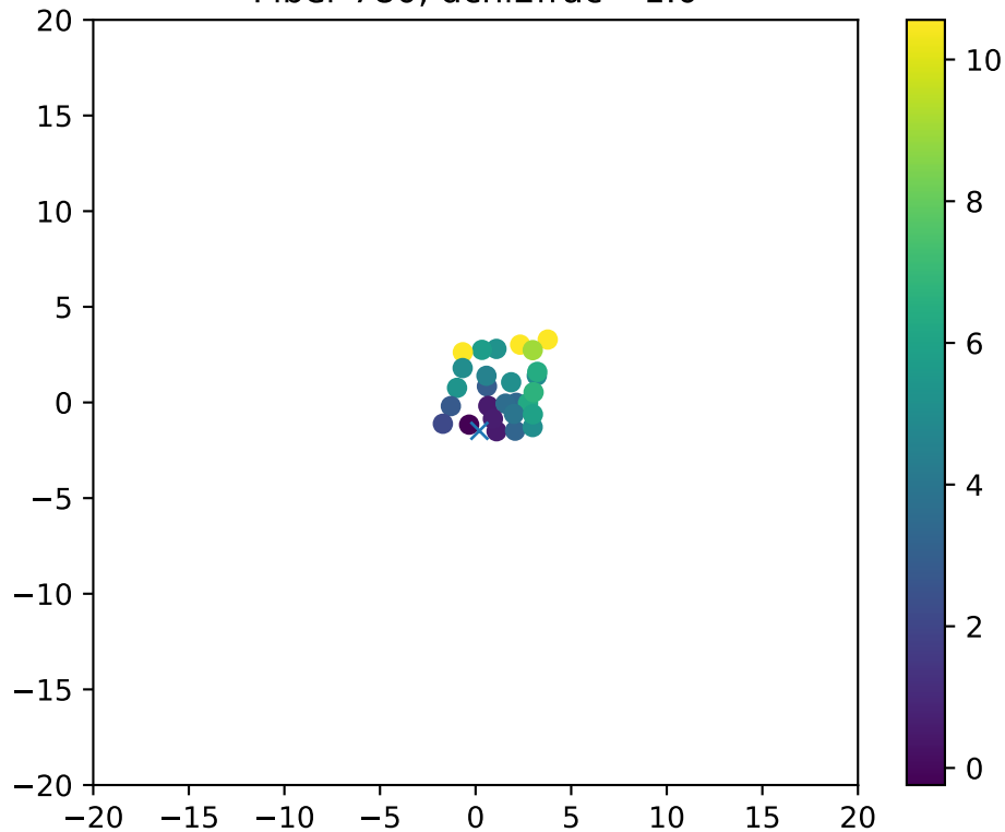
Fiber 780, dchi2frac= 1.0
