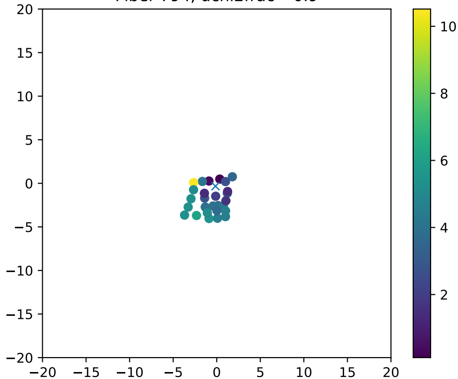
Fiber 794, dchi2frac= 0.9
