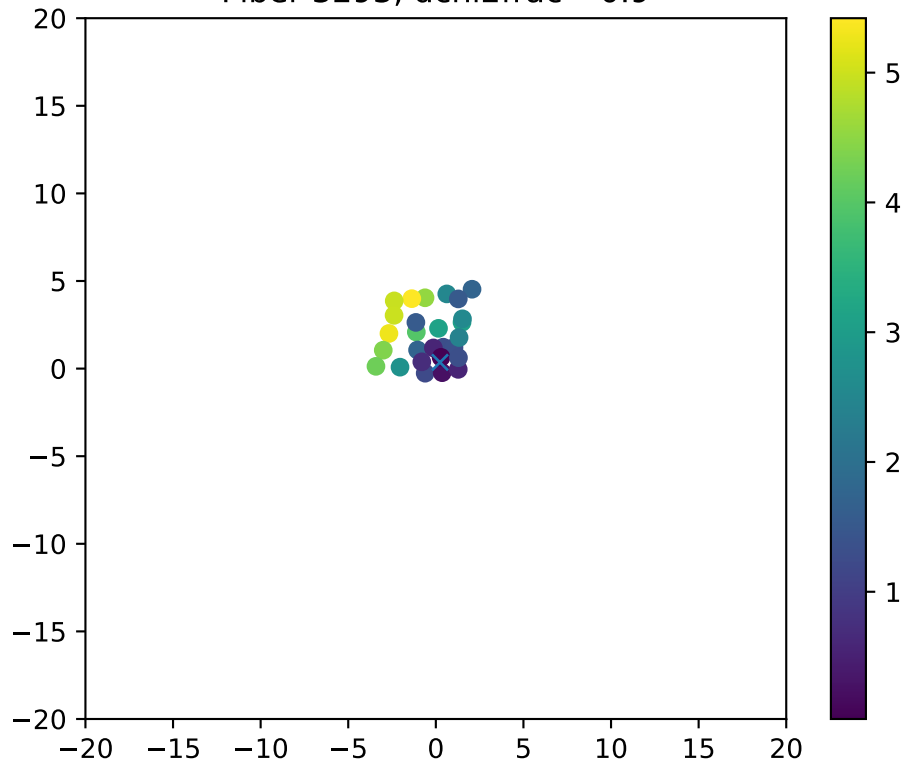
Fiber 3293, dchi2frac= 0.9
