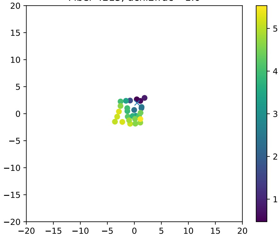
Fiber 4215, dchi2frac= 1.0
