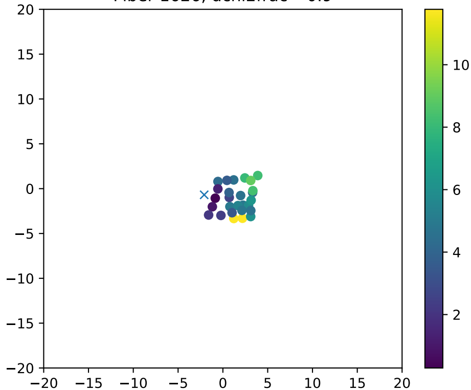
Fiber 1626, dchi2frac= 0.9
