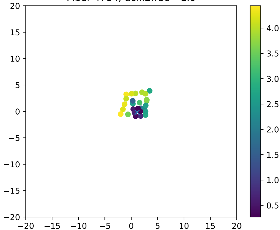
Fiber 4784, dchi2frac= 1.0
