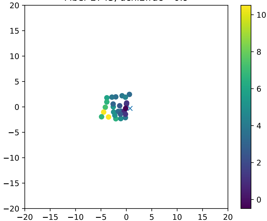
Fiber 2743, dchi2frac= 0.9
