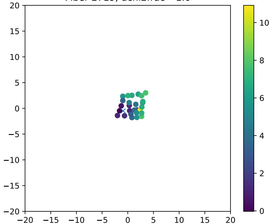
Fiber 2719, dchi2frac= 1.0
