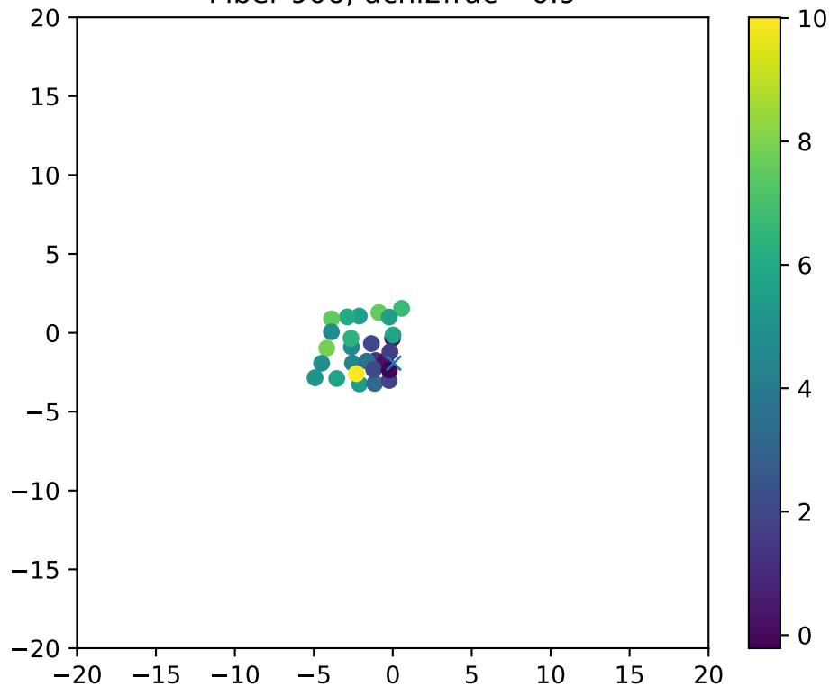
Fiber 906, dchi2frac= 0.9
