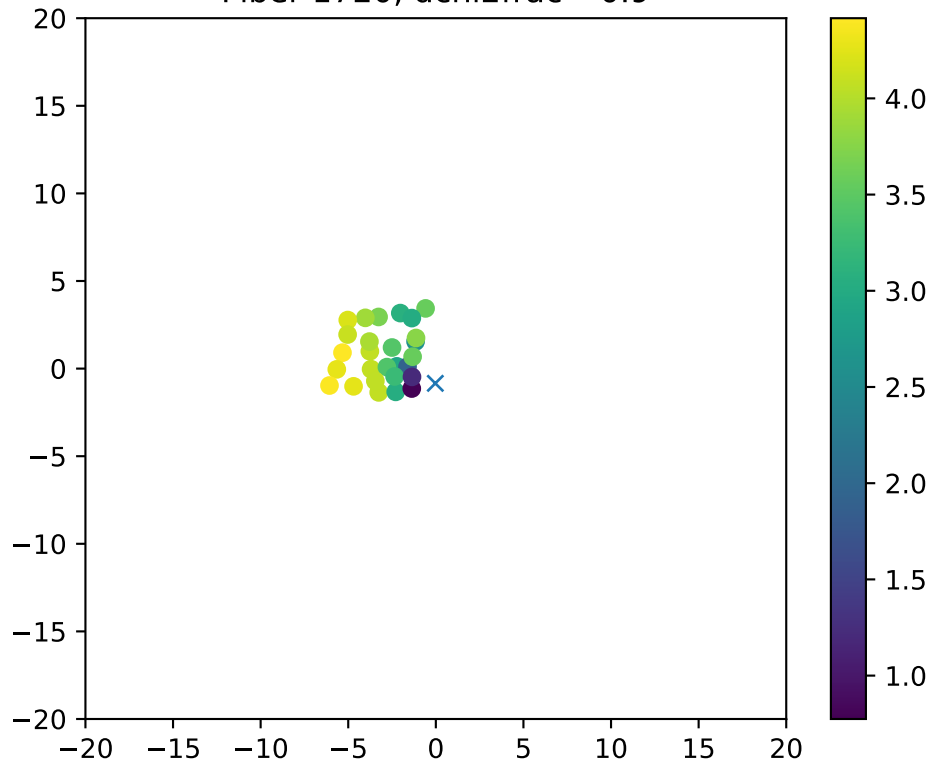
Fiber 1720, dchi2frac= 0.9
