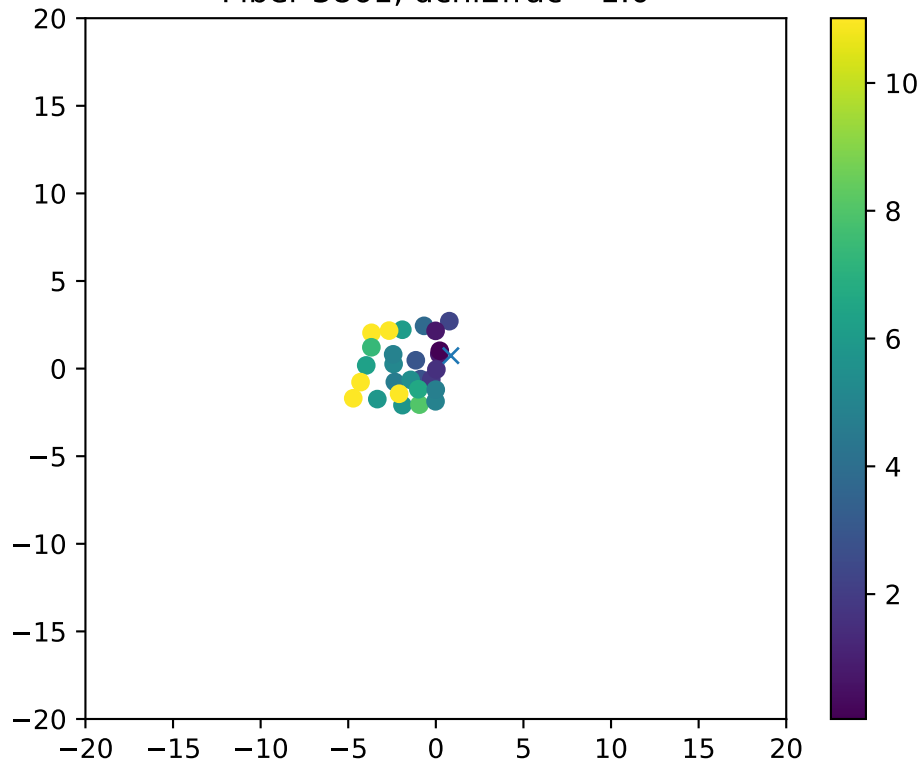
Fiber 3861, dchi2frac= 1.0
