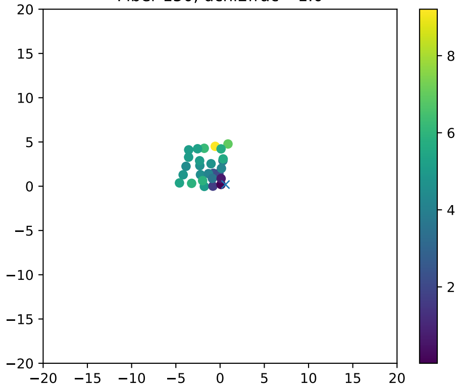
Fiber 150, dchi2frac= 1.0
