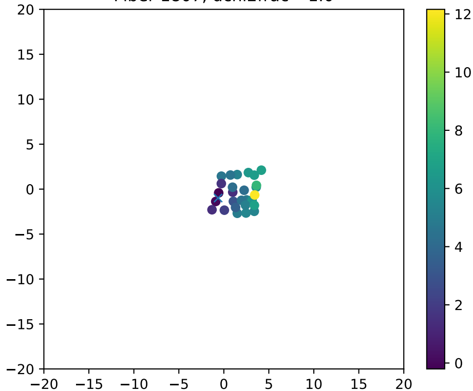
Fiber 1807, dchi2frac= 1.0
