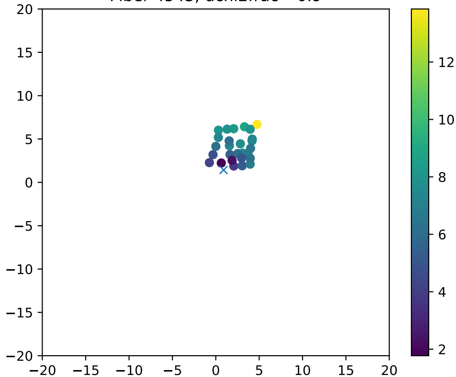
Fiber 4543, dchi2frac= 0.9
