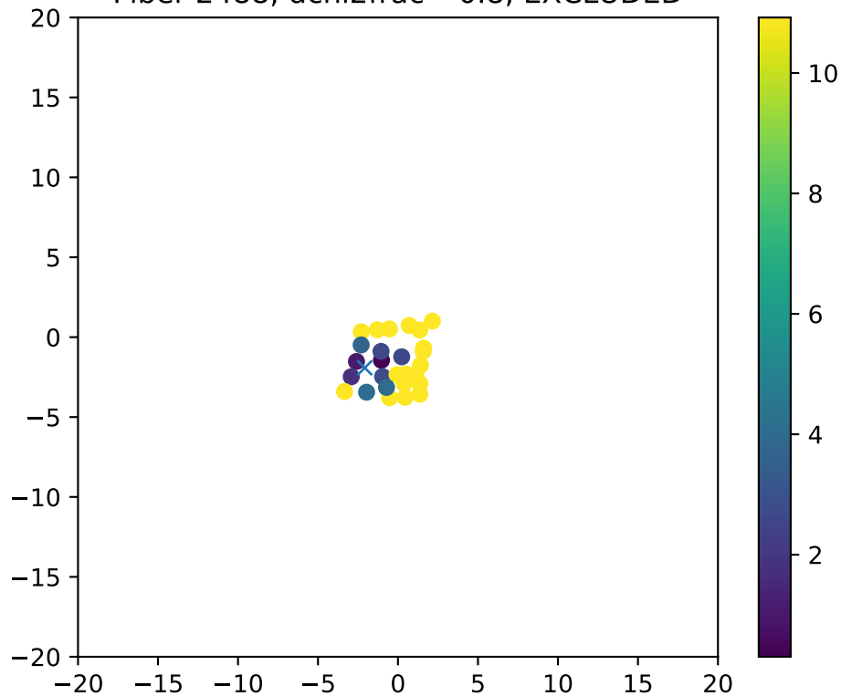
Fiber 2488, dchi2frac= 0.8, EXCLUDED
