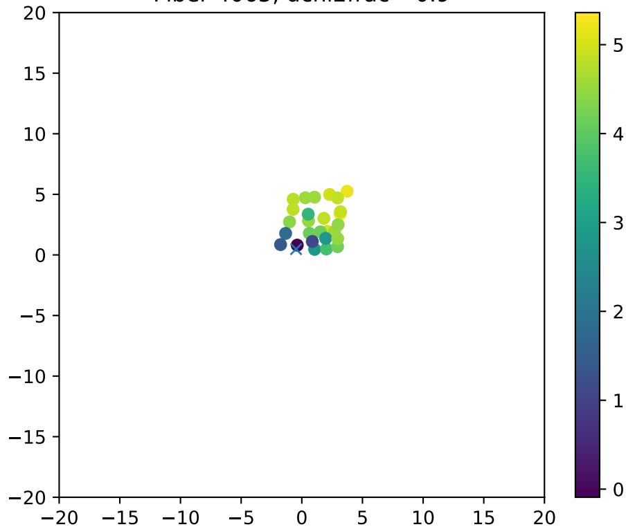
Fiber 4065, dchi2frac= 0.9
