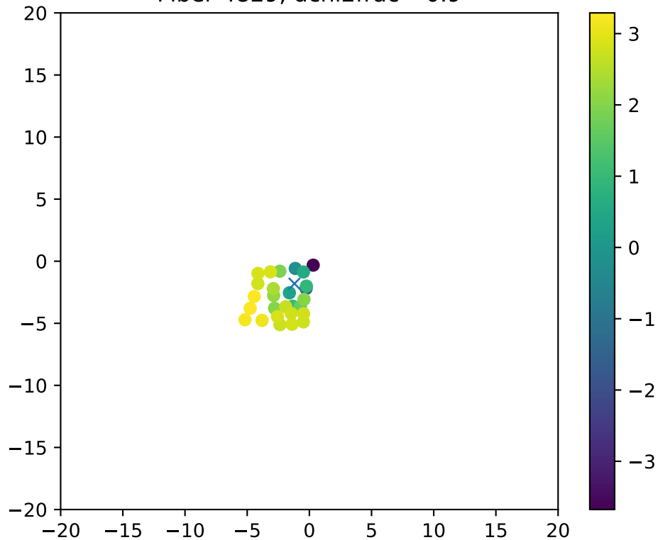
Fiber 4829, dchi2frac= 0.9
