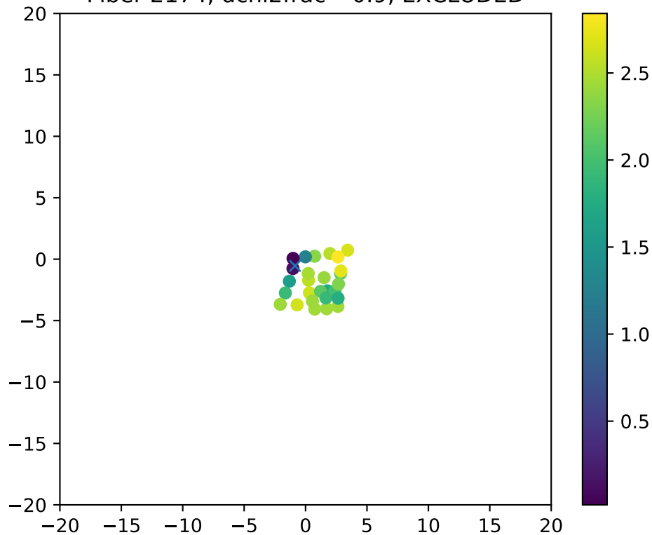
Fiber 2174, dchi2frac= 0.9, EXCLUDED
