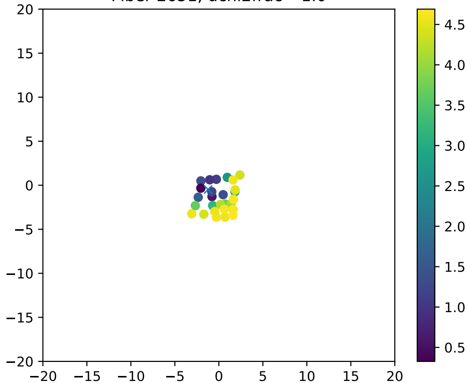
Fiber 2651, dchi2frac= 1.0
