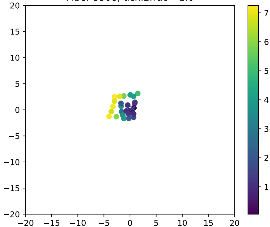
Fiber 3508, dchi2frac= 1.0
