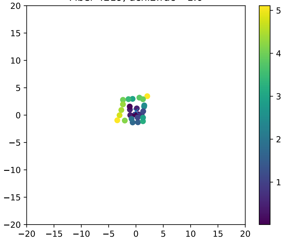
Fiber 4219, dchi2frac= 1.0
