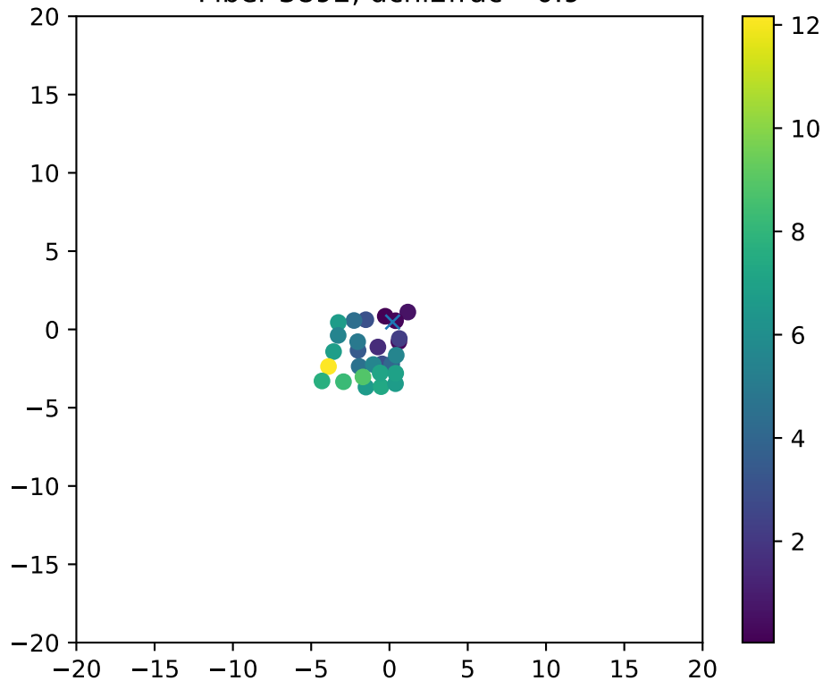
Fiber 3892, dchi2frac= 0.9
