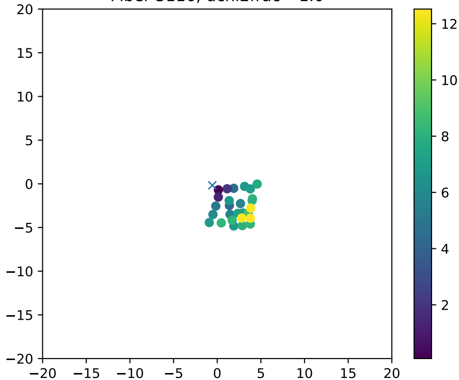
Fiber 3116, dchi2frac= 1.0
