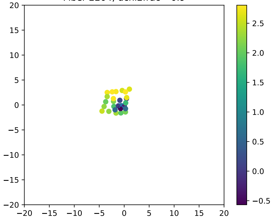
Fiber 2204, dchi2frac= 0.9
