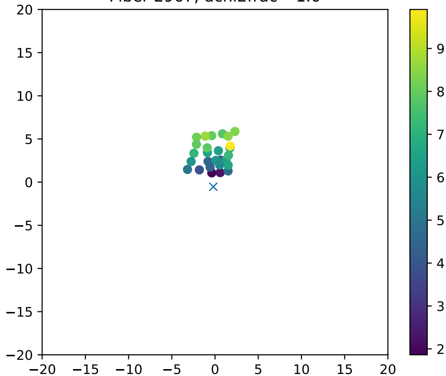
Fiber 2967, dchi2frac= 1.0
