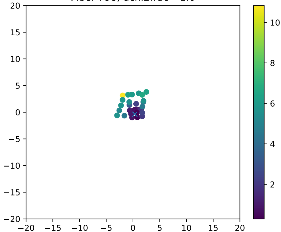
Fiber 798, dchi2frac= 1.0
