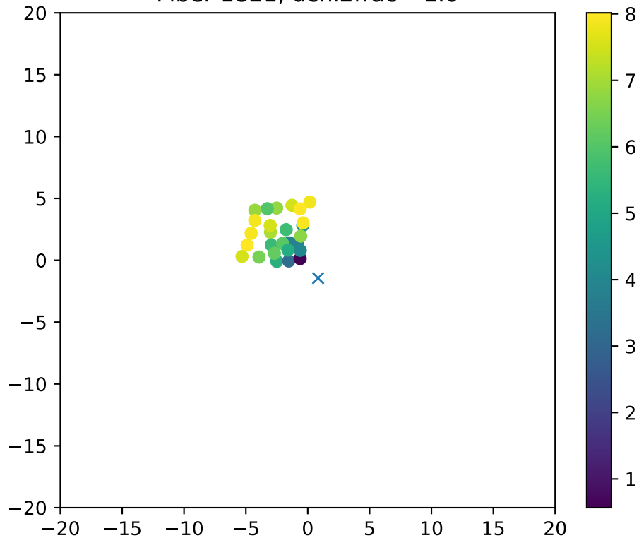
Fiber 1821, dchi2frac= 1.0
