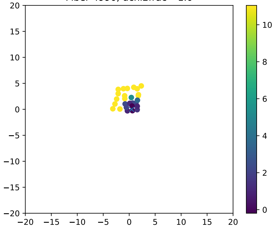
Fiber 4990, dchi2frac= 1.0
