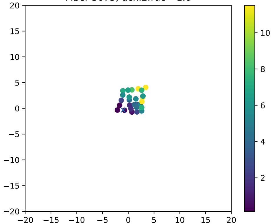
Fiber 3075, dchi2frac= 1.0
