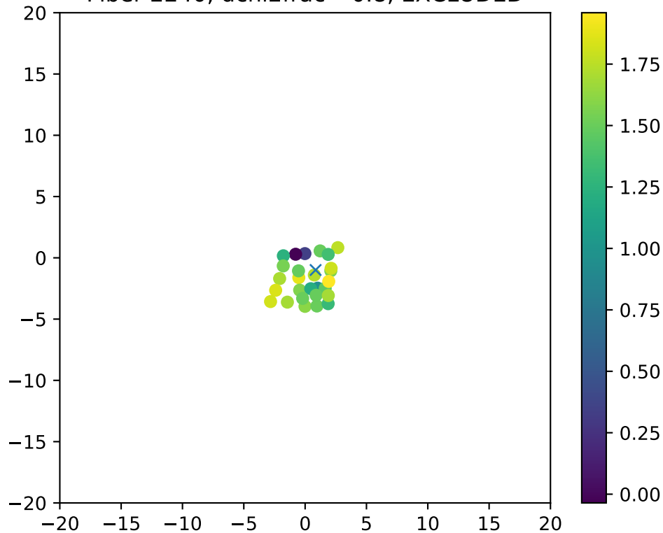
Fiber 2240, dchi2frac= 0.8, EXCLUDED
