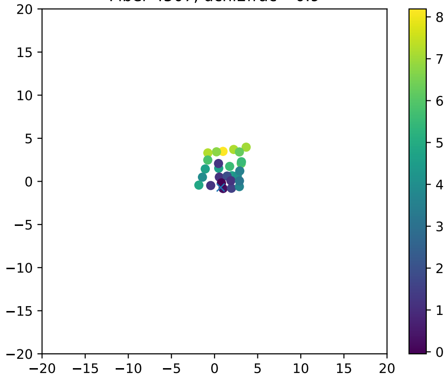
Fiber 4507, dchi2frac= 0.9
