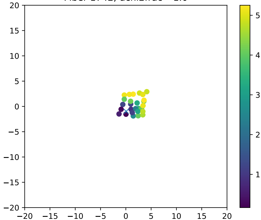
Fiber 1742, dchi2frac= 1.0
