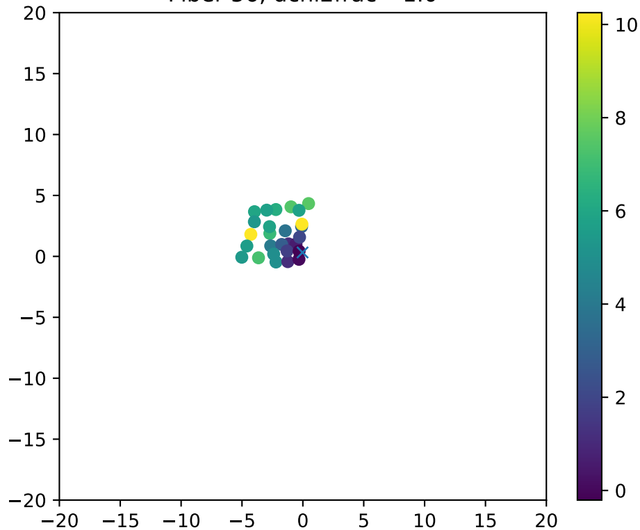
Fiber 56, dchi2frac= 1.0
