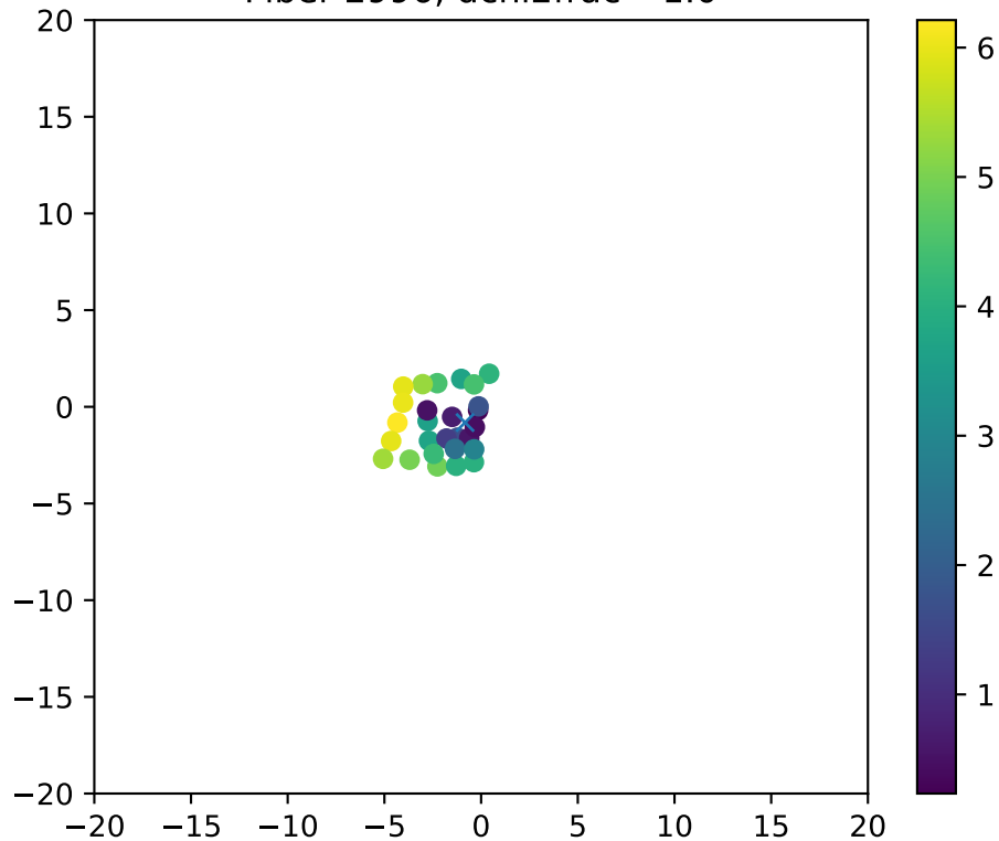
Fiber 2996, dchi2frac= 1.0
