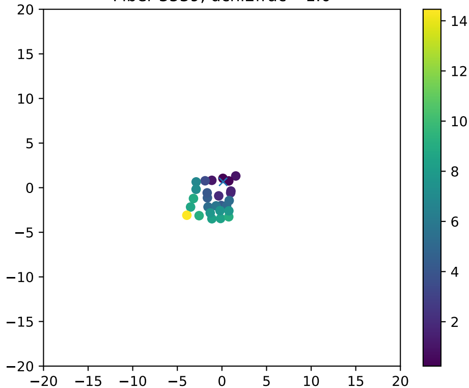
Fiber 3539, dchi2frac= 1.0
