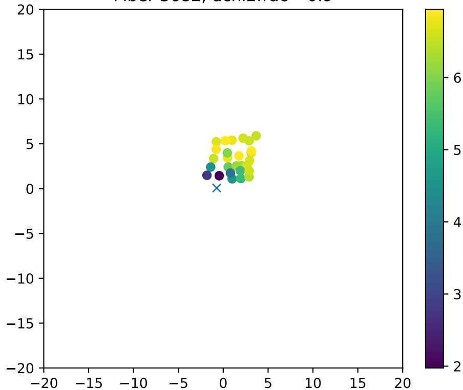
Fiber 3682, dchi2frac= 0.9
