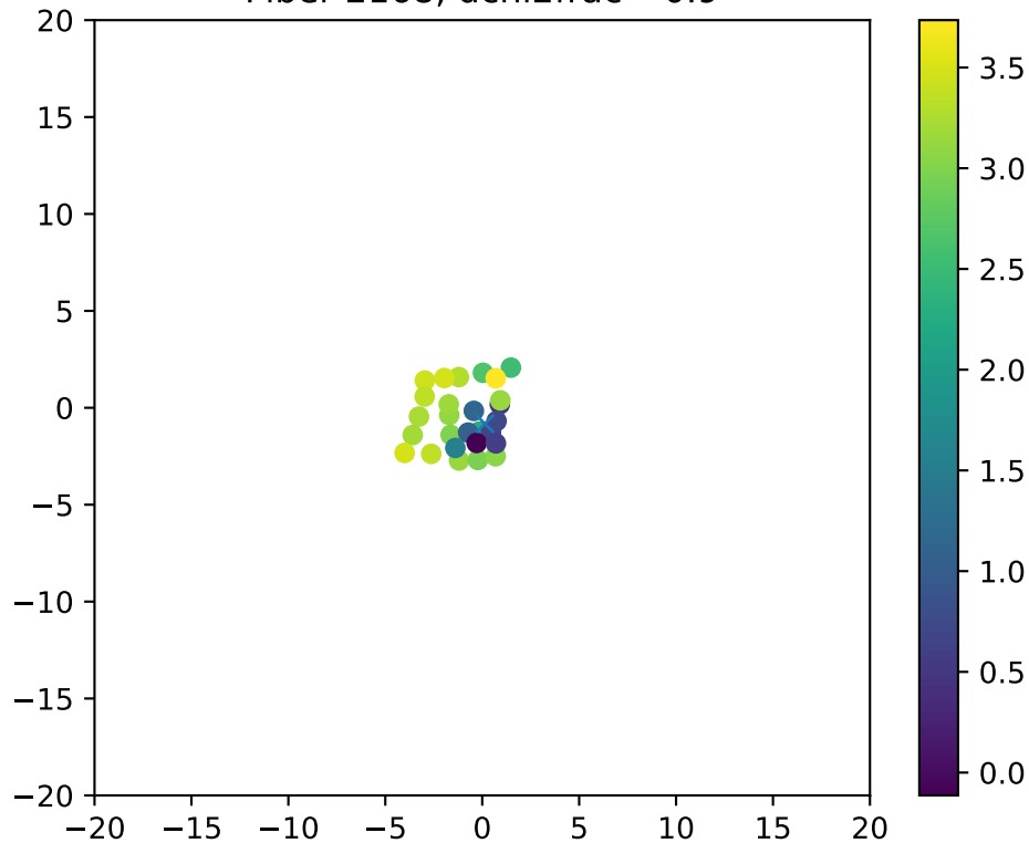
Fiber 2168, dchi2frac= 0.9
