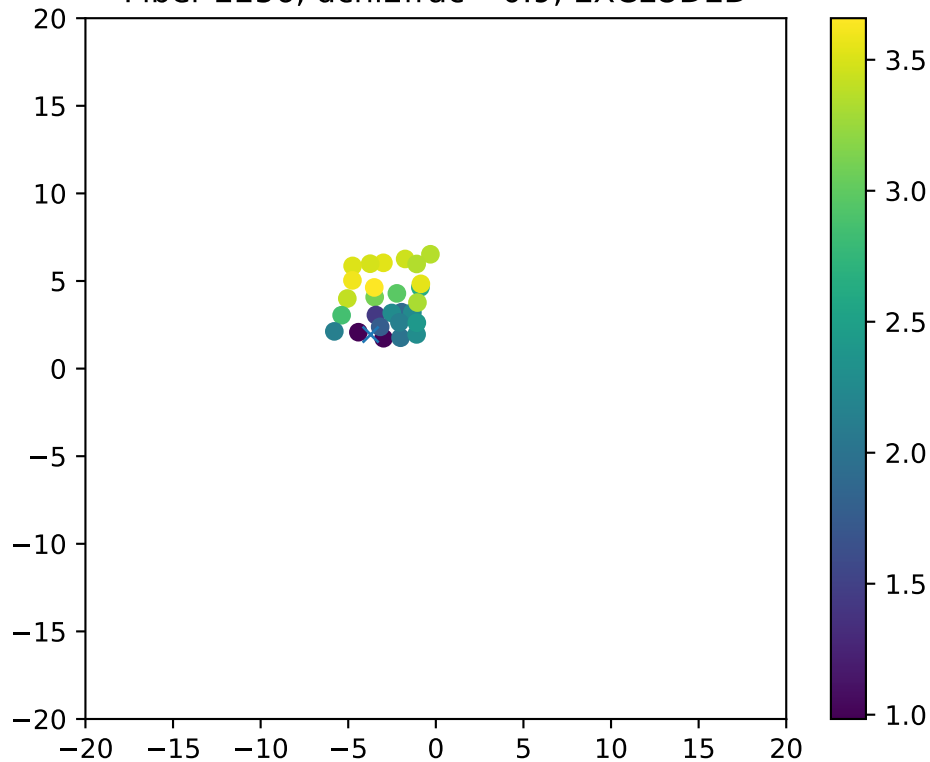
Fiber 2256, dchi2frac= 0.9, EXCLUDED
