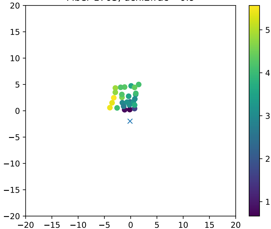
Fiber 1703, dchi2frac= 0.9
