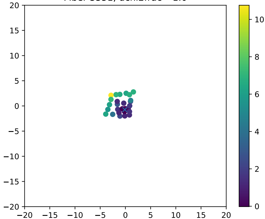
Fiber 3351, dchi2frac= 1.0
