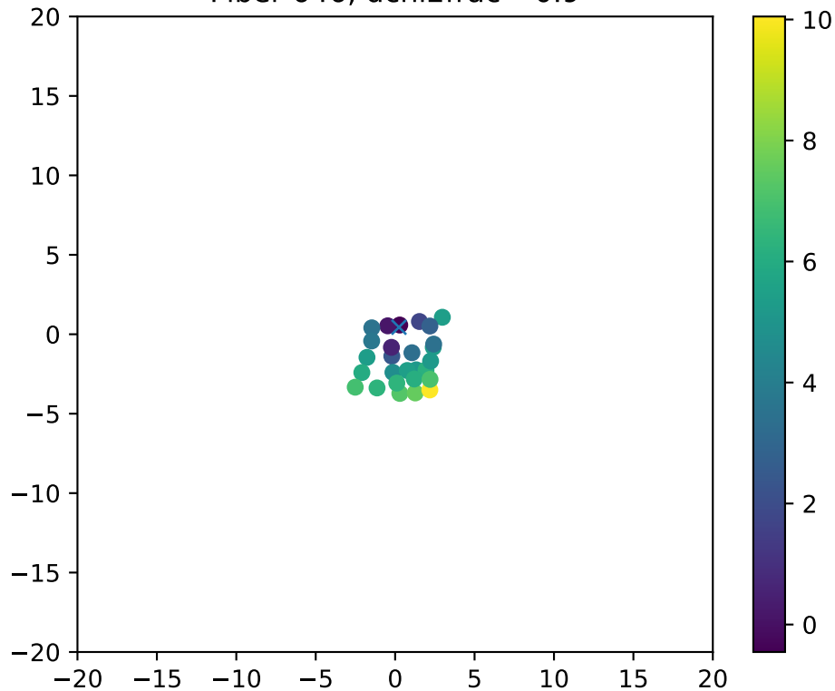
Fiber 646, dchi2frac= 0.9
