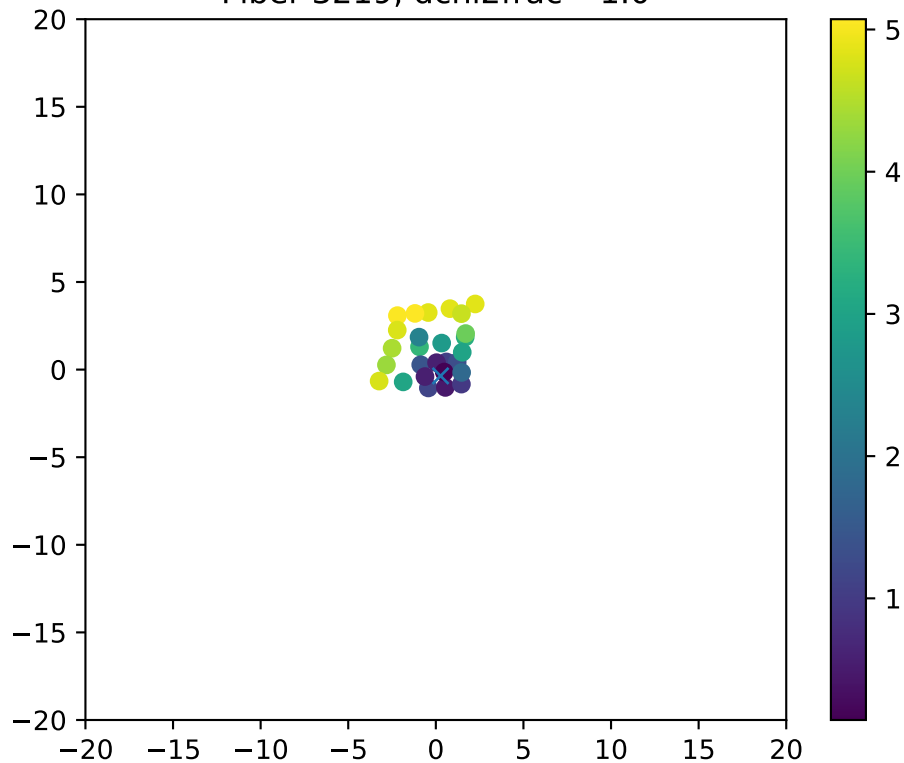
Fiber 3219, dchi2frac= 1.0
