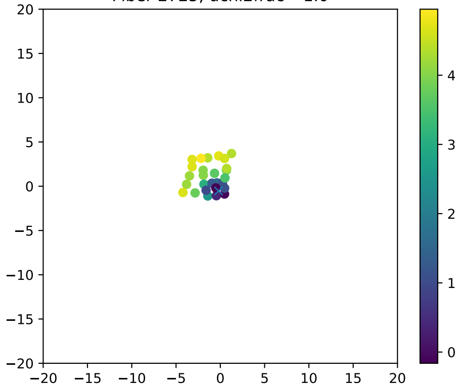
Fiber 2725, dchi2frac= 1.0
