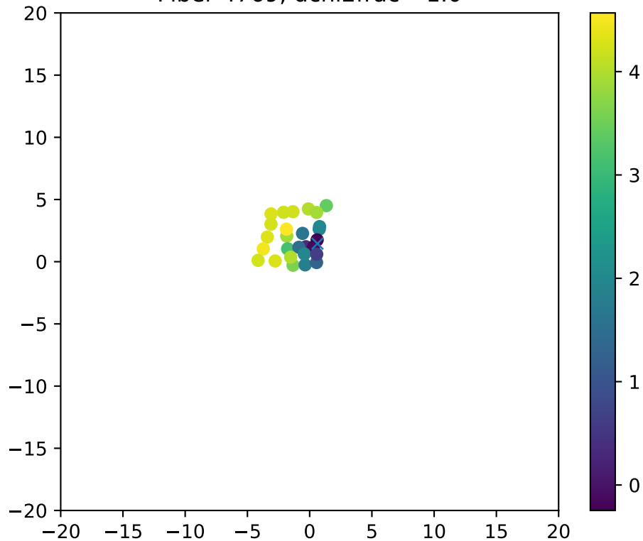
Fiber 4769, dchi2frac= 1.0
