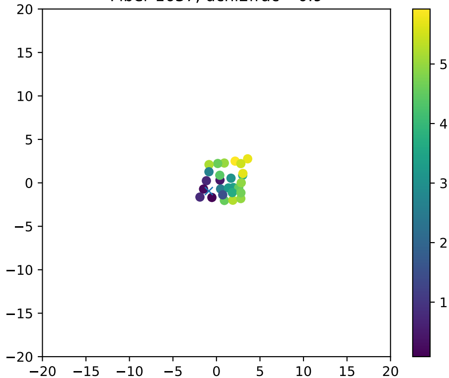
Fiber 1637, dchi2frac= 0.9
