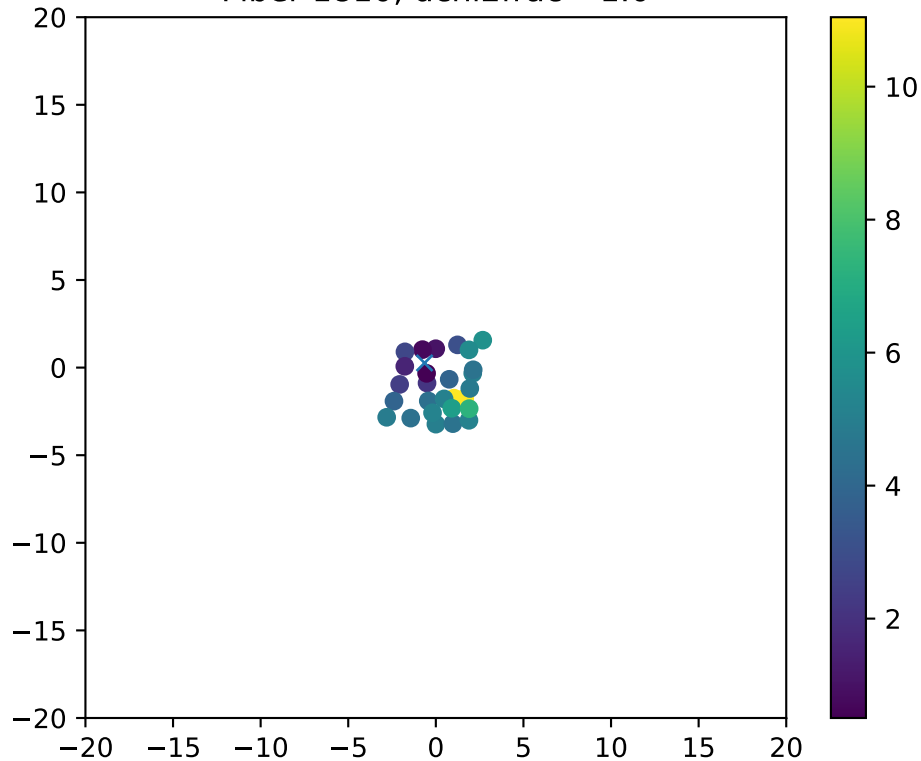
Fiber 1810, dchi2frac= 1.0
