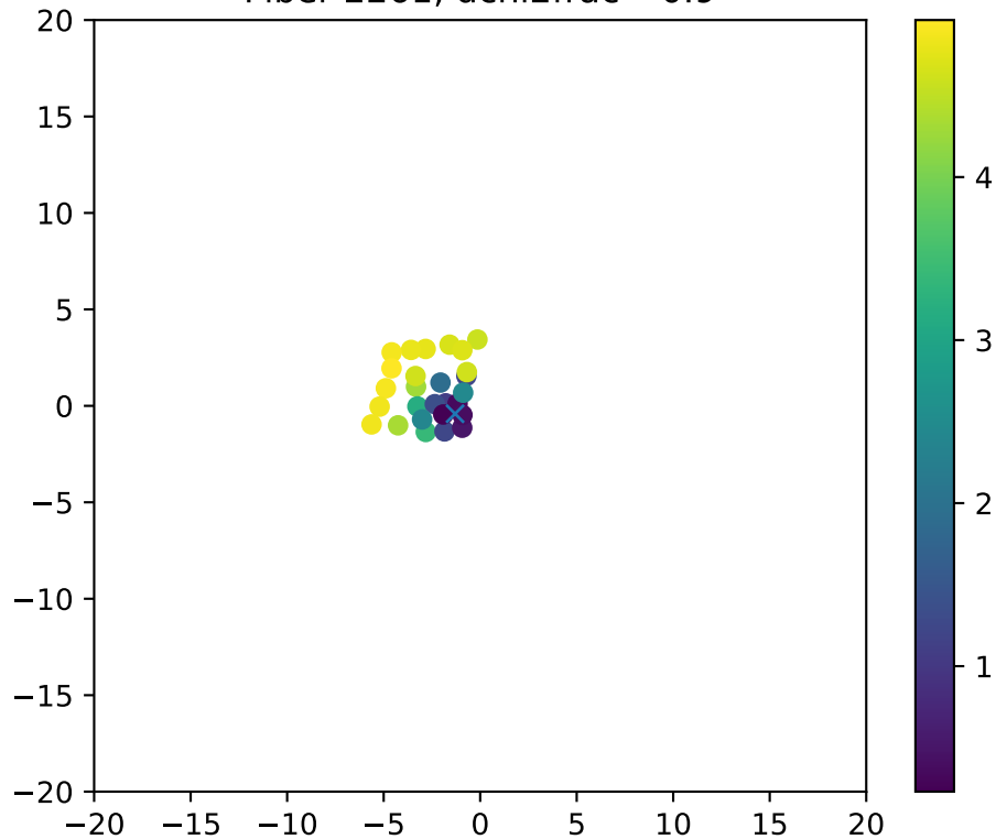
Fiber 2261, dchi2frac= 0.9
