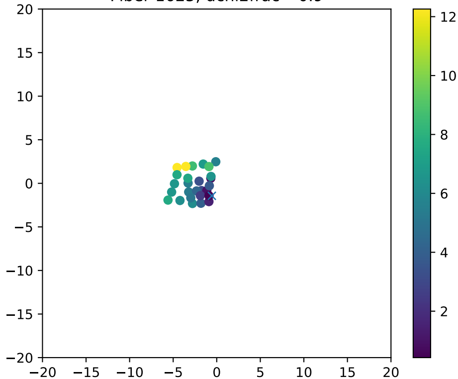
Fiber 1625, dchi2frac= 0.9
