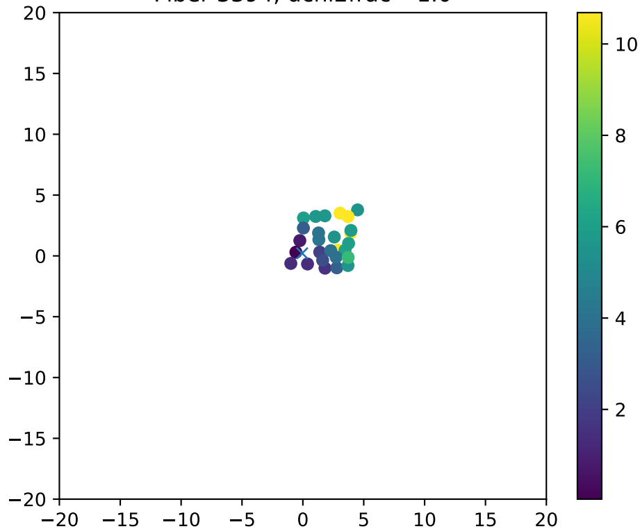
Fiber 3394, dchi2frac= 1.0
