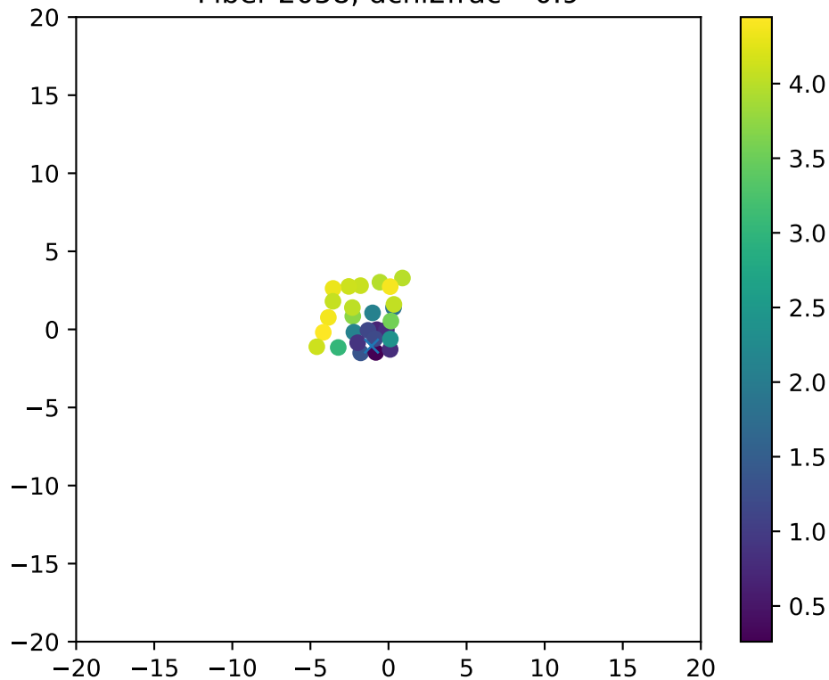
Fiber 2058, dchi2frac= 0.9
