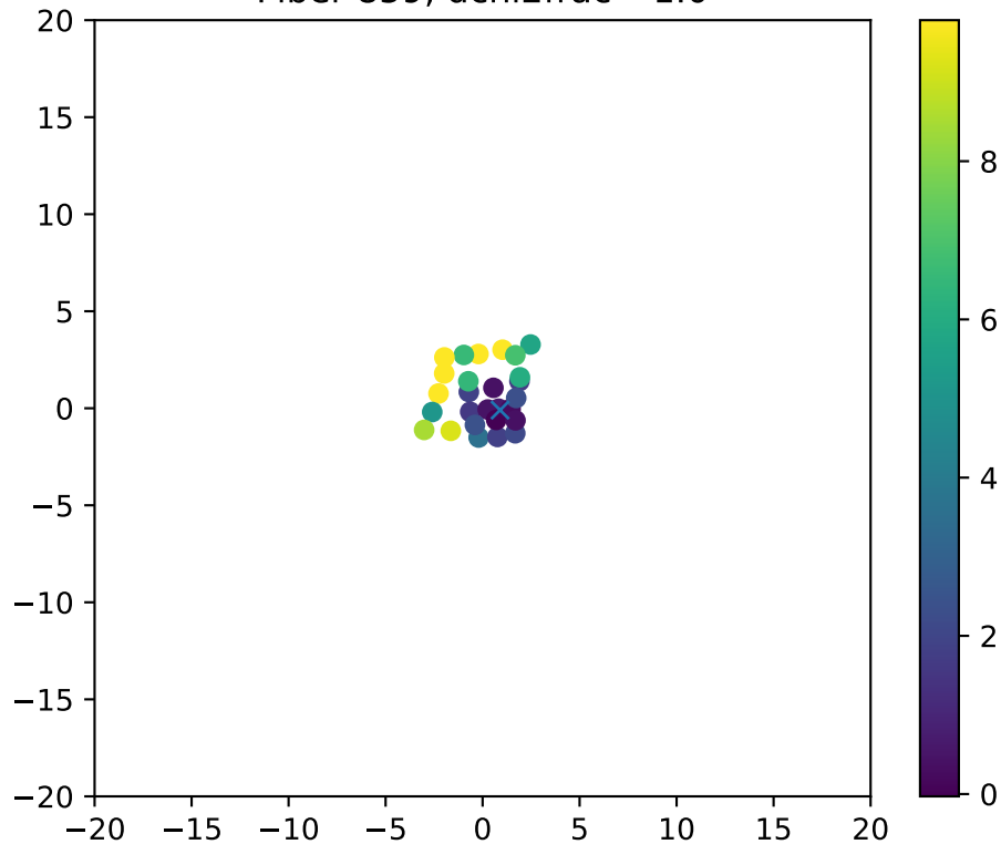
Fiber 859, dchi2frac= 1.0
