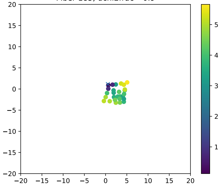
Fiber 185, dchi2frac= 0.9
