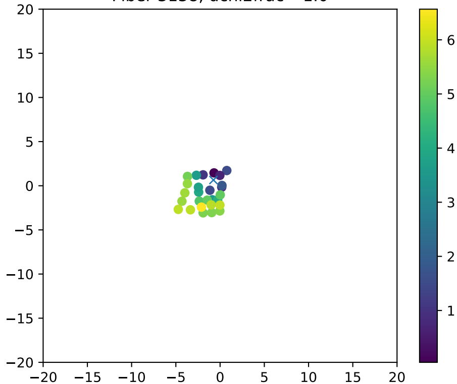
Fiber 3138, dchi2frac= 1.0
