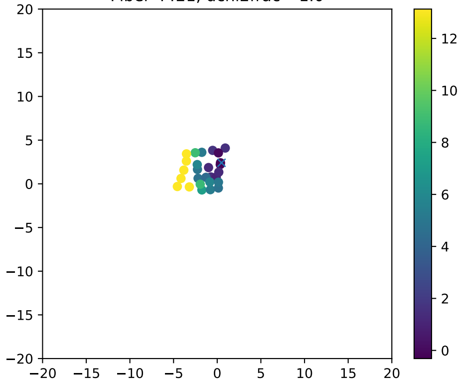
Fiber 4421, dchi2frac= 1.0
