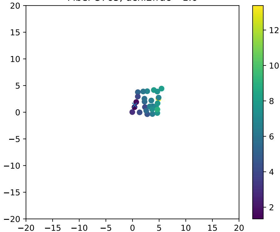
Fiber 3765, dchi2frac= 1.0
