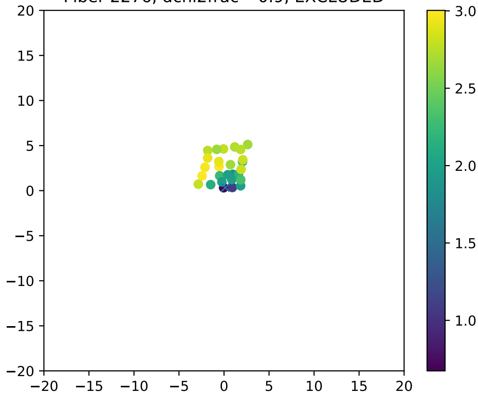
Fiber 2276, dchi2frac= 0.9, EXCLUDED
