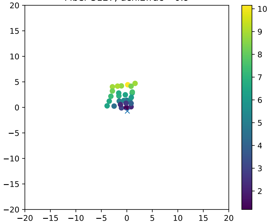
Fiber 3127, dchi2frac= 0.9
