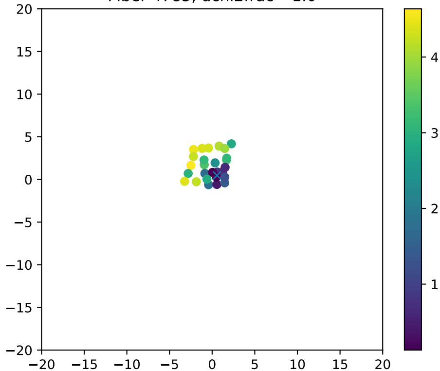
Fiber 4785, dchi2frac= 1.0
