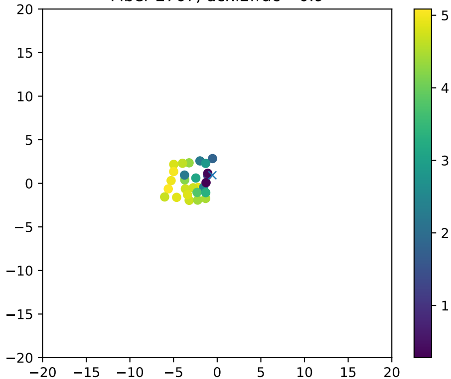
Fiber 2767, dchi2frac= 0.9
