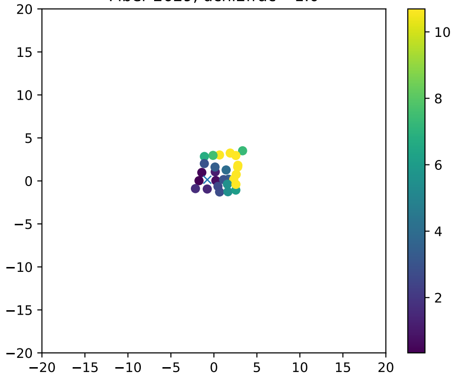
Fiber 2629, dchi2frac= 1.0
