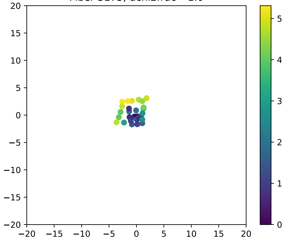
Fiber 3175, dchi2frac= 1.0
