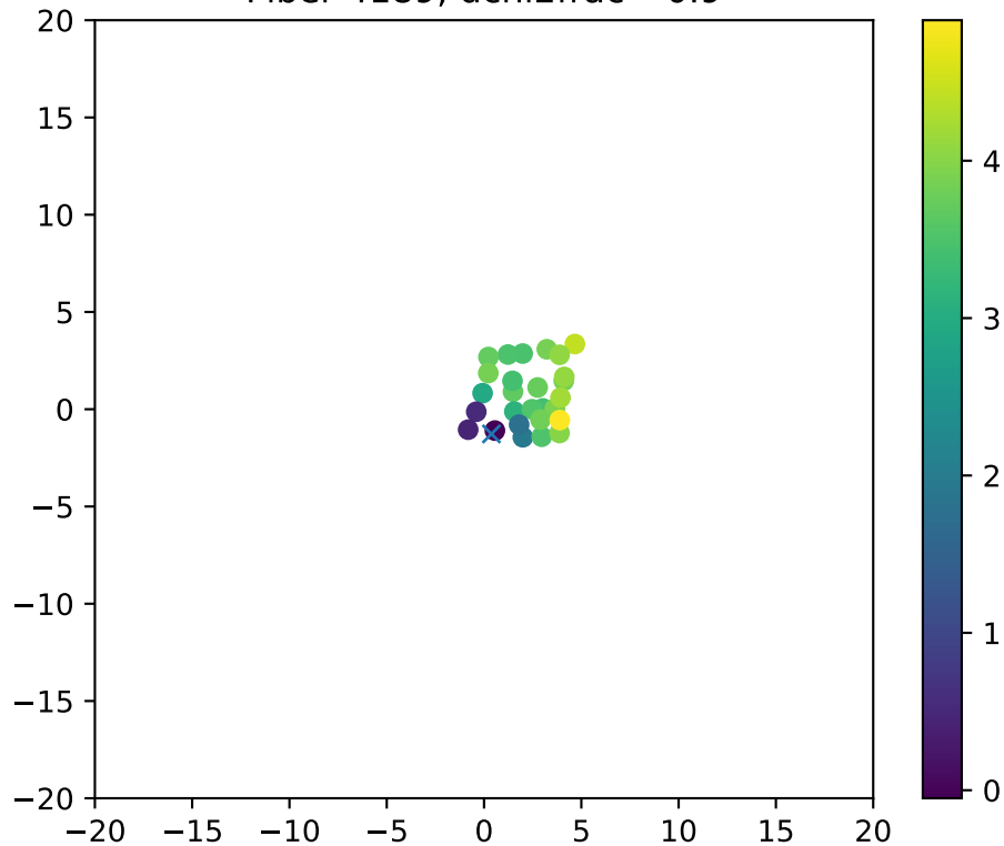
Fiber 4189, dchi2frac= 0.9
