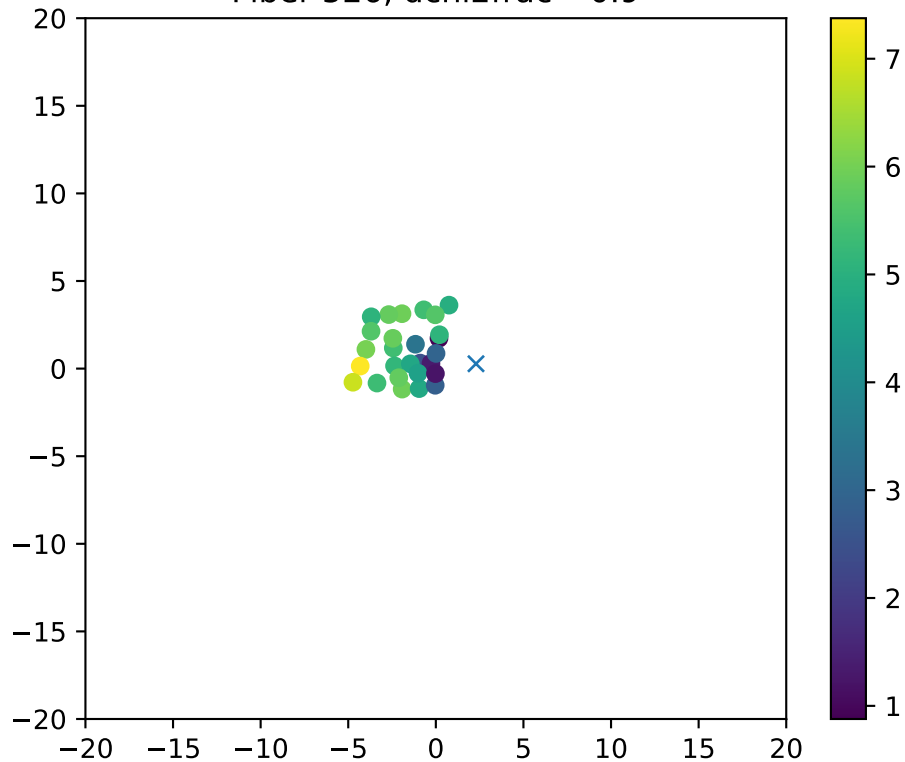
Fiber 526, dchi2frac= 0.9
