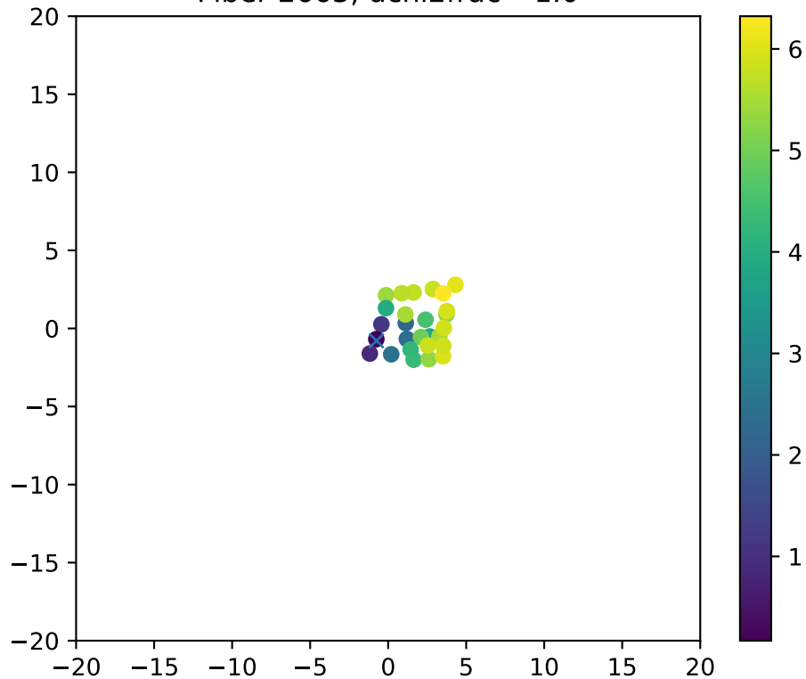
Fiber 2663, dchi2frac= 1.0
