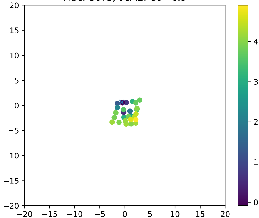
Fiber 3673, dchi2frac= 0.9
