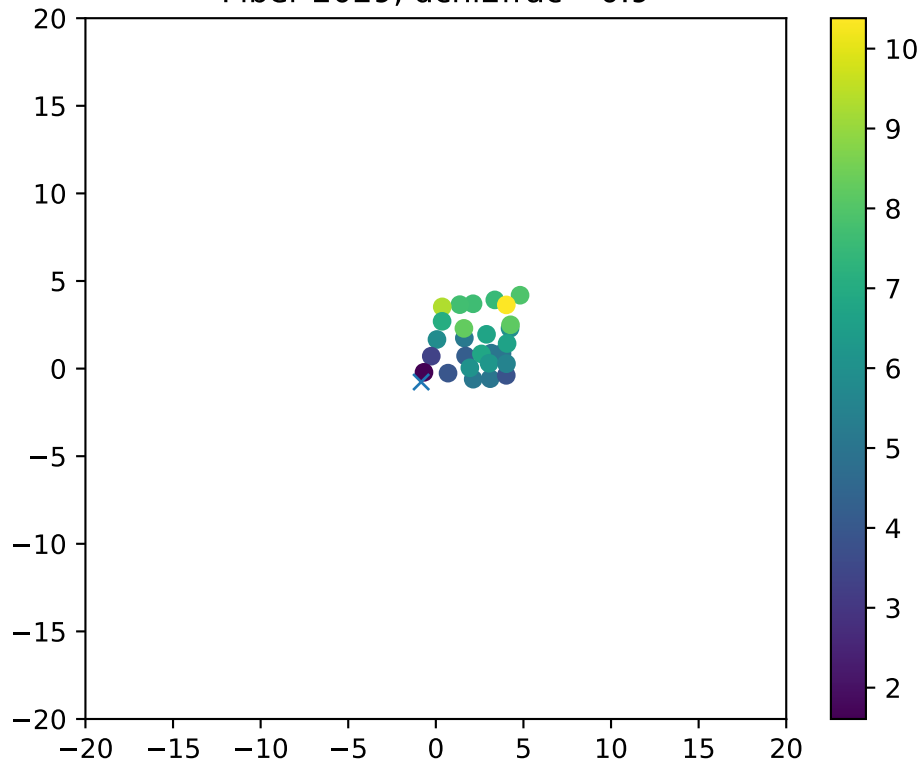
Fiber 2029, dchi2frac= 0.9
