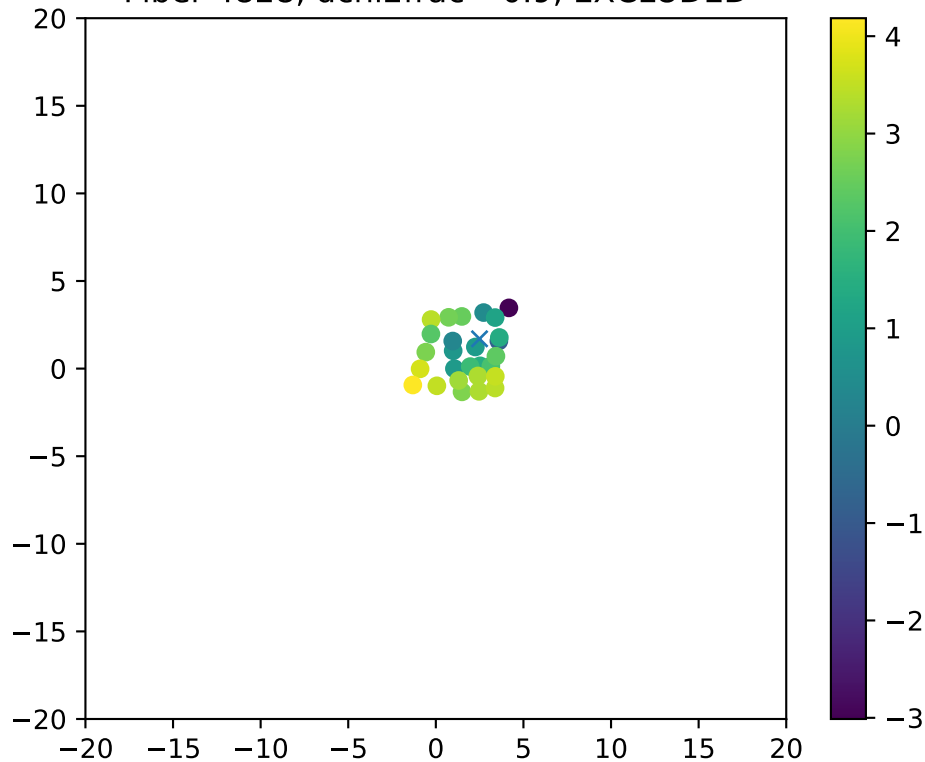
Fiber 4828, dchi2frac= 0.9, EXCLUDED
