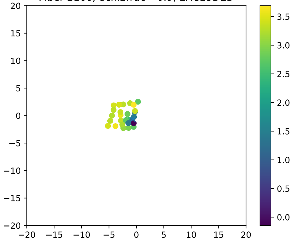
Fiber 2166, dchi2frac= 0.9, EXCLUDED
