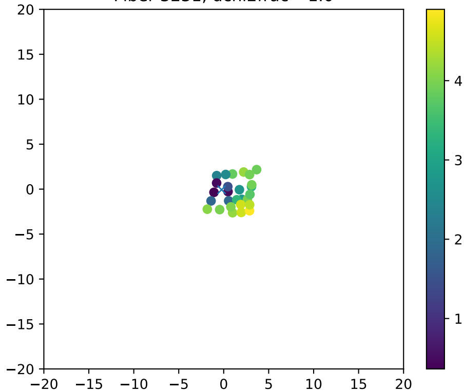
Fiber 3231, dchi2frac= 1.0
