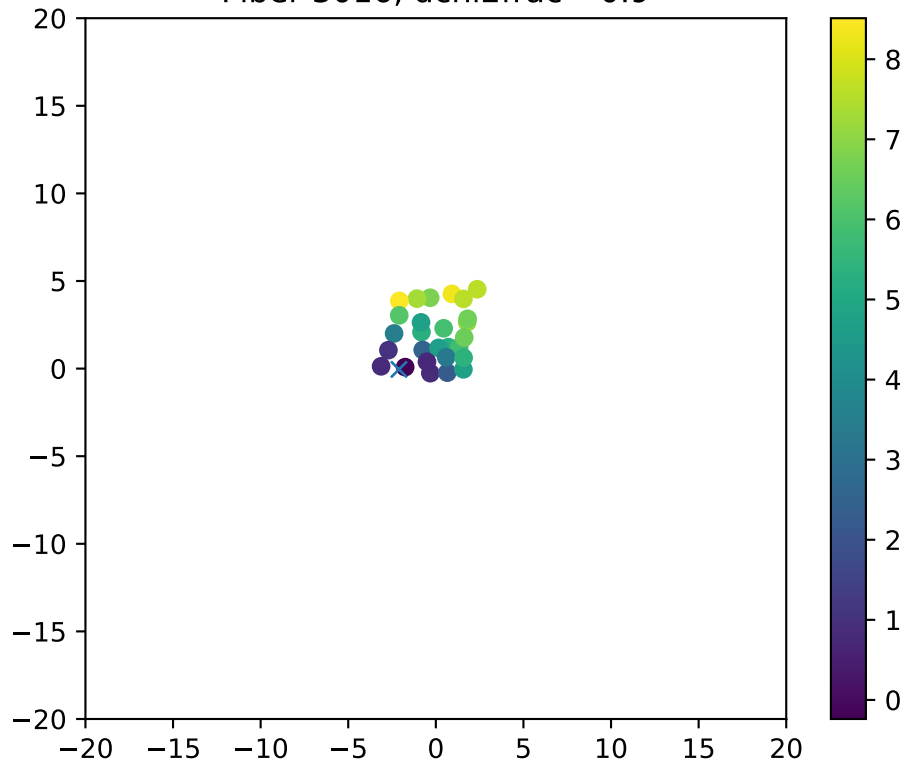
Fiber 3016, dchi2frac= 0.9
