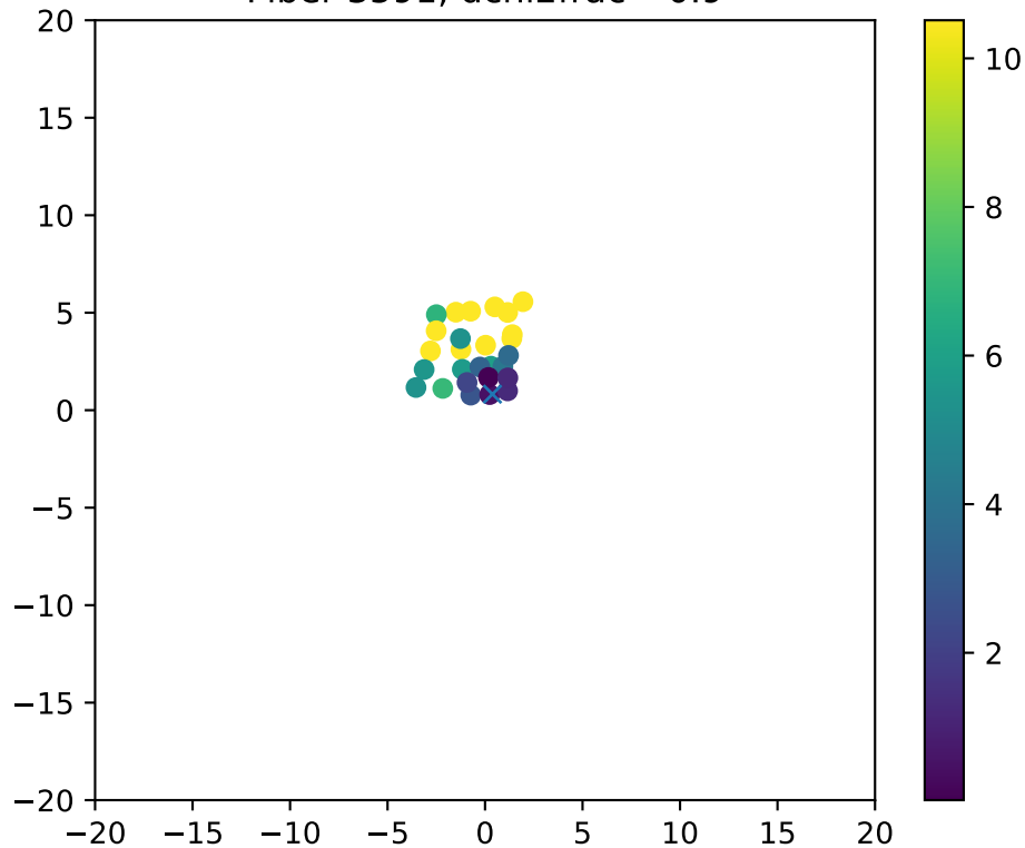
Fiber 3591, dchi2frac= 0.9
