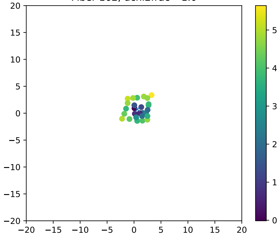
Fiber 162, dchi2frac= 1.0
