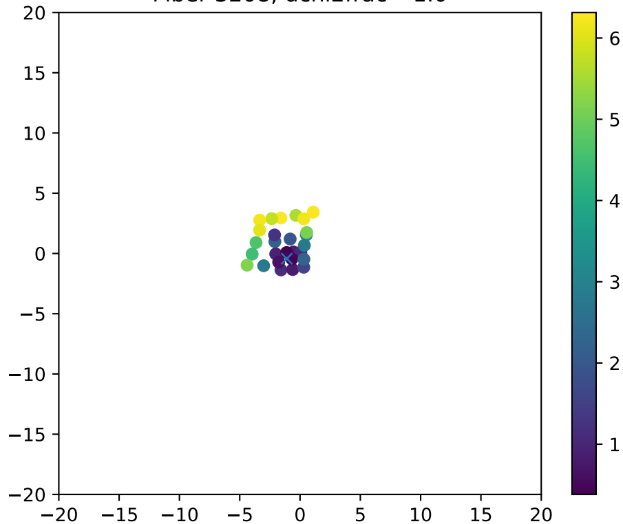
Fiber 3208, dchi2frac= 1.0
