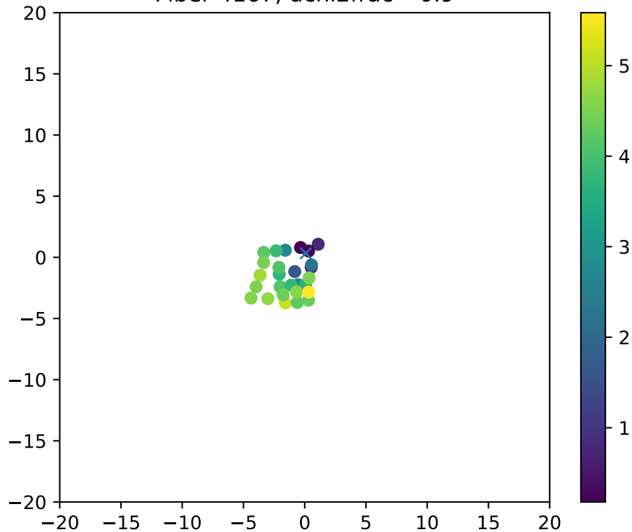
Fiber 4167, dchi2frac= 0.9
