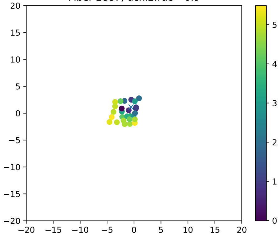
Fiber 2887, dchi2frac= 0.9
