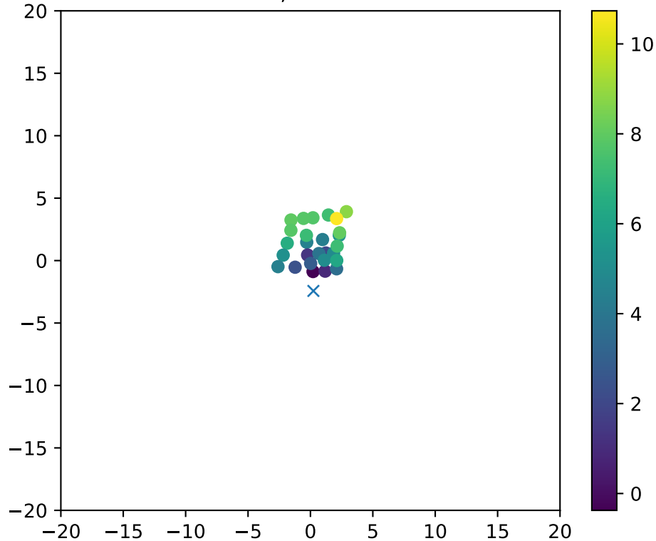
Fiber 1918, dchi2frac= 0.9
