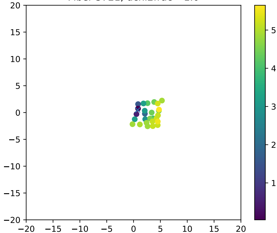
Fiber 3721, dchi2frac= 1.0
