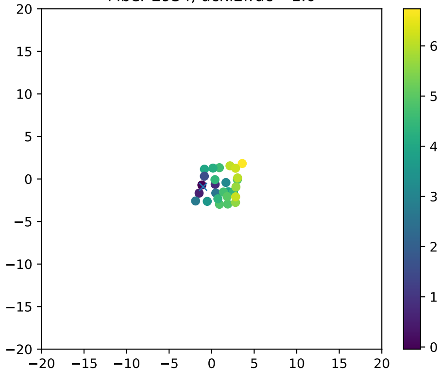
Fiber 2934, dchi2frac= 1.0
