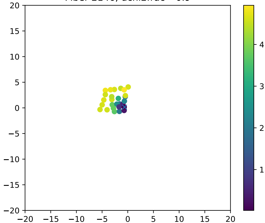
Fiber 2146, dchi2frac= 0.9
