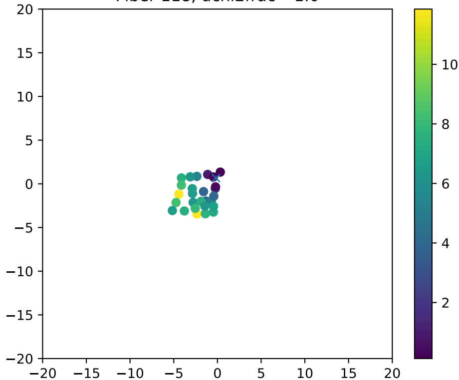
Fiber 118, dchi2frac= 1.0
