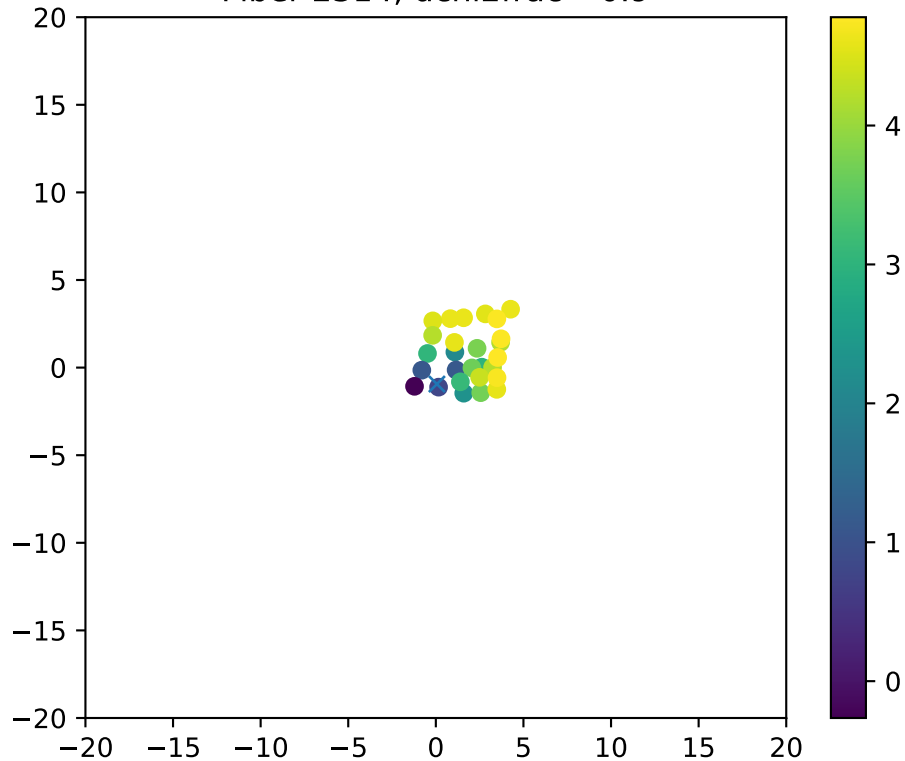
Fiber 2314, dchi2frac= 0.9
