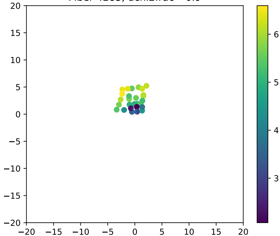
Fiber 4283, dchi2frac= 0.9
