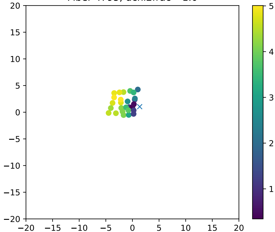
Fiber 4795, dchi2frac= 1.0
