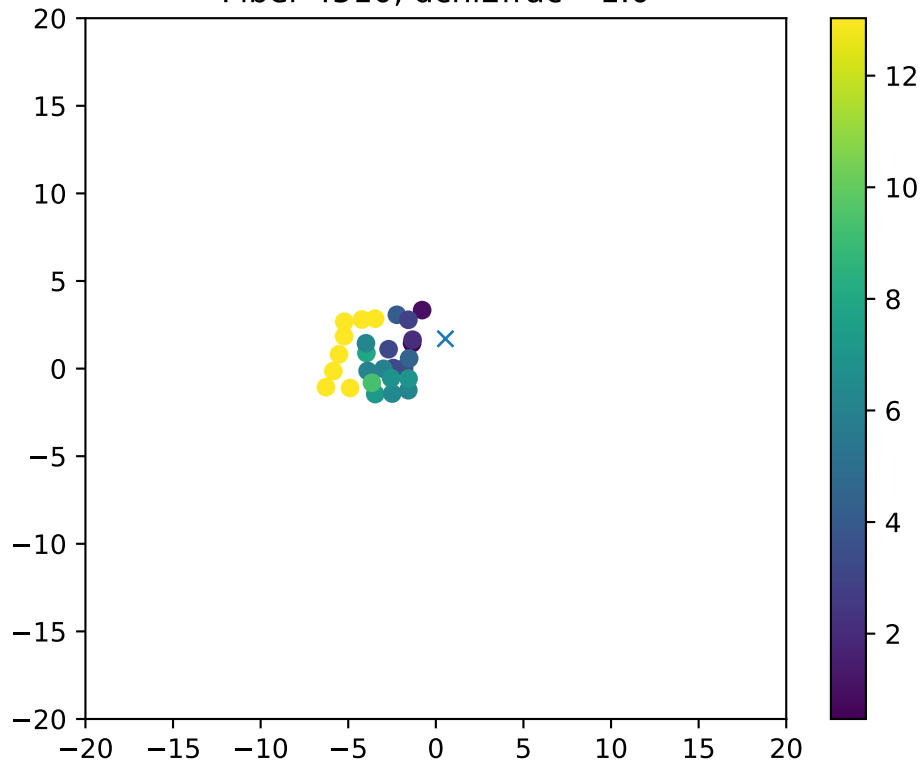
Fiber 4510, dchi2frac= 1.0
