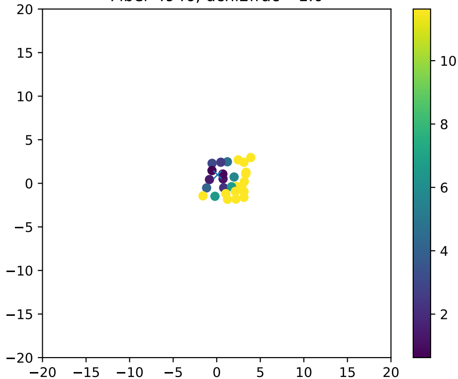
Fiber 4946, dchi2frac= 1.0
