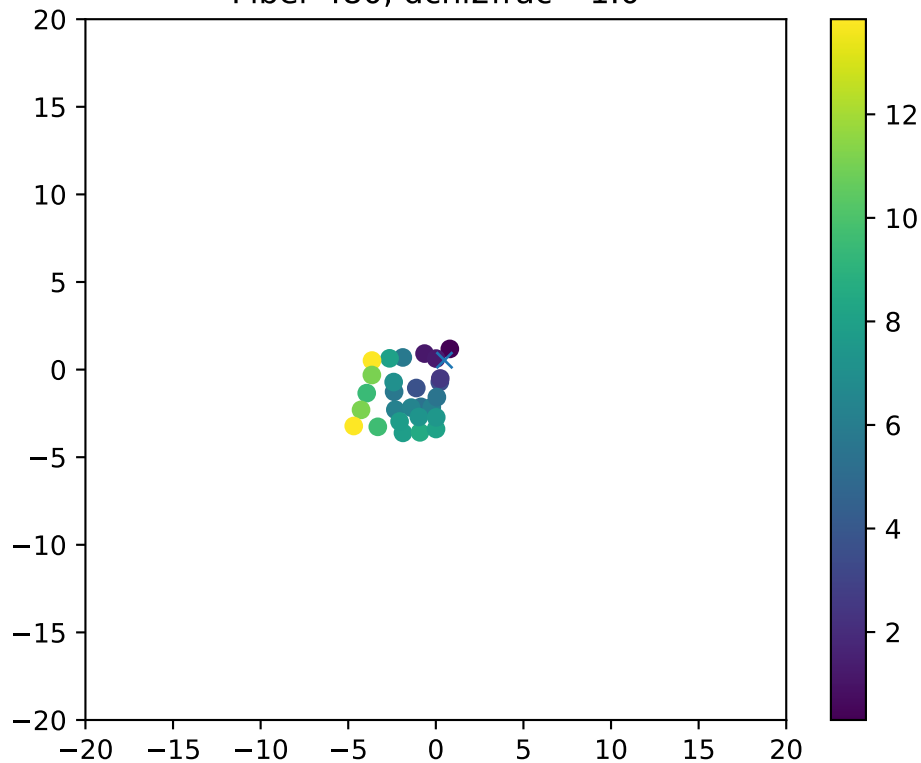
Fiber 480, dchi2frac= 1.0
