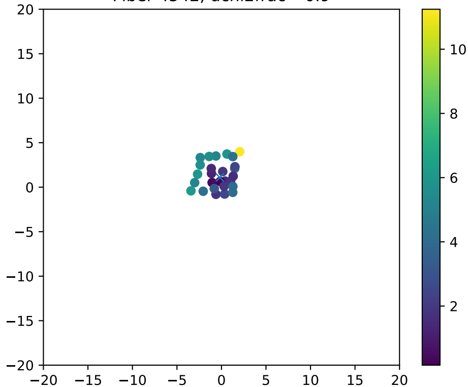
Fiber 4542, dchi2frac= 0.9
