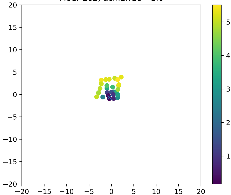
Fiber 262, dchi2frac= 1.0
