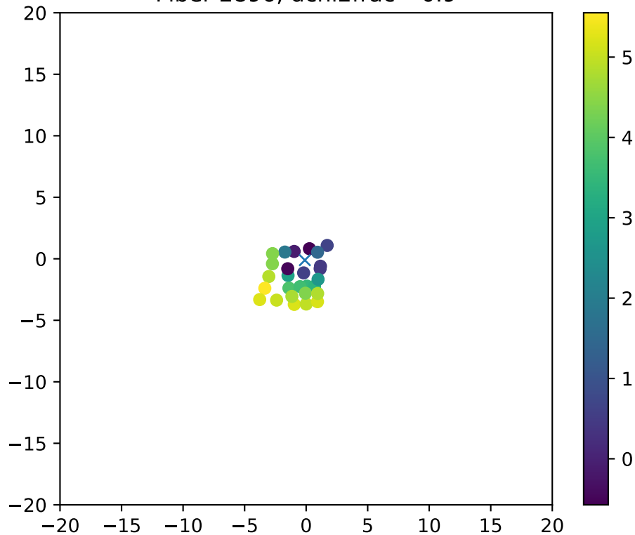
Fiber 2896, dchi2frac= 0.9
