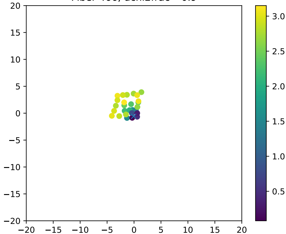
Fiber 466, dchi2frac= 0.9
