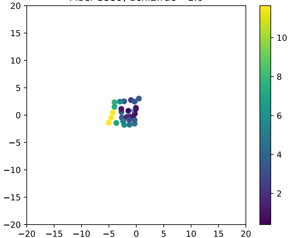
Fiber 3359, dchi2frac= 1.0
