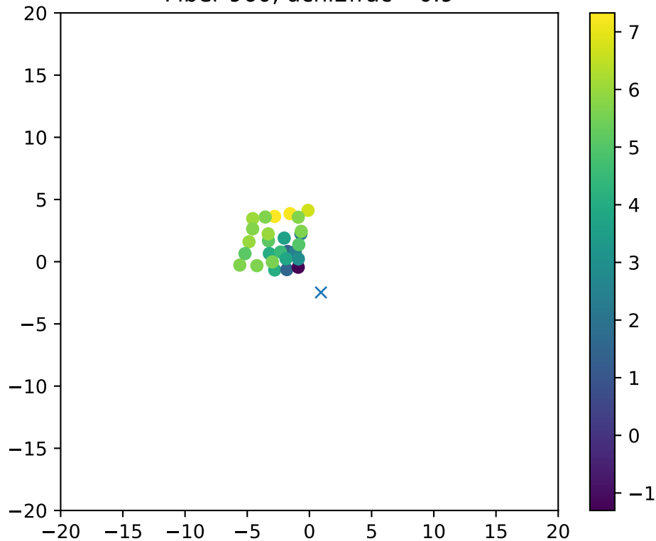
Fiber 960, dchi2frac= 0.9
