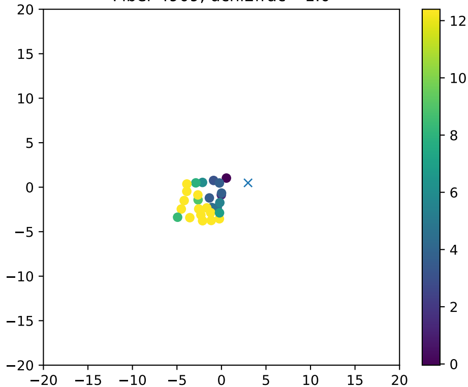
Fiber 4909, dchi2frac= 1.0
