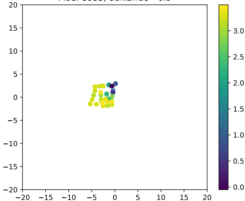
Fiber 3935, dchi2frac= 0.9
