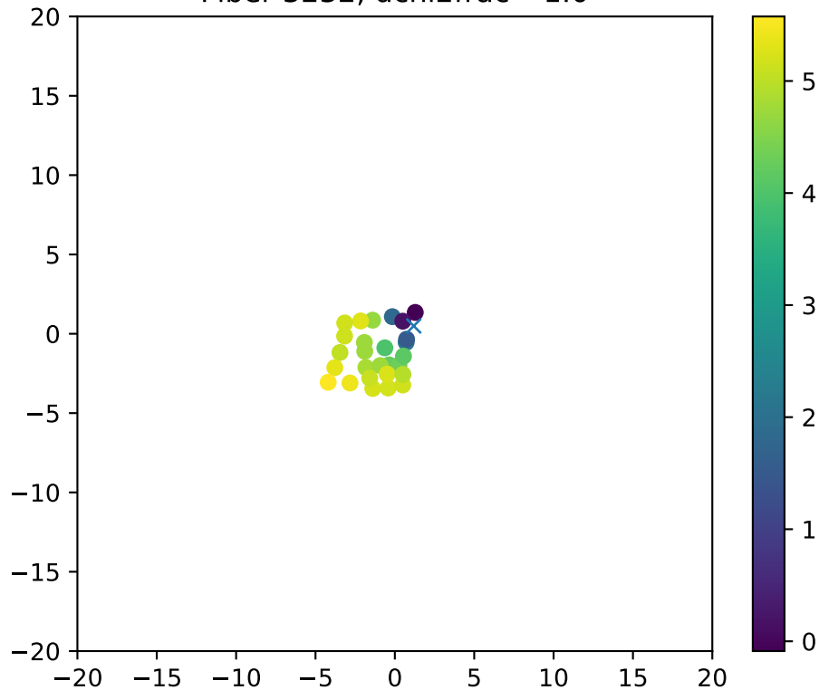
Fiber 3232, dchi2frac= 1.0
