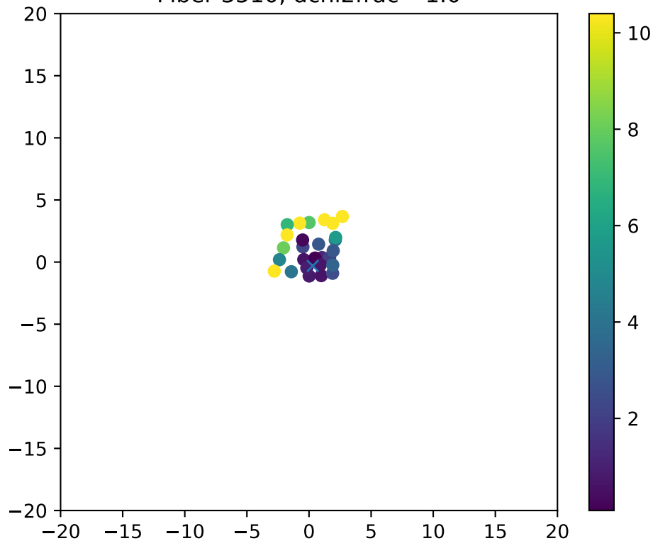
Fiber 3510, dchi2frac= 1.0
