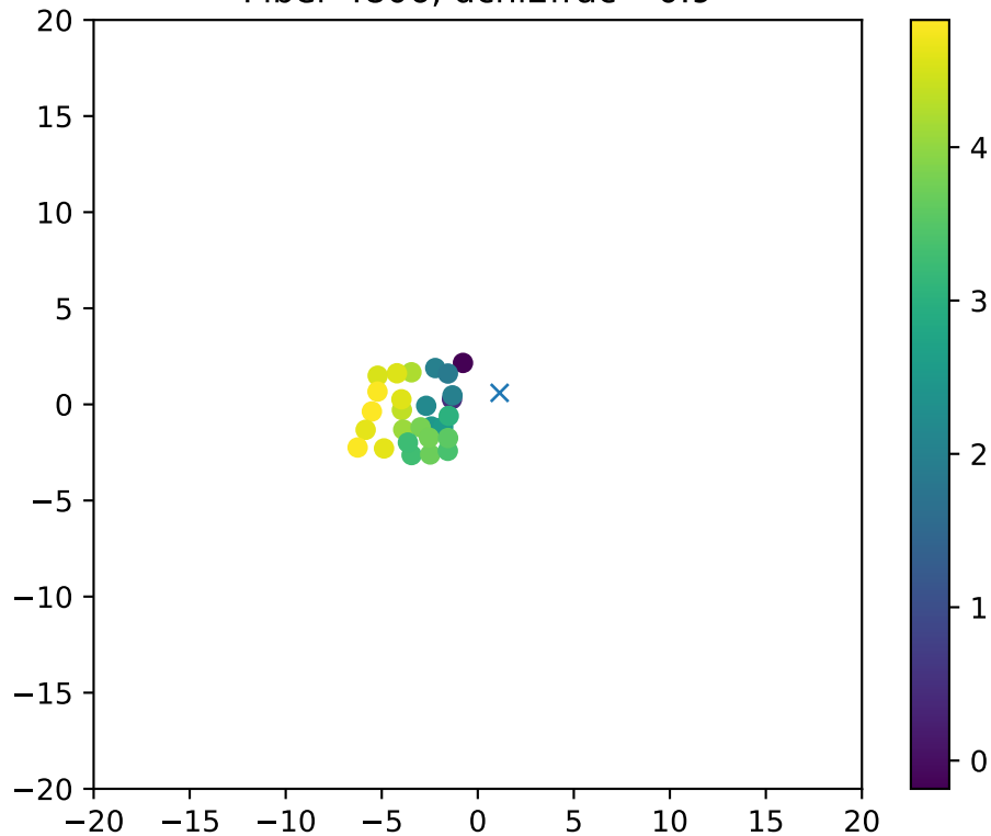
Fiber 4806, dchi2frac= 0.9
