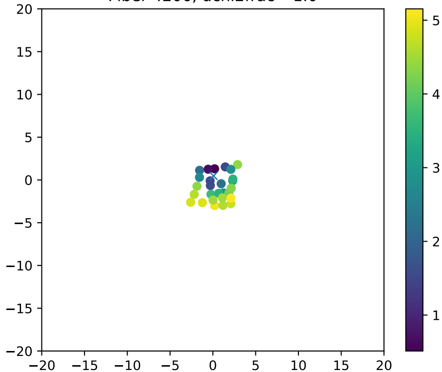
Fiber 4206, dchi2frac= 1.0
