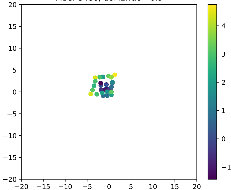
Fiber 3488, dchi2frac= 0.9
