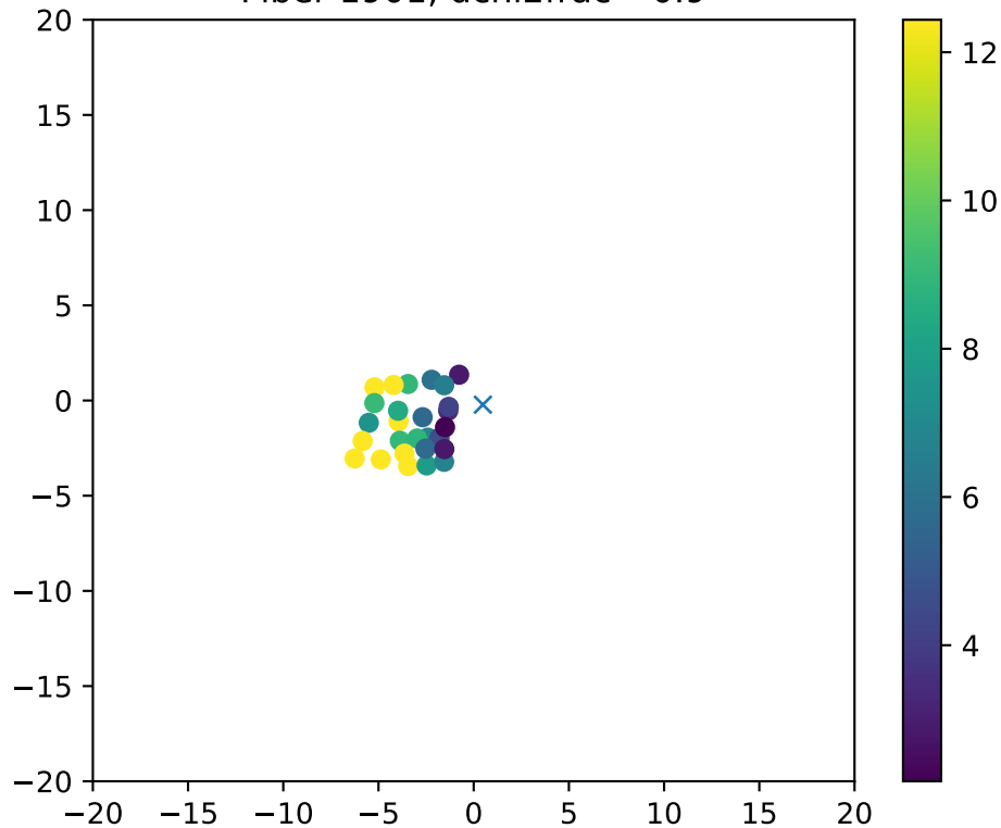
Fiber 1901, dchi2frac= 0.9
