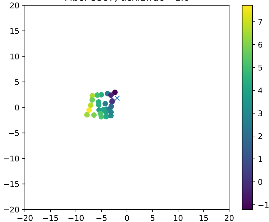
Fiber 3387, dchi2frac= 1.0
