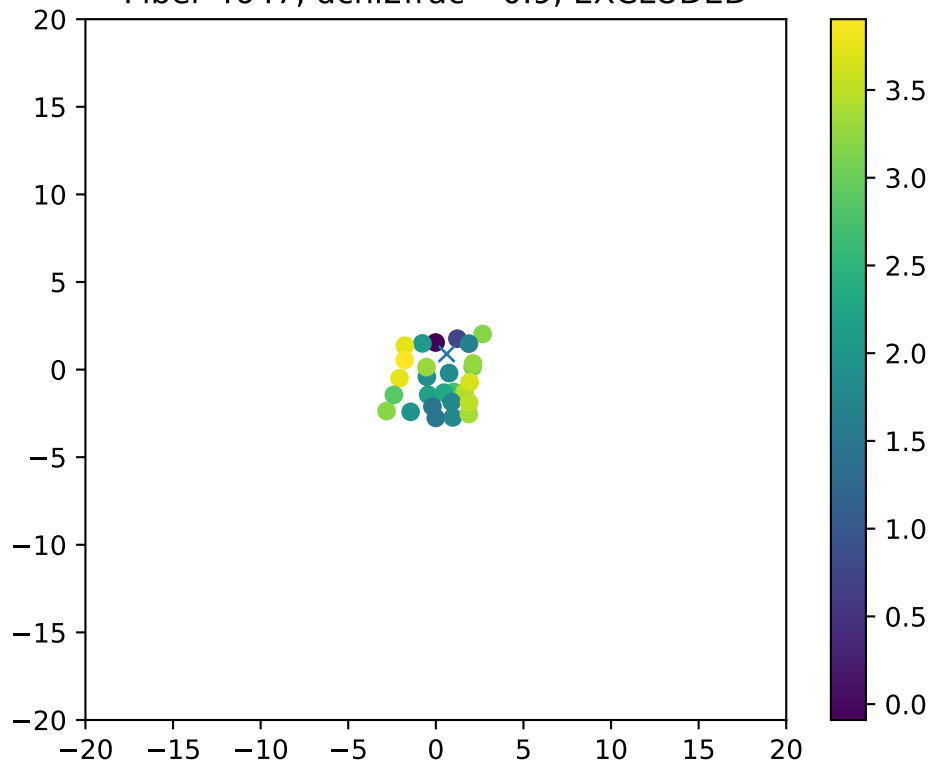
Fiber 4647, dchi2frac= 0.9, EXCLUDED
