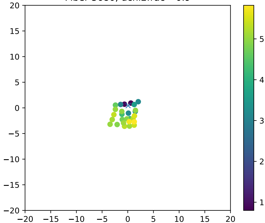
Fiber 3680, dchi2frac= 0.9
