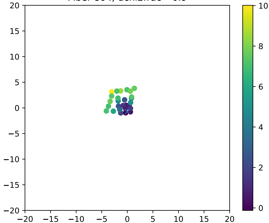
Fiber 804, dchi2frac= 0.9
