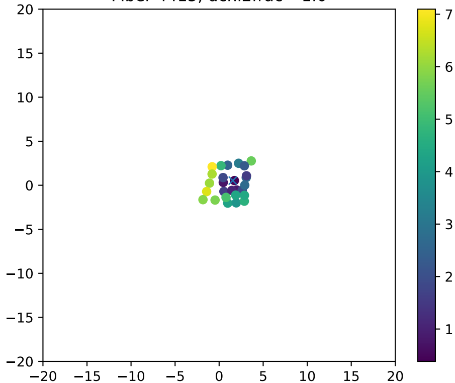
Fiber 4415, dchi2frac= 1.0
