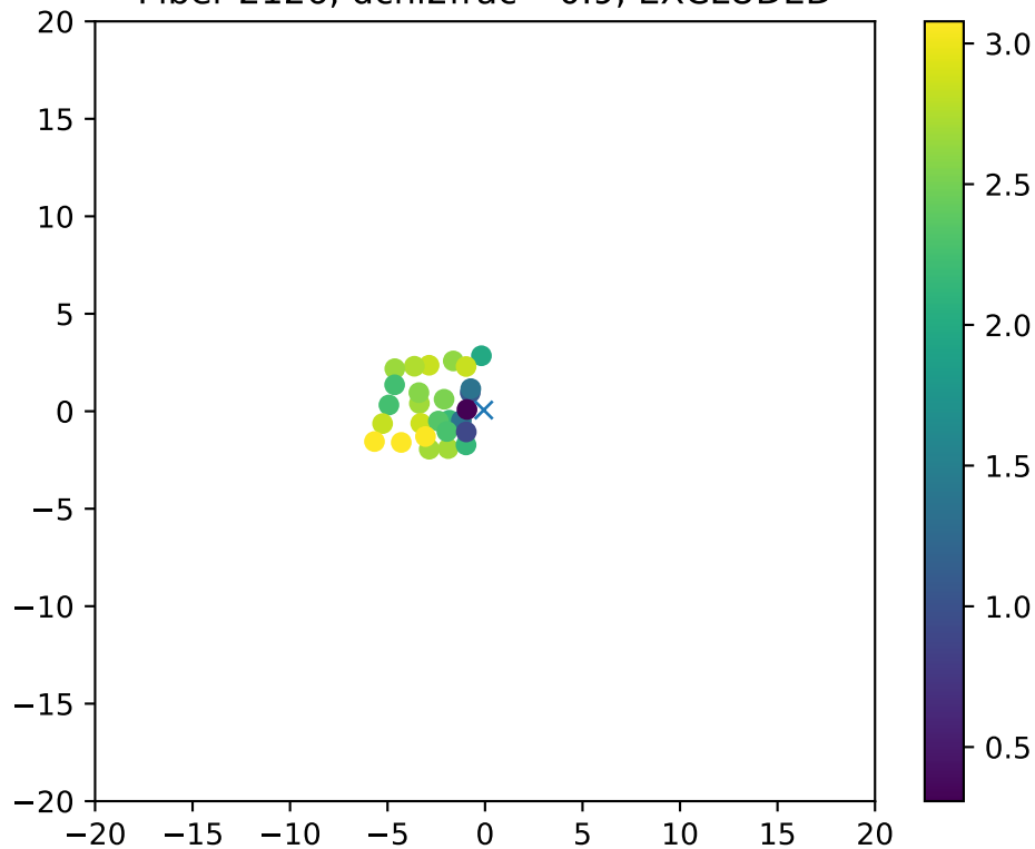
Fiber 2126, dchi2frac= 0.9, EXCLUDED
