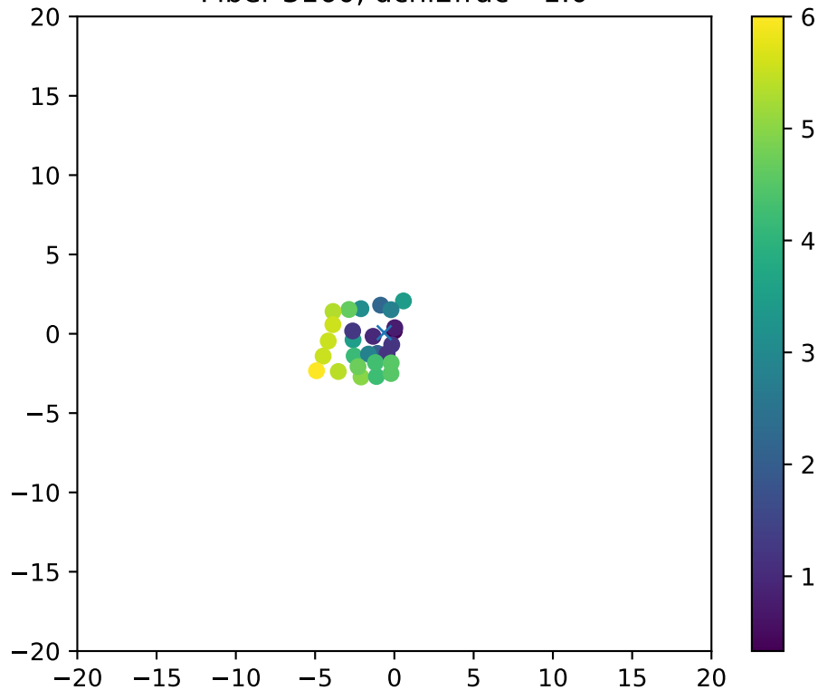
Fiber 3160, dchi2frac= 1.0
