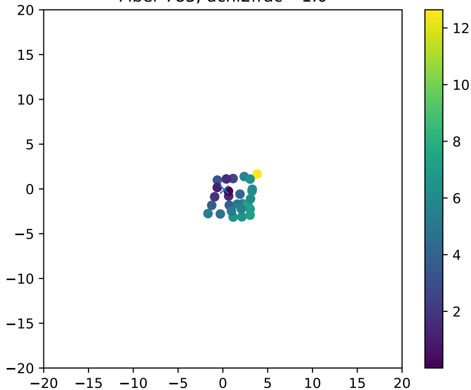
Fiber 783, dchi2frac= 1.0
