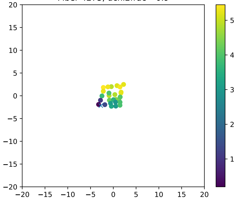
Fiber 4273, dchi2frac= 0.9
