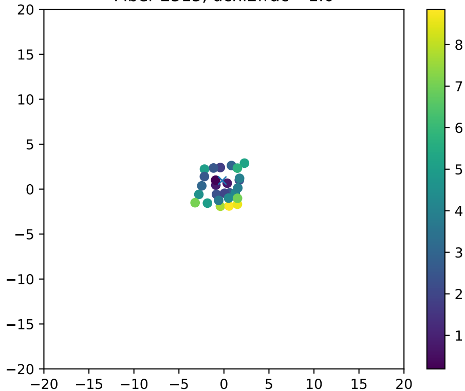
Fiber 2515, dchi2frac= 1.0
