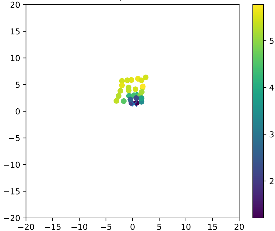
Fiber 4678, dchi2frac= 0.9
