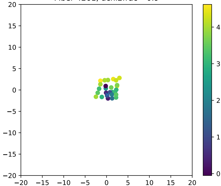
Fiber 4261, dchi2frac= 0.9
