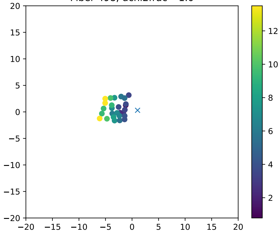
Fiber 498, dchi2frac= 1.0
