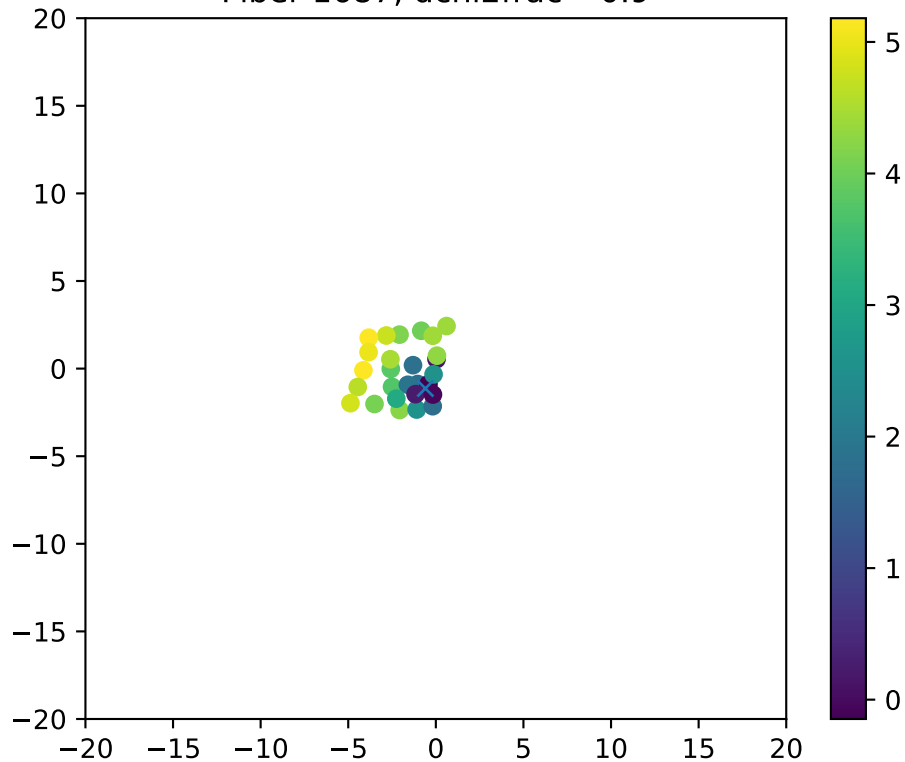
Fiber 1687, dchi2frac= 0.9
