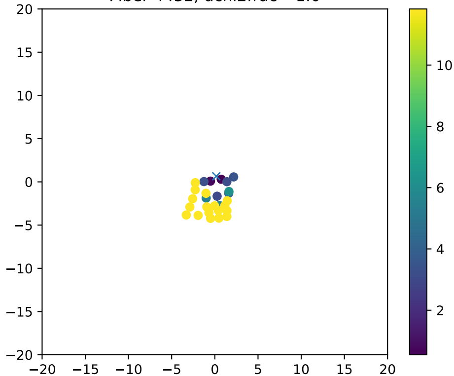
Fiber 4432, dchi2frac= 1.0
