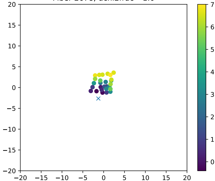
Fiber 2678, dchi2frac= 1.0
