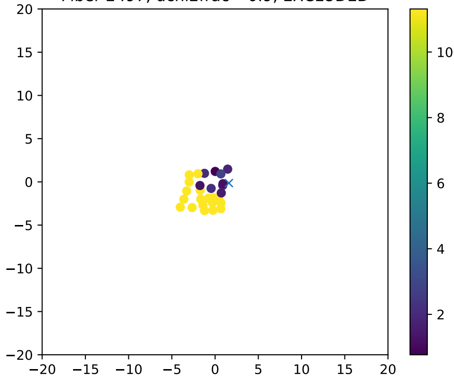
Fiber 2497, dchi2frac= 0.9, EXCLUDED
