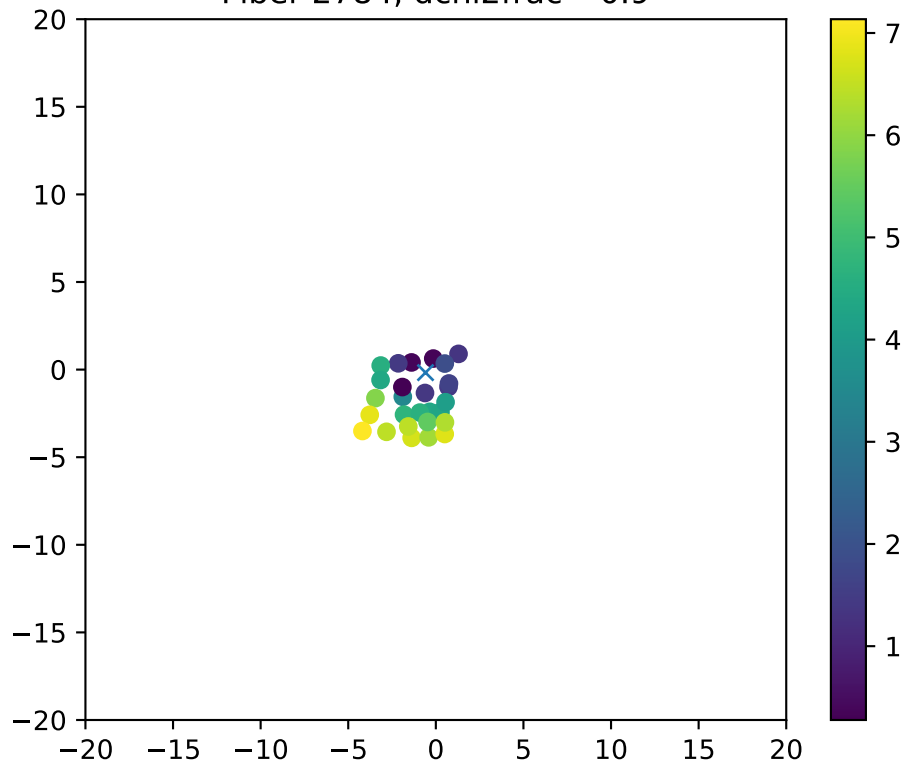
Fiber 2784, dchi2frac= 0.9
