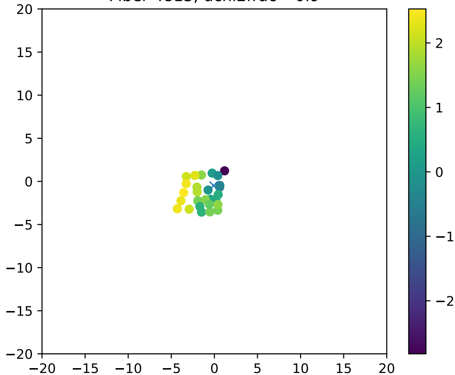
Fiber 4813, dchi2frac= 0.9
