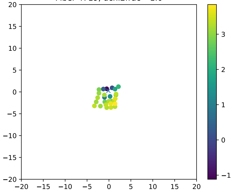
Fiber 4719, dchi2frac= 1.0
