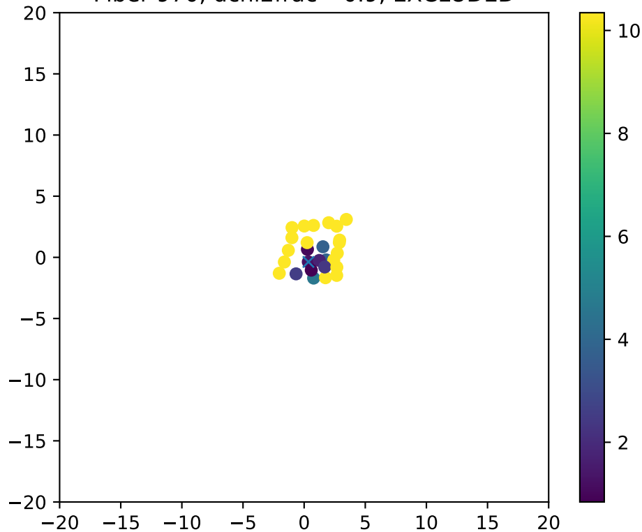
Fiber 970, dchi2frac= 0.9, EXCLUDED
