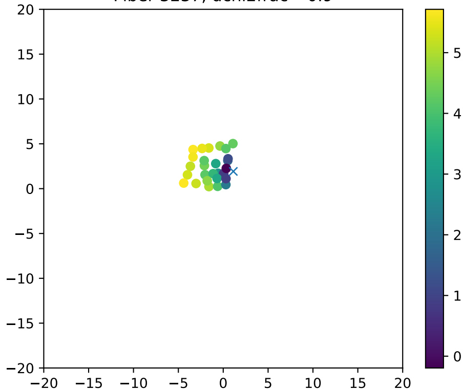
Fiber 3237, dchi2frac= 0.9
