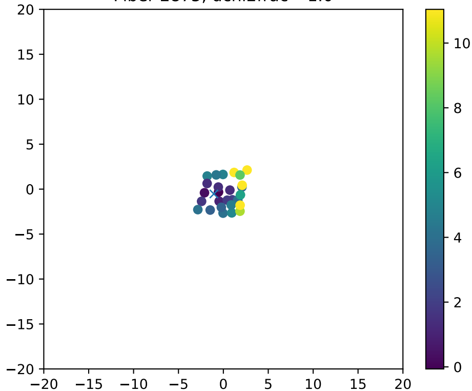
Fiber 2875, dchi2frac= 1.0
