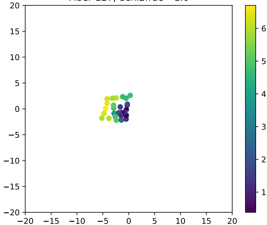
Fiber 127, dchi2frac= 1.0
