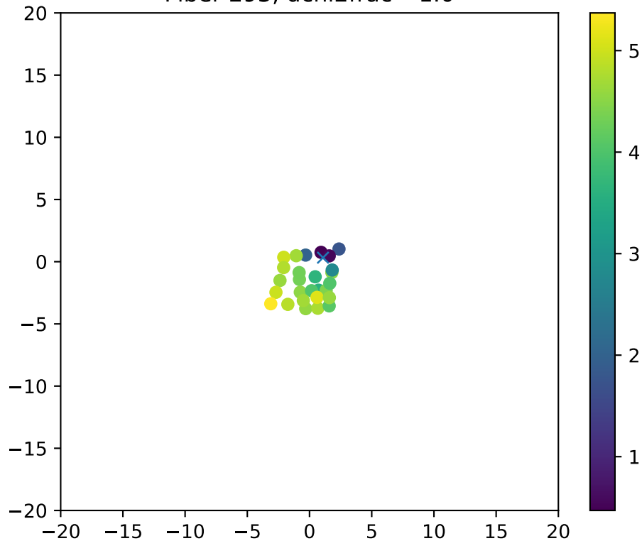
Fiber 293, dchi2frac= 1.0
