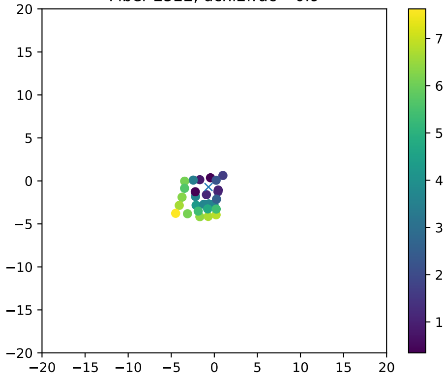
Fiber 2522, dchi2frac= 0.9
