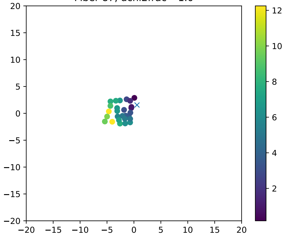
Fiber 87, dchi2frac= 1.0
