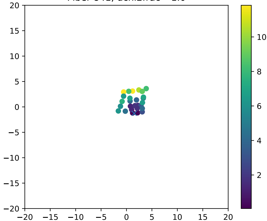
Fiber 841, dchi2frac= 1.0
