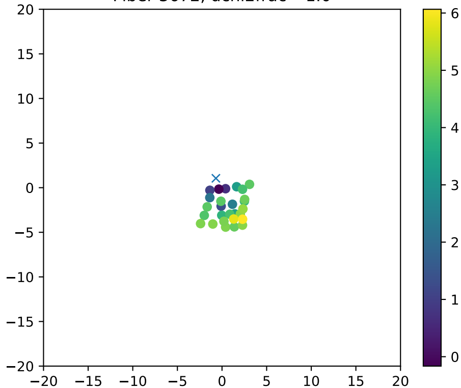
Fiber 3672, dchi2frac= 1.0
