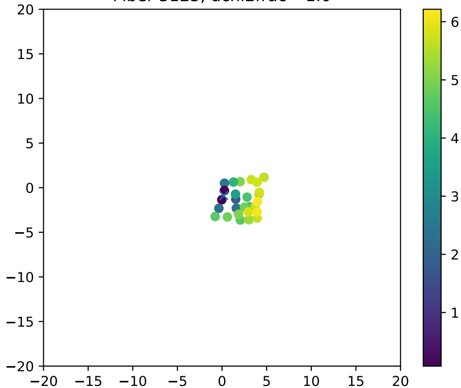
Fiber 3123, dchi2frac= 1.0
