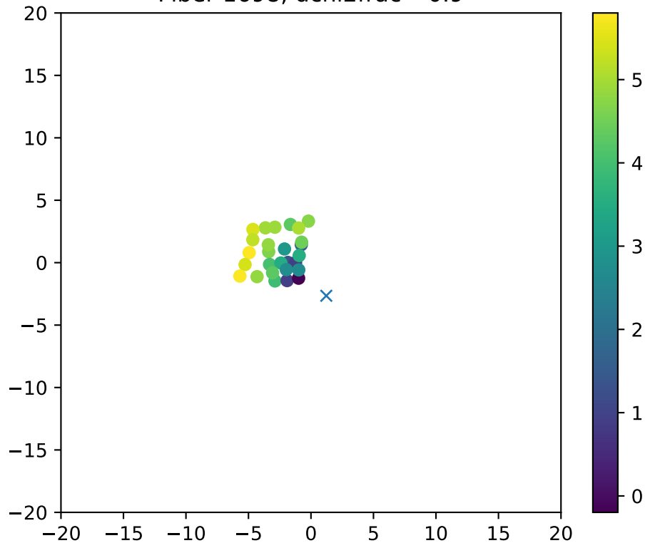
Fiber 1698, dchi2frac= 0.9
