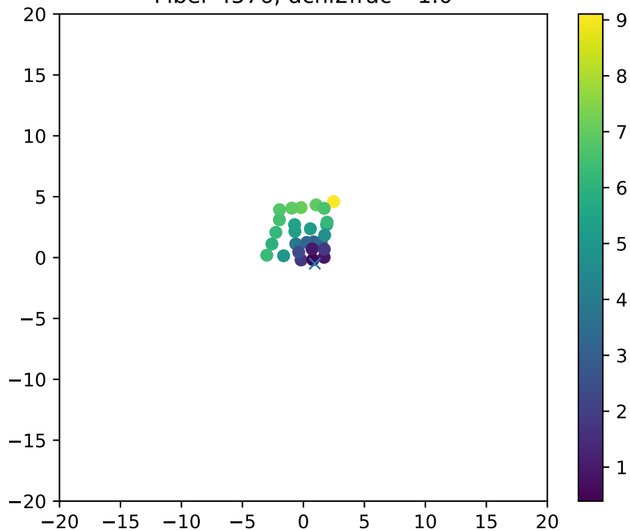
Fiber 4576, dchi2frac= 1.0
