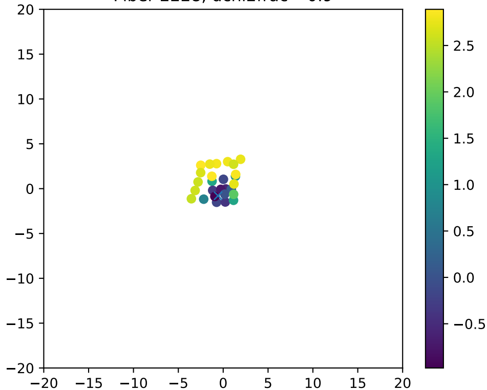
Fiber 2228, dchi2frac= 0.9
