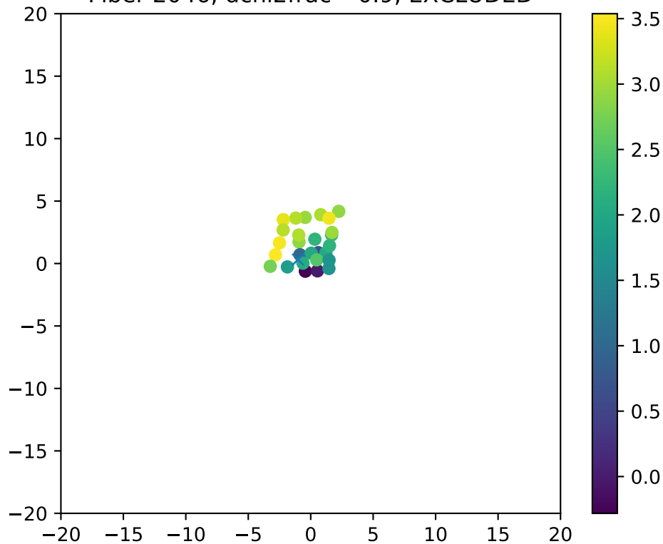
Fiber 2046, dchi2frac= 0.9, EXCLUDED
