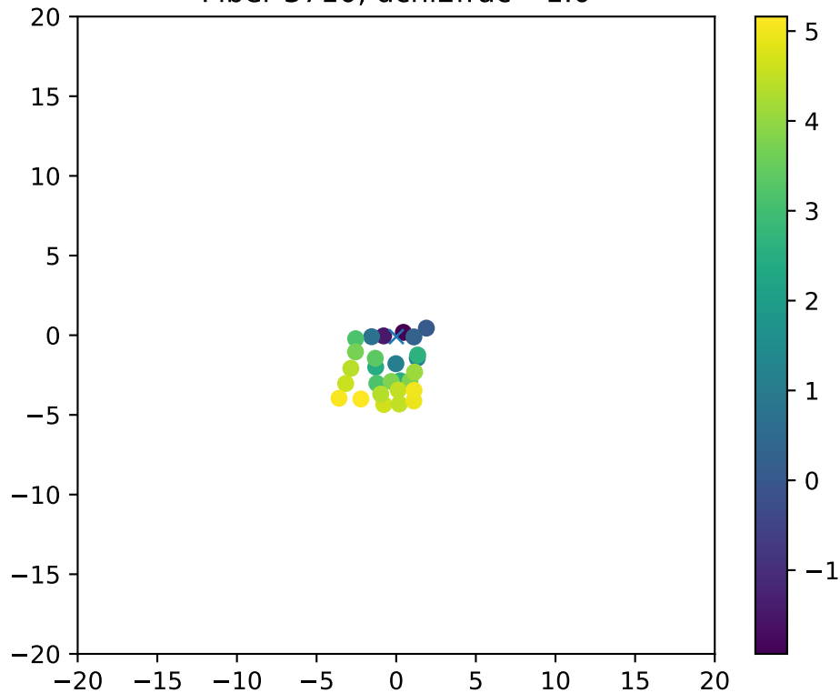
Fiber 3710, dchi2frac= 1.0
