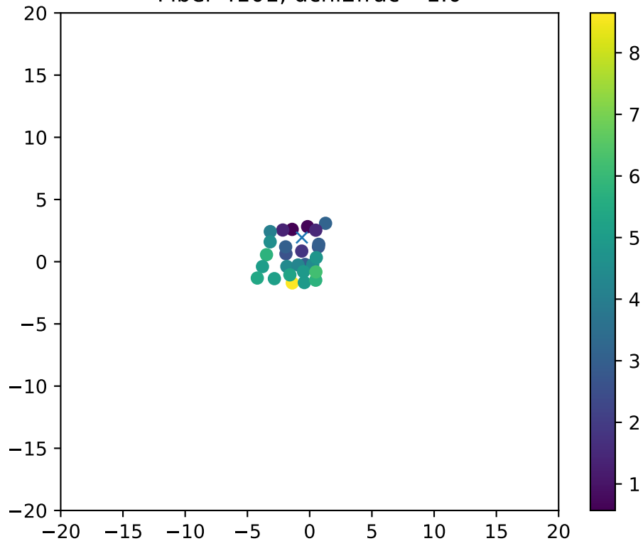
Fiber 4101, dchi2frac= 1.0
