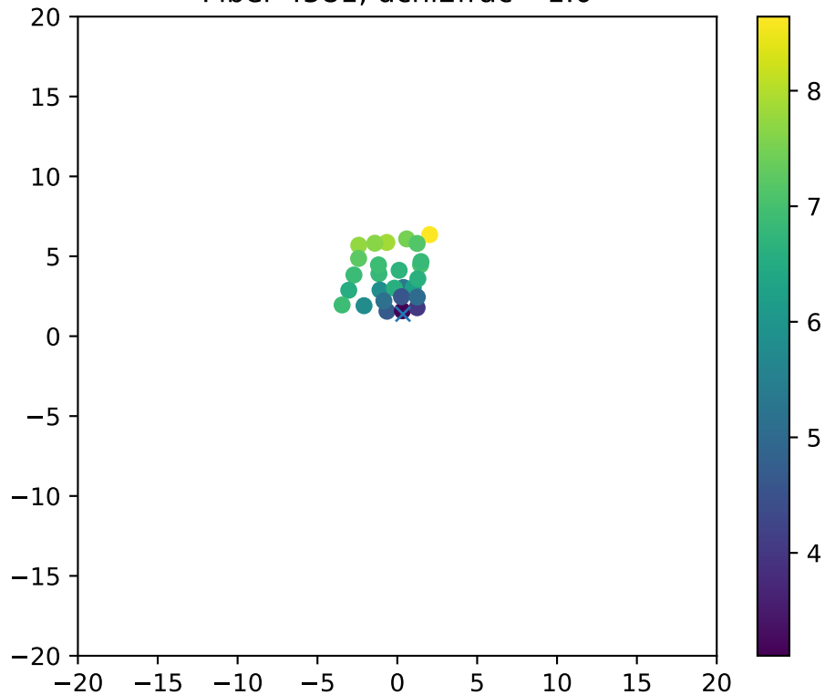
Fiber 4581, dchi2frac= 1.0
