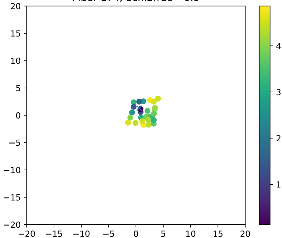
Fiber 174, dchi2frac= 0.9
