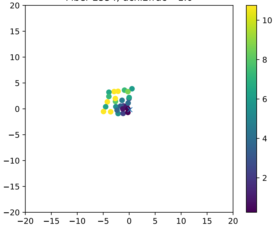
Fiber 2554, dchi2frac= 1.0
