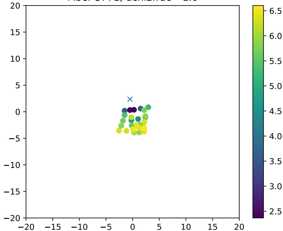
Fiber 3771, dchi2frac= 1.0
