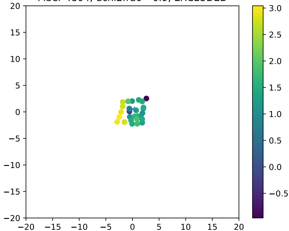
Fiber 4804, dchi2frac= 0.9, EXCLUDED
