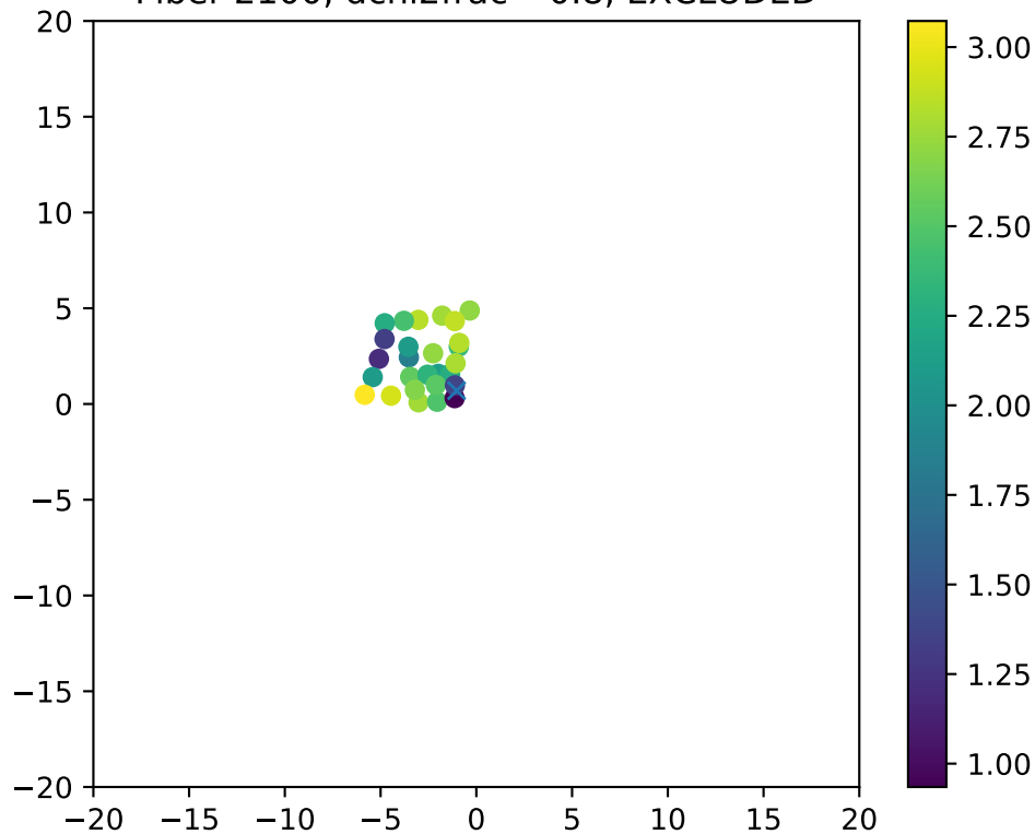
Fiber 2100, dchi2frac= 0.8, EXCLUDED
