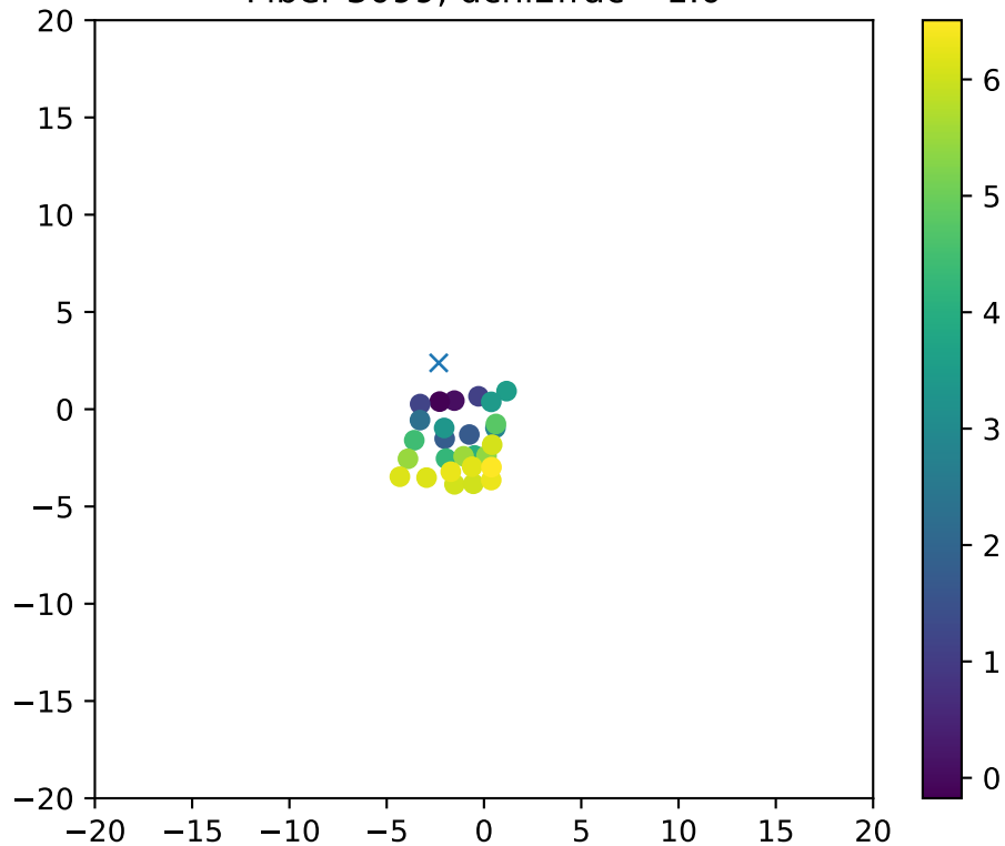
Fiber 3099, dchi2frac= 1.0
