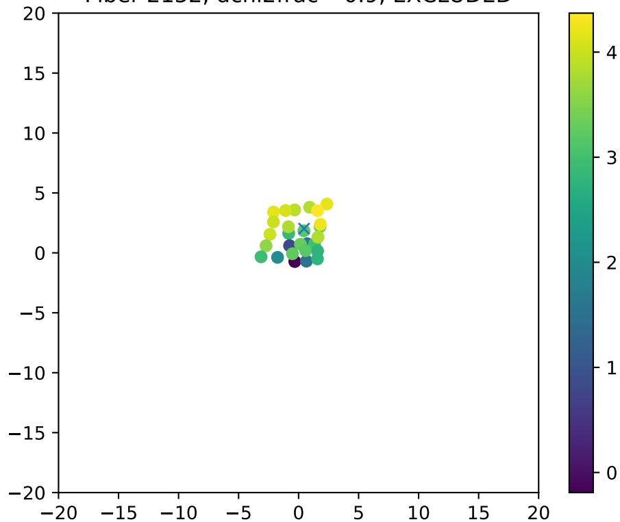
Fiber 2152, dchi2frac= 0.9, EXCLUDED
