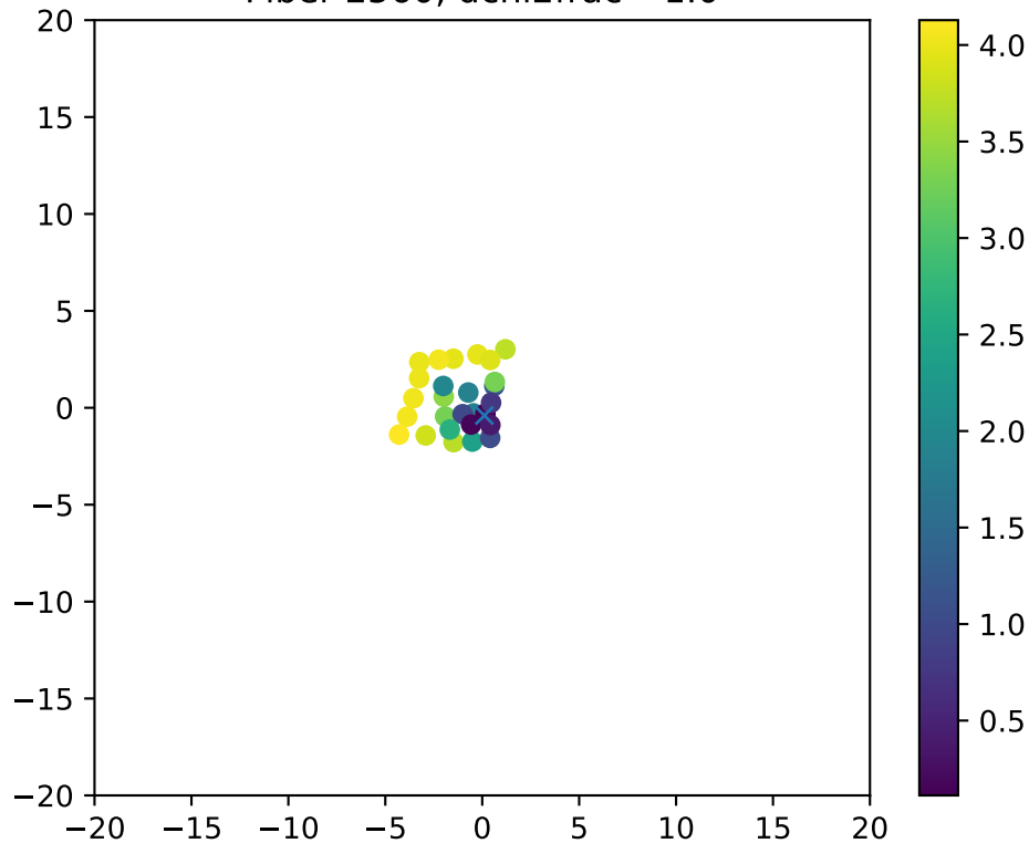
Fiber 2560, dchi2frac= 1.0
