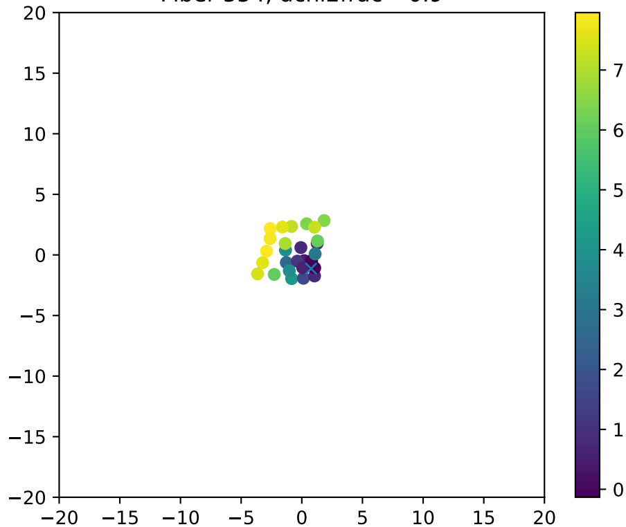
Fiber 554, dchi2frac= 0.9
