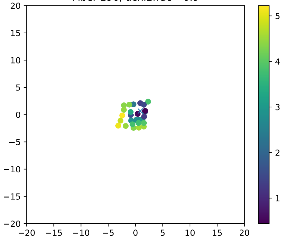
Fiber 196, dchi2frac= 0.9
