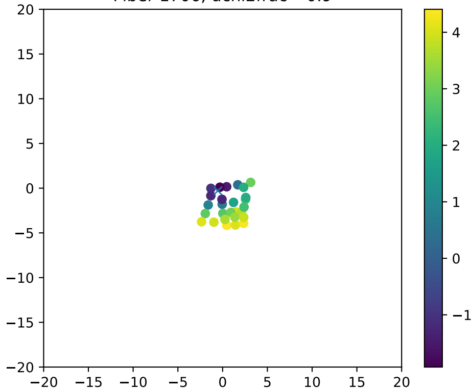
Fiber 1706, dchi2frac= 0.9
