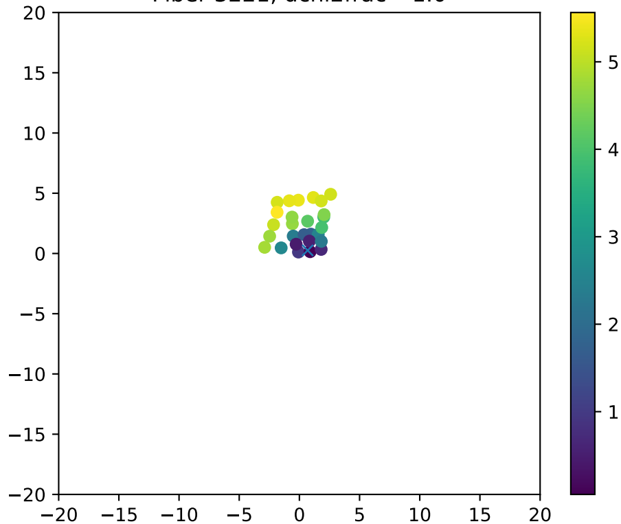
Fiber 3221, dchi2frac= 1.0
