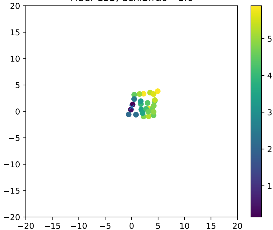
Fiber 153, dchi2frac= 1.0
