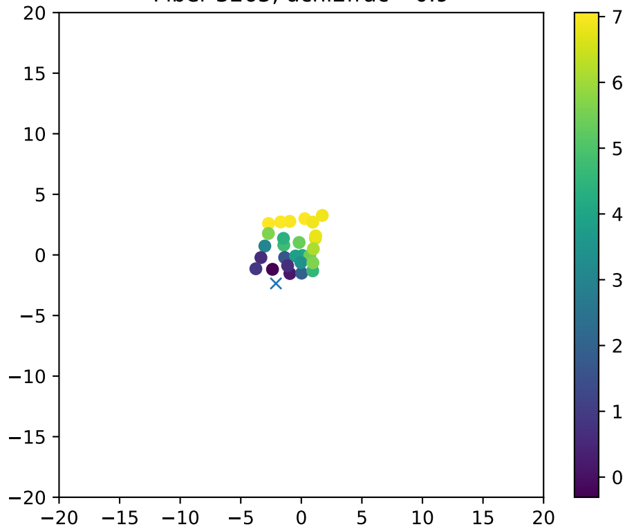
Fiber 3265, dchi2frac= 0.9
