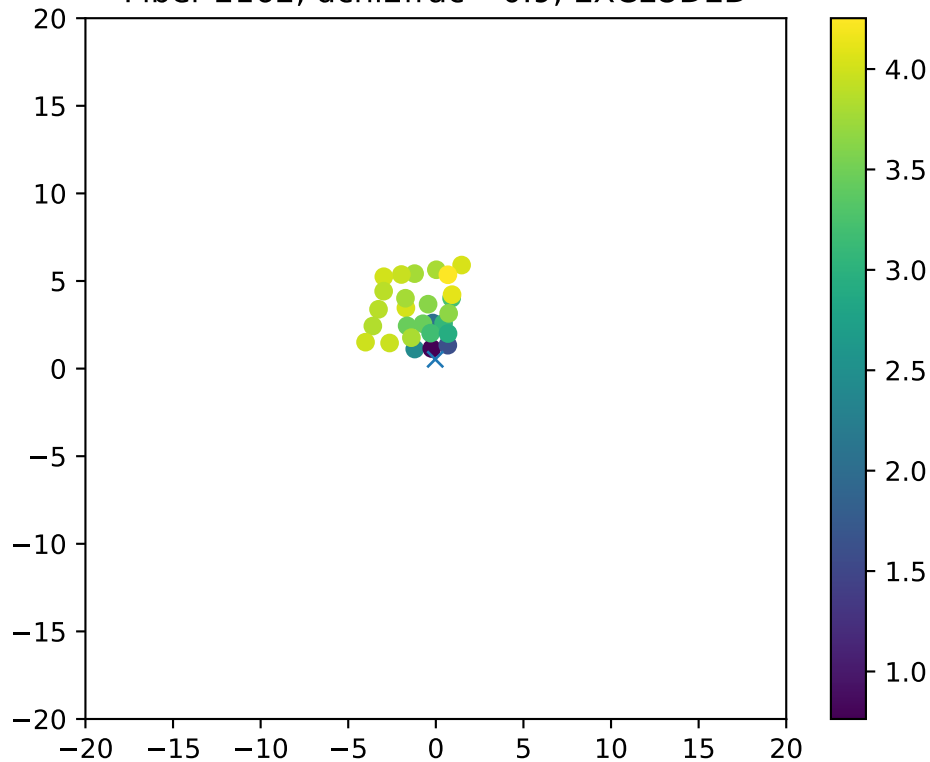
Fiber 2162, dchi2frac= 0.9, EXCLUDED
