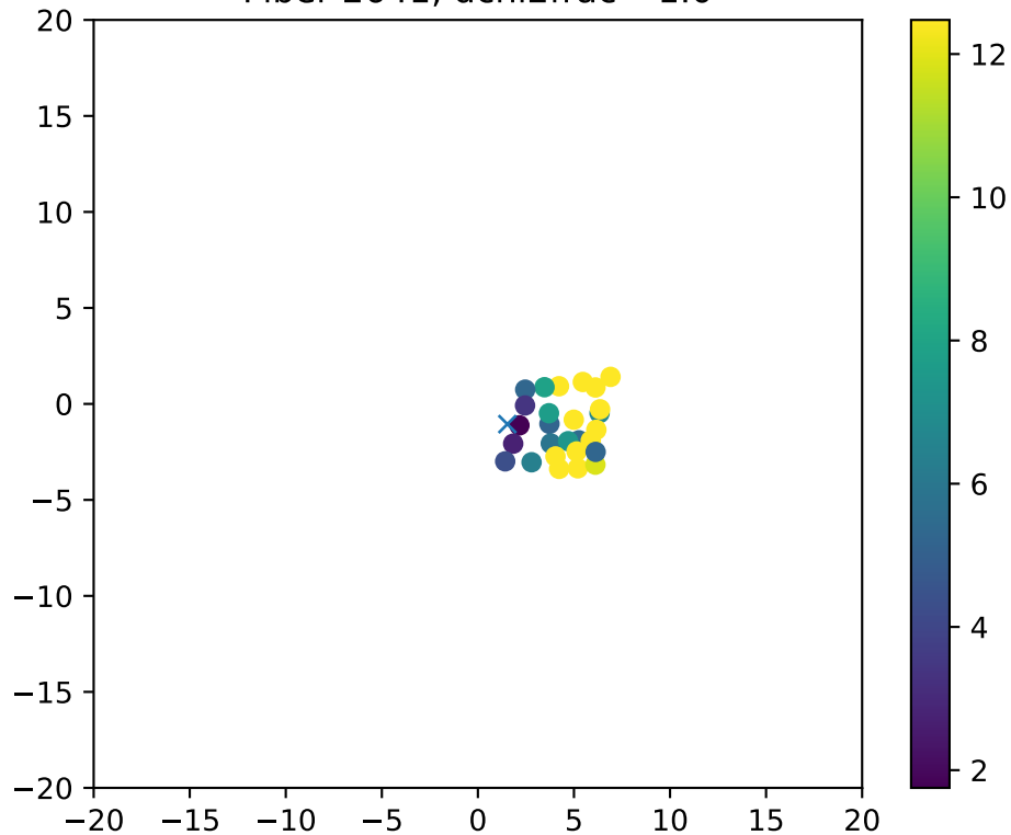
Fiber 2641, dchi2frac= 1.0
