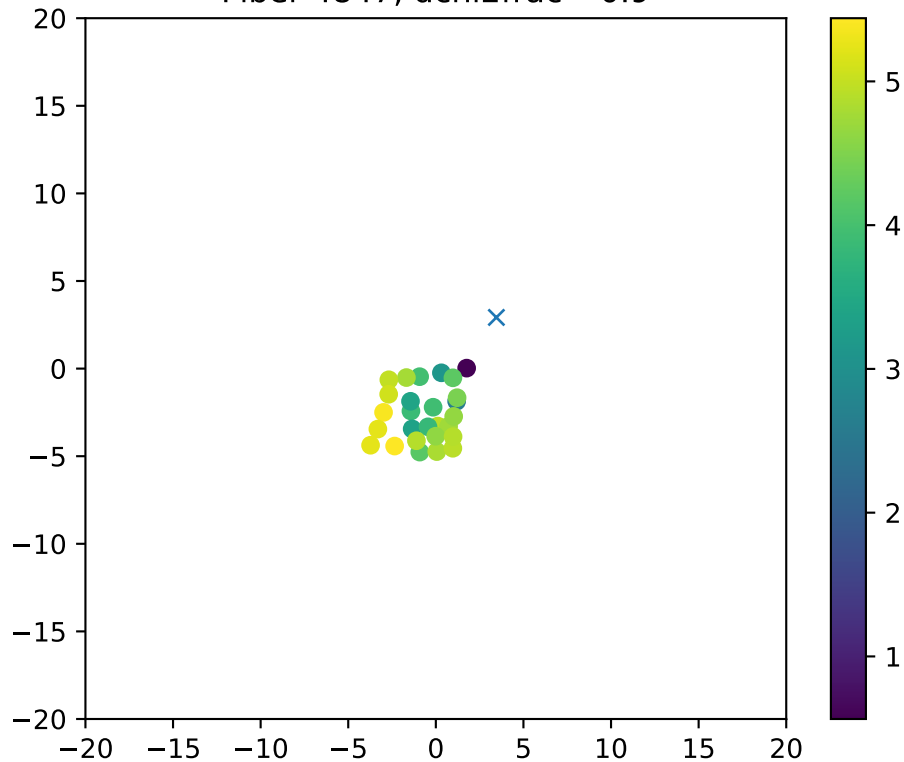
Fiber 4847, dchi2frac= 0.9
