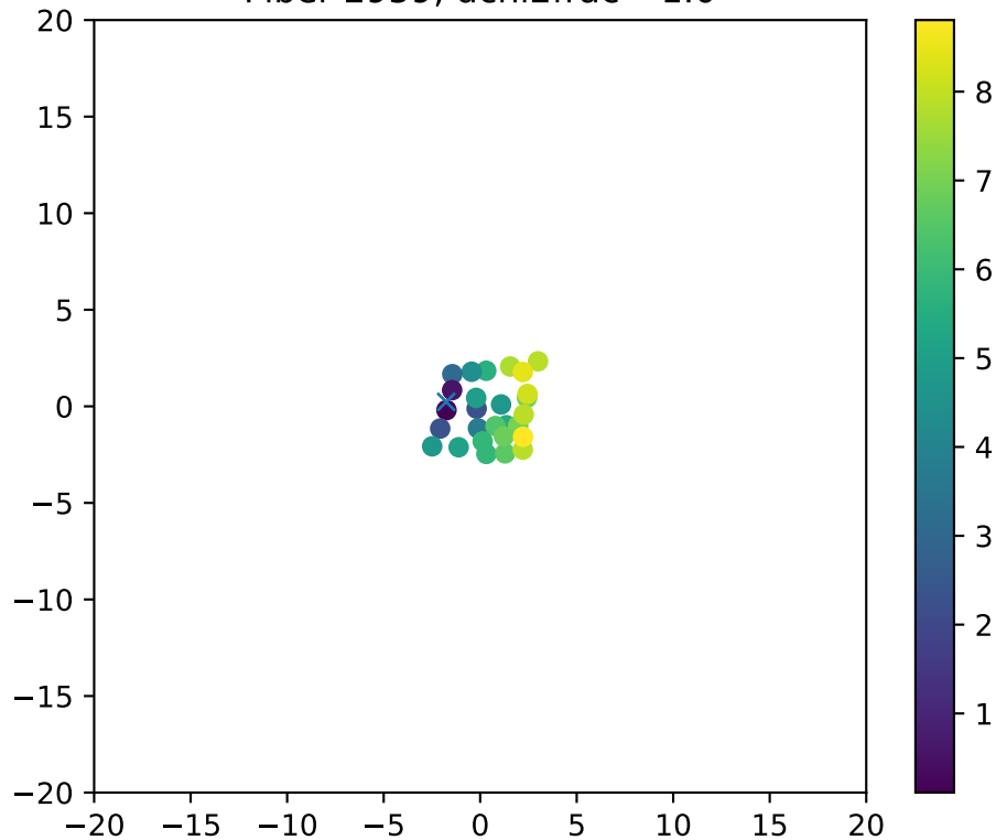
Fiber 2959, dchi2frac= 1.0
