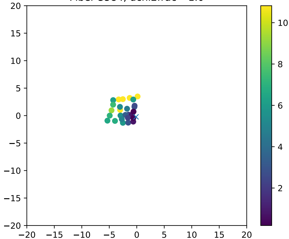
Fiber 3584, dchi2frac= 1.0
