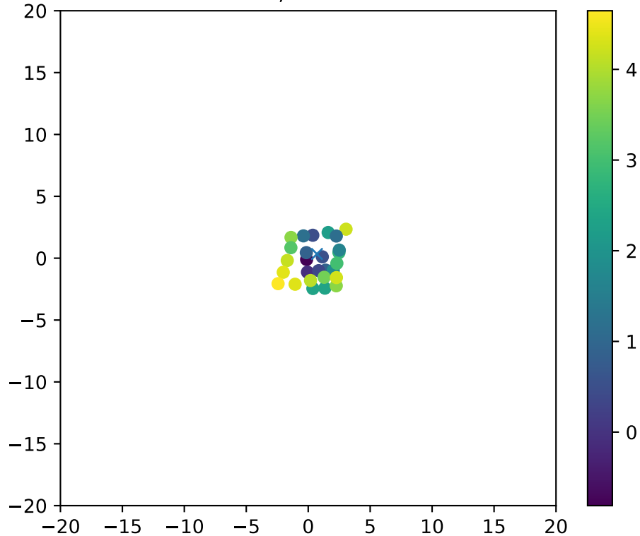
Fiber 4250, dchi2frac= 0.9
