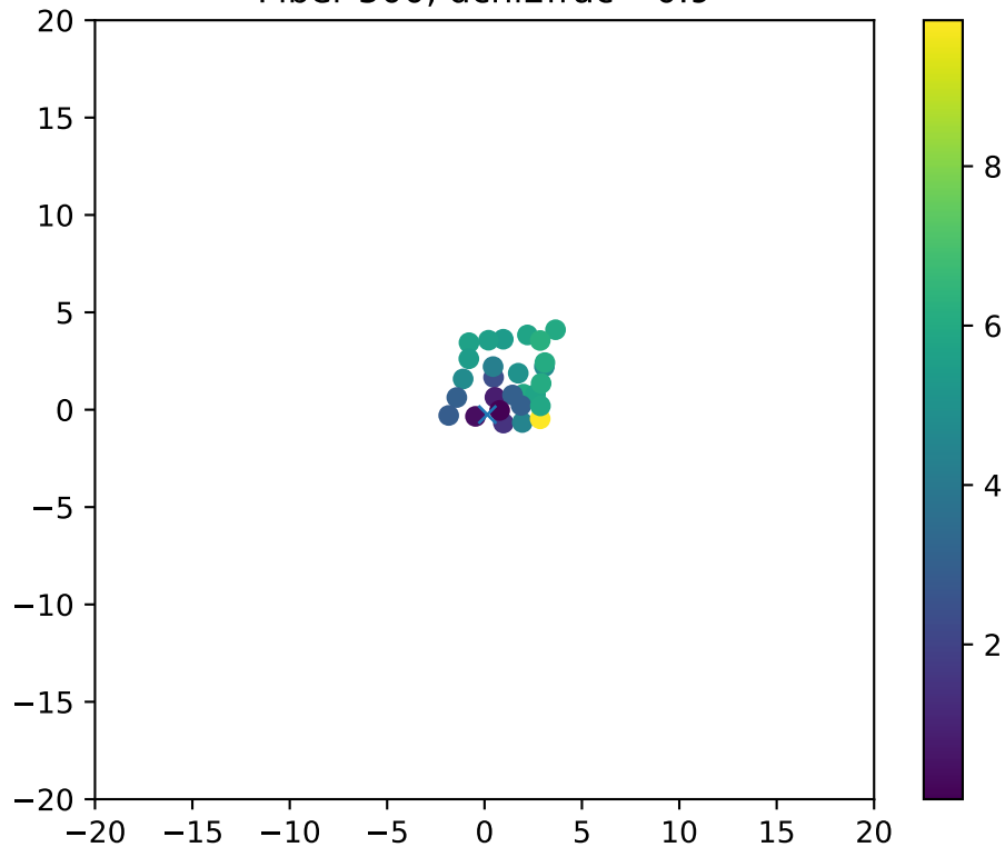
Fiber 500, dchi2frac= 0.9
