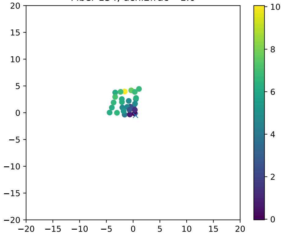
Fiber 134, dchi2frac= 1.0
