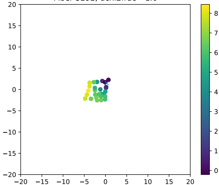
Fiber 3292, dchi2frac= 1.0
