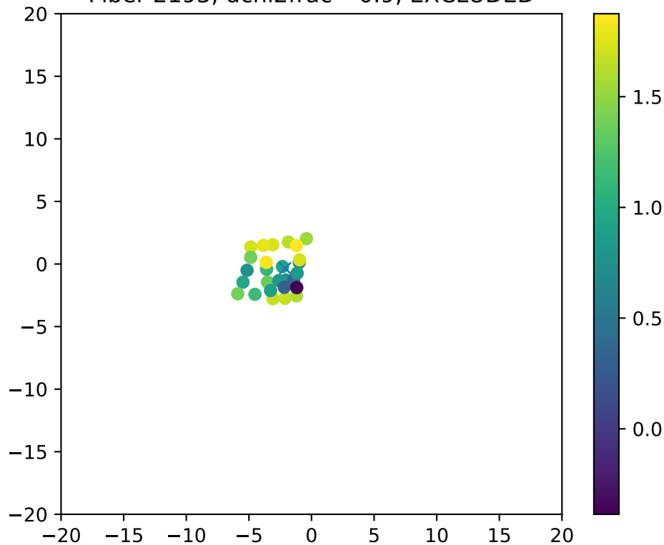
Fiber 2193, dchi2frac= 0.9, EXCLUDED
