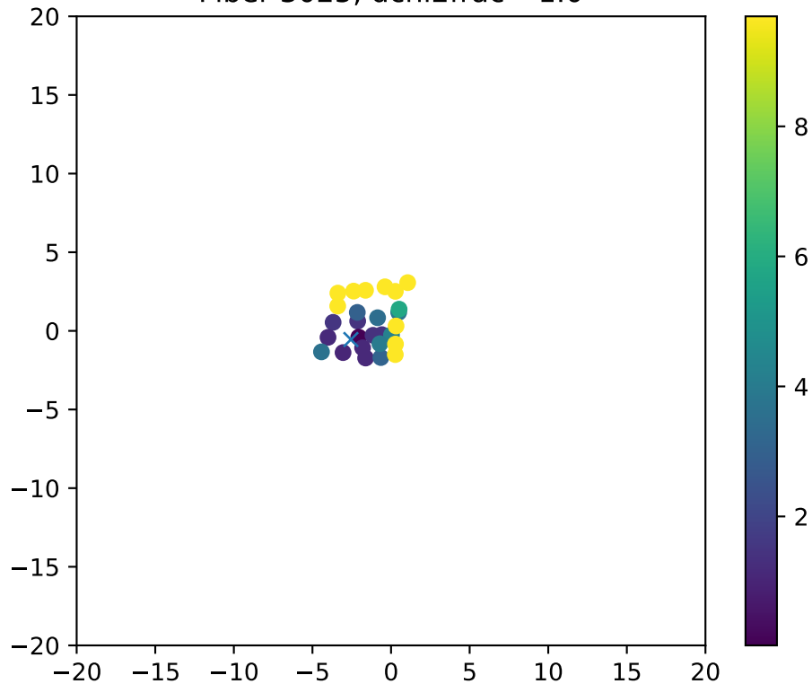
Fiber 3025, dchi2frac= 1.0
