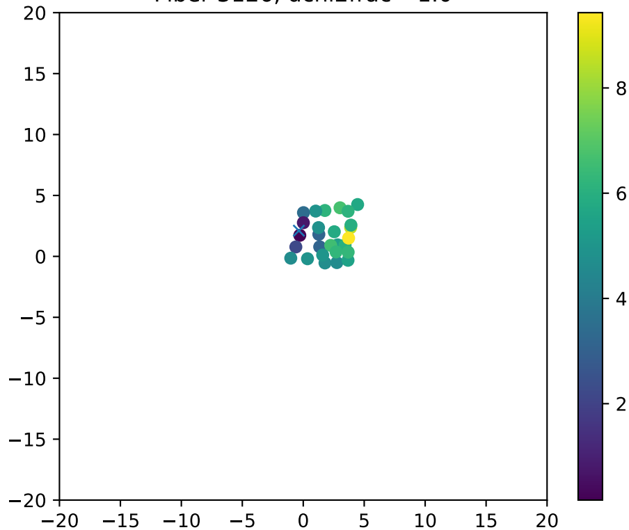
Fiber 3126, dchi2frac= 1.0
