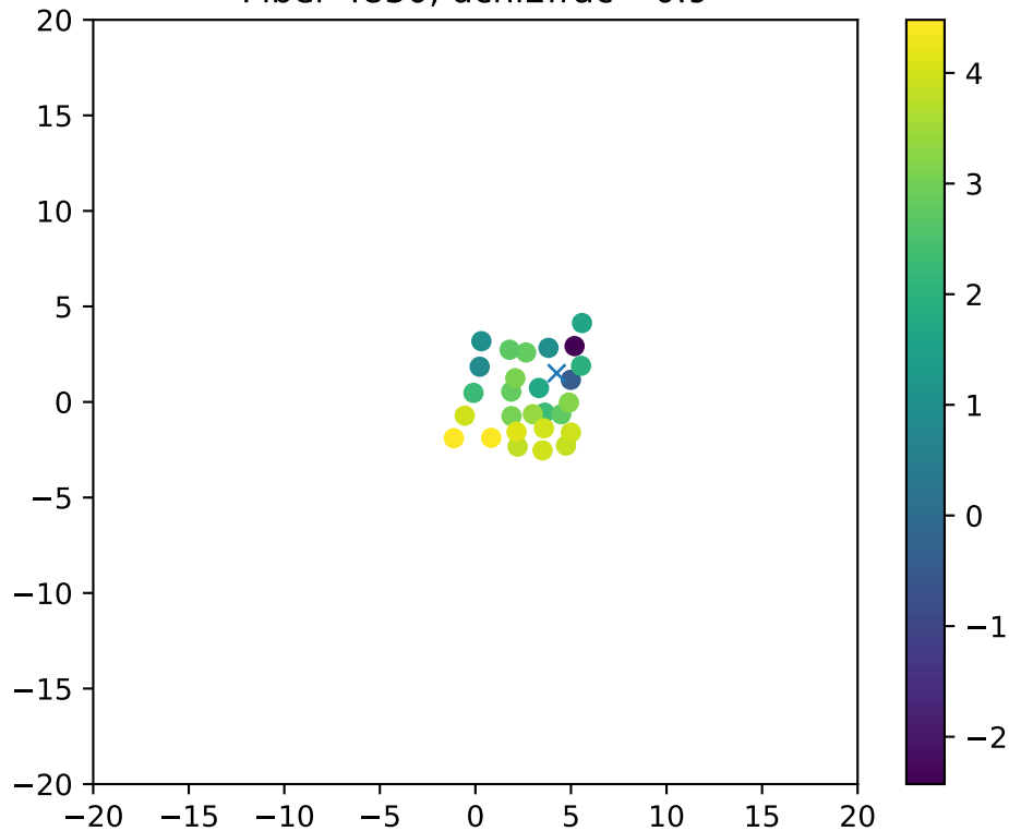
Fiber 4830, dchi2frac= 0.9
