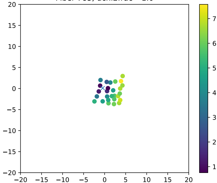
Fiber 783, dchi2frac= 1.0
