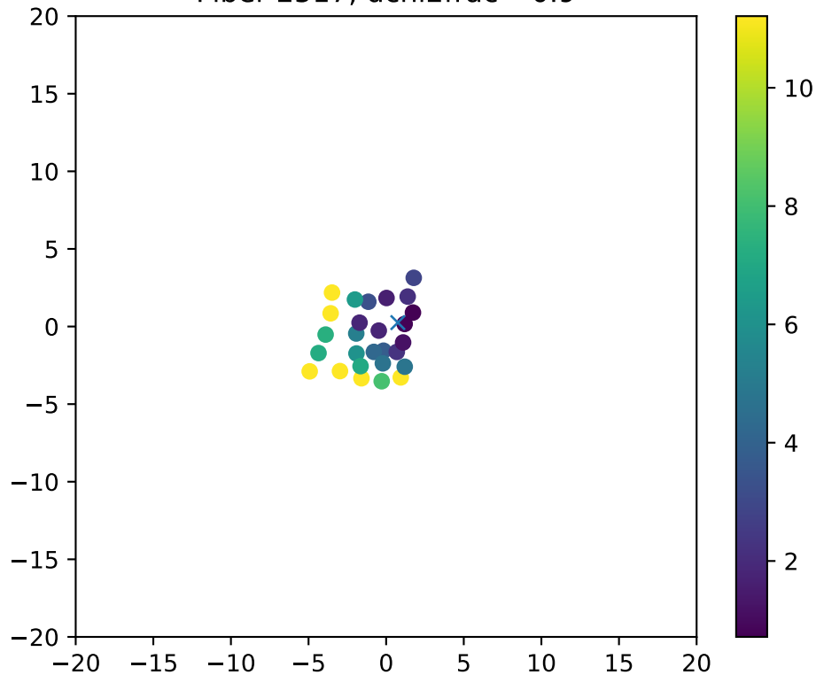
Fiber 2517, dchi2frac= 0.9
