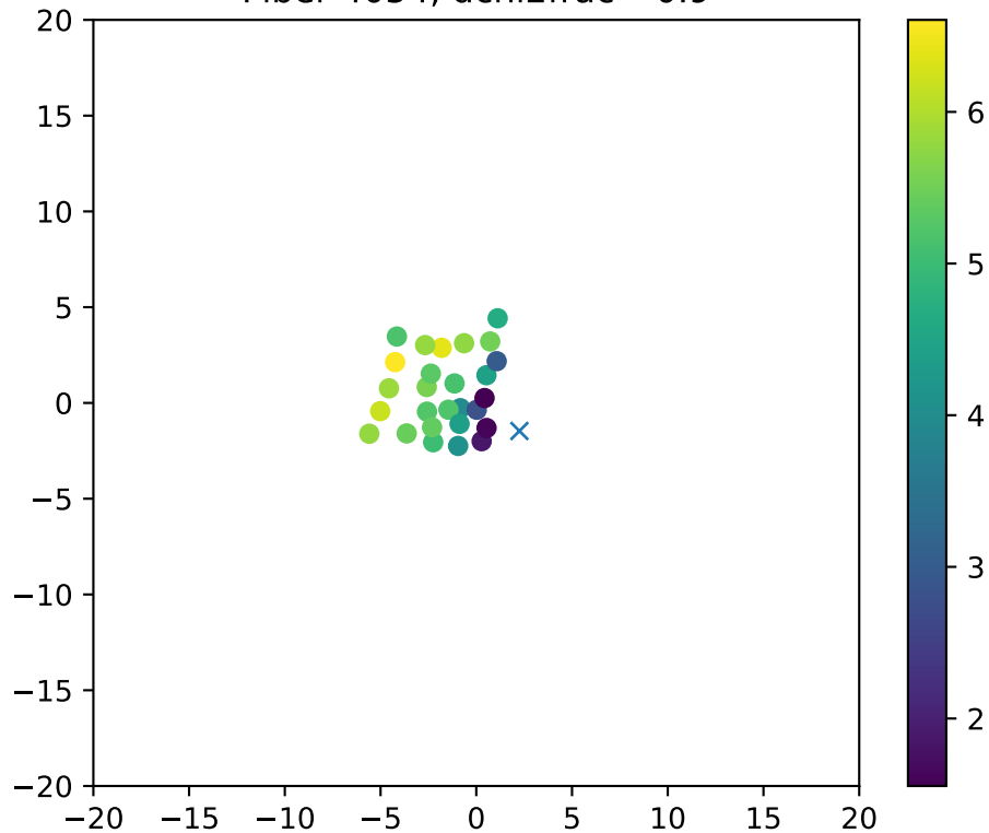
Fiber 4054, dchi2frac= 0.9
