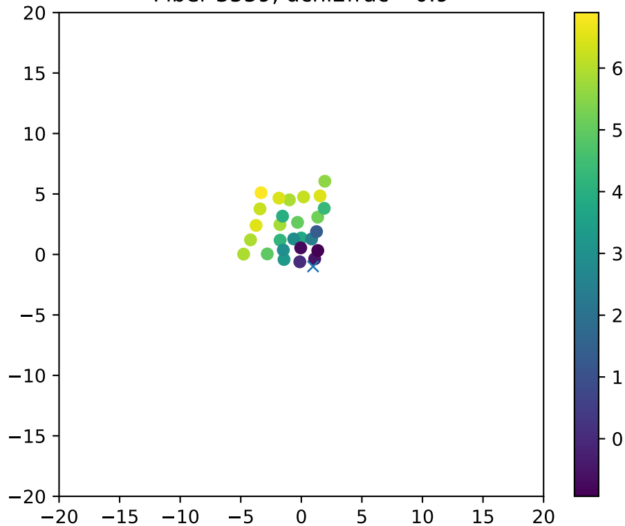
Fiber 3559, dchi2frac= 0.9
