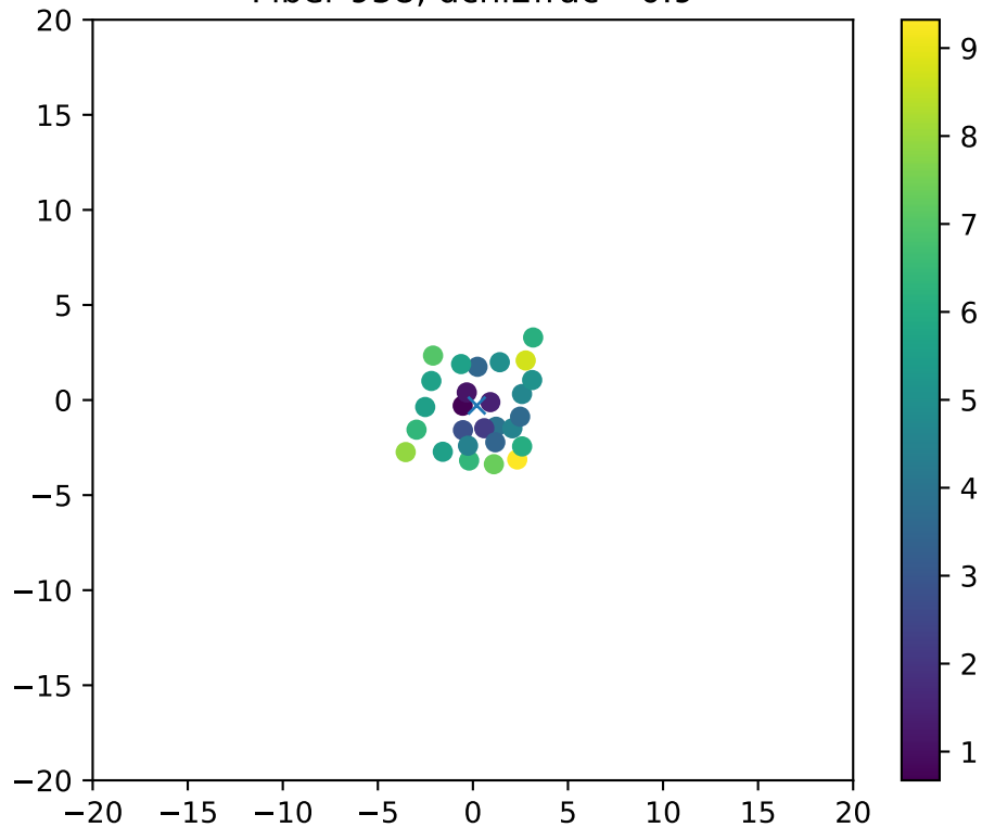
Fiber 958, dchi2frac= 0.9
