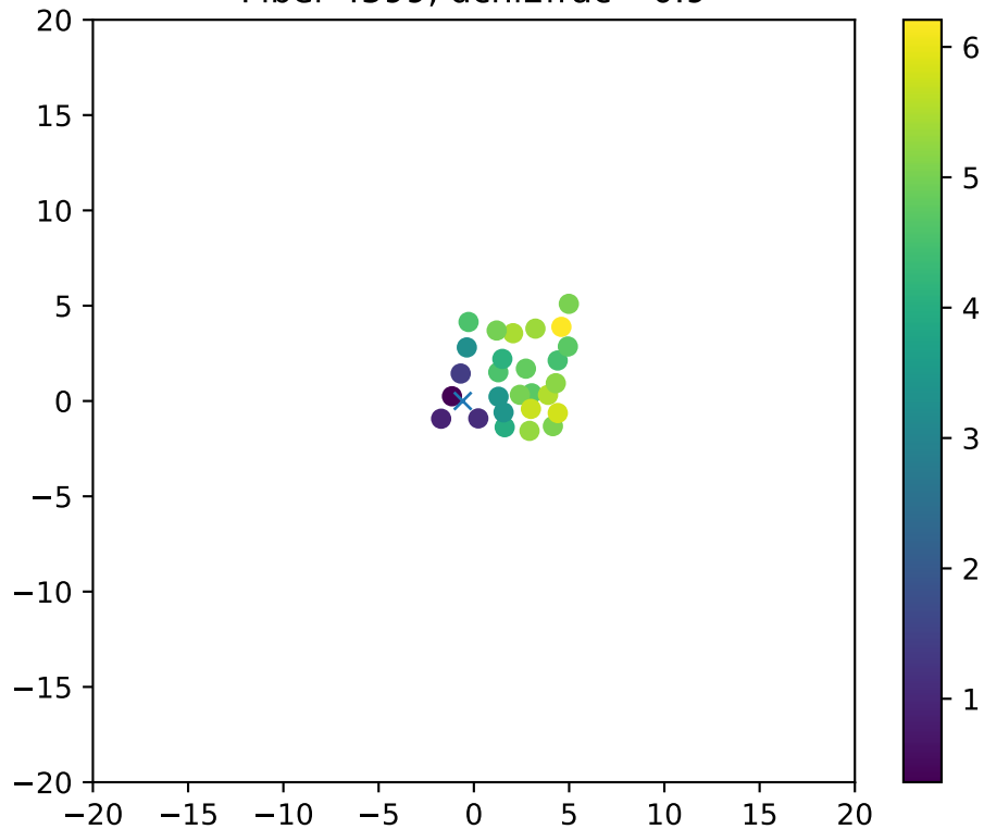
Fiber 4599, dchi2frac= 0.9
