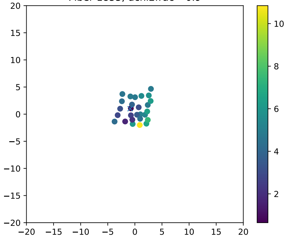
Fiber 1853, dchi2frac= 0.9
