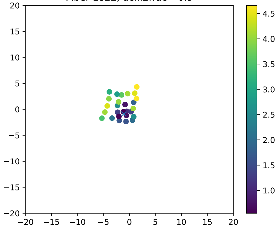
Fiber 1822, dchi2frac= 0.9
