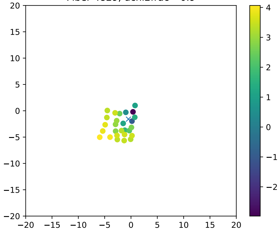
Fiber 4829, dchi2frac= 0.9
