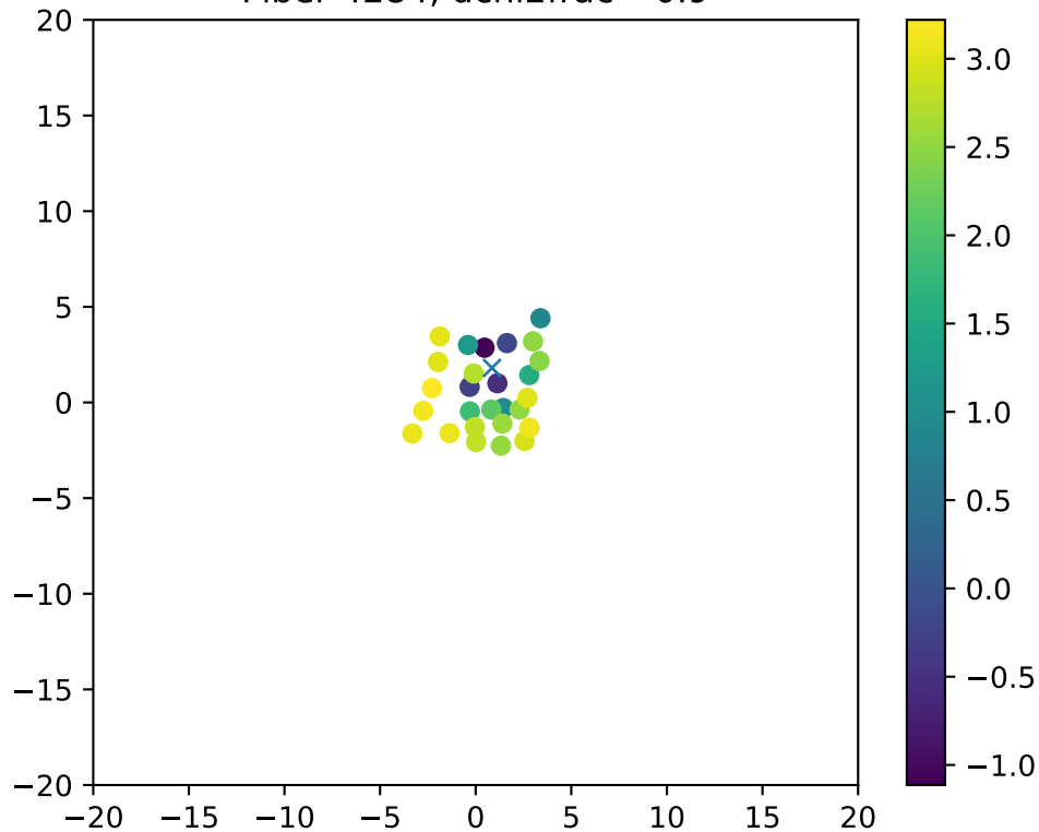
Fiber 4284, dchi2frac= 0.9
