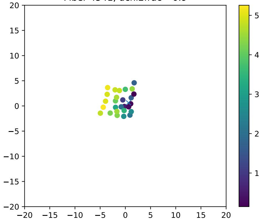
Fiber 4541, dchi2frac= 0.9
