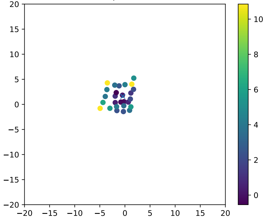
Fiber 3488, dchi2frac= 0.9
