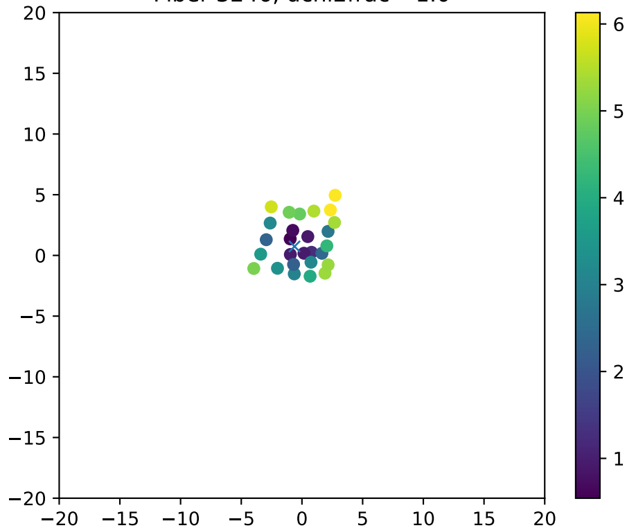
Fiber 3246, dchi2frac= 1.0
