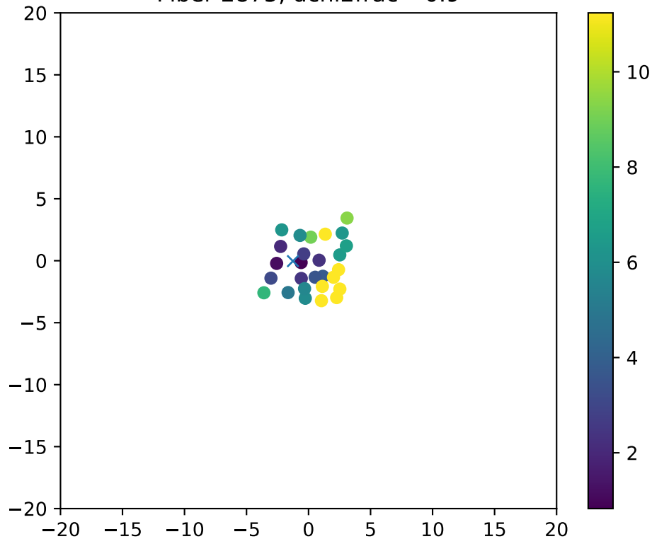
Fiber 2875, dchi2frac= 0.9
