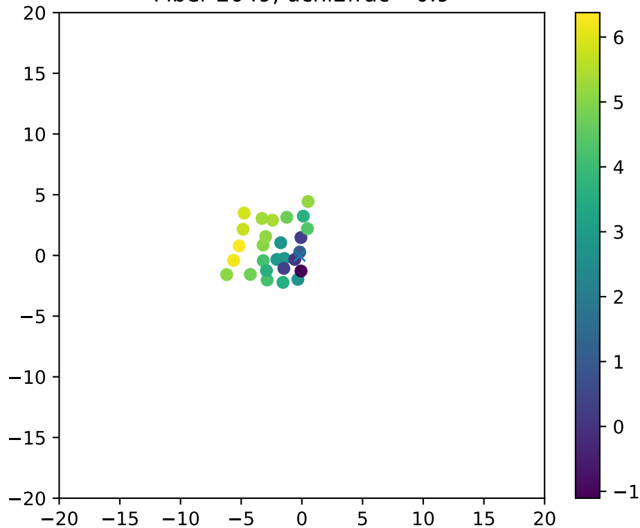
Fiber 2049, dchi2frac= 0.9
