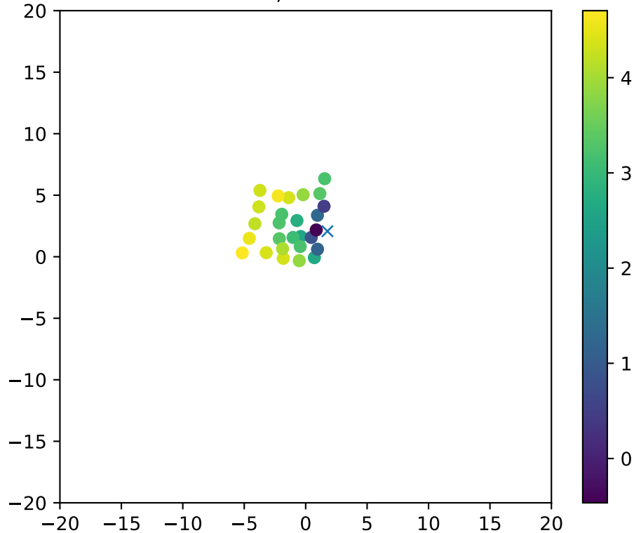
Fiber 3237, dchi2frac= 0.9
