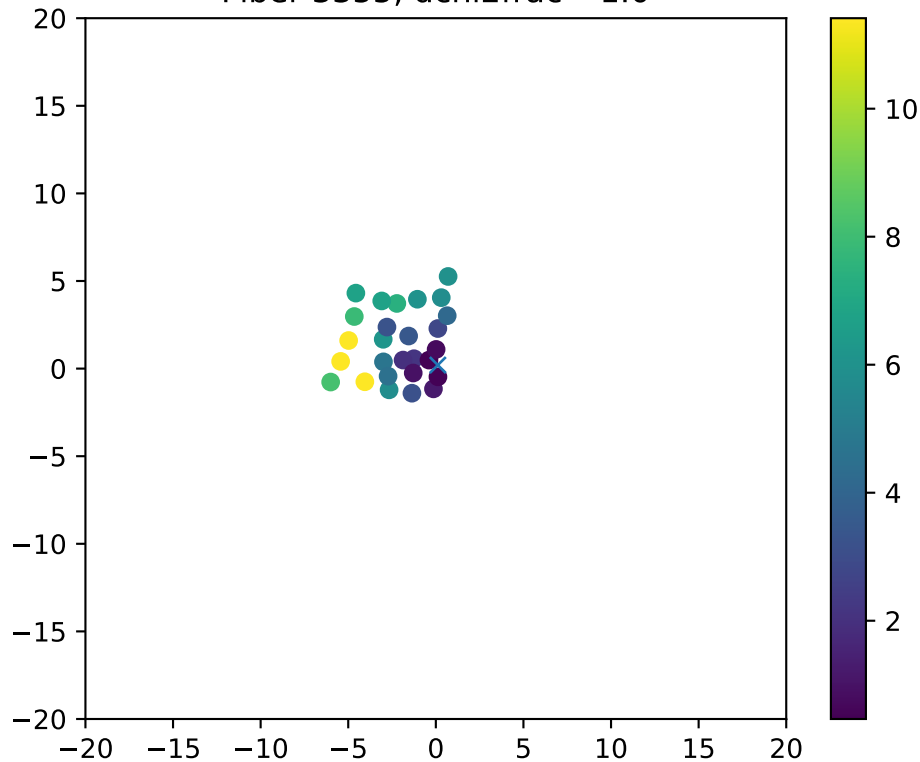
Fiber 3355, dchi2frac= 1.0
