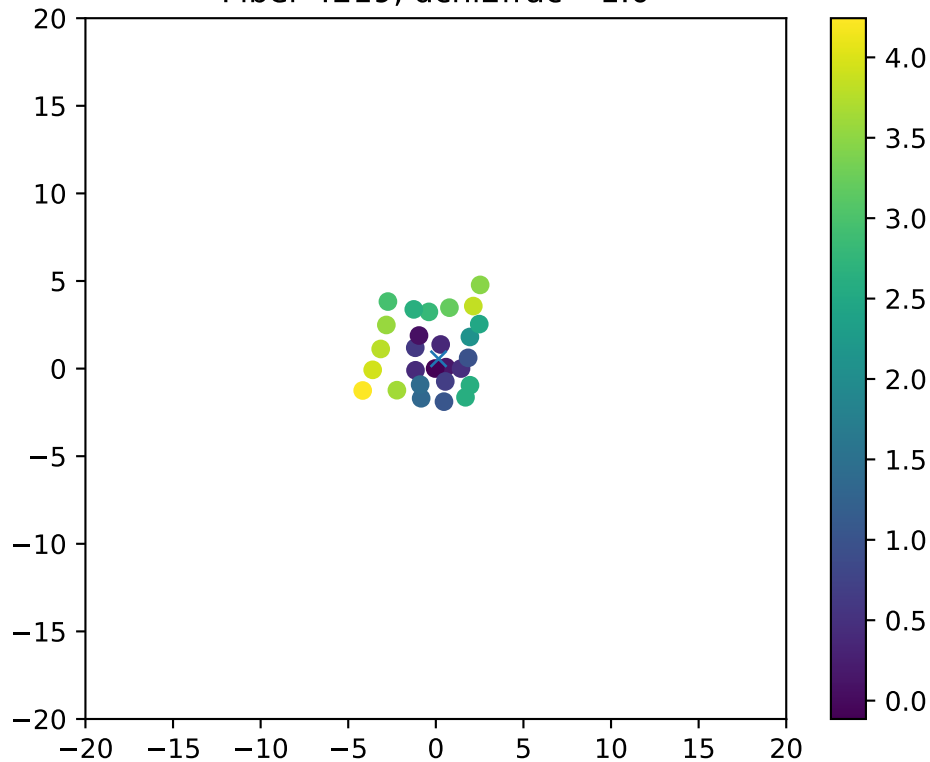
Fiber 4219, dchi2frac= 1.0
