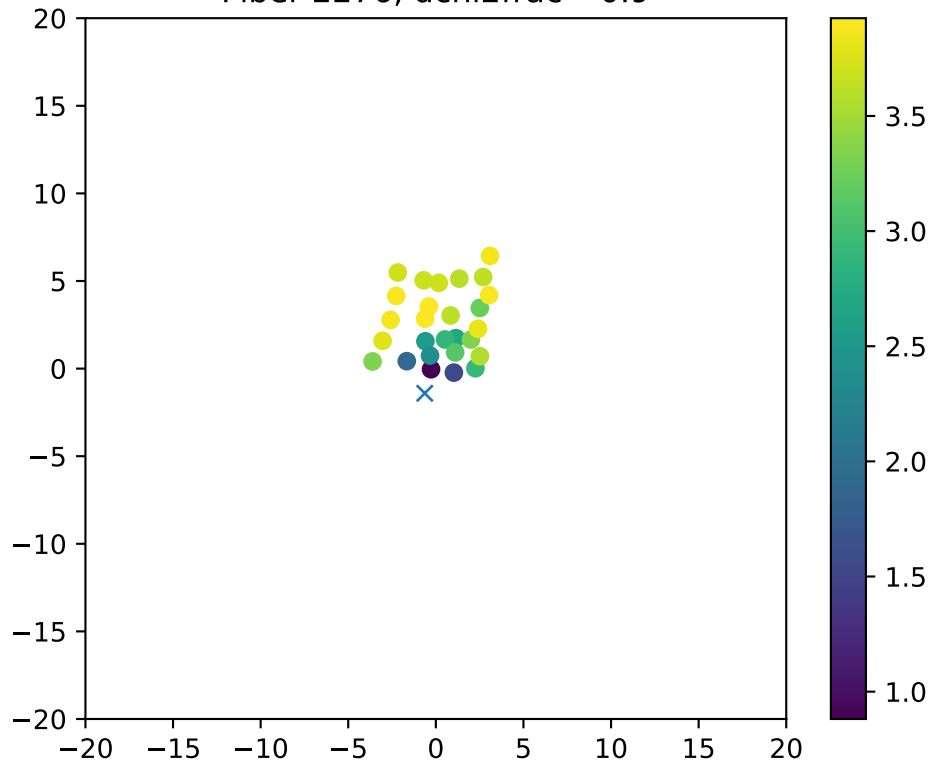
Fiber 2276, dchi2frac= 0.9
