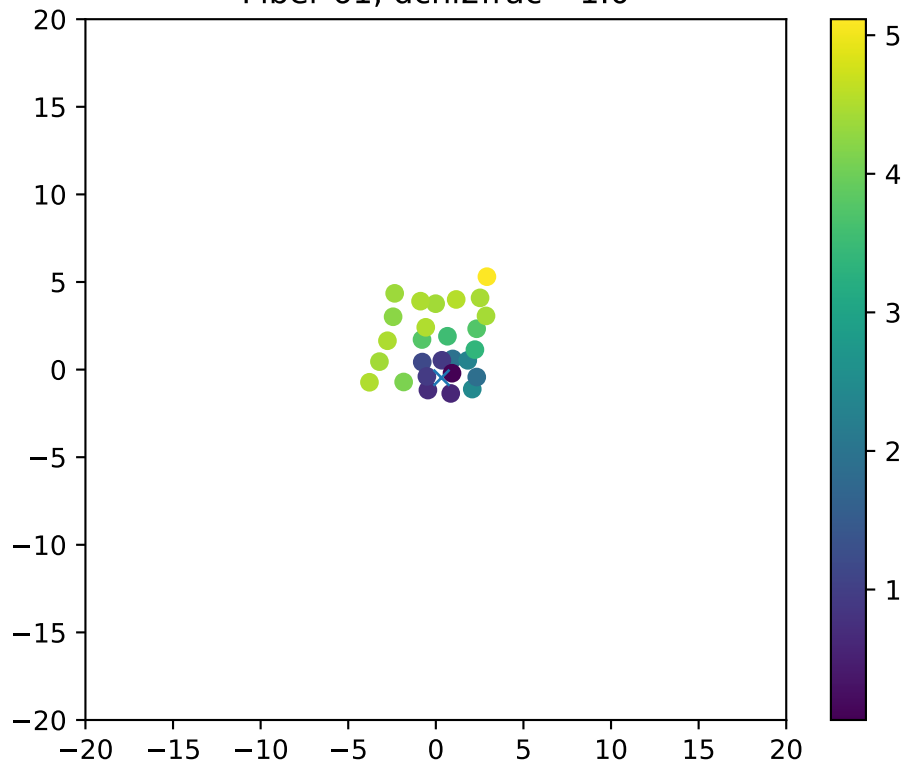
Fiber 61, dchi2frac= 1.0
