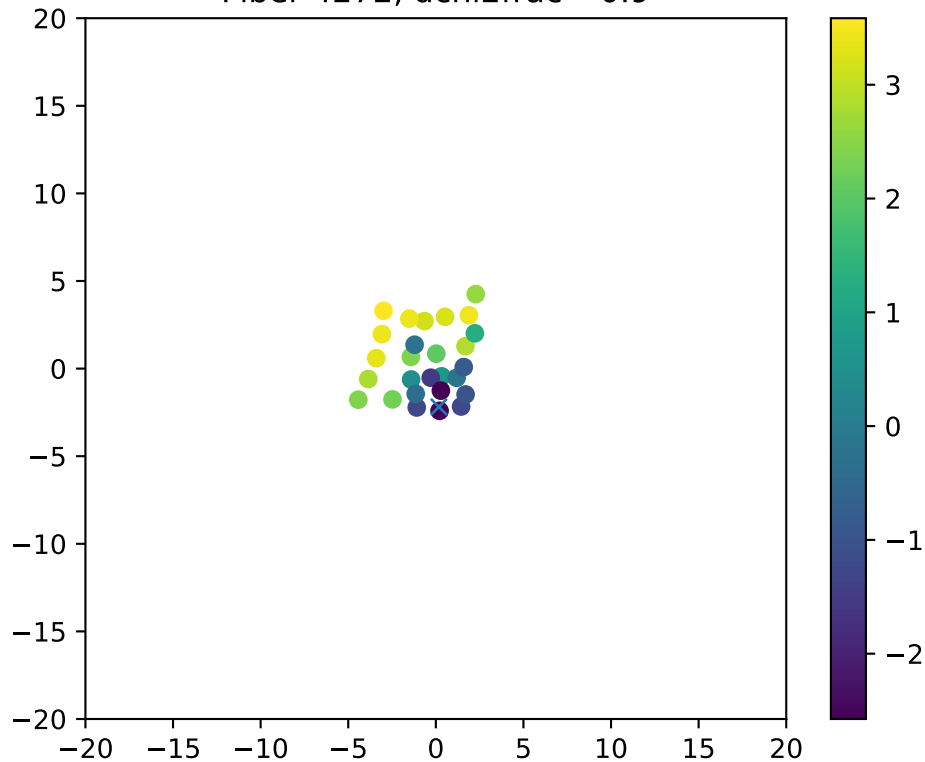
Fiber 4272, dchi2frac= 0.9
