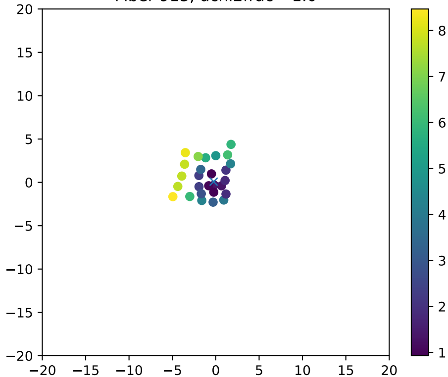
Fiber 913, dchi2frac= 1.0
