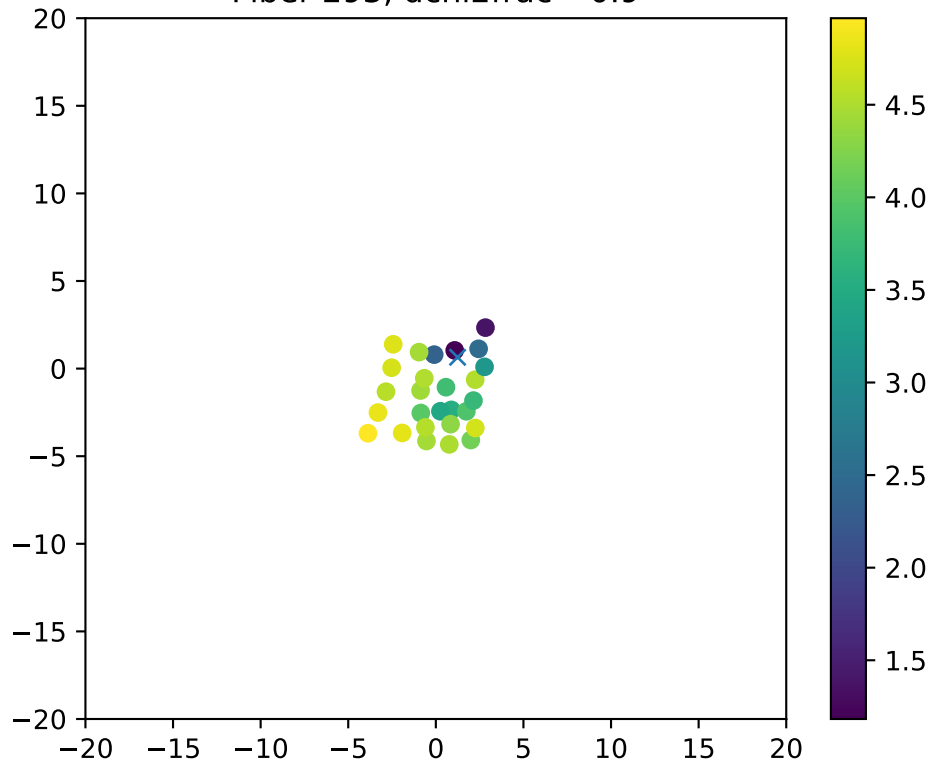
Fiber 293, dchi2frac= 0.9
