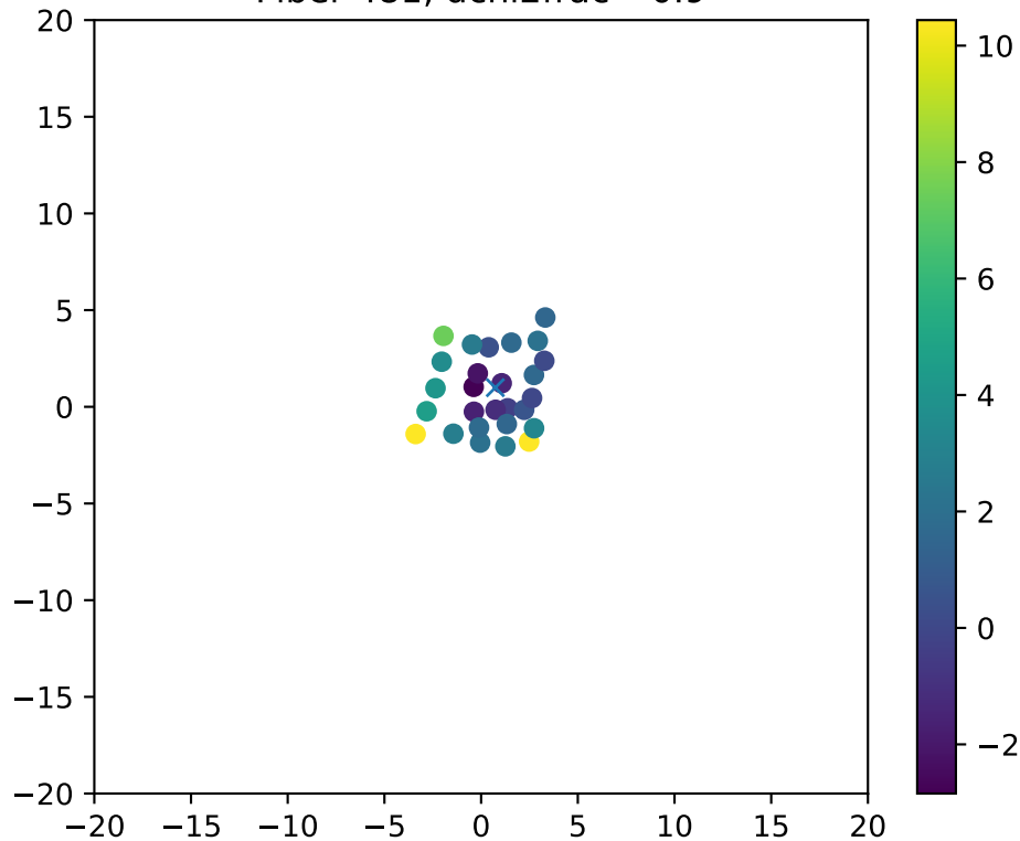
Fiber 481, dchi2frac= 0.9
