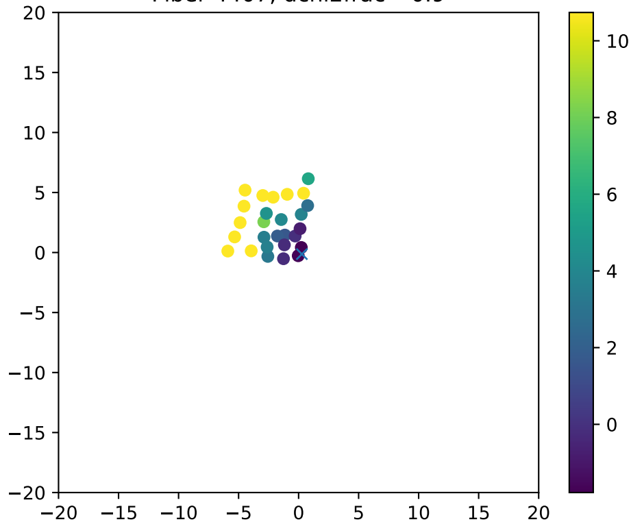
Fiber 4407, dchi2frac= 0.9
