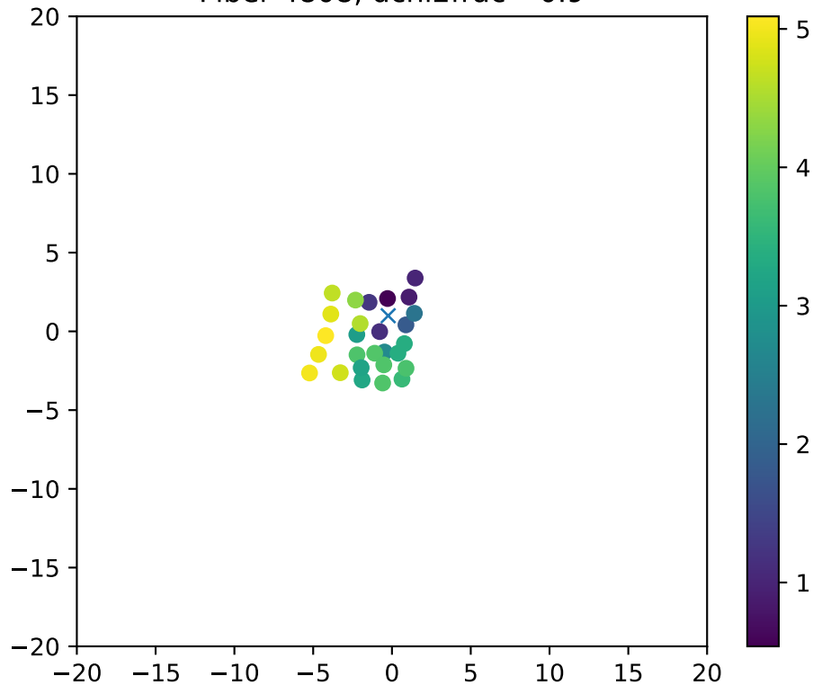
Fiber 4808, dchi2frac= 0.9
