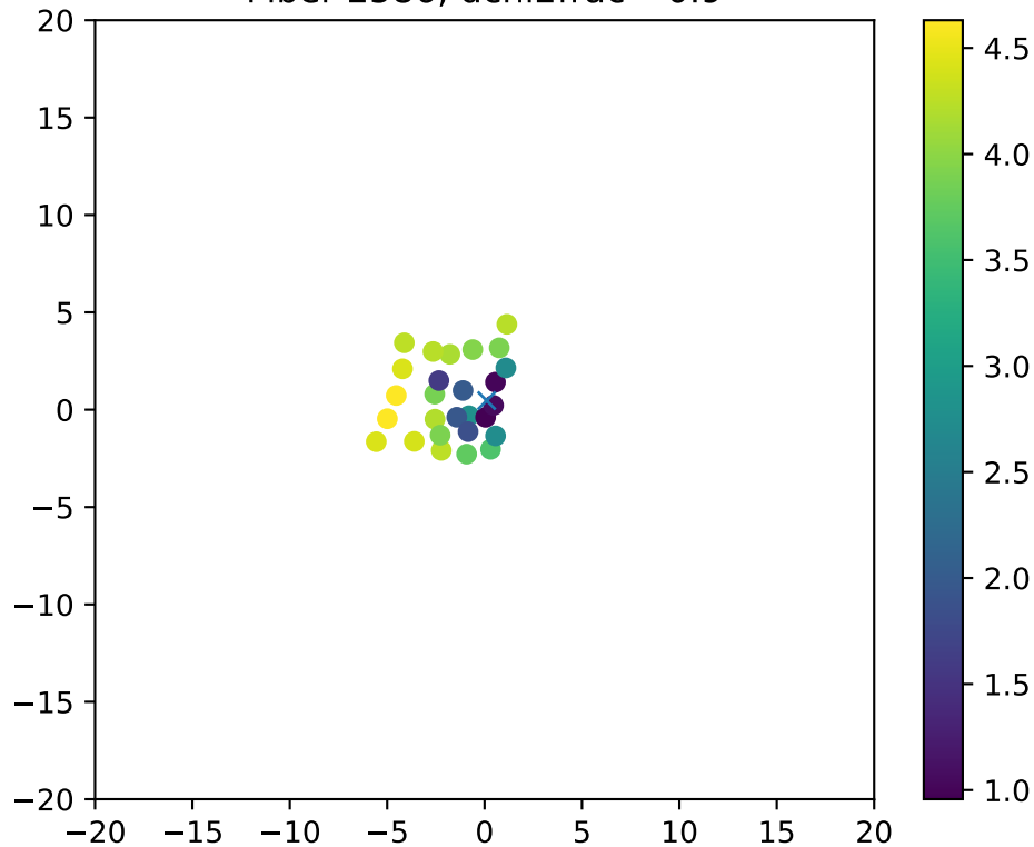
Fiber 2586, dchi2frac= 0.9
