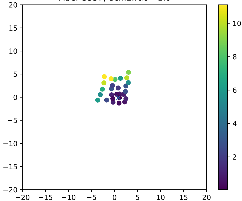
Fiber 3337, dchi2frac= 1.0
