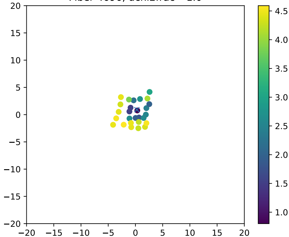
Fiber 4696, dchi2frac= 1.0
