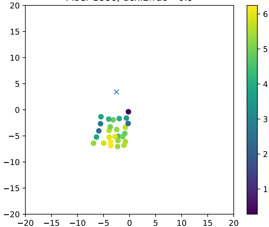
Fiber 1886, dchi2frac= 0.9
