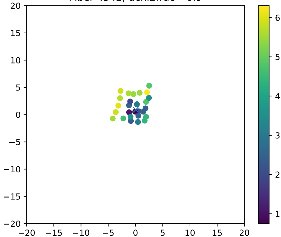
Fiber 4542, dchi2frac= 0.9
