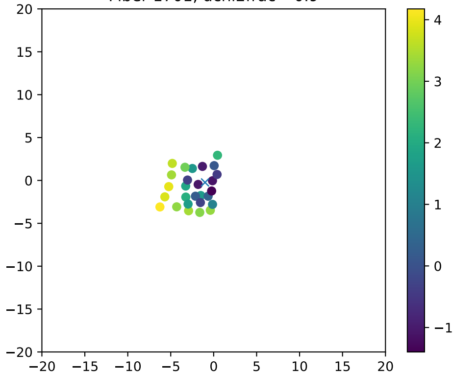
Fiber 1701, dchi2frac= 0.9
