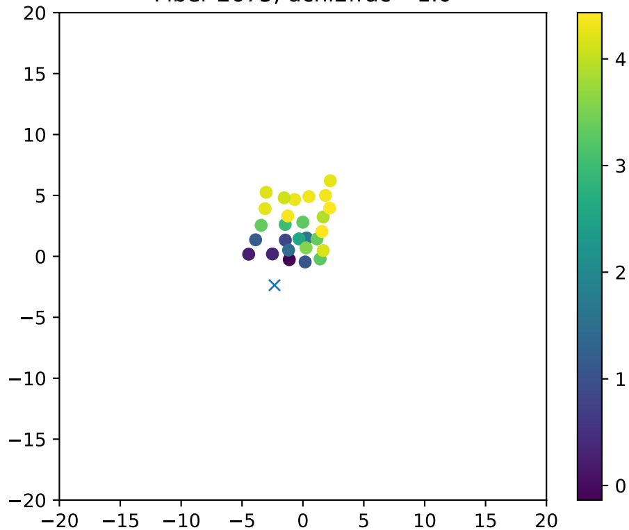
Fiber 2675, dchi2frac= 1.0
