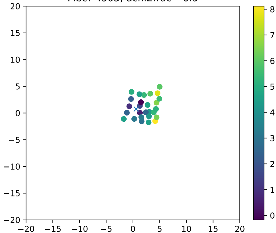
Fiber 4505, dchi2frac= 0.9
