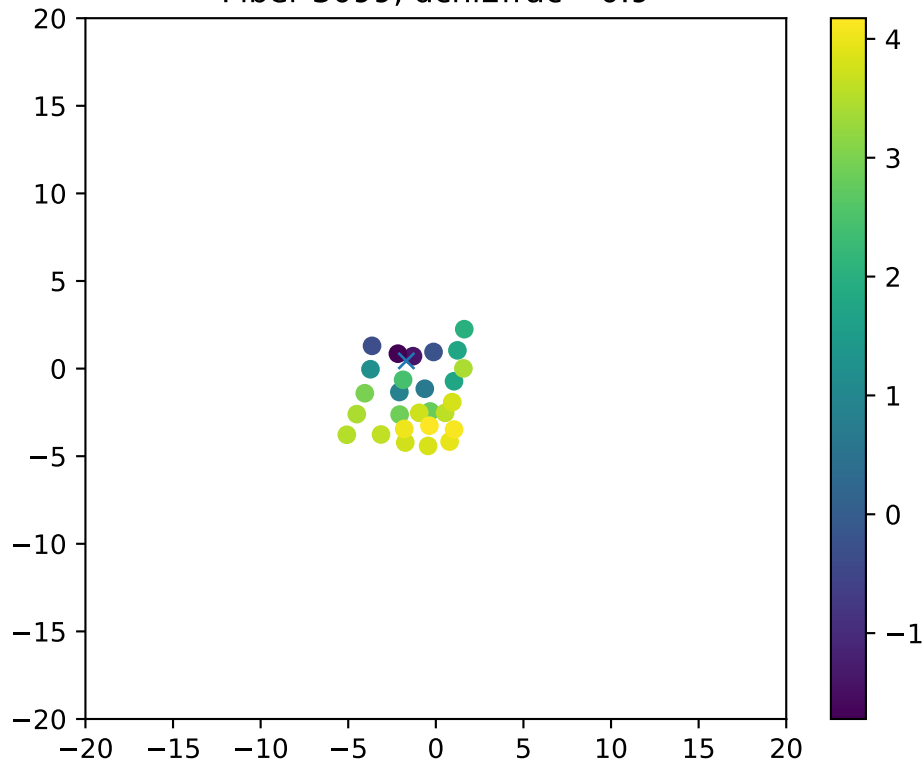
Fiber 3099, dchi2frac= 0.9
