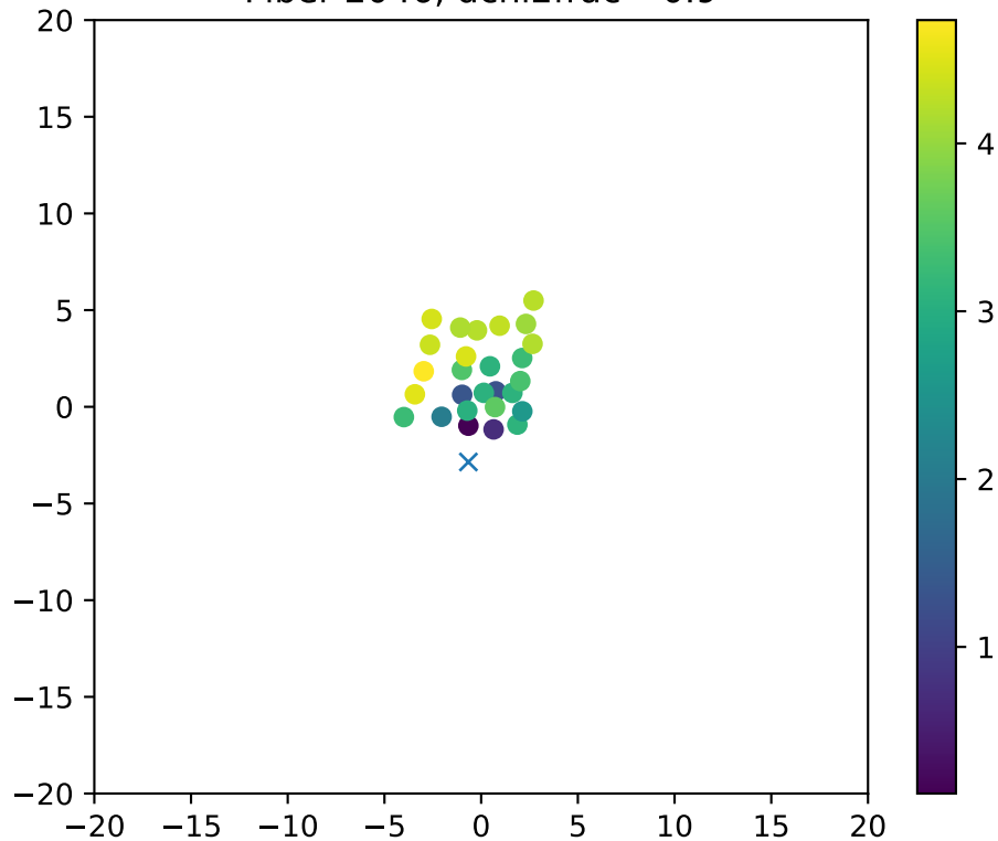
Fiber 2046, dchi2frac= 0.9
