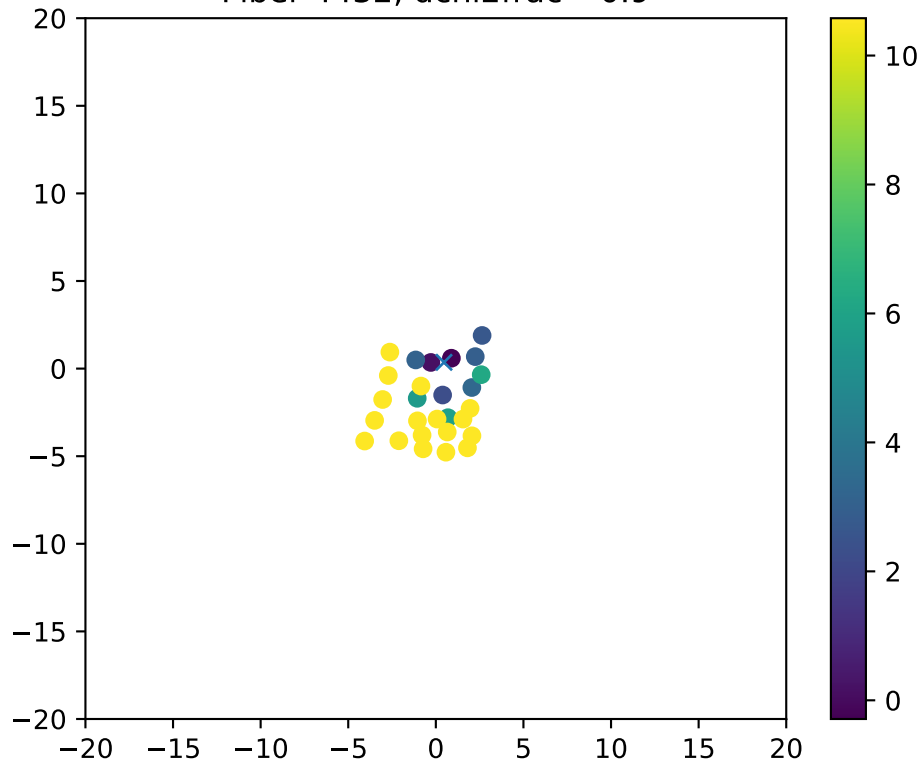
Fiber 4432, dchi2frac= 0.9
