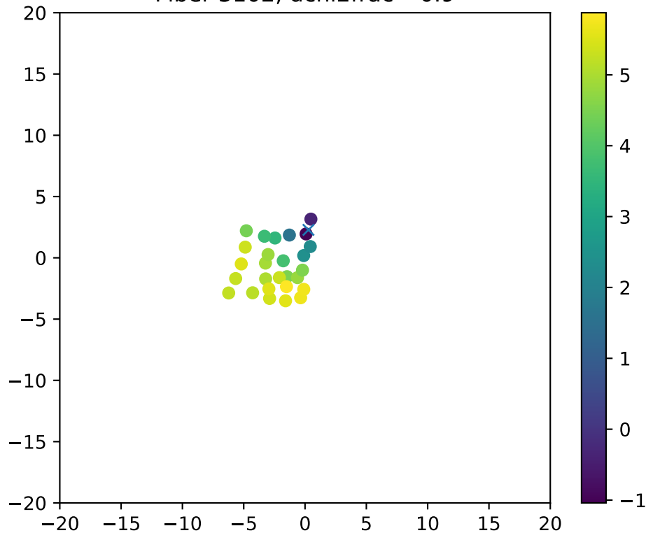
Fiber 3102, dchi2frac= 0.9
