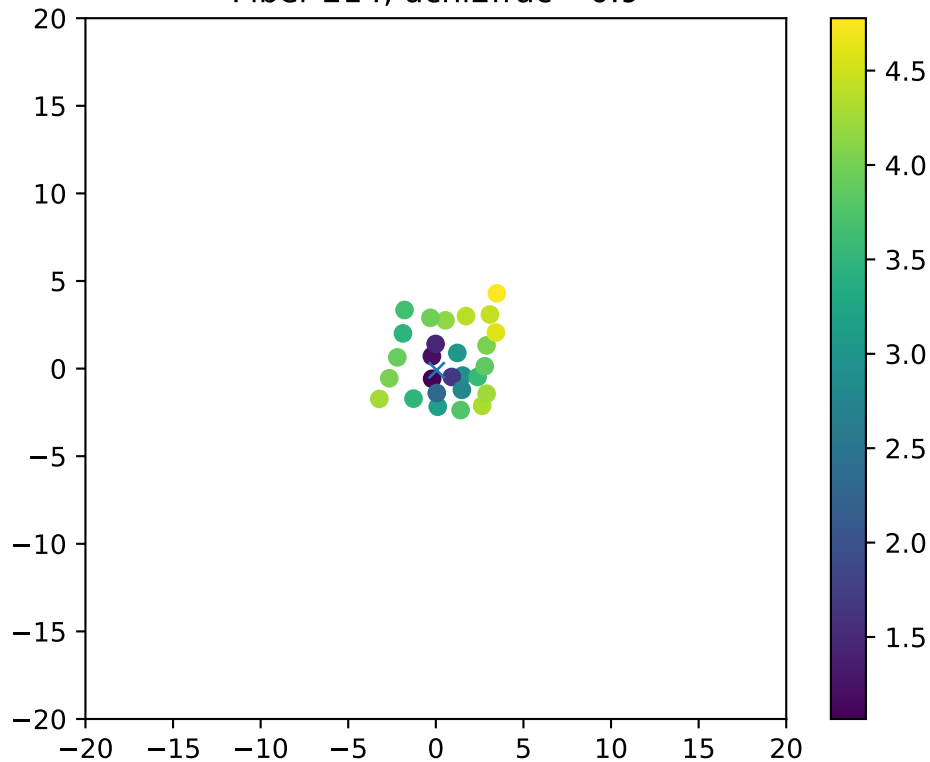
Fiber 214, dchi2frac= 0.9
