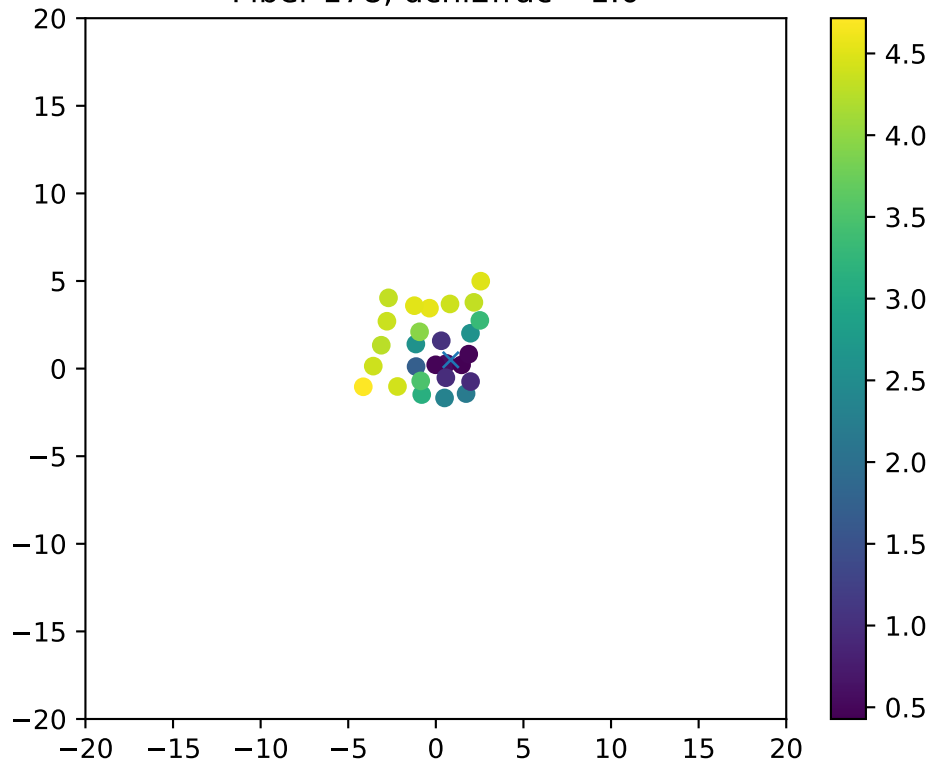
Fiber 178, dchi2frac= 1.0
