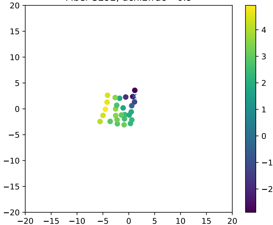
Fiber 3292, dchi2frac= 0.9
