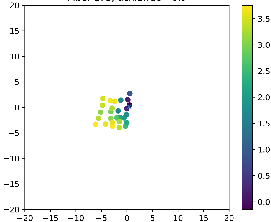
Fiber 173, dchi2frac= 0.9
