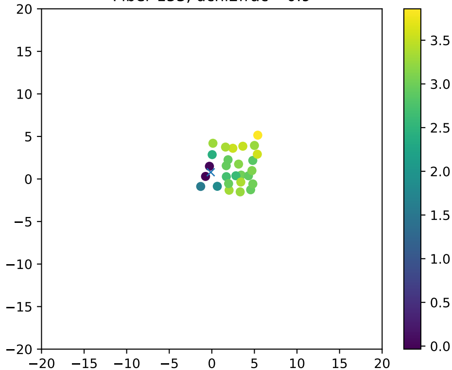
Fiber 153, dchi2frac= 0.9
