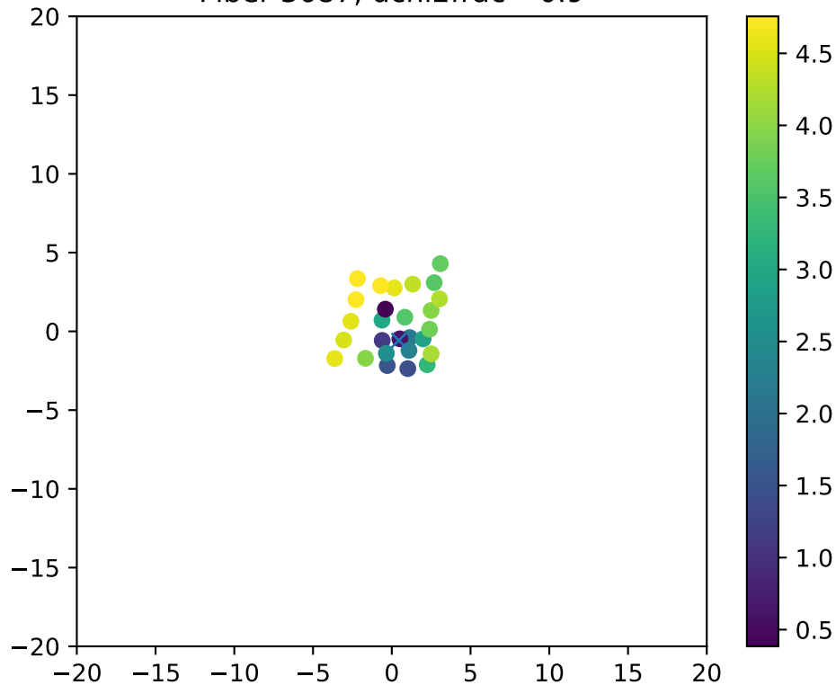
Fiber 3687, dchi2frac= 0.9
