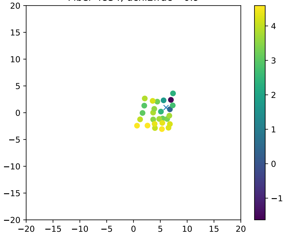
Fiber 4834, dchi2frac= 0.9
