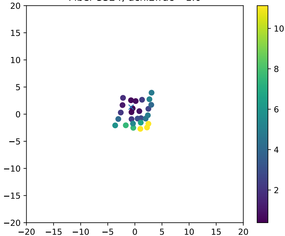
Fiber 3324, dchi2frac= 1.0
