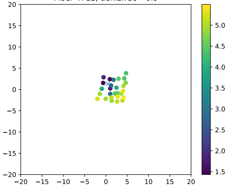
Fiber 4712, dchi2frac= 0.9
