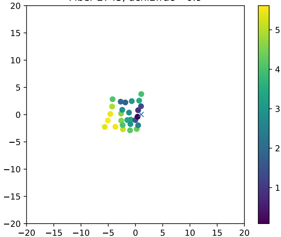
Fiber 2743, dchi2frac= 0.9
