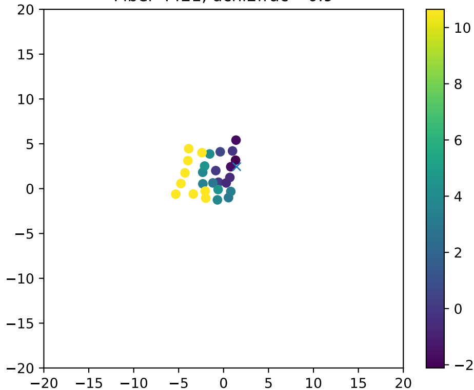
Fiber 4421, dchi2frac= 0.9
