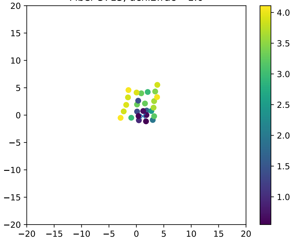
Fiber 3713, dchi2frac= 1.0
