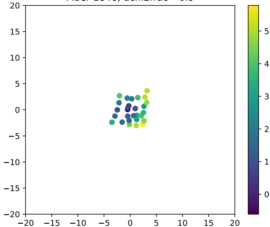
Fiber 1846, dchi2frac= 0.9
