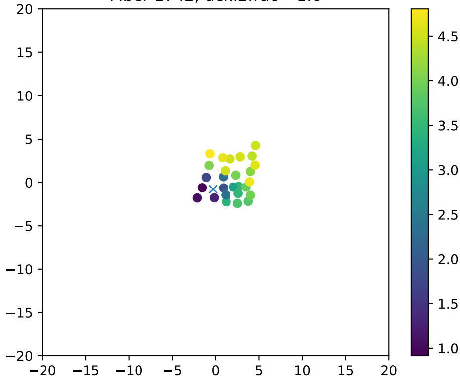
Fiber 1742, dchi2frac= 1.0
