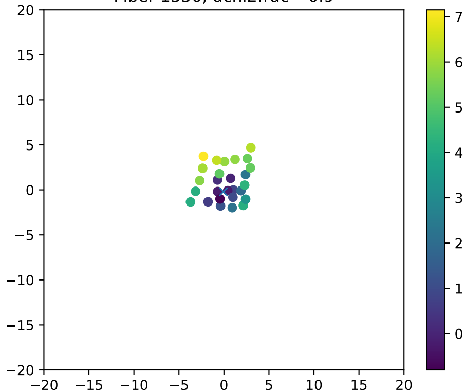
Fiber 1550, dchi2frac= 0.9
