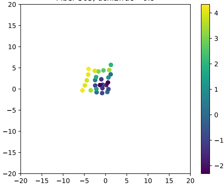
Fiber 305, dchi2frac= 0.9
