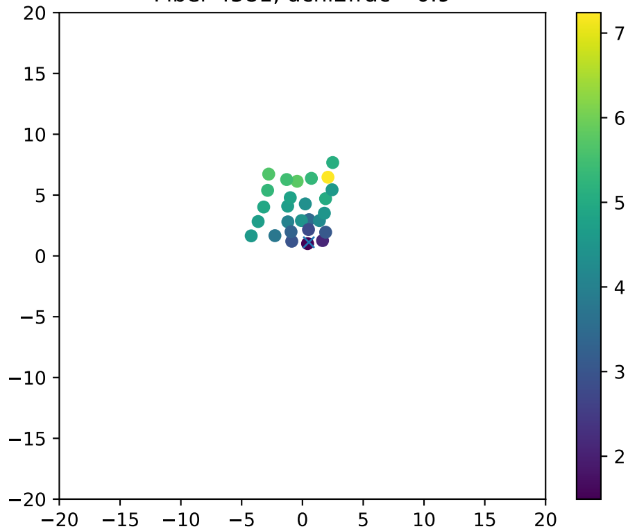
Fiber 4581, dchi2frac= 0.9
