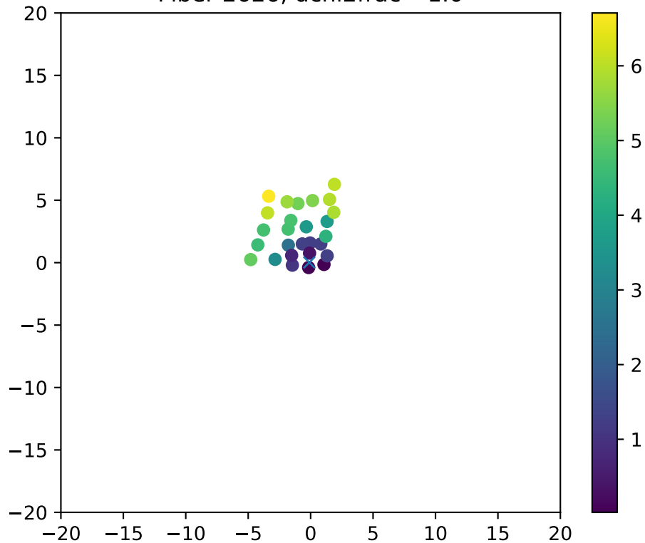
Fiber 2626, dchi2frac= 1.0
