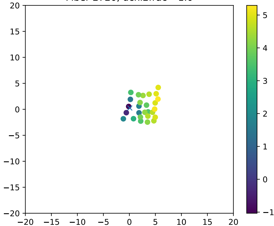
Fiber 2720, dchi2frac= 1.0
