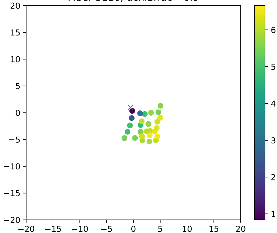
Fiber 3116, dchi2frac= 0.9
