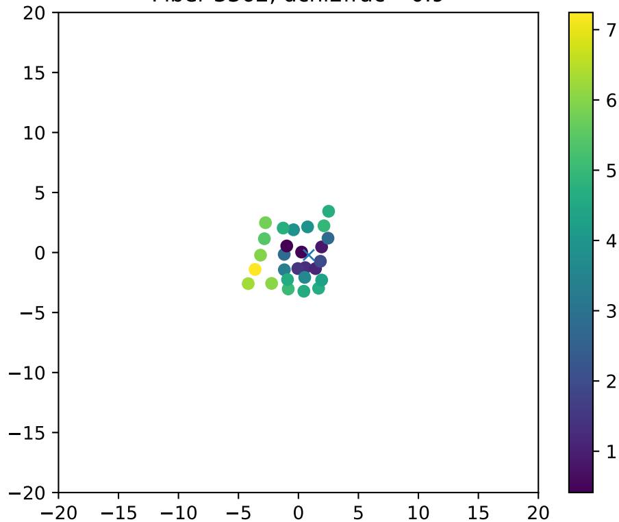
Fiber 3362, dchi2frac= 0.9
