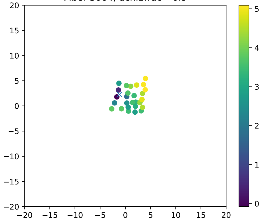
Fiber 3064, dchi2frac= 0.9
