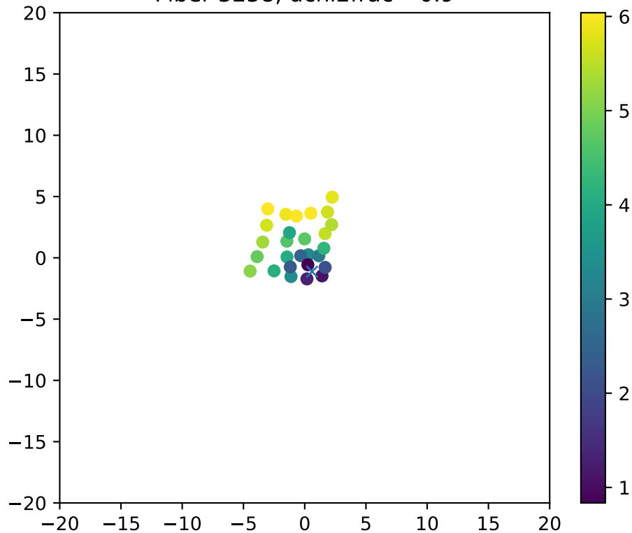
Fiber 3258, dchi2frac= 0.9
