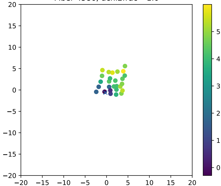
Fiber 4586, dchi2frac= 1.0
