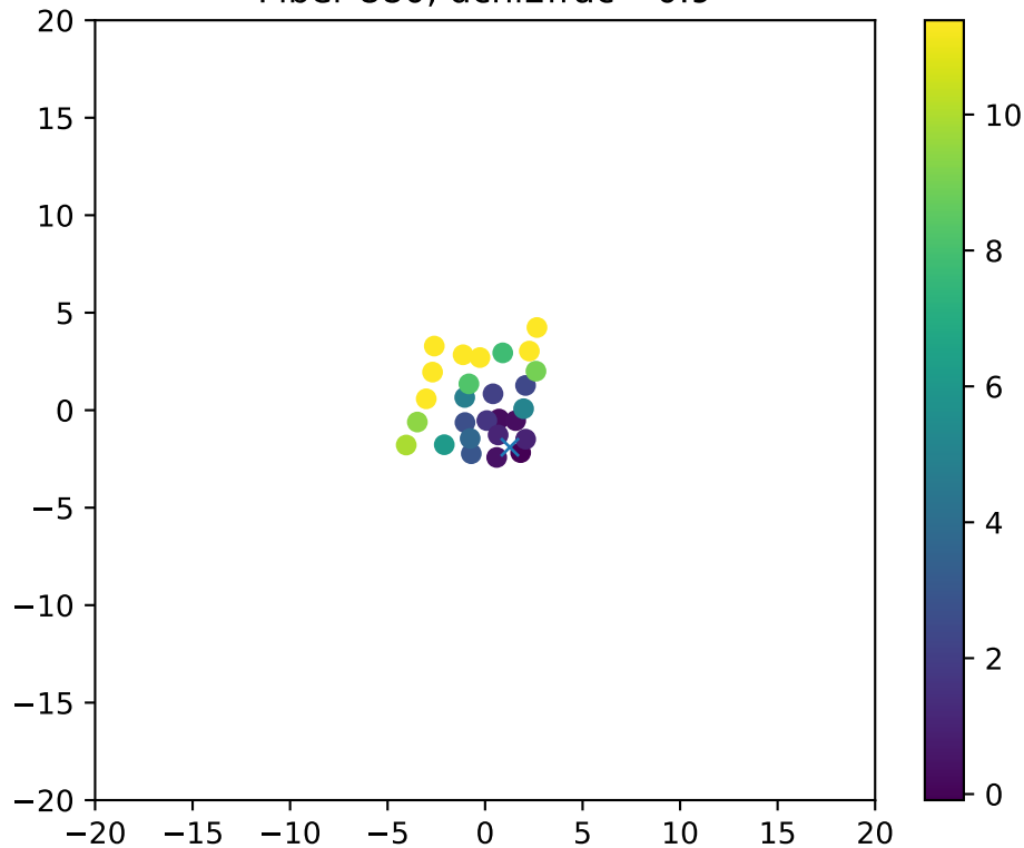
Fiber 880, dchi2frac= 0.9
