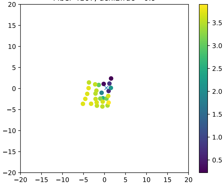
Fiber 4167, dchi2frac= 0.9
