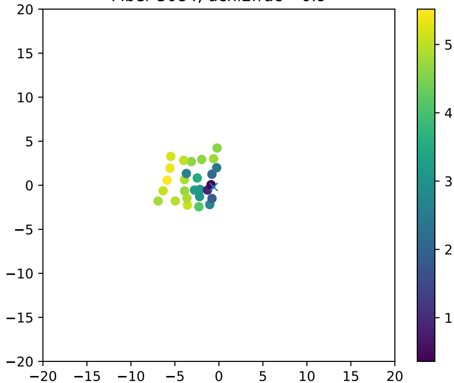
Fiber 3084, dchi2frac= 0.9
