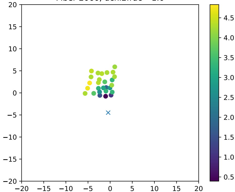
Fiber 2060, dchi2frac= 1.0
