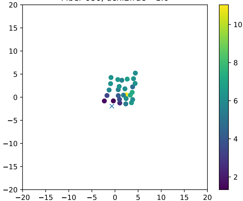
Fiber 686, dchi2frac= 1.0
