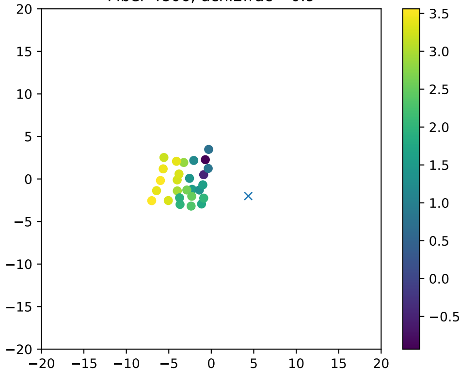
Fiber 4806, dchi2frac= 0.9
