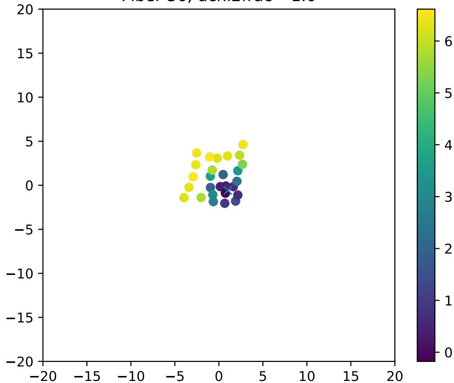
Fiber 36, dchi2frac= 1.0
