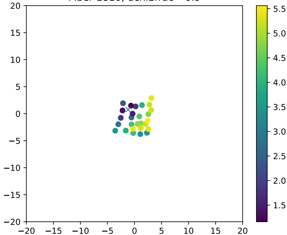
Fiber 1810, dchi2frac= 0.9
