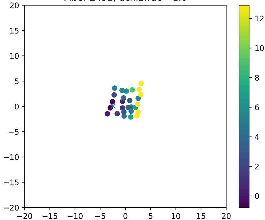
Fiber 2492, dchi2frac= 1.0
