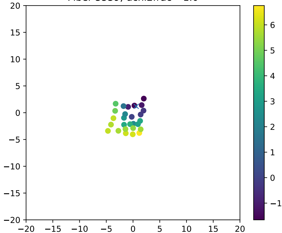
Fiber 3539, dchi2frac= 1.0
