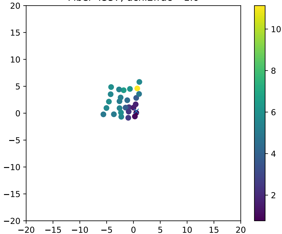
Fiber 4557, dchi2frac= 1.0
