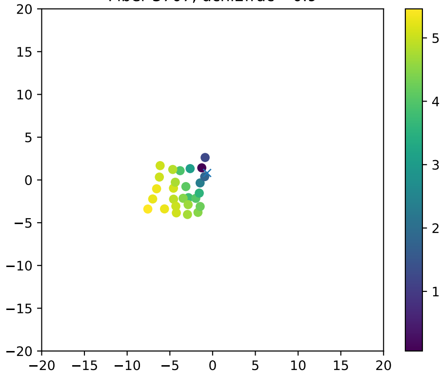
Fiber 3707, dchi2frac= 0.9
