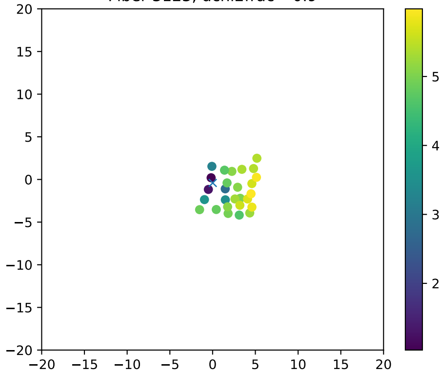
Fiber 3123, dchi2frac= 0.9
