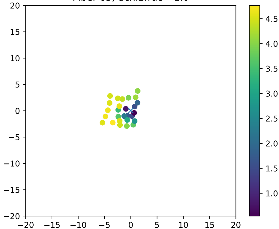
Fiber 65, dchi2frac= 1.0
