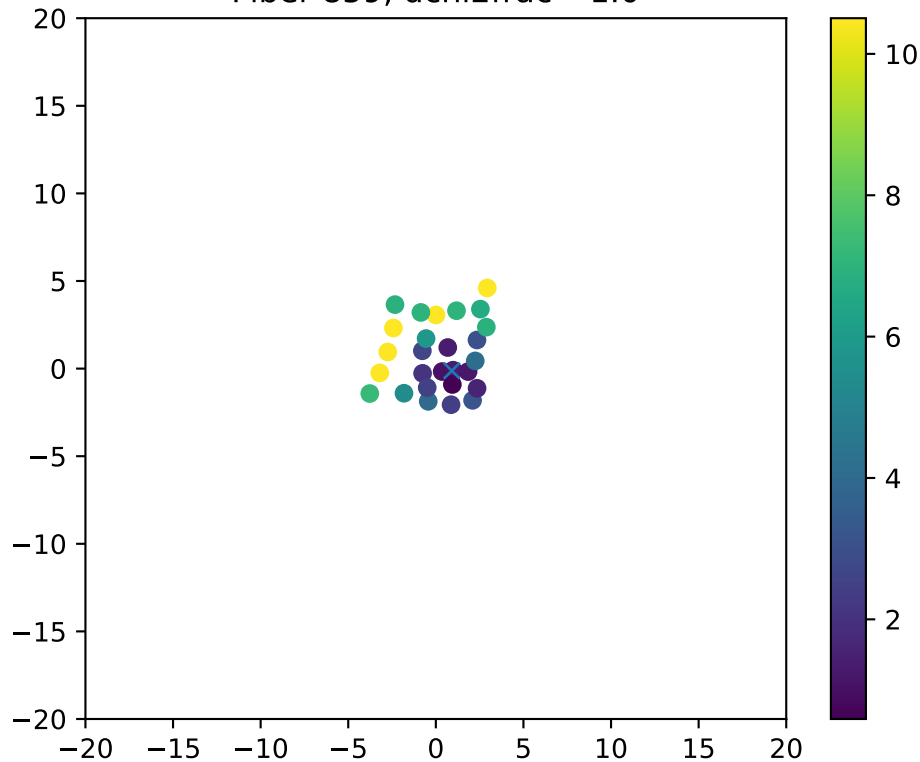
Fiber 859, dchi2frac= 1.0
