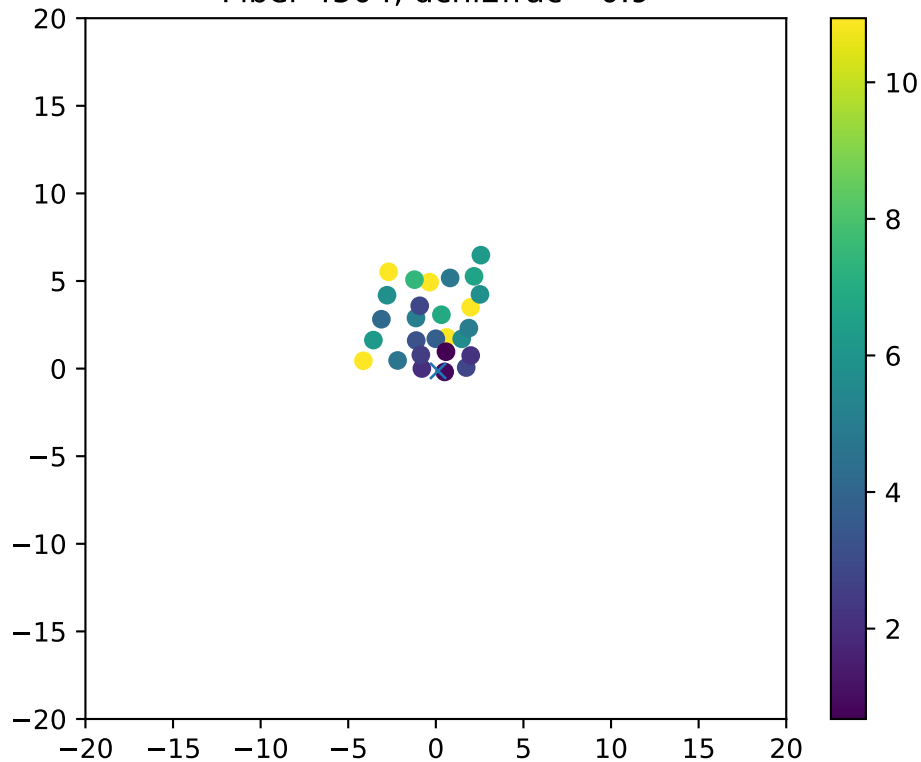
Fiber 4504, dchi2frac= 0.9
