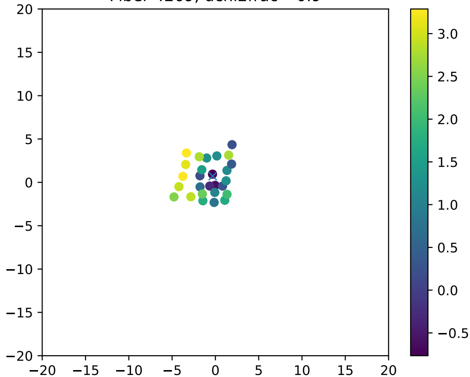
Fiber 4269, dchi2frac= 0.9
