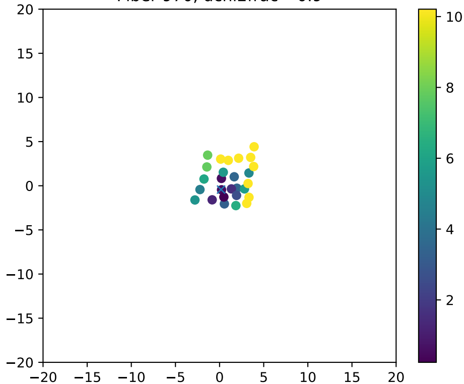
Fiber 970, dchi2frac= 0.9
