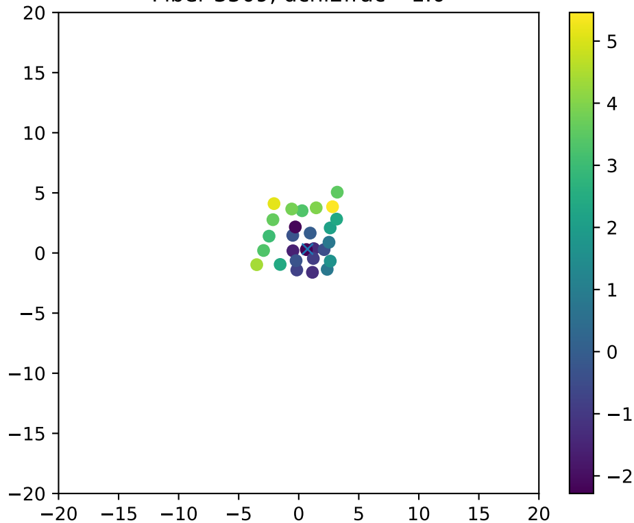
Fiber 3509, dchi2frac= 1.0
