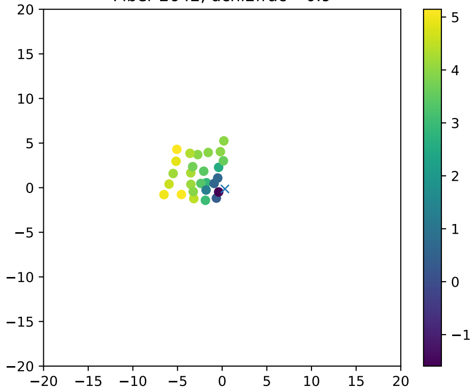
Fiber 2642, dchi2frac= 0.9
