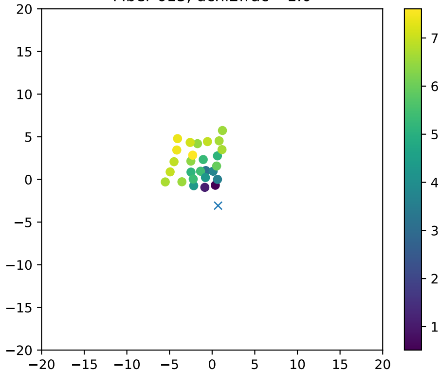
Fiber 613, dchi2frac= 1.0
