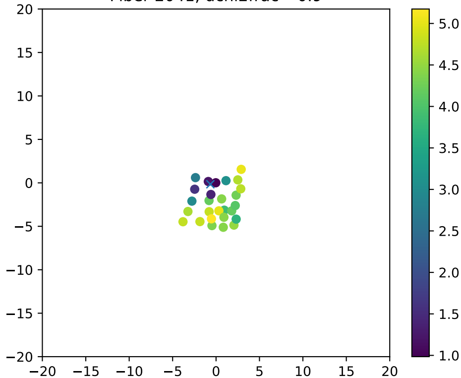
Fiber 2041, dchi2frac= 0.9
