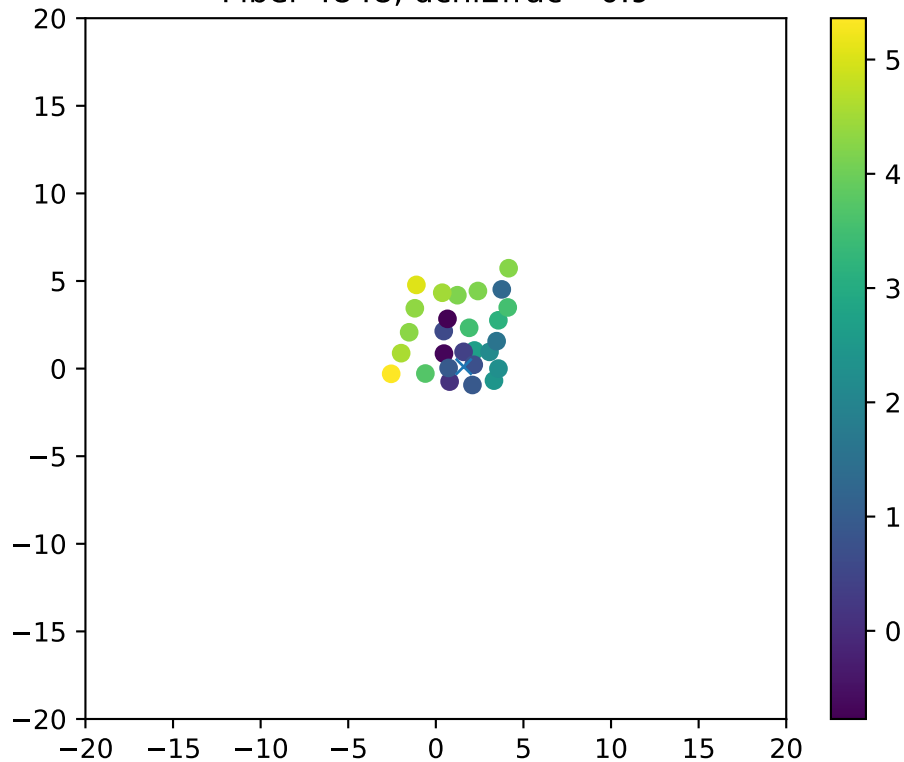
Fiber 4848, dchi2frac= 0.9
