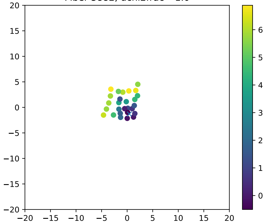
Fiber 3882, dchi2frac= 1.0
