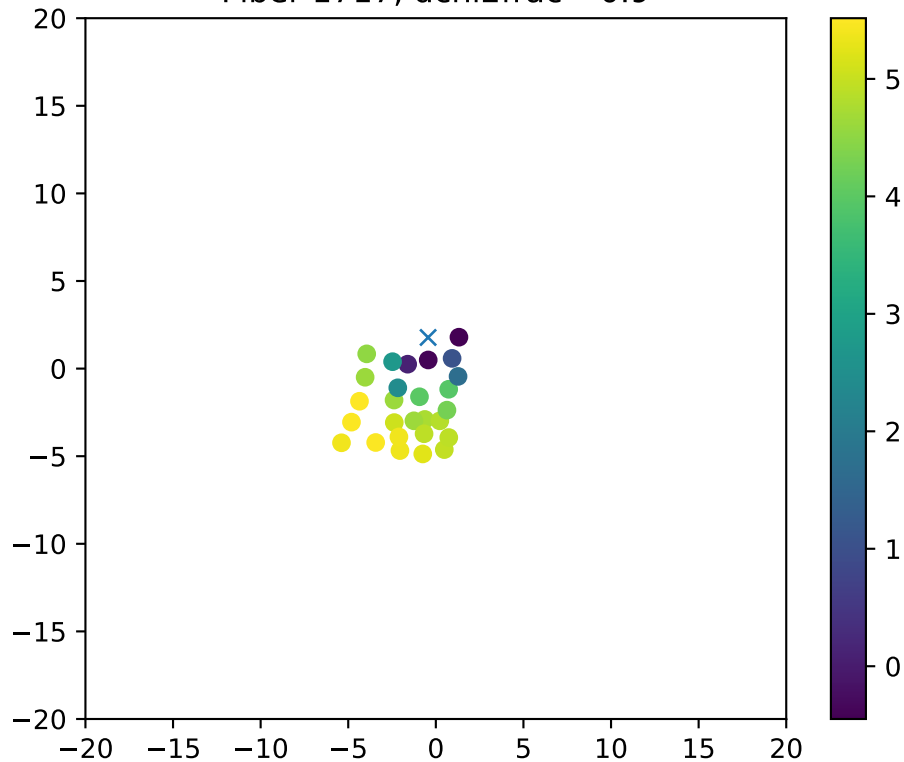
Fiber 1717, dchi2frac= 0.9
