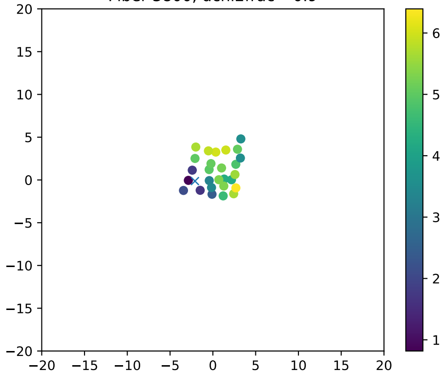
Fiber 3800, dchi2frac= 0.9
