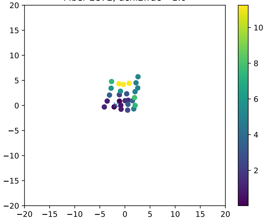
Fiber 2872, dchi2frac= 1.0
