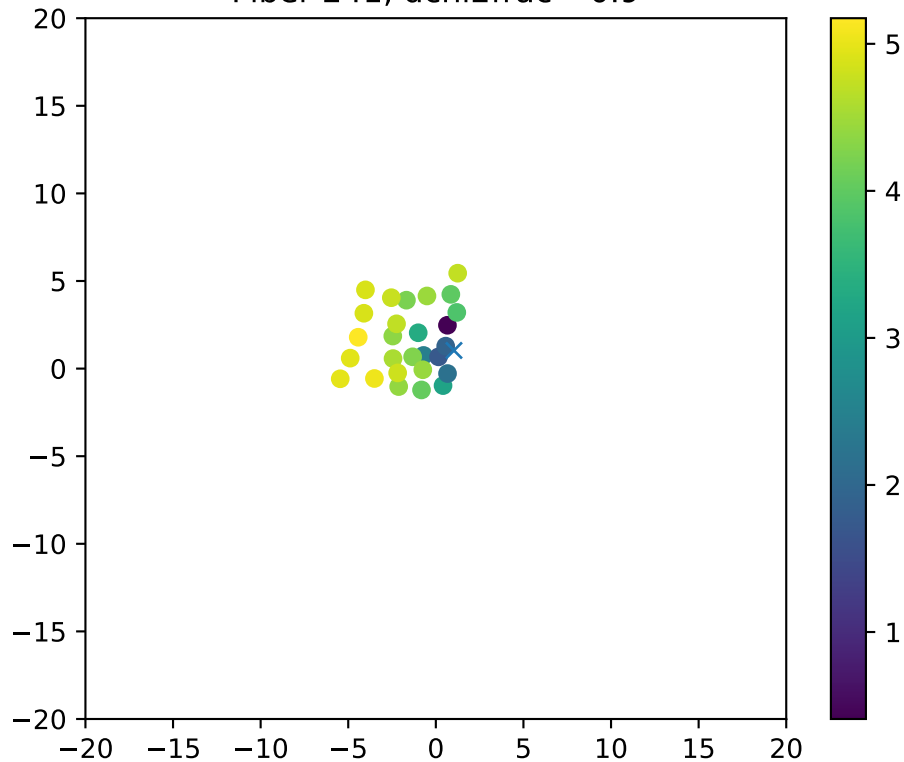
Fiber 241, dchi2frac= 0.9
