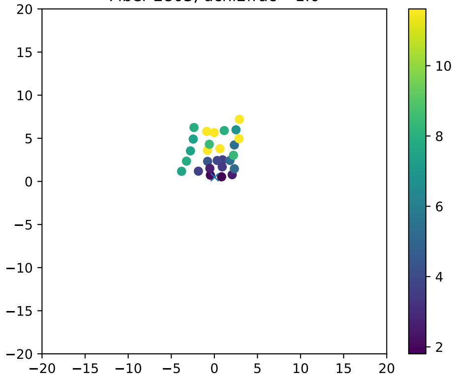
Fiber 2803, dchi2frac= 1.0
