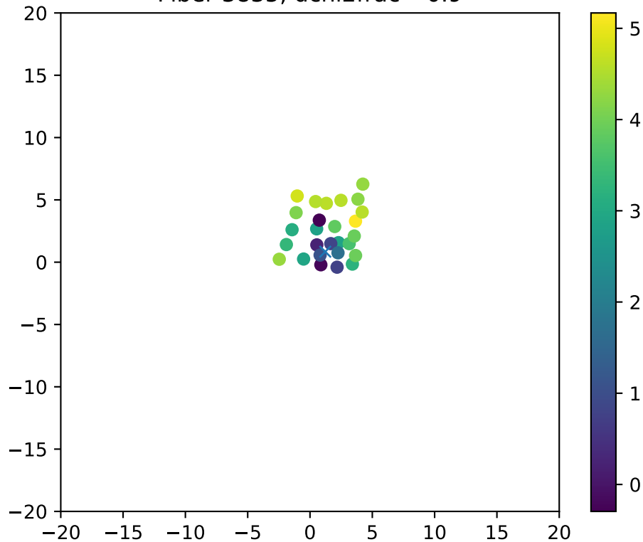
Fiber 3835, dchi2frac= 0.9
