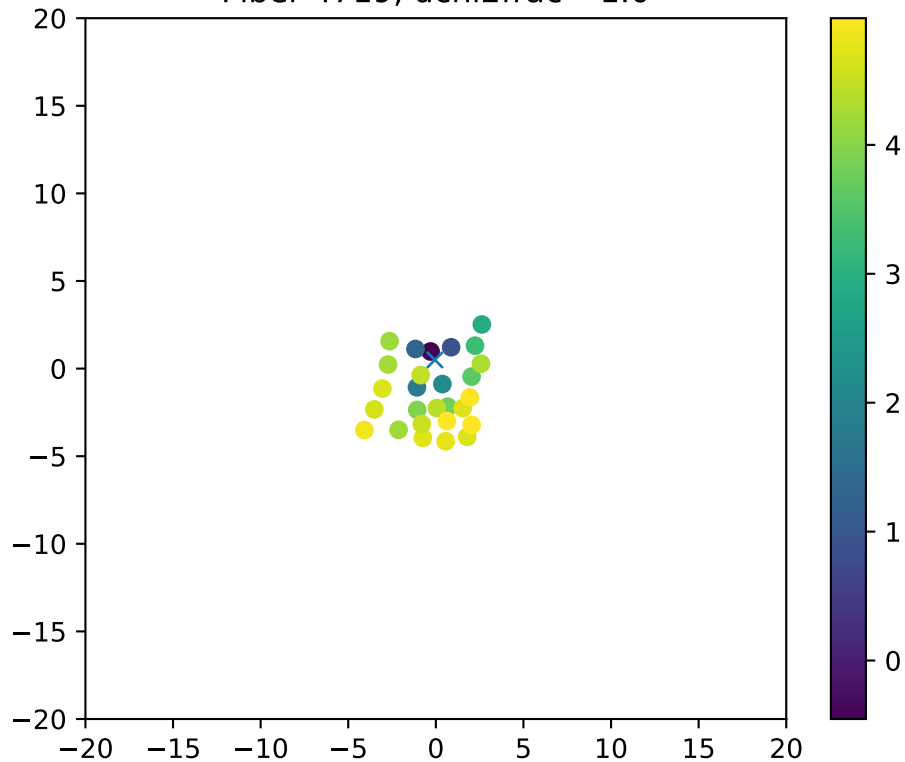
Fiber 4719, dchi2frac= 1.0
