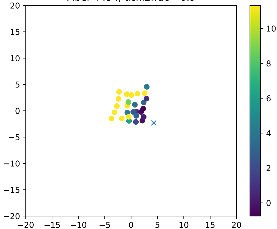
Fiber 4434, dchi2frac= 0.9
