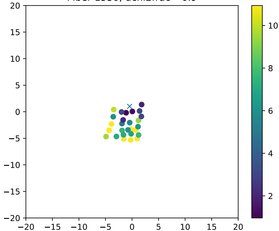
Fiber 1530, dchi2frac= 0.9
