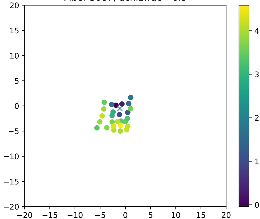
Fiber 3087, dchi2frac= 0.9
