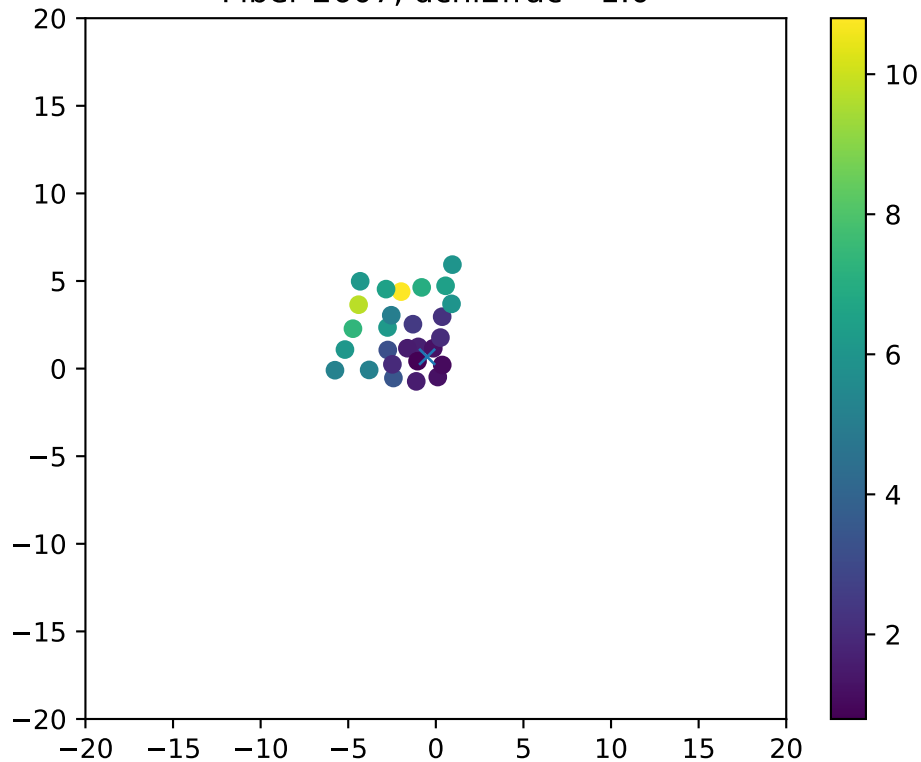
Fiber 2607, dchi2frac= 1.0
