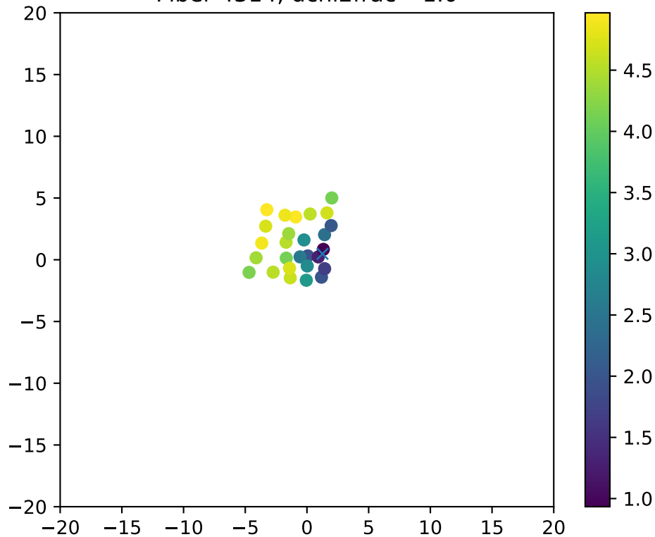
Fiber 4314, dchi2frac= 1.0
