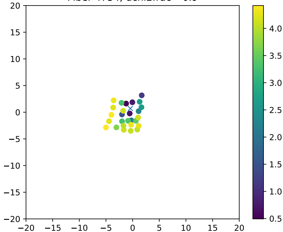
Fiber 4734, dchi2frac= 0.9
