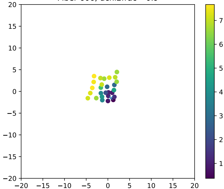
Fiber 606, dchi2frac= 0.9
