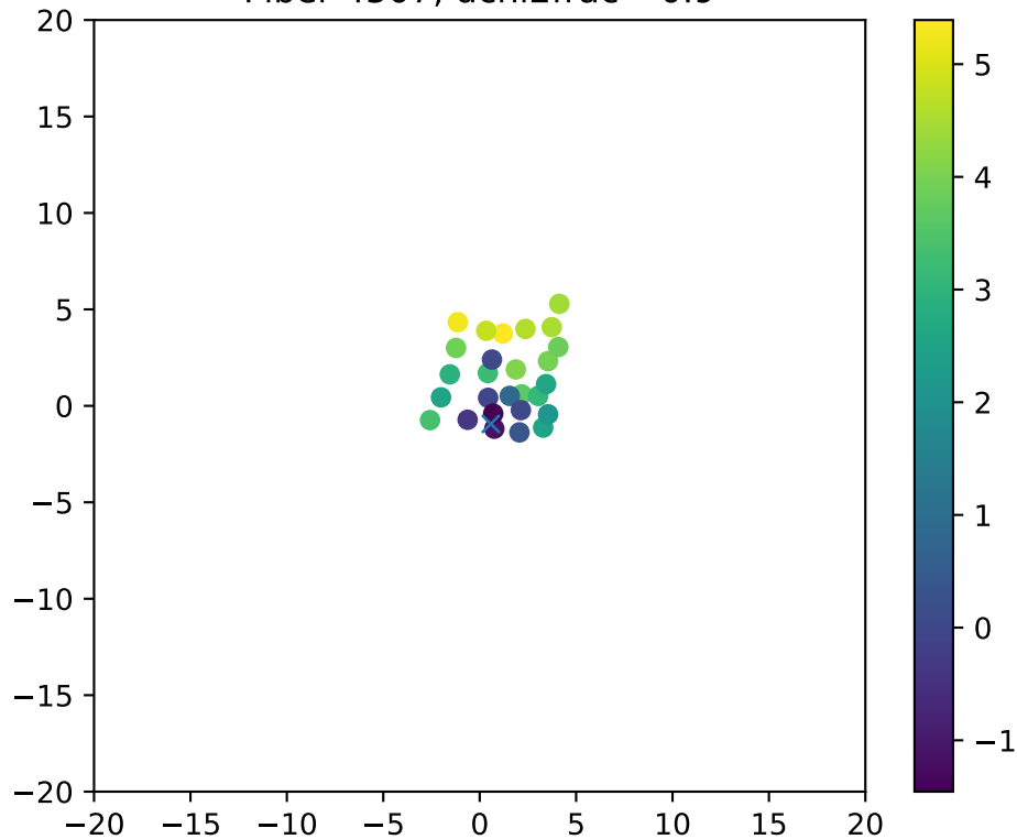
Fiber 4507, dchi2frac= 0.9
