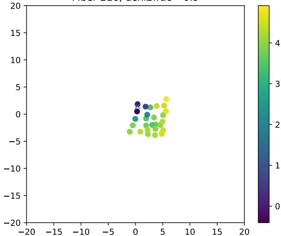
Fiber 216, dchi2frac= 0.9
