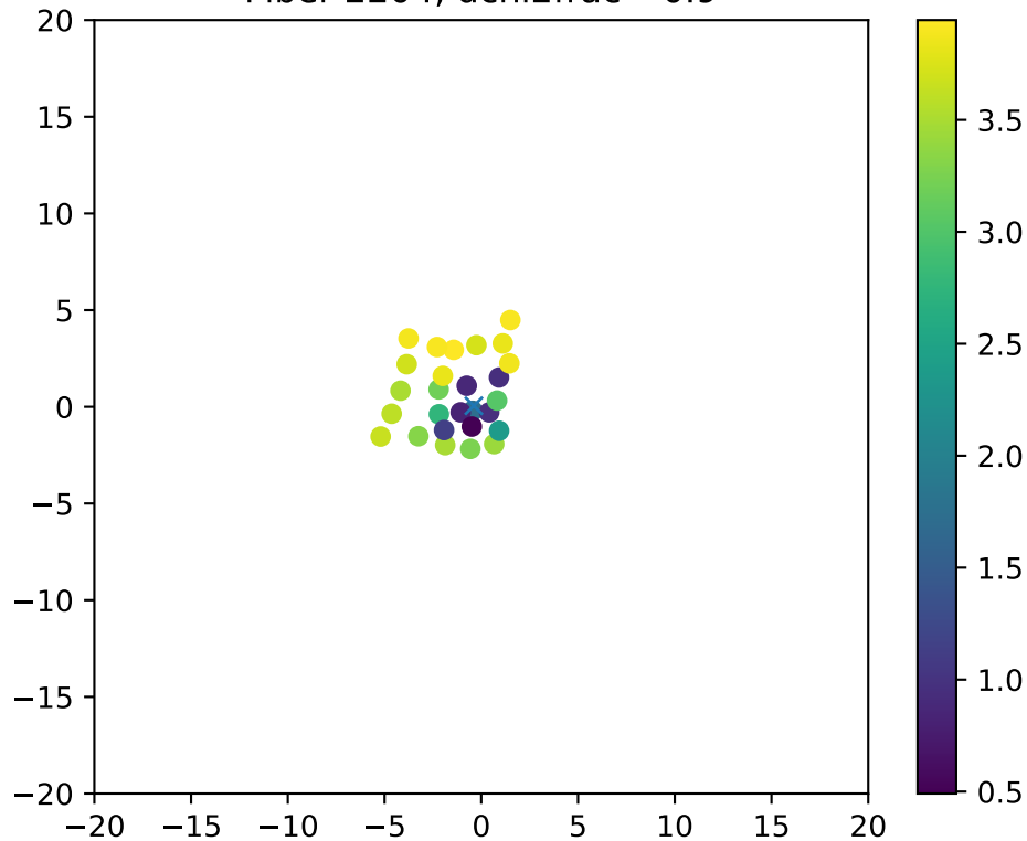
Fiber 2204, dchi2frac= 0.9
