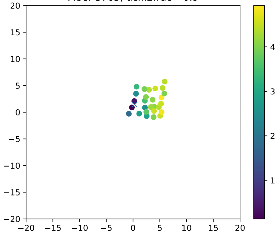
Fiber 3765, dchi2frac= 0.9
