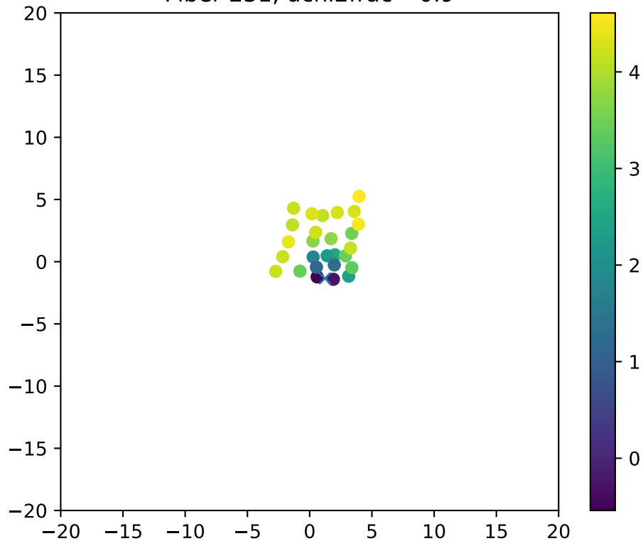
Fiber 231, dchi2frac= 0.9
