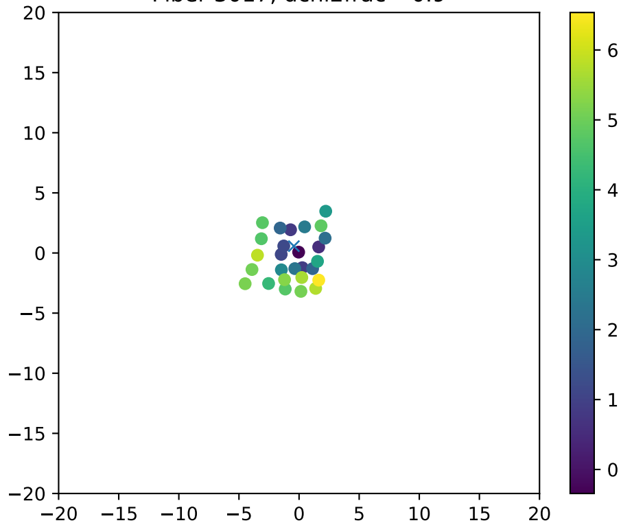
Fiber 3017, dchi2frac= 0.9
