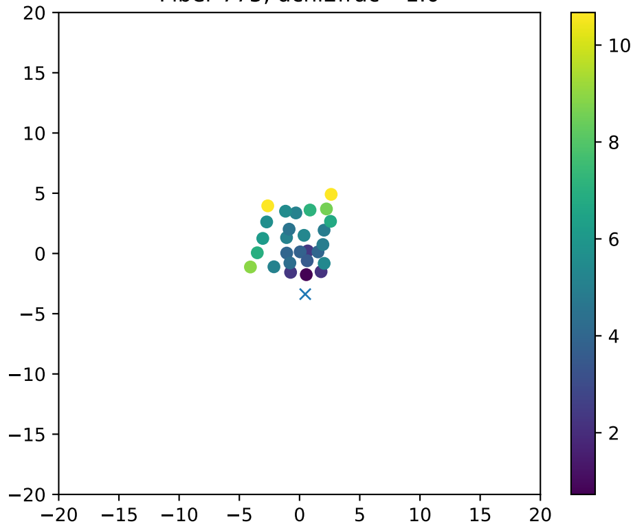
Fiber 775, dchi2frac= 1.0
