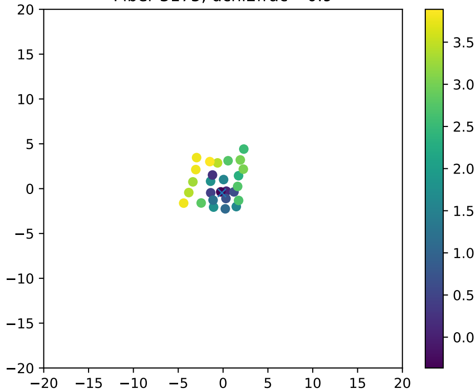
Fiber 3175, dchi2frac= 0.9
