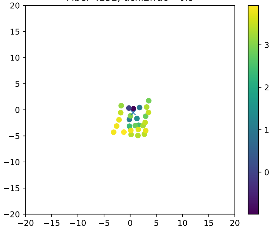
Fiber 4252, dchi2frac= 0.9
