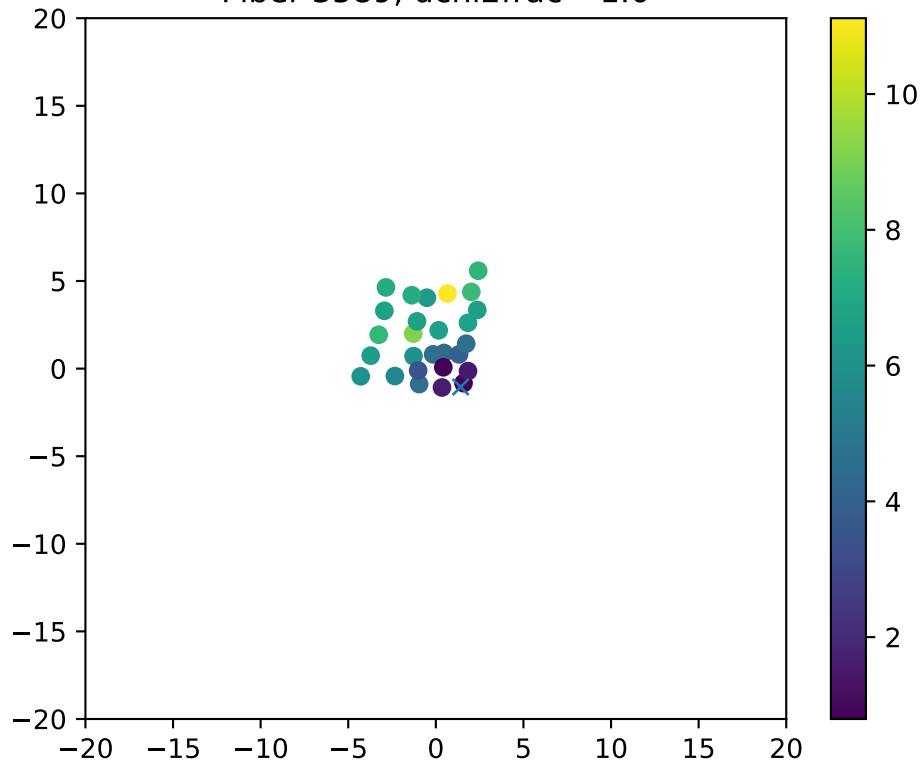
Fiber 3589, dchi2frac= 1.0
