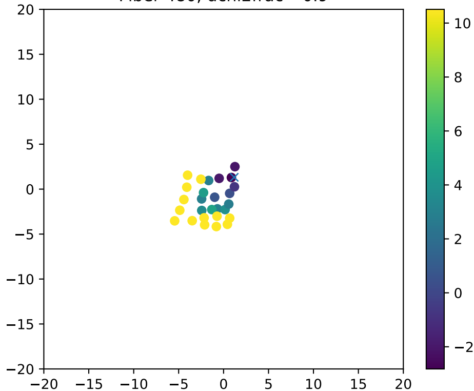
Fiber 480, dchi2frac= 0.9
