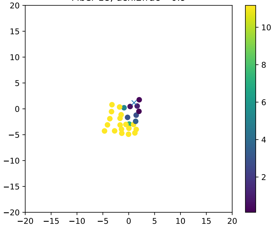
Fiber 18, dchi2frac= 0.9
