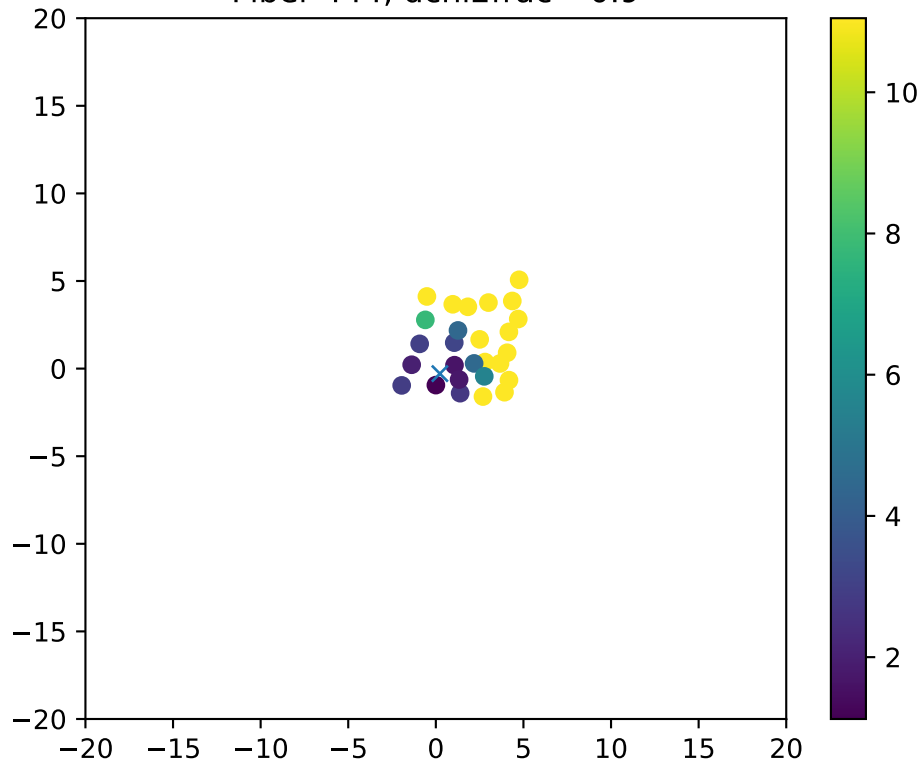
Fiber 444, dchi2frac= 0.9
