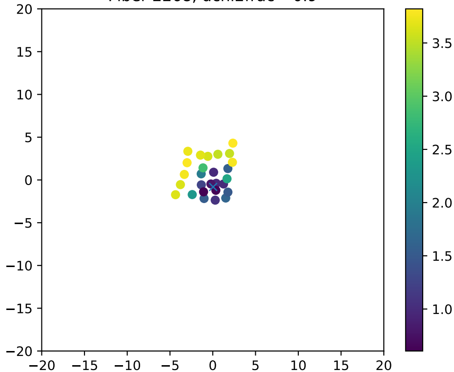
Fiber 2268, dchi2frac= 0.9
