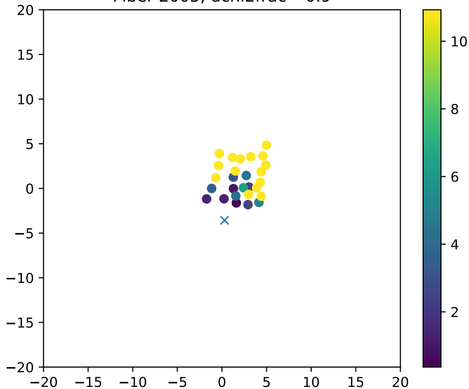
Fiber 2005, dchi2frac= 0.9
