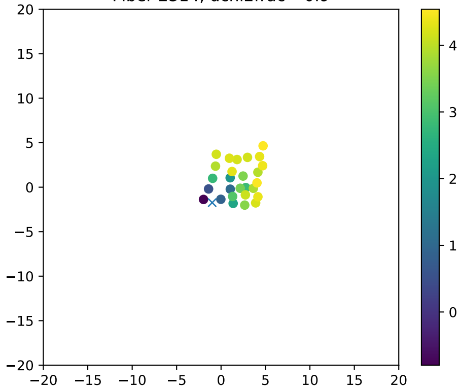
Fiber 2314, dchi2frac= 0.9
