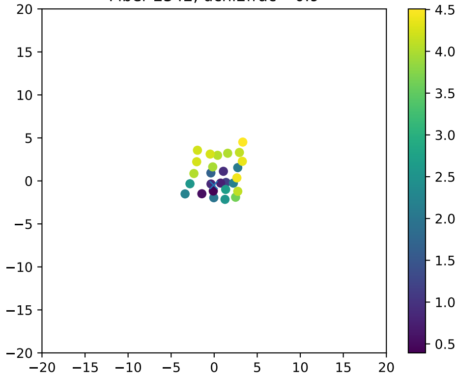
Fiber 2342, dchi2frac= 0.9
