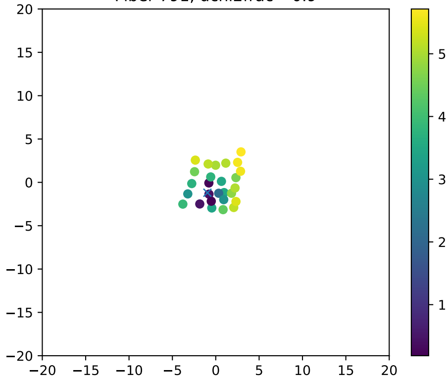
Fiber 791, dchi2frac= 0.9
