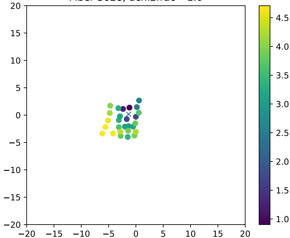
Fiber 3628, dchi2frac= 1.0
