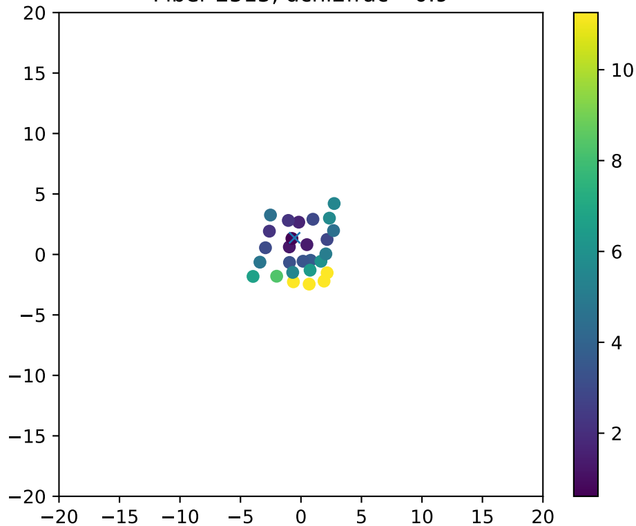
Fiber 2515, dchi2frac= 0.9
