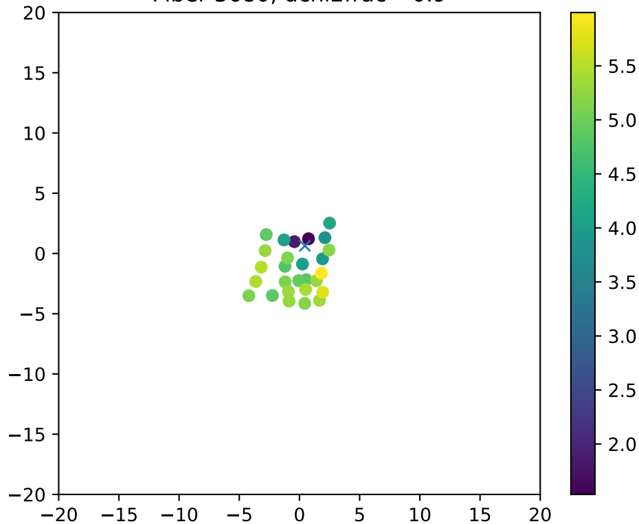
Fiber 3680, dchi2frac= 0.9
