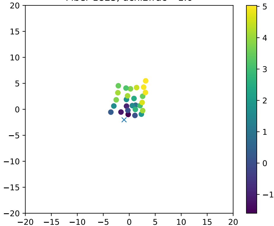
Fiber 1823, dchi2frac= 1.0
