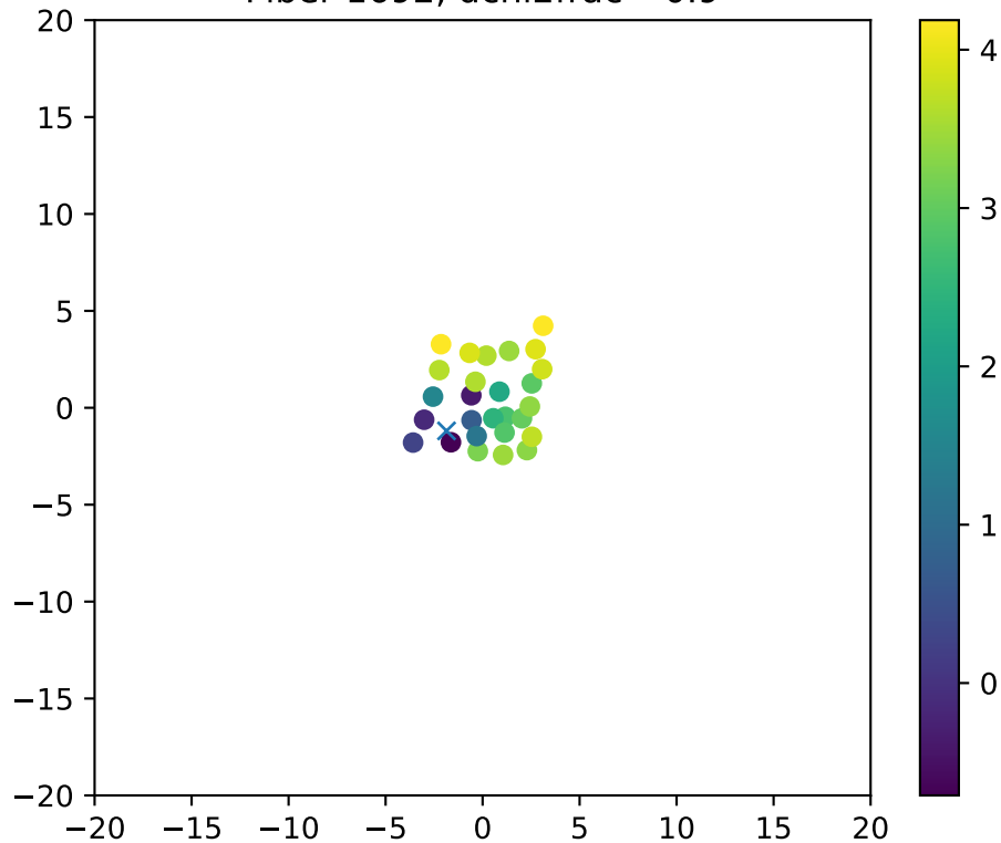
Fiber 1692, dchi2frac= 0.9
