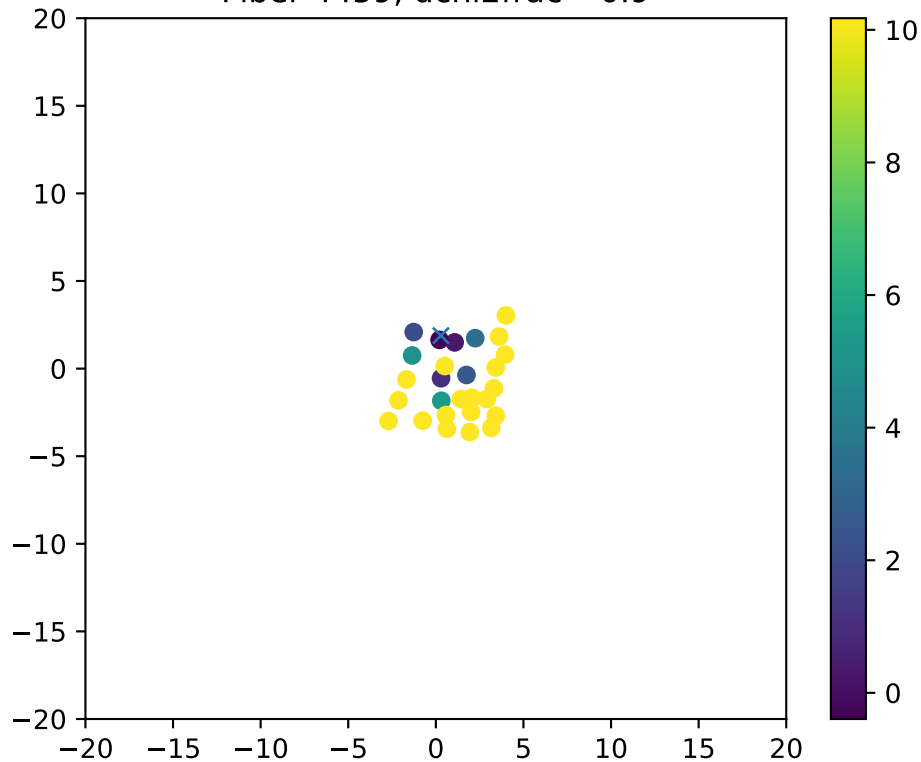
Fiber 4459, dchi2frac= 0.9
