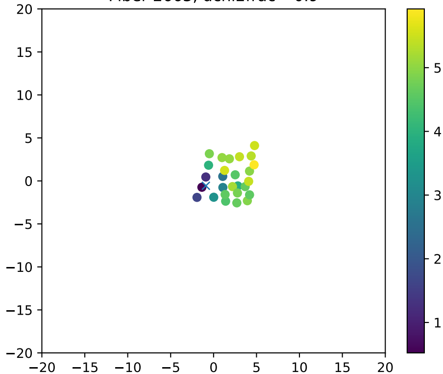
Fiber 2663, dchi2frac= 0.9
