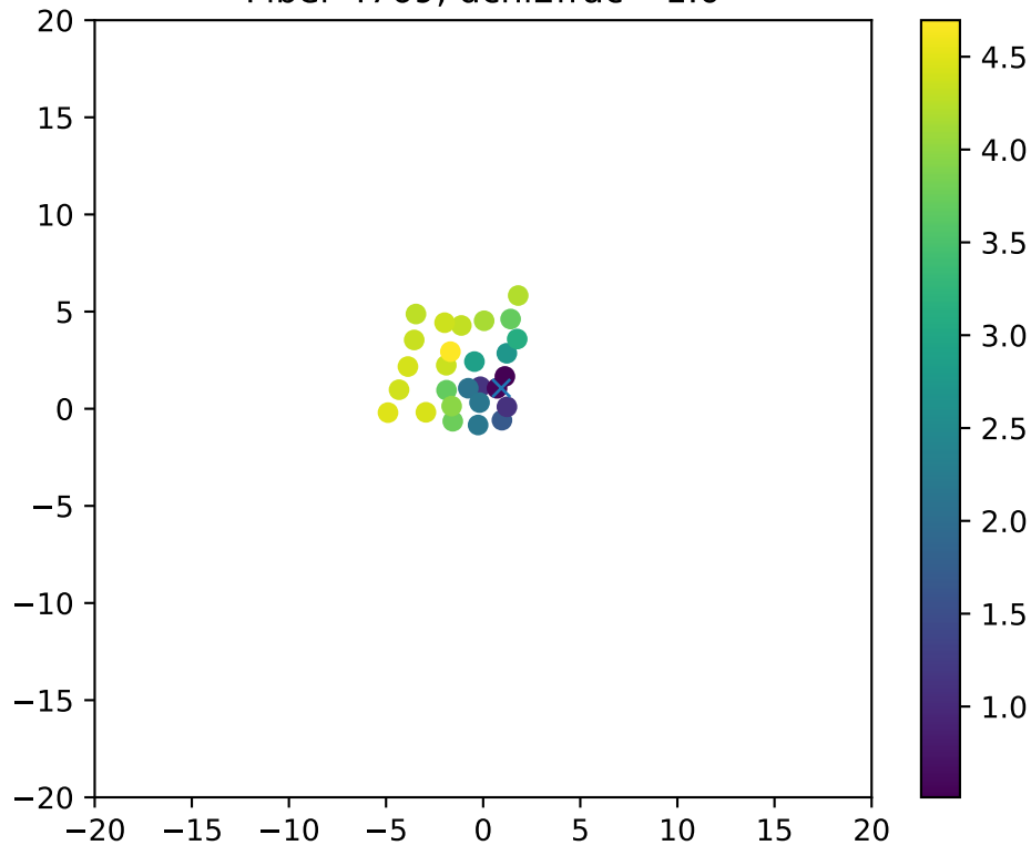
Fiber 4769, dchi2frac= 1.0
