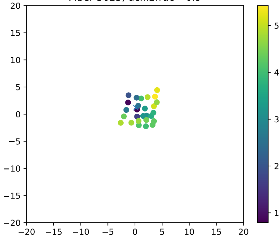
Fiber 3623, dchi2frac= 0.9
