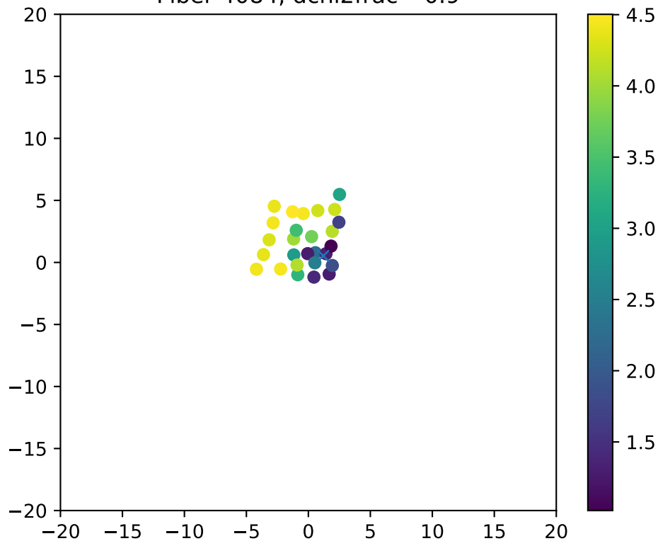
Fiber 4084, dchi2frac= 0.9
