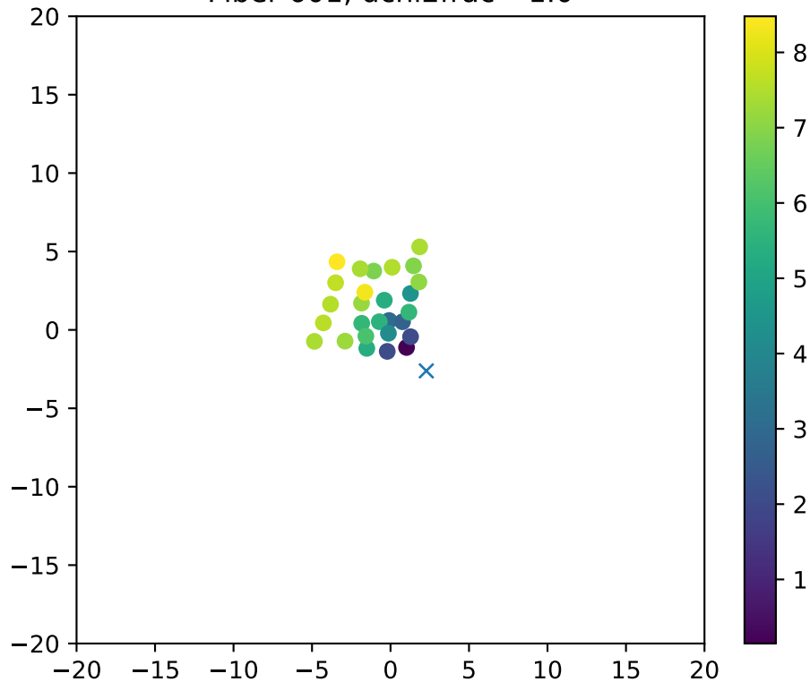
Fiber 601, dchi2frac= 1.0
