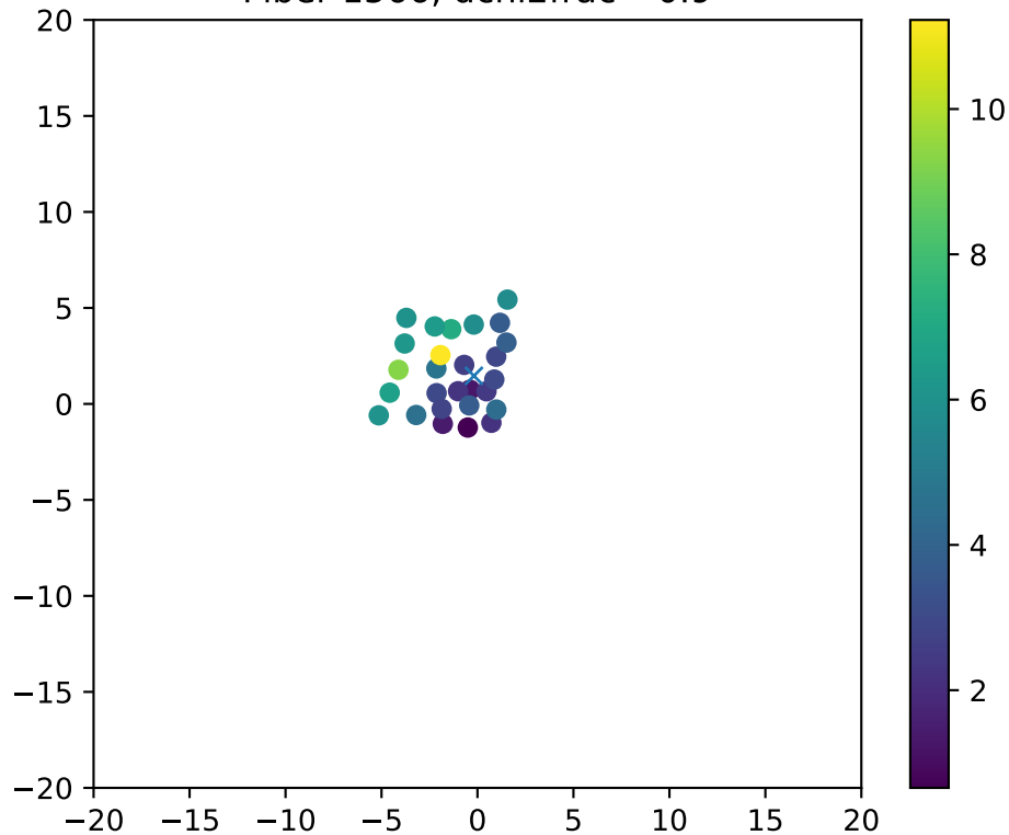
Fiber 1566, dchi2frac= 0.9
