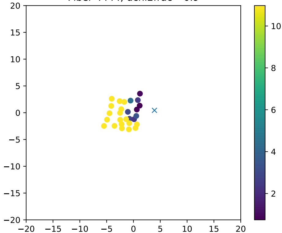
Fiber 4444, dchi2frac= 0.9
