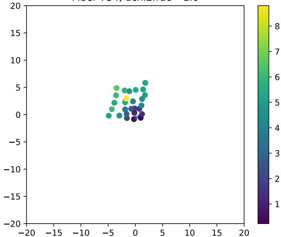
Fiber 734, dchi2frac= 1.0
