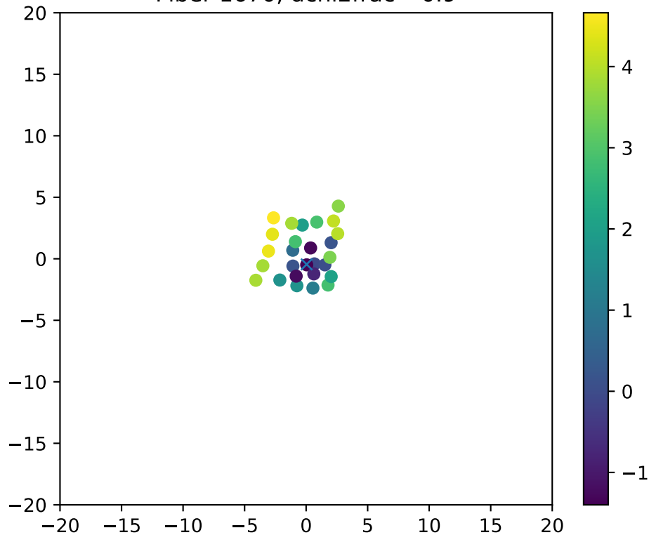
Fiber 1670, dchi2frac= 0.9
