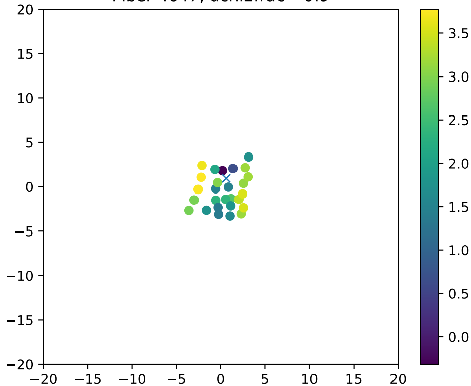
Fiber 4647, dchi2frac= 0.9
