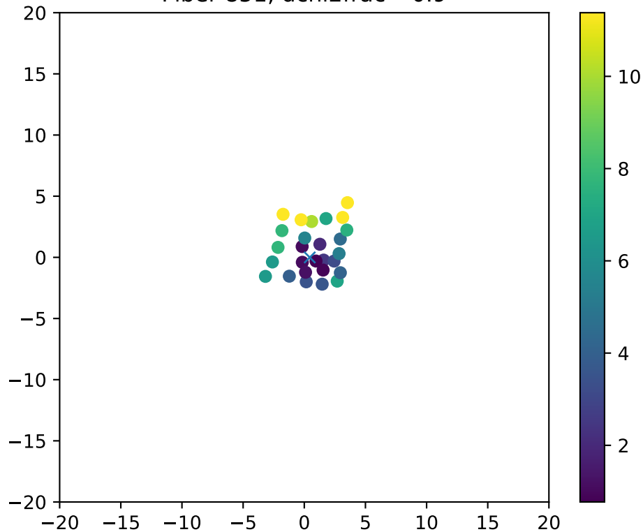
Fiber 851, dchi2frac= 0.9
