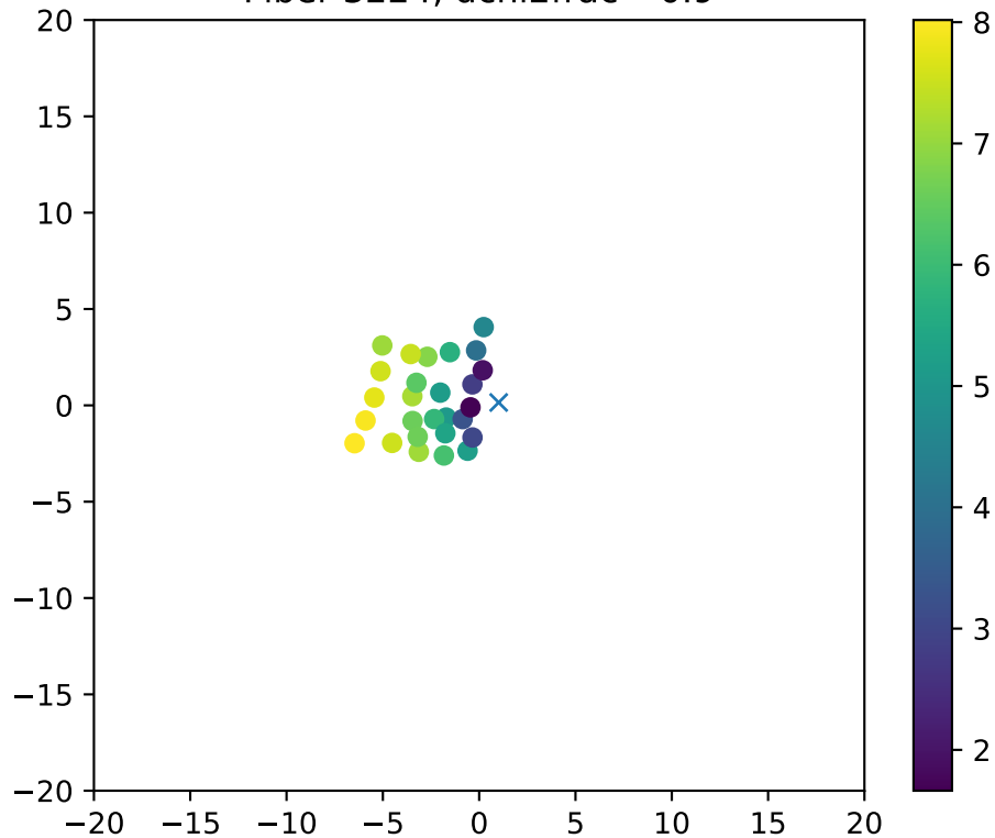
Fiber 3224, dchi2frac= 0.9
