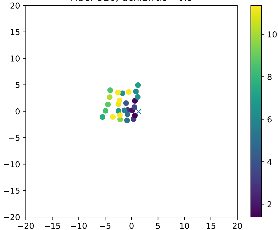
Fiber 526, dchi2frac= 0.9
