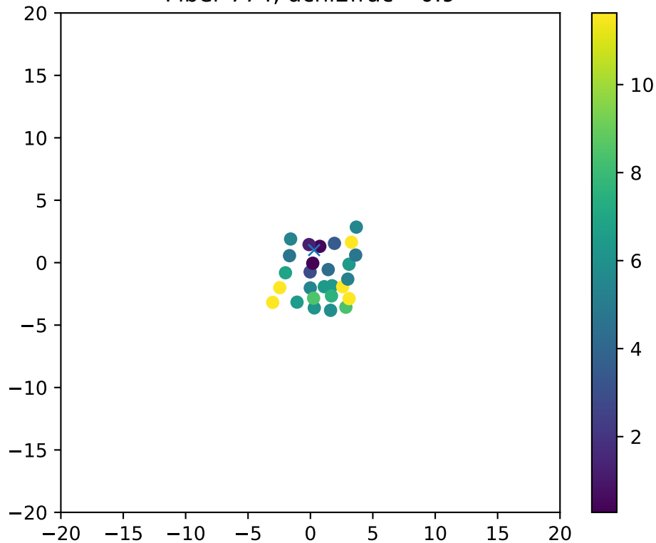
Fiber 774, dchi2frac= 0.9
