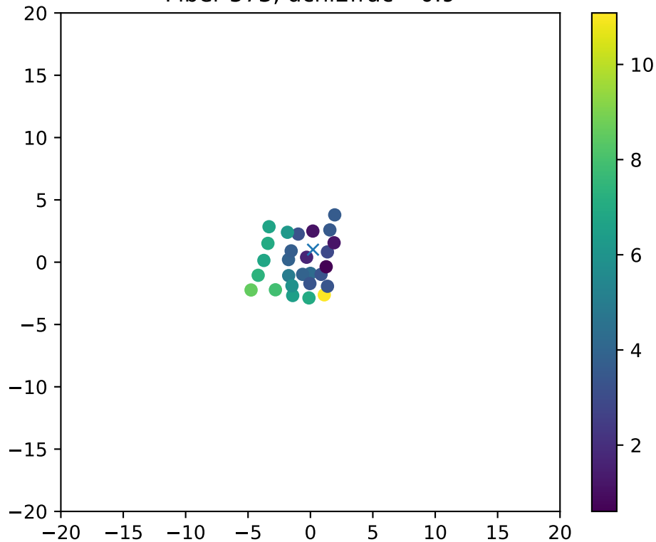
Fiber 573, dchi2frac= 0.9
