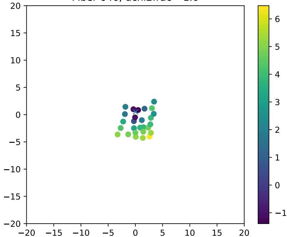
Fiber 646, dchi2frac= 1.0
