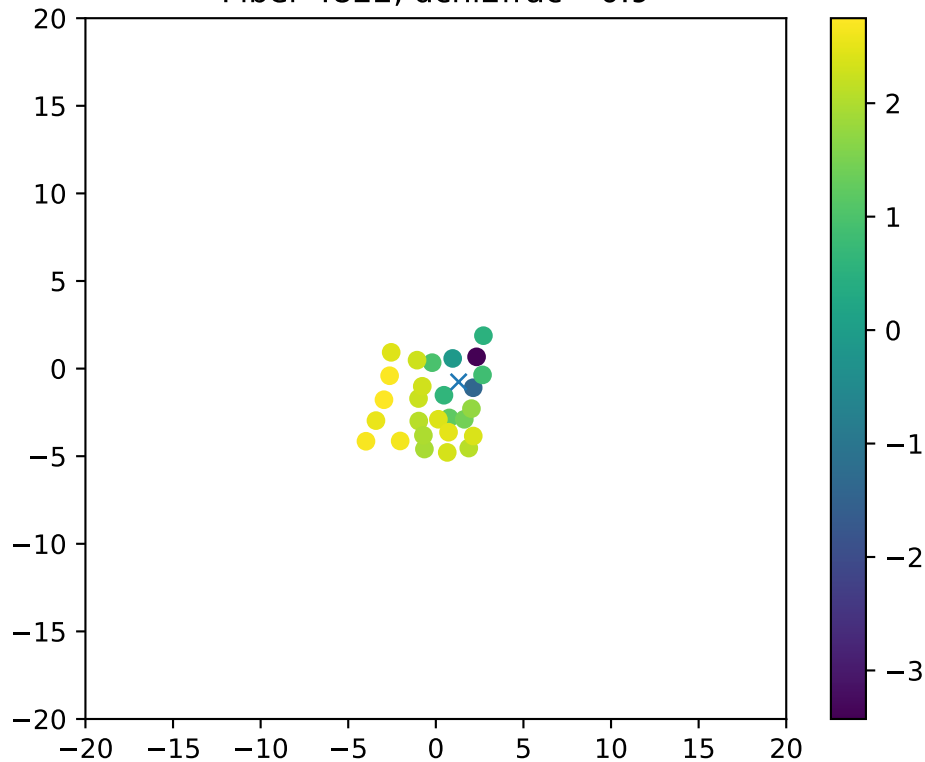
Fiber 4822, dchi2frac= 0.9
