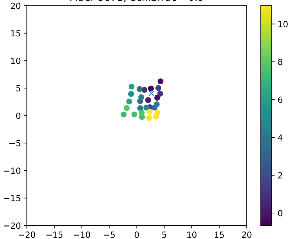
Fiber 3872, dchi2frac= 0.9
