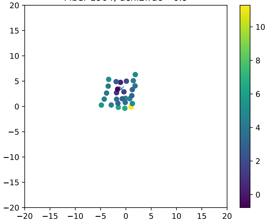
Fiber 1904, dchi2frac= 0.9
