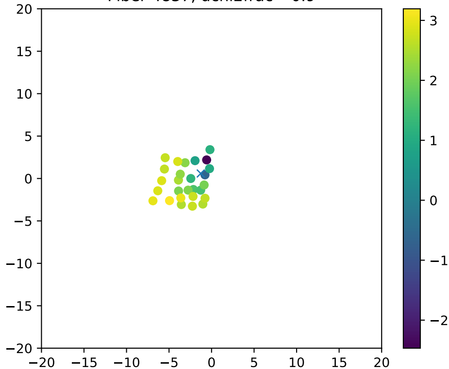
Fiber 4837, dchi2frac= 0.9
