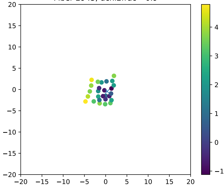
Fiber 2943, dchi2frac= 0.9
