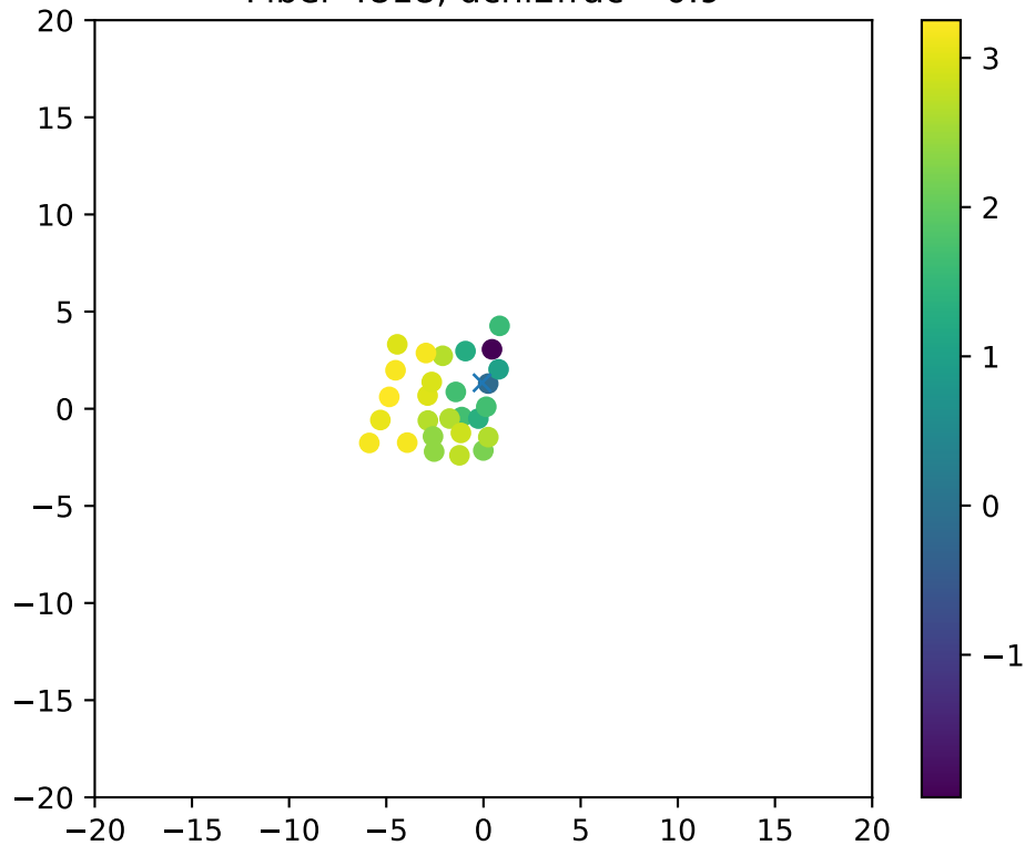
Fiber 4818, dchi2frac= 0.9
