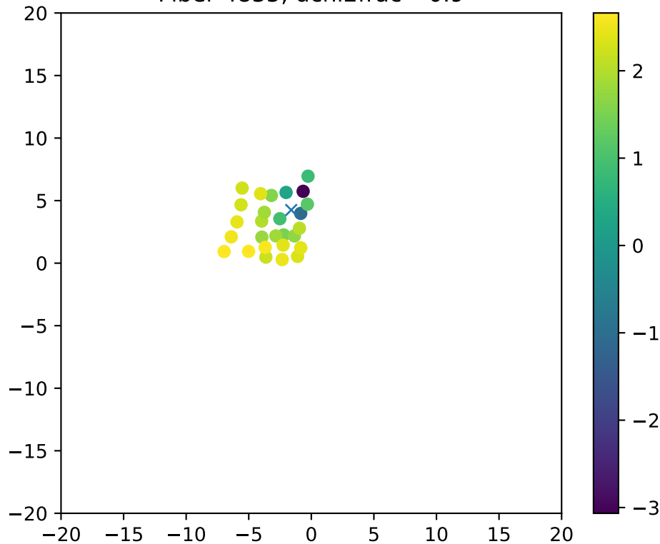
Fiber 4835, dchi2frac= 0.9
