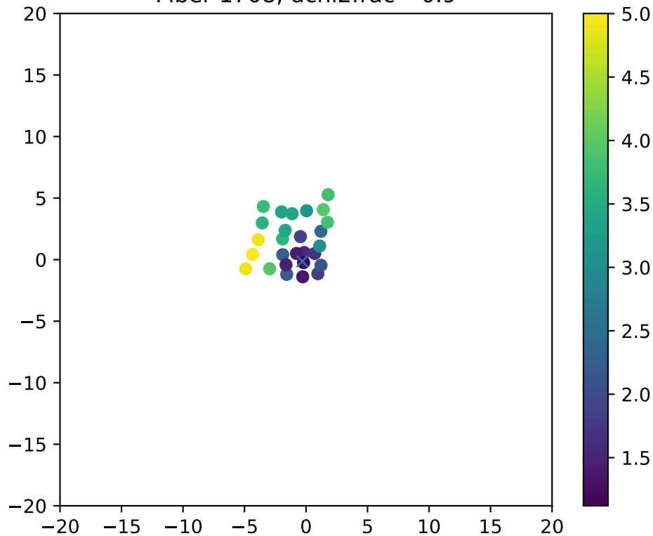
Fiber 1708, dchi2frac= 0.9
