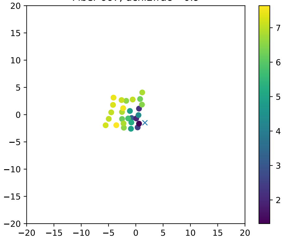
Fiber 667, dchi2frac= 0.9
