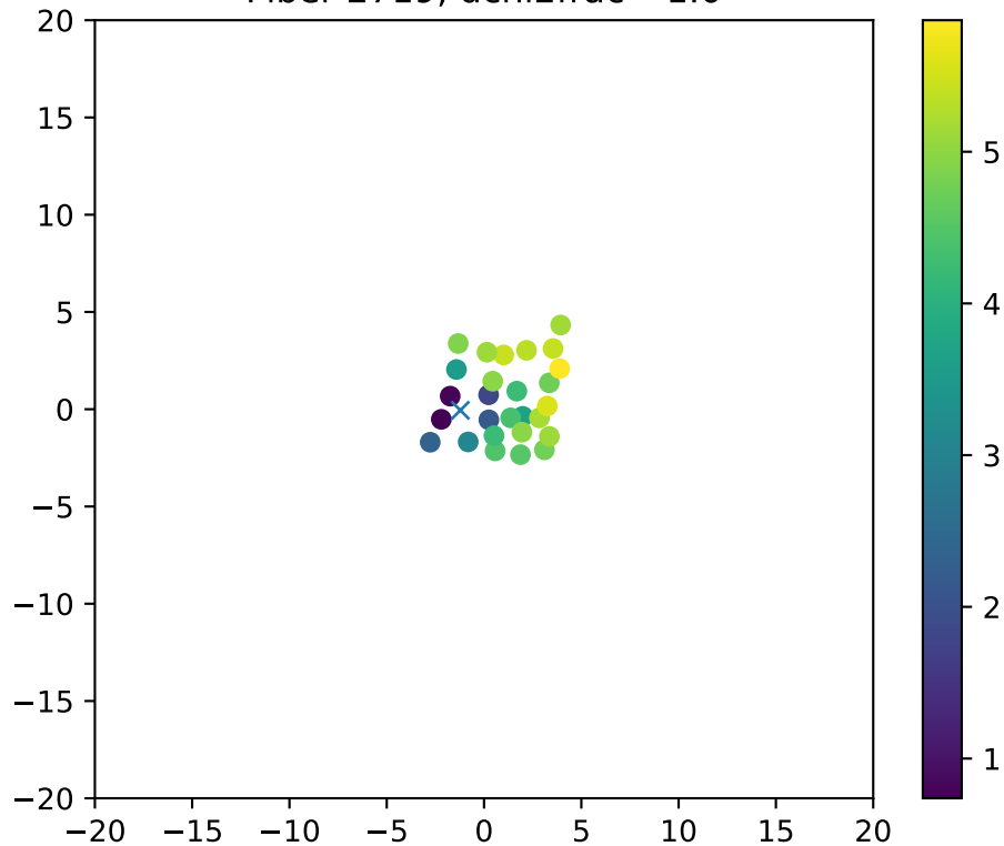
Fiber 2719, dchi2frac= 1.0
