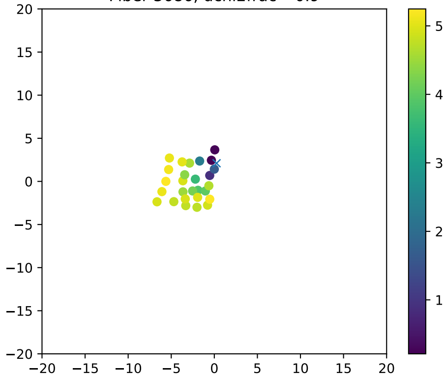
Fiber 3686, dchi2frac= 0.9
