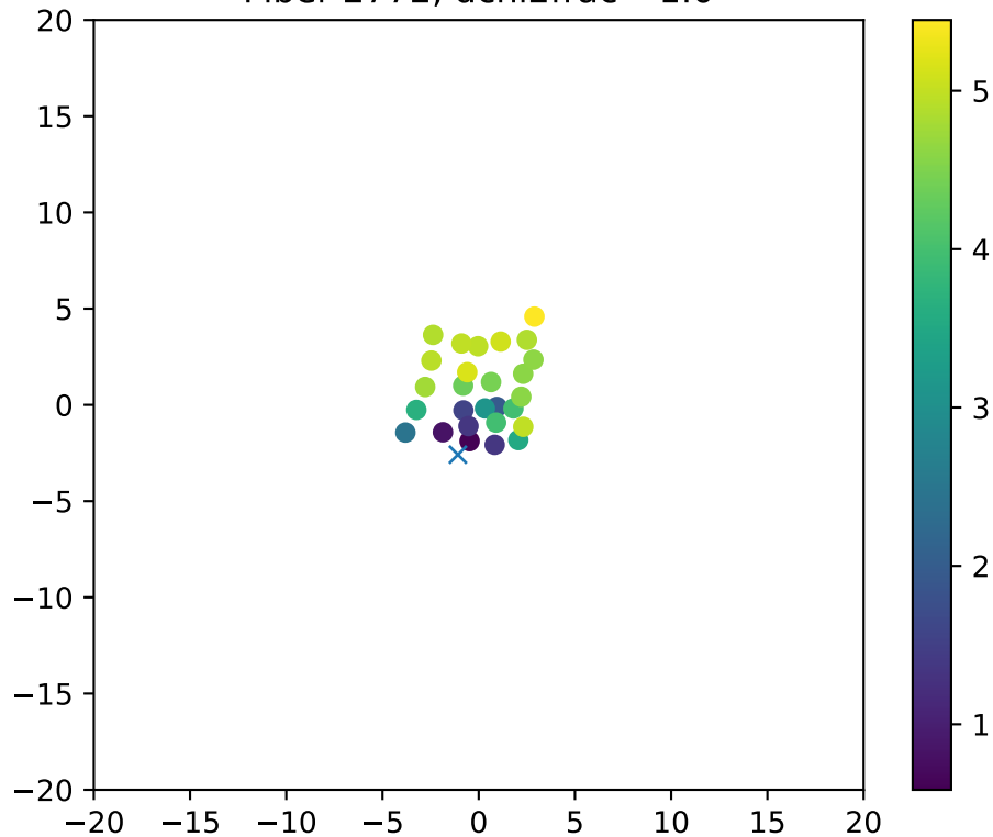
Fiber 2772, dchi2frac= 1.0
