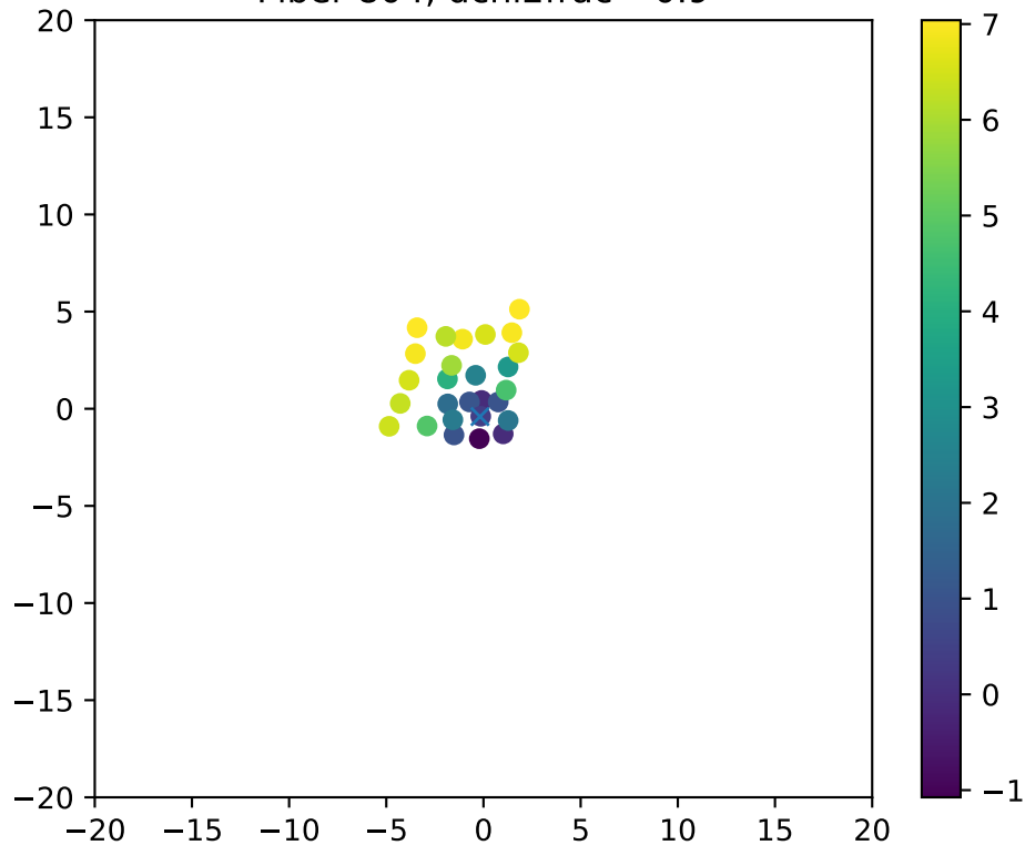
Fiber 804, dchi2frac= 0.9
