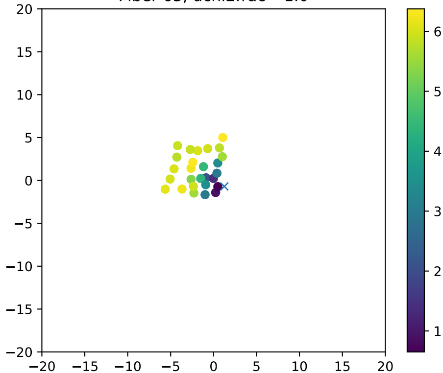
Fiber 63, dchi2frac= 1.0
