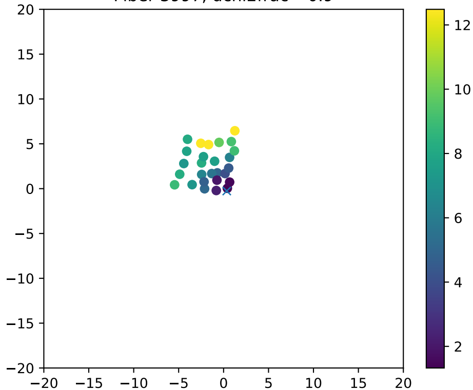
Fiber 3997, dchi2frac= 0.9
