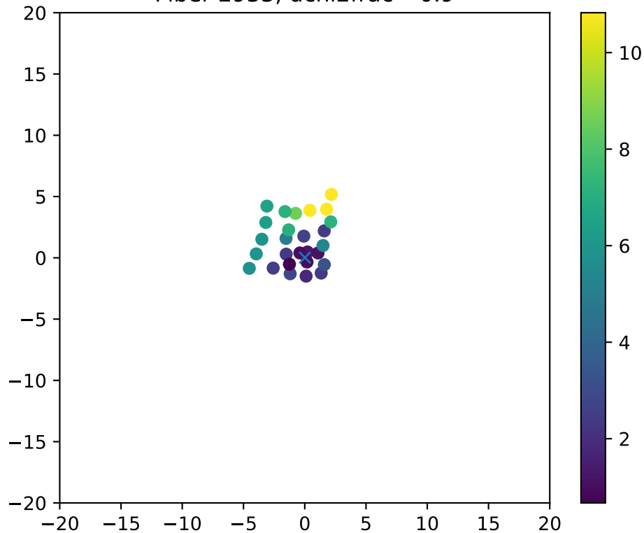
Fiber 2933, dchi2frac= 0.9
