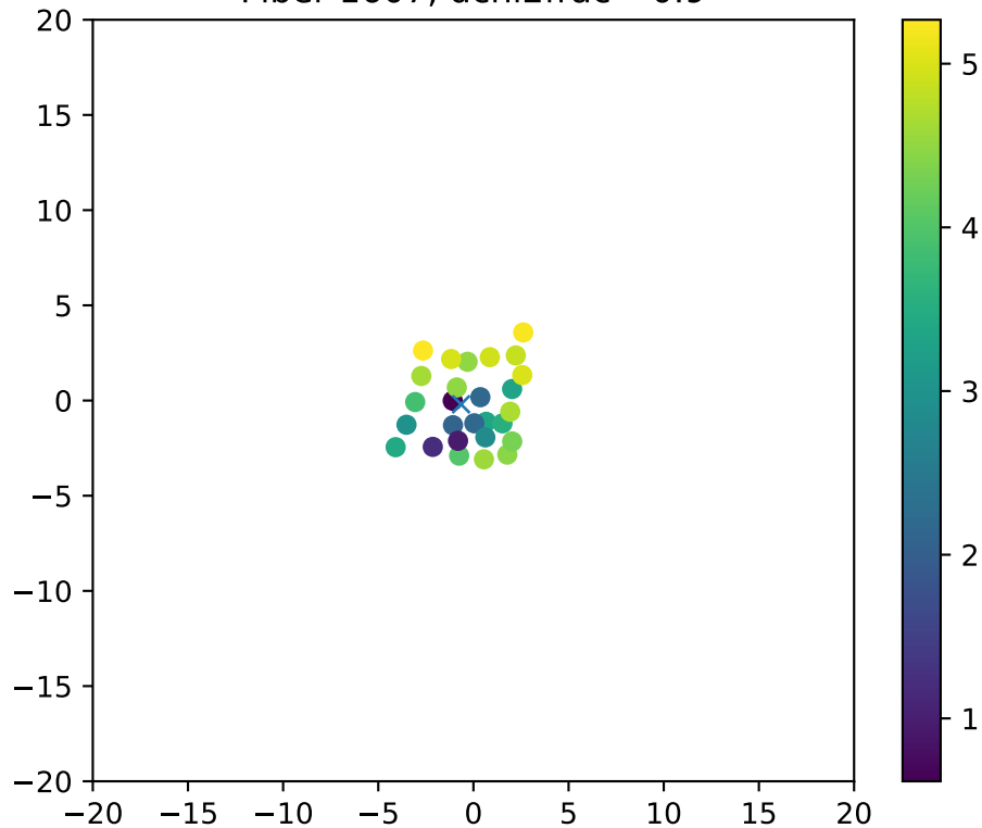
Fiber 1607, dchi2frac= 0.9
