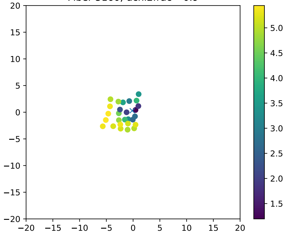
Fiber 3160, dchi2frac= 0.9
