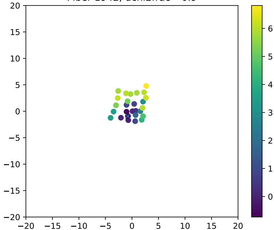
Fiber 1942, dchi2frac= 0.9
