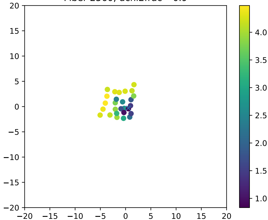
Fiber 2560, dchi2frac= 0.9
