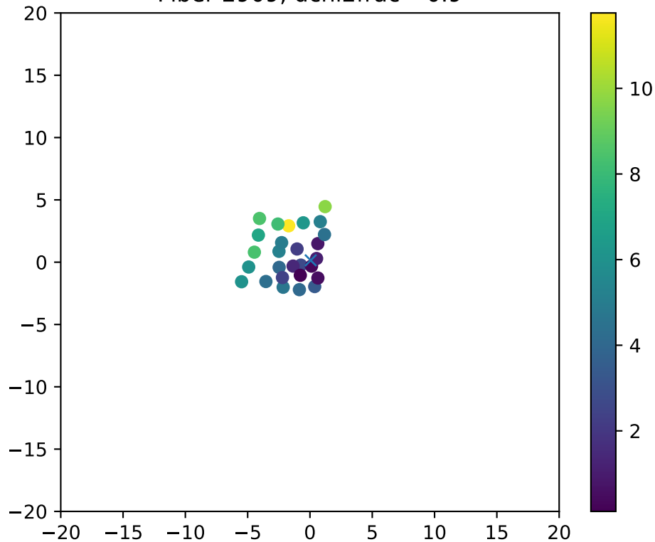
Fiber 2909, dchi2frac= 0.9
