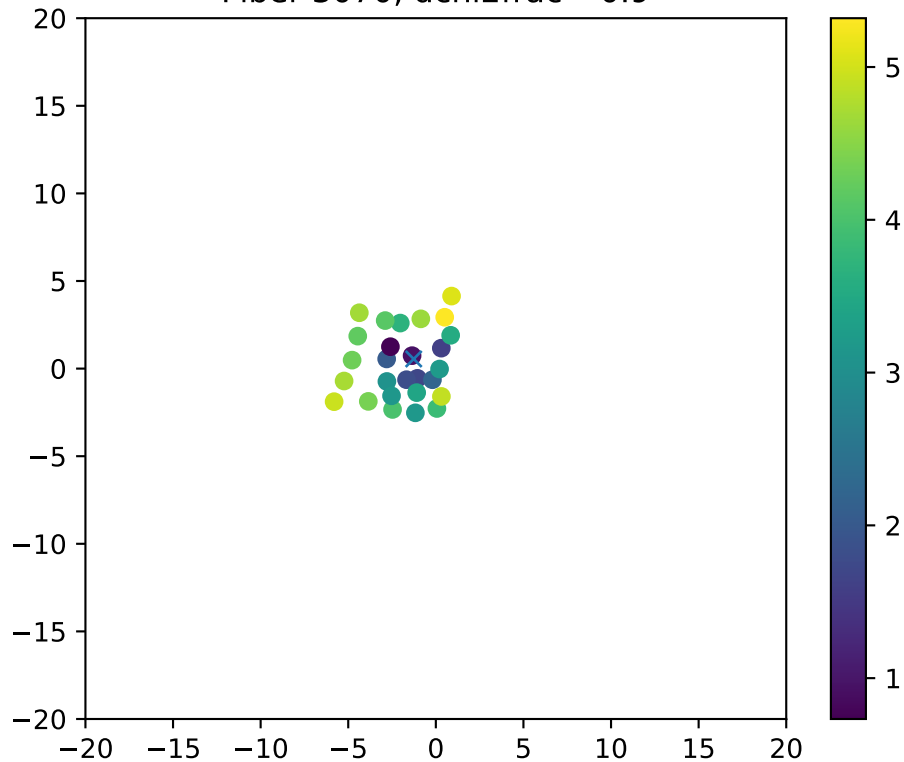
Fiber 3070, dchi2frac= 0.9
