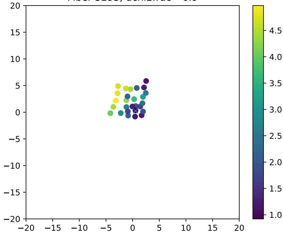
Fiber 3293, dchi2frac= 0.9
