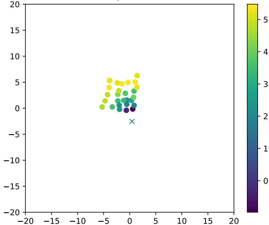
Fiber 2703, dchi2frac= 1.0
