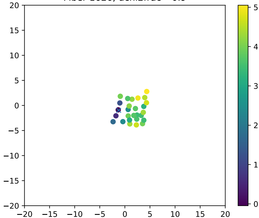
Fiber 1626, dchi2frac= 0.9
