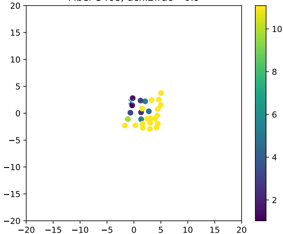
Fiber 3468, dchi2frac= 0.9
