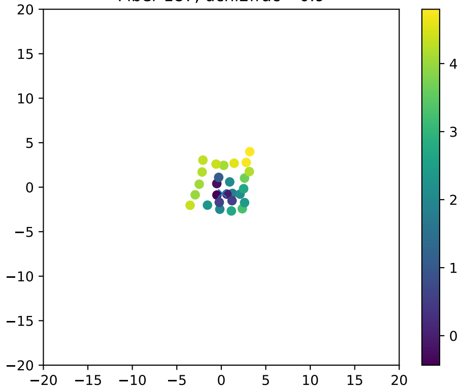
Fiber 187, dchi2frac= 0.9
