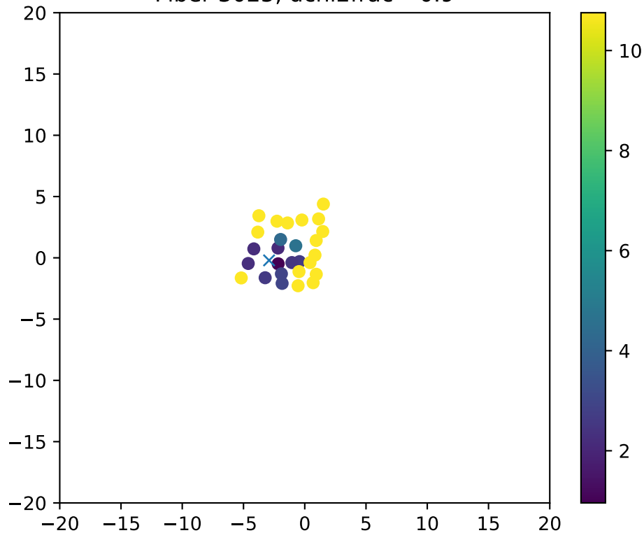
Fiber 3025, dchi2frac= 0.9
