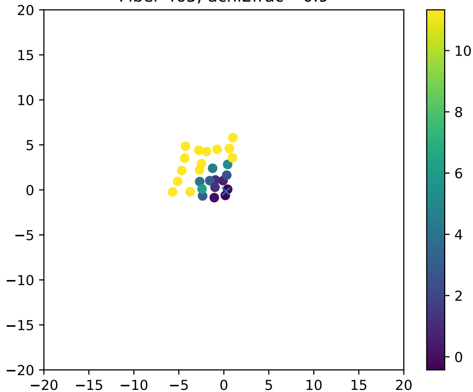
Fiber 465, dchi2frac= 0.9
