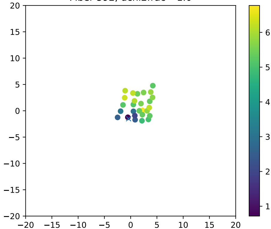
Fiber 592, dchi2frac= 1.0
