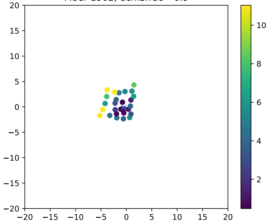
Fiber 1902, dchi2frac= 0.9
