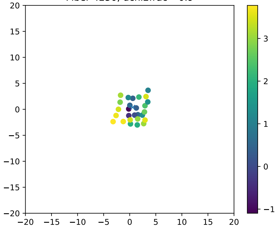
Fiber 4250, dchi2frac= 0.9
