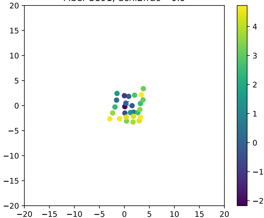
Fiber 3891, dchi2frac= 0.9
