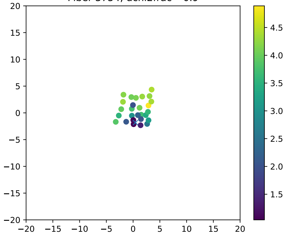
Fiber 3754, dchi2frac= 0.9
