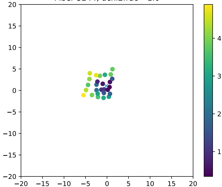
Fiber 3244, dchi2frac= 1.0
