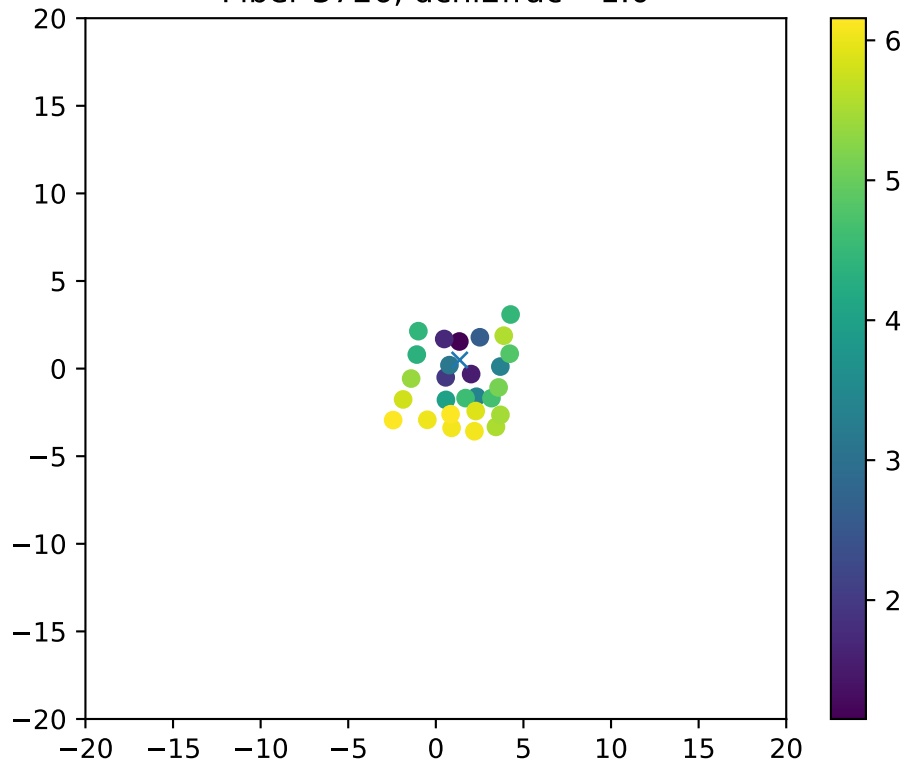
Fiber 3726, dchi2frac= 1.0
