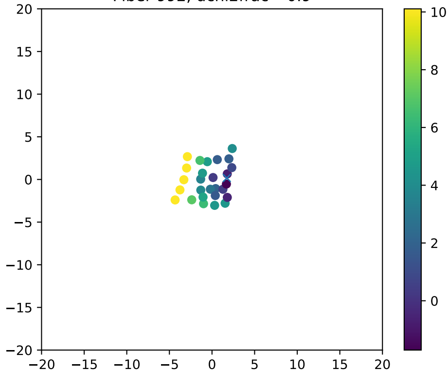
Fiber 992, dchi2frac= 0.9
