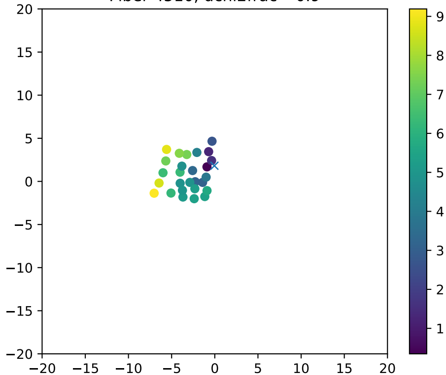
Fiber 4510, dchi2frac= 0.9
