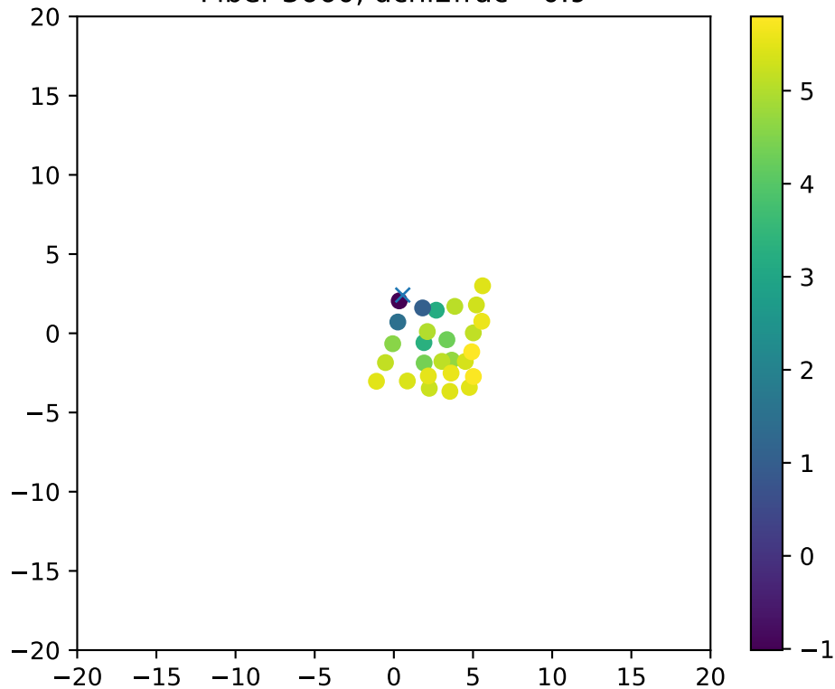
Fiber 3660, dchi2frac= 0.9
