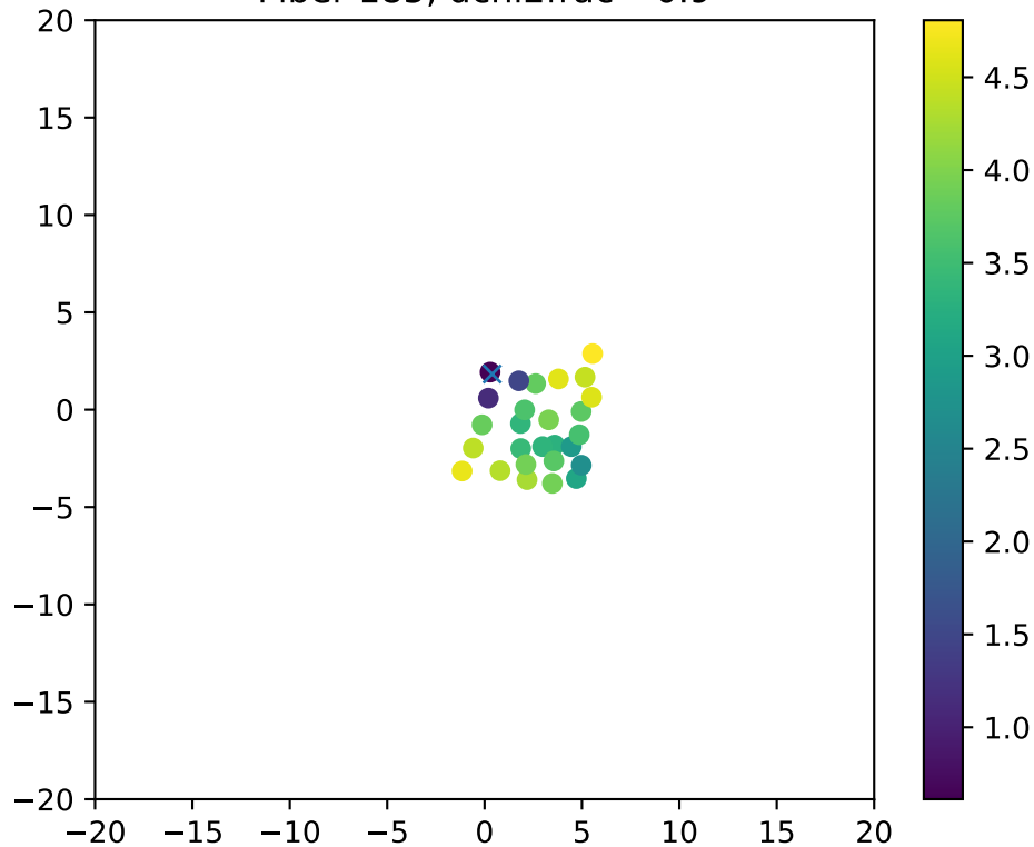
Fiber 185, dchi2frac= 0.9
