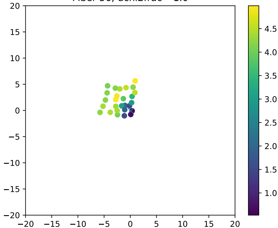
Fiber 56, dchi2frac= 1.0
