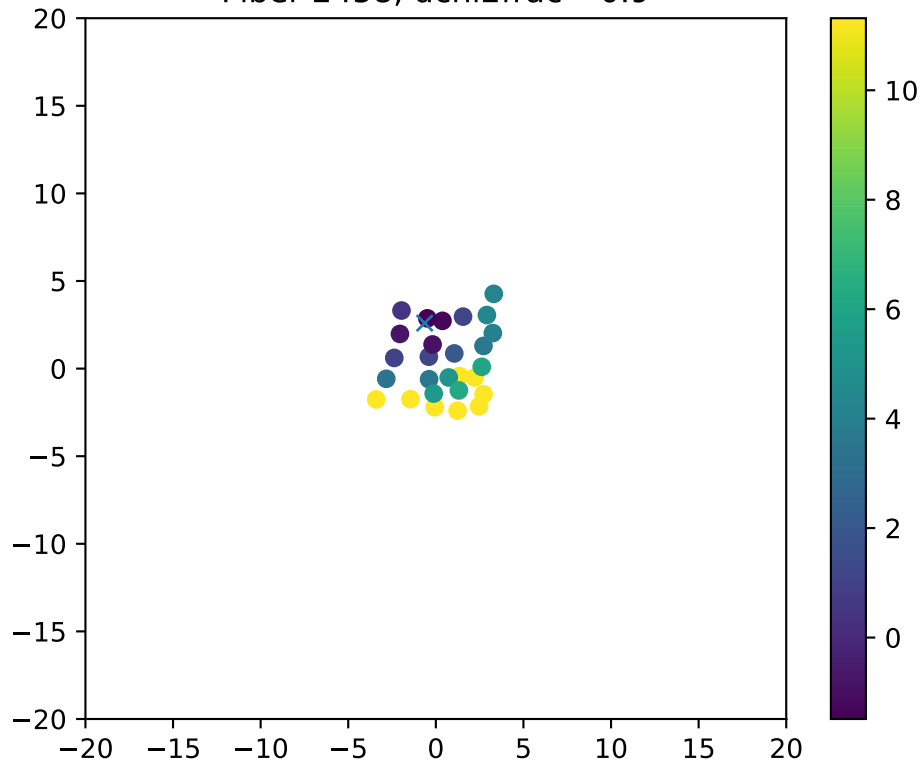
Fiber 2458, dchi2frac= 0.9
