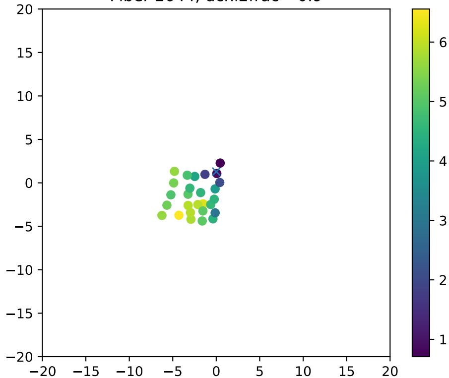
Fiber 2644, dchi2frac= 0.9
