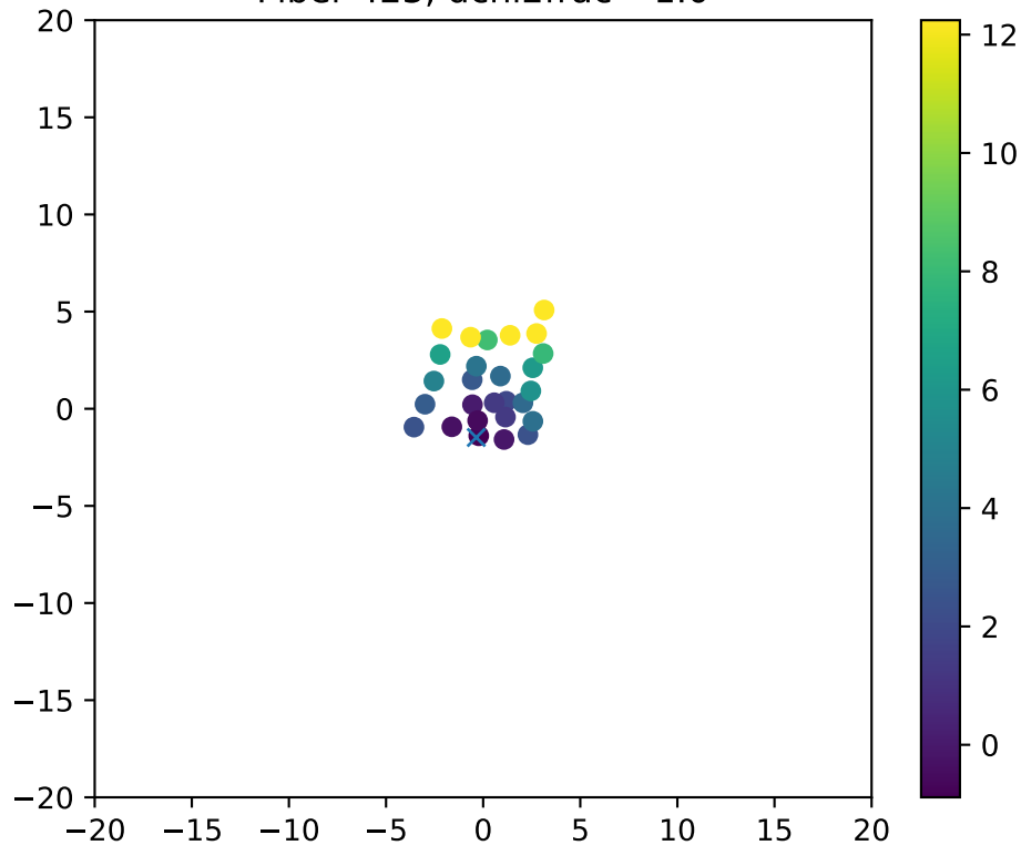
Fiber 423, dchi2frac= 1.0
