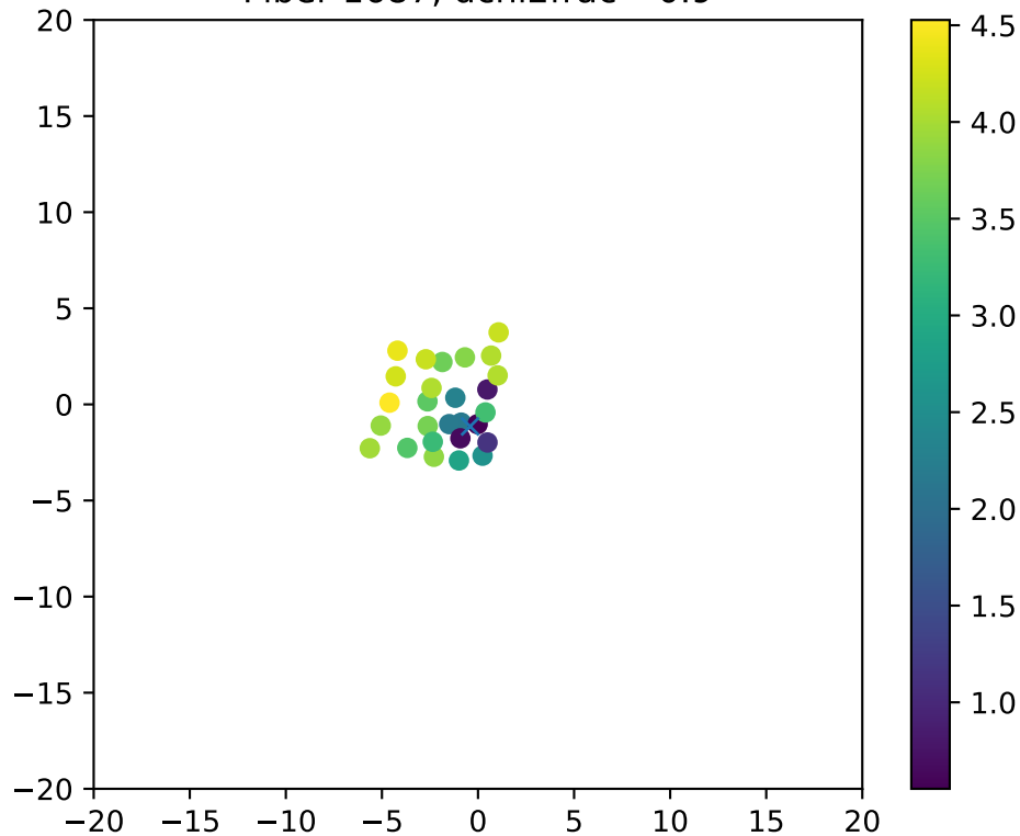
Fiber 1687, dchi2frac= 0.9
