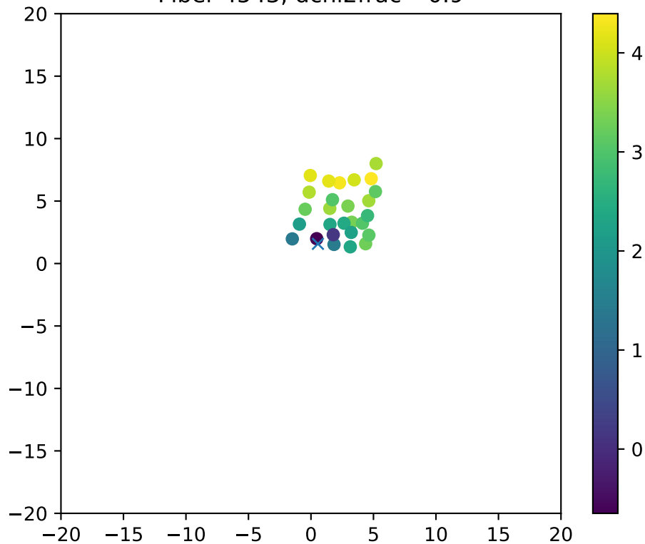
Fiber 4543, dchi2frac= 0.9
