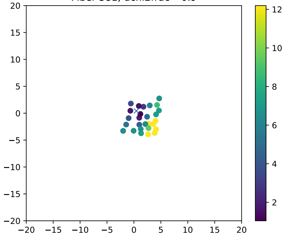
Fiber 381, dchi2frac= 0.9
