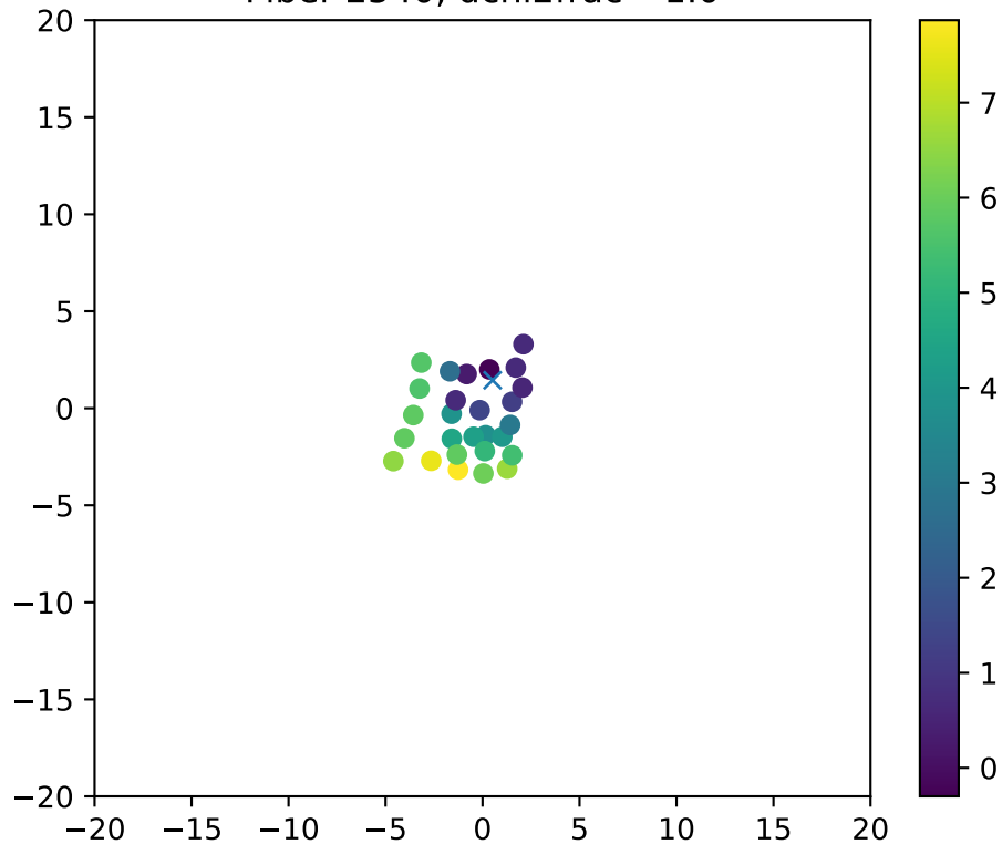
Fiber 2540, dchi2frac= 1.0
