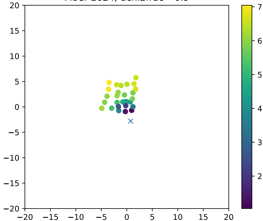
Fiber 2624, dchi2frac= 0.9
