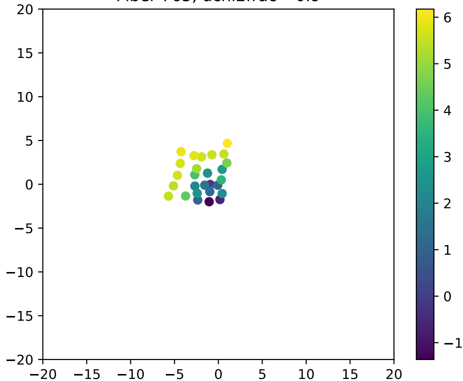
Fiber 765, dchi2frac= 0.9
