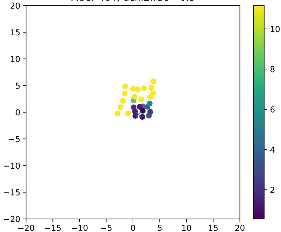
Fiber 464, dchi2frac= 0.9
