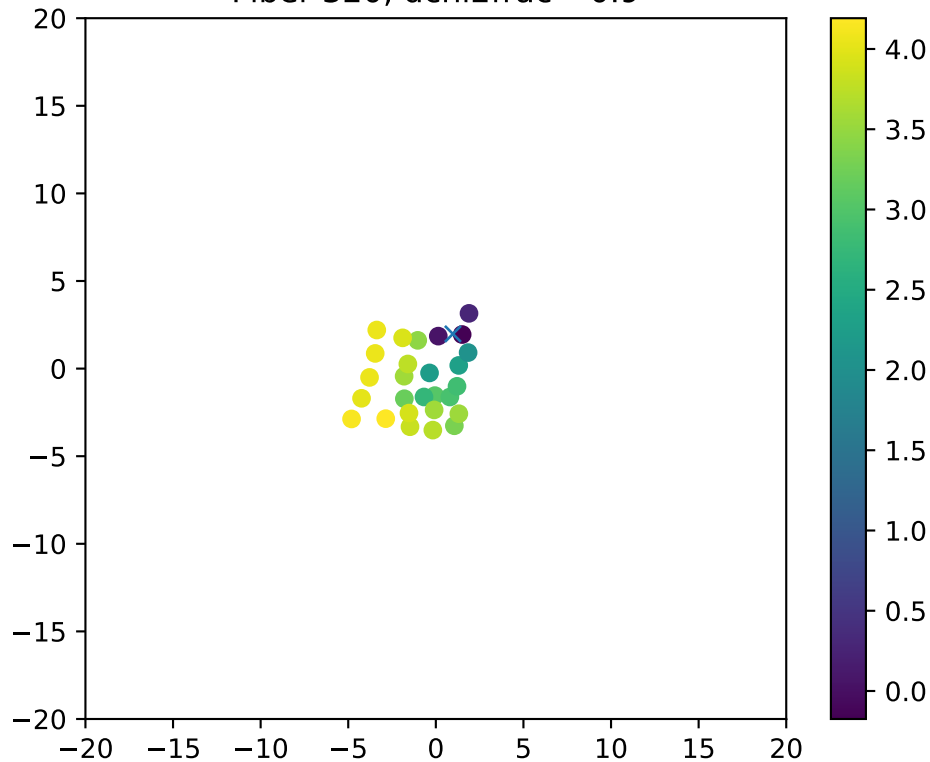
Fiber 320, dchi2frac= 0.9
