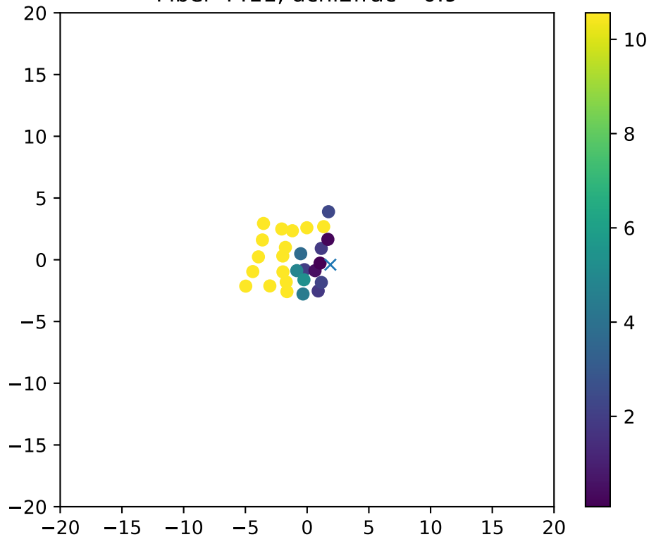
Fiber 4411, dchi2frac= 0.9
