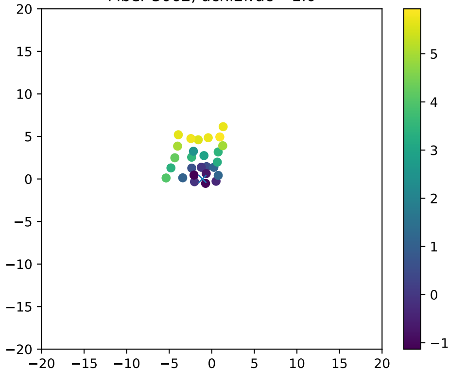
Fiber 3062, dchi2frac= 1.0
