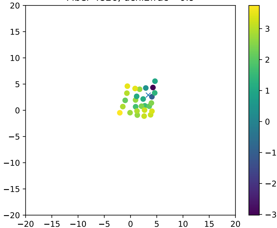
Fiber 4826, dchi2frac= 0.9
