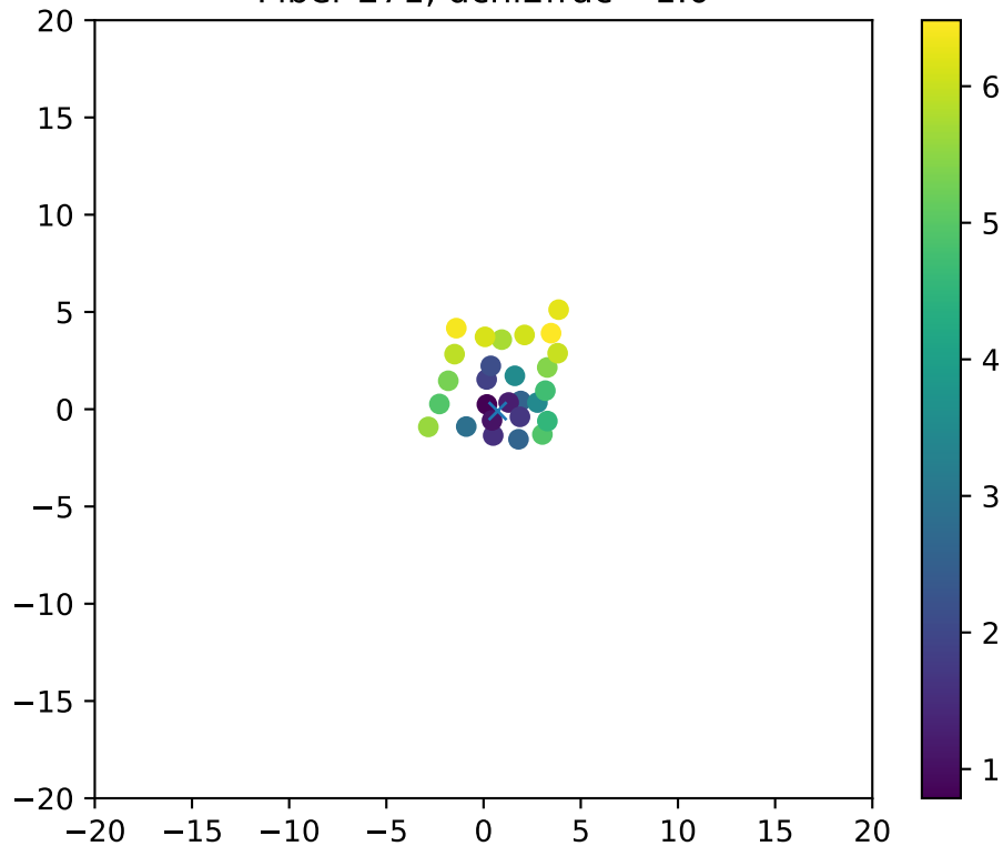
Fiber 271, dchi2frac= 1.0
