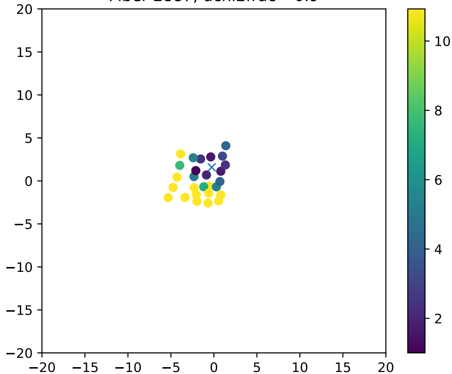
Fiber 2887, dchi2frac= 0.9
