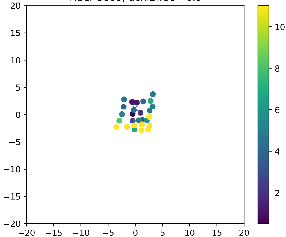
Fiber 3868, dchi2frac= 0.9
