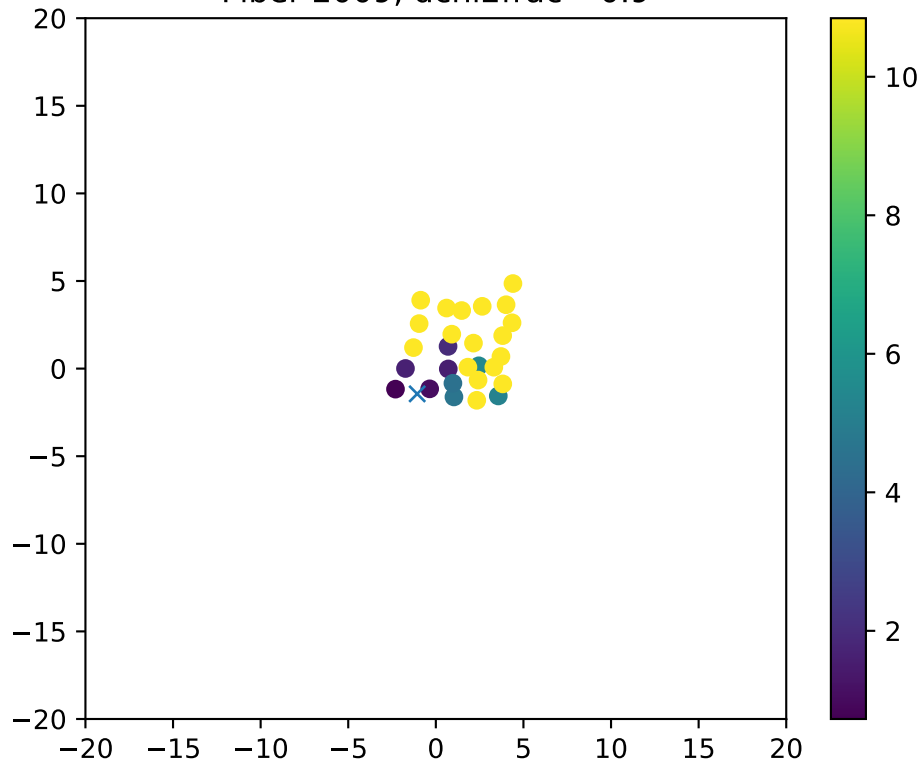
Fiber 2009, dchi2frac= 0.9
