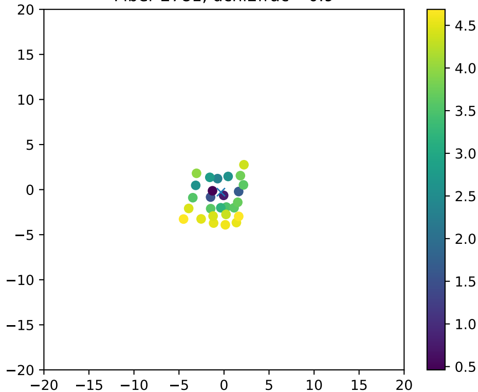
Fiber 2781, dchi2frac= 0.9
