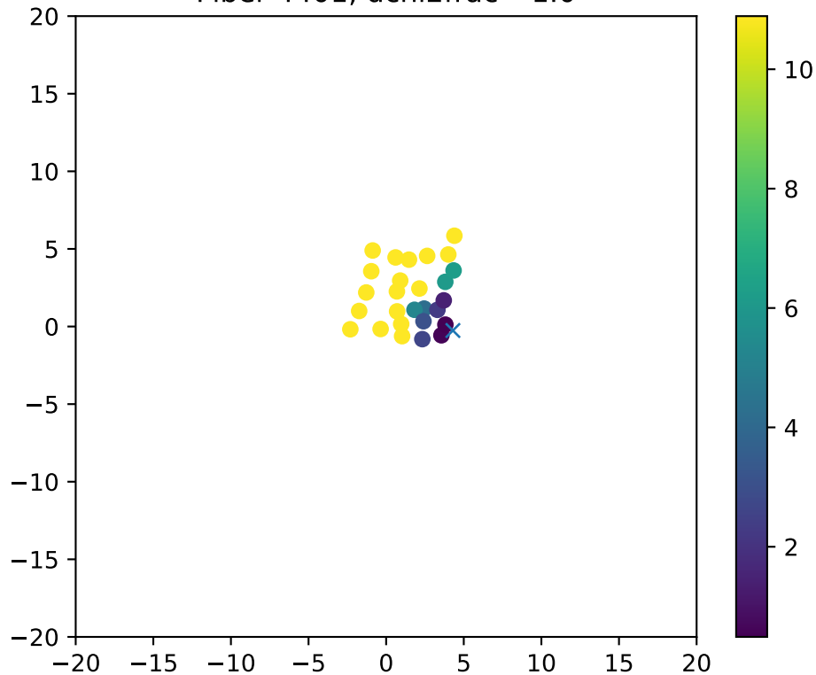
Fiber 4401, dchi2frac= 1.0
