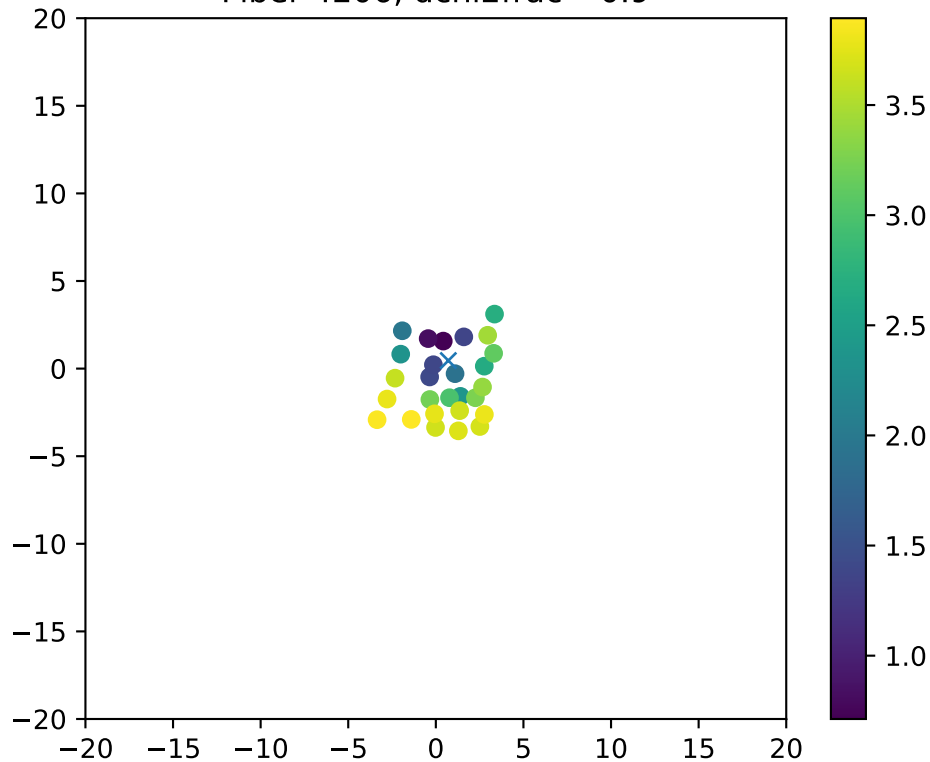
Fiber 4206, dchi2frac= 0.9
