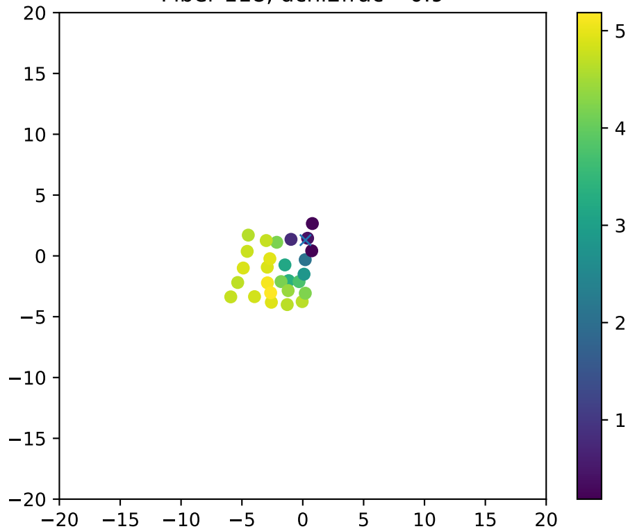
Fiber 118, dchi2frac= 0.9
