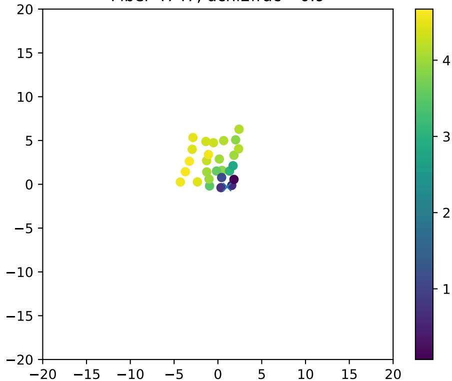
Fiber 4747, dchi2frac= 0.9
