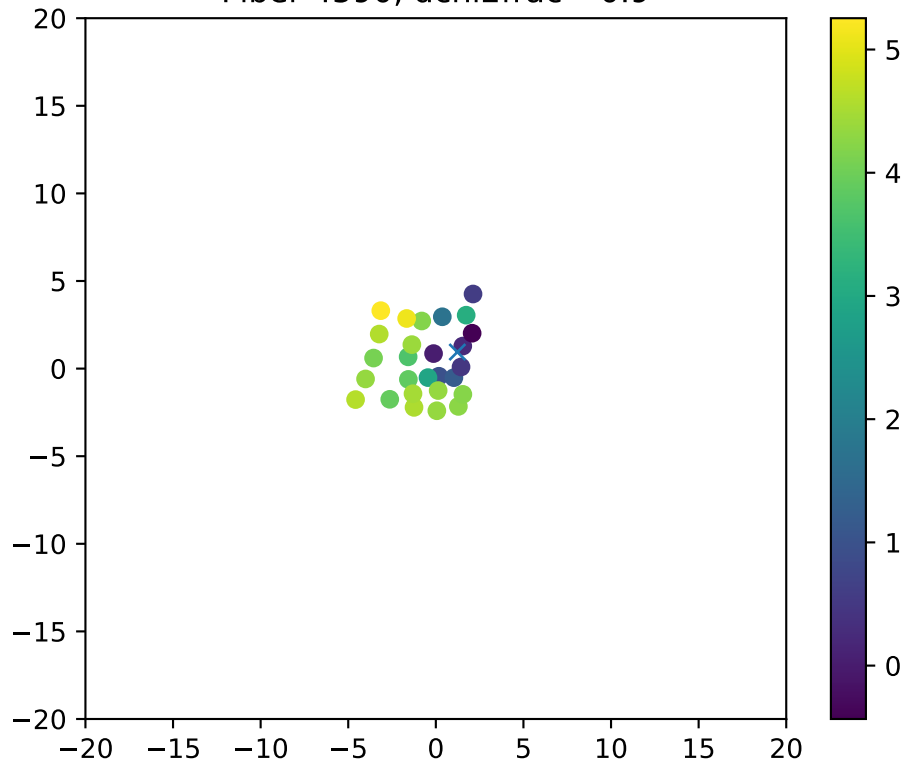
Fiber 4590, dchi2frac= 0.9
