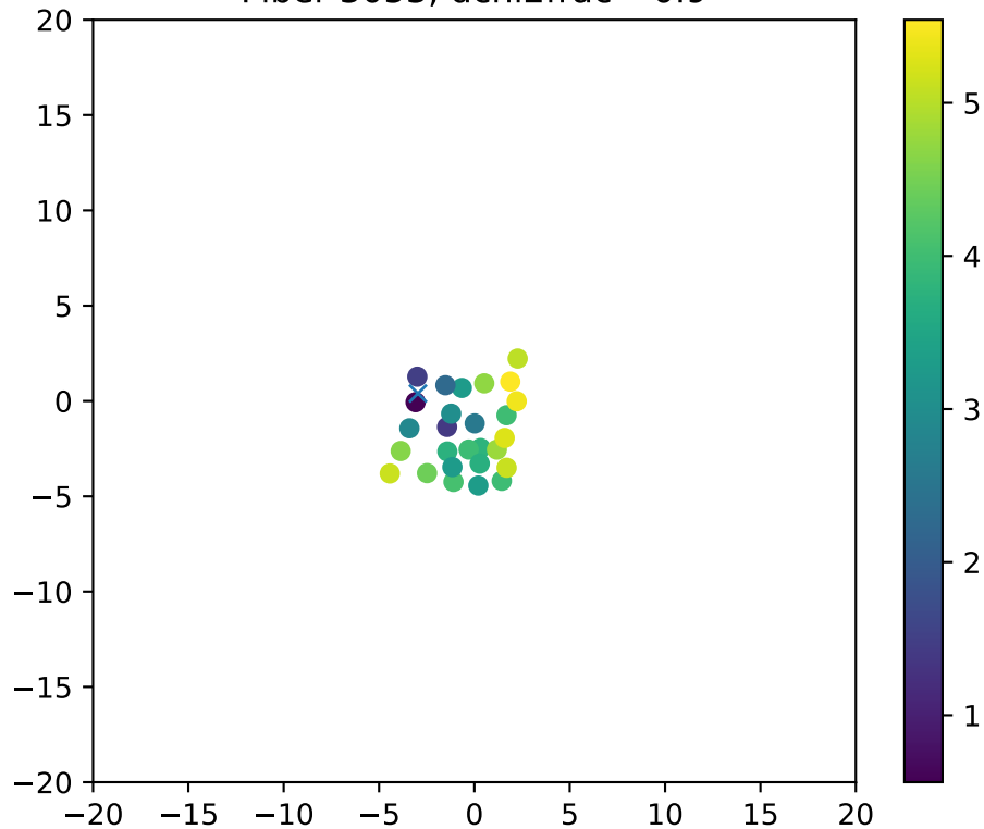
Fiber 3053, dchi2frac= 0.9
