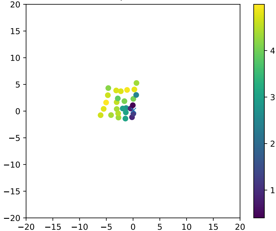
Fiber 3642, dchi2frac= 0.9
