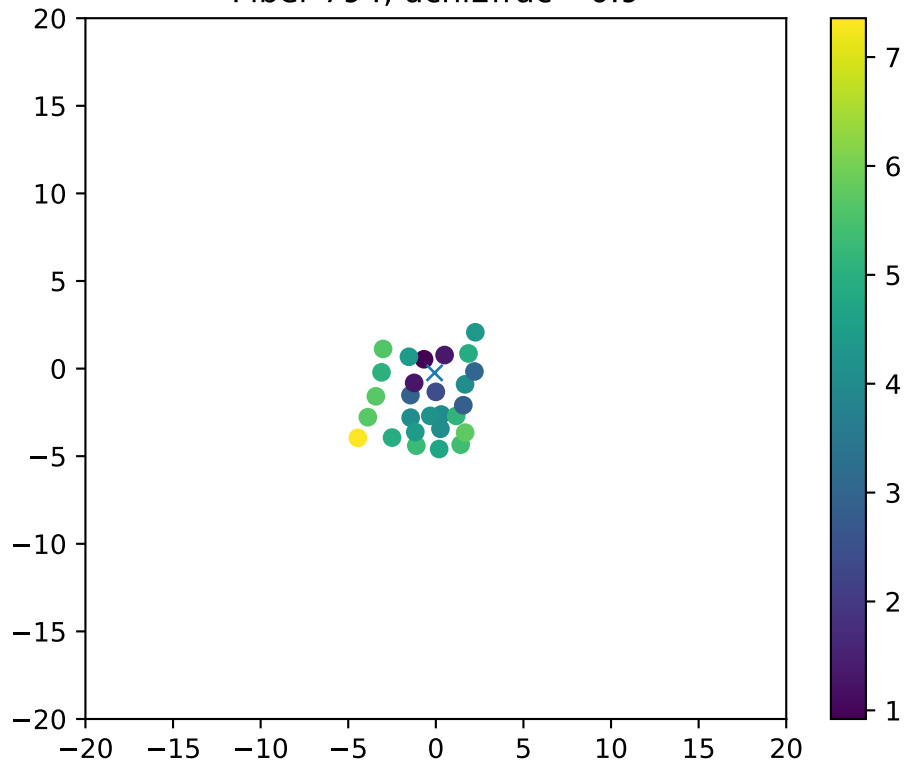
Fiber 794, dchi2frac= 0.9
