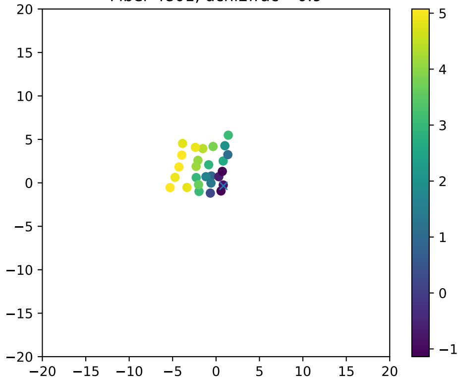
Fiber 4801, dchi2frac= 0.9
