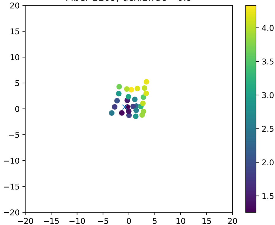
Fiber 2109, dchi2frac= 0.9
