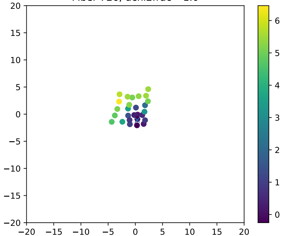
Fiber 726, dchi2frac= 1.0
