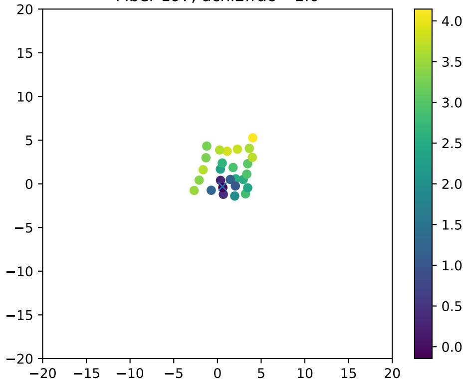
Fiber 197, dchi2frac= 1.0
