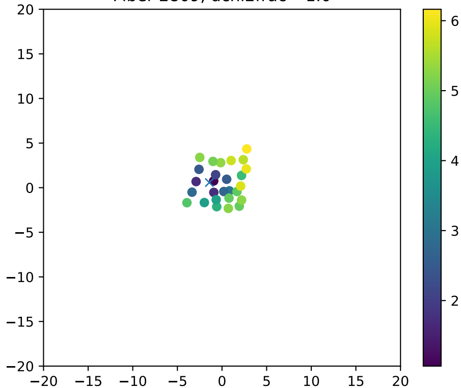
Fiber 2809, dchi2frac= 1.0
