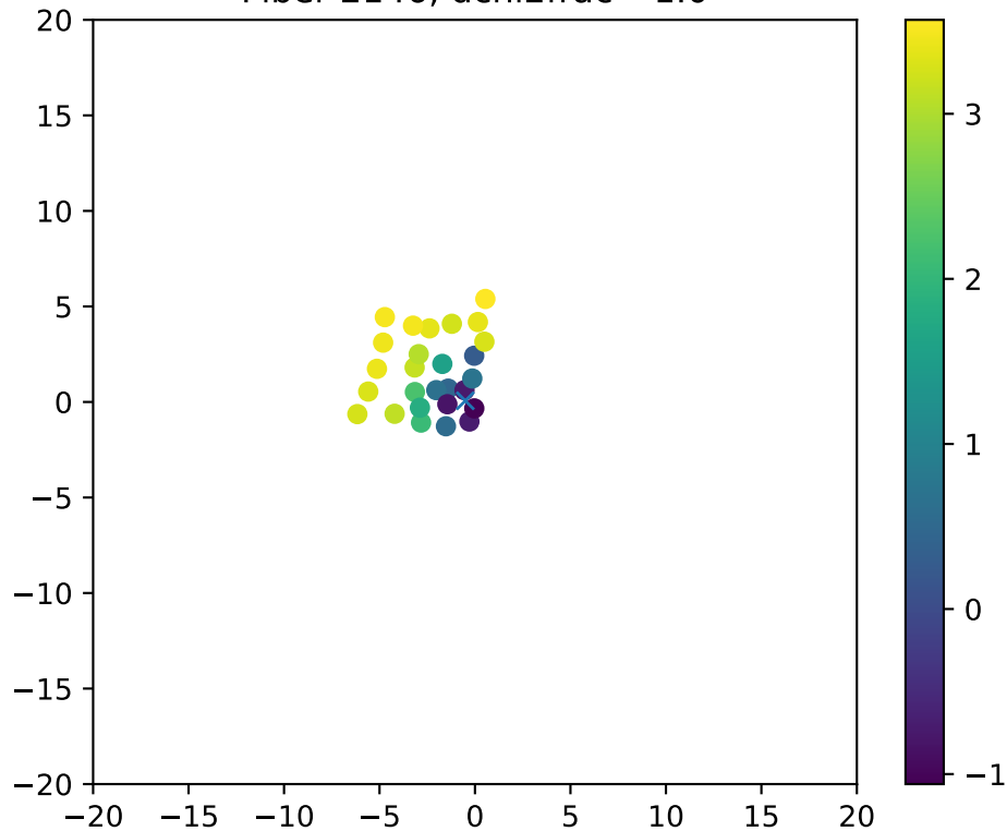
Fiber 2146, dchi2frac= 1.0
