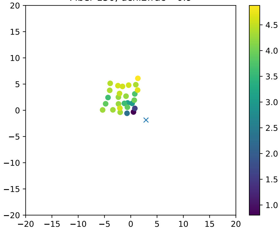
Fiber 150, dchi2frac= 0.9
