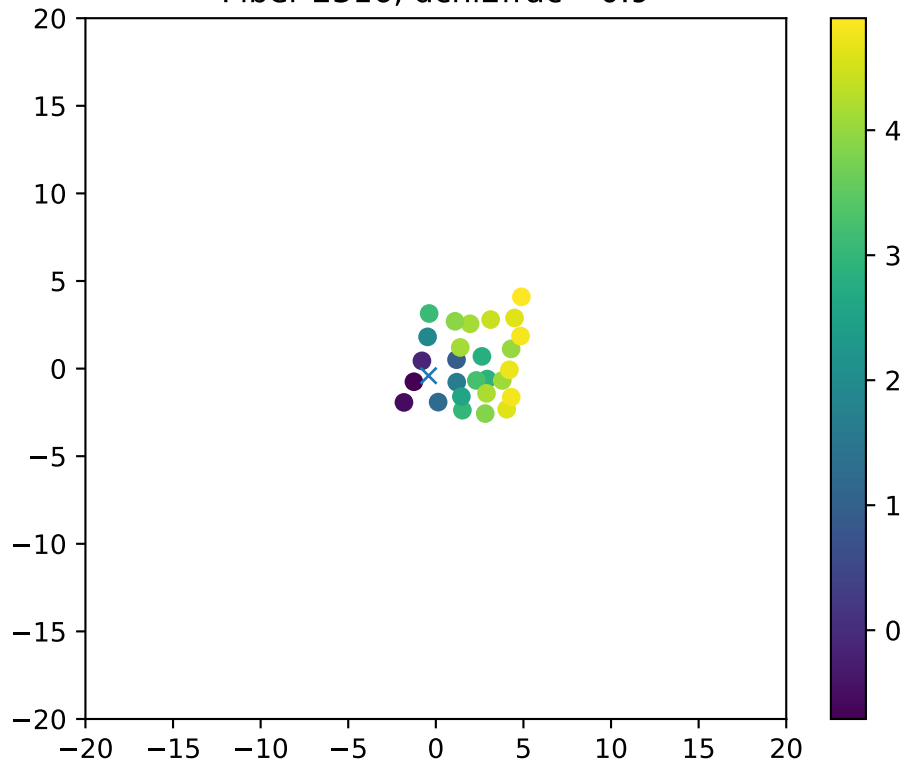
Fiber 2316, dchi2frac= 0.9
