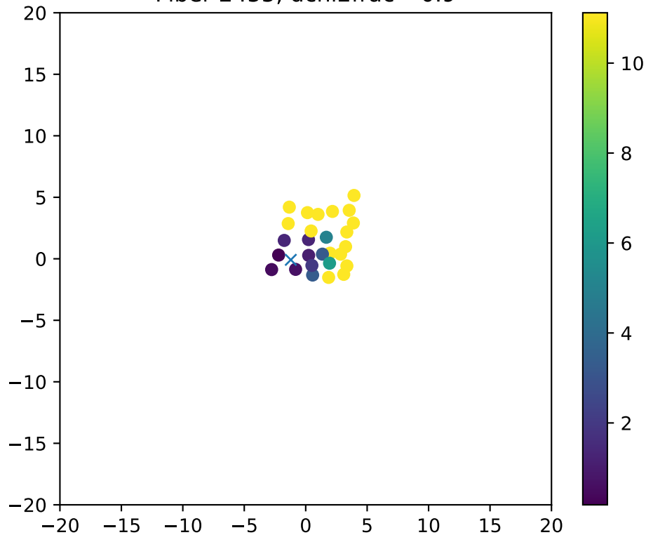
Fiber 2455, dchi2frac= 0.9
