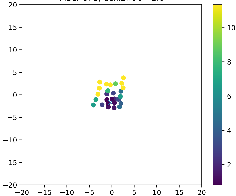
Fiber 871, dchi2frac= 1.0
