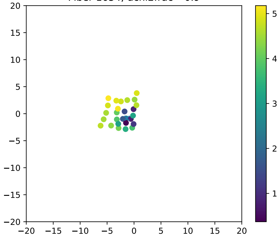
Fiber 1634, dchi2frac= 0.9
