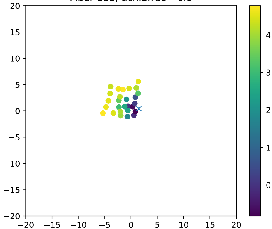
Fiber 183, dchi2frac= 0.9
