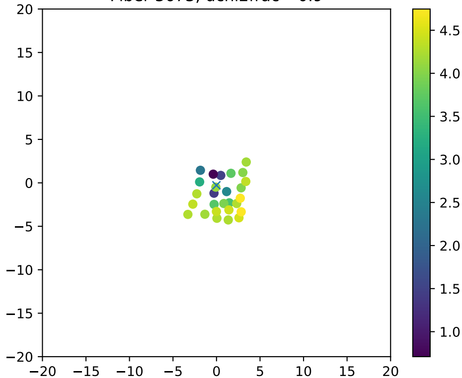
Fiber 3673, dchi2frac= 0.9
