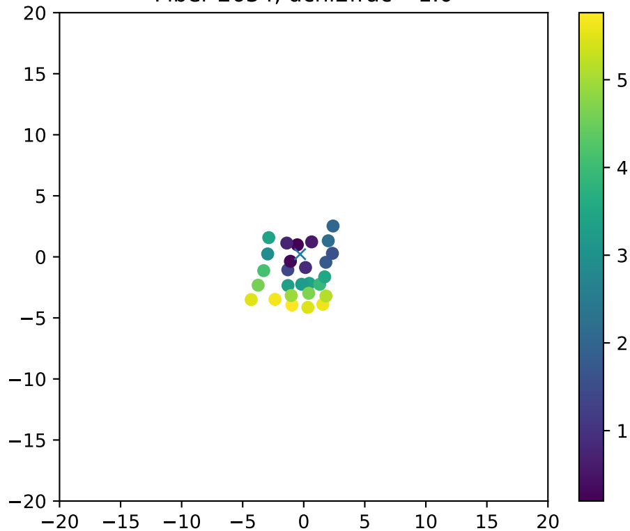
Fiber 2634, dchi2frac= 1.0
