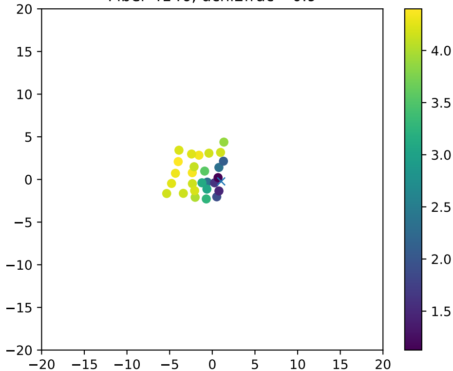
Fiber 4146, dchi2frac= 0.9
