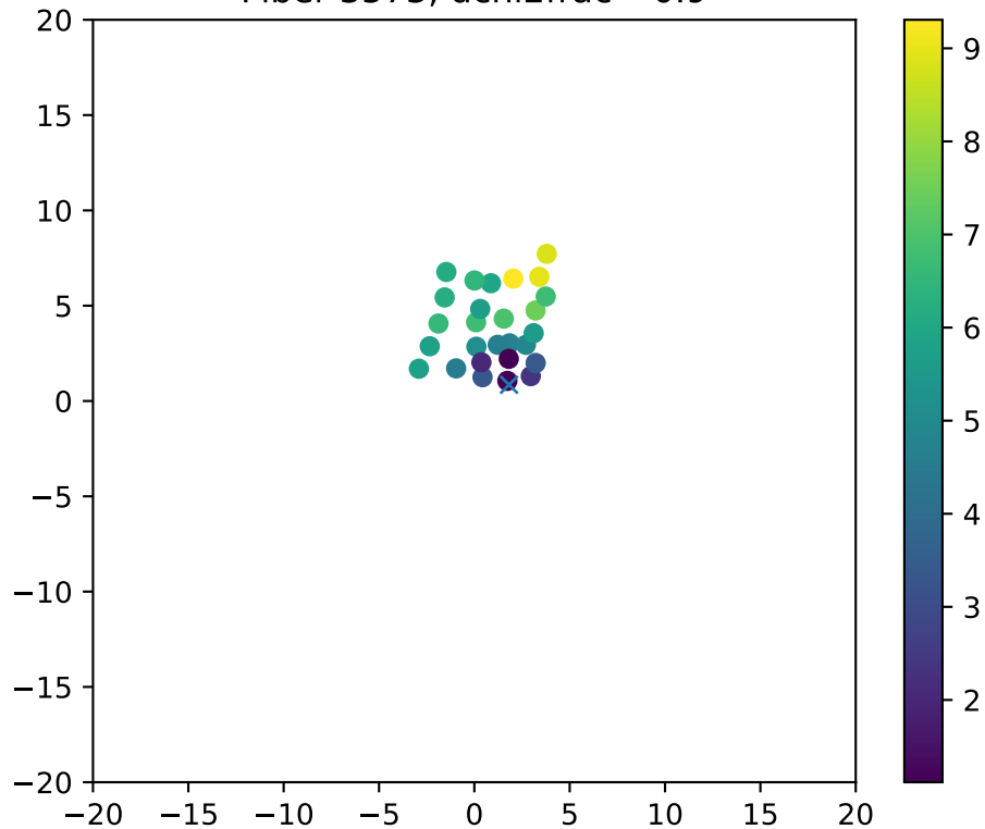
Fiber 3573, dchi2frac= 0.9
