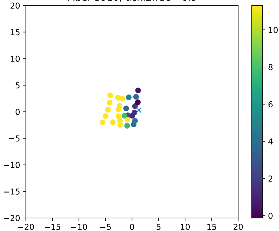
Fiber 3910, dchi2frac= 0.9
