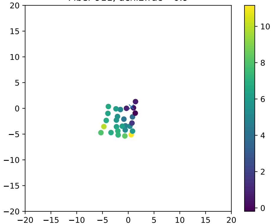
Fiber 911, dchi2frac= 0.9
