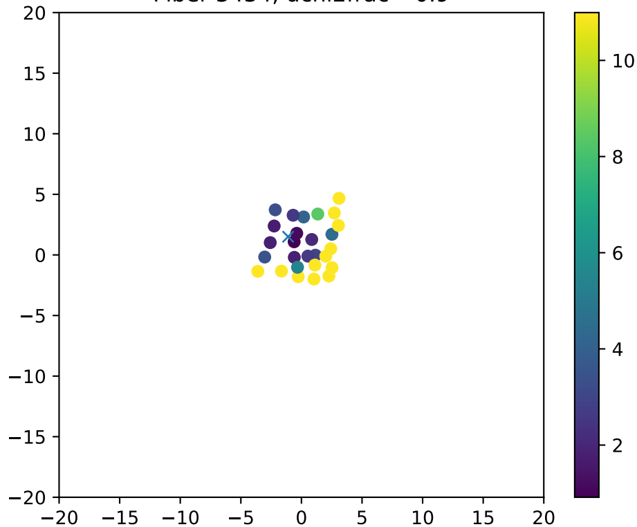
Fiber 3434, dchi2frac= 0.9
