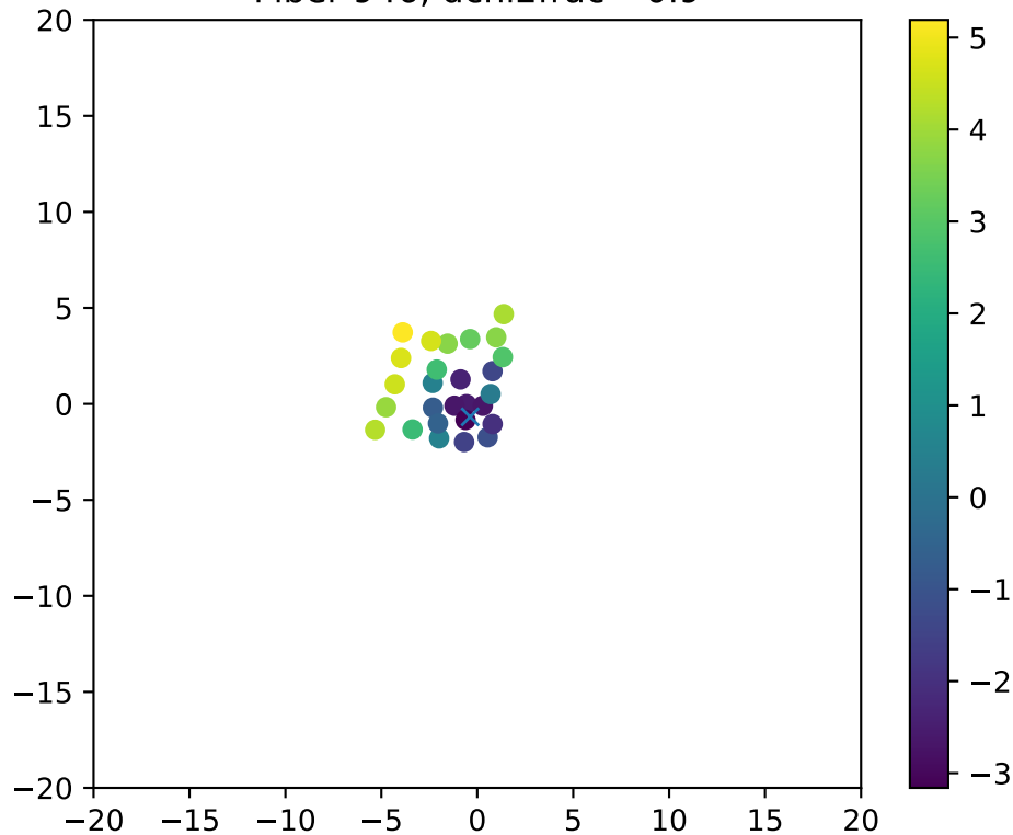
Fiber 946, dchi2frac= 0.9
