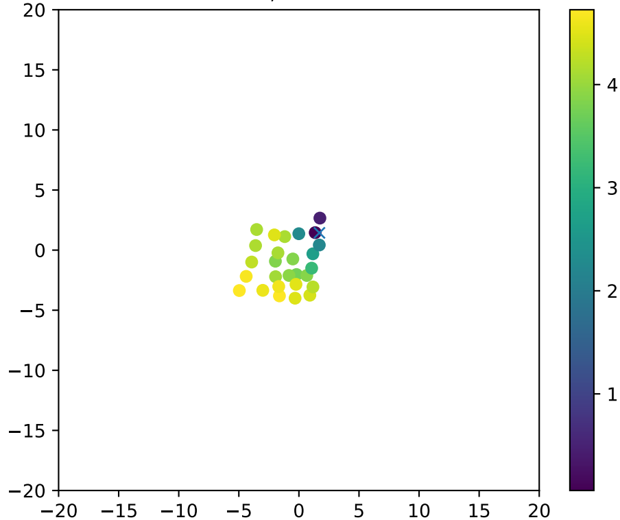
Fiber 3232, dchi2frac= 0.9
