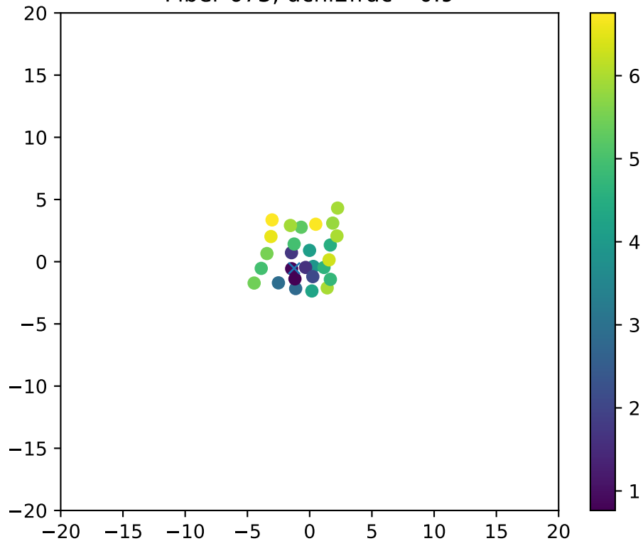
Fiber 673, dchi2frac= 0.9
