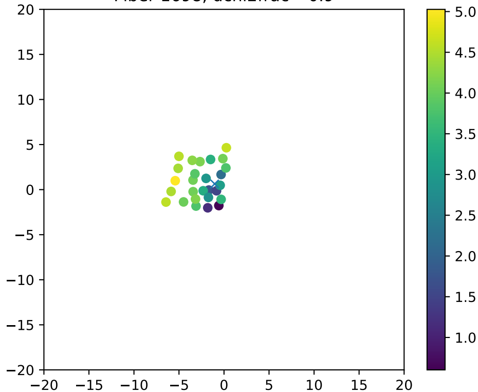
Fiber 1698, dchi2frac= 0.9
