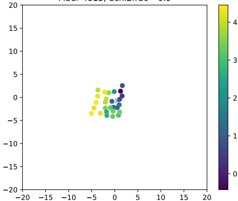
Fiber 4813, dchi2frac= 0.9
