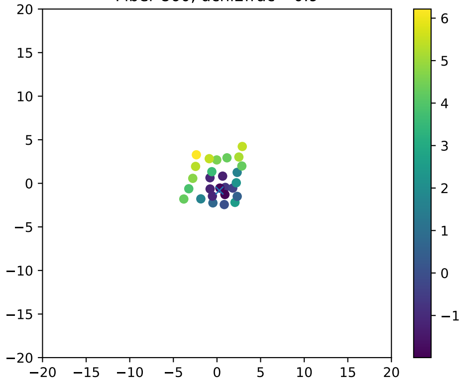
Fiber 860, dchi2frac= 0.9
