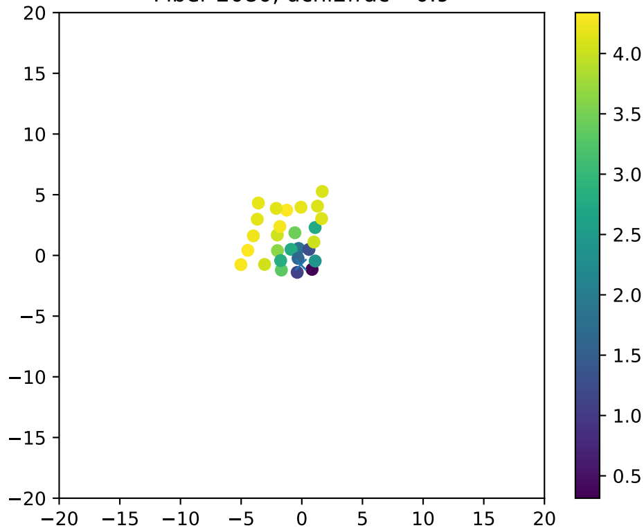
Fiber 2080, dchi2frac= 0.9
