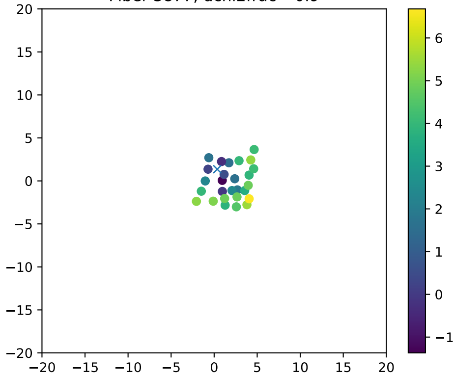
Fiber 3877, dchi2frac= 0.9
