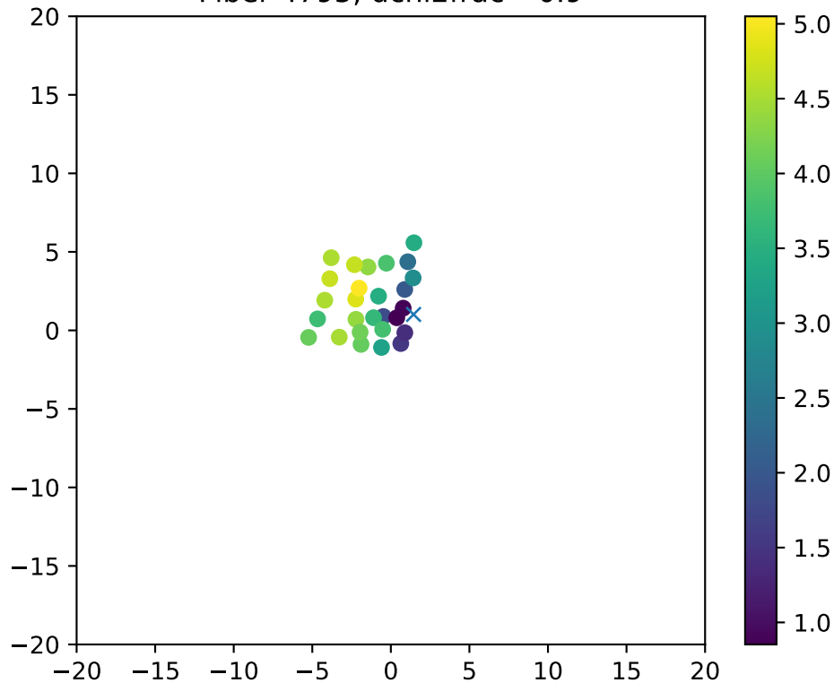
Fiber 4795, dchi2frac= 0.9
