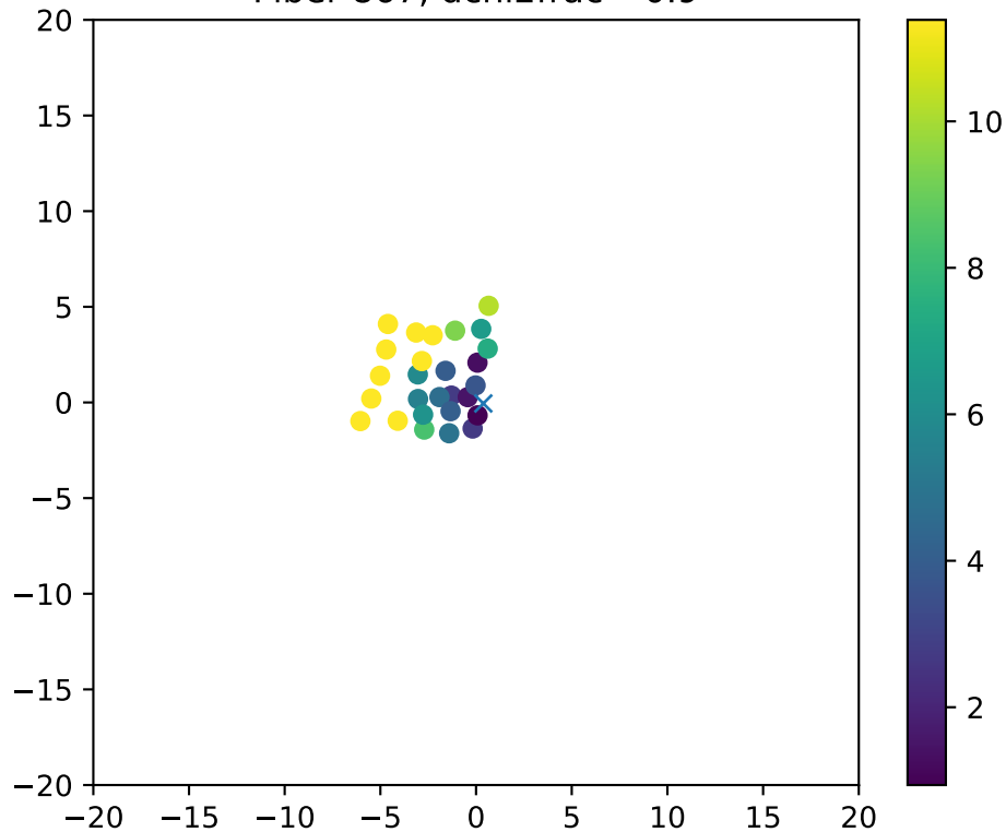
Fiber 867, dchi2frac= 0.9
