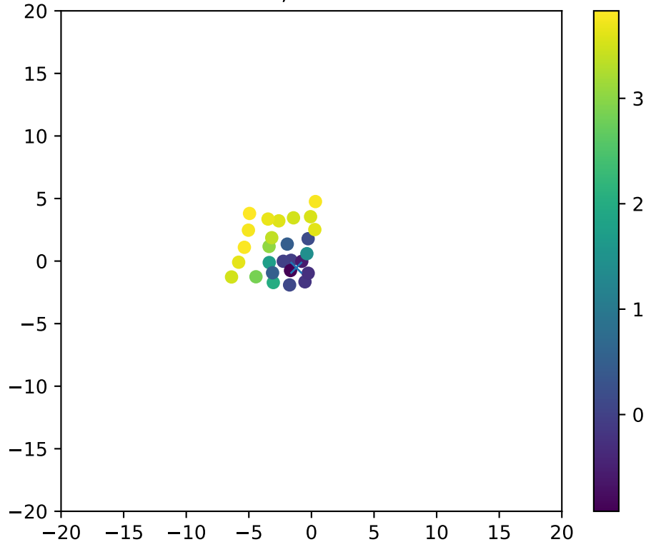
Fiber 2261, dchi2frac= 1.0
