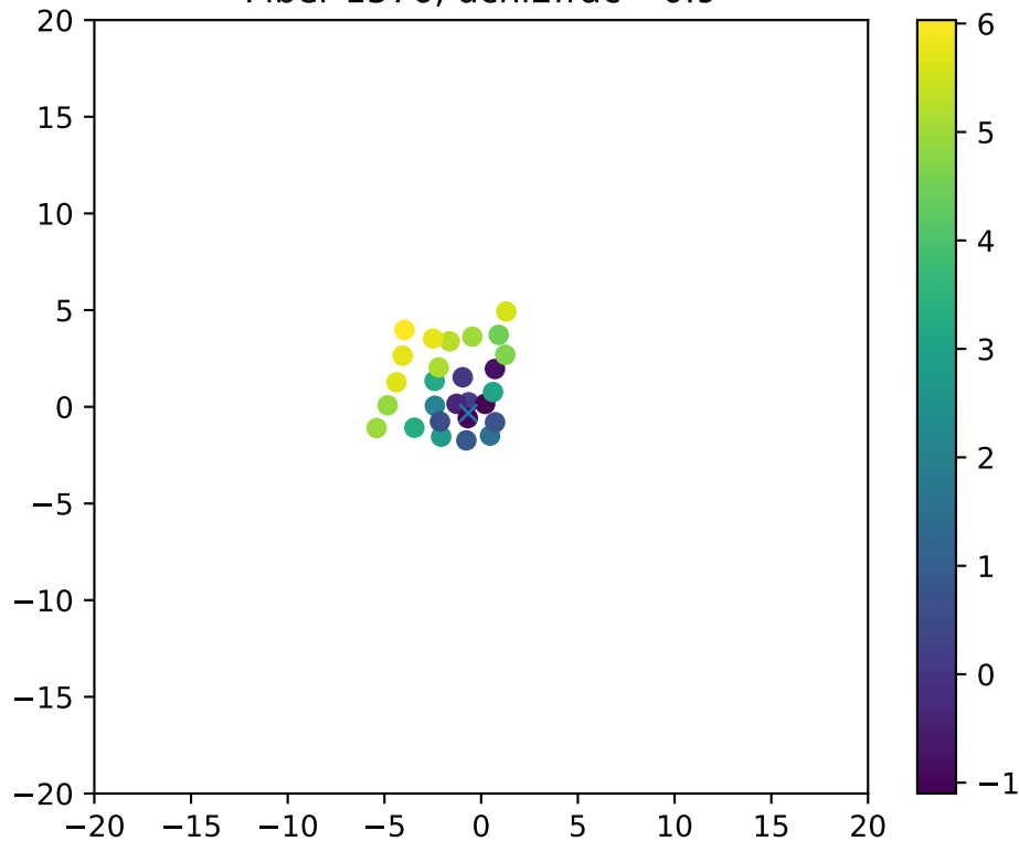
Fiber 1576, dchi2frac= 0.9
