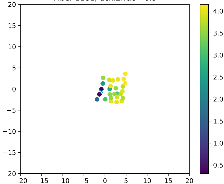
Fiber 2181, dchi2frac= 0.9
