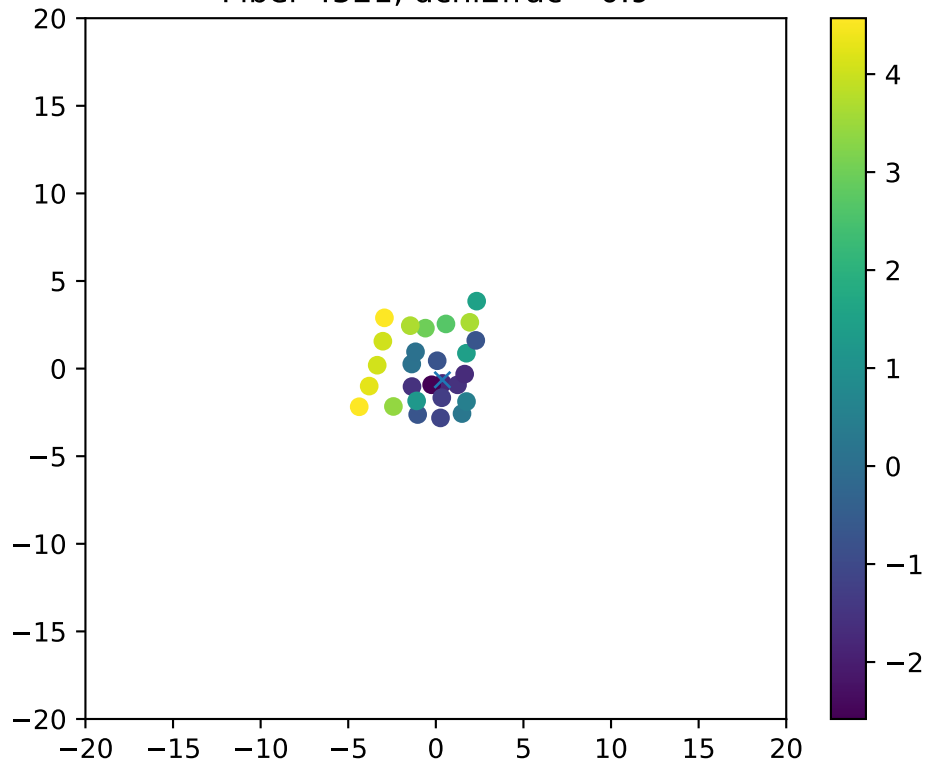
Fiber 4521, dchi2frac= 0.9
