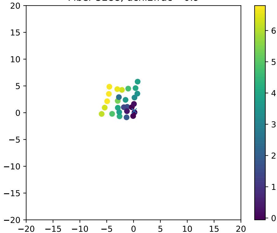
Fiber 3288, dchi2frac= 0.9
