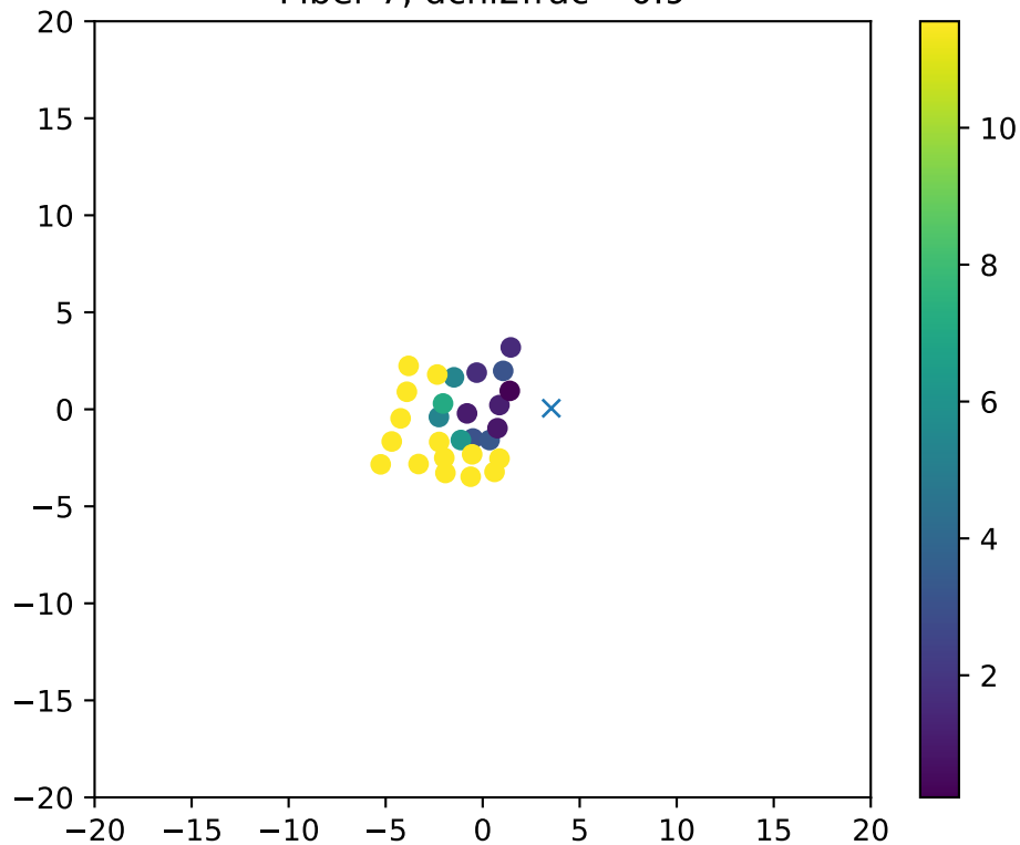
Fiber 7, dchi2frac= 0.9
