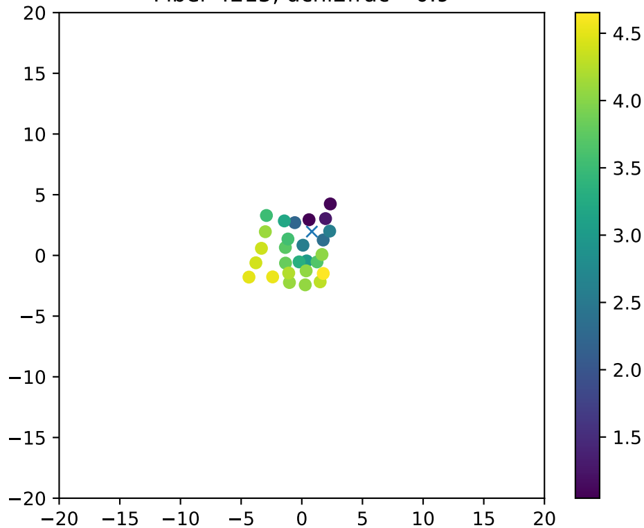
Fiber 4215, dchi2frac= 0.9
