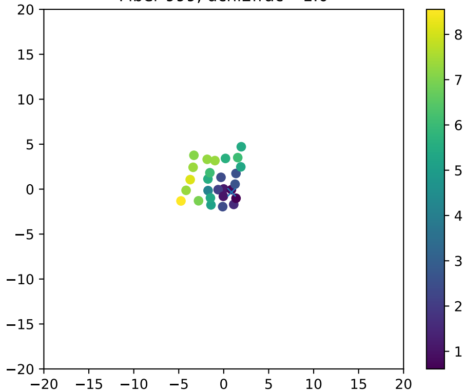
Fiber 999, dchi2frac= 1.0
