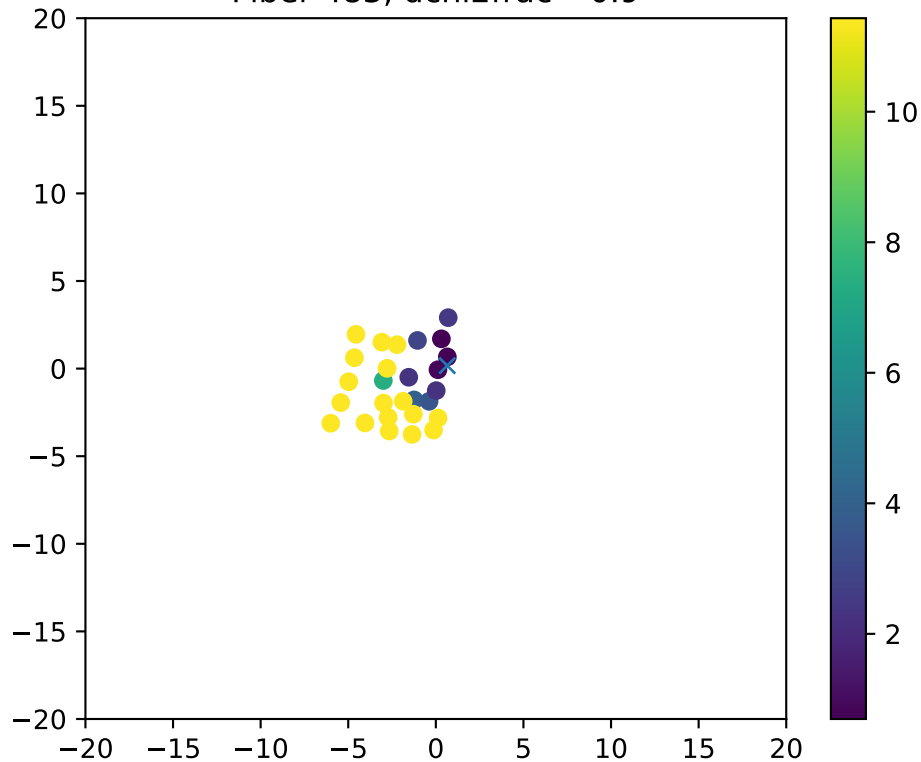
Fiber 483, dchi2frac= 0.9
