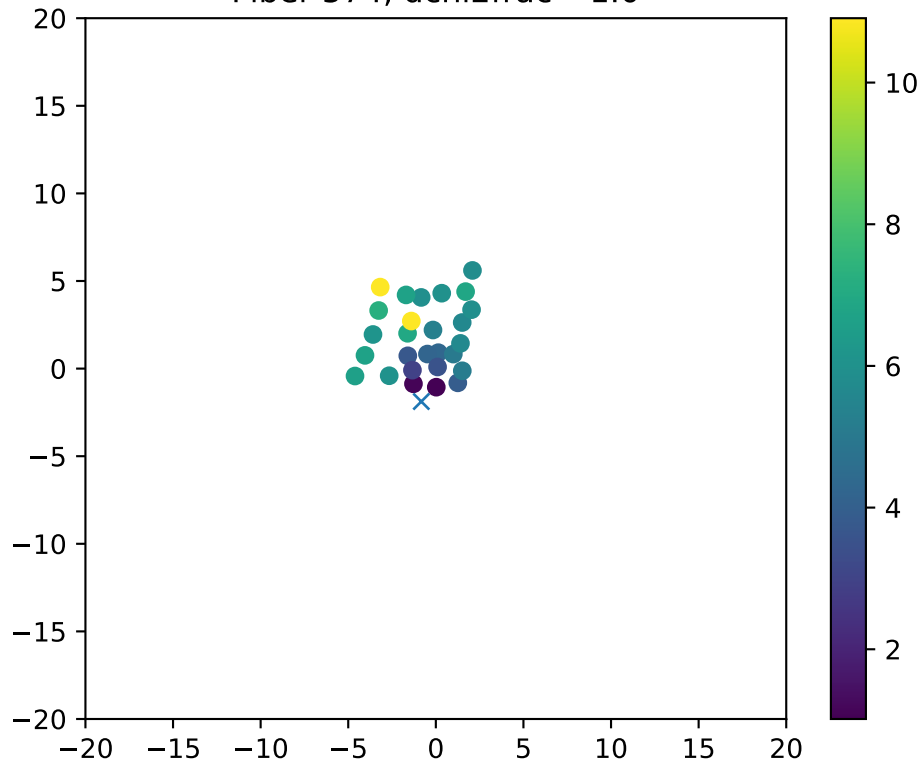
Fiber 574, dchi2frac= 1.0
