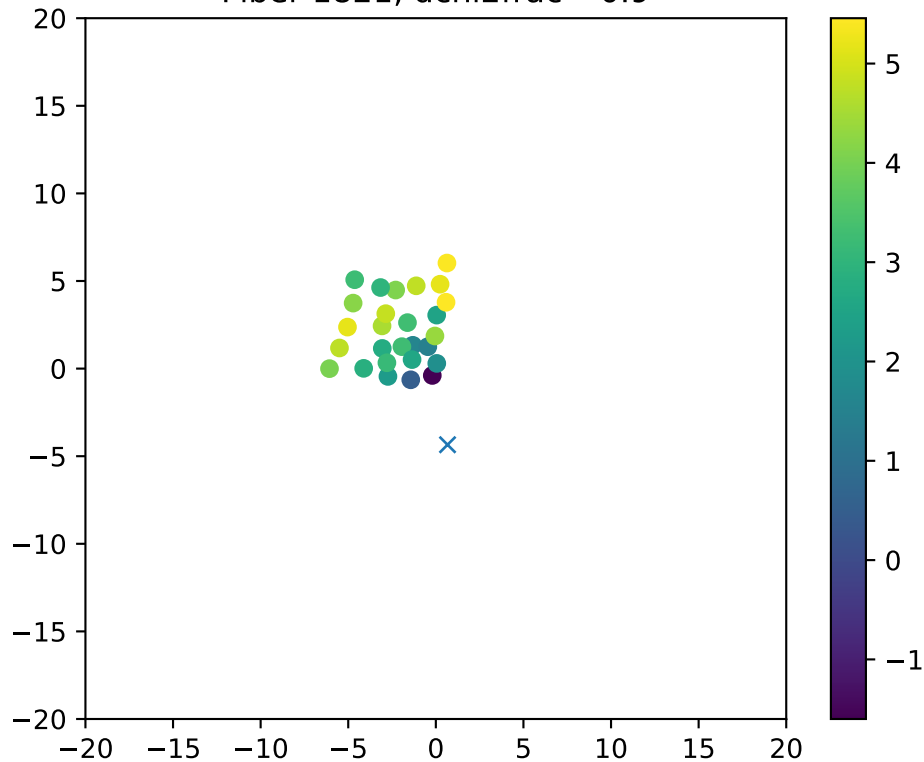
Fiber 1821, dchi2frac= 0.9
