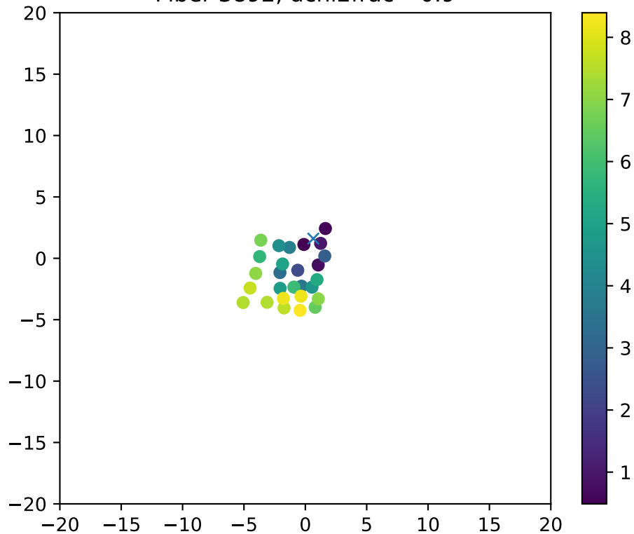
Fiber 3892, dchi2frac= 0.9
