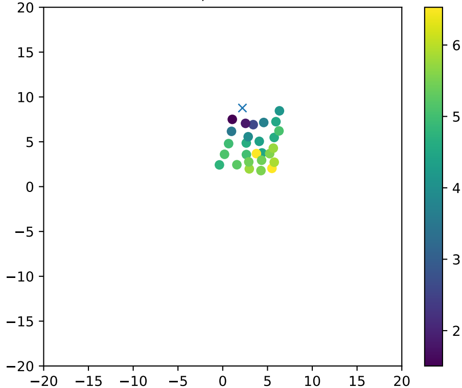
Fiber 2597, dchi2frac= 1.0
