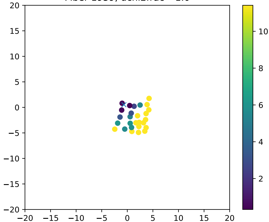
Fiber 1939, dchi2frac= 1.0
