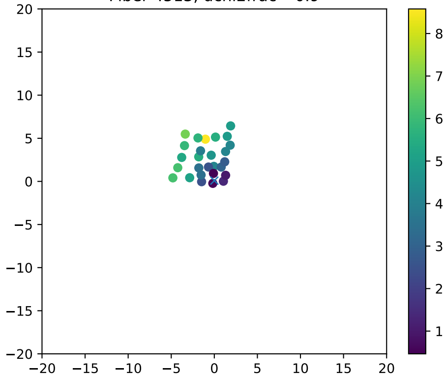
Fiber 4513, dchi2frac= 0.9
