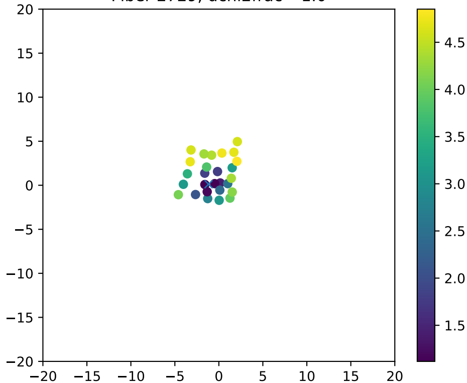
Fiber 2729, dchi2frac= 1.0
