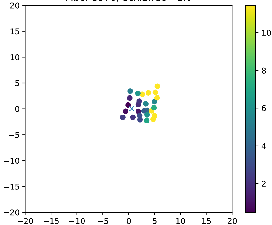
Fiber 3976, dchi2frac= 1.0
