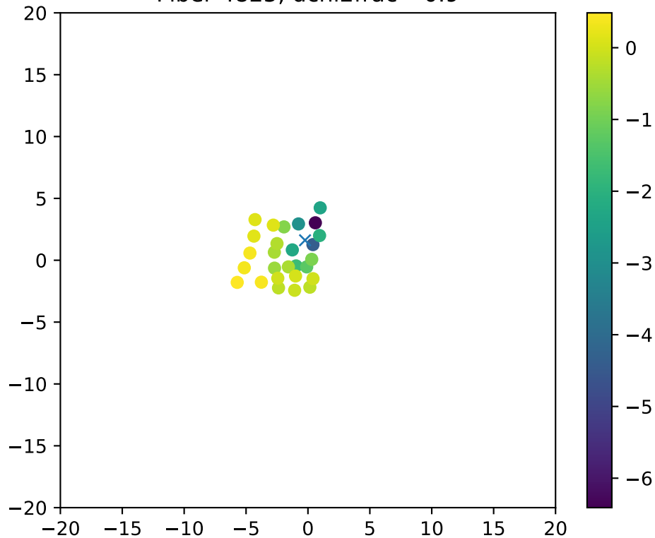
Fiber 4825, dchi2frac= 0.9
