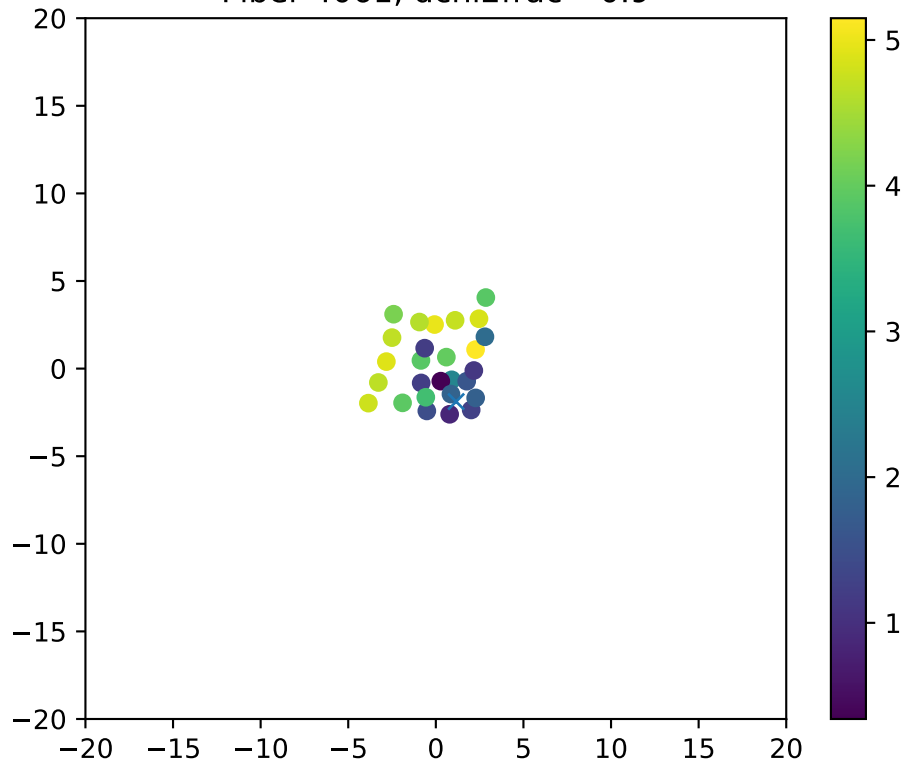
Fiber 4061, dchi2frac= 0.9
