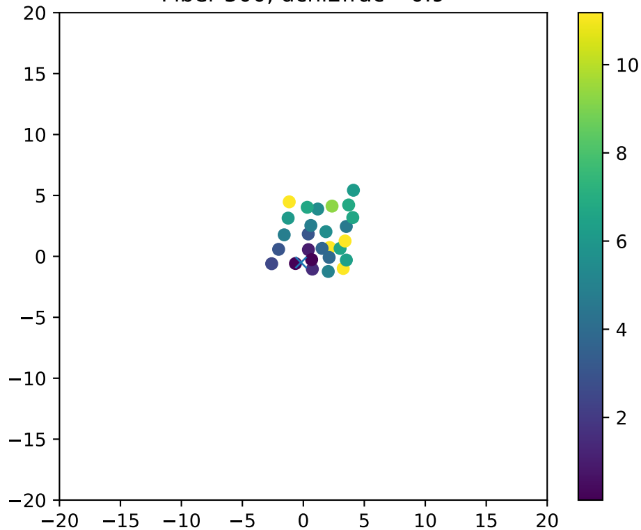
Fiber 500, dchi2frac= 0.9
