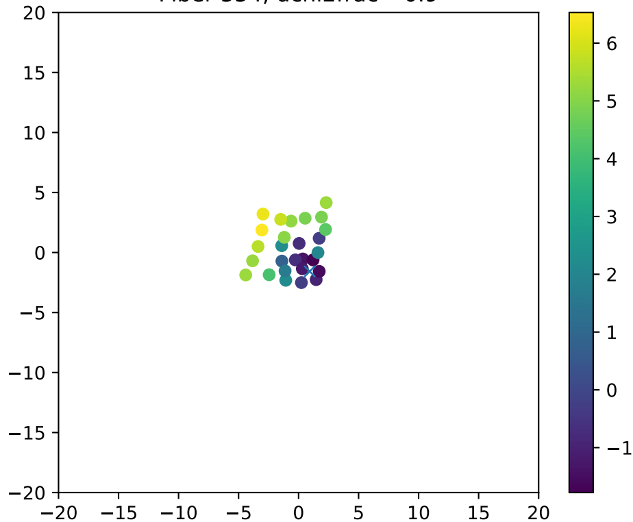
Fiber 554, dchi2frac= 0.9
