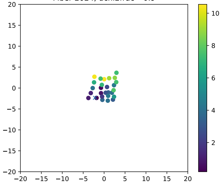
Fiber 2024, dchi2frac= 0.9
