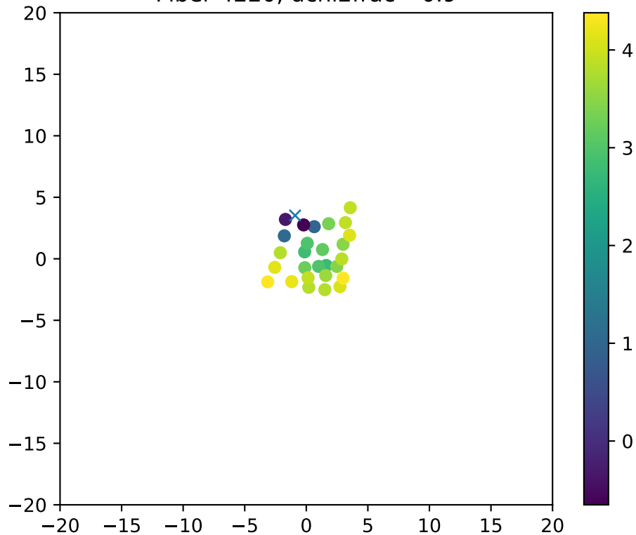
Fiber 4220, dchi2frac= 0.9
