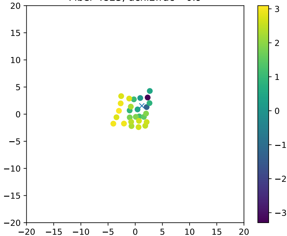
Fiber 4823, dchi2frac= 0.9
