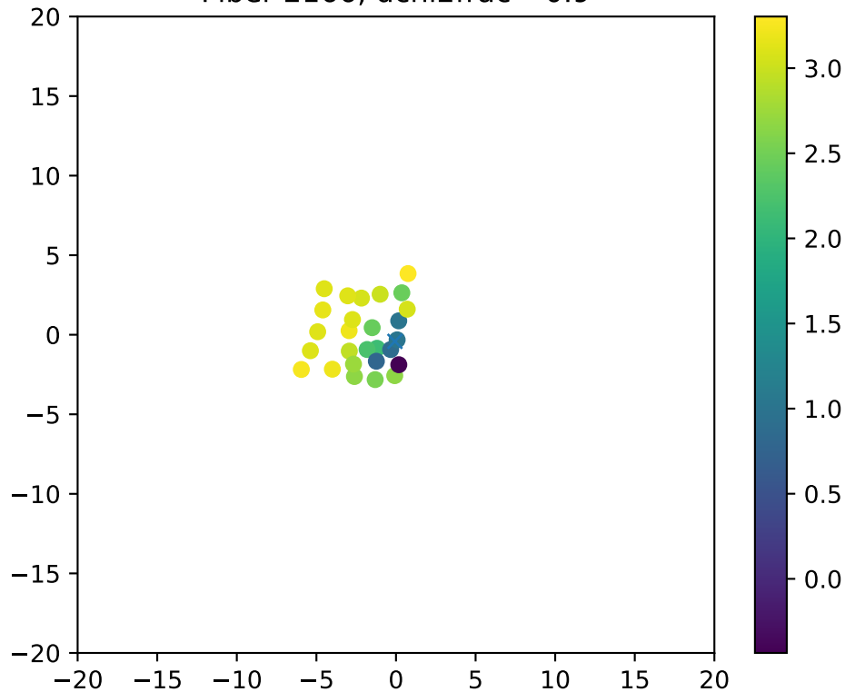
Fiber 2166, dchi2frac= 0.9
