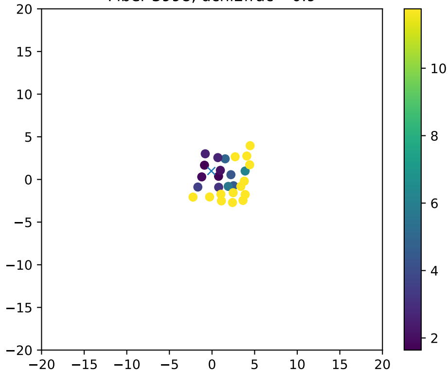
Fiber 3998, dchi2frac= 0.9
