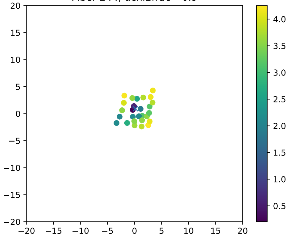
Fiber 244, dchi2frac= 0.9
