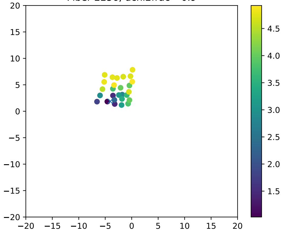
Fiber 2256, dchi2frac= 0.9
