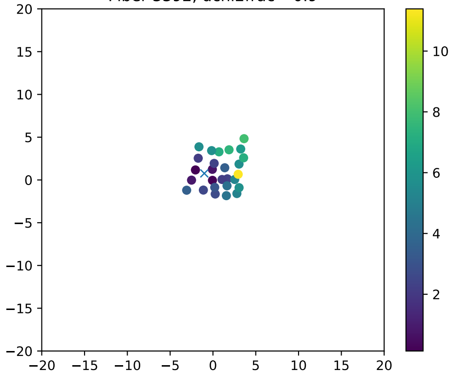
Fiber 3392, dchi2frac= 0.9
