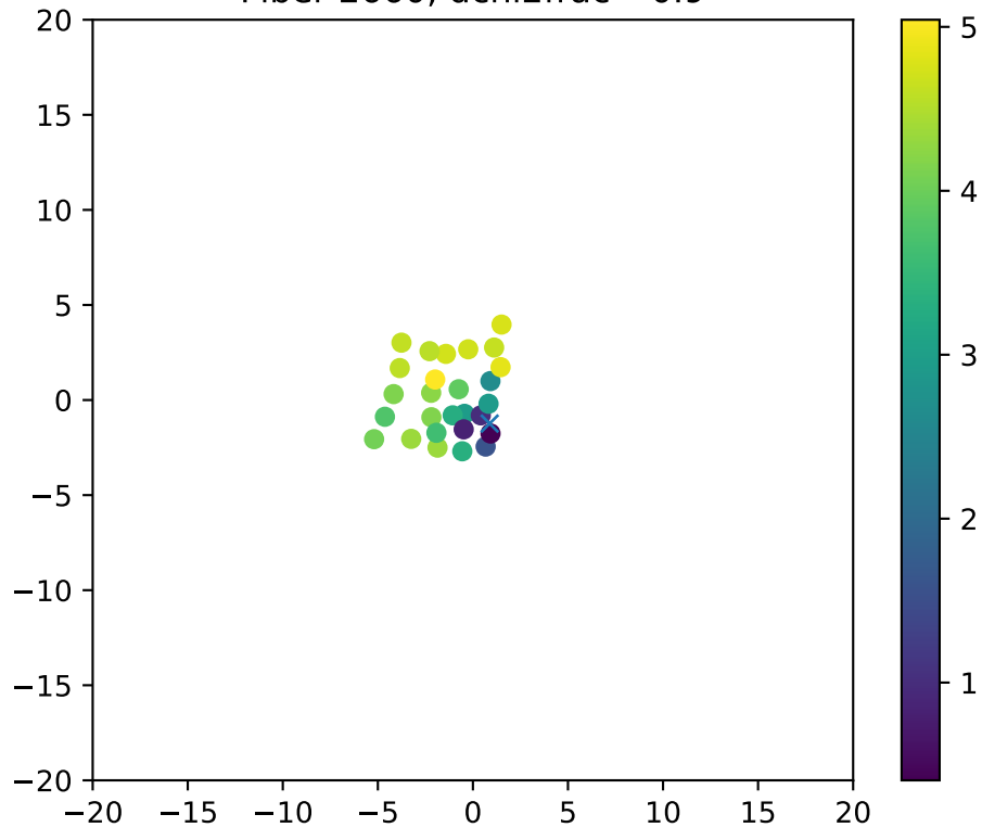
Fiber 2660, dchi2frac= 0.9
