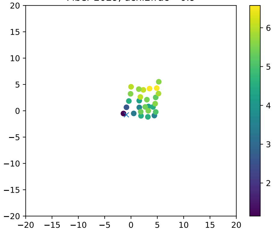
Fiber 2029, dchi2frac= 0.9
