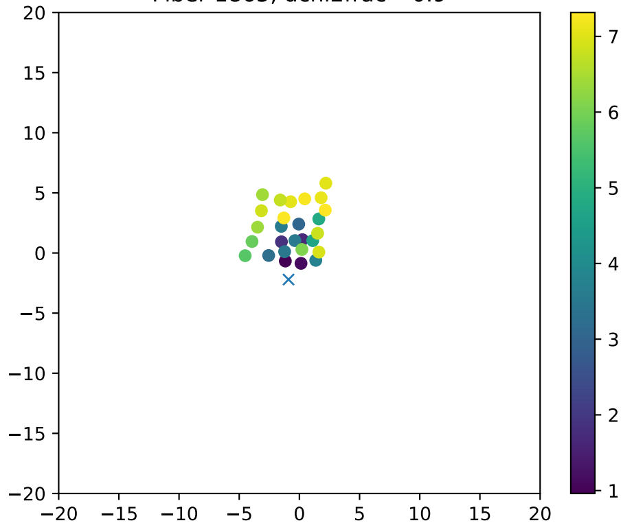
Fiber 1865, dchi2frac= 0.9
