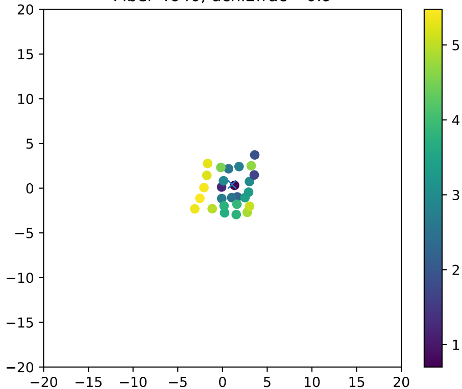
Fiber 4640, dchi2frac= 0.9
