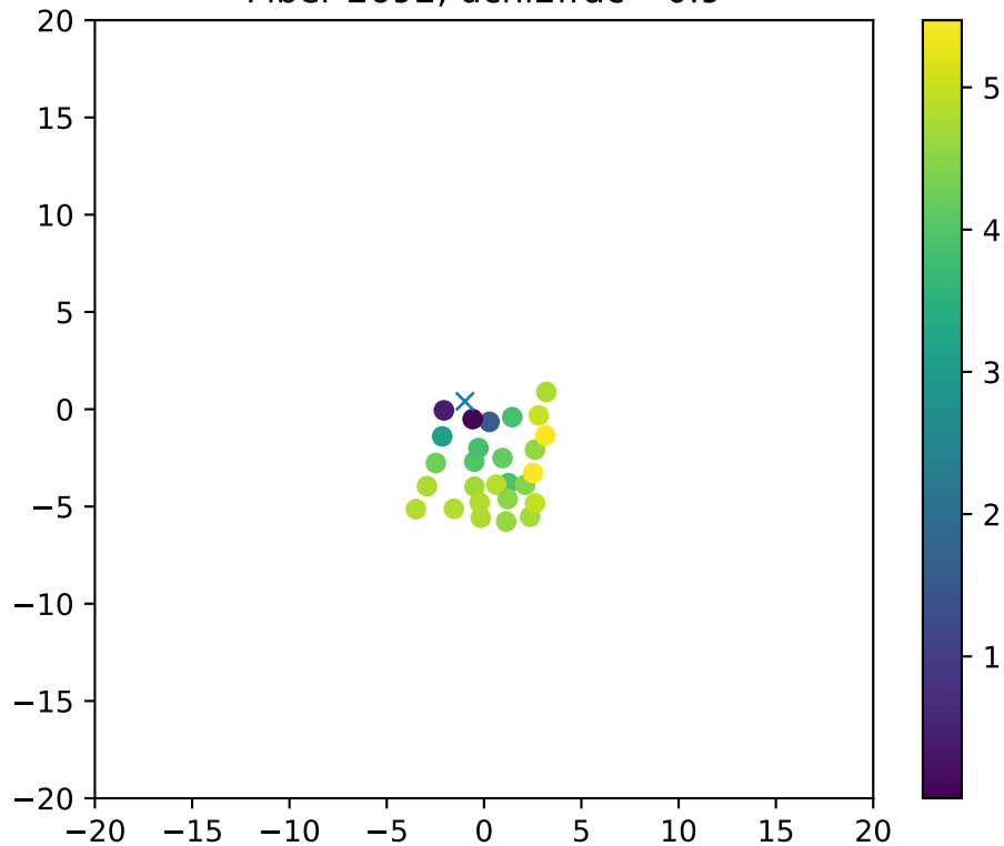
Fiber 2692, dchi2frac= 0.9
