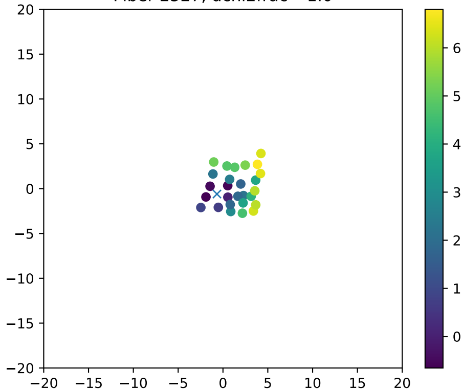
Fiber 2527, dchi2frac= 1.0
