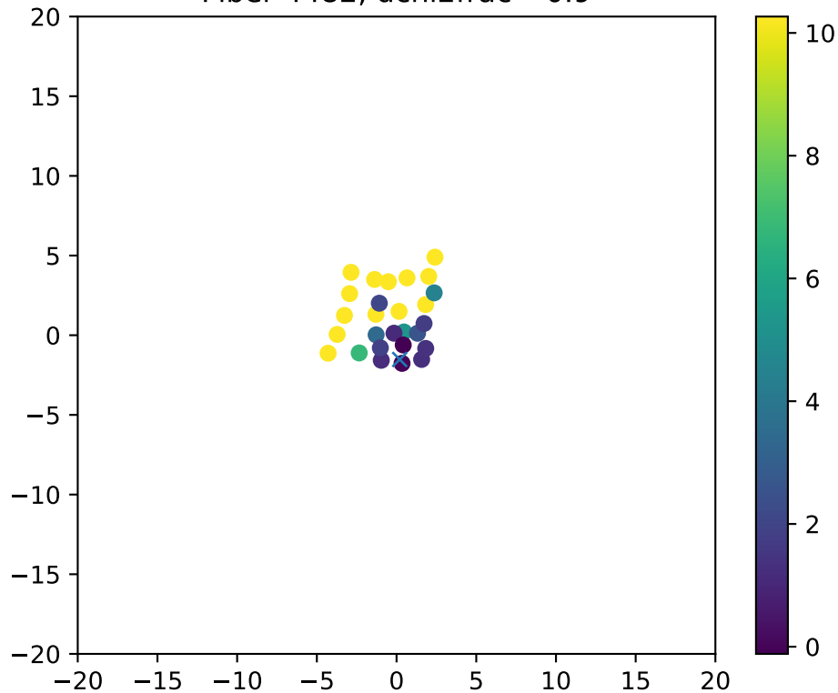
Fiber 4482, dchi2frac= 0.9
