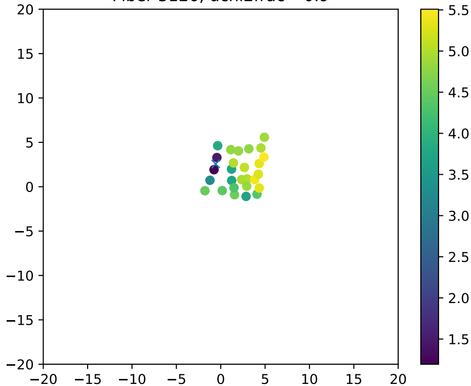
Fiber 3126, dchi2frac= 0.9
