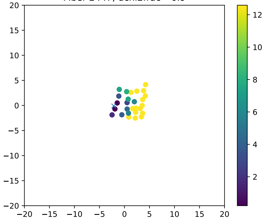
Fiber 2447, dchi2frac= 0.9
