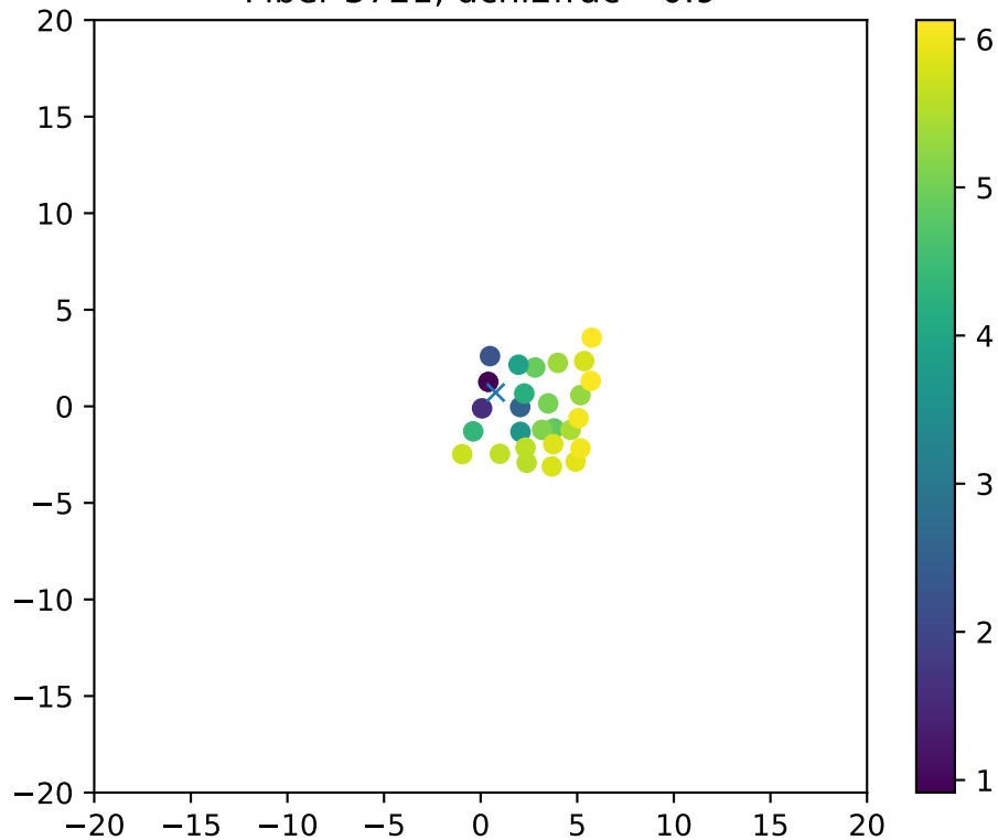
Fiber 3721, dchi2frac= 0.9
