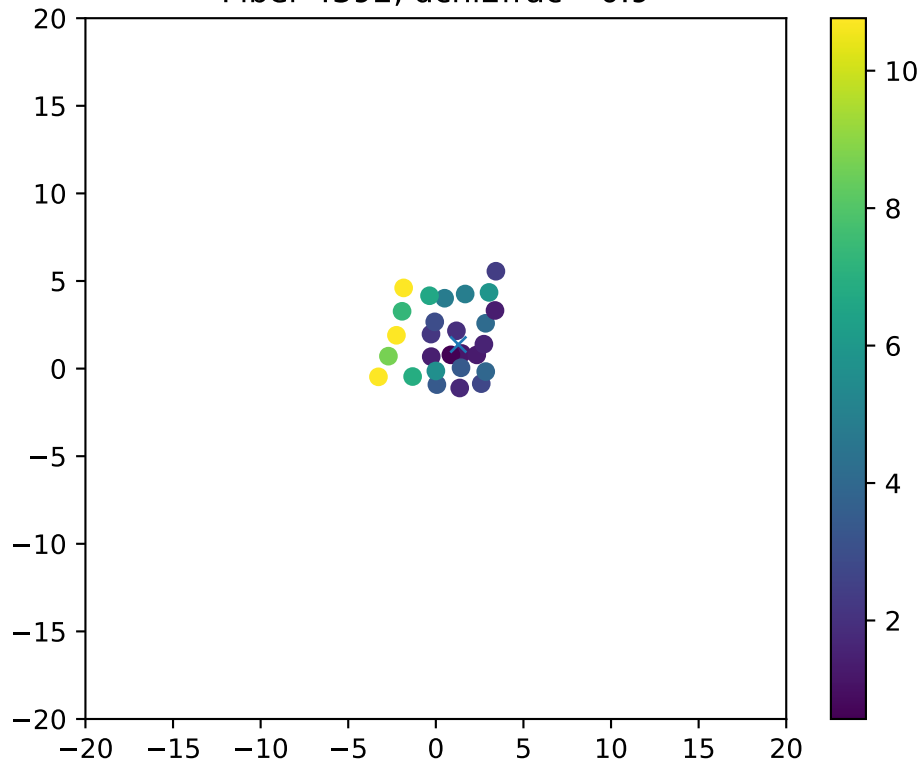
Fiber 4392, dchi2frac= 0.9
