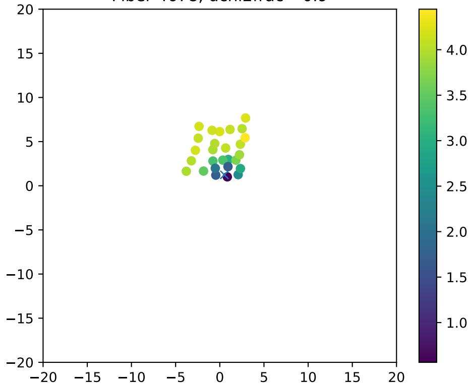
Fiber 4678, dchi2frac= 0.9
