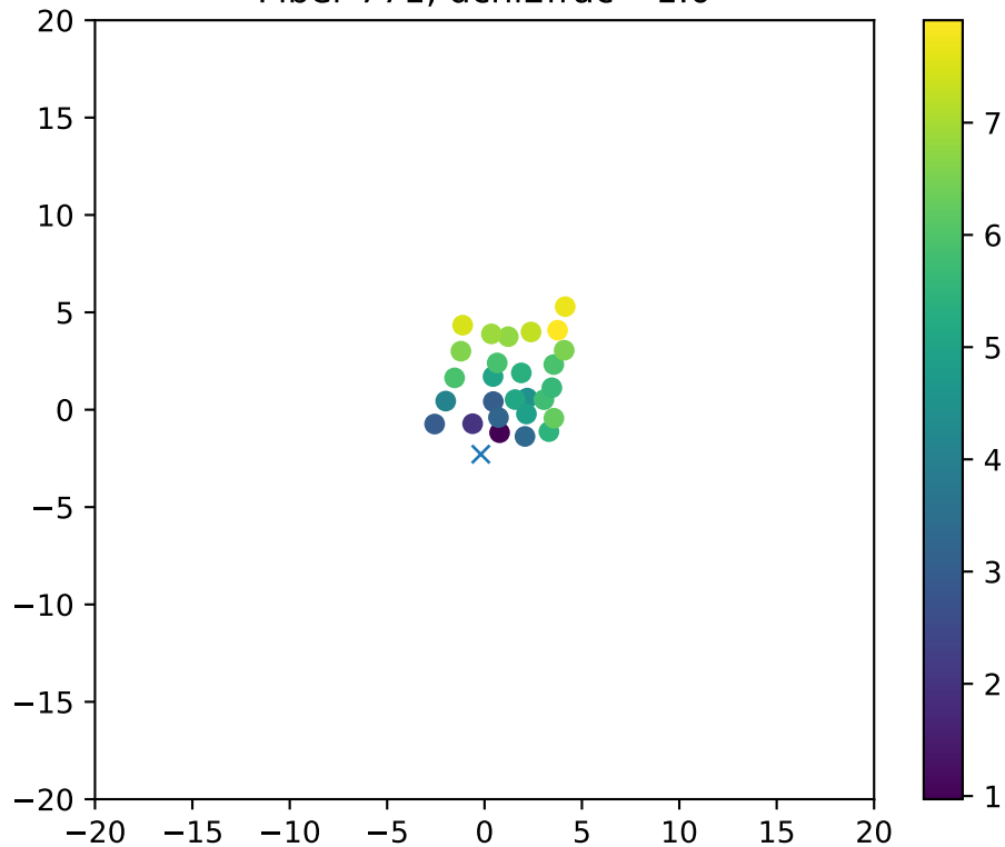
Fiber 771, dchi2frac= 1.0
