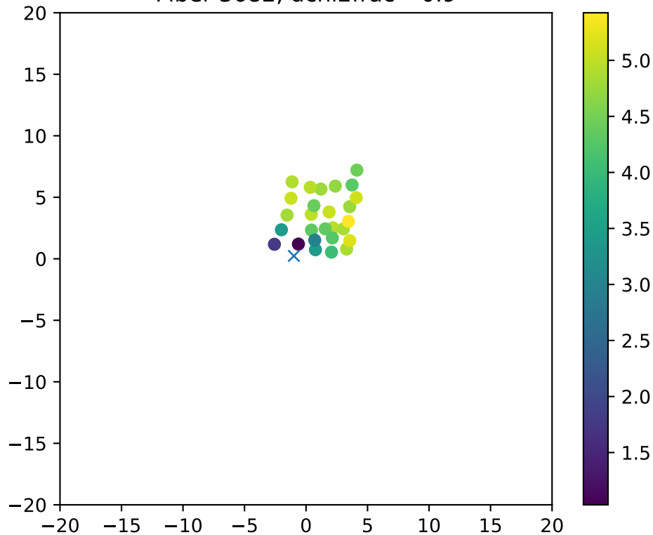
Fiber 3682, dchi2frac= 0.9
