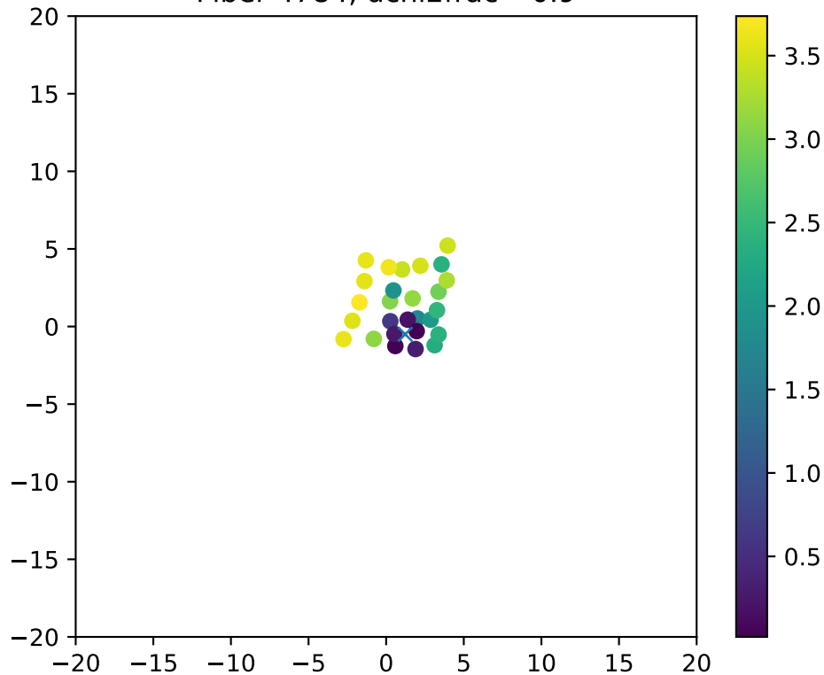
Fiber 4784, dchi2frac= 0.9
