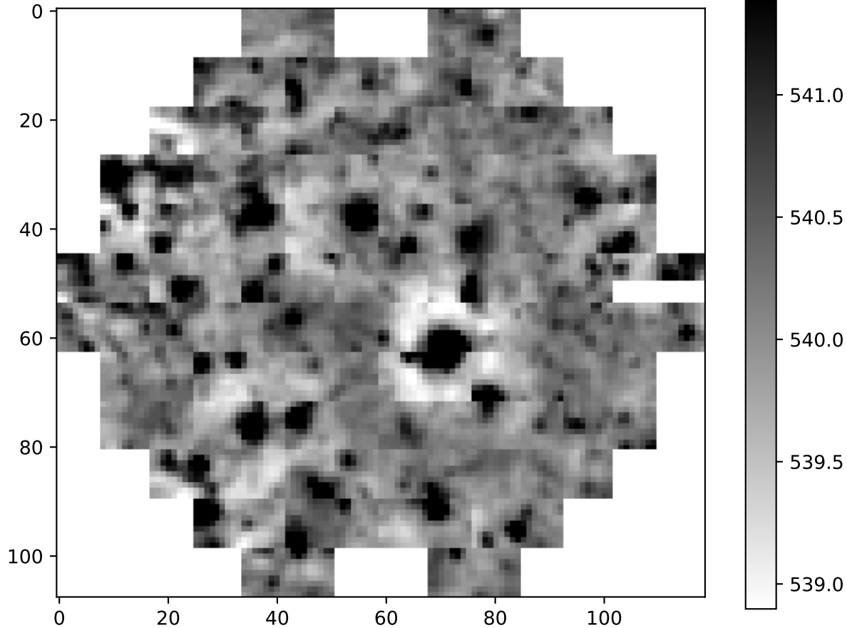
decam-00483698.fits
