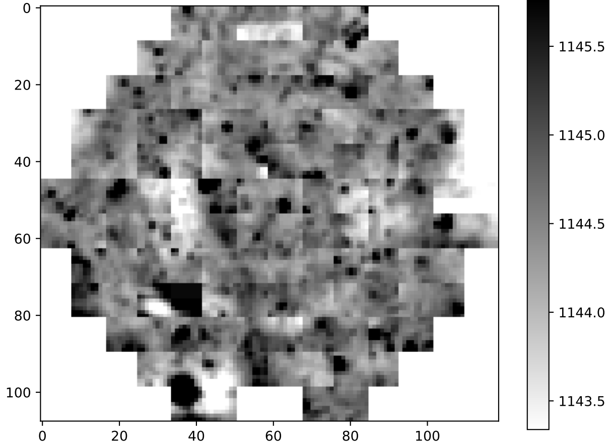
decam-00695111.fits
