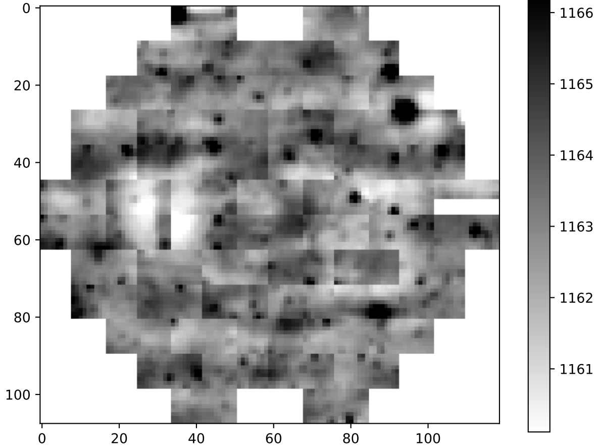
decam-00438340.fits
