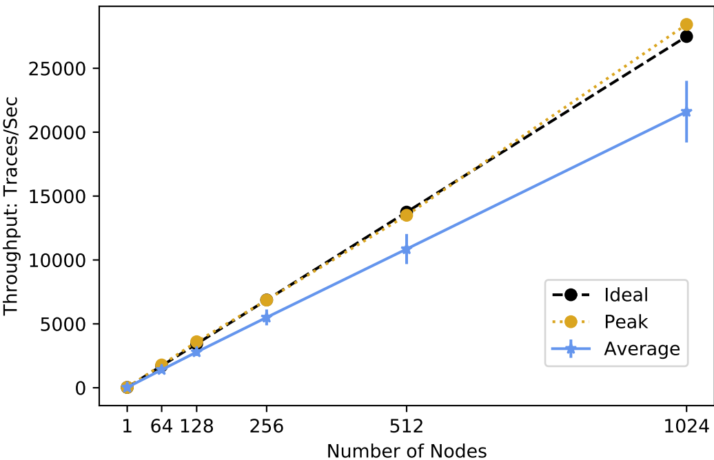
Weak Scaling on Edison
