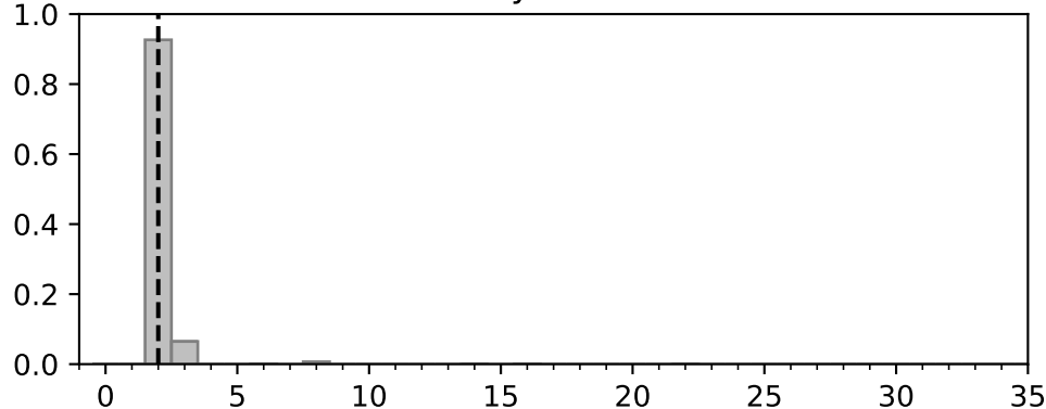
Decay Channel
