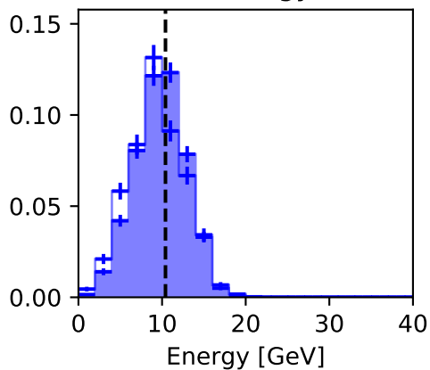
FSP Energy 2
