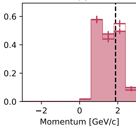
\tau p_y
