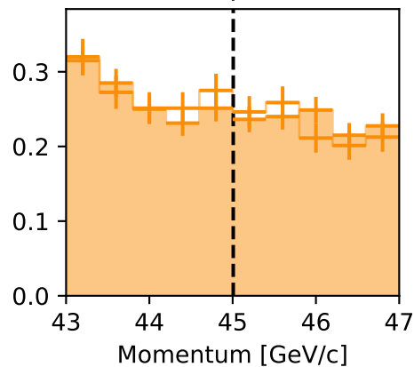
Decay Channel
