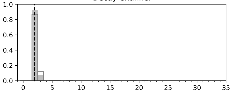
Decay Channel
