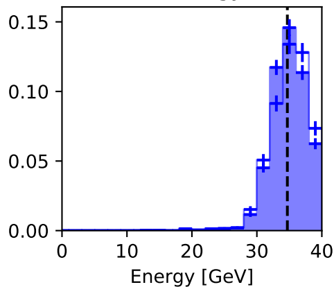
FSP Energy 1
