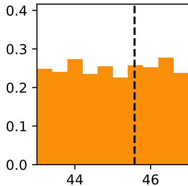
\tau pz
