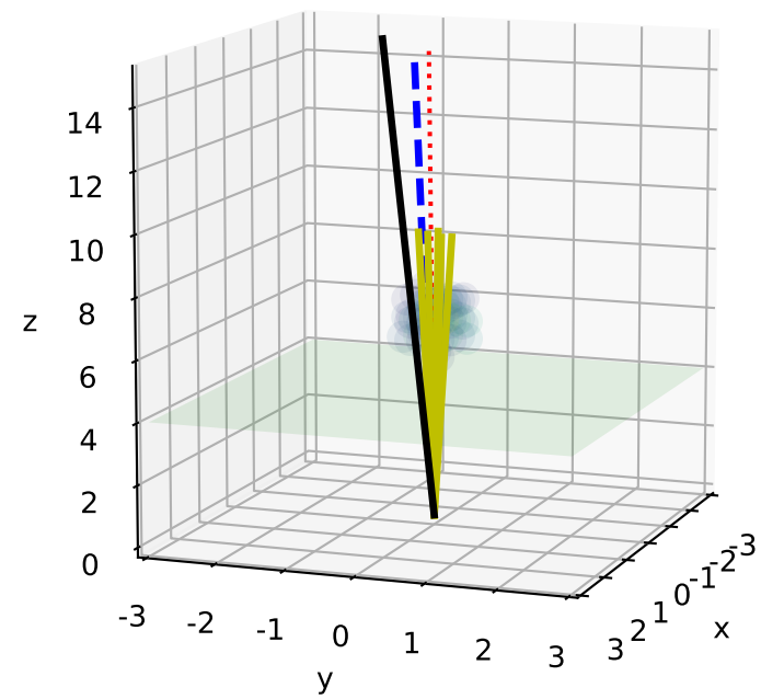
Observed Calorimeter
