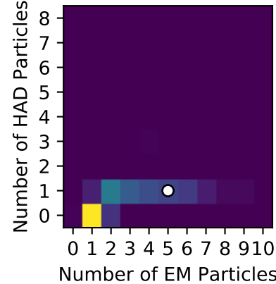
Event Composition
