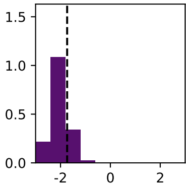
\tau px
