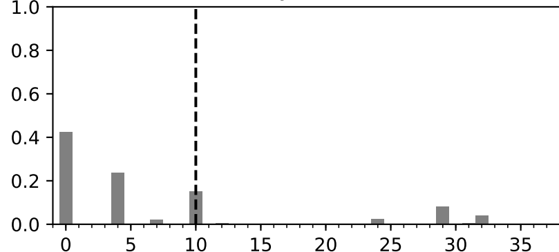
Decay Channel
