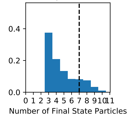
Decay Products
