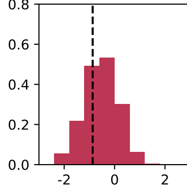
\tau py
