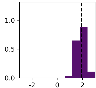
\tau px
