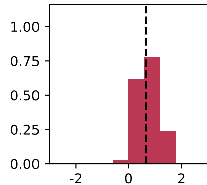
\tau py
