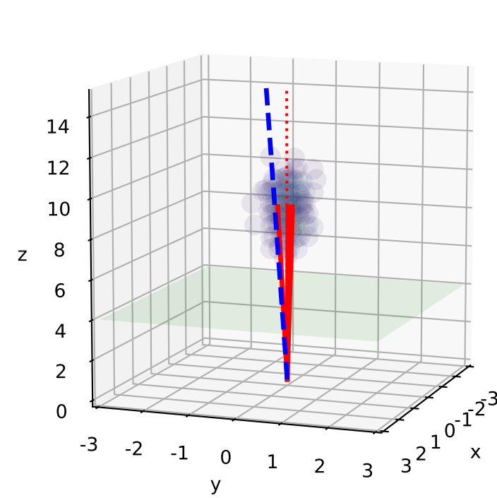
Observed Calorimeter
