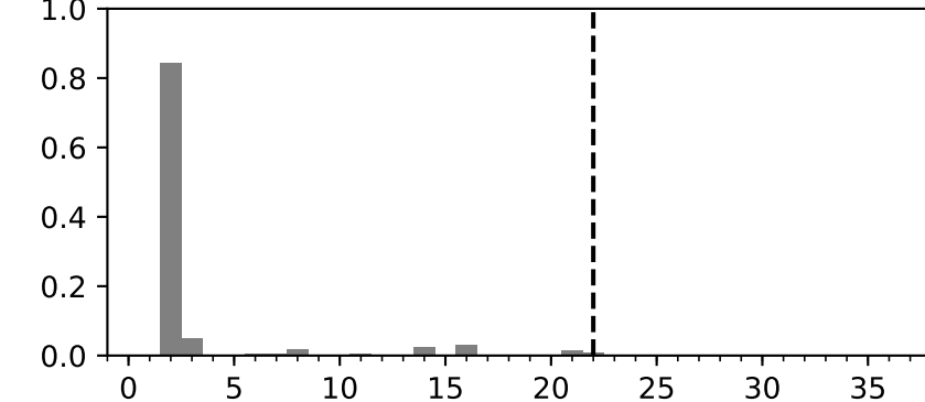
Decay Channel
