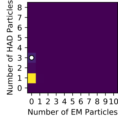
Event Composition
