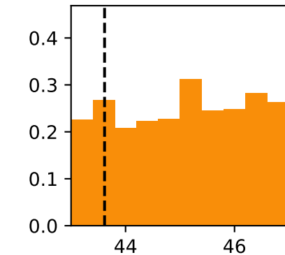
\tau pz
