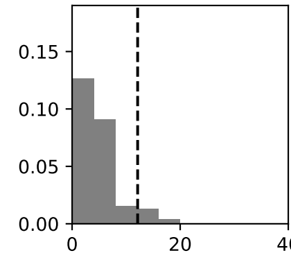
FSP Energy 2
