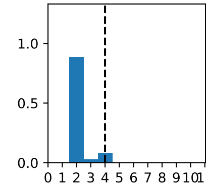
Decay Products
