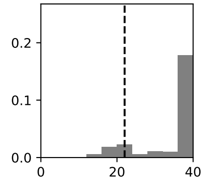
FSP Energy 1
