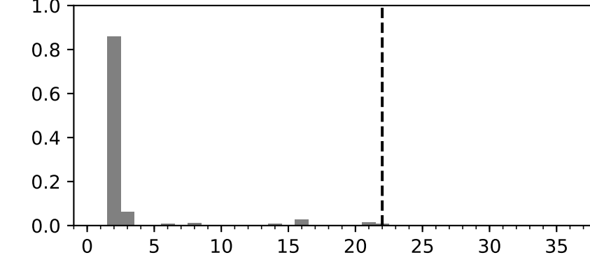
Decay Channel
