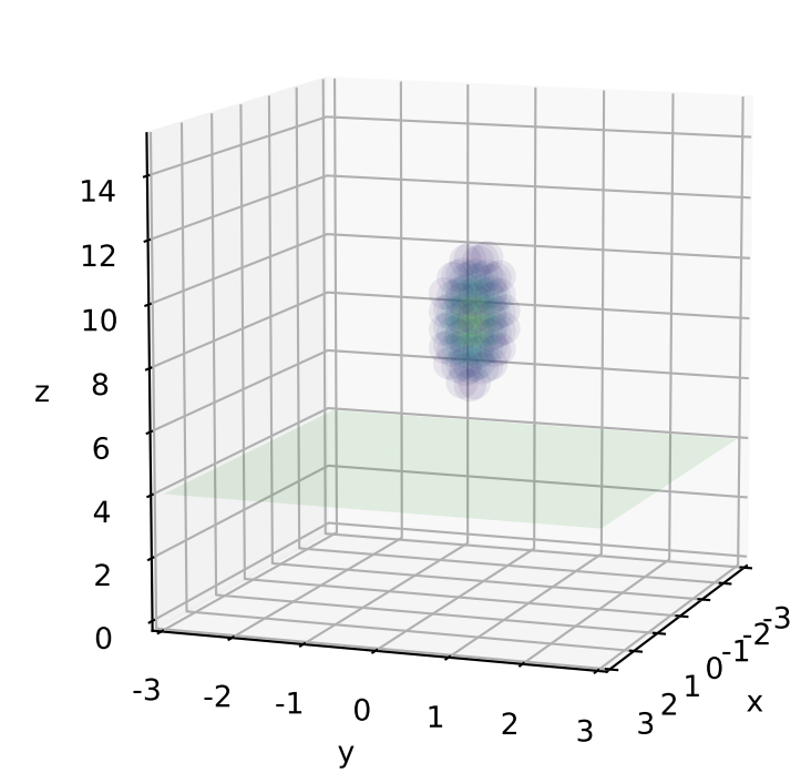
Simulated Calorimeter (Mean)
