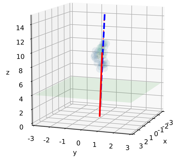
Observed Calorimeter
