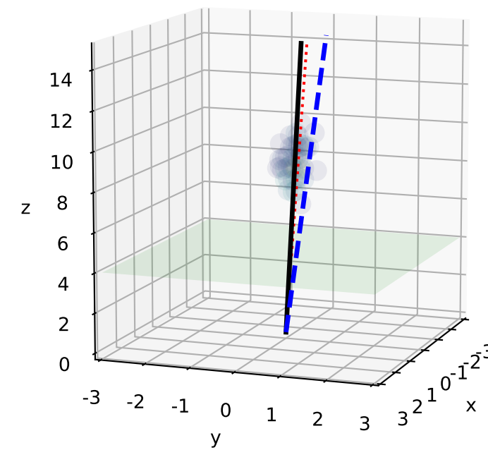
Observed Calorimeter
