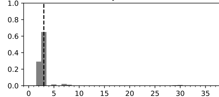
Decay Channel
