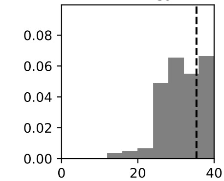
FSP Energy 1
