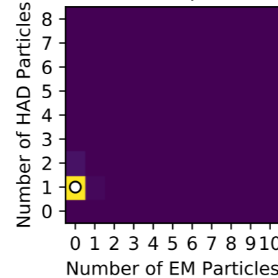
Decay Products
