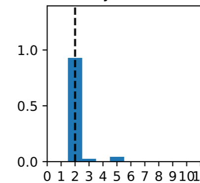
Decay Products
