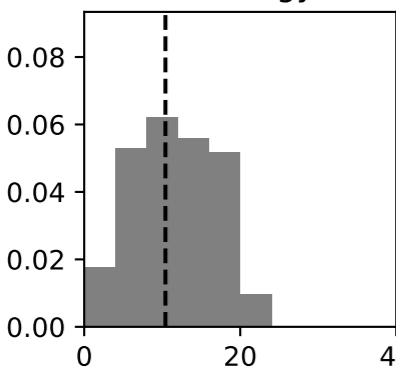
FSP Energy 2
