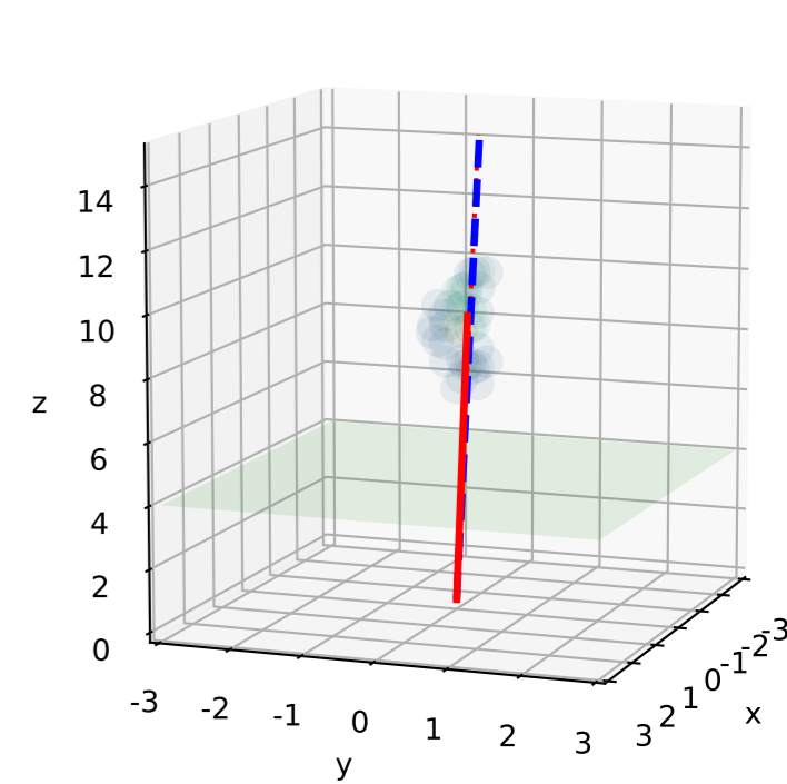
Observed Calorimeter
