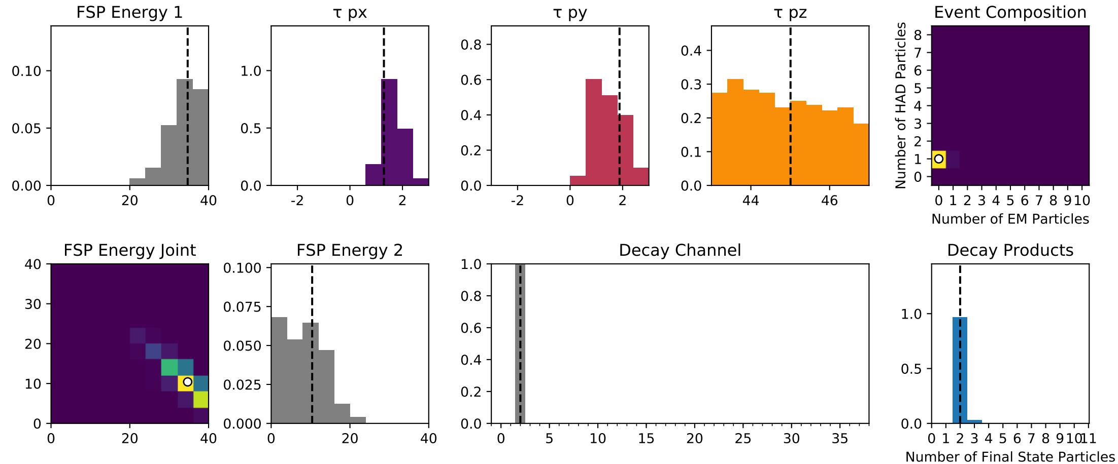
Simulated Calorimeter (Mean)
