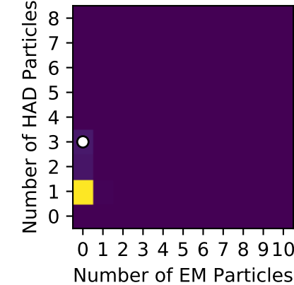
Event Composition
