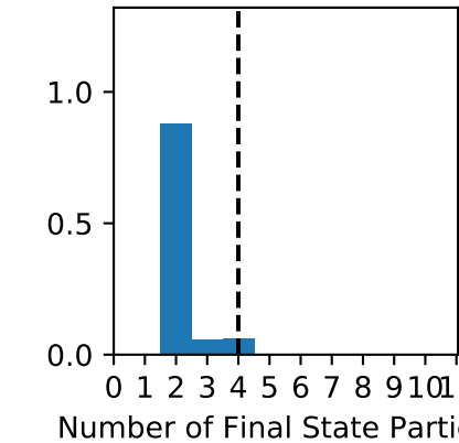
Decay Products
