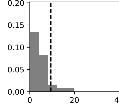
FSP Energy 2
