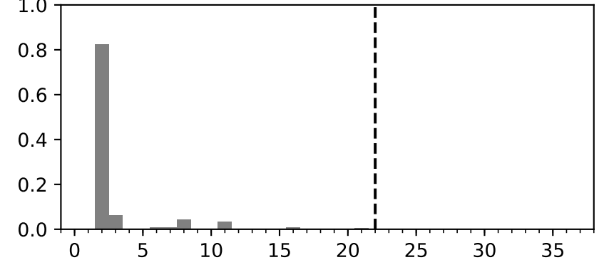
Decay Channel
