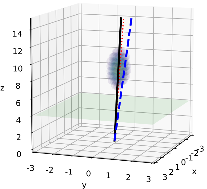
Observed Calorimeter
