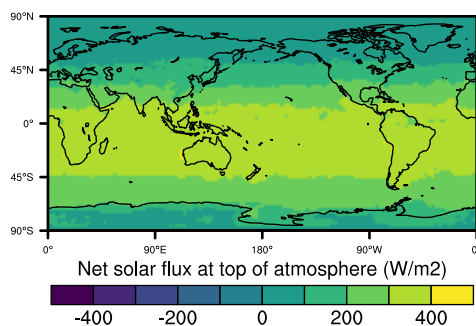
SCREAM (258.4)
