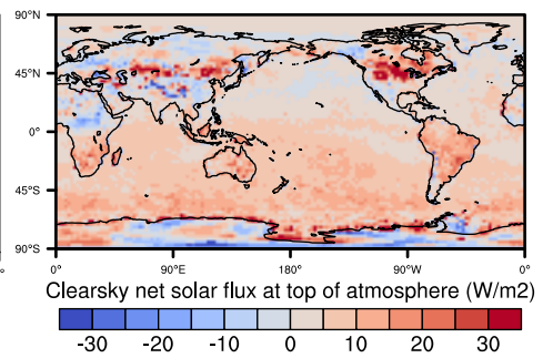
SCREAM minus CERES-EBAF (5.6)
