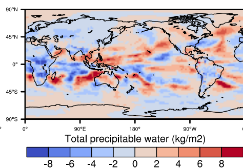
SCREAM minus ERA5 (0.1)
