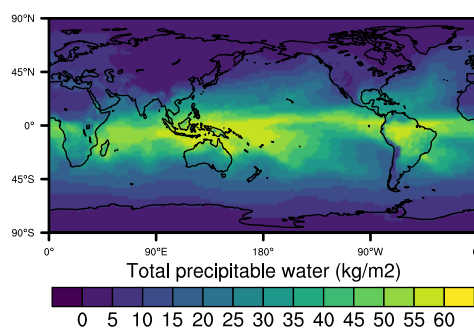
SCREAM (24.4)
