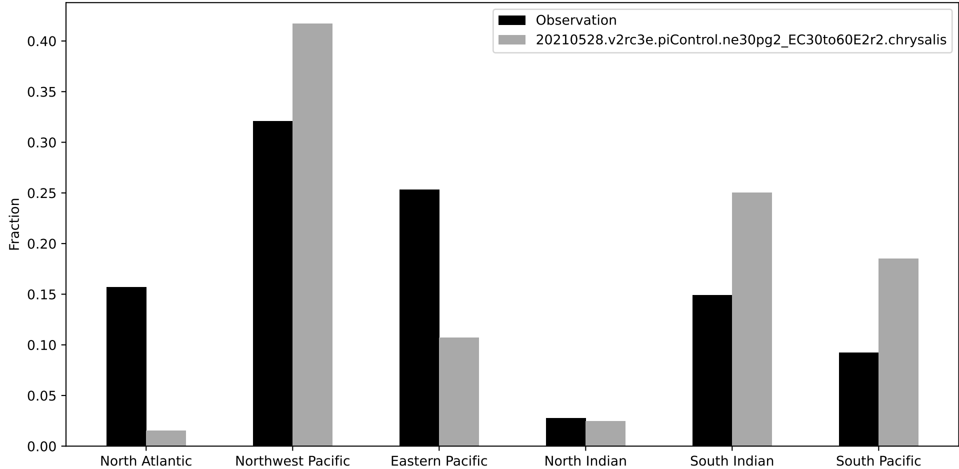
Distribution of accumulated cyclone energy (ACE) among various ocean basins
