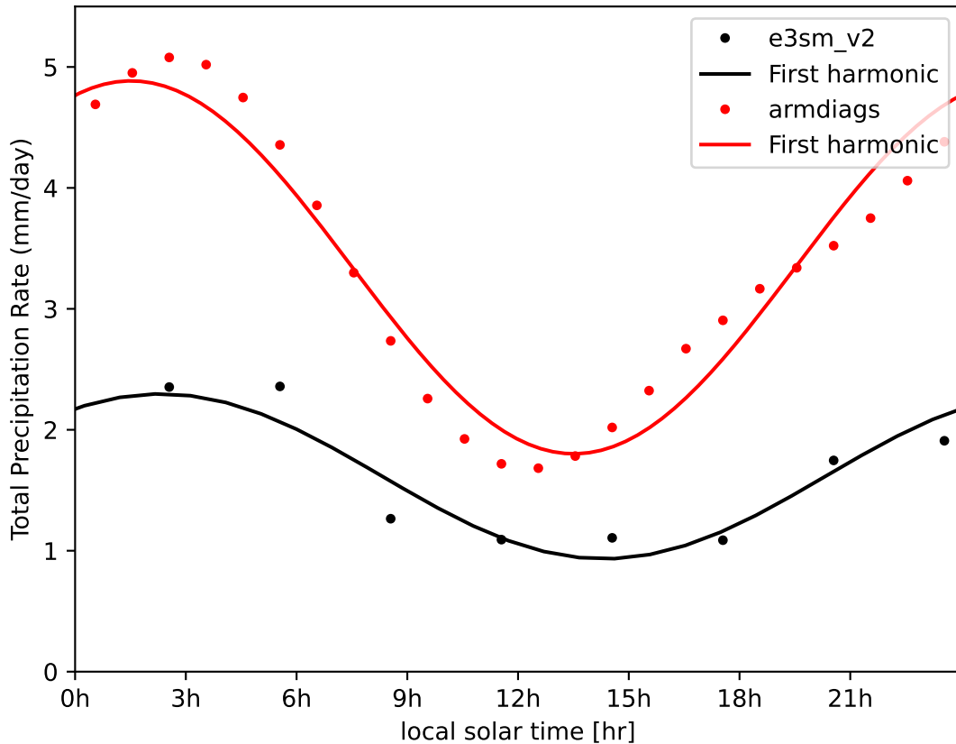
armdiags PRECT JJA sgp diurnal cycle
