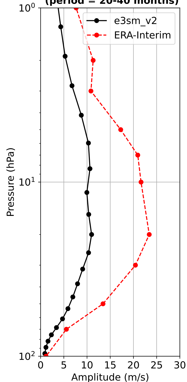
QBO Amplitude (period = 20-40 months)
