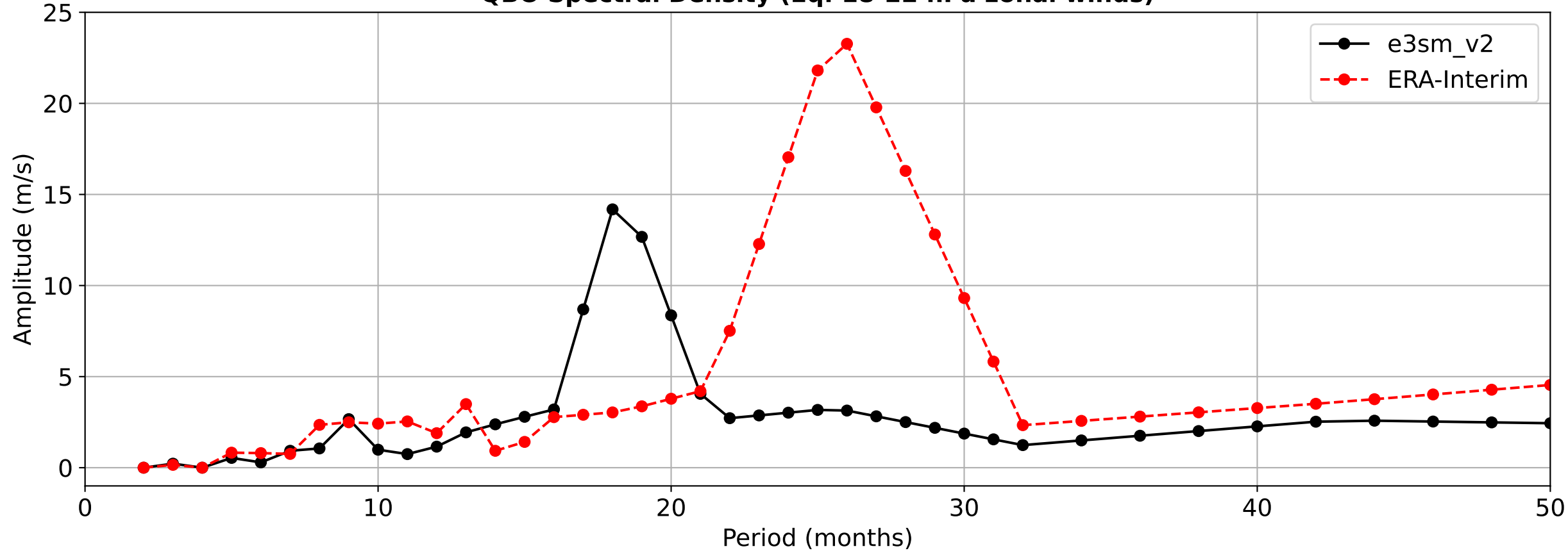
QBO Spectral Density (Eq. 18-22 hPa zonal winds)
