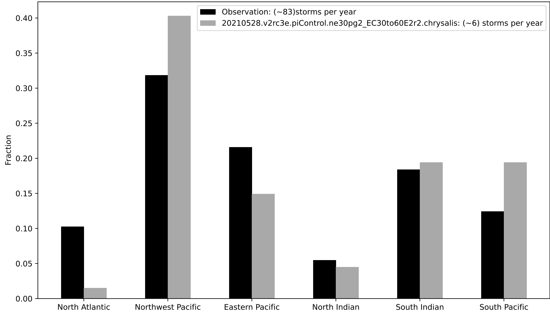
Relative frequency of TCs for each ocean basins
