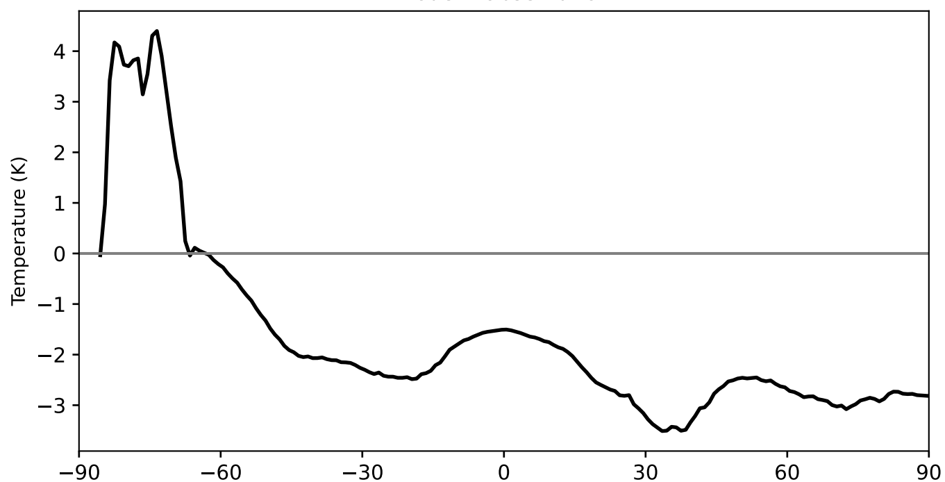
Model - Observation
