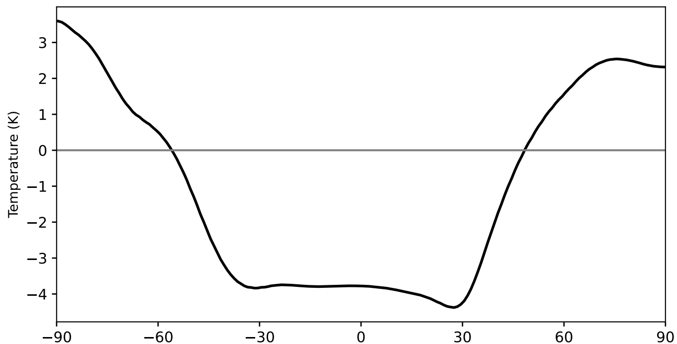
Model - Observation
