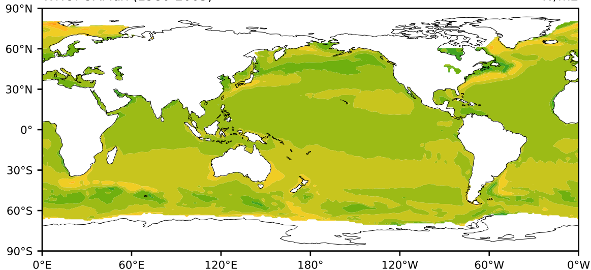
WHOI OAFlux (1980-2005)
