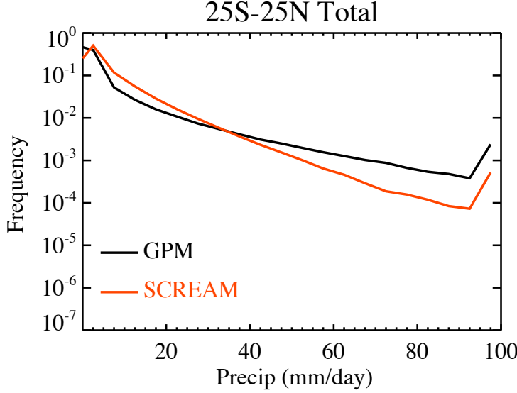
Figure 16. Histogram of tropical precipitation over the ocean from Jan 30 through Feb 28th in SCREAM and GPM.
