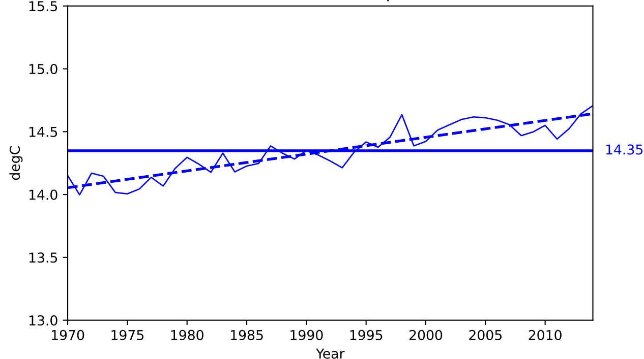
Global surface air temperature
