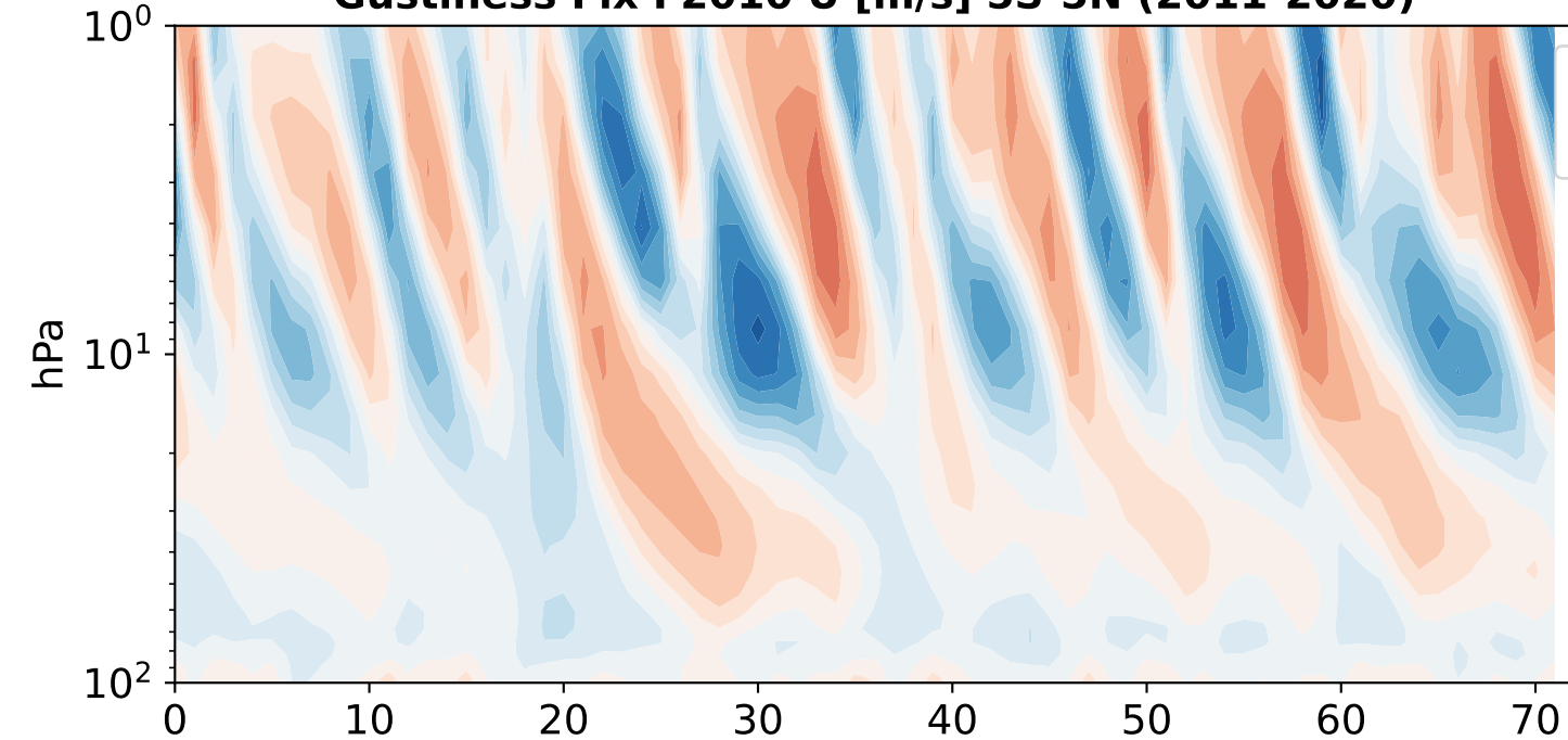
Gustiness Fix F2010 U [m/s] 5S-5N (2011-2020)
