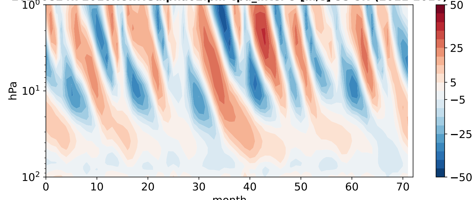
20230824.F2010New.v3alpha02.pm-cpu_intel U [m/s] 5S-5N (2011-2016)
