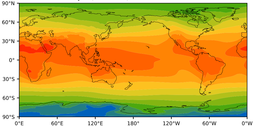
ERA-Interim Reanalysis (1979-2016)
