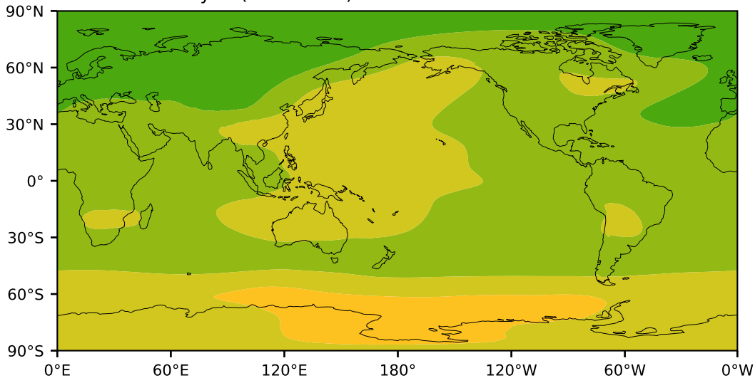
MERRA2 Reanalysis (1980-2016)
