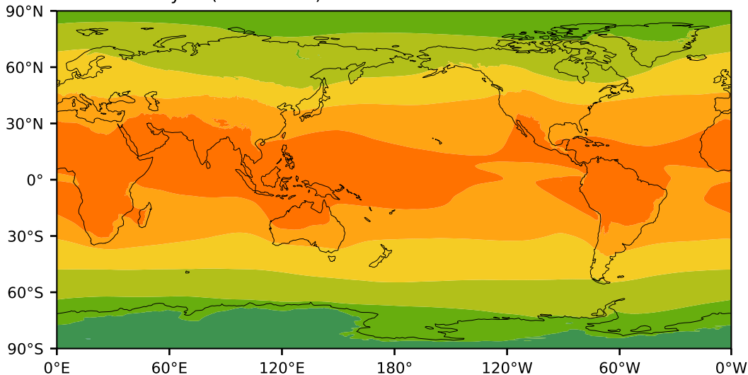
ERA5 Reanalysis (1979-2019)
