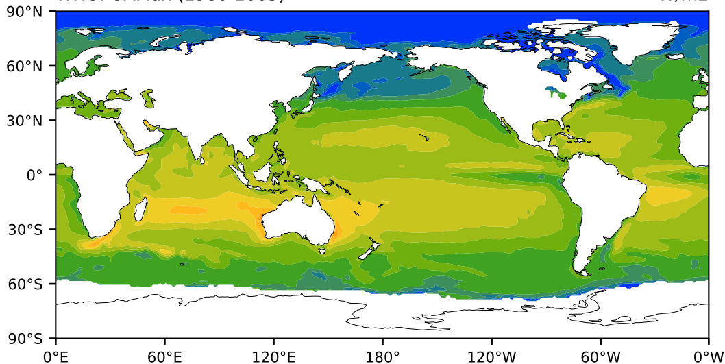
WHOI OAFlux (1980-2005)
