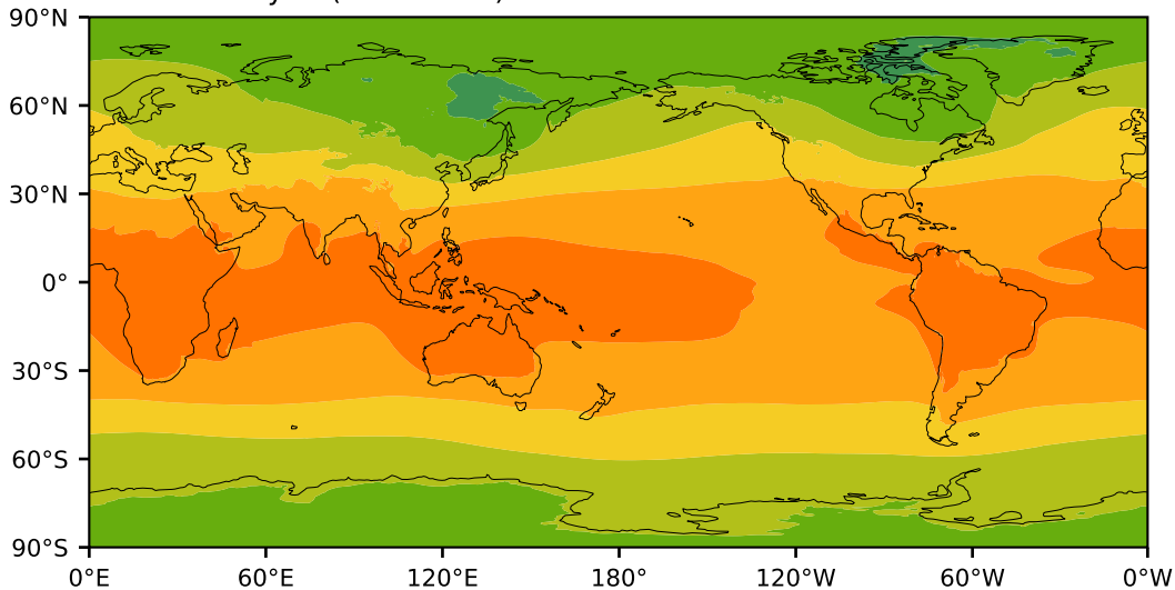
ERA5 Reanalysis (1979-2019)
