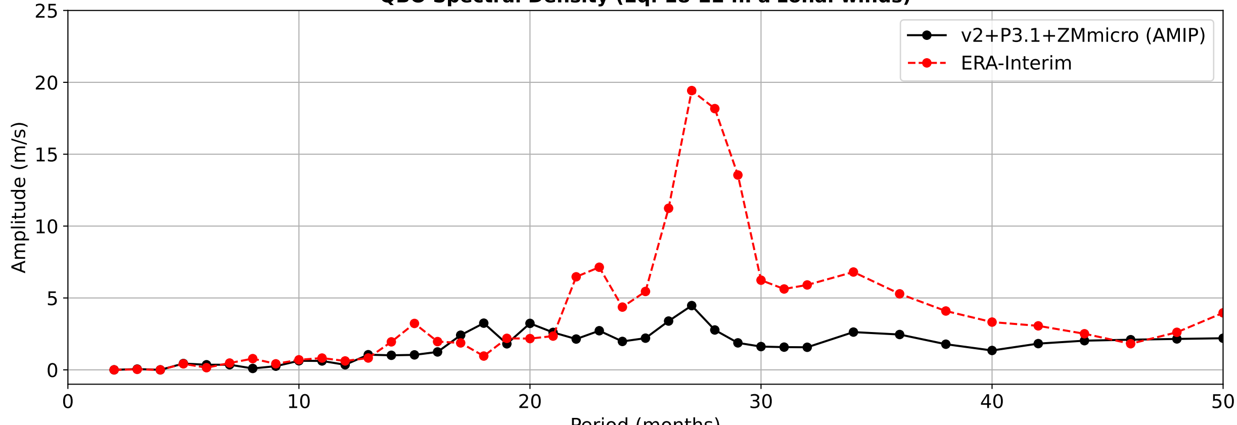
QBO Spectral Density (Eq. 18-22 hPa zonal winds)
