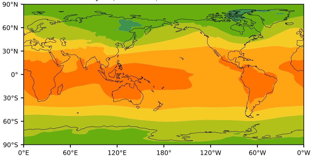
ERA-Interim Reanalysis (1979-2016)
