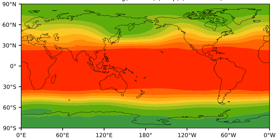
v3 baseline+MCSP+mc+tuning(ke+wbf) (amip) (1985-2009) hectometer
