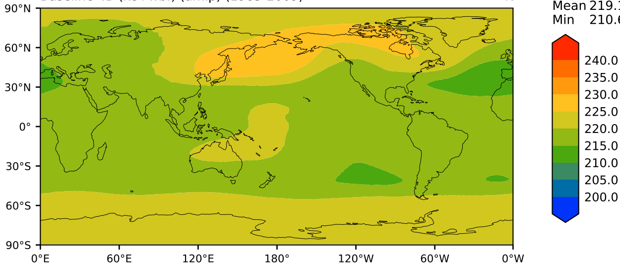
Baseline 4B (ke+wbfb) (amip) (1985-2009)
