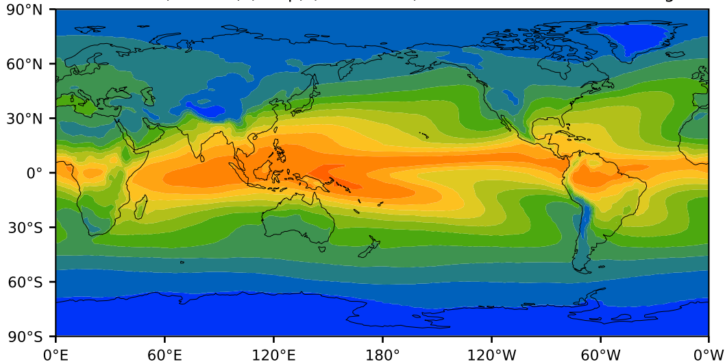
Baseline 4B (ke+wbfb) (amip) (1985-2009)
