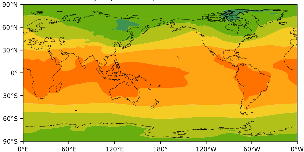
ERA-Interim Reanalysis (1979-2016)
