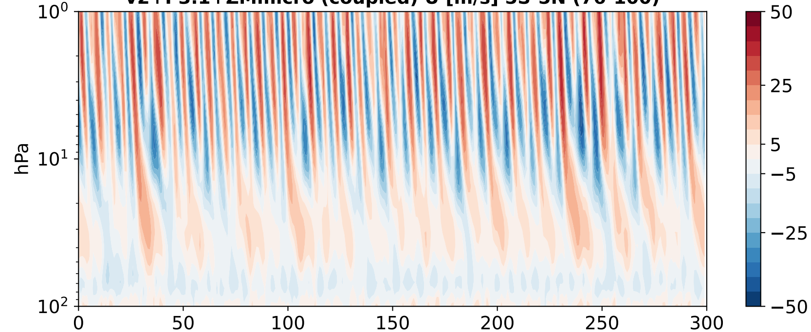
v2+P3.1+ZMmicro (coupled) U [m/s] 5S-5N (76-100)
