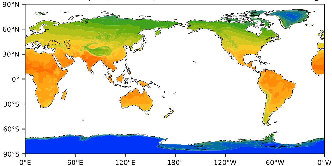
MERRA2 Reanalysis (1980-2016)
