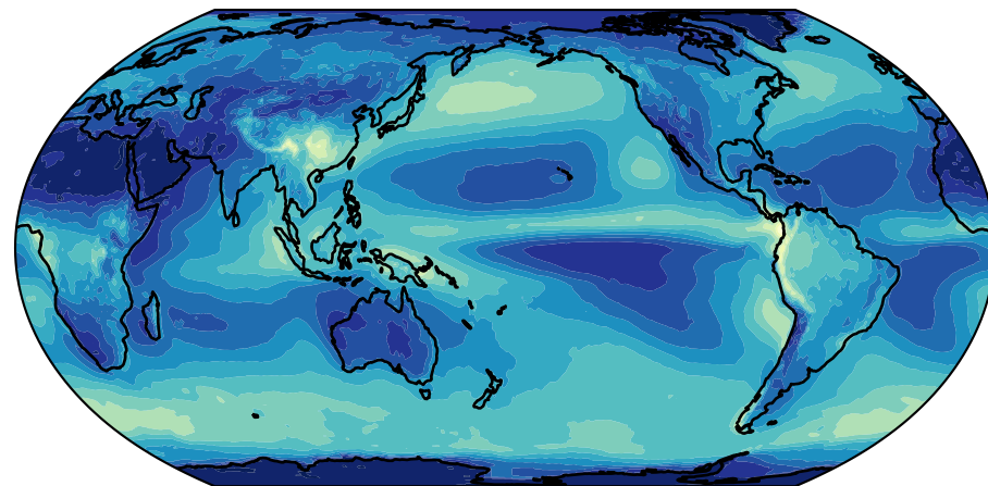
Shortwave Cloud Forcing CERES-EBAF
