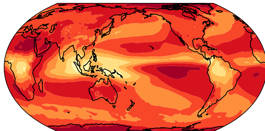
Longwave Cloud Forcing CERES-EBAF
