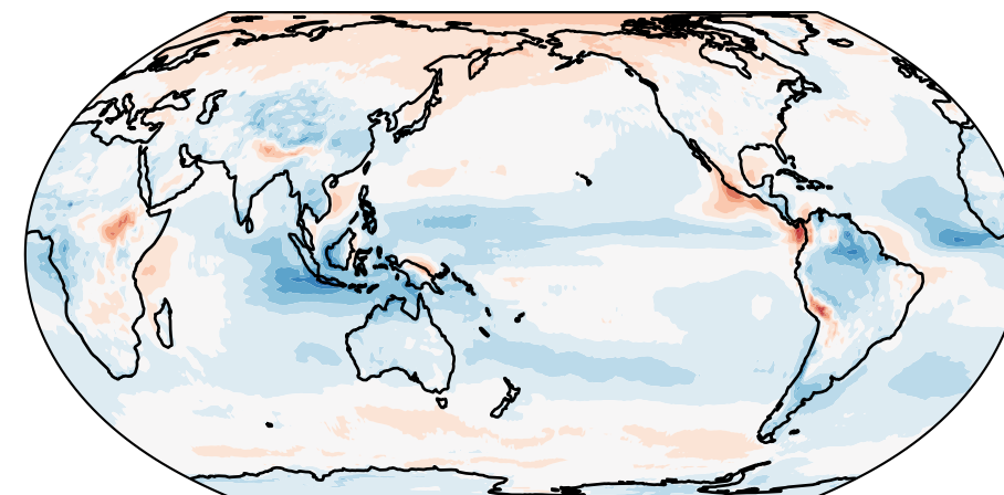
Longwave Cloud Forcing EAMv2 - CERES-EBAF
