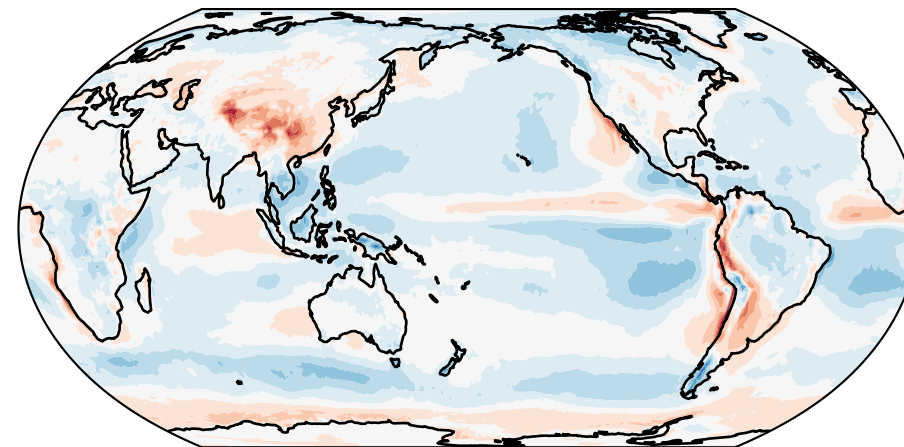
Shortwave Cloud Forcing EAMv3 - CERES-EBAF
