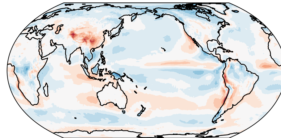
Shortwave Cloud Forcing EAMv2 - CERES-EBAF
