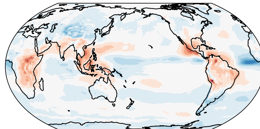
Longwave Cloud Forcing EAMv3 - CERES-EBAF
