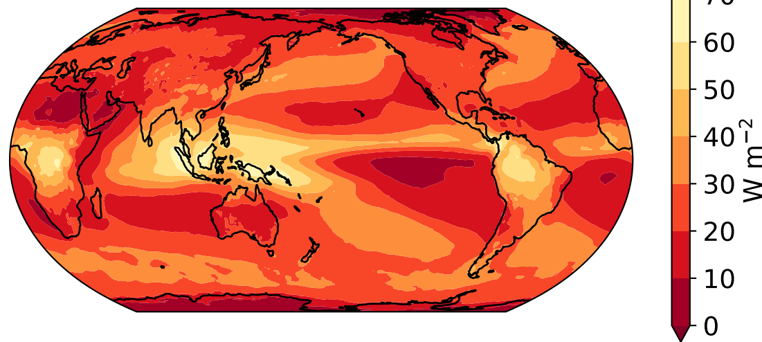
Longwave Cloud Forcing CERES-EBAF
