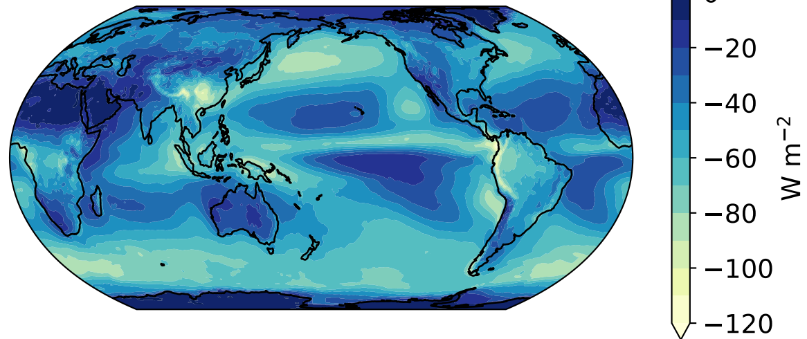
Shortwave Cloud Forcing CERES-EBAF
